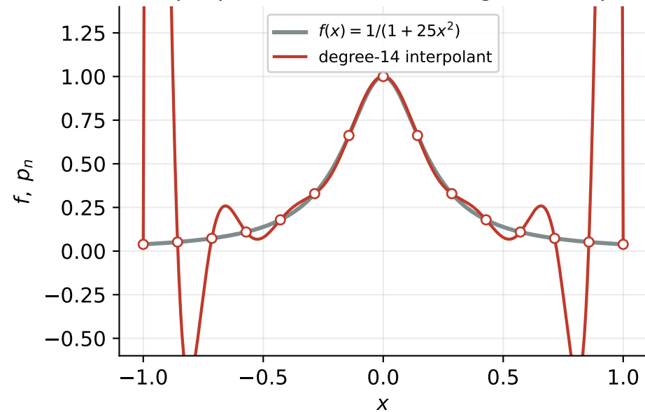
Equispaced nodes — Runge blow-up
