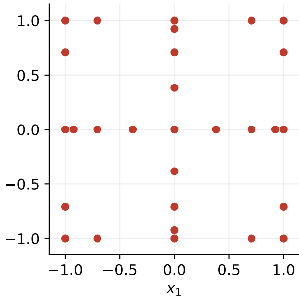
Smolyak \mu = 3 29 points
