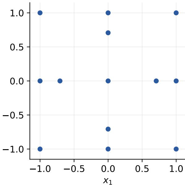
Smolyak \mu = 2 13 points
