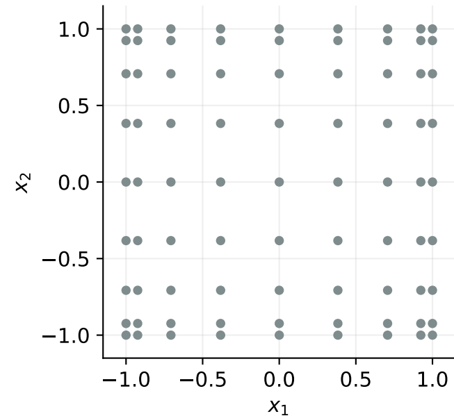
Full tensor grid 9 \times 9 = 81 points
