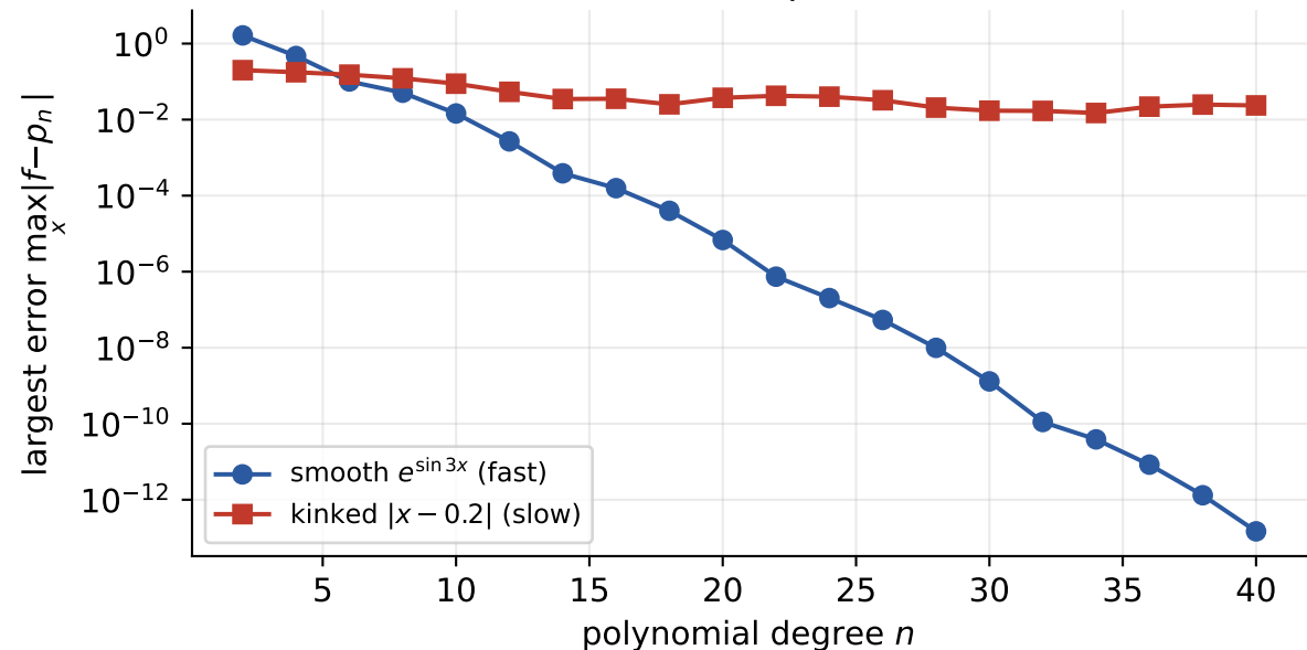
How fast the error falls depends on smoothness
