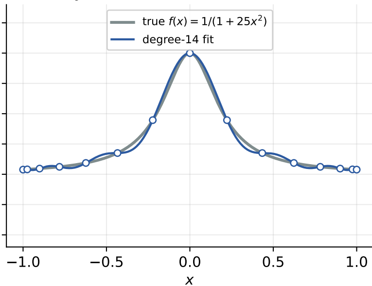
Chebyshev nodes — the fit is stable
