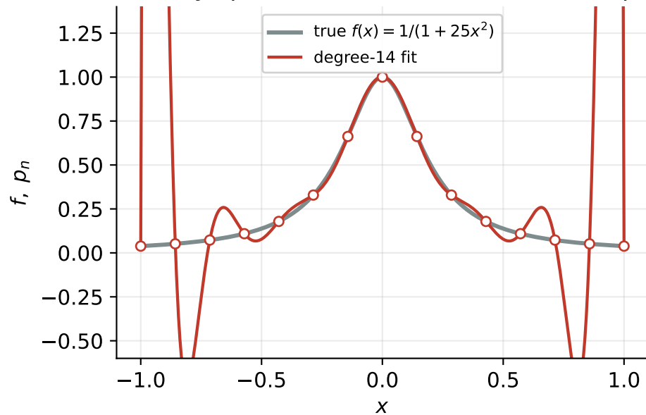
Evenly spaced nodes — the fit blows up
