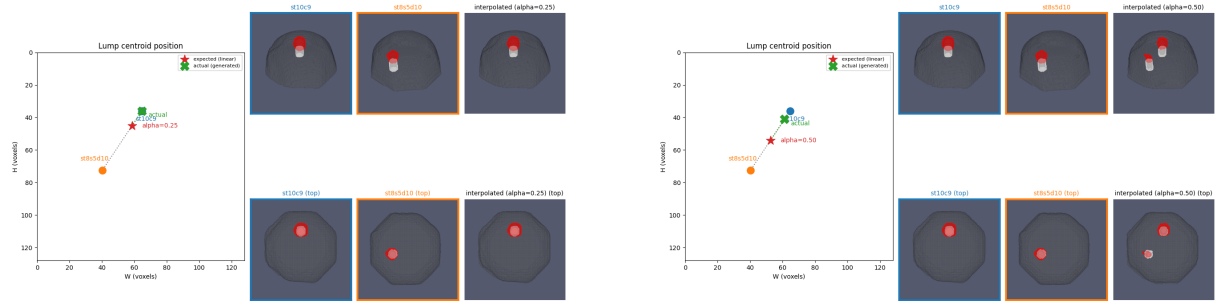
Figure 6: Same pair (st10c9 \leftrightarrow st8s5d10), t_{\text{mid}} = 0.5 . Left, \alpha = 0.25 : output matches phantom A almost exactly. Right, \alpha = 0.5 : both A’s and B’s lumps appear simultaneously instead of one blended lump.
