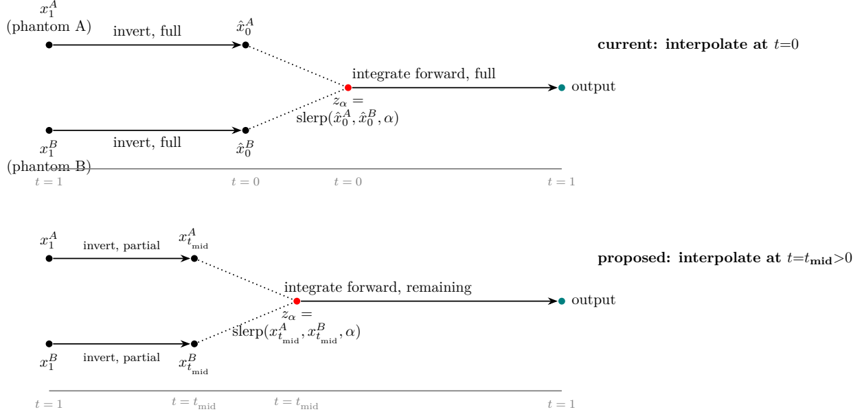
Figure 5: Both rows invert A, invert B, slerp, and integrate forward — the only difference is how far back each phantom is inverted before interpolating. Both A and B are still inverted independently and symmetrically; the proposal only stops the backward integration early.
