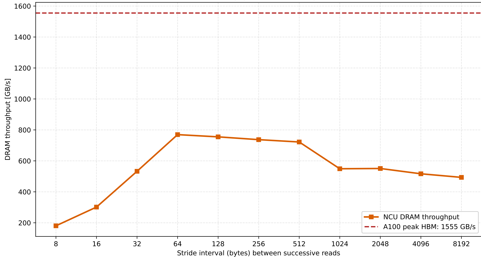
NCU DRAM Throughput vs Stride (8-byte reads)
