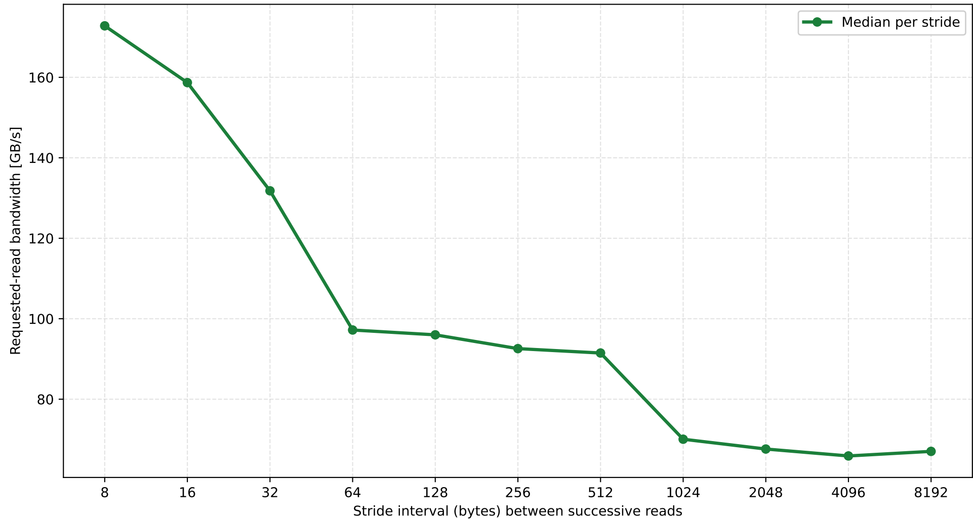
Requested Throughput vs Stride (8-byte reads, median over raw runs)
