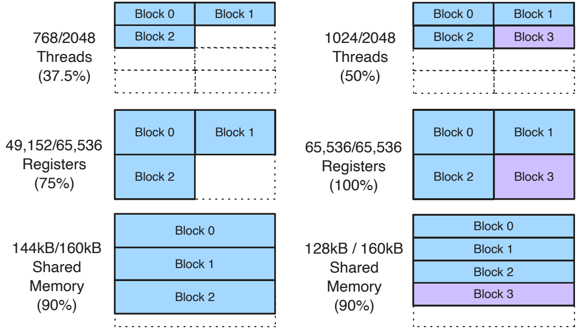
(a) Initial setup with 48 kB shared memory per block. Shared memory is the binding occupancy limit. (b) After reducing to 32 kB shared memory per block. One additional block fits; registers become the binding limit.
