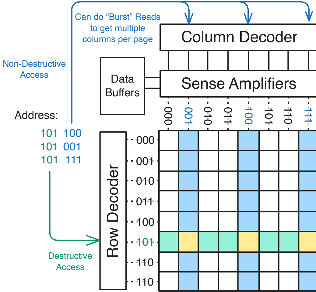
Figure 2.7.: Custom schematic for HBM/DRAM row-column access. A read activates one row, latches it into the sense amplifiers, and then uses the column decoder to select transferred data (including burst reads from the open row buffer).
