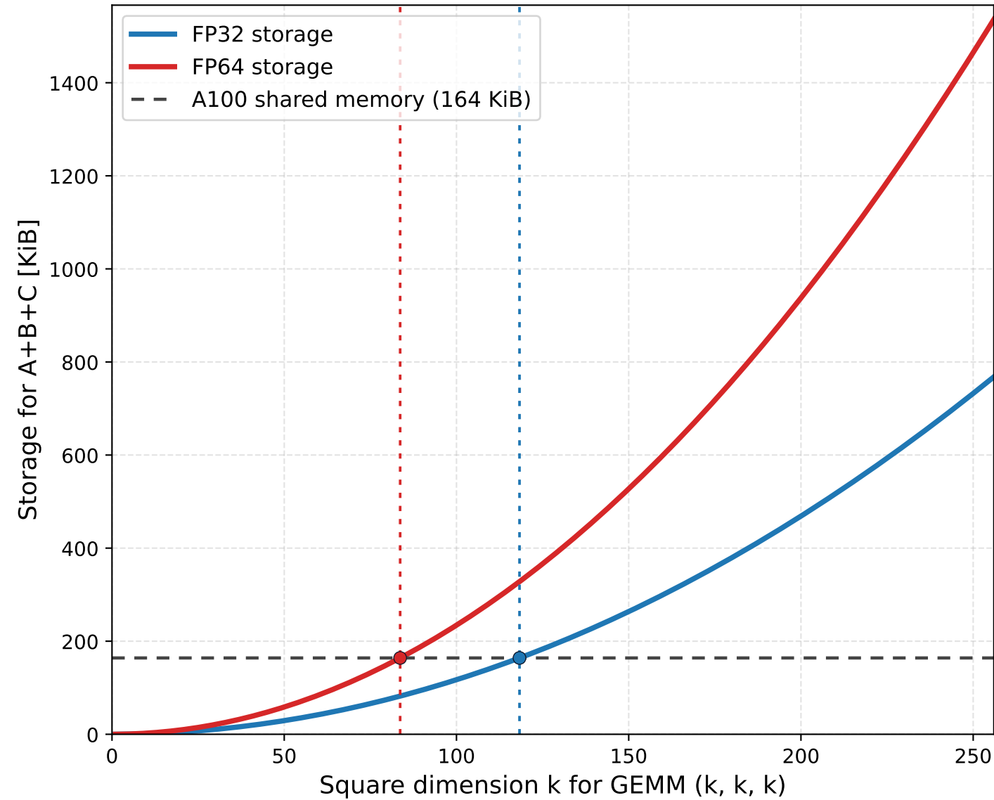
Per-SM Shared-Memory Limit
