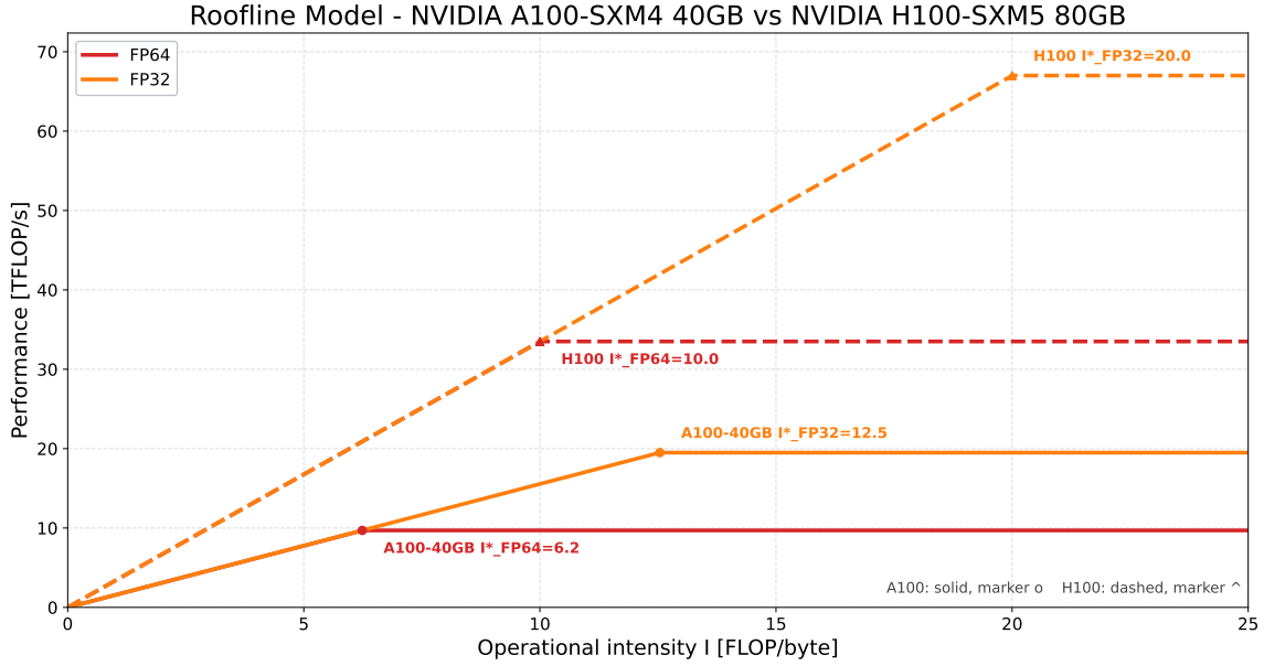
Figure 3.4.: Combined roofline envelopes for A100-SXM4-40GB and H100-SXM5-80GB in one shared axis, using FP64 and FP32 ceilings. Solid lines correspond to A100-SXM4-40GB, dashed lines to H100-SXM5-80GB; ridge markers indicate arithmetic-intensity crossover points.
