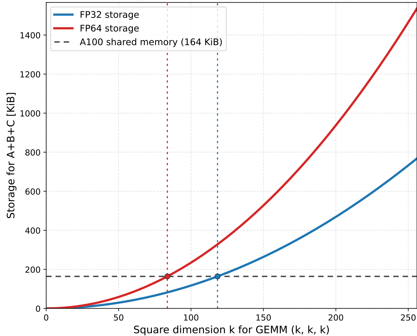
Same Footprint Model vs Per-SM Shared-Memory Limit
