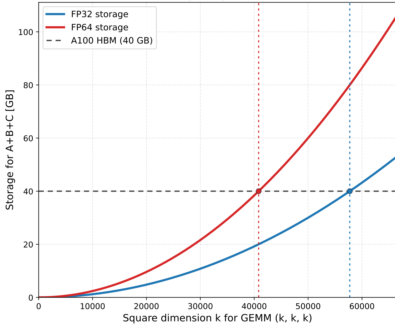
Global-Memory Footprint vs A100 HBM
