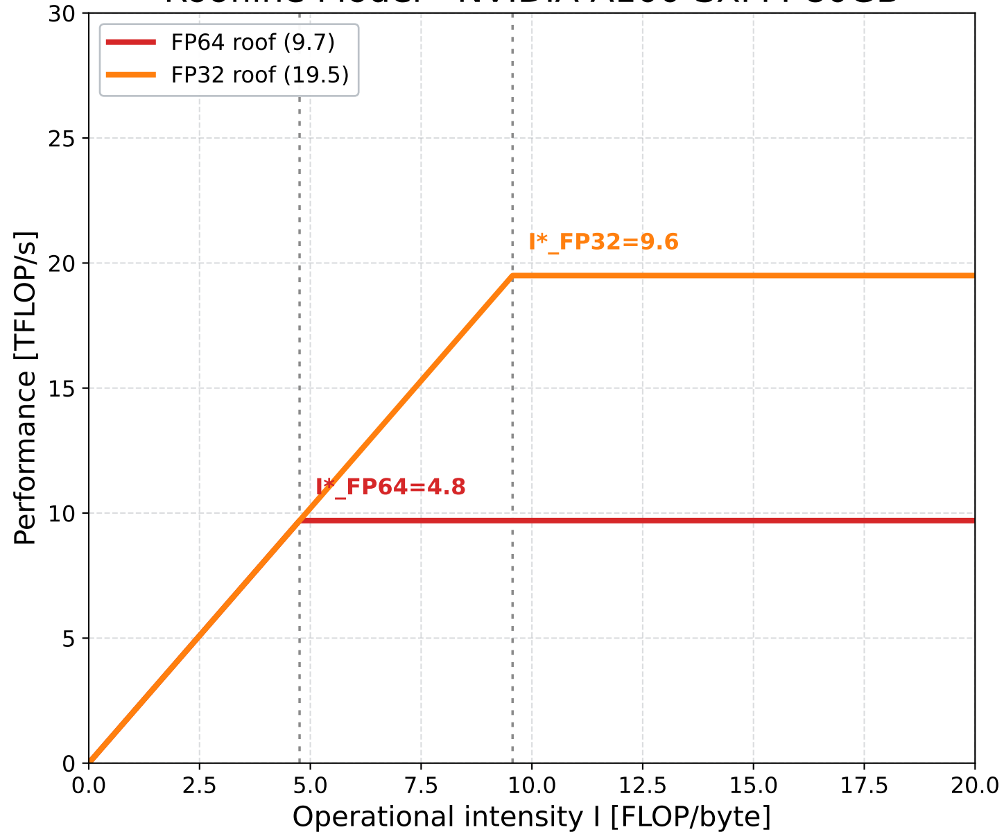
Roofline Model - NVIDIA A100-SXM4 80GB
