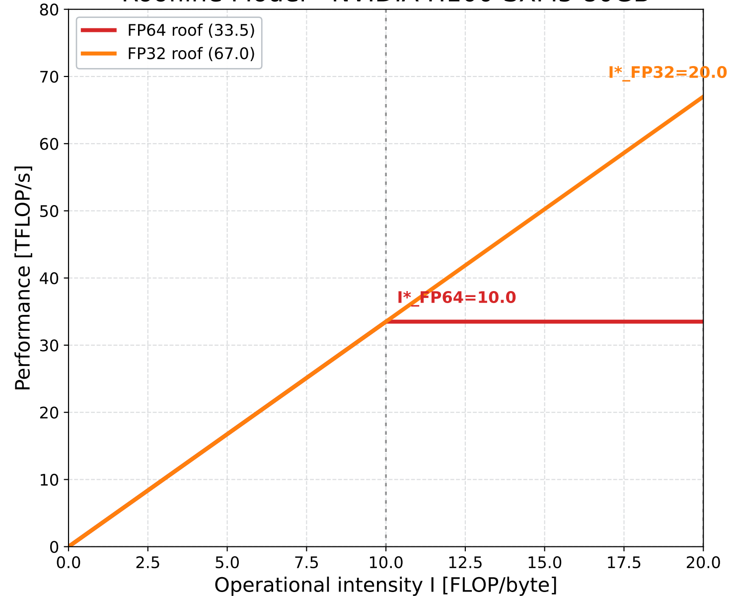
Roofline Model - NVIDIA H100-SXM5 80GB
