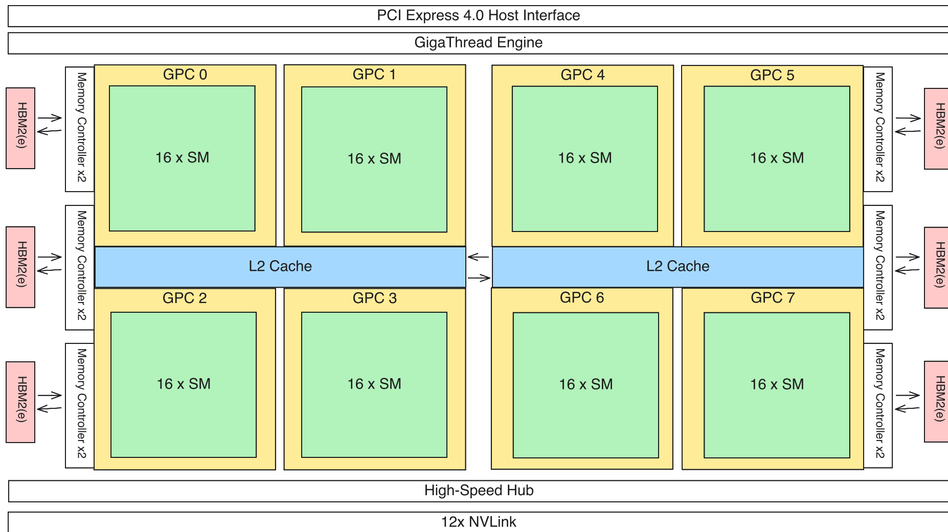
Figure D.1.: Full GA100 floorplan schematic (landscape view). Graphics processing clusters (GPCs), L2 cache fabric, memory controllers, and NVLink/PCIe interfaces are shown. Compare with Figure 2.2 in the main text and the per-SM detail in Figure 2.3.
