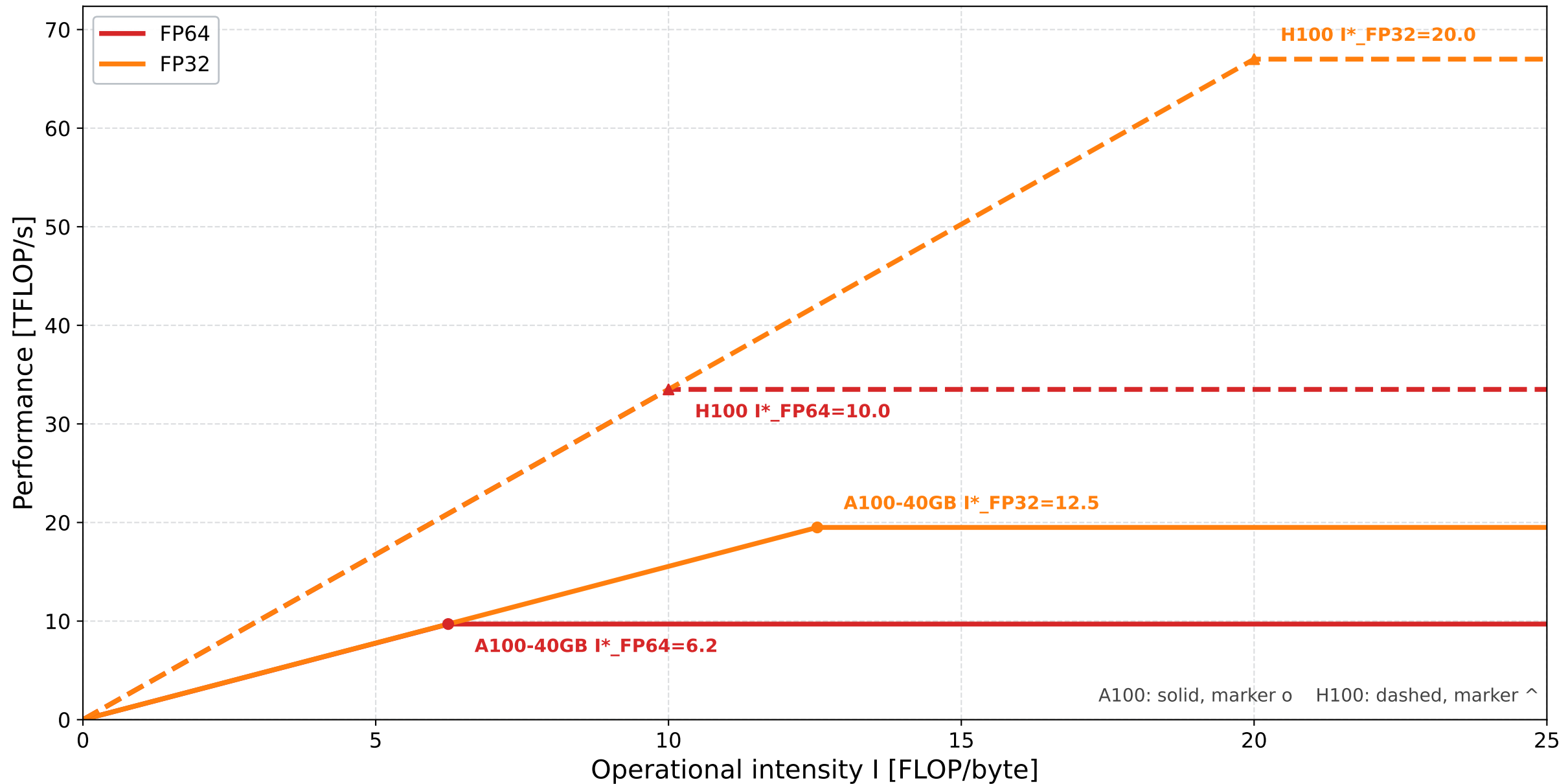
Roofline Model - NVIDIA A100-SXM4 40GB vs NVIDIA H100-SXM5 80GB
