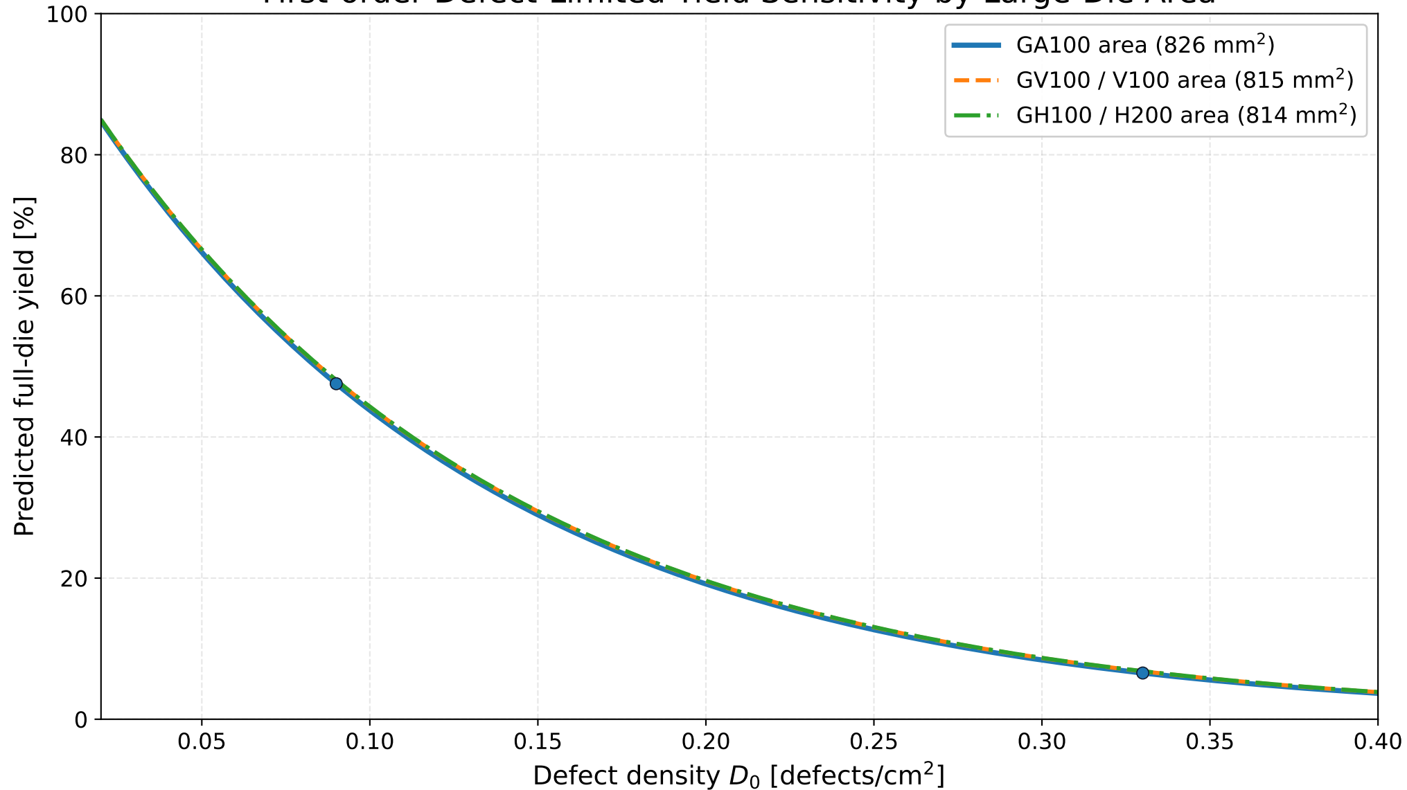
First-order Defect-Limited Yield Sensitivity by Large-Die Area
