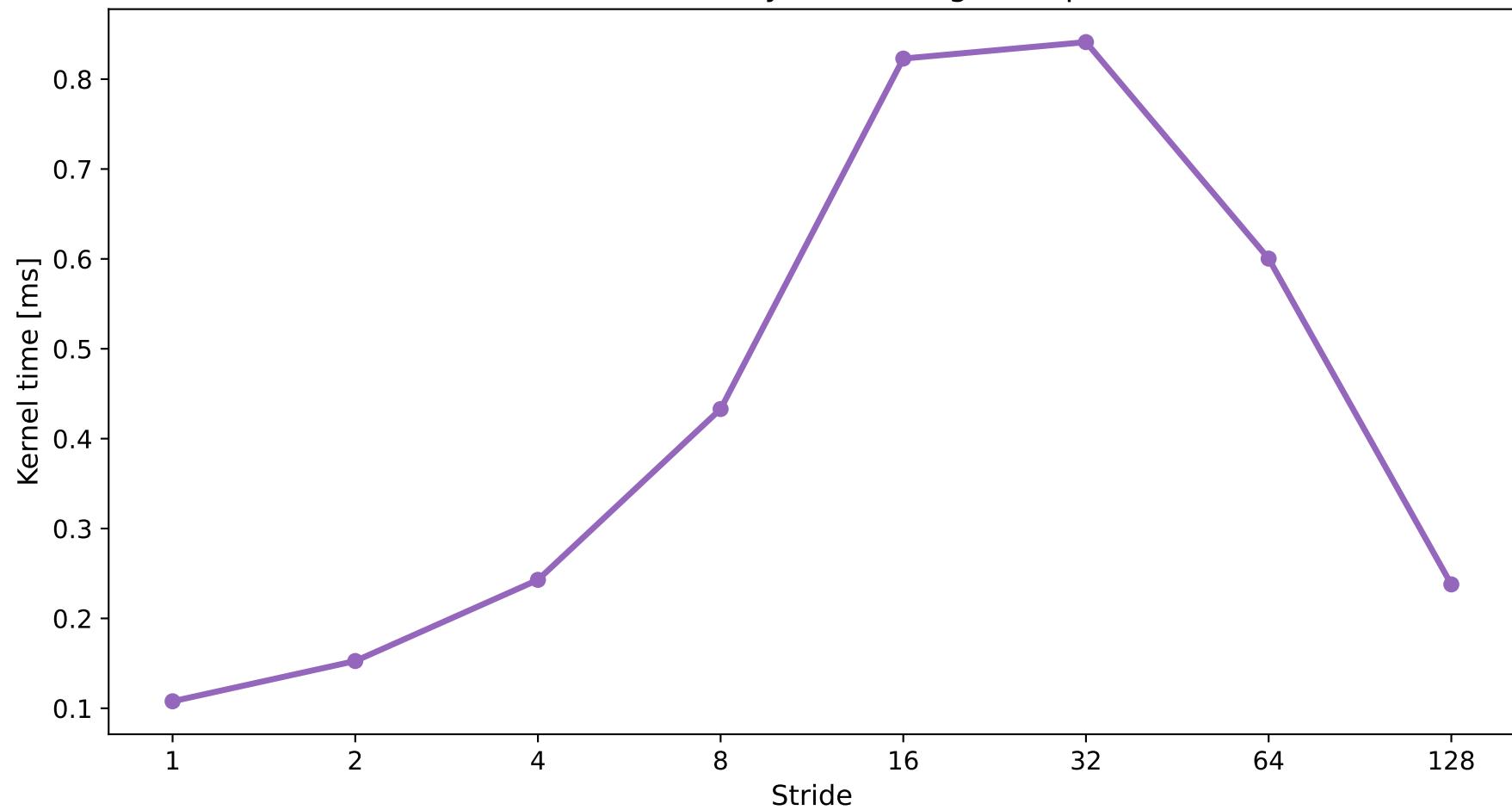
Global-Memory Coalescing Sweep
