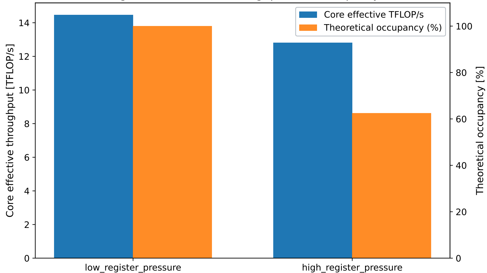
Register Pressure vs Throughput and Occupancy
