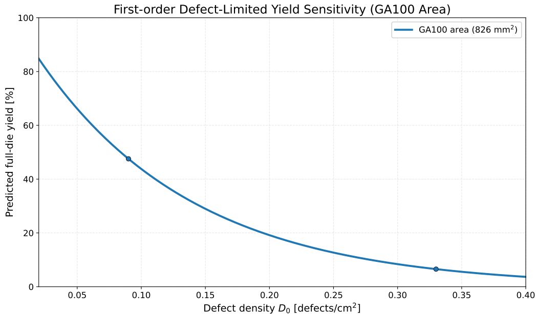
Figure C.1.: First-order defect-limited yield sensitivity under Y_{\text{full}} \approx e^{-AD_0} for GA100 area (826 mm 2 ). Marker points use industry-reported N7 anchor values ( D_0 \approx 0.33 and D_0 \approx 0.09 ).
