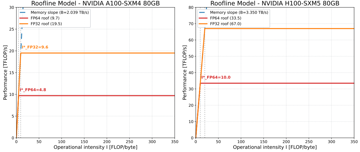
Figure 3.5.: Combined roofline envelopes for A100-SXM4-80GB and H100-SXM5-80GB using FP64 and FP32 ceilings. The H100 panel shifts both roofs upward and to higher operational intensity due to higher compute throughput and memory bandwidth.
