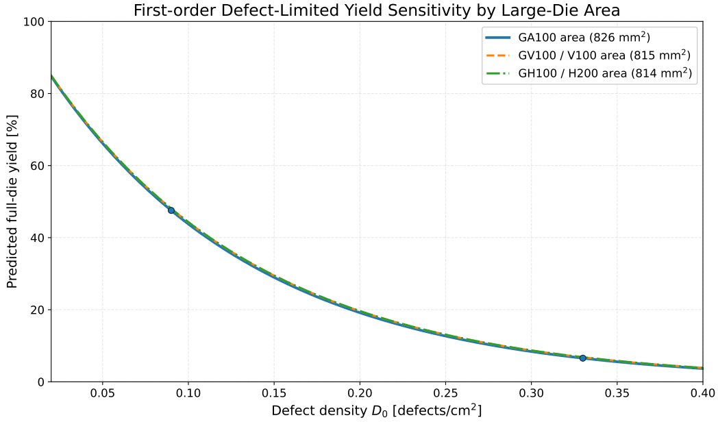
Figure 2.8.: First-order defect-limited yield sensitivity under Y_{\text{full}} \approx e^{-AD_0} for GA100 area ( 826 \text{ mm}^2 ), GV100/V100 area ( 815 \text{ mm}^2 ), and GH100/H200 area ( 814 \text{ mm}^2 ). Marker points use industry-reported N7 anchor values ( D_0 \approx 0.33 and D_0 \approx 0.09 ).
