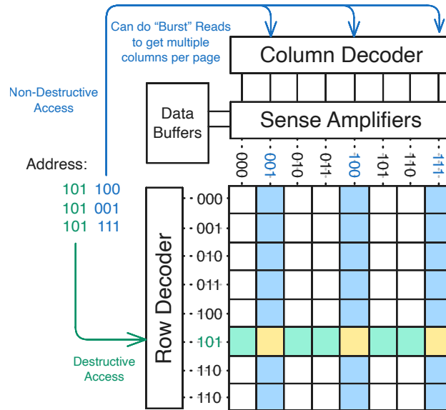
Figure 2.7.: Schematic for HBM/DRAM row-column access. A read activates one row, latches it into the sense amplifiers, and then uses the column decoder to select transferred data (including burst reads from the open row buffer).
