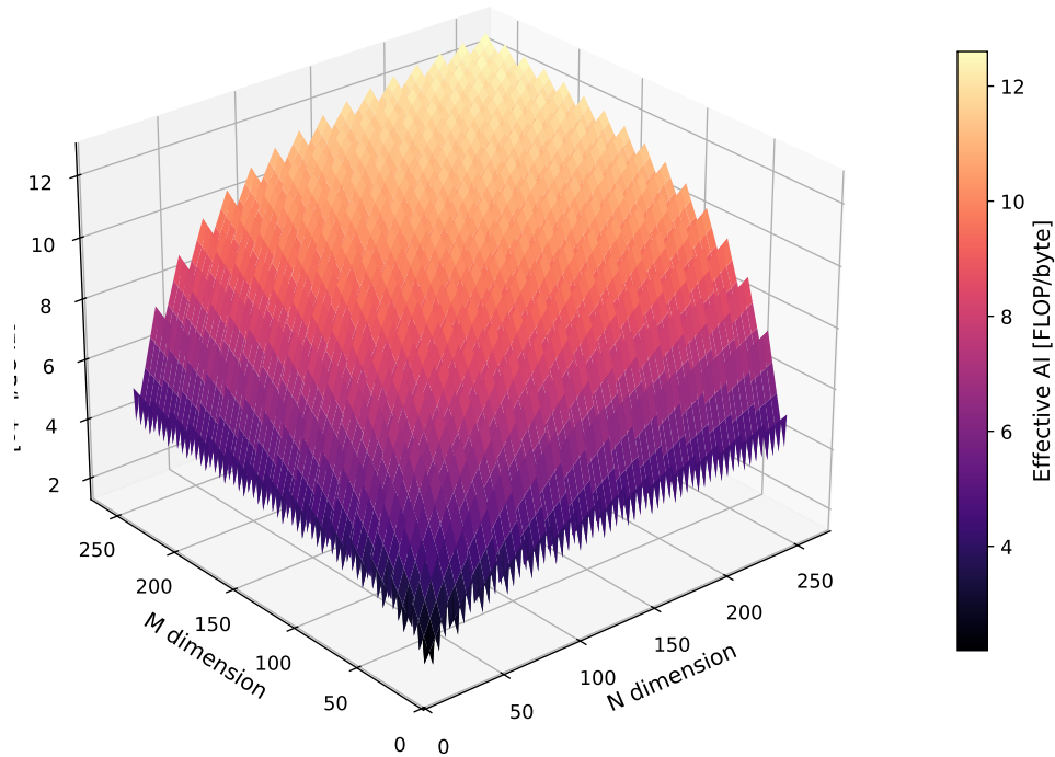
Figure 3.4.: 3D surface of effective arithmetic intensity I_{\text{eff}}(M, N, K; t) for FP32 at fixed K = 64 with t = 16 padding.
