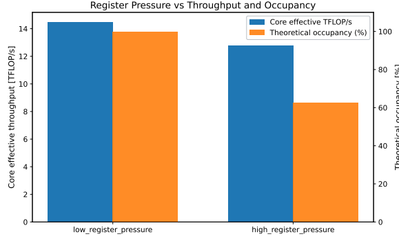
Figure 5.3.: Register pressure versus throughput and occupancy.
