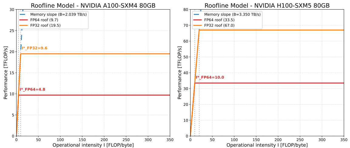
Figure 3.6.: Combined roofline envelopes for A100-SXM4-80GB and H100-SXM5-80GB using FP64 and FP32 ceilings. The H100 panel shifts both roofs upward and to higher operational intensity due to higher compute throughput and memory bandwidth.
