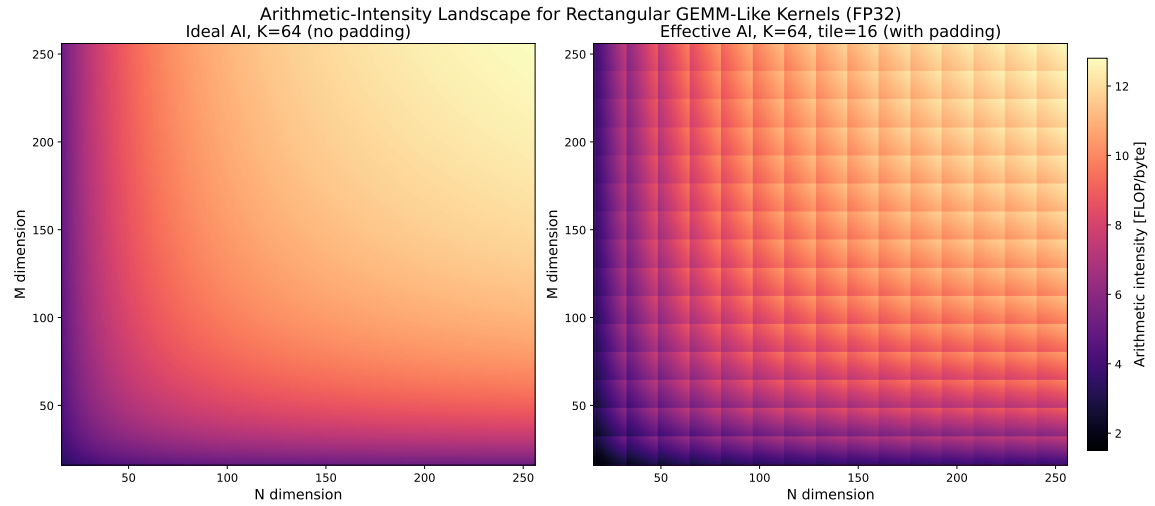
Figure 3.3.: Arithmetic-intensity map for rectangular GEMM-like kernels in FP32 at fixed K = 64 . Left: ideal intensity without padding. Right: effective intensity with 16-element padding on M, N, K (useful FLOPs over padded traffic).
