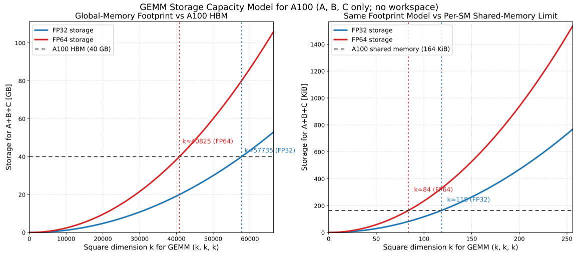
Figure 3.5.: Storage model M(k; s) = 3k^2 s for square GEMM in FP32 and FP64. Left: intersection with A100 HBM capacity (40 GB). Right: same model against per-SM shared-memory capacity (164 KiB).
