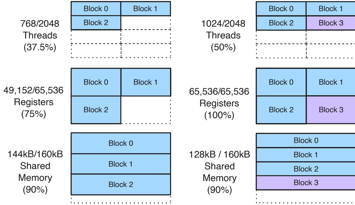
(a) Initial setup with 48 kB shared memory per block. Occupancy is limited by shared memory. (b) After reducing to 32 kB shared memory per block. Occupancy increases by one block, then registers become the occupancy limit.
