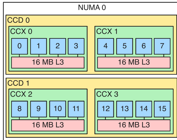
Figure 2.9.: NUMA and chiplet hierarchy of a single AMD EPYC 7742 socket. Each socket contains 8 CCDs grouped into 4 NUMA domains (NPS=4 configuration). Each CCD holds two CCXes, each with 4 cores and a private 16 MB L3 cache. All CCDs connect to a central I/O die that houses the memory controllers and PCIe root complexes.
