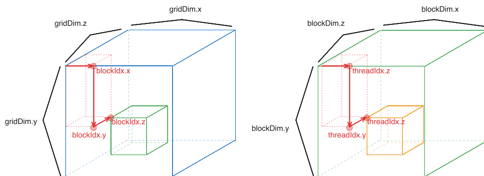
Figure 2.11.: CUDA execution hierarchy showing the mapping of grids to thread blocks and threads. Threads are organised in up to three dimensions and identified using the built-in variables threadIdx and blockIdx .
