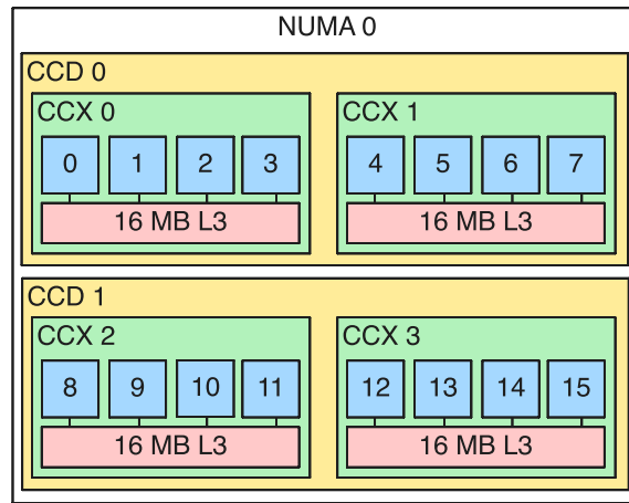
Figure 2.8.: NUMA and chiplet hierarchy of a single AMD EPYC 7742 socket. Each socket contains 8 CCDs grouped into 4 NUMA domains (NPS=4 configuration). Each CCD holds two CCXes, each with 4 cores and a private 16 MB L3 cache. All CCDs connect to a central I/O die that houses the memory controllers and PCIe root complexes.
