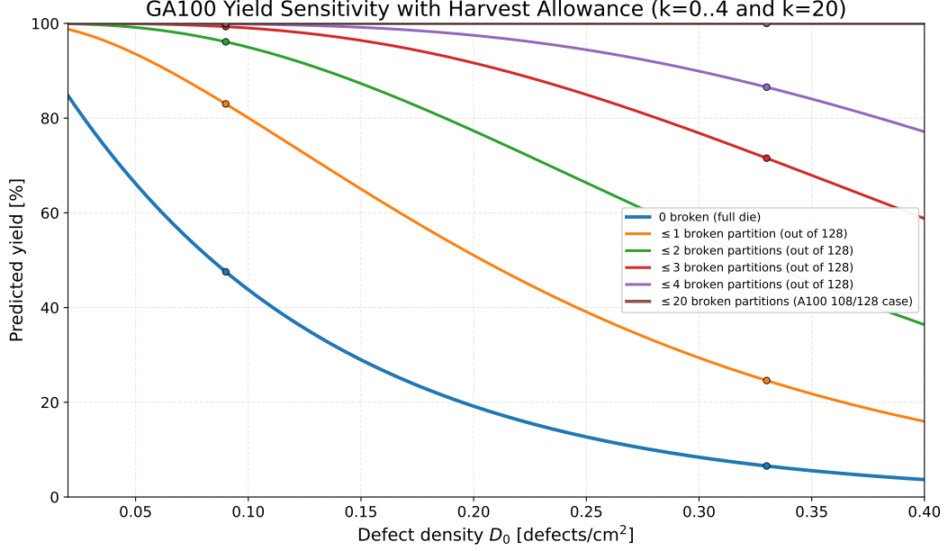
Figure C.1.: First-order defect-limited yield sensitivity for GA100 area (826 mm 2 ) using harvest allowances k \in \{0, 1, 2, 3, 4, 20\} broken partitions out of 128. Marker points use industry-reported N7 anchor values ( D_0 \approx 0.33 and D_0 \approx 0.09 ).
