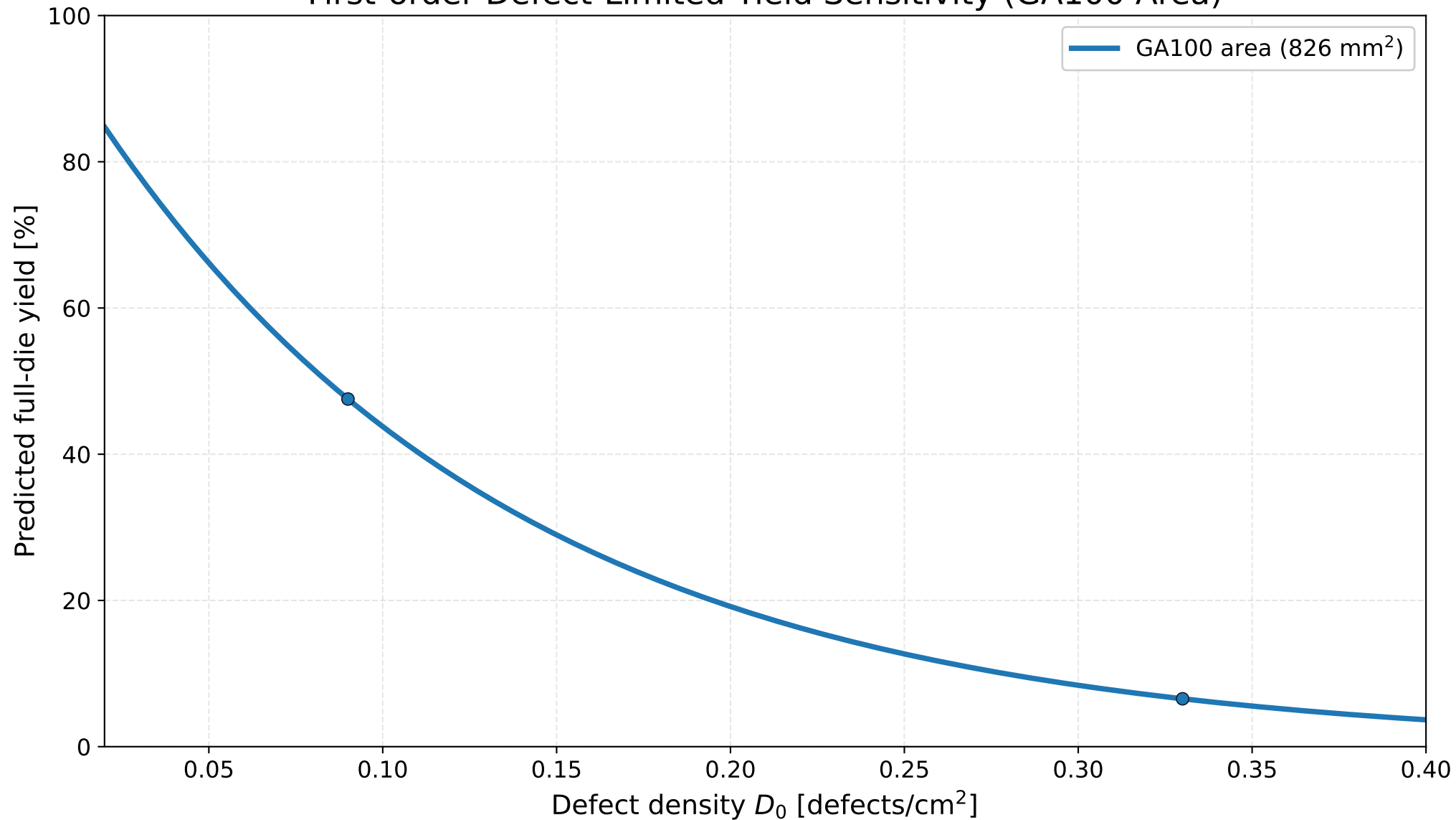
First-order Defect-Limited Yield Sensitivity (GA100 Area)
