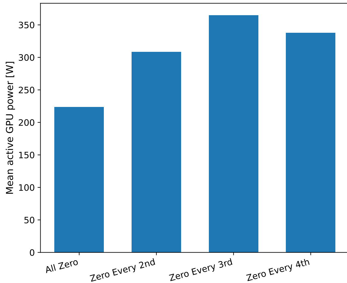
GEMM Value-Pattern Power
