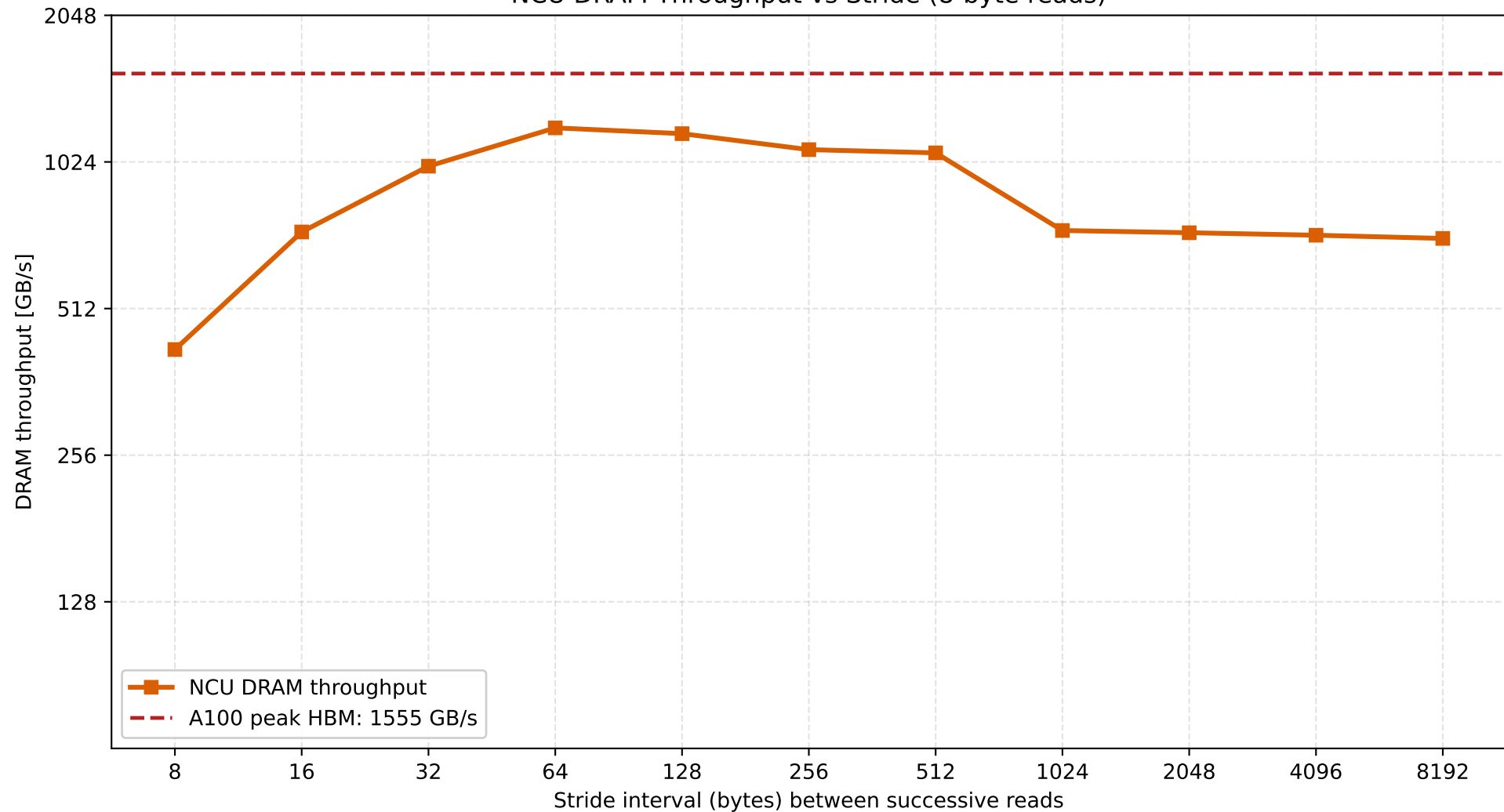
NCU DRAM Throughput vs Stride (8-byte reads)
