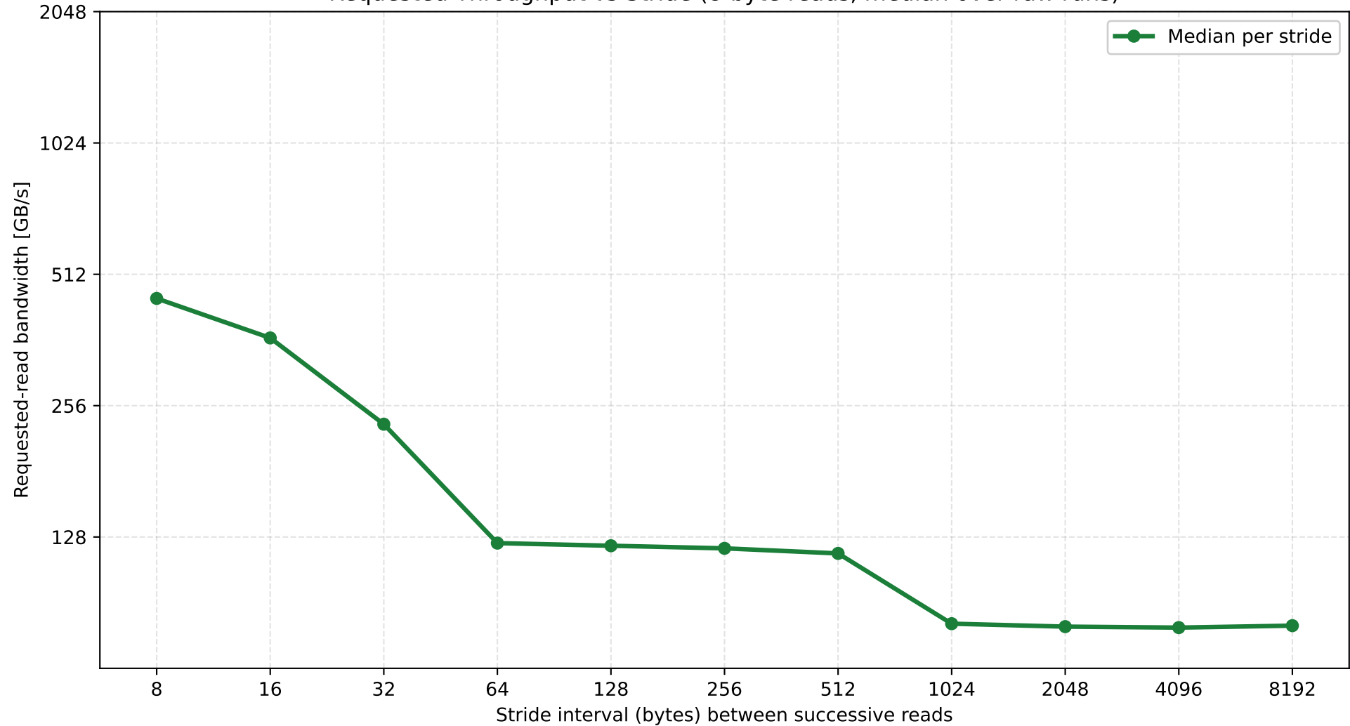
Requested Throughput vs Stride (8-byte reads, median over raw runs)
