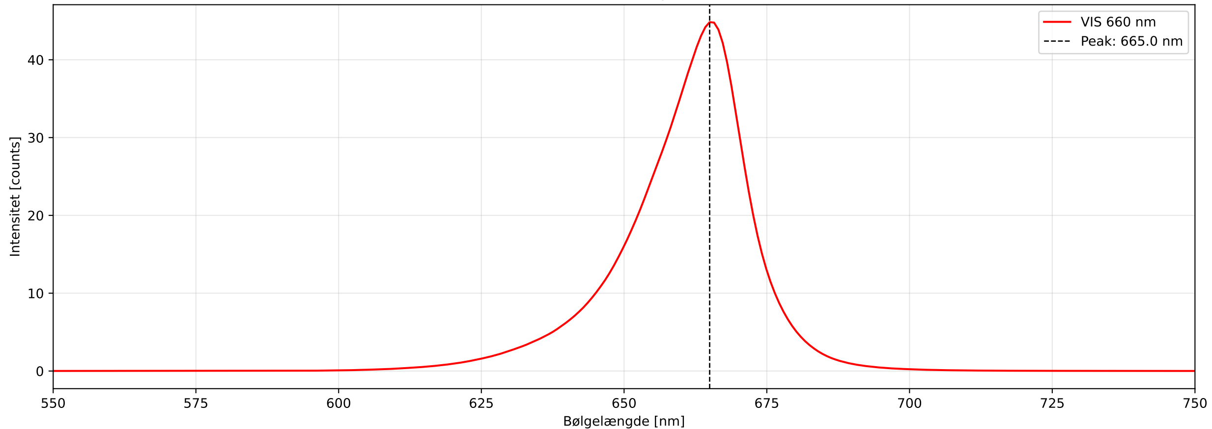
VIS 660 nm LED spektrum
