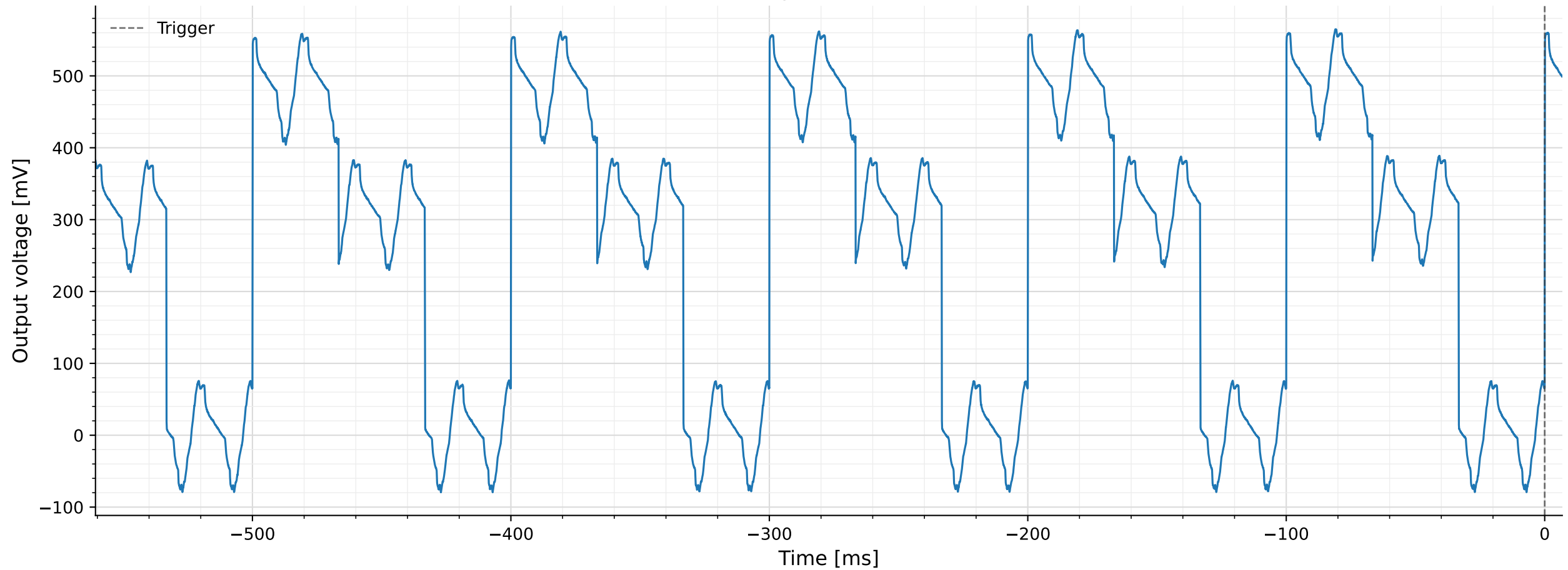
TIA output, R_f = 2.1\text{ M}\Omega
