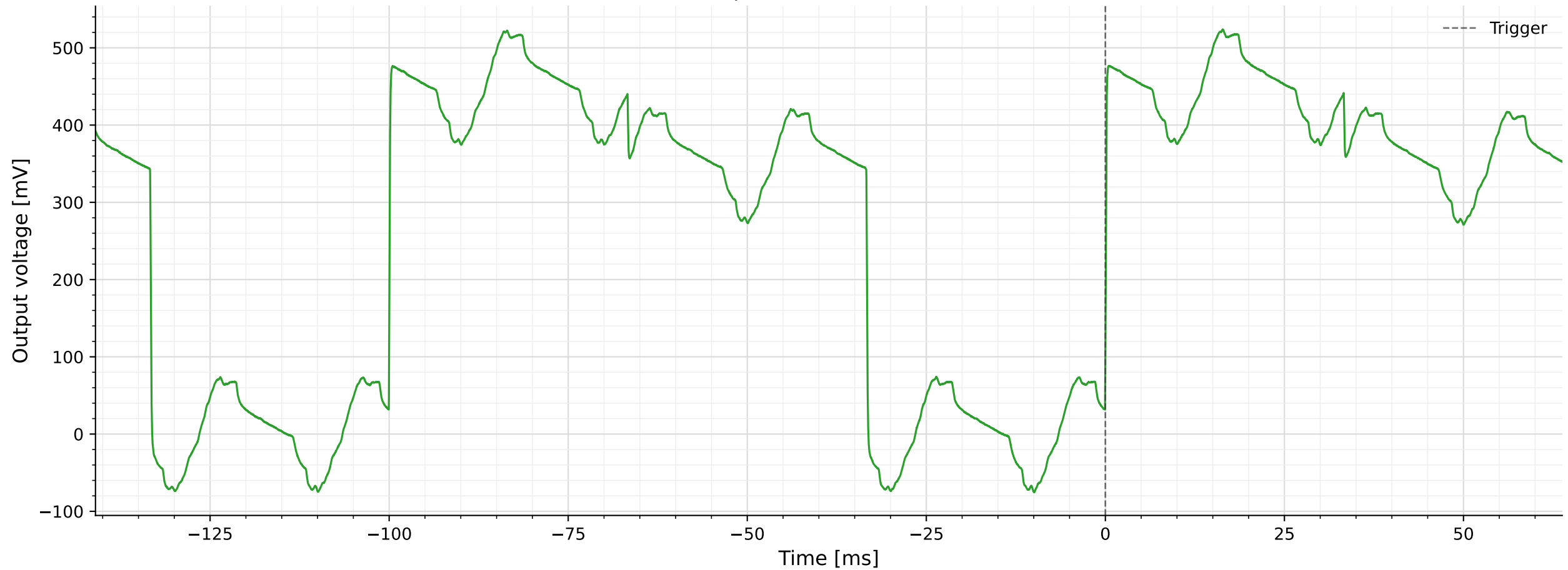
TIA output with LPF, R_f = 2.1\text{ M}\Omega
