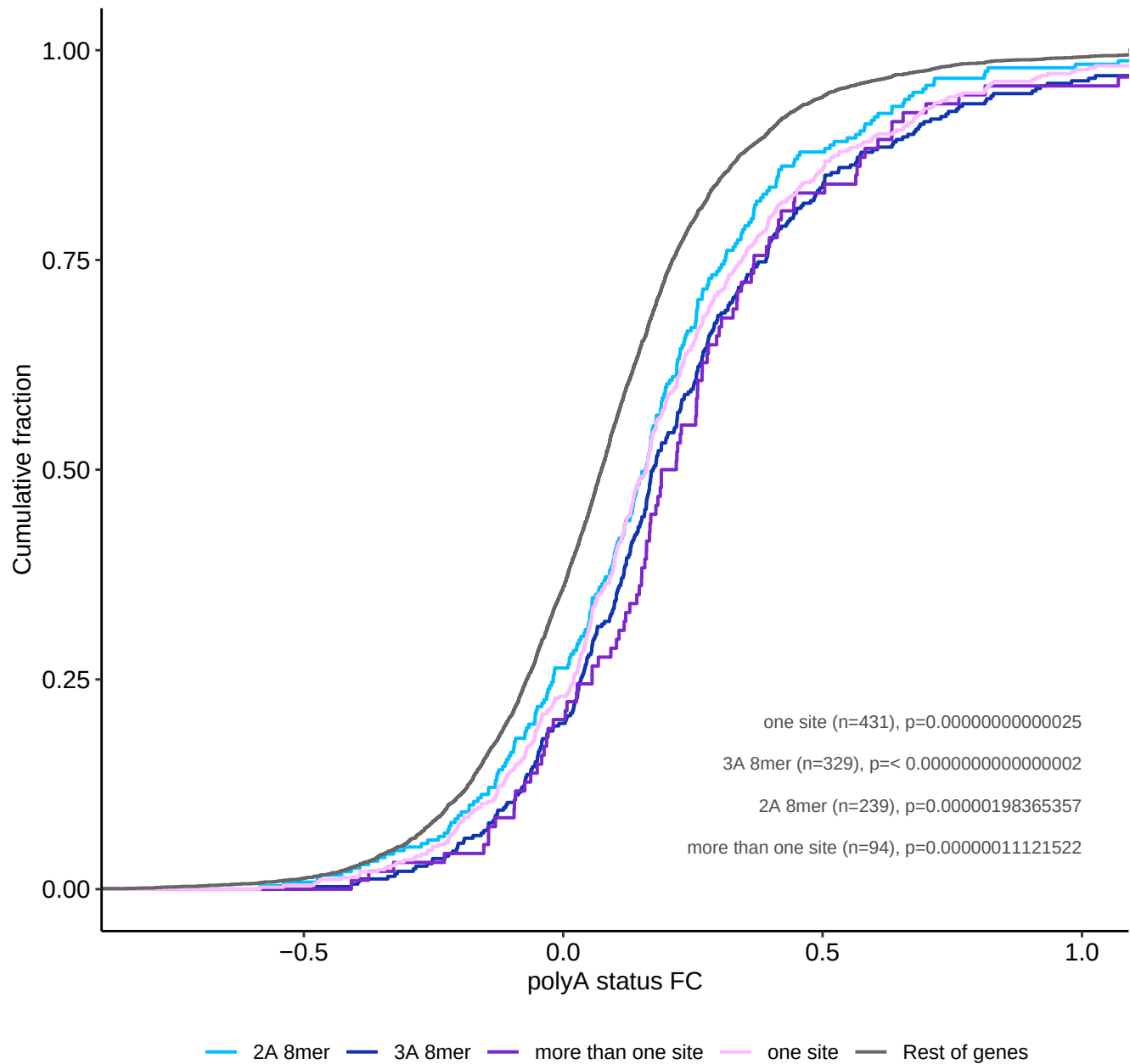
alone vs g2 (with alpha)
