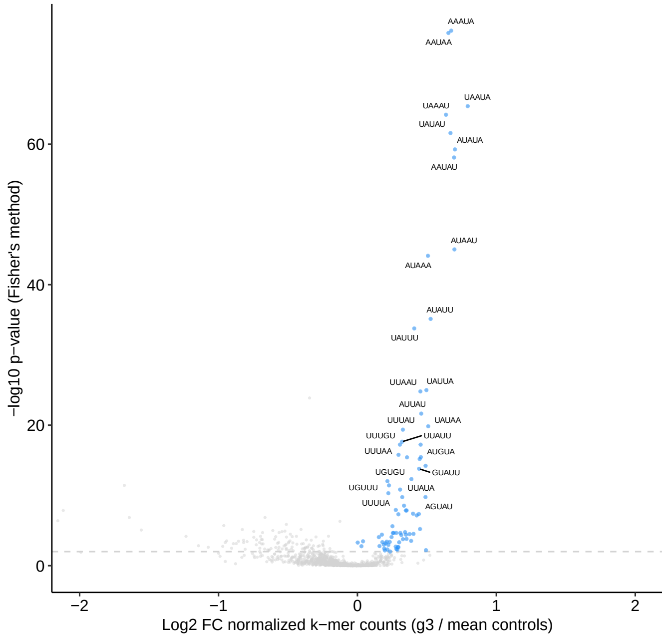
Enriched 5-mers in g3 vs control groups
