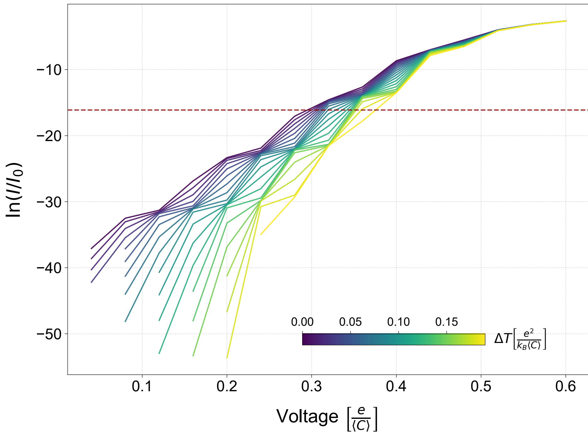
Semi-Log I-V for Fixed Island Temperature T = 5T_0
