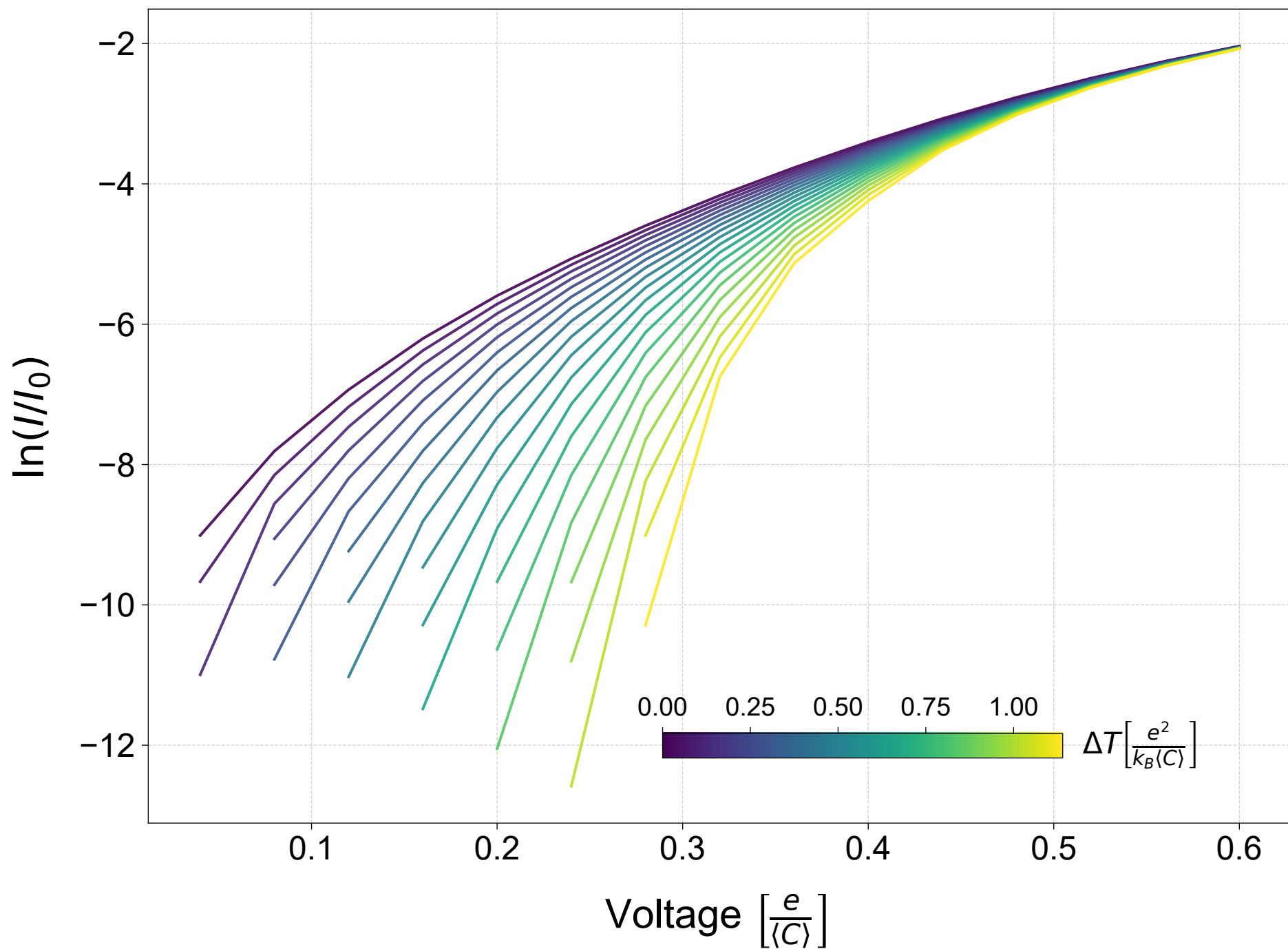
Semi-Log I-V for Fixed Island Temperature T = 30T_0
