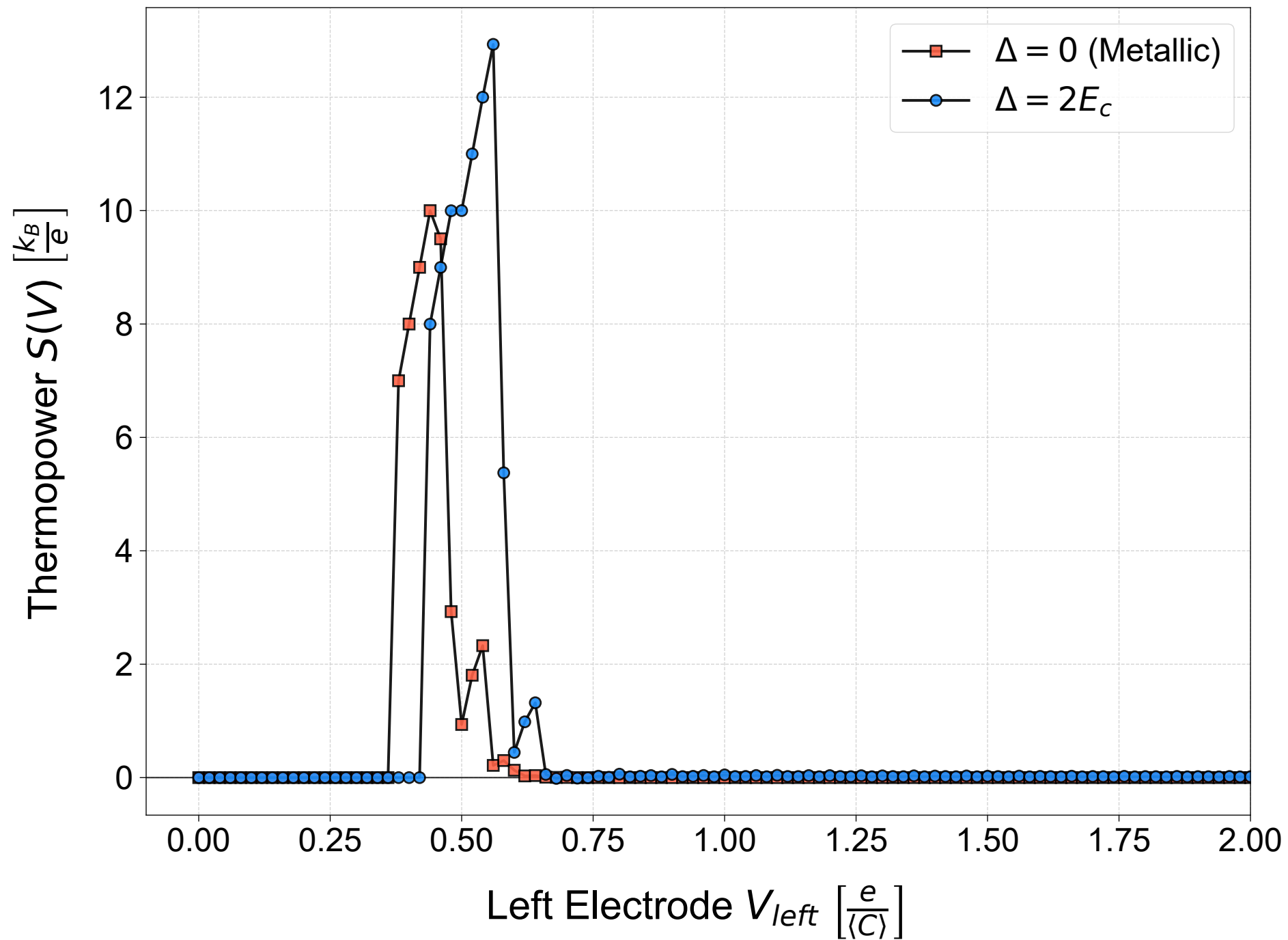
Thermopower vs. Voltage ( \Delta T/E_c = 0.8 )
