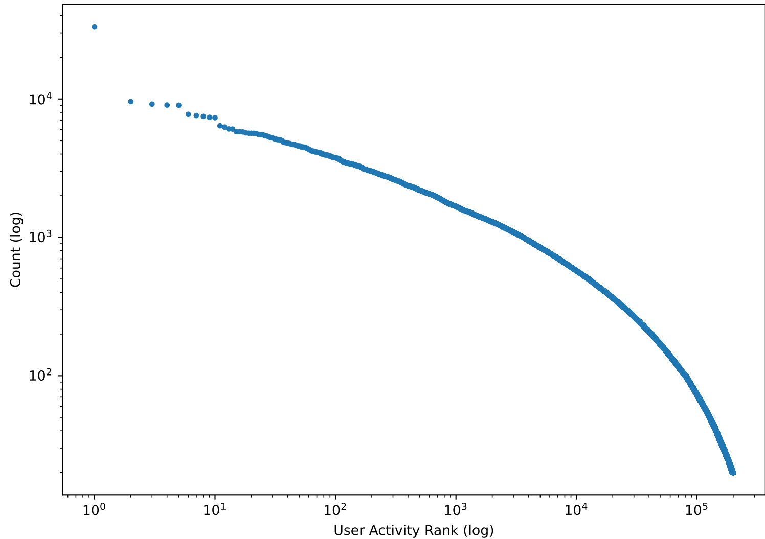
User Activity Rank-Count (log-log)
