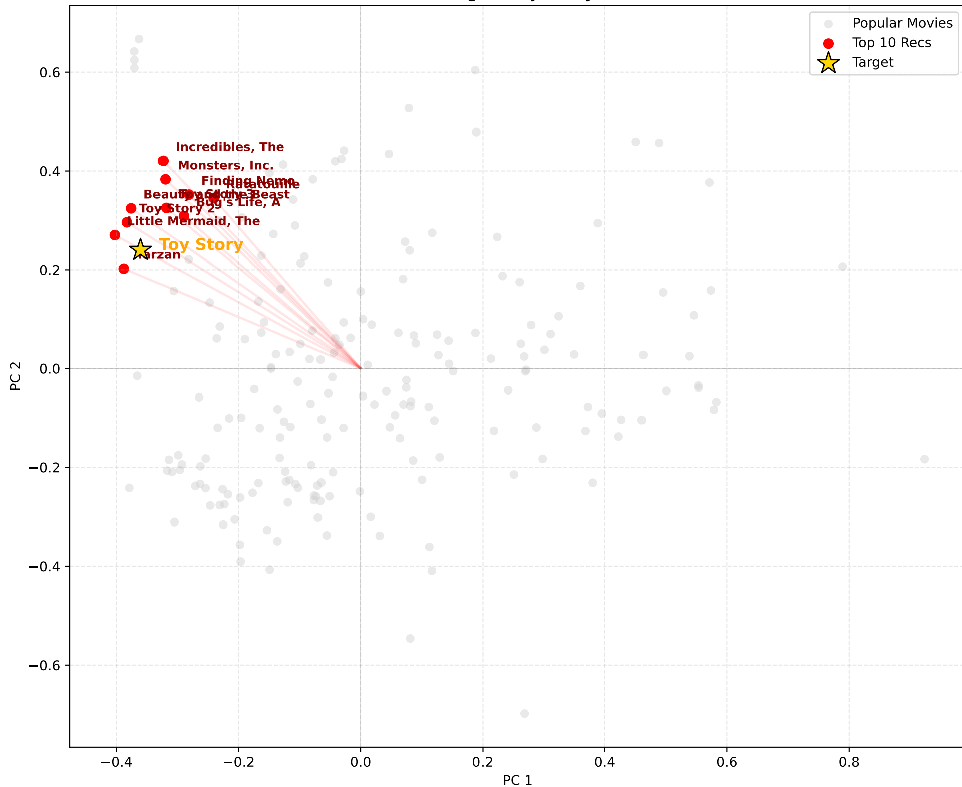
Latent Space Map (K=20) Target: Toy Story
