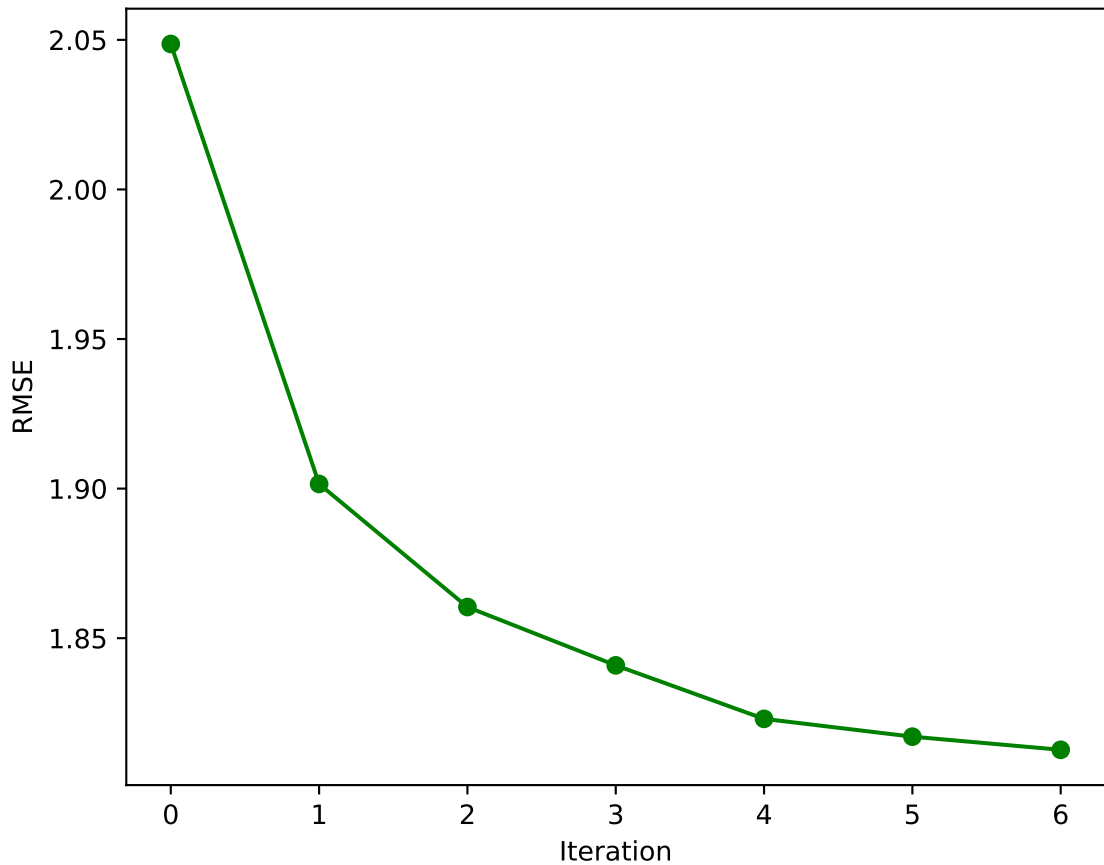
Test RMSE
