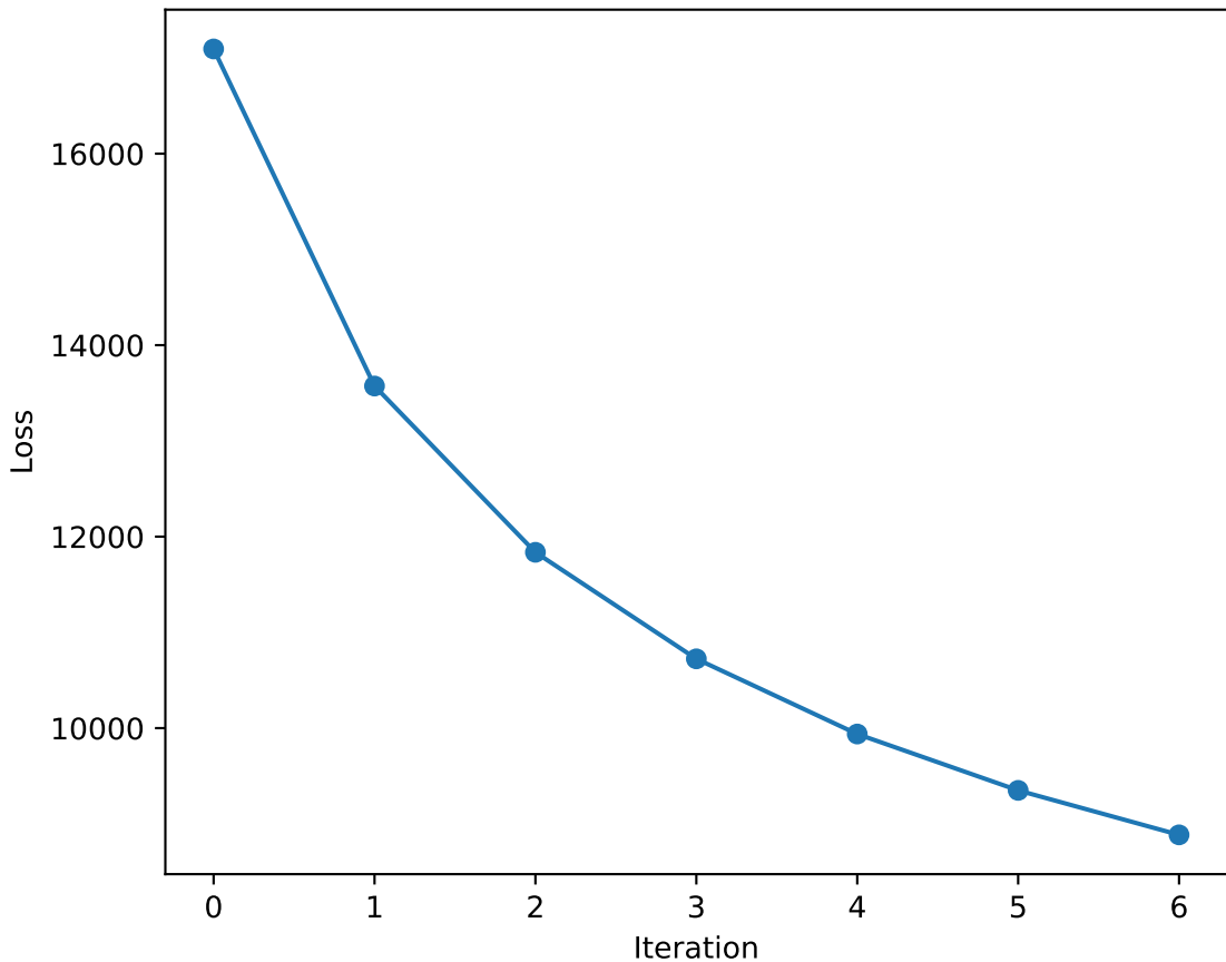
Regularized Negative Log Likelihood
