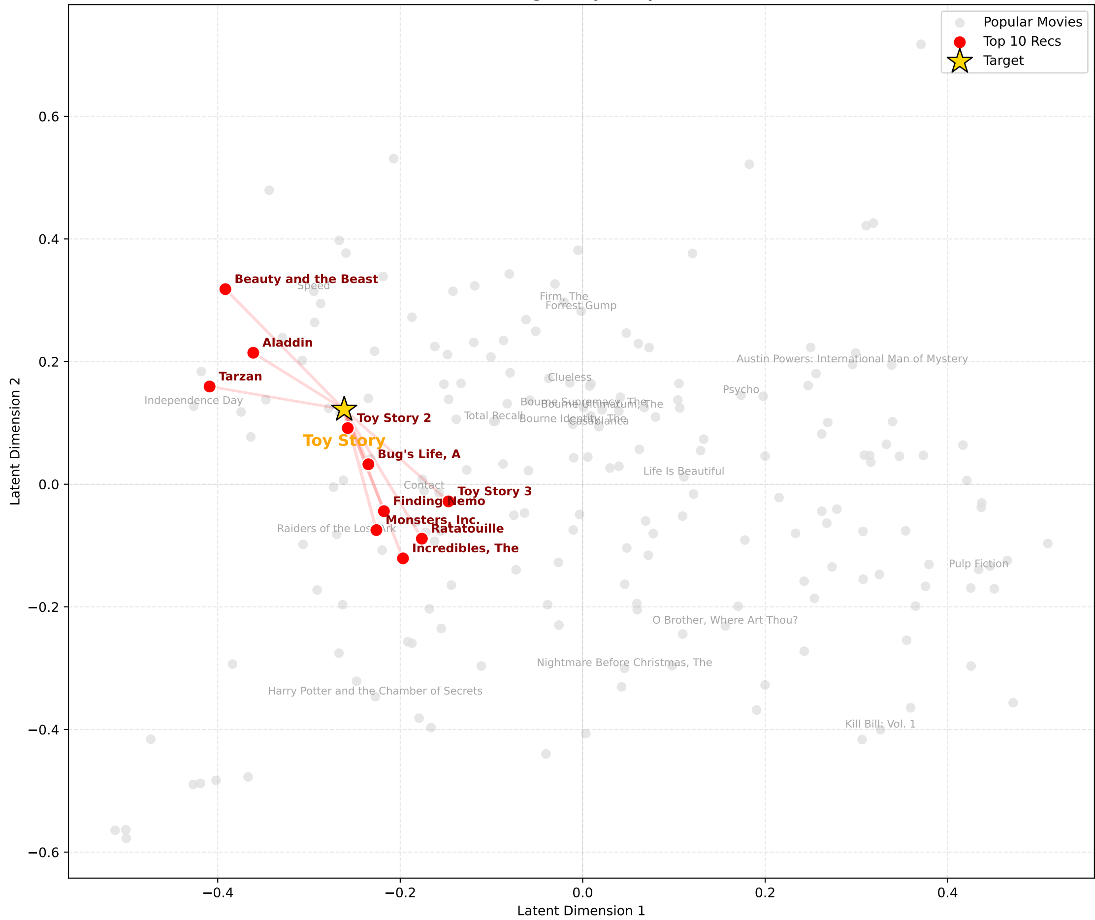
Movie Map (K=10) Target: Toy Story
