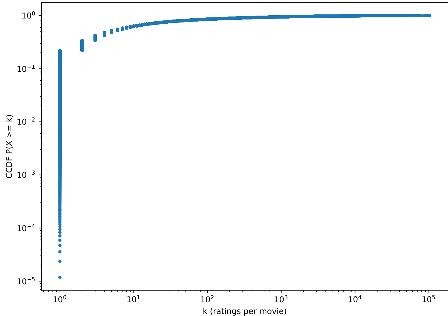
Movie Popularity CCDF (log-log)
