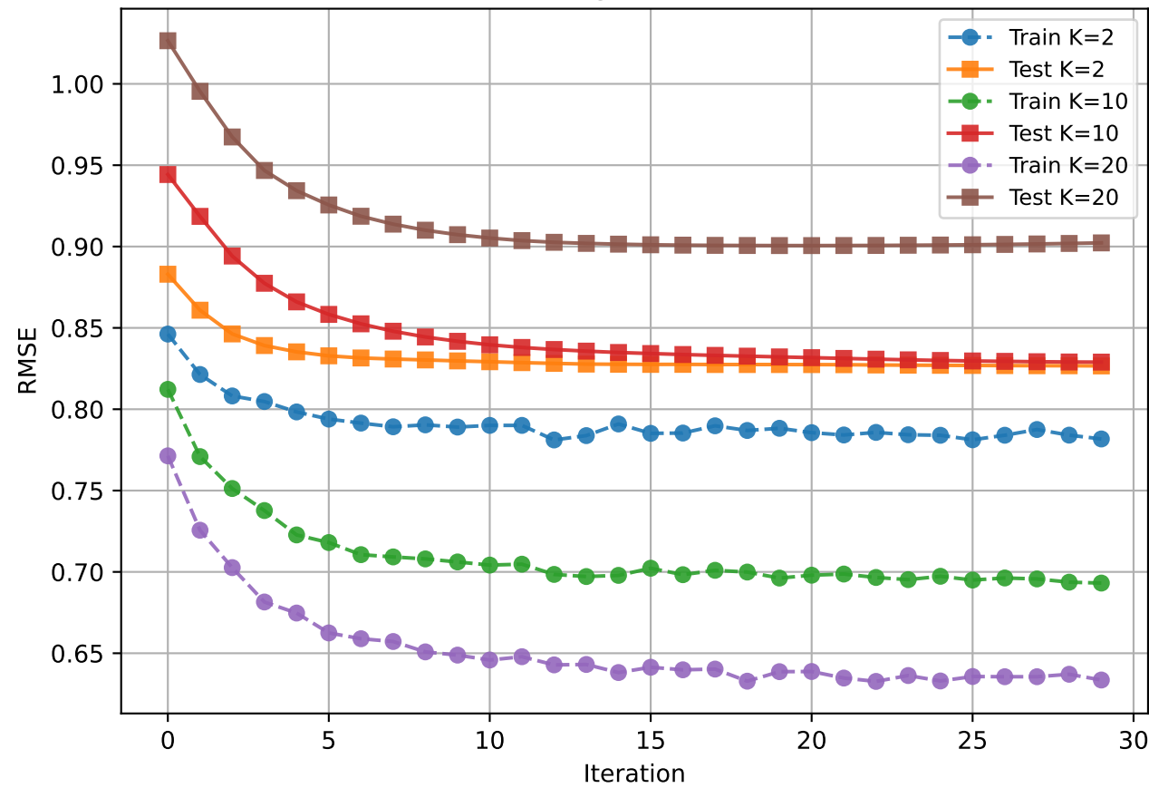
a. Training vs Test RMSE
