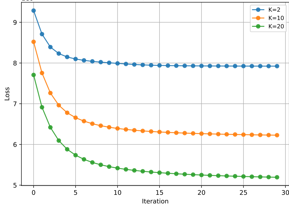
b. Training Negative Log-Likelihood
