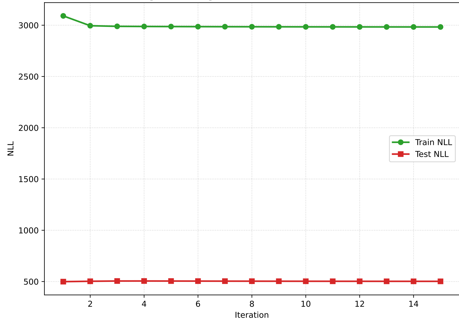
Negative Log-Likelihood: Train vs Test
