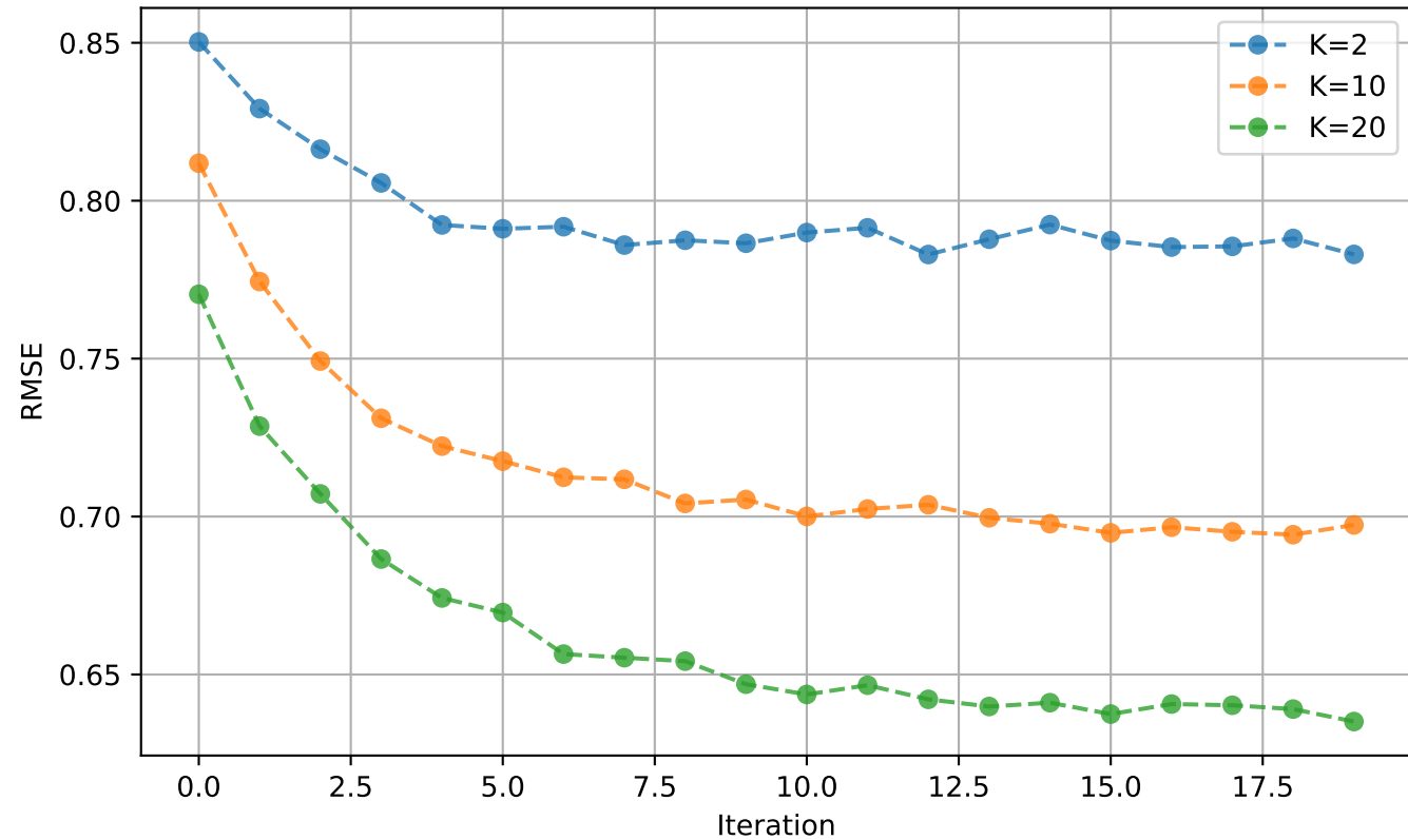
Training RMSE
