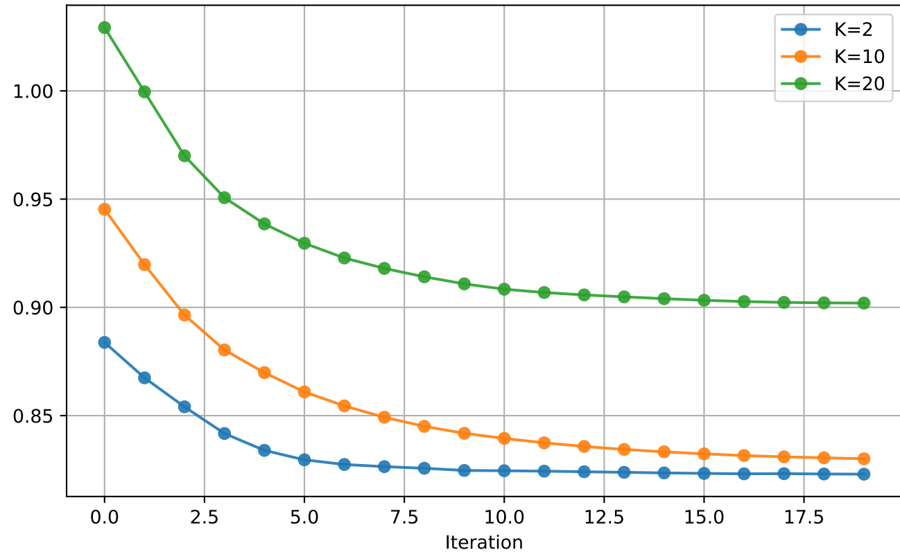
Test RMSE
