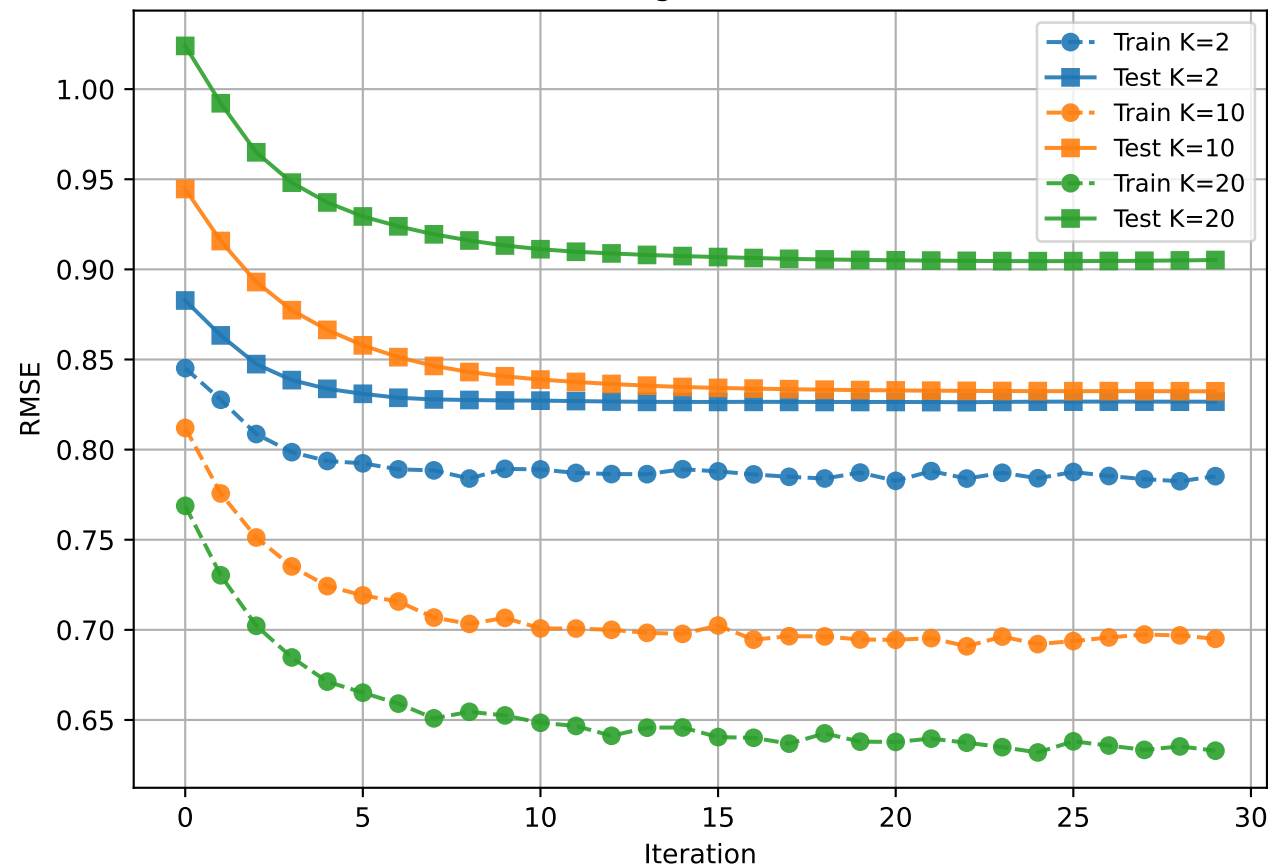
a. Training vs Test RMSE
