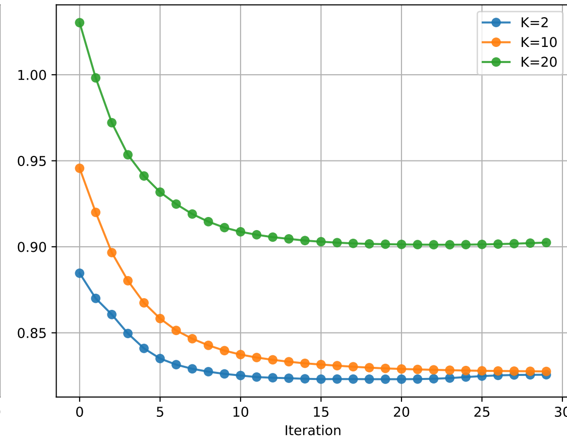
b. Test RMSE
