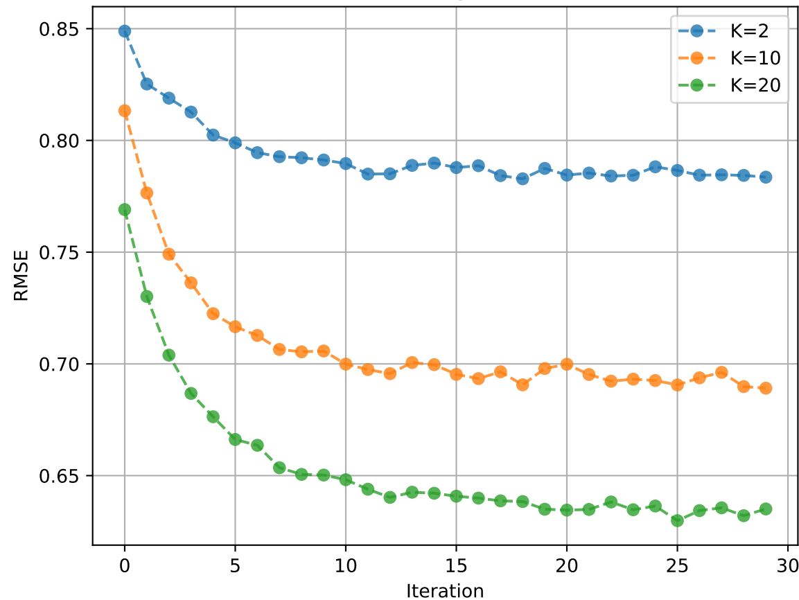
a. Training RMSE
