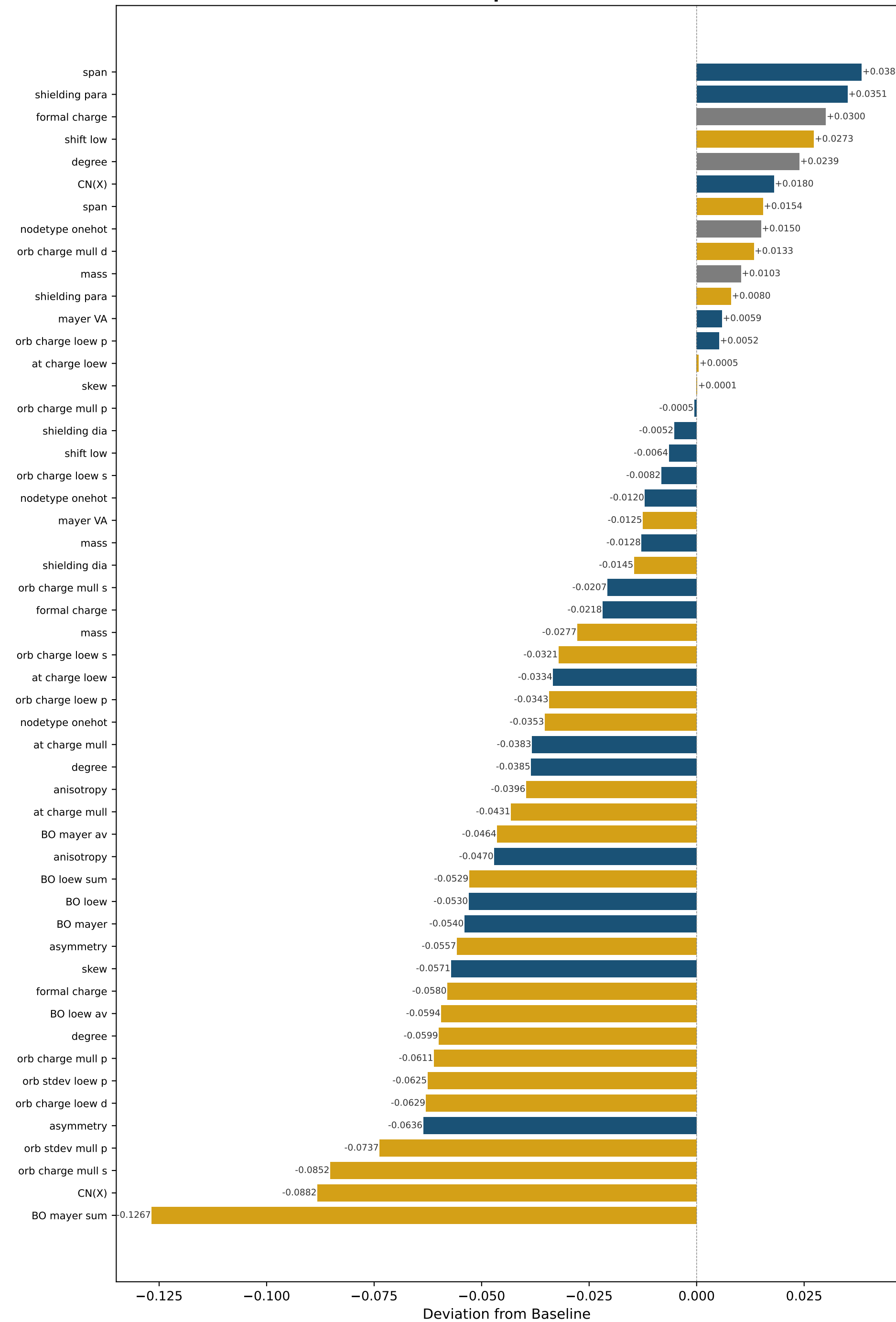
13 C Shift Top 53 Features
