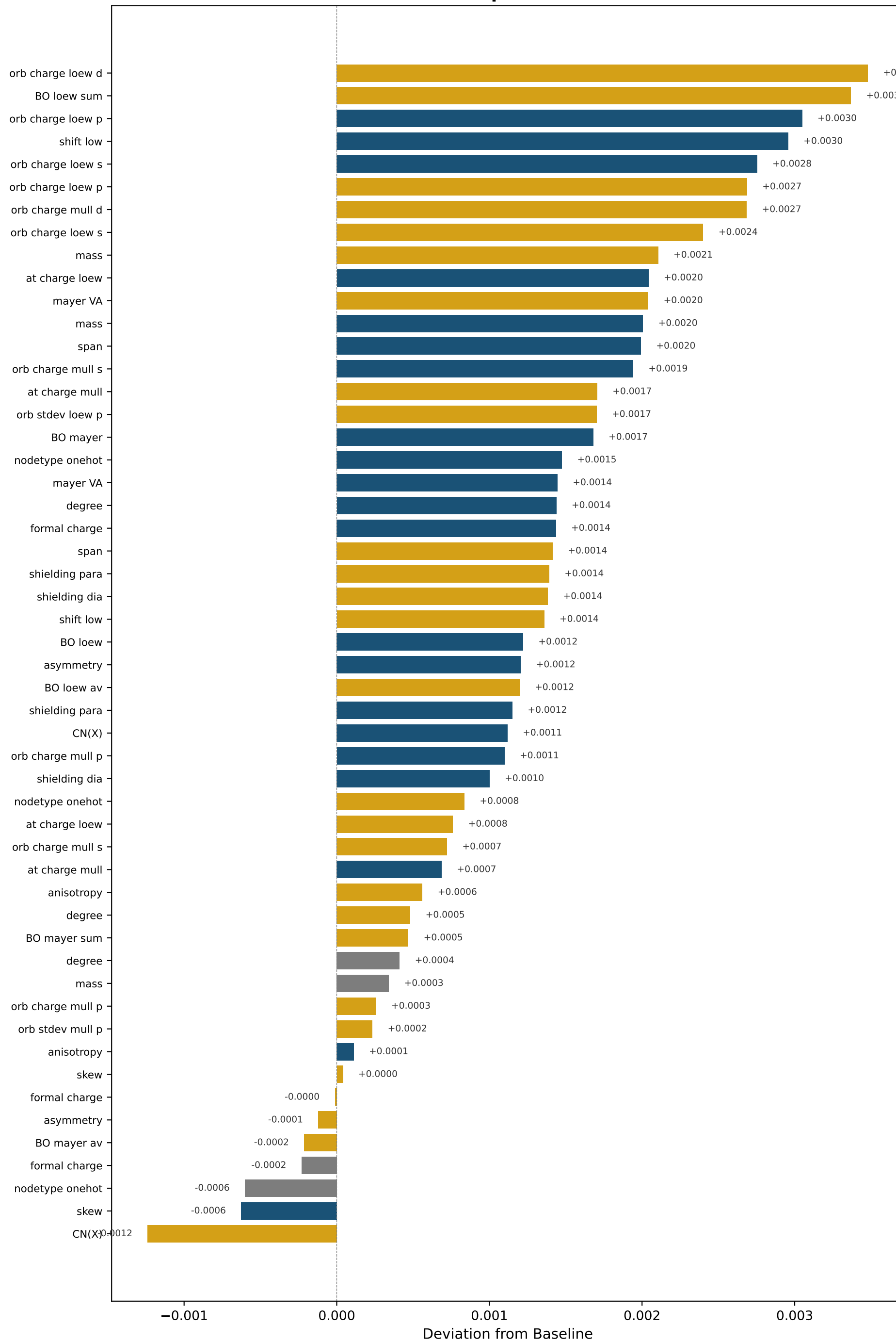
1 H Shift Top 53 Features
