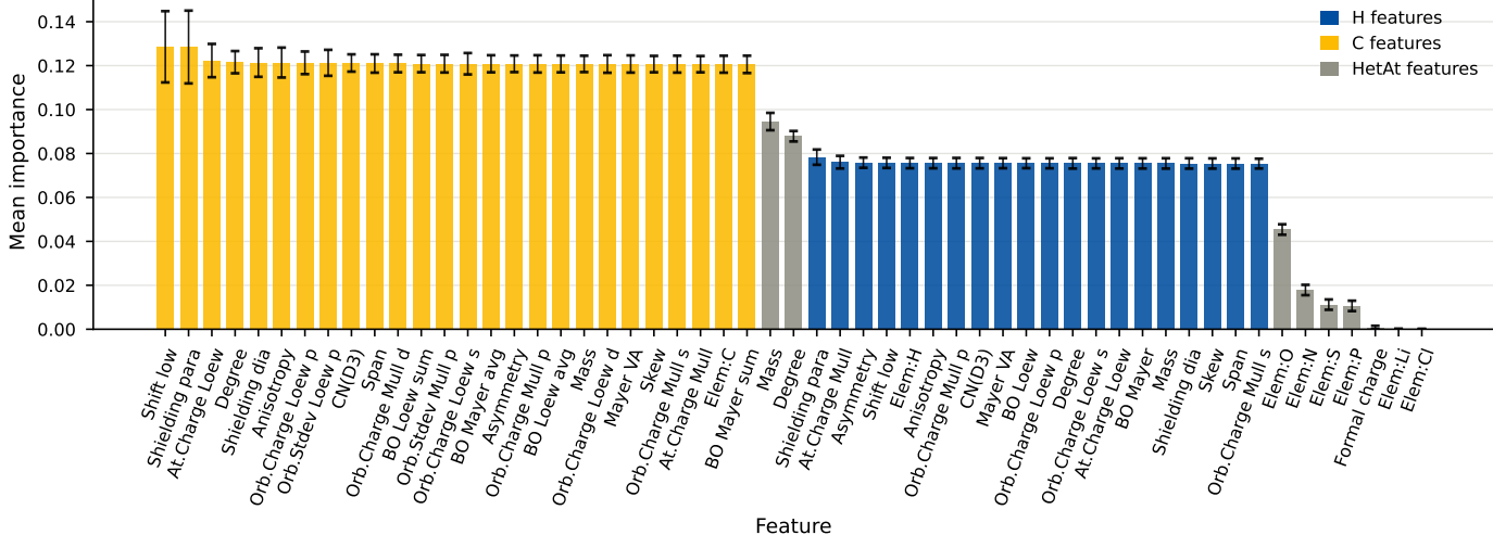
Mean feature importance +/- std (Target = C)
