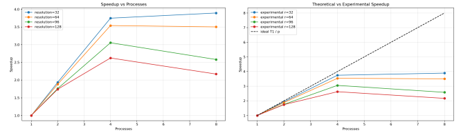
Fig. 2. Measured speedup by process count and comparison against the ideal T_1/p trend.
