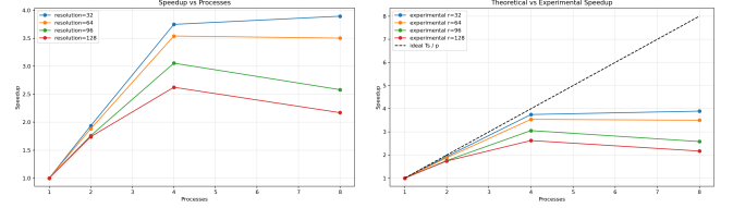
Fig. 2. Measured speedup by process count and comparison against the ideal T_s/p trend.
