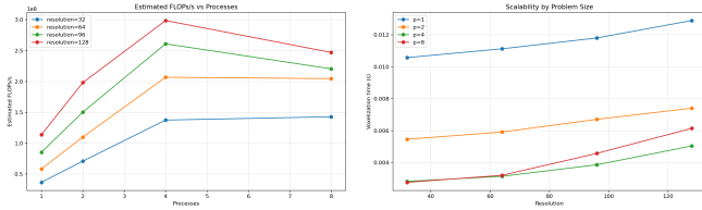
Fig. 3. Estimated FLOPs/s and scalability as grid resolution increases.
