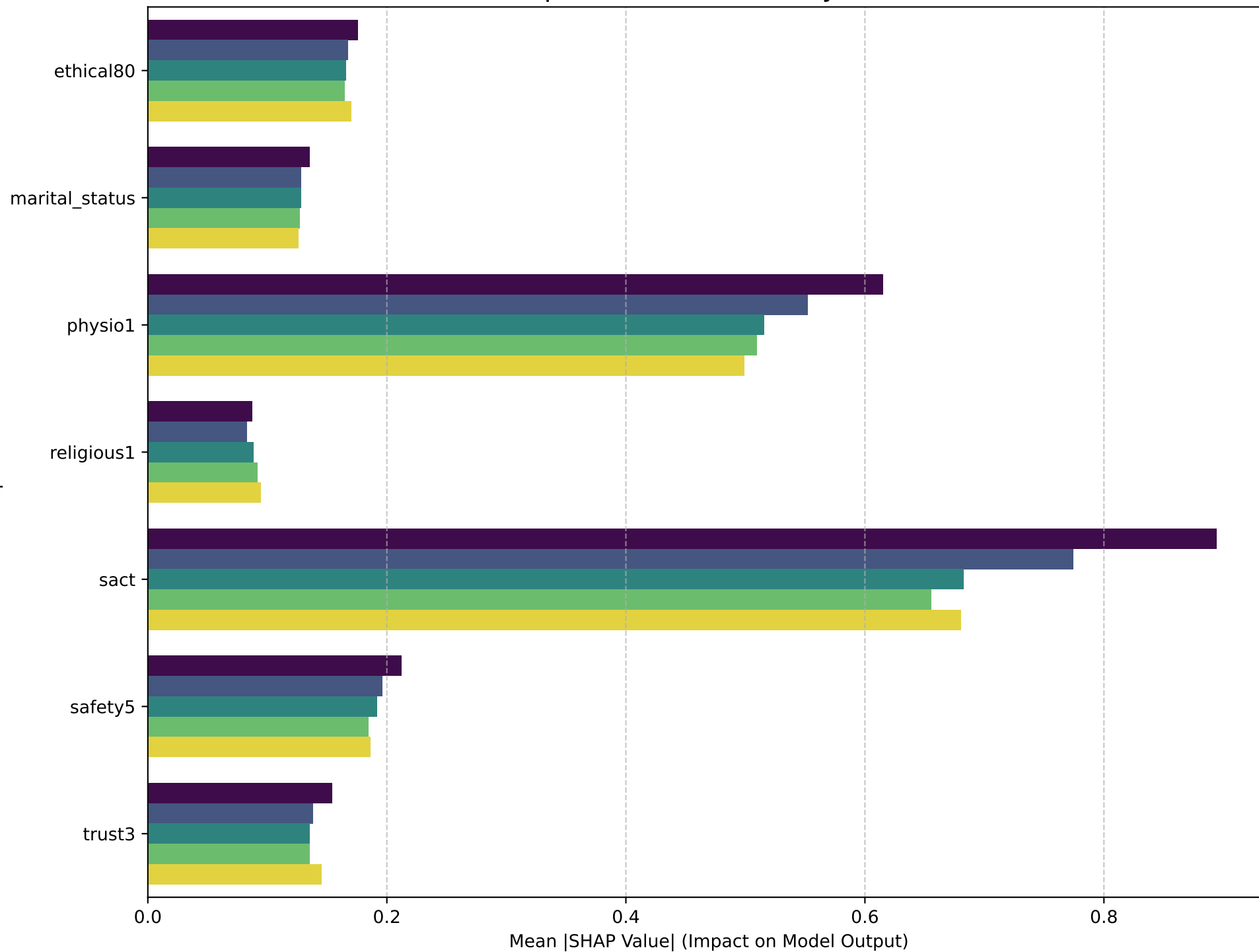
SHAP Feature Importance Classified by Income Scale (1-5)
