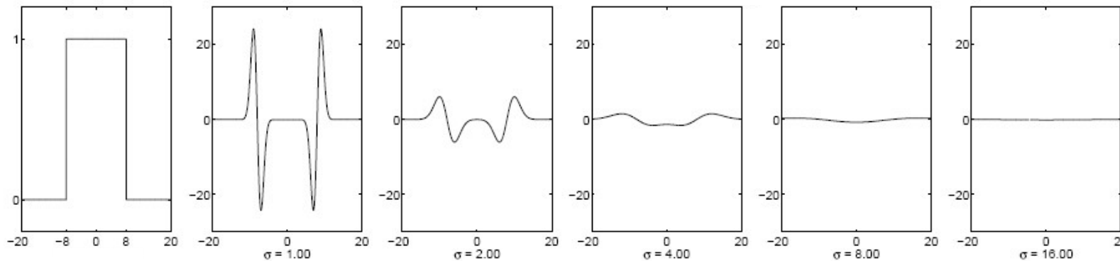
Scale-normalized Laplacian response
