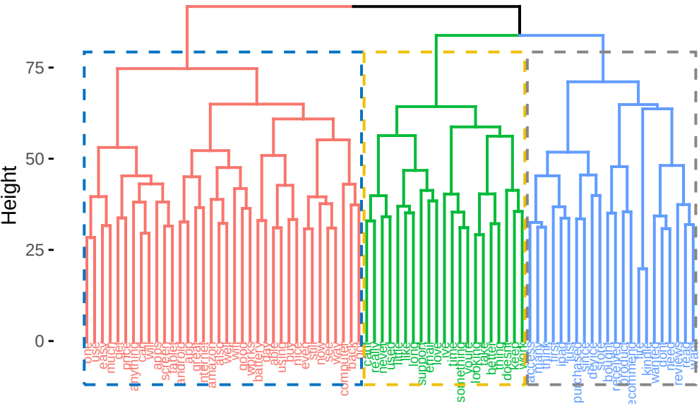
Cluster Dendrogram
