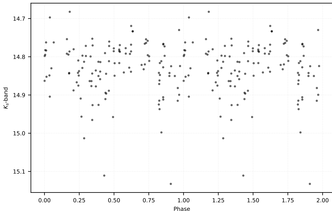
P: 0.25379 d | Class: EB | Subclass: EA | Field b278
