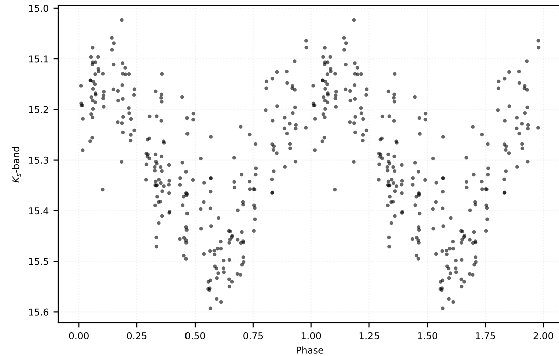
P: 0.46854 d | Class: RP | Subclass: RRc | Field b279
