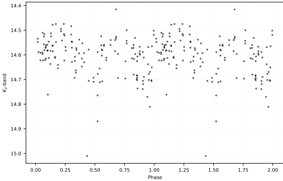
P: 0.35542 d | Class: EB | Subclass: EA | Field b279
