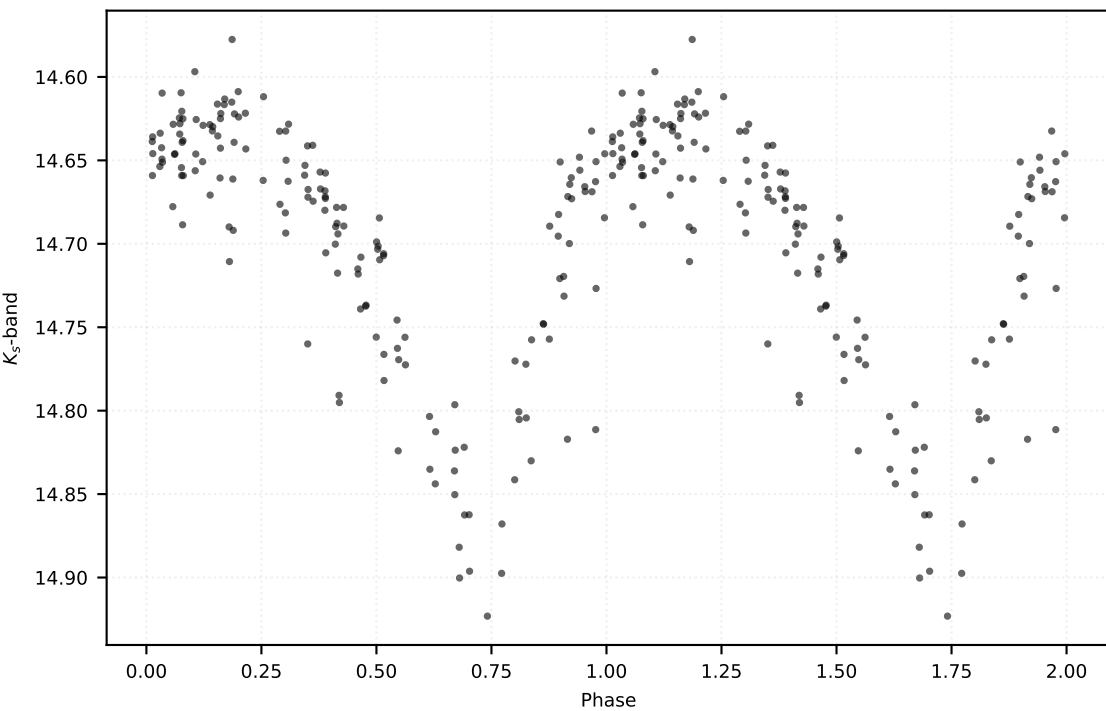
P: 0.38667 d | Class: RP | Subclass: RRab | Field b278
