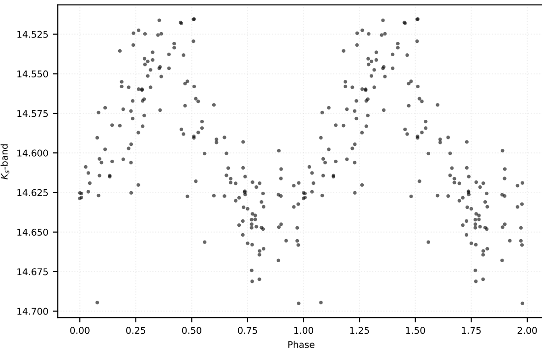
P: 2.25160 d | Class: RP | Subclass: CEP-10T | Field b278
