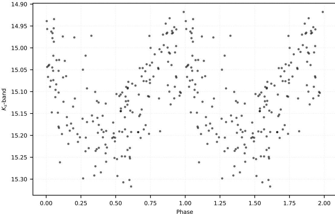
P: 2.27132 d | Class: RP | Subclass: CEP-F | Field b278
