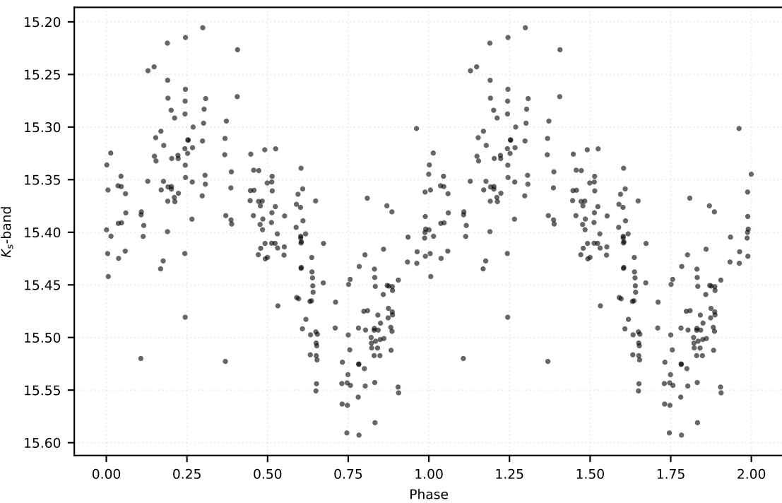
P: 0.46820 d | Class: RP | Subclass: R Rab | Field b278
