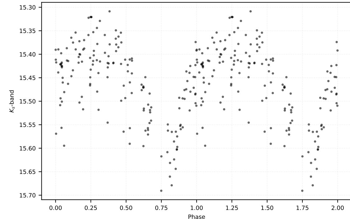
P: 0.33272 d | Class: RP | Subclass: RRab | Field b278
