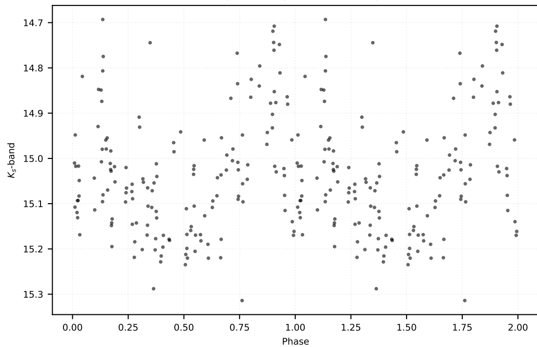
P: 0.10390 d | Class: RP | Subclass: UVAR | Field b278
