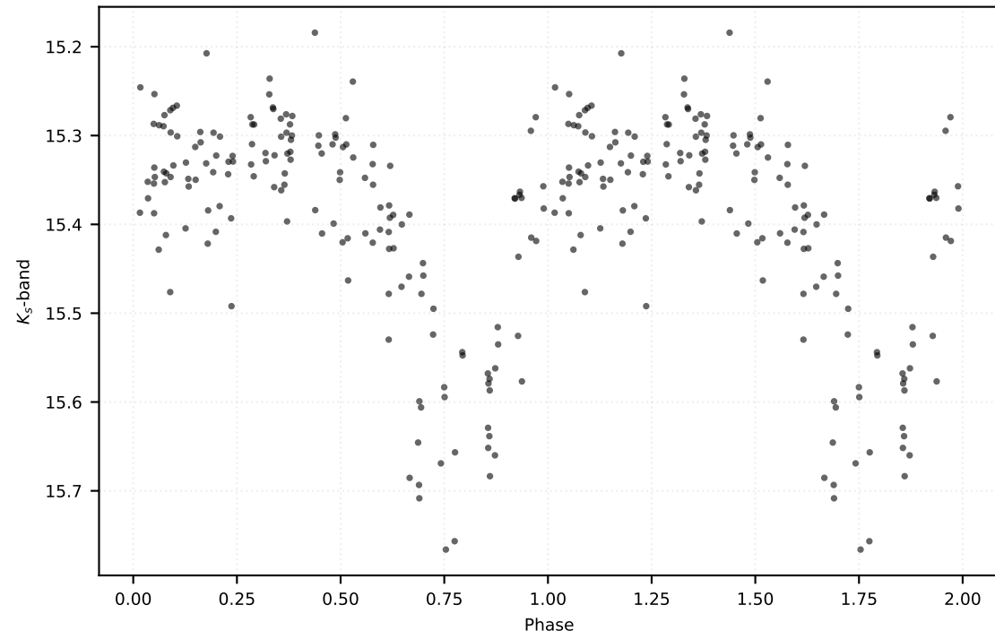
P: 0.50352 d | Class: RP | Subclass: CEP-1OT | Field b278
