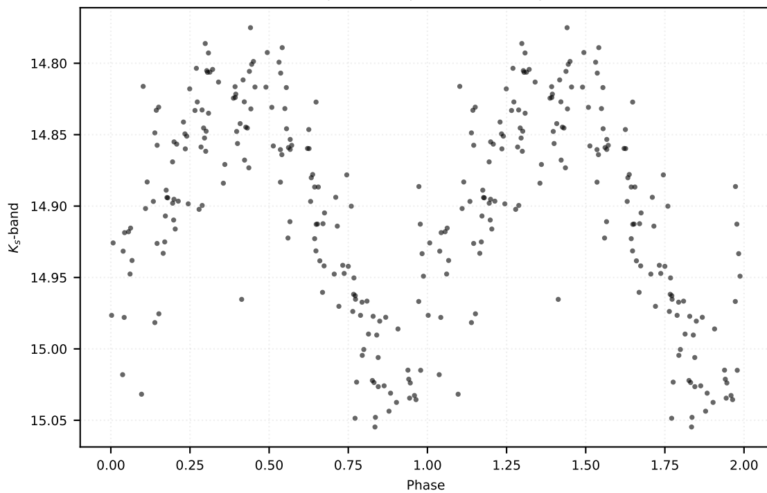
P: 0.13374 d | Class: RP | Subclass: UVAR | Field b278
