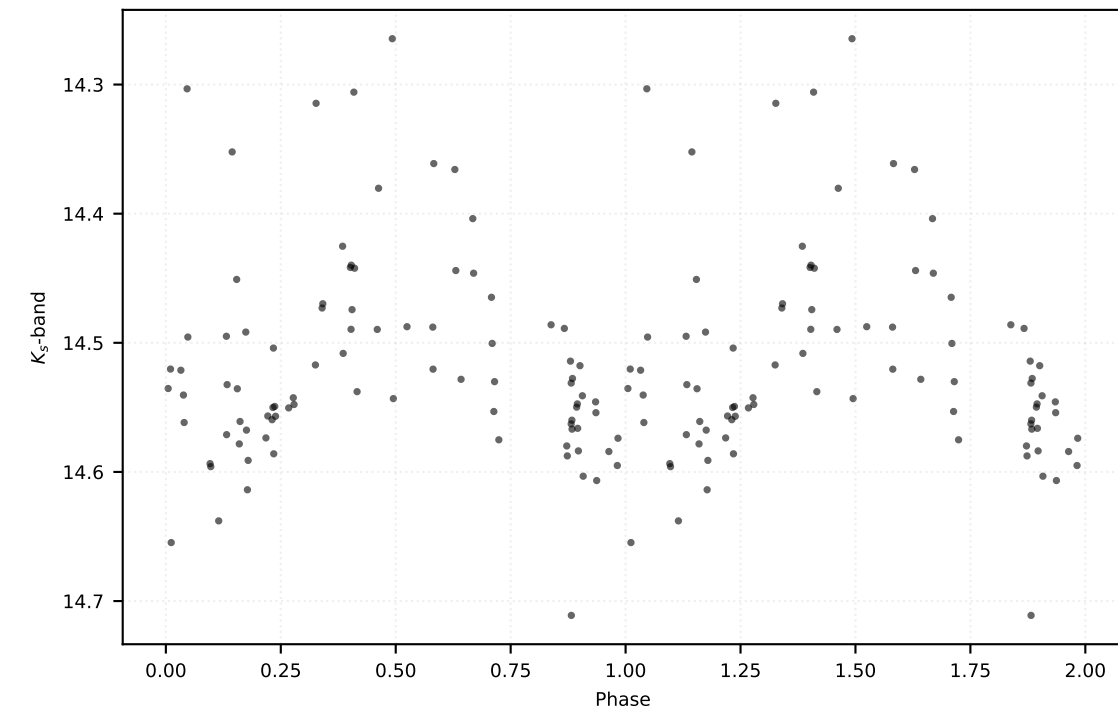
P: 0.25900 d | Class: RP | Subclass: UVAR | Field b279
