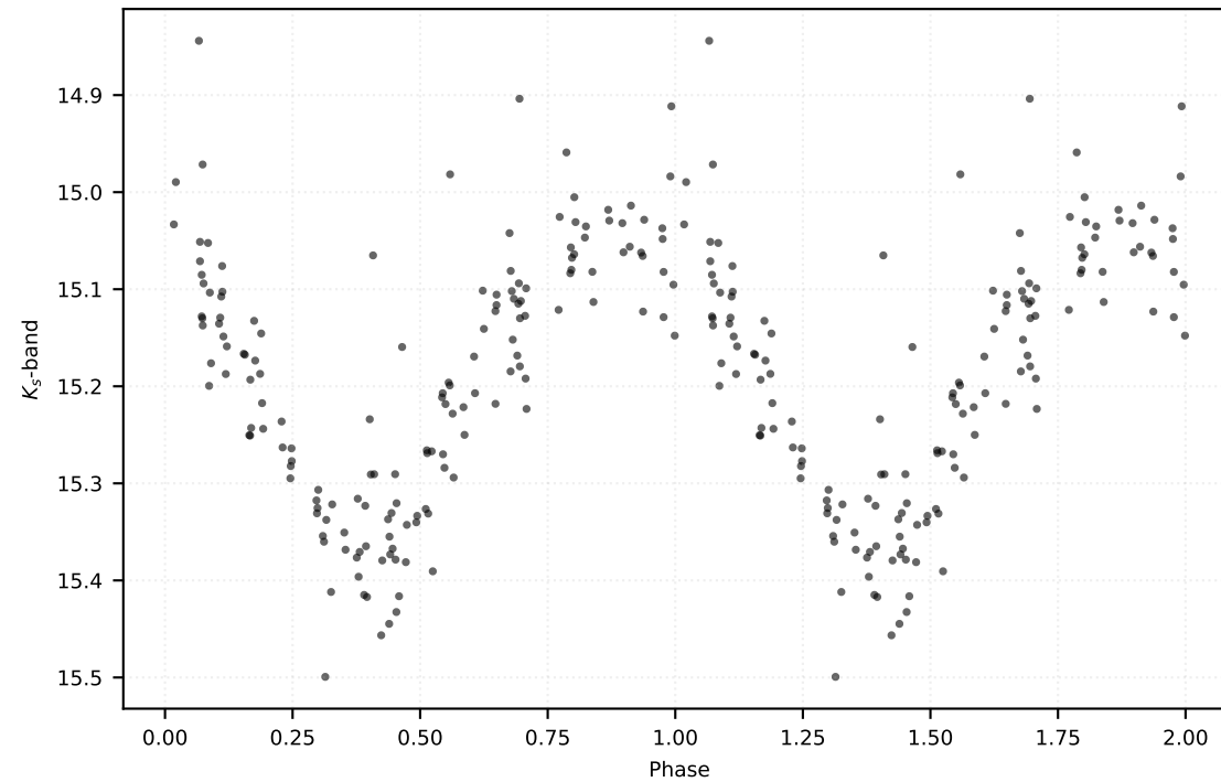
P: 1.07757 d | Class: EB | Subclass: UVAR | Field b278
