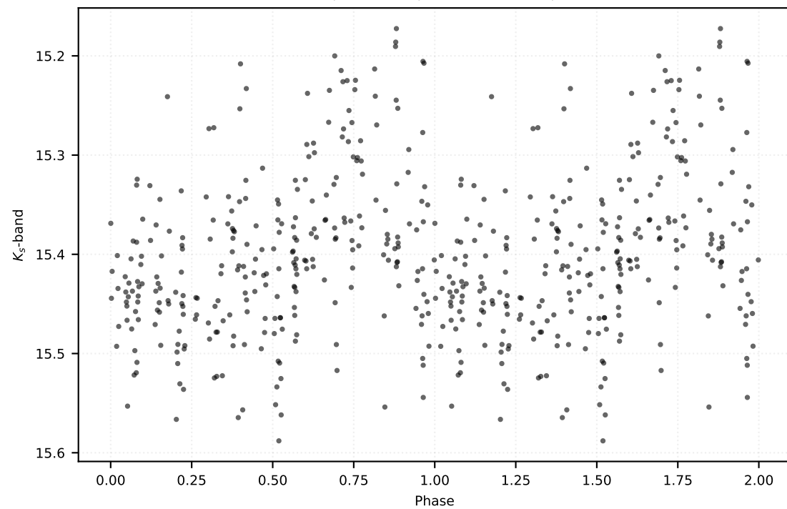
P: 0.22526 d | Class: RP | Subclass: UVAR | Field b278
