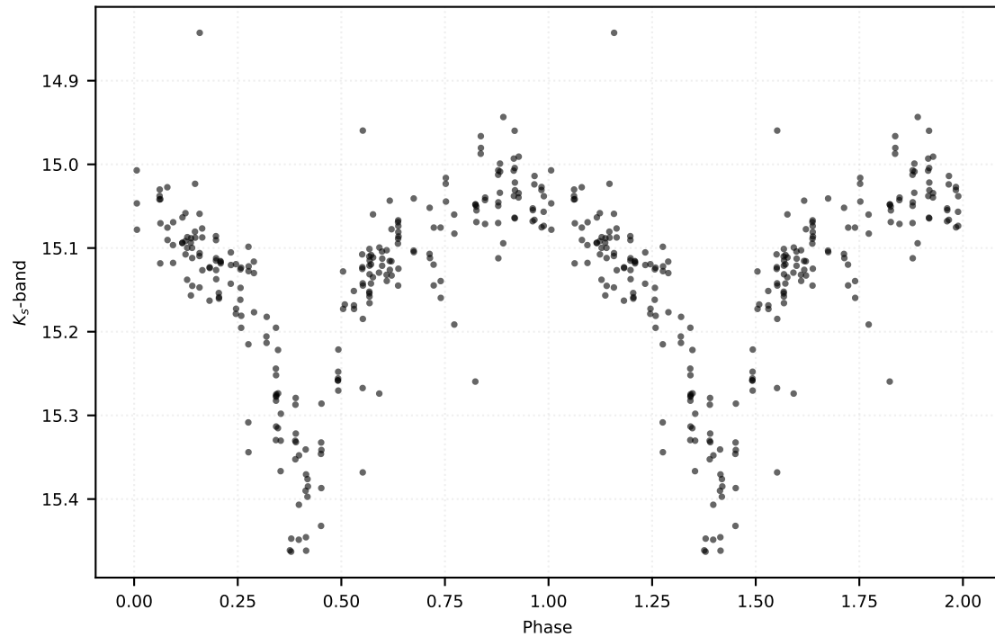
P: 3.98568 d | Class: RP | Subclass: CEP-F | Field b279
