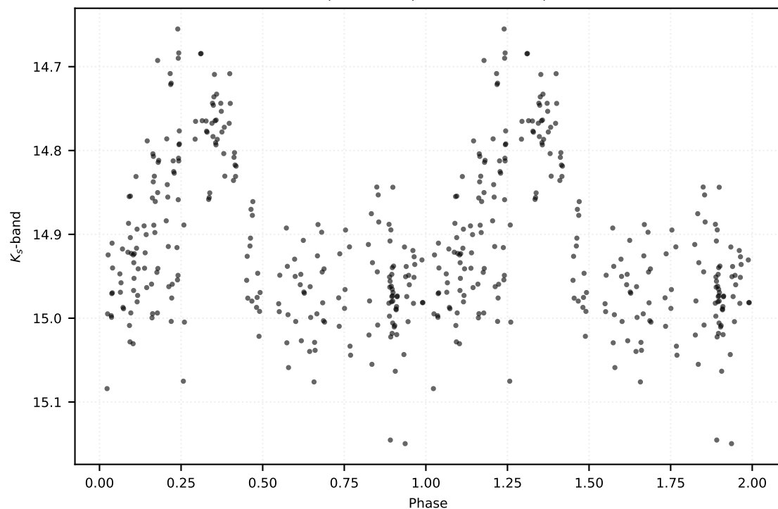
P: 31.51622 d | Class: RP | Subclass: UVAR | Field b278
