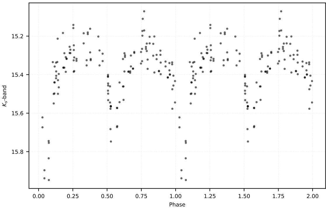
P: 0.49427 d | Class: EB | Subclass: EA | Field b279
