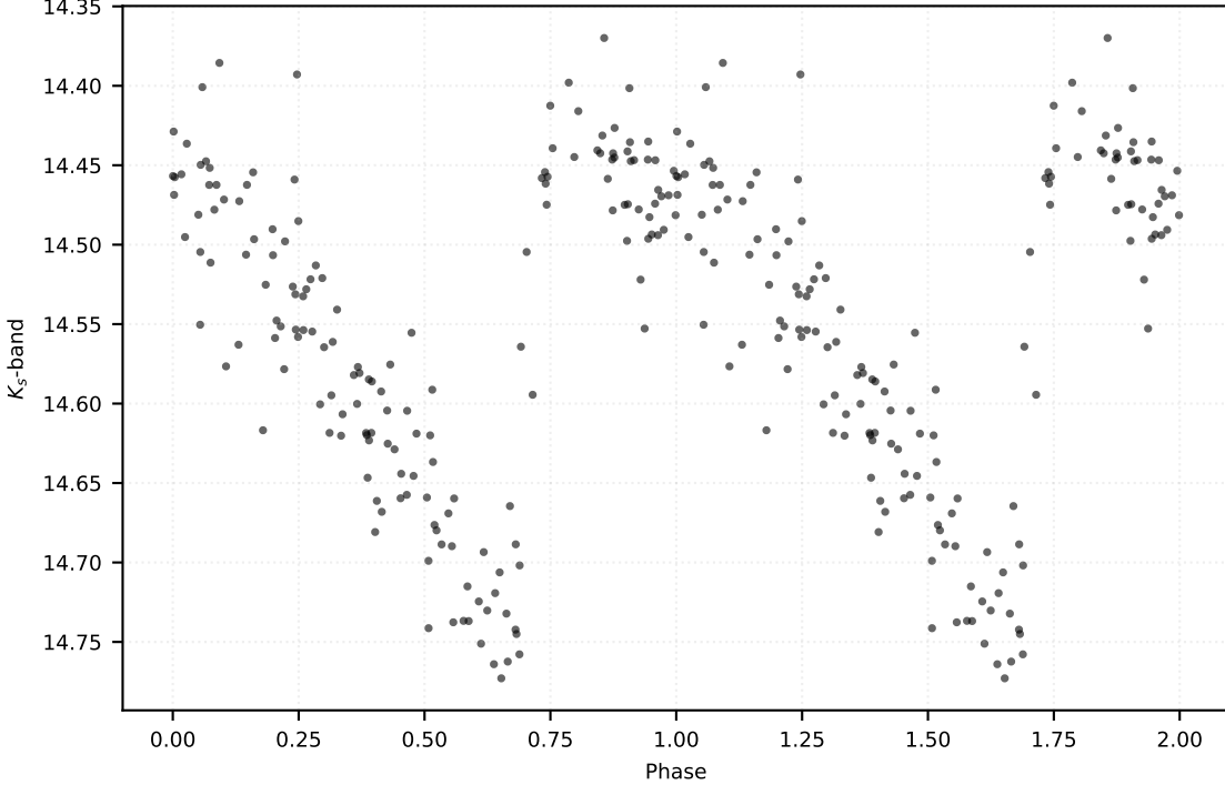
P: 0.47464 d | Class: RP | Subclass: RRab | Field b278
