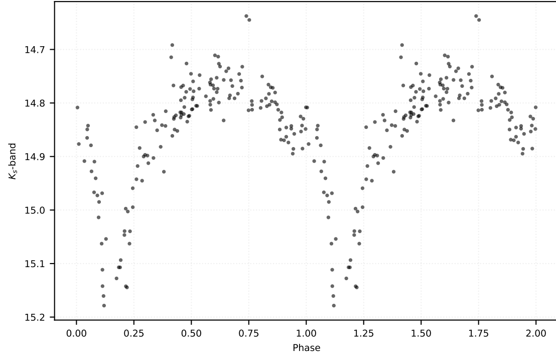
P: 2.66785 d | Class: RP | Subclass: CEP-F | Field b279
