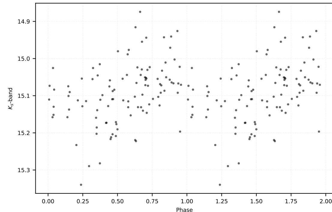
P: 0.26508 d | Class: RP | Subclass: UVAR | Field b278
