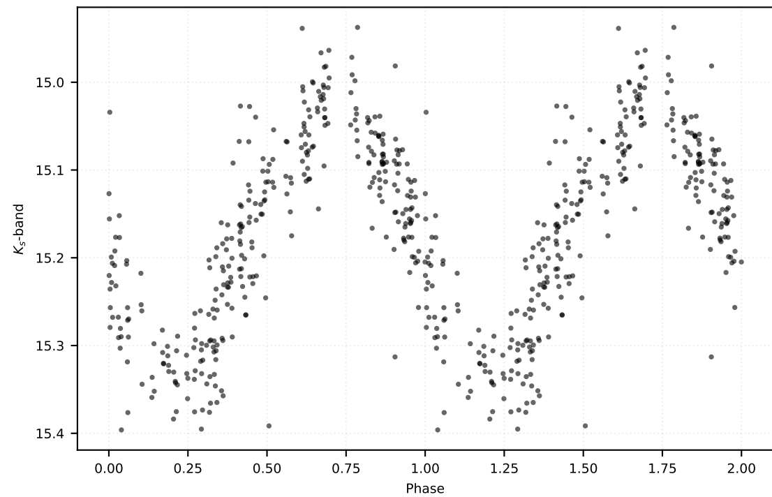
P: 0.41857 d | Class: RP | Subclass: RRc | Field b278
