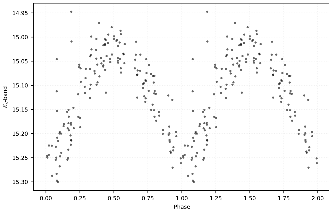
P: 0.57737 d | Class: RP | Subclass: RRc | Field b279
