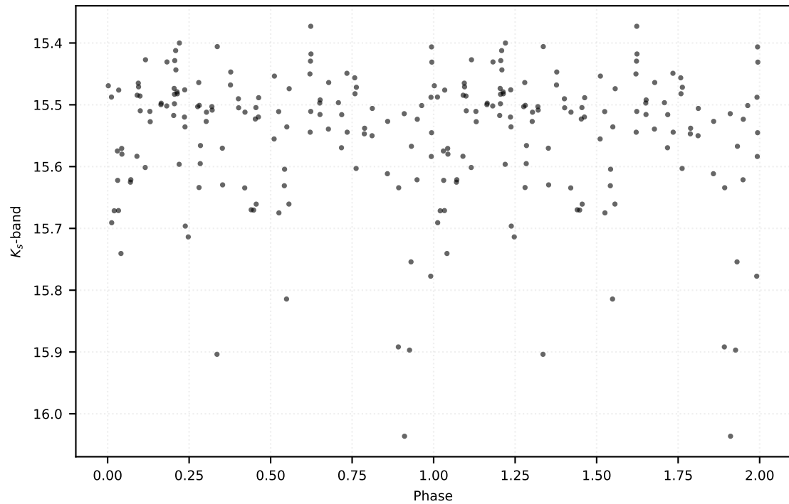
P: 0.21803 d | Class: EB | Subclass: EA | Field b278
