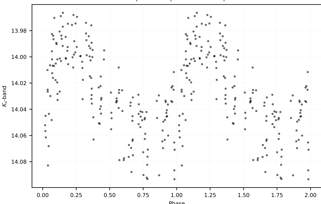
P: 0.36147 d | Class: RP | Subclass: RRab | Field b279
