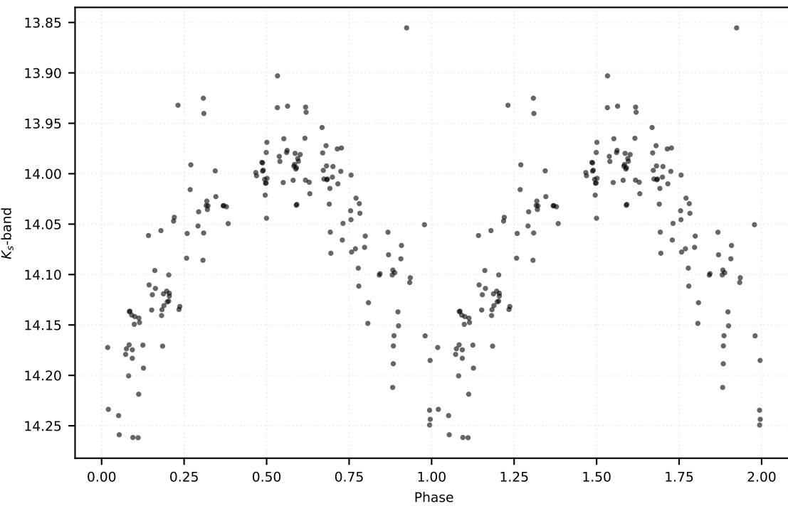
P: 0.20504 d | Class: RP | Subclass: UVAR | Field b279
