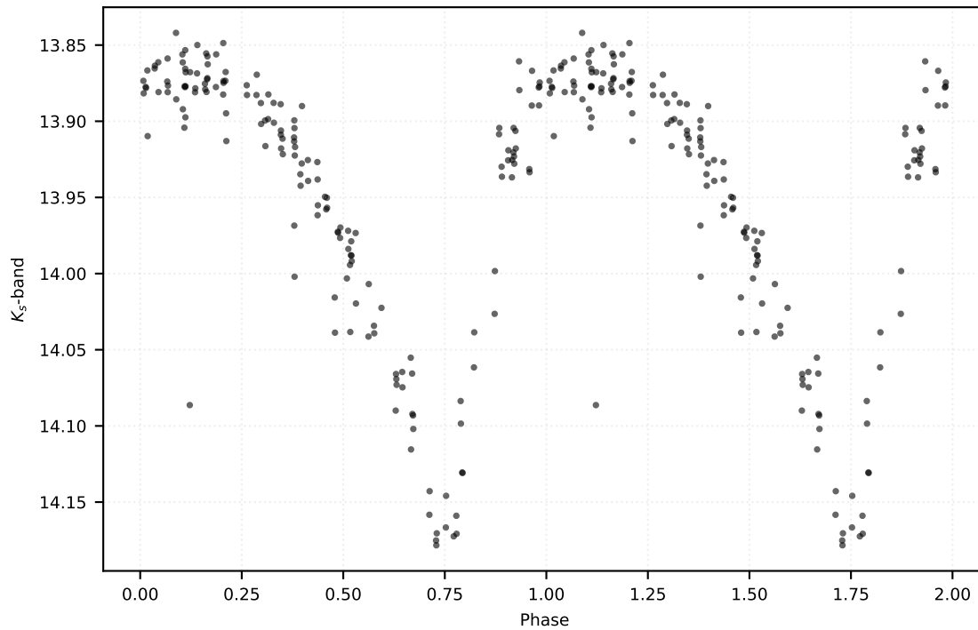
P: 0.55566 d | Class: RP | Subclass: RRab | Field b278
