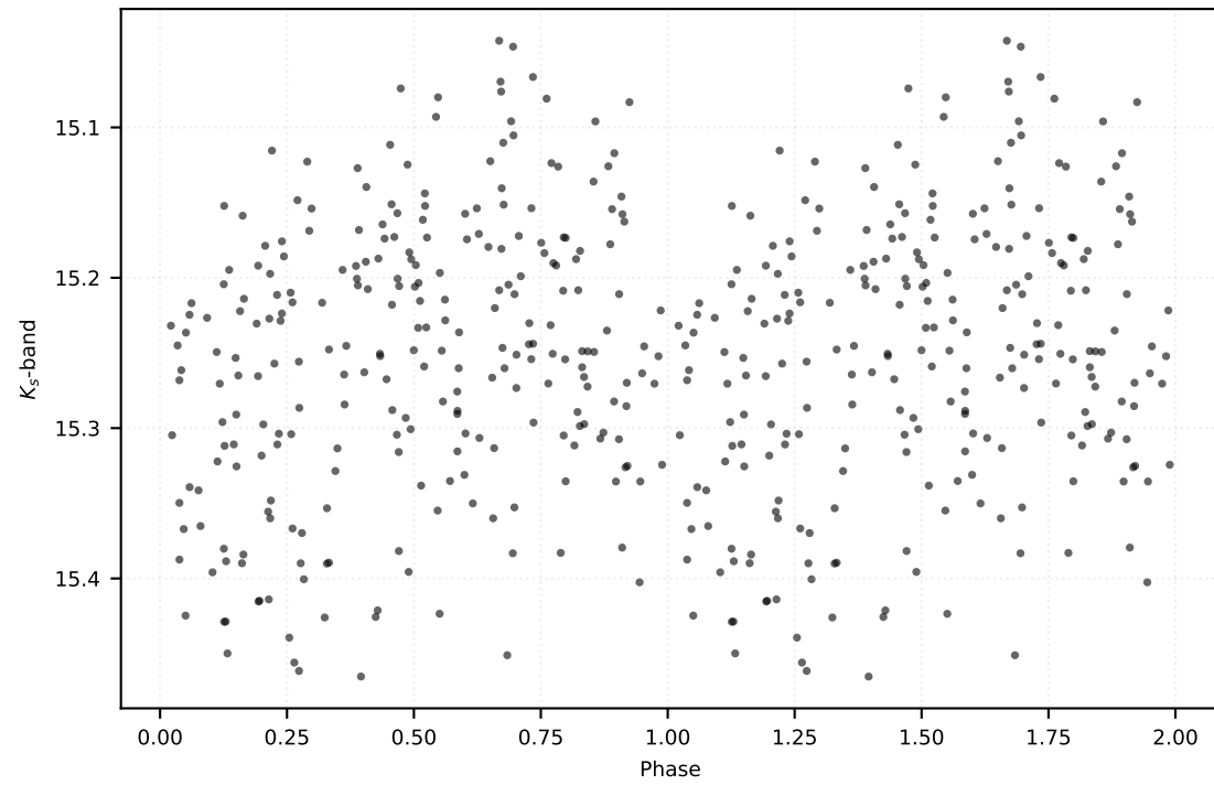
P: 0.10533 d | Class: RP | Subclass: UVAR | Field b278
