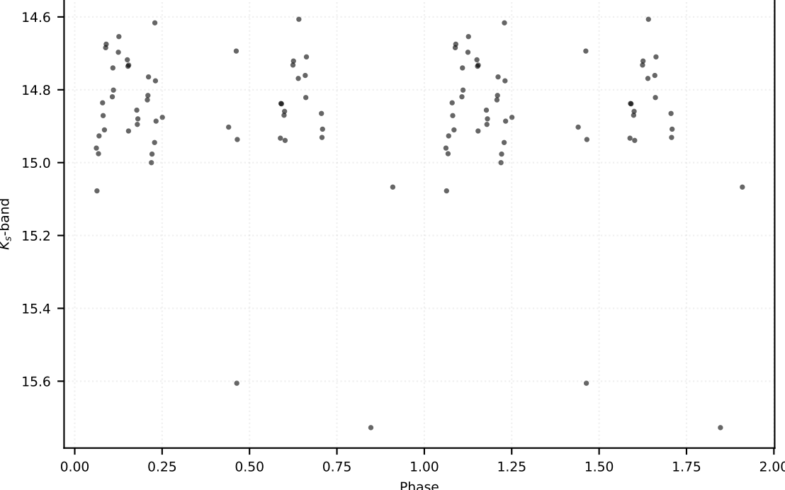
P: 0.24692 d | Class: EB | Subclass: EA | Field b278
