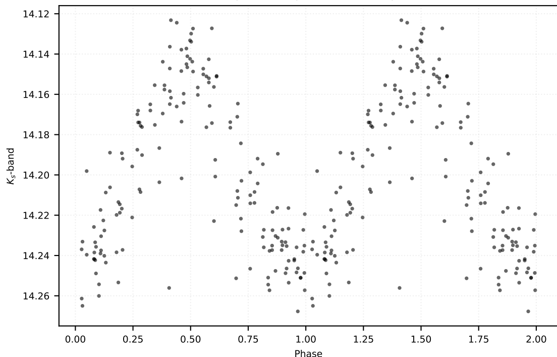
P: 1.43235 d | Class: RP | Subclass: CEP-F | Field b278
