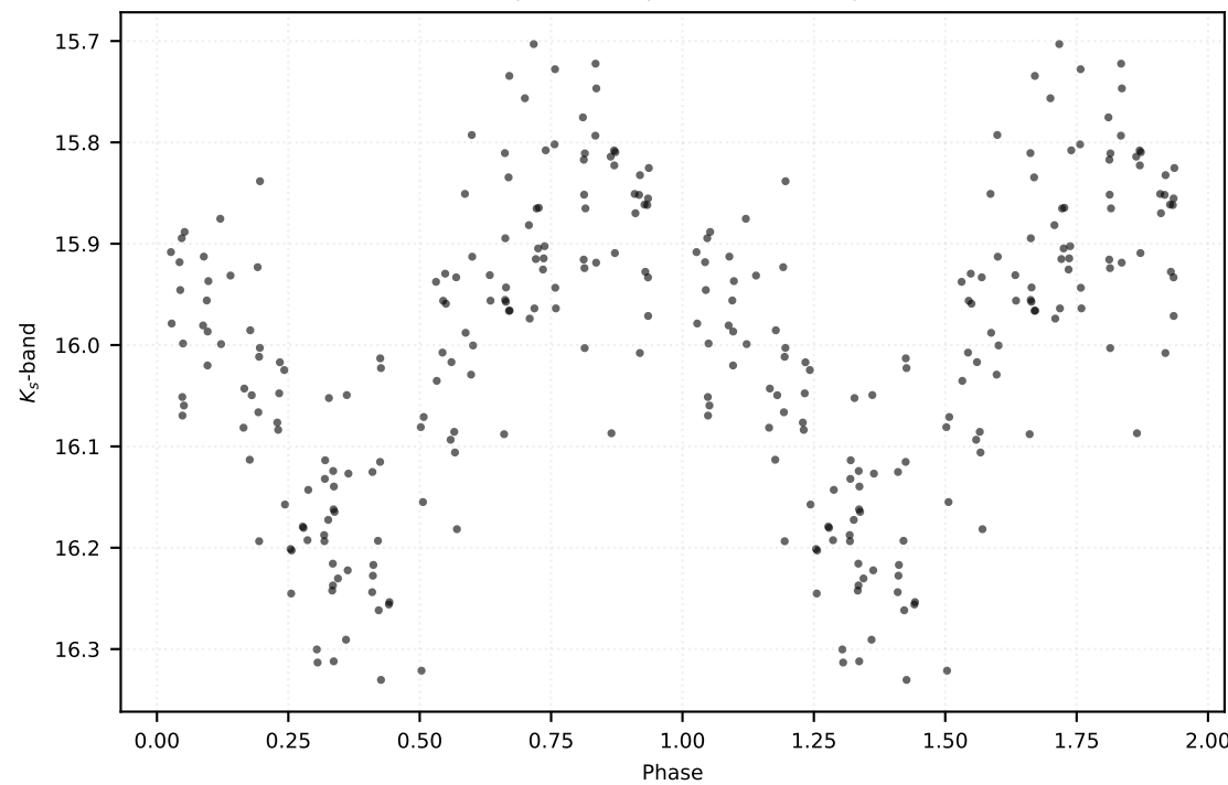
P: 0.15582 d | Class: RP | Subclass: UVAR | Field b279
