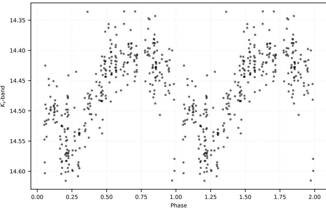
P: 0.56155 d | Class: RP | Subclass: RRab | Field b279
