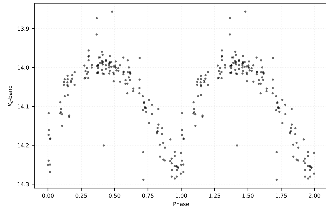
P: 0.60323 d | Class: RP | Subclass: RRab | Field b279
