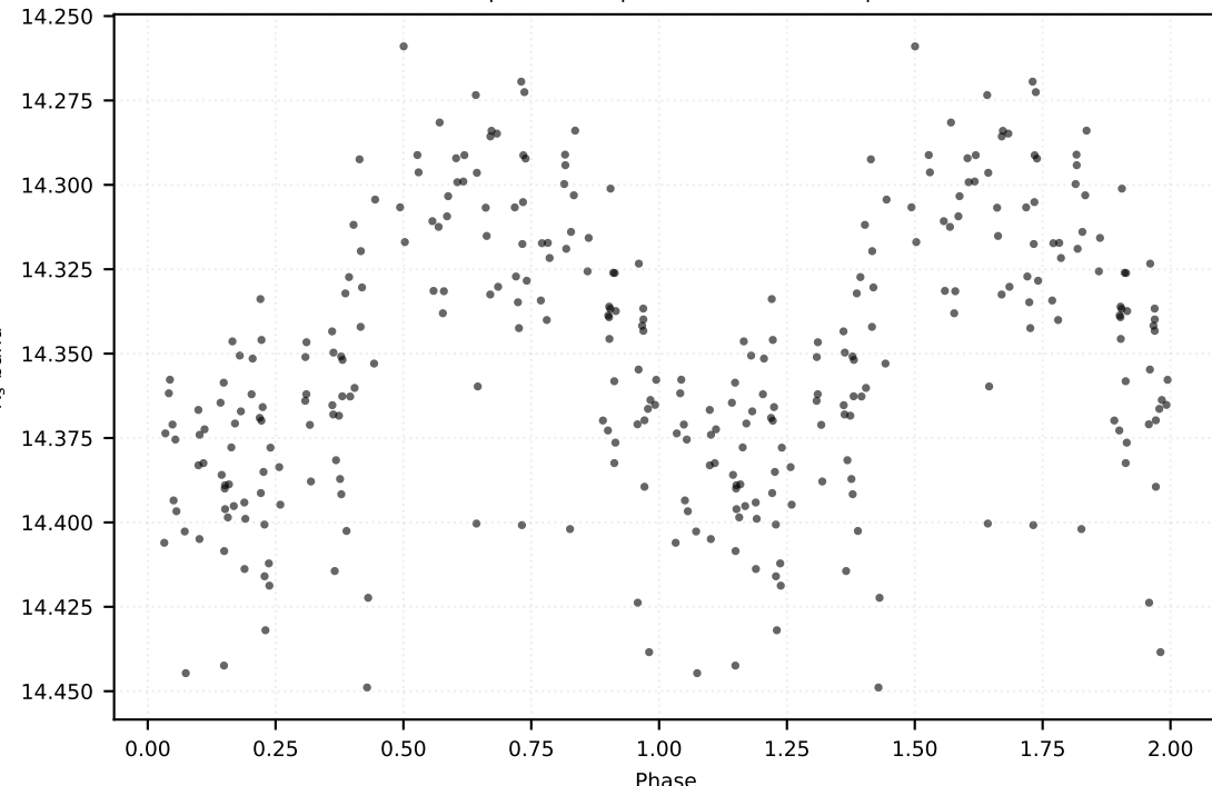
P: 0.24932 d | Class: RP | Subclass: CEP-10T | Field b278
