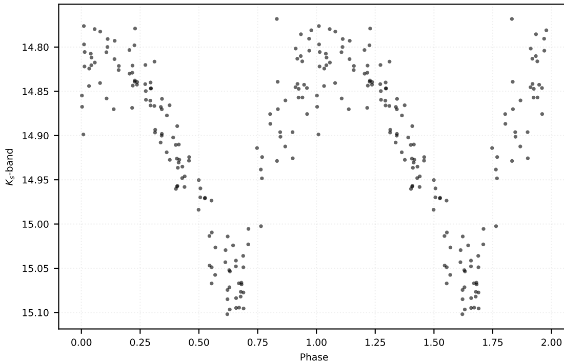
P: 0.48933 d | Class: RP | Subclass: RRab | Field b279
