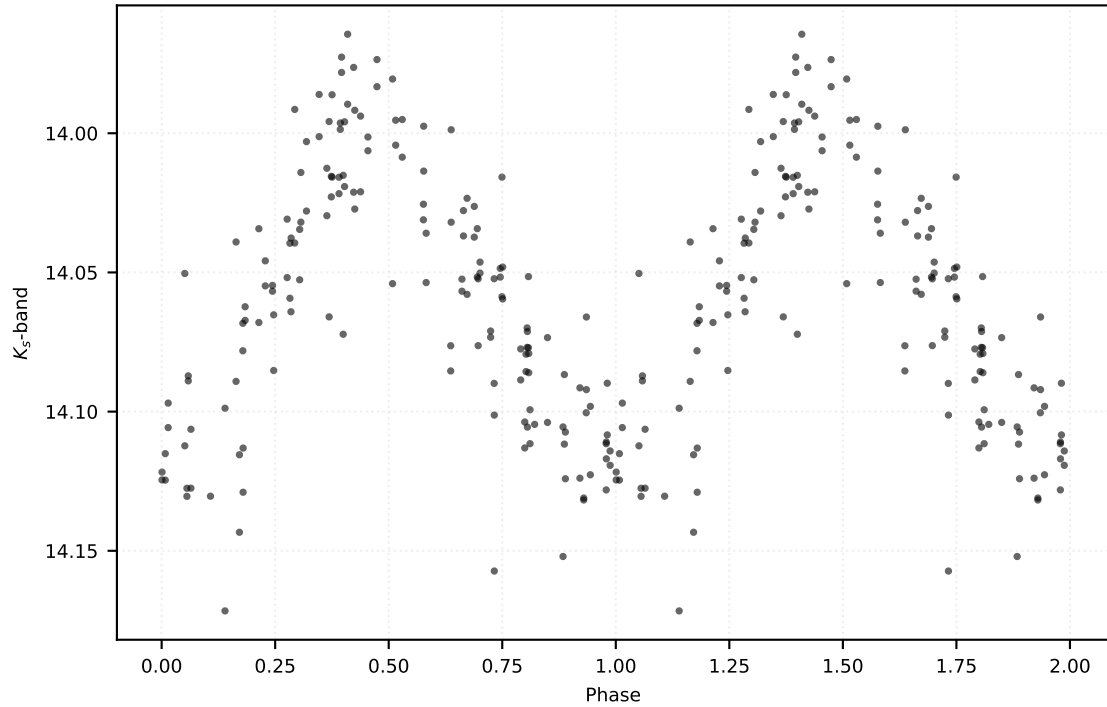
P: 30.17269 d | Class: RP | Subclass: CEP-F | Field b279
