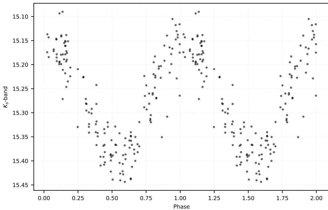
P: 0.59569 d | Class: RP | Subclass: RRab | Field b279
