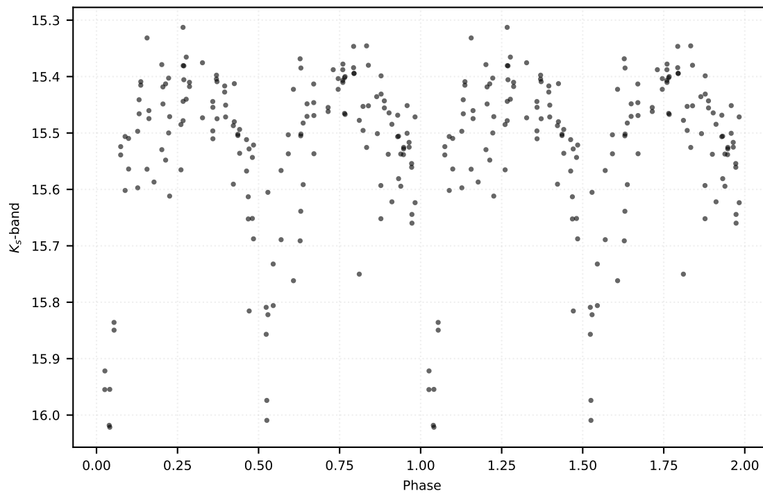
P: 2.35011 d | Class: EB | Subclass: EA | Field b279
