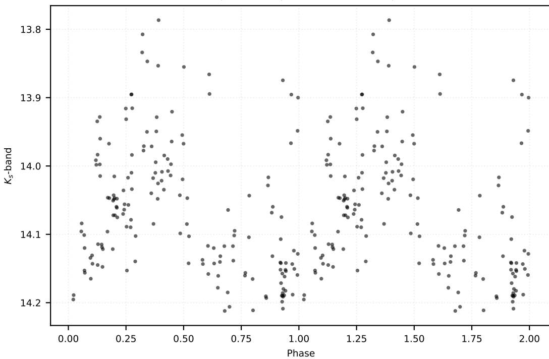
P: 0.25847 d | Class: RP | Subclass: CEP-10T | Field b278
