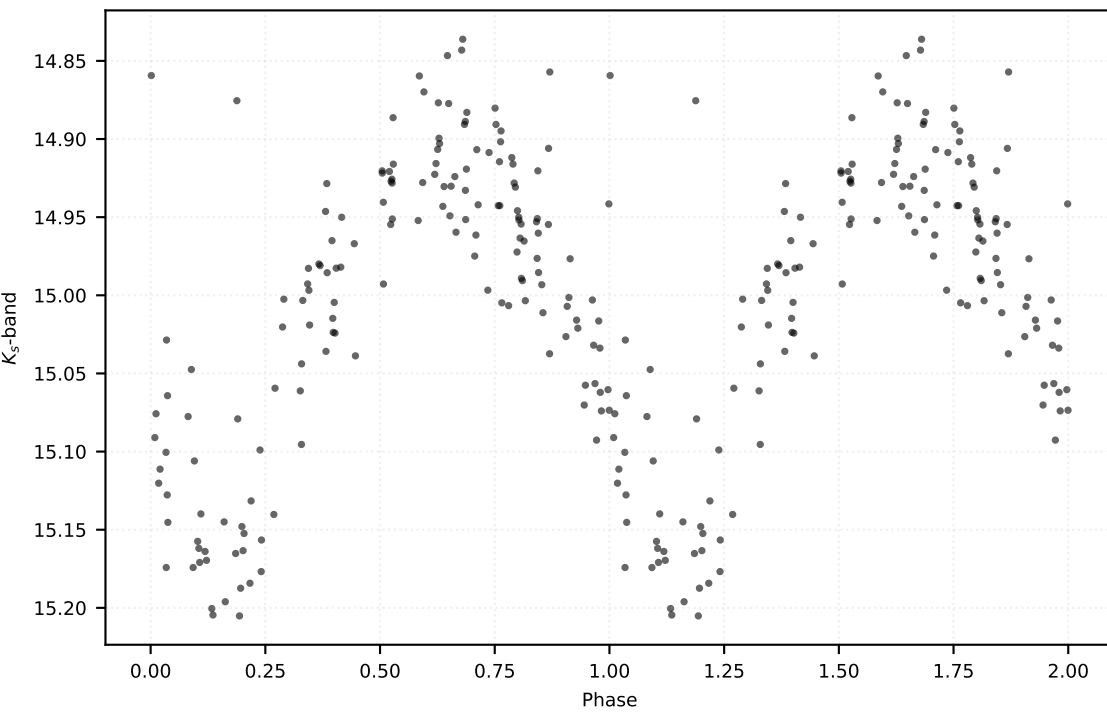
P: 0.34031 d | Class: EB | Subclass: UVAR | Field b279
