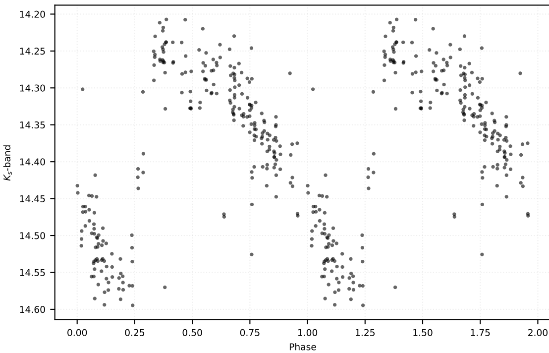
P: 0.54772 d | Class: RP | Subclass: RRab | Field b279
