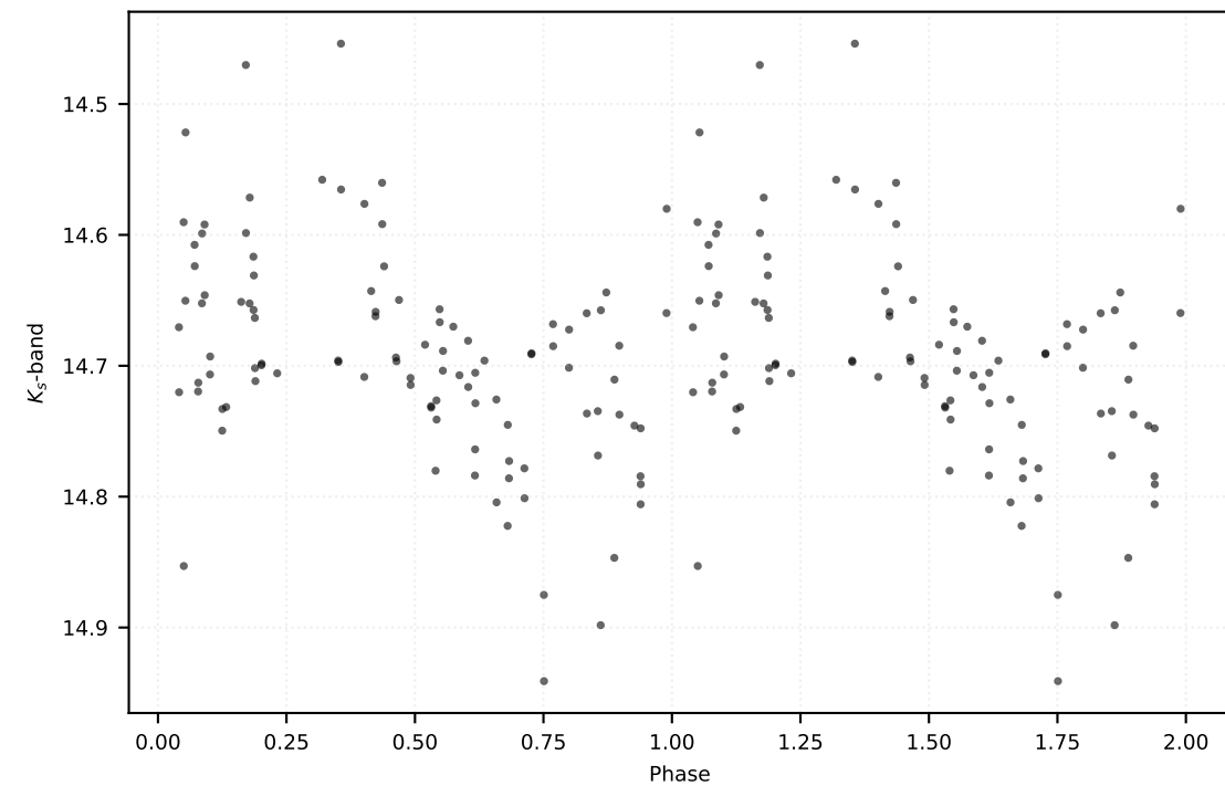
P: 11.36033 d | Class: RP | Subclass: CEP-F | Field b278
