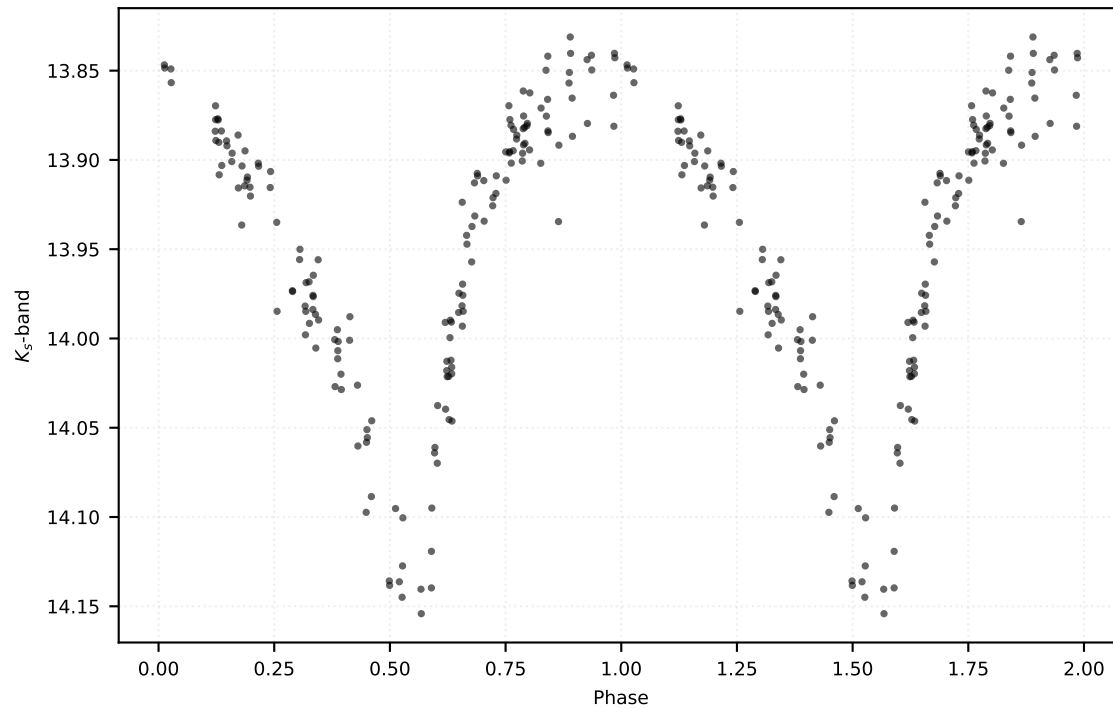
P: 0.52500 d | Class: RP | Subclass: RRab | Field b278
