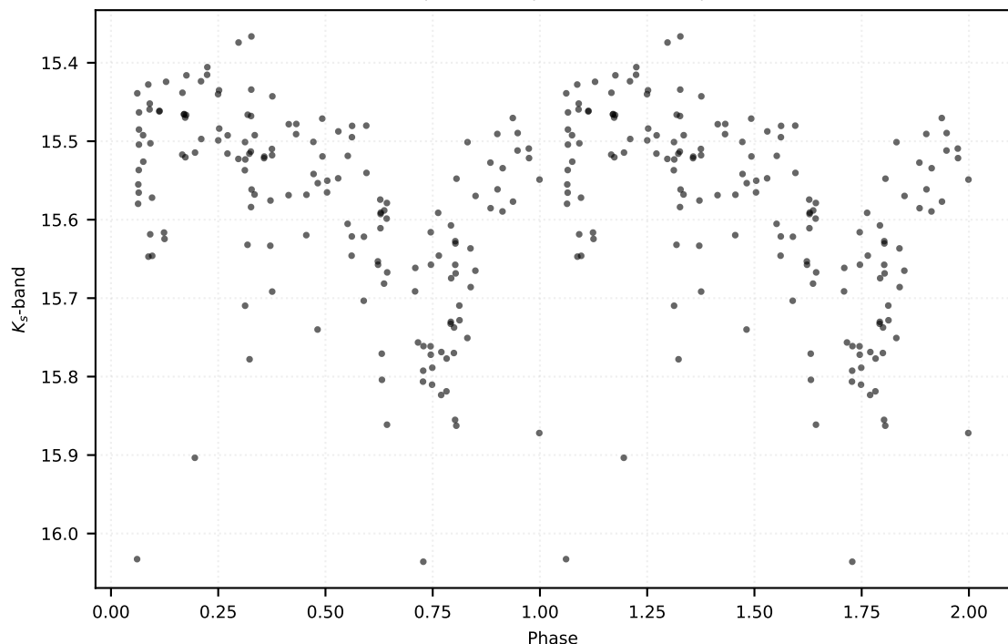
P: 0.43446 d | Class: RP | Subclass: RRab | Field b279
