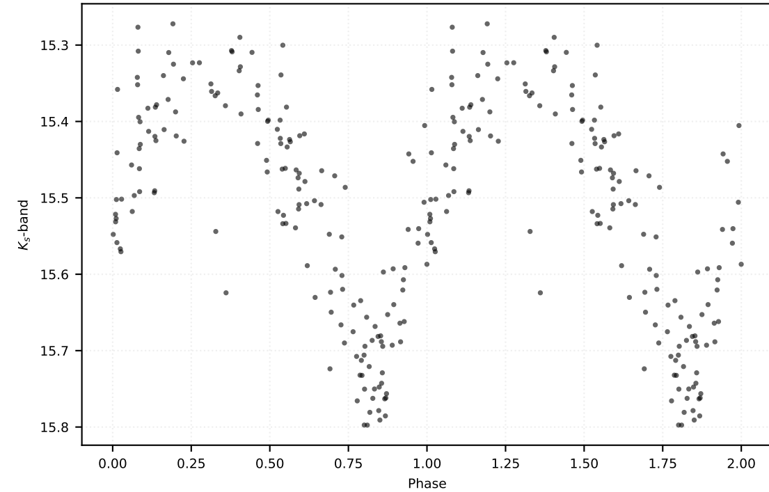
P: 0.21475 d | Class: RP | Subclass: UVAR | Field b278
