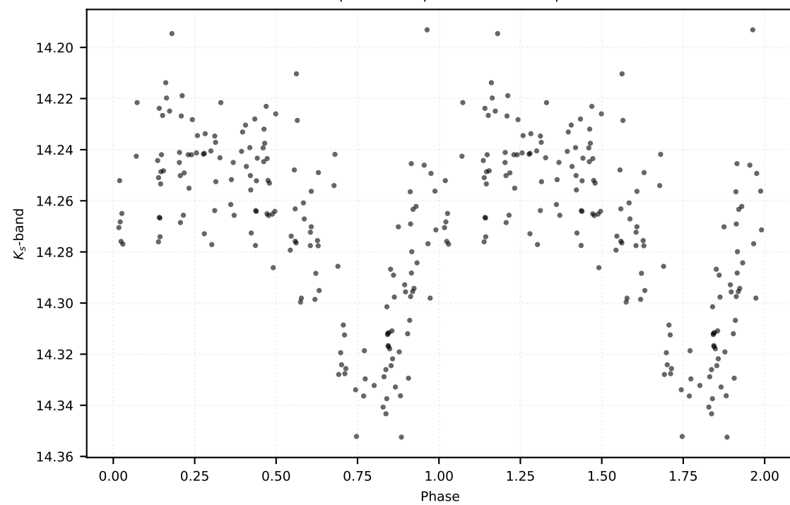
P: 0.16304 d | Class: RP | Subclass: UVAR | Field b279
