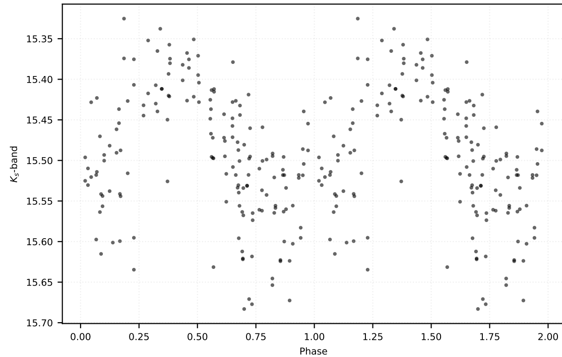
P: 0.19259 d | Class: RP | Subclass: UVAR | Field b279
