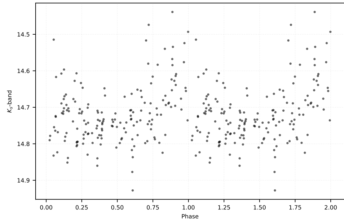
P: 0.19870 d | Class: RP | Subclass: UVAR | Field b278
