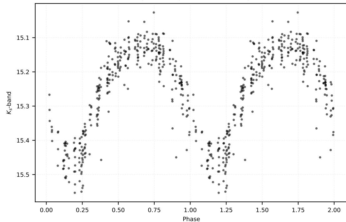
P: 0.46773 d | Class: RP | Subclass: CEP-10T | Field b278
