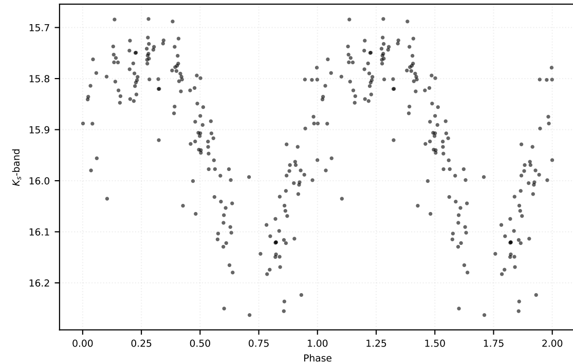
P: 0.17219 d | Class: RP | Subclass: UVAR | Field b278
