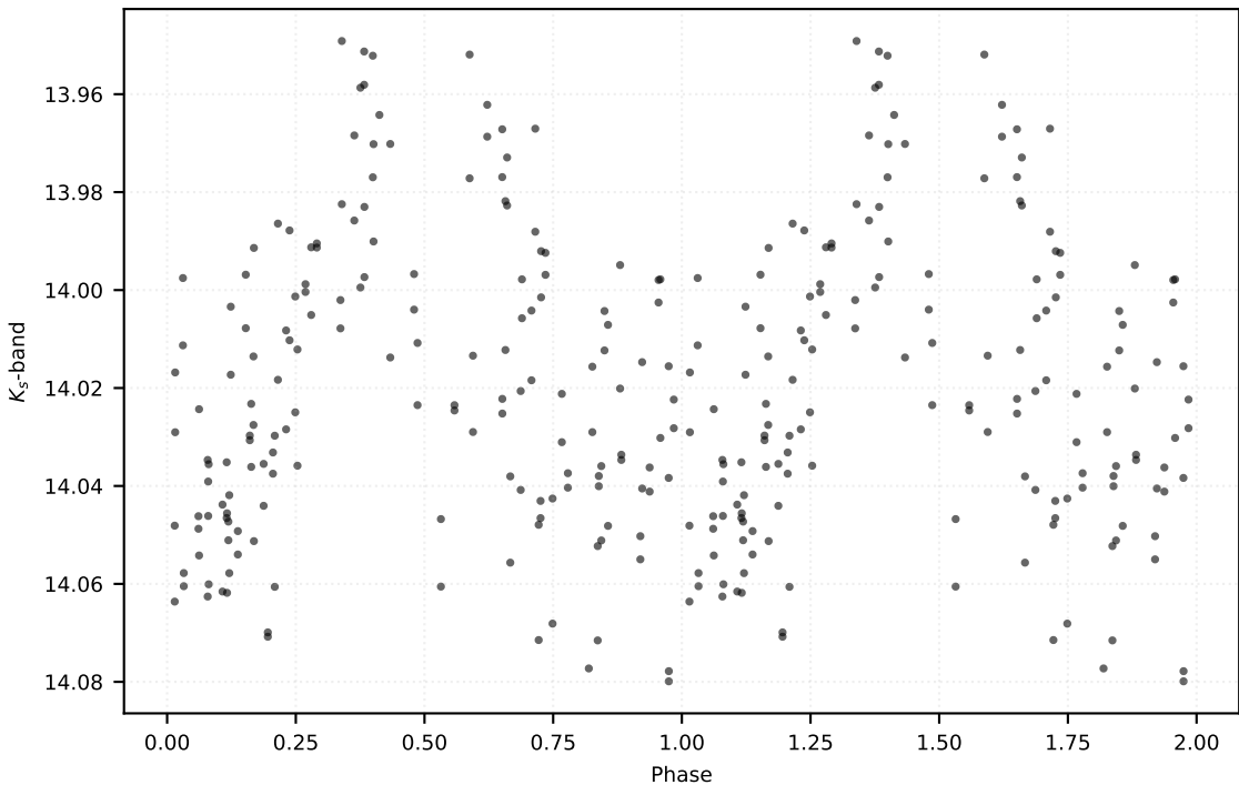
P: 54.19650 d | Class: RP | Subclass: UVAR | Field b279
