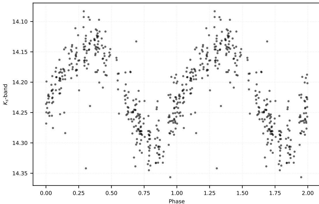
P: 0.22202 d | Class: RP | Subclass: UVAR | Field b278
