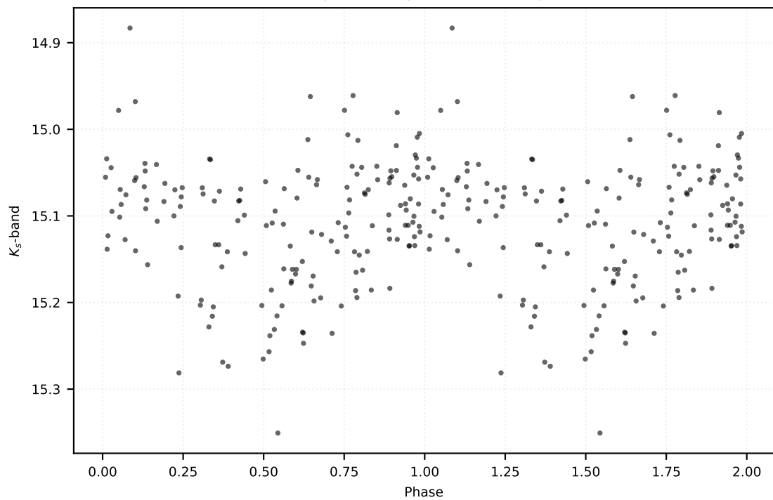
P: 0.19945 d | Class: RP | Subclass: UVAR | Field b279
