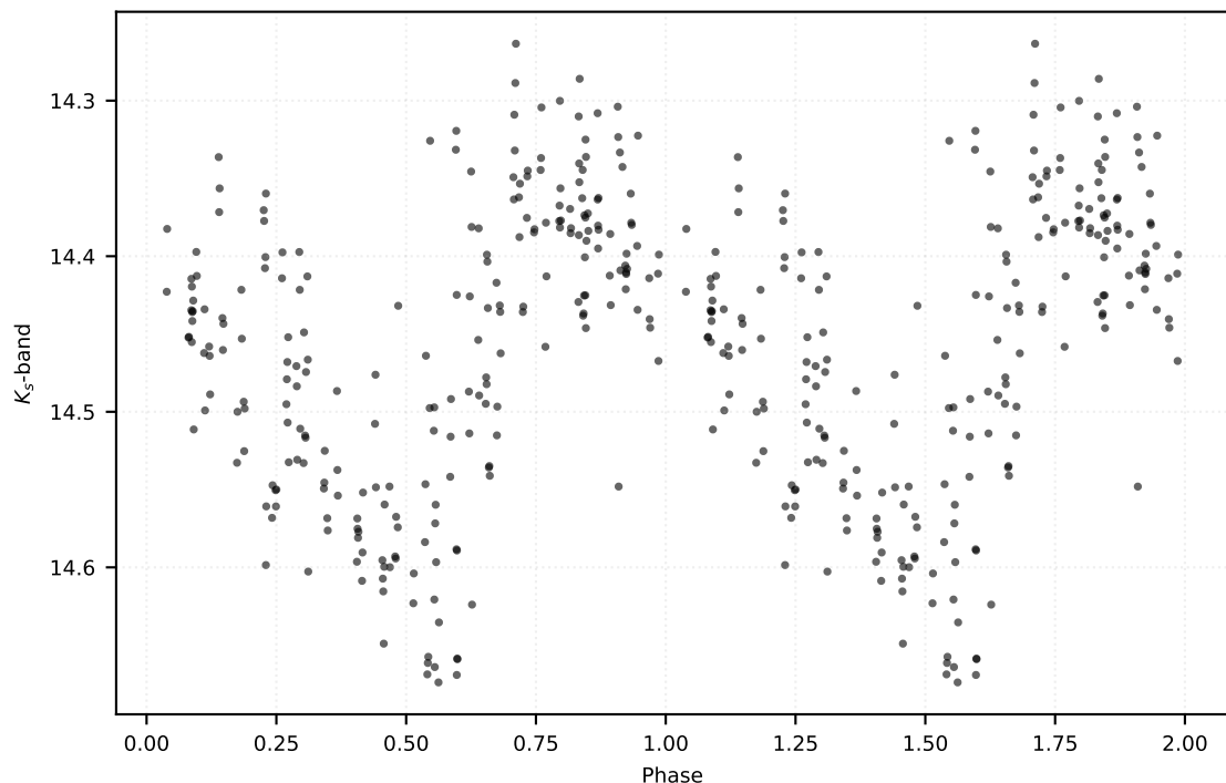
P: 0.36047 d | Class: RP | Subclass: RRab | Field b278
