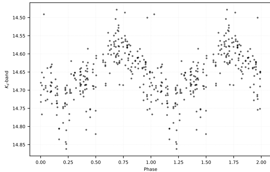
P: 4.54119 d | Class: RP | Subclass: CEP-10T | Field b279
