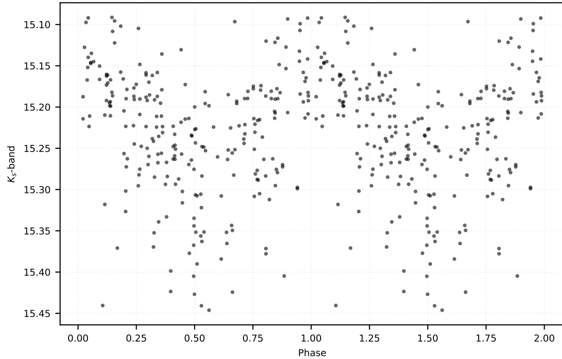
P: 1.29271 d | Class: RP | Subclass: CEP-F | Field b279
