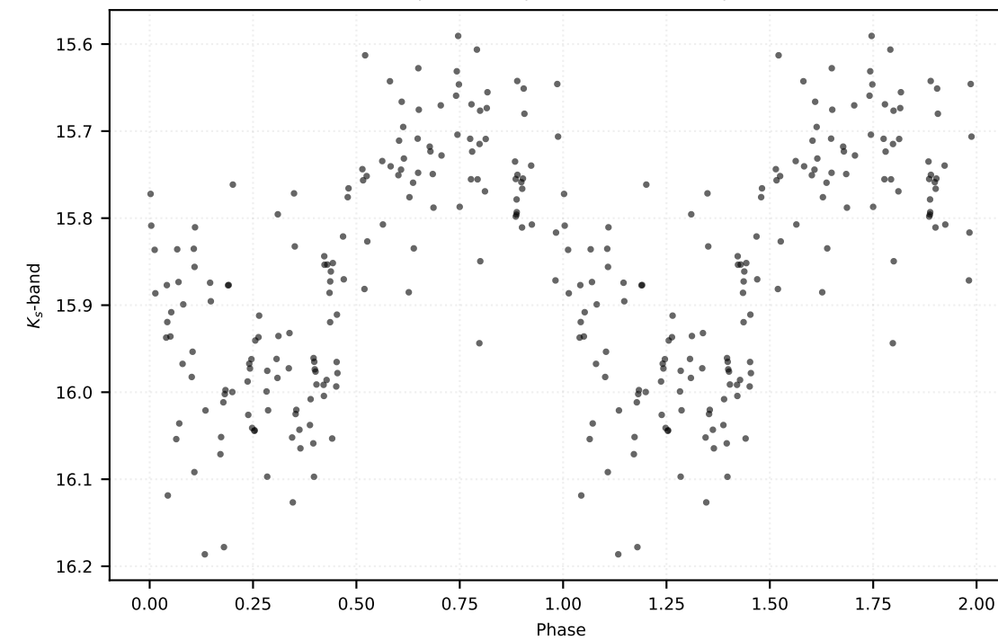
P: 0.41661 d | Class: RP | Subclass: CEP-10T | Field b279
