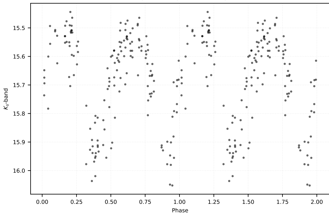
P: 7.98636 d | Class: EB | Subclass: EW | Field b279
