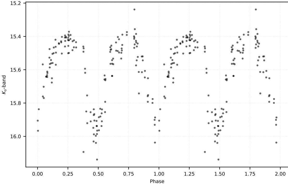
P: 0.19008 d | Class: RP | Subclass: UVAR | Field b279
