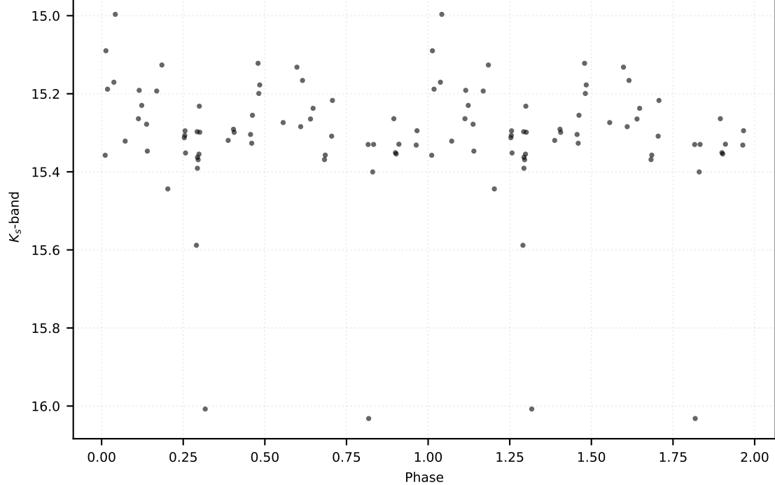
P: 0.34898 d | Class: EB | Subclass: EA | Field b278
