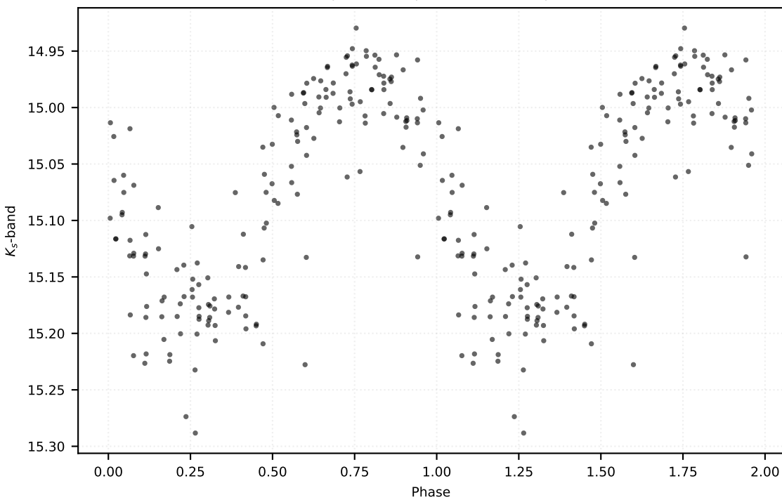
P: 0.77103 d | Class: RP | Subclass: RRab | Field b278
