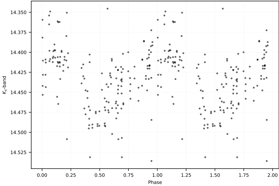
P: 66.62716 d | Class: RP | Subclass: CEP-F | Field b279
