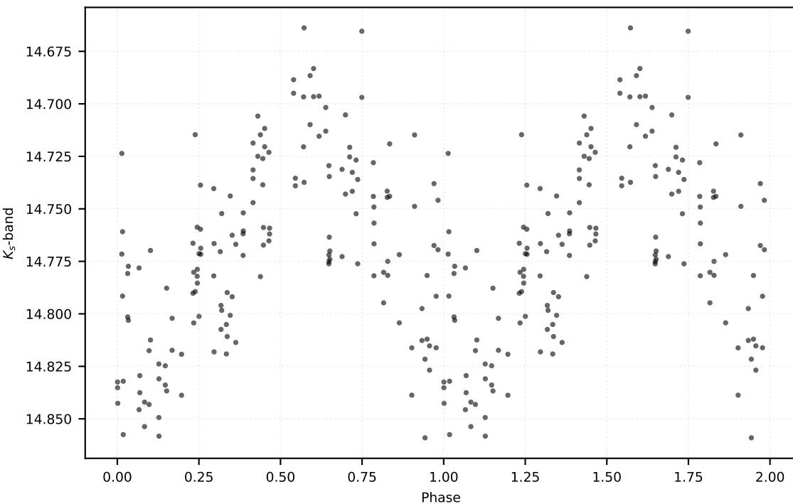
P: 3.27517 d | Class: EB | Subclass: UVAR | Field b279
