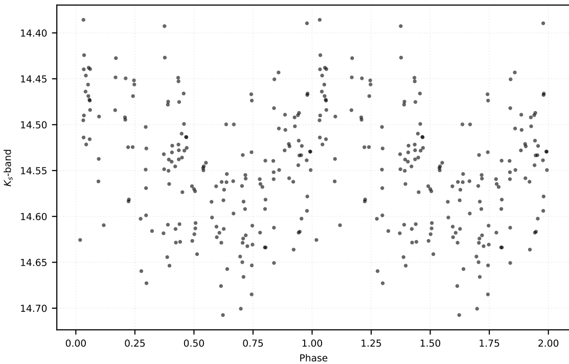
P: 0.15083 d | Class: RP | Subclass: UVAR | Field b279
