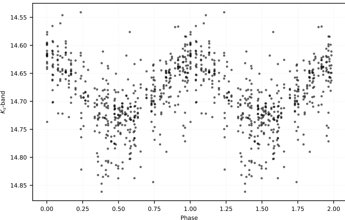
P: 0.41875 d | Class: RP | Subclass: CEP-10T | Field b279
