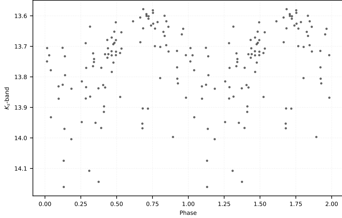
P: 0.44264 d | Class: RP | Subclass: RRab | Field b279
