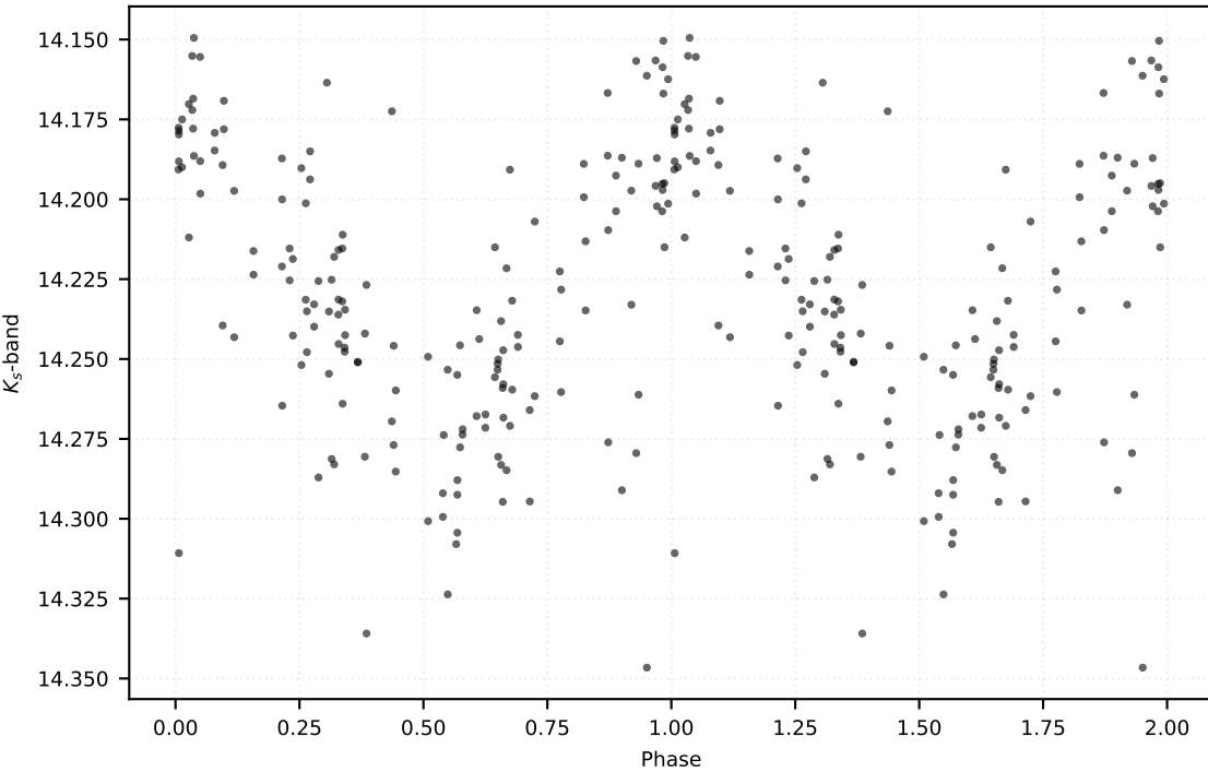
P: 1.07358 d | Class: RP | Subclass: CEP-F | Field b279
