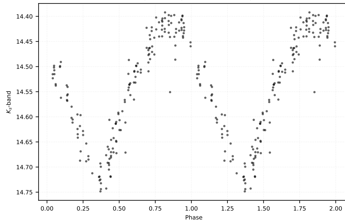
P: 0.73902 d | Class: RP | Subclass: CEP-1OT | Field b279
