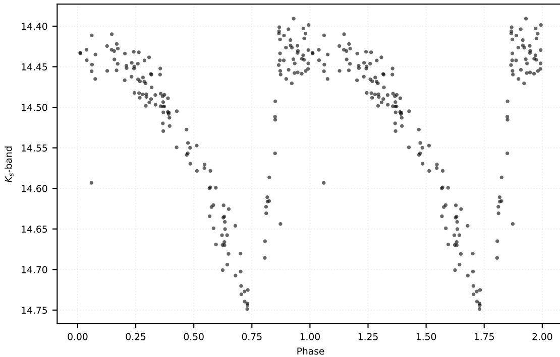
P: 0.50709 d | Class: RP | Subclass: RRab | Field b278
