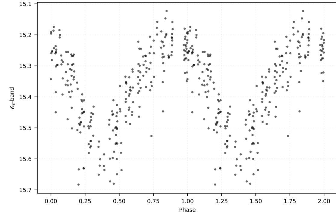
P: 0.20890 d | Class: RP | Subclass: UVAR | Field b278
