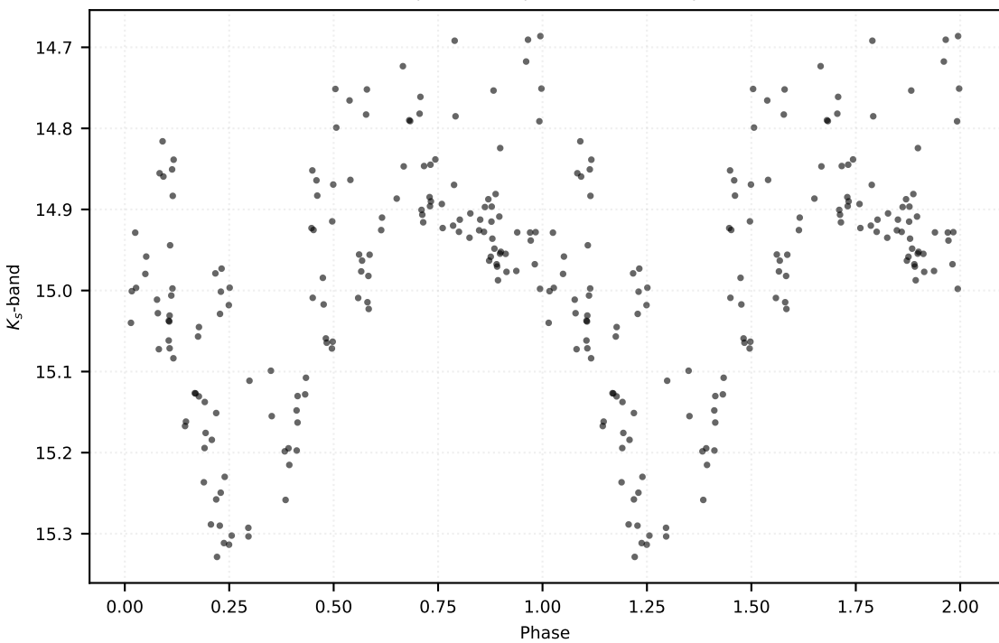
P: 0.19108 d | Class: RP | Subclass: UVAR | Field b278
