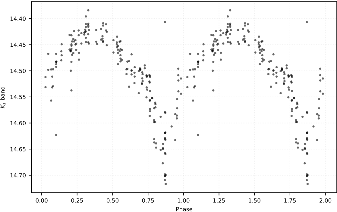
P: 0.56520 d | Class: RP | Subclass: CEP-10T | Field b278
