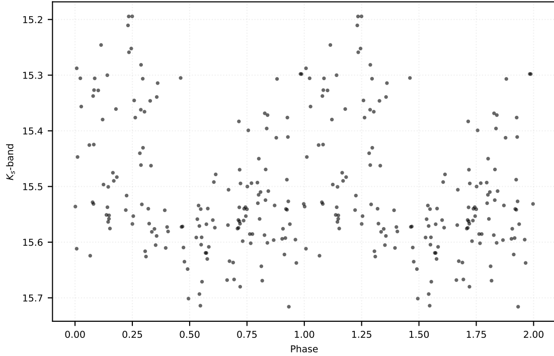
P: 0.11186 d | Class: RP | Subclass: UVAR | Field b278
