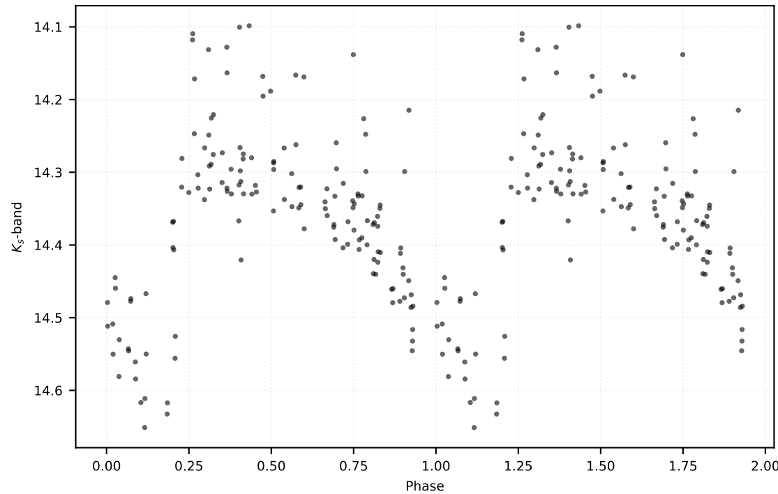
P: 0.56508 d | Class: RP | Subclass: RRab | Field b279
