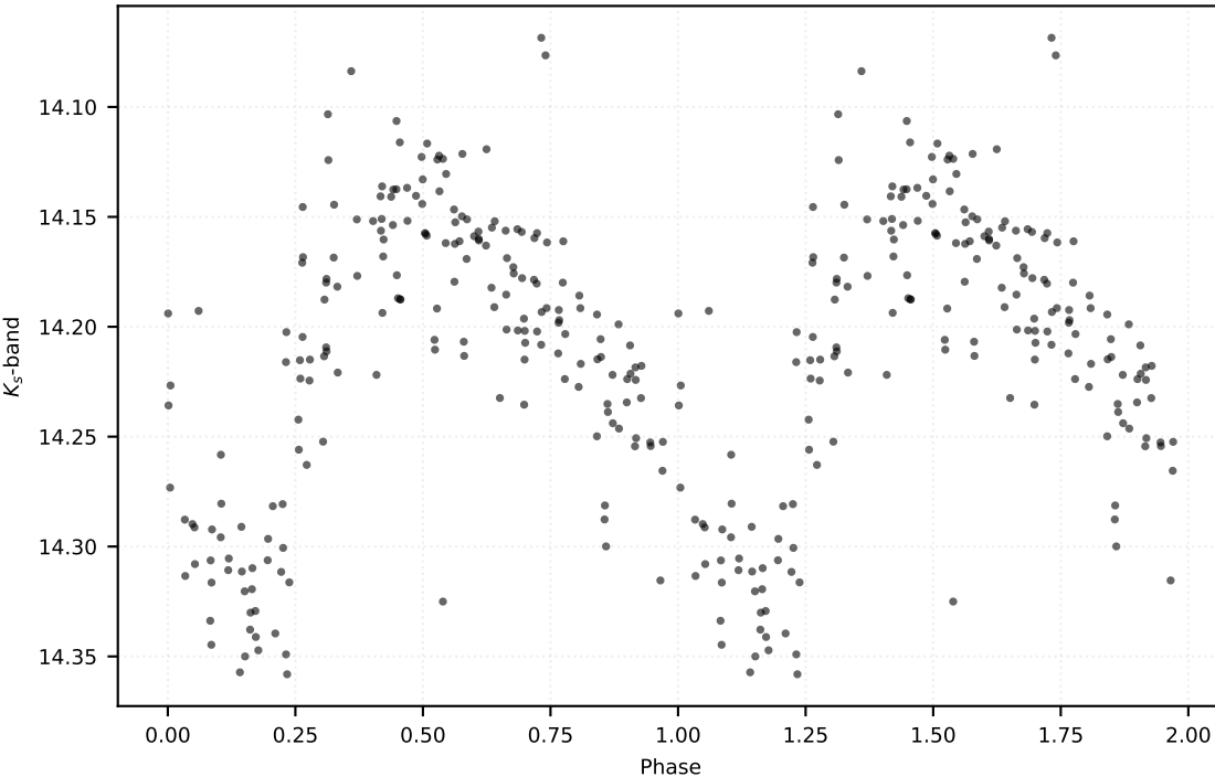
P: 0.50228 d | Class: RP | Subclass: RRab | Field b279
