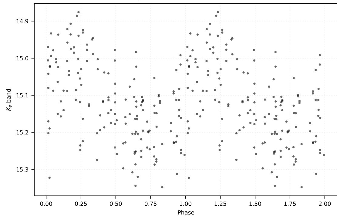
P: 2.18381 d | Class: RP | Subclass: CEP-10T | Field b278
