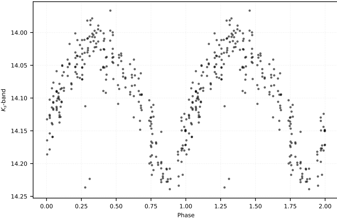
P: 0.47956 d | Class: RP | Subclass: CEP-10T | Field b278
