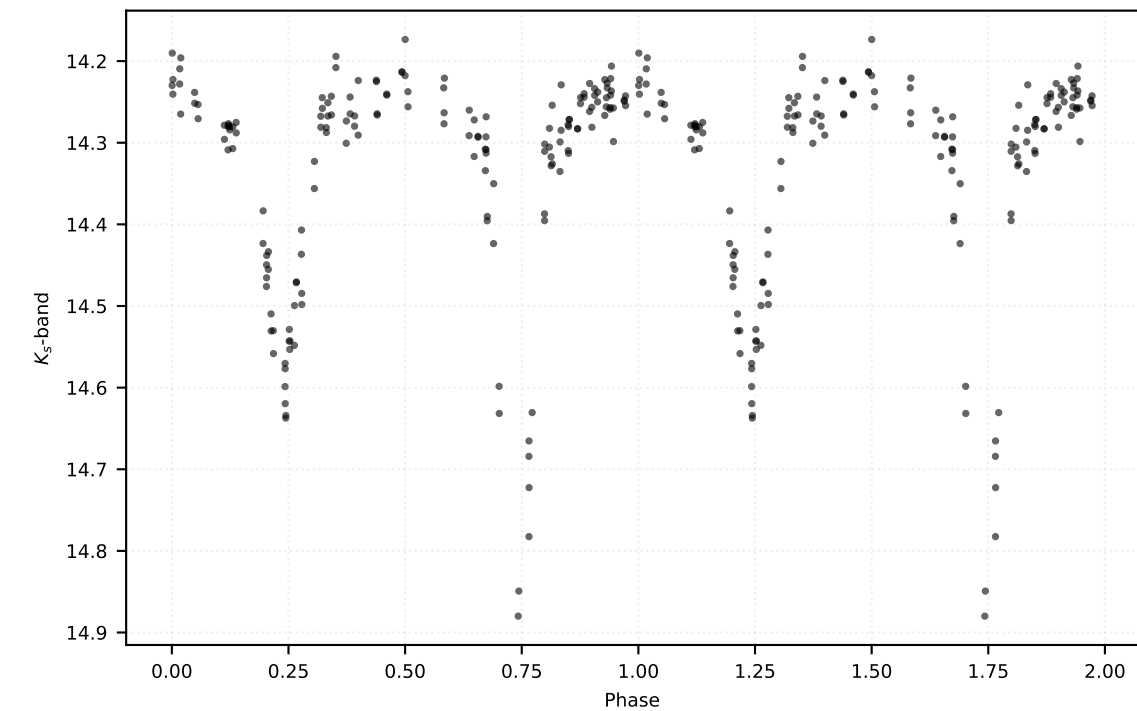
P: 1.79122 d | Class: EB | Subclass: EA | Field b278
