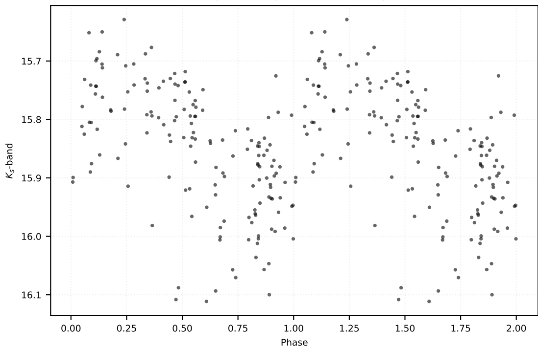
P: 4.25981 d | Class: RP | Subclass: CEP-10T | Field b279
