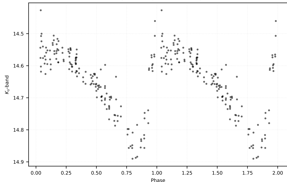
P: 0.40000 d | Class: RP | Subclass: RRab | Field b279
