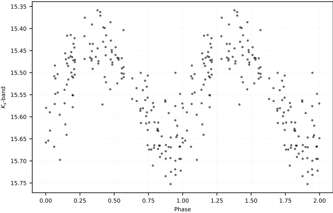
P: 0.35301 d | Class: RP | Subclass: RRab | Field b278
