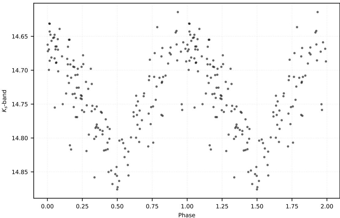
P: 0.15372 d | Class: RP | Subclass: UVAR | Field b278
