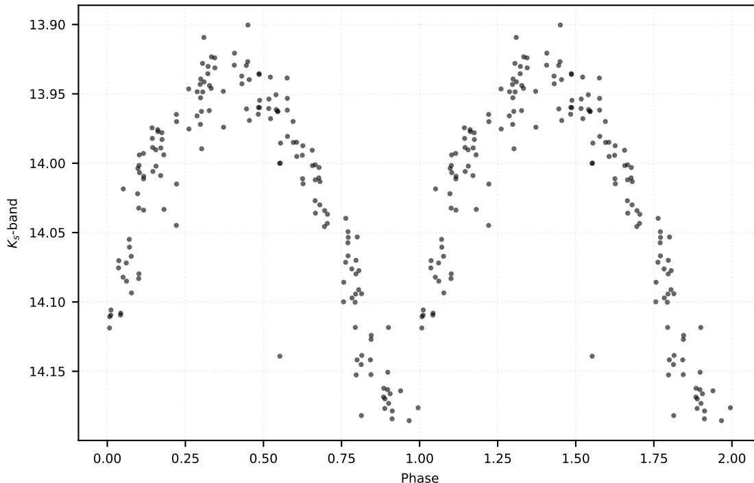
P: 0.31554 d | Class: RP | Subclass: RRab | Field b279
