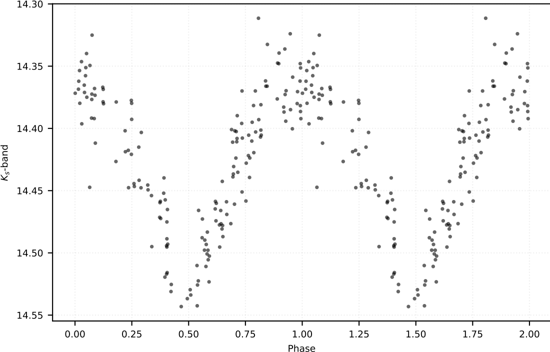
P: 0.66370 d | Class: RP | Subclass: RRab | Field b279
