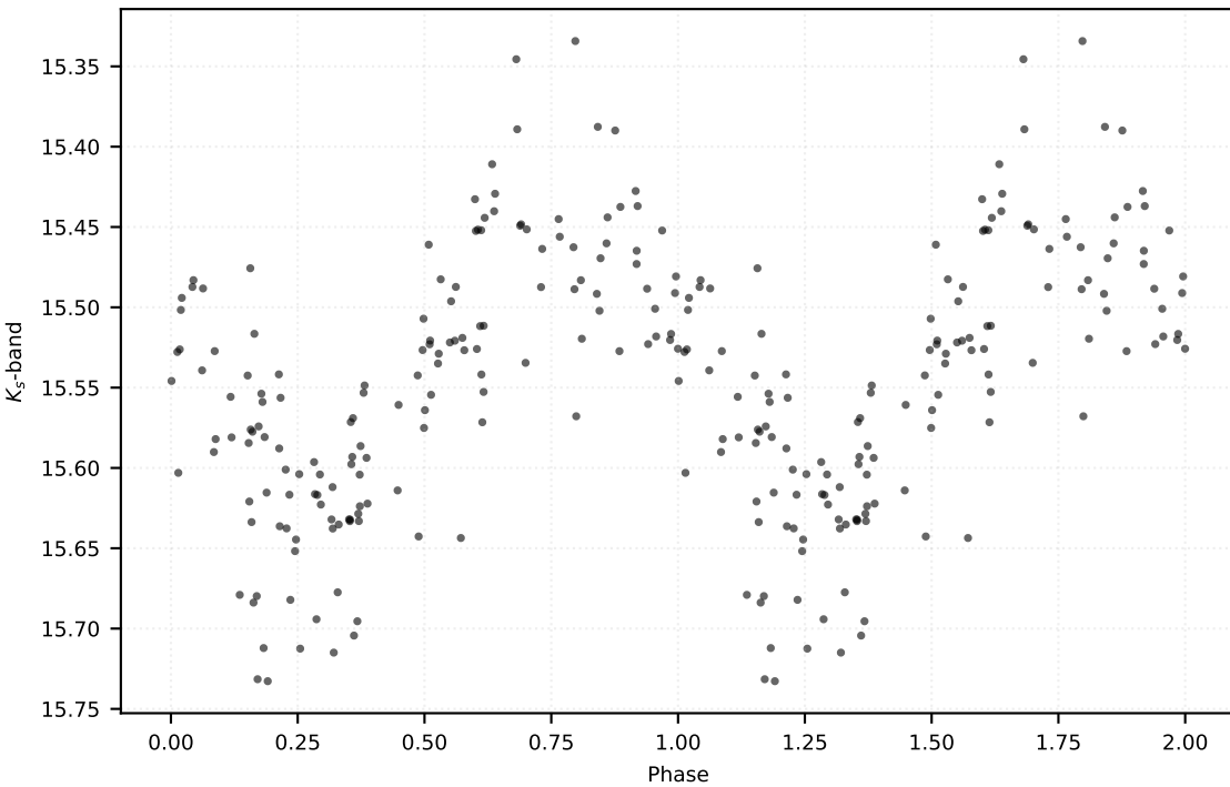
P: 0.43929 d | Class: RP | Subclass: RRab | Field b279
