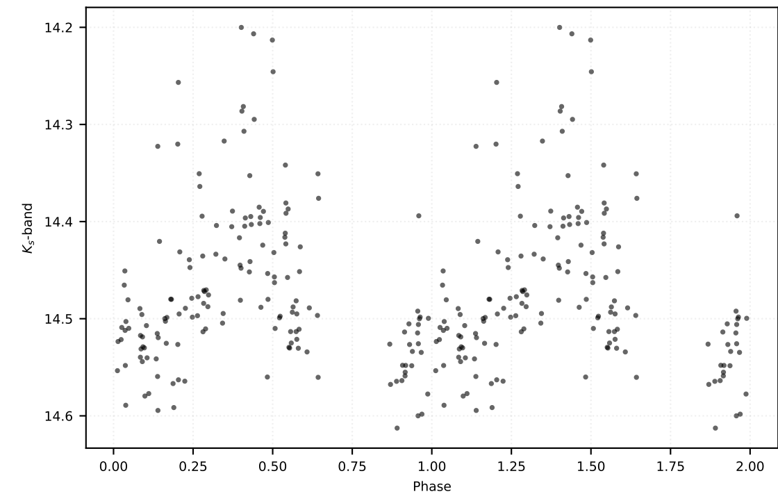
P: 0.14352 d | Class: RP | Subclass: UVAR | Field b279
