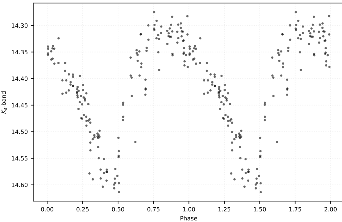
P: 0.54555 d | Class: RP | Subclass: RRab | Field b279
