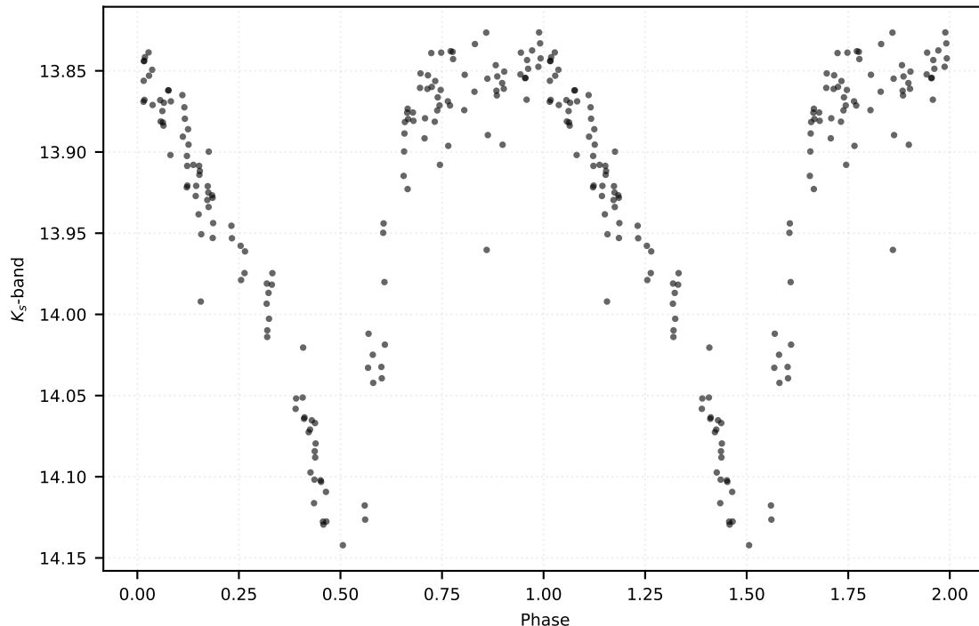
P: 0.50246 d | Class: RP | Subclass: RRab | Field b278
