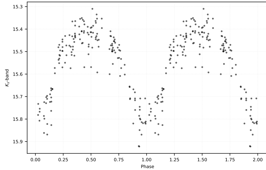
P: 0.35910 d | Class: RP | Subclass: RRc | Field b278
