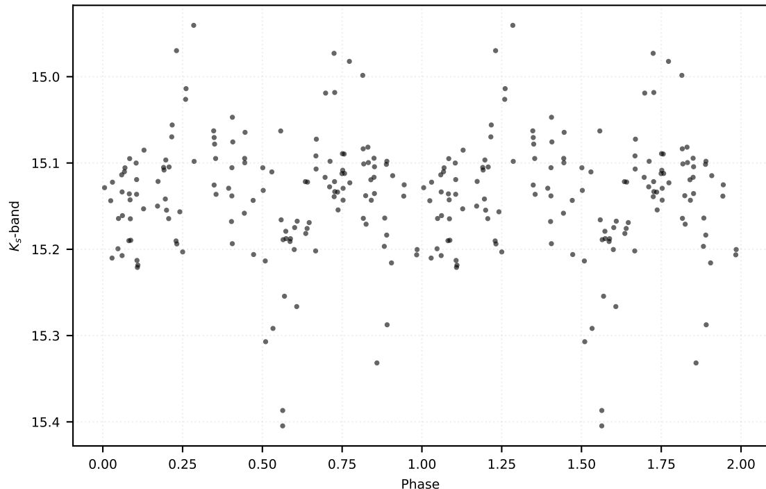
P: 3.02179 d | Class: EB | Subclass: EA | Field b279
