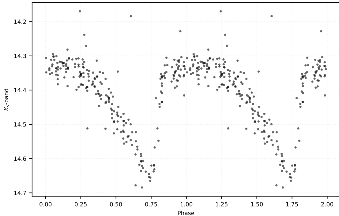
P: 0.53526 d | Class: RP | Subclass: RRab | Field b278
