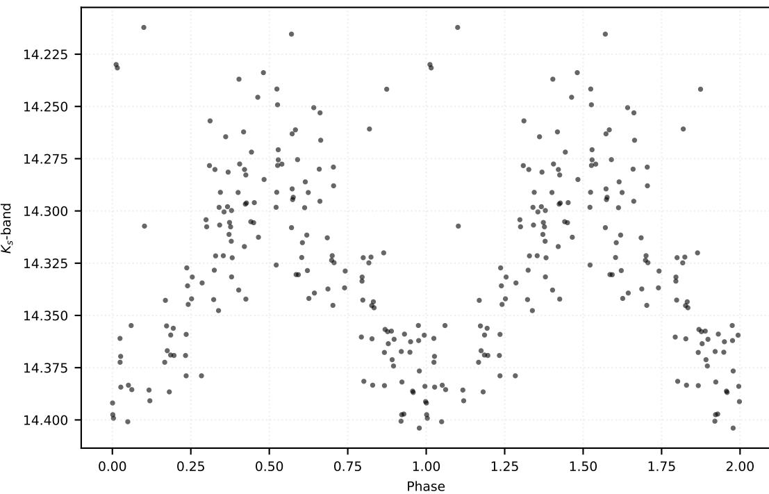
P: 0.46640 d | Class: RP | Subclass: RRab | Field b279
