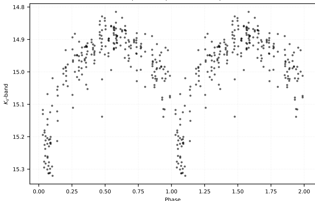
P: 17.19344 d | Class: RP | Subclass: CEP-F | Field b278
