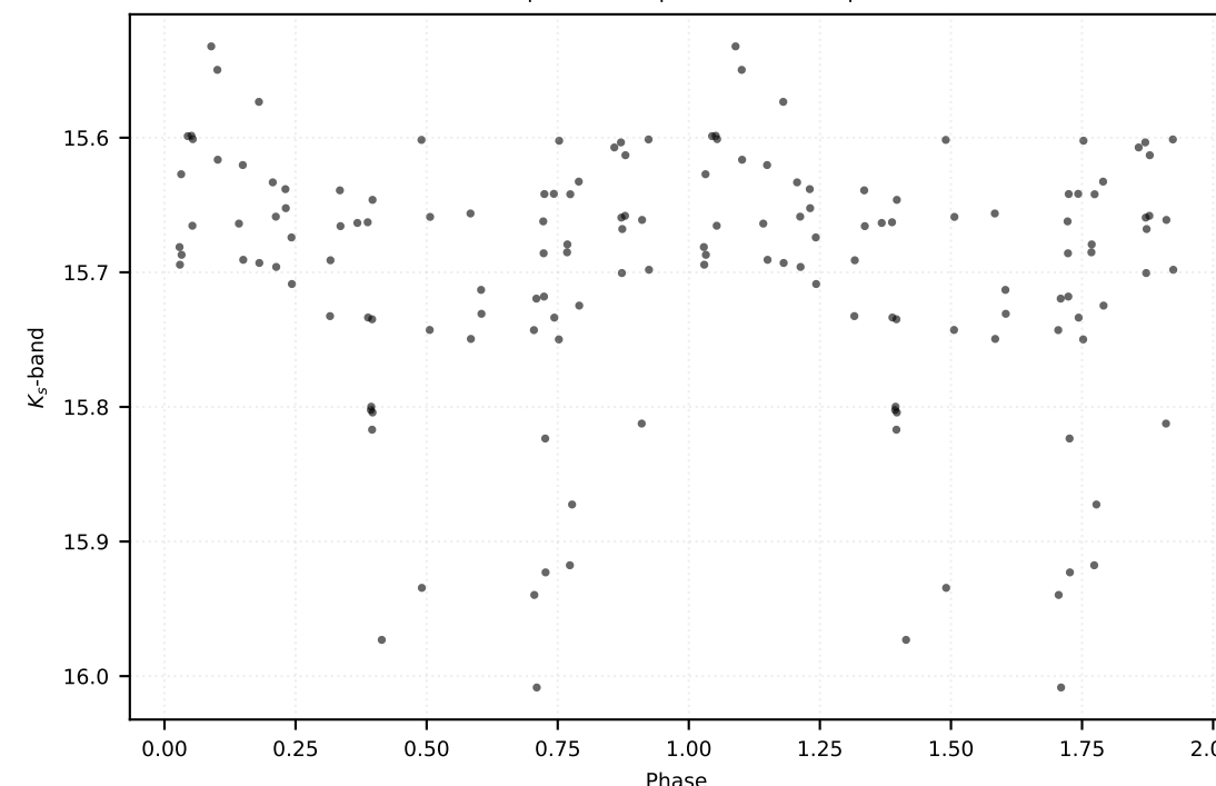
P: 0.20310 d | Class: RP | Subclass: RRc | Field b279
