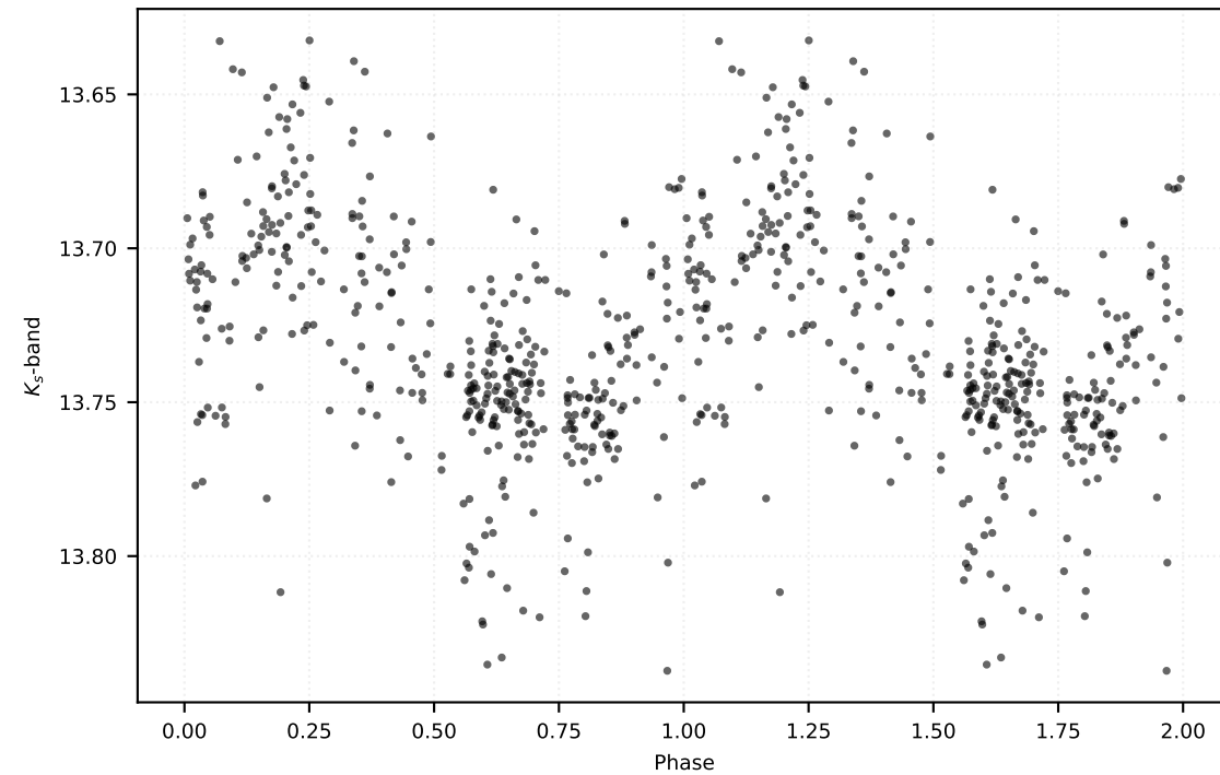
P: 0.35244 d | Class: RP | Subclass: RRab | Field b279
