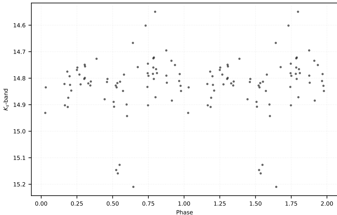
P: 1.73502 d | Class: EB | Subclass: EA | Field b278
