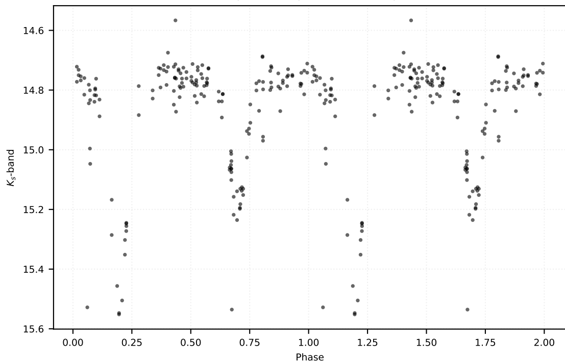
P: 0.15247 d | Class: RP | Subclass: UVAR | Field b278
