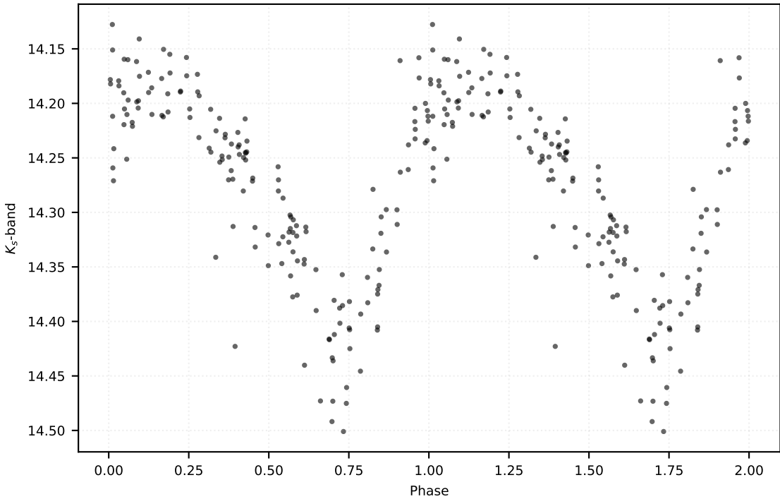
P: 0.60023 d | Class: RP | Subclass: RRab | Field b278
