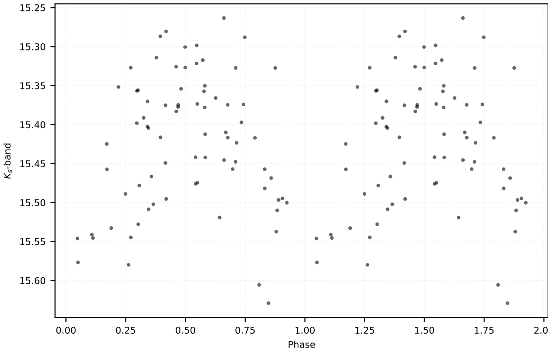
P: 0.51295 d | Class: RP | Subclass: RRab | Field b278
