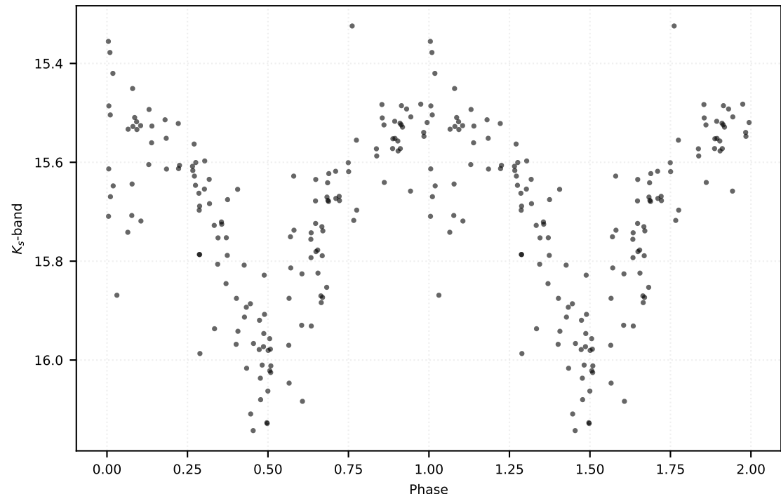
P: 0.63828 d | Class: RP | Subclass: CEP-1OT | Field b278
