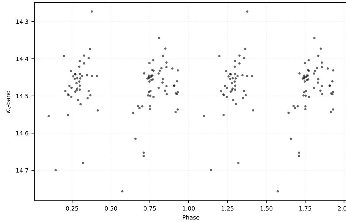
P: 1.99402 d | Class: EB | Subclass: EA | Field b279
