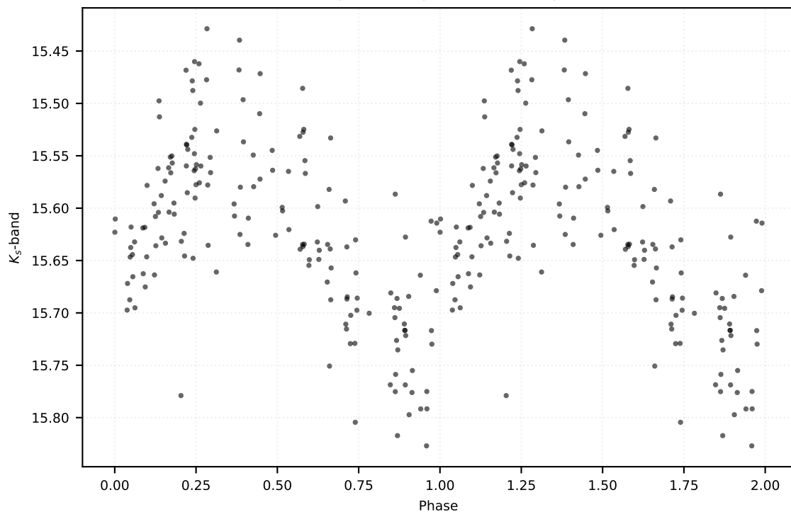
P: 0.31553 d | Class: RP | Subclass: RRab | Field b278
