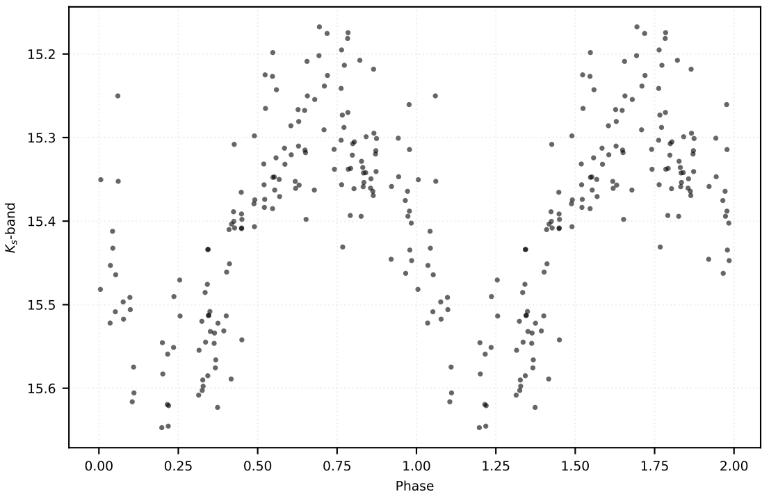
P: 0.26750 d | Class: RP | Subclass: CEP-10T | Field b279
