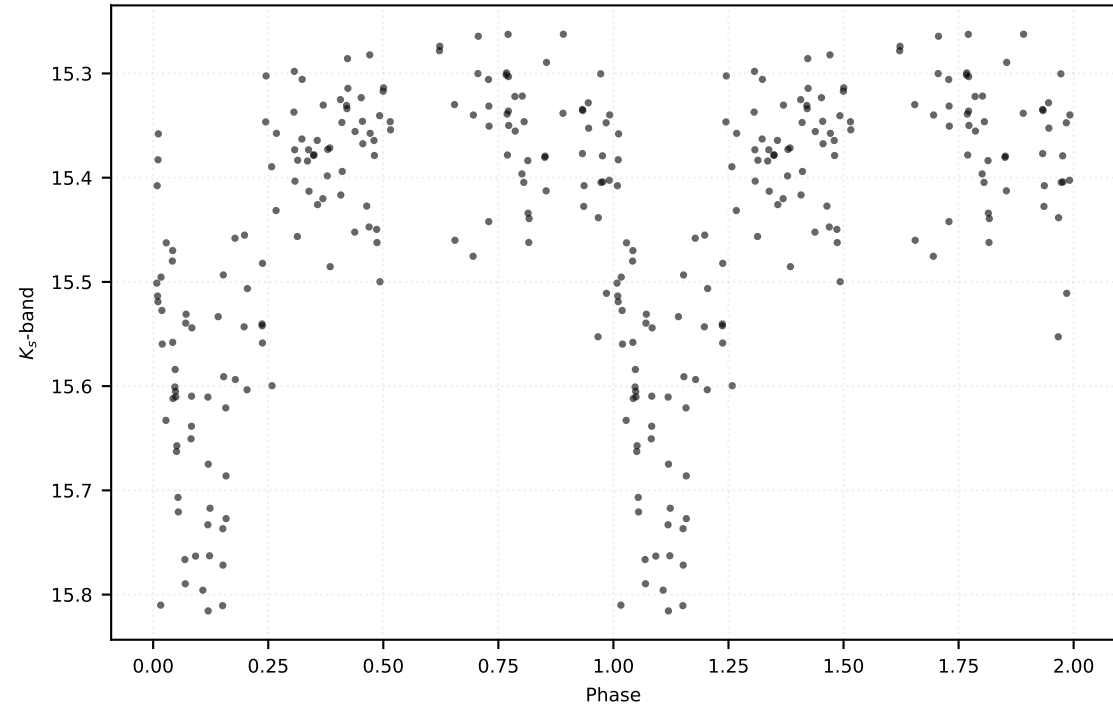
P: 0.49846 d | Class: RP | Subclass: CEP-1OT | Field b278
