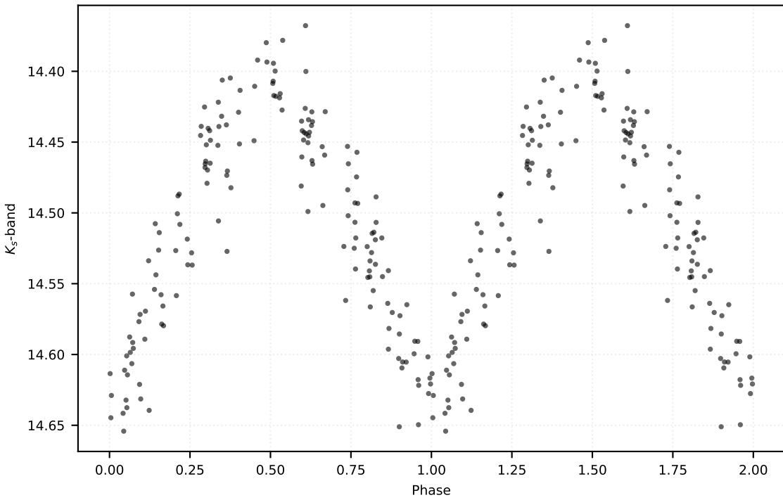
P: 0.58447 d | Class: RP | Subclass: RRc | Field b278
