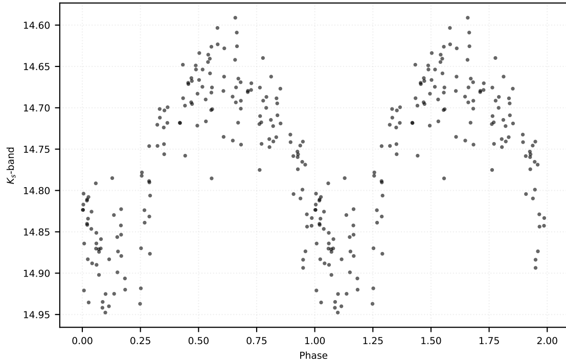
P: 0.34070 d | Class: RP | Subclass: RRab | Field b278
