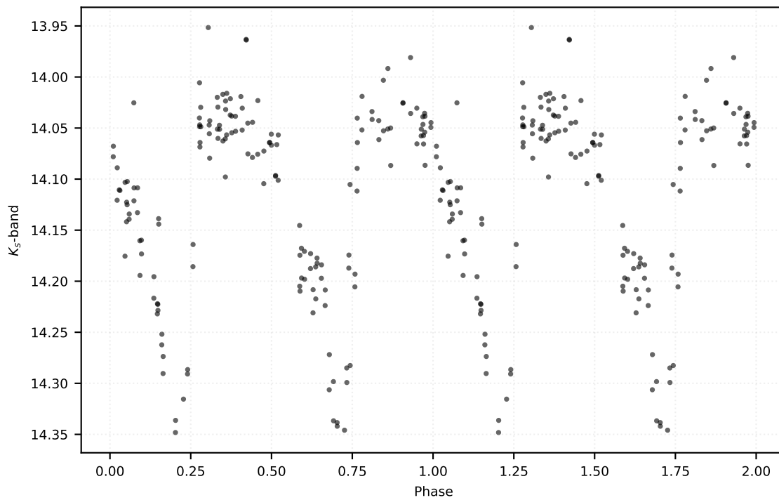
P: 0.22093 d | Class: RP | Subclass: RRc | Field b278
