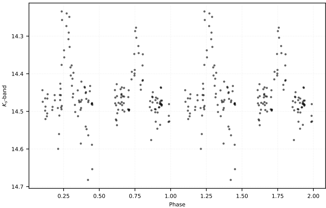
P: 0.21073 d | Class: EB | Subclass: EA | Field b279
