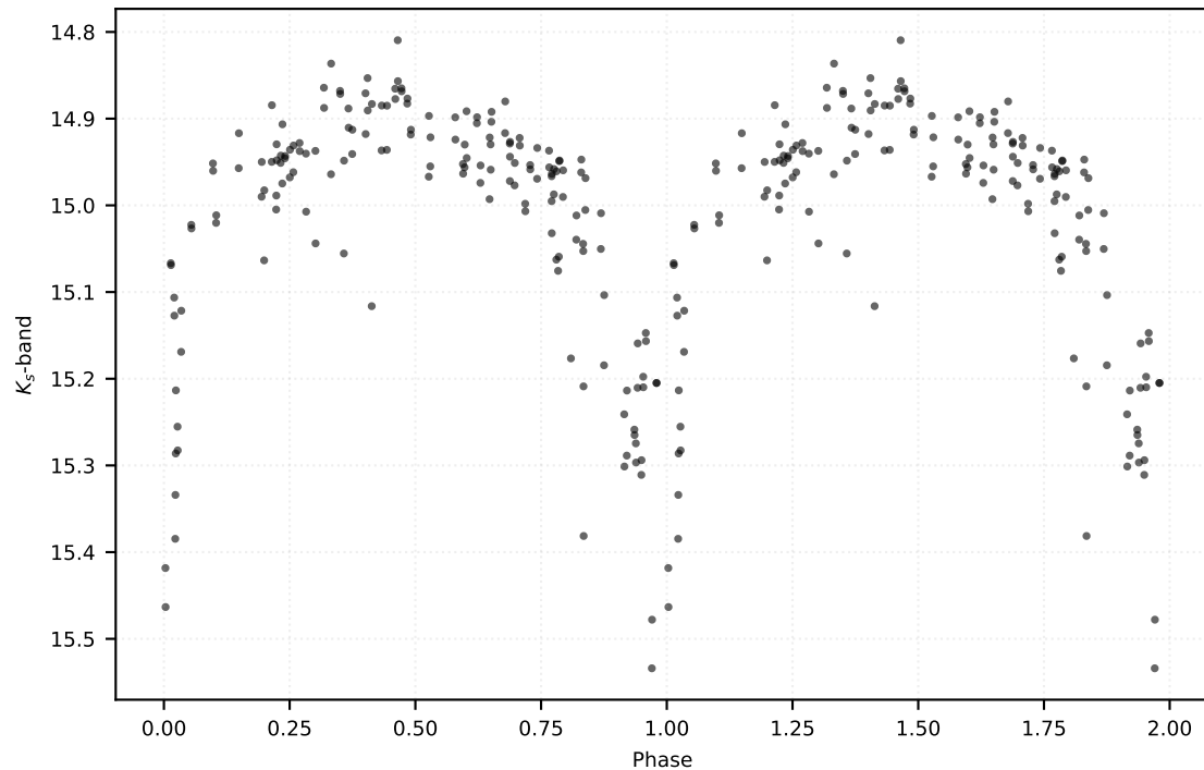
P: 1.19894 d | Class: RP | Subclass: CEP-1OT | Field b278
