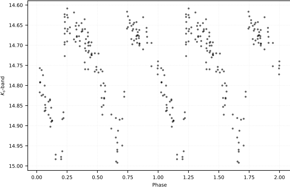
P: 0.80222 d | Class: EB | Subclass: EW | Field b278
