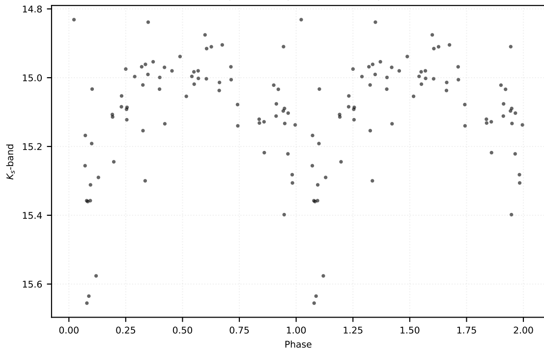
P: 0.53521 d | Class: RP | Subclass: RRab | Field b278
