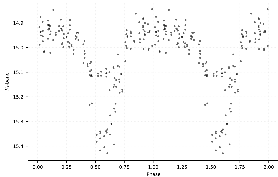
P: 0.61463 d | Class: RP | Subclass: RRab | Field b278
