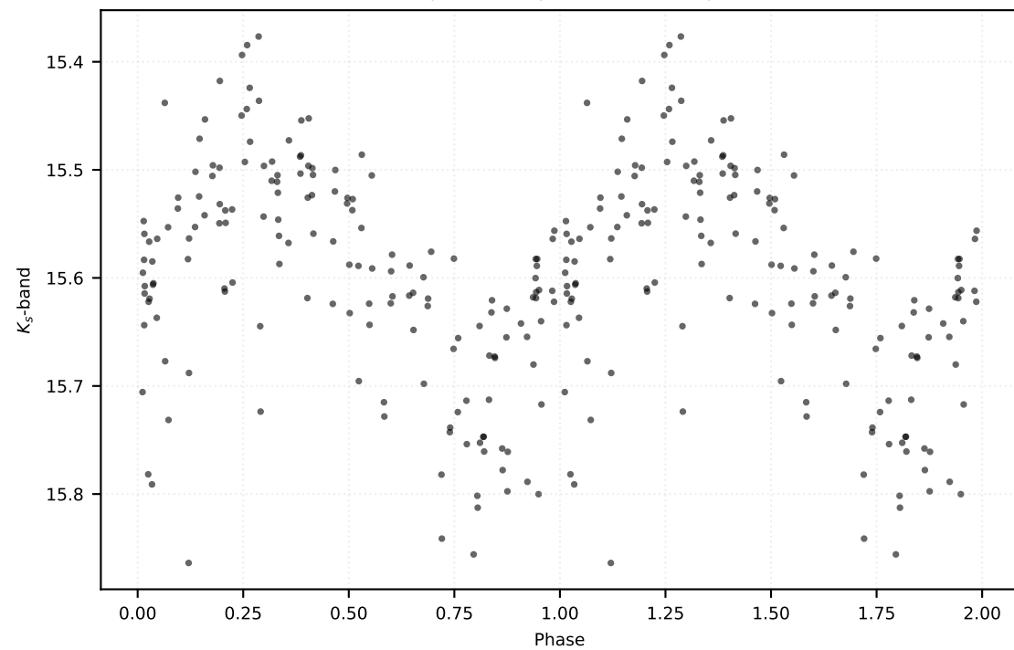
P: 0.57196 d | Class: RP | Subclass: RRab | Field b279
