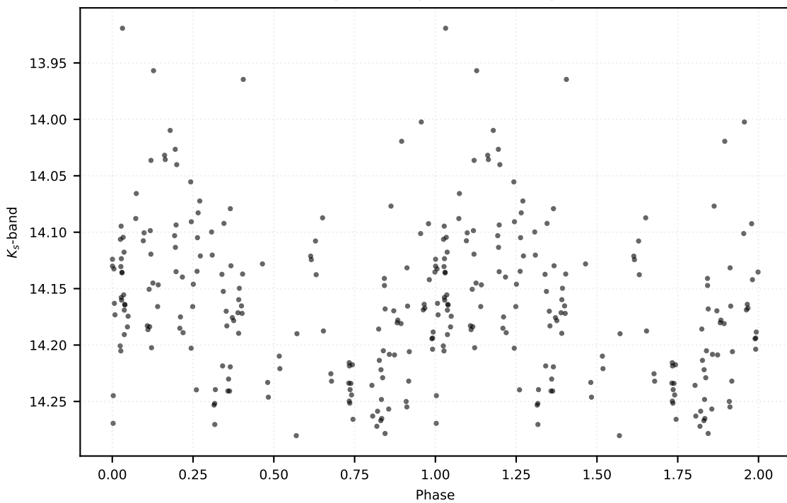
P: 0.17771 d | Class: RP | Subclass: UVAR | Field b279
