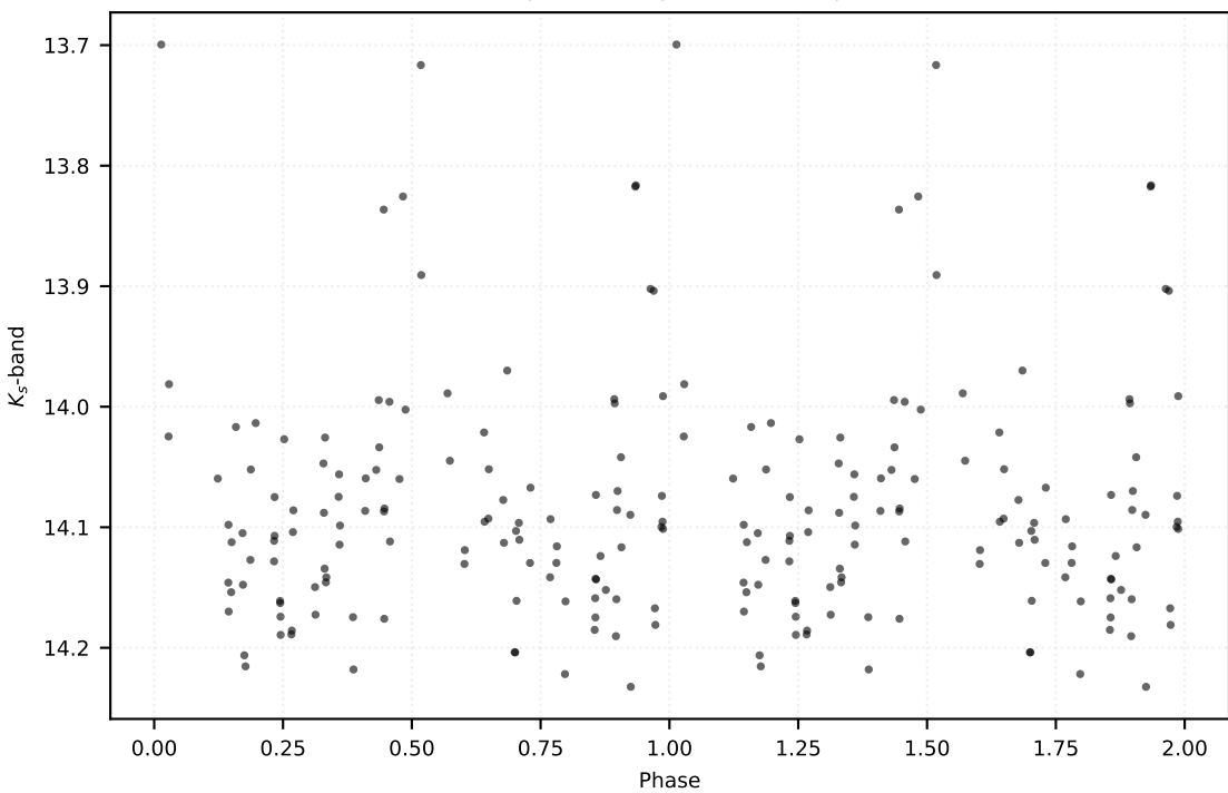
P: 5.11393 d | Class: EB | Subclass: EA | Field b279
