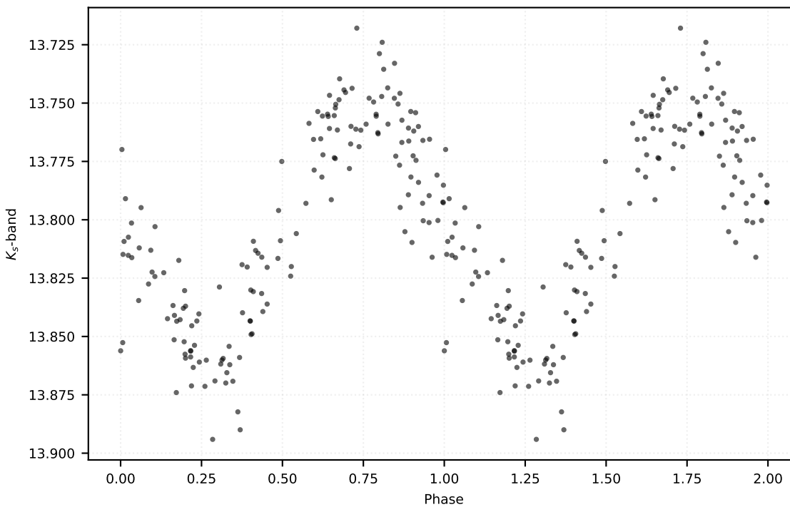
P: 0.36050 d | Class: RP | Subclass: CEP-1OT | Field b279
