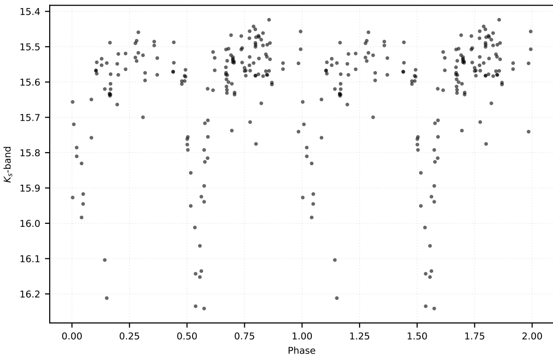
P: 4.14874 d | Class: EB | Subclass: EA | Field b279
