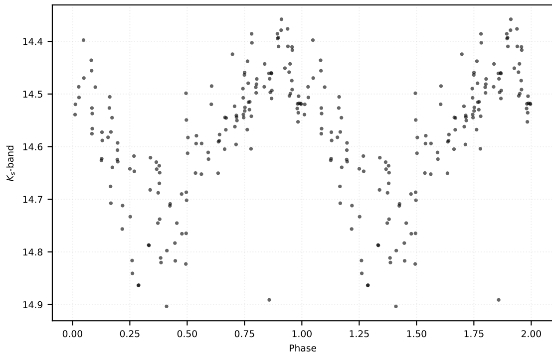
P: 0.35780 d | Class: RP | Subclass: CEP-10T | Field b279
