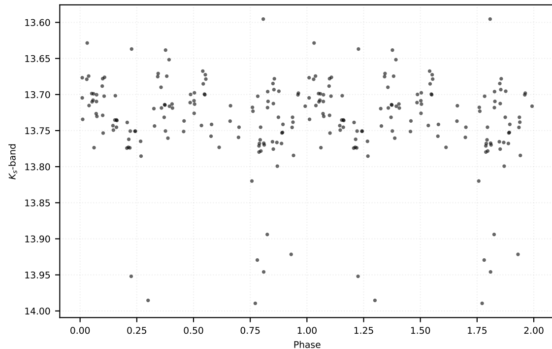
P: 0.41775 d | Class: EB | Subclass: EA | Field b279
