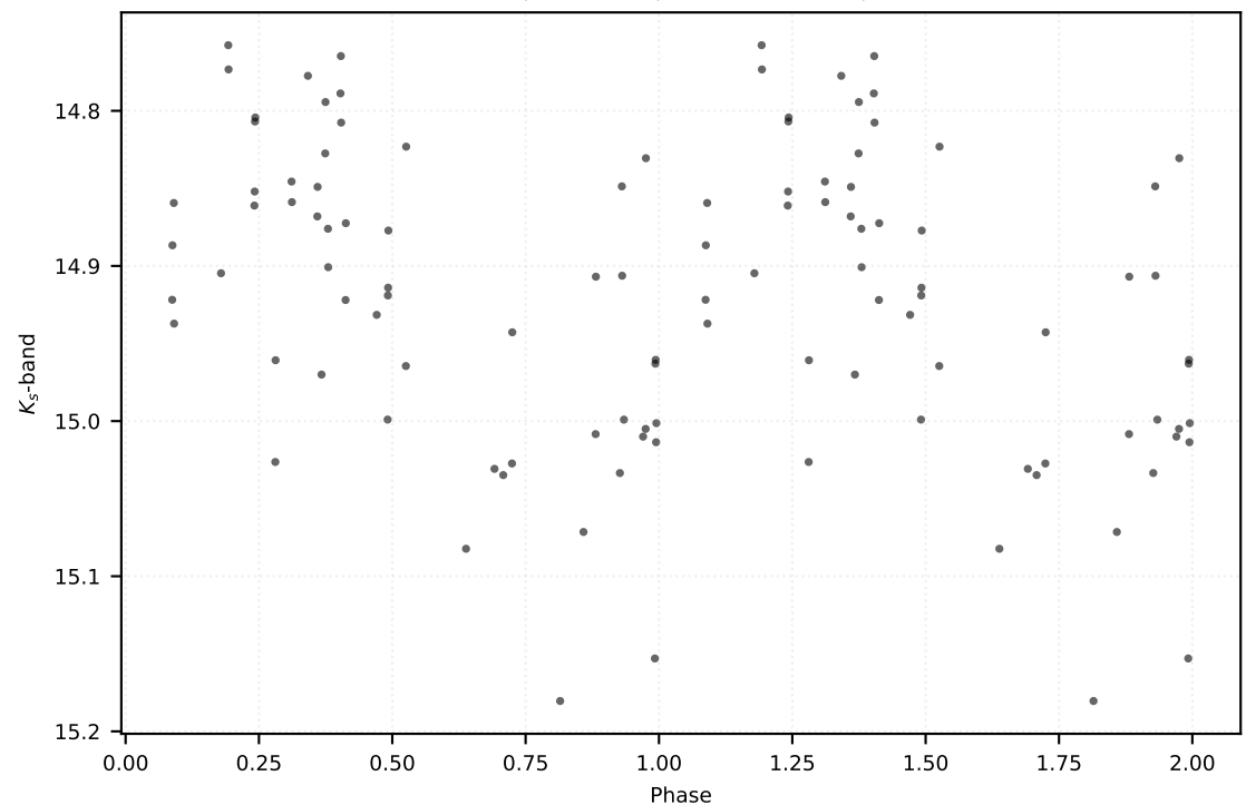
P: 0.51056 d | Class: RP | Subclass: RRab | Field b278
