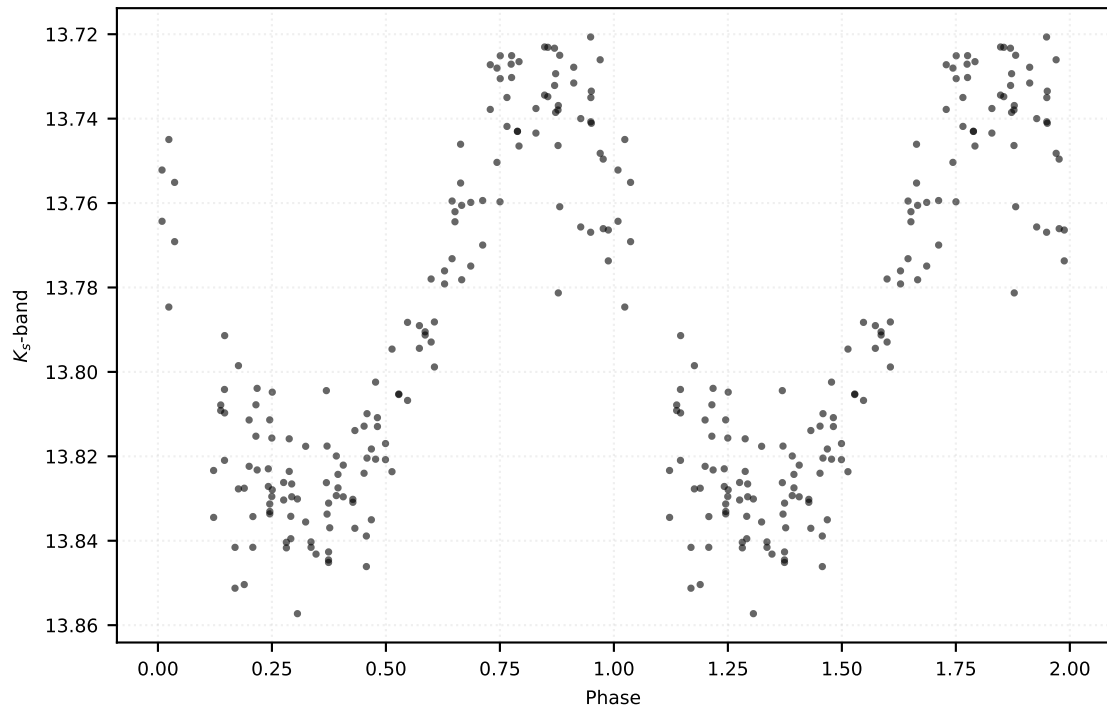
P: 17.14645 d | Class: RP | Subclass: CEP-F | Field b279
