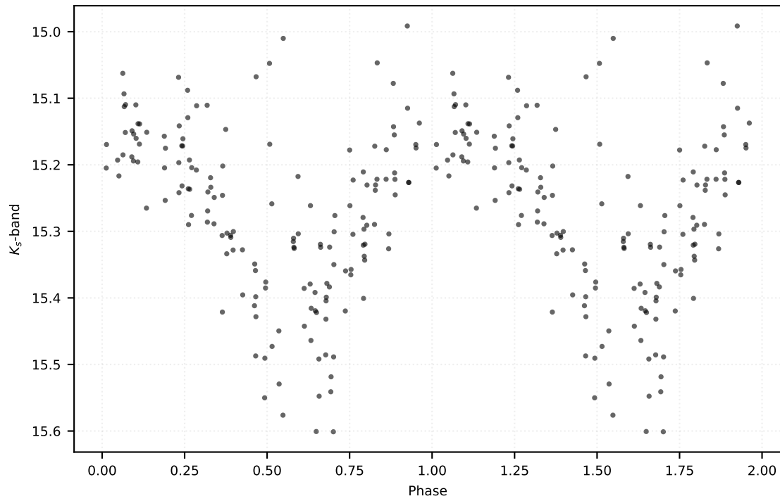
P: 0.53469 d | Class: RP | Subclass: R Rab | Field b278
