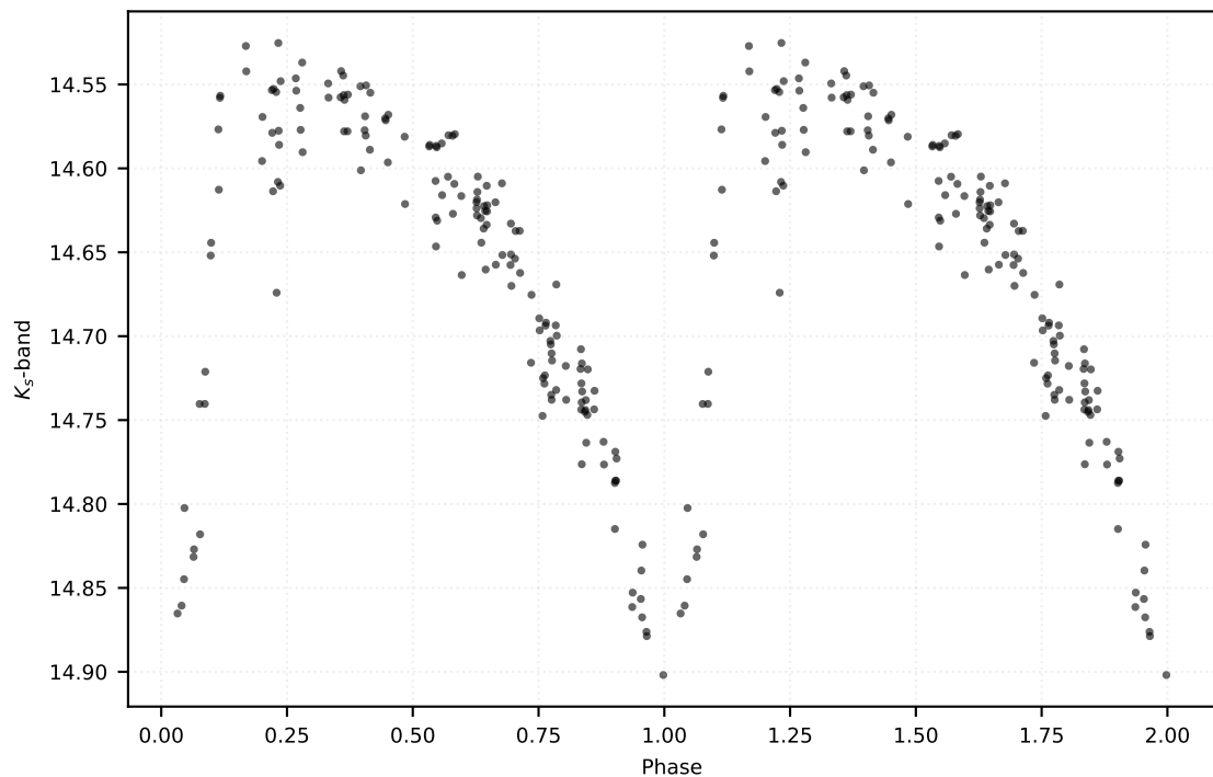
P: 0.38726 d | Class: RP | Subclass: RRab | Field b279
