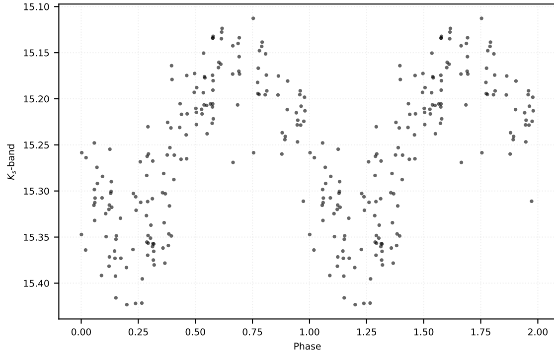
P: 0.21778 d | Class: RP | Subclass: UVAR | Field b279
