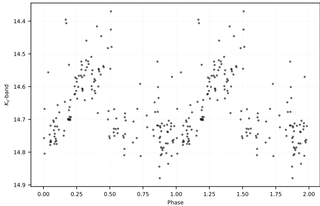
P: 0.16756 d | Class: RP | Subclass: UVAR | Field b278
