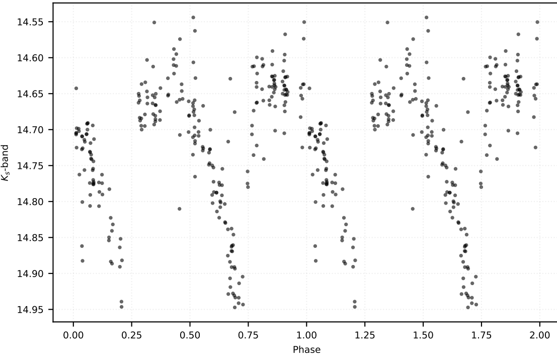
P: 0.23494 d | Class: RP | Subclass: UVAR | Field b279
