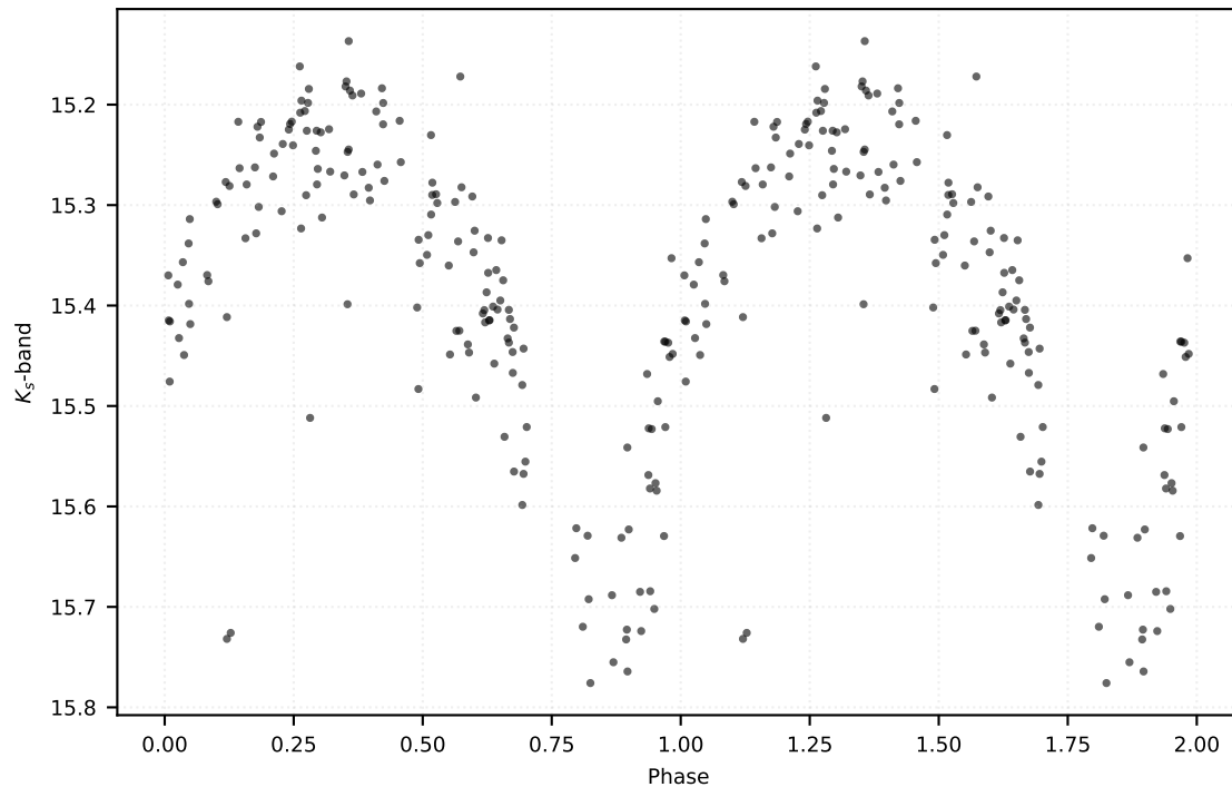
P: 0.16857 d | Class: RP | Subclass: UVAR | Field b278
