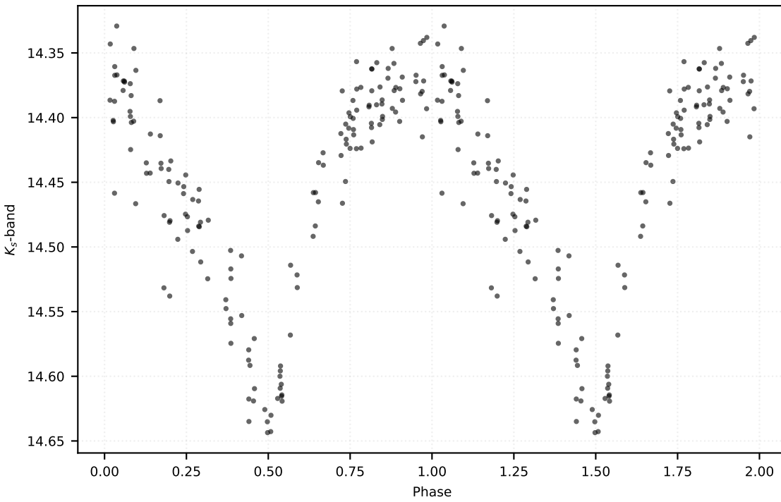
P: 0.60299 d | Class: RP | Subclass: CEP-10T | Field b279
