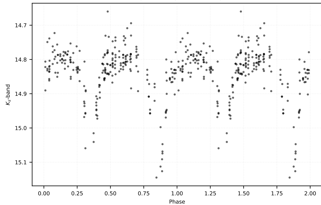
P: 0.51481 d | Class: EB | Subclass: EA | Field b278
