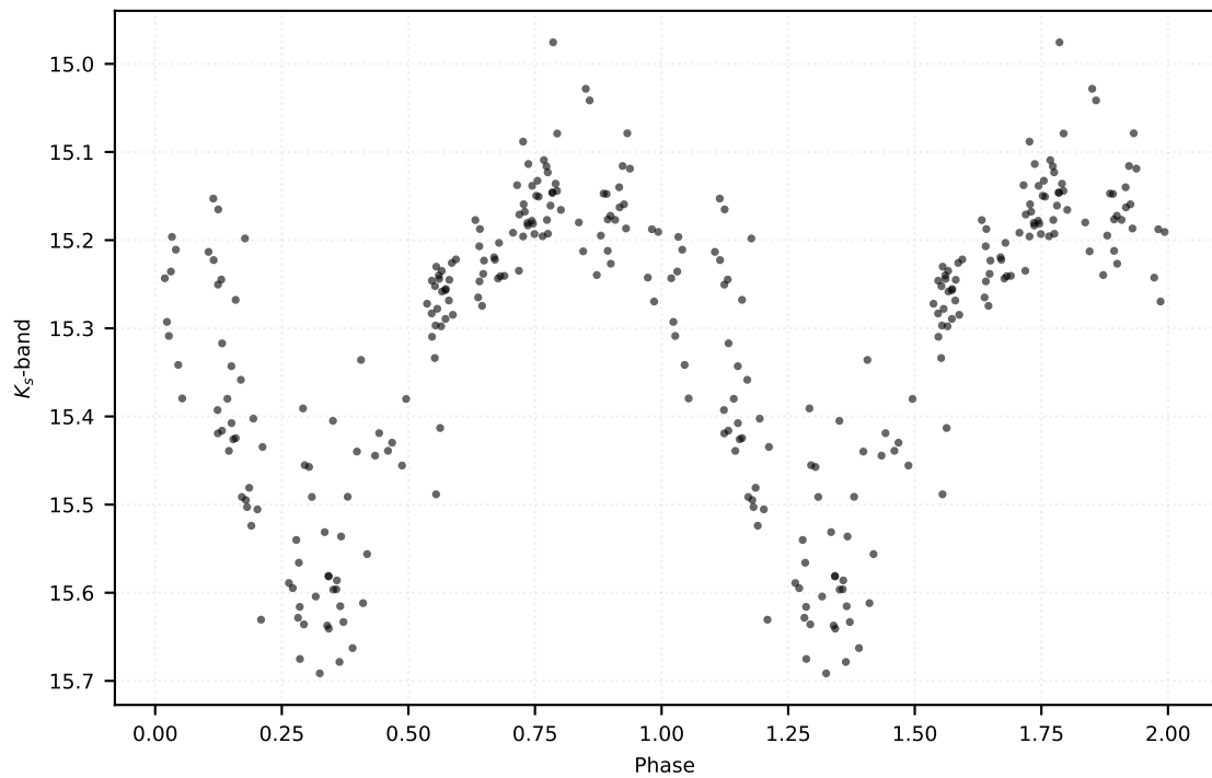
P: 0.19768 d | Class: RP | Subclass: UVAR | Field b278
