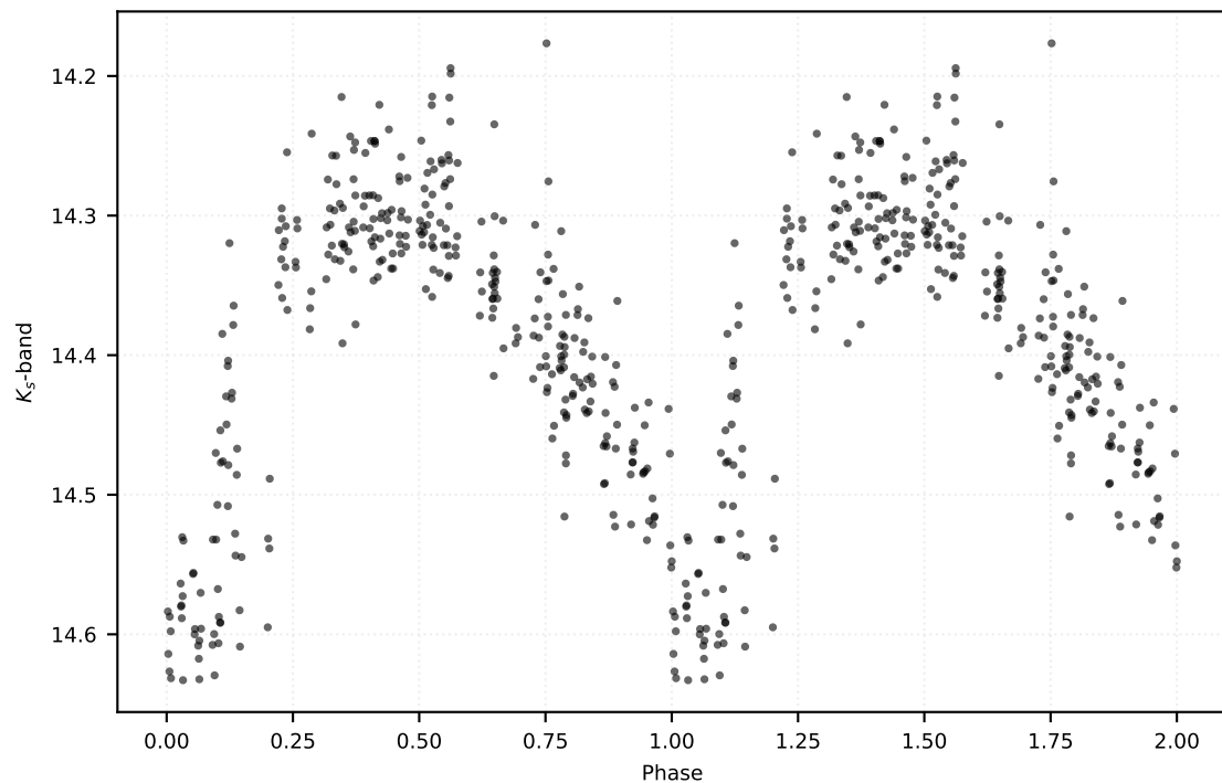
P: 0.56484 d | Class: RP | Subclass: RRab | Field b278
