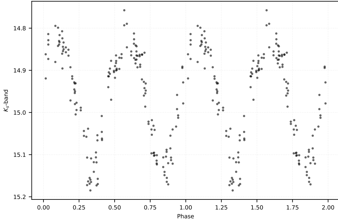
P: 0.49433 d | Class: EB | Subclass: EW | Field b278
