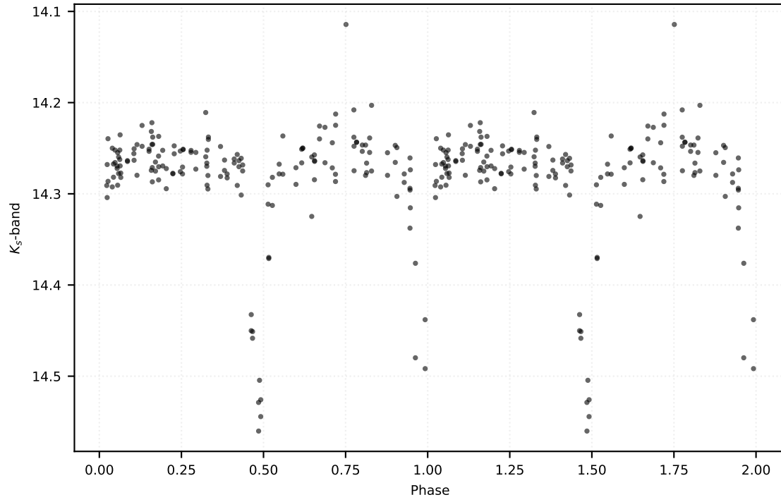
P: 0.40055 d | Class: EB | Subclass: EA | Field b278
