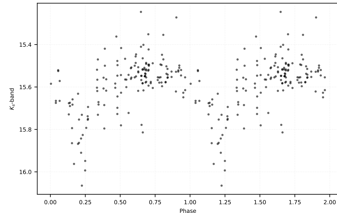
P: 0.49514 d | Class: RP | Subclass: CEP-10T | Field b279
