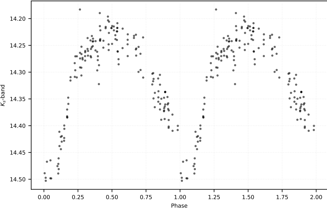
P: 0.56186 d | Class: RP | Subclass: RRc | Field b279
