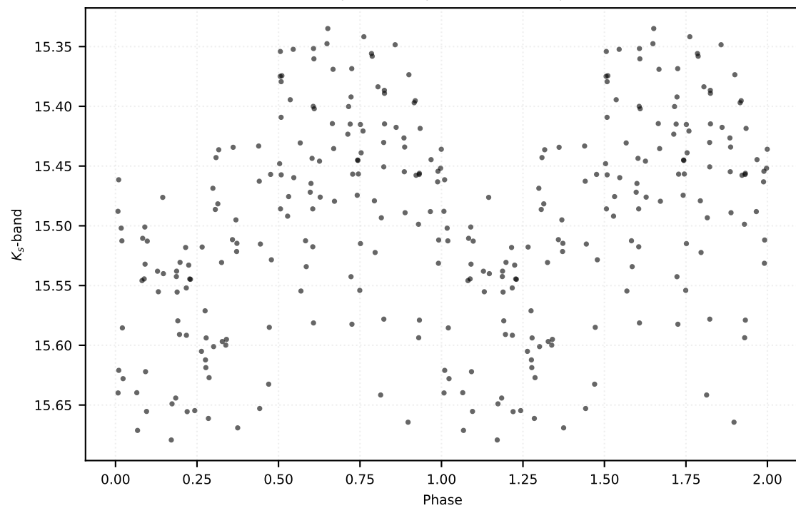
P: 60.16084 d | Class: RP | Subclass: UVAR | Field b279
