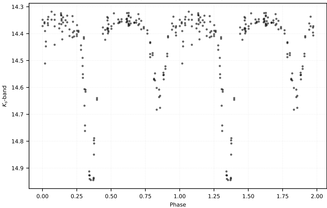
P: 5.42626 d | Class: EB | Subclass: EA | Field b279
