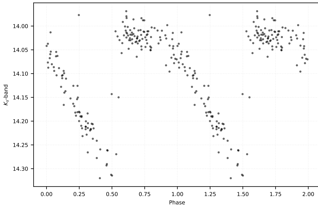
P: 0.56632 d | Class: RP | Subclass: RRab | Field b278
