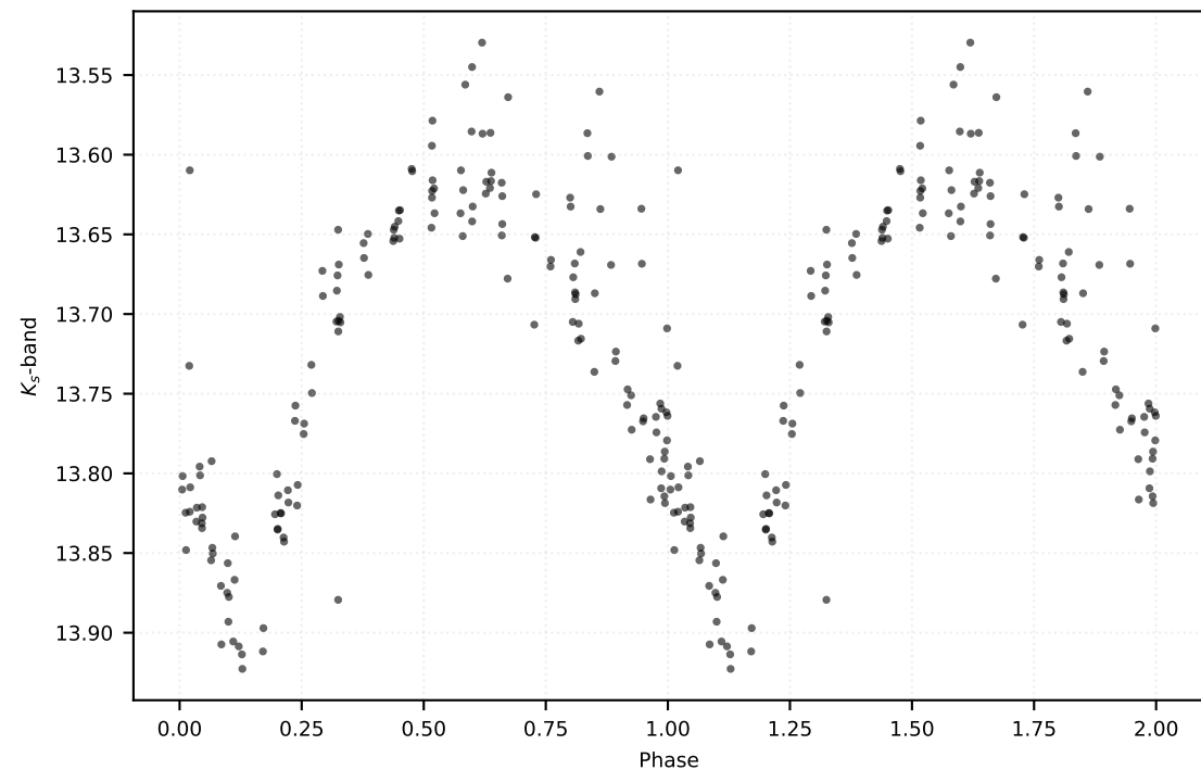
P: 0.27968 d | Class: RP | Subclass: CEP-10T | Field b279
