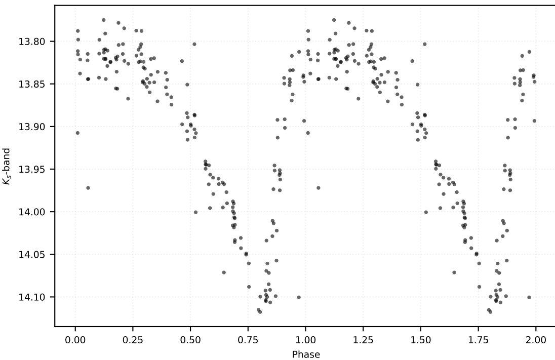
P: 0.55124 d | Class: RP | Subclass: RRab | Field b279
