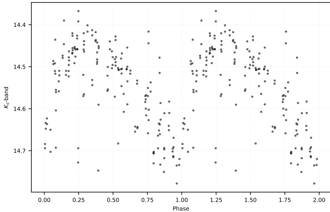
P: 0.61729 d | Class: RP | Subclass: RRab | Field b279
