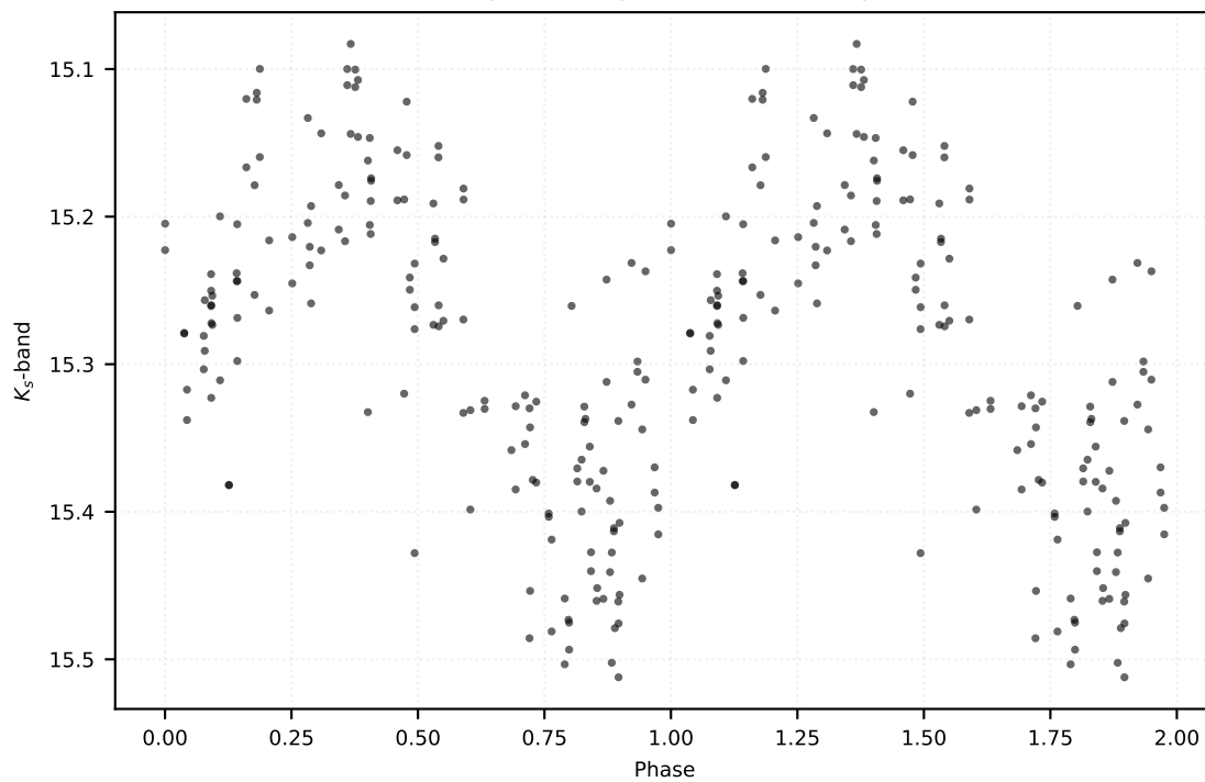
P: 9.94860 d | Class: RP | Subclass: CEP-10T | Field b279
