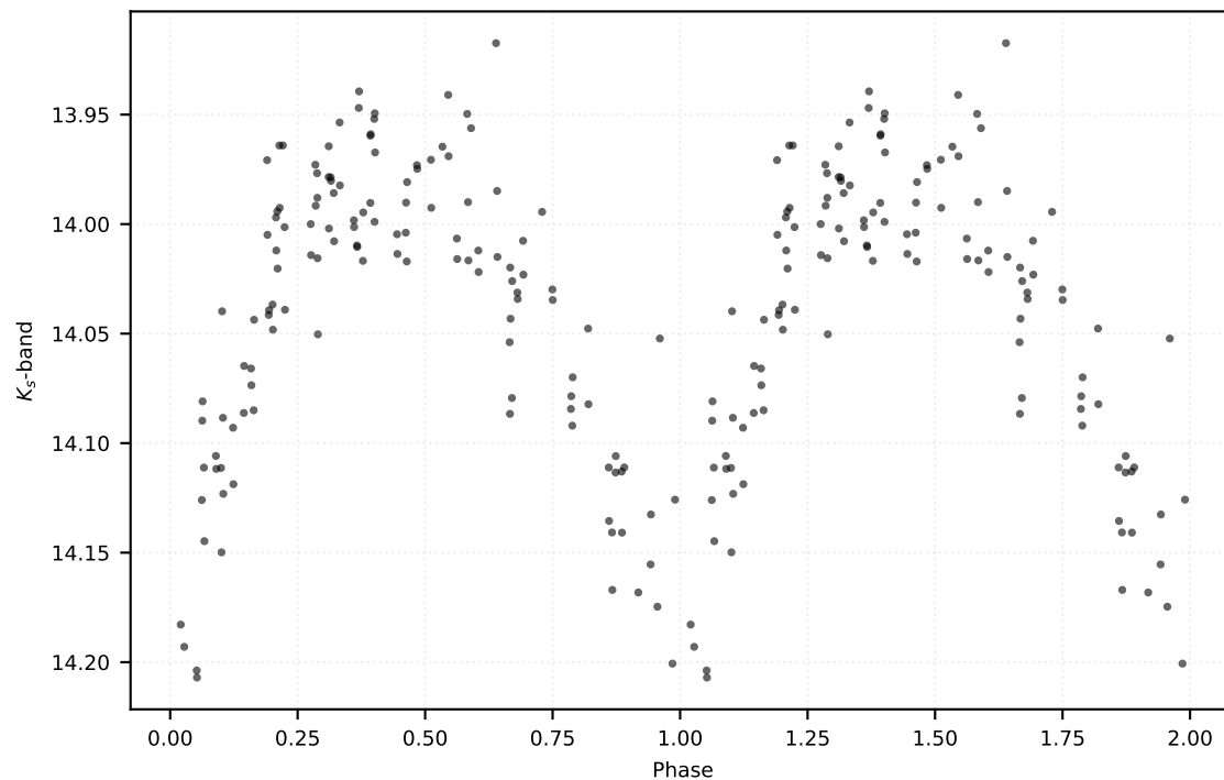
P: 0.43919 d | Class: RP | Subclass: RRab | Field b279
