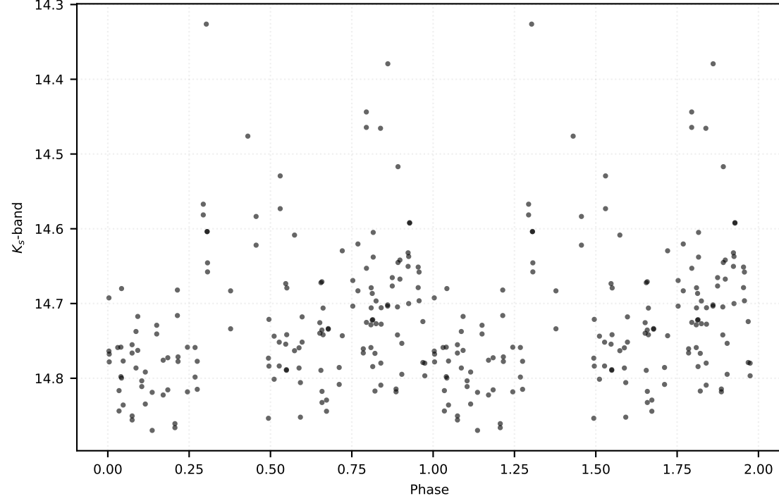
P: 0.30322 d | Class: EB | Subclass: EA | Field b279
