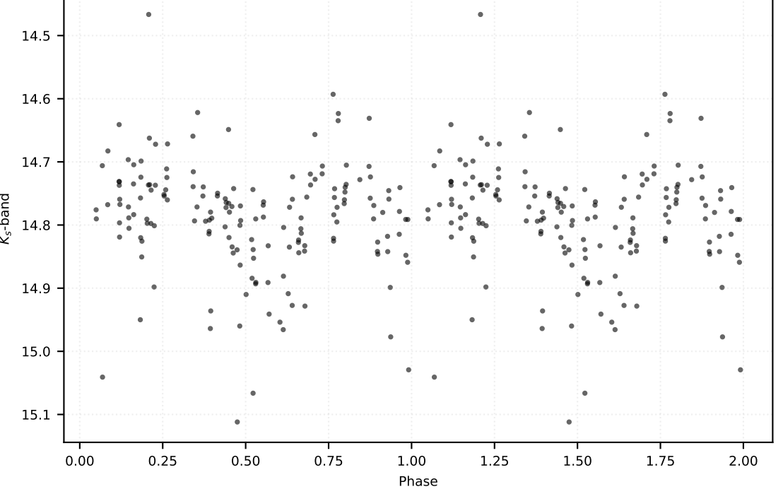
P: 0.67239 d | Class: EB | Subclass: EA | Field b278
