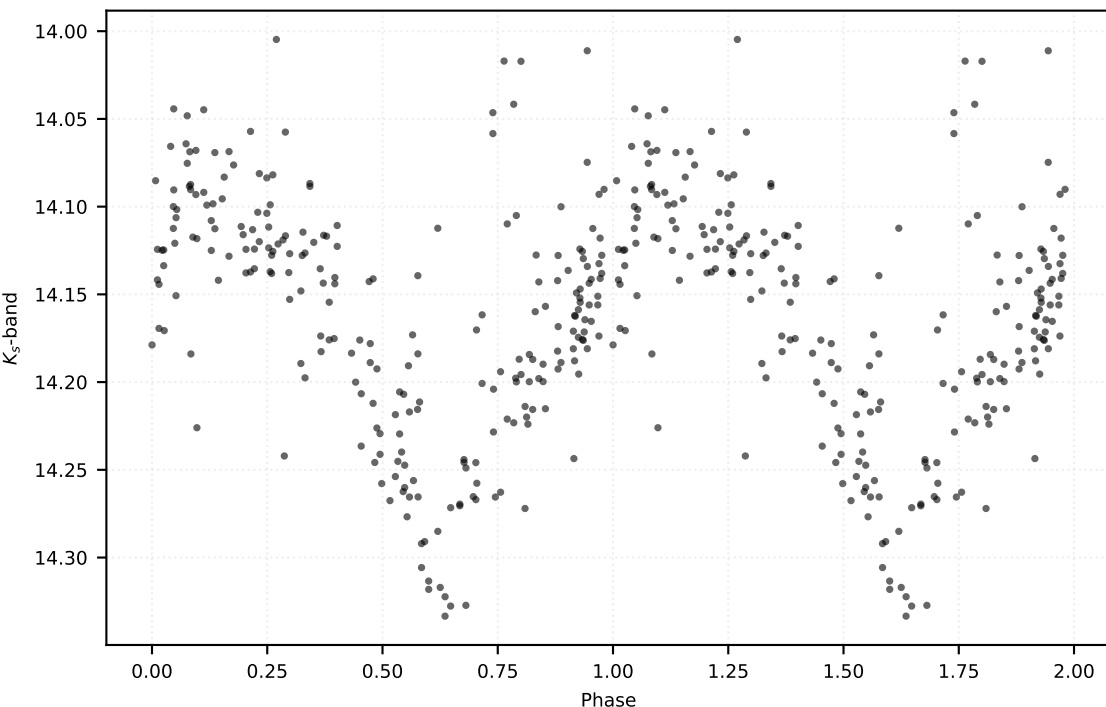
P: 1.23137 d | Class: RP | Subclass: CEP-F | Field b278
