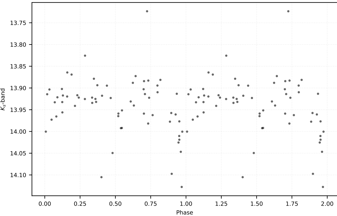
P: 0.20202 d | Class: EB | Subclass: EA | Field b278
