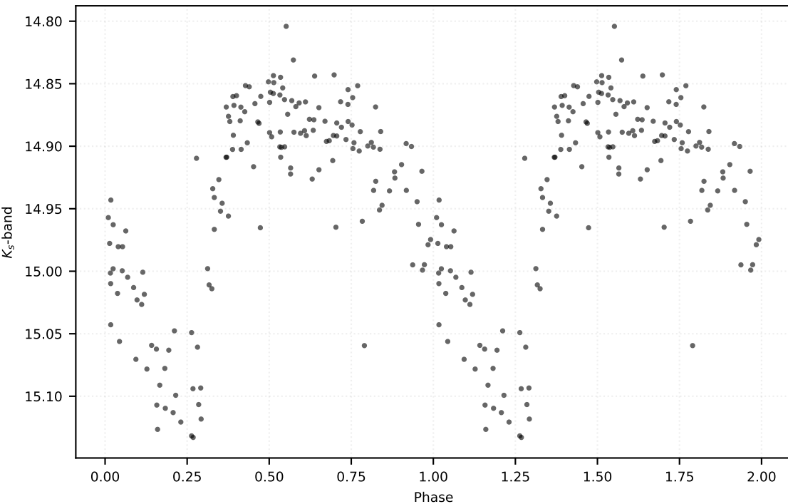
P: 0.39690 d | Class: RP | Subclass: RRab | Field b279
