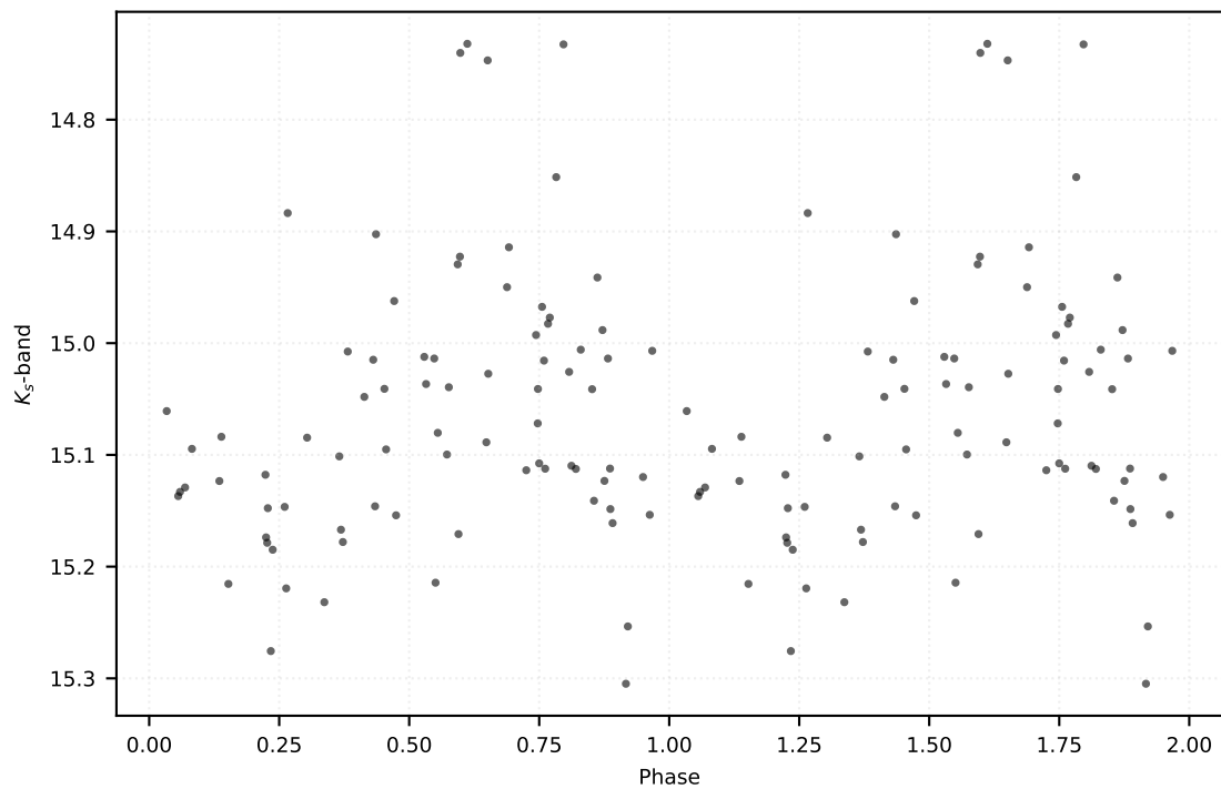
P: 0.13459 d | Class: RP | Subclass: UVAR | Field b279
