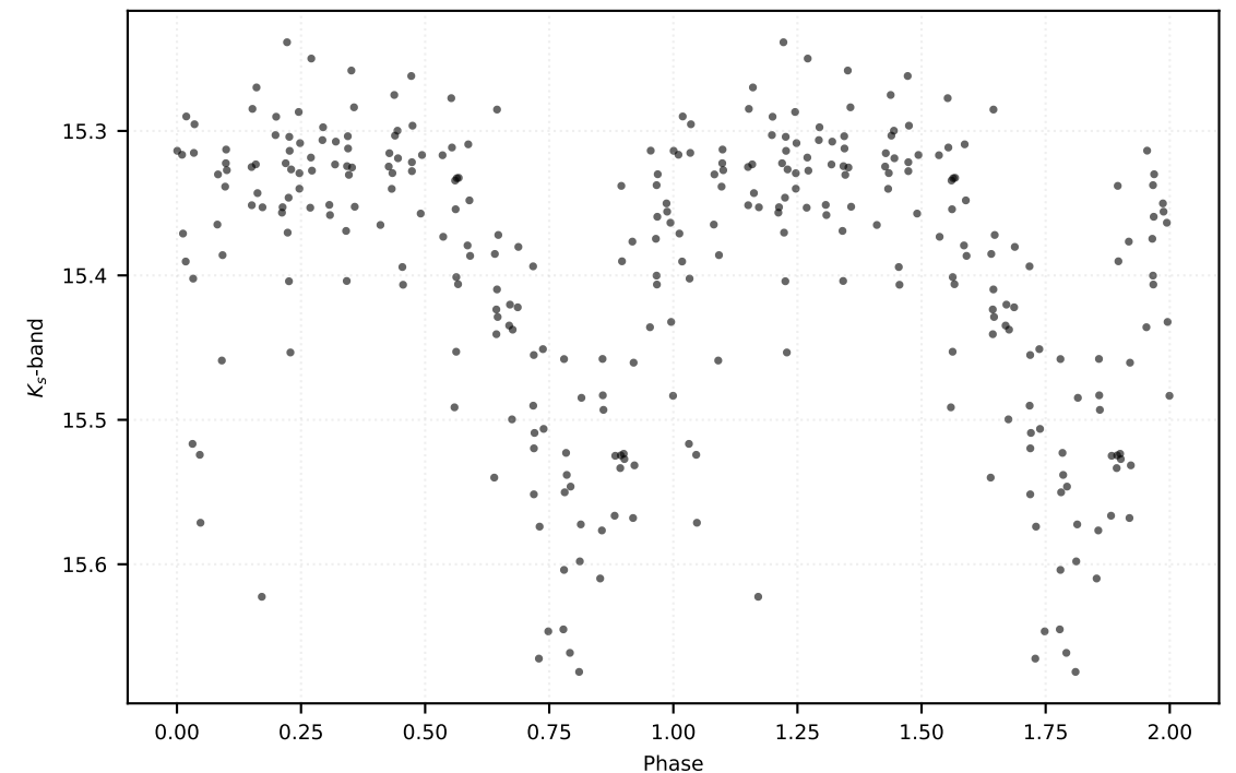
P: 1.36768 d | Class: RP | Subclass: CEP-10T | Field b279
