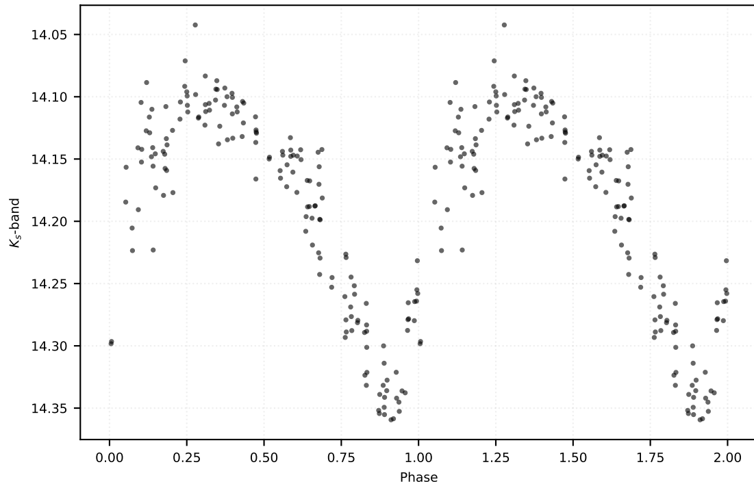
P: 3.28233 d | Class: RP | Subclass: CEP-10T | Field b278
