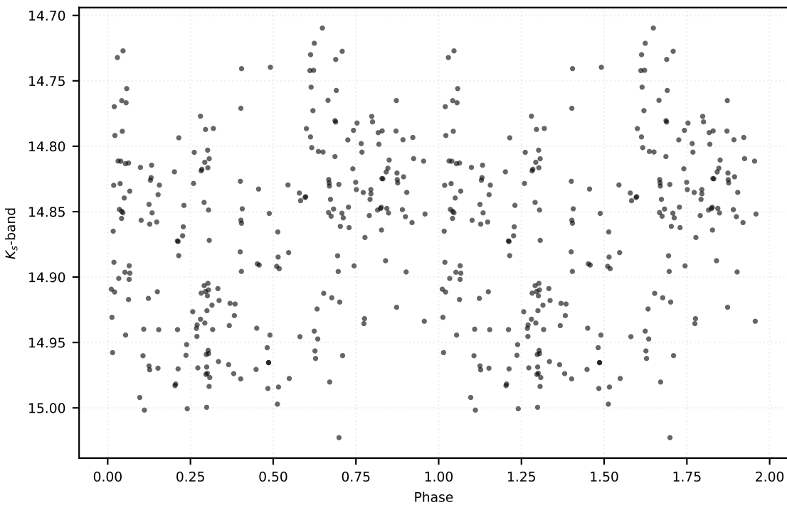
P: 0.10681 d | Class: RP | Subclass: UVAR | Field b278
