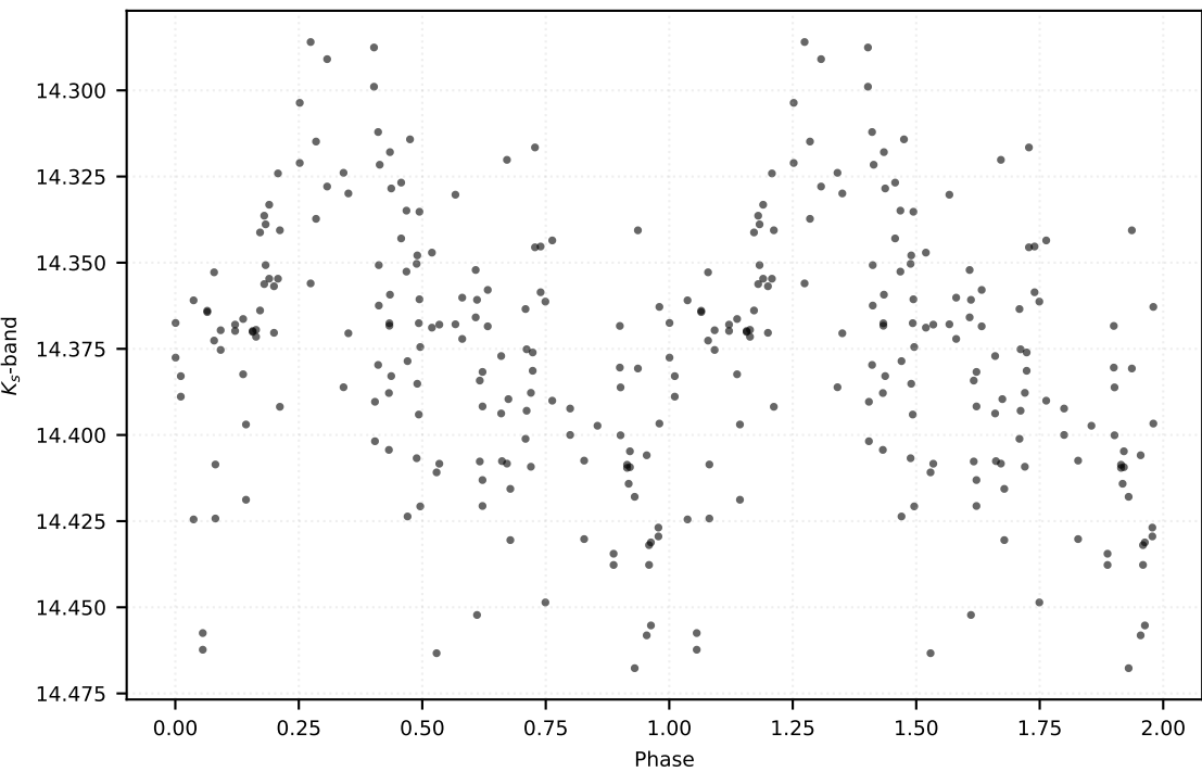
P: 1.82027 d | Class: RP | Subclass: CEP-F | Field b279
