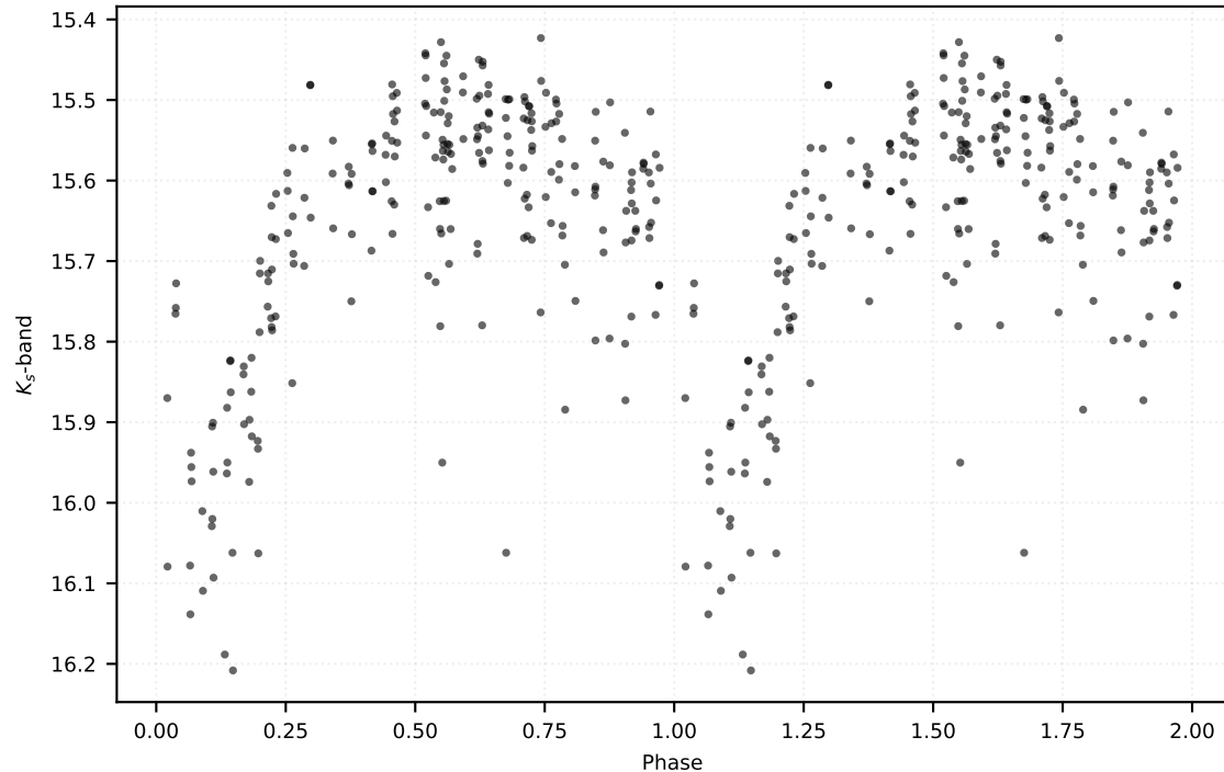
P: 0.83183 d | Class: RP | Subclass: CEP-10T | Field b278
