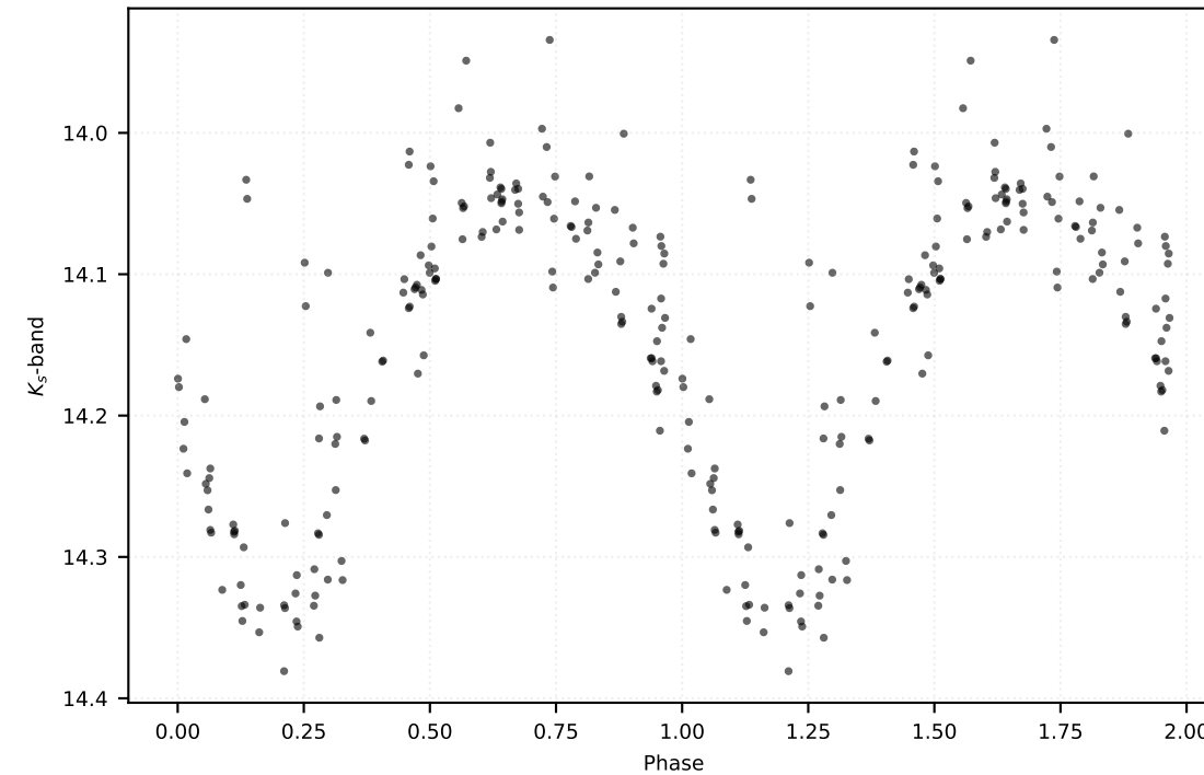
P: 0.51399 d | Class: RP | Subclass: RRc | Field b279
