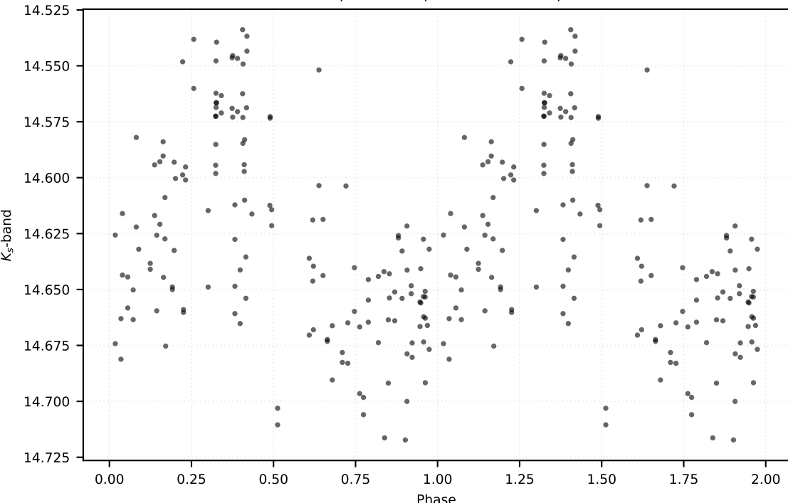
P: 0.24932 d | Class: RP | Subclass: UVAR | Field b278
