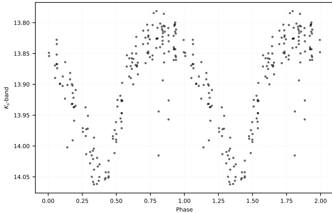
P: 0.61075 d | Class: RP | Subclass: CEP-10T | Field b278
