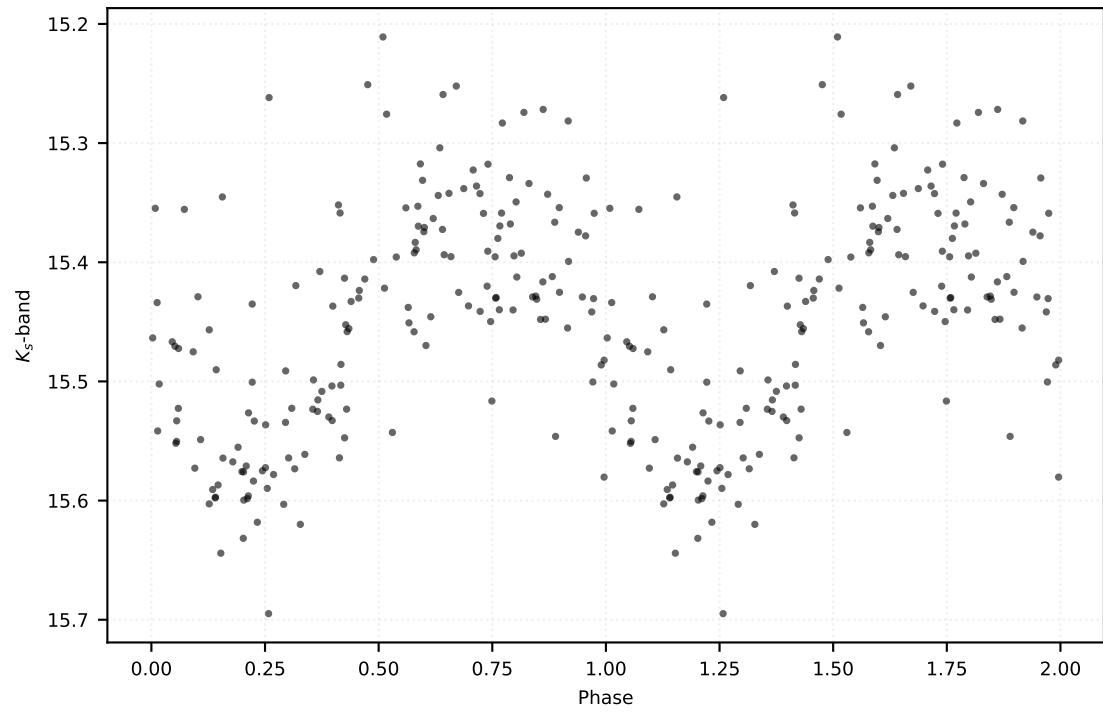
P: 0.29594 d | Class: RP | Subclass: UVAR | Field b278
