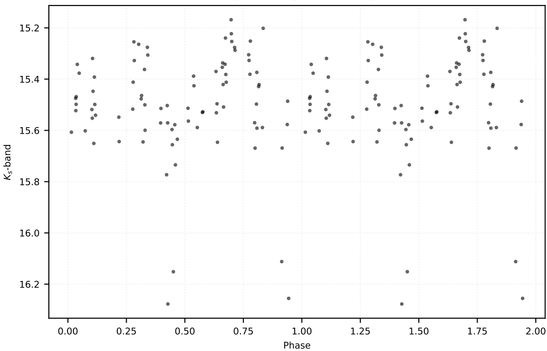
P: 0.32442 d | Class: EB | Subclass: EA | Field b278
