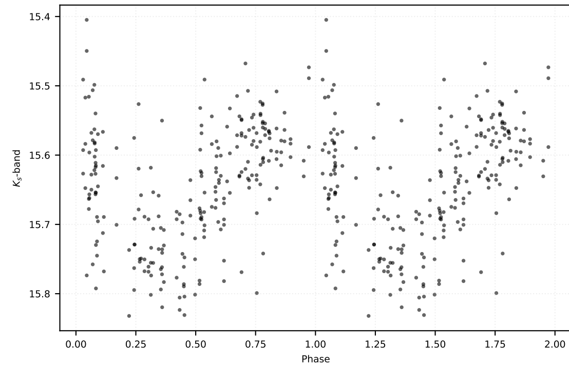
P: 2.79909 d | Class: RP | Subclass: CEP-F | Field b278
