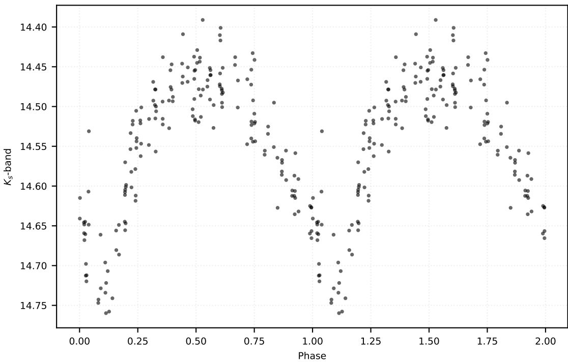
P: 0.55978 d | Class: RP | Subclass: RRc | Field b278
