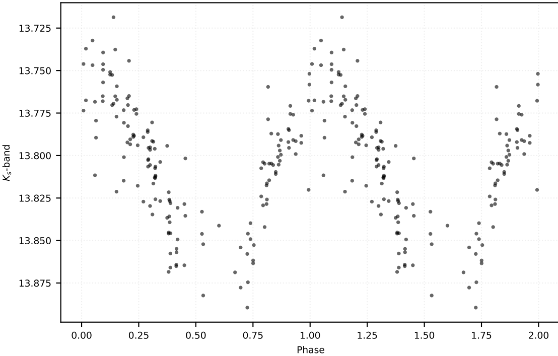
P: 28.27457 d | Class: RP | Subclass: CEP-F | Field b279
