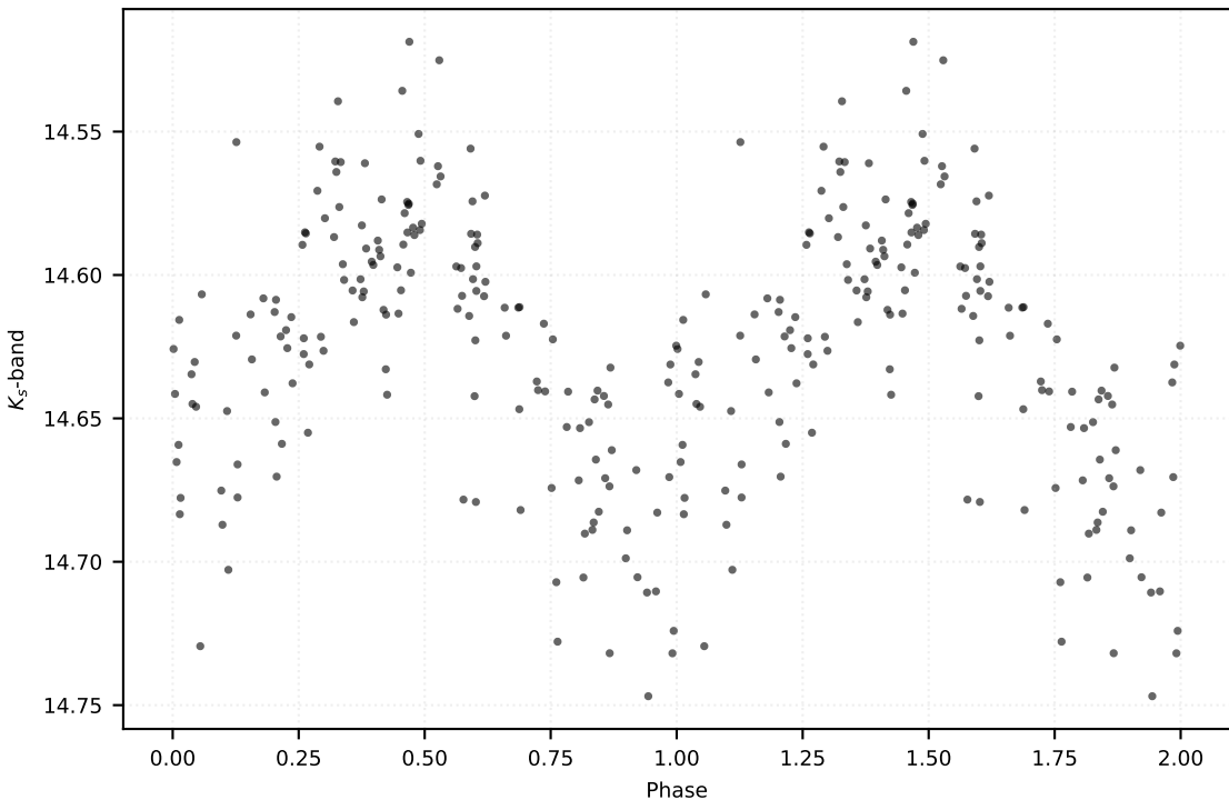
P: 0.47764 d | Class: RP | Subclass: RRab | Field b279
