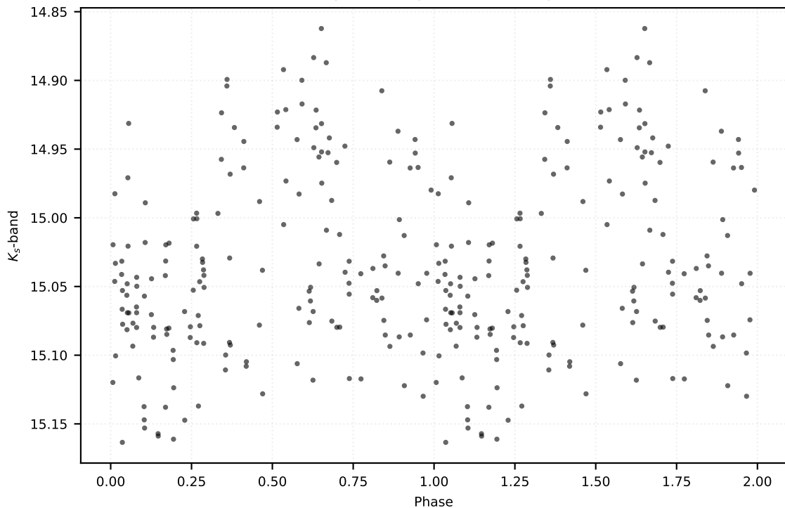
P: 0.49866 d | Class: RP | Subclass: RRab | Field b278
