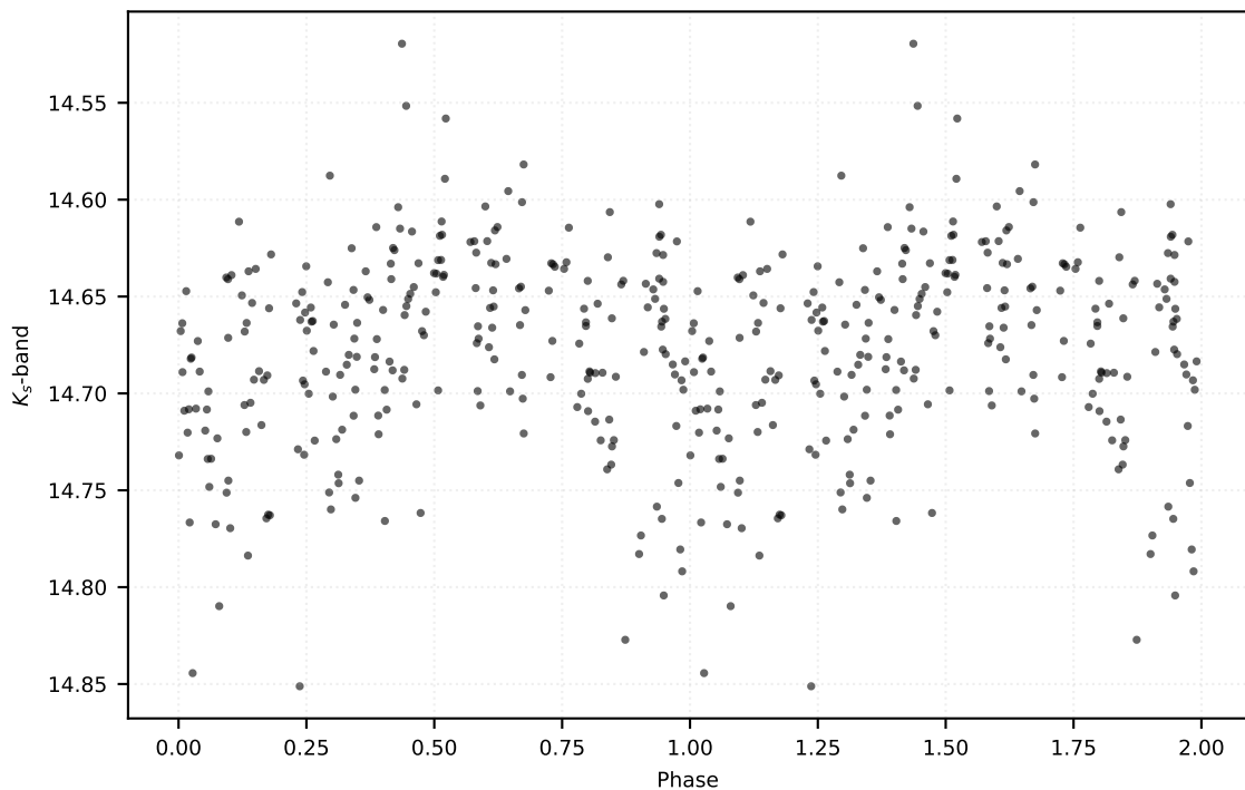
P: 0.11077 d | Class: RP | Subclass: UVAR | Field b279
