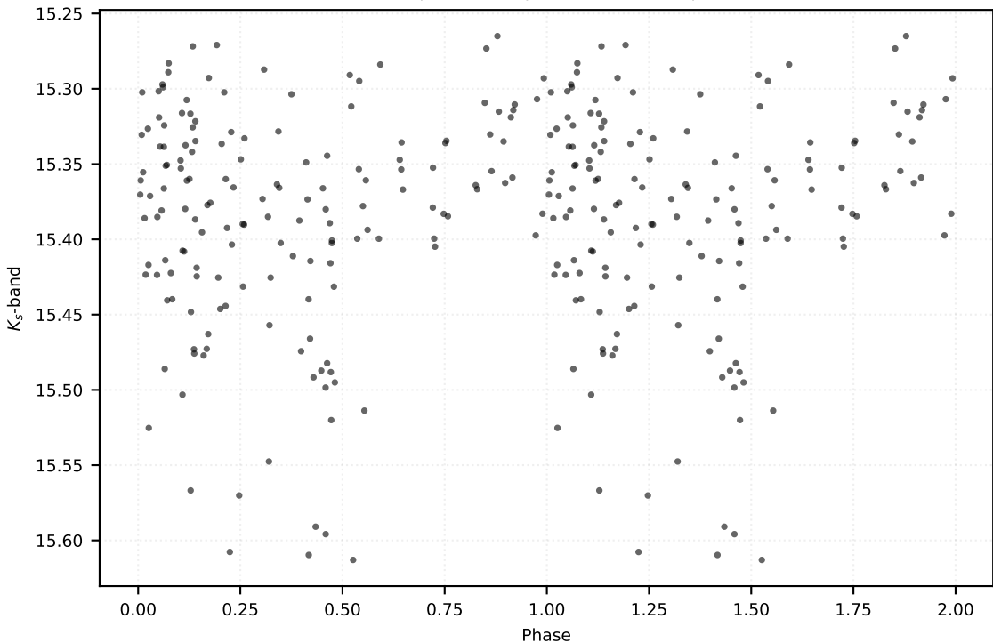
P: 0.17318 d | Class: RP | Subclass: UVAR | Field b278
