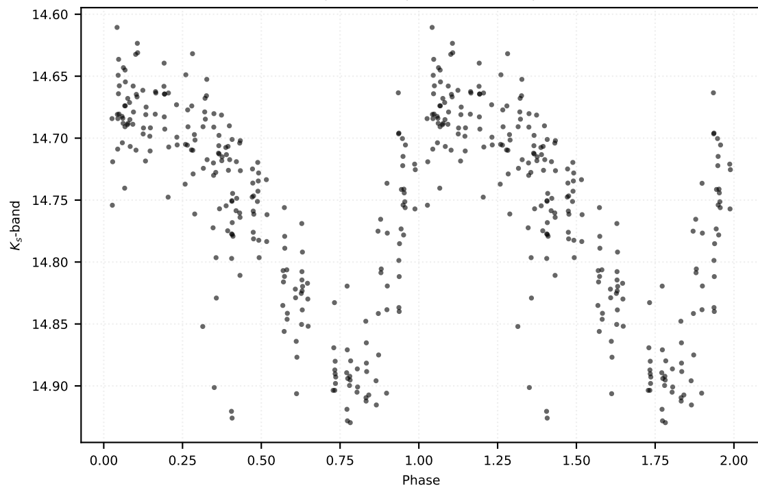
P: 0.45430 d | Class: RP | Subclass: RRab | Field b278
