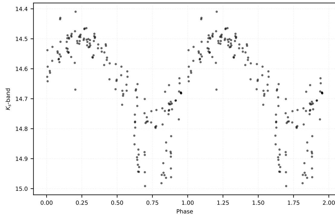
P: 0.57337 d | Class: RP | Subclass: RRab | Field b279
