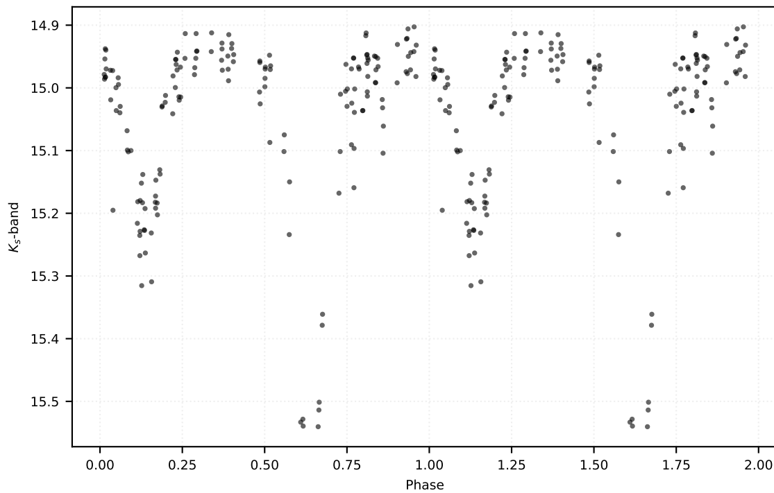
P: 1.21745 d | Class: EB | Subclass: EA | Field b279
