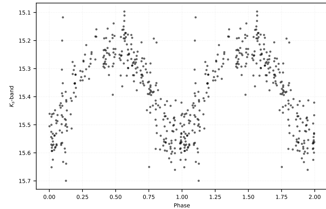
P: 0.63270 d | Class: RP | Subclass: RRab | Field b278
