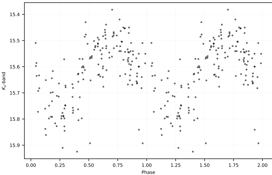
P: 0.11834 d | Class: RP | Subclass: UVAR | Field b279
