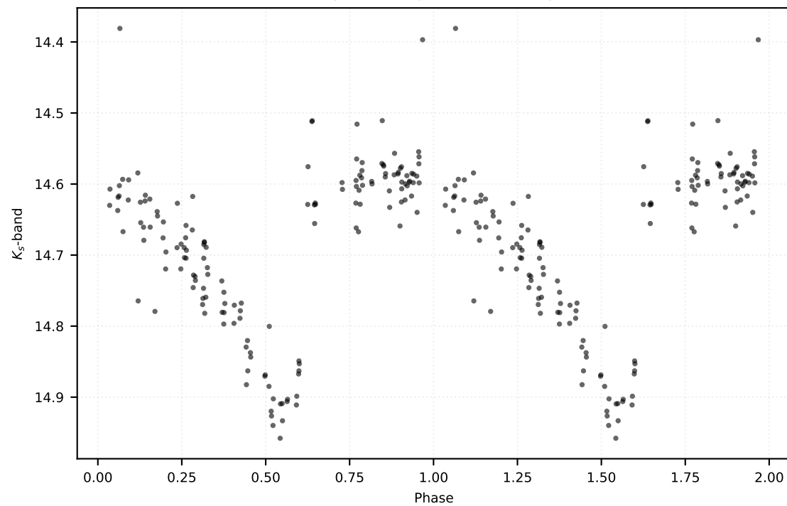
P: 0.53023 d | Class: RP | Subclass: RRab | Field b278
