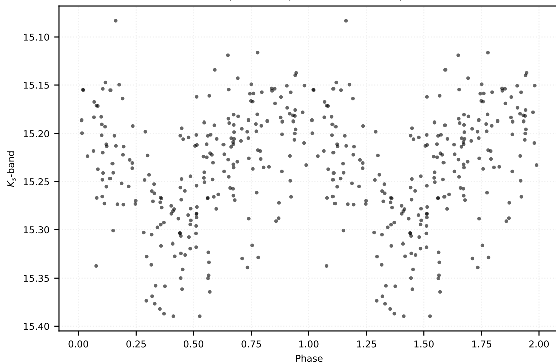
P: 0.25752 d | Class: RP | Subclass: CEP-1OT | Field b279
