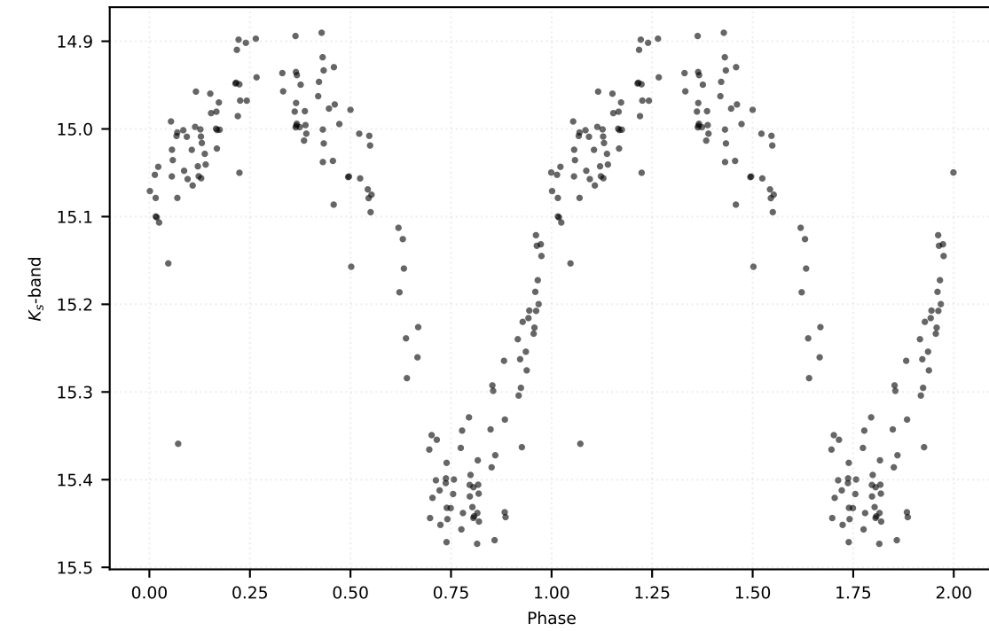
P: 0.19547 d | Class: RP | Subclass: UVAR | Field b278
