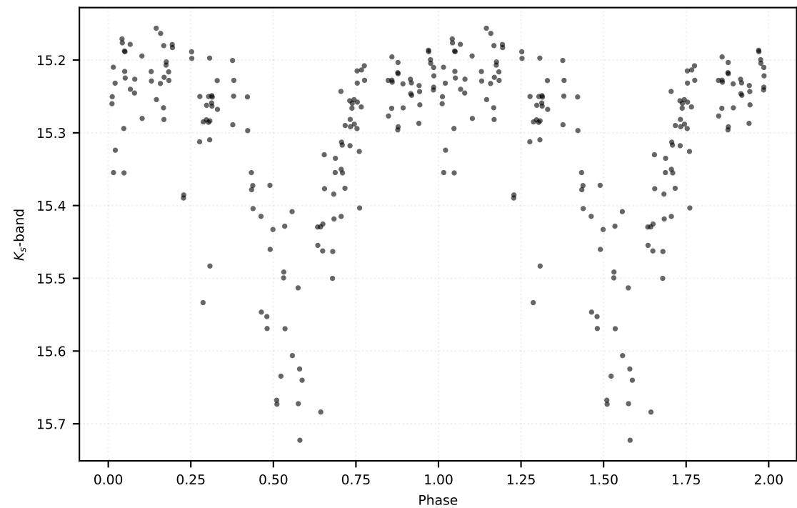
P: 0.43564 d | Class: RP | Subclass: RRc | Field b278
