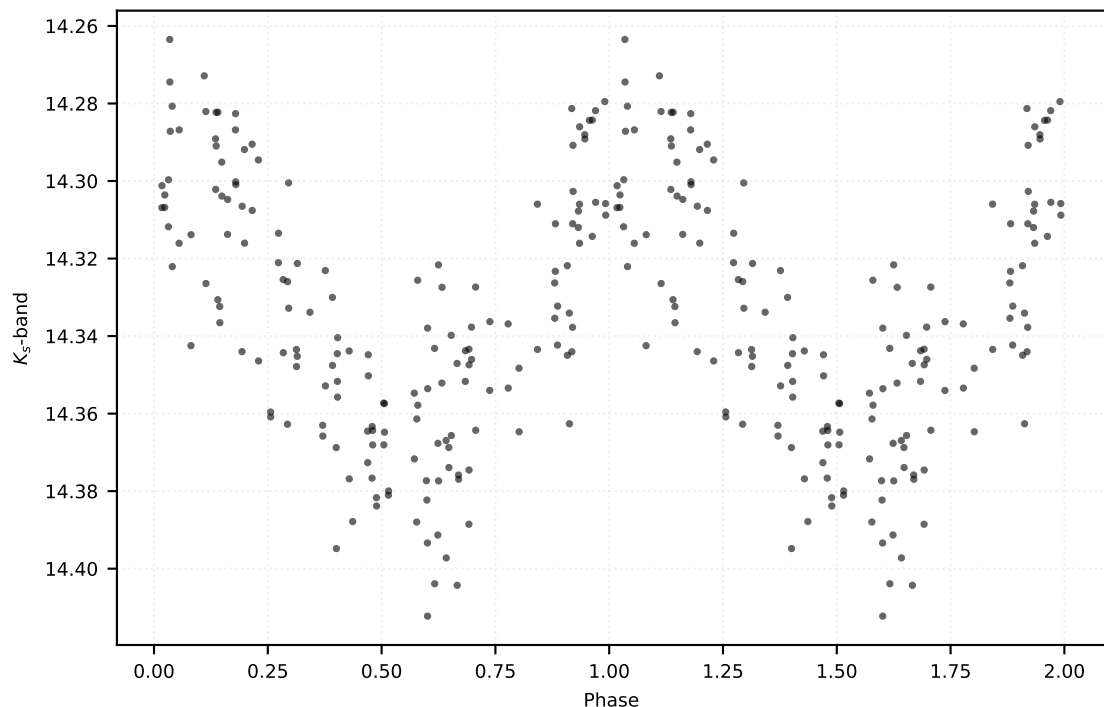
P: 4.50233 d | Class: RP | Subclass: CEP-F | Field b278
