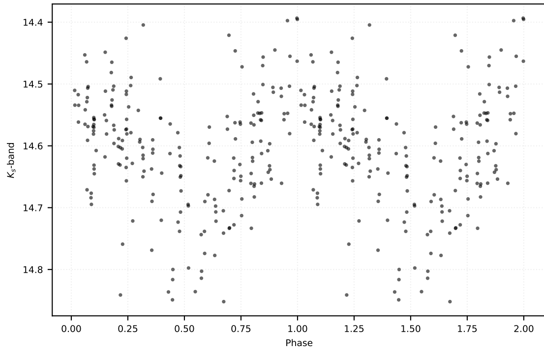
P: 0.44090 d | Class: RP | Subclass: R Rab | Field b278
