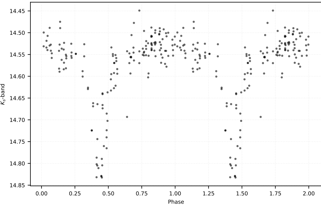
P: 4.85449 d | Class: RP | Subclass: CEP-F | Field b279
