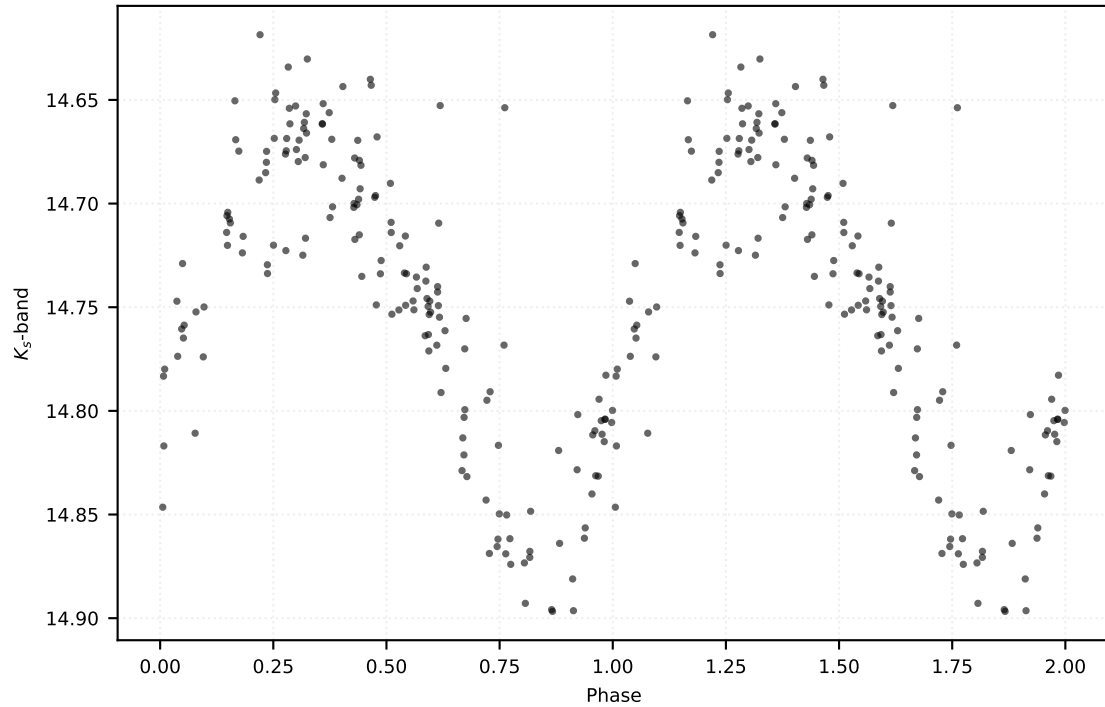
P: 0.18041 d | Class: RP | Subclass: UVAR | Field b278
