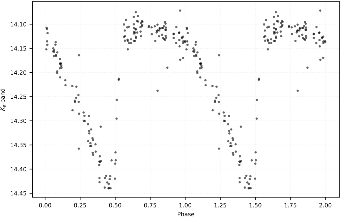
P: 0.61896 d | Class: RP | Subclass: RRab | Field b278
