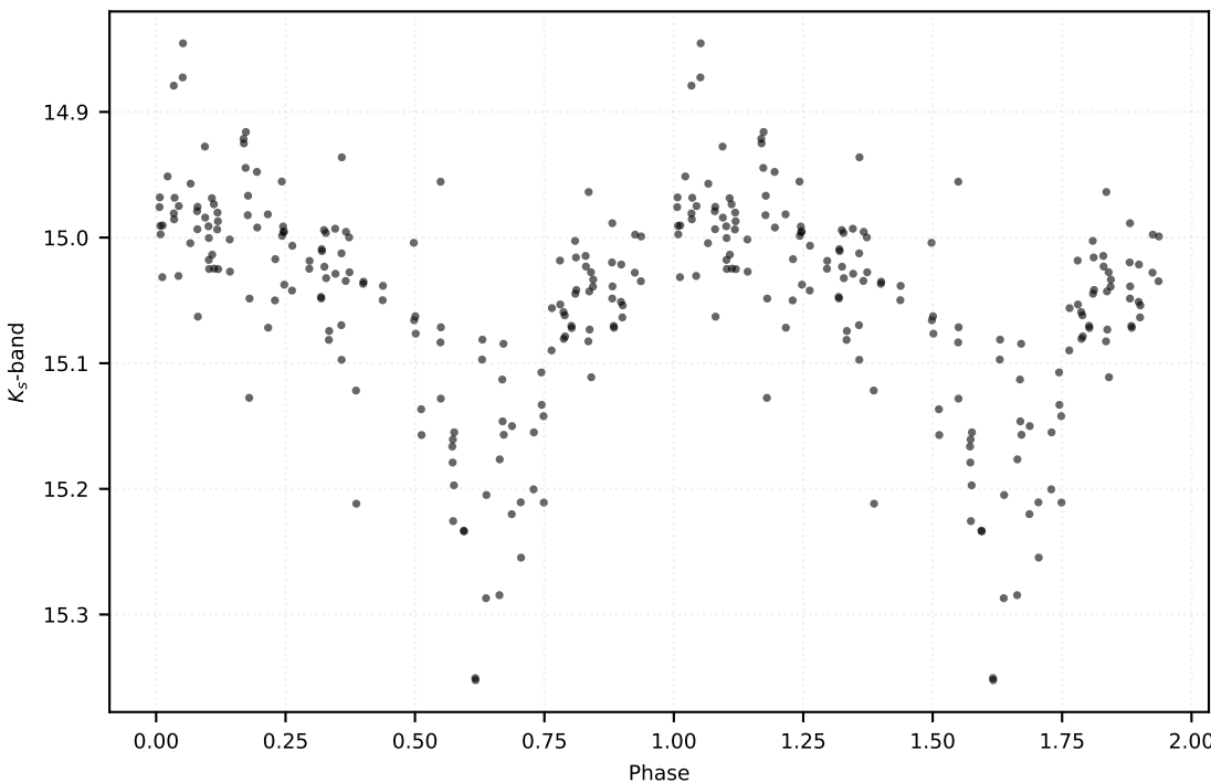
P: 0.25646 d | Class: RP | Subclass: CEP-10T | Field b279
