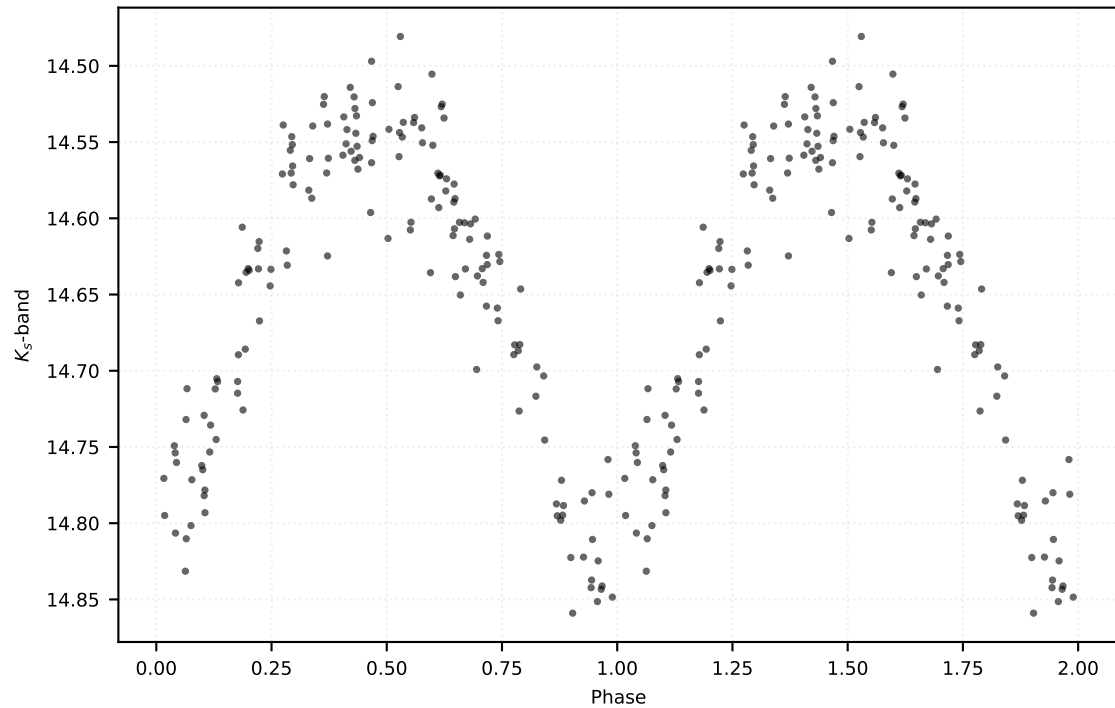
P: 0.20387 d | Class: RP | Subclass: UVAR | Field b279
