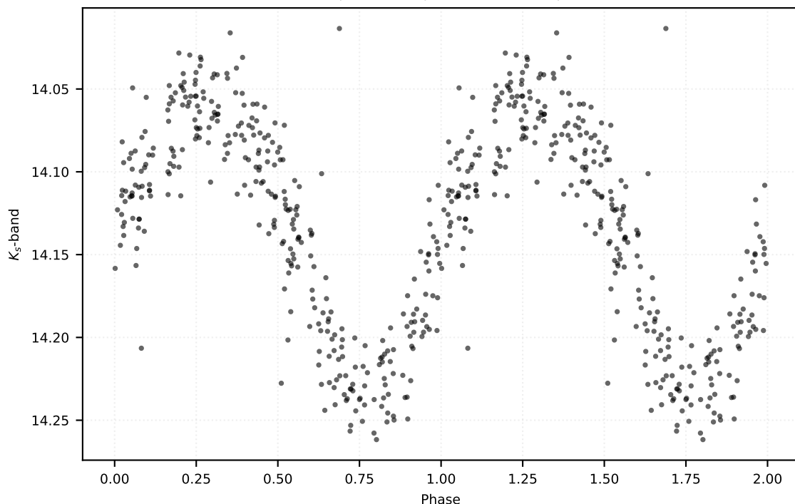
P: 0.19966 d | Class: RP | Subclass: UVAR | Field b278
