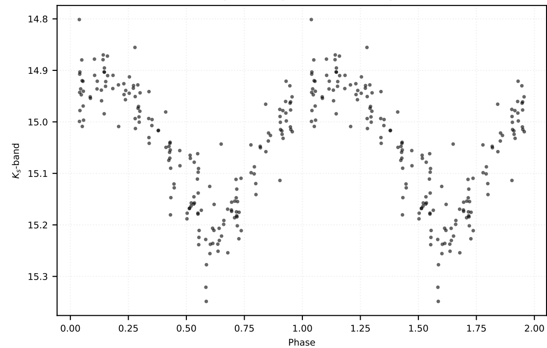
P: 4.97526 d | Class: RP | Subclass: CEP-10T | Field b278
