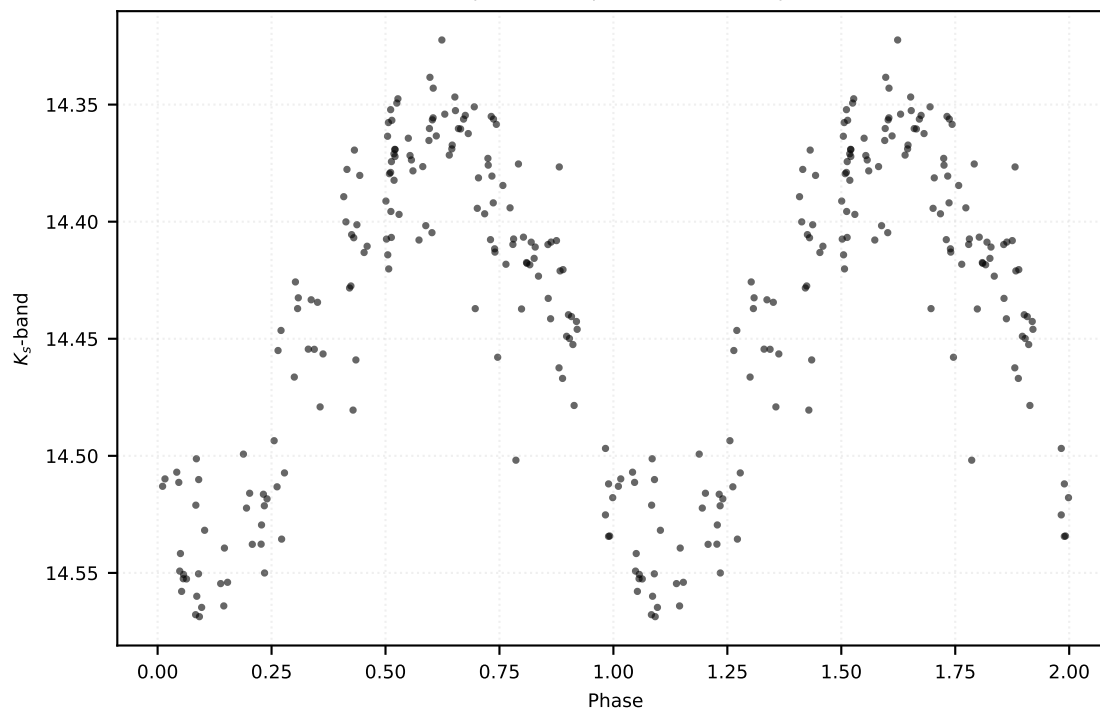
P: 0.21621 d | Class: RP | Subclass: UVAR | Field b278
