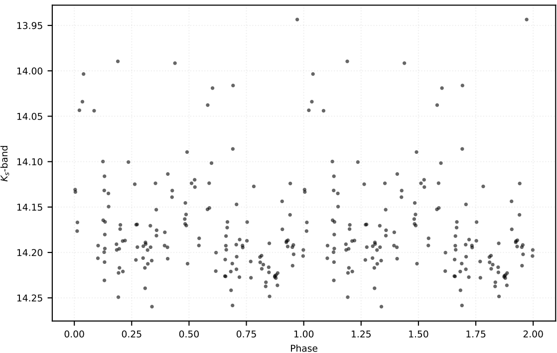
P: 1.75358 d | Class: EB | Subclass: EA | Field b278
