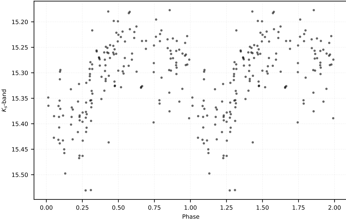
P: 0.39558 d | Class: RP | Subclass: RRab | Field b279
