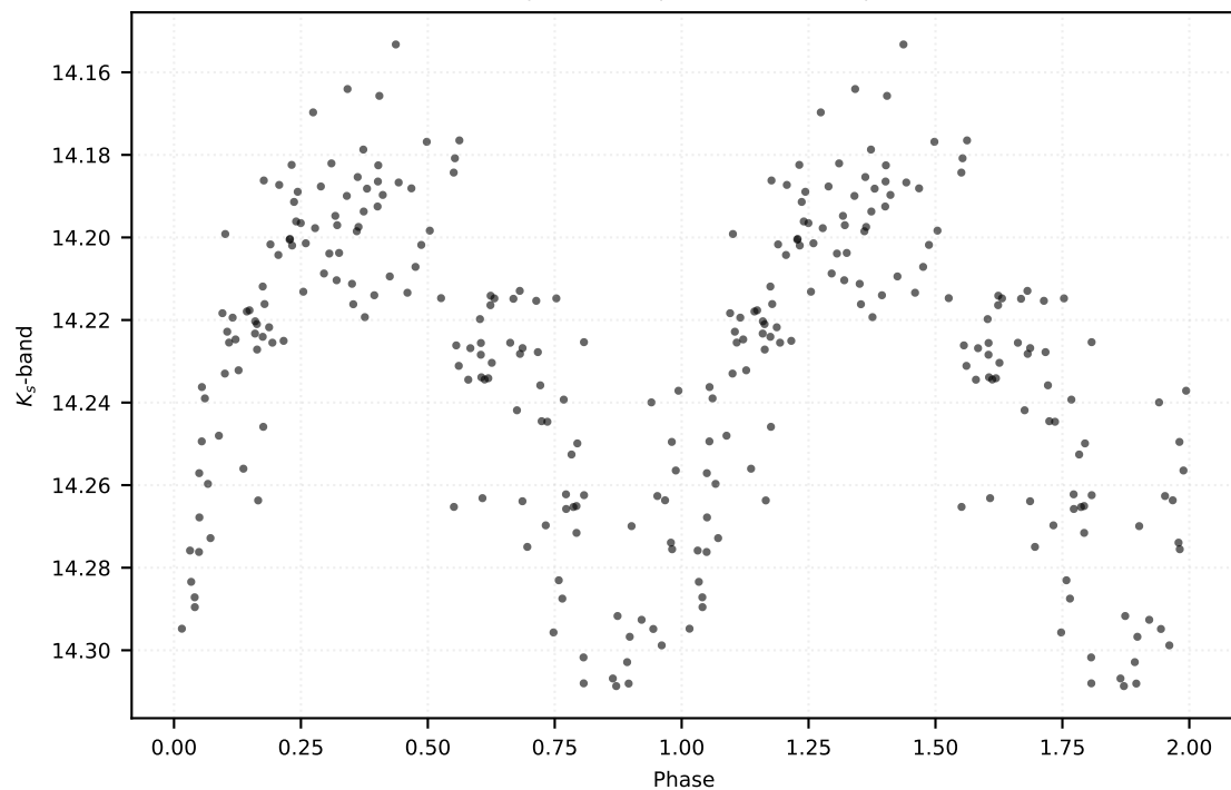
P: 0.64769 d | Class: RP | Subclass: RRab | Field b278
