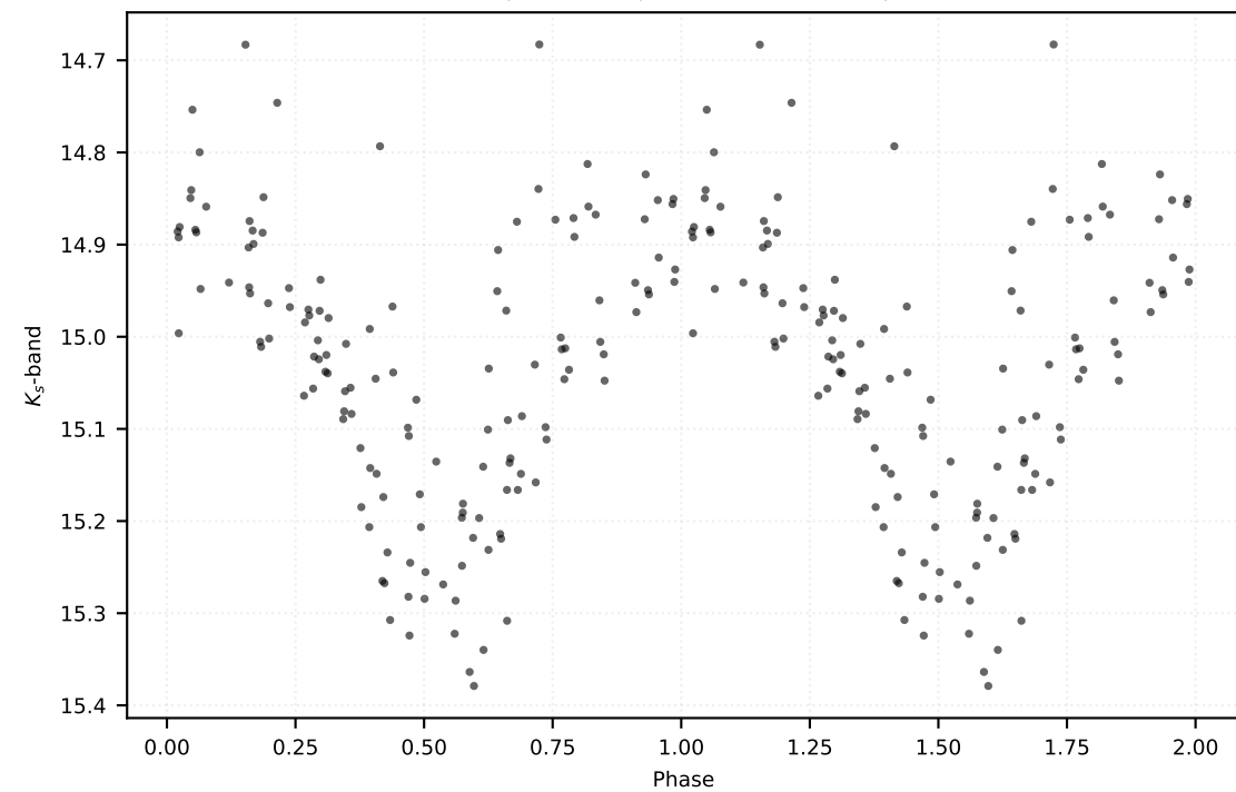
P: 0.32160 d | Class: RP | Subclass: CEP-10T | Field b278
