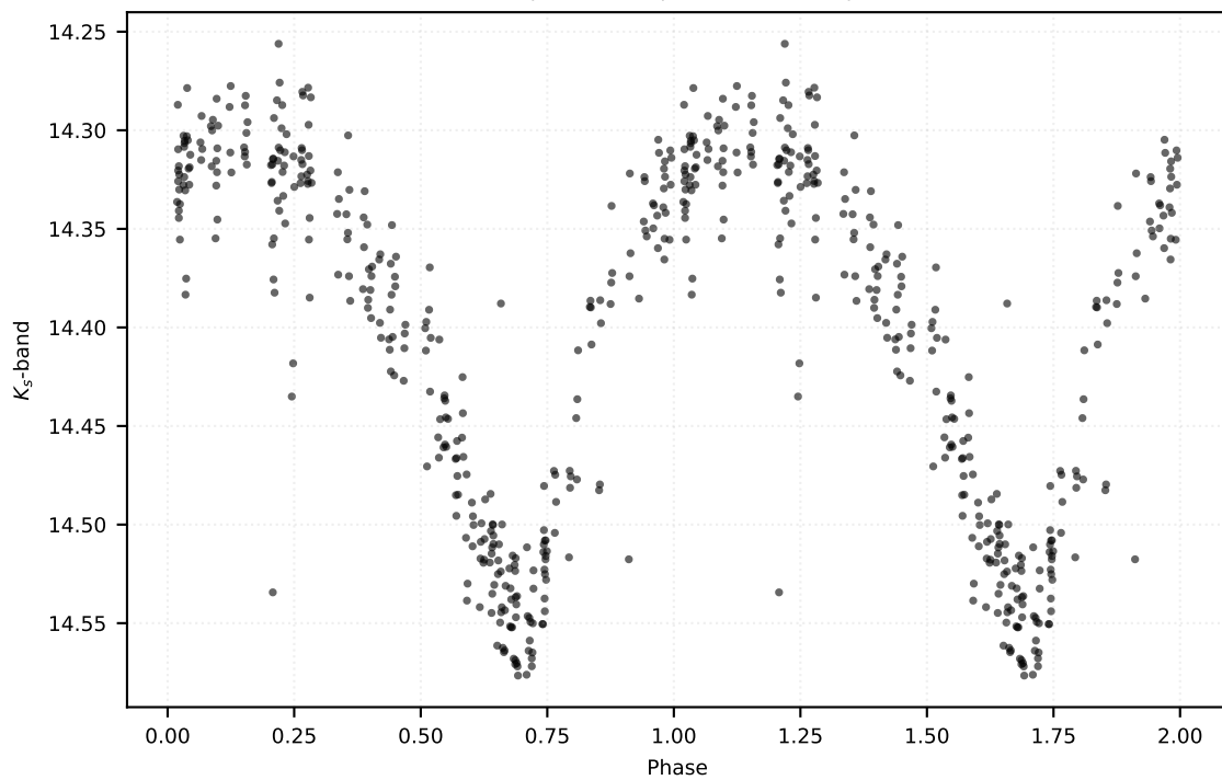
P: 0.43417 d | Class: RP | Subclass: RRc | Field b279
