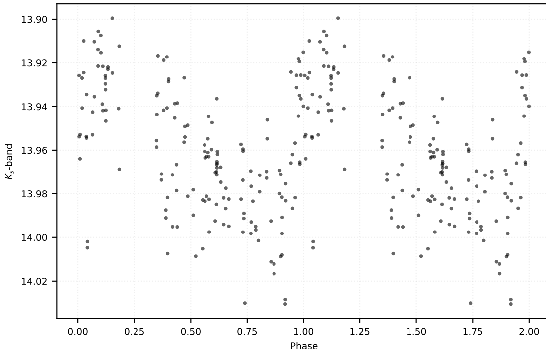
P: 0.99789 d | Class: RP | Subclass: RRab | Field b278
