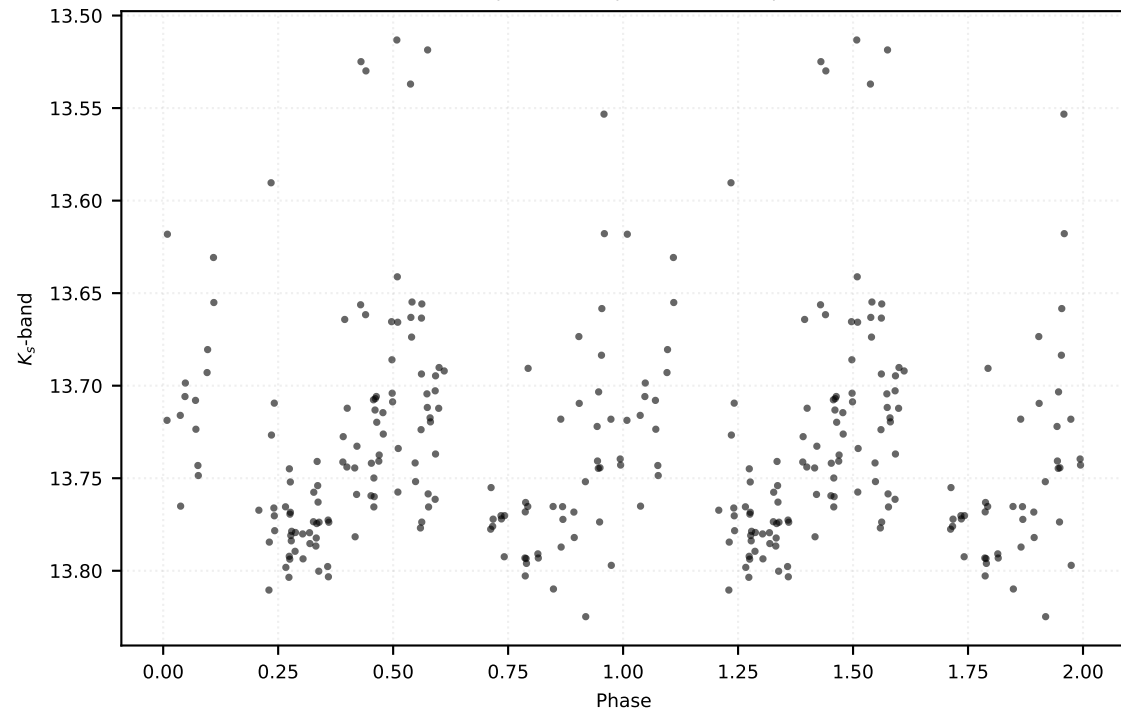
P: 0.31121 d | Class: EB | Subclass: EA | Field b279
