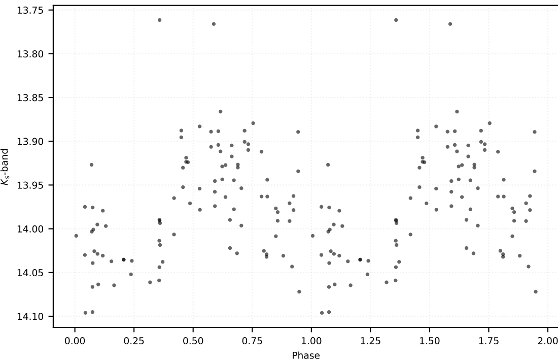
P: 0.99719 d | Class: RP | Subclass: CEP-1OT | Field b278
