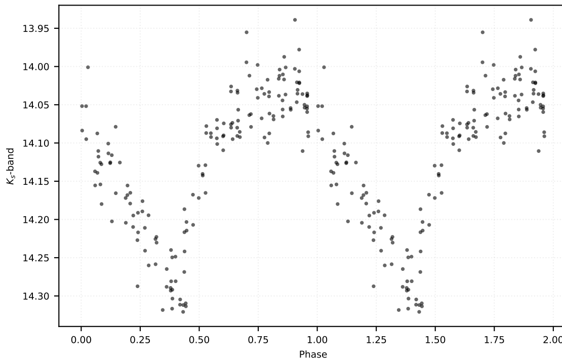
P: 0.59858 d | Class: RP | Subclass: RRab | Field b279
