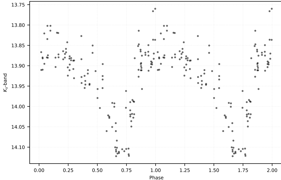
P: 0.71350 d | Class: RP | Subclass: RRab | Field b278
