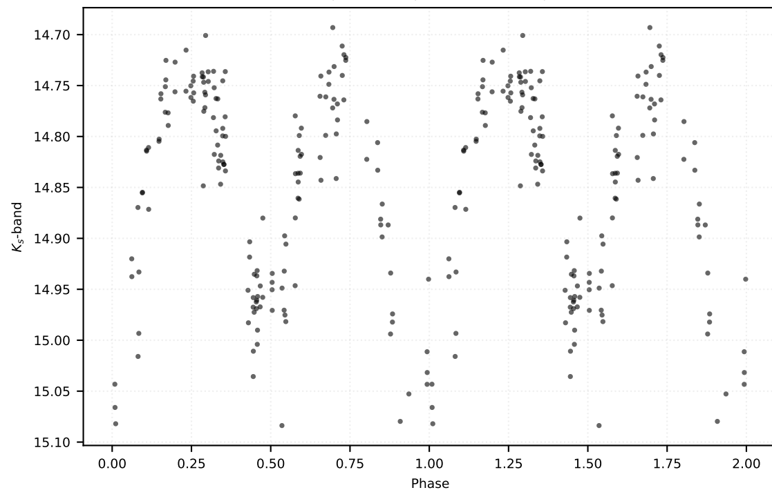
P: 1.12533 d | Class: EB | Subclass: UVAR | Field b279
