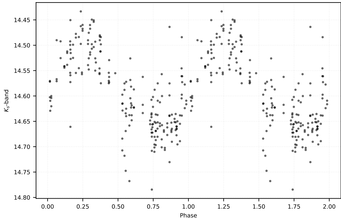
P: 0.37174 d | Class: RP | Subclass: CEP-10T | Field b279
