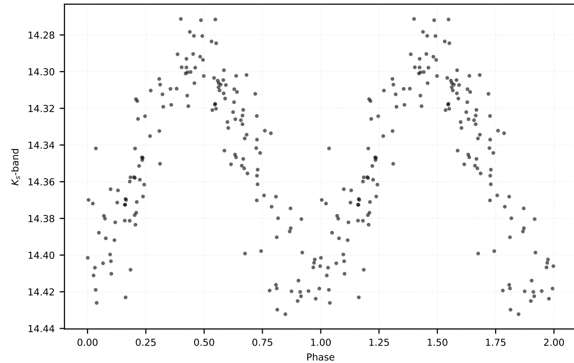
P: 0.16894 d | Class: RP | Subclass: UVAR | Field b279
