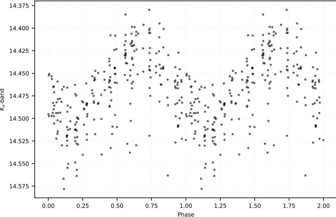
P: 0.33036 d | Class: RP | Subclass: RRc | Field b279
