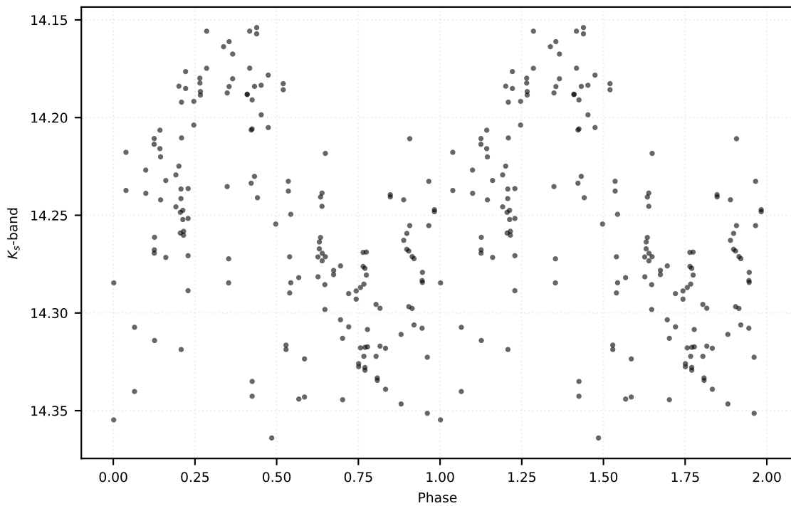
P: 0.75808 d | Class: RP | Subclass: CEP-10T | Field b278
