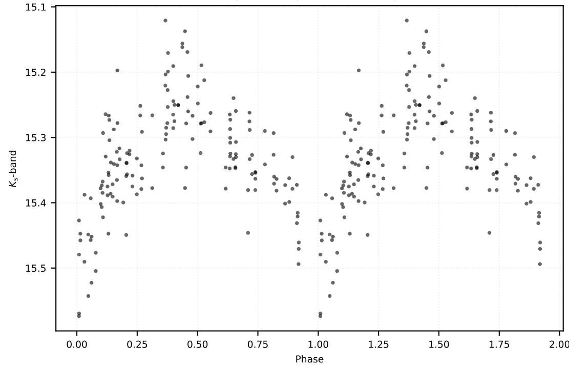
P: 8.92350 d | Class: RP | Subclass: CEP-F | Field b279
