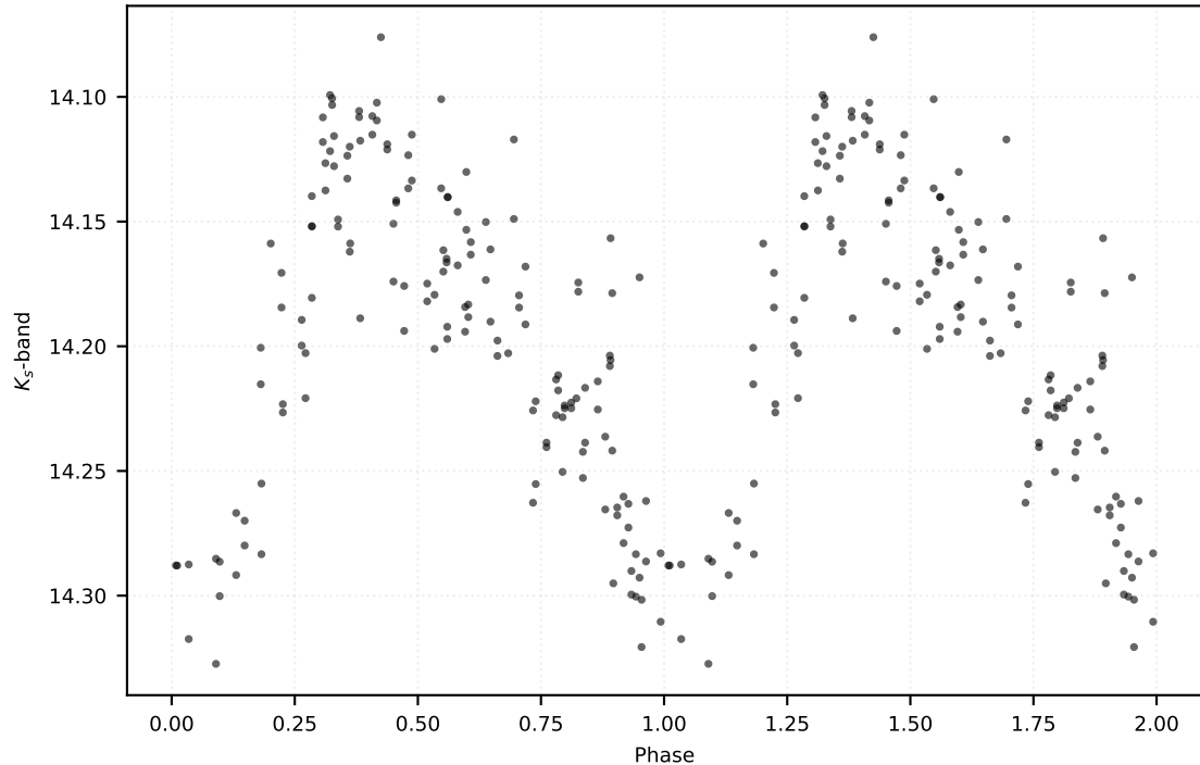
P: 0.74502 d | Class: RP | Subclass: CEP-10T | Field b278
