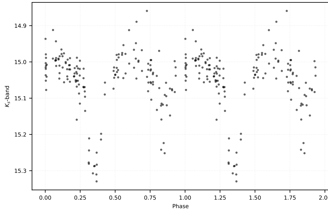
P: 0.89979 d | Class: EB | Subclass: EA | Field b279
