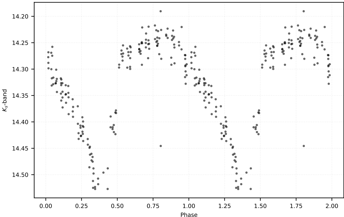
P: 0.99661 d | Class: RP | Subclass: CEP-1OT | Field b278
