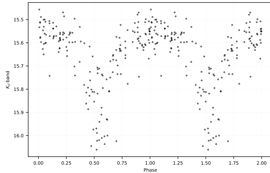
P: 0.48269 d | Class: RP | Subclass: RRab | Field b278
