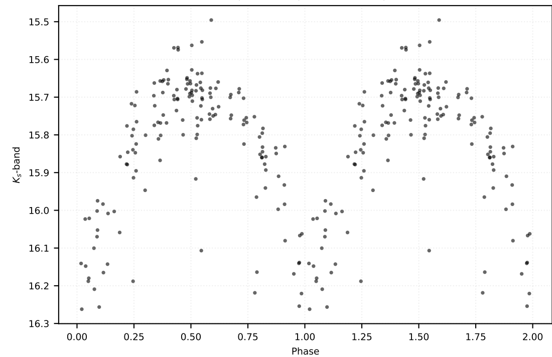
P: 0.52108 d | Class: RP | Subclass: RRc | Field b279
