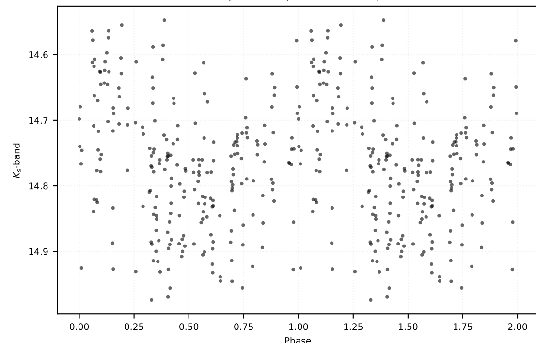
P: 0.20615 d | Class: RP | Subclass: UVAR | Field b278
