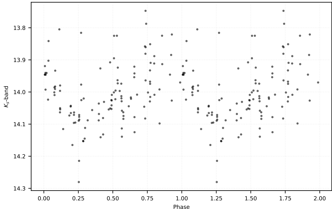
P: 0.48969 d | Class: RP | Subclass: CEP-10T | Field b278
