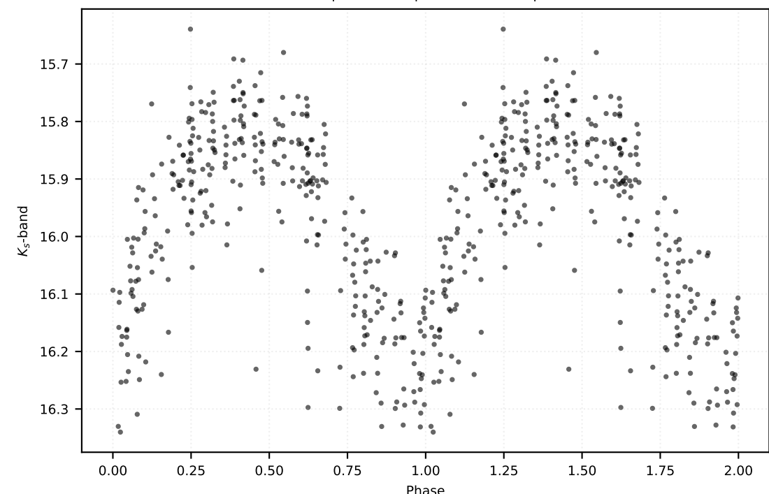
P: 0.50203 d | Class: RP | Subclass: RRc | Field b279
