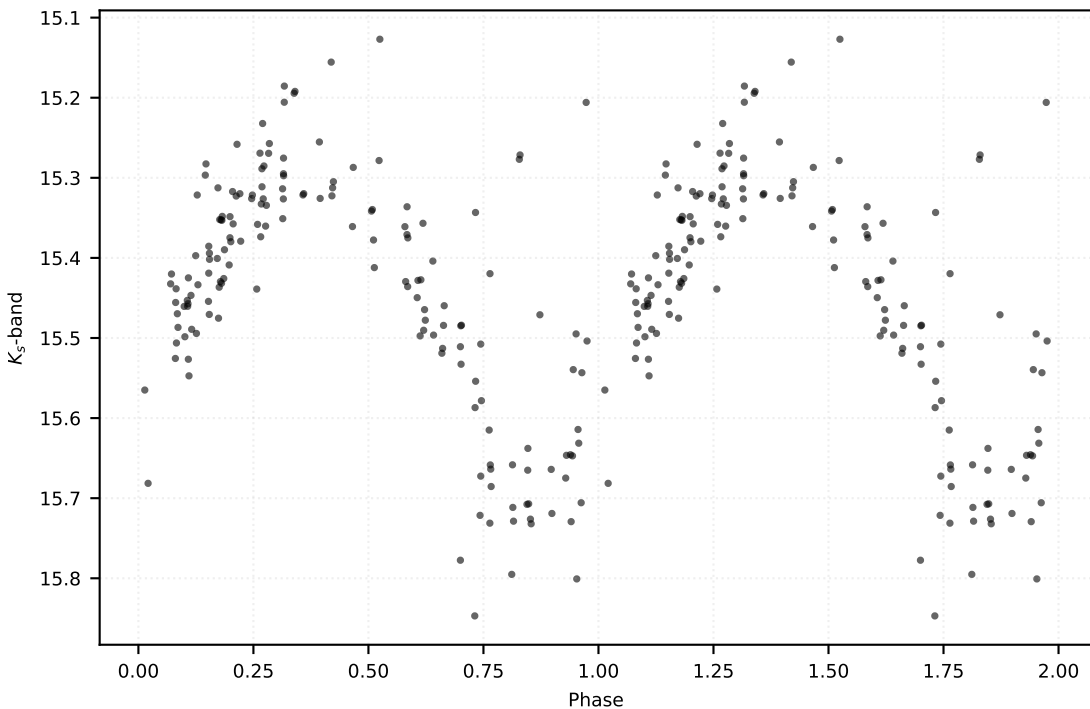
P: 4.45082 d | Class: RP | Subclass: CEP-10T | Field b278
