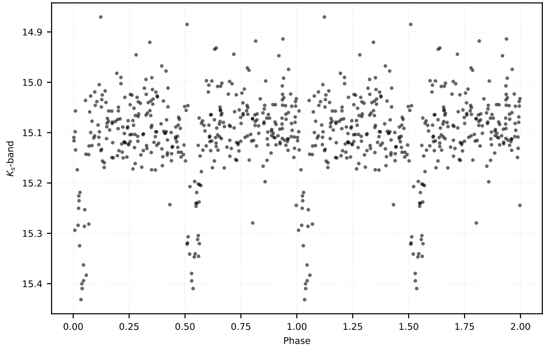
P: 0.69620 d | Class: EB | Subclass: EA | Field b279
