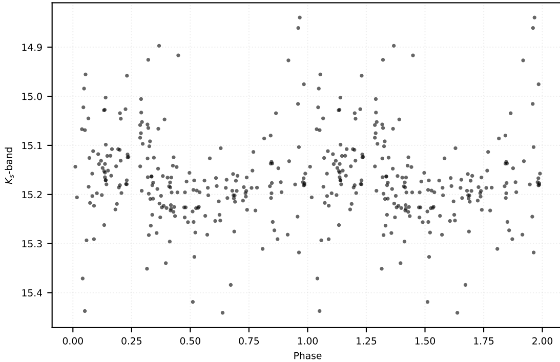
P: 0.21140 d | Class: RP | Subclass: UVAR | Field b278
