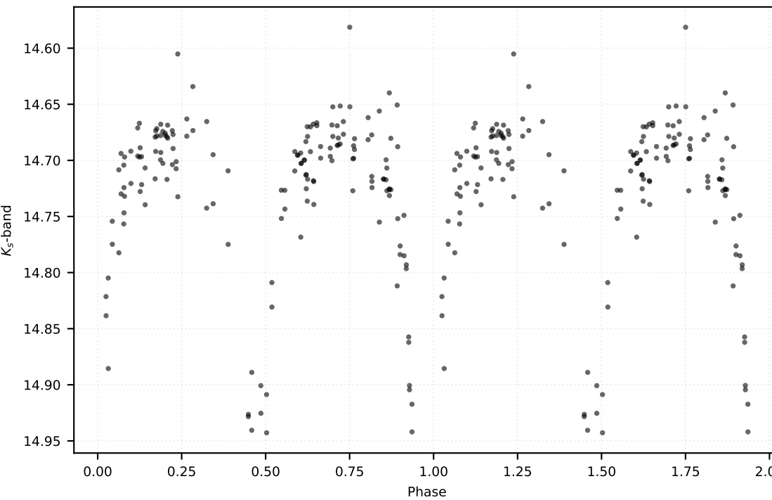
P: 0.22055 d | Class: EB | Subclass: EA | Field b279
