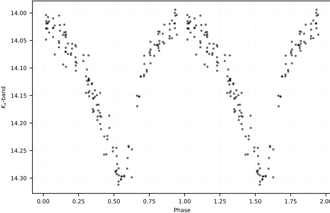
P: 0.73516 d | Class: RP | Subclass: CEP-10T | Field b278
