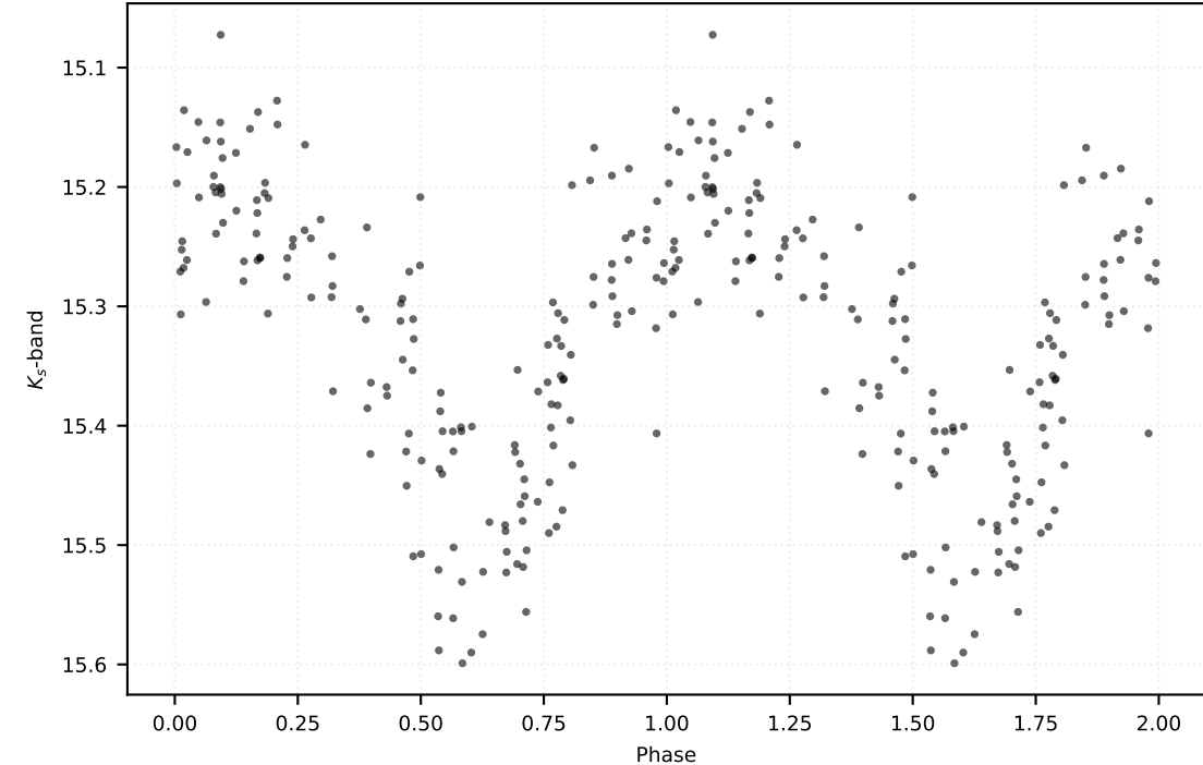
P: 0.42483 d | Class: RP | Subclass: CEP-10T | Field b278
