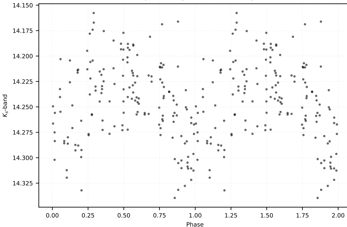
P: 0.30212 d | Class: RP | Subclass: CEP-1OT | Field b279
