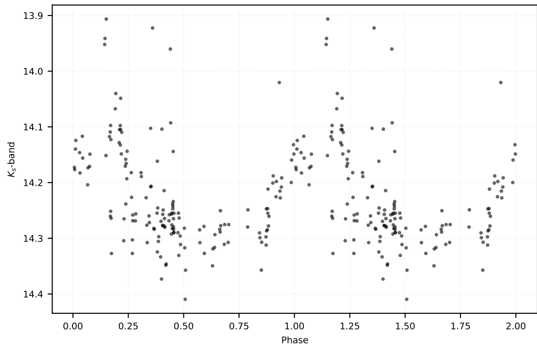
P: 0.13020 d | Class: RP | Subclass: UVAR | Field b278
