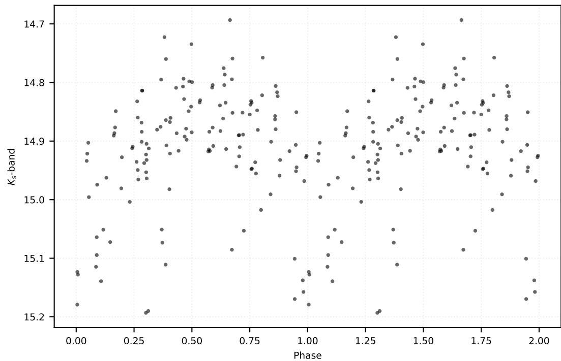
P: 0.11081 d | Class: RP | Subclass: UVAR | Field b278
