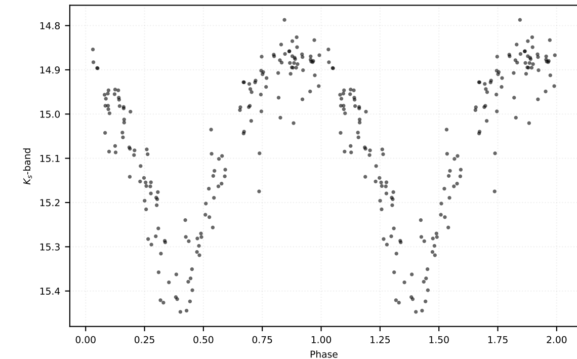
P: 0.16299 d | Class: RP | Subclass: UVAR | Field b279
