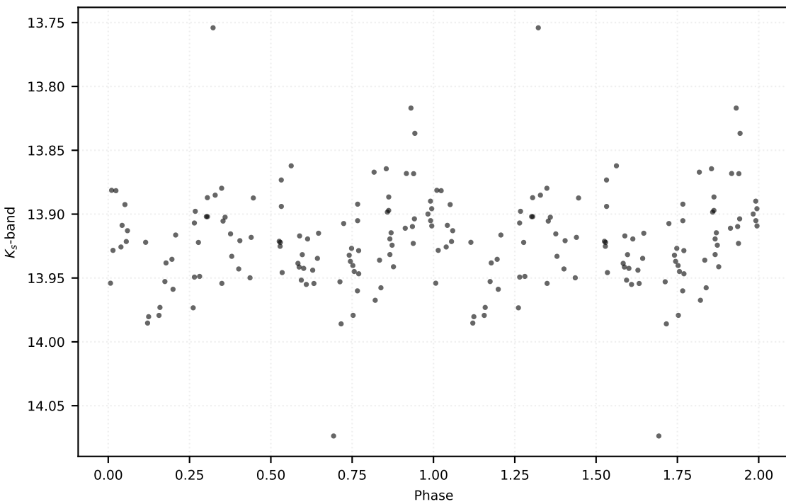
P: 0.37502 d | Class: EB | Subclass: EA | Field b279
