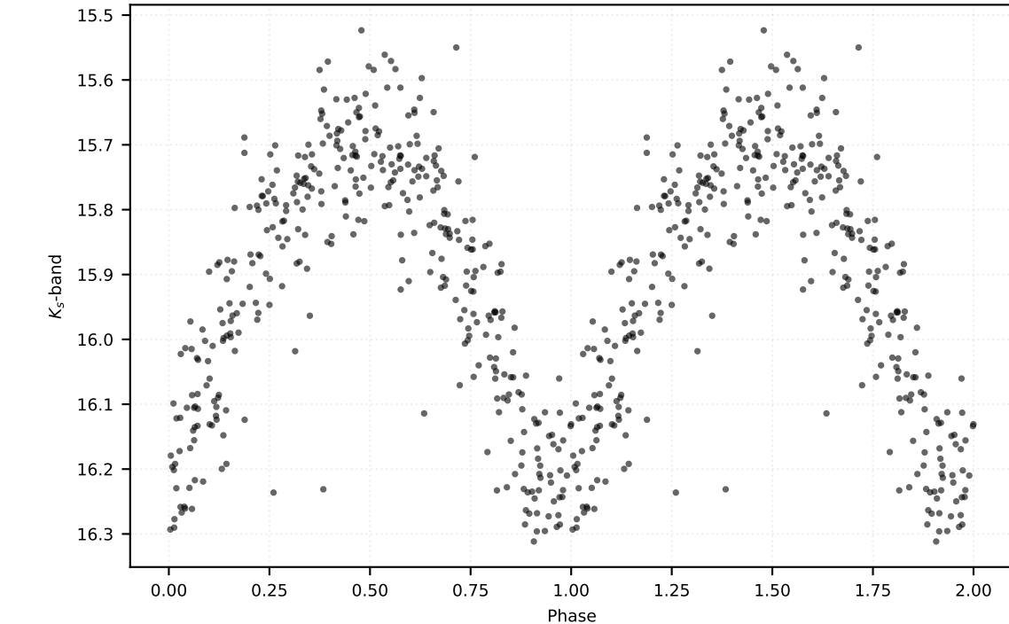
P: 0.60396 d | Class: RP | Subclass: RRab | Field b279
