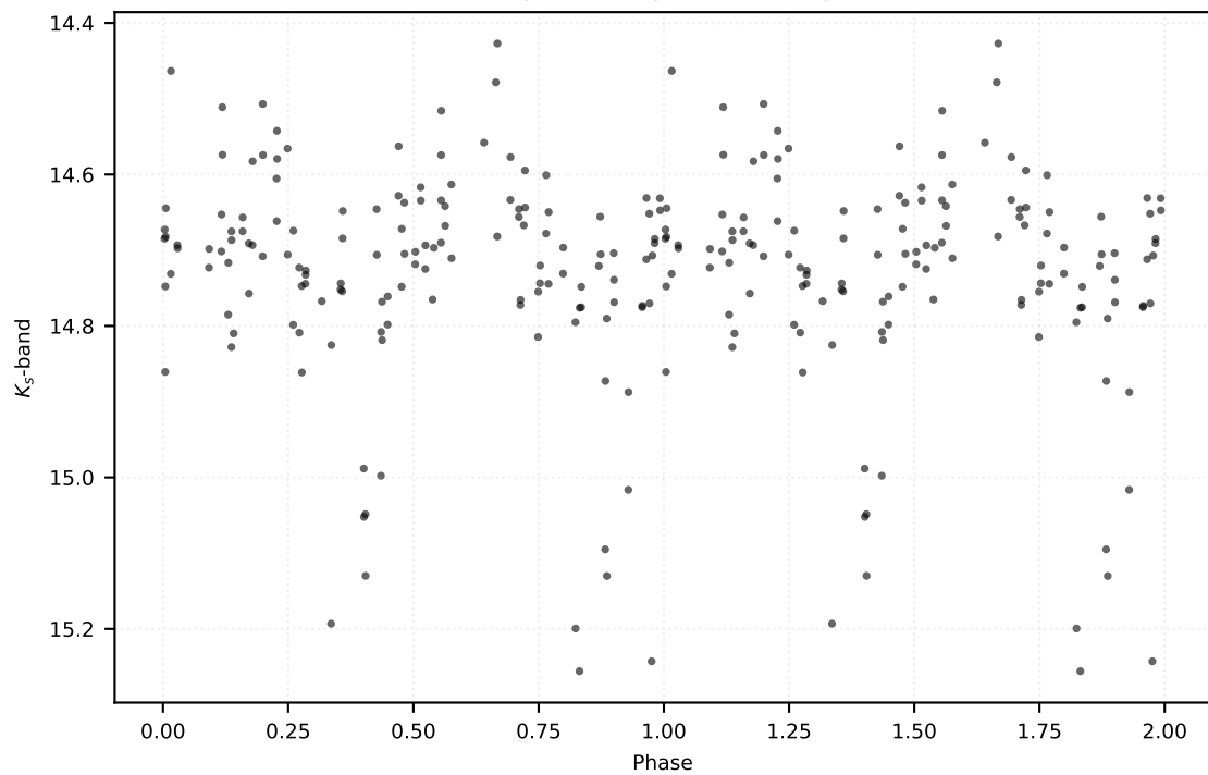
P: 0.87257 d | Class: EB | Subclass: EA | Field b278
