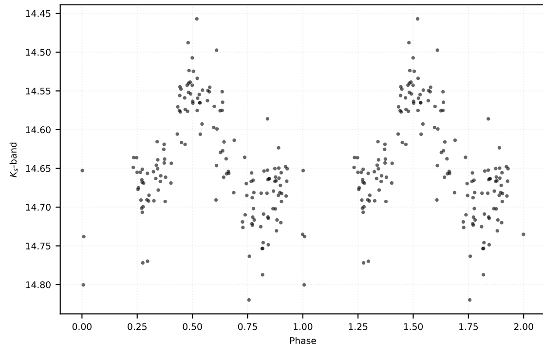
P: 33.35930 d | Class: RP | Subclass: UVAR | Field b279
