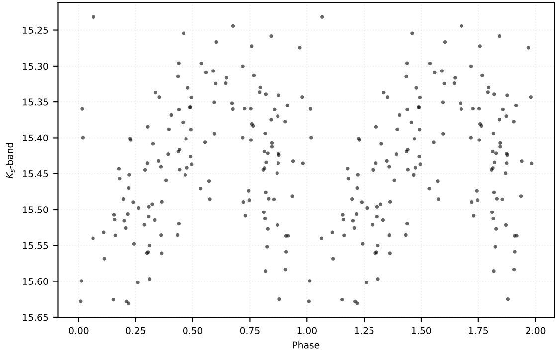
P: 0.15123 d | Class: RP | Subclass: UVAR | Field b278
