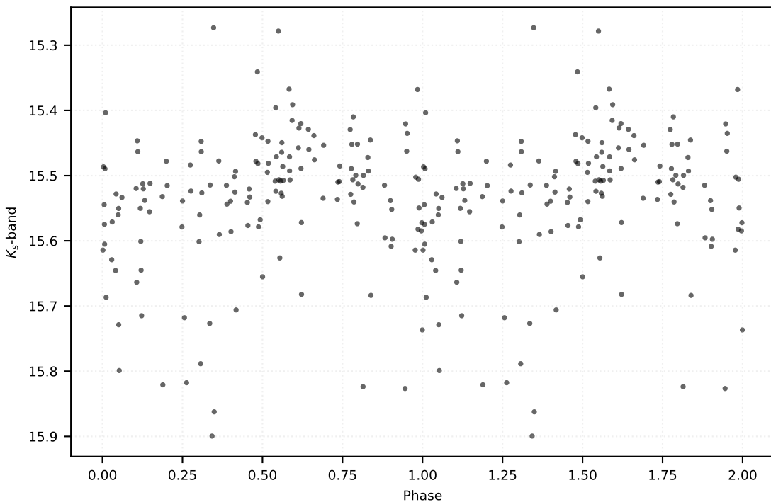
P: 3.15983 d | Class: RP | Subclass: CEP-10T | Field b278
