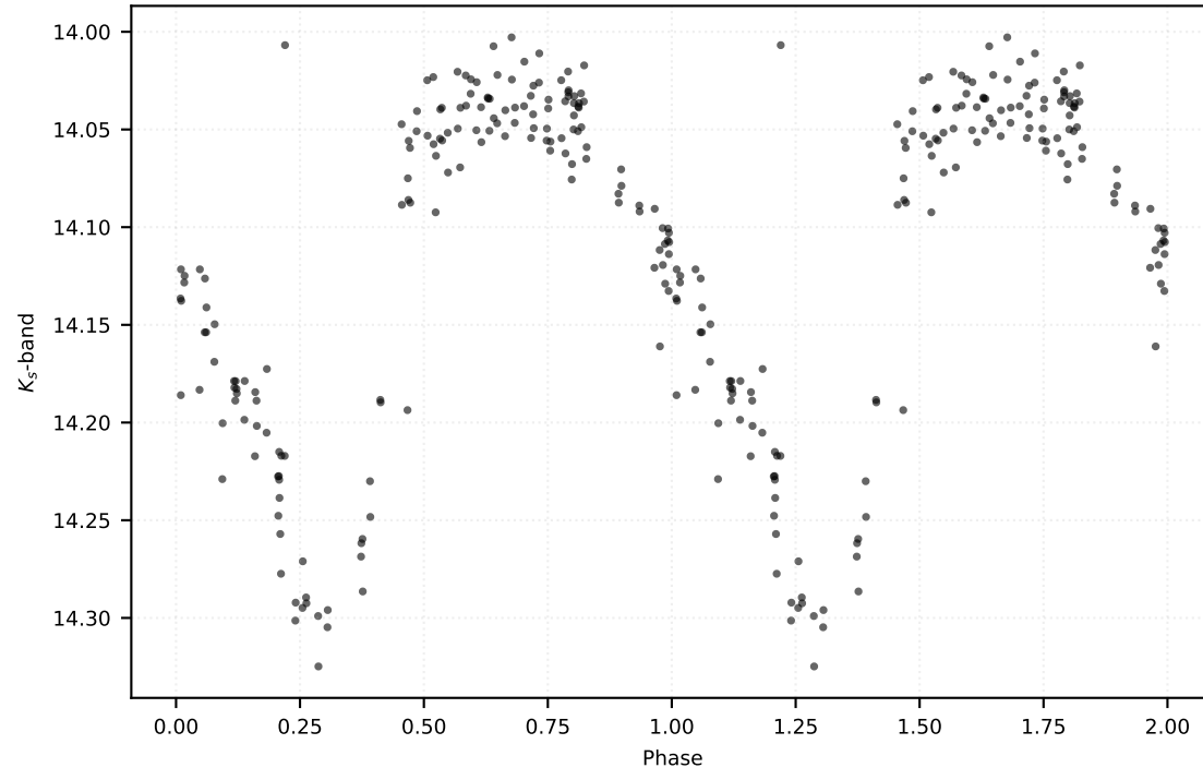
P: 0.57765 d | Class: RP | Subclass: RRab | Field b278
