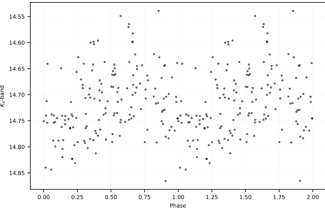
P: 0.23165 d | Class: RP | Subclass: UVAR | Field b278
