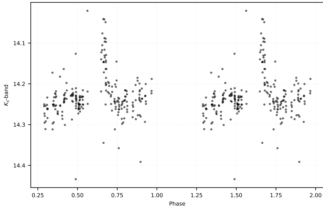
P: 0.51011 d | Class: EB | Subclass: EA | Field b279
