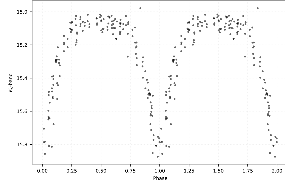
P: 0.47402 d | Class: RP | Subclass: RRab | Field b278
