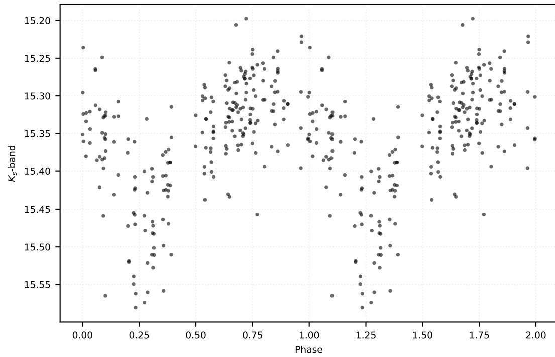
P: 1.02602 d | Class: RP | Subclass: CEP-F | Field b279
