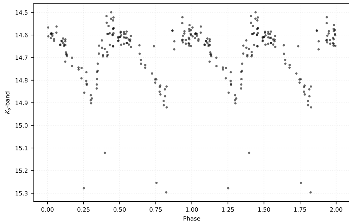
P: 5.39241 d | Class: EB | Subclass: EA | Field b278
