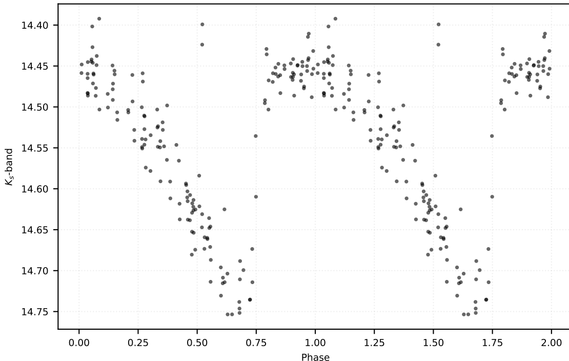
P: 0.58665 d | Class: RP | Subclass: RRab | Field b278
