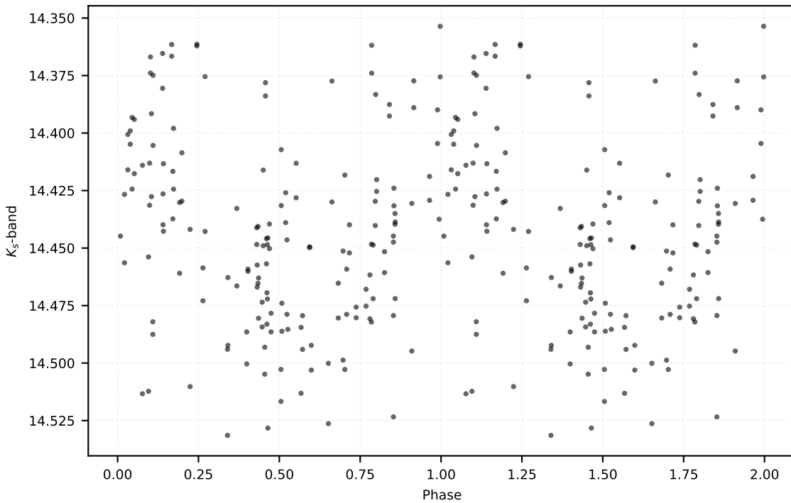
P: 0.12465 d | Class: RP | Subclass: UVAR | Field b279
