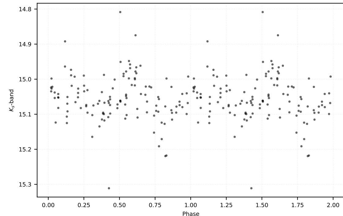
P: 0.20548 d | Class: EB | Subclass: EA | Field b279
