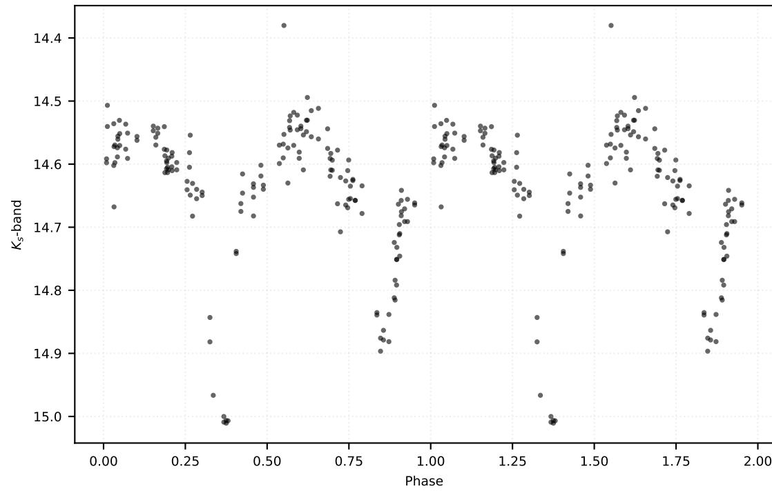
P: 7.01711 d | Class: EB | Subclass: EA | Field b278
