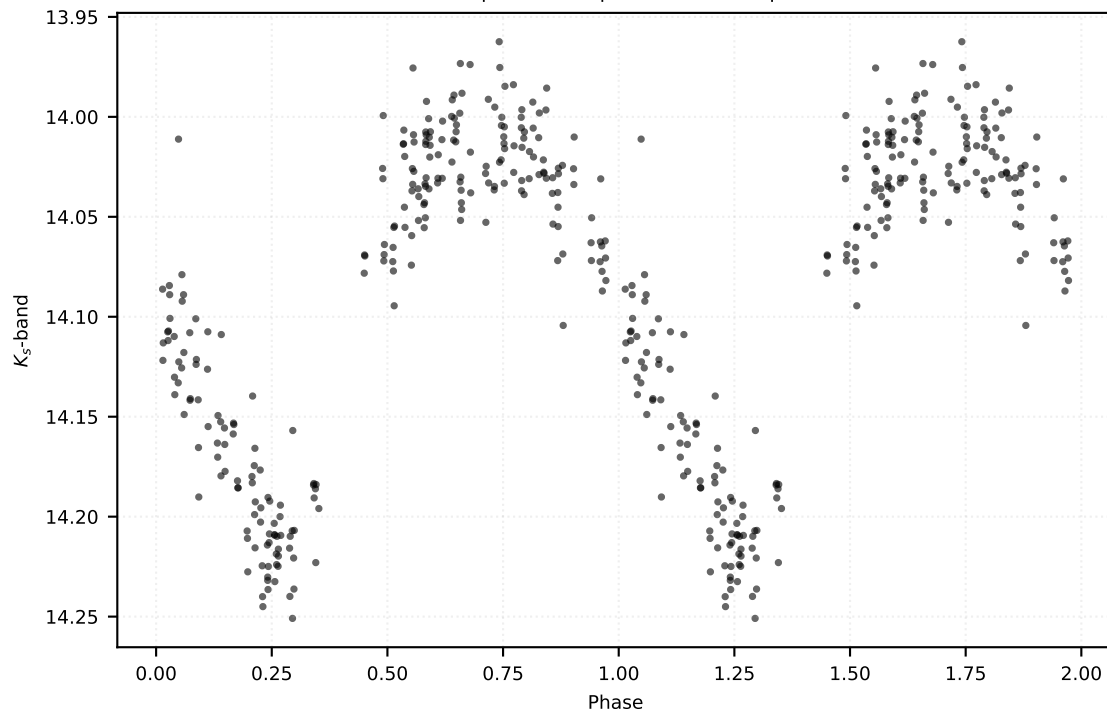
P: 0.45696 d | Class: RP | Subclass: RRc | Field b278
