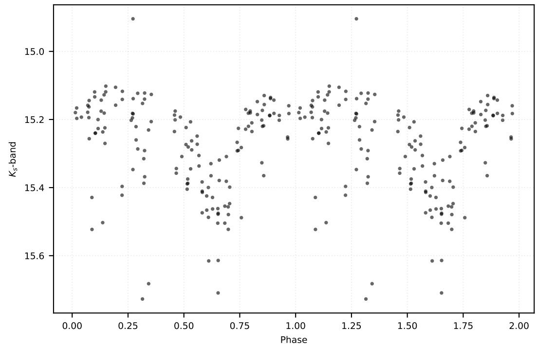
P: 2.05180 d | Class: RP | Subclass: CEP-10T | Field b279
