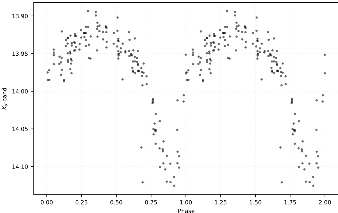
P: 1.05838 d | Class: RP | Subclass: CEP-1OT | Field b278
