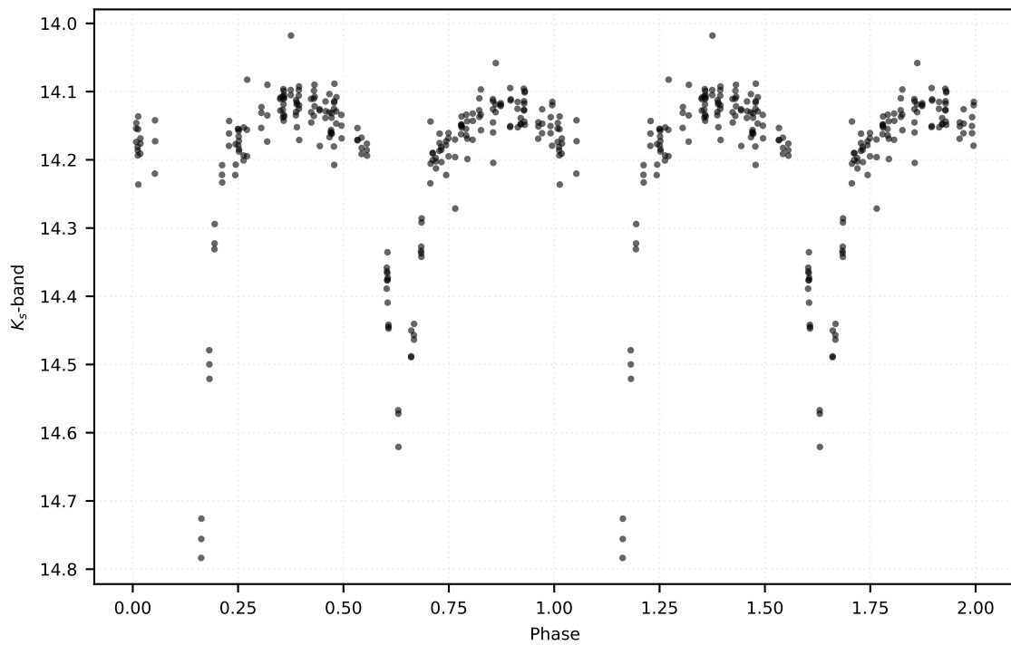
P: 2.23586 d | Class: EB | Subclass: EA | Field b279
