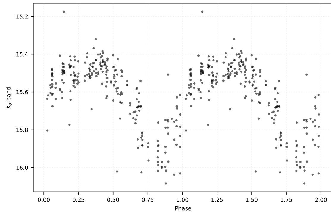
P: 0.44221 d | Class: RP | Subclass: RRc | Field b278
