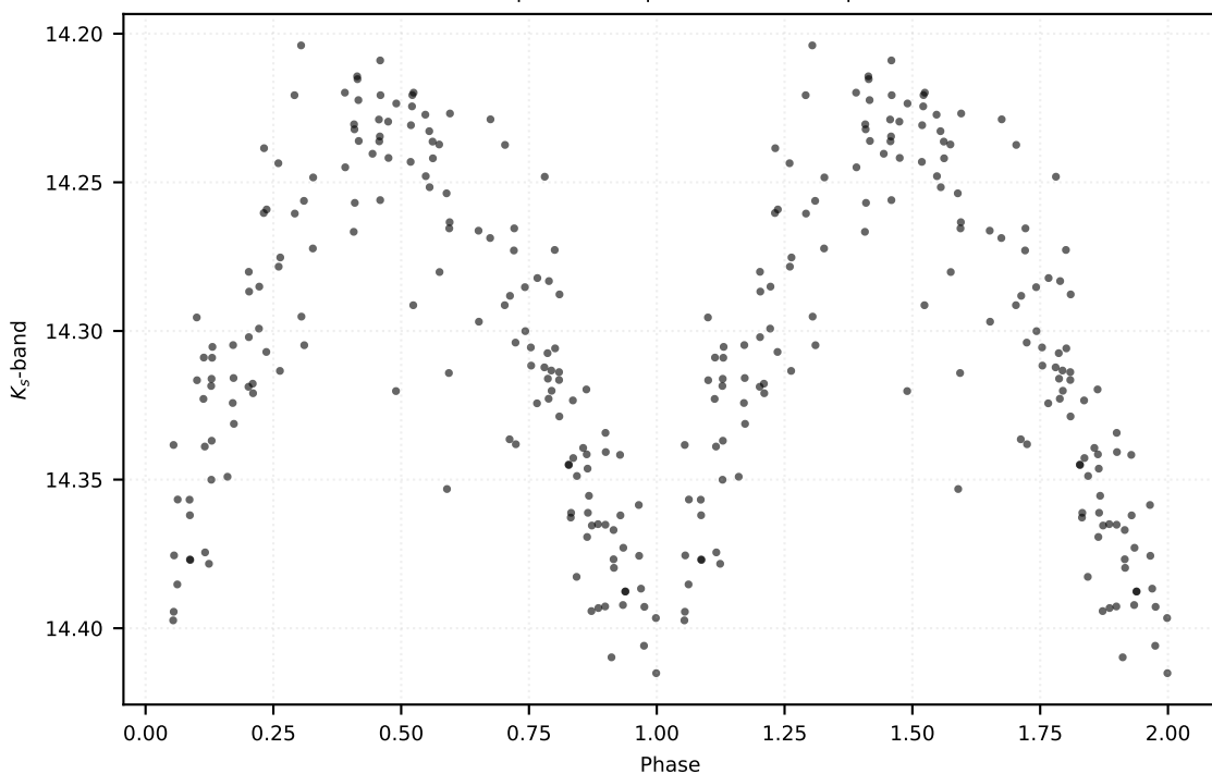
P: 0.47396 d | Class: RP | Subclass: RRab | Field b278
