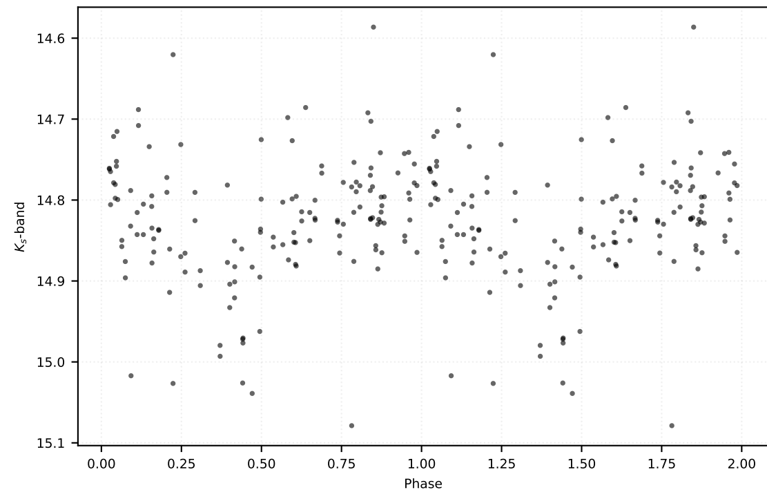
P: 2.49812 d | Class: RP | Subclass: CEP-10T | Field b278
