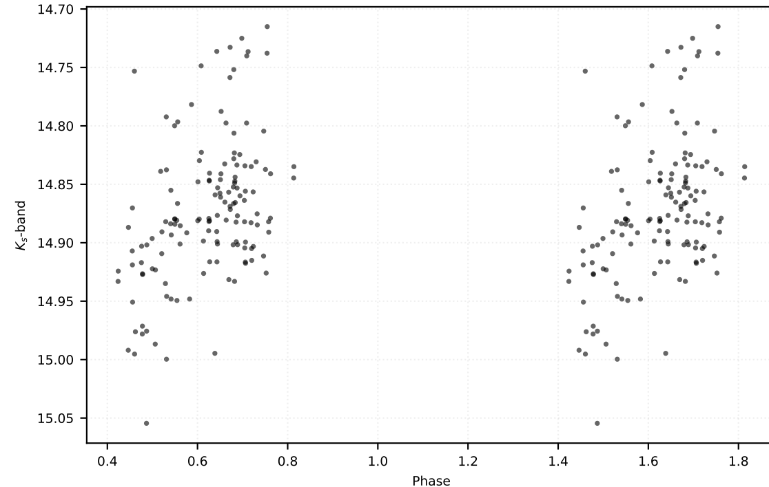
P: 0.37593 d | Class: RP | Subclass: RRab | Field b279
