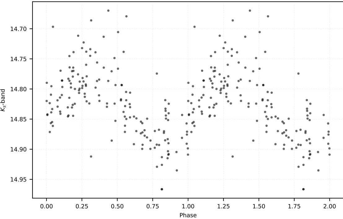
P: 0.31734 d | Class: RP | Subclass: RRab | Field b279
