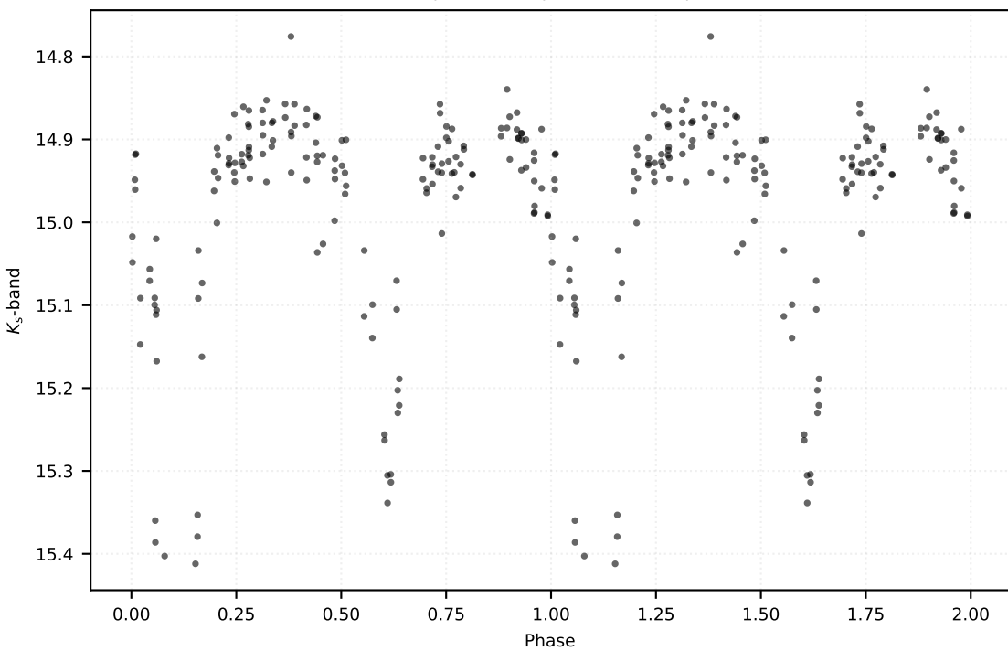
P: 3.25351 d | Class: EB | Subclass: EA | Field b279
