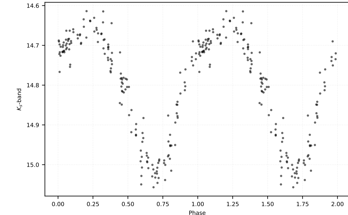
P: 0.56267 d | Class: RP | Subclass: RRab | Field b279
