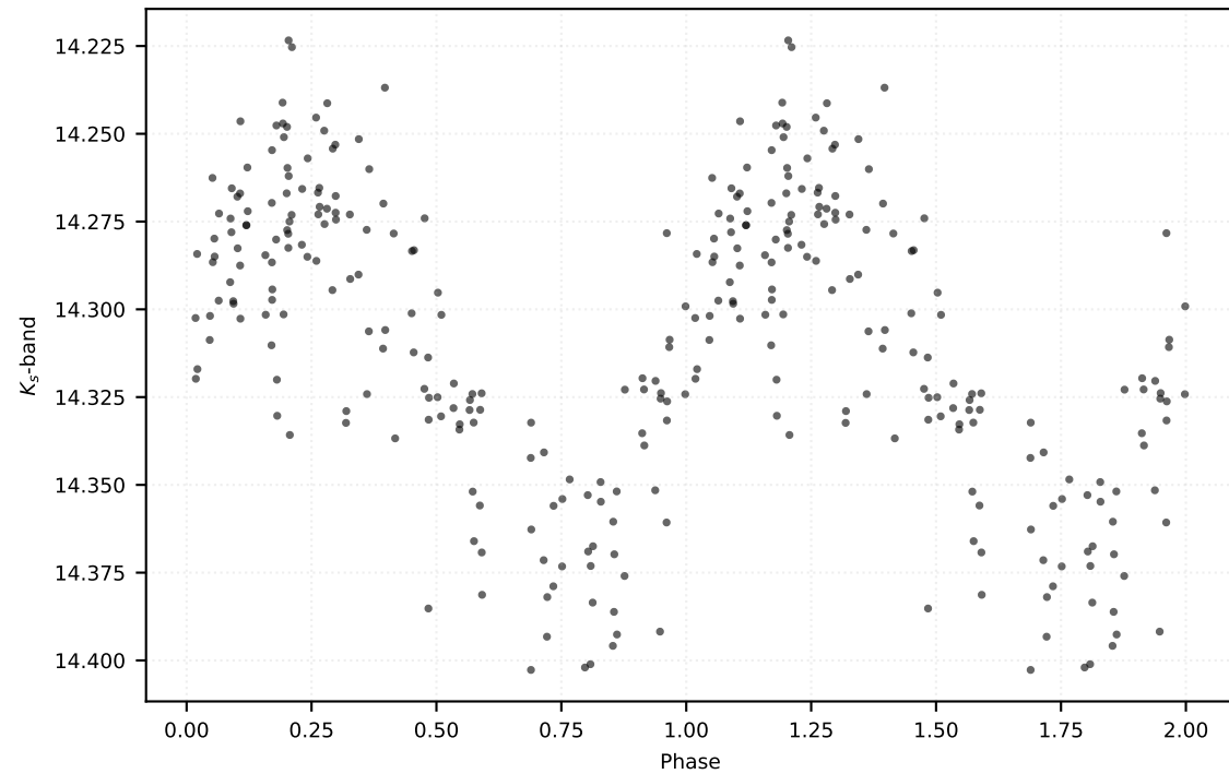
P: 0.56384 d | Class: RP | Subclass: RRab | Field b278
