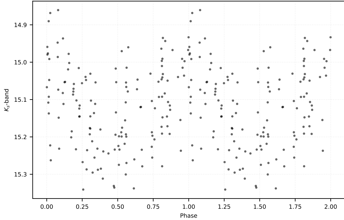
P: 0.17131 d | Class: RP | Subclass: UVAR | Field b279
