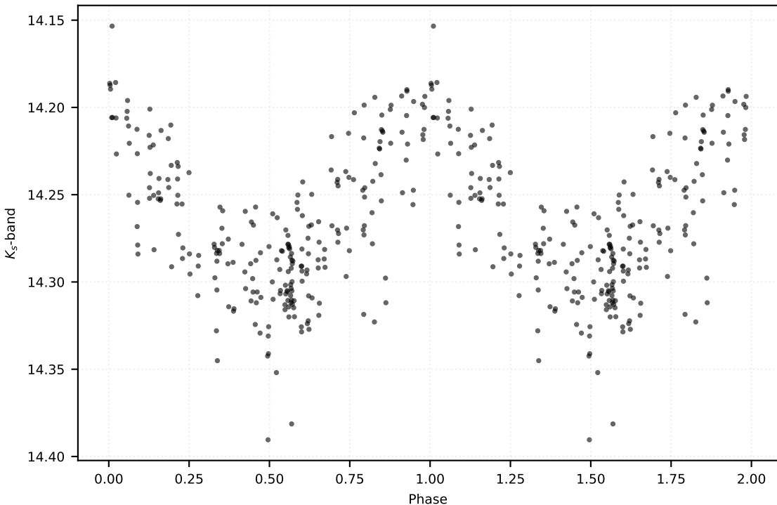
P: 0.32753 d | Class: RP | Subclass: RRab | Field b279
