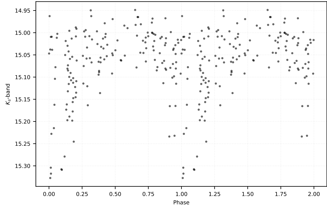
P: 0.14906 d | Class: RP | Subclass: UVAR | Field b278
