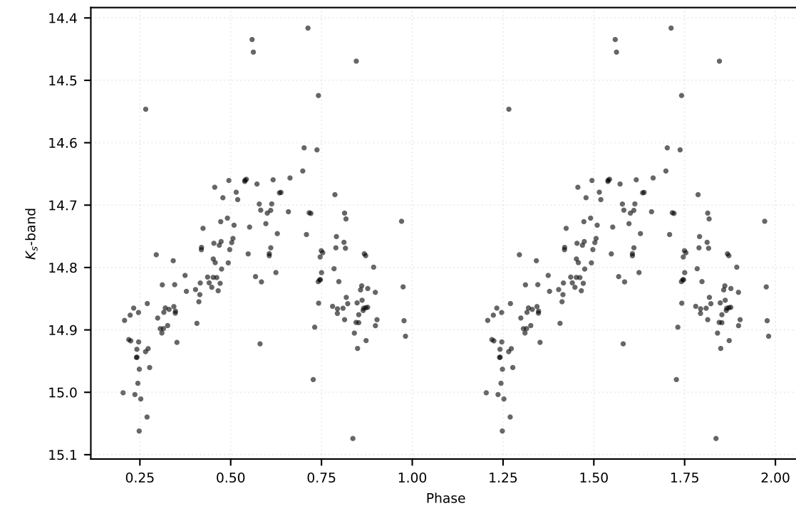
P: 0.18411 d | Class: RP | Subclass: UVAR | Field b279
