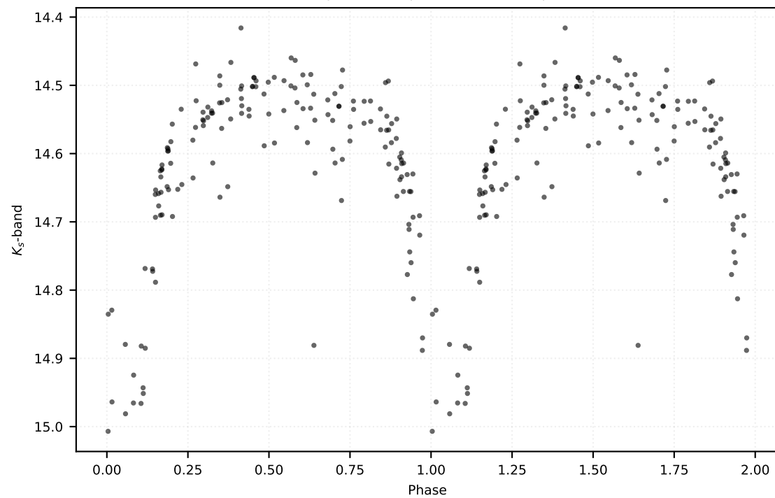
P: 3.44858 d | Class: RP | Subclass: CEP-F | Field b278
