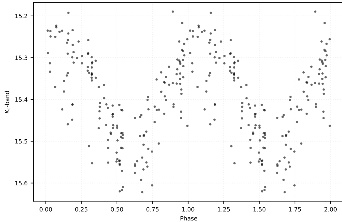
P: 0.67699 d | Class: RP | Subclass: CEP-10T | Field b278
