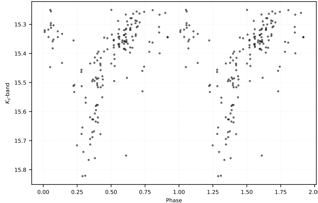
P: 0.83024 d | Class: RP | Subclass: CEP-10T | Field b279
