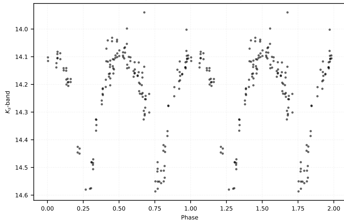
P: 0.95865 d | Class: EB | Subclass: UVAR | Field b278
