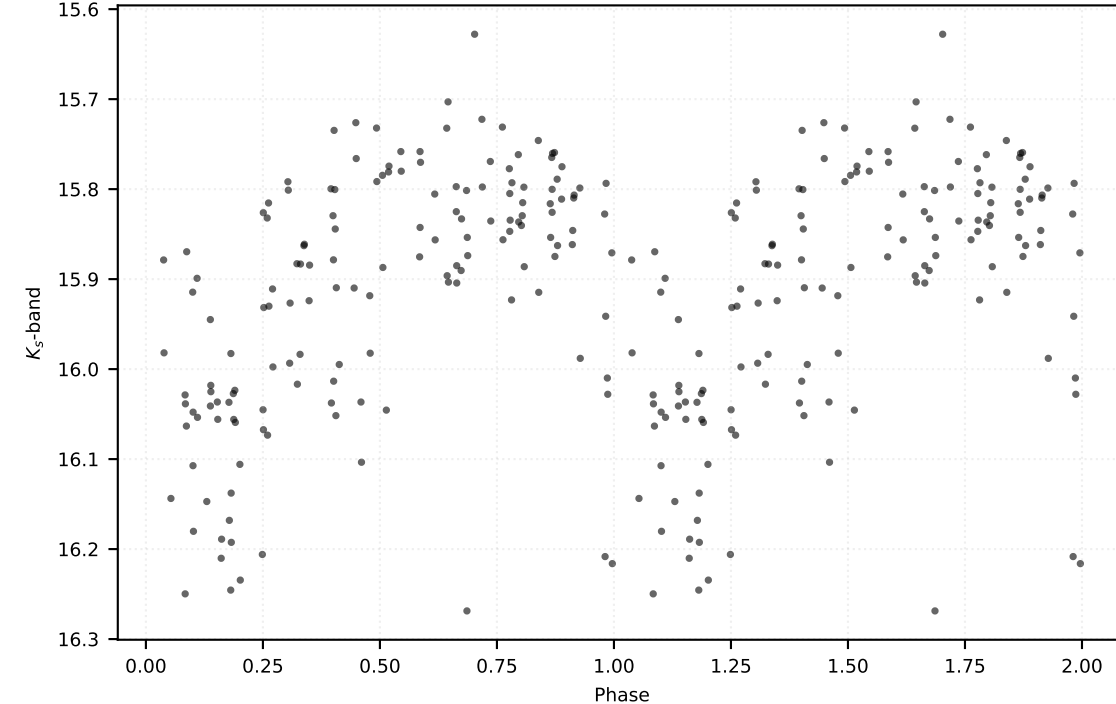
P: 0.80729 d | Class: RP | Subclass: RRab | Field b279
