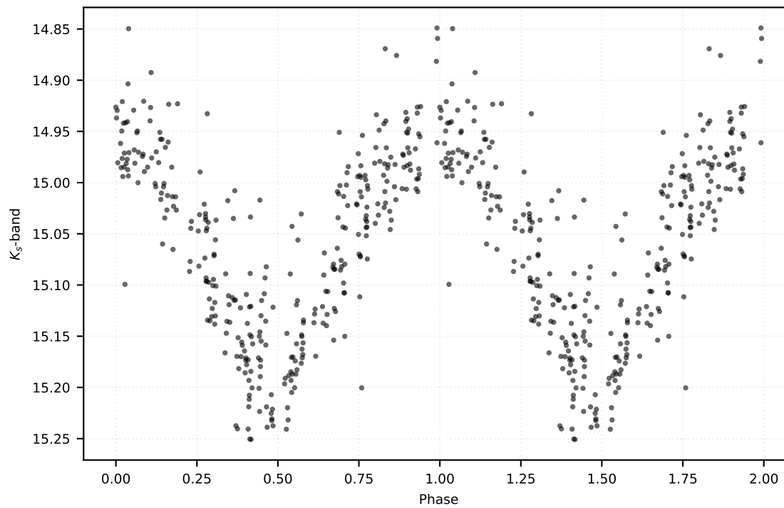
P: 0.22149 d | Class: RP | Subclass: UVAR | Field b278
