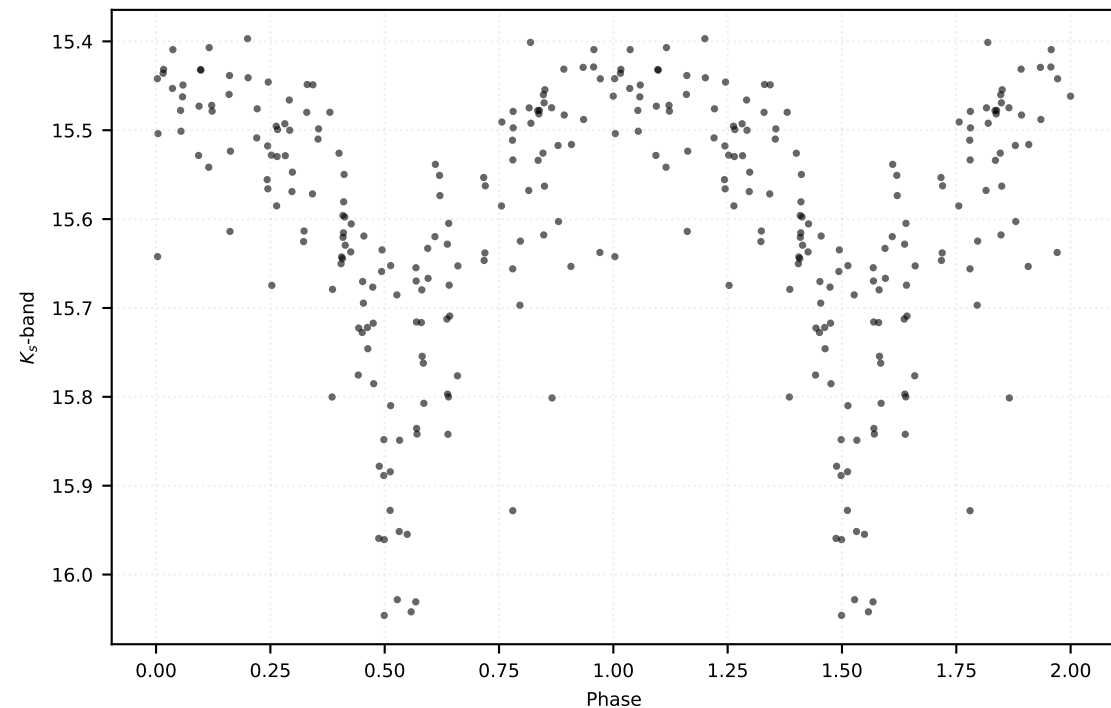
P: 0.54160 d | Class: RP | Subclass: RRab | Field b278
