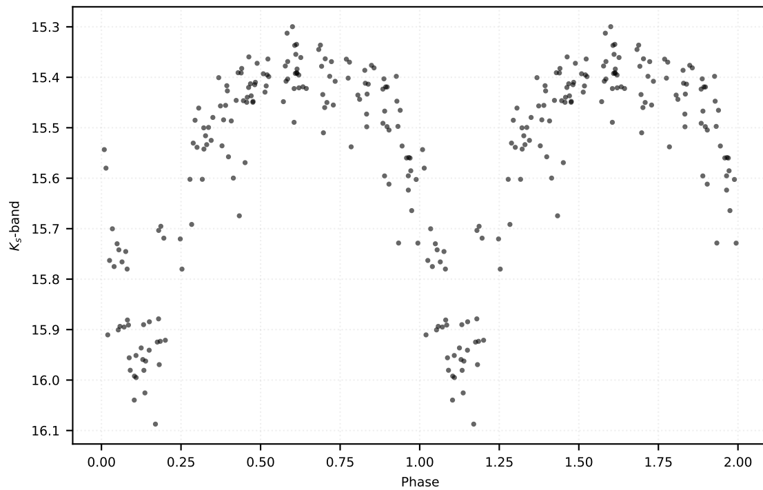
P: 1.05446 d | Class: EB | Subclass: UVAR | Field b279
