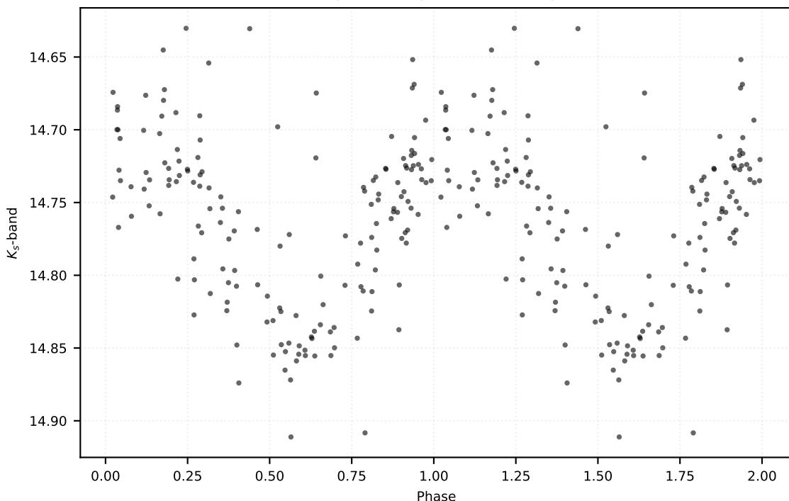
P: 0.32354 d | Class: RP | Subclass: RRab | Field b279
