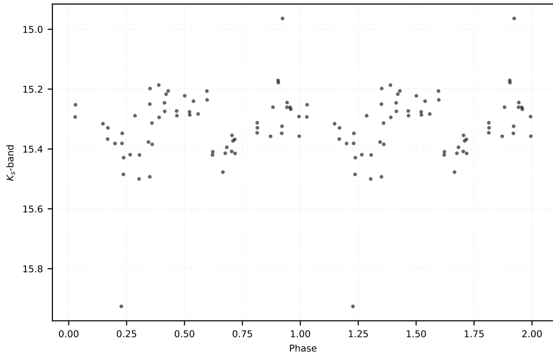
P: 0.35655 d | Class: EB | Subclass: EA | Field b278
