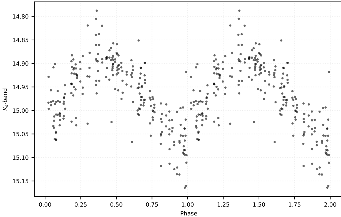
P: 0.42486 d | Class: RP | Subclass: RRab | Field b279
