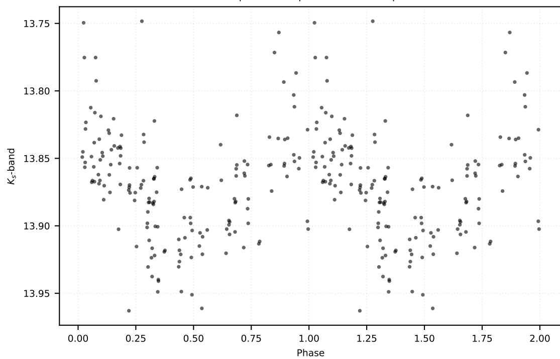
P: 0.10856 d | Class: RP | Subclass: UVAR | Field b279
