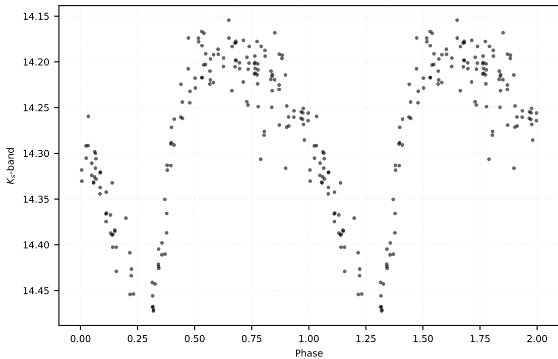
P: 0.48031 d | Class: RP | Subclass: RRab | Field b279
