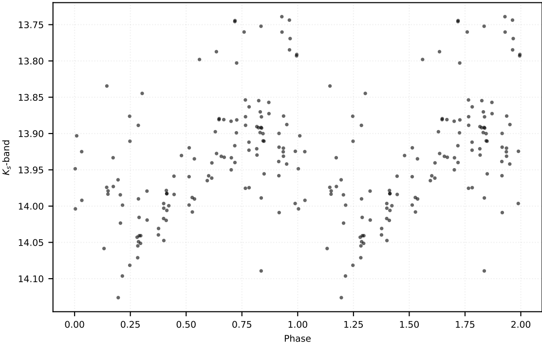
P: 0.73030 d | Class: RP | Subclass: CEP-1OT | Field b278
