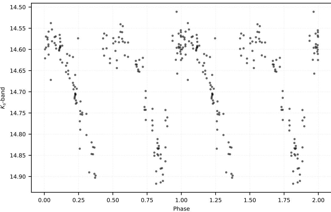
P: 0.10201 d | Class: RP | Subclass: UVAR | Field b278
