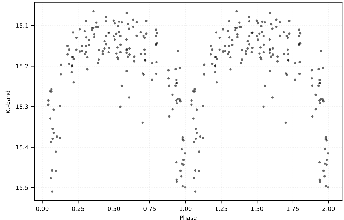
P: 1.04370 d | Class: RP | Subclass: CEP-10T | Field b279
