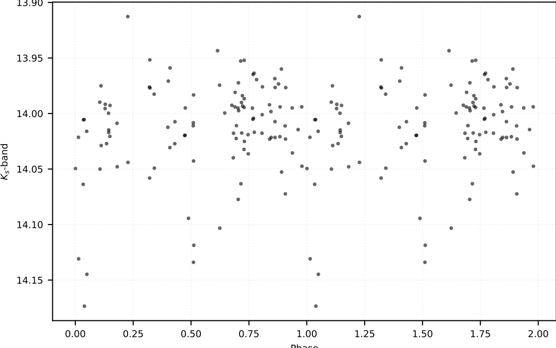
P: 0.46009 d | Class: EB | Subclass: EA | Field b278
