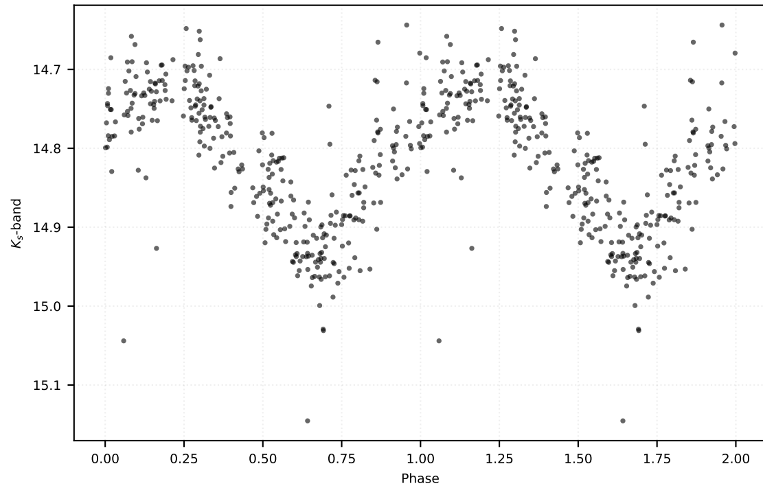
P: 0.21186 d | Class: RP | Subclass: UVAR | Field b279
