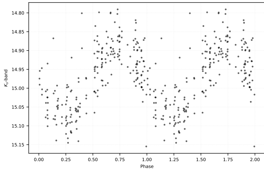
P: 0.44332 d | Class: RP | Subclass: RRab | Field b279
