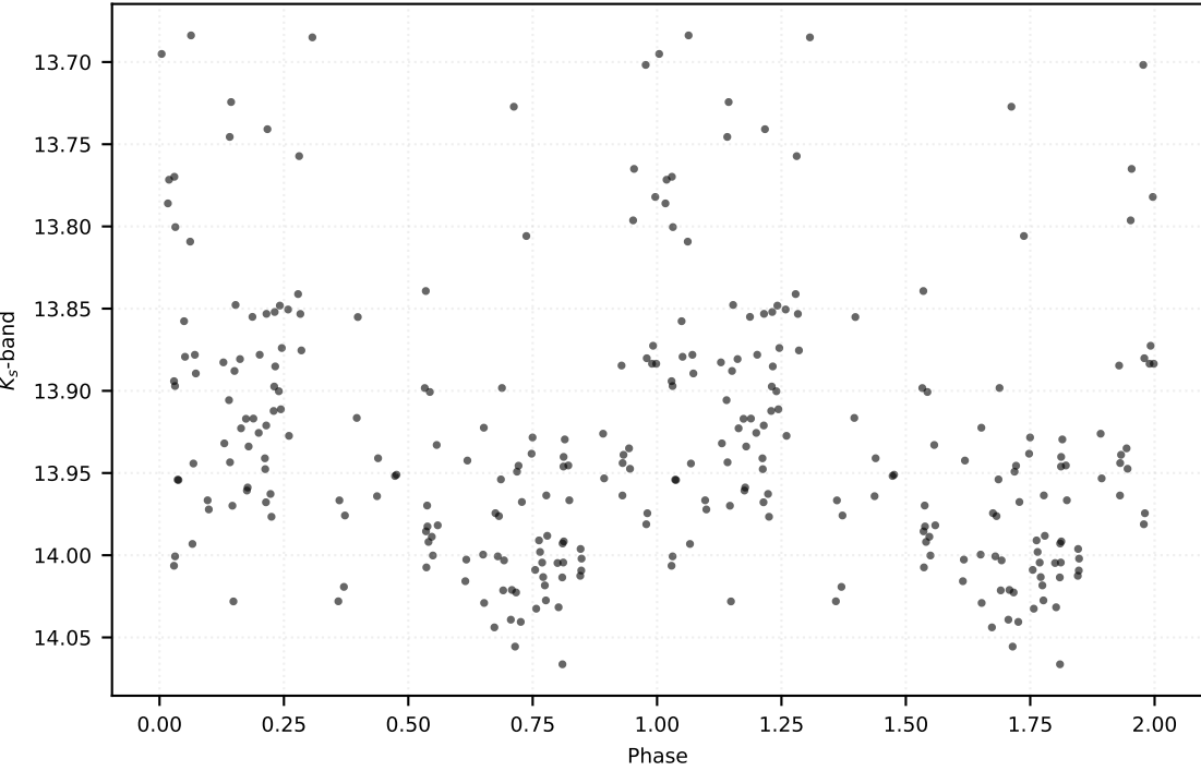
P: 0.29192 d | Class: RP | Subclass: UVAR | Field b278
