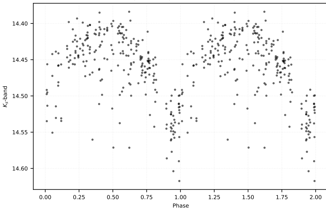
P: 0.62216 d | Class: RP | Subclass: CEP-10T | Field b279
