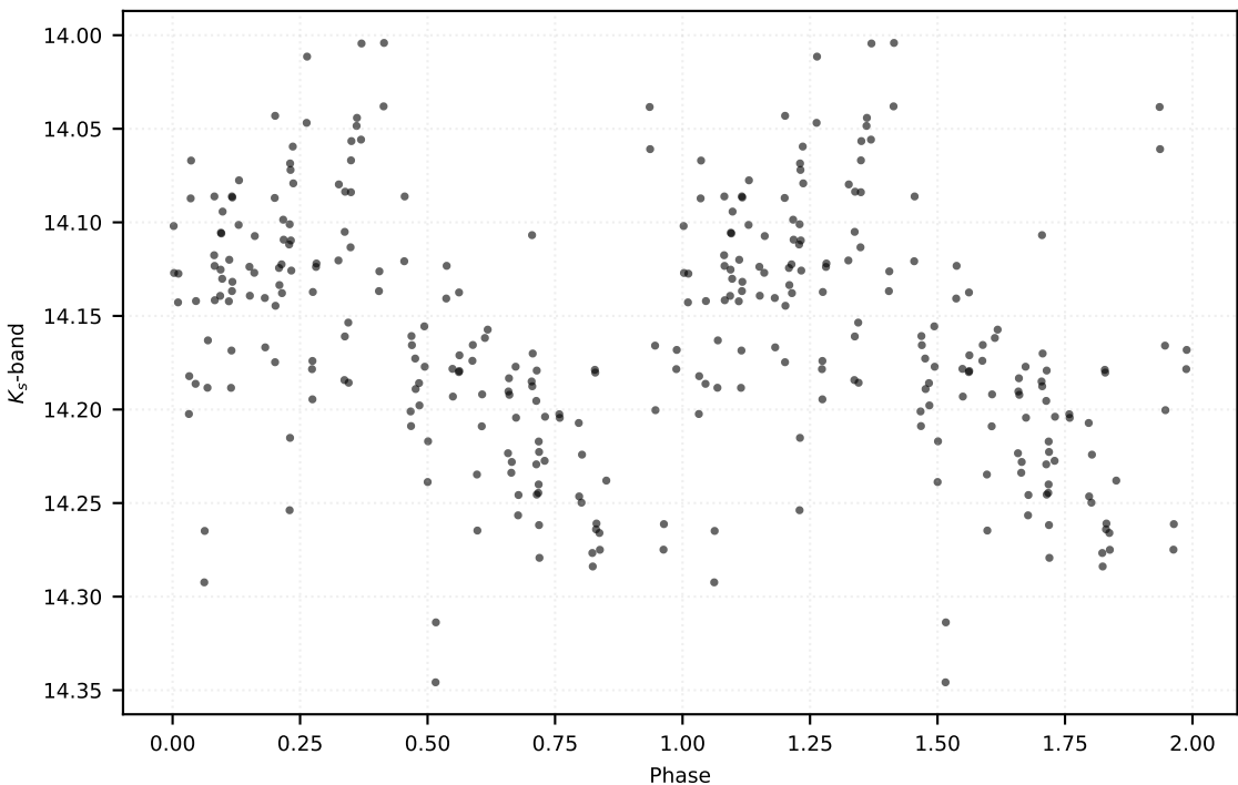
P: 0.62667 d | Class: RP | Subclass: CEP-1OT | Field b278
