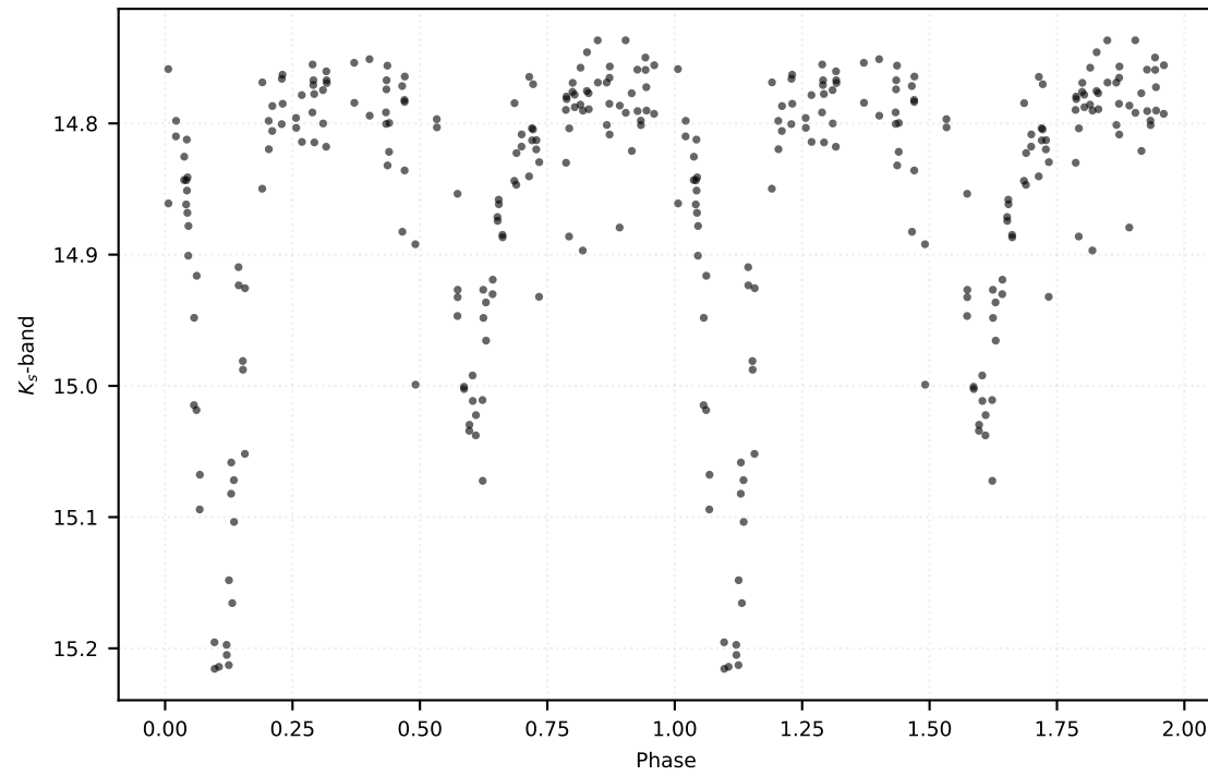
P: 1.23970 d | Class: EB | Subclass: UVAR | Field b278
