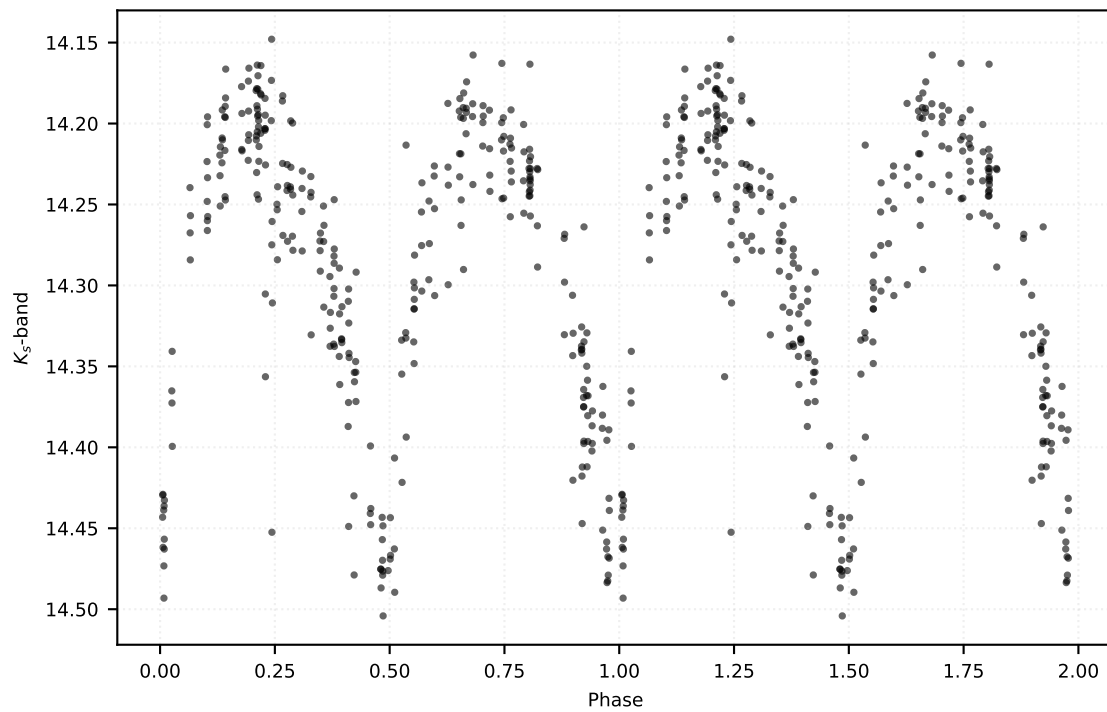
P: 0.20764 d | Class: RP | Subclass: RRc | Field b278
