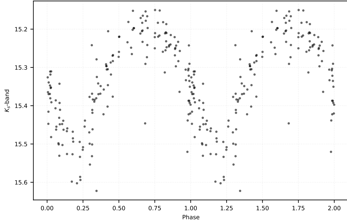
P: 0.41675 d | Class: RP | Subclass: RRc | Field b278
