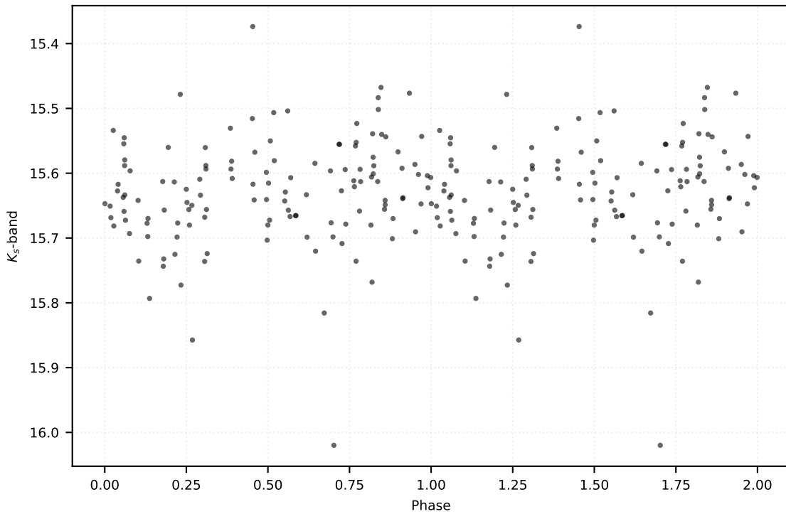
P: 0.43970 d | Class: EB | Subclass: EA | Field b278
