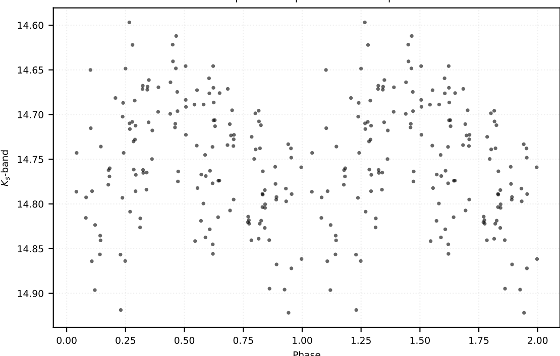
P: 0.40696 d | Class: RP | Subclass: RRab | Field b279
