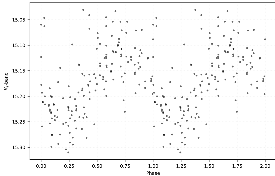
P: 0.51429 d | Class: RP | Subclass: RRab | Field b278
