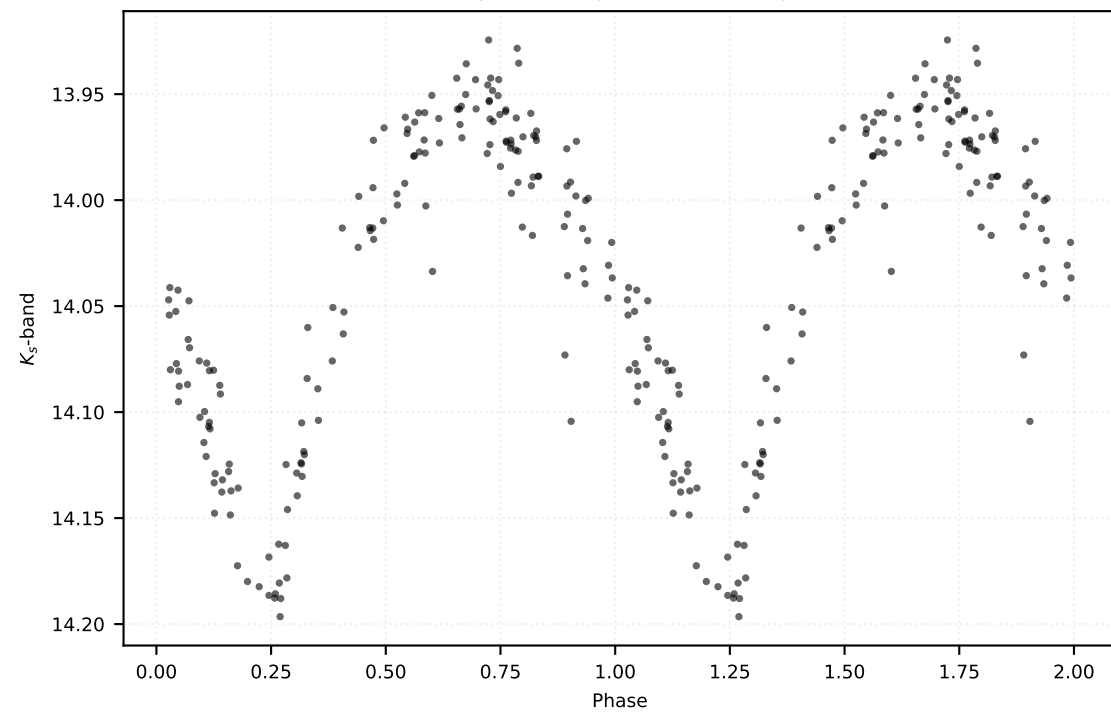
P: 0.52360 d | Class: RP | Subclass: RRab | Field b278
