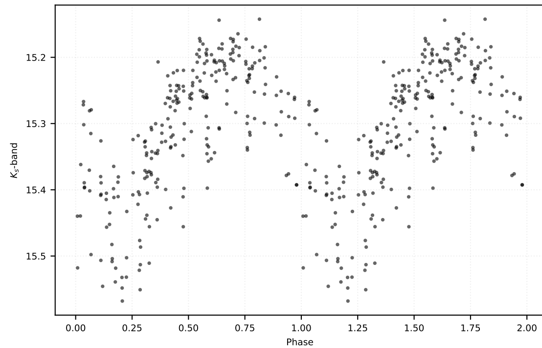
P: 0.99776 d | Class: RP | Subclass: CEP-10T | Field b278
