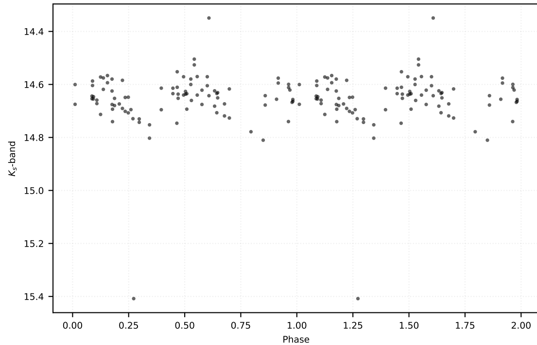
P: 15.22845 d | Class: EB | Subclass: EA | Field b279
