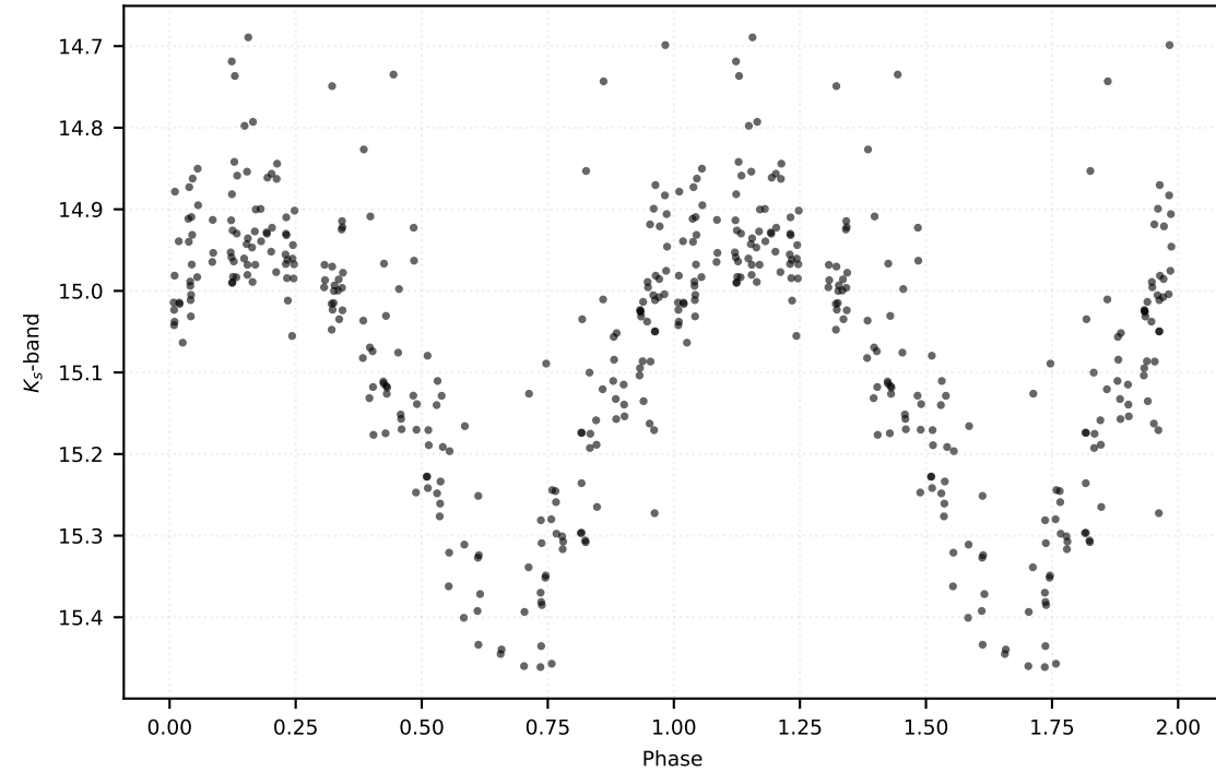
P: 0.52956 d | Class: RP | Subclass: RRab | Field b278
