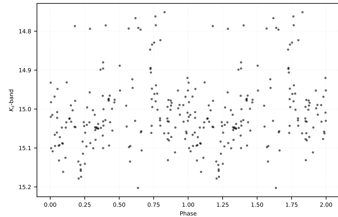
P: 0.17834 d | Class: RP | Subclass: UVAR | Field b278
