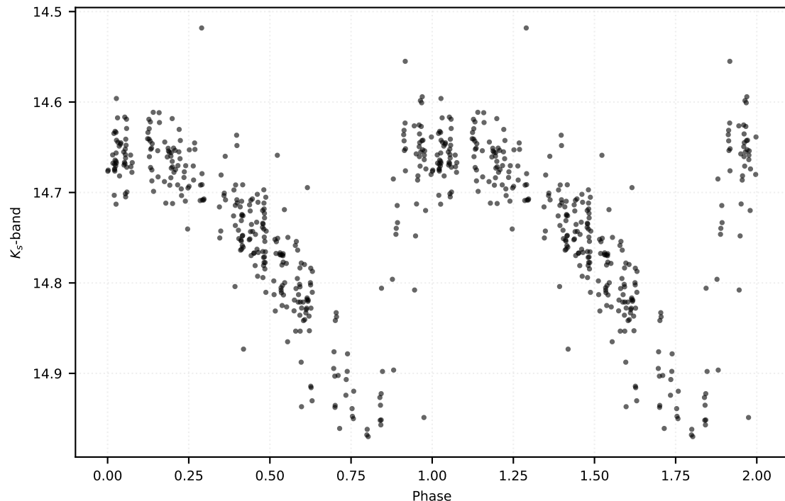
P: 0.55401 d | Class: RP | Subclass: RRab | Field b278
