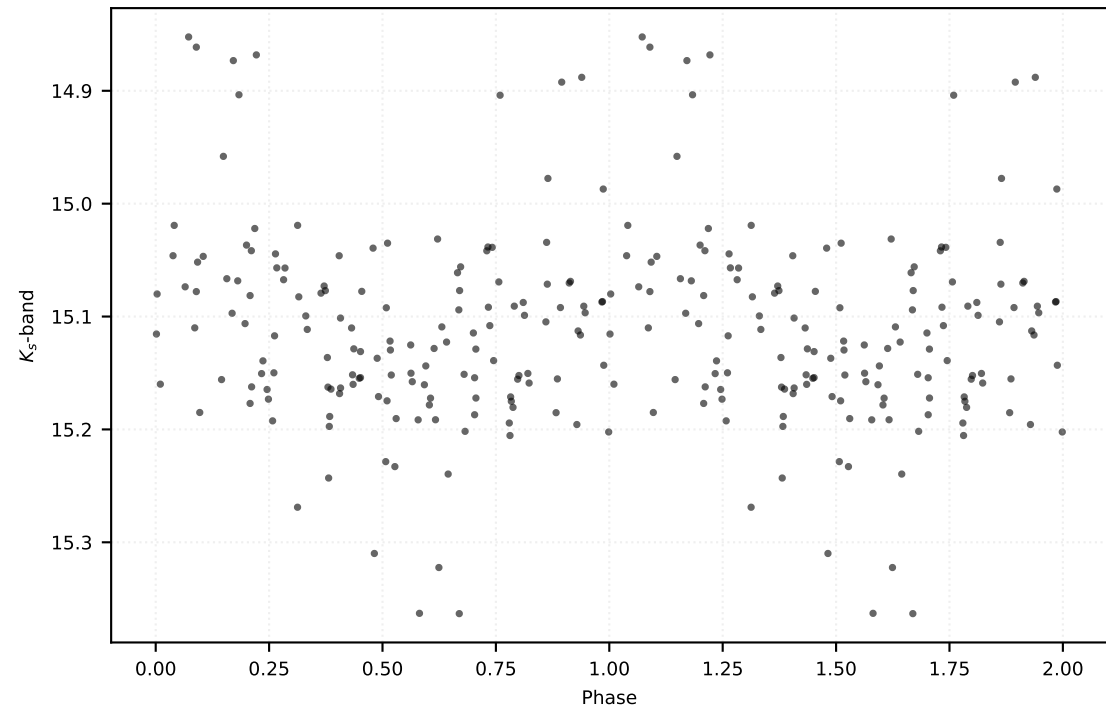
P: 0.14147 d | Class: RP | Subclass: UVAR | Field b279
