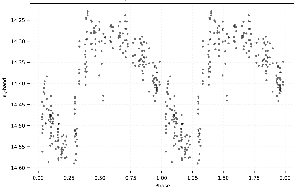
P: 0.68051 d | Class: RP | Subclass: RRab | Field b278
