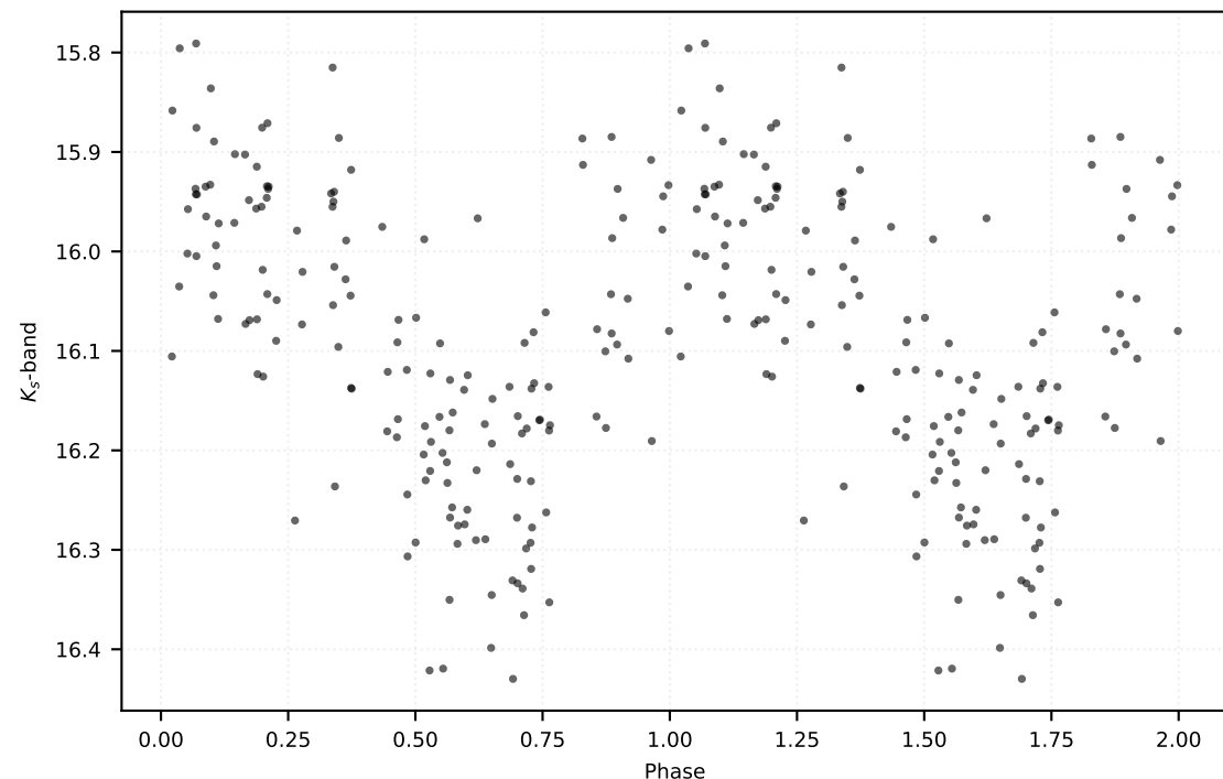
P: 0.36739 d | Class: RP | Subclass: RRab | Field b279
