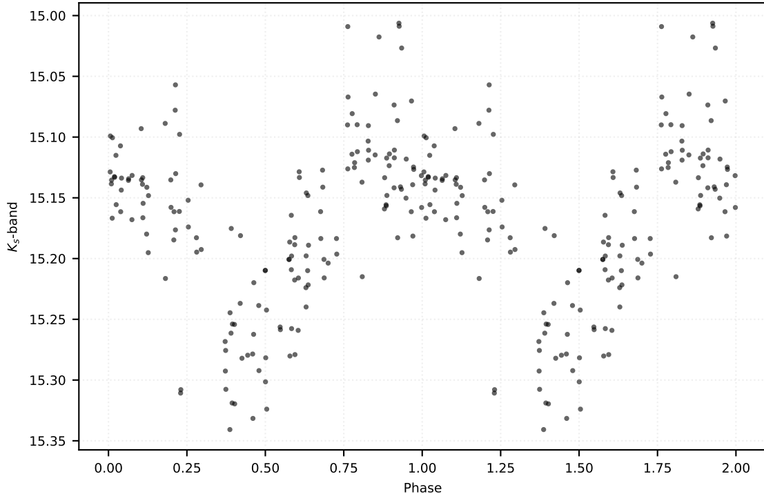
P: 0.25710 d | Class: RP | Subclass: RRc | Field b279
