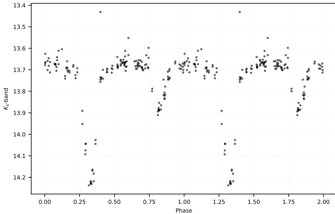
P: 1.40976 d | Class: EB | Subclass: EA | Field b279
