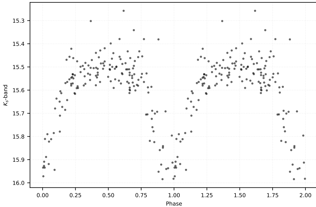
P: 0.36637 d | Class: RP | Subclass: CEP-10T | Field b279
