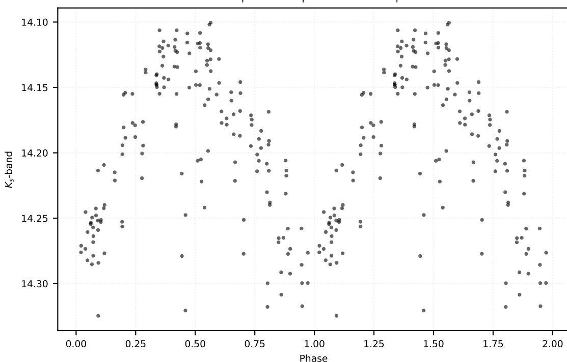
P: 0.60424 d | Class: RP | Subclass: RRab | Field b278
