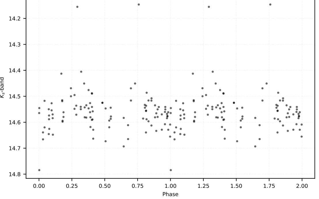
P: 2.44601 d | Class: EB | Subclass: EA | Field b278
