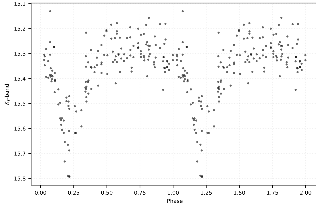
P: 1.42002 d | Class: RP | Subclass: CEP-10T | Field b278
