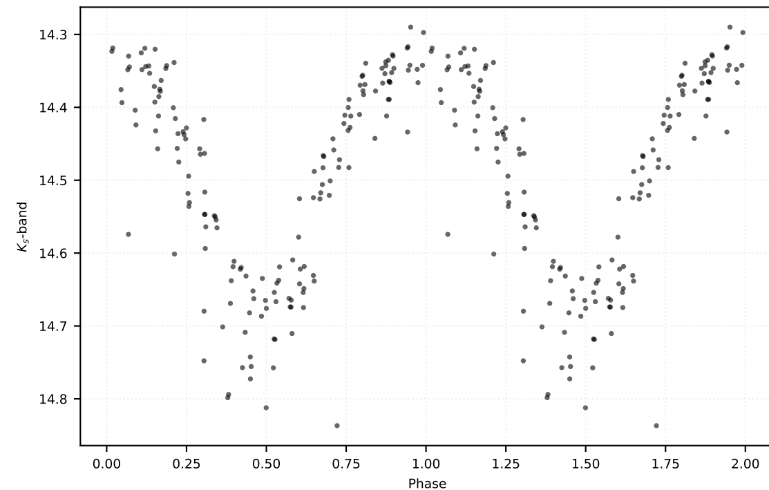
P: 0.17524 d | Class: RP | Subclass: UVAR | Field b278
