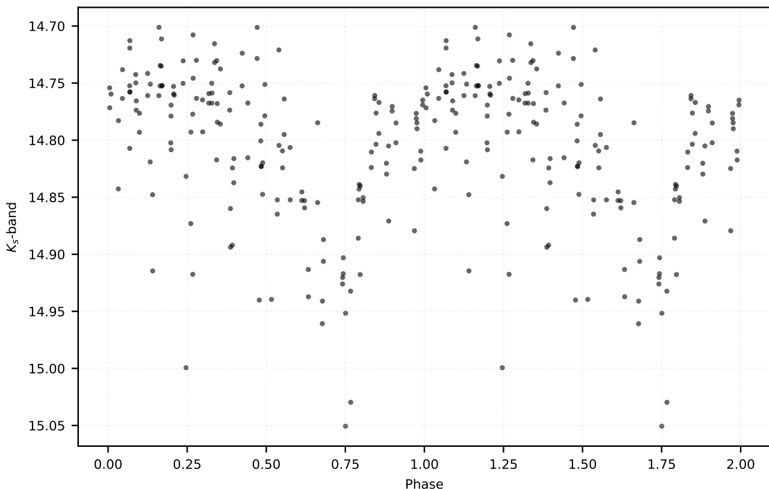
P: 4.80695 d | Class: RP | Subclass: CEP-10T | Field b278
