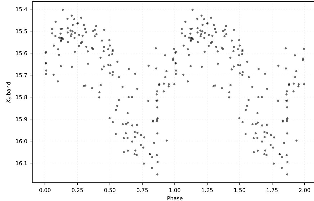
P: 0.61361 d | Class: RP | Subclass: RRab | Field b279
