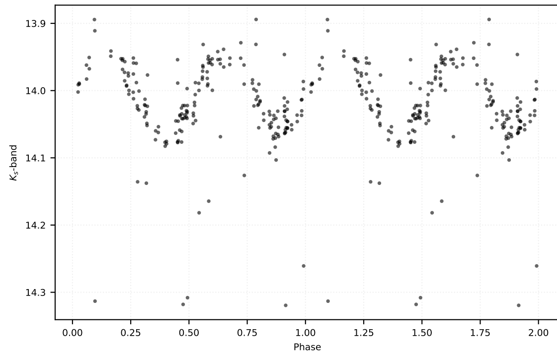
P: 0.21076 d | Class: EB | Subclass: EA | Field b279
