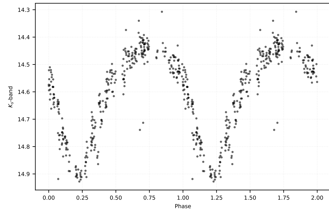
P: 0.24465 d | Class: RP | Subclass: UVAR | Field b279
