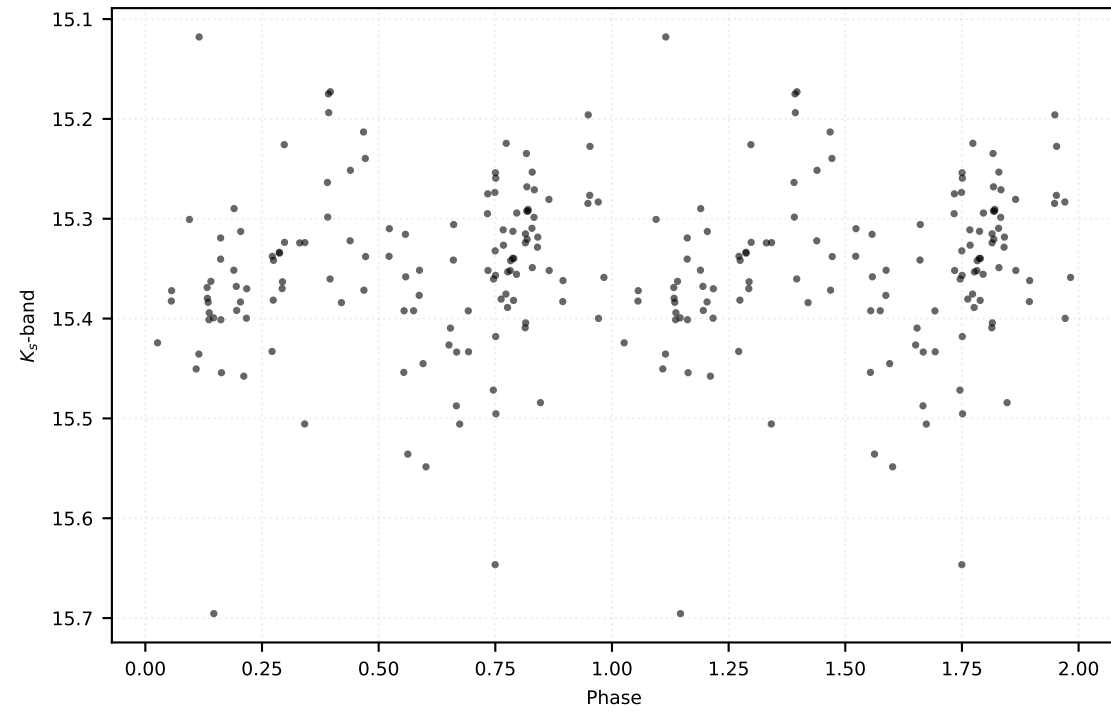
P: 0.66538 d | Class: EB | Subclass: EA | Field b279
