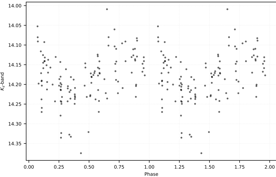
P: 0.52094 d | Class: RP | Subclass: RRab | Field b279
