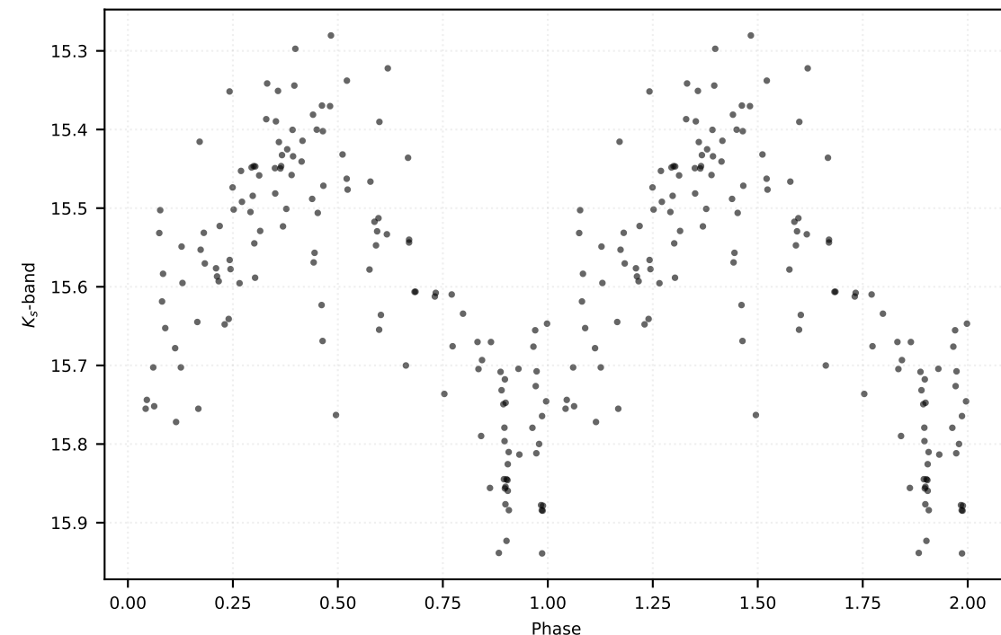
P: 0.12736 d | Class: RP | Subclass: UVAR | Field b278
