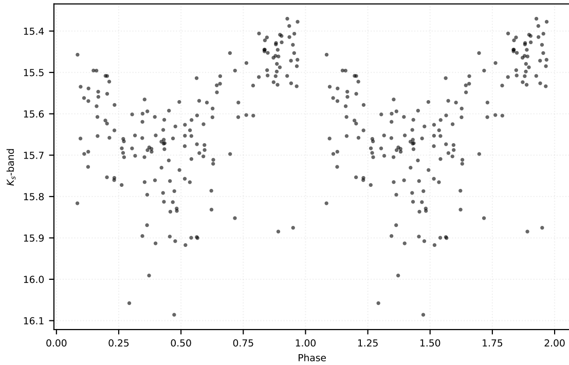
P: 0.46179 d | Class: RP | Subclass: RRab | Field b278
