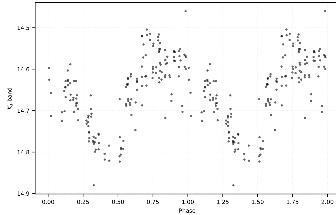
P: 0.52265 d | Class: RP | Subclass: RRab | Field b279
