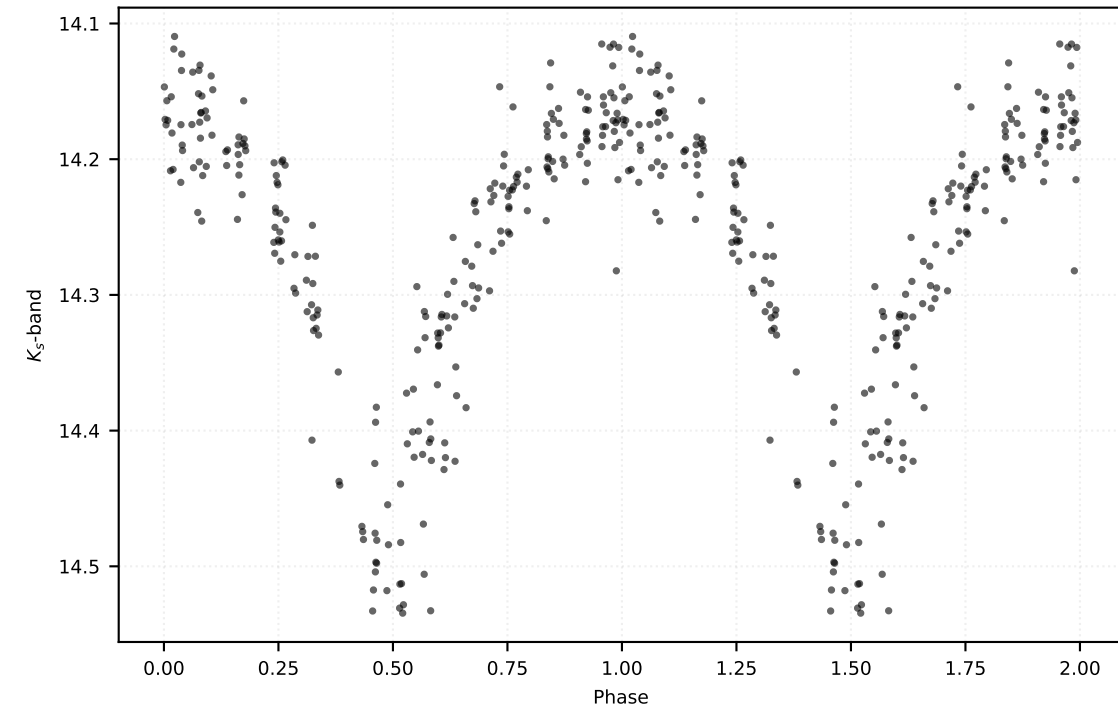
P: 0.38051 d | Class: RP | Subclass: CEP-1OT | Field b278
