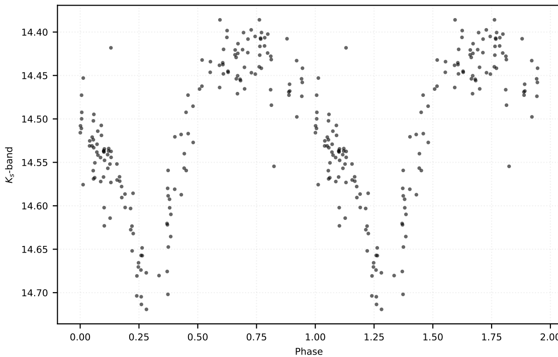
P: 0.58771 d | Class: RP | Subclass: RRab | Field b279
