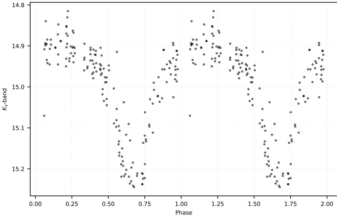
P: 0.22748 d | Class: RP | Subclass: UVAR | Field b278
