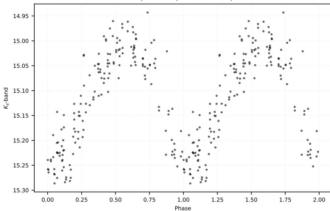
P: 0.52374 d | Class: RP | Subclass: RRab | Field b278
