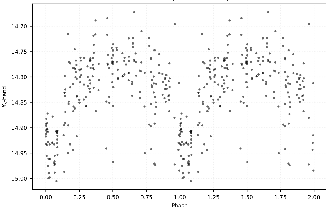
P: 0.39909 d | Class: RP | Subclass: RRab | Field b279
