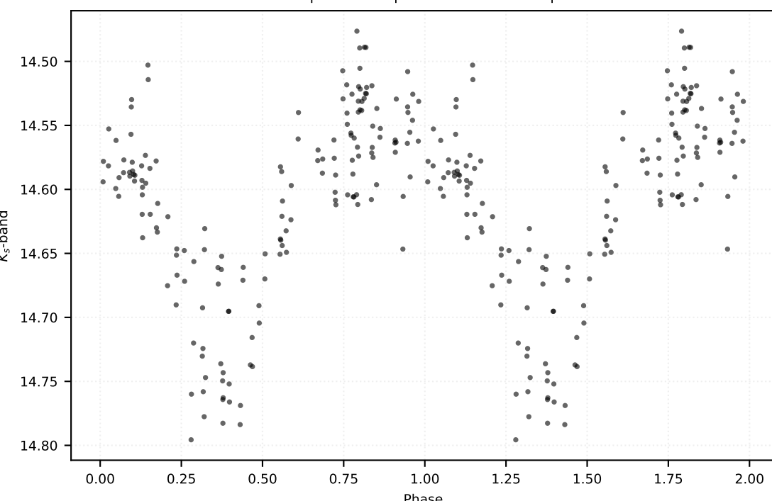
P: 0.85164 d | Class: RP | Subclass: CEP-10T | Field b278
