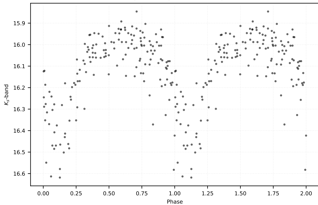
P: 0.42735 d | Class: RP | Subclass: R Rab | Field b278
