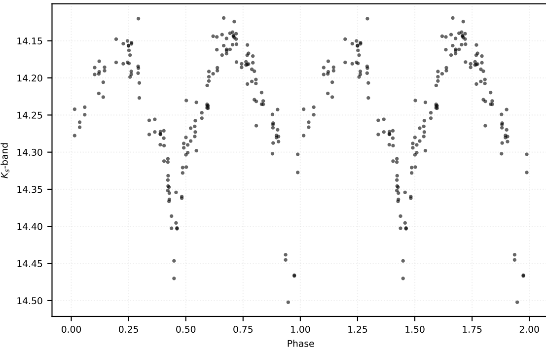
P: 0.12300 d | Class: RP | Subclass: UVAR | Field b278
