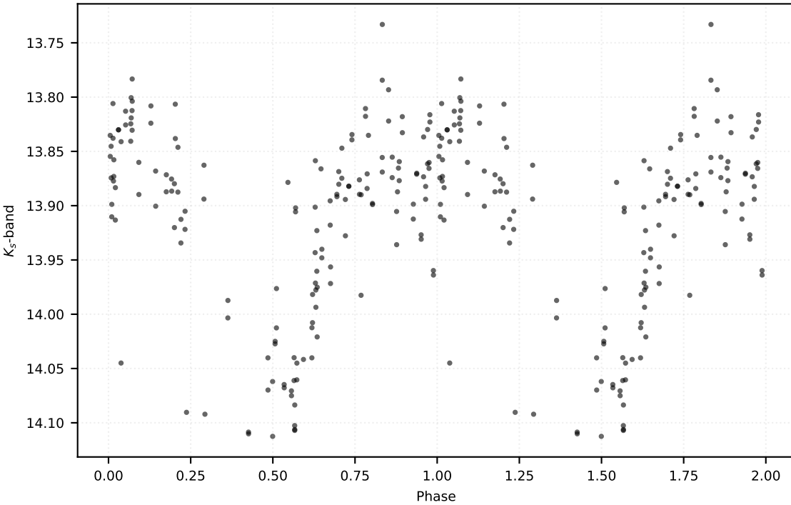
P: 1.13195 d | Class: RP | Subclass: CEP-F | Field b279
