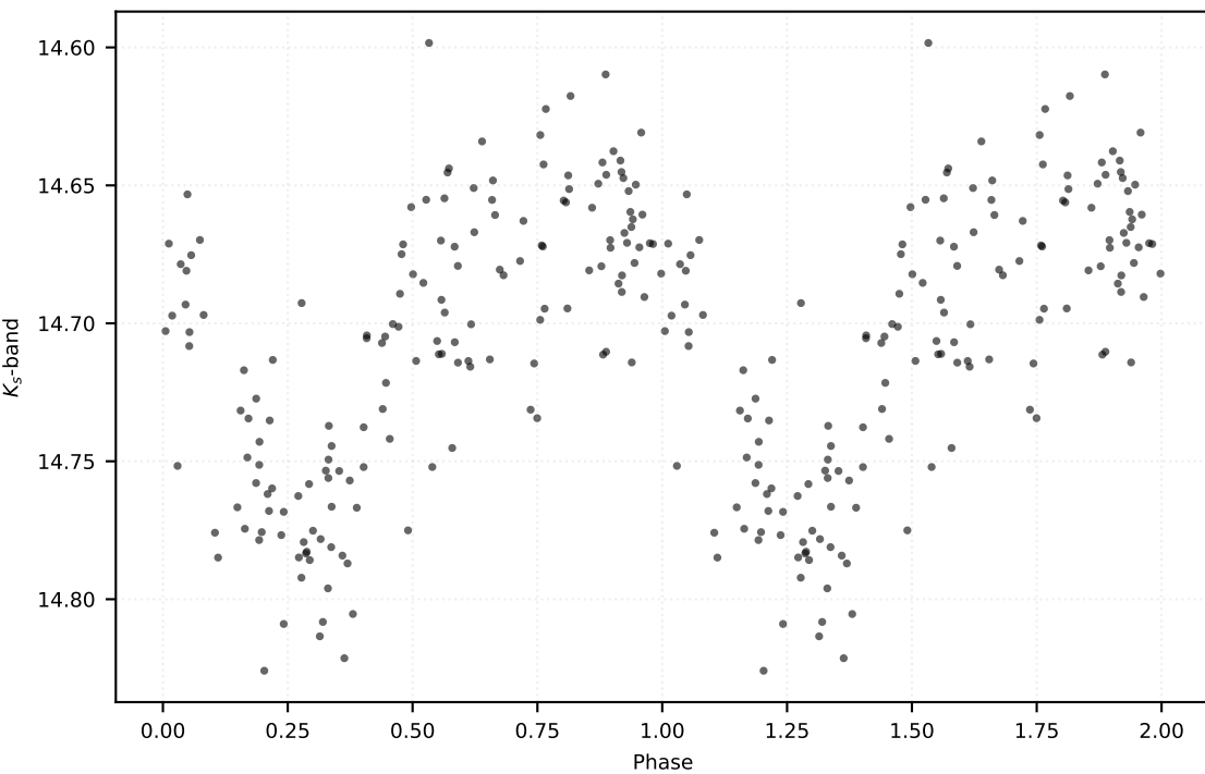
P: 0.18441 d | Class: RP | Subclass: UVAR | Field b279
