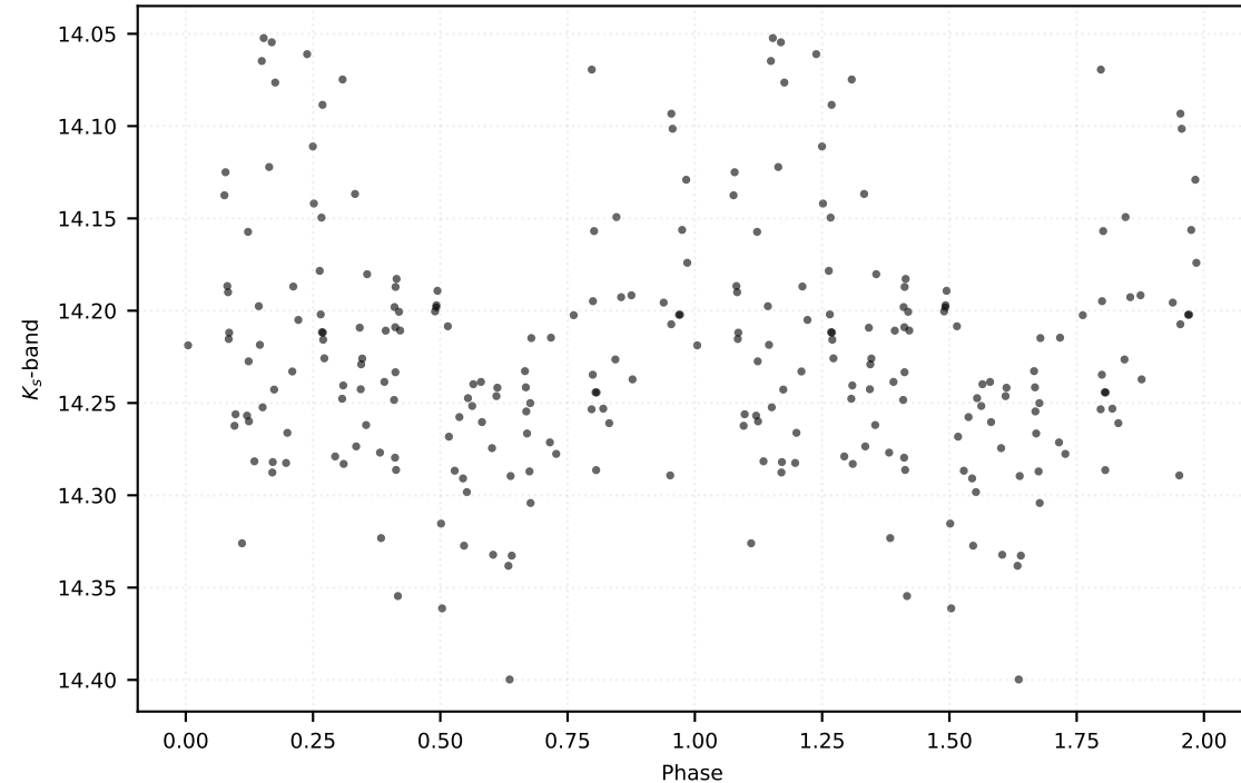
P: 19.33445 d | Class: RP | Subclass: UVAR | Field b279
