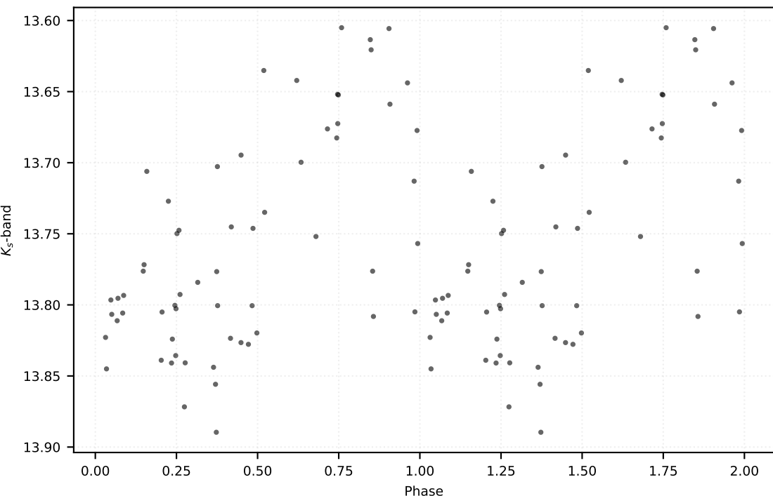
P: 0.10988 d | Class: RP | Subclass: UVAR | Field b279
