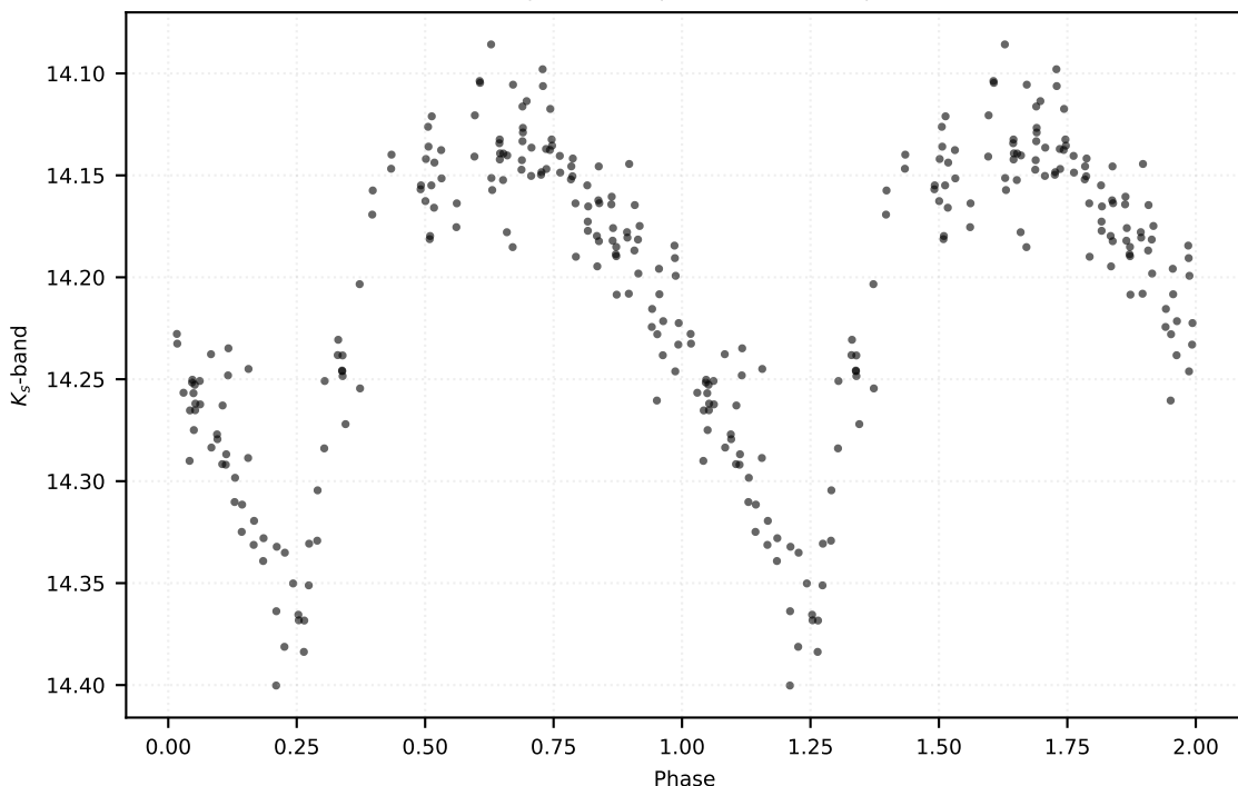
P: 0.52877 d | Class: RP | Subclass: RRab | Field b279
