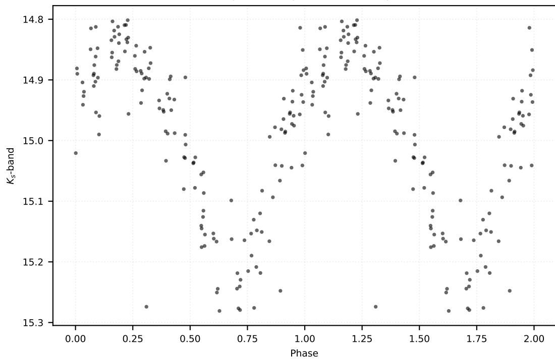
P: 0.15218 d | Class: RP | Subclass: UVAR | Field b278
