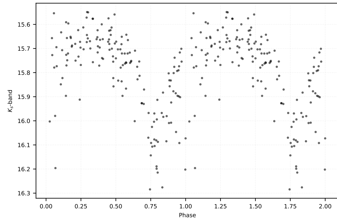
P: 0.32027 d | Class: RP | Subclass: RRc | Field b279
