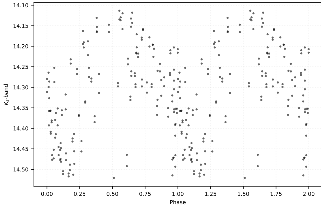
P: 1.07552 d | Class: RP | Subclass: CEP-F | Field b278
