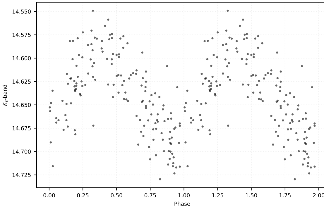
P: 0.36760 d | Class: RP | Subclass: RRab | Field b278
