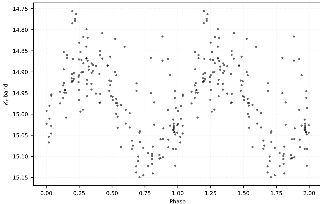
P: 0.22848 d | Class: RP | Subclass: UVAR | Field b278
