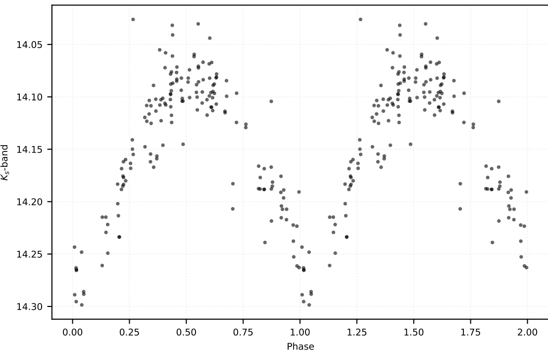
P: 0.60853 d | Class: RP | Subclass: RRab | Field b278
