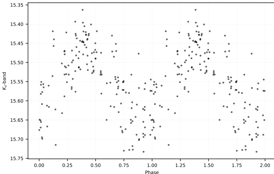
P: 0.31557 d | Class: RP | Subclass: CEP-10T | Field b279
