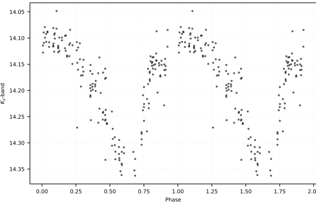
P: 0.56043 d | Class: RP | Subclass: RRab | Field b278
