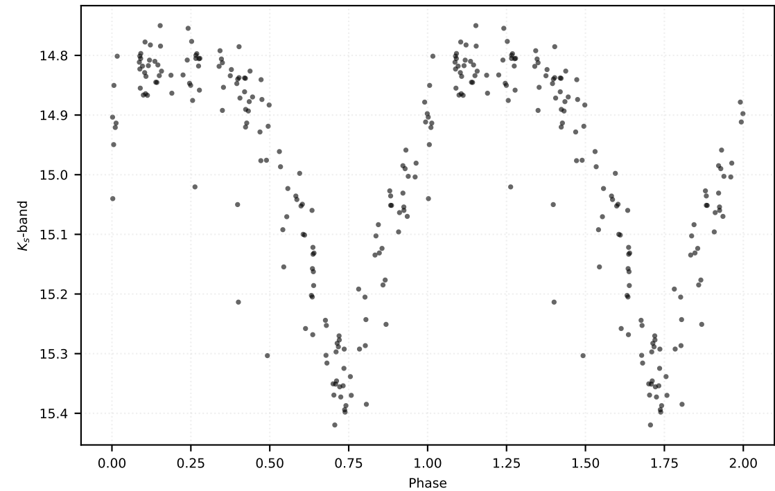
P: 0.21393 d | Class: RP | Subclass: UVAR | Field b279
