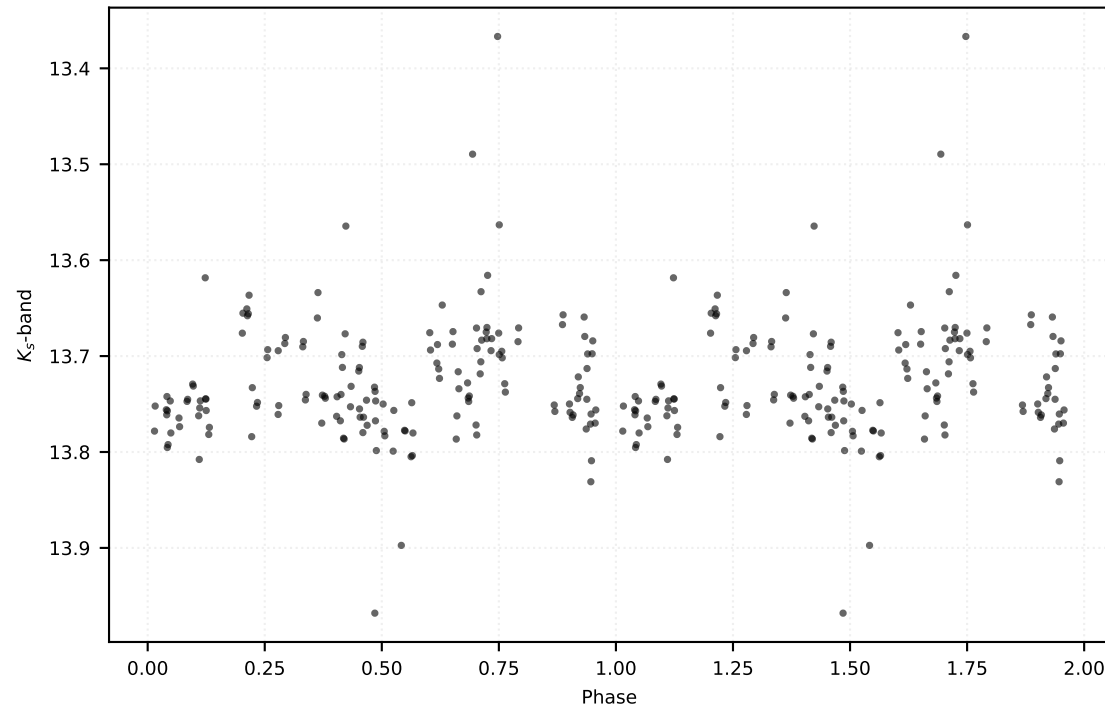
P: 0.55671 d | Class: EB | Subclass: EA | Field b279
