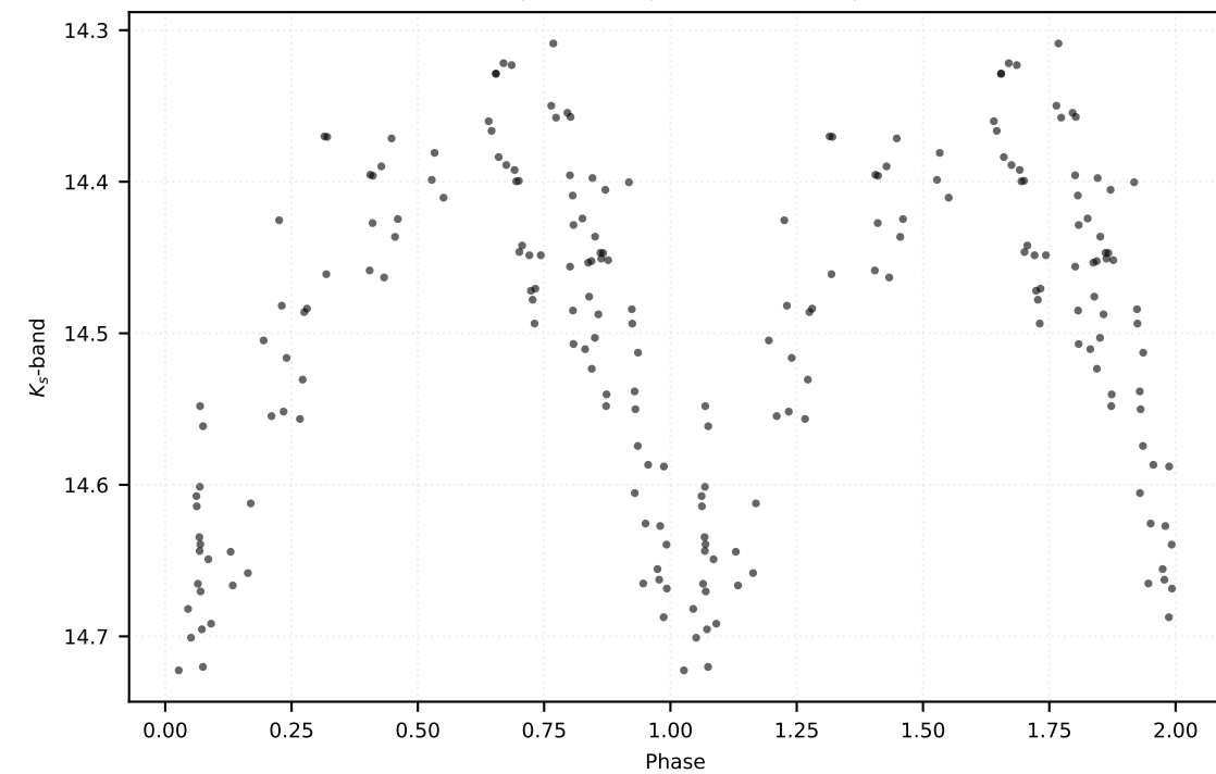
P: 1.01592 d | Class: EB | Subclass: UVAR | Field b278
