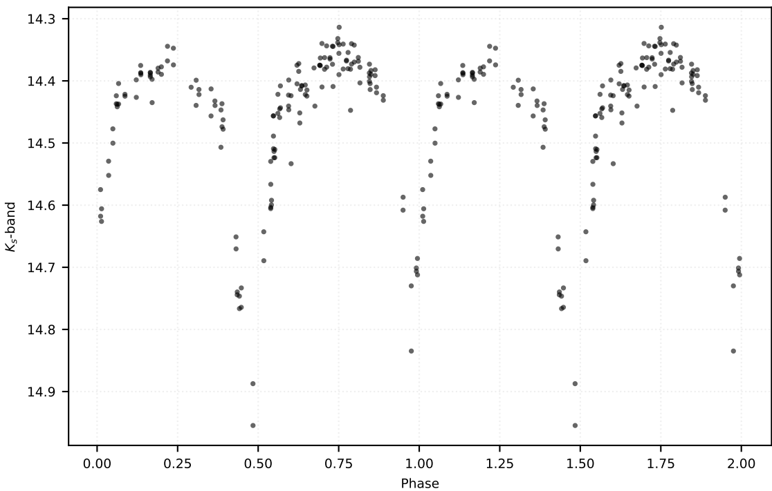
P: 2.17716 d | Class: EB | Subclass: EA | Field b279
