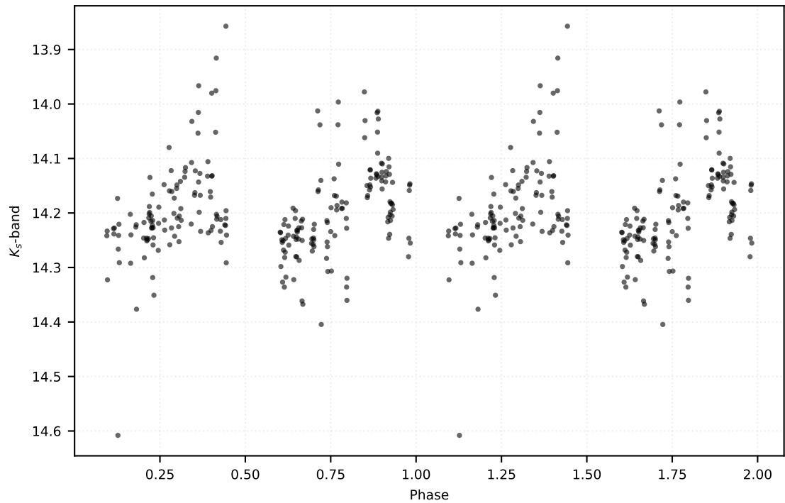
P: 1.12053 d | Class: EB | Subclass: EA | Field b279
