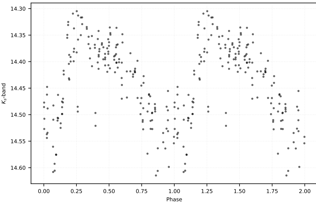
P: 0.57747 d | Class: RP | Subclass: RRab | Field b278
