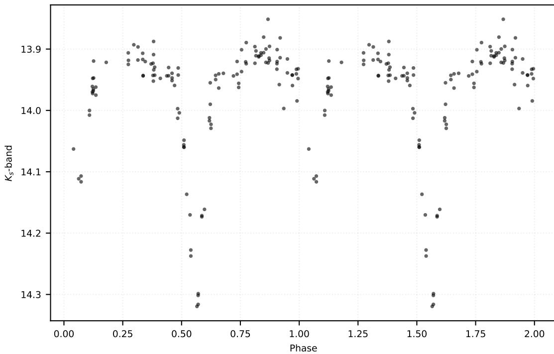
P: 3.87408 d | Class: EB | Subclass: EA | Field b279
