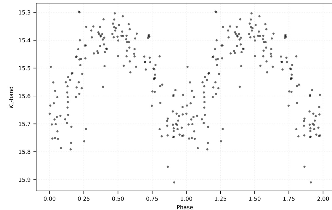
P: 0.13620 d | Class: RP | Subclass: UVAR | Field b279
