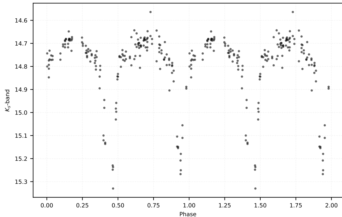
P: 0.97383 d | Class: EB | Subclass: EA | Field b278
