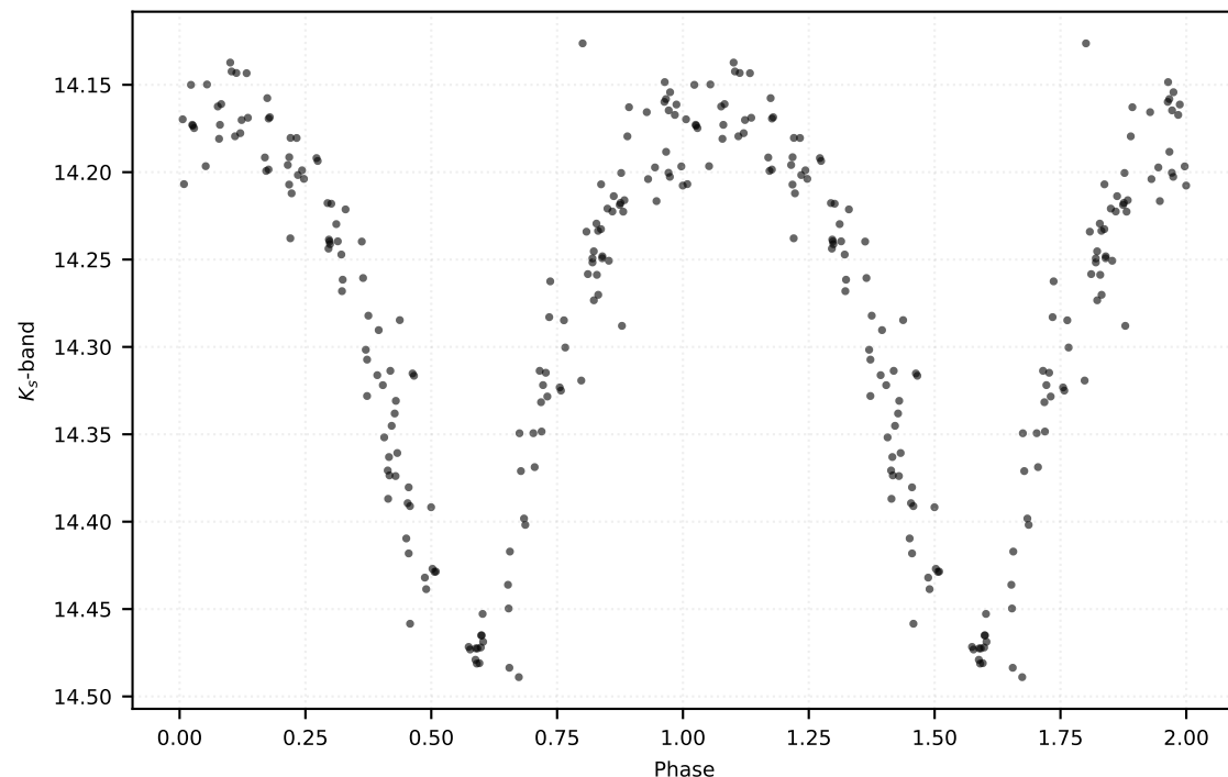
P: 0.25428 d | Class: RP | Subclass: UVAR | Field b279
