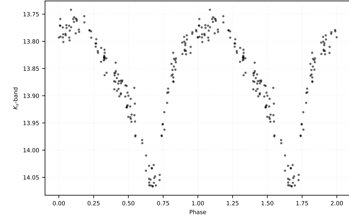
P: 0.72188 d | Class: RP | Subclass: RRab | Field b279
