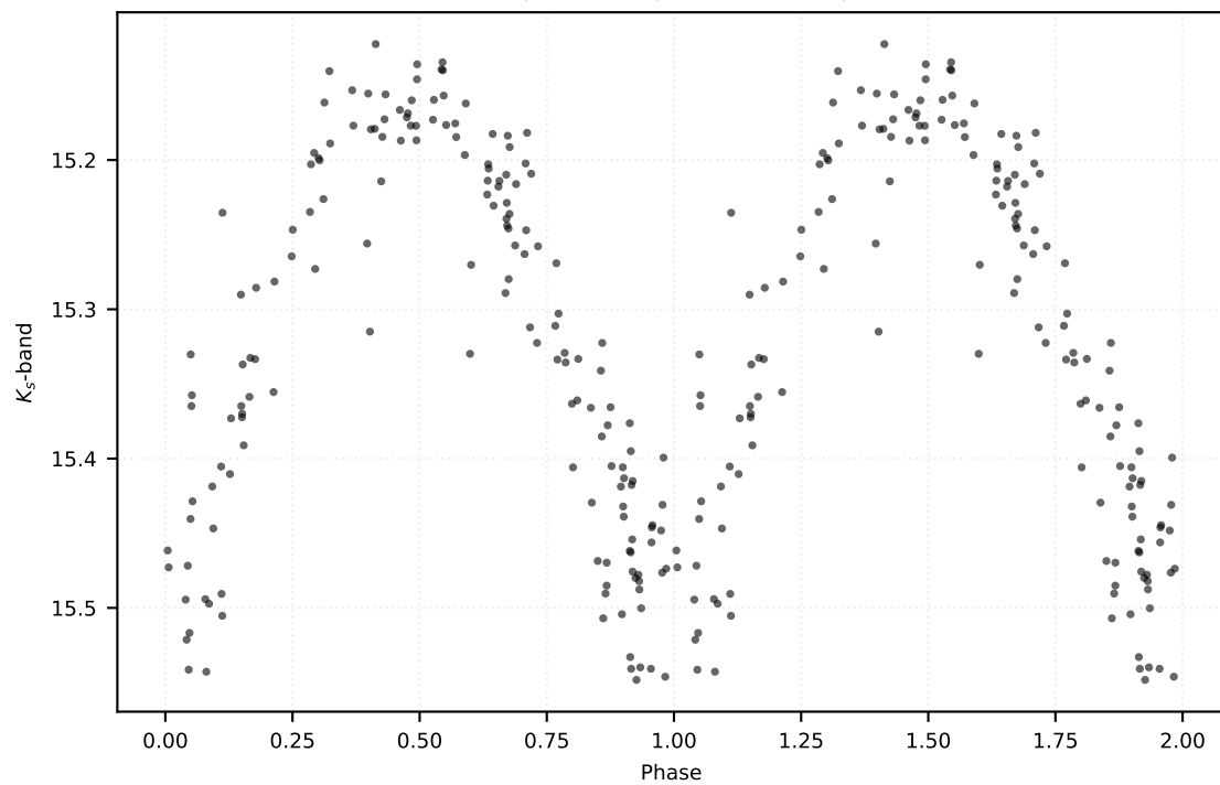
P: 0.24118 d | Class: RP | Subclass: RRc | Field b278
