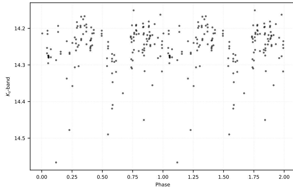
P: 0.66071 d | Class: EB | Subclass: EA | Field b279
