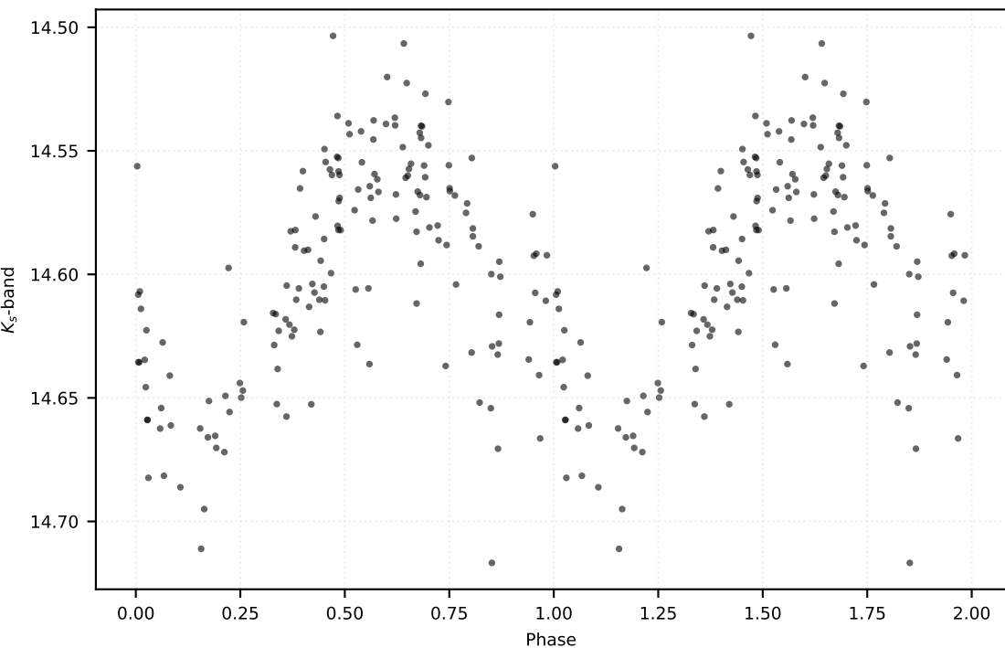
P: 3.16080 d | Class: RP | Subclass: CEP-1OT | Field b278
