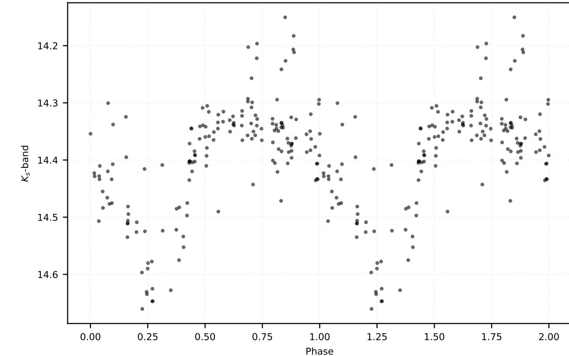
P: 0.45525 d | Class: RP | Subclass: RRab | Field b278
