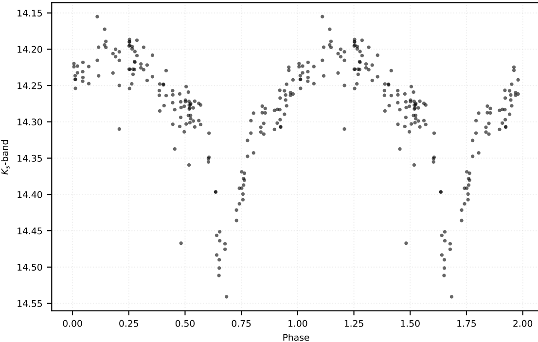
P: 0.60395 d | Class: RP | Subclass: CEP-1OT | Field b278
