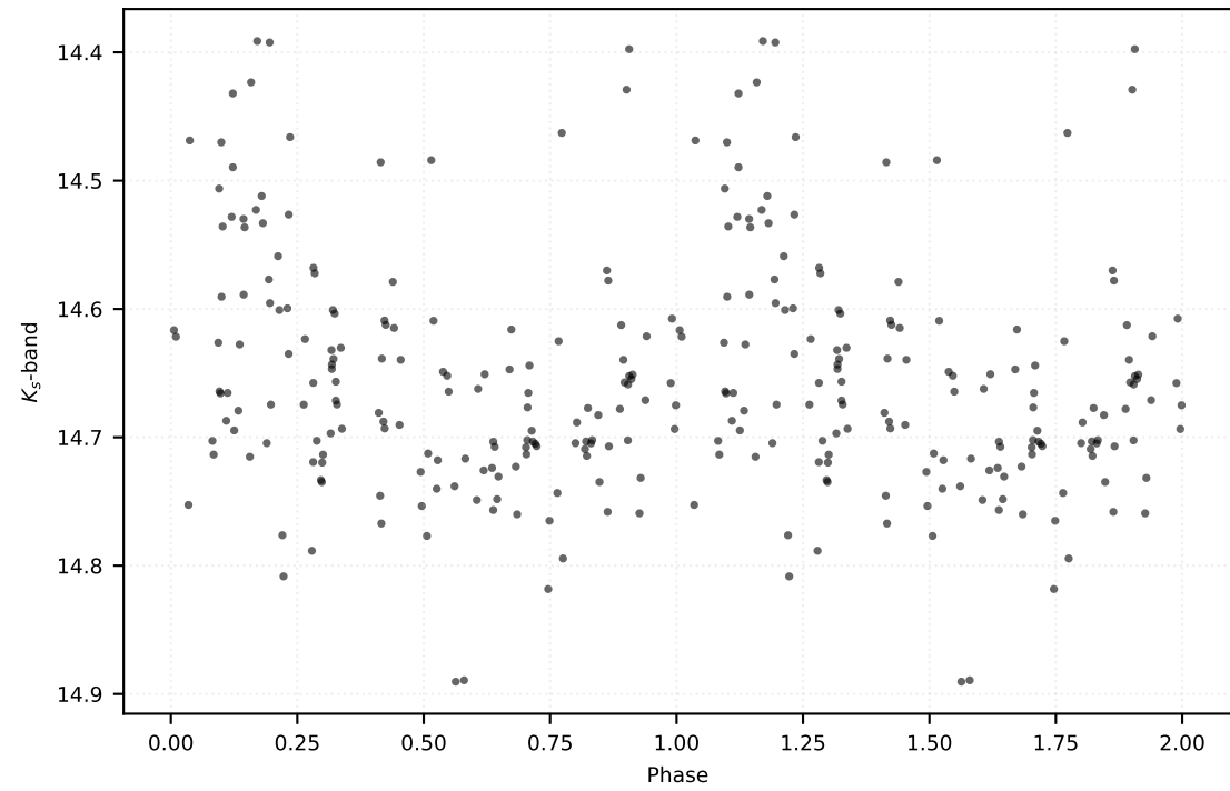
P: 0.17611 d | Class: RP | Subclass: UVAR | Field b278
