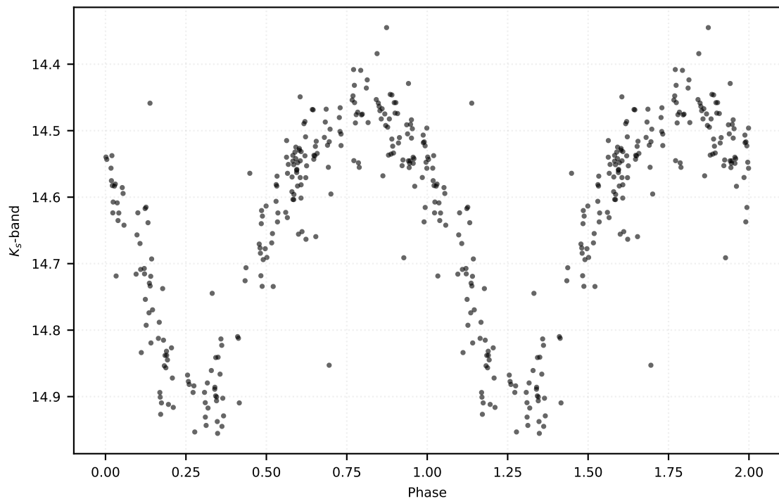
P: 1.10178 d | Class: EB | Subclass: UVAR | Field b278
