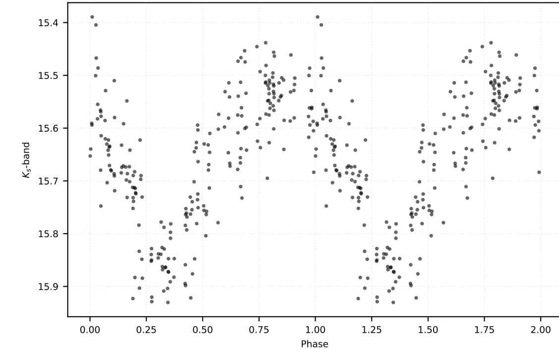
P: 0.44339 d | Class: RP | Subclass: RRc | Field b279
