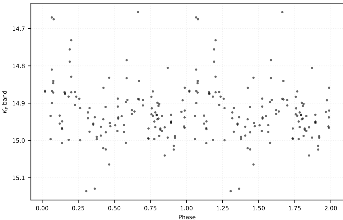
P: 0.21580 d | Class: EB | Subclass: EA | Field b279
