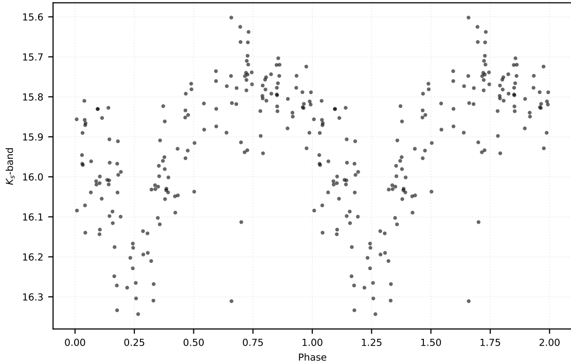
P: 0.84063 d | Class: RP | Subclass: RRab | Field b279
