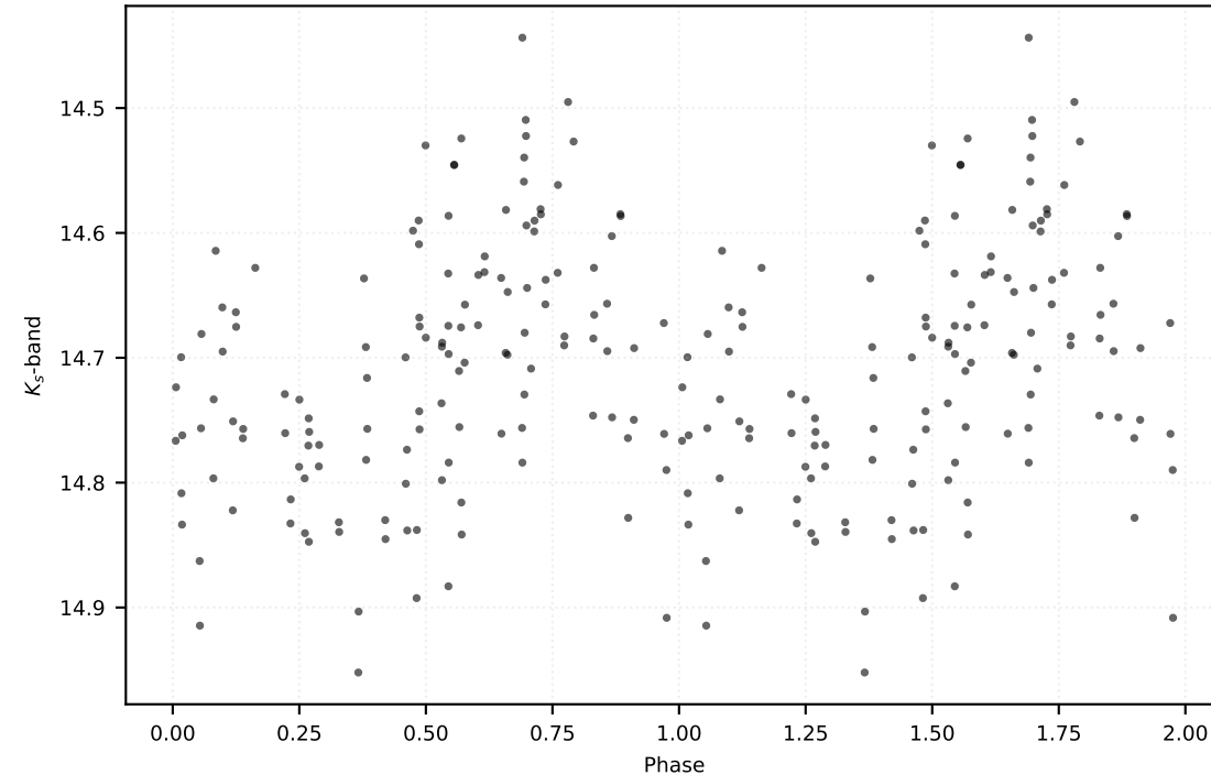
P: 0.73001 d | Class: RP | Subclass: RRab | Field b278
