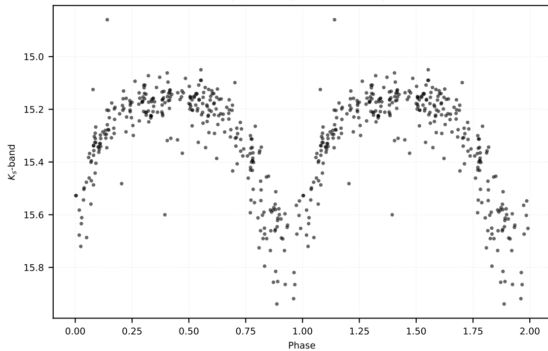
P: 0.20086 d | Class: RP | Subclass: UVAR | Field b279
