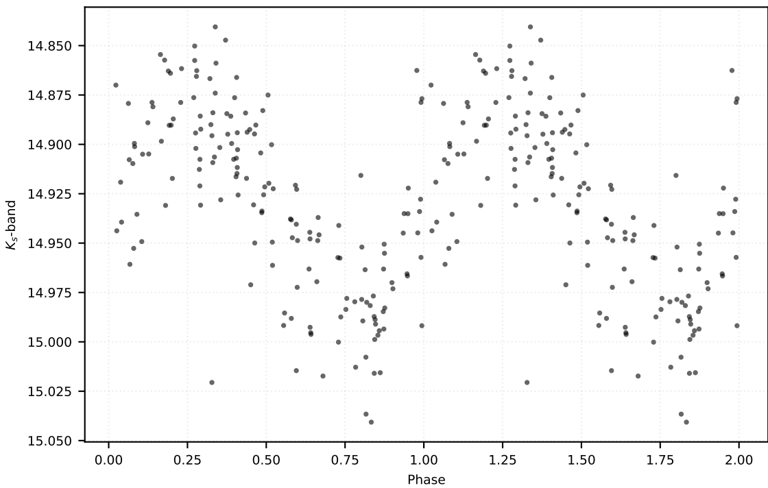
P: 0.28072 d | Class: RP | Subclass: RRc | Field b278
