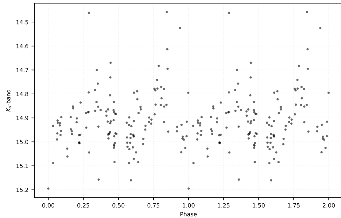
P: 2.11112 d | Class: EB | Subclass: EA | Field b279
