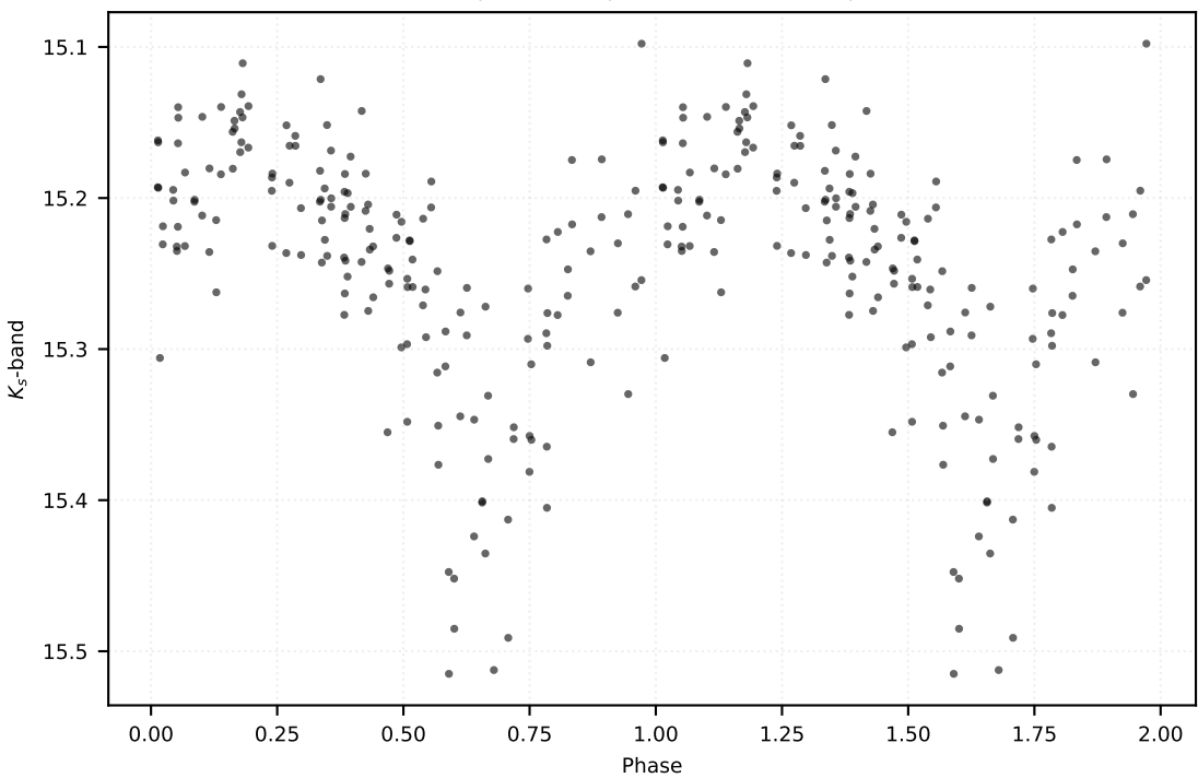
P: 0.68863 d | Class: RP | Subclass: CEP-10T | Field b279
