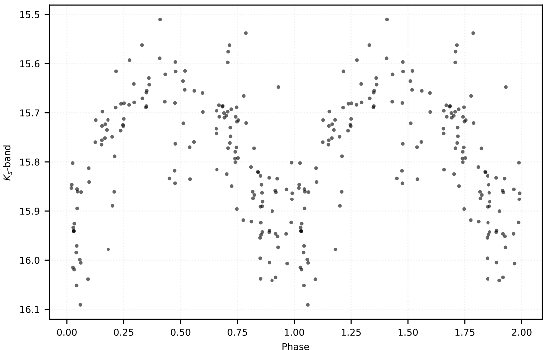
P: 0.33322 d | Class: RP | Subclass: CEP-10T | Field b279
