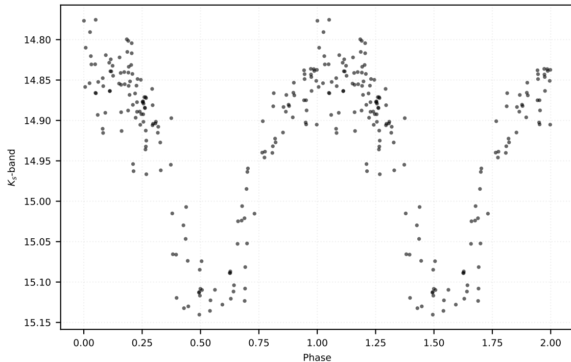
P: 4.25496 d | Class: RP | Subclass: CEP-1OT | Field b278
