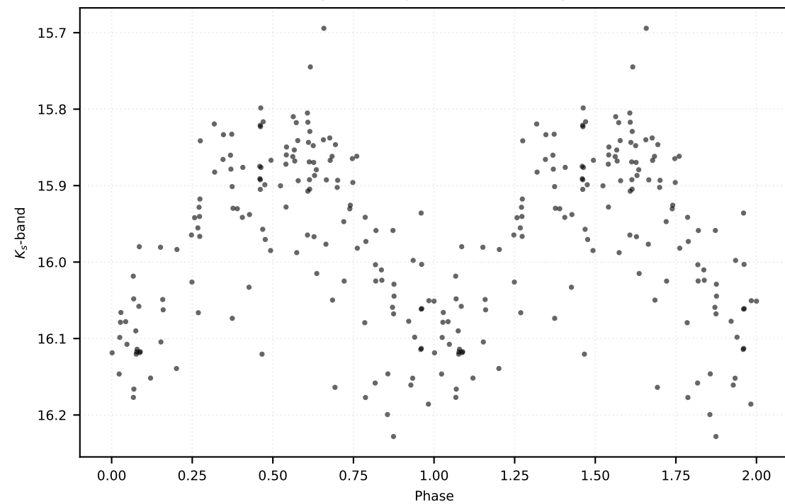
P: 0.46160 d | Class: RP | Subclass: CEP-10T | Field b278
