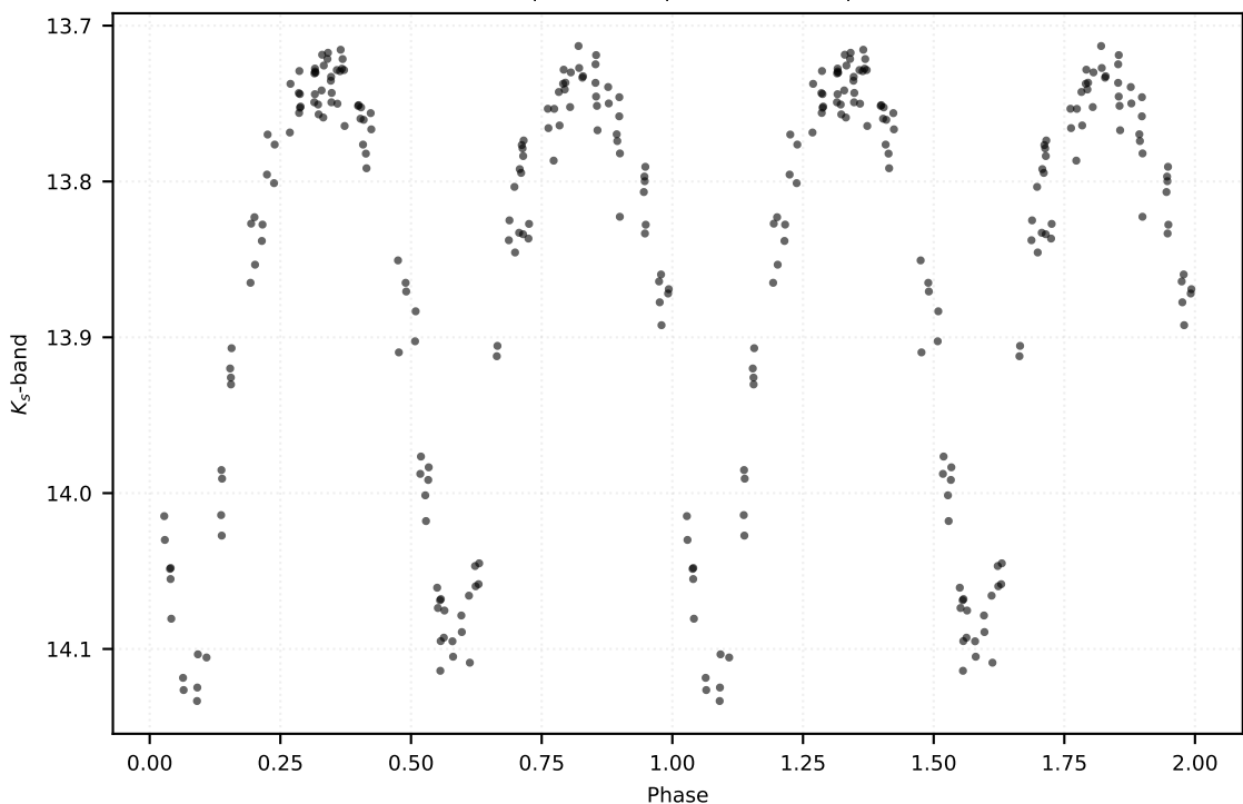
P: 0.34780 d | Class: EB | Subclass: EW | Field b279
