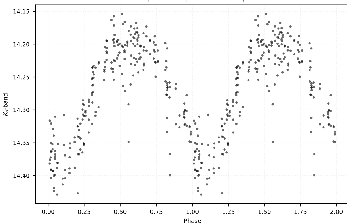
P: 0.42784 d | Class: RP | Subclass: RRab | Field b278
