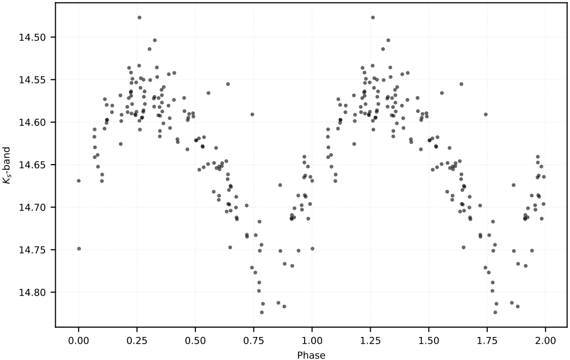
P: 0.38828 d | Class: RP | Subclass: RRab | Field b279
