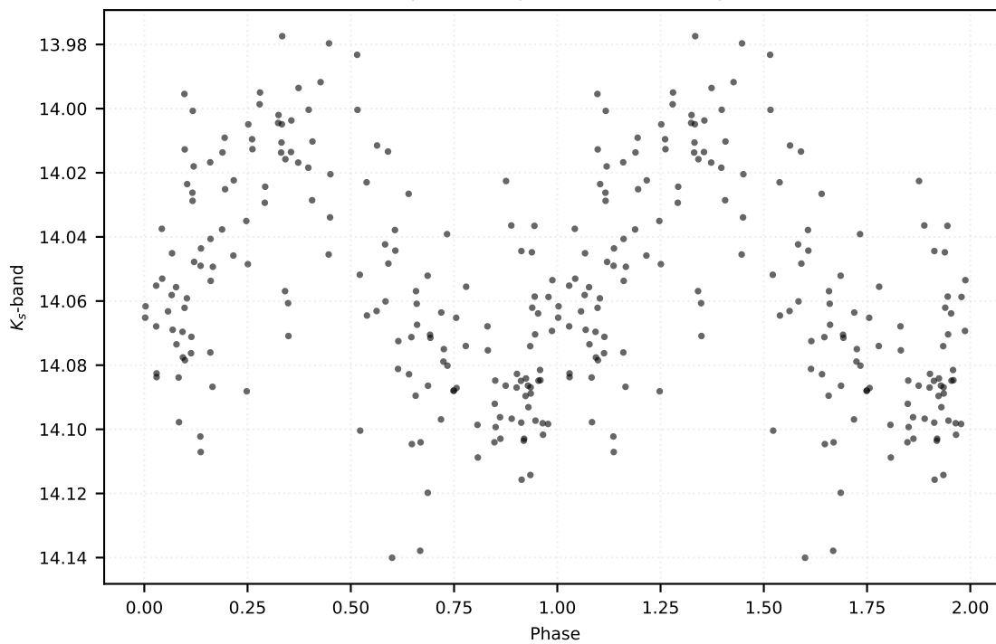
P: 0.54558 d | Class: RP | Subclass: CEP-1OT | Field b278
