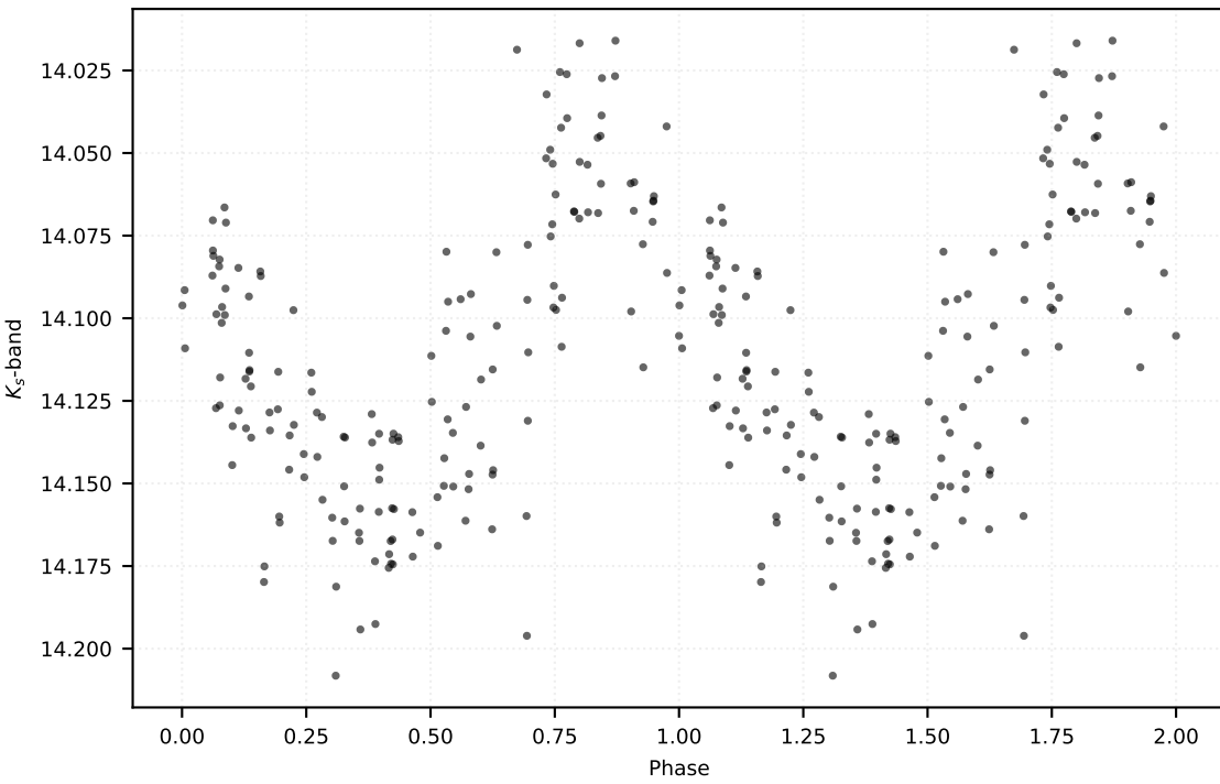
P: 0.47427 d | Class: RP | Subclass: RRab | Field b279
