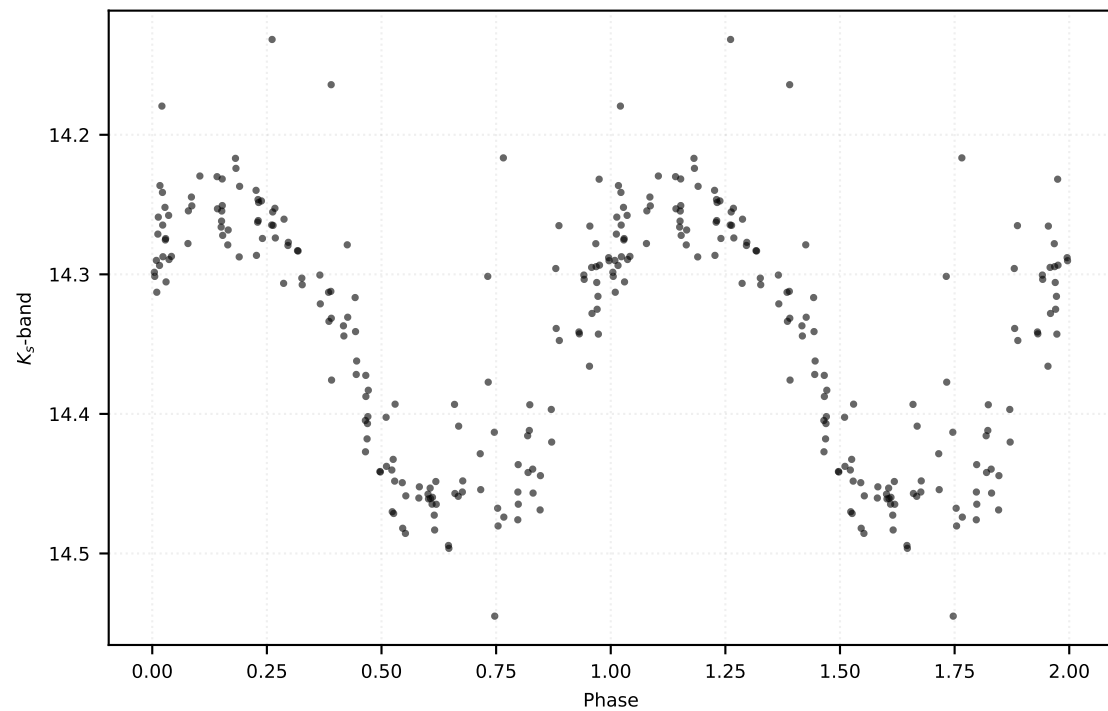
P: 0.48902 d | Class: RP | Subclass: RRab | Field b279
