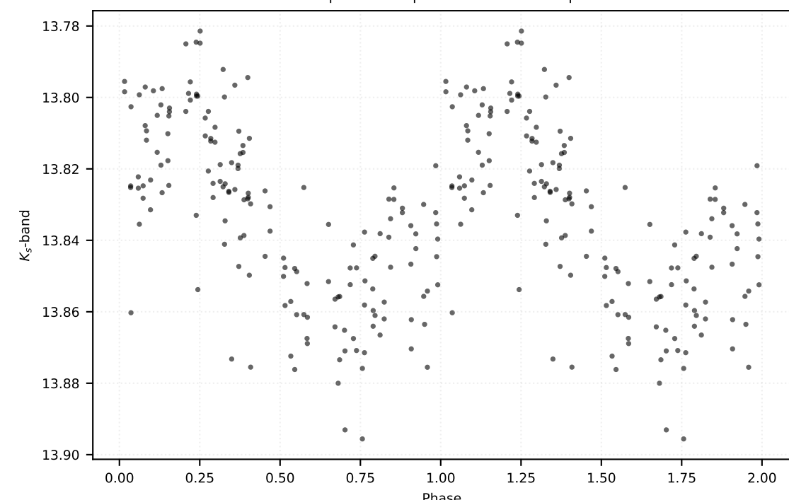
P: 5.25430 d | Class: RP | Subclass: CEP-10T | Field b279
