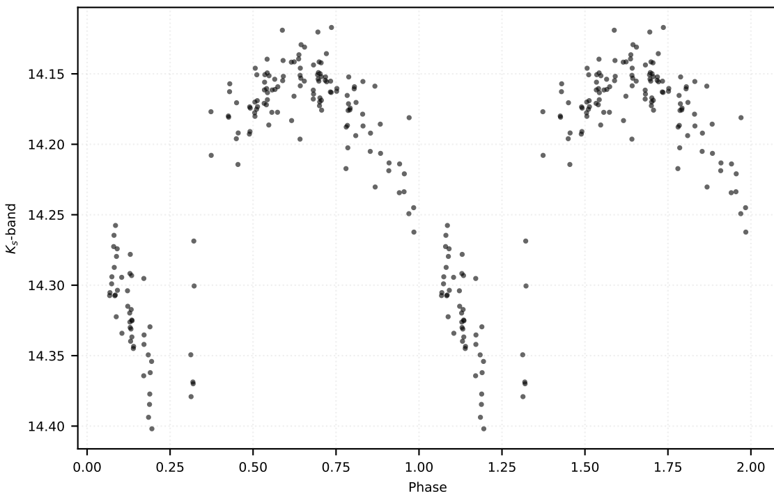
P: 0.84086 d | Class: RP | Subclass: RRab | Field b278
