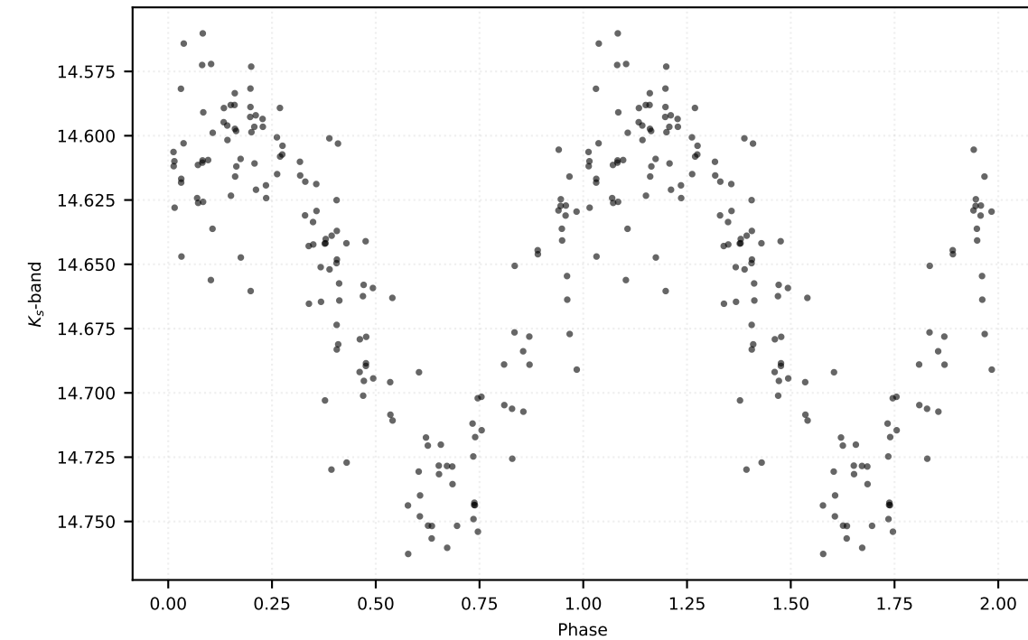
P: 0.36109 d | Class: RP | Subclass: RRab | Field b279
