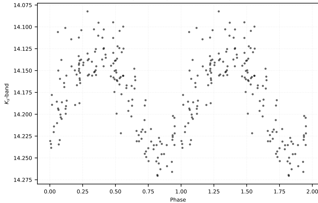
P: 0.40495 d | Class: RP | Subclass: CEP-10T | Field b279
