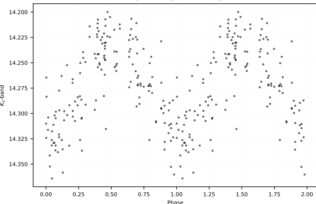
P: 0.21674 d | Class: RP | Subclass: RRc | Field b279
