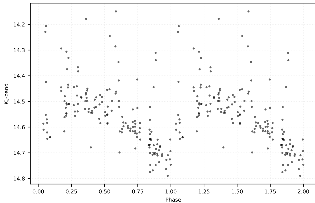
P: 0.51881 d | Class: RP | Subclass: RRab | Field b278
