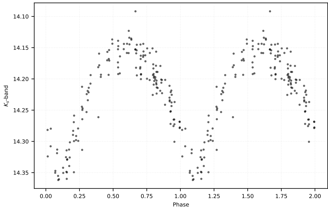
P: 1.54400 d | Class: RP | Subclass: CEP-10T | Field b278
