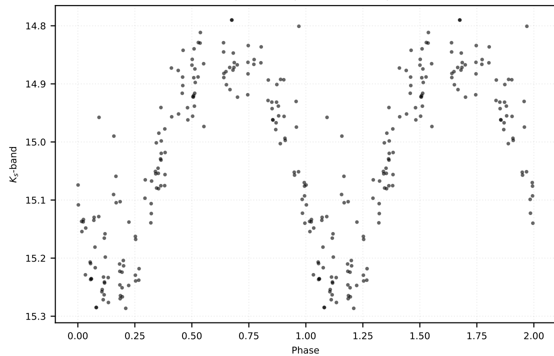
P: 0.45122 d | Class: RP | Subclass: RRab | Field b279
