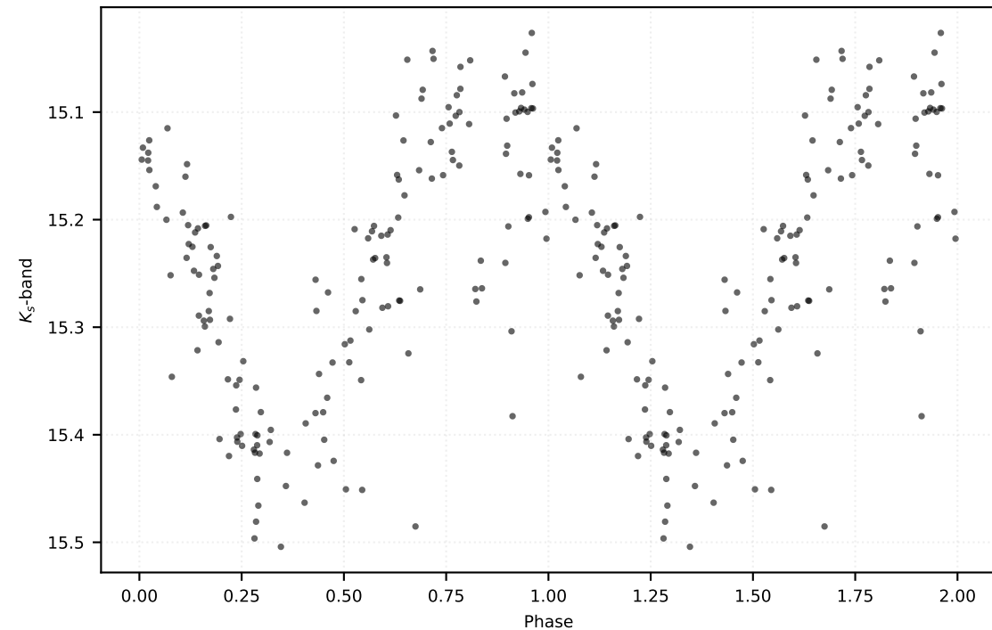
P: 0.14813 d | Class: RP | Subclass: UVAR | Field b278
