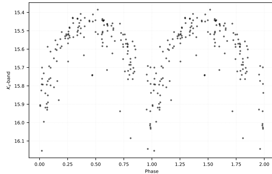
P: 0.45960 d | Class: RP | Subclass: RRab | Field b279
