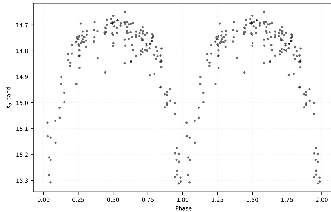
P: 0.43739 d | Class: RP | Subclass: RRc | Field b278
