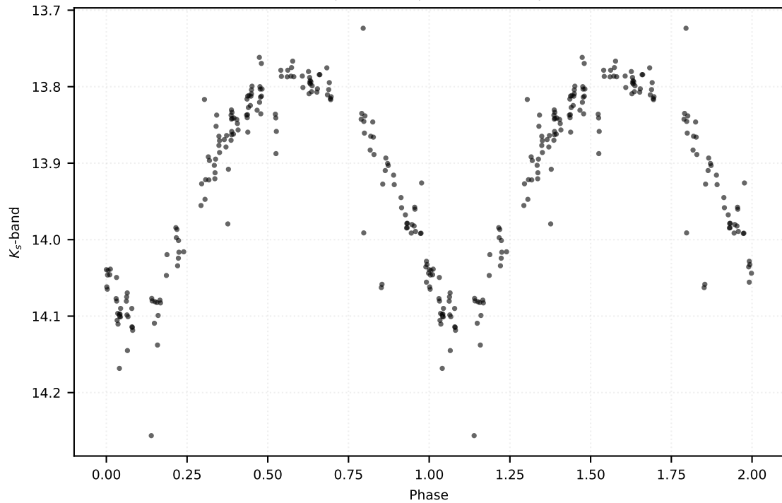
P: 0.24453 d | Class: RP | Subclass: RRc | Field b278
