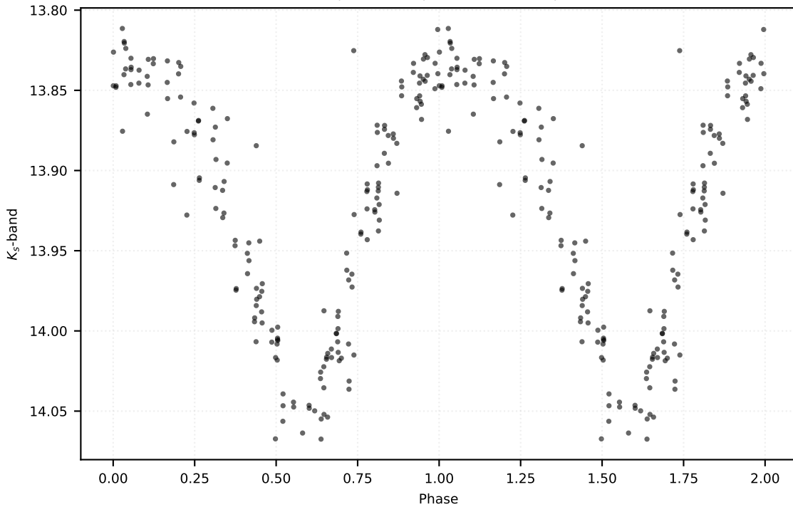
P: 0.49705 d | Class: RP | Subclass: RRab | Field b278
