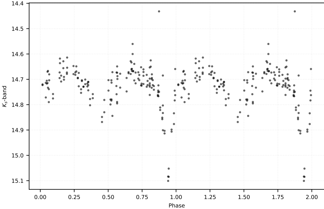
P: 0.25924 d | Class: EB | Subclass: EA | Field b279
