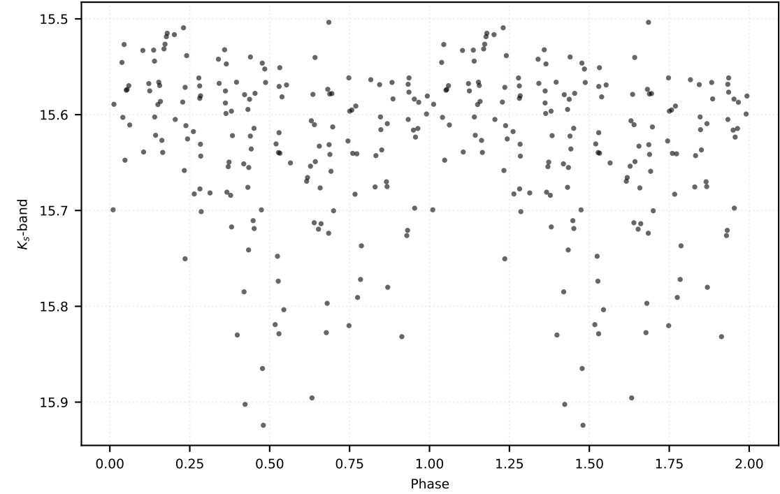
P: 0.15120 d | Class: RP | Subclass: UVAR | Field b278
