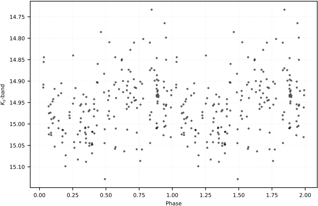
P: 0.42791 d | Class: RP | Subclass: RRc | Field b279
