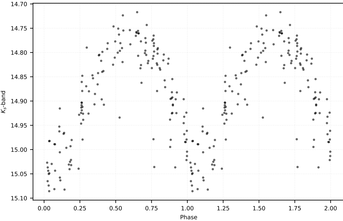
P: 0.37689 d | Class: RP | Subclass: RRc | Field b278
