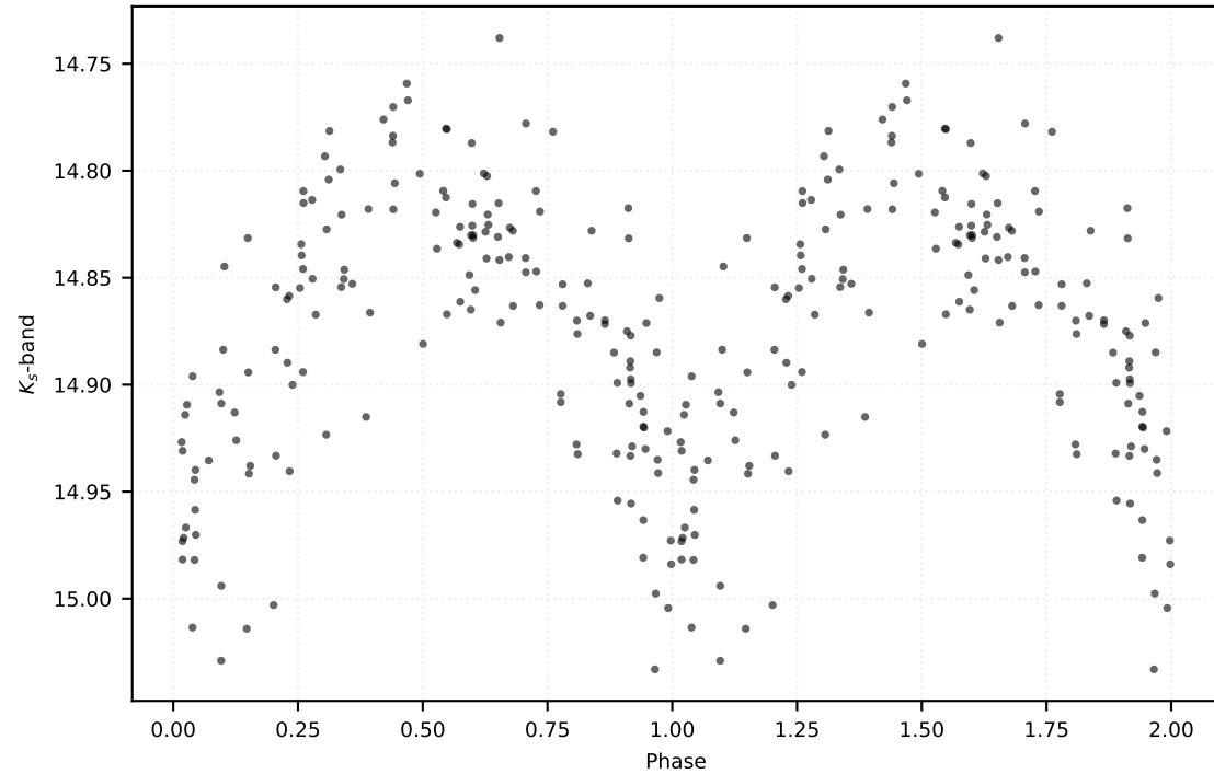
P: 79.78355 d | Class: RP | Subclass: CEP-F | Field b279
