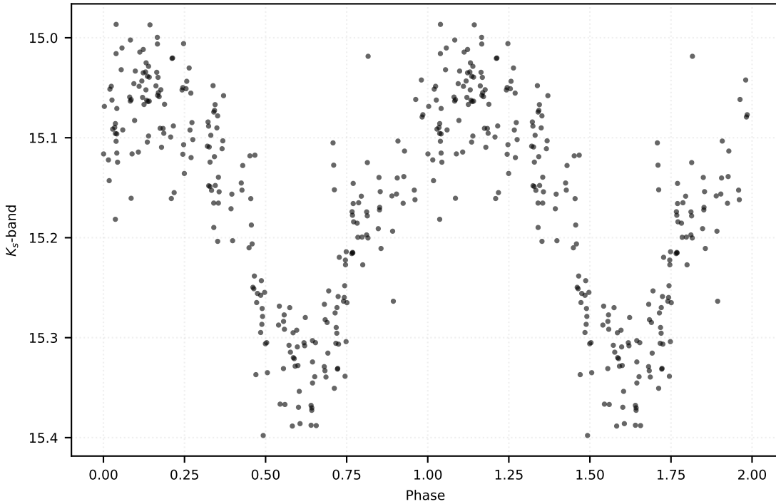
P: 0.19885 d | Class: RP | Subclass: UVAR | Field b278
