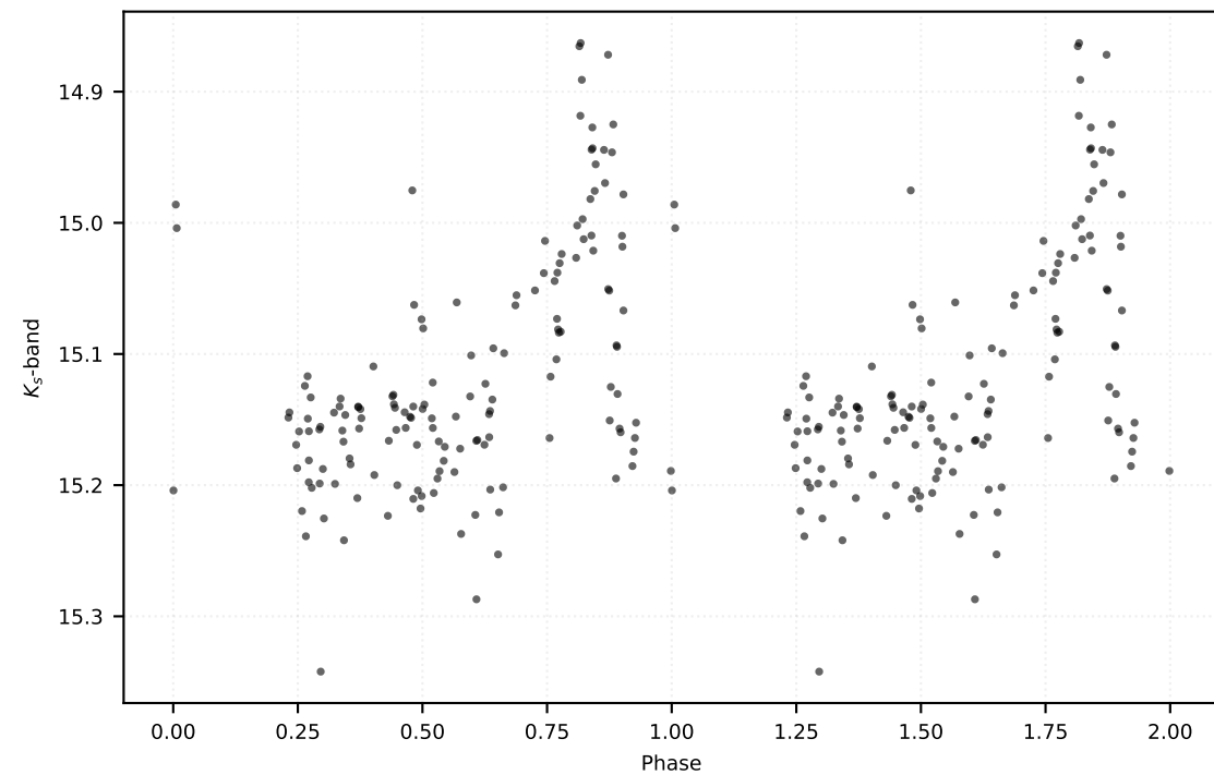
P: 0.11028 d | Class: RP | Subclass: UVAR | Field b279
