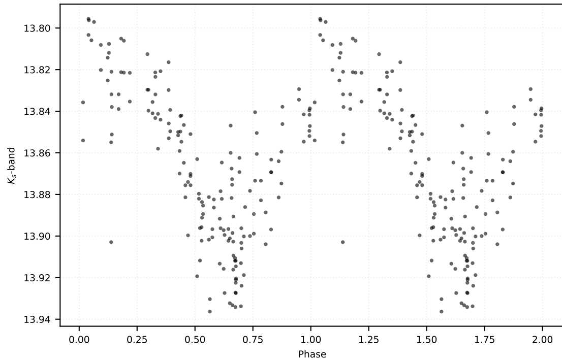
P: 7.21905 d | Class: RP | Subclass: CEP-F | Field b279
