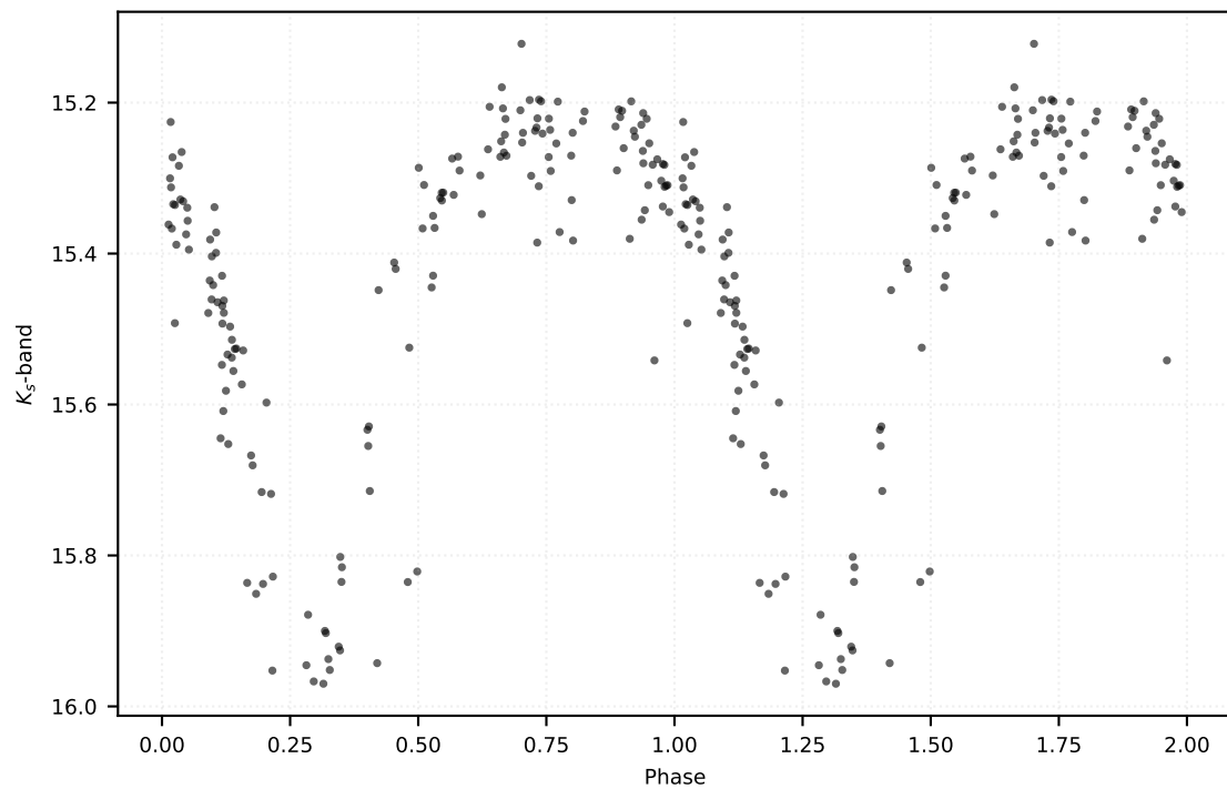
P: 19.07863 d | Class: RP | Subclass: UVAR | Field b278
