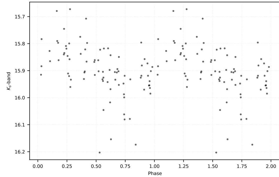
P: 0.10134 d | Class: RP | Subclass: UVAR | Field b279
