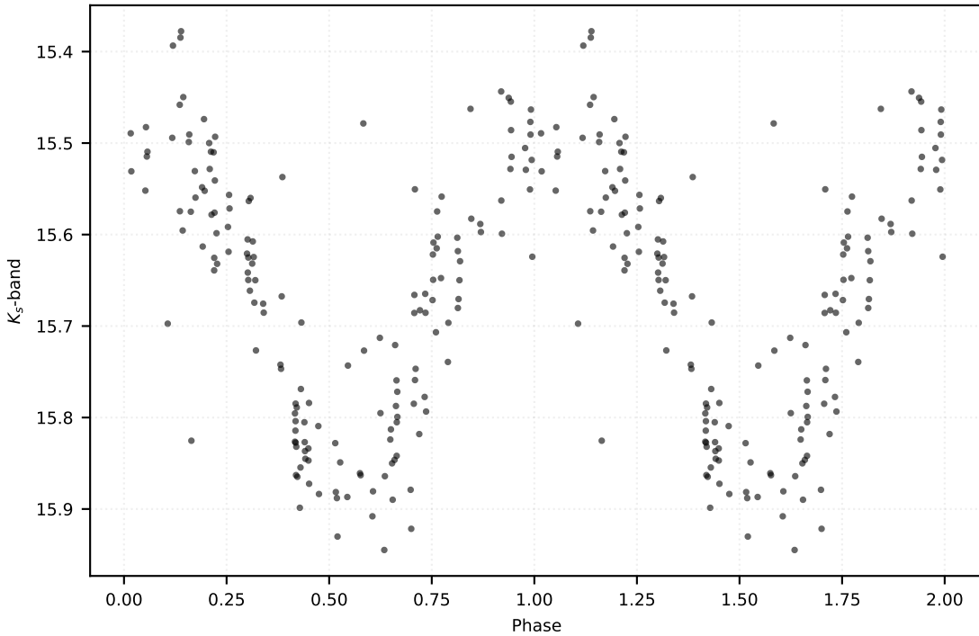
P: 0.18856 d | Class: RP | Subclass: UVAR | Field b278
