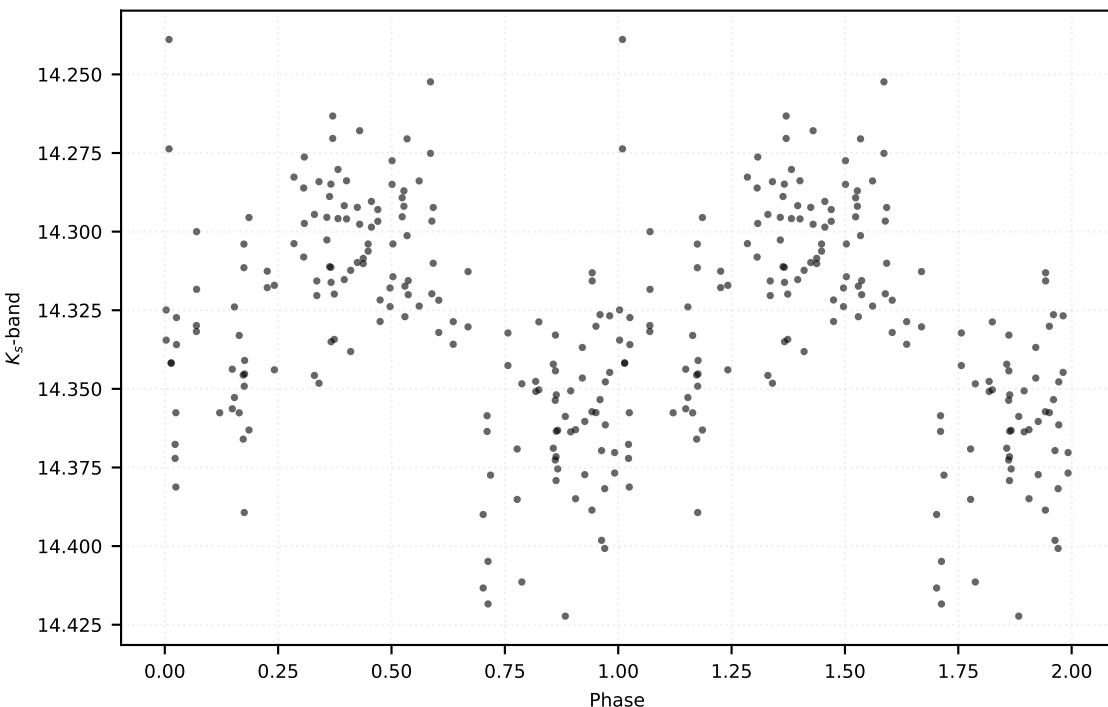
P: 0.16528 d | Class: RP | Subclass: UVAR | Field b278
