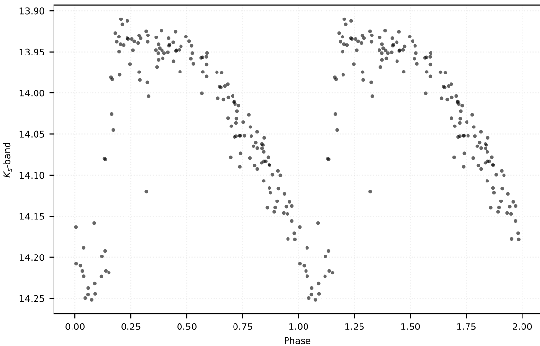
P: 0.55705 d | Class: RP | Subclass: RRab | Field b279
