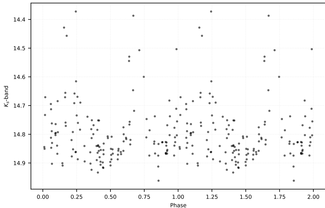
P: 0.22169 d | Class: EB | Subclass: EA | Field b278
