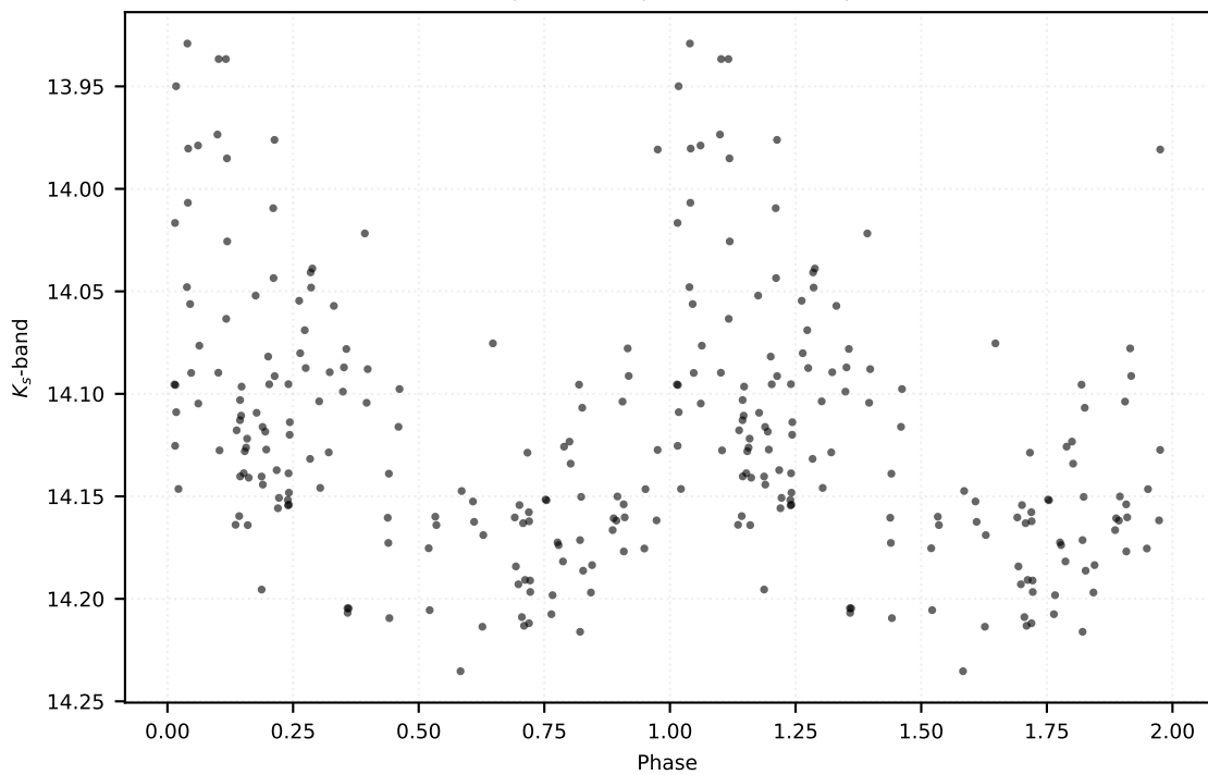
P: 19.70174 d | Class: RP | Subclass: UVAR | Field b278
