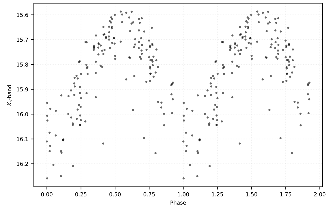
P: 0.79207 d | Class: RP | Subclass: CEP-10T | Field b279
