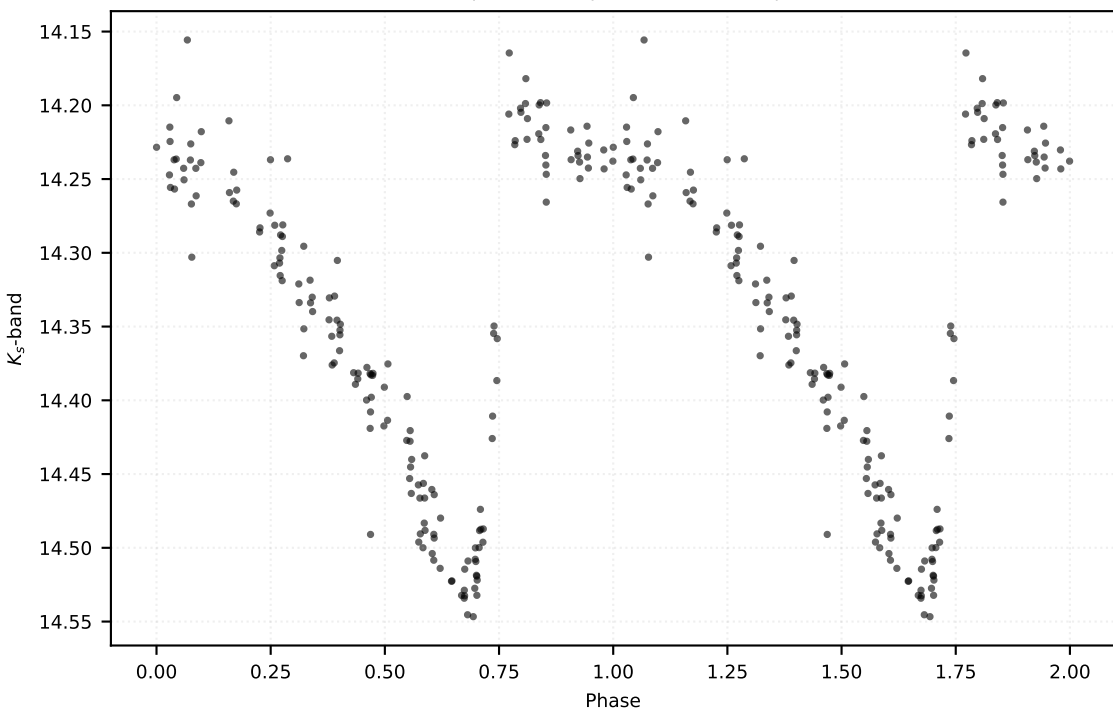
P: 0.46136 d | Class: RP | Subclass: RRab | Field b278
