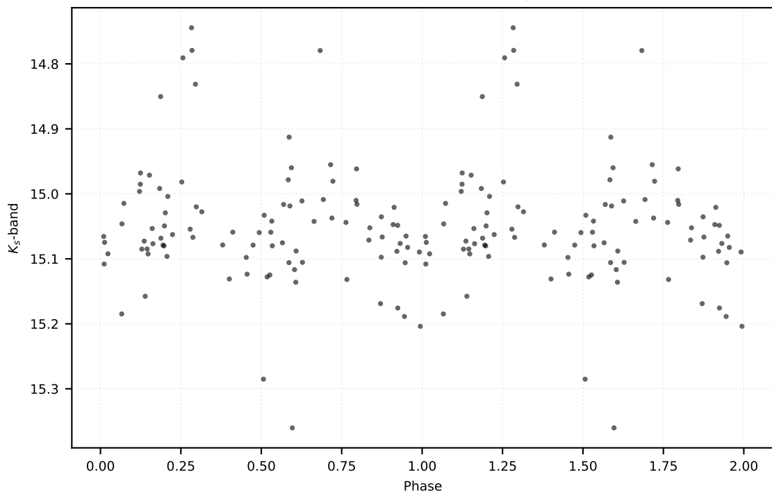
P: 0.56216 d | Class: EB | Subclass: EA | Field b278
