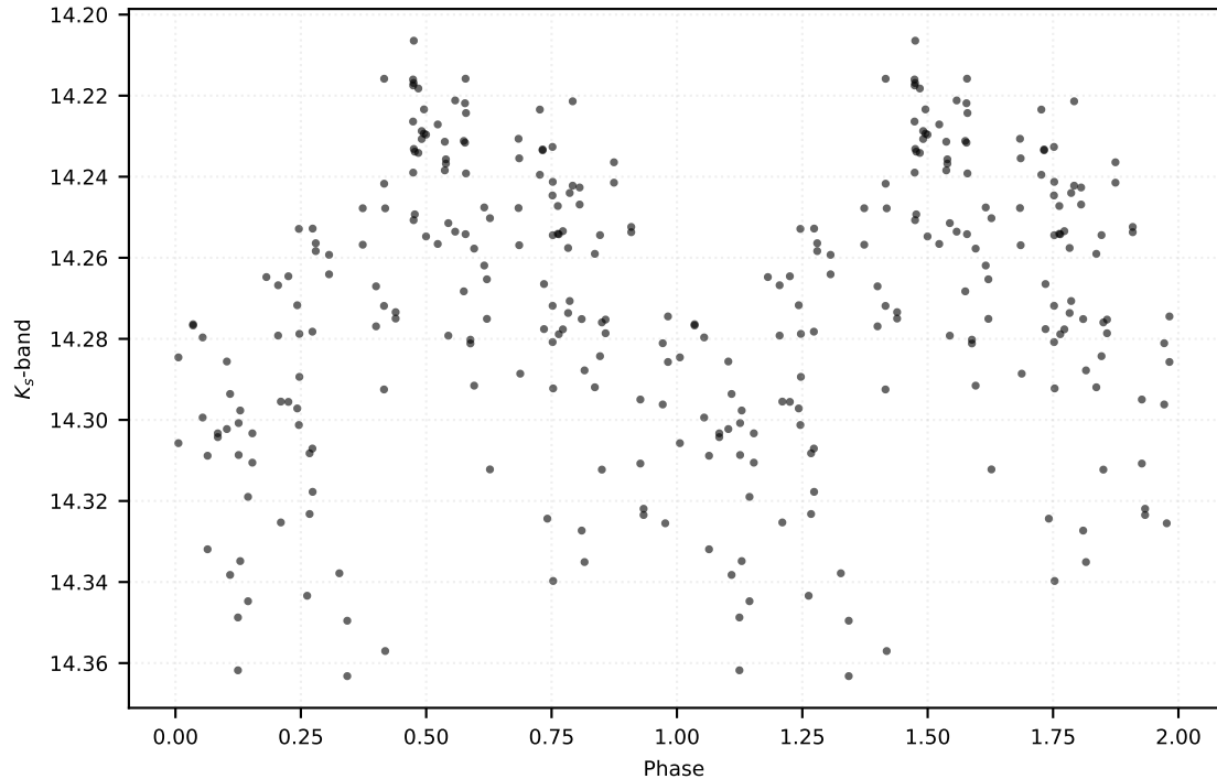
P: 48.14498 d | Class: RP | Subclass: CEP-F | Field b278
