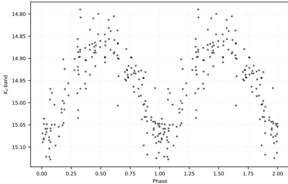
P: 0.22639 d | Class: RP | Subclass: UVAR | Field b278
