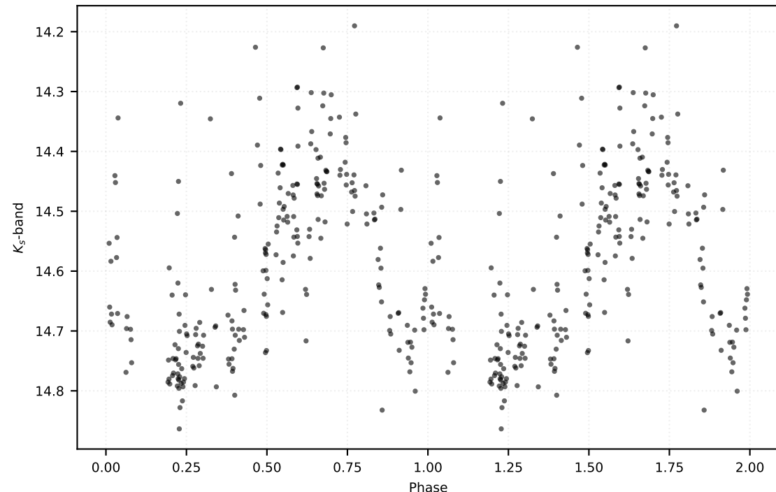
P: 0.57134 d | Class: RP | Subclass: CEP-1OT | Field b278
