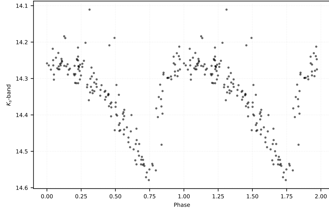
P: 0.47363 d | Class: RP | Subclass: RRab | Field b278
