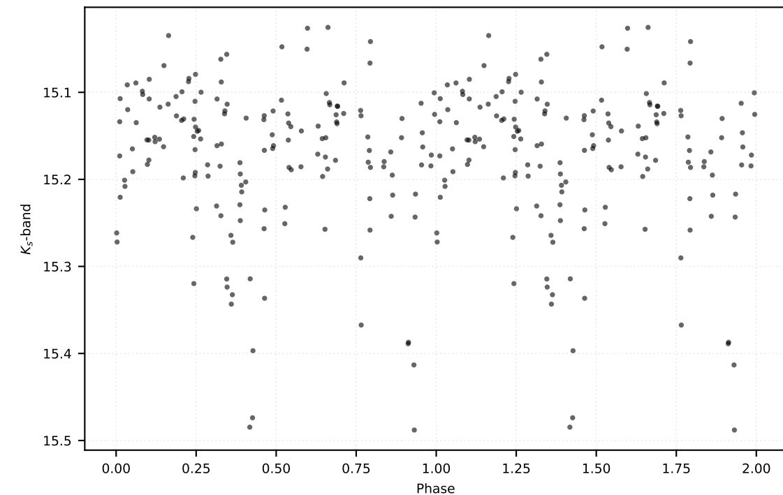
P: 0.70420 d | Class: EB | Subclass: EA | Field b279
