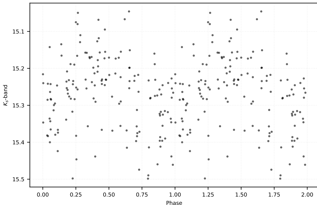
P: 0.37755 d | Class: RP | Subclass: CEP-10T | Field b278
