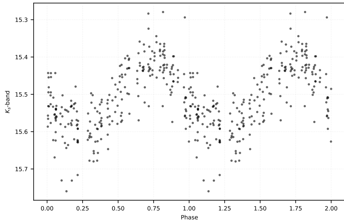
P: 0.43318 d | Class: RP | Subclass: RRab | Field b278
