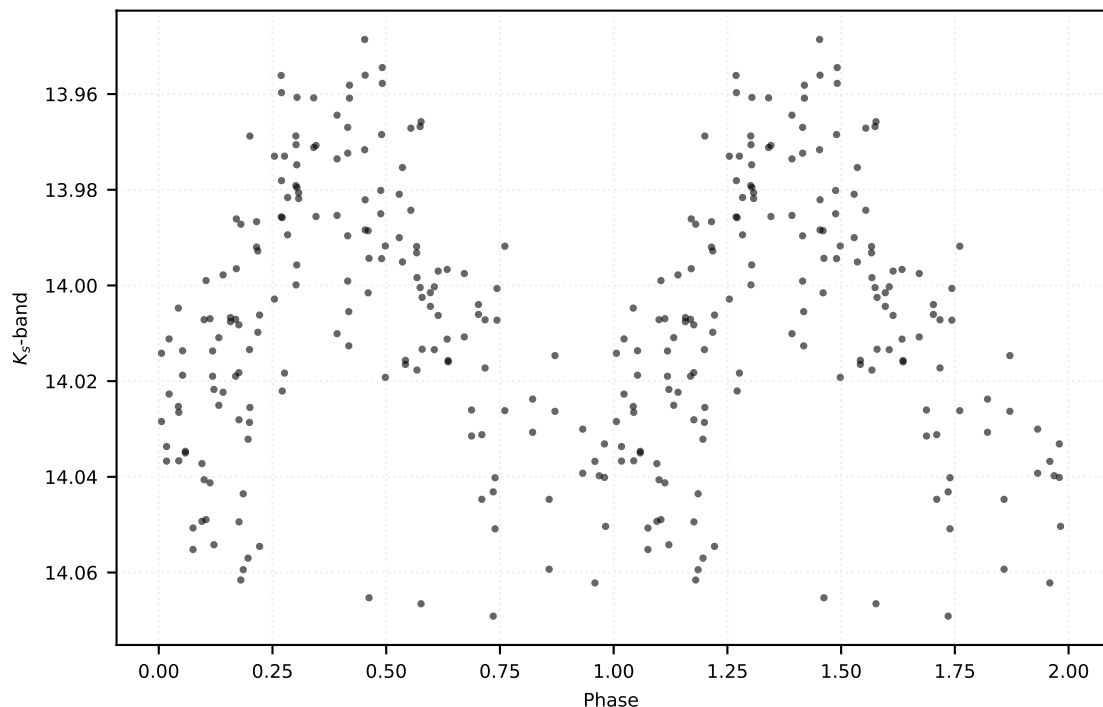
P: 71.02515 d | Class: RP | Subclass: CEP-F | Field b278
