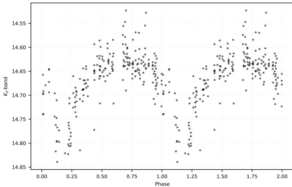
P: 2.26141 d | Class: RP | Subclass: CEP-F | Field b278
