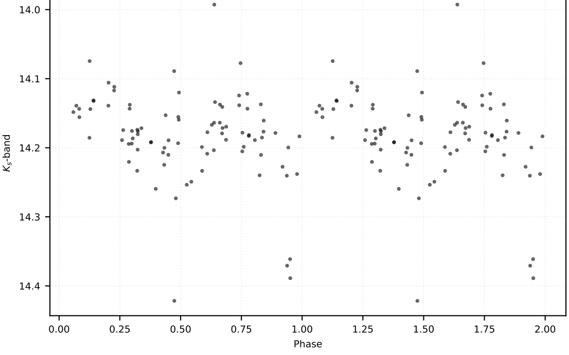
P: 0.54058 d | Class: EB | Subclass: EA | Field b278
