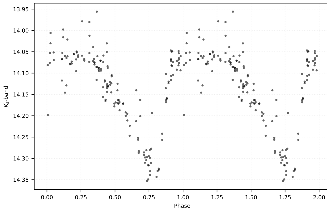
P: 0.54965 d | Class: RP | Subclass: RRab | Field b279
