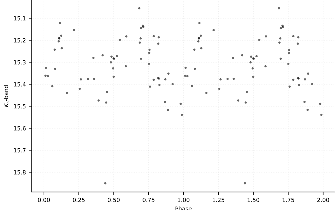
P: 0.22056 d | Class: EB | Subclass: EA | Field b278
