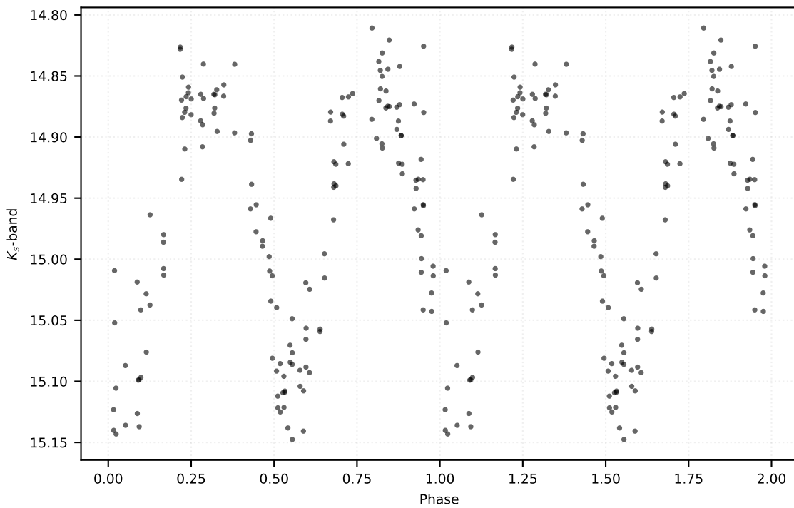
P: 0.20424 d | Class: RP | Subclass: RRc | Field b279
