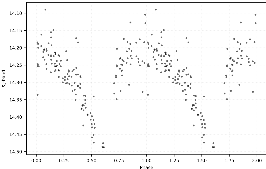
P: 0.39755 d | Class: RP | Subclass: RRab | Field b279
