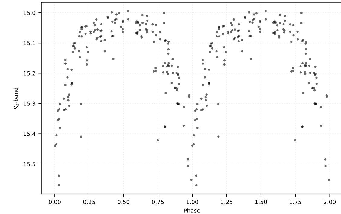
P: 0.35070 d | Class: RP | Subclass: RRc | Field b279
