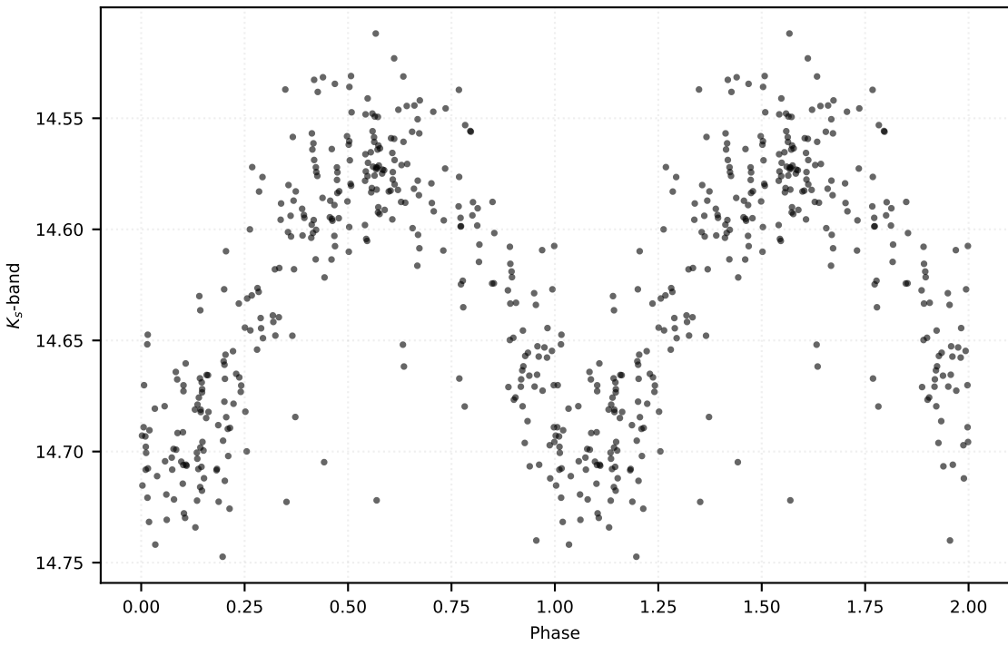
P: 0.37369 d | Class: RP | Subclass: RRab | Field b279
