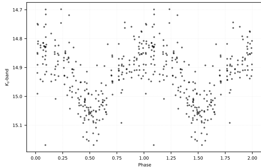
P: 0.34299 d | Class: RP | Subclass: CEP-10T | Field b279
