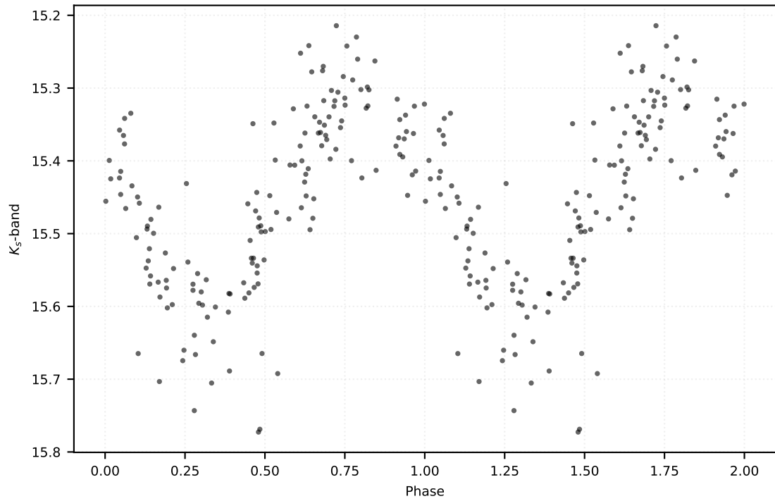
P: 0.20300 d | Class: RP | Subclass: UVAR | Field b278
