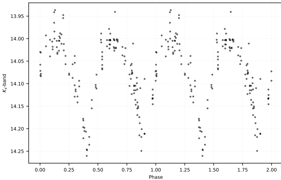
P: 0.53270 d | Class: RP | Subclass: RRc | Field b278
