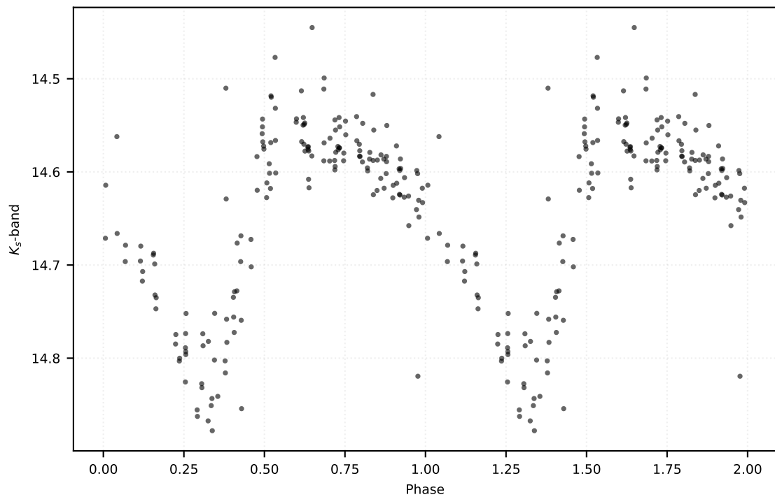
P: 0.36960 d | Class: RP | Subclass: RRab | Field b279
