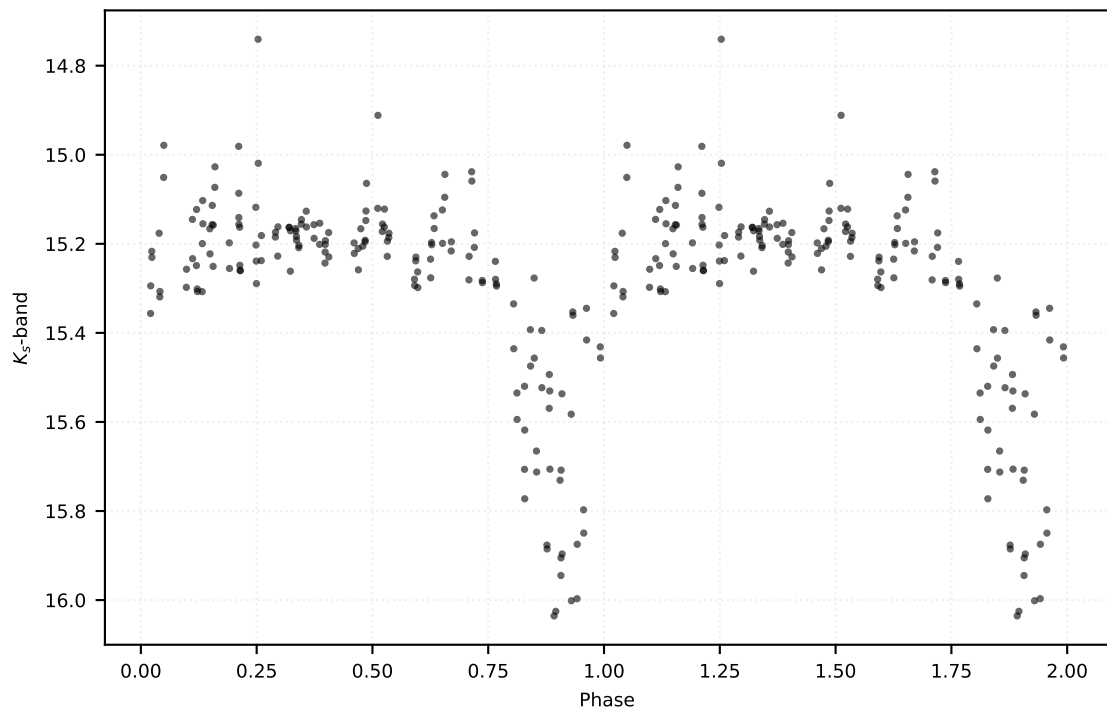
P: 1.88924 d | Class: RP | Subclass: CEP-F | Field b278
