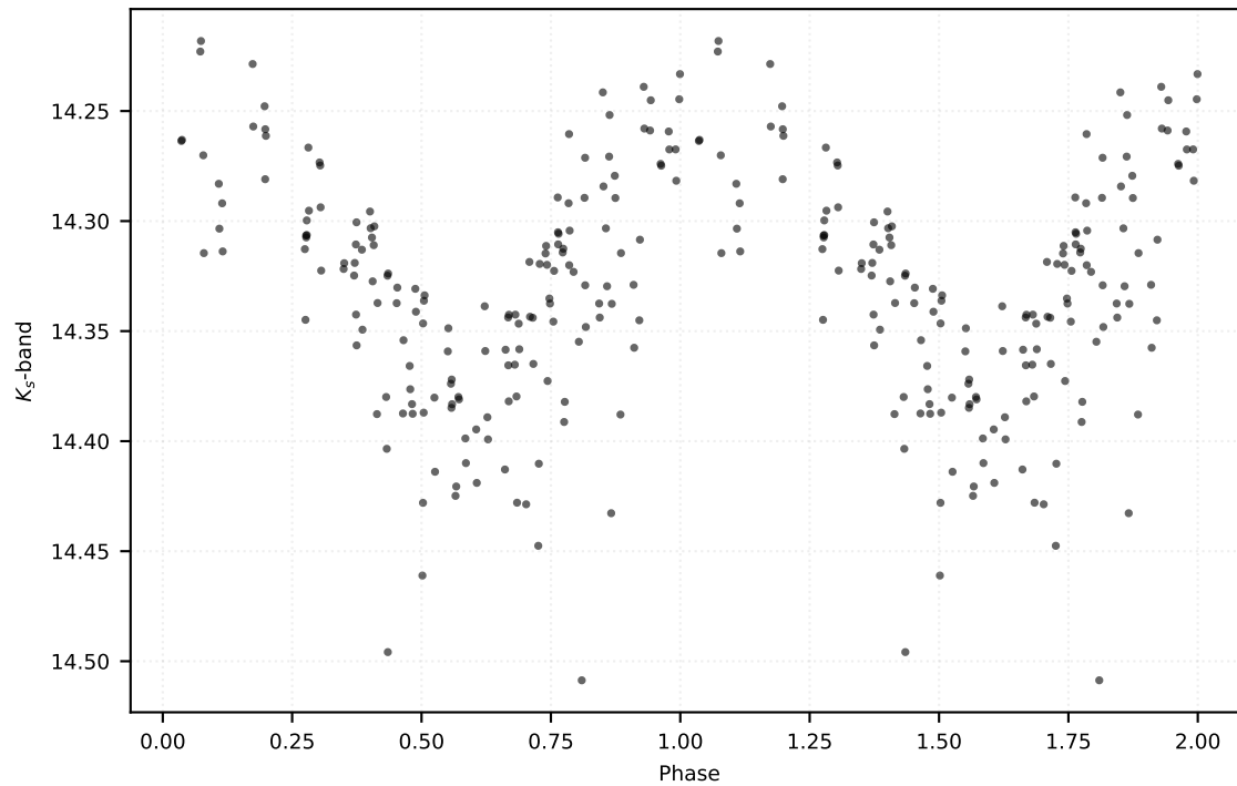
P: 0.45874 d | Class: RP | Subclass: RRab | Field b279
