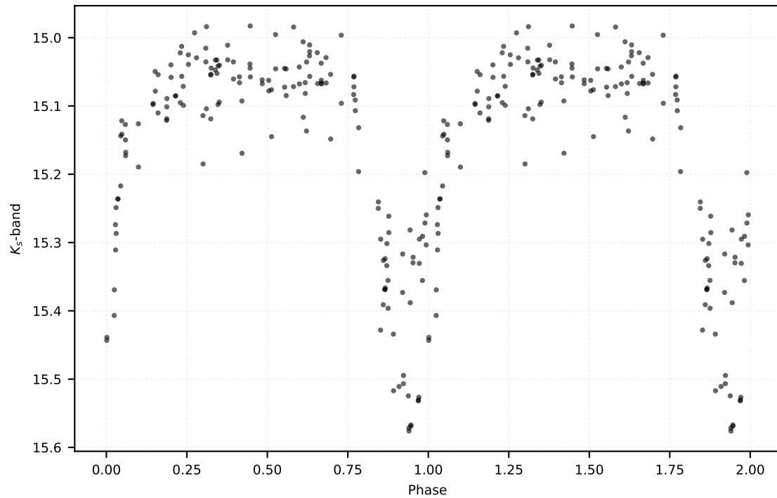
P: 1.93571 d | Class: RP | Subclass: CEP-F | Field b279
