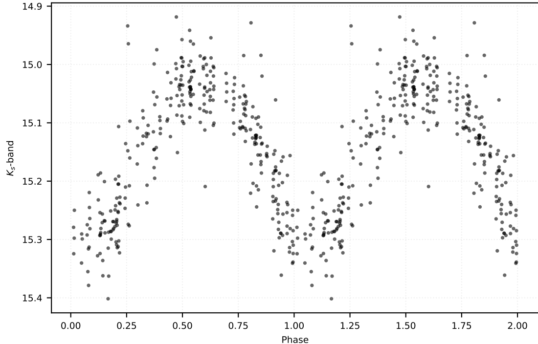
P: 0.68104 d | Class: RP | Subclass: RRab | Field b279
