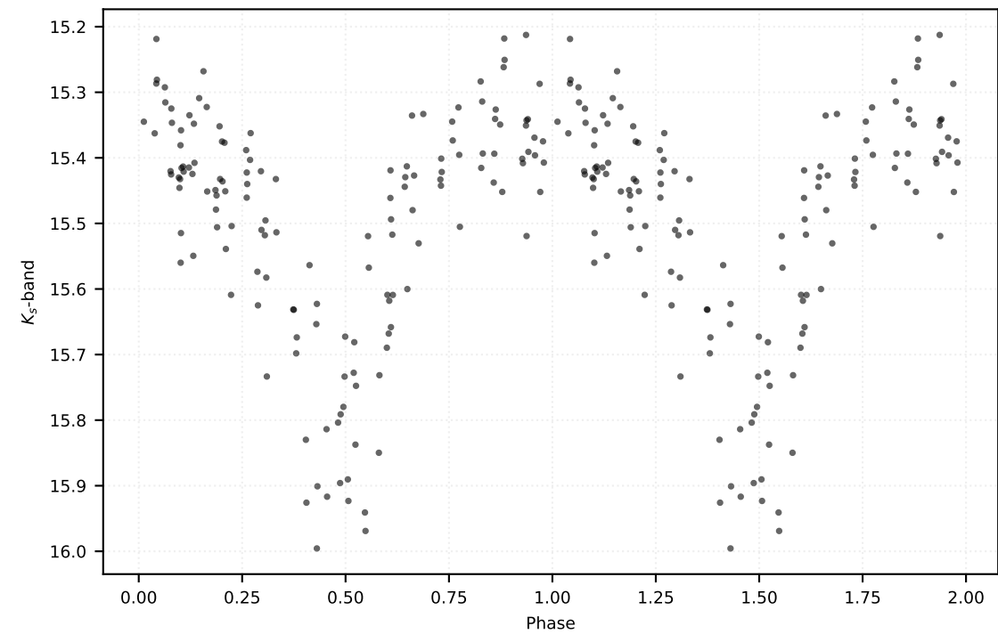
P: 1.23190 d | Class: EB | Subclass: RRc | Field b278
