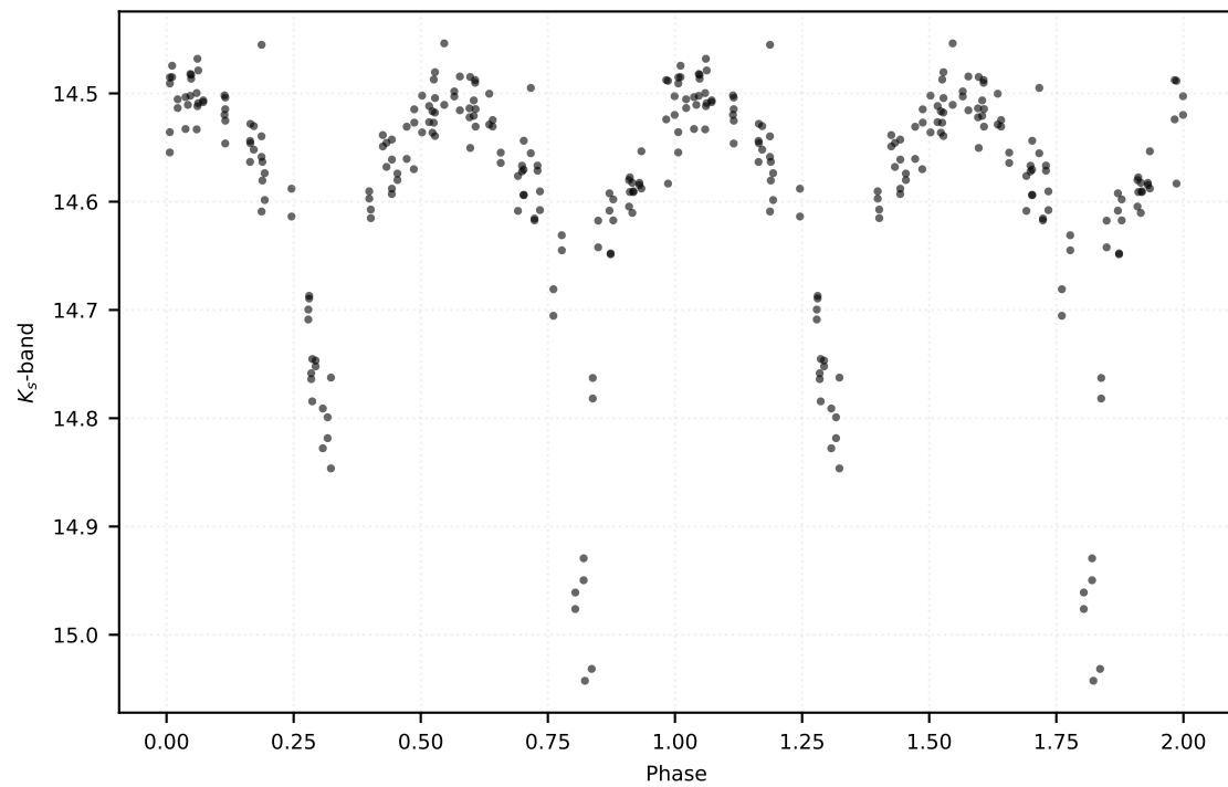
P: 4.07083 d | Class: EB | Subclass: EA | Field b278
