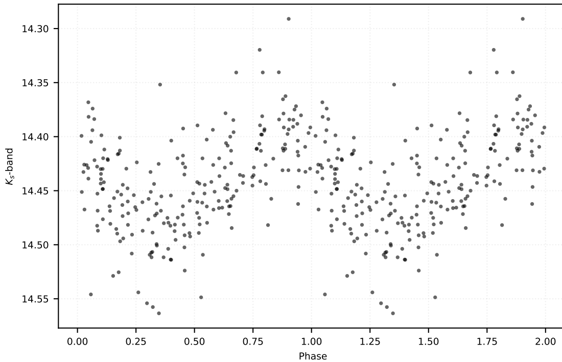
P: 0.70350 d | Class: RP | Subclass: RRab | Field b278
