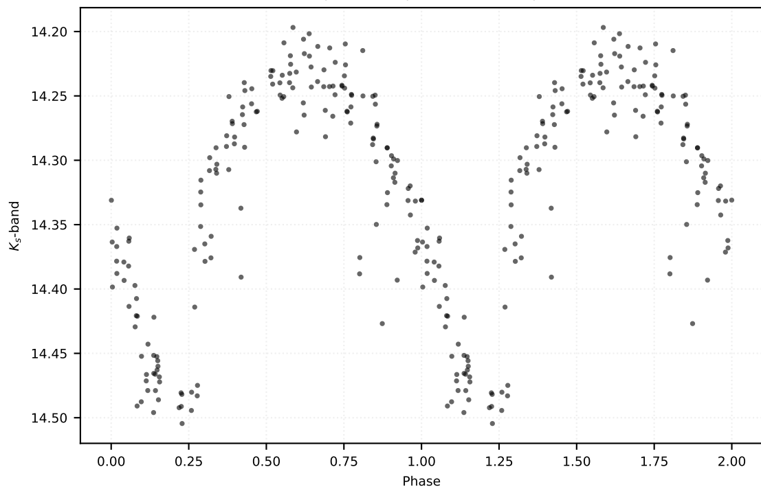
P: 0.45873 d | Class: RP | Subclass: RRab | Field b278
