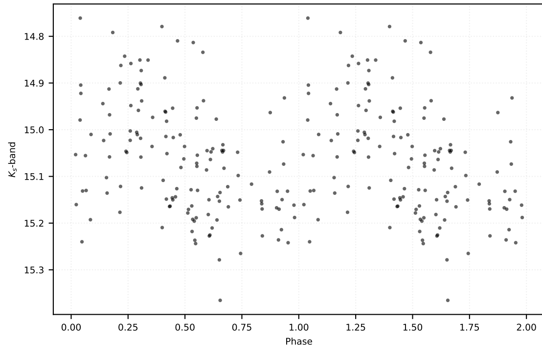
P: 0.15977 d | Class: RP | Subclass: UVAR | Field b279
