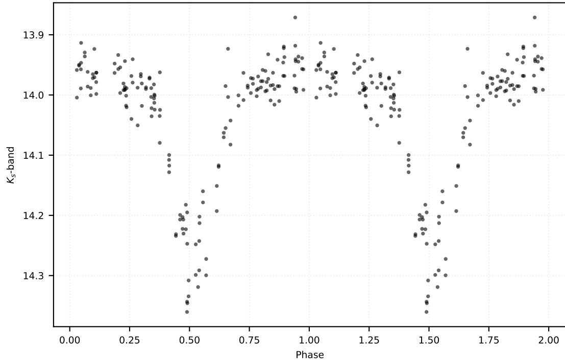
P: 1.59331 d | Class: RP | Subclass: CEP-F | Field b279
