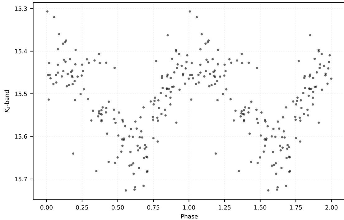
P: 0.29508 d | Class: RP | Subclass: UVAR | Field b279
