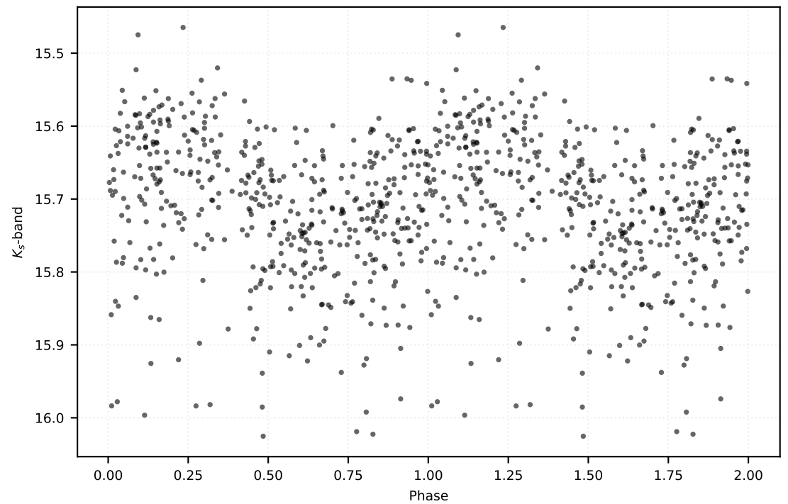
P: 2.56198 d | Class: RP | Subclass: CEP-F | Field b279
