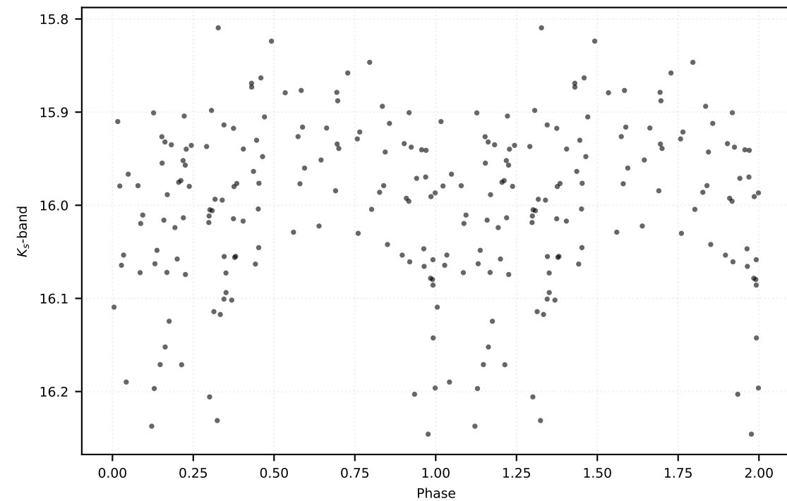
P: 0.16196 d | Class: RP | Subclass: UVAR | Field b279
