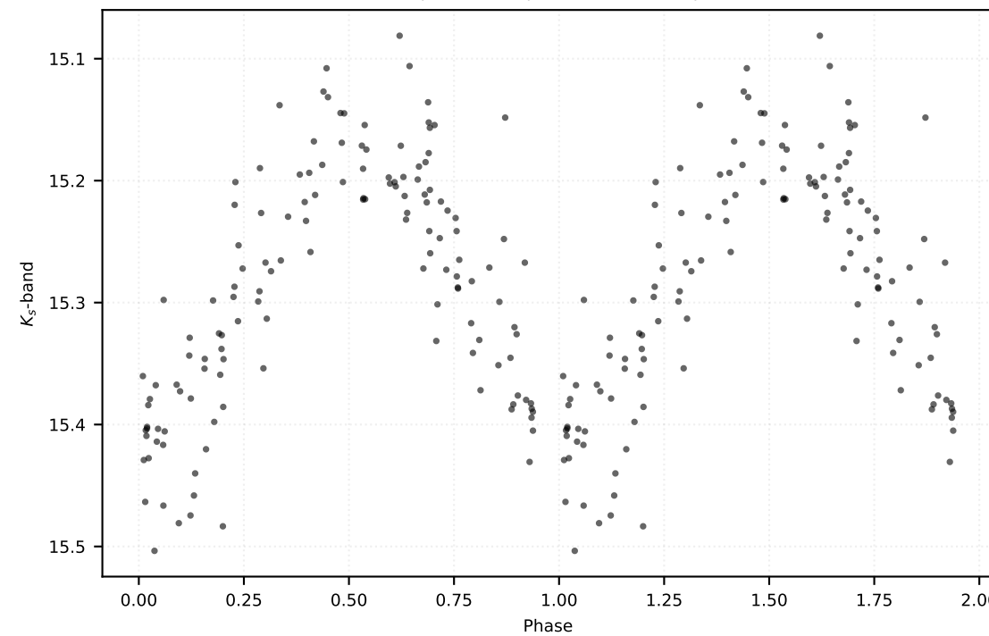
P: 0.22872 d | Class: RP | Subclass: UVAR | Field b278
