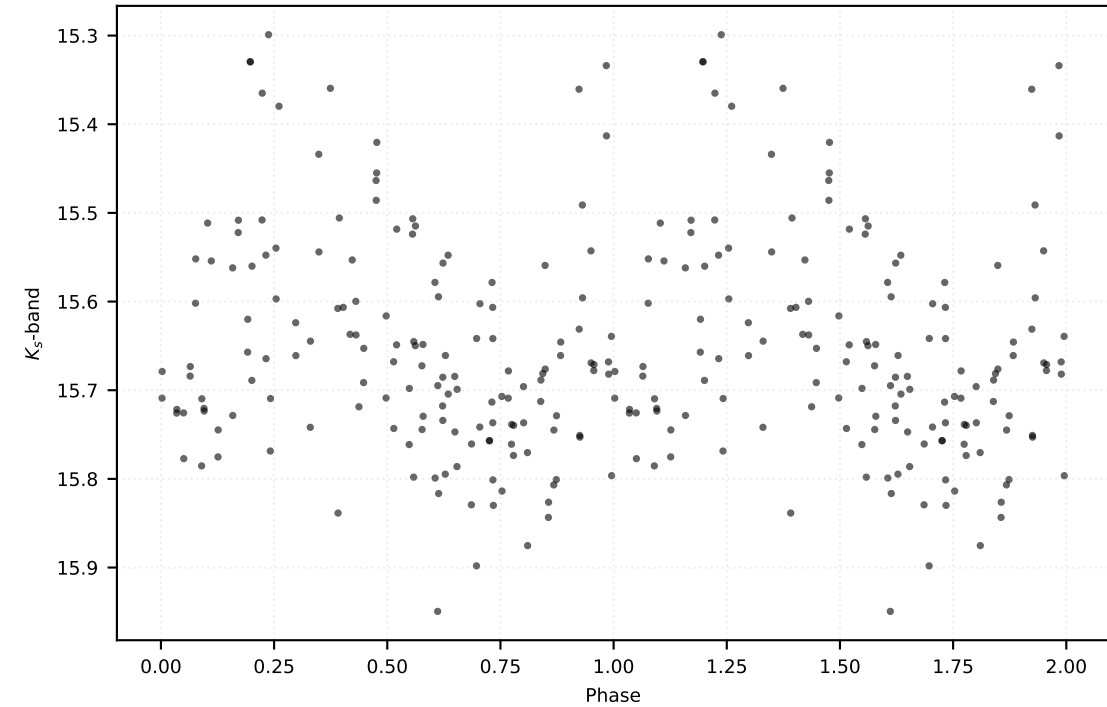
P: 51.16042 d | Class: RP | Subclass: CEP-F | Field b279
