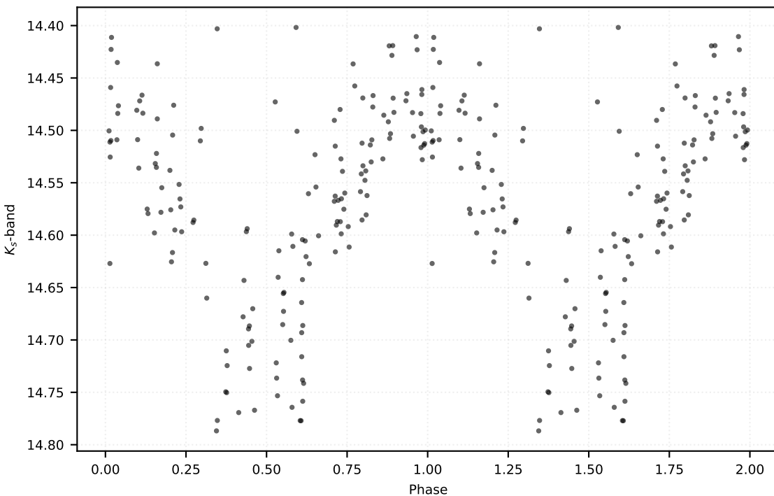
P: 1.37368 d | Class: RP | Subclass: CEP-10T | Field b279
