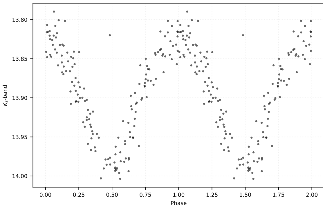
P: 0.20579 d | Class: RP | Subclass: UVAR | Field b278
