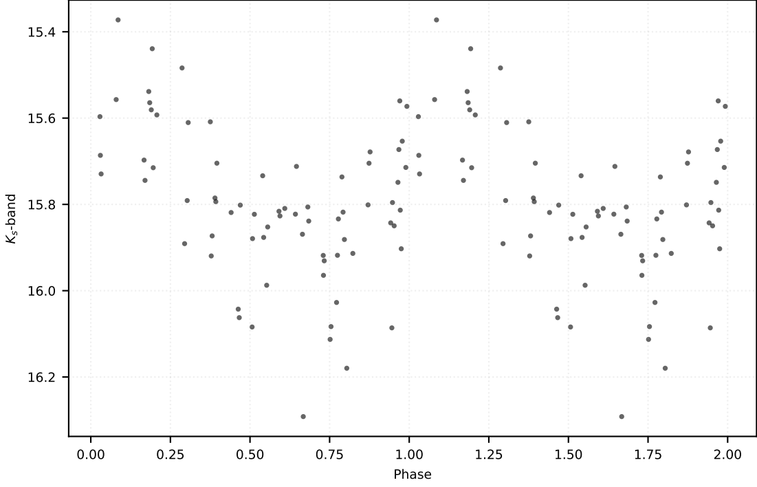
P: 0.13110 d | Class: RP | Subclass: UVAR | Field b278
