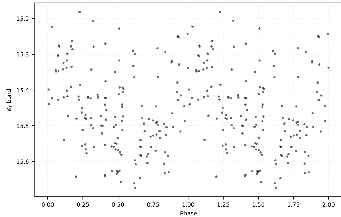
P: 0.10039 d | Class: RP | Subclass: UVAR | Field b279
