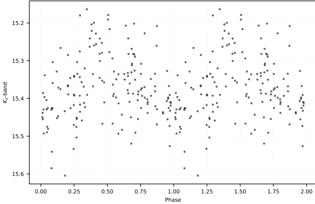
P: 0.24012 d | Class: RP | Subclass: UVAR | Field b278
