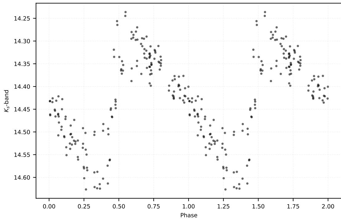
P: 0.80291 d | Class: RP | Subclass: RRab | Field b278
