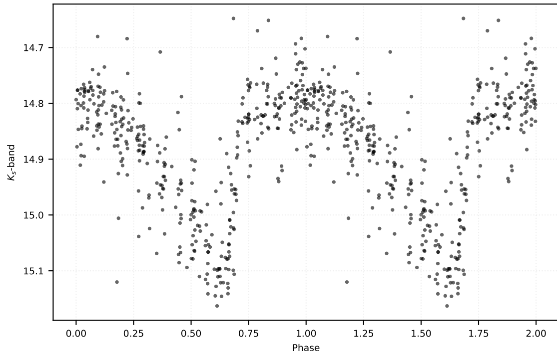
P: 3.77088 d | Class: RP | Subclass: CEP-10T | Field b278
