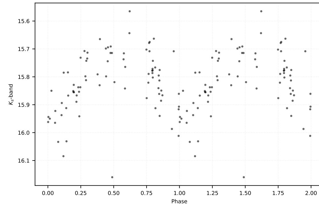
P: 3.45287 d | Class: RP | Subclass: CEP-10T | Field b279
