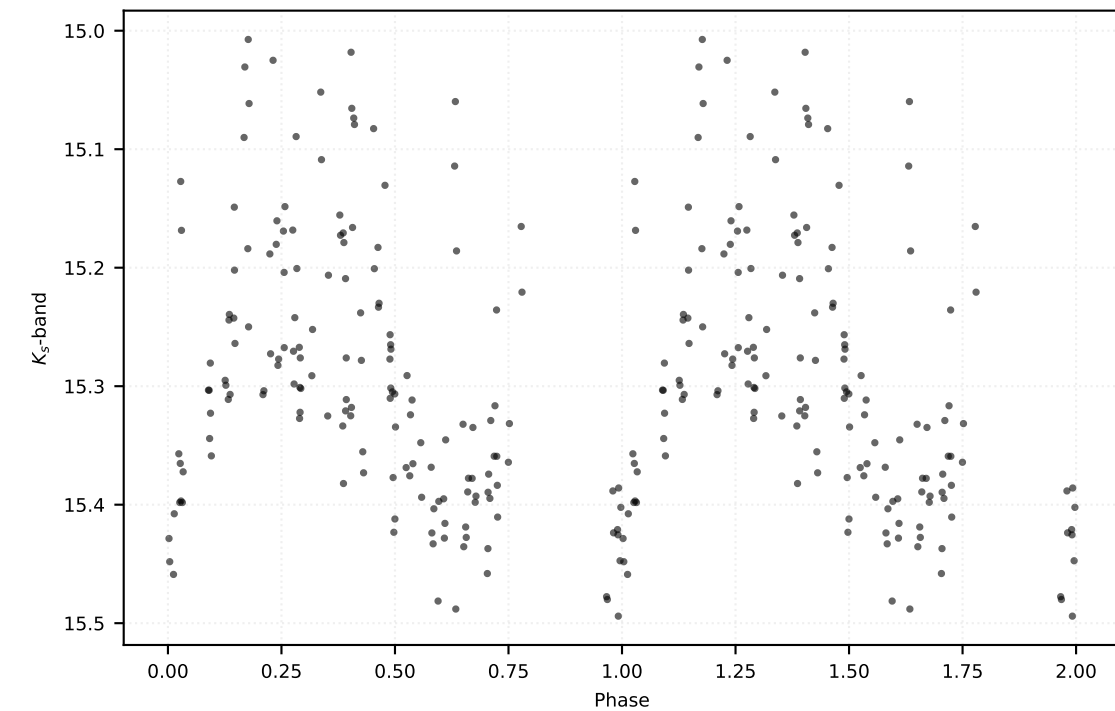
P: 0.16071 d | Class: RP | Subclass: UVAR | Field b279
