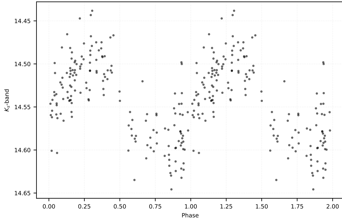
P: 0.50435 d | Class: RP | Subclass: RRab | Field b278
