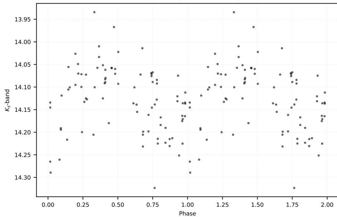
P: 1.18358 d | Class: RP | Subclass: CEP-F | Field b279
