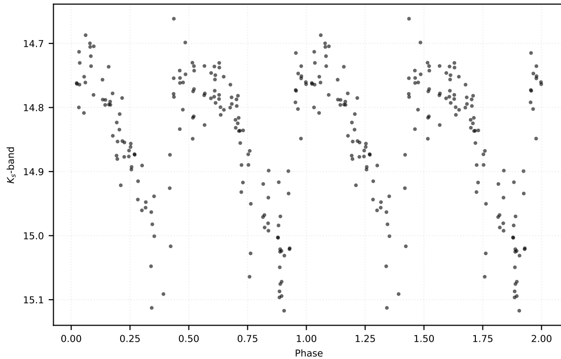
P: 0.25732 d | Class: RP | Subclass: UVAR | Field b278
