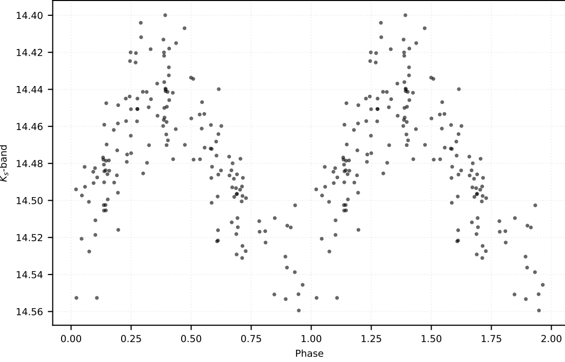
P: 0.16349 d | Class: RP | Subclass: UVAR | Field b278
