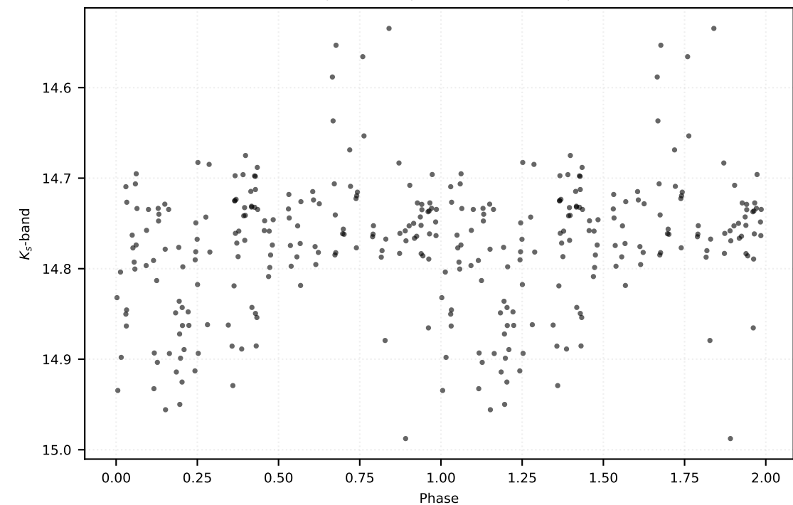
P: 0.36104 d | Class: RP | Subclass: CEP-1OT | Field b278
