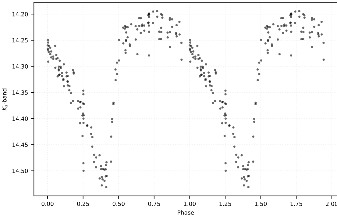
P: 0.55276 d | Class: RP | Subclass: RRab | Field b278
