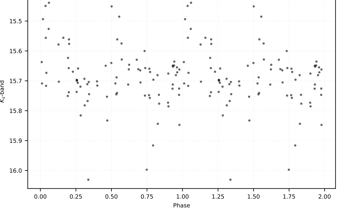
P: 0.20548 d | Class: EB | Subclass: EA | Field b278
