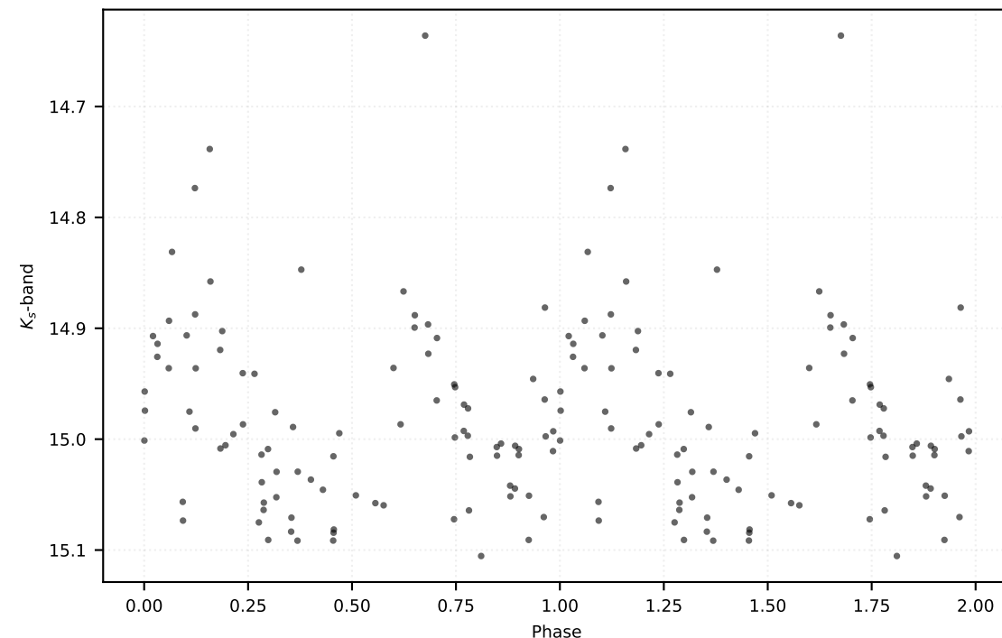
P: 0.65221 d | Class: EB | Subclass: EA | Field b279
