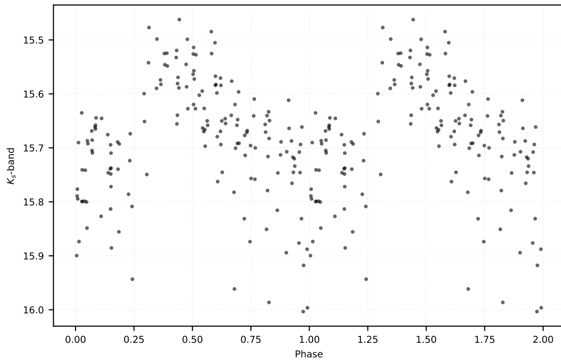
P: 0.24194 d | Class: RP | Subclass: UVAR | Field b279
