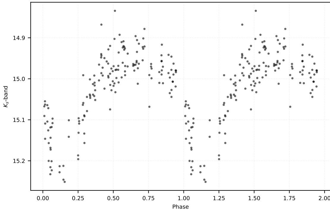
P: 0.38579 d | Class: RP | Subclass: RRab | Field b279
