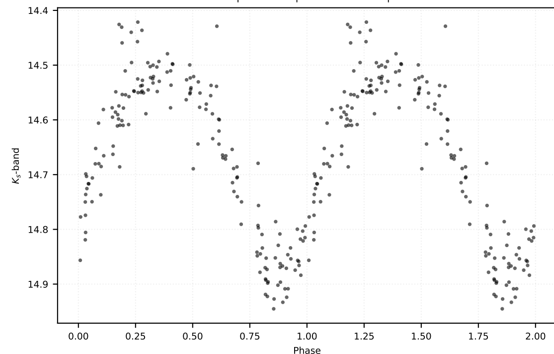
P: 0.50632 d | Class: RP | Subclass: RRab | Field b278
