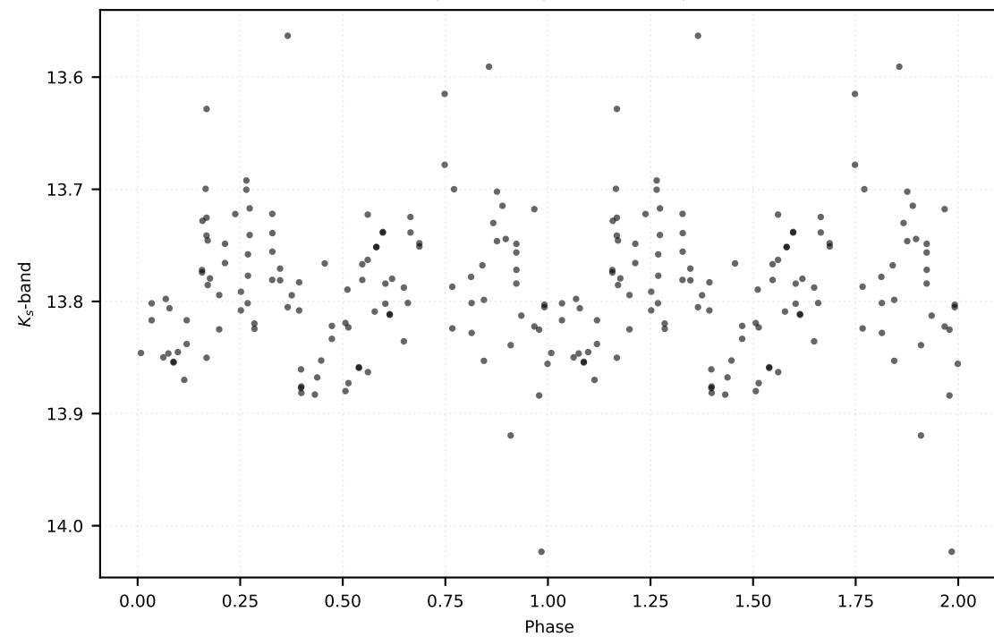
P: 0.23022 d | Class: EB | Subclass: EA | Field b279
