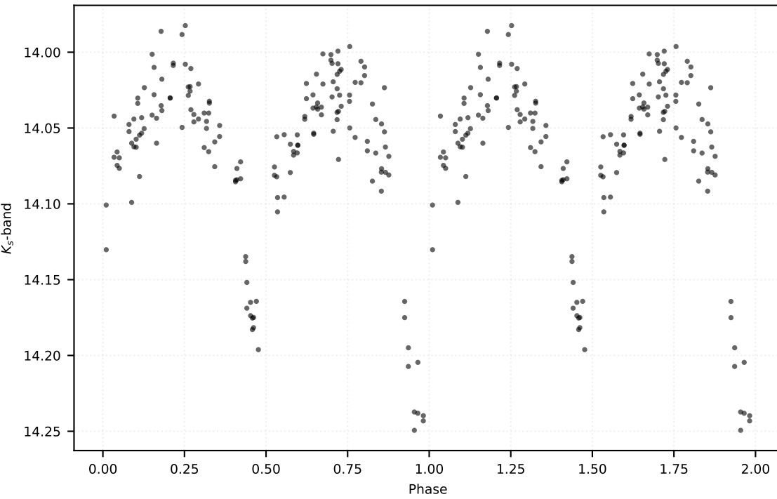
P: 3.63718 d | Class: EB | Subclass: EA | Field b278
