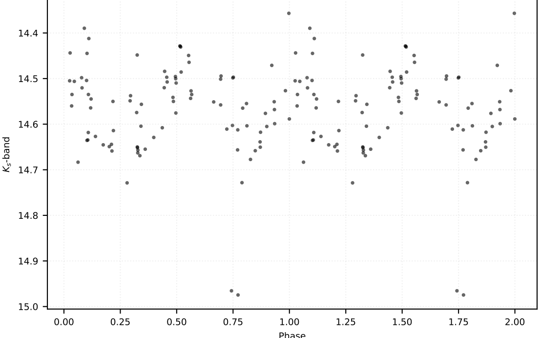
P: 0.20063 d | Class: EB | Subclass: EA | Field b278
