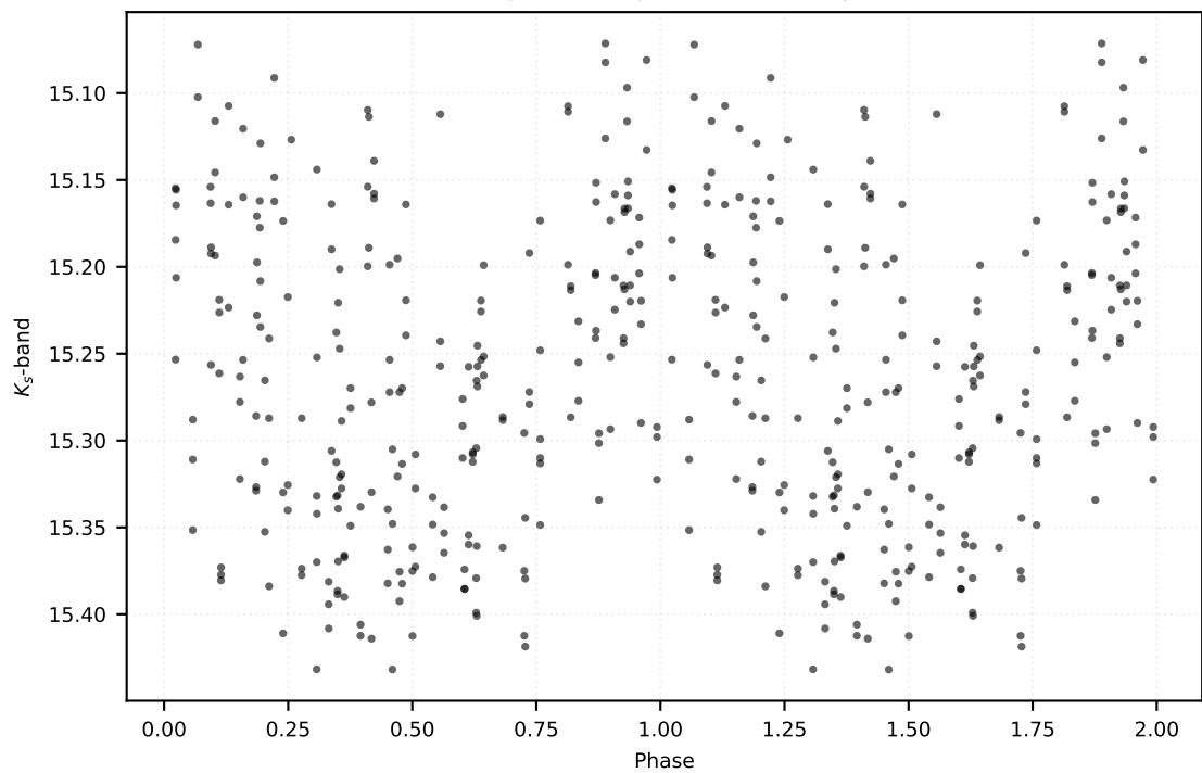
P: 71.99808 d | Class: RP | Subclass: CEP-F | Field b279
