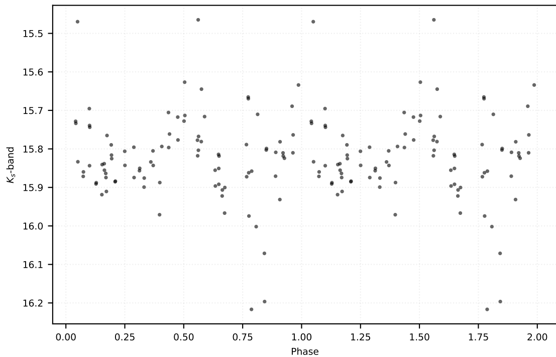
P: 0.35955 d | Class: EB | Subclass: EA | Field b279
