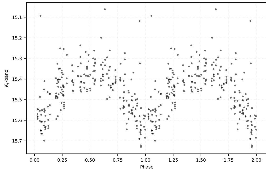
P: 0.96470 d | Class: RP | Subclass: RRab | Field b279
