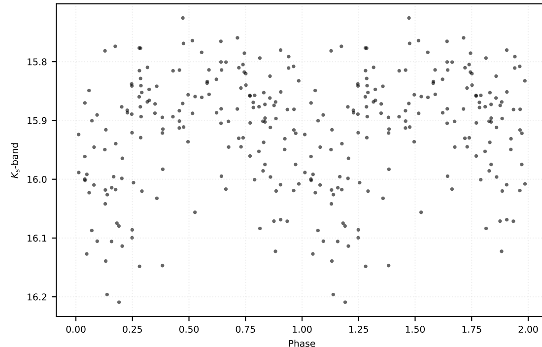
P: 0.46602 d | Class: RP | Subclass: RRab | Field b278
