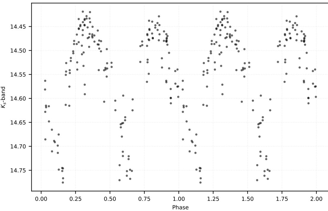
P: 0.13681 d | Class: RP | Subclass: UVAR | Field b278
