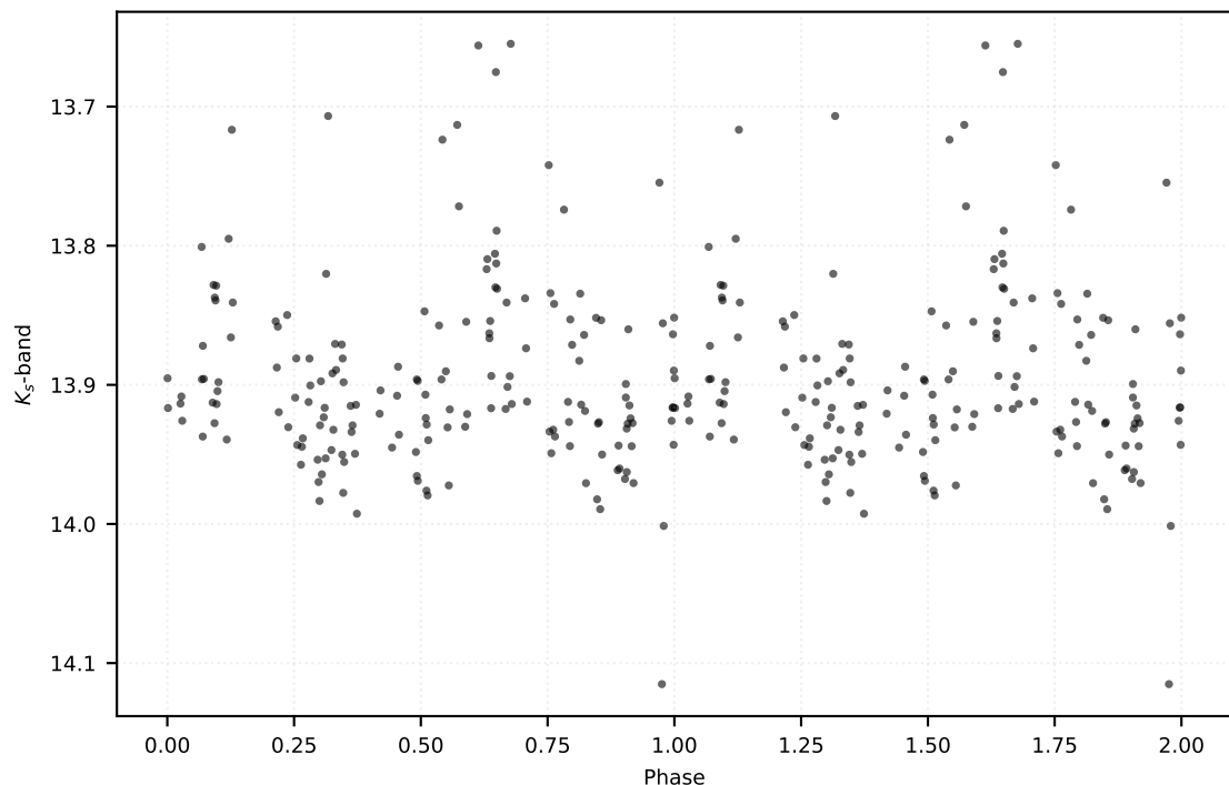
P: 11.83435 d | Class: EB | Subclass: EA | Field b278
