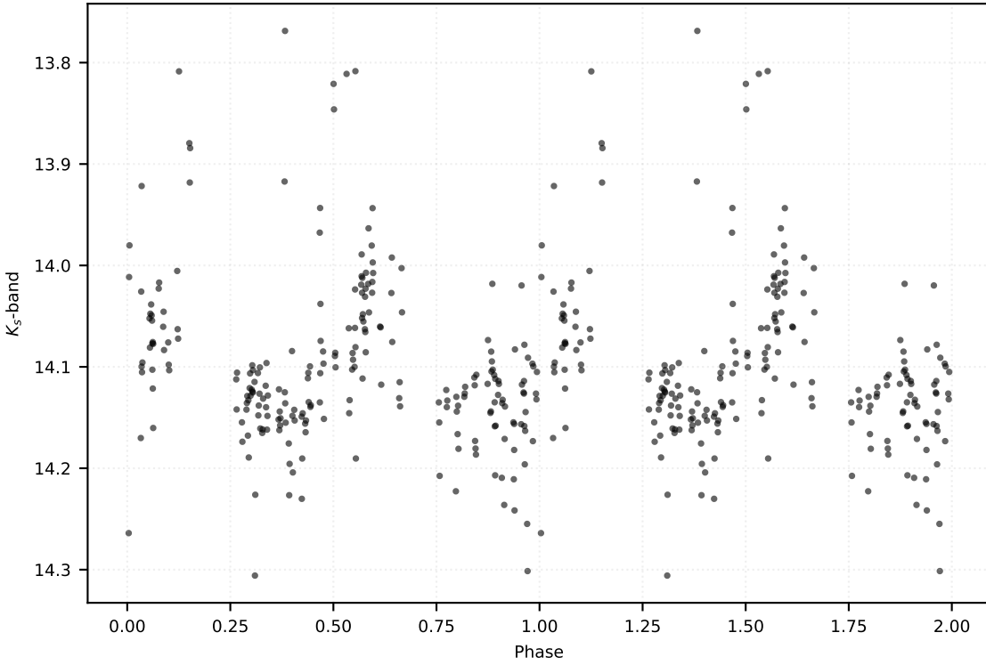
P: 0.39890 d | Class: EB | Subclass: EA | Field b279
