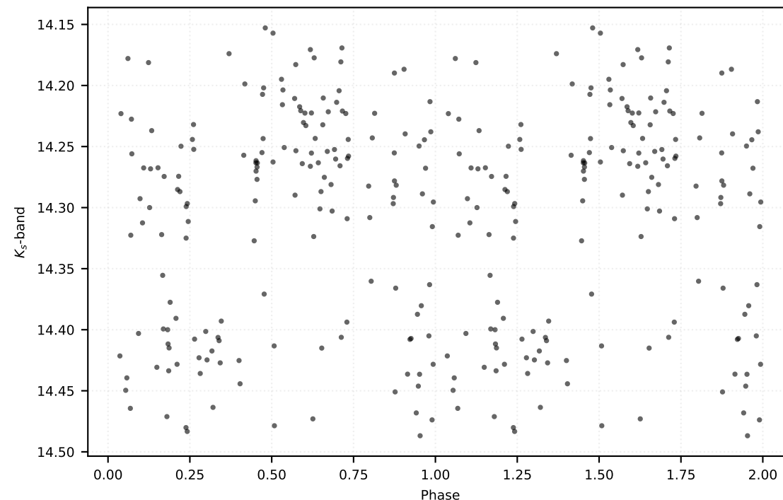
P: 48.38867 d | Class: RP | Subclass: UVAR | Field b279
