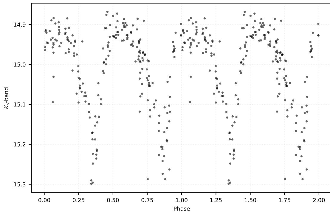
P: 1.07406 d | Class: EB | Subclass: UVAR | Field b278
