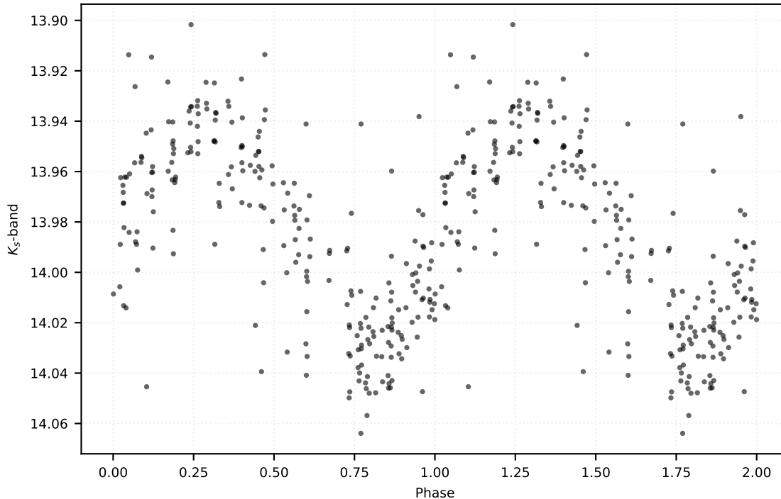
P: 0.44661 d | Class: RP | Subclass: RRab | Field b279
