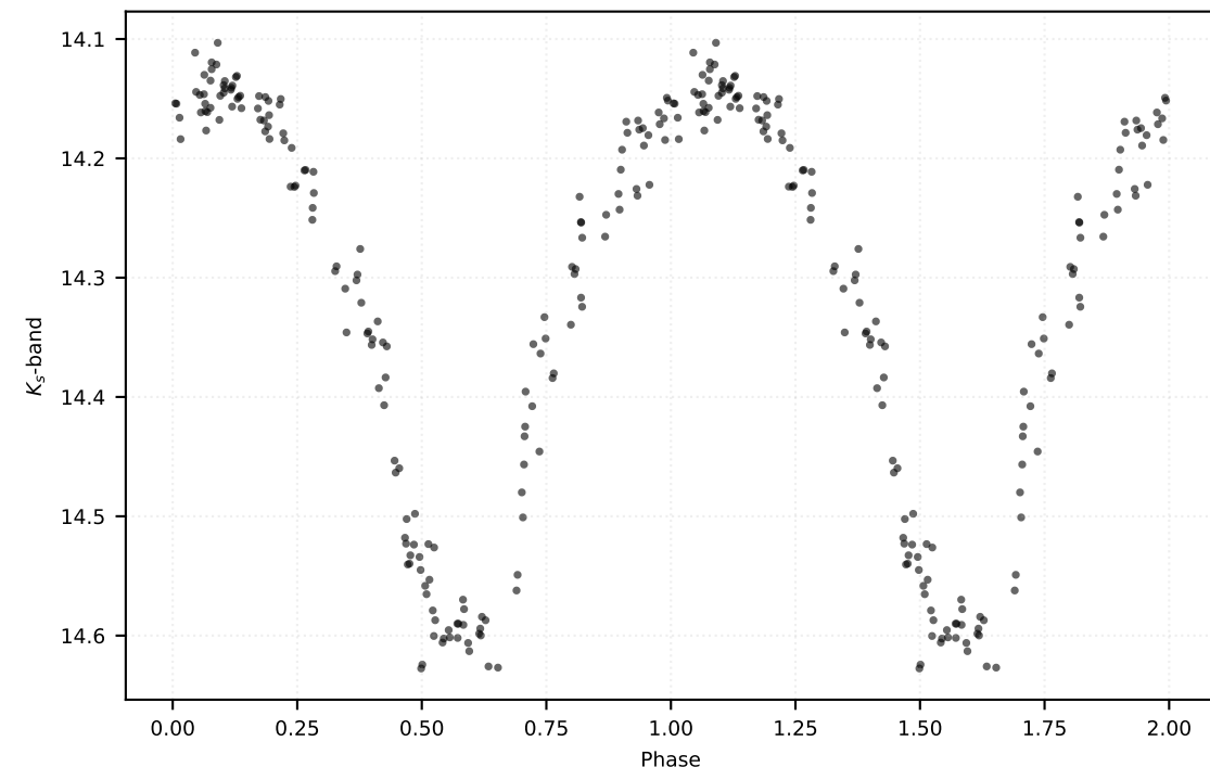
P: 0.17246 d | Class: RP | Subclass: UVAR | Field b278
