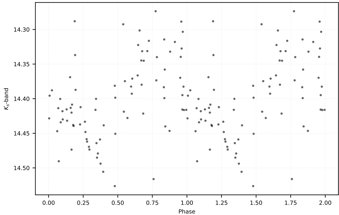
P: 0.13360 d | Class: RP | Subclass: UVAR | Field b278
