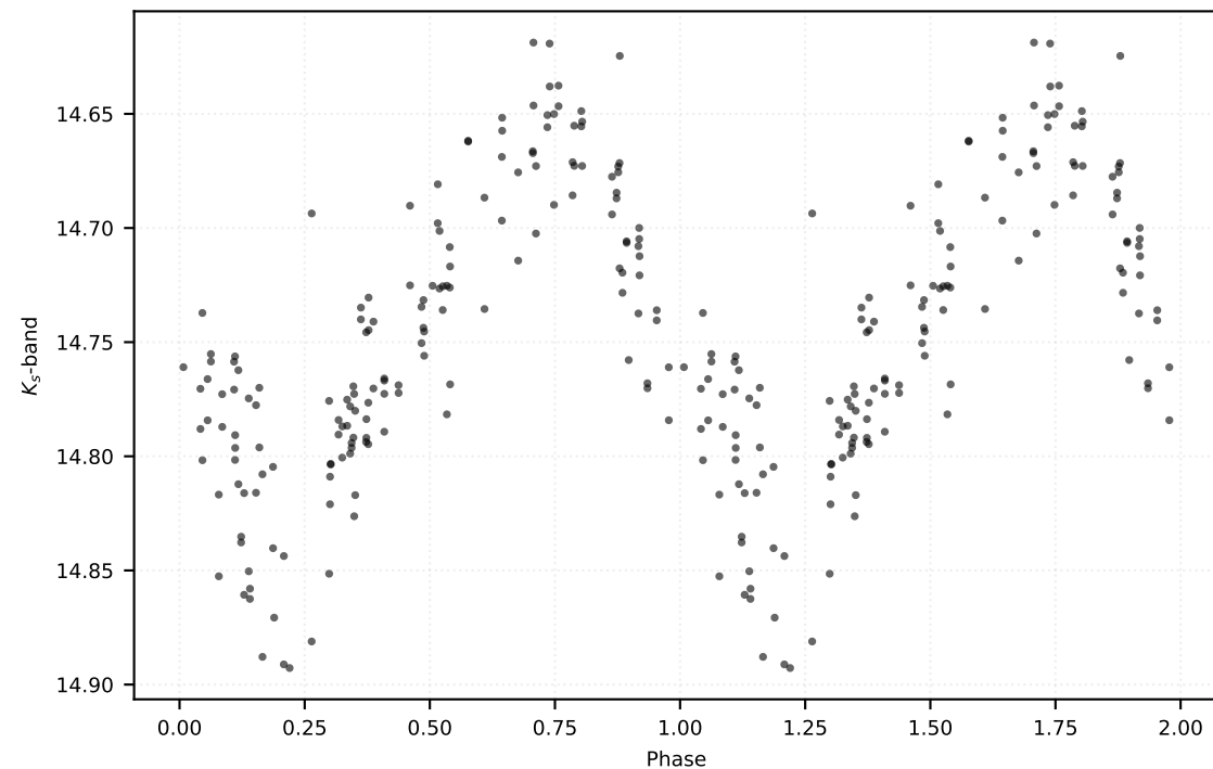
P: 1.07141 d | Class: RP | Subclass: CEP-10T | Field b279
