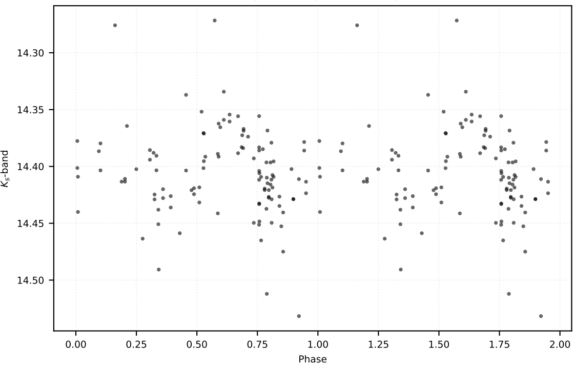
P: 0.38507 d | Class: EB | Subclass: EA | Field b278
