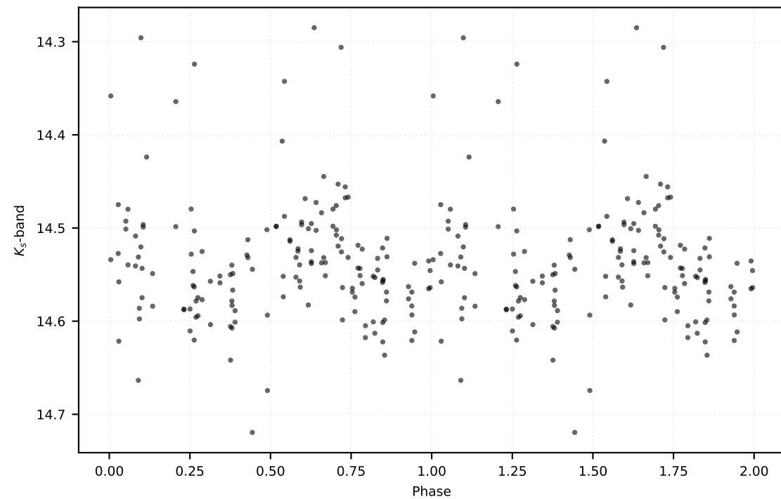
P: 0.21082 d | Class: EB | Subclass: EA | Field b279
