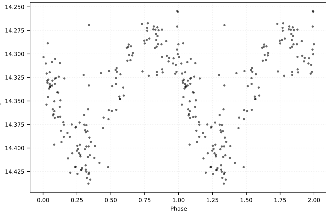
P: 0.27568 d | Class: RP | Subclass: UVAR | Field b278
