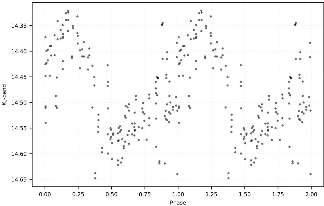
P: 0.72493 d | Class: RP | Subclass: CEP-1OT | Field b278
