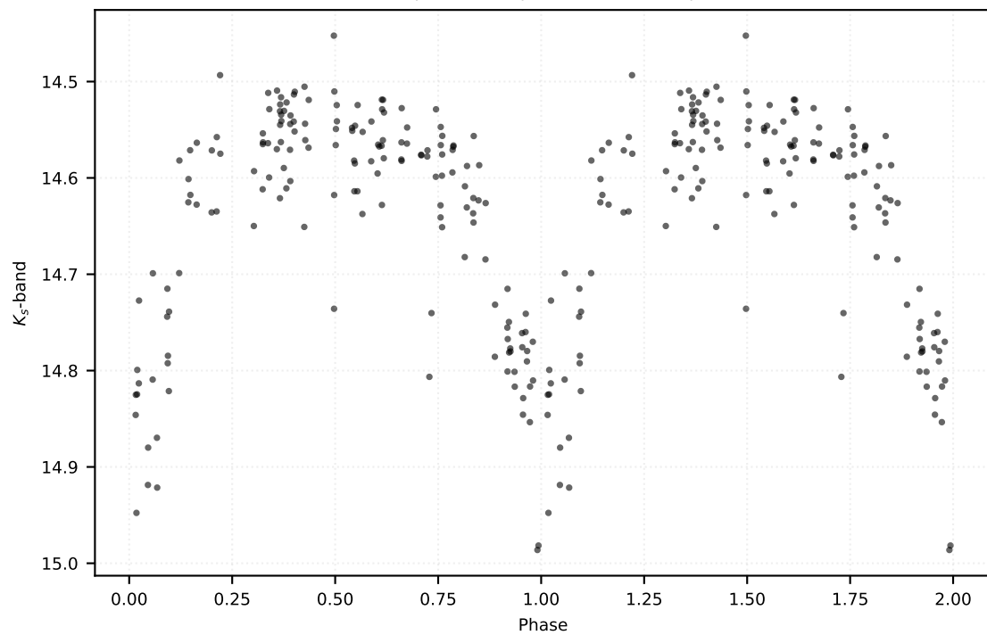
P: 3.45863 d | Class: RP | Subclass: CEP-F | Field b278
