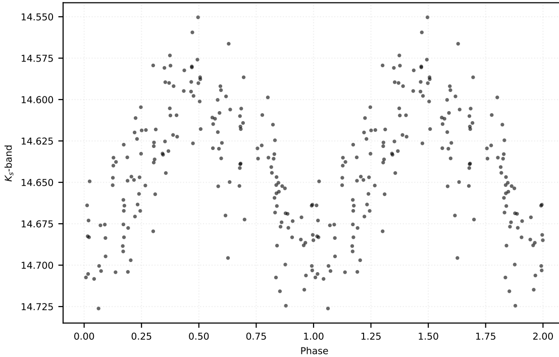
P: 0.32037 d | Class: RP | Subclass: RRab | Field b278
