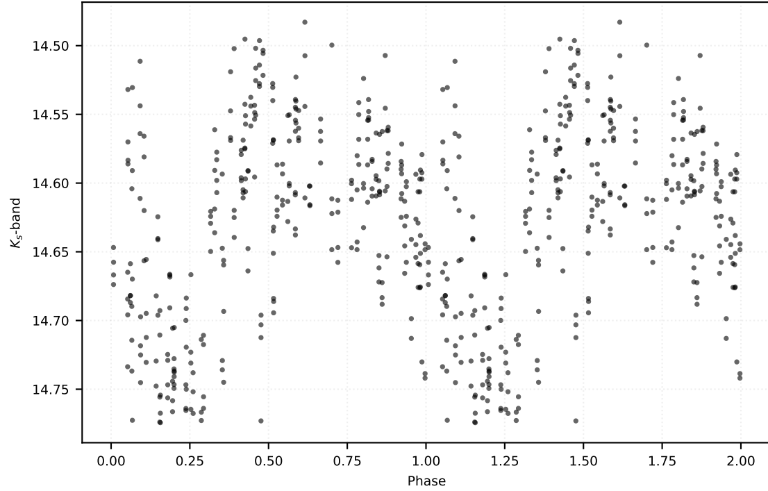
P: 4.40694 d | Class: RP | Subclass: CEP-F | Field b279
