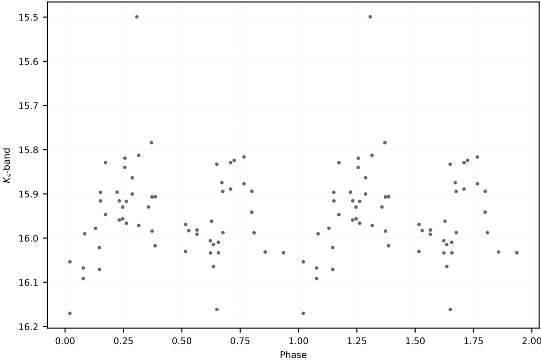
P: 1.08528 d | Class: EB | Subclass: EA | Field b279
