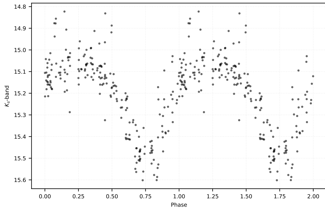
P: 0.21561 d | Class: RP | Subclass: UVAR | Field b279
