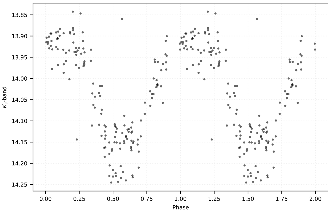
P: 0.24487 d | Class: RP | Subclass: CEP-1OT | Field b279
