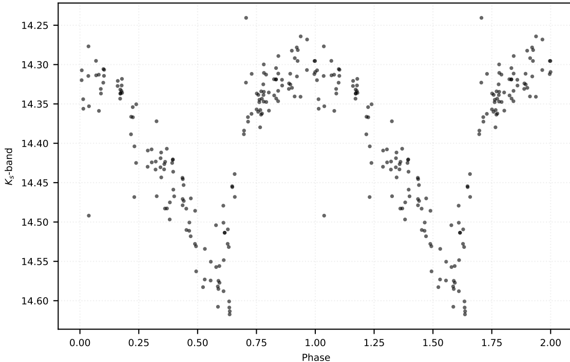
P: 0.63960 d | Class: RP | Subclass: RRab | Field b278
