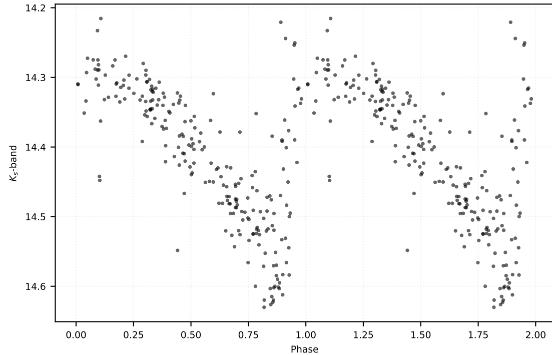
P: 0.44444 d | Class: RP | Subclass: RRab | Field b278
