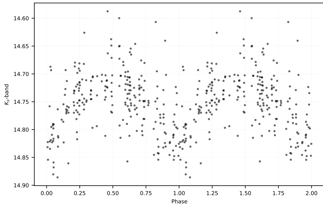
P: 0.24573 d | Class: RP | Subclass: UVAR | Field b279
