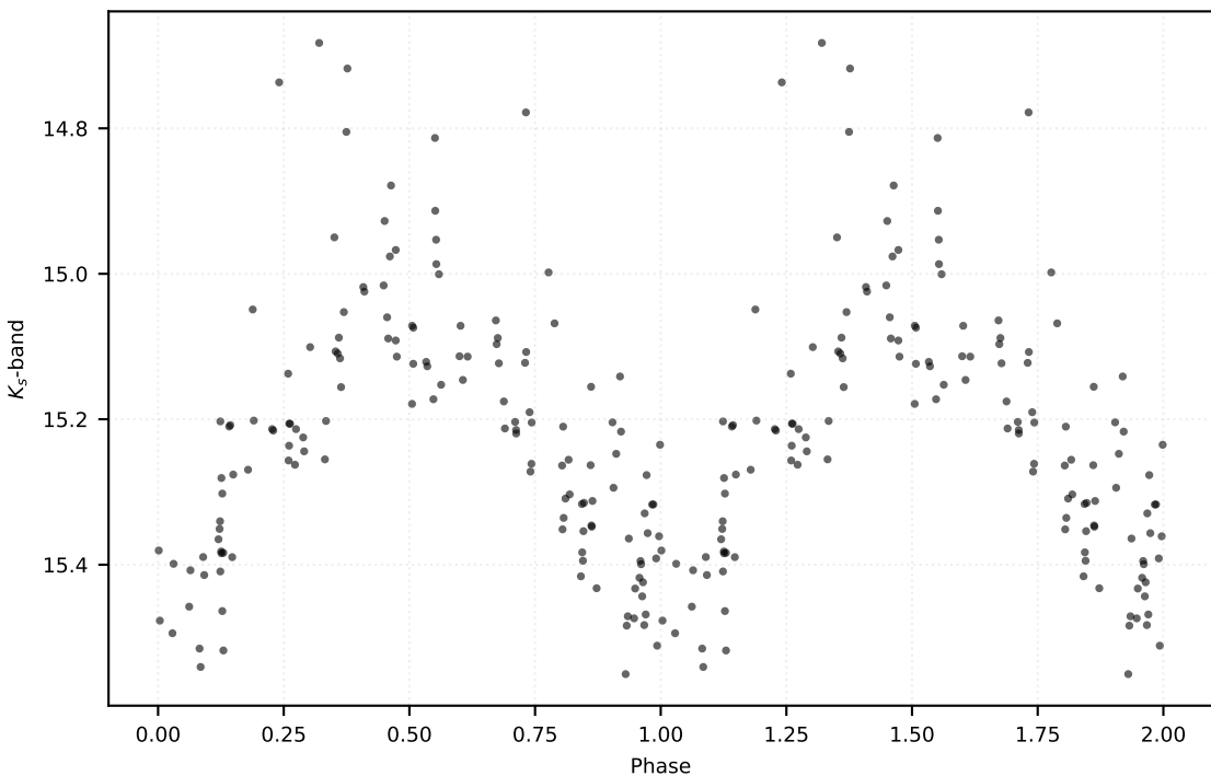
P: 2.03428 d | Class: EB | Subclass: UVAR | Field b278
