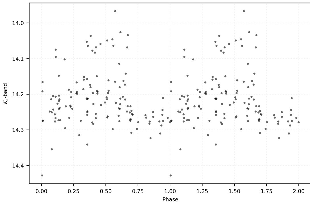
P: 0.36197 d | Class: RP | Subclass: CEP-10T | Field b278
