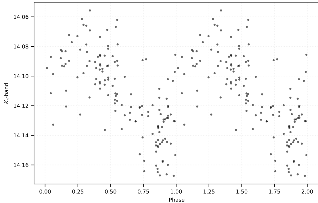
P: 4.23748 d | Class: RP | Subclass: CEP-F | Field b279
