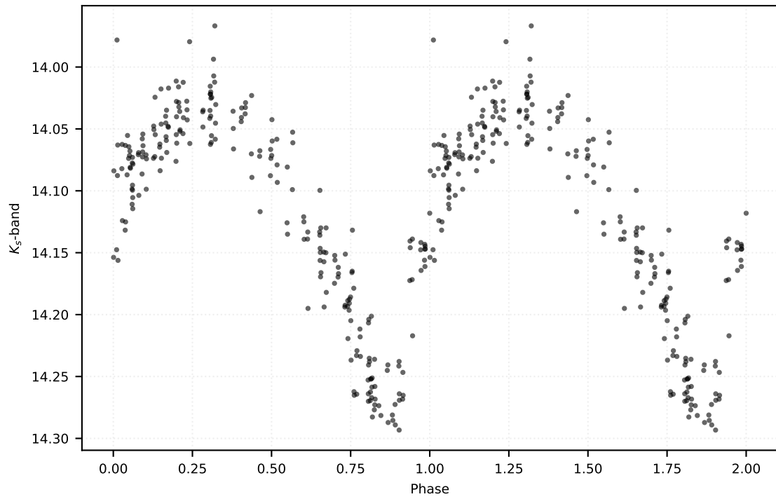
P: 0.57762 d | Class: RP | Subclass: RRab | Field b279
