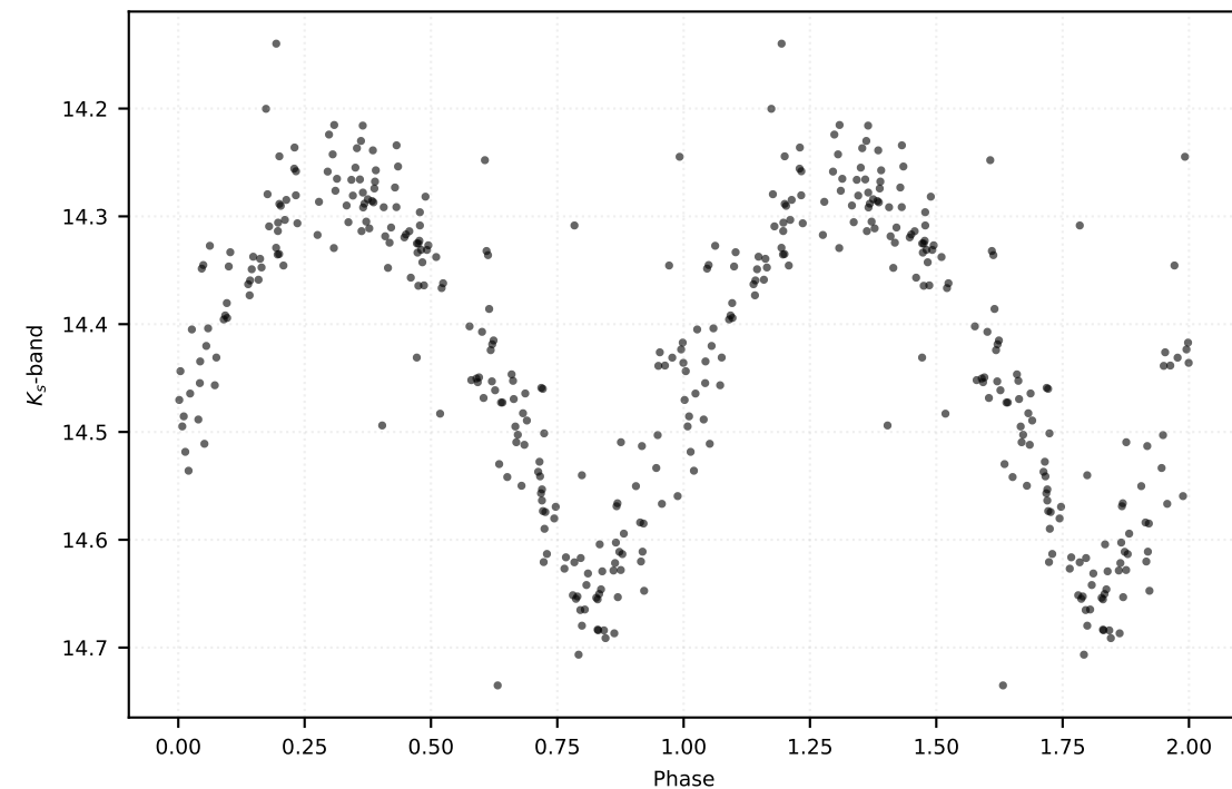
P: 0.18907 d | Class: RP | Subclass: UVAR | Field b278
