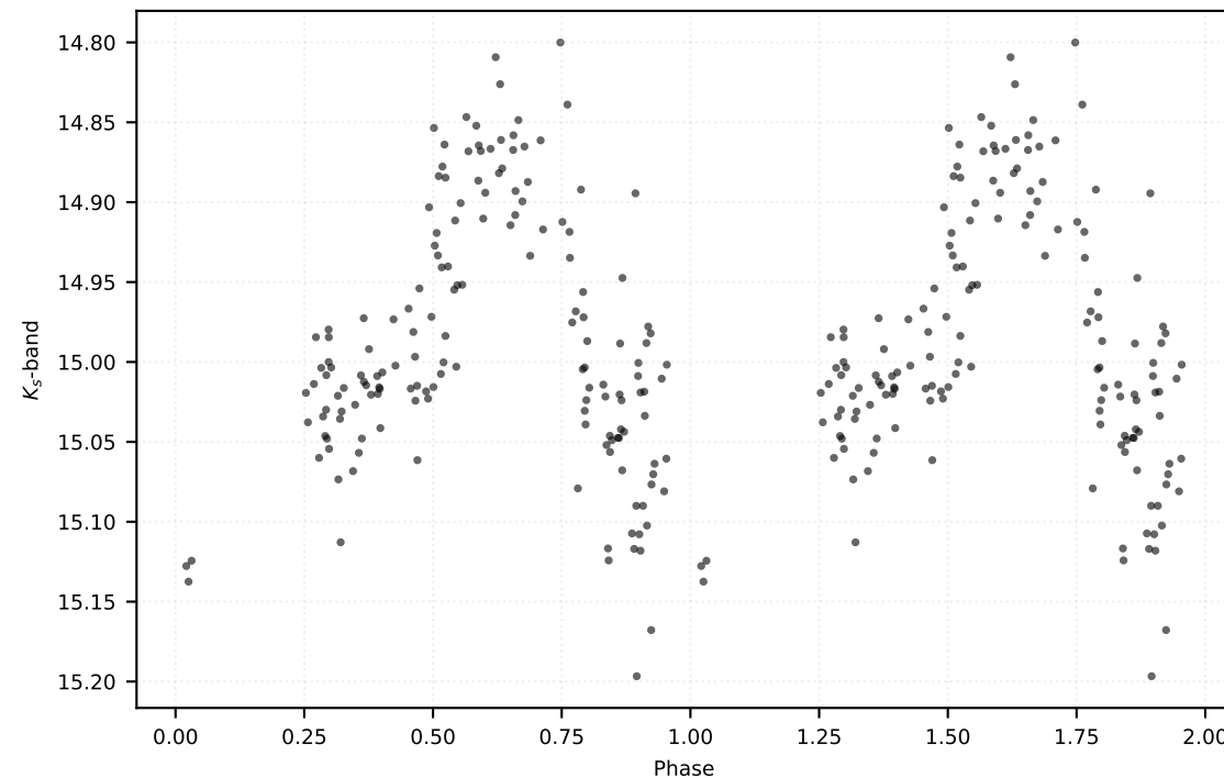
P: 0.10556 d | Class: RP | Subclass: UVAR | Field b279
