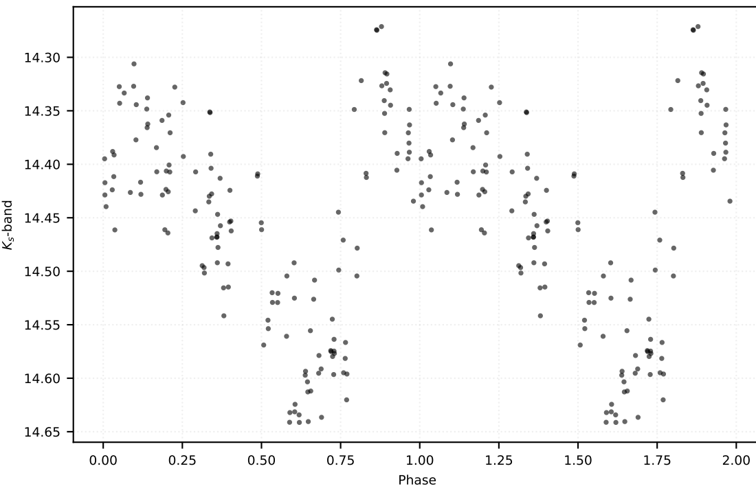
P: 0.44987 d | Class: RP | Subclass: RRab | Field b279
