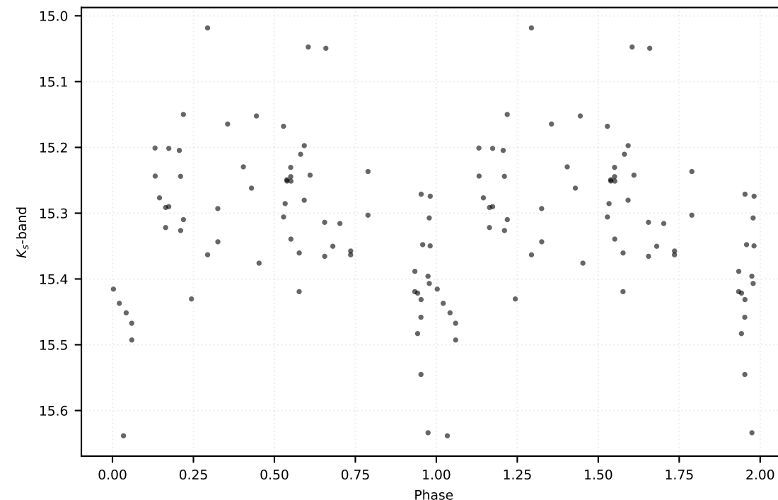
P: 0.49868 d | Class: RP | Subclass: CEP-1OT | Field b278
