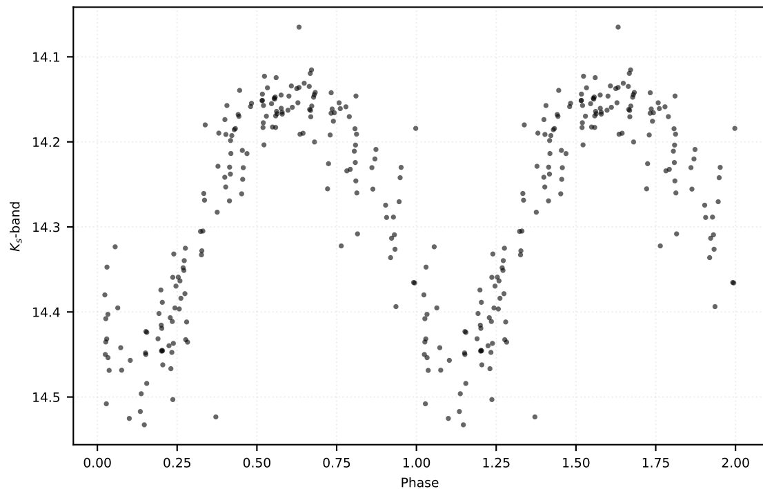
P: 0.12745 d | Class: RP | Subclass: UVAR | Field b279
