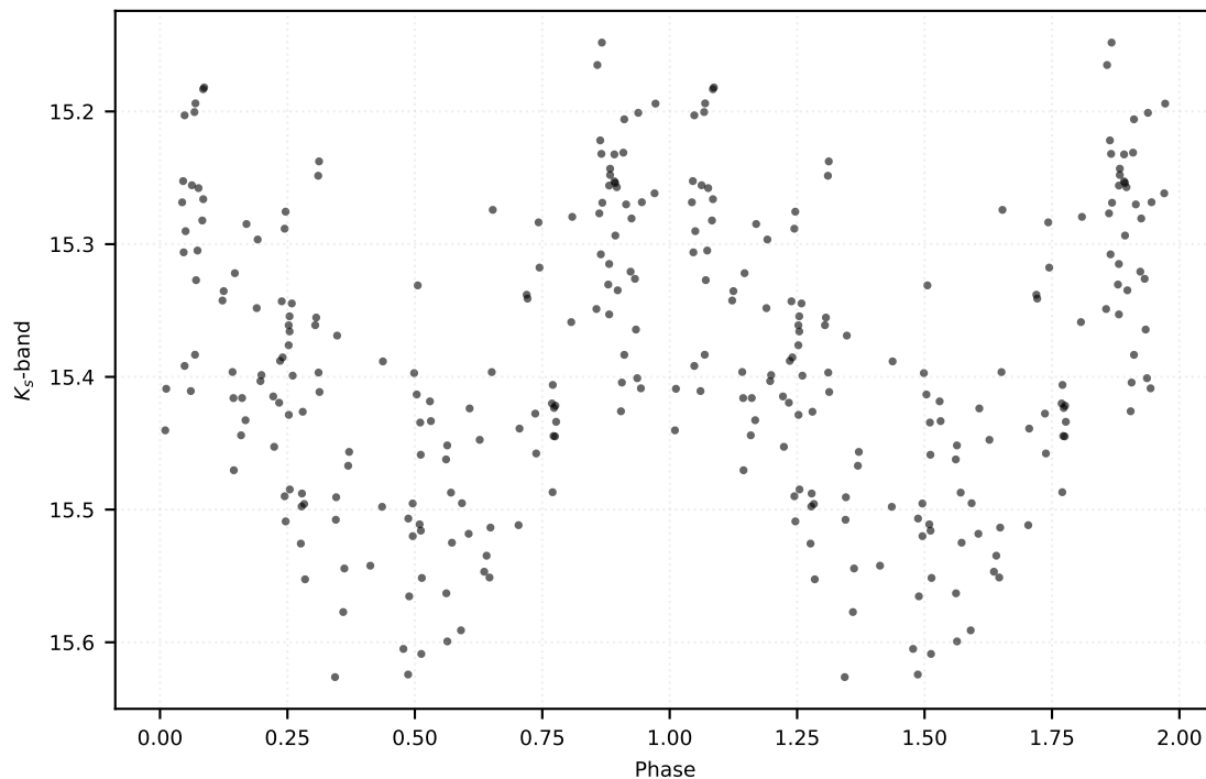
P: 1.83048 d | Class: RP | Subclass: CEP-10T | Field b279
