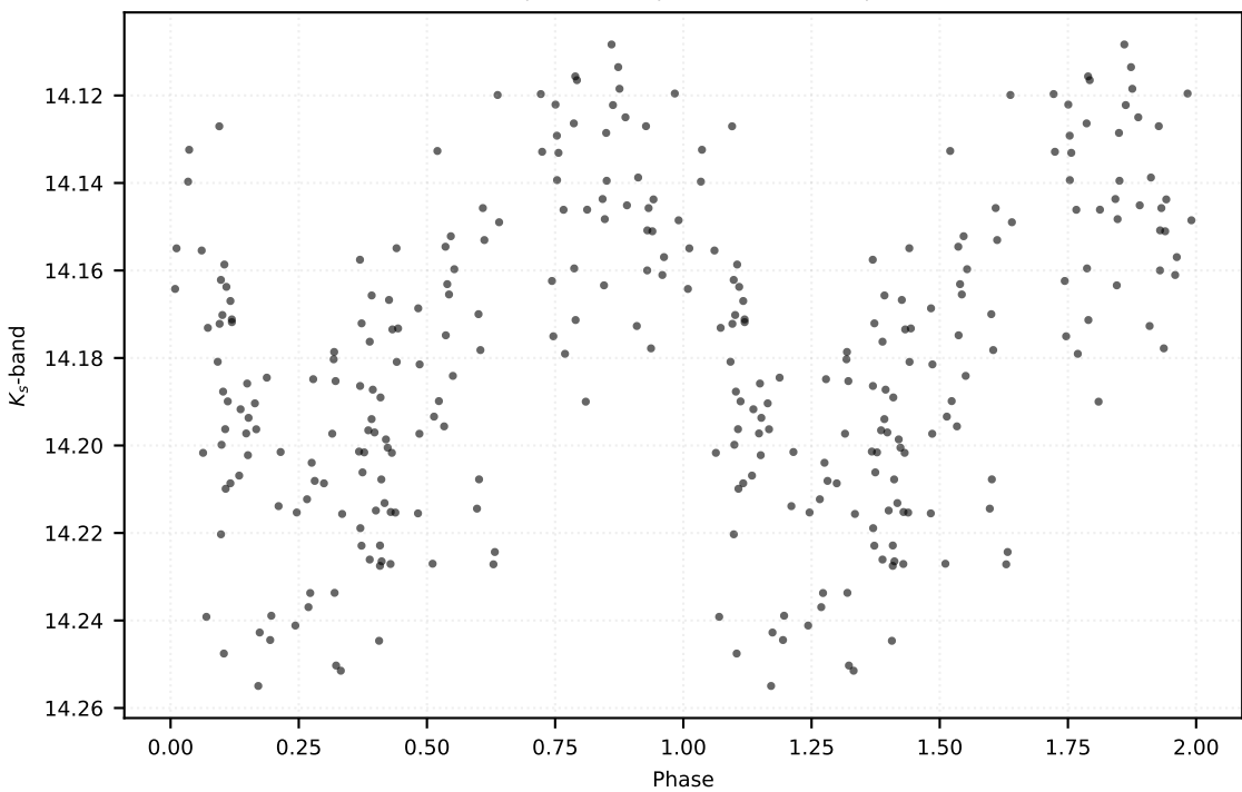
P: 0.27519 d | Class: RP | Subclass: UVAR | Field b279
