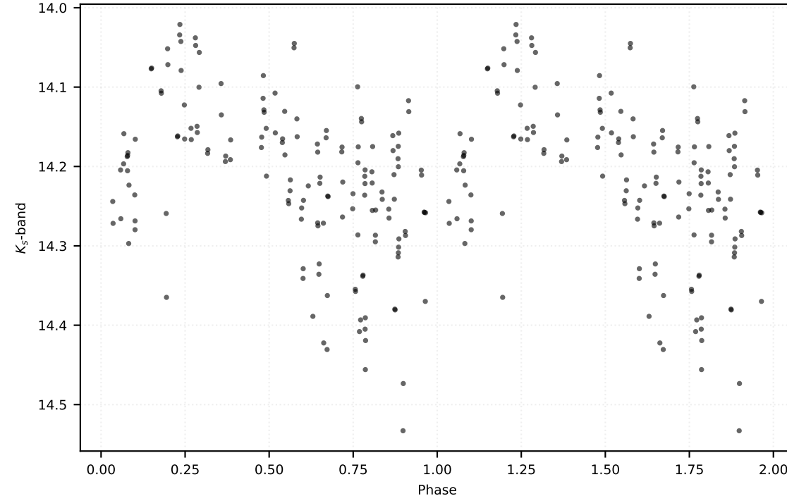
P: 0.78936 d | Class: RP | Subclass: CEP-10T | Field b278
