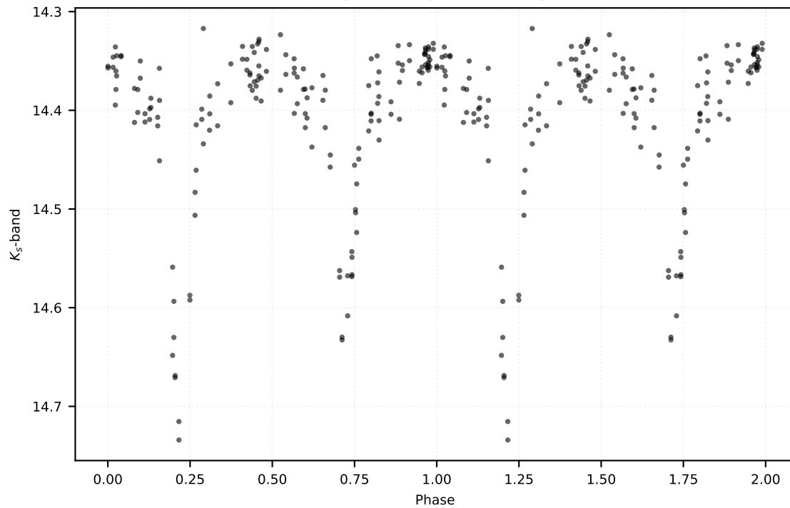
P: 2.34186 d | Class: EB | Subclass: EA | Field b278
