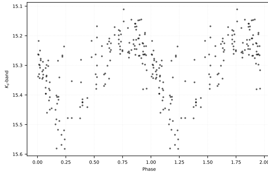
P: 0.21610 d | Class: RP | Subclass: UVAR | Field b279
