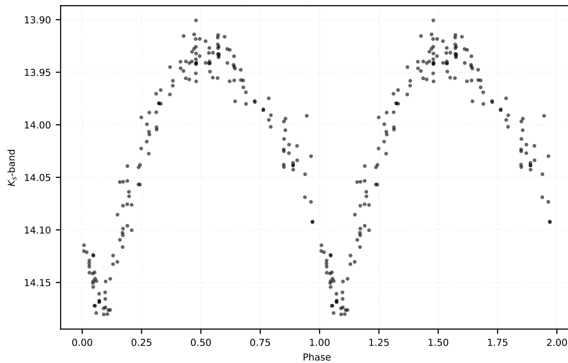
P: 0.39403 d | Class: RP | Subclass: RRab | Field b278
