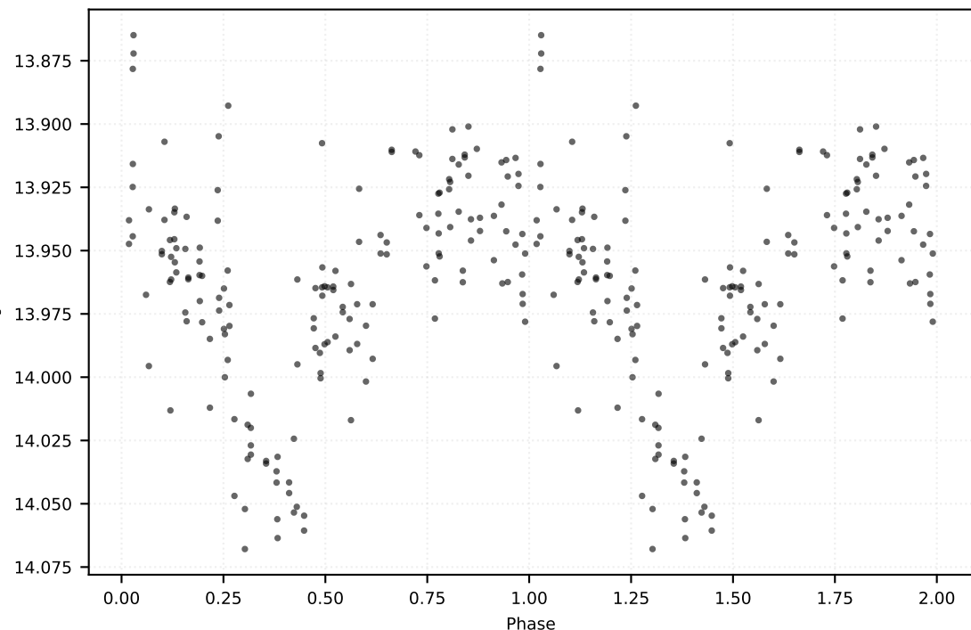
P: 0.40922 d | Class: RP | Subclass: CEP-10T | Field b278
