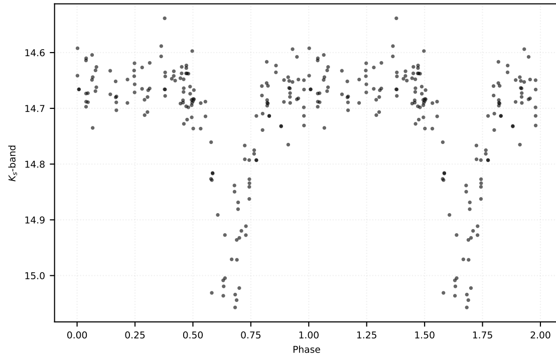
P: 5.09191 d | Class: RP | Subclass: CEP-F | Field b279
