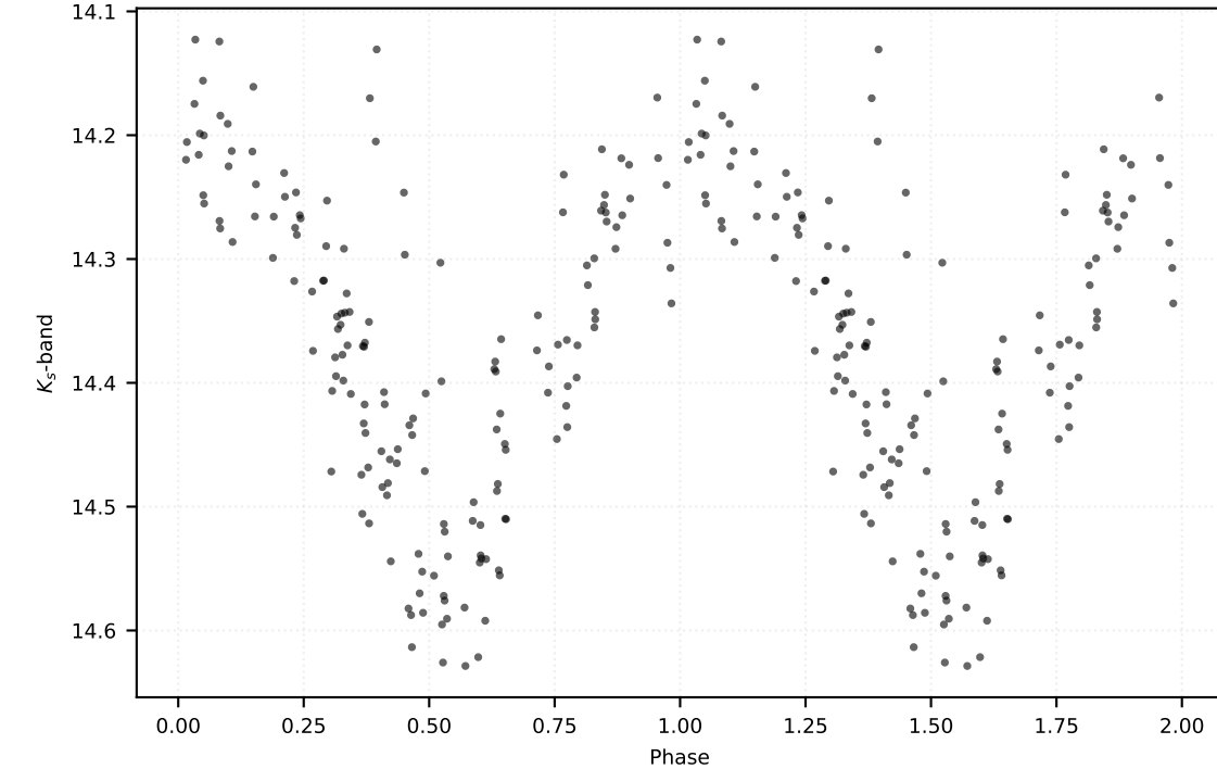
P: 0.24923 d | Class: RP | Subclass: UVAR | Field b279
