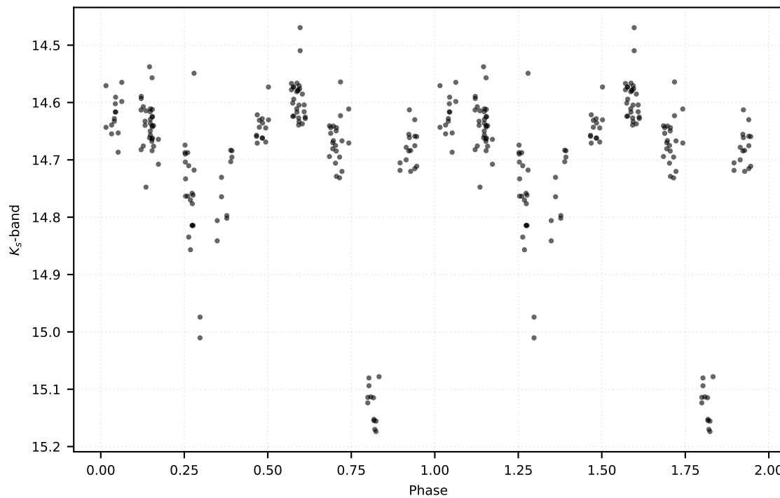
P: 2.08091 d | Class: EB | Subclass: EA | Field b278
