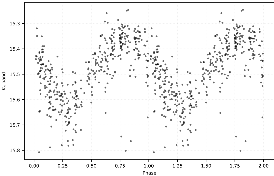
P: 0.26190 d | Class: RP | Subclass: UVAR | Field b279
