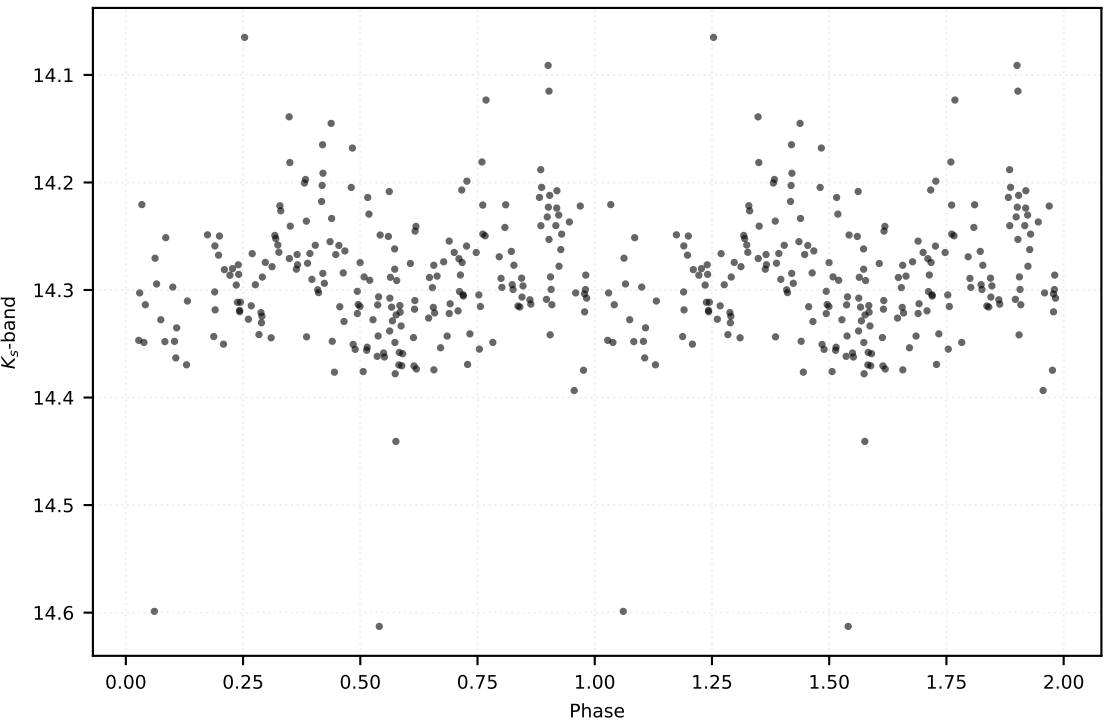
P: 0.21516 d | Class: EB | Subclass: EA | Field b278
