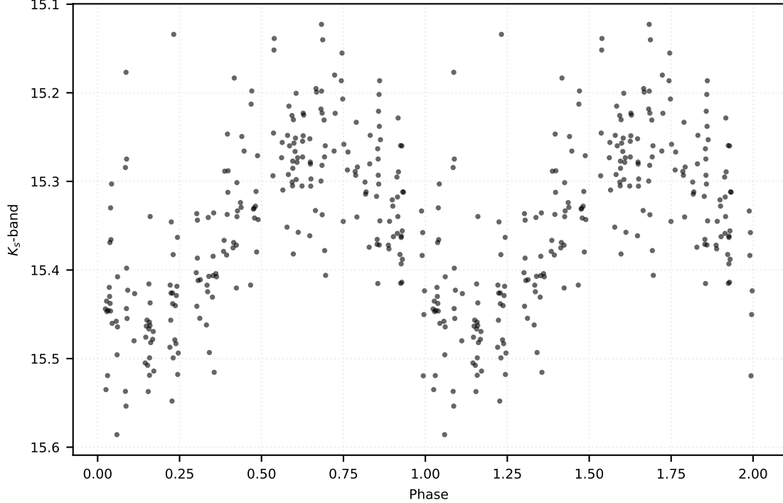
P: 0.19945 d | Class: RP | Subclass: UVAR | Field b278
