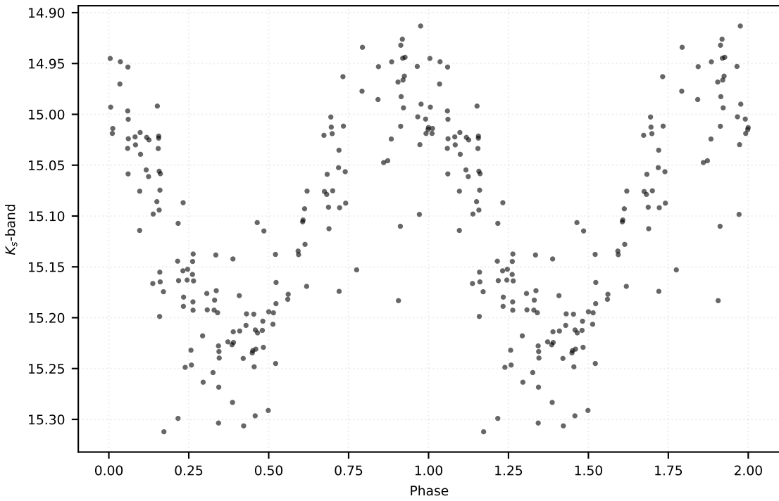
P: 0.56627 d | Class: RP | Subclass: CEP-1OT | Field b279
