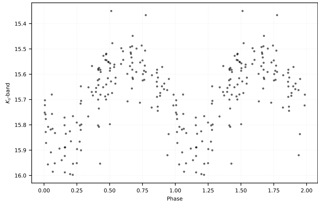
P: 0.45389 d | Class: RP | Subclass: RRc | Field b278
