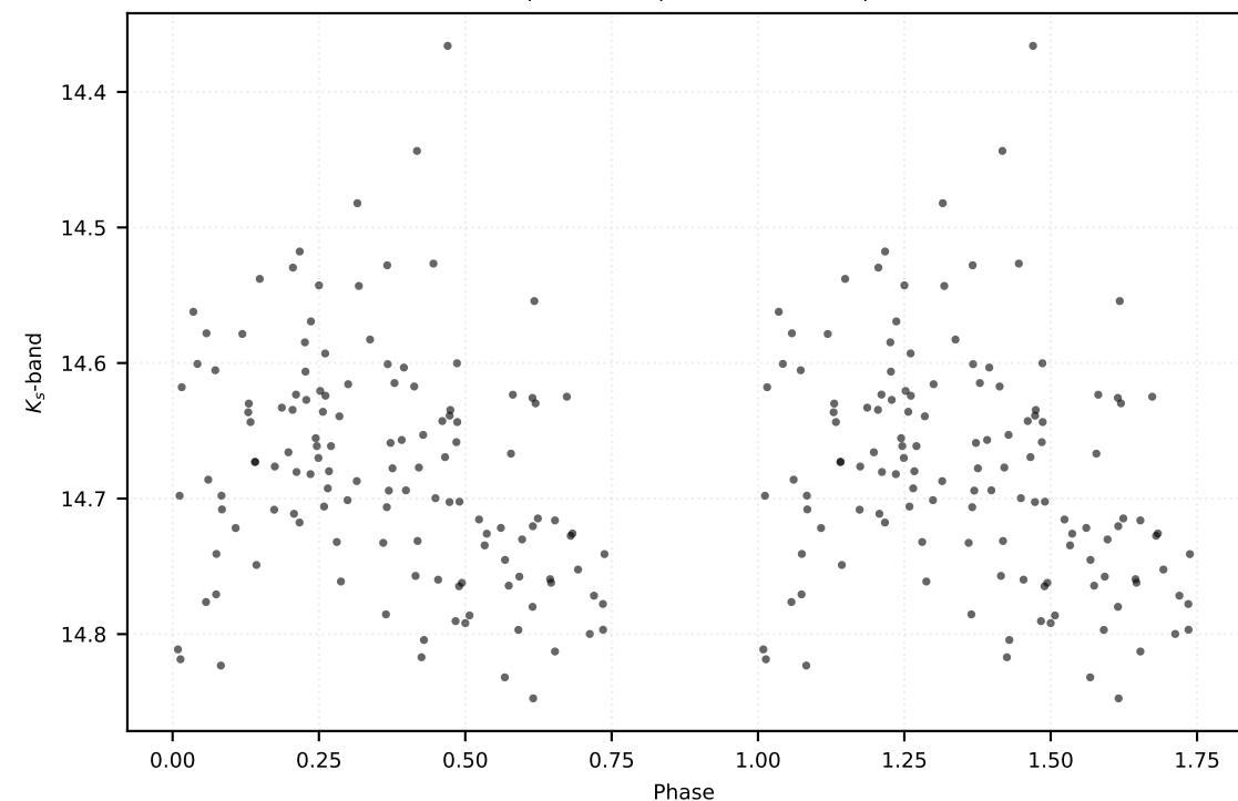
P: 0.44955 d | Class: RP | Subclass: RRab | Field b278
