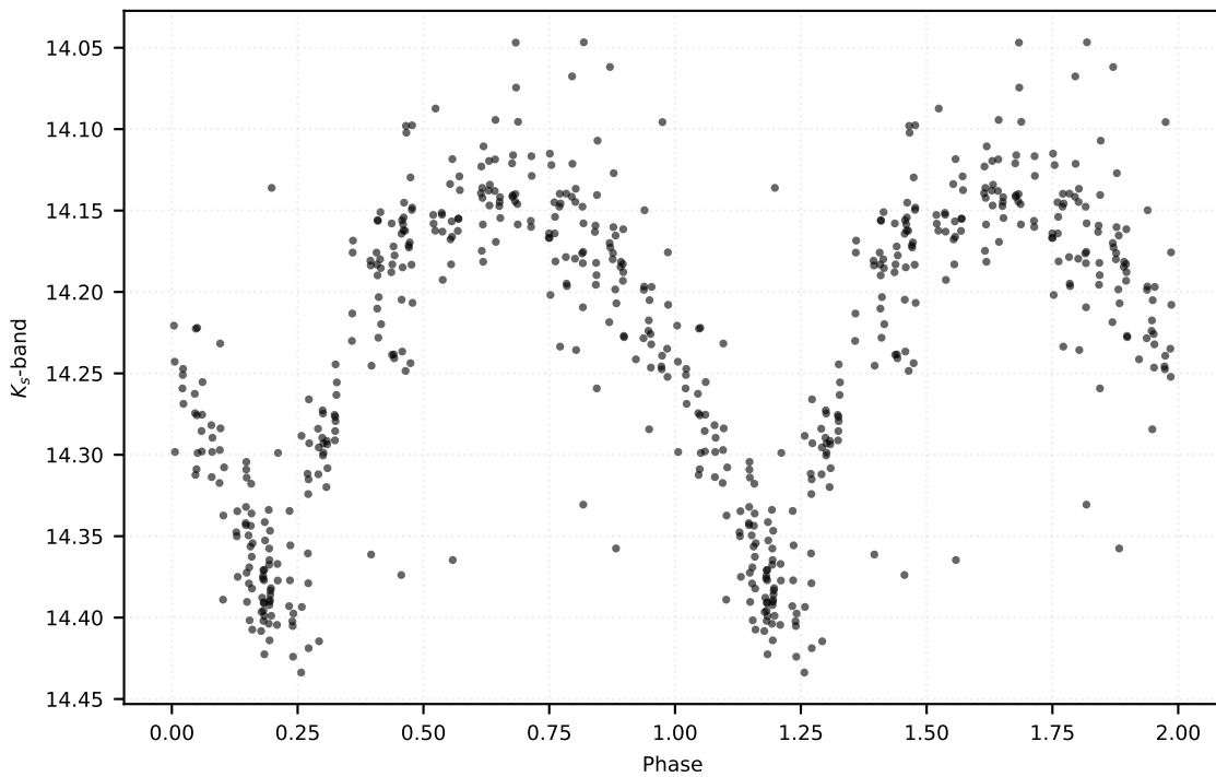
P: 0.26189 d | Class: RP | Subclass: RRc | Field b279
