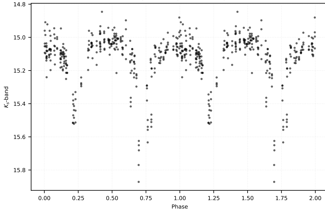
P: 4.39479 d | Class: EB | Subclass: EA | Field b279
