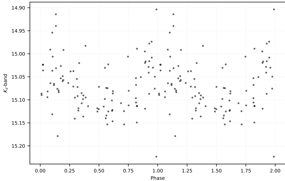
P: 0.66108 d | Class: RP | Subclass: RRab | Field b279
