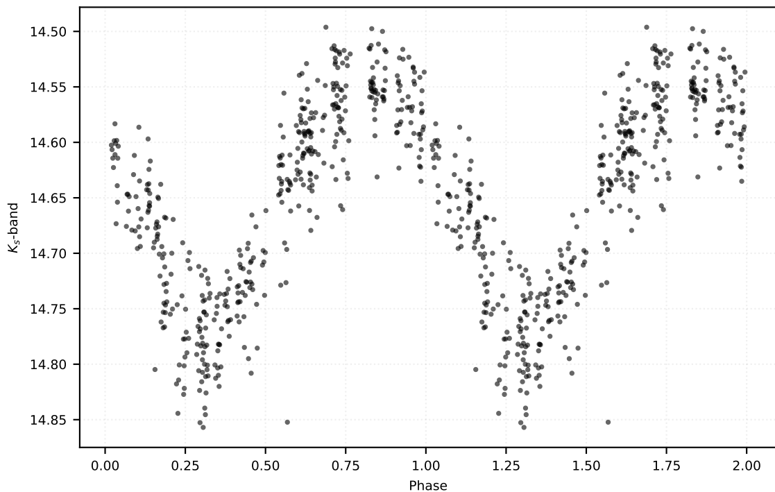
P: 0.16789 d | Class: RP | Subclass: UVAR | Field b278
