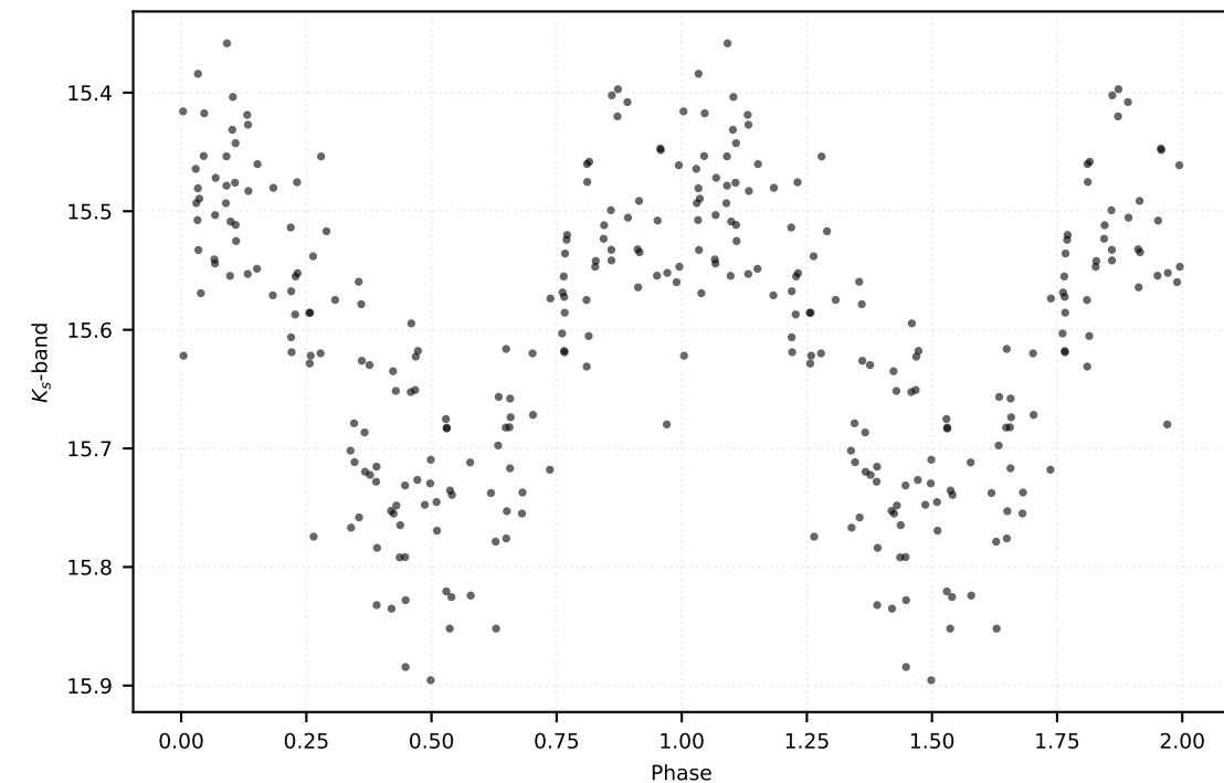
P: 0.31972 d | Class: RP | Subclass: RRab | Field b279
