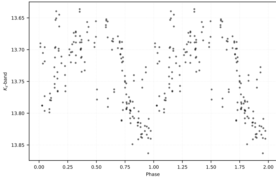
P: 3.08503 d | Class: RP | Subclass: CEP-F | Field b279
