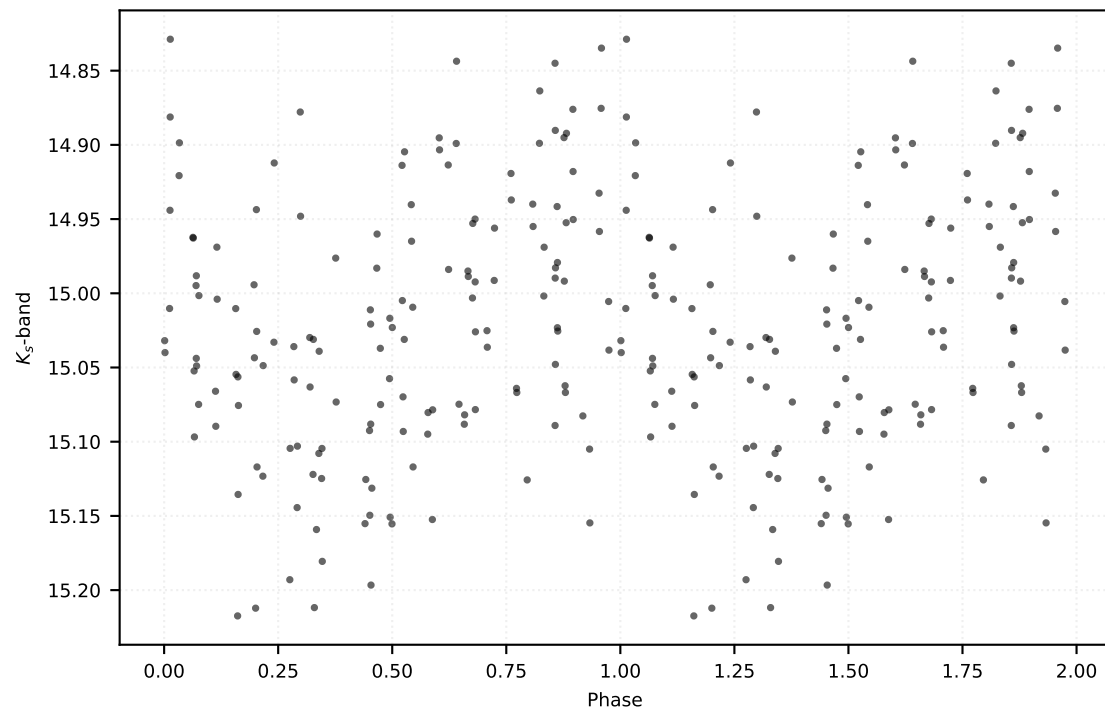
P: 34.79573 d | Class: RP | Subclass: CEP-F | Field b279
