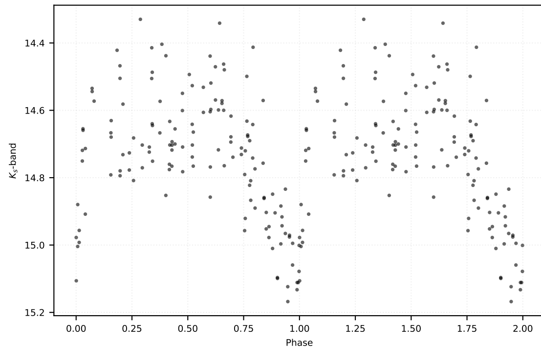
P: 0.53358 d | Class: RP | Subclass: CEP-10T | Field b279
