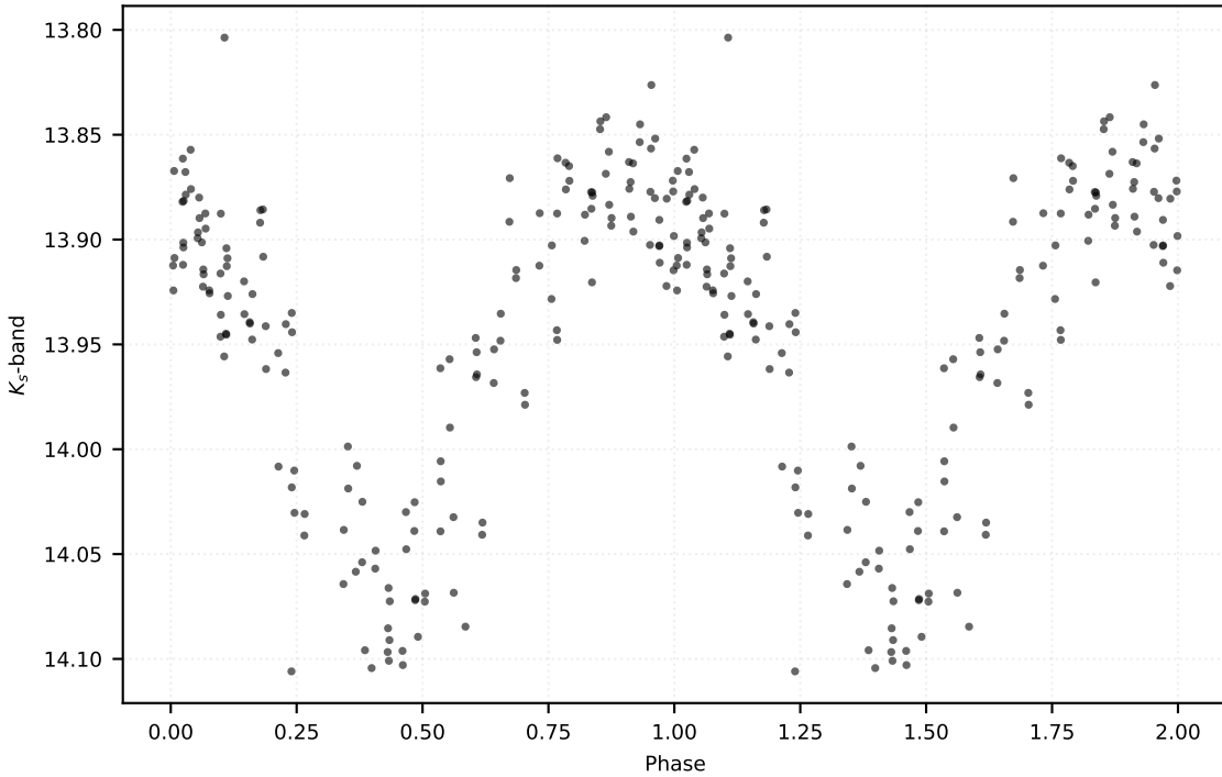
P: 0.47484 d | Class: RP | Subclass: RRab | Field b278
