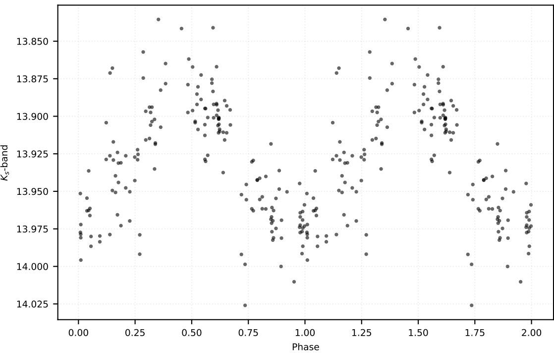
P: 0.43609 d | Class: RP | Subclass: CEP-10T | Field b278
