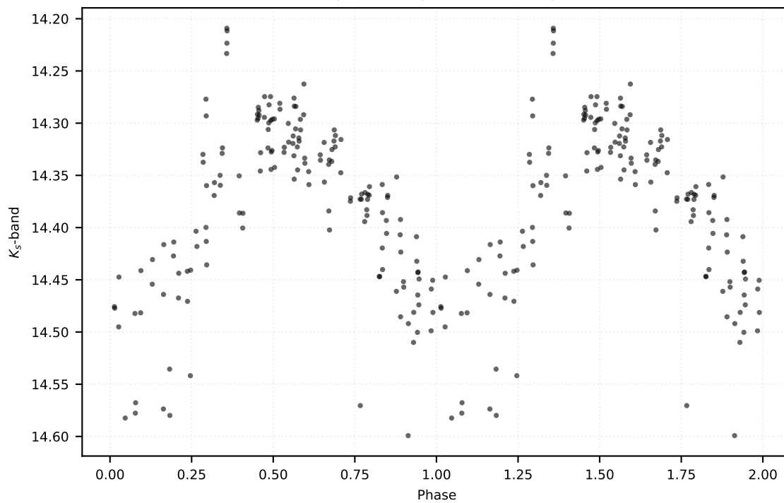
P: 0.63686 d | Class: RP | Subclass: RRab | Field b279
