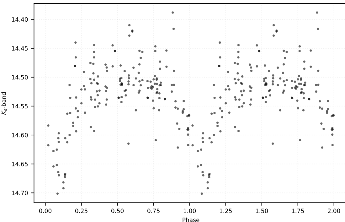
P: 1.30087 d | Class: RP | Subclass: CEP-10T | Field b278
