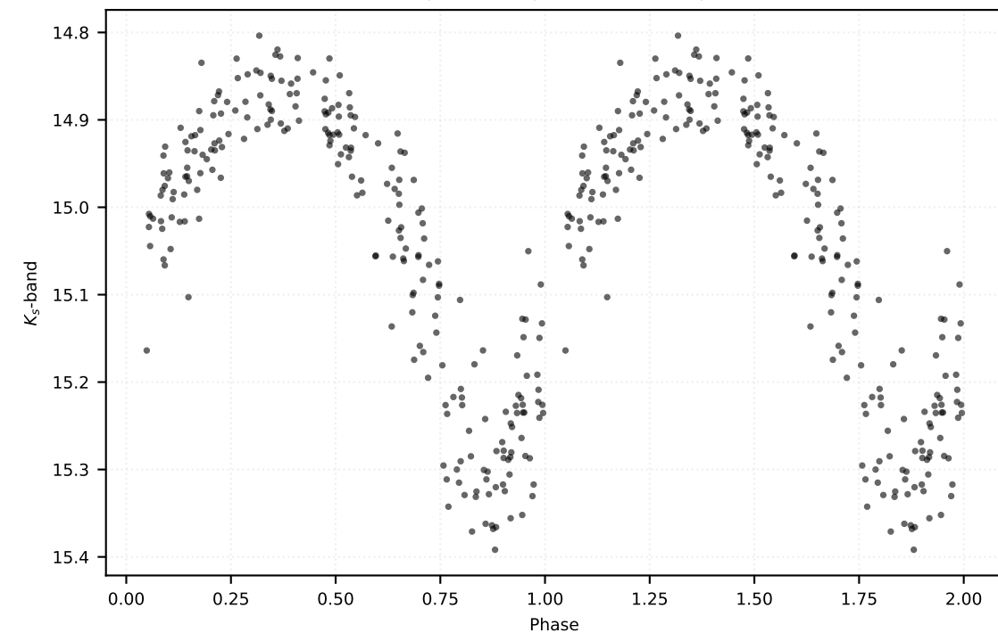
P: 0.14191 d | Class: RP | Subclass: UVAR | Field b278
