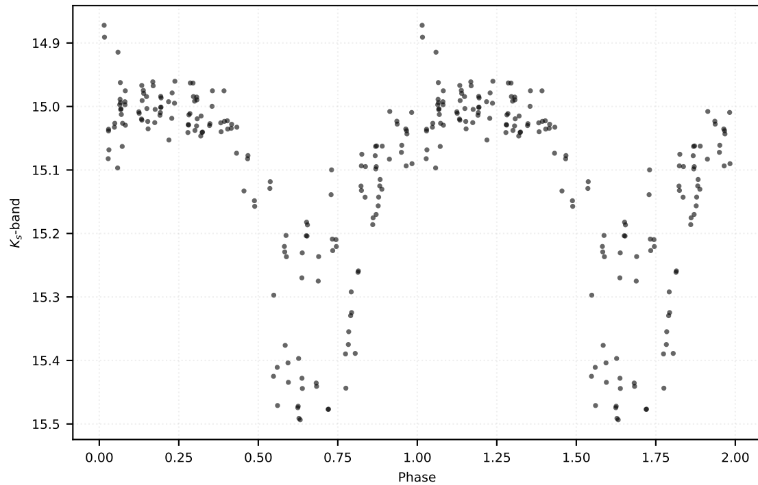
P: 4.06547 d | Class: RP | Subclass: CEP-1OT | Field b278
