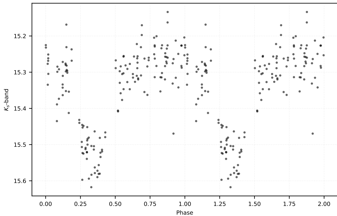
P: 0.57841 d | Class: RP | Subclass: RRab | Field b278
