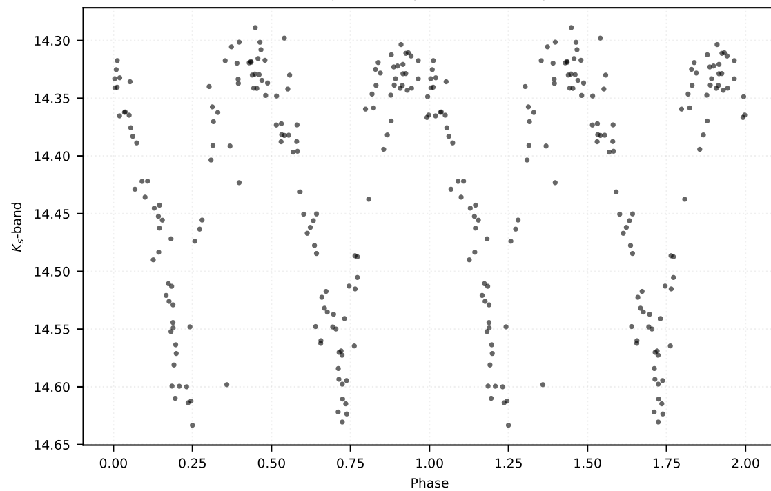
P: 0.17362 d | Class: RP | Subclass: UVAR | Field b279
