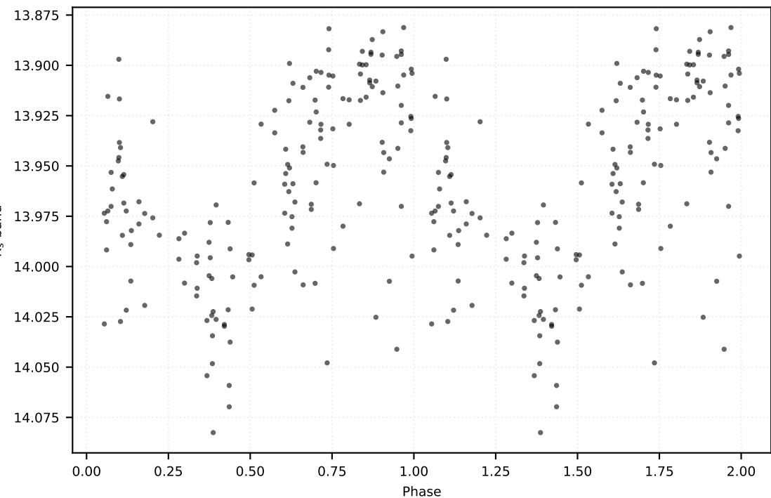
P: 0.49901 d | Class: RP | Subclass: CEP-10T | Field b279
