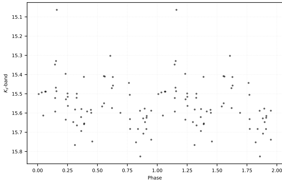
P: 0.40750 d | Class: EB | Subclass: EA | Field b278
