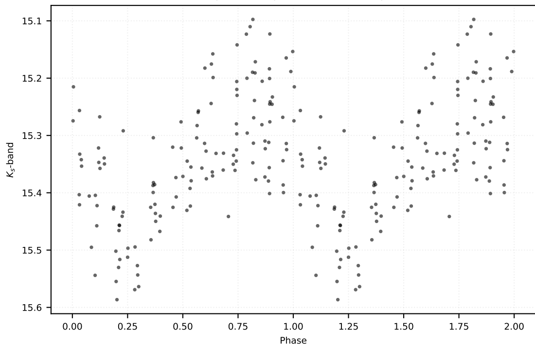
P: 0.31227 d | Class: RP | Subclass: CEP-1OT | Field b278
