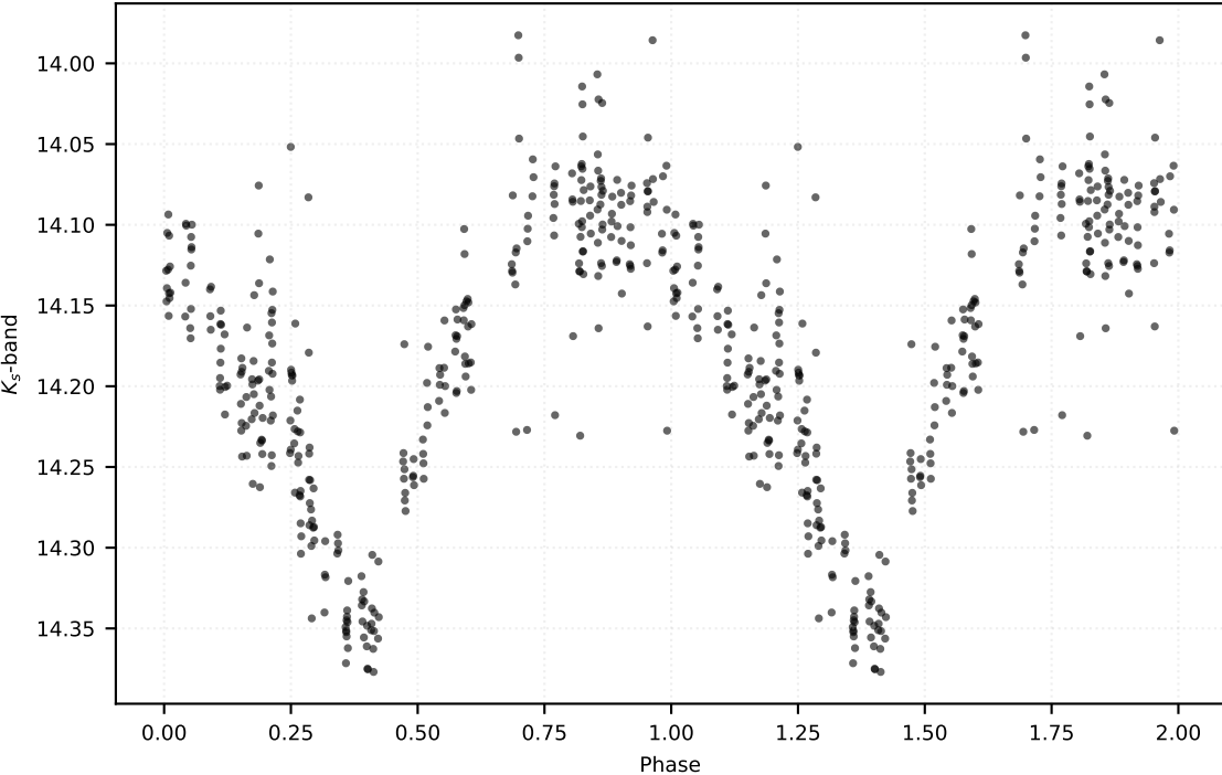
P: 0.58732 d | Class: RP | Subclass: RRab | Field b278
