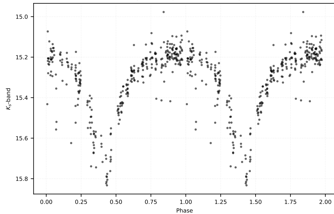
P: 0.43007 d | Class: RP | Subclass: CEP-10T | Field b279
