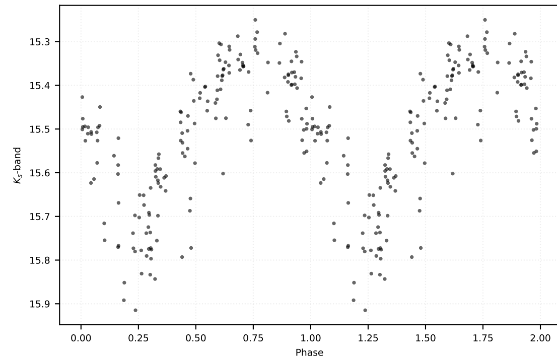
P: 0.41650 d | Class: RP | Subclass: RRab | Field b278
