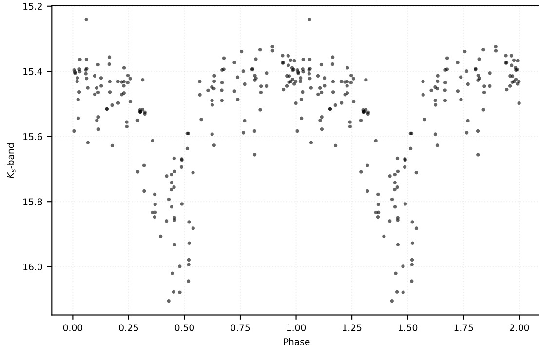
P: 0.50722 d | Class: RP | Subclass: RRab | Field b278
