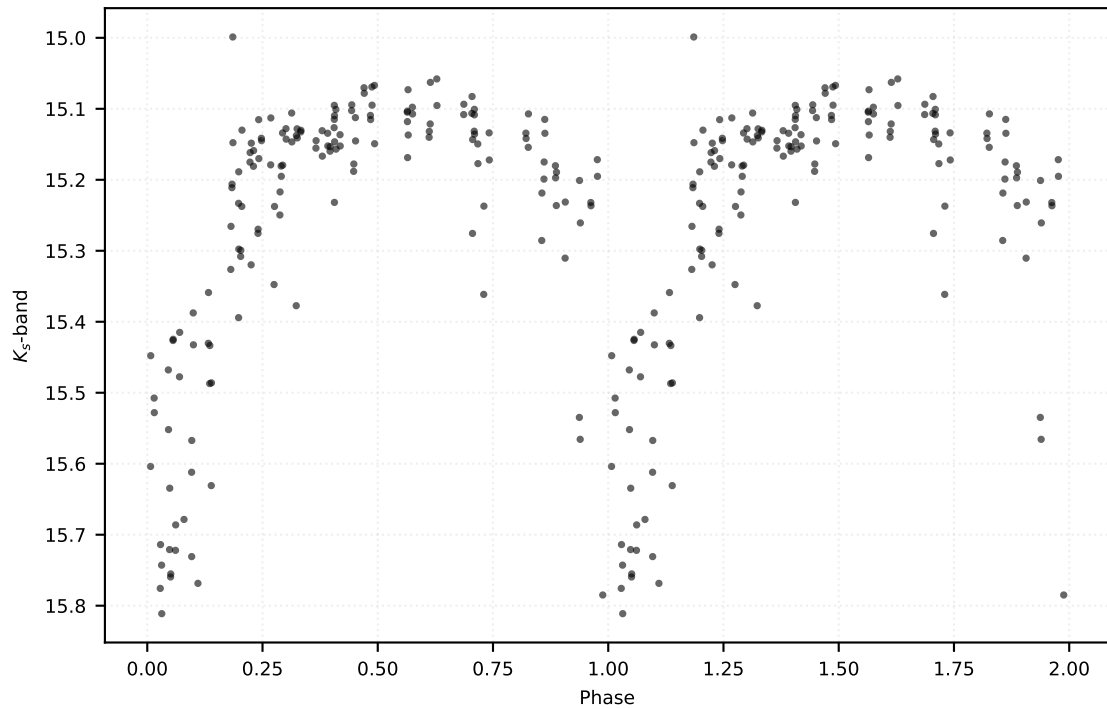
P: 1.80267 d | Class: RP | Subclass: CEP-F | Field b279
