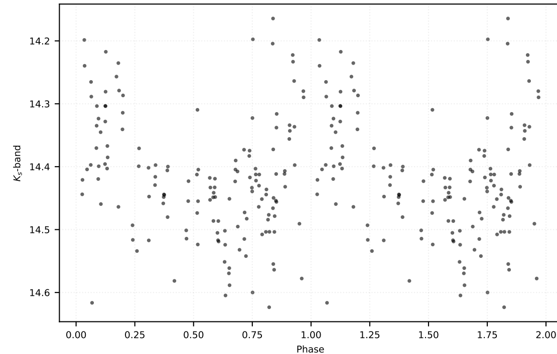
P: 0.34913 d | Class: RP | Subclass: RRab | Field b279
