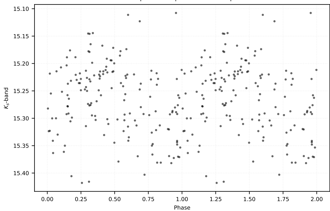
P: 68.31087 d | Class: RP | Subclass: UVAR | Field b279
