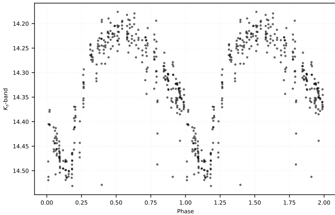
P: 0.55637 d | Class: RP | Subclass: RRab | Field b279
