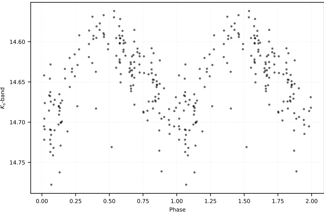
P: 0.24932 d | Class: RP | Subclass: RRc | Field b278
