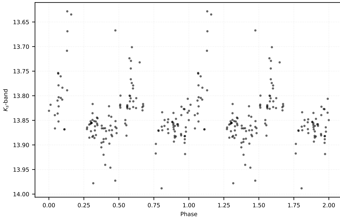
P: 0.39890 d | Class: EB | Subclass: EA | Field b279
