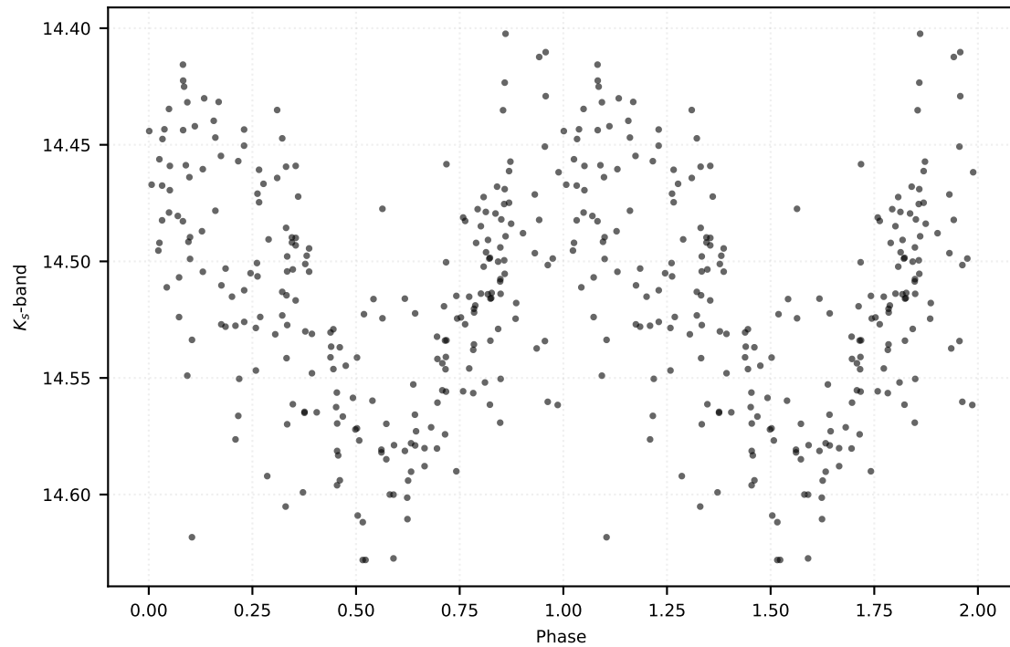
P: 5.86766 d | Class: RP | Subclass: CEP-F | Field b279
