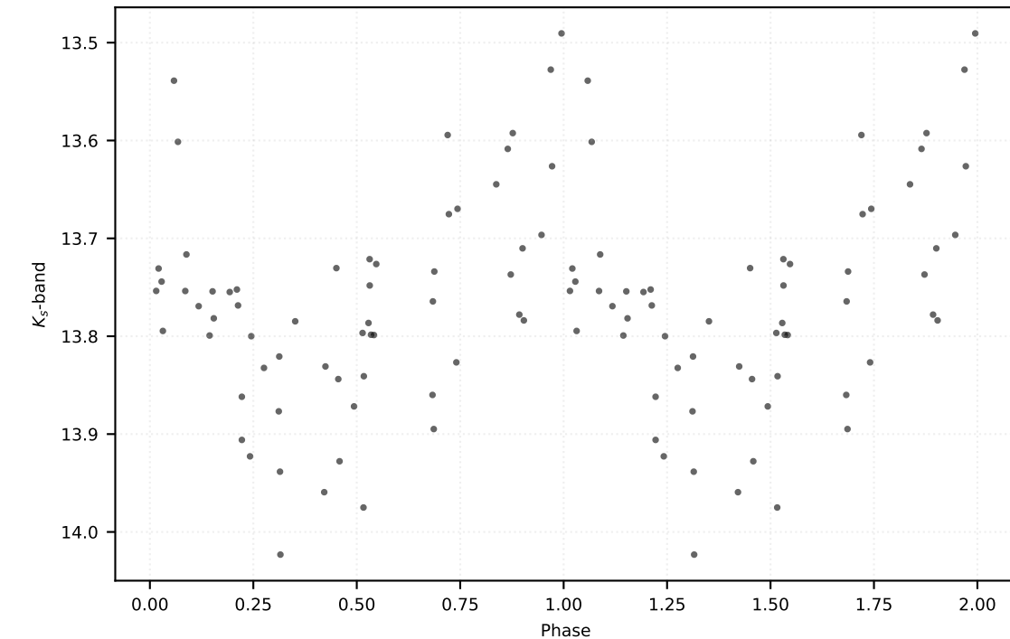
P: 0.13643 d | Class: RP | Subclass: UVAR | Field b279
