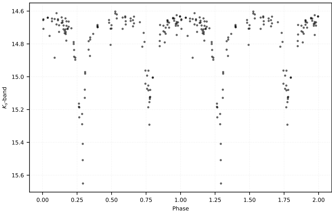
P: 5.02460 d | Class: EB | Subclass: EA | Field b279
