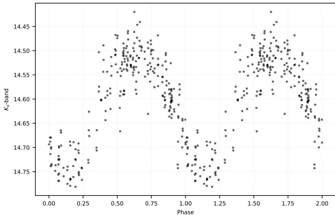
P: 0.46722 d | Class: RP | Subclass: RRab | Field b278
