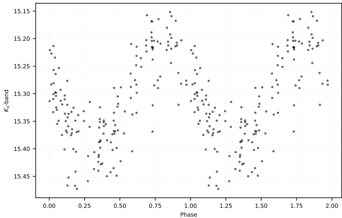
P: 0.66057 d | Class: RP | Subclass: CEP-10T | Field b278
