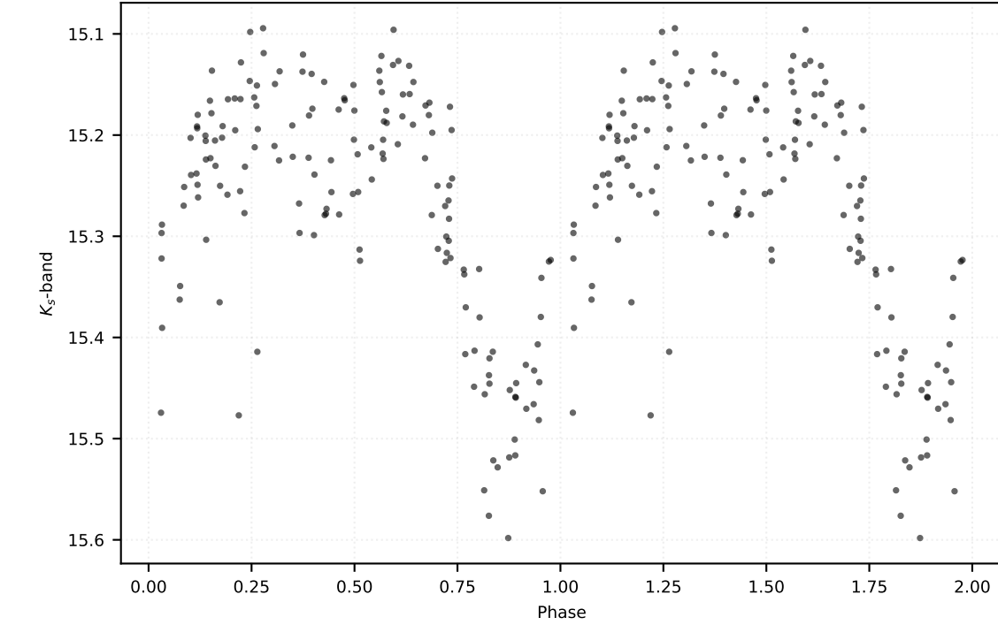
P: 0.33244 d | Class: RP | Subclass: RRc | Field b279
