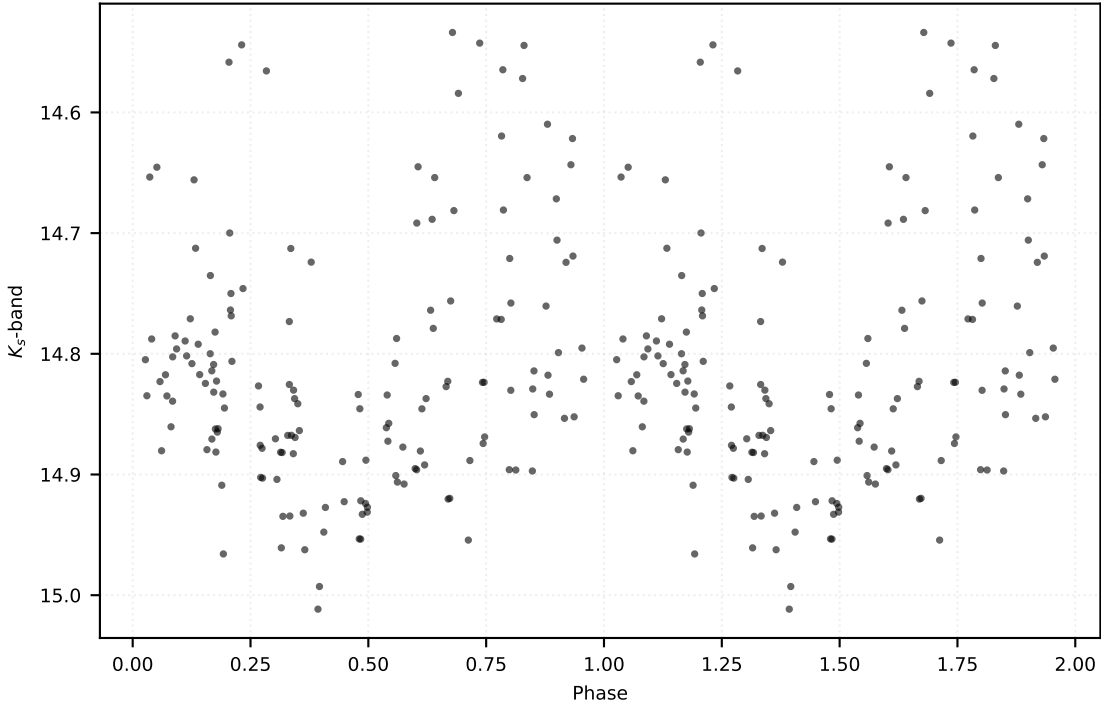
P: 38.50255 d | Class: RP | Subclass: UVAR | Field b278
