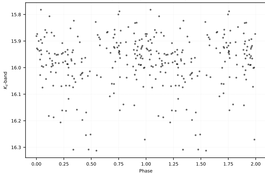
P: 0.16504 d | Class: RP | Subclass: UVAR | Field b278
