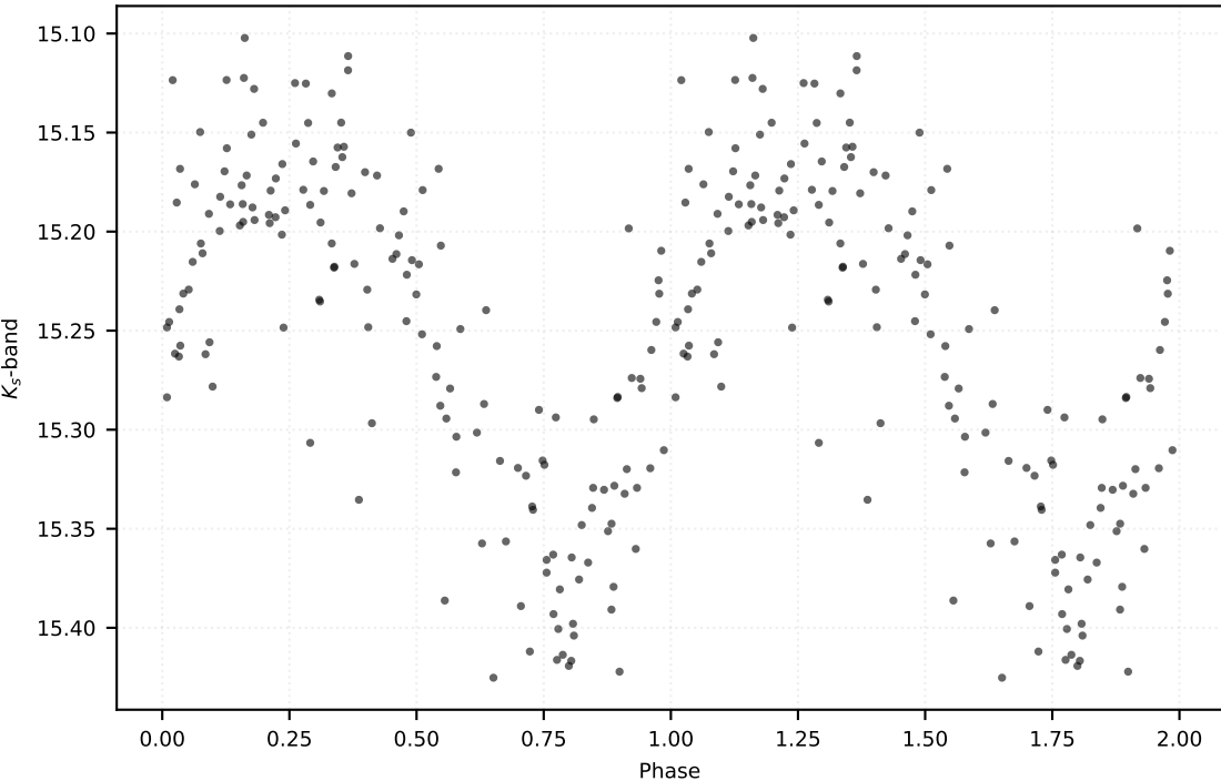
P: 0.61215 d | Class: RP | Subclass: RRab | Field b279
