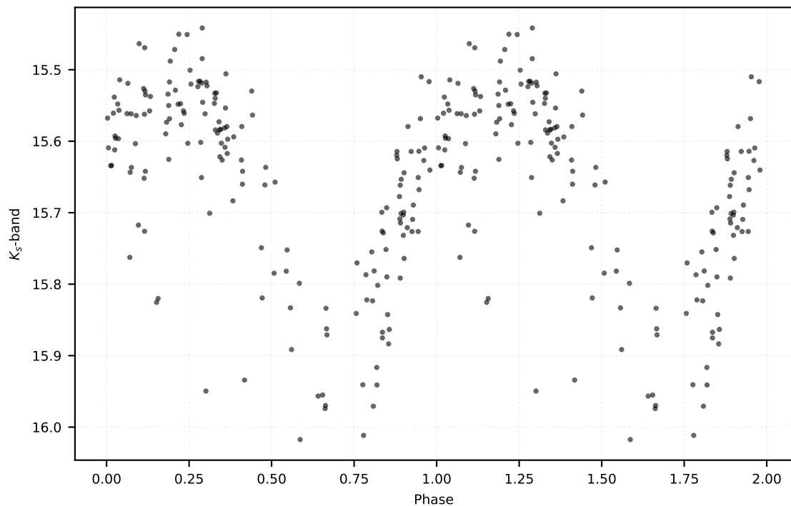
P: 0.62057 d | Class: RP | Subclass: RRab | Field b279
