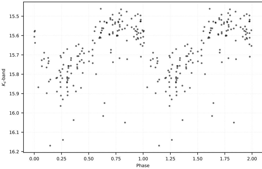
P: 0.29309 d | Class: RP | Subclass: UVAR | Field b279
