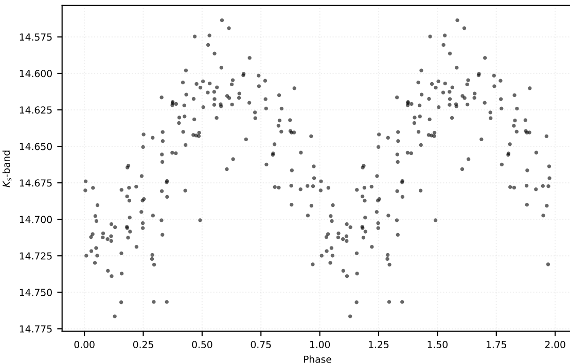
P: 0.43308 d | Class: RP | Subclass: RRab | Field b278
