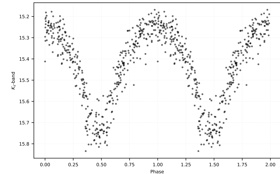
P: 0.21365 d | Class: RP | Subclass: UVAR | Field b279
