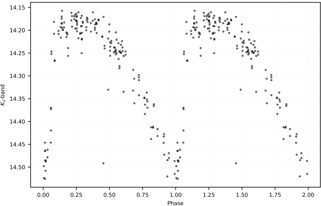
P: 0.55601 d | Class: RP | Subclass: RRab | Field b278
