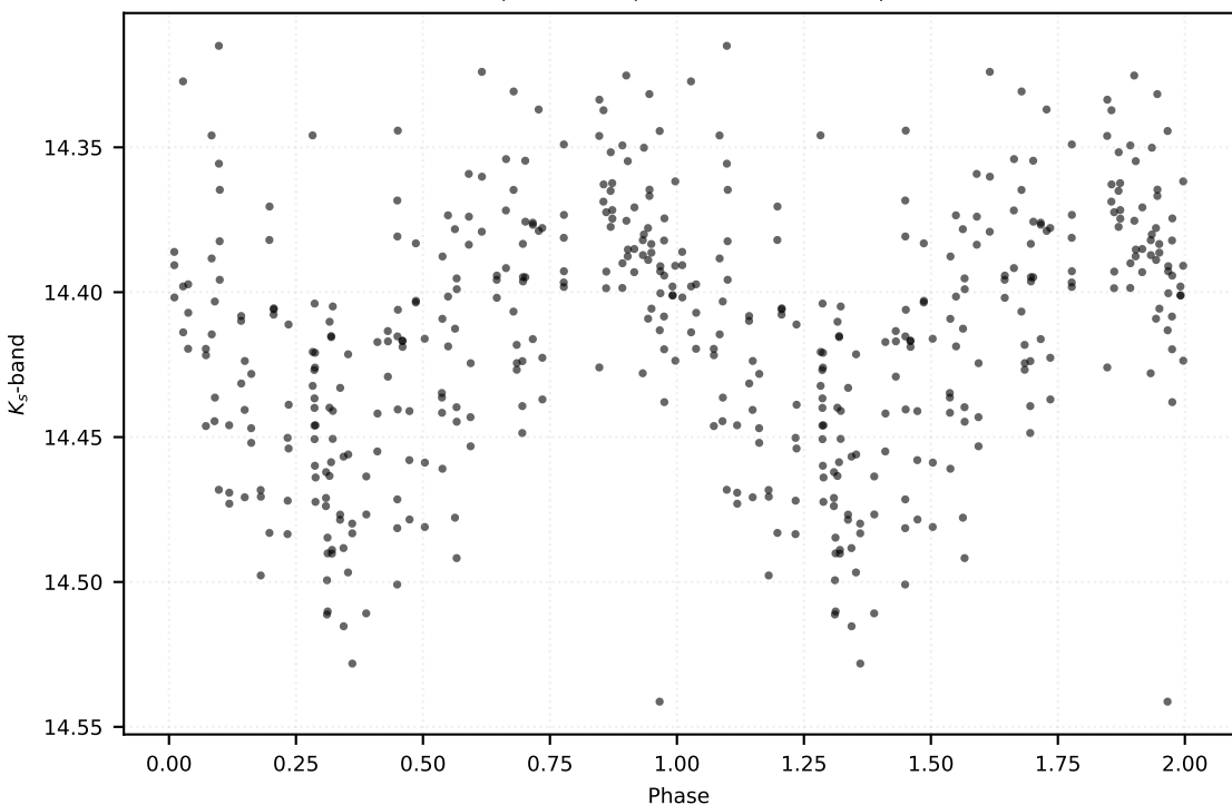
P: 6.95027 d | Class: RP | Subclass: CEP-1OT | Field b279
