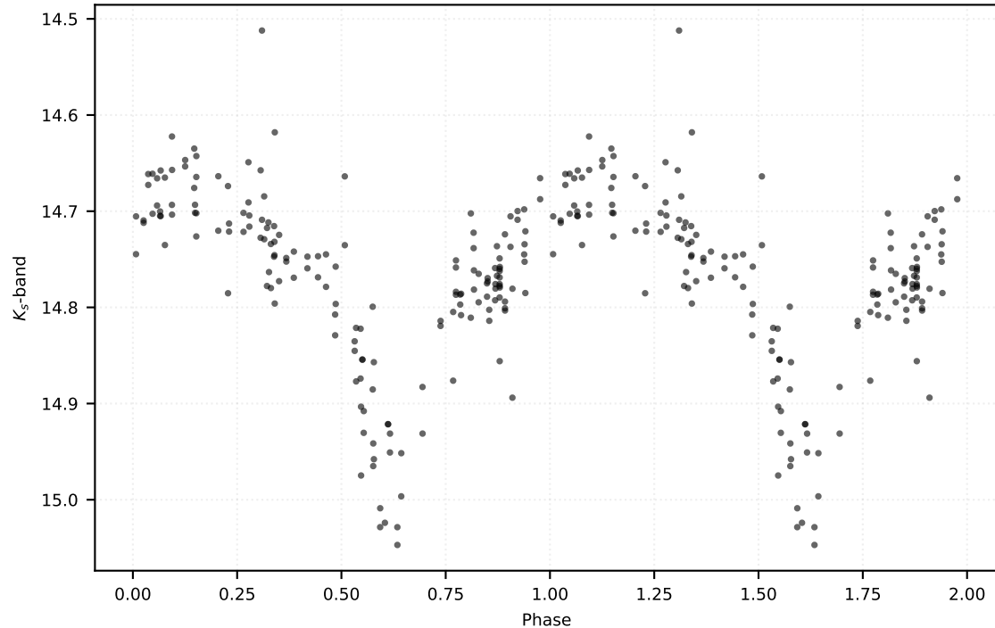
P: 0.72201 d | Class: RP | Subclass: CEP-10T | Field b278
