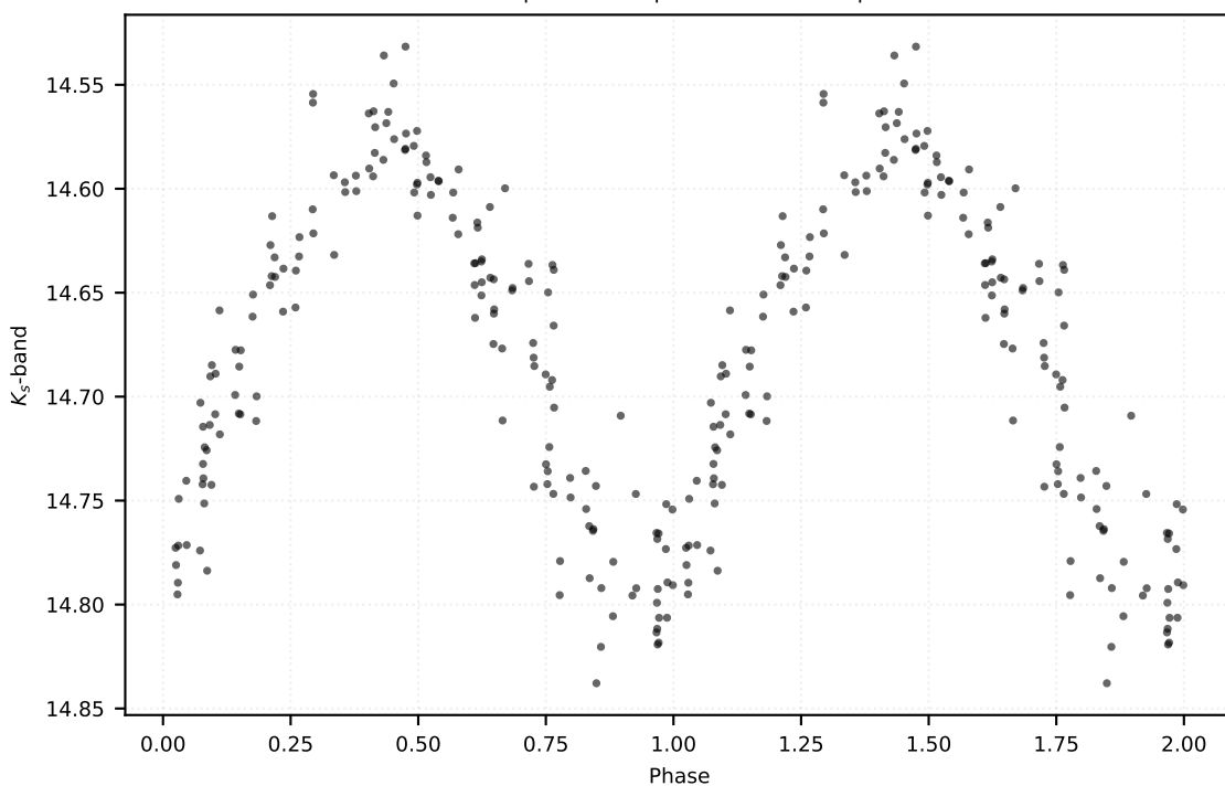
P: 0.68405 d | Class: RP | Subclass: RRab | Field b278
