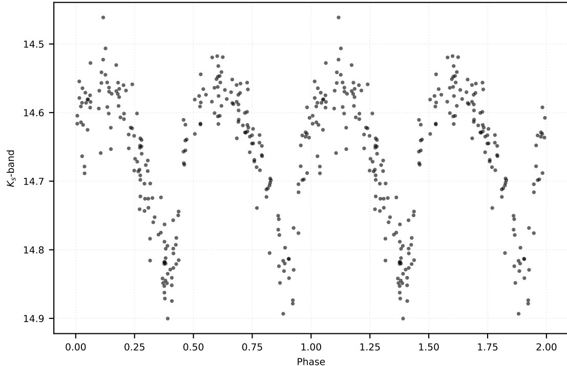
P: 1.15184 d | Class: EB | Subclass: EW | Field b278
