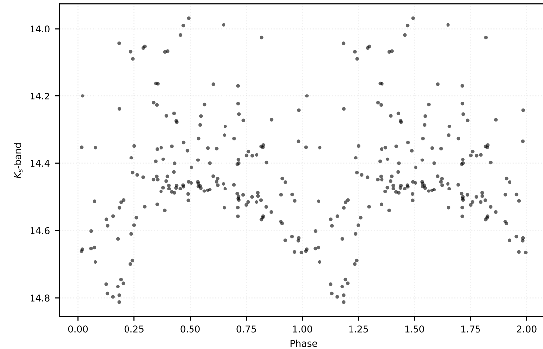
P: 0.66693 d | Class: RP | Subclass: RRab | Field b278
