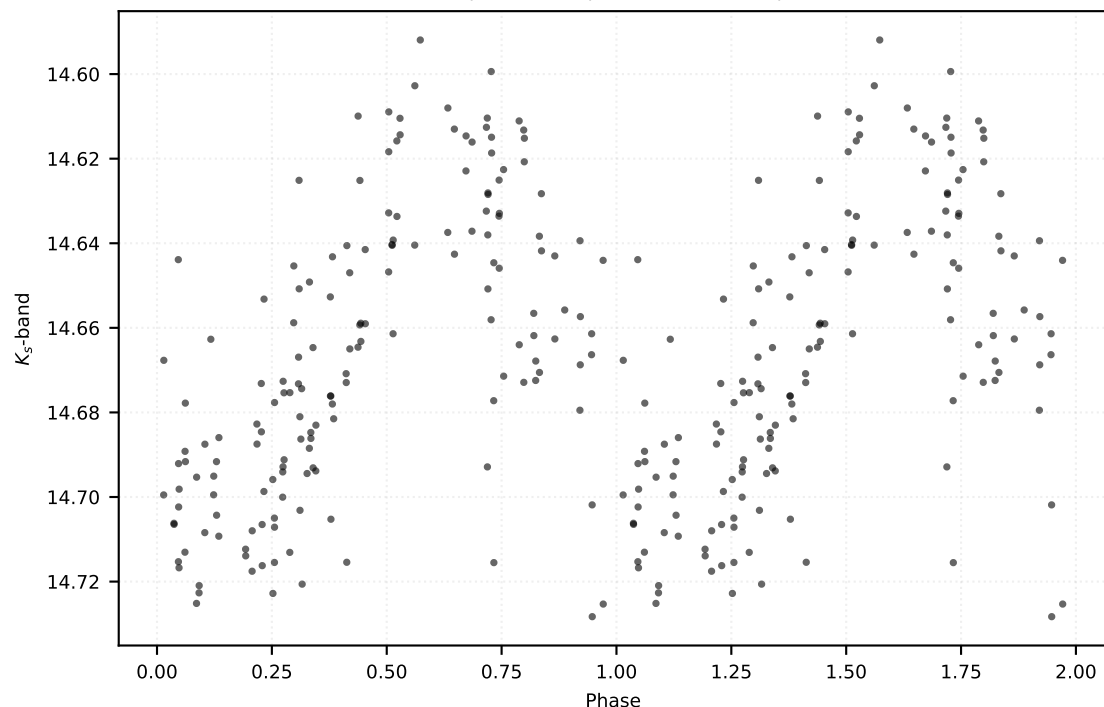
P: 3.81668 d | Class: RP | Subclass: CEP-F | Field b278
