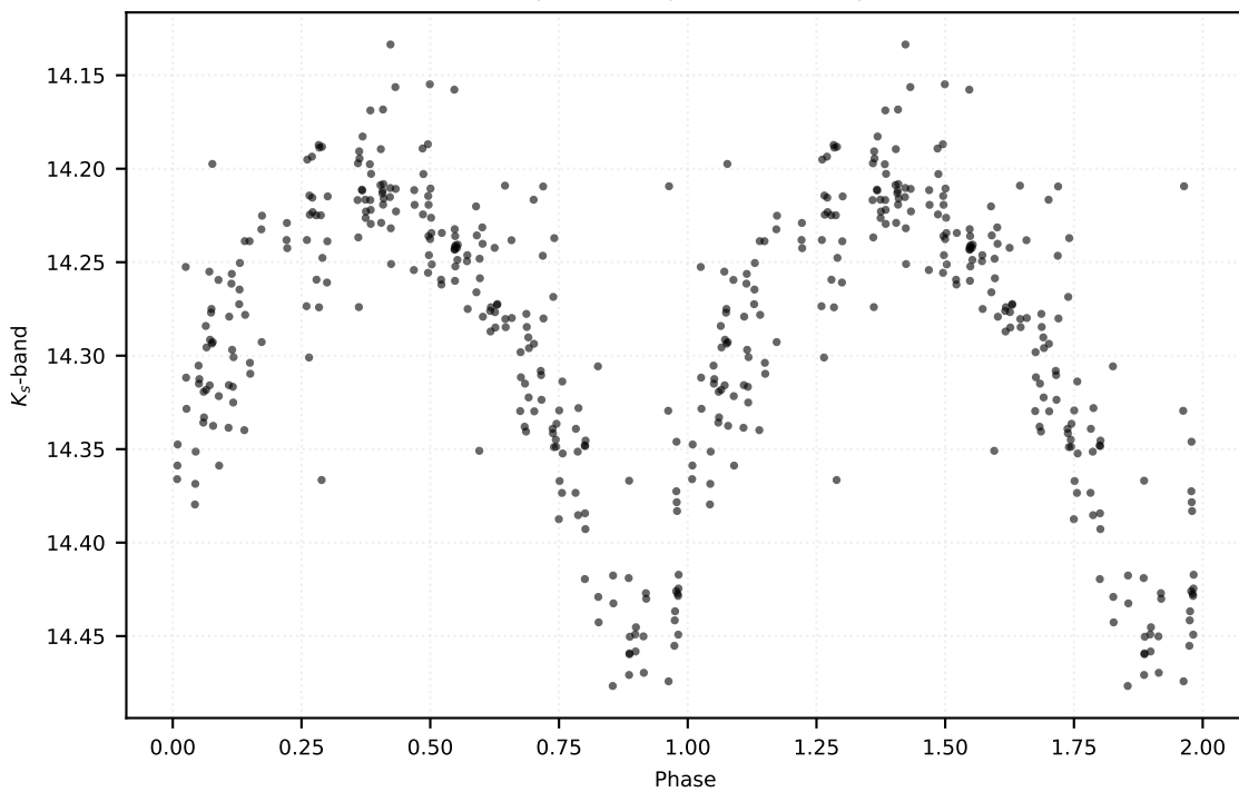
P: 0.39480 d | Class: RP | Subclass: RRc | Field b278
