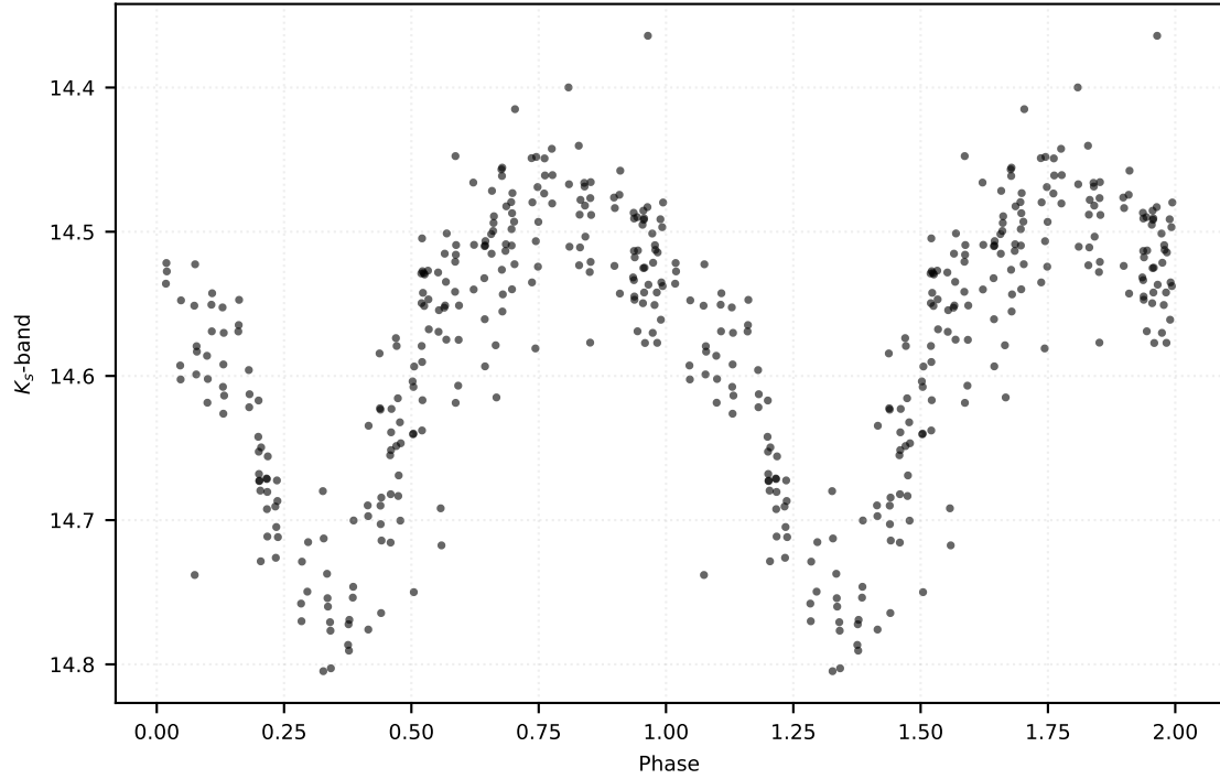
P: 0.45763 d | Class: RP | Subclass: RRab | Field b278
