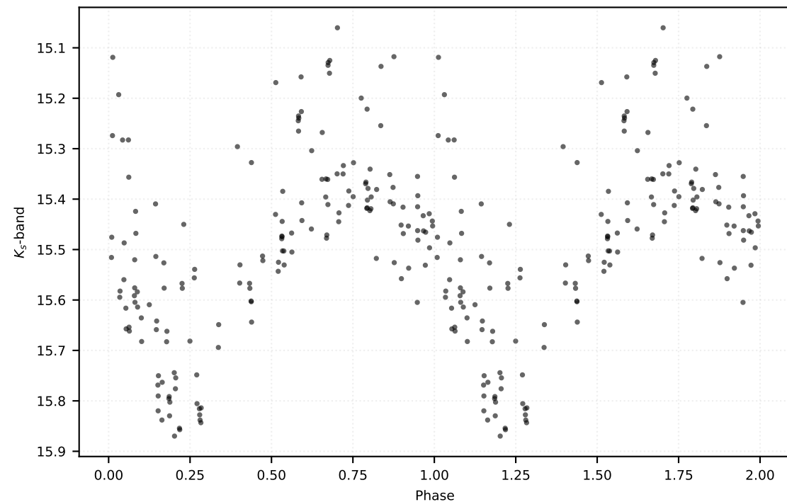
P: 0.51261 d | Class: RP | Subclass: RRab | Field b278
