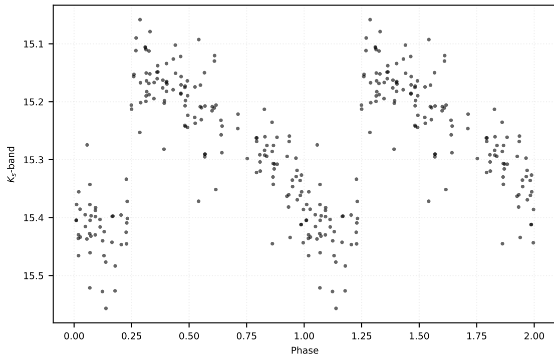
P: 0.40333 d | Class: RP | Subclass: RRab | Field b278
