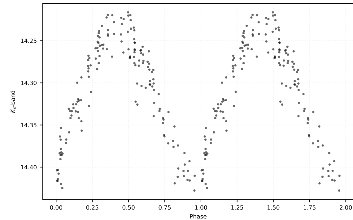
P: 0.19255 d | Class: RP | Subclass: UVAR | Field b279
