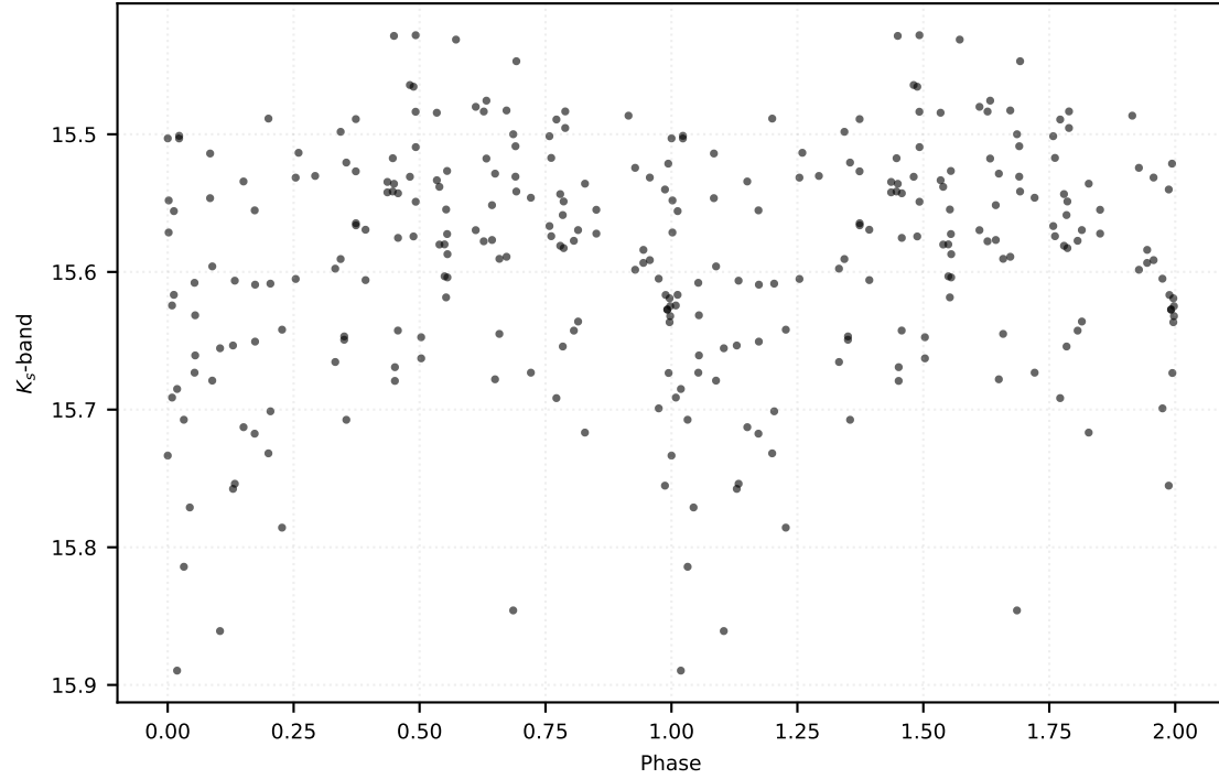
P: 10.41285 d | Class: RP | Subclass: UVAR | Field b279
