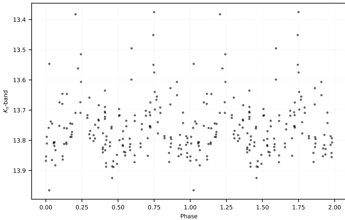
P: 101.10162 d | Class: EB | Subclass: EA | Field b279
