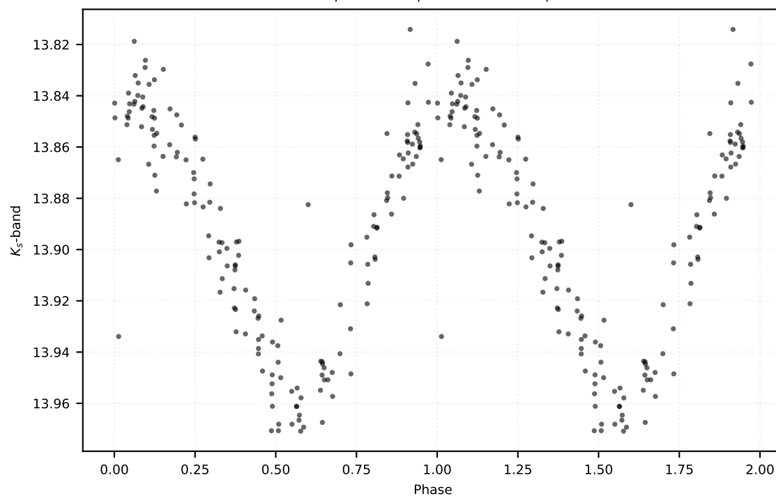
P: 0.62430 d | Class: RP | Subclass: RRab | Field b278
