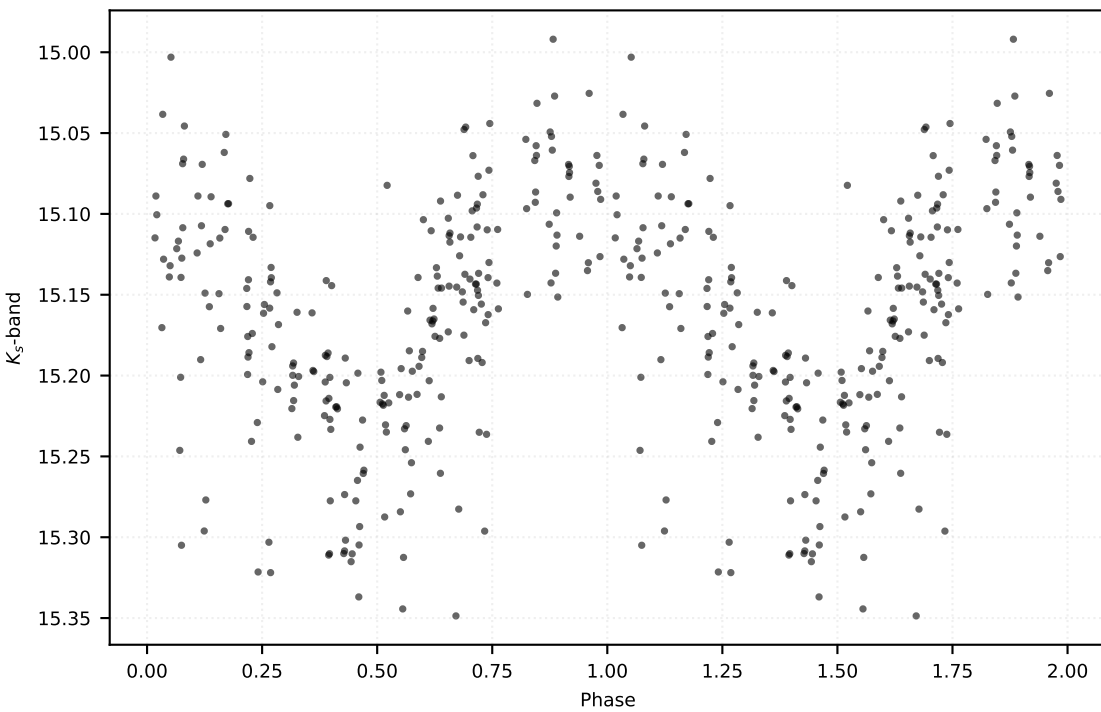
P: 0.15403 d | Class: RP | Subclass: UVAR | Field b278
