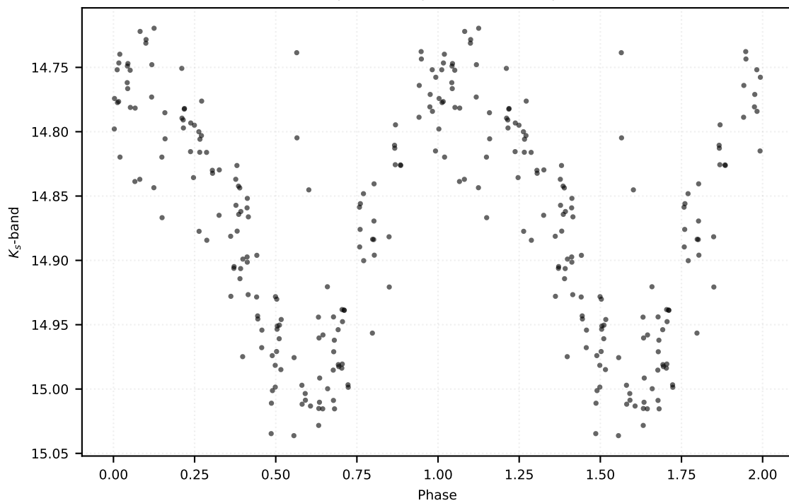
P: 0.47589 d | Class: RP | Subclass: RRab | Field b278
