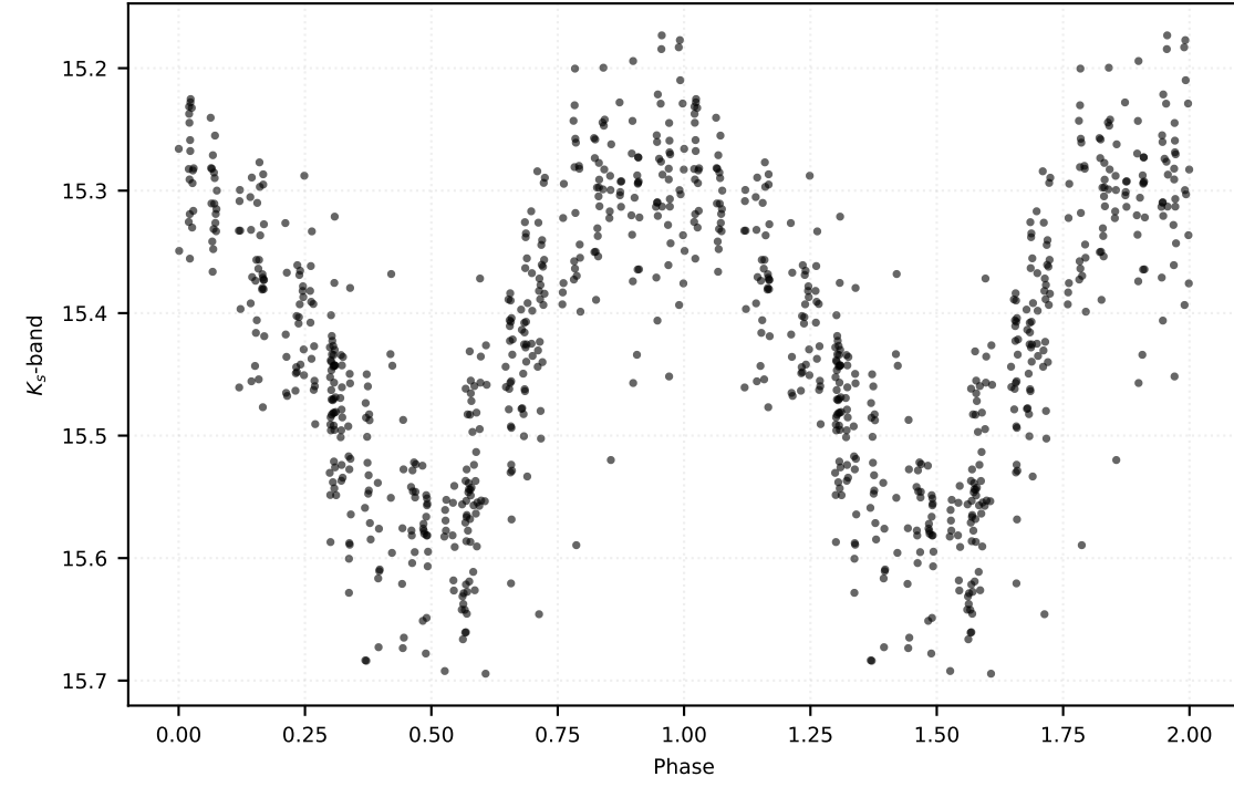
P: 0.55905 d | Class: RP | Subclass: RRc | Field b278
