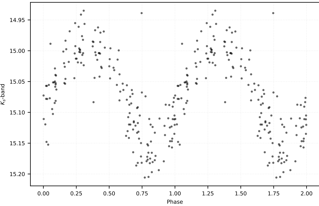
P: 0.14361 d | Class: RP | Subclass: UVAR | Field b278
