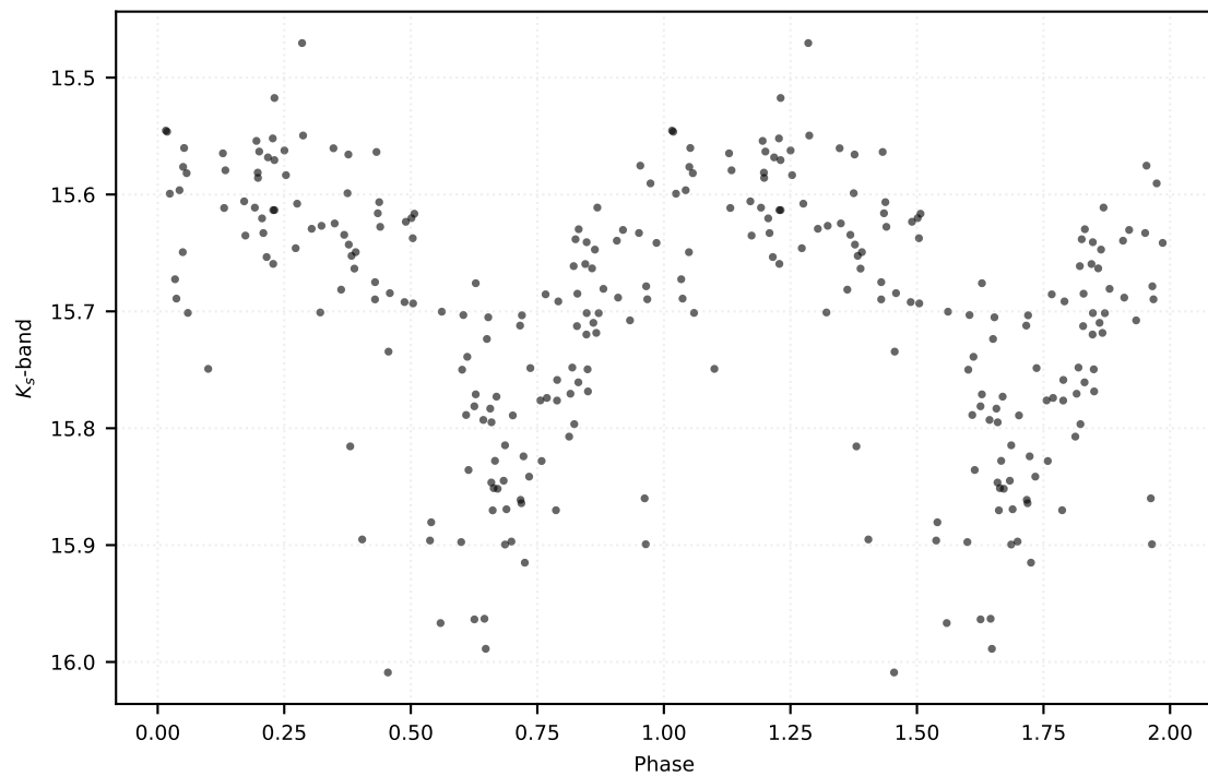
P: 0.75814 d | Class: RP | Subclass: RRab | Field b278
