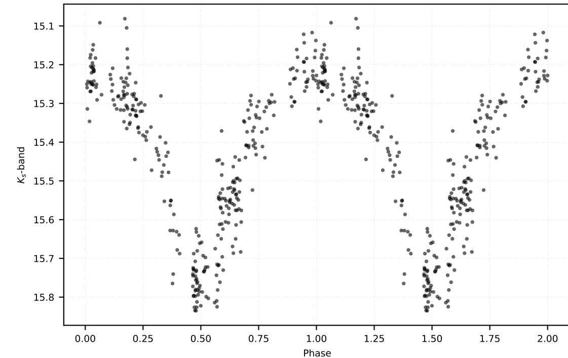
P: 0.15092 d | Class: RP | Subclass: UVAR | Field b279
