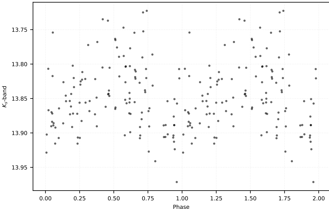
P: 35.01110 d | Class: RP | Subclass: UVAR | Field b279
