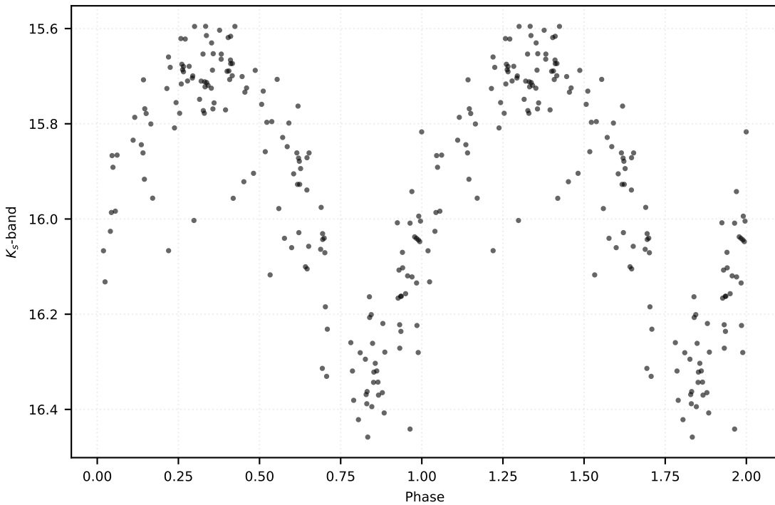
P: 0.17838 d | Class: RP | Subclass: UVAR | Field b278
