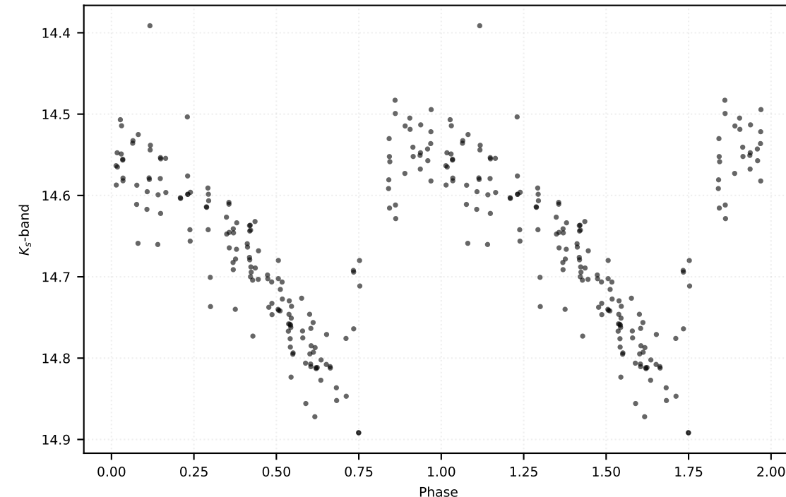
P: 0.49027 d | Class: RP | Subclass: RRab | Field b278
