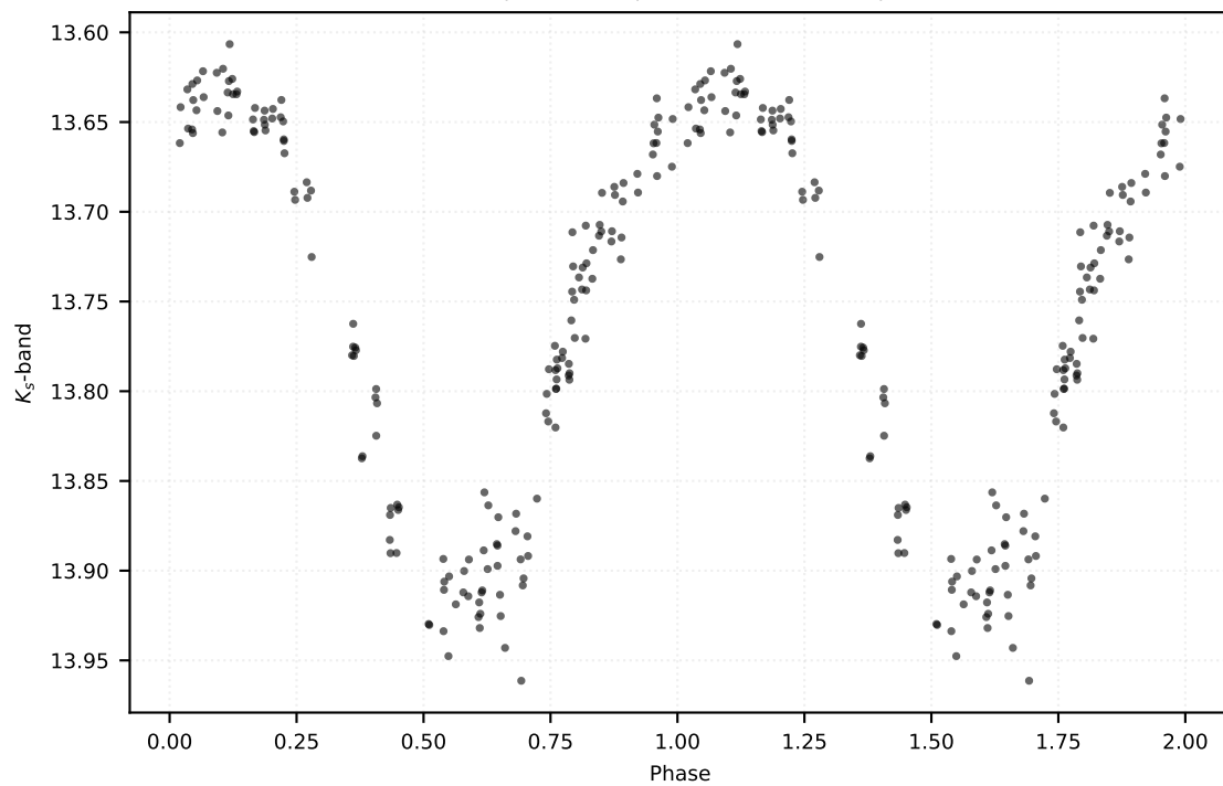
P: 0.58130 d | Class: RP | Subclass: CEP-1OT | Field b279
