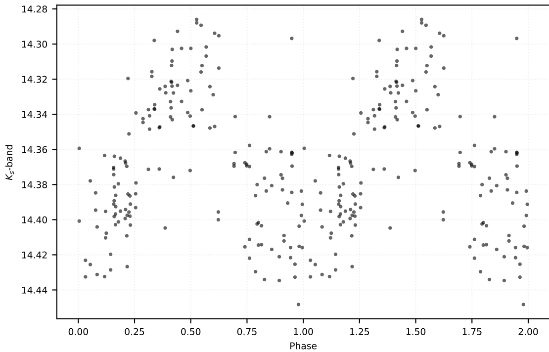
P: 11.59407 d | Class: RP | Subclass: UVAR | Field b278
