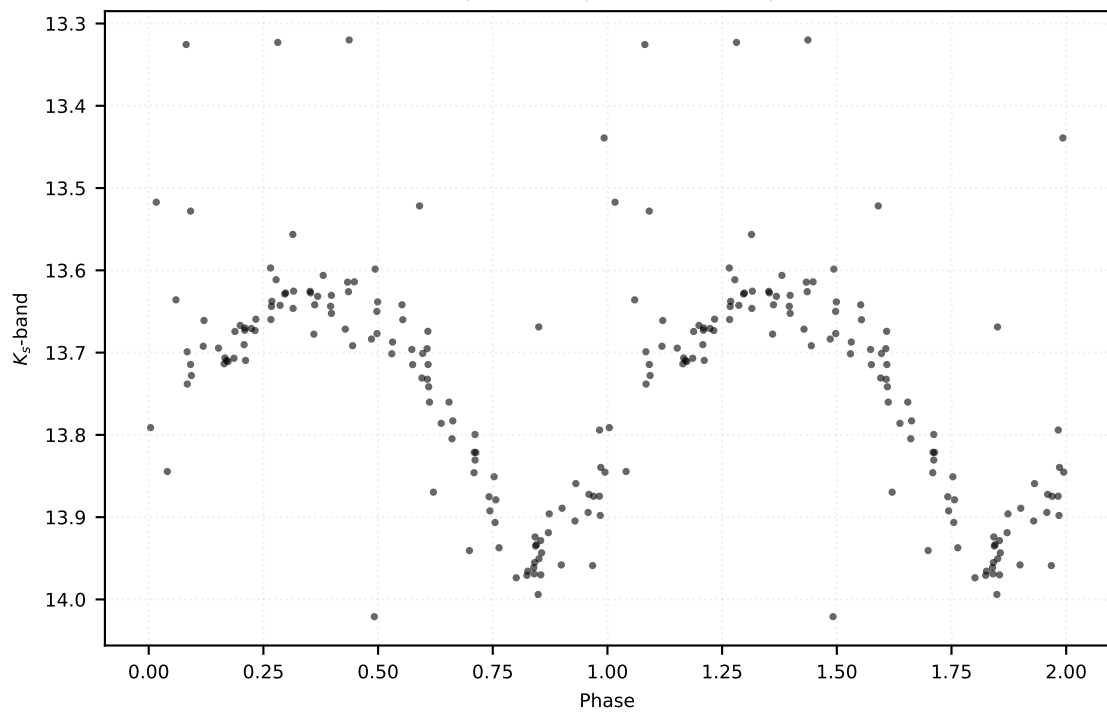
P: 0.57432 d | Class: RP | Subclass: RRab | Field b279
