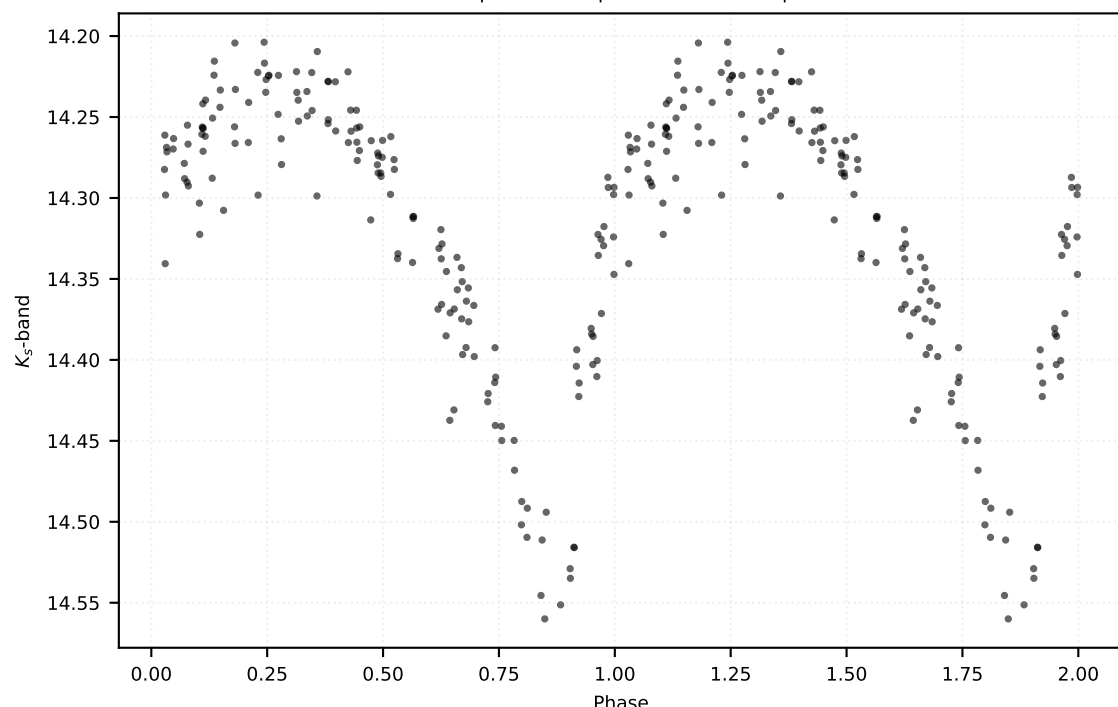
P: 0.60001 d | Class: RP | Subclass: RRab | Field b279
