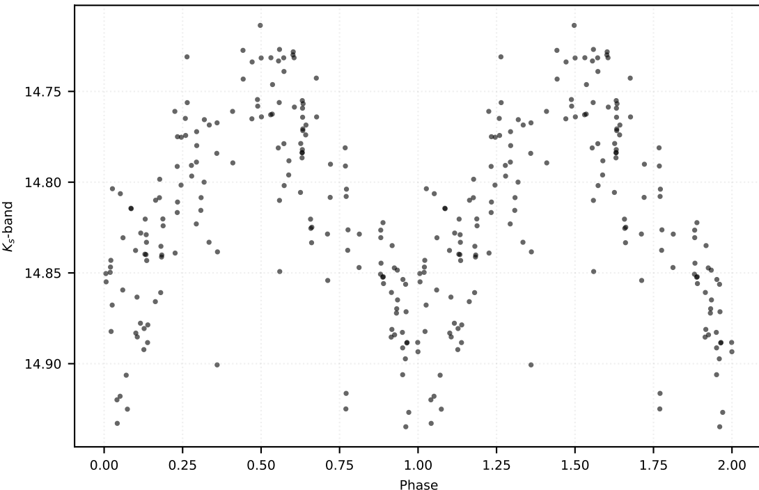
P: 0.31221 d | Class: RP | Subclass: CEP-10T | Field b278
