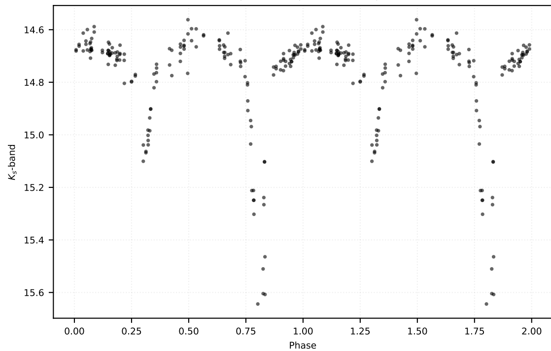
P: 4.74512 d | Class: EB | Subclass: EA | Field b278
