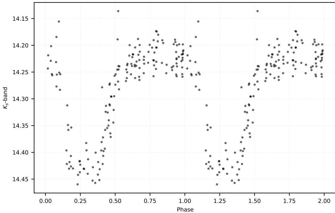
P: 0.45892 d | Class: RP | Subclass: RRab | Field b278
