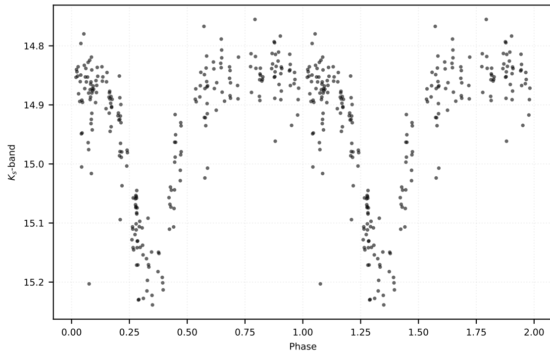
P: 0.16509 d | Class: RP | Subclass: UVAR | Field b279
