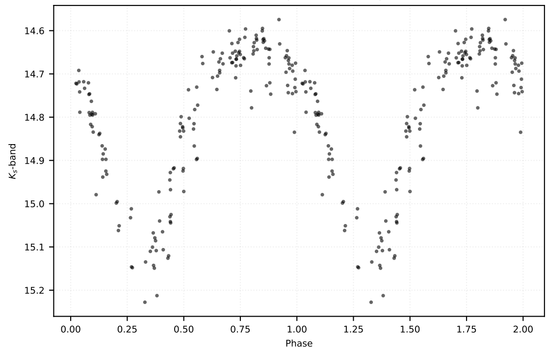
P: 0.12484 d | Class: RP | Subclass: UVAR | Field b279
