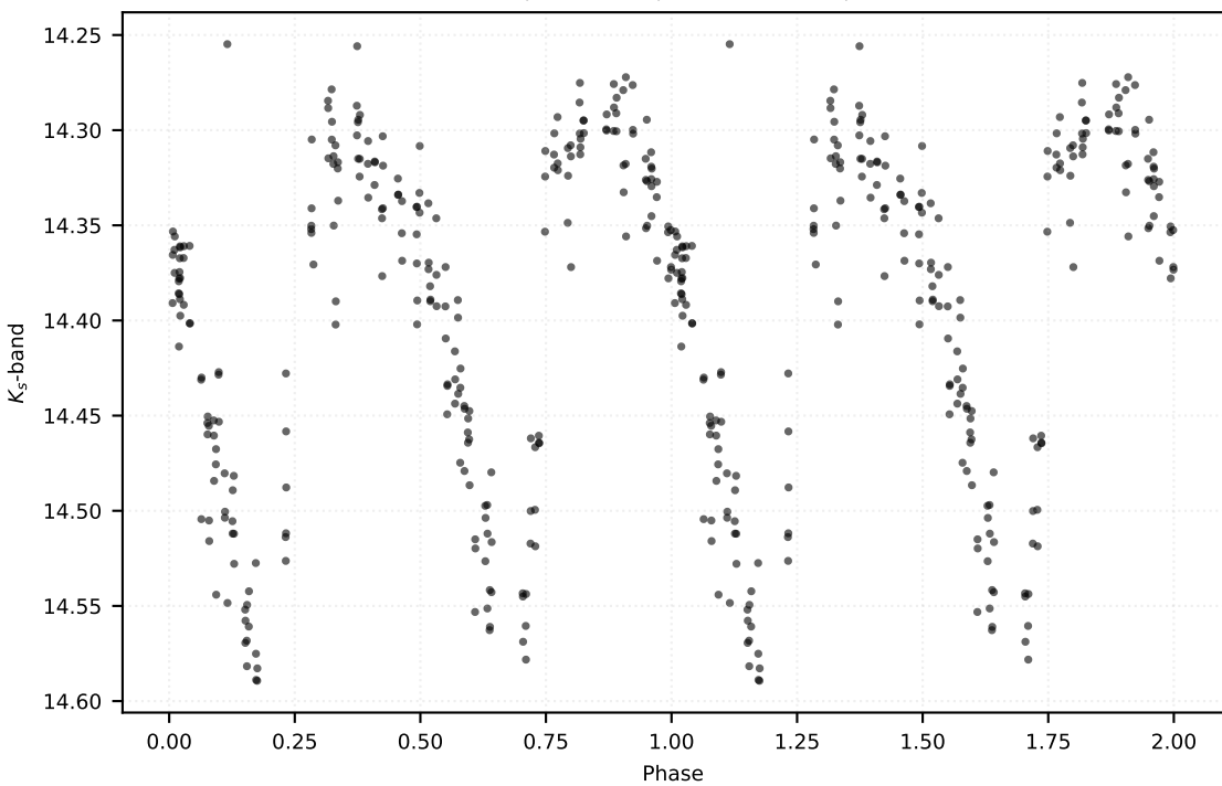
P: 0.50683 d | Class: RP | Subclass: RRc | Field b278
