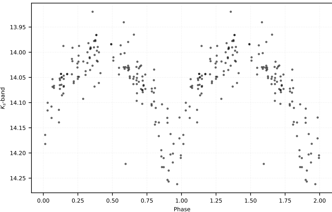
P: 0.64261 d | Class: RP | Subclass: CEP-10T | Field b279
