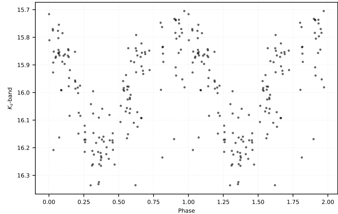
P: 0.27218 d | Class: RP | Subclass: UVAR | Field b279
