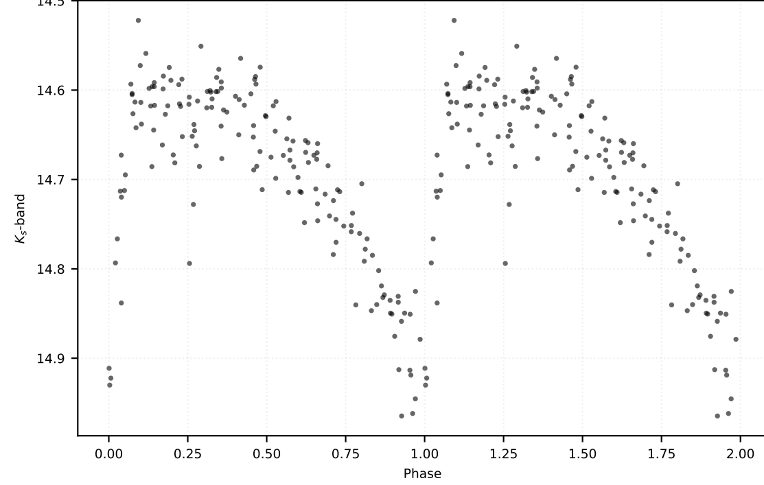
P: 0.45412 d | Class: RP | Subclass: RRab | Field b278
