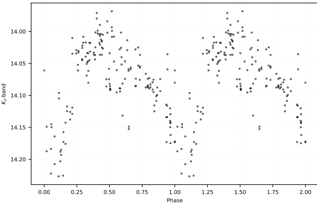
P: 6.34428 d | Class: RP | Subclass: CEP-F | Field b278
