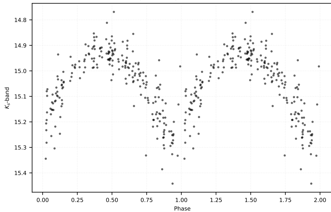
P: 0.16346 d | Class: RP | Subclass: UVAR | Field b279
