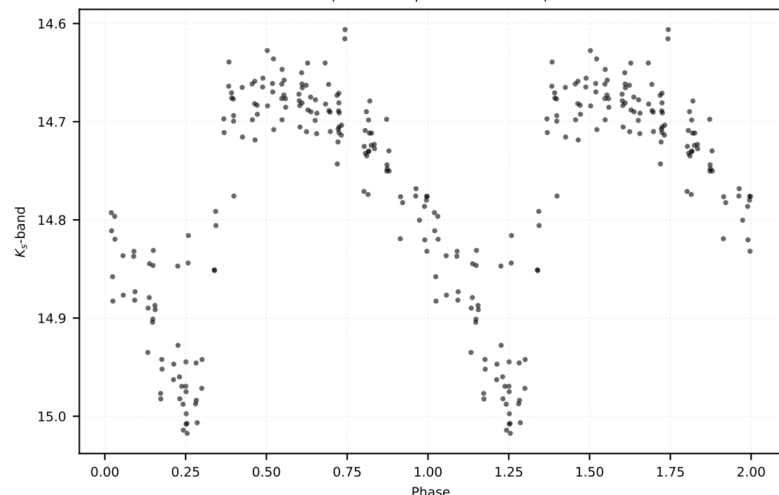
P: 0.60620 d | Class: RP | Subclass: RRab | Field b279
