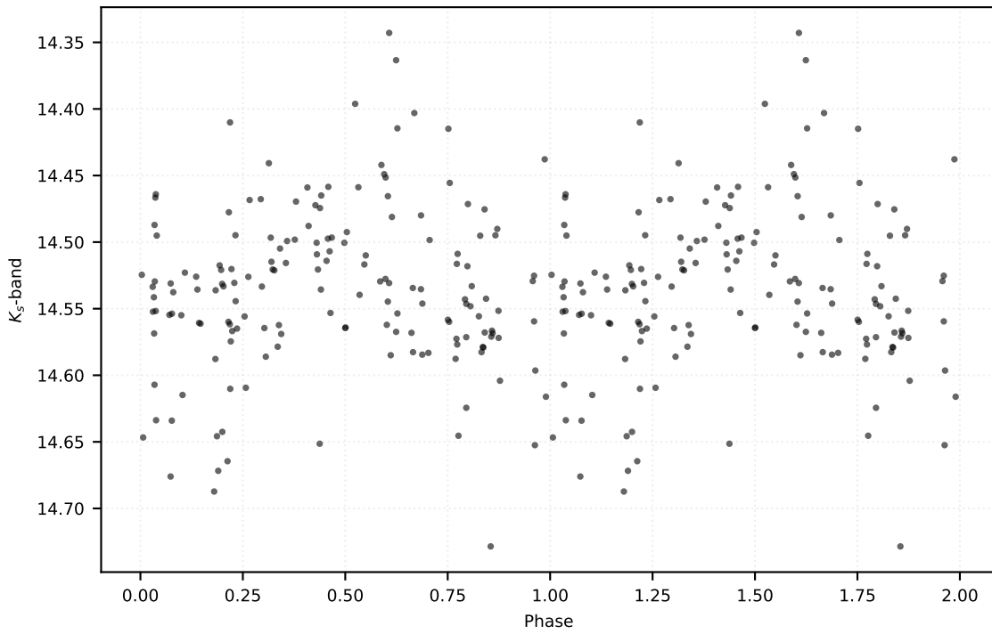
P: 0.13041 d | Class: RP | Subclass: UVAR | Field b279
