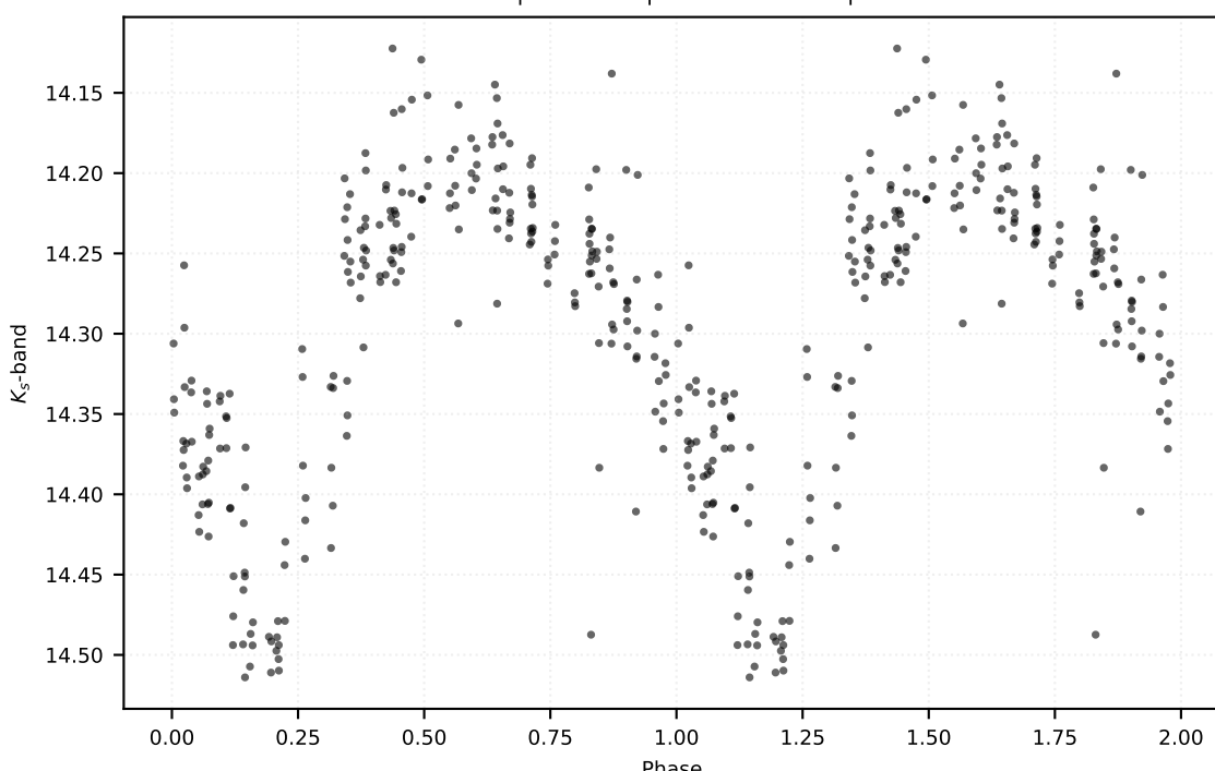
P: 0.52780 d | Class: RP | Subclass: RRab | Field b279
