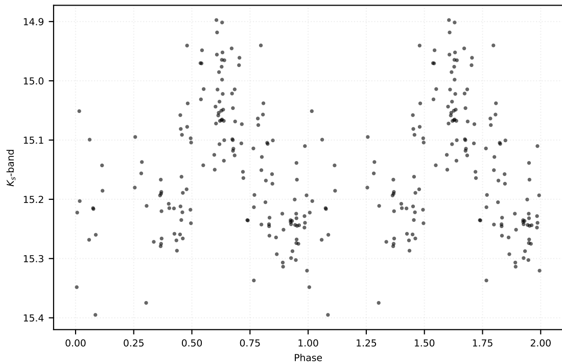
P: 0.22221 d | Class: RP | Subclass: UVAR | Field b279
