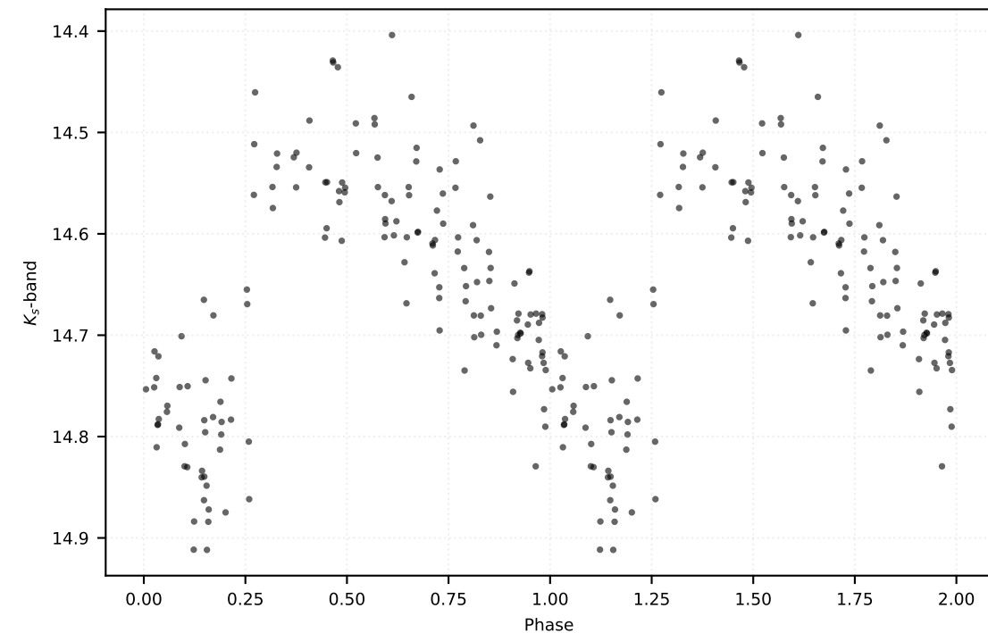
P: 0.44704 d | Class: RP | Subclass: RRab | Field b278
