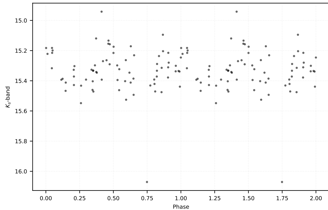
P: 0.63859 d | Class: EB | Subclass: EA | Field b279
