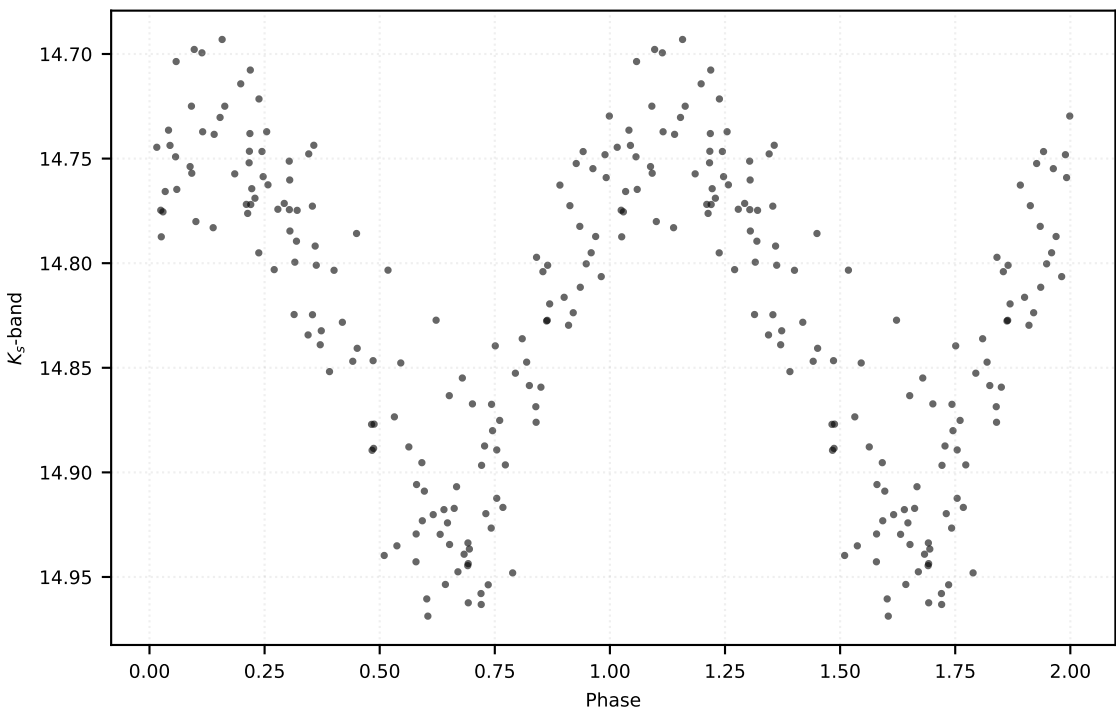
P: 0.20730 d | Class: RP | Subclass: RRc | Field b279
