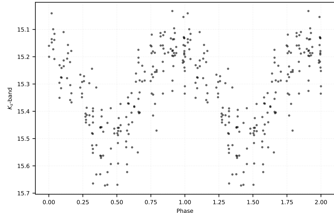
P: 0.34627 d | Class: RP | Subclass: CEP-10T | Field b278
