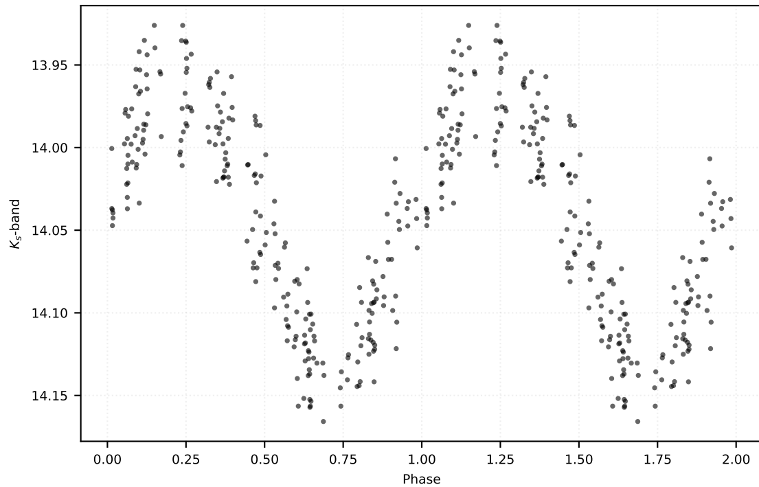
P: 0.19593 d | Class: RP | Subclass: UVAR | Field b278
