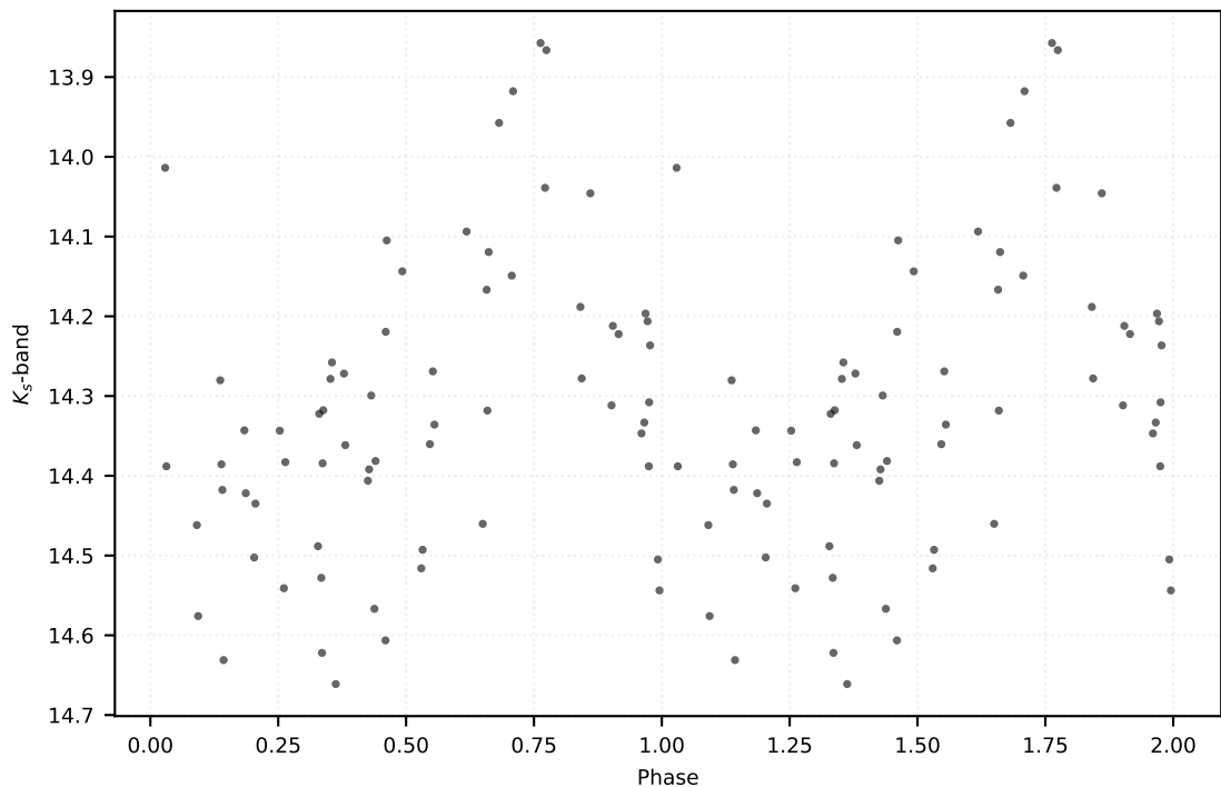
P: 0.49285 d | Class: RP | Subclass: CEP-10T | Field b279
