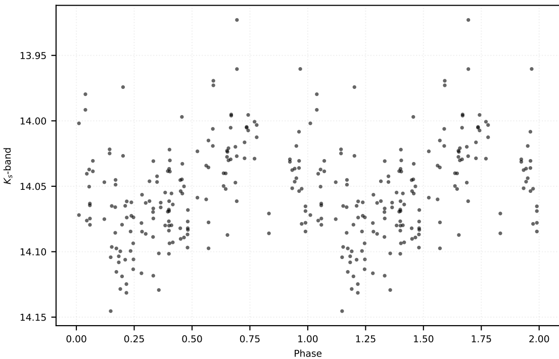
P: 1.59785 d | Class: RP | Subclass: CEP-F | Field b278
