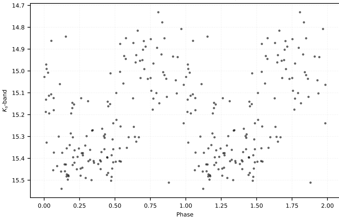
P: 0.16381 d | Class: RP | Subclass: UVAR | Field b279
