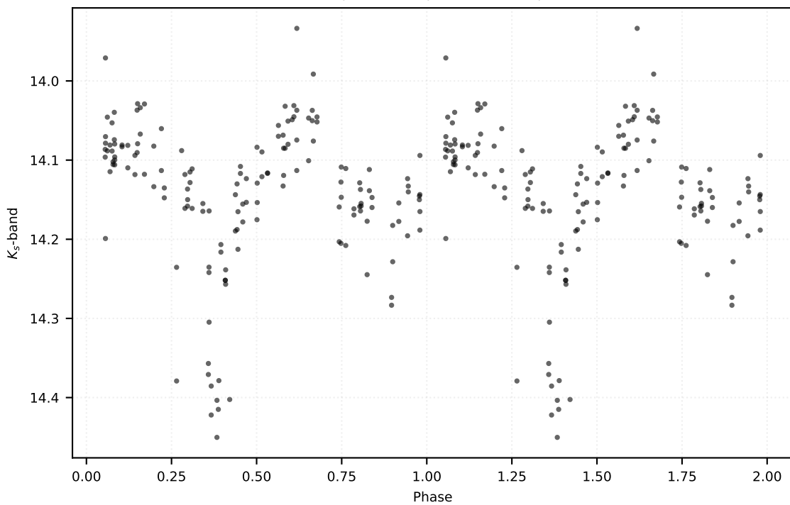
P: 0.47072 d | Class: EB | Subclass: EA | Field b279
