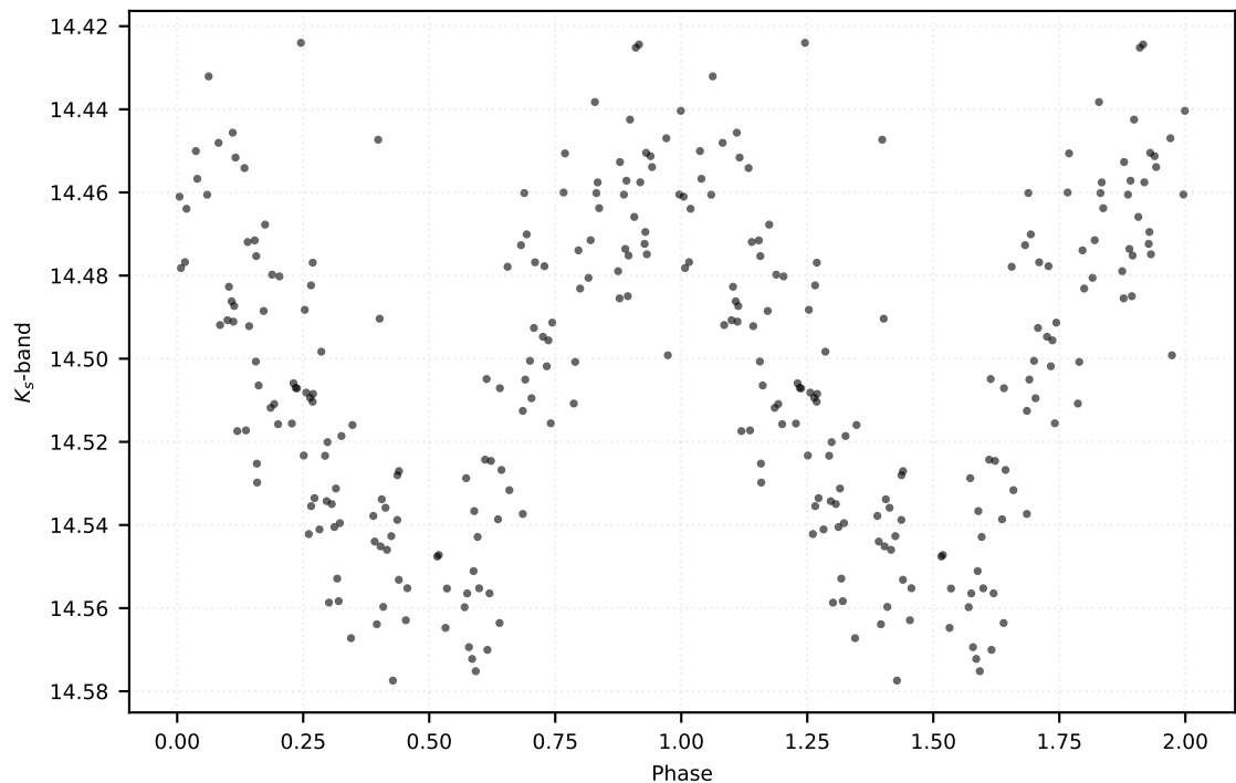
P: 0.15256 d | Class: RP | Subclass: UVAR | Field b279
