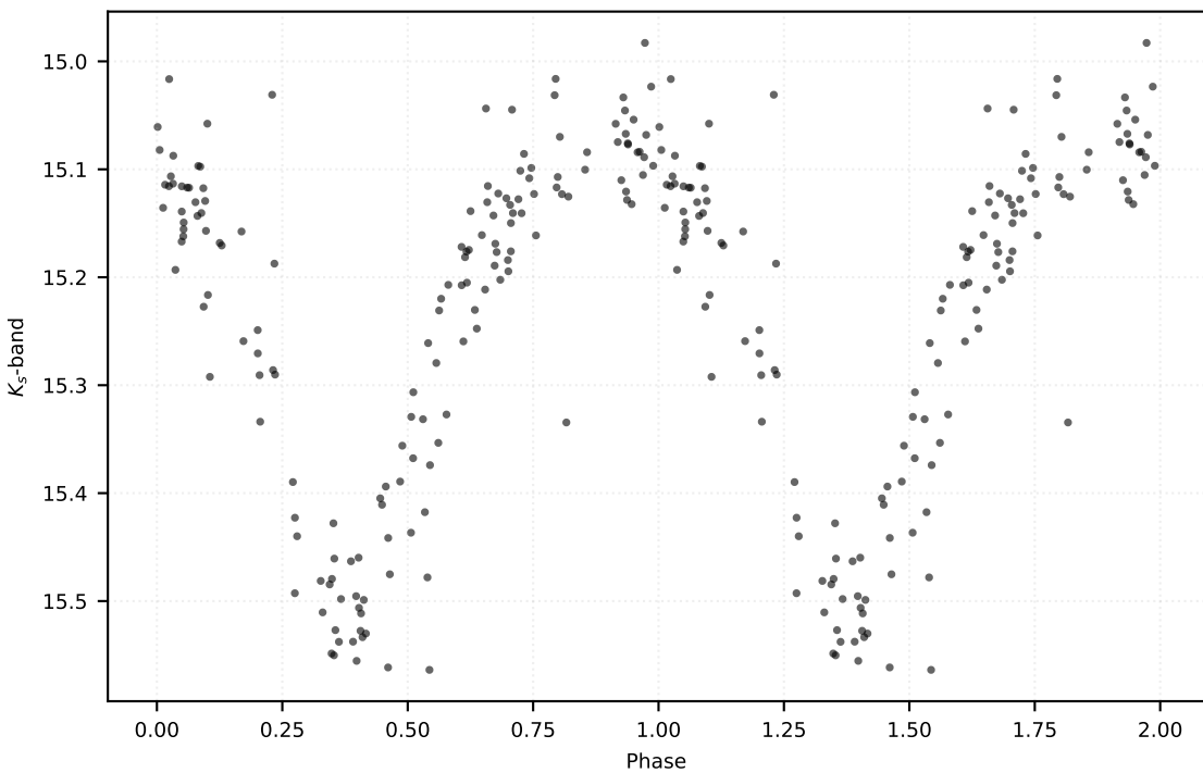
P: 0.19411 d | Class: RP | Subclass: UVAR | Field b279
