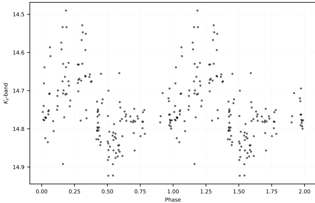
P: 0.20569 d | Class: RP | Subclass: UVAR | Field b278
