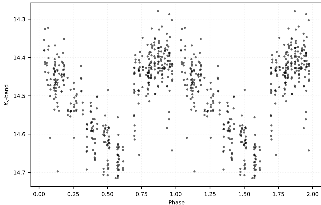
P: 0.39370 d | Class: RP | Subclass: RRab | Field b278
