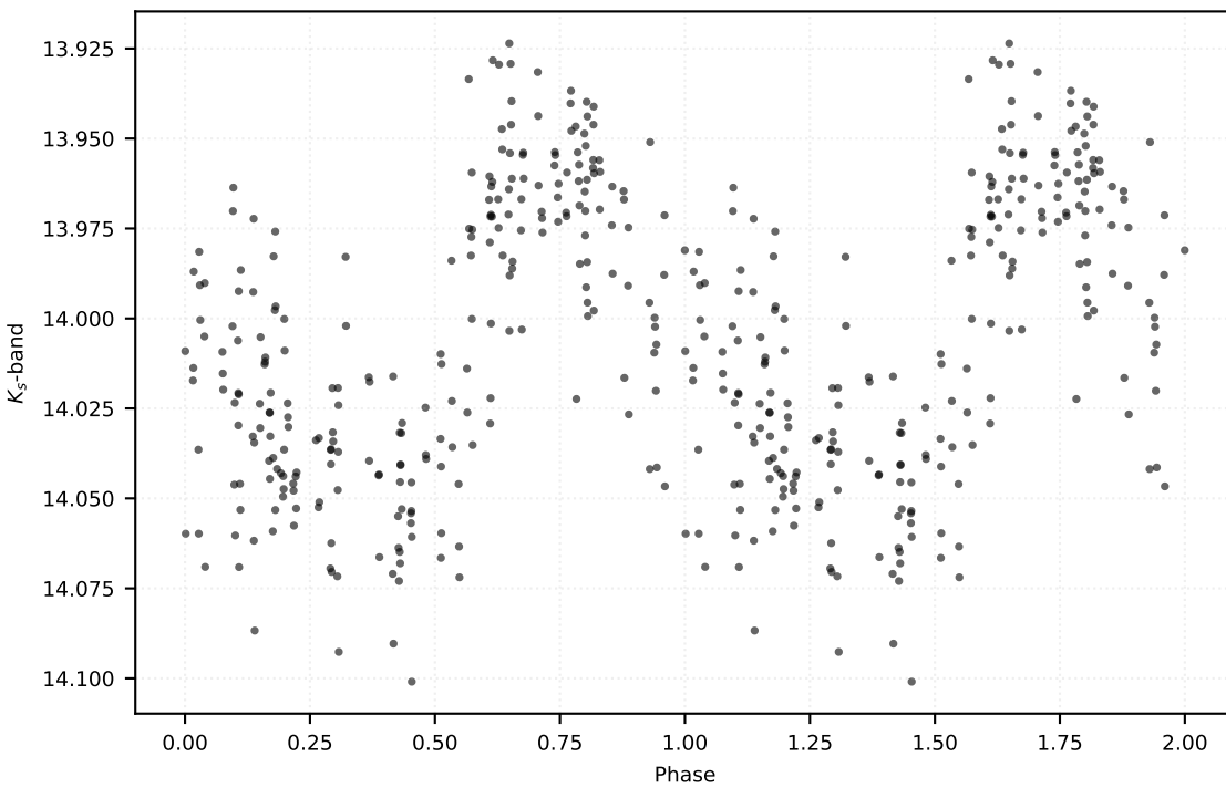
P: 0.38672 d | Class: RP | Subclass: RRab | Field b278
