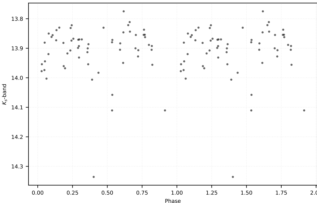
P: 0.59137 d | Class: EB | Subclass: EA | Field b279
