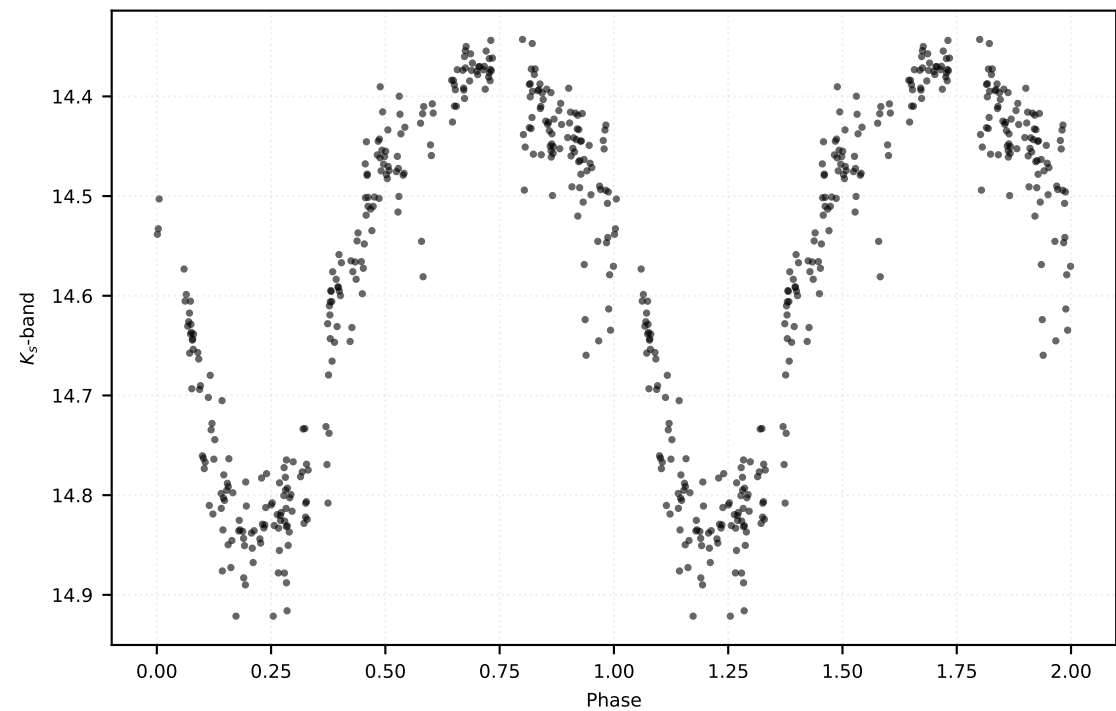
P: 0.17231 d | Class: RP | Subclass: UVAR | Field b279
