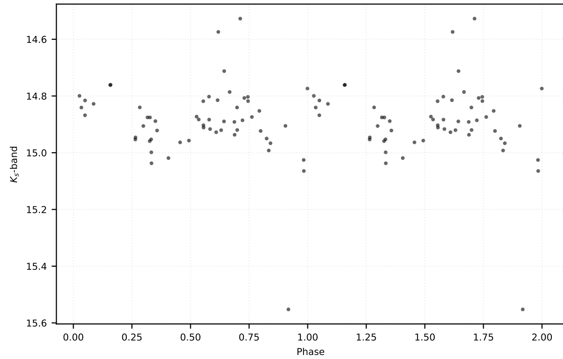
P: 0.56138 d | Class: EB | Subclass: EA | Field b278
