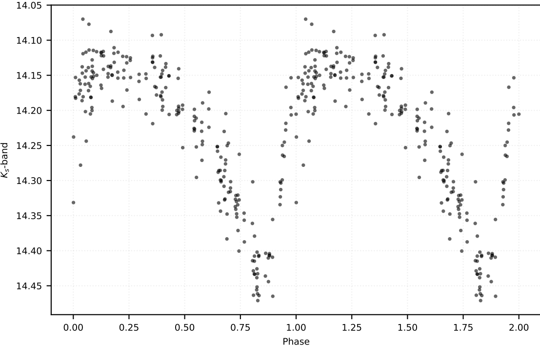
P: 0.48019 d | Class: RP | Subclass: RRab | Field b279
