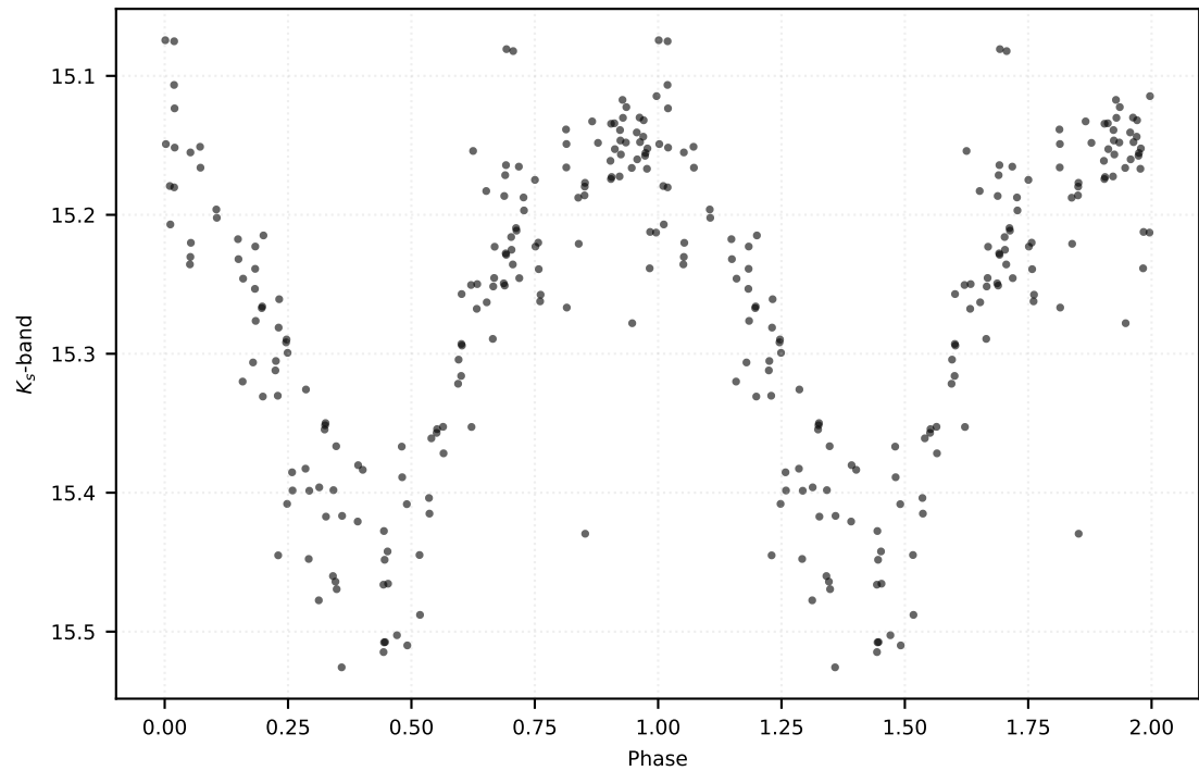
P: 0.37627 d | Class: RP | Subclass: RRab | Field b278
