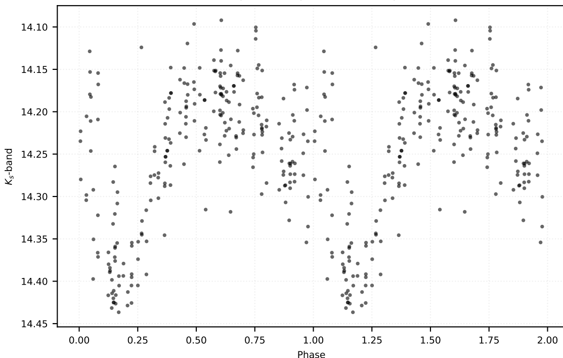
P: 0.33036 d | Class: RP | Subclass: RRab | Field b279
