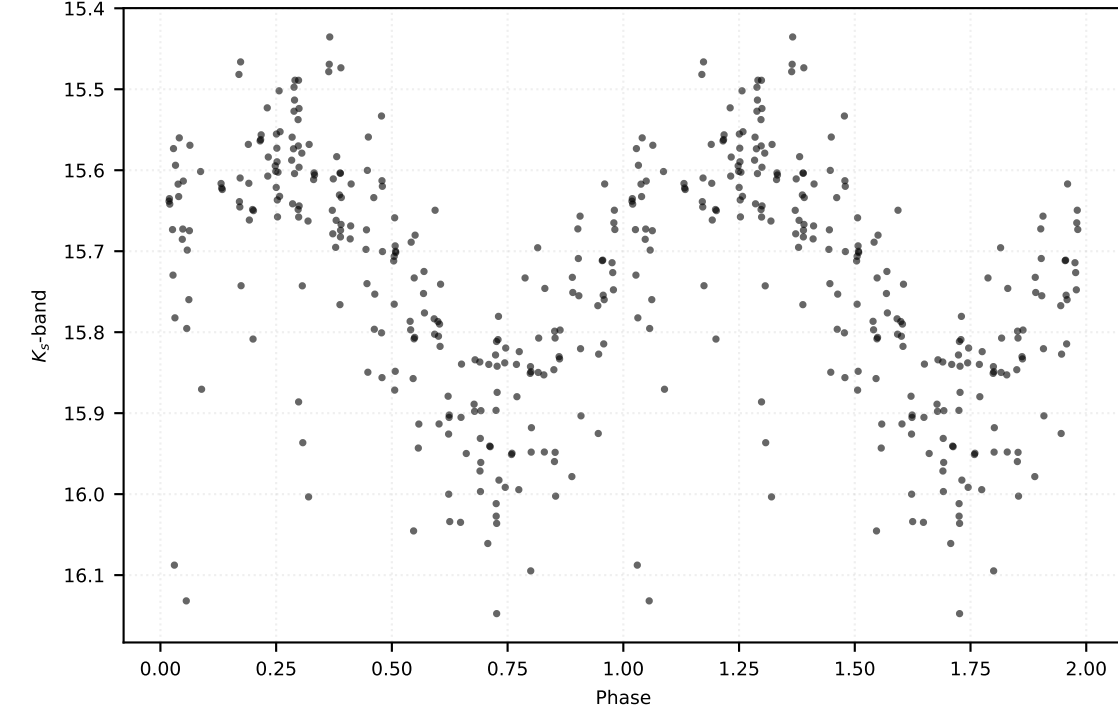
P: 0.38548 d | Class: RP | Subclass: CEP-10T | Field b279
