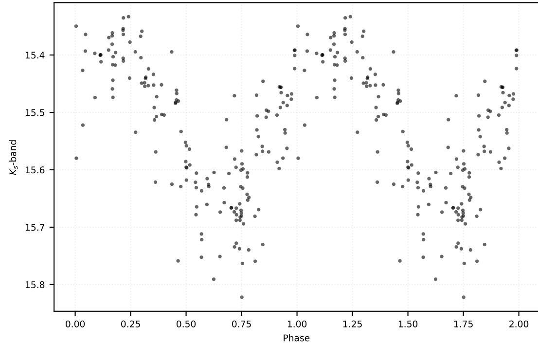
P: 0.53860 d | Class: RP | Subclass: RRab | Field b278
