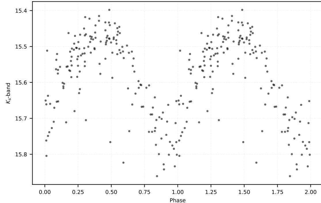
P: 0.41452 d | Class: RP | Subclass: RRab | Field b279
