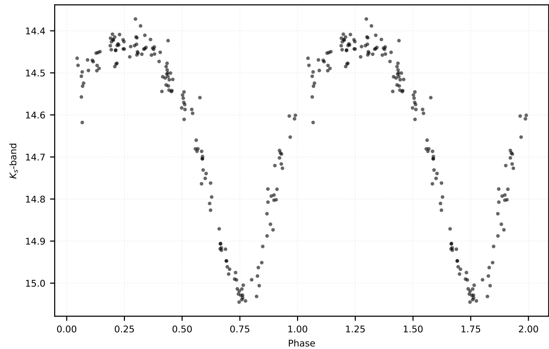
P: 0.49475 d | Class: RP | Subclass: RRc | Field b279
