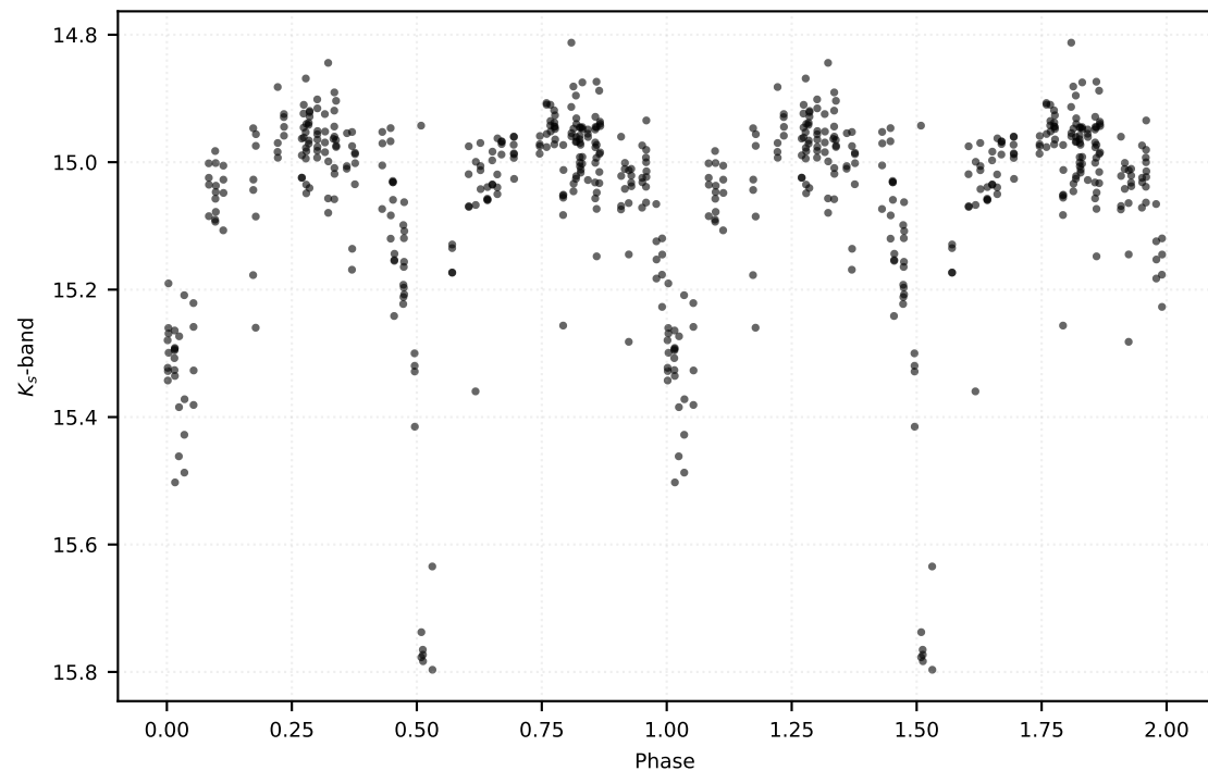
P: 0.83025 d | Class: EB | Subclass: EA | Field b279
