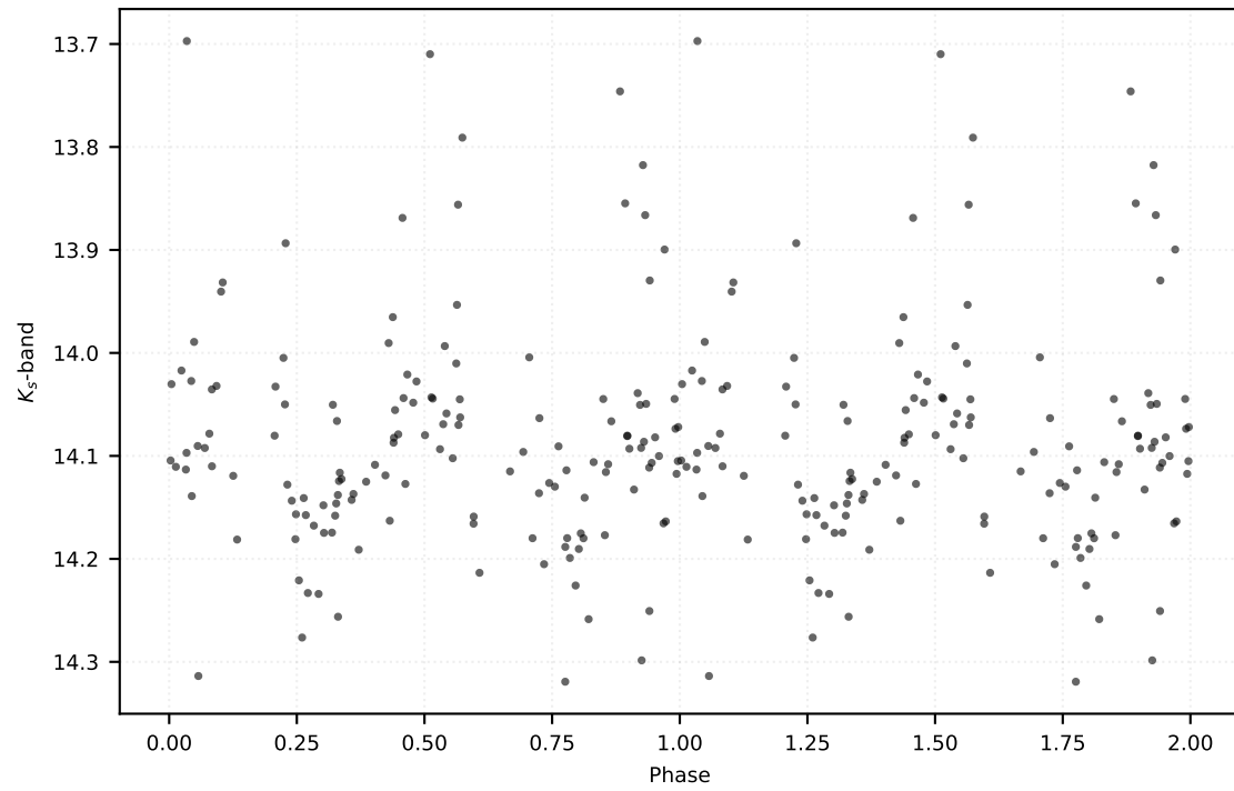
P: 0.39891 d | Class: EB | Subclass: EA | Field b278
