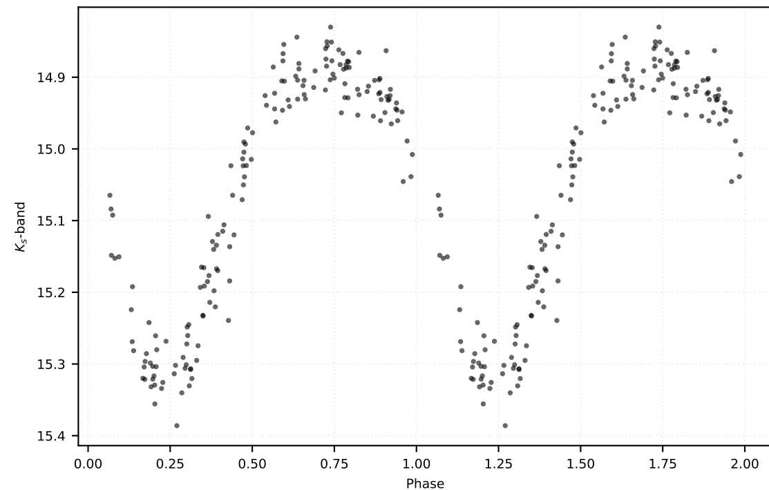
P: 0.14837 d | Class: RP | Subclass: UVAR | Field b278
