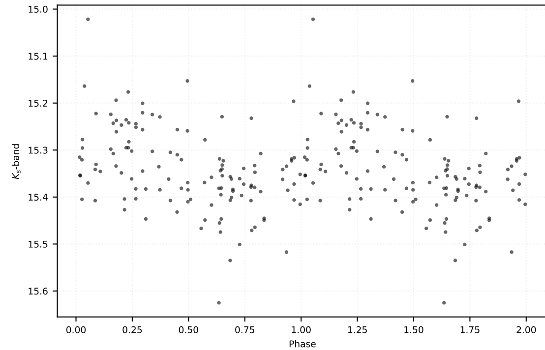
P: 1.36274 d | Class: RP | Subclass: CEP-F | Field b278
