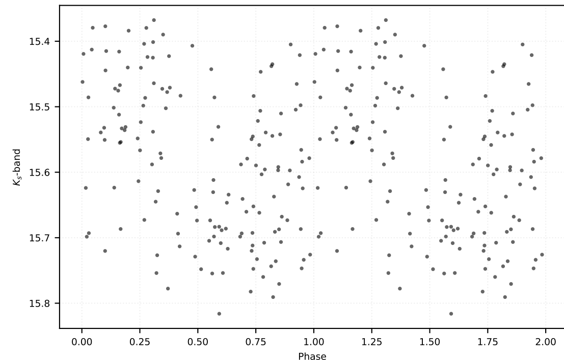
P: 60.88042 d | Class: RP | Subclass: UVAR | Field b278
