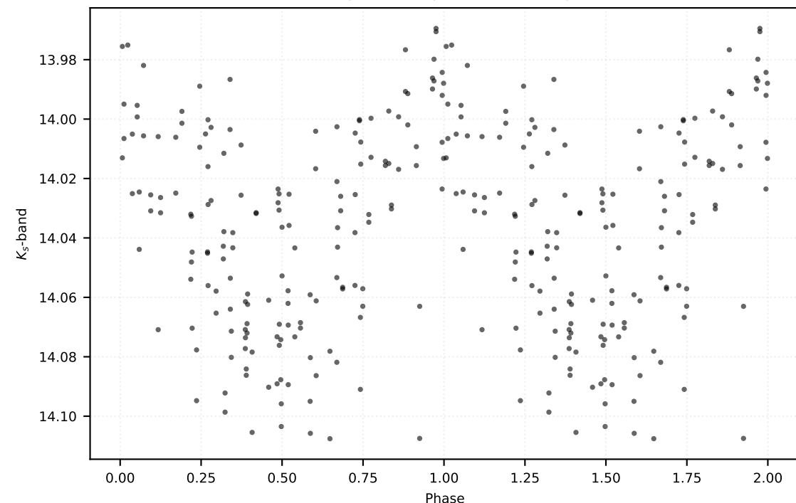
P: 20.82957 d | Class: RP | Subclass: UVAR | Field b279
