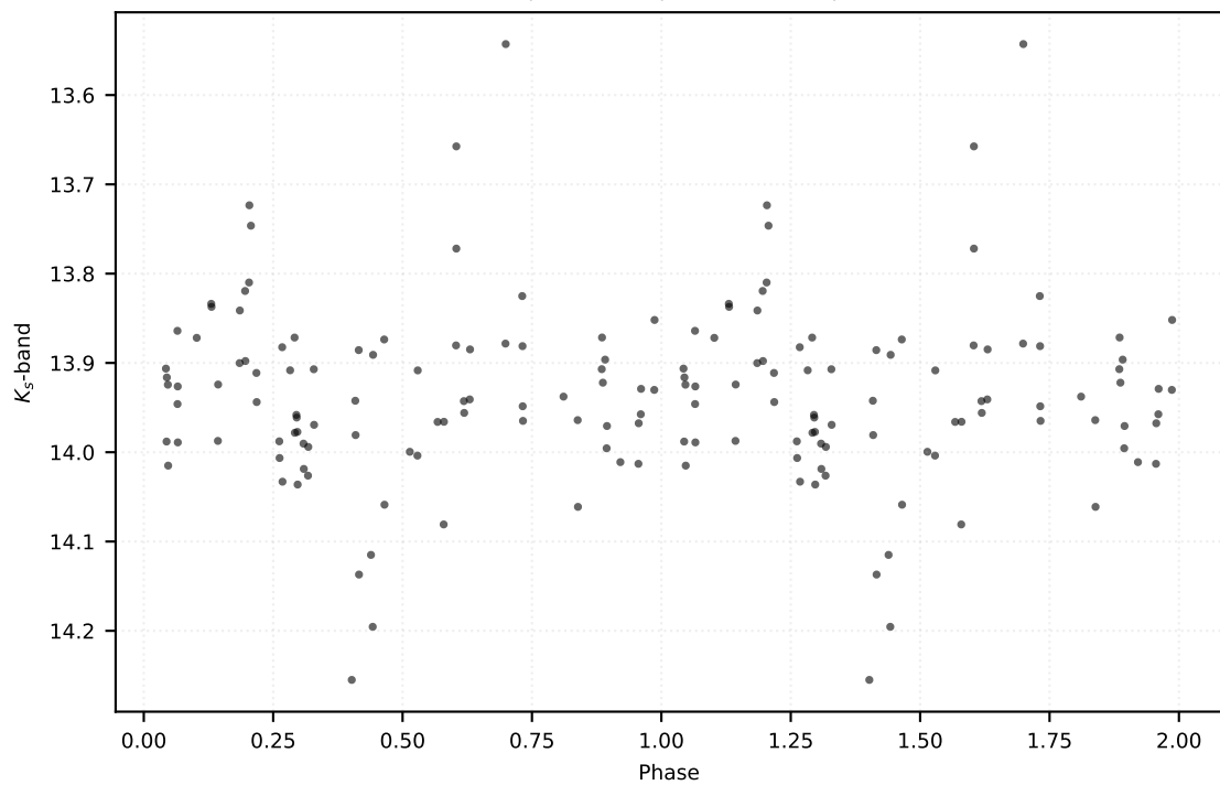
P: 0.39226 d | Class: EB | Subclass: EA | Field b279
