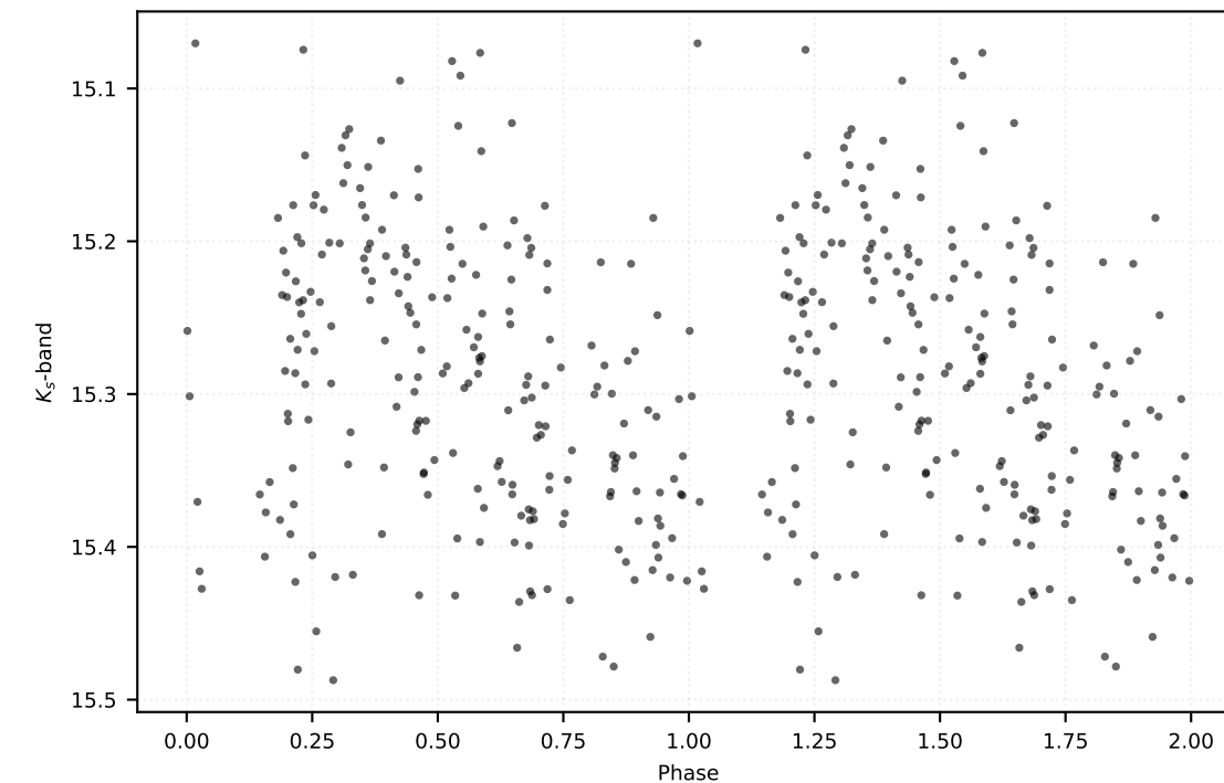
P: 0.12141 d | Class: RP | Subclass: UVAR | Field b279
