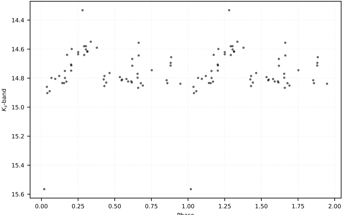
P: 0.87847 d | Class: EB | Subclass: EA | Field b278
