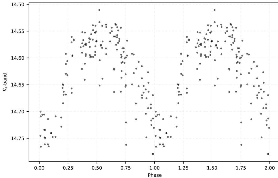
P: 1.08846 d | Class: EB | Subclass: RRc | Field b278
