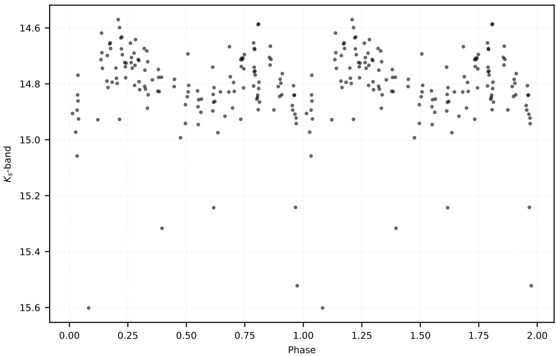
P: 3.31189 d | Class: EB | Subclass: EA | Field b278
