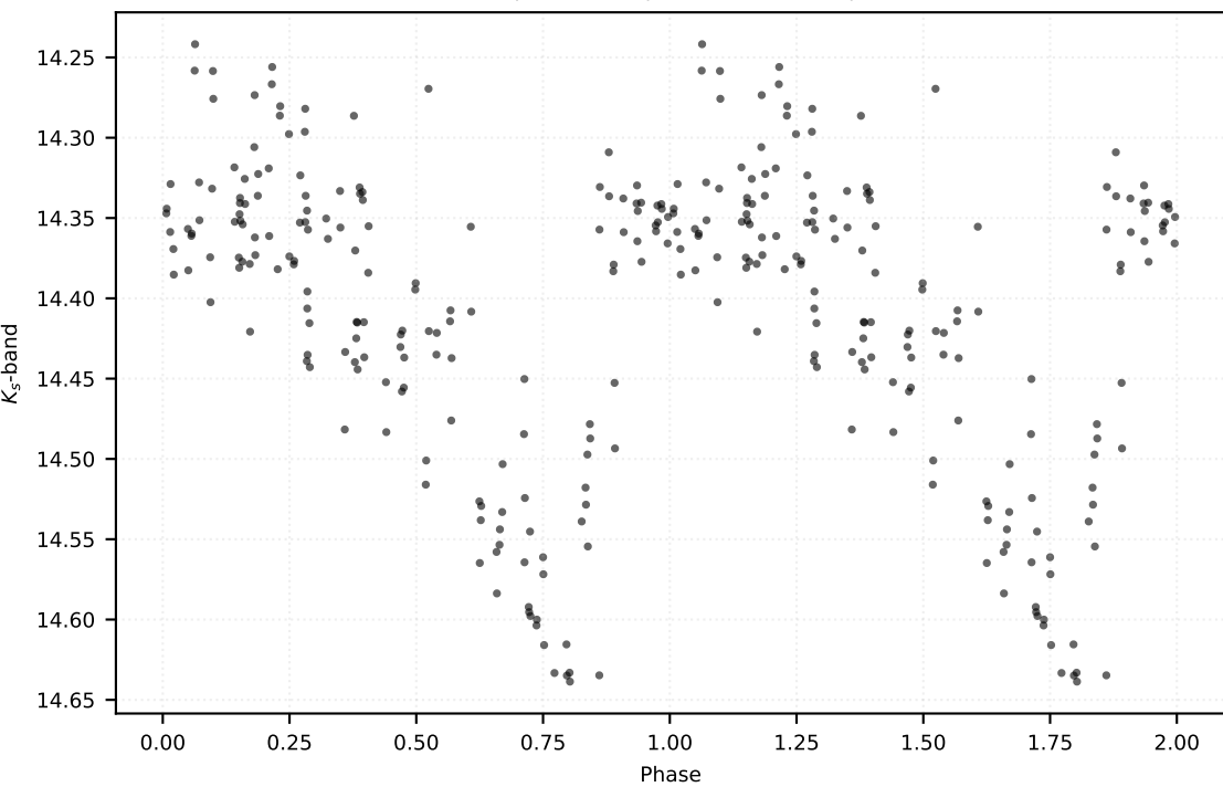
P: 0.33242 d | Class: RP | Subclass: RRab | Field b278
