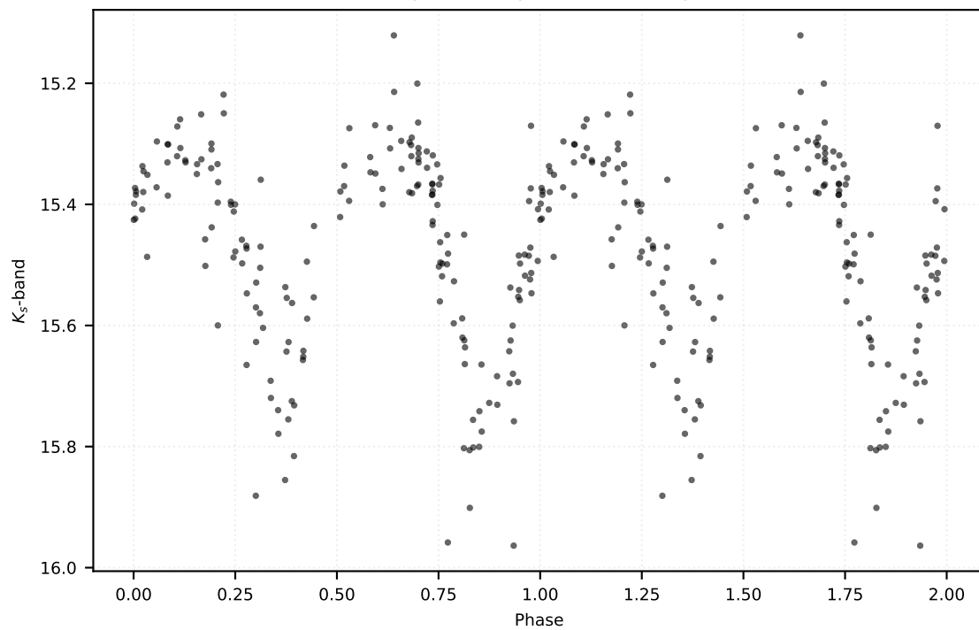
P: 0.21959 d | Class: RP | Subclass: UVAR | Field b279
