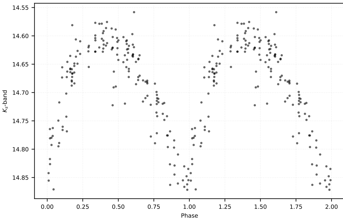
P: 1.11852 d | Class: RP | Subclass: CEP-10T | Field b279
