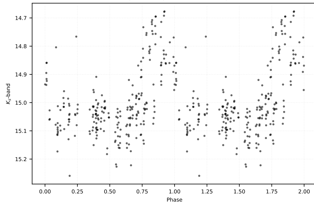
P: 0.54920 d | Class: RP | Subclass: CEP-10T | Field b278
