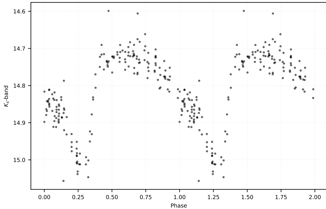
P: 0.49582 d | Class: RP | Subclass: RRab | Field b278
