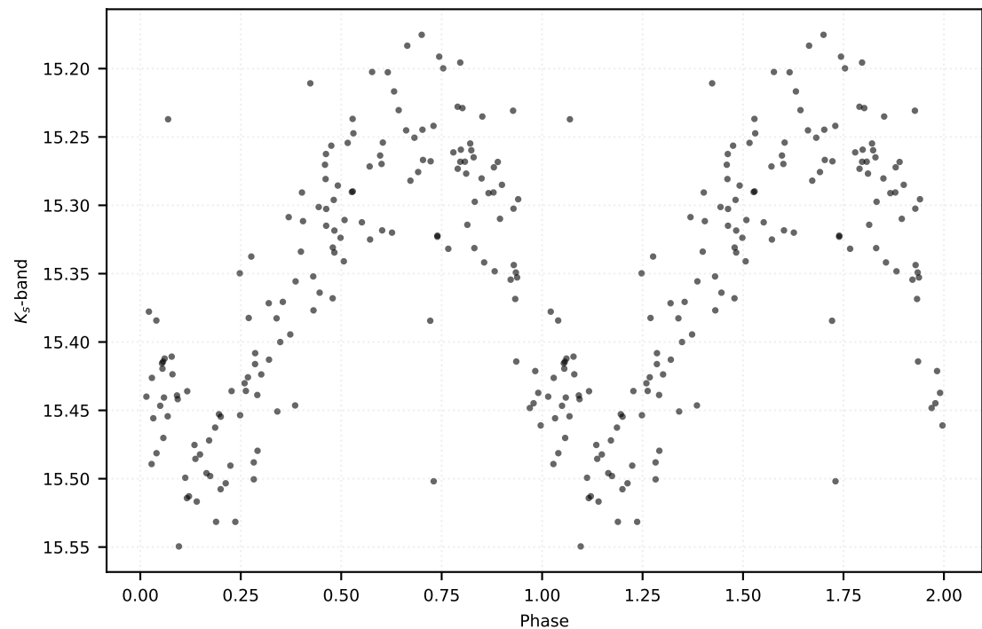
P: 1.60841 d | Class: RP | Subclass: CEP-10T | Field b279
