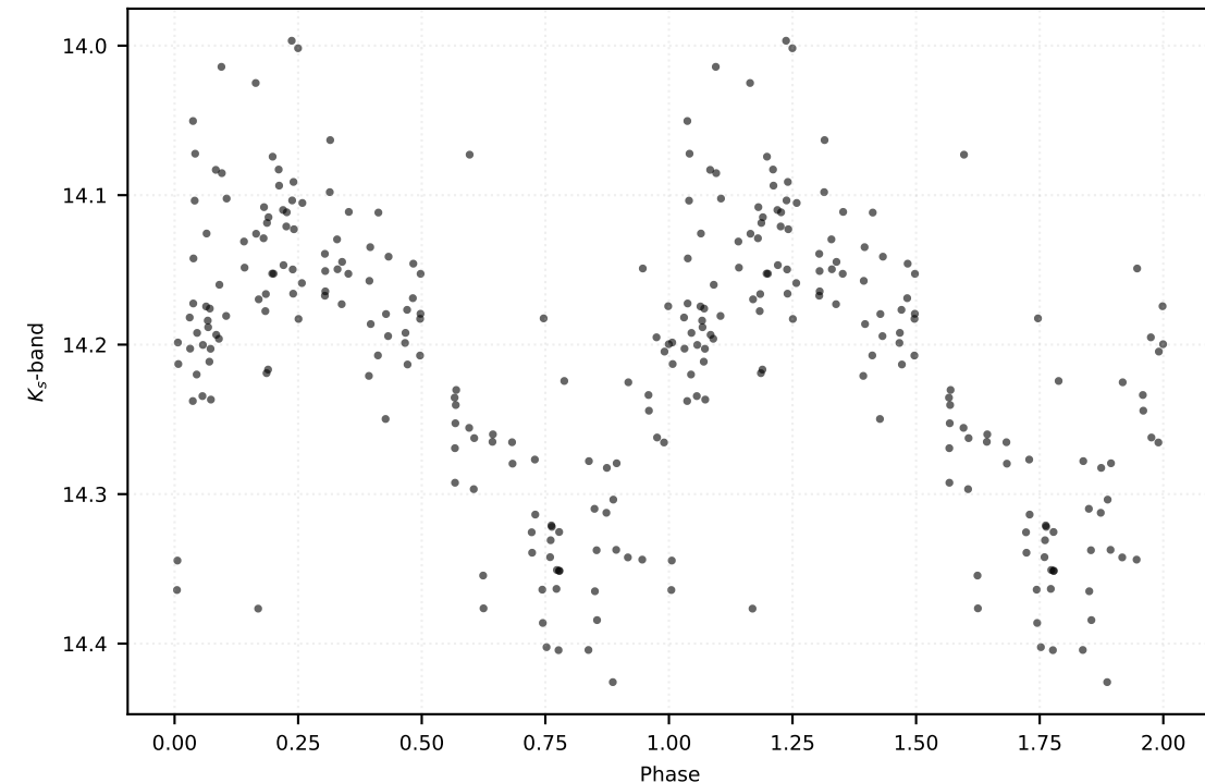
P: 0.31749 d | Class: RP | Subclass: RRab | Field b279
