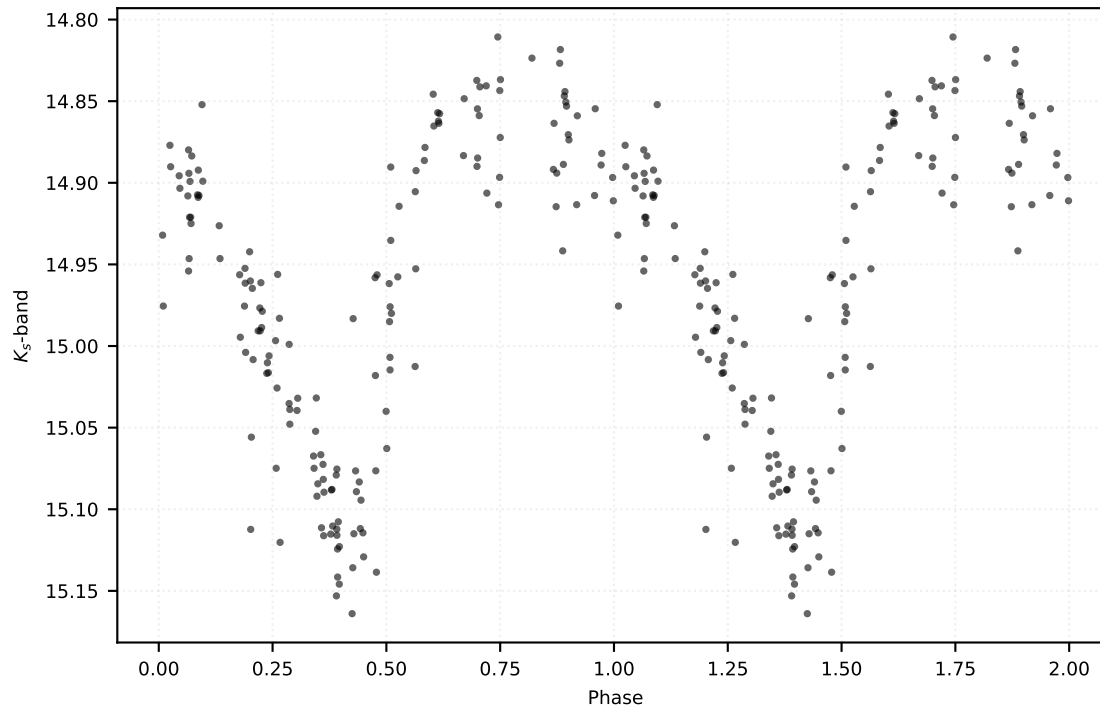
P: 0.44103 d | Class: RP | Subclass: RRc | Field b279
