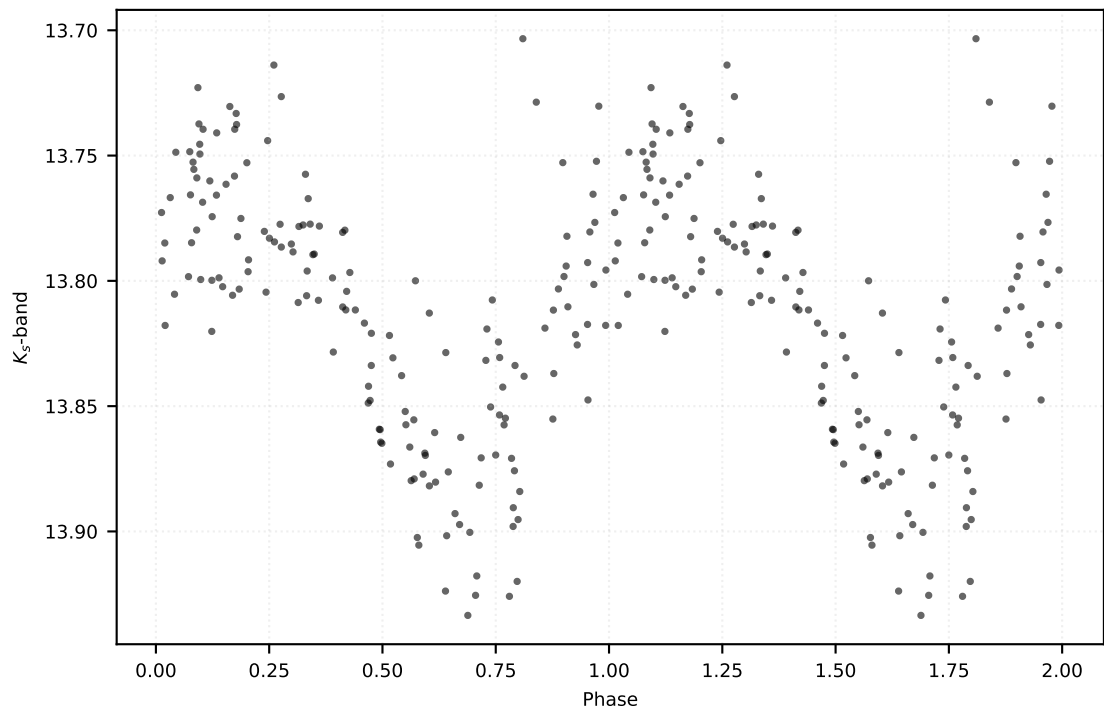
P: 0.81604 d | Class: RP | Subclass: CEP-10T | Field b279
