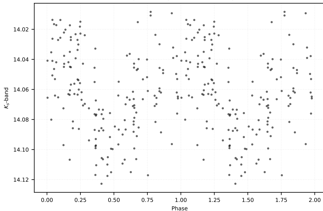
P: 0.27206 d | Class: RP | Subclass: CEP-1OT | Field b279
