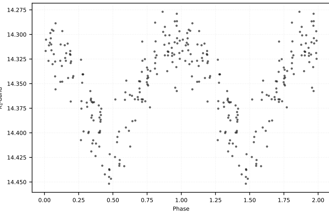
P: 0.13063 d | Class: RP | Subclass: UVAR | Field b278
