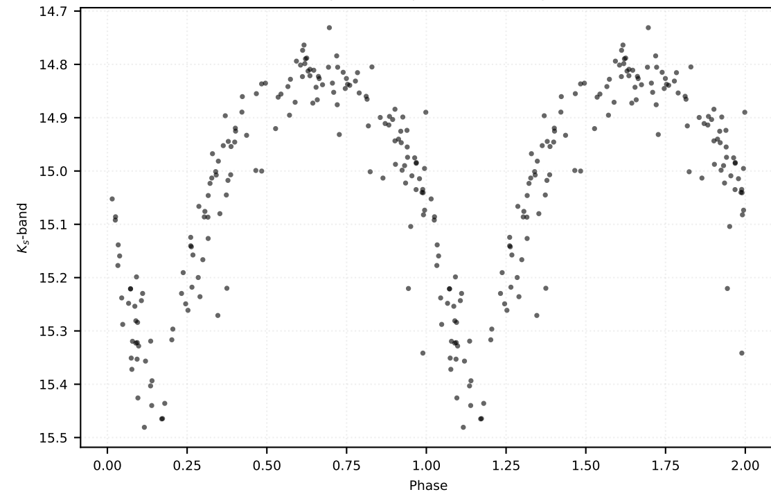
P: 0.17531 d | Class: RP | Subclass: UVAR | Field b278
