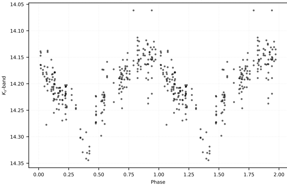
P: 1.58175 d | Class: RP | Subclass: CEP-F | Field b278
