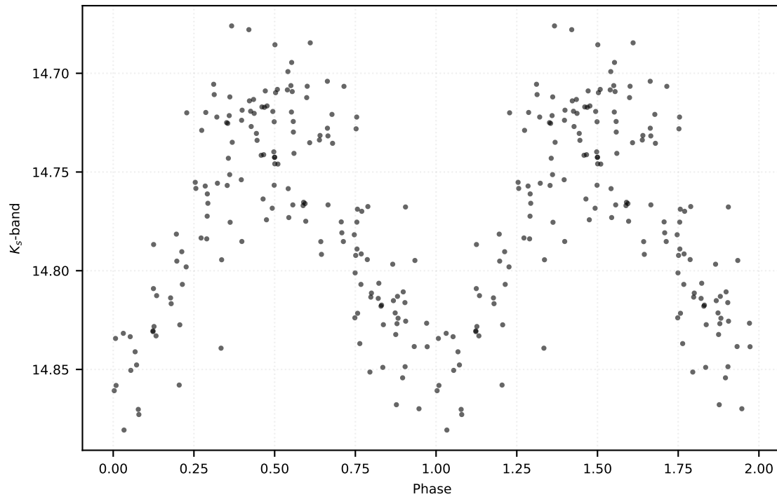
P: 0.44347 d | Class: RP | Subclass: CEP-1OT | Field b279
