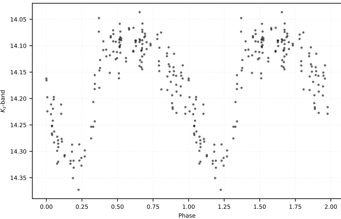
P: 0.53070 d | Class: RP | Subclass: RRab | Field b279
