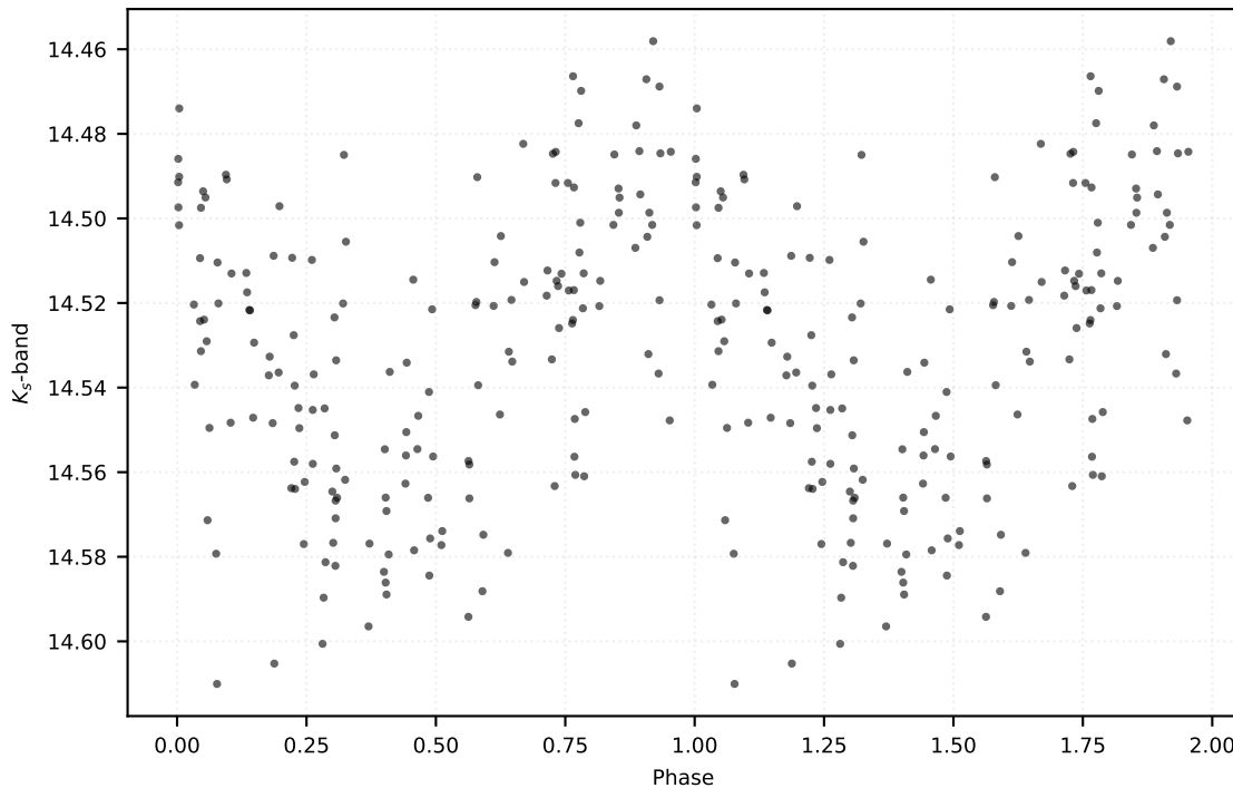
P: 0.23582 d | Class: RP | Subclass: UVAR | Field b278
