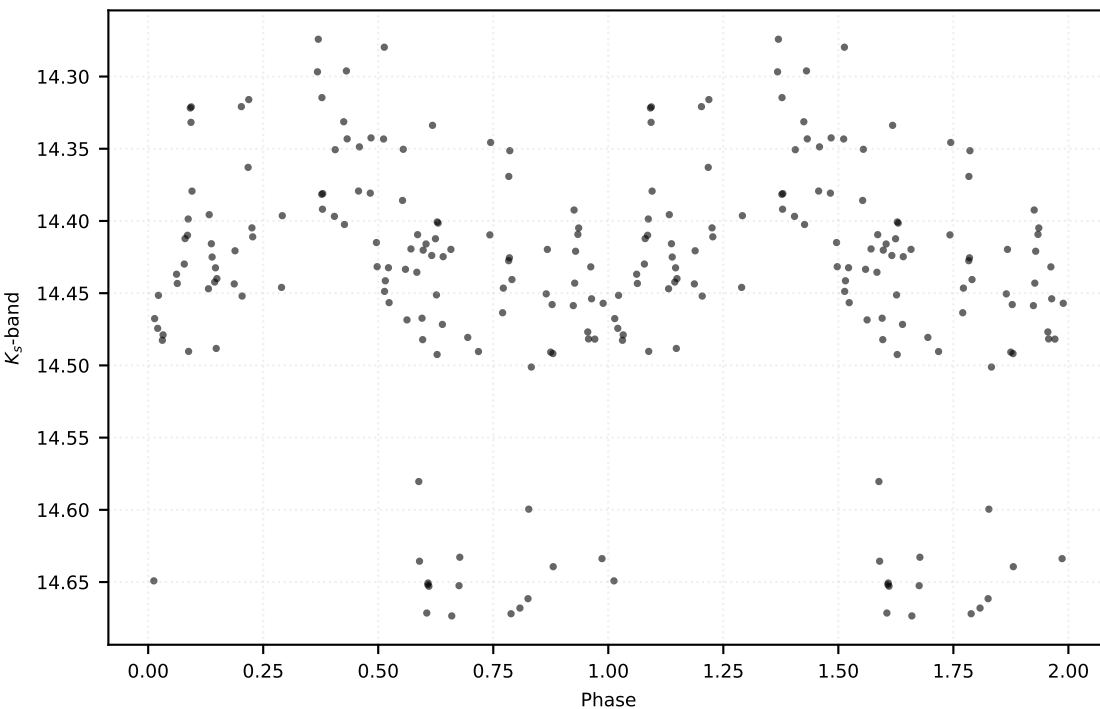
P: 0.88293 d | Class: RP | Subclass: CEP-10T | Field b278
