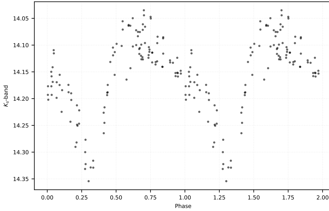
P: 0.31963 d | Class: RP | Subclass: RRab | Field b278
