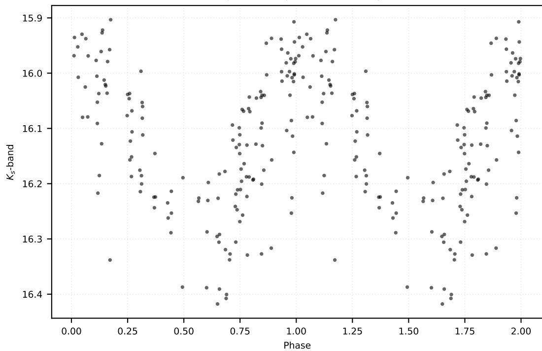
P: 0.10231 d | Class: RP | Subclass: UVAR | Field b279
