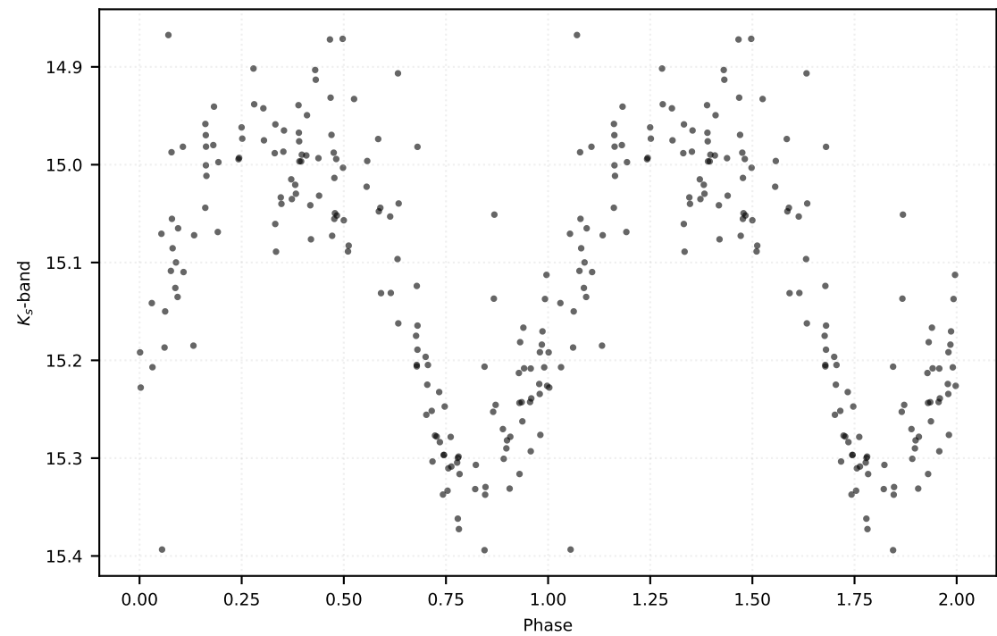
P: 0.52006 d | Class: RP | Subclass: RRc | Field b279
