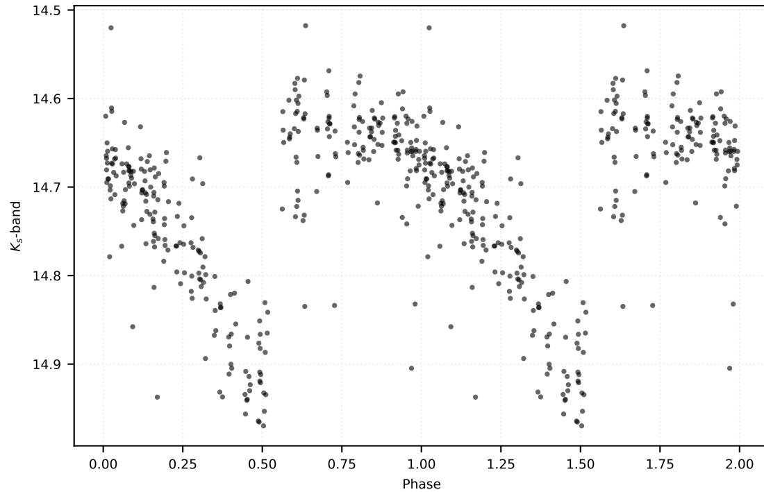
P: 0.48553 d | Class: RP | Subclass: RRab | Field b279
