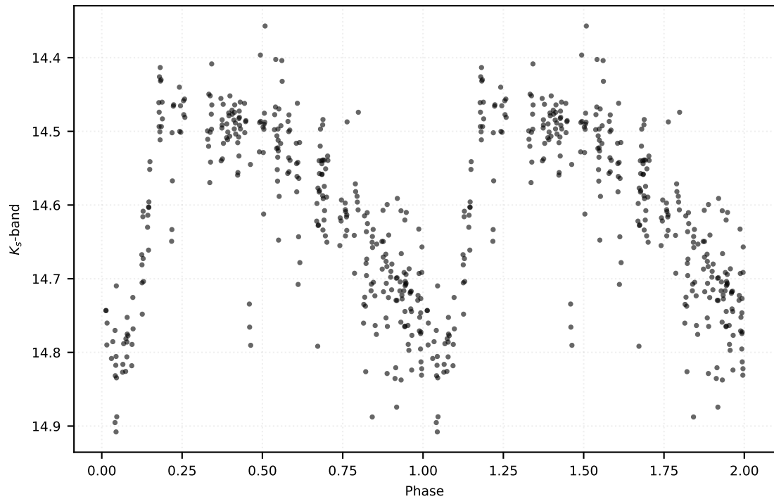
P: 0.46258 d | Class: RP | Subclass: RRab | Field b279
