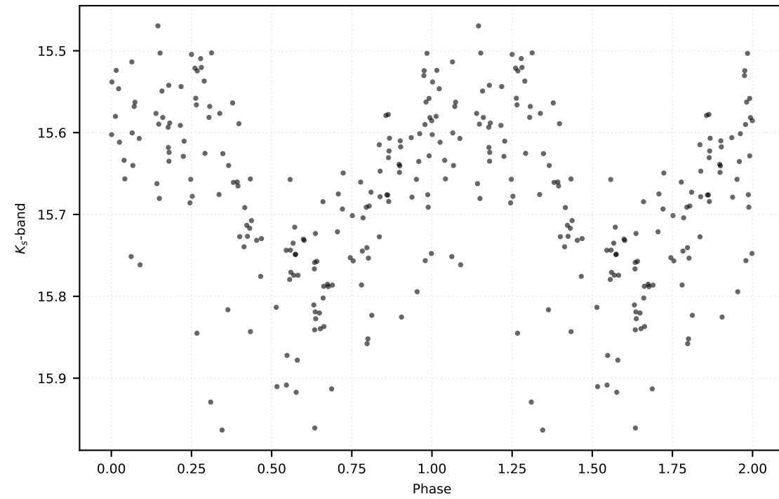
P: 0.33606 d | Class: RP | Subclass: RRab | Field b278
