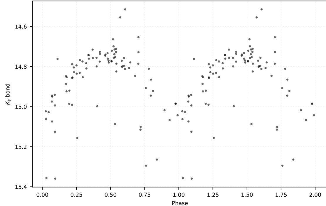
P: 0.55625 d | Class: RP | Subclass: CEP-1OT | Field b278
