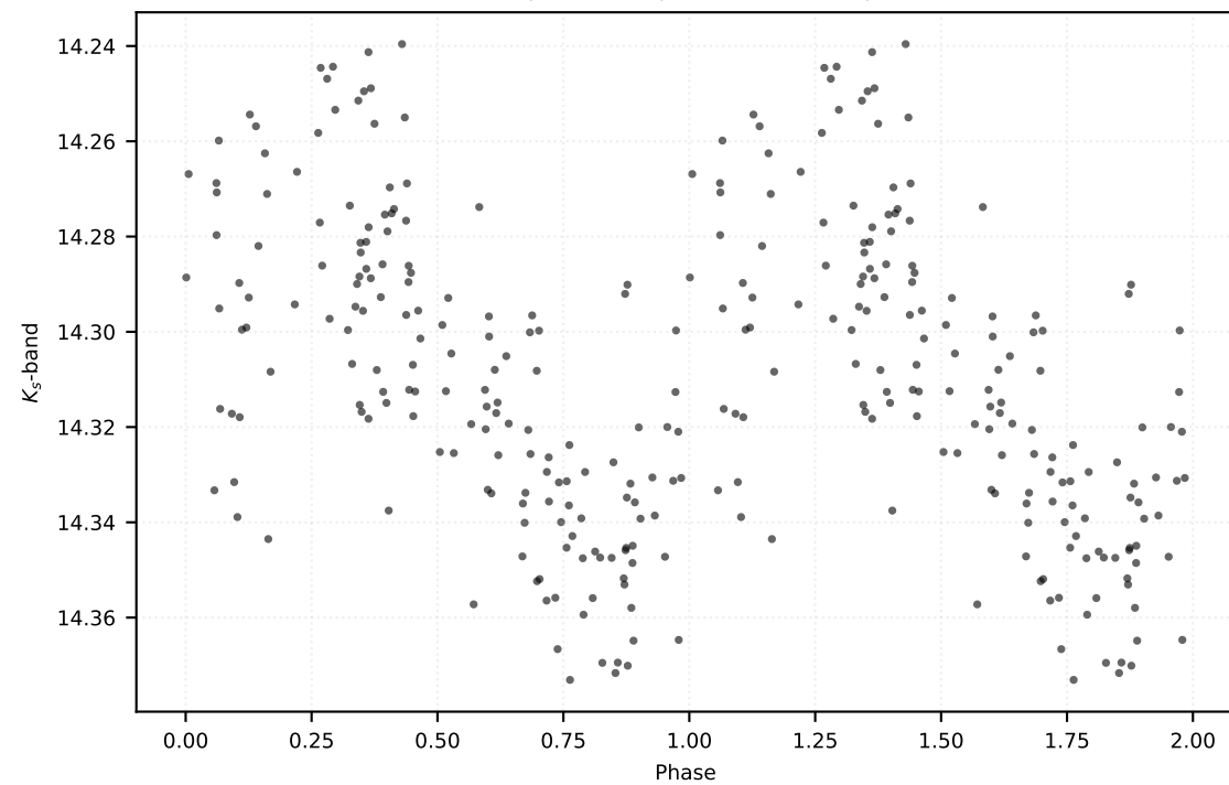
P: 0.12849 d | Class: RP | Subclass: UVAR | Field b278
