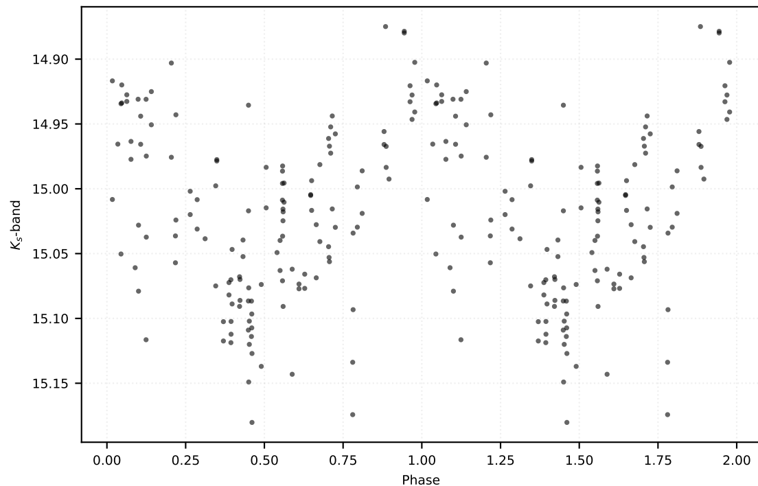
P: 1.00094 d | Class: RP | Subclass: CEP-F | Field b278
