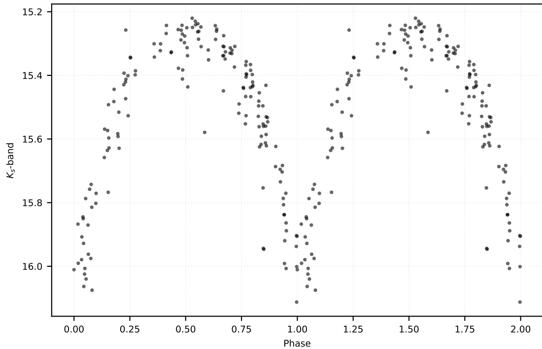
P: 0.25539 d | Class: RP | Subclass: RRc | Field b279
