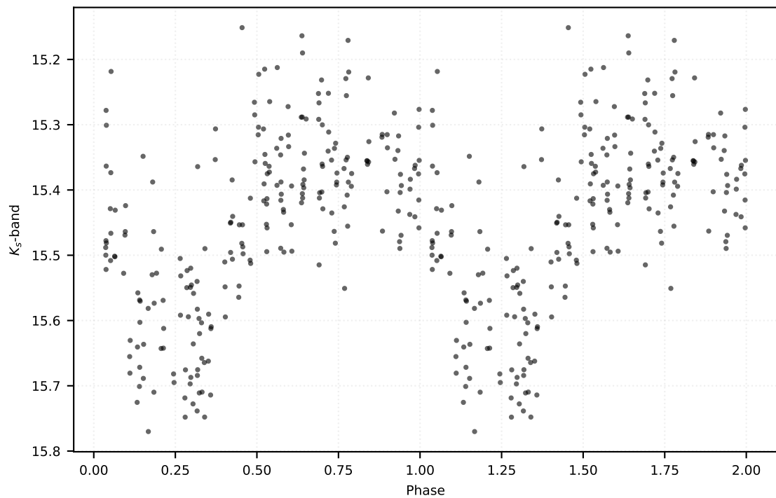
P: 0.39541 d | Class: RP | Subclass: R Rab | Field b278
