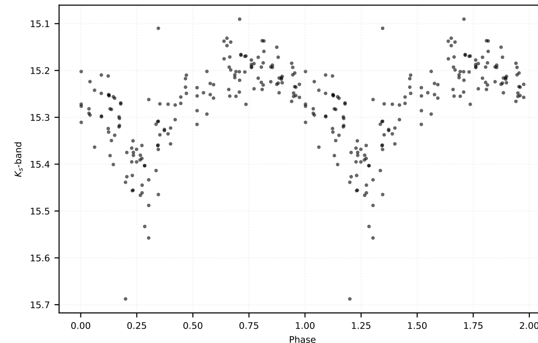
P: 3.36189 d | Class: RP | Subclass: CEP-10T | Field b279
