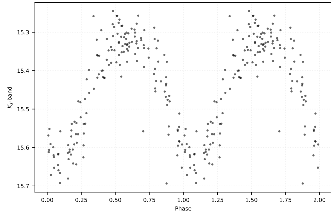
P: 0.16647 d | Class: RP | Subclass: UVAR | Field b278
