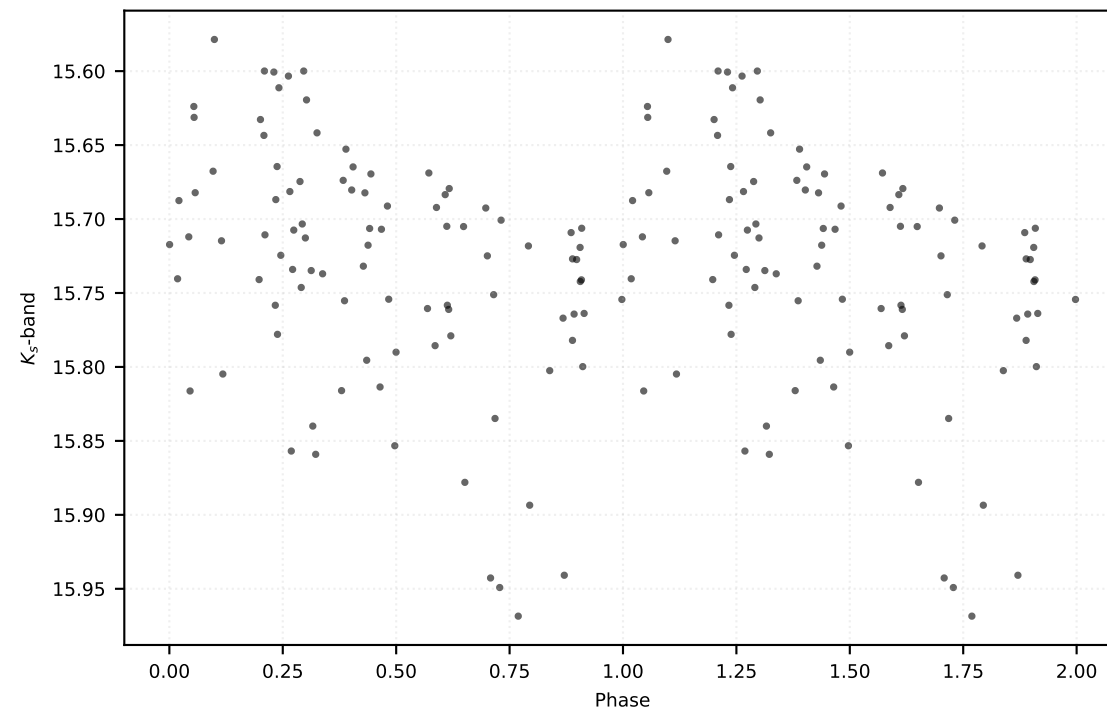
P: 0.19816 d | Class: RP | Subclass: UVAR | Field b279
