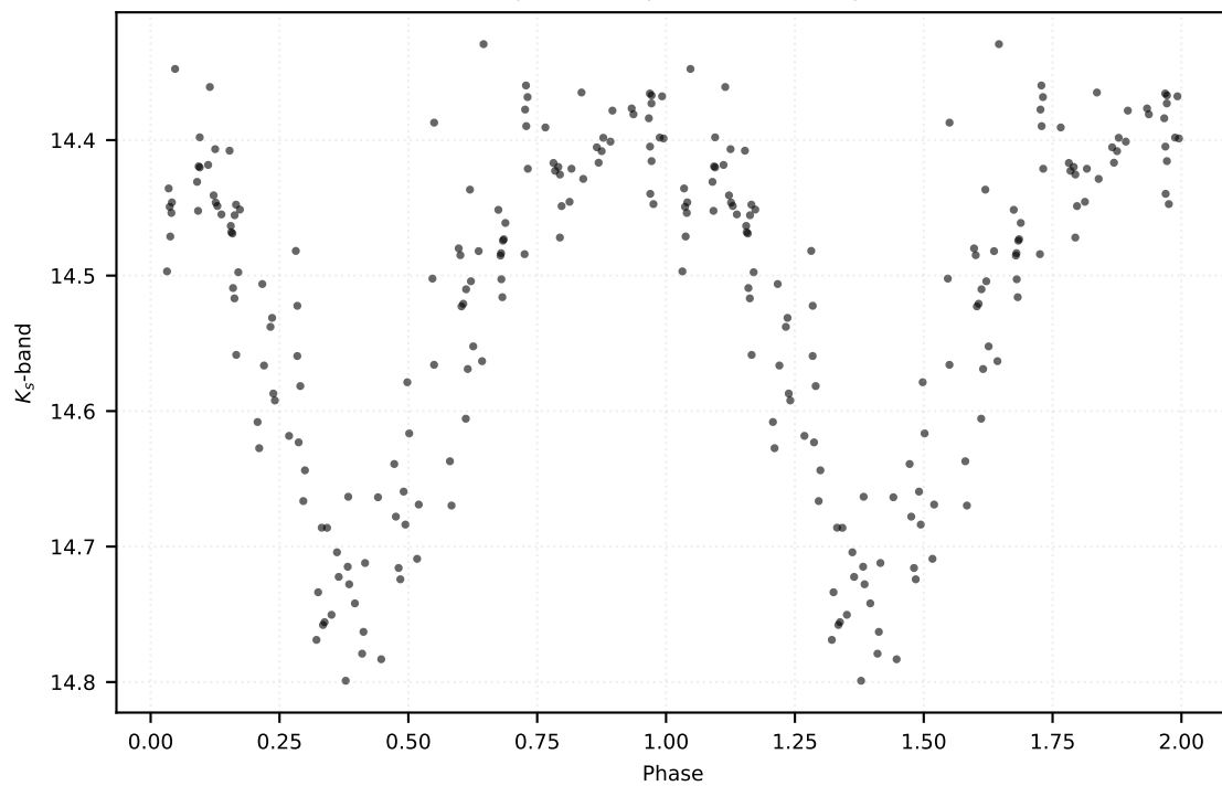
P: 1.03706 d | Class: EB | Subclass: UVAR | Field b279
