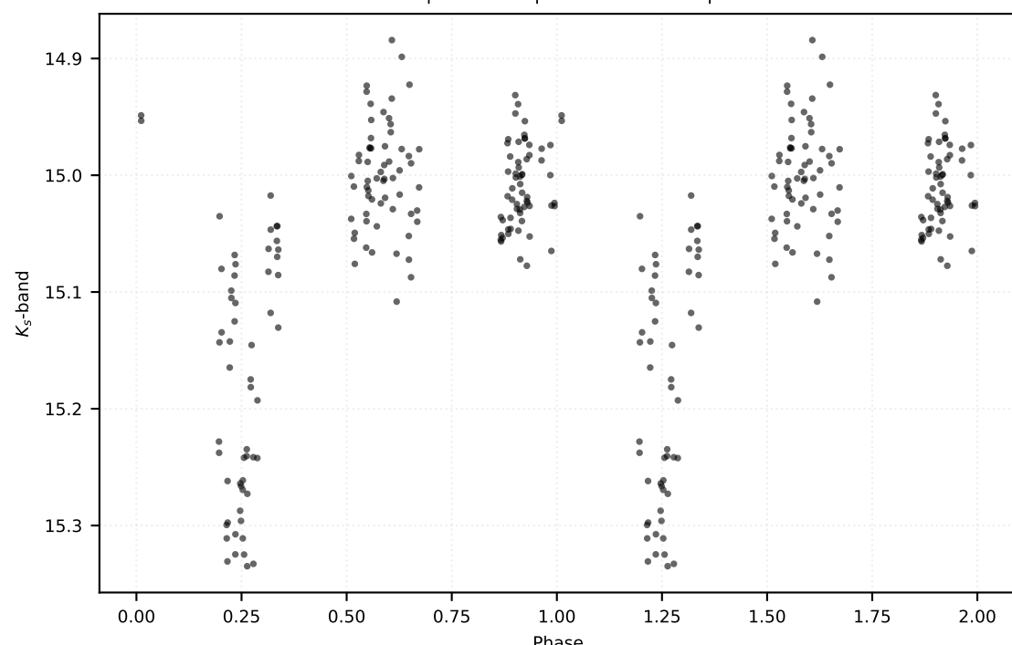
P: 3.00029 d | Class: RP | Subclass: CEP-F | Field b278
