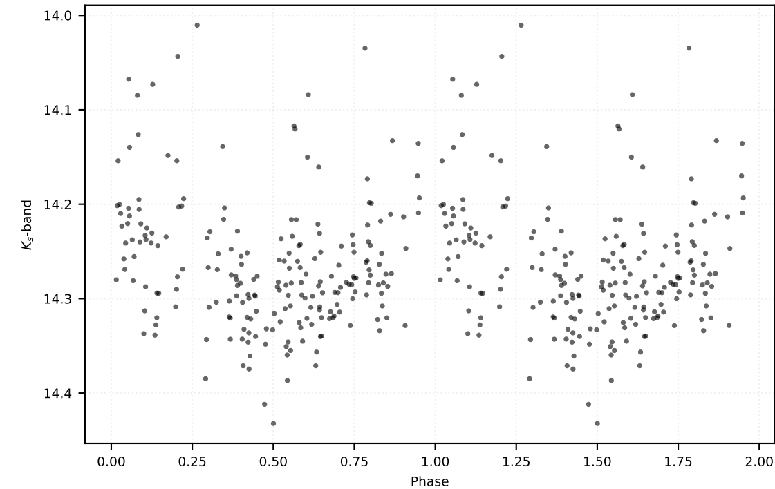
P: 0.14407 d | Class: RP | Subclass: UVAR | Field b278
