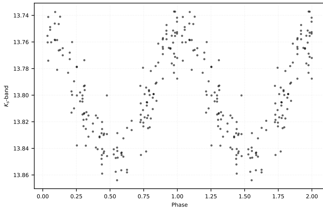
P: 0.48791 d | Class: RP | Subclass: CEP-1OT | Field b279
