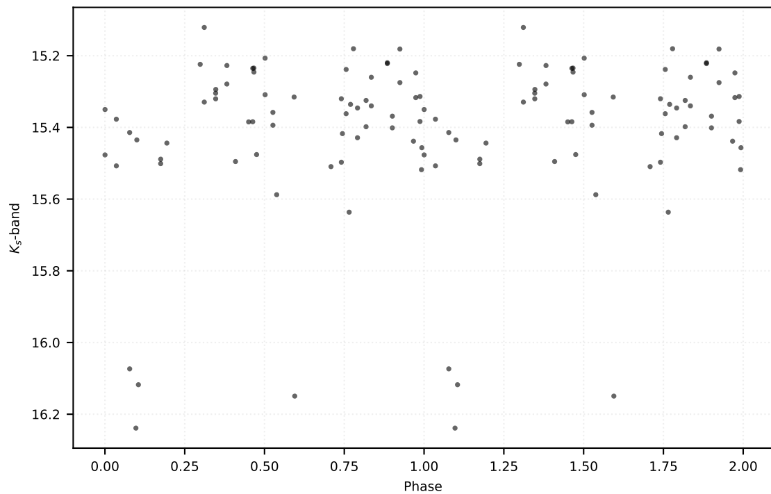
P: 0.28596 d | Class: EB | Subclass: EA | Field b278
