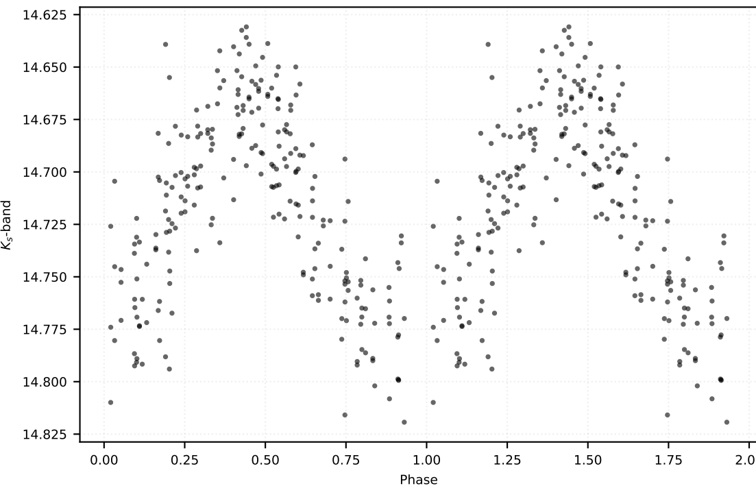
P: 26.72649 d | Class: RP | Subclass: CEP-F | Field b278
