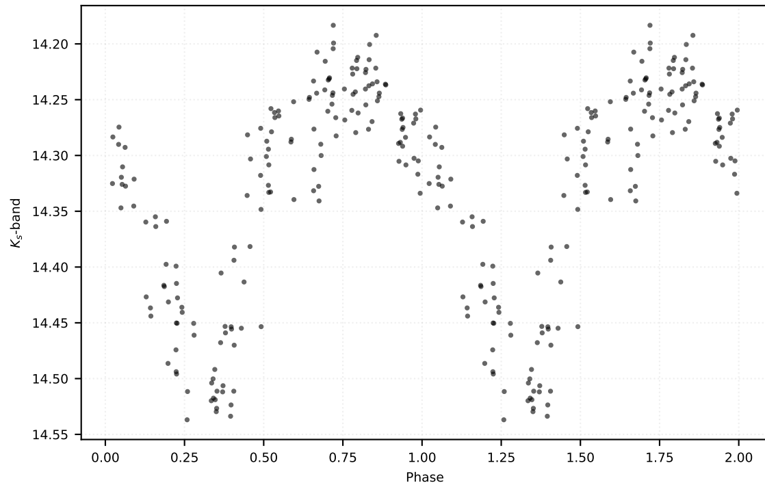
P: 2.63884 d | Class: RP | Subclass: CEP-1OT | Field b278
