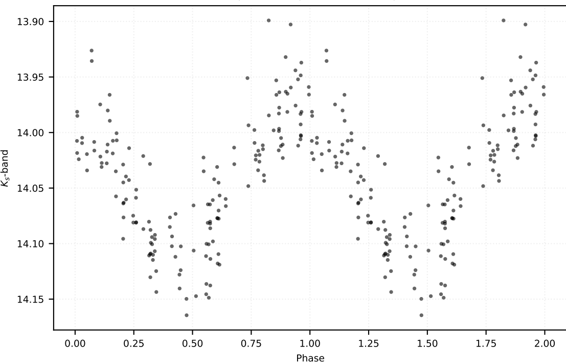
P: 0.33353 d | Class: RP | Subclass: RRab | Field b279
