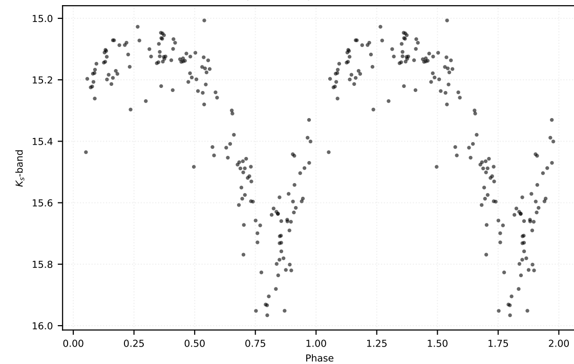
P: 0.19336 d | Class: RP | Subclass: UVAR | Field b279
