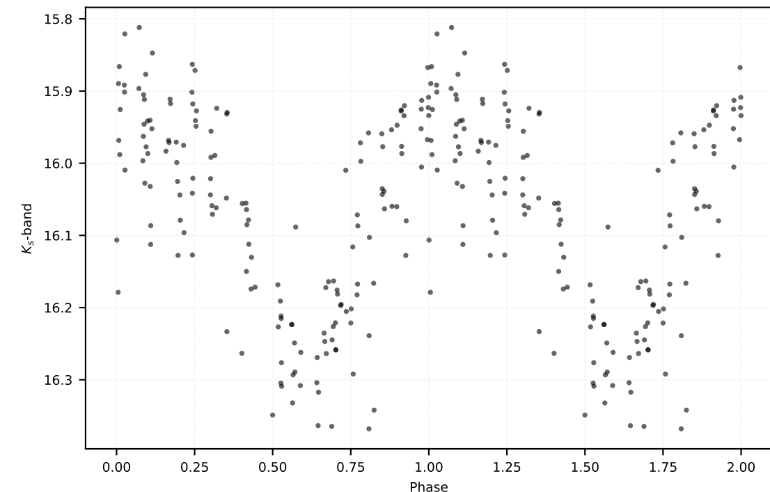
P: 0.45760 d | Class: RP | Subclass: CEP-10T | Field b279
