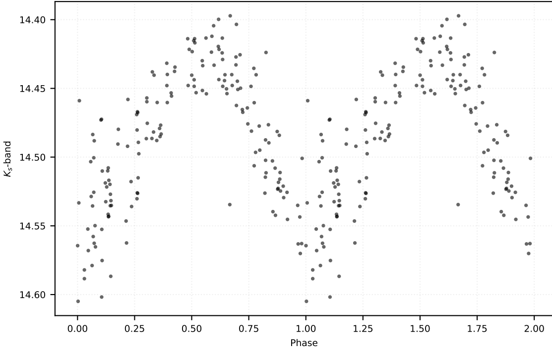
P: 0.20448 d | Class: RP | Subclass: RRc | Field b278
