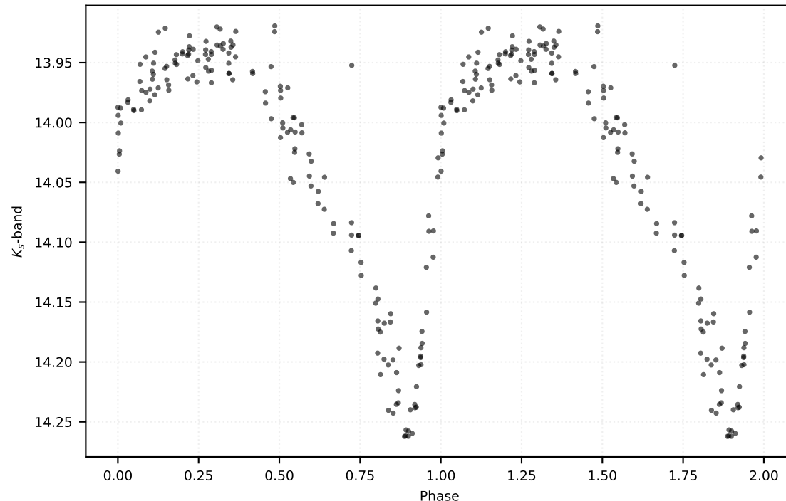
P: 0.59479 d | Class: RP | Subclass: RRab | Field b278
