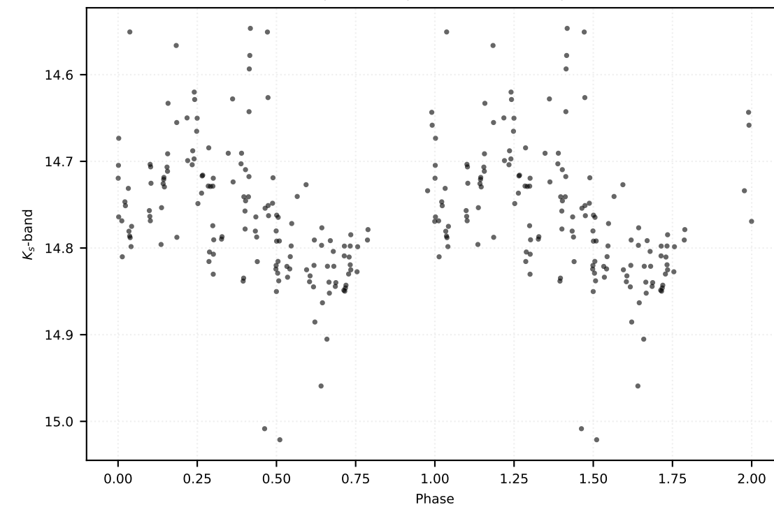
P: 1.22343 d | Class: RP | Subclass: CEP-1OT | Field b279
