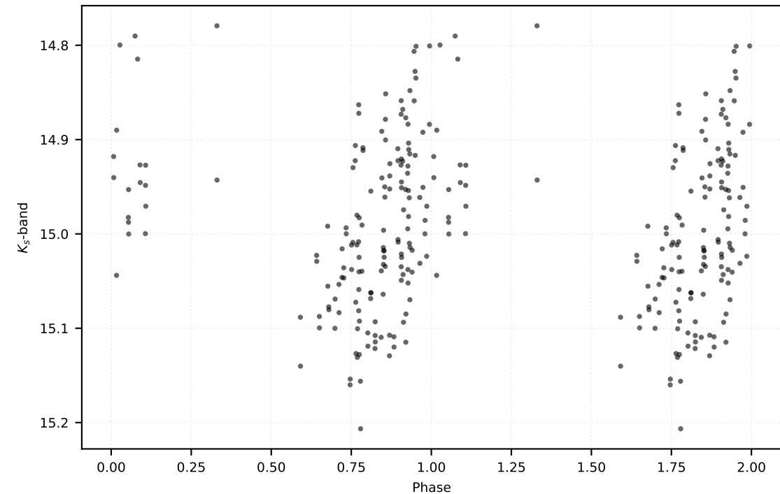
P: 0.99713 d | Class: RP | Subclass: RRab | Field b279
