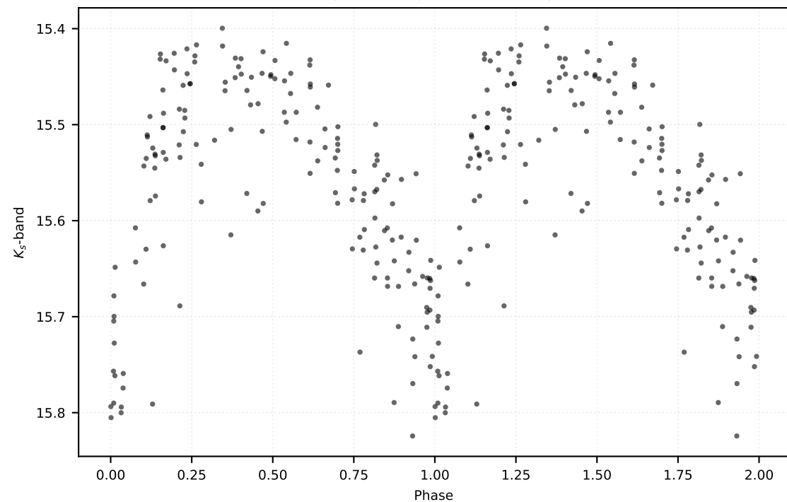
P: 0.68154 d | Class: RP | Subclass: RRab | Field b278
