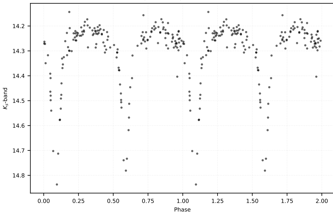
P: 2.46498 d | Class: EB | Subclass: EA | Field b279
