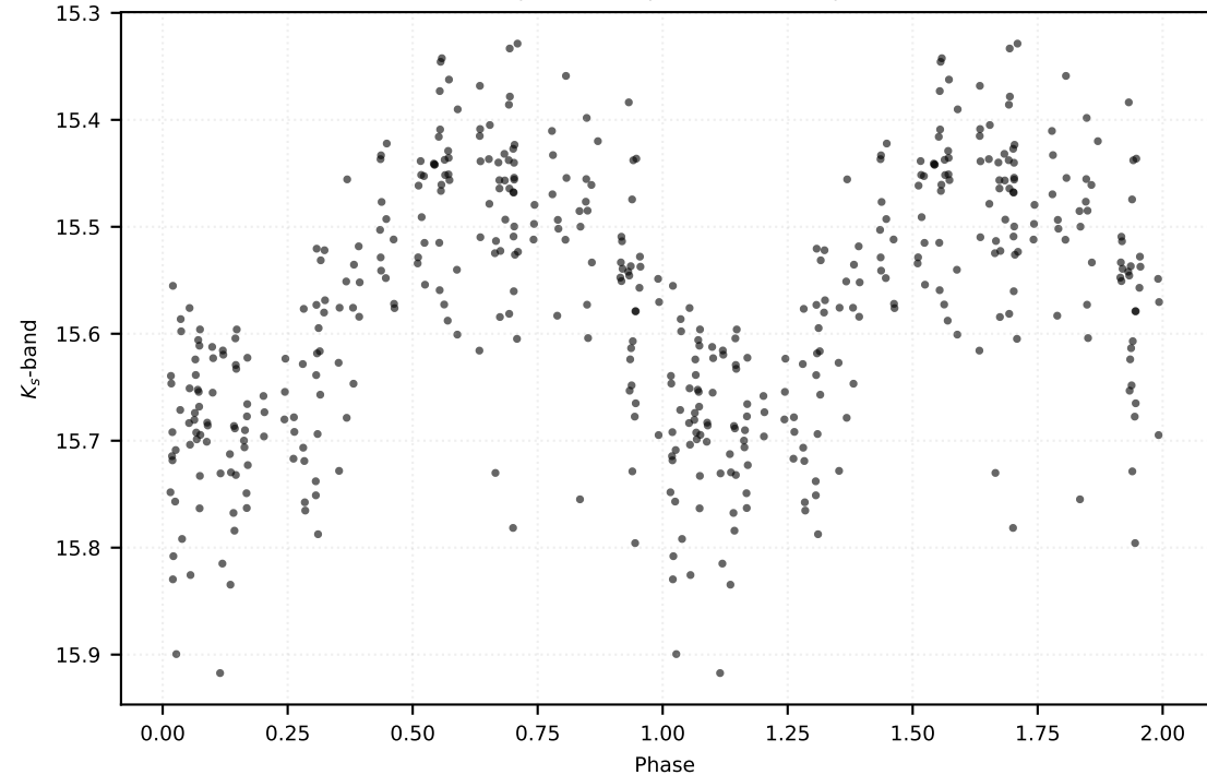
P: 0.41881 d | Class: RP | Subclass: RRc | Field b278
