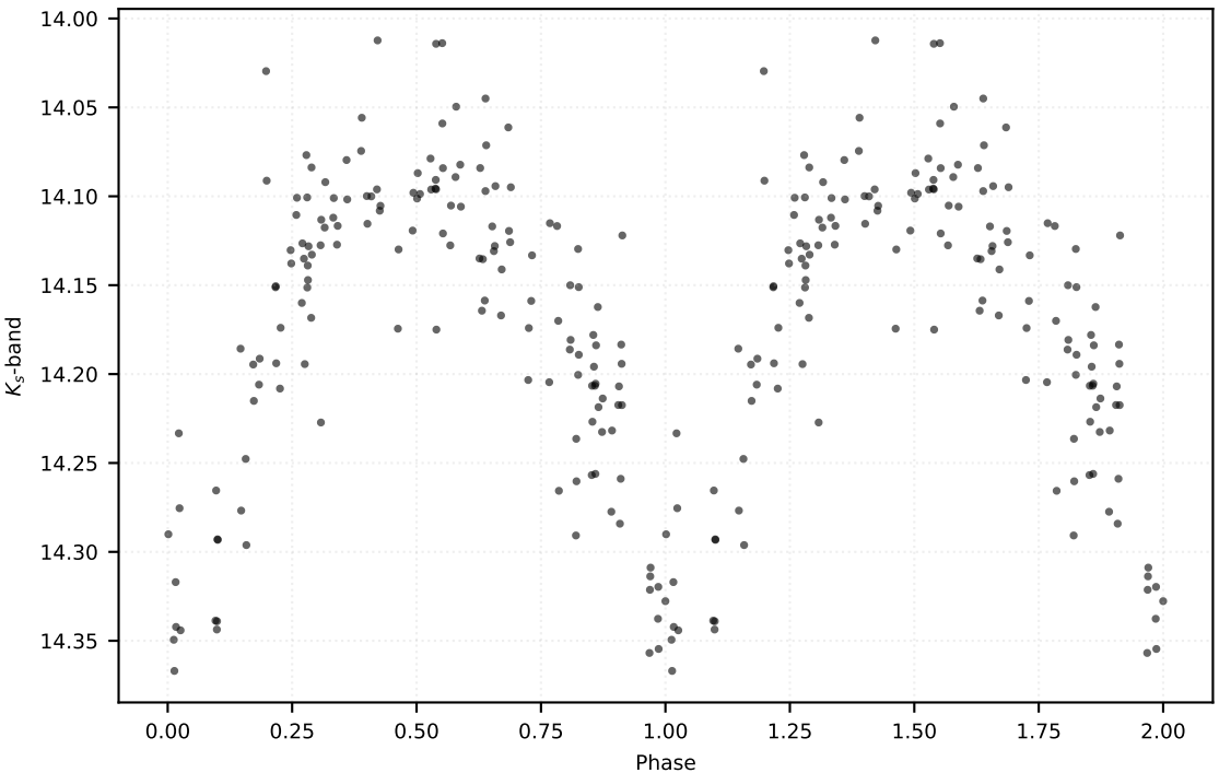
P: 0.60281 d | Class: RP | Subclass: RRab | Field b279
