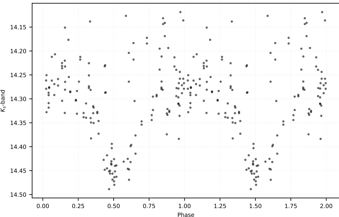
P: 3.36410 d | Class: RP | Subclass: CEP-F | Field b278
