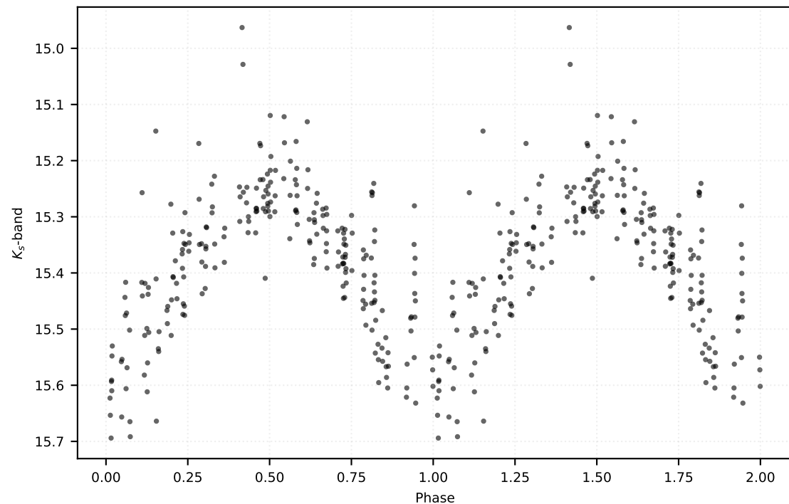
P: 0.99930 d | Class: RP | Subclass: RRab | Field b279
