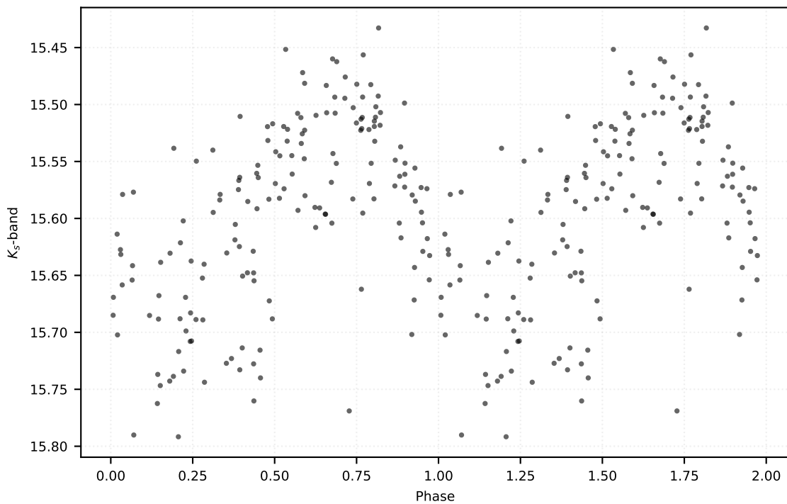
P: 7.10652 d | Class: RP | Subclass: CEP-10T | Field b278
