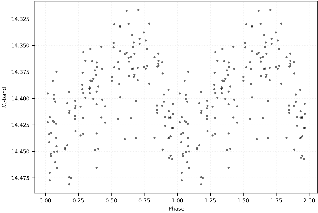
P: 20.25767 d | Class: RP | Subclass: CEP-F | Field b279
