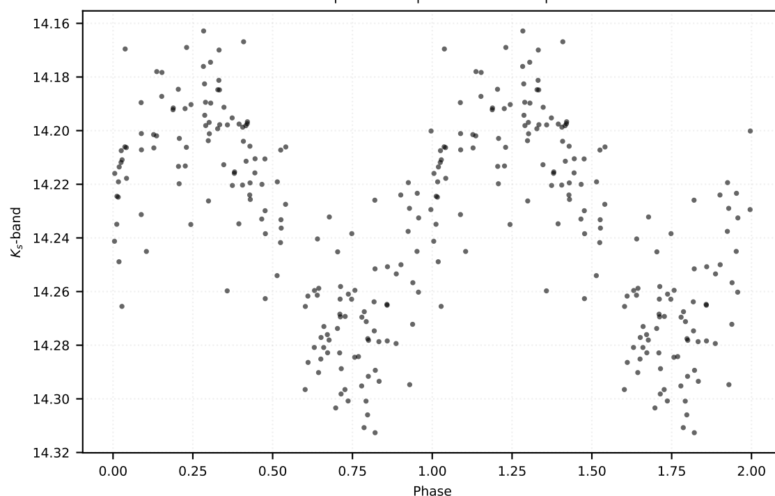
P: 0.69085 d | Class: RP | Subclass: RRab | Field b278
