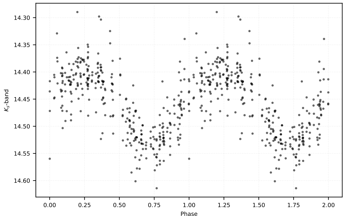
P: 0.60207 d | Class: RP | Subclass: CEP-10T | Field b279
