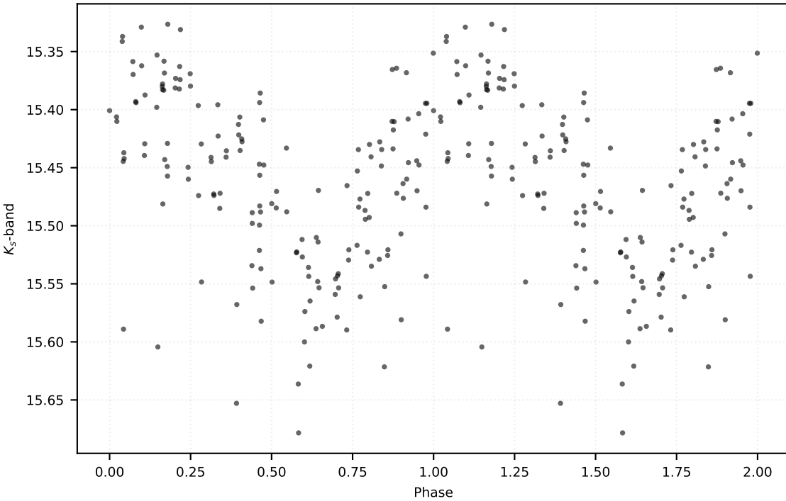
P: 0.38470 d | Class: RP | Subclass: RRab | Field b279
