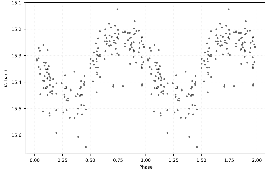
P: 0.64289 d | Class: RP | Subclass: R Rab | Field b278
