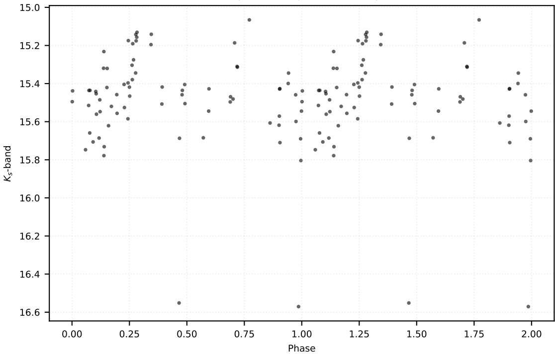
P: 0.39891 d | Class: EB | Subclass: EA | Field b279
