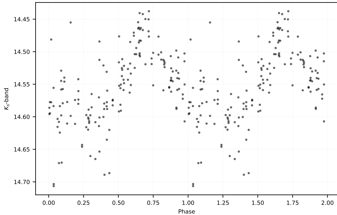
P: 4.11320 d | Class: RP | Subclass: CEP-F | Field b279
