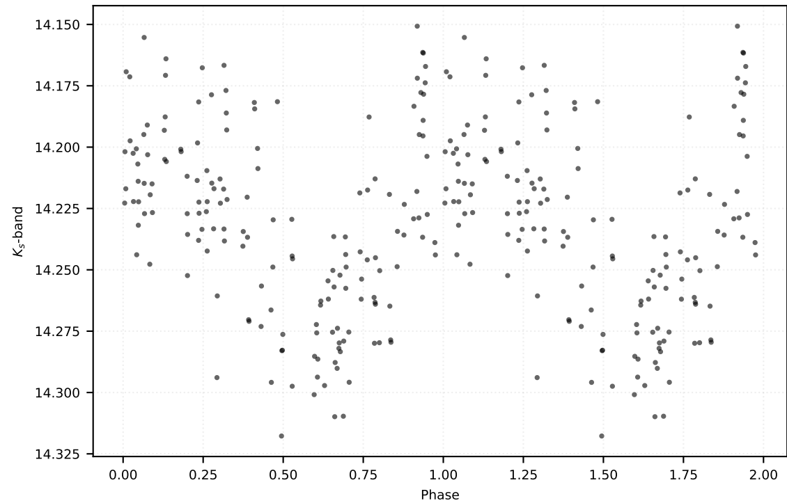
P: 0.30682 d | Class: RP | Subclass: RRab | Field b279
