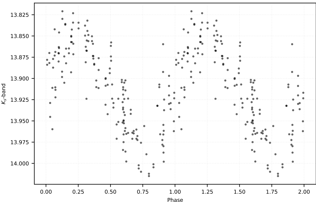
P: 0.53359 d | Class: RP | Subclass: CEP-10T | Field b279
