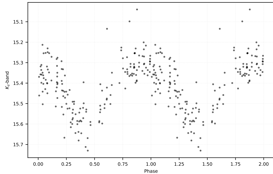
P: 0.29336 d | Class: RP | Subclass: RRc | Field b278
