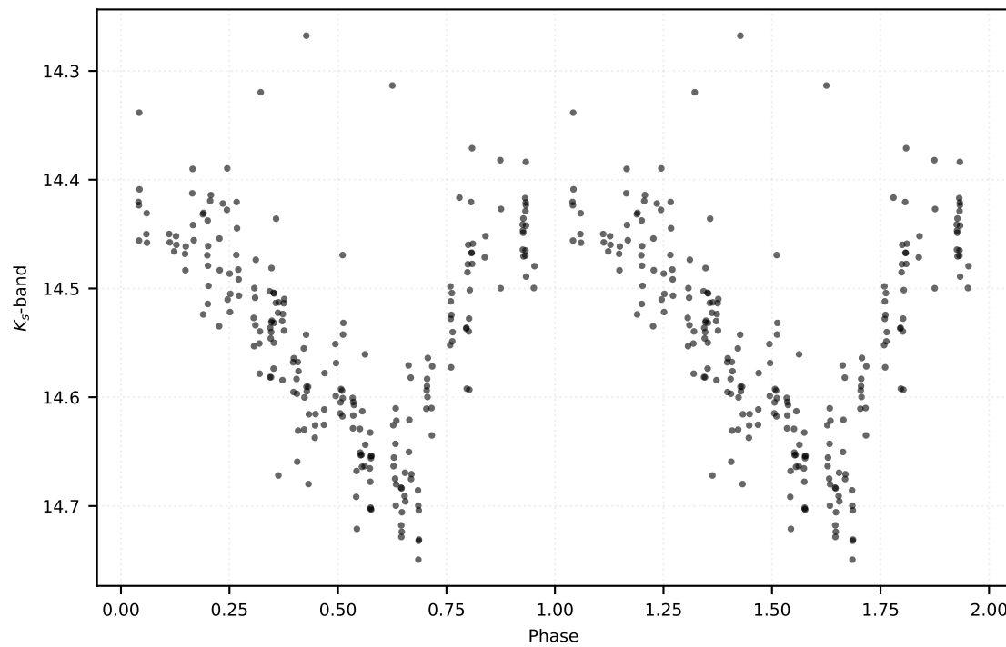
P: 0.48653 d | Class: RP | Subclass: RRab | Field b278
