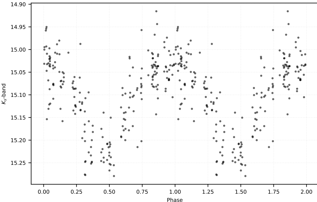
P: 0.39470 d | Class: RP | Subclass: RRab | Field b279
