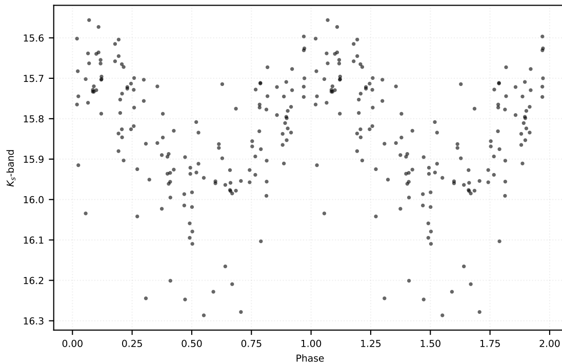
P: 0.35515 d | Class: RP | Subclass: CEP-10T | Field b279
