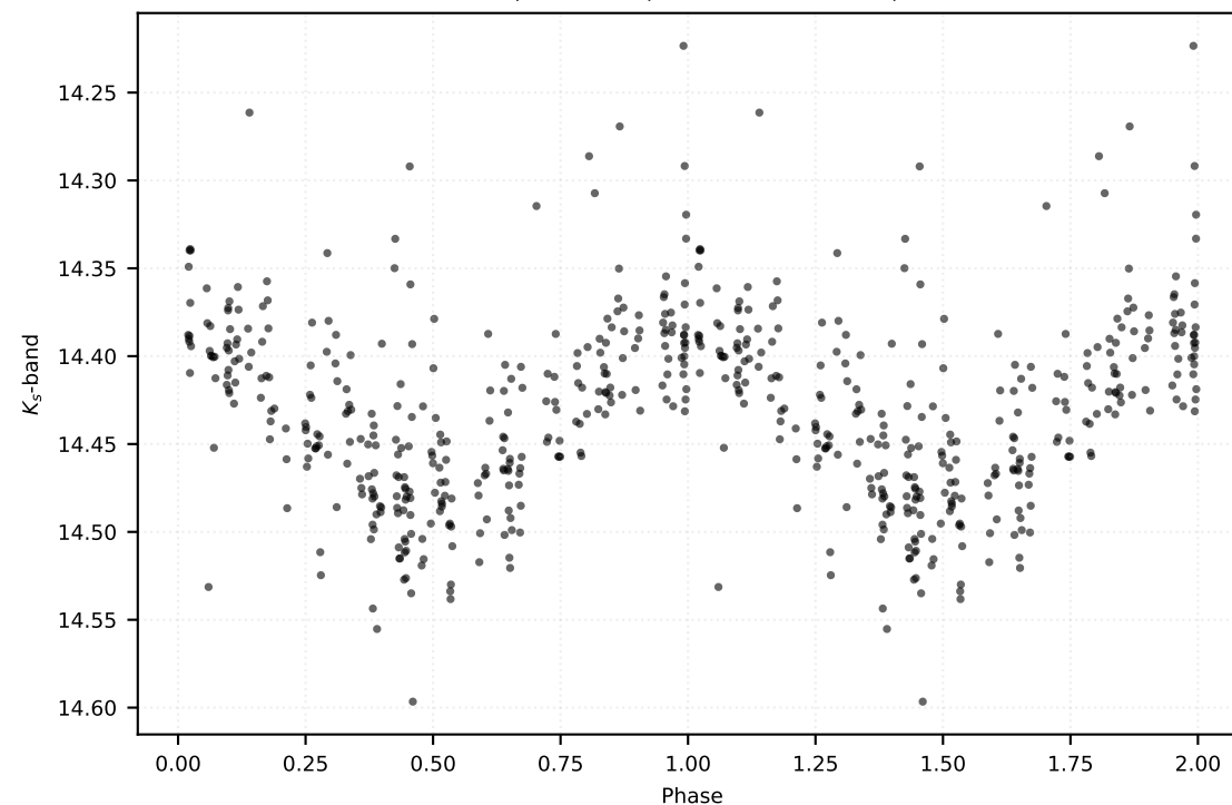
P: 0.36319 d | Class: RP | Subclass: CEP-1OT | Field b279
