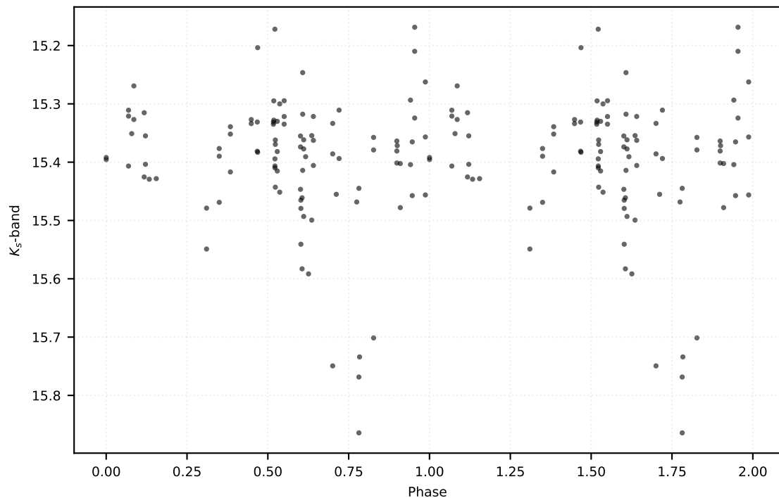
P: 0.39046 d | Class: EB | Subclass: EA | Field b278
