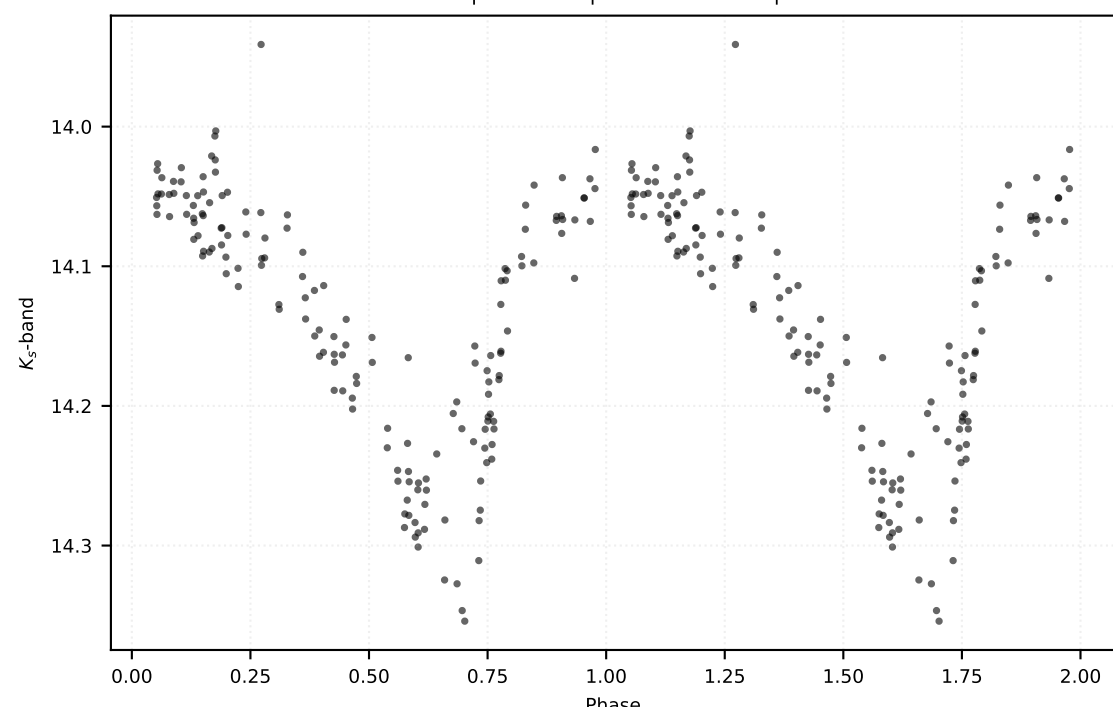
P: 0.55216 d | Class: RP | Subclass: RRab | Field b279
