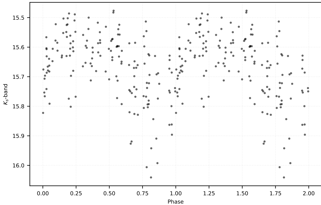
P: 0.31931 d | Class: RP | Subclass: RRab | Field b279
