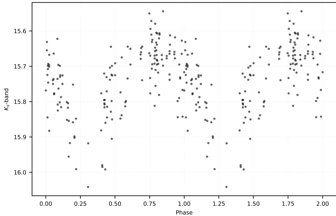
P: 0.99728 d | Class: RP | Subclass: RRab | Field b278
