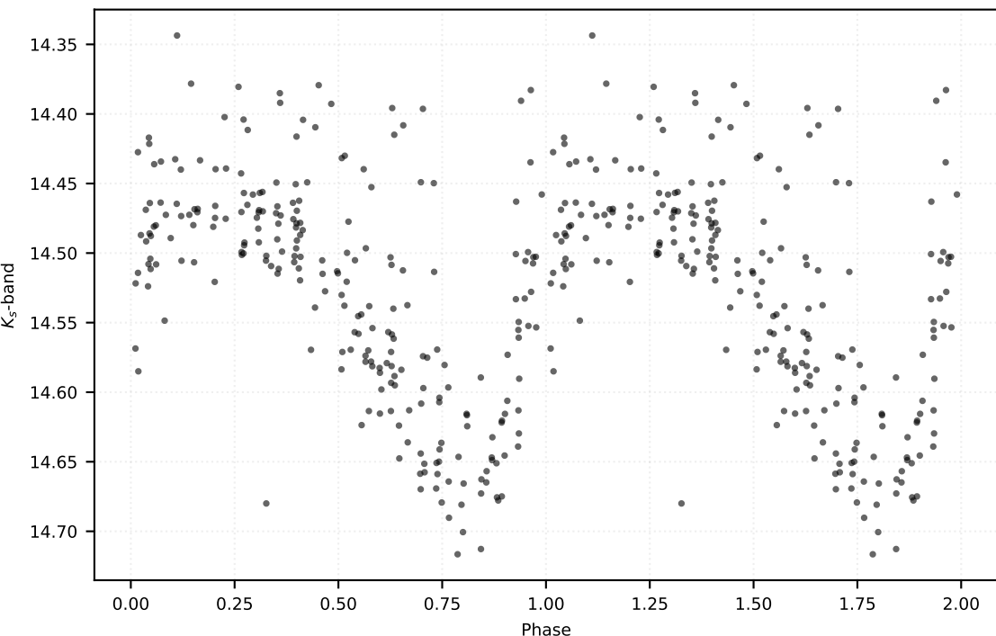
P: 0.43211 d | Class: RP | Subclass: RRab | Field b279
