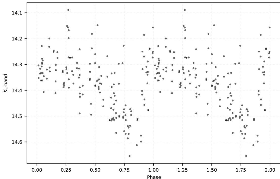
P: 0.69638 d | Class: RP | Subclass: RRab | Field b279
