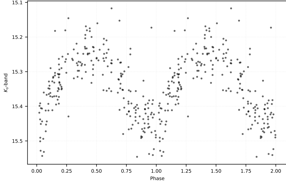
P: 0.49795 d | Class: RP | Subclass: RRab | Field b279
