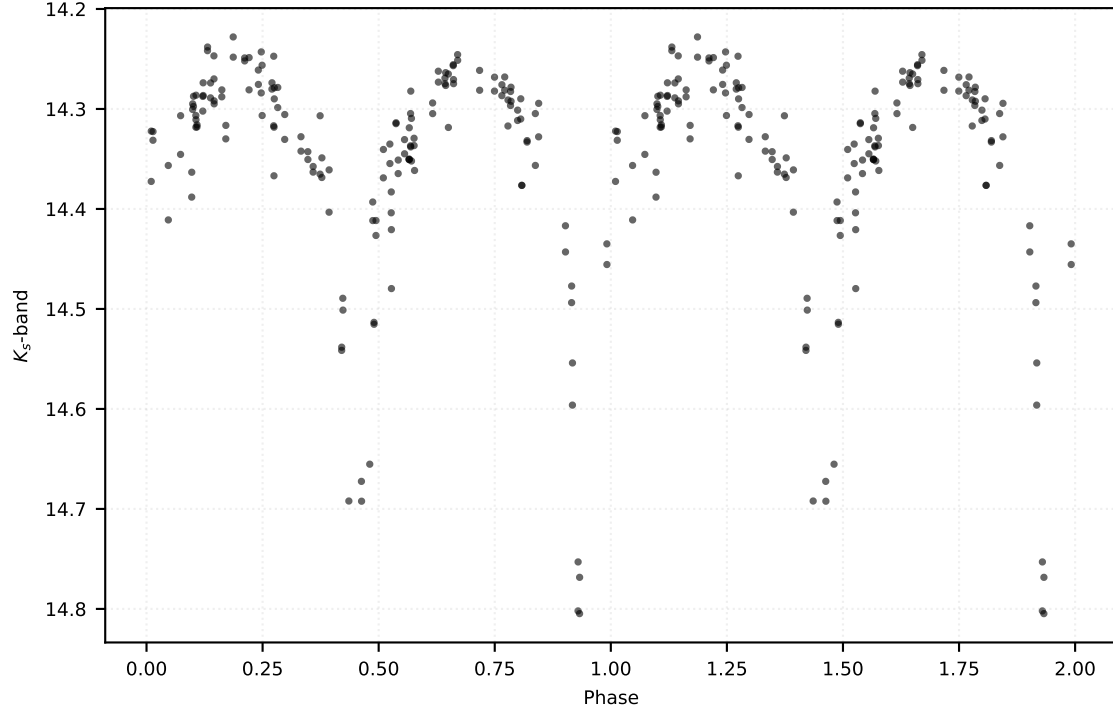
P: 7.42188 d | Class: EB | Subclass: EA | Field b278
