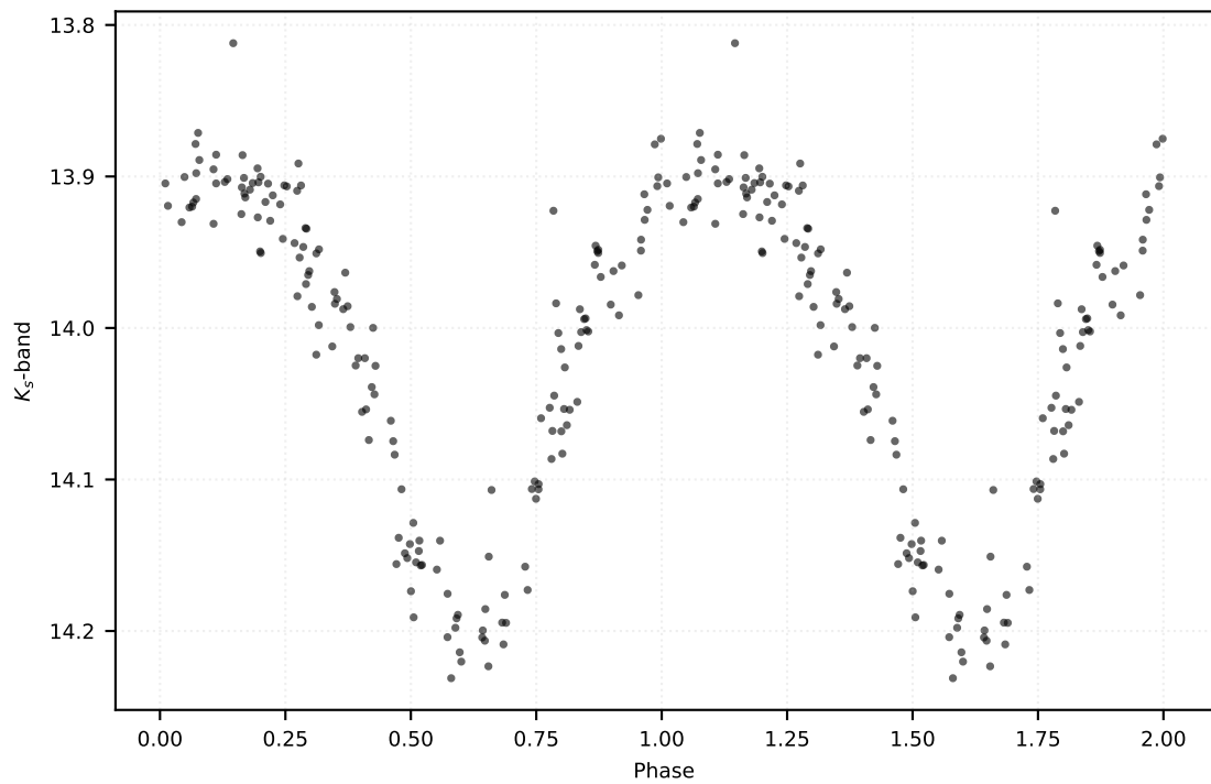
P: 0.22485 d | Class: RP | Subclass: UVAR | Field b278
