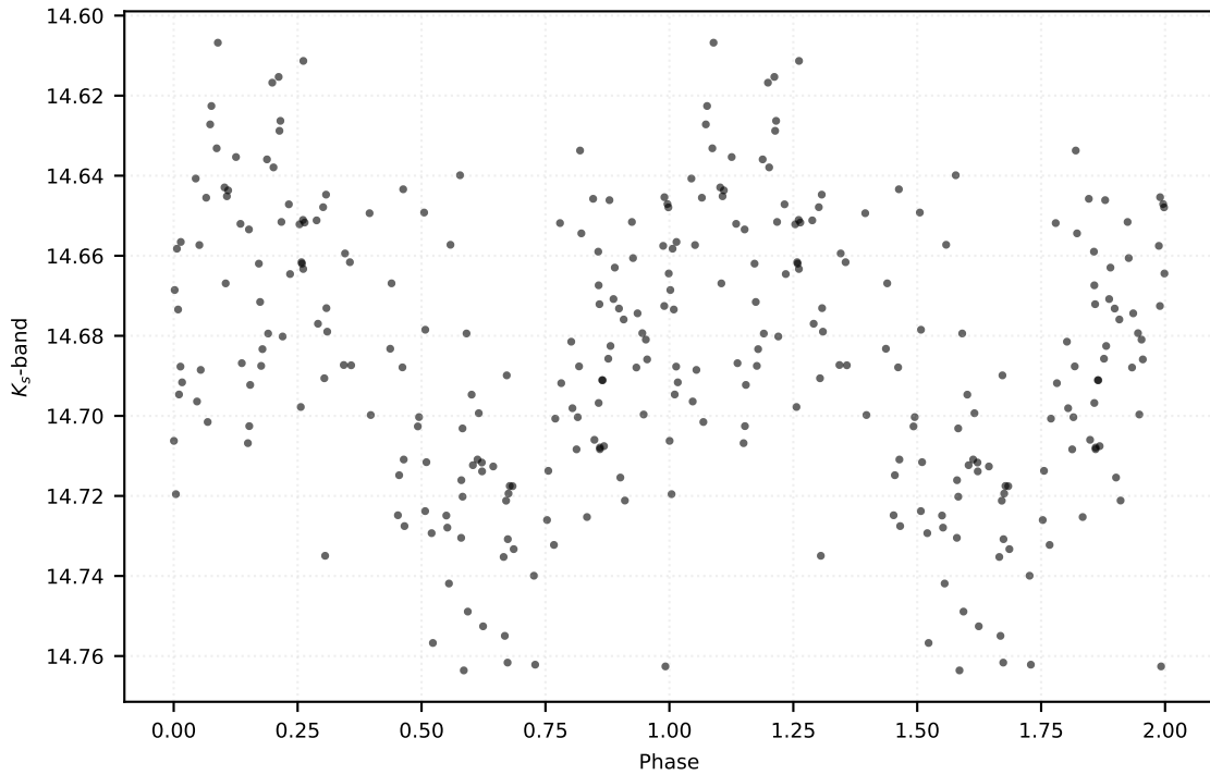
P: 0.35341 d | Class: RP | Subclass: CEP-10T | Field b278
