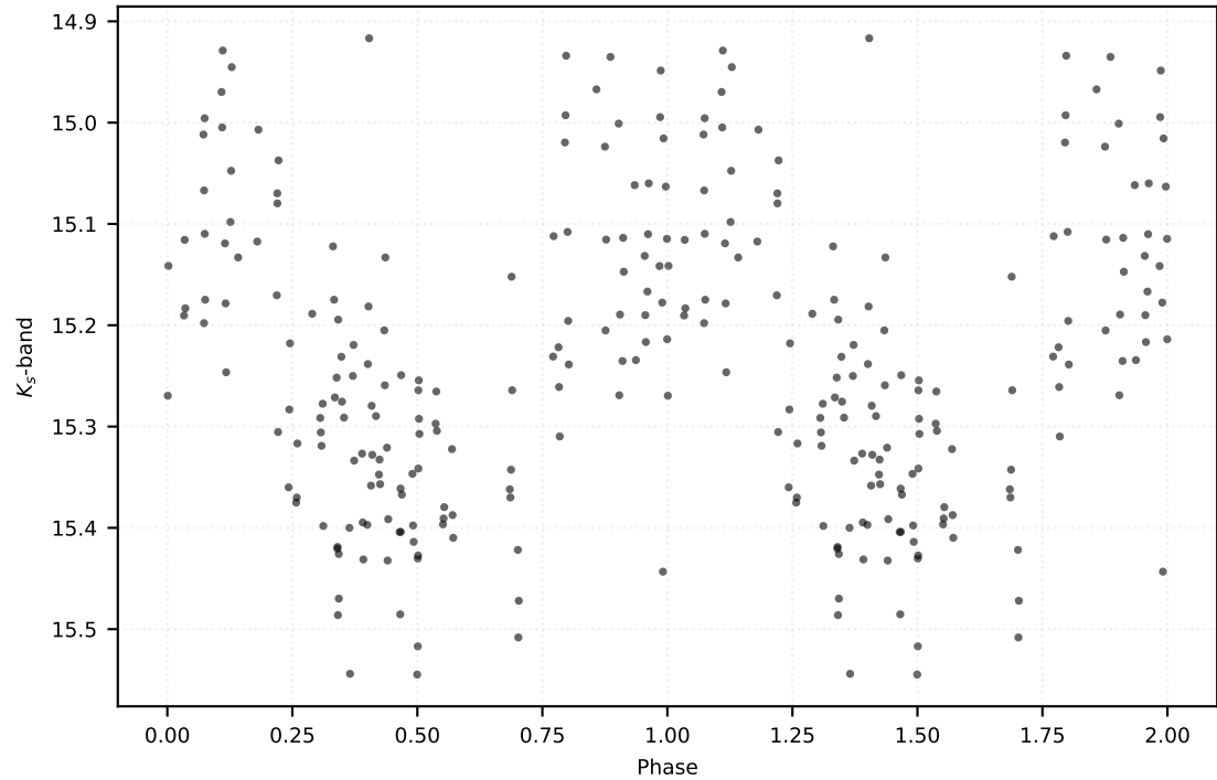
P: 0.73629 d | Class: RP | Subclass: RRab | Field b278
