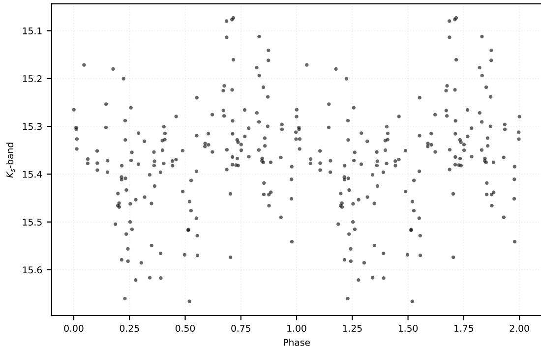
P: 0.35029 d | Class: RP | Subclass: RRab | Field b278
