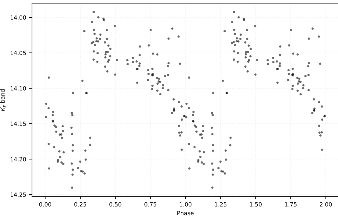
P: 0.50524 d | Class: RP | Subclass: RRab | Field b279
