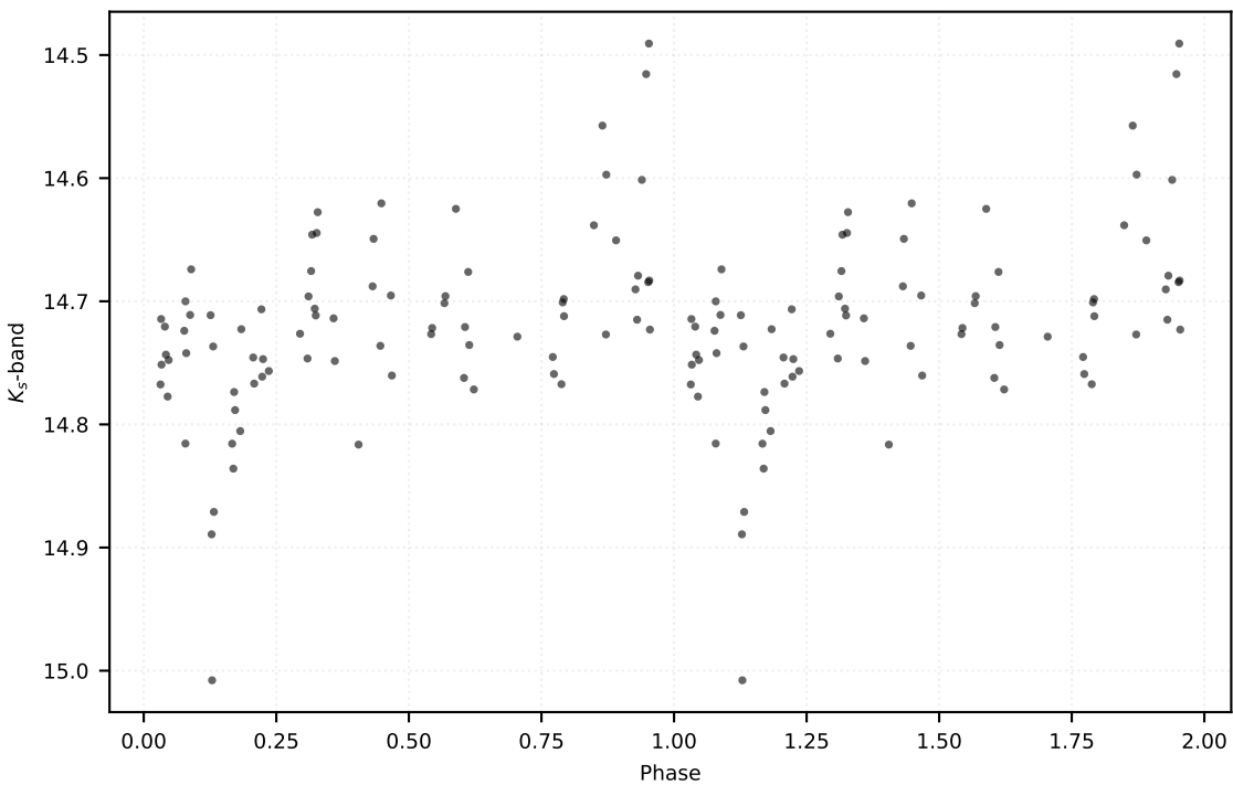
P: 2.28087 d | Class: EB | Subclass: EA | Field b279
