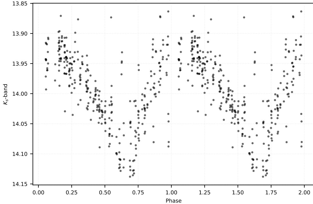
P: 0.46203 d | Class: RP | Subclass: RRc | Field b279
