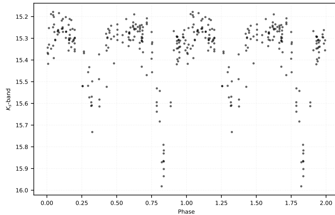
P: 0.19276 d | Class: RP | Subclass: UVAR | Field b278
