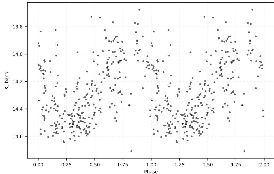
P: 58.78048 d | Class: RP | Subclass: UVAR | Field b279
