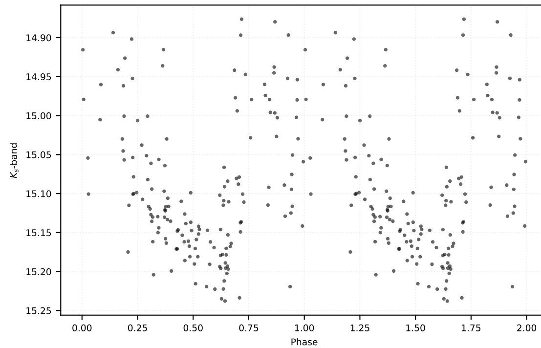
P: 0.13481 d | Class: RP | Subclass: UVAR | Field b279
