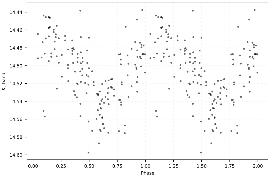
P: 2.70061 d | Class: RP | Subclass: CEP-1OT | Field b279
