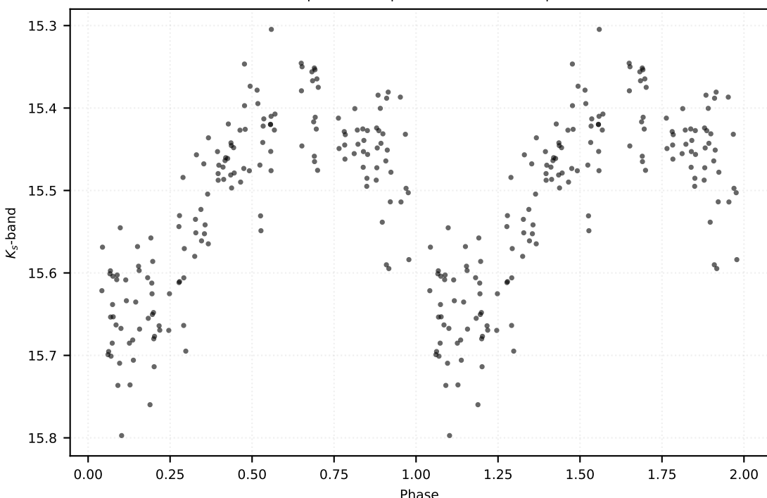
P: 0.99728 d | Class: RP | Subclass: CEP-10T | Field b278
