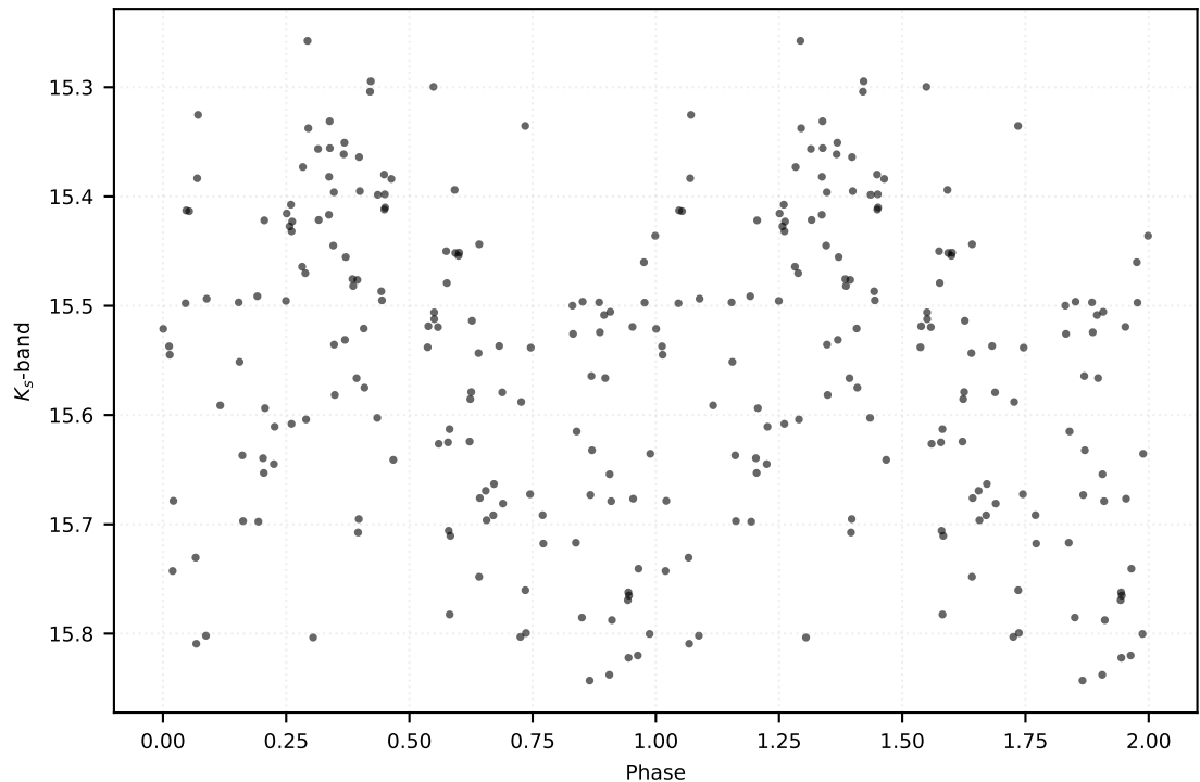
P: 0.53598 d | Class: RP | Subclass: RRc | Field b278
