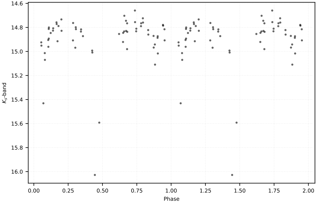
P: 0.35881 d | Class: EB | Subclass: EA | Field b278
