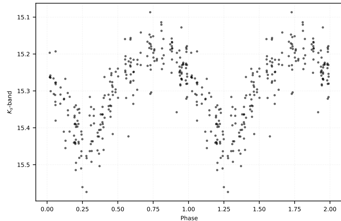
P: 0.53216 d | Class: RP | Subclass: RRc | Field b279
