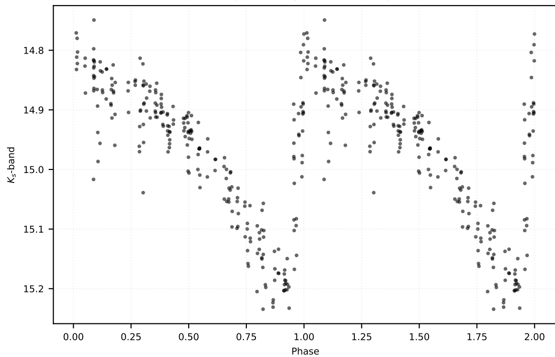
P: 0.44166 d | Class: RP | Subclass: RRab | Field b278
