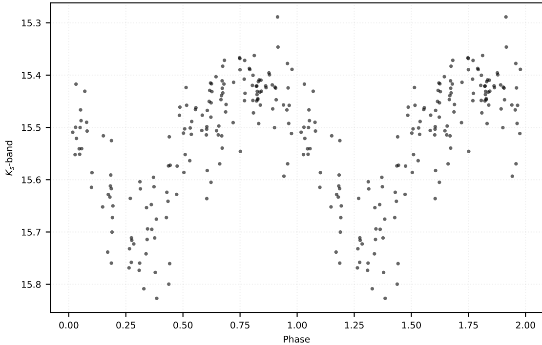
P: 0.57057 d | Class: RP | Subclass: RRab | Field b279
