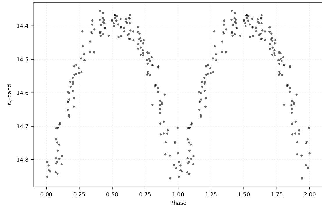
P: 0.19232 d | Class: RP | Subclass: UVAR | Field b278
