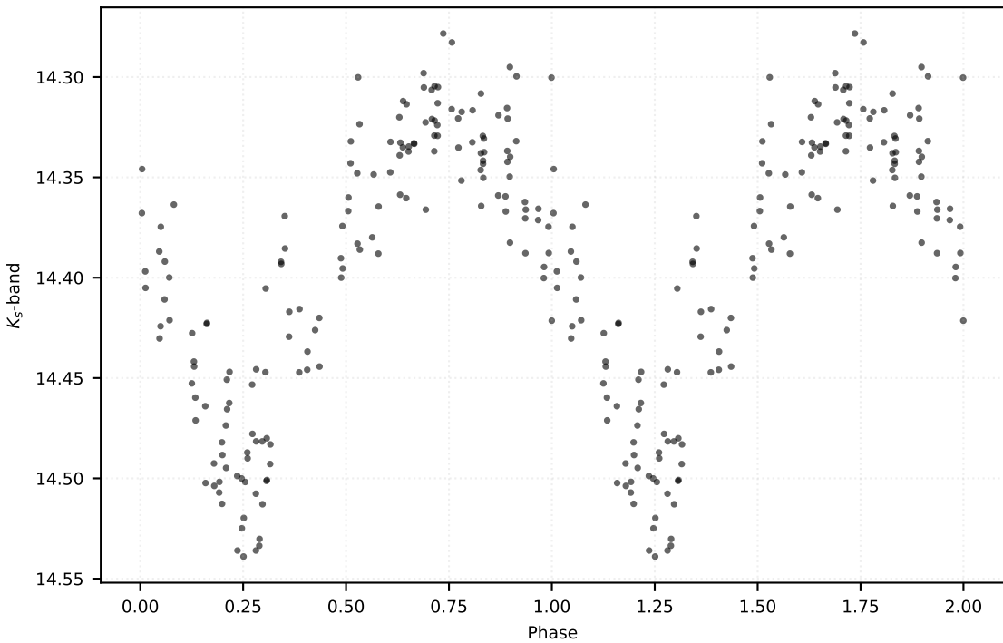
P: 0.35979 d | Class: RP | Subclass: RRab | Field b278
