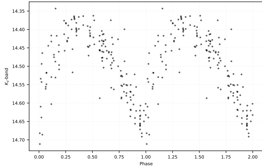
P: 0.62004 d | Class: RP | Subclass: RRab | Field b278
