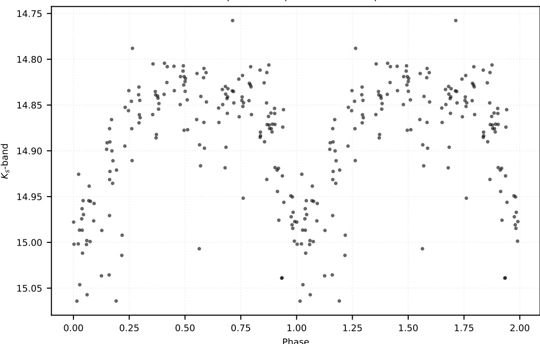
P: 0.70632 d | Class: RP | Subclass: RRab | Field b279
