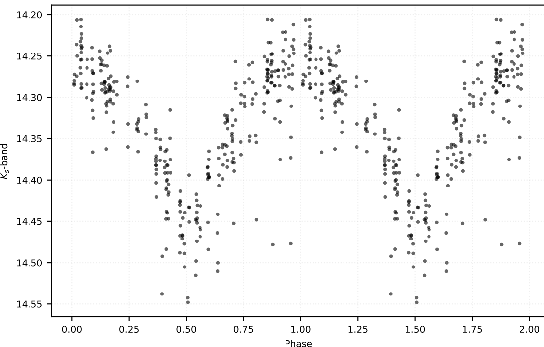
P: 0.36418 d | Class: RP | Subclass: RRab | Field b278
