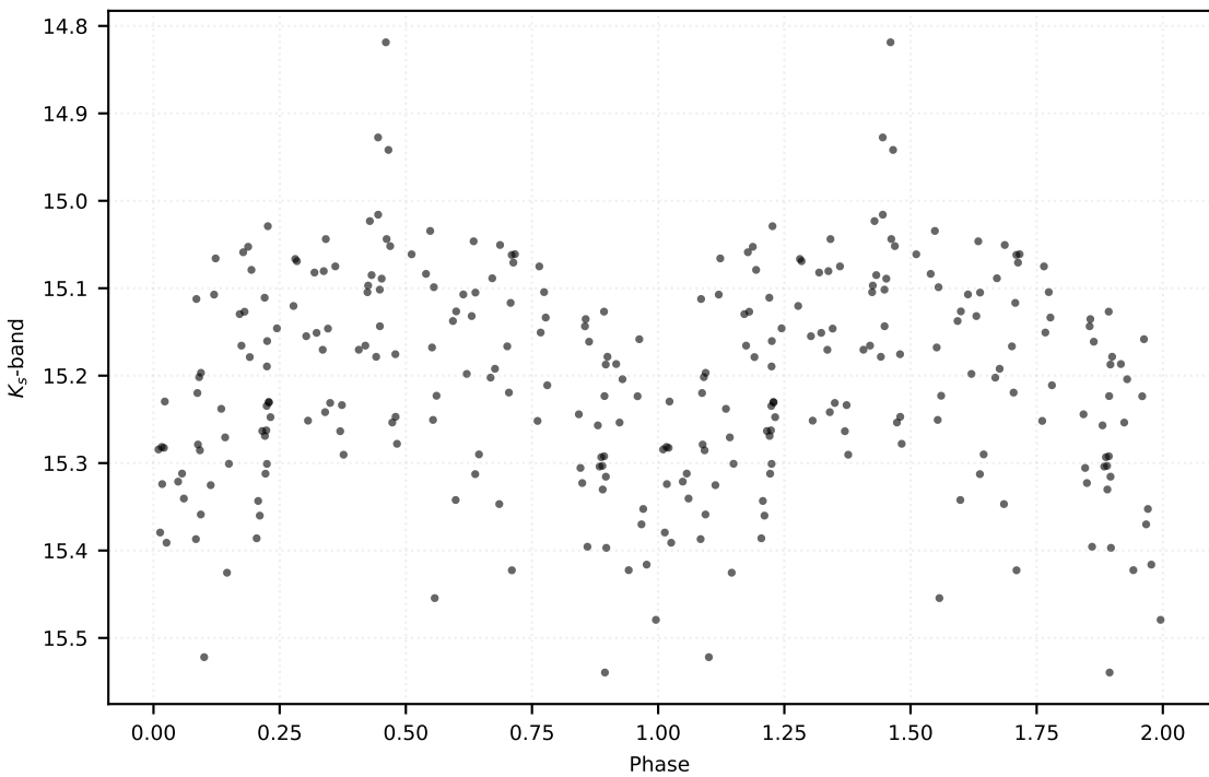
P: 0.19798 d | Class: RP | Subclass: UVAR | Field b279
