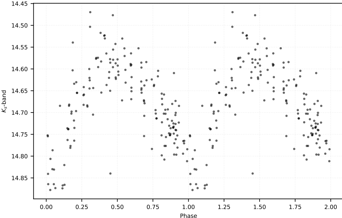
P: 0.61276 d | Class: RP | Subclass: RRab | Field b278
