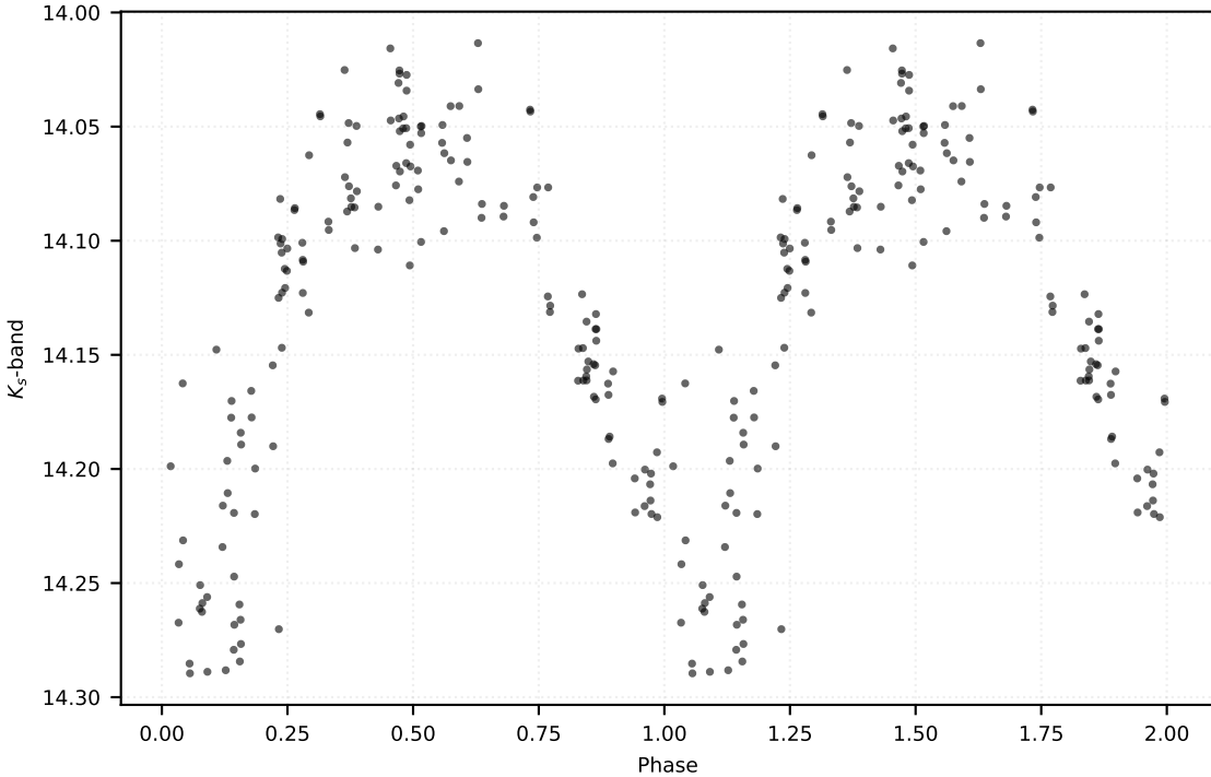
P: 0.48144 d | Class: RP | Subclass: RRab | Field b279
