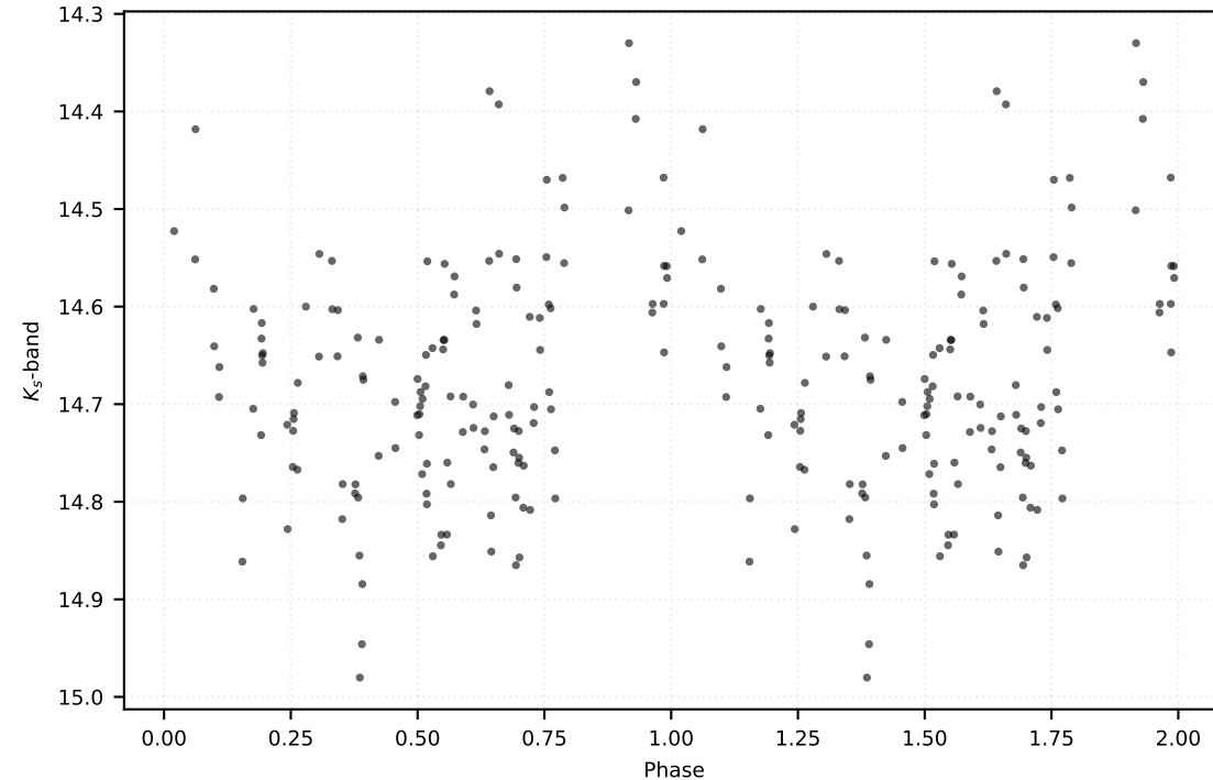
P: 1.86126 d | Class: RP | Subclass: CEP-10T | Field b278
