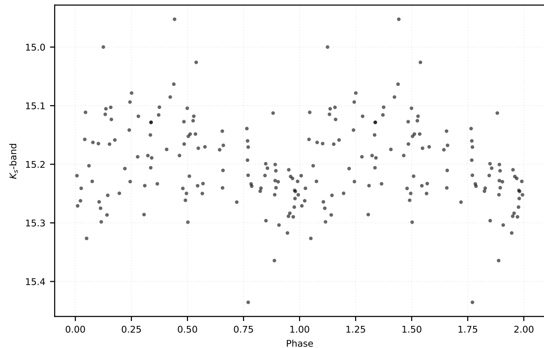
P: 0.12136 d | Class: RP | Subclass: UVAR | Field b279
