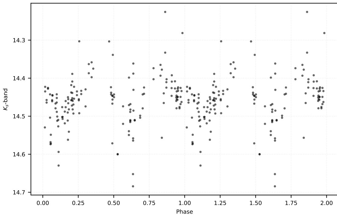
P: 0.20237 d | Class: EB | Subclass: EA | Field b279
