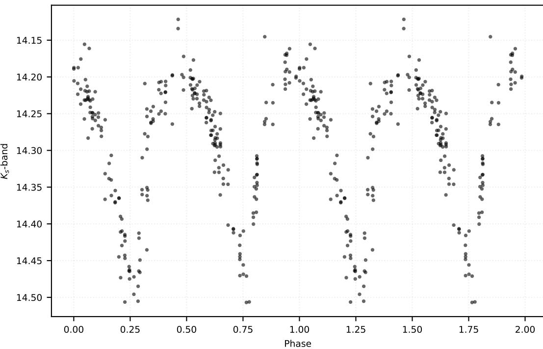
P: 1.02311 d | Class: EB | Subclass: RRc | Field b278
