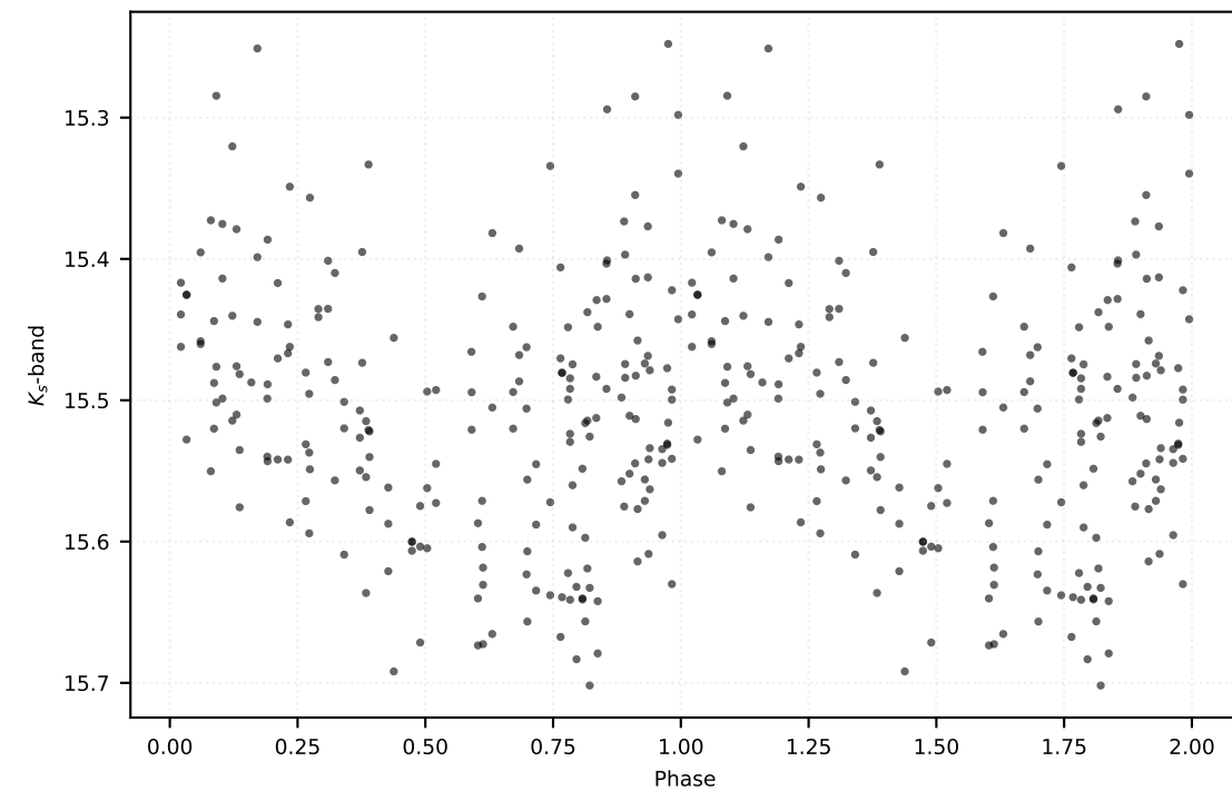
P: 1.35021 d | Class: RP | Subclass: CEP-F | Field b278
