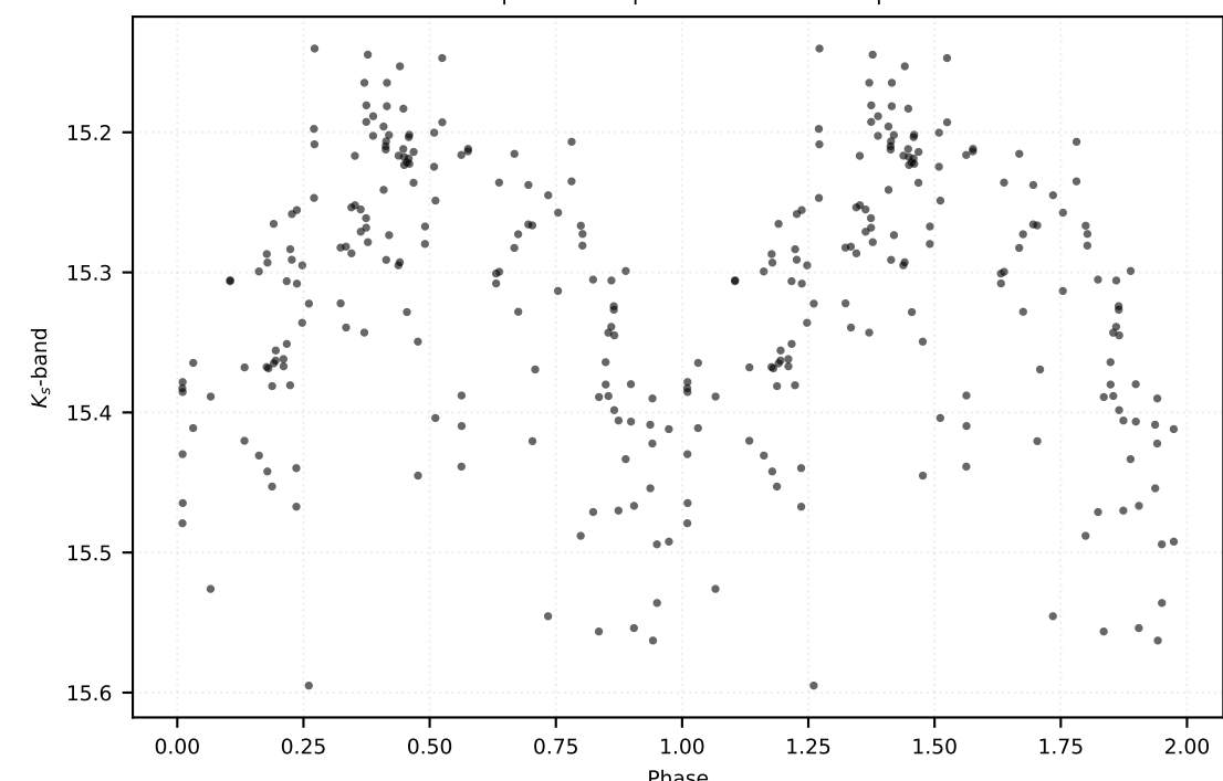
P: 2.06302 d | Class: RP | Subclass: CEP-10T | Field b279
