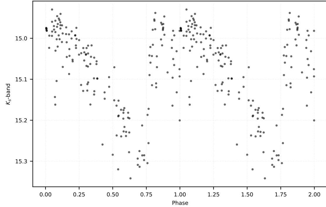
P: 0.58764 d | Class: RP | Subclass: RRab | Field b278
