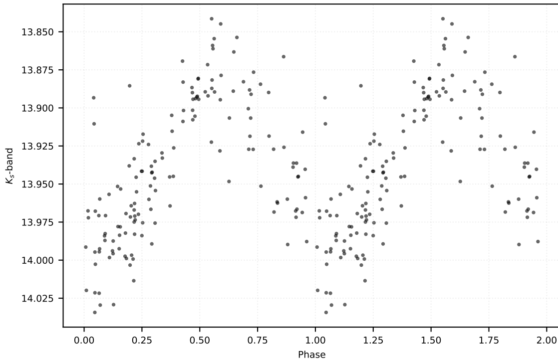
P: 0.40185 d | Class: RP | Subclass: RRc | Field b278
