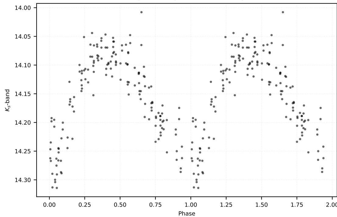
P: 0.46033 d | Class: RP | Subclass: CEP-10T | Field b279
