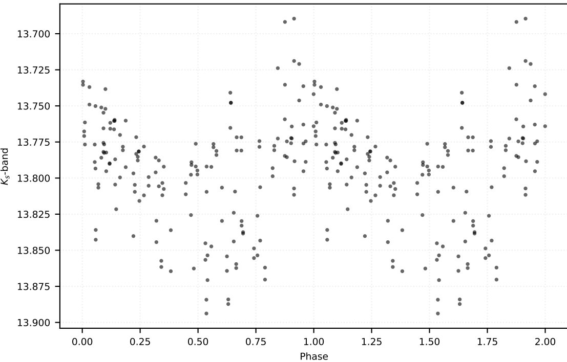
P: 1.10936 d | Class: RP | Subclass: CEP-F | Field b279
