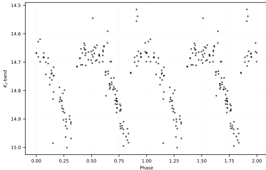
P: 0.19261 d | Class: RP | Subclass: UVAR | Field b279
