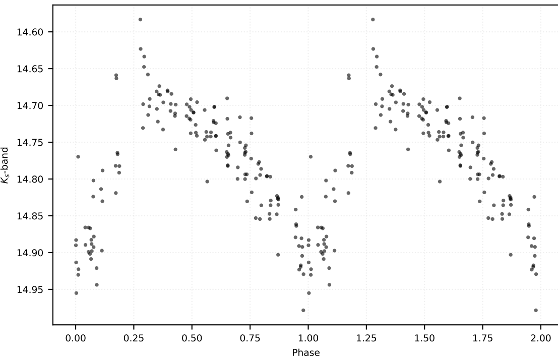
P: 0.51044 d | Class: RP | Subclass: RRab | Field b279
