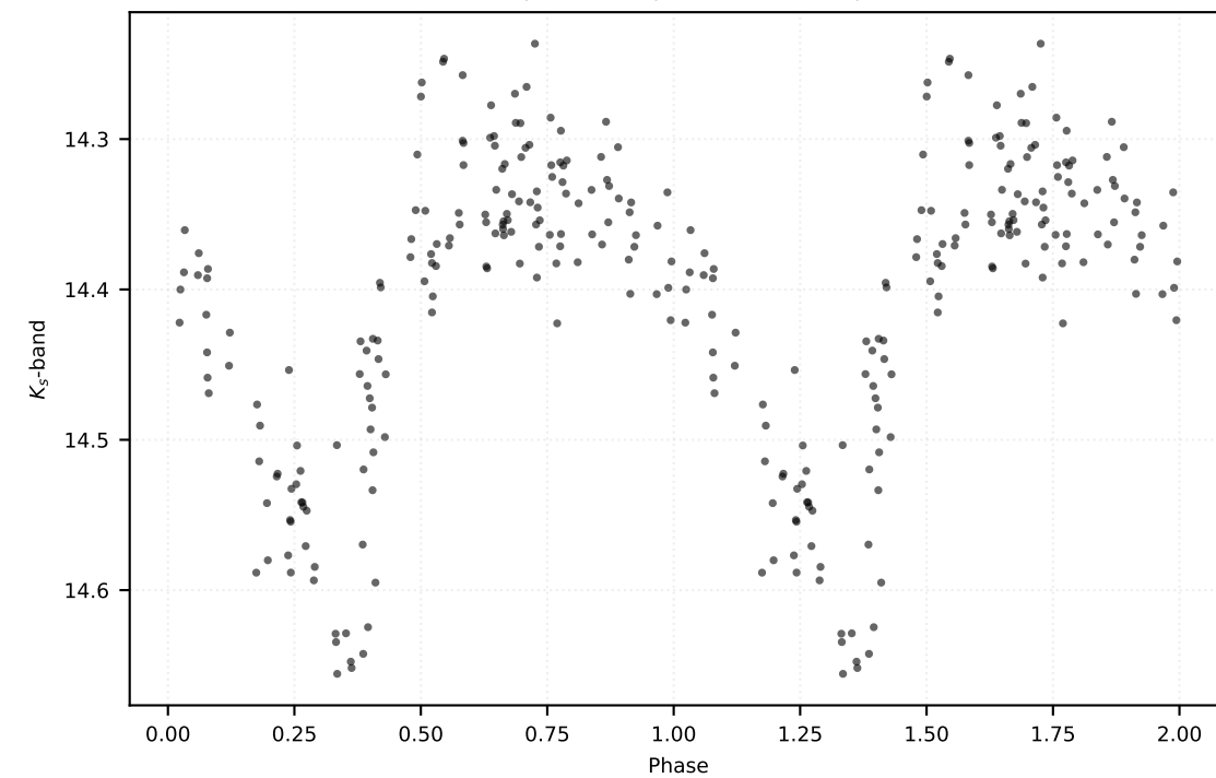
P: 0.62256 d | Class: RP | Subclass: RRab | Field b279
