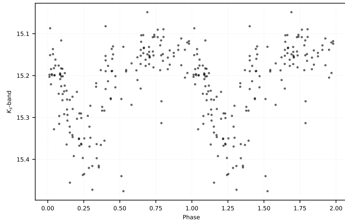
P: 0.64533 d | Class: RP | Subclass: RRab | Field b278
