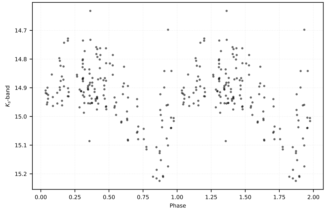
P: 1.00042 d | Class: RP | Subclass: CEP-10T | Field b279
