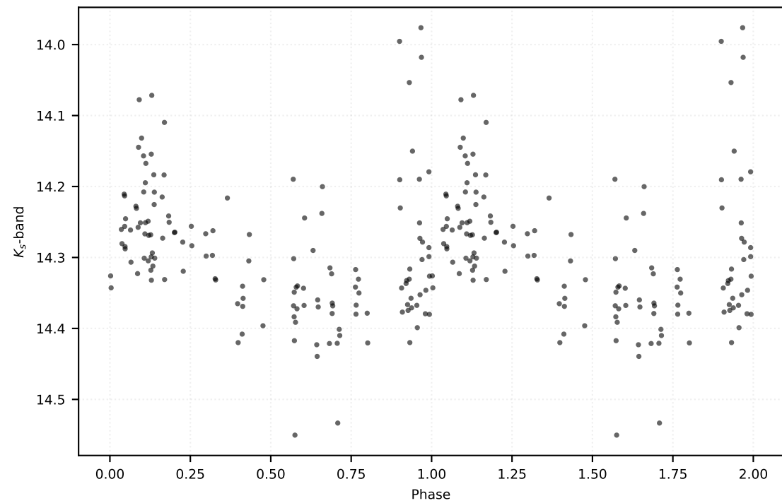
P: 0.19963 d | Class: RP | Subclass: UVAR | Field b278
