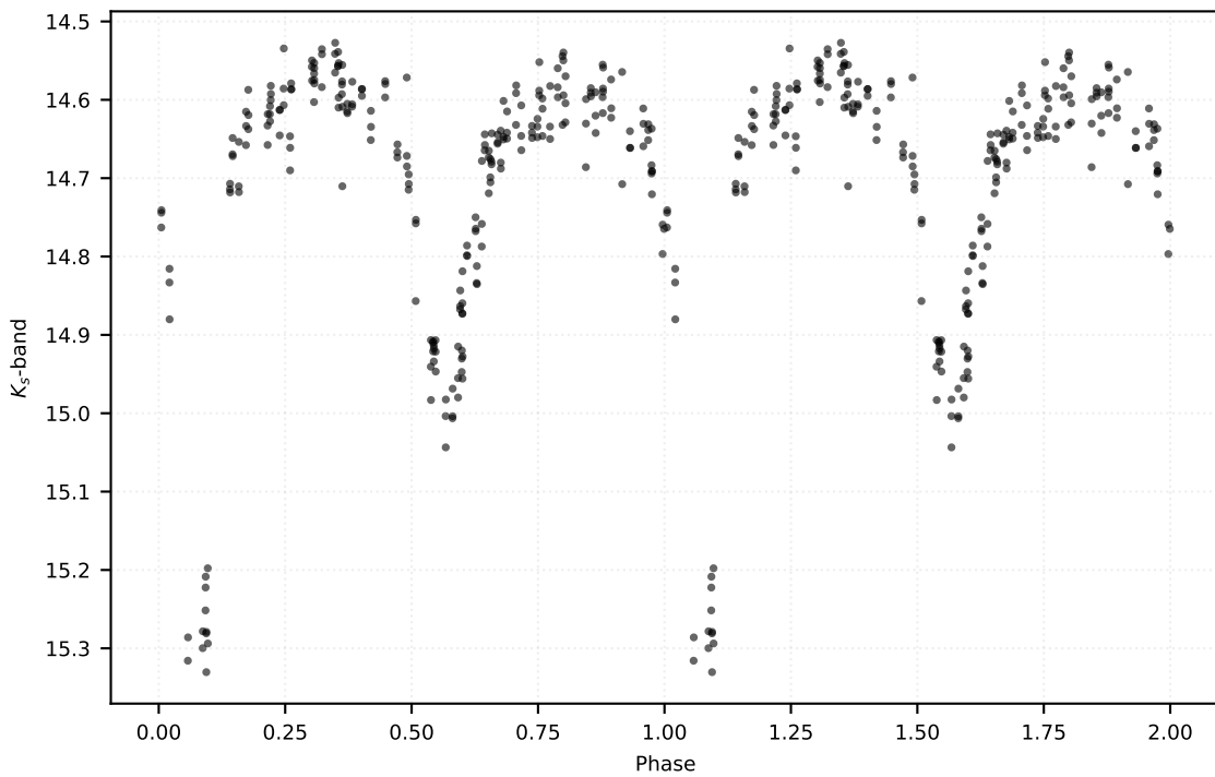
P: 3.82302 d | Class: EB | Subclass: EA | Field b279
