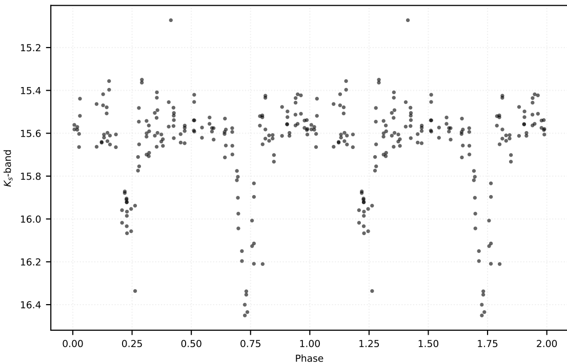
P: 0.80691 d | Class: EB | Subclass: UVAR | Field b278
