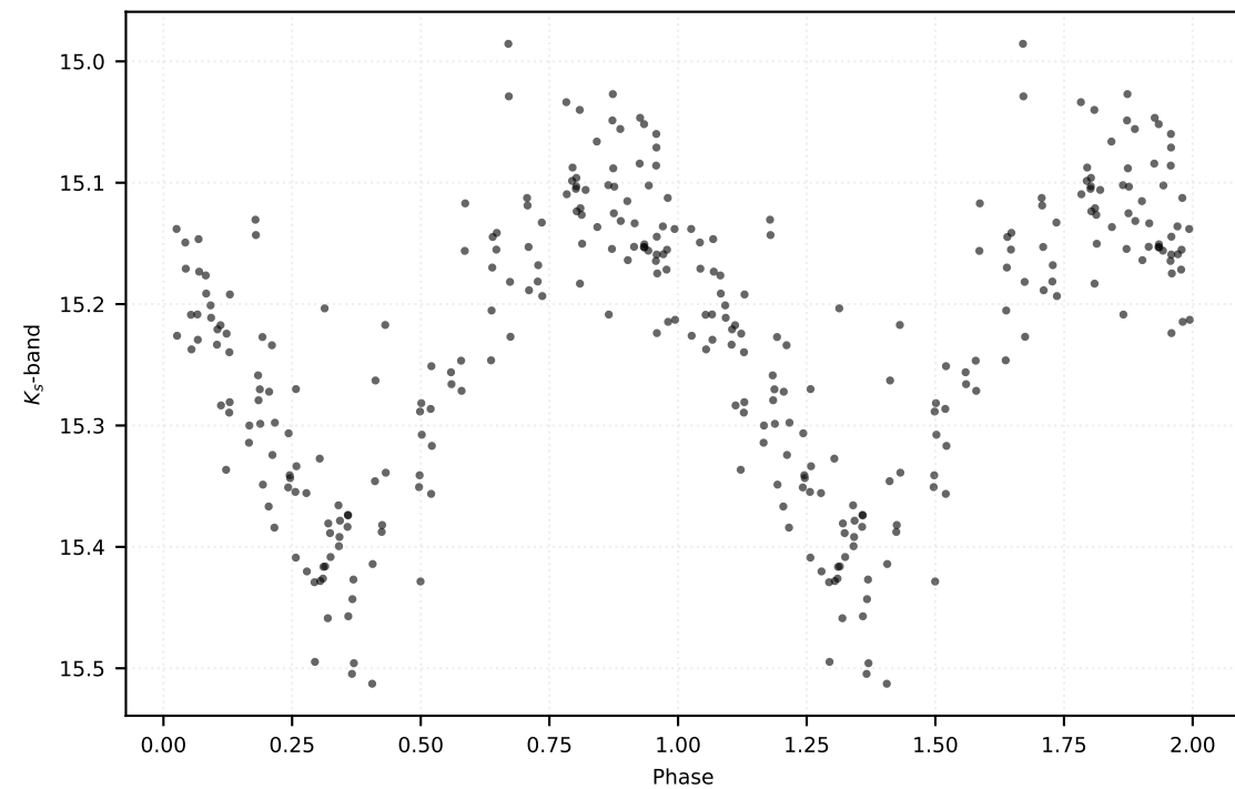
P: 0.32997 d | Class: RP | Subclass: RRc | Field b278
