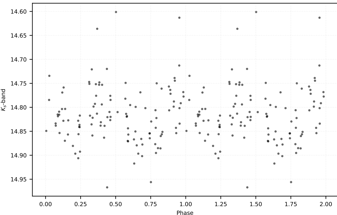
P: 0.28490 d | Class: EB | Subclass: EA | Field b278
