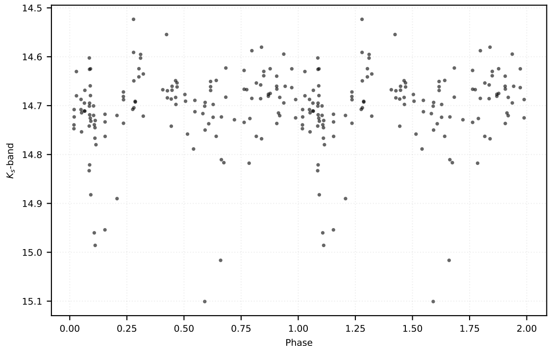
P: 0.39890 d | Class: EB | Subclass: EA | Field b278
