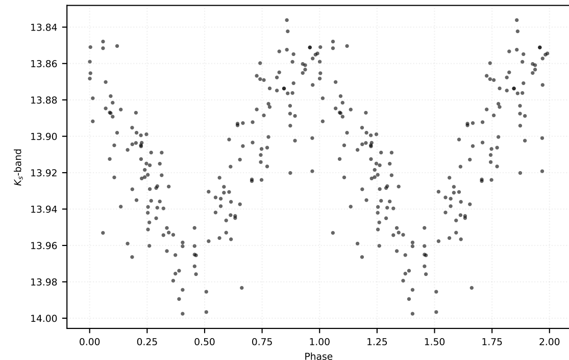
P: 0.28482 d | Class: RP | Subclass: CEP-10T | Field b279
