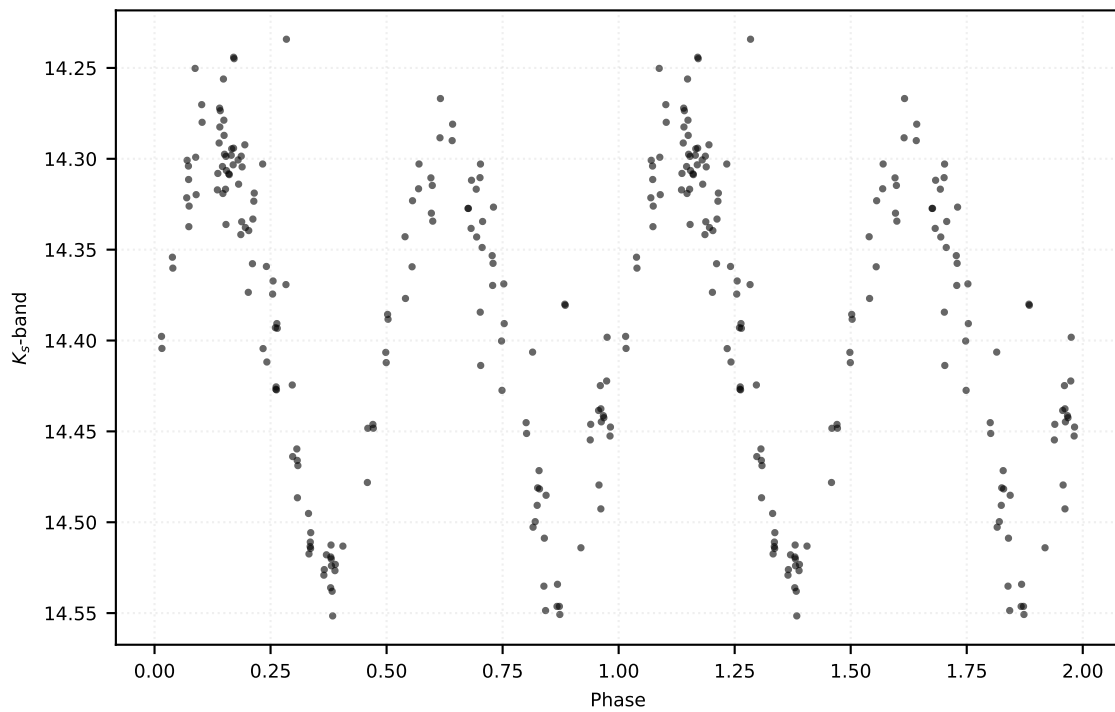
P: 0.50910 d | Class: RP | Subclass: RRc | Field b278
