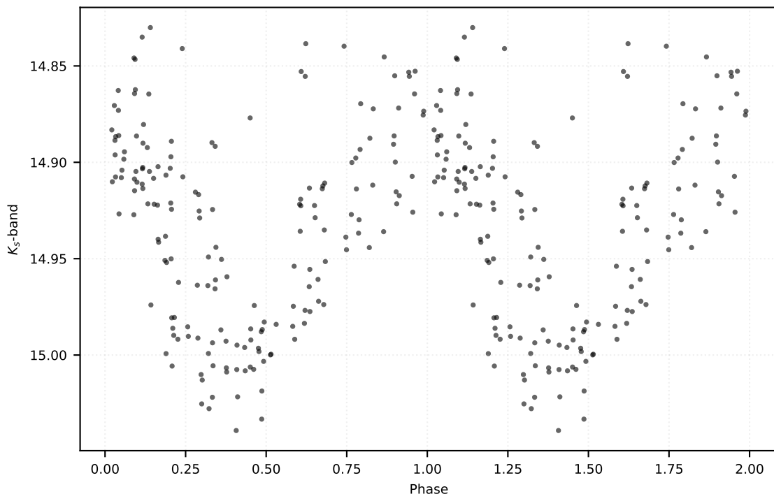
P: 0.17697 d | Class: RP | Subclass: UVAR | Field b278
