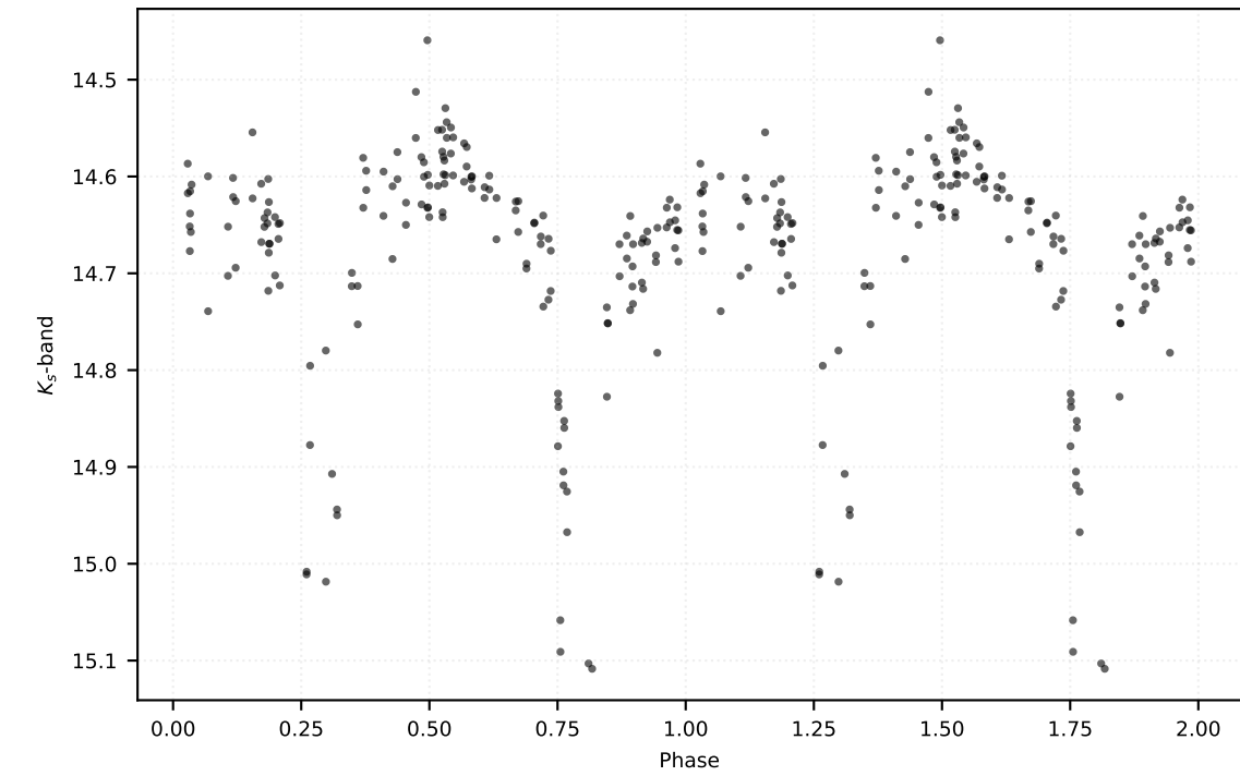
P: 3.71280 d | Class: EB | Subclass: EA | Field b278
