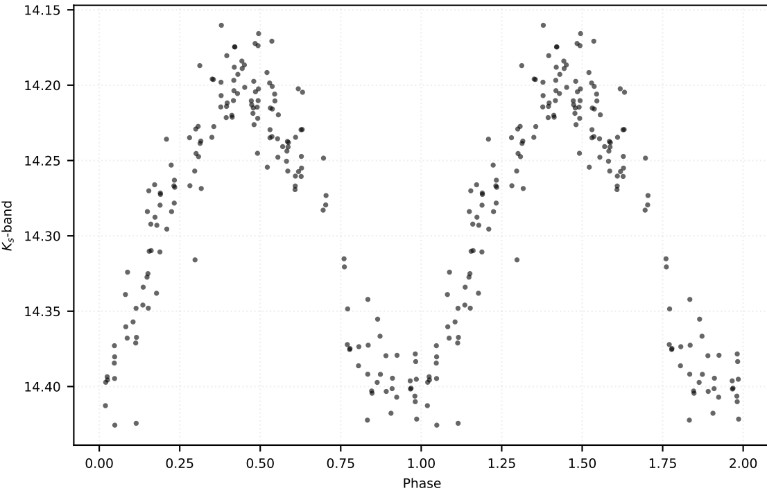
P: 1.01636 d | Class: EB | Subclass: RRc | Field b278
