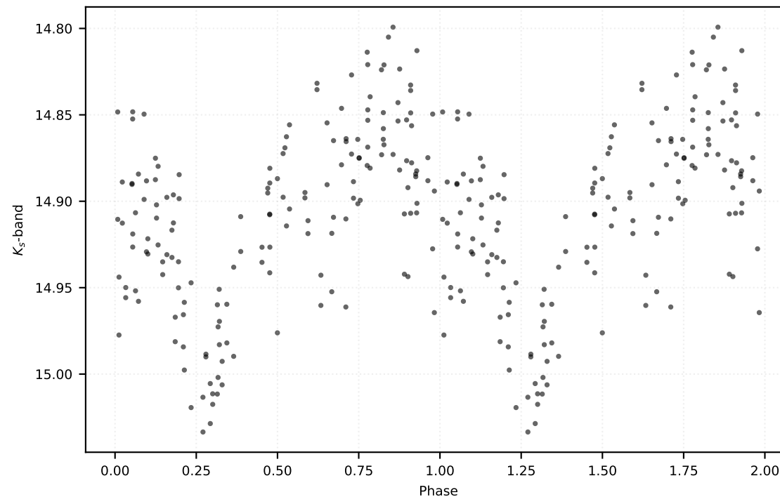
P: 2.44669 d | Class: RP | Subclass: CEP-10T | Field b279
