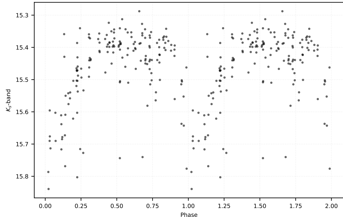
P: 0.52874 d | Class: RP | Subclass: CEP-1OT | Field b278
