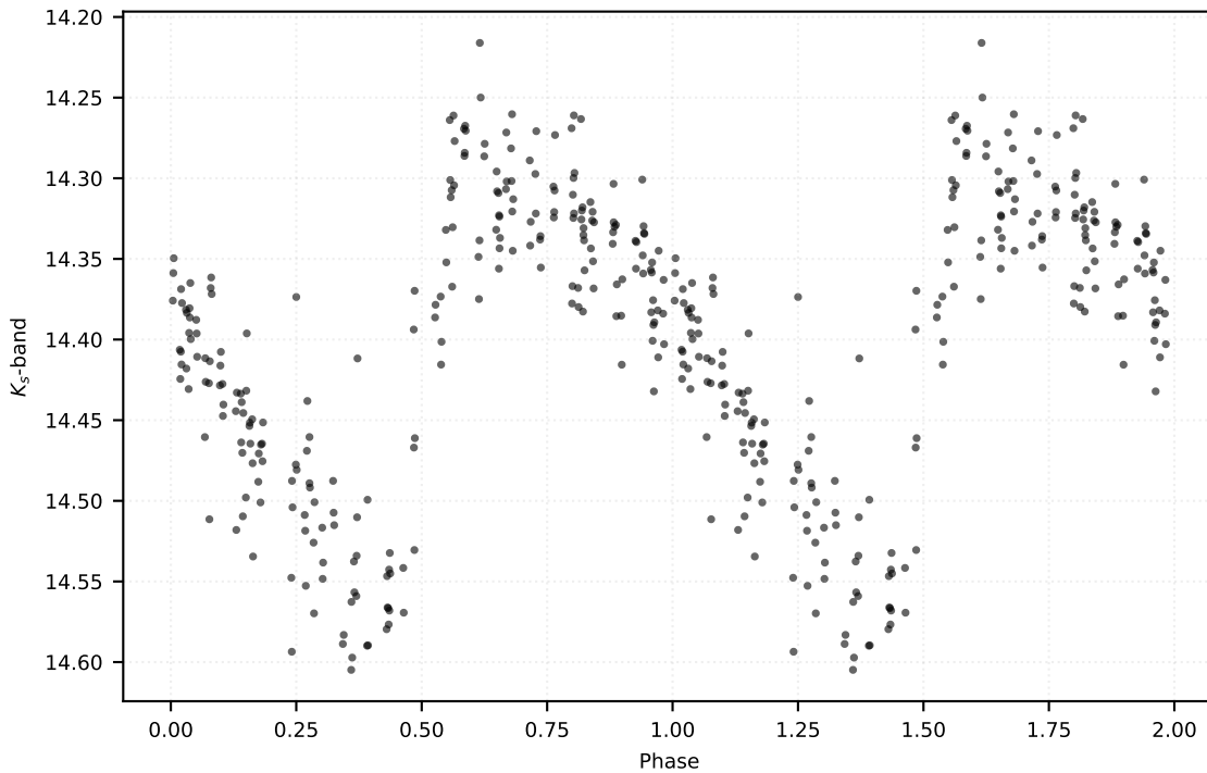
P: 0.46511 d | Class: RP | Subclass: RRc | Field b278
