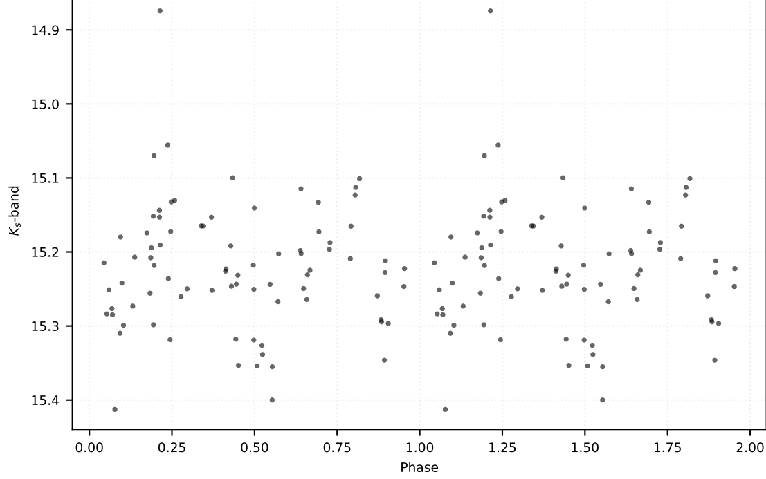
P: 0.22538 d | Class: EB | Subclass: EA | Field b278
