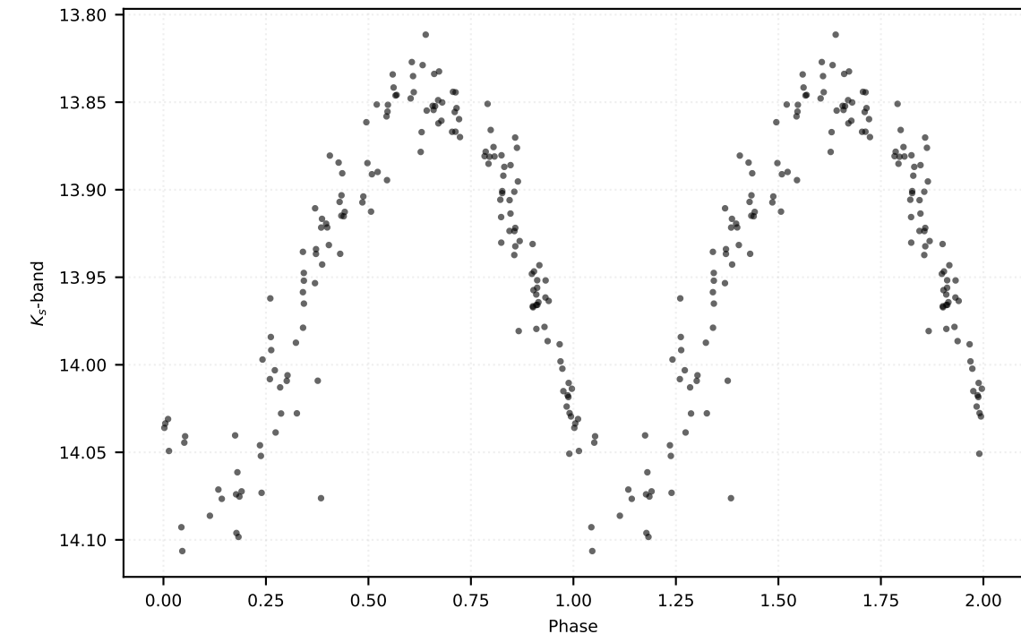
P: 0.21365 d | Class: RP | Subclass: UVAR | Field b279
