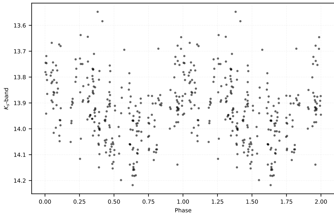
P: 0.63023 d | Class: RP | Subclass: RRab | Field b278
