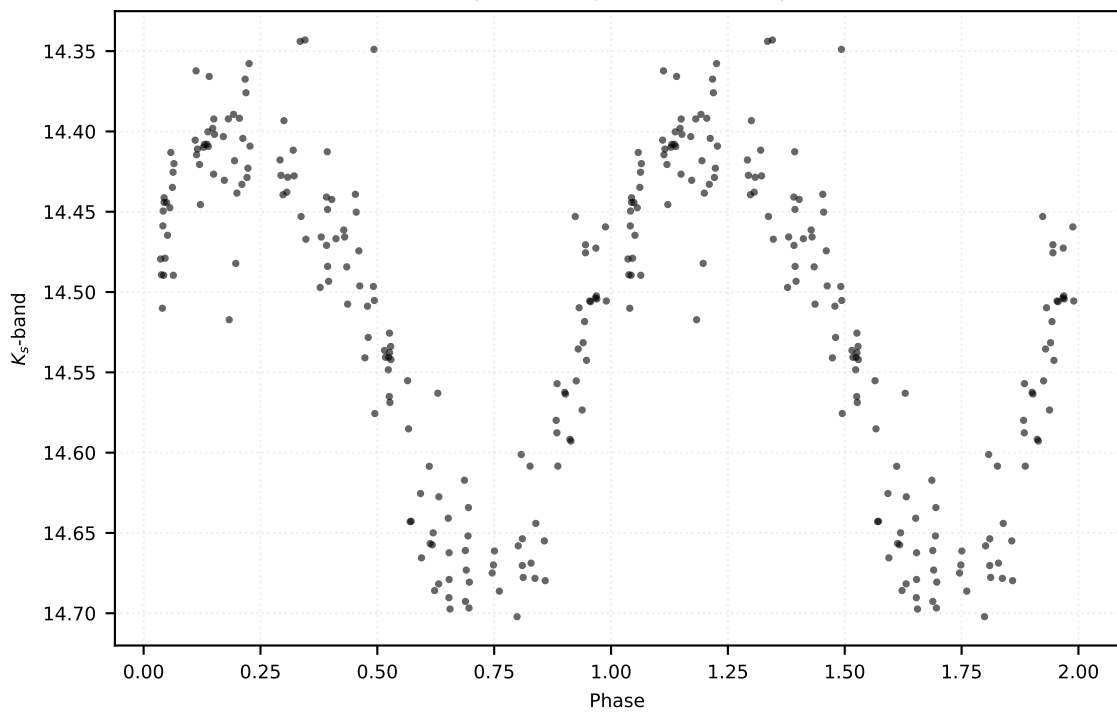
P: 0.18546 d | Class: RP | Subclass: UVAR | Field b278
