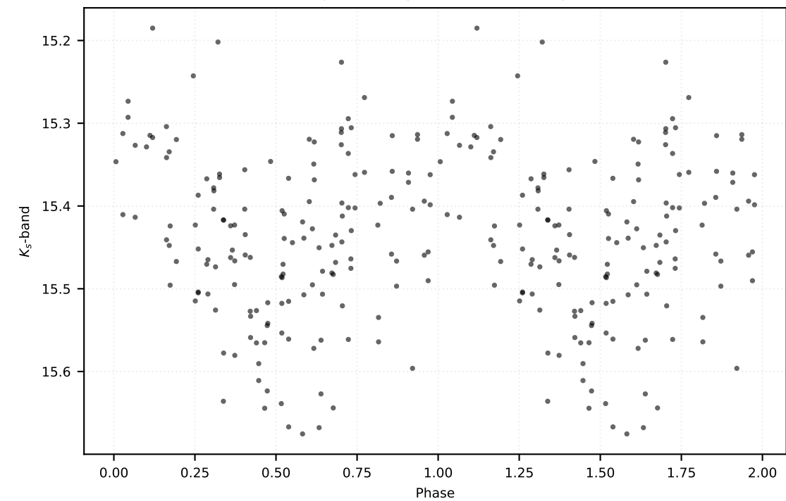
P: 0.99558 d | Class: RP | Subclass: CEP-1OT | Field b278
