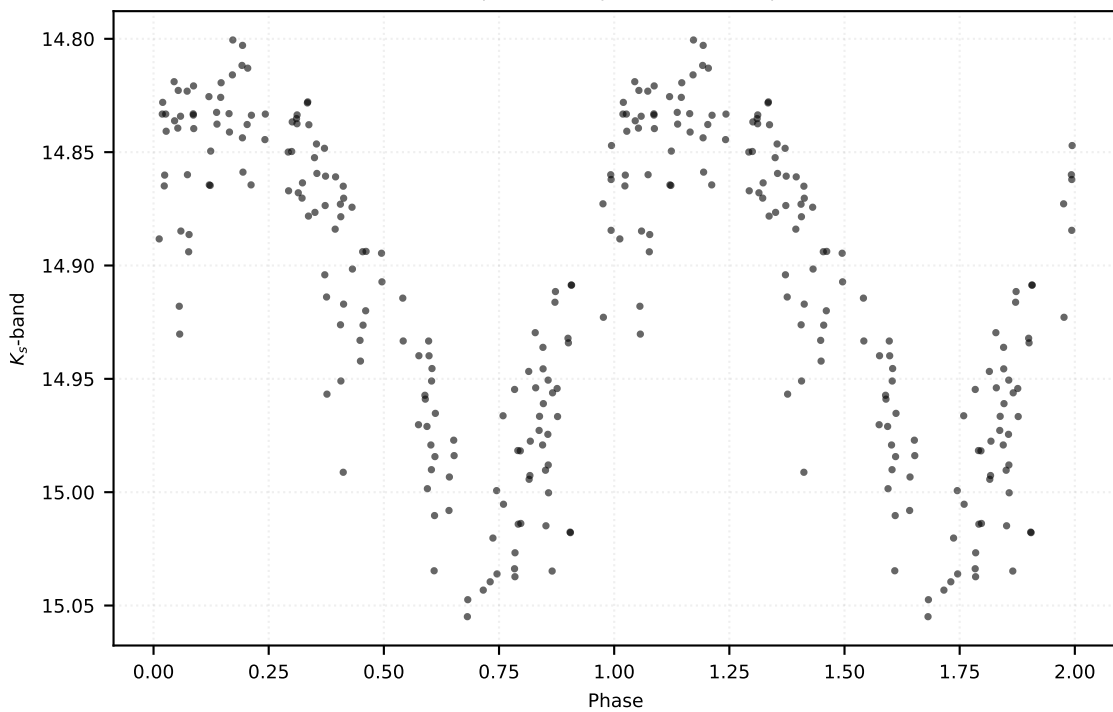
P: 0.96930 d | Class: EB | Subclass: RRc | Field b279
