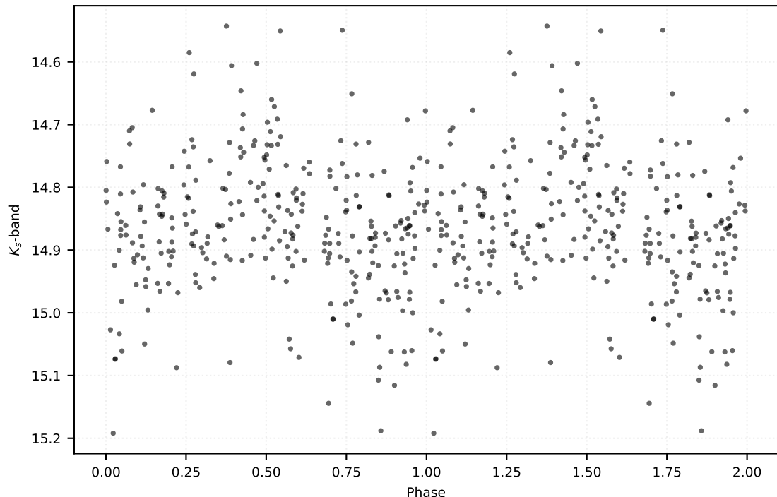
P: 0.51324 d | Class: RP | Subclass: RRab | Field b278
