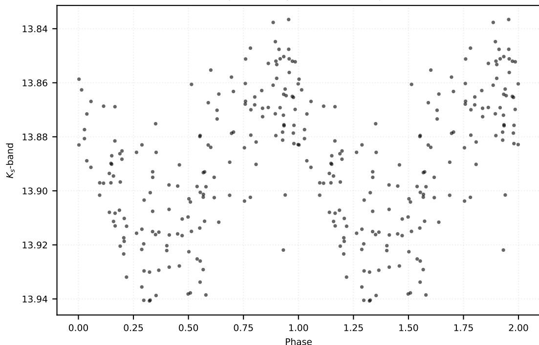
P: 3.63338 d | Class: RP | Subclass: CEP-F | Field b278
