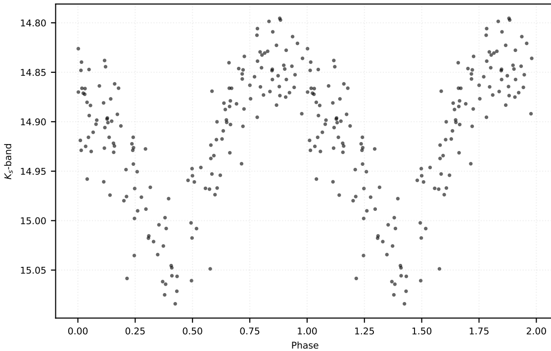
P: 0.48951 d | Class: RP | Subclass: RRab | Field b279
