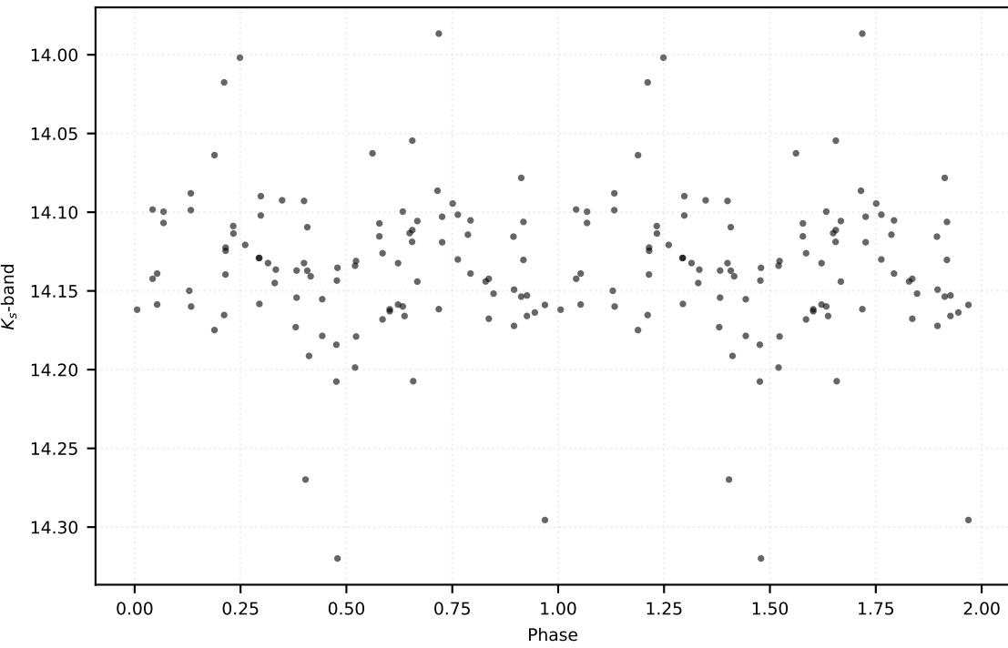
P: 12.48828 d | Class: EB | Subclass: EA | Field b279
