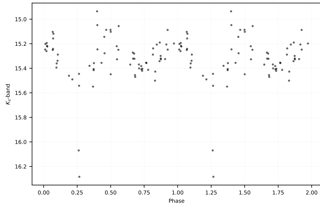
P: 3.19112 d | Class: EB | Subclass: EA | Field b278
