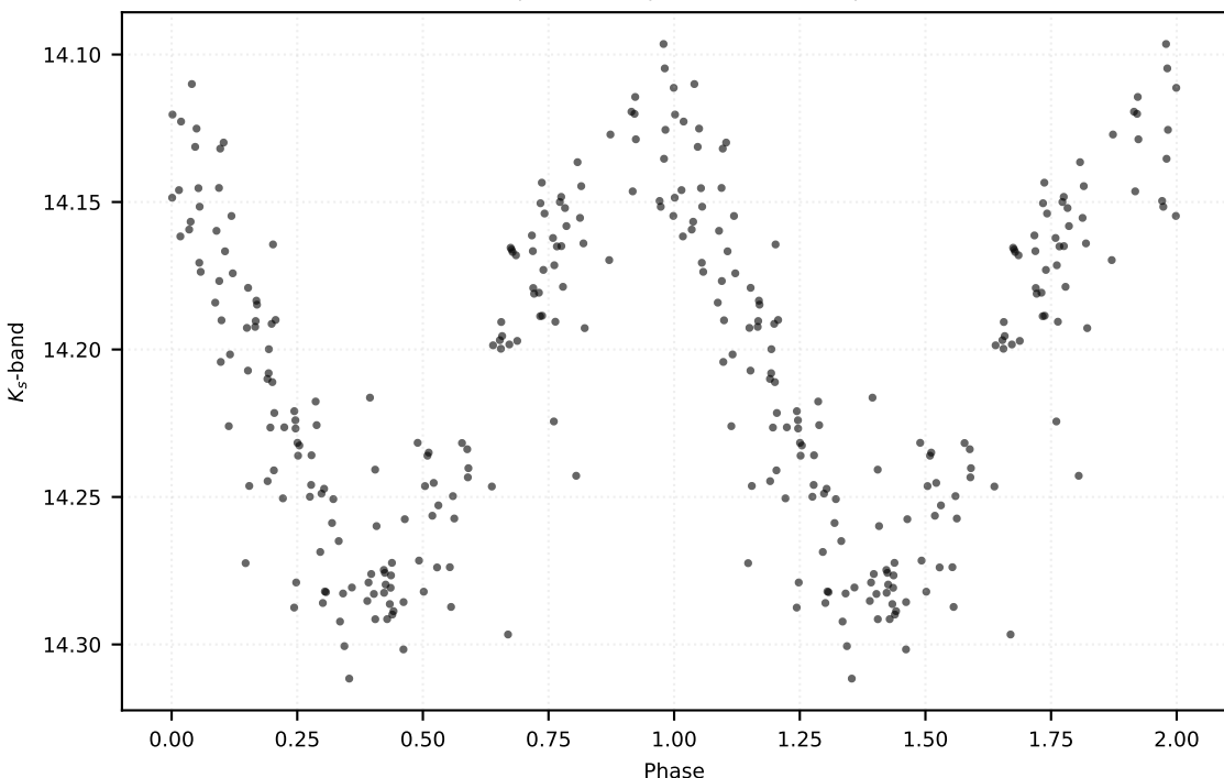
P: 0.19095 d | Class: RP | Subclass: UVAR | Field b278
