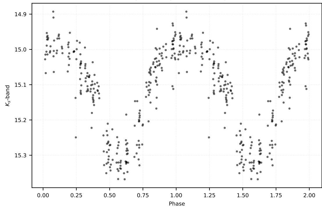
P: 0.18830 d | Class: RP | Subclass: UVAR | Field b278
