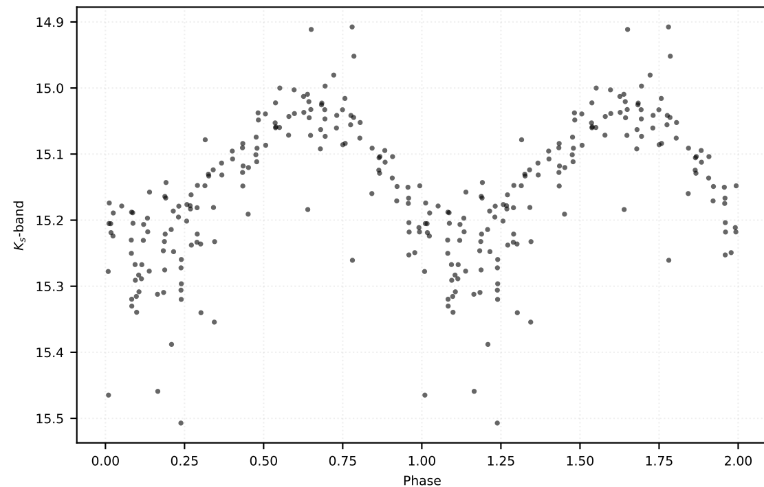
P: 0.60829 d | Class: RP | Subclass: CEP-10T | Field b279
