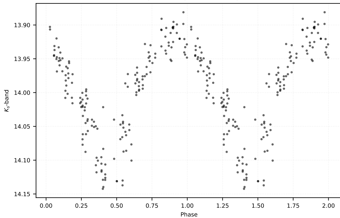
P: 1.11445 d | Class: EB | Subclass: RRc | Field b278
