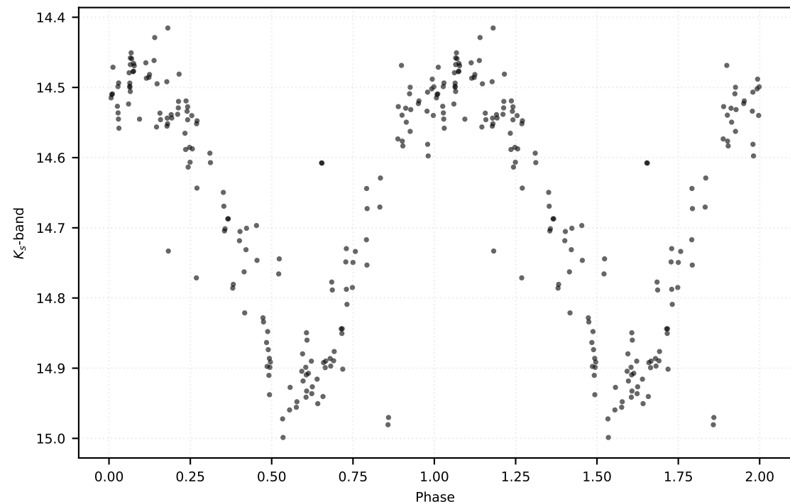
P: 0.21180 d | Class: RP | Subclass: UVAR | Field b278
