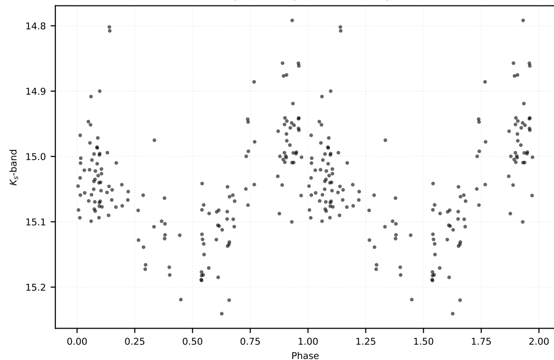
P: 0.24931 d | Class: RP | Subclass: UVAR | Field b278
