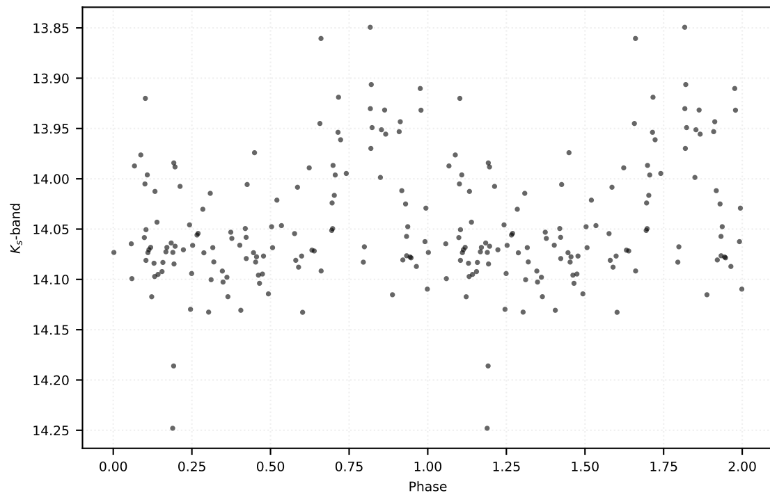
P: 0.11355 d | Class: RP | Subclass: UVAR | Field b278
