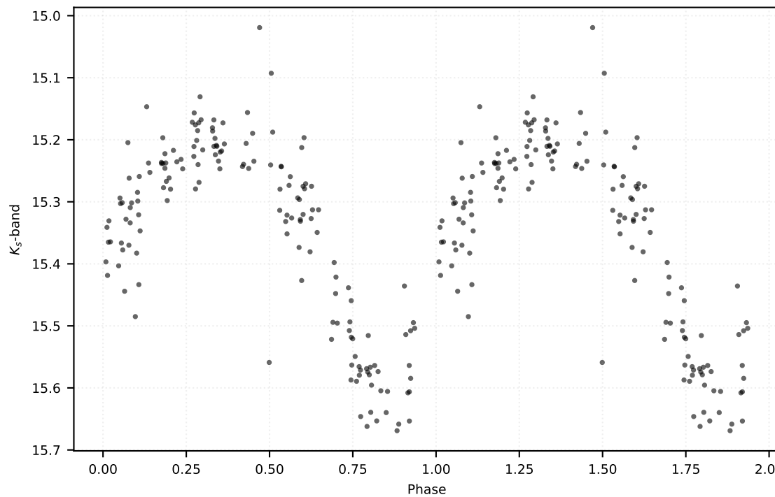
P: 0.14710 d | Class: RP | Subclass: UVAR | Field b279
