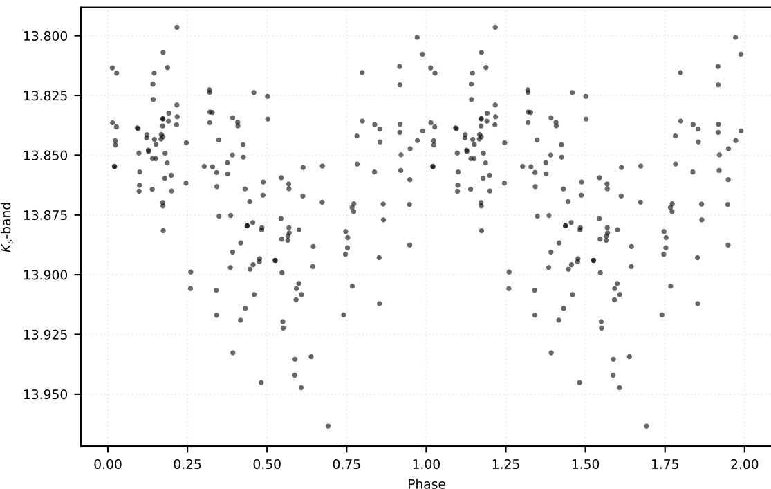
P: 0.99795 d | Class: RP | Subclass: RRab | Field b279
