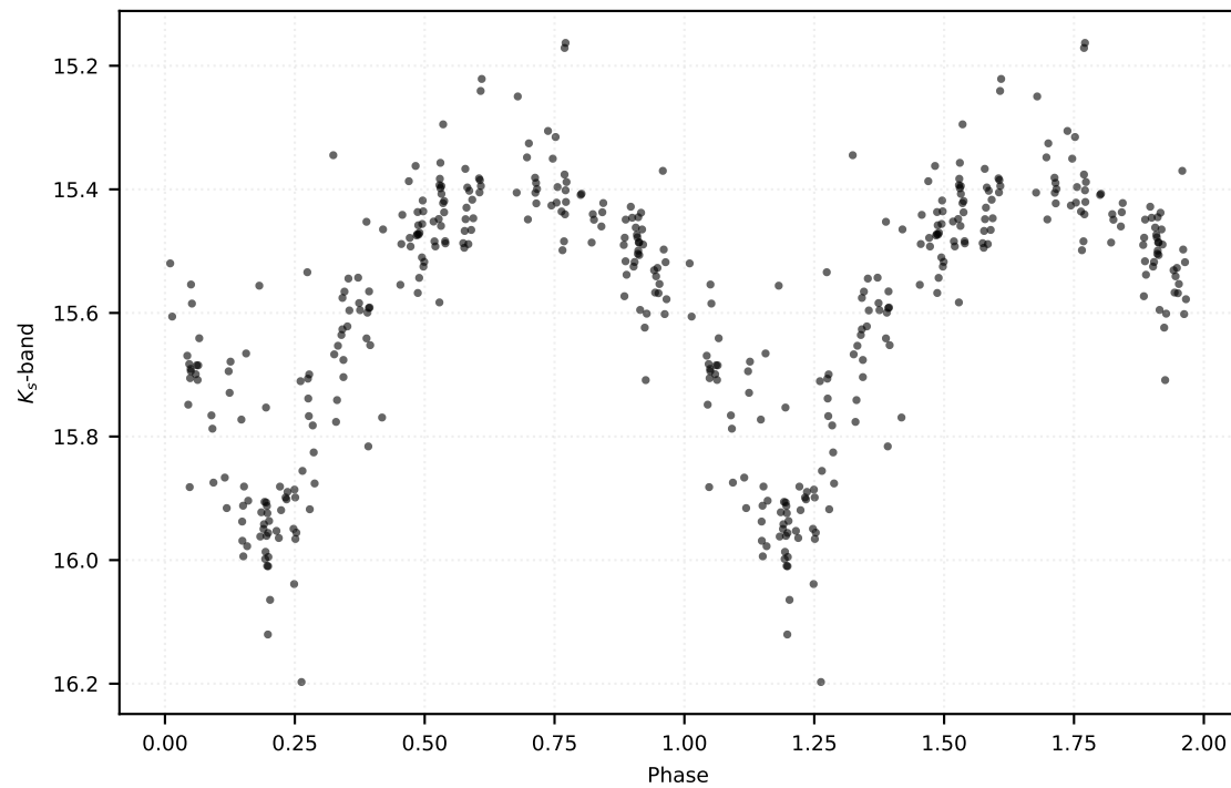
P: 1.00103 d | Class: EB | Subclass: UVAR | Field b279
