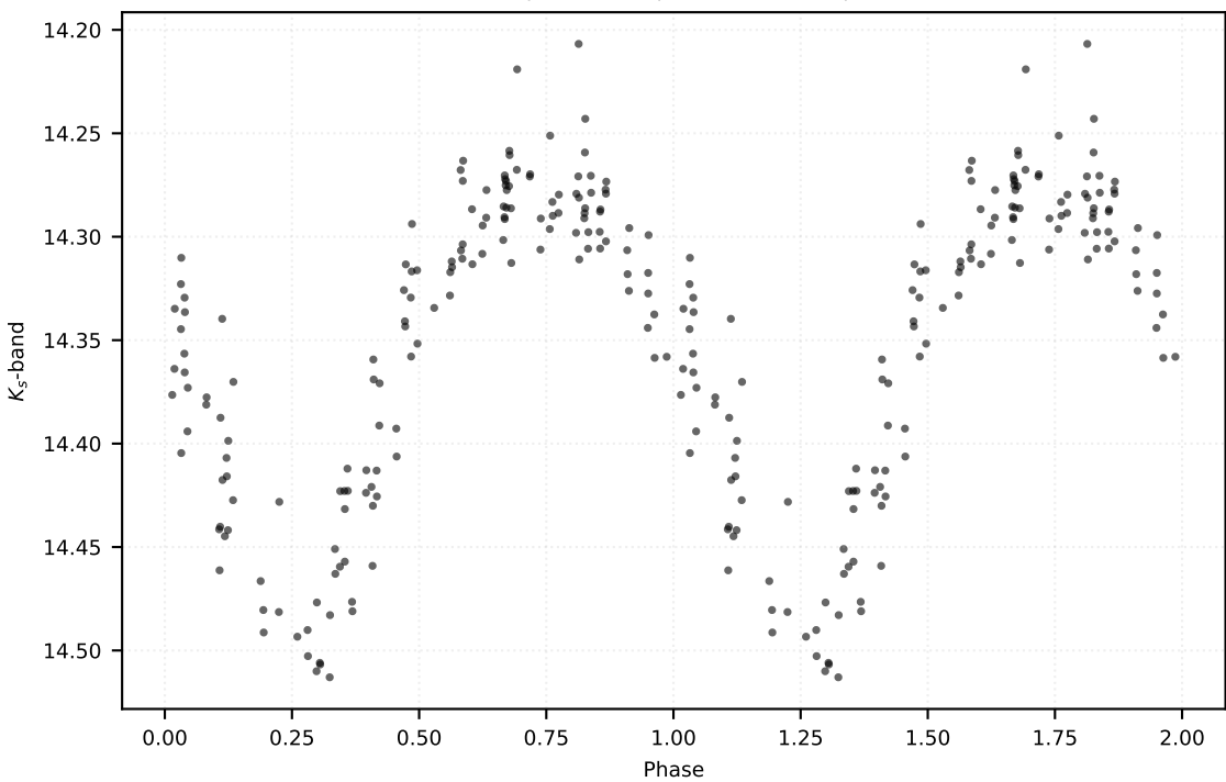
P: 0.53595 d | Class: RP | Subclass: RRc | Field b278
