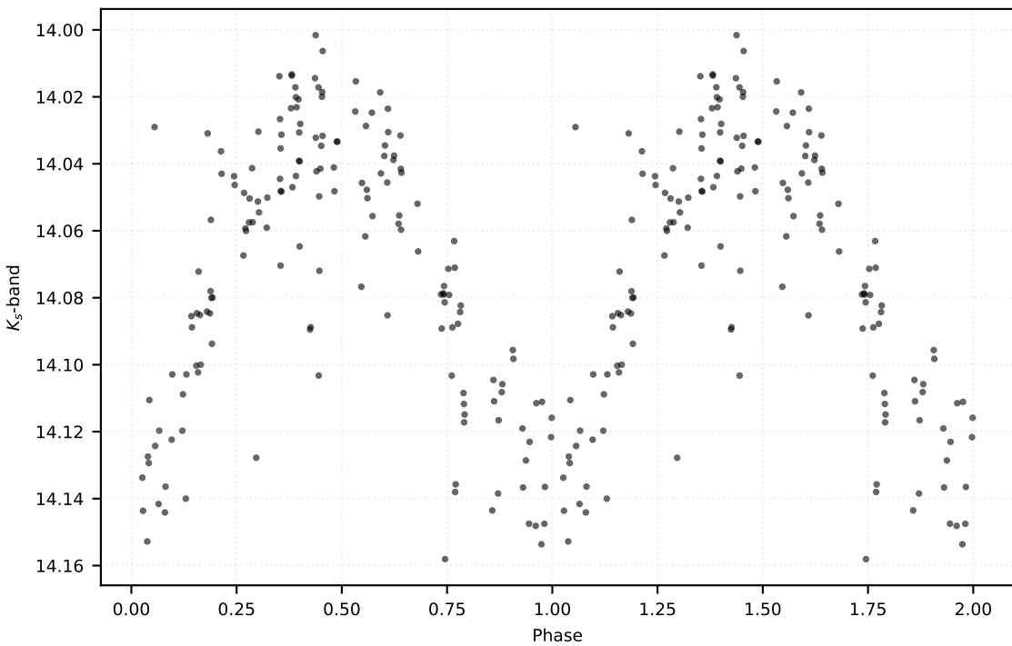
P: 0.16756 d | Class: RP | Subclass: UVAR | Field b279
