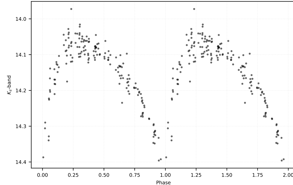
P: 0.52009 d | Class: RP | Subclass: RRab | Field b278
