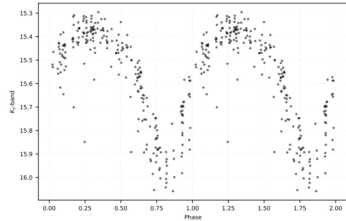
P: 0.22017 d | Class: RP | Subclass: UVAR | Field b278
