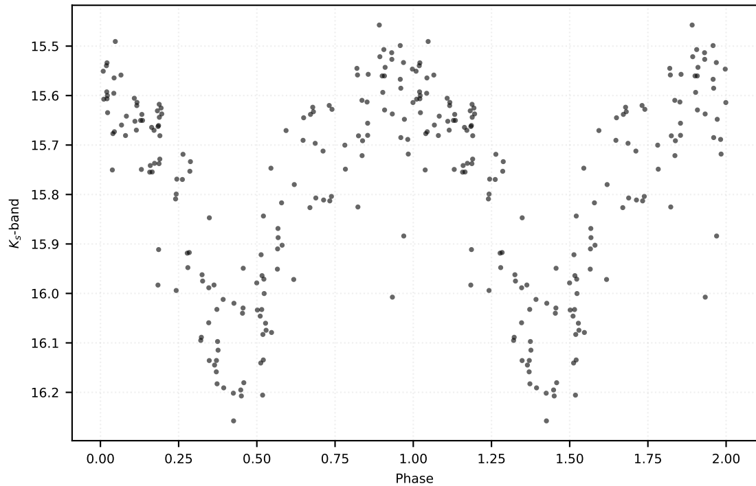
P: 1.08915 d | Class: EB | Subclass: RRc | Field b279
