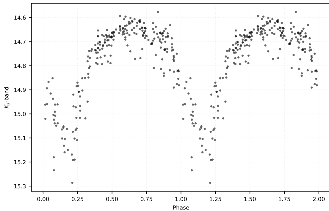
P: 0.47208 d | Class: RP | Subclass: RRab | Field b279
