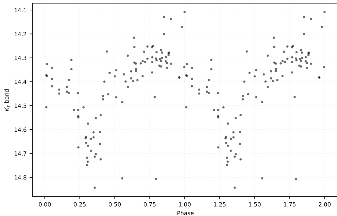
P: 4.89185 d | Class: RP | Subclass: CEP-F | Field b278
