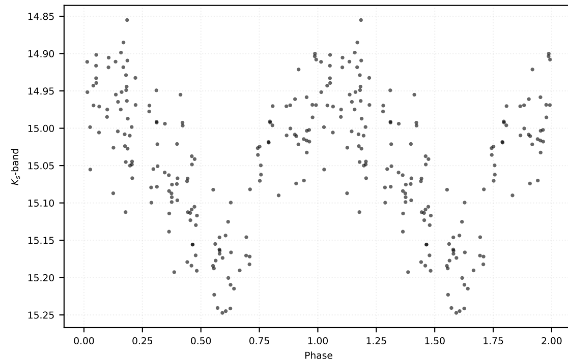
P: 0.99724 d | Class: RP | Subclass: RRab | Field b279
