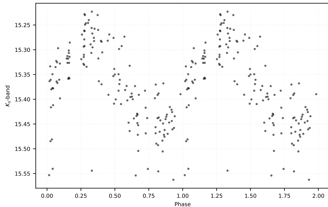
P: 0.15426 d | Class: RP | Subclass: UVAR | Field b279
