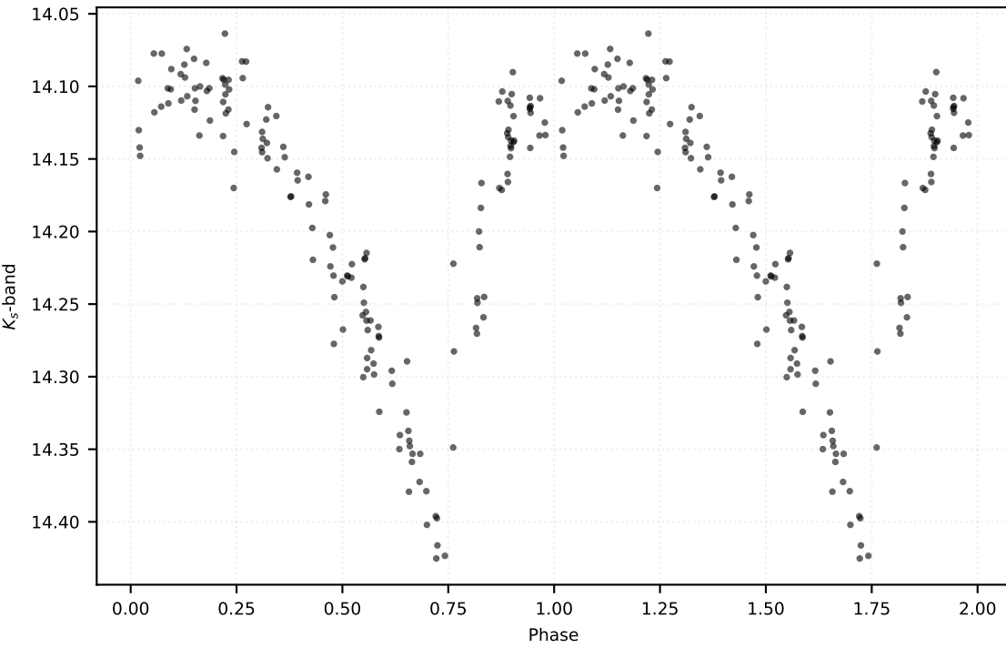
P: 0.60516 d | Class: RP | Subclass: RRab | Field b279
