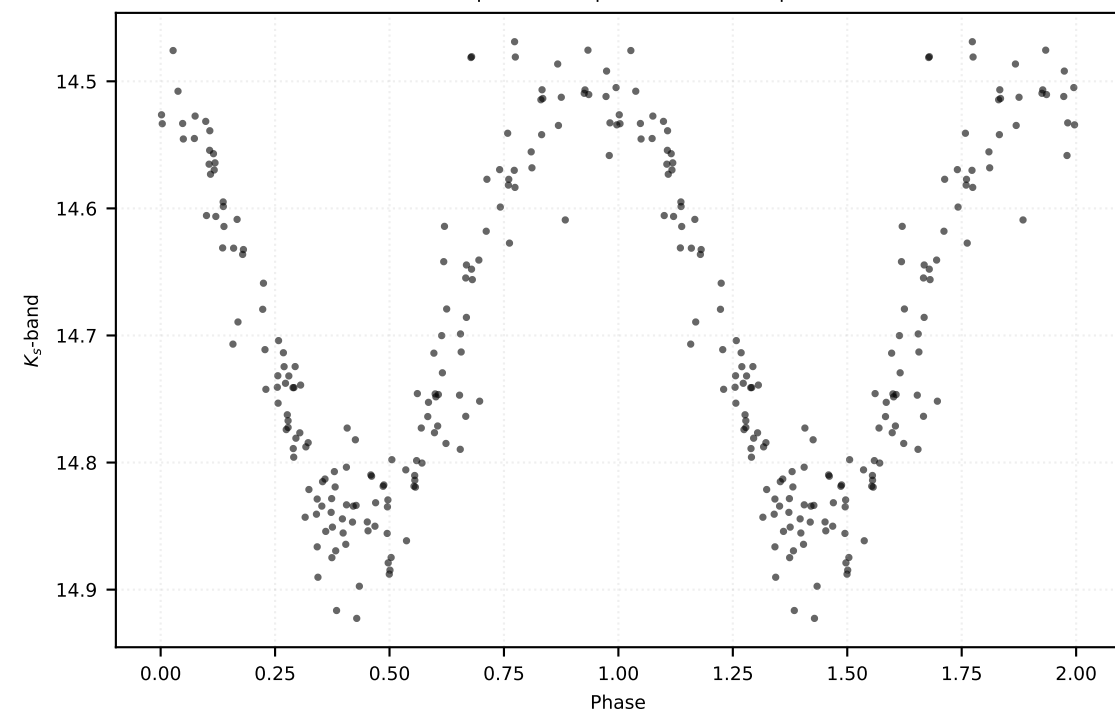
P: 0.48536 d | Class: RP | Subclass: RRab | Field b278
