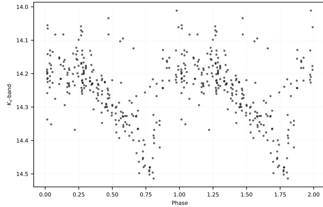
P: 0.49321 d | Class: RP | Subclass: RRab | Field b278
