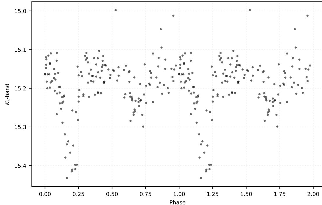
P: 0.21083 d | Class: EB | Subclass: EA | Field b279
