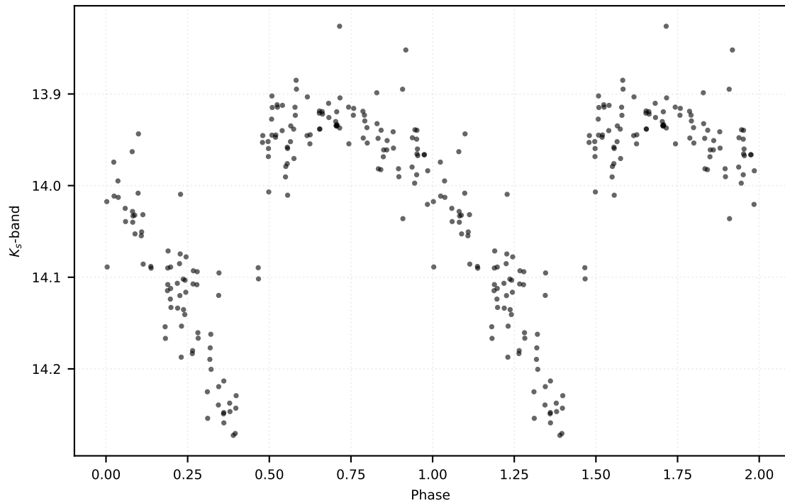
P: 0.64121 d | Class: RP | Subclass: RRab | Field b278
