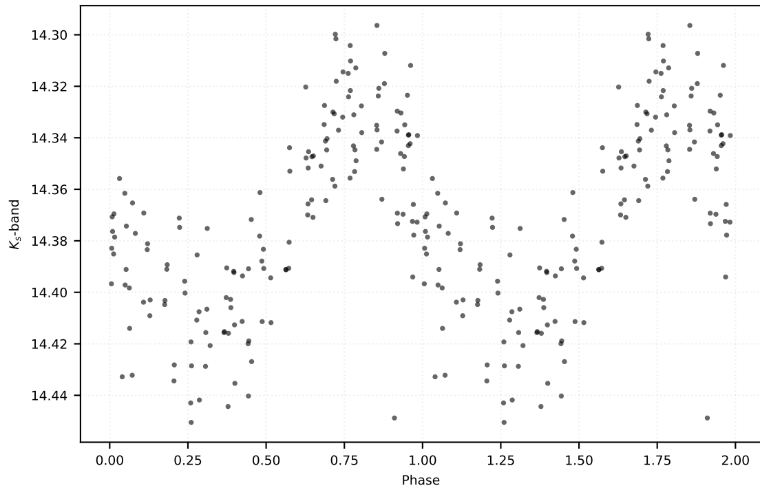
P: 9.03023 d | Class: RP | Subclass: CEP-10T | Field b278
