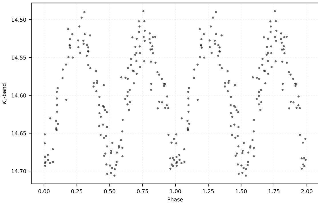
P: 0.40574 d | Class: RP | Subclass: RRc | Field b278
