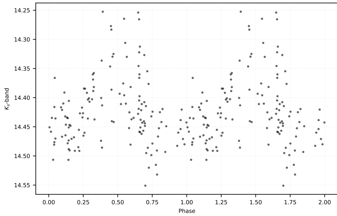
P: 0.10752 d | Class: RP | Subclass: UVAR | Field b279
