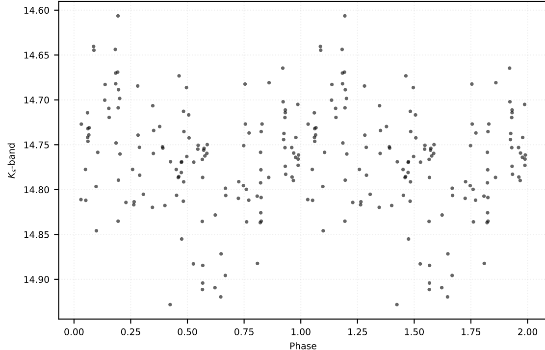
P: 0.28150 d | Class: RP | Subclass: RRc | Field b279
