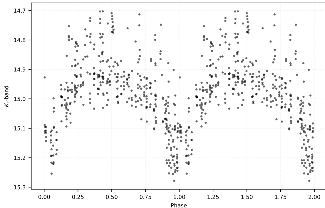
P: 0.61088 d | Class: RP | Subclass: RRab | Field b278
