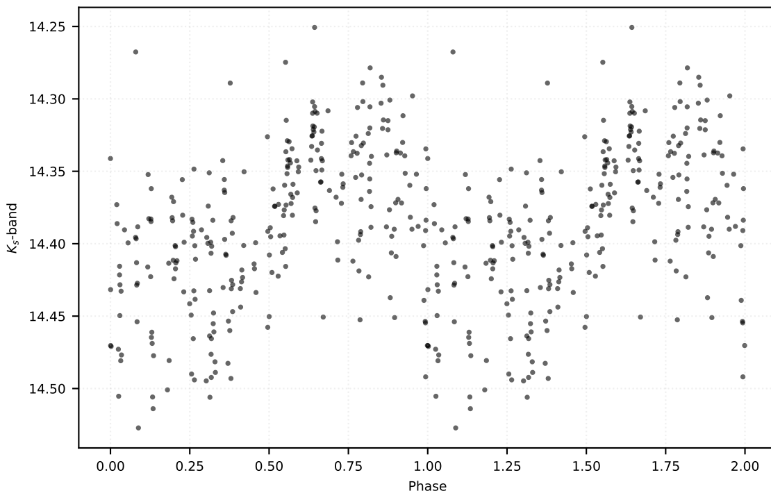
P: 4.40738 d | Class: RP | Subclass: CEP-10T | Field b279
