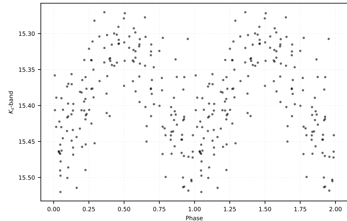
P: 5.70617 d | Class: RP | Subclass: CEP-10T | Field b279
