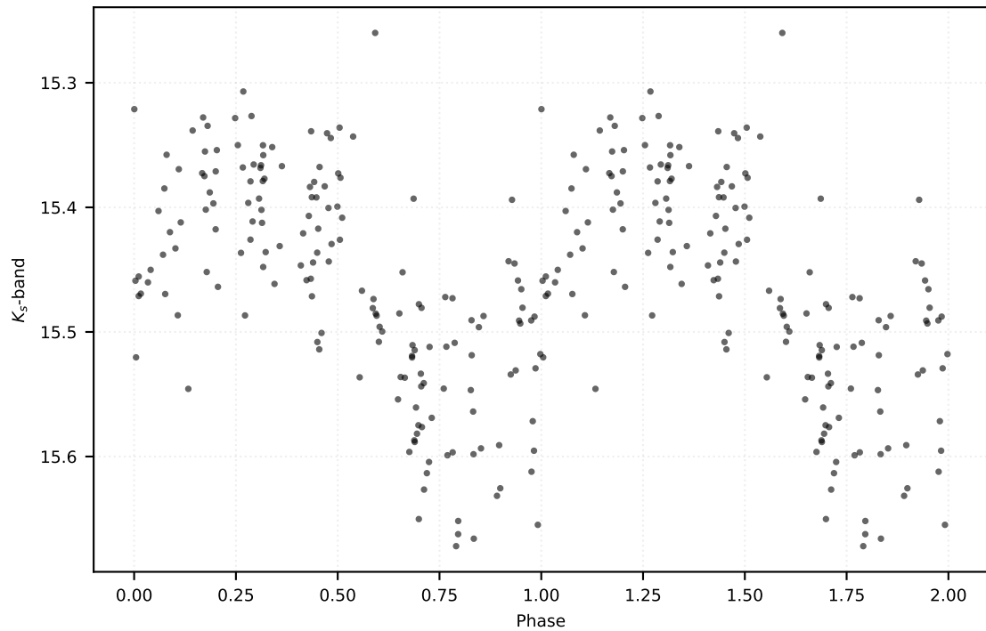
P: 0.20192 d | Class: RP | Subclass: UVAR | Field b279
