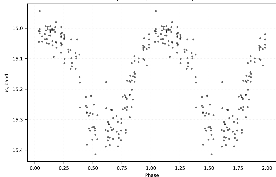
P: 0.77307 d | Class: RP | Subclass: RRab | Field b278
