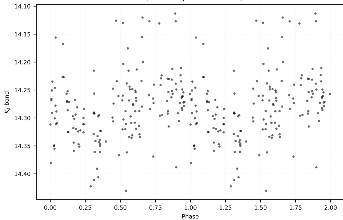
P: 0.14235 d | Class: RP | Subclass: UVAR | Field b279
