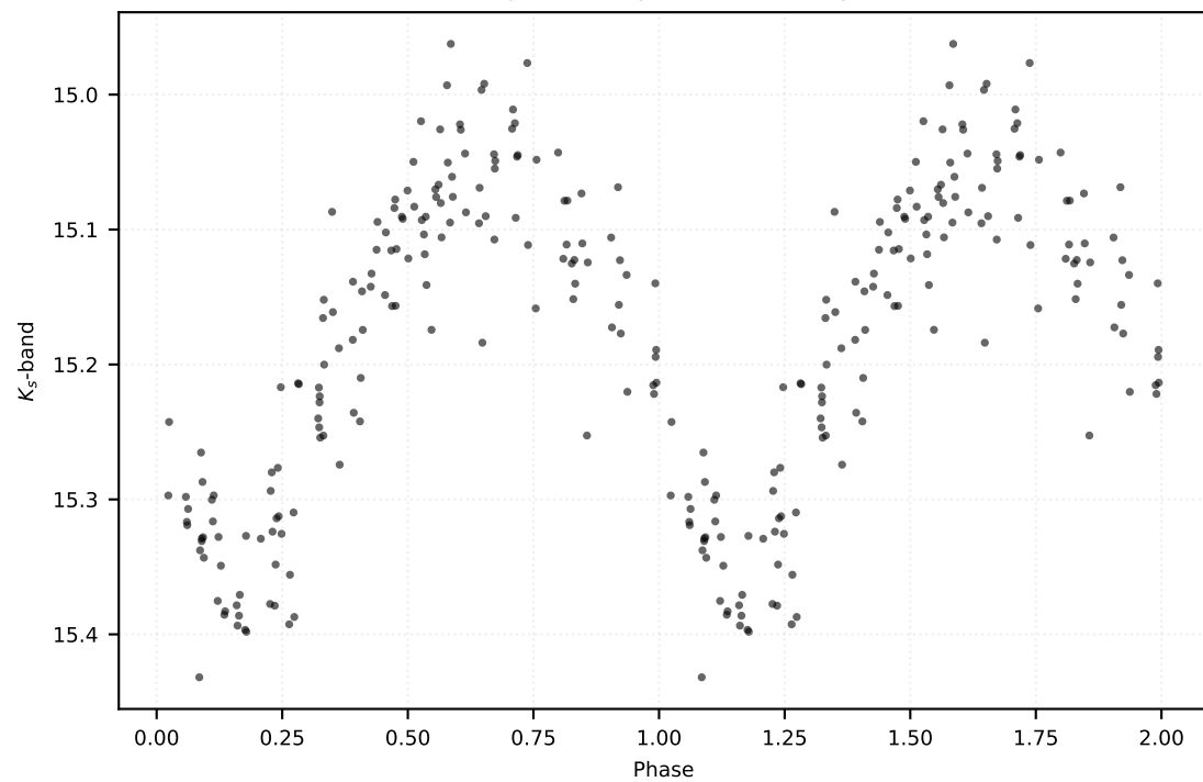
P: 0.47343 d | Class: RP | Subclass: RRab | Field b279
