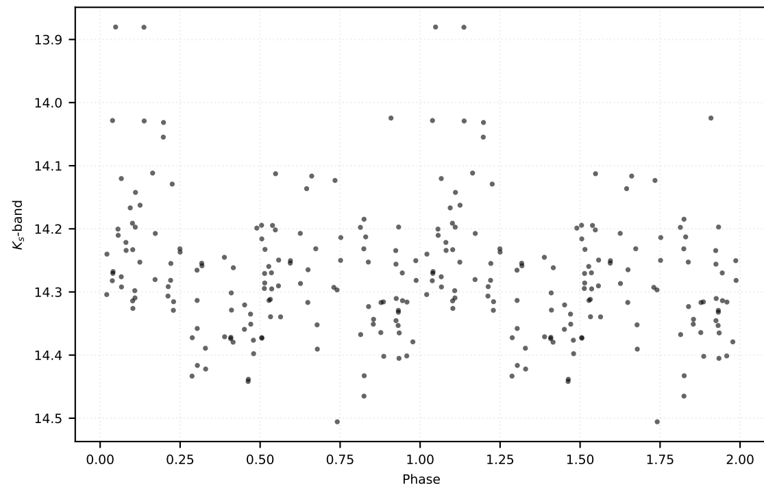
P: 0.27989 d | Class: EB | Subclass: EA | Field b278
