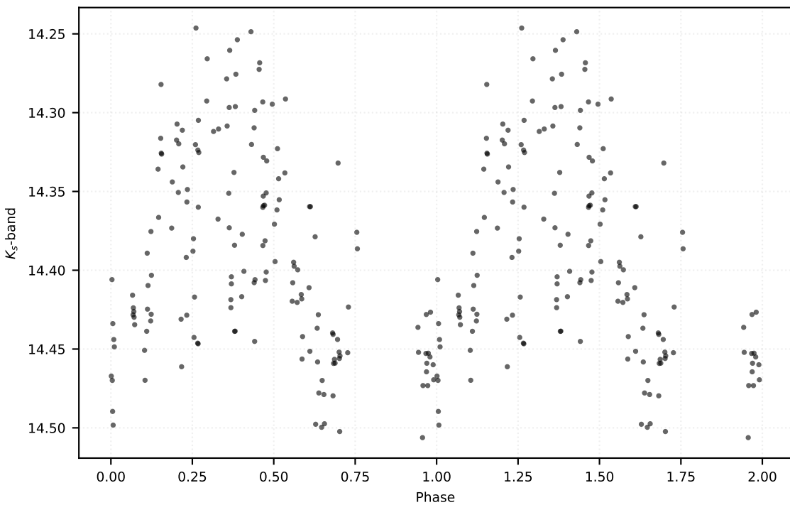
P: 0.28996 d | Class: RP | Subclass: UVAR | Field b279
