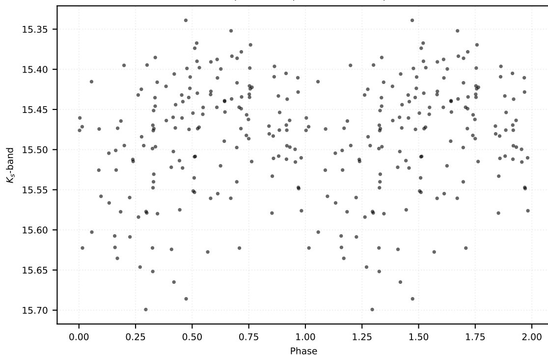
P: 0.32484 d | Class: RP | Subclass: RRab | Field b278
