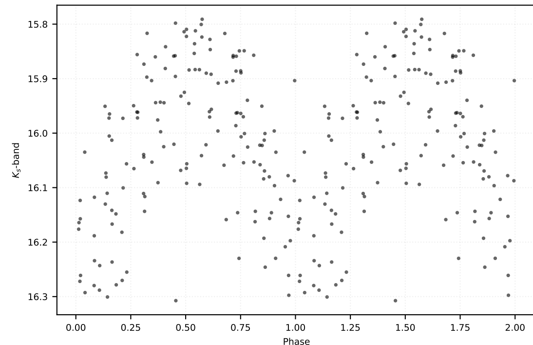
P: 0.54299 d | Class: RP | Subclass: RRc | Field b279
