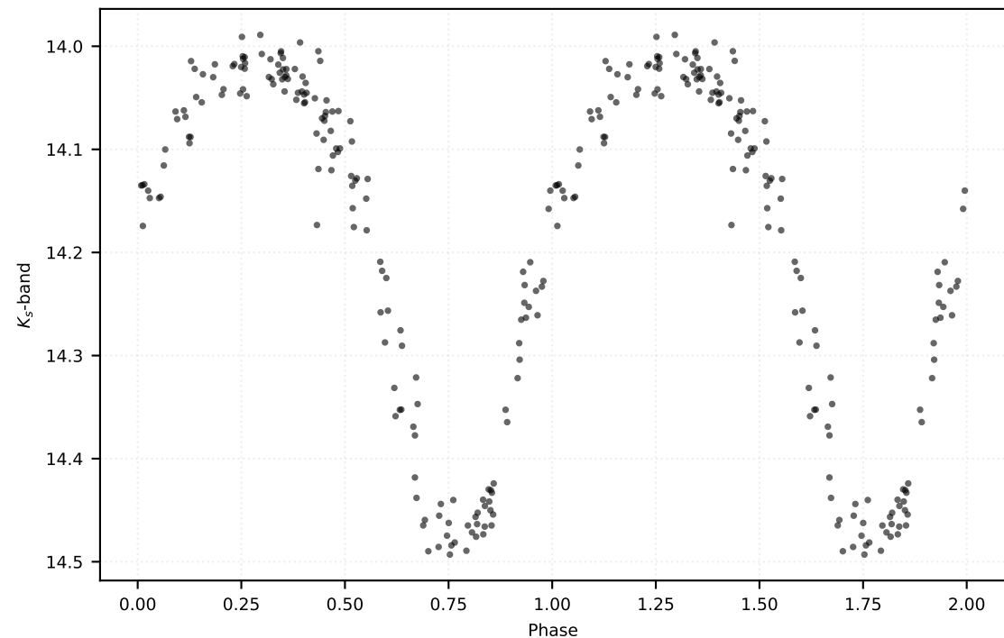
P: 1.01574 d | Class: EB | Subclass: UVAR | Field b278
