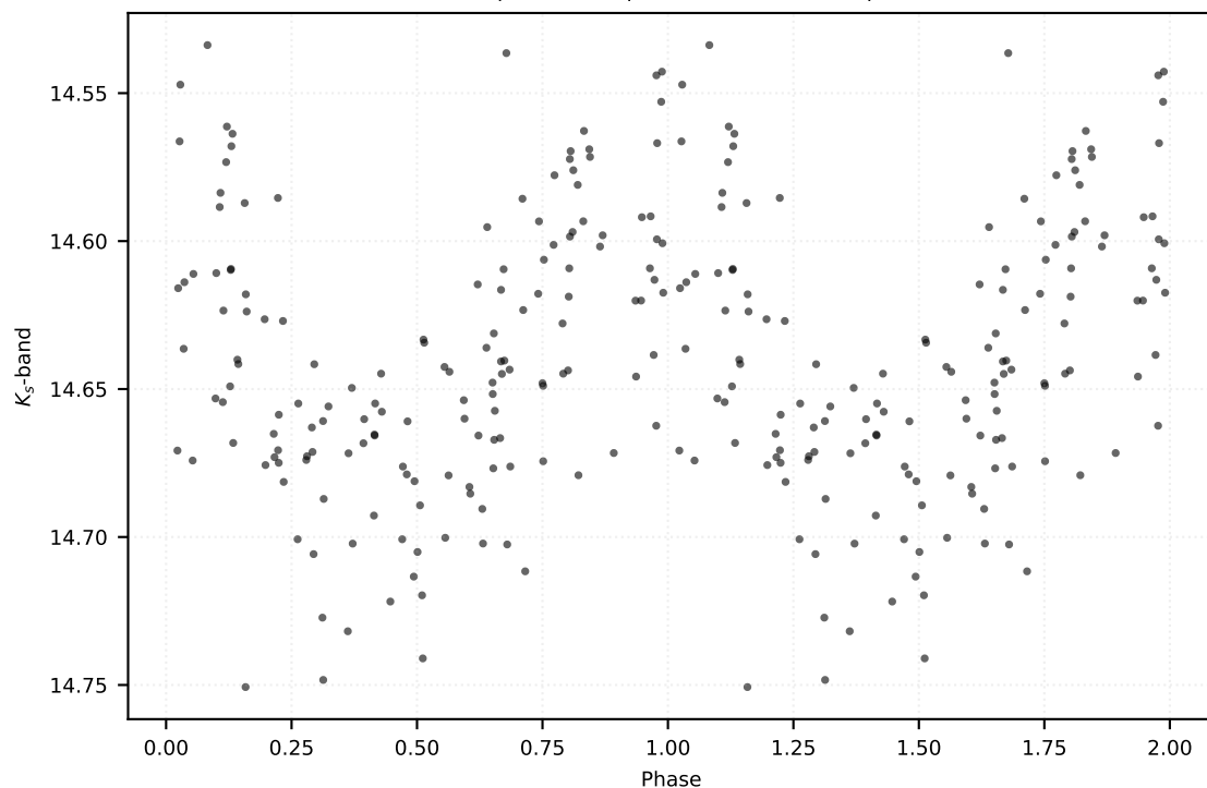
P: 0.35389 d | Class: RP | Subclass: CEP-1OT | Field b279
