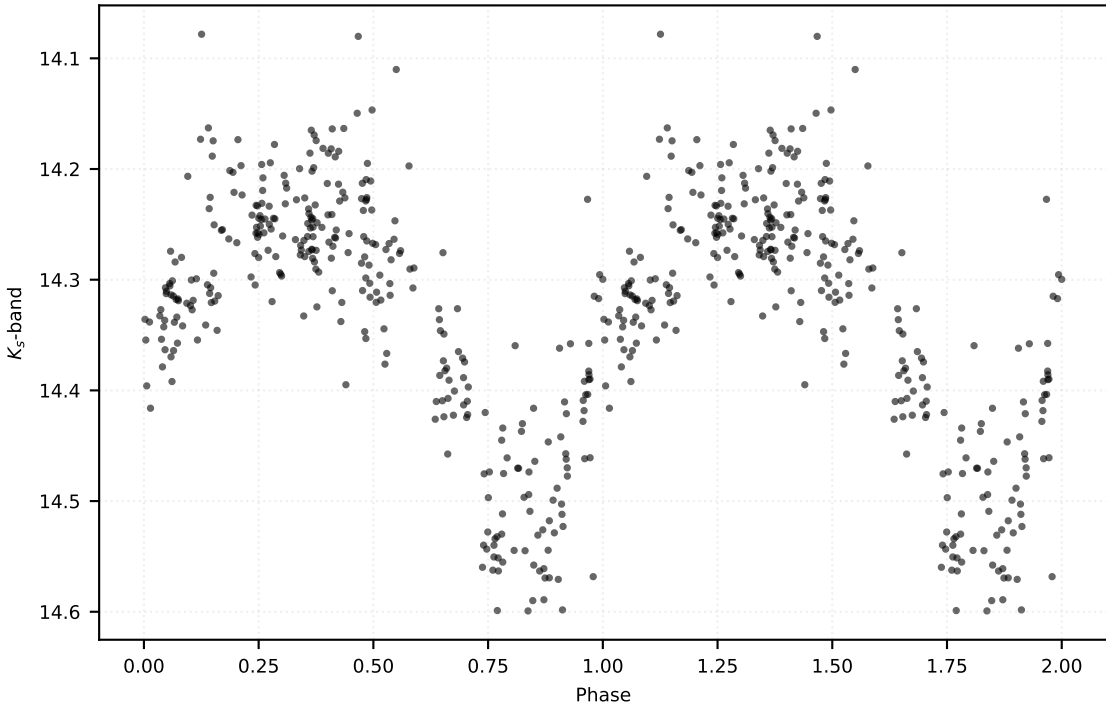
P: 0.29548 d | Class: RP | Subclass: UVAR | Field b278
