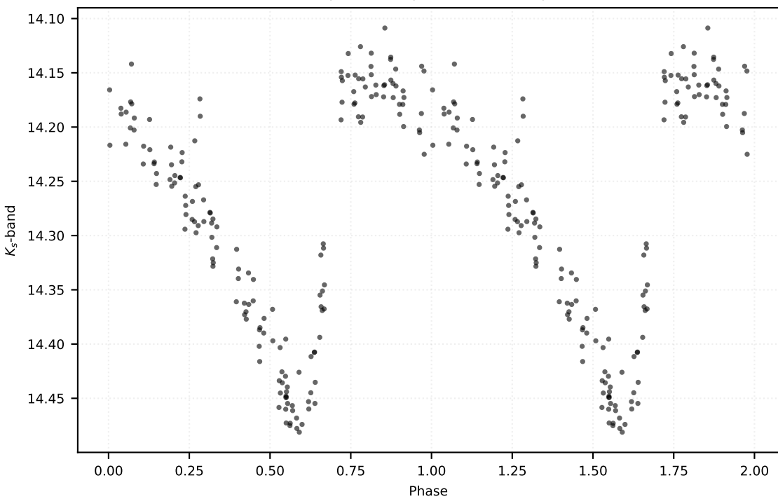
P: 0.53652 d | Class: RP | Subclass: RRab | Field b279
