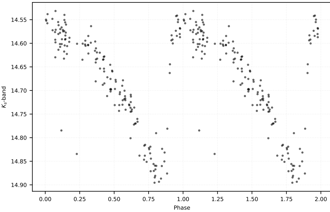
P: 0.44957 d | Class: RP | Subclass: RRab | Field b279
