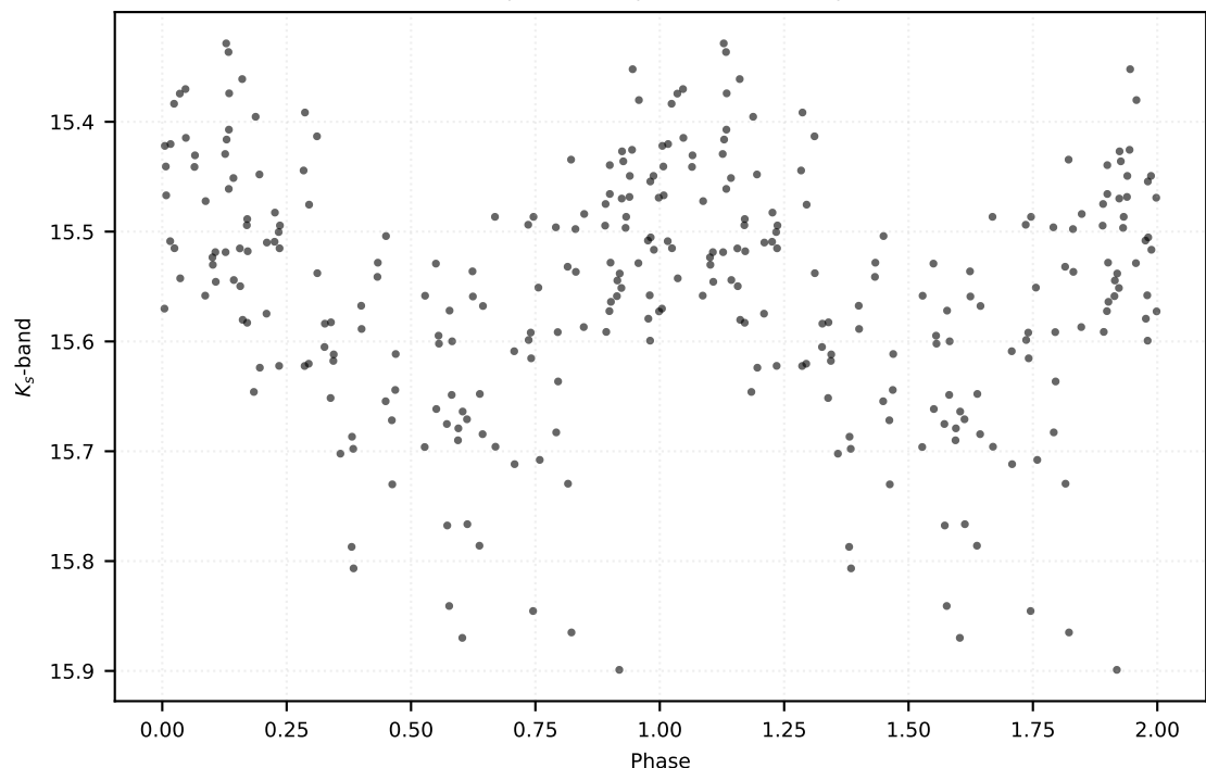
P: 0.50997 d | Class: RP | Subclass: RRab | Field b279
