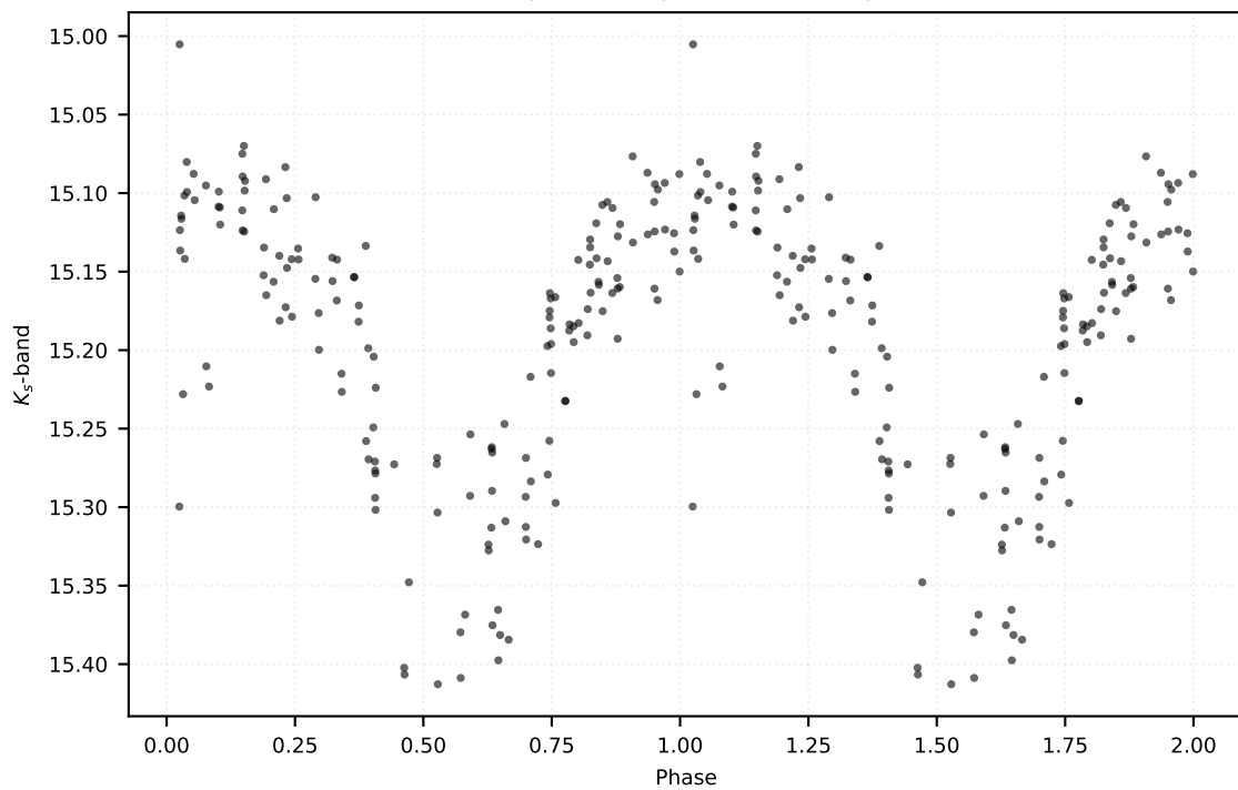
P: 0.35094 d | Class: RP | Subclass: RRab | Field b279
