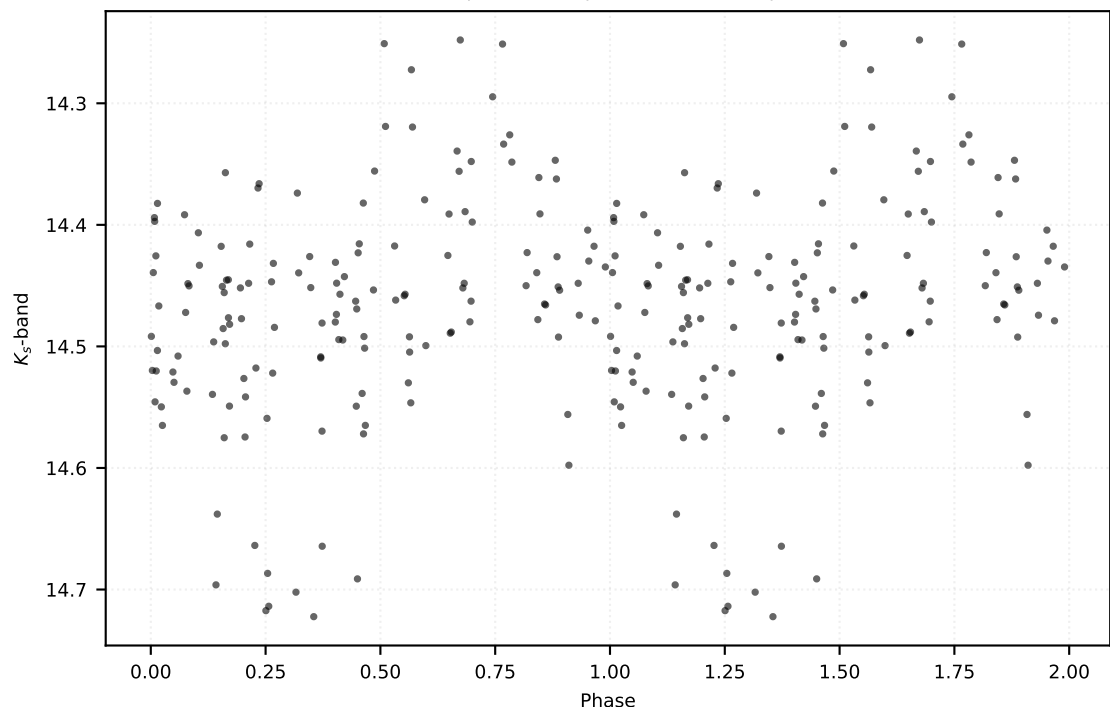
P: 0.50810 d | Class: RP | Subclass: RRab | Field b279
