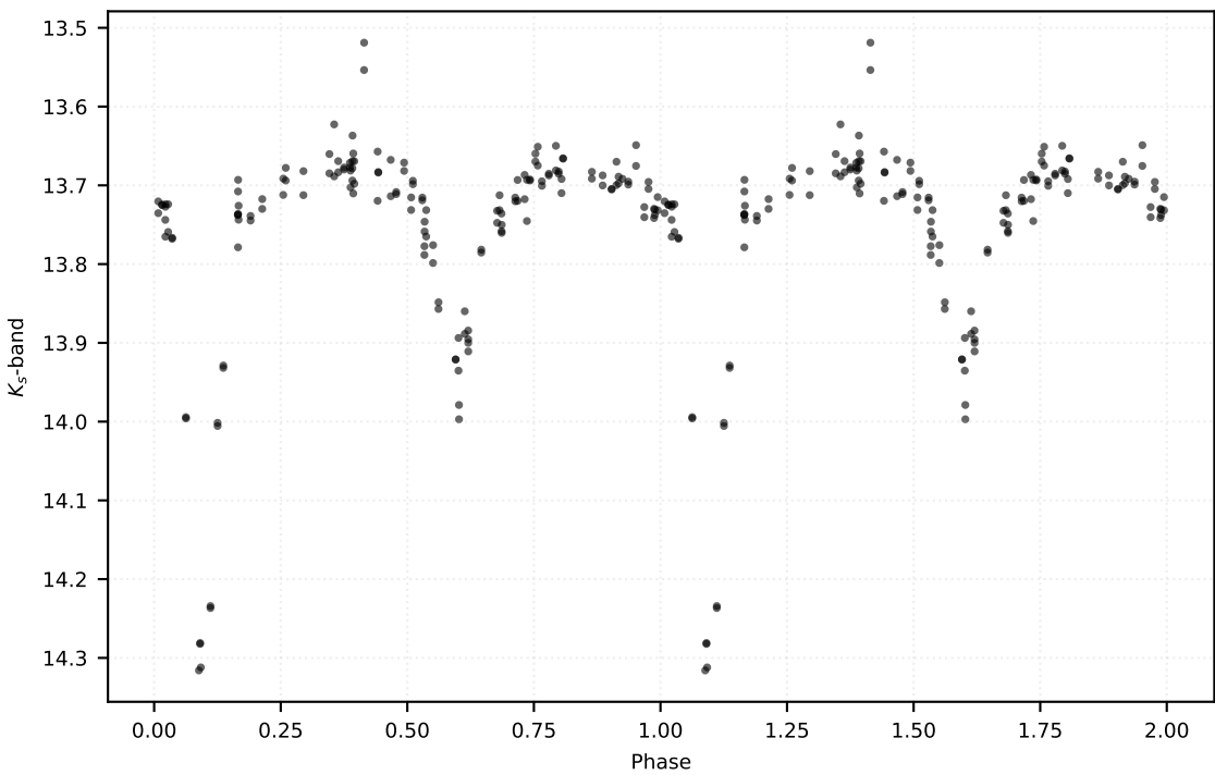
P: 2.40678 d | Class: EB | Subclass: EA | Field b279
