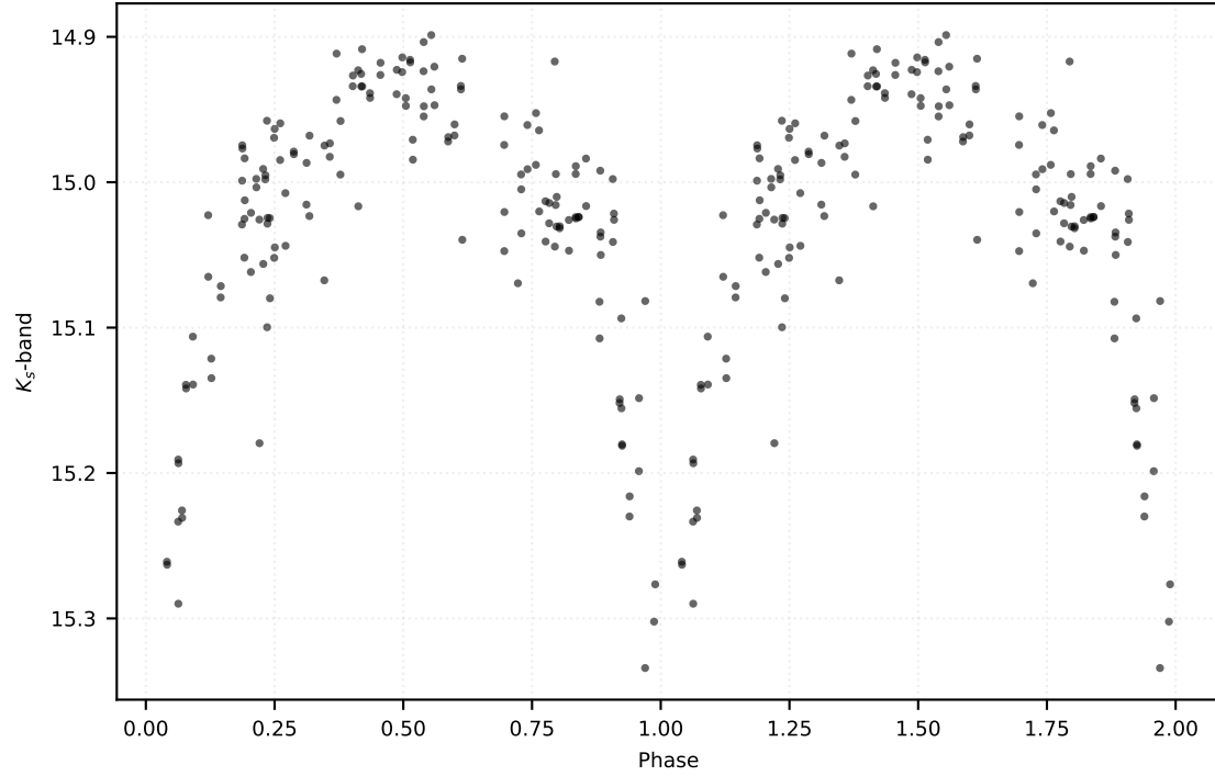
P: 1.49360 d | Class: RP | Subclass: CEP-F | Field b279
