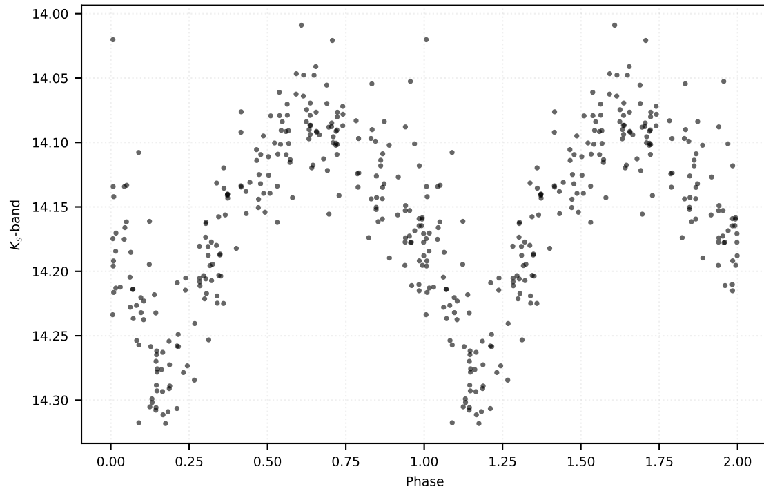
P: 0.33553 d | Class: RP | Subclass: RRab | Field b278
