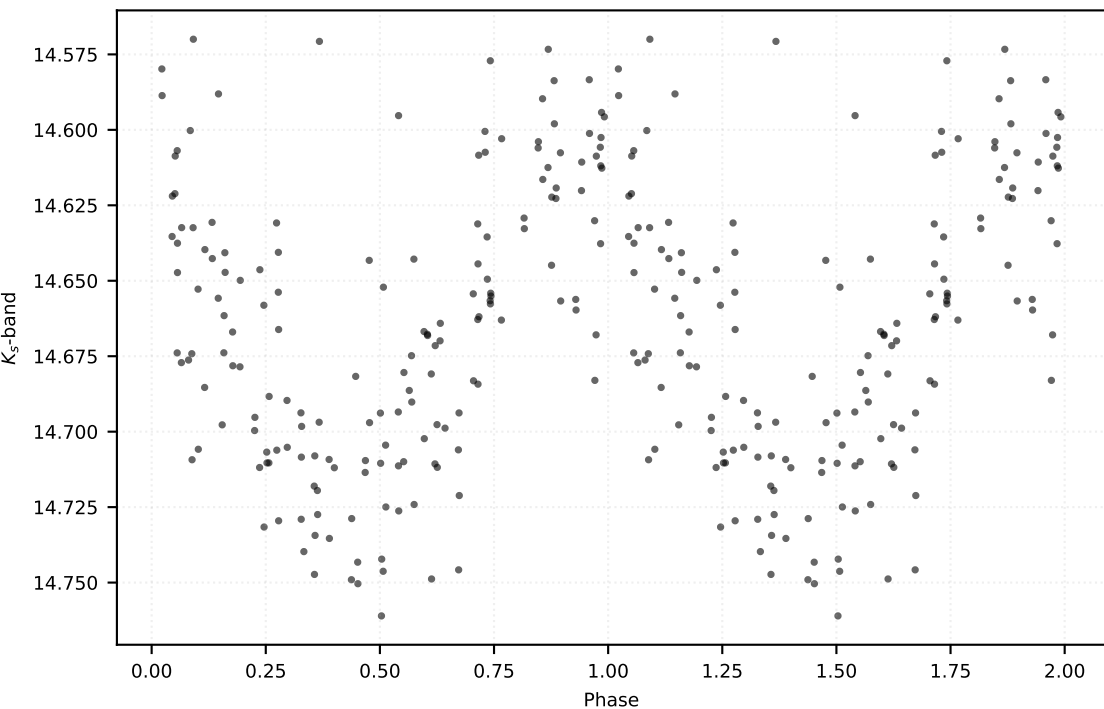
P: 1.57754 d | Class: RP | Subclass: CEP-F | Field b278
