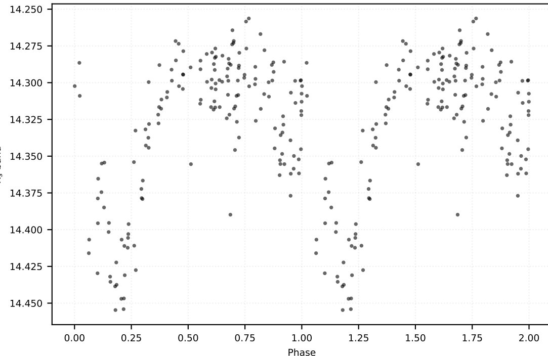
P: 0.43115 d | Class: RP | Subclass: CEP-10T | Field b279
