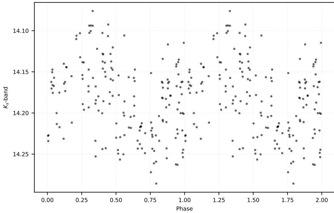
P: 0.26173 d | Class: RP | Subclass: UVAR | Field b279
