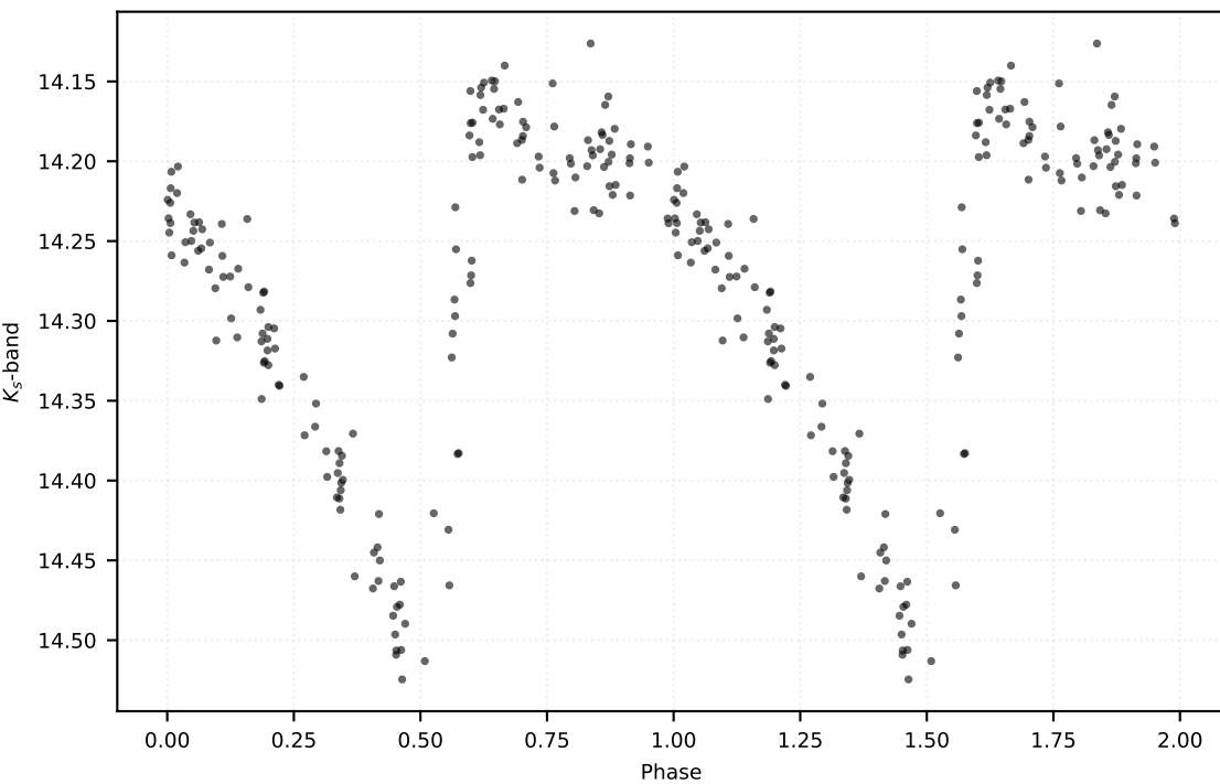
P: 0.52228 d | Class: RP | Subclass: RRab | Field b279
