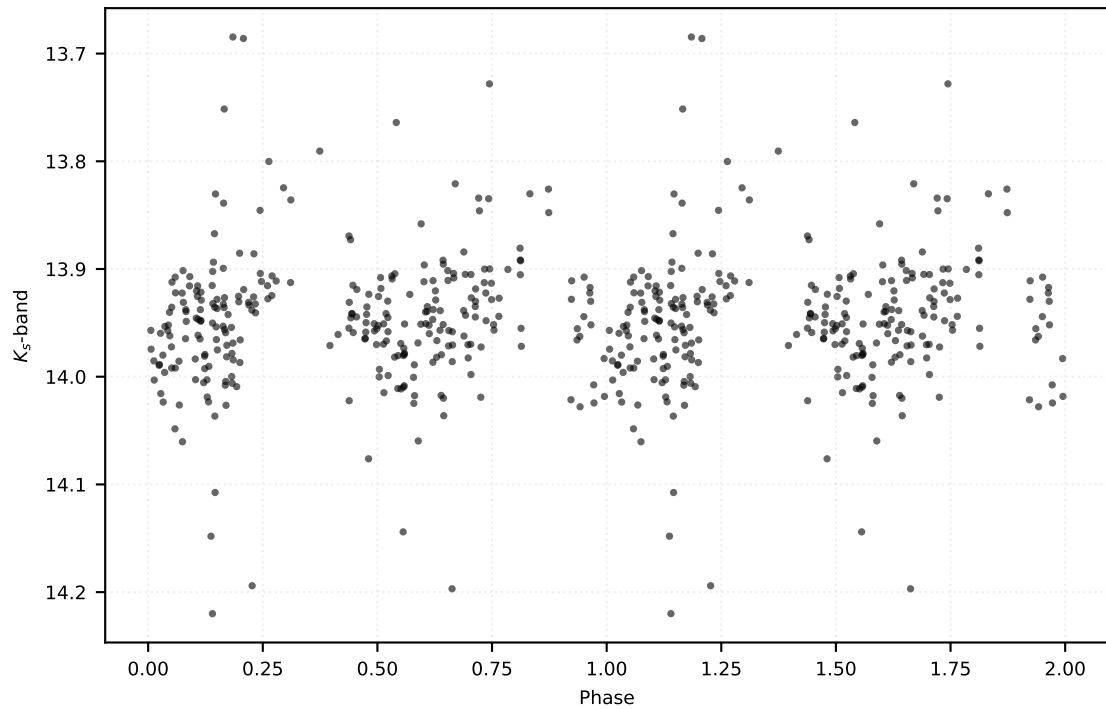
P: 0.23190 d | Class: EB | Subclass: EA | Field b278
