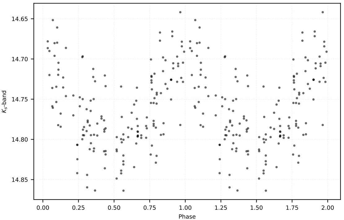
P: 6.19631 d | Class: RP | Subclass: CEP-F | Field b279
