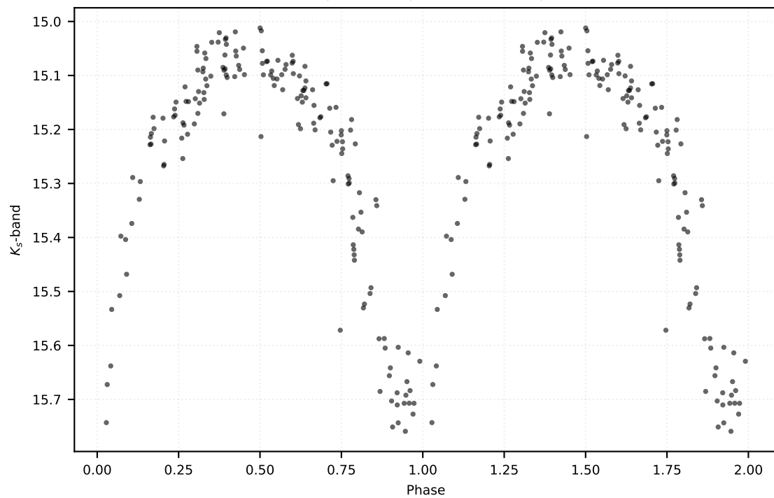
P: 1.02237 d | Class: EB | Subclass: UVAR | Field b278
