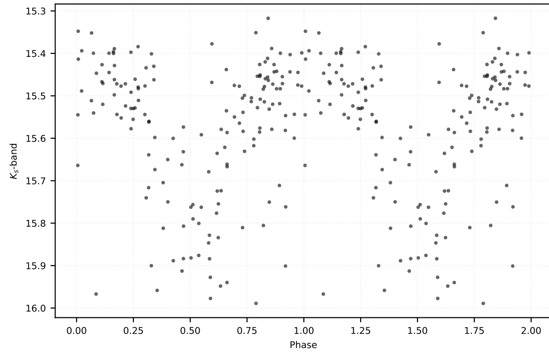
P: 1.49058 d | Class: RP | Subclass: CEP-10T | Field b279
