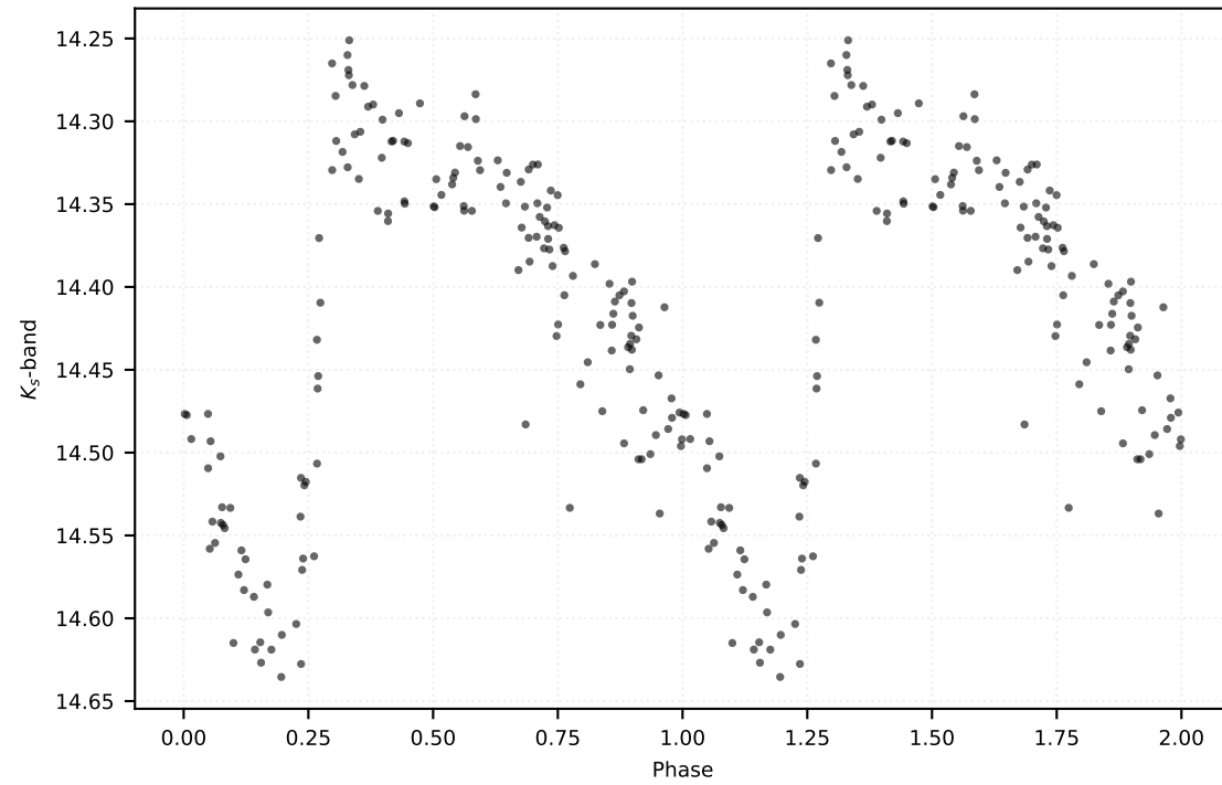
P: 0.54740 d | Class: RP | Subclass: RRab | Field b278
