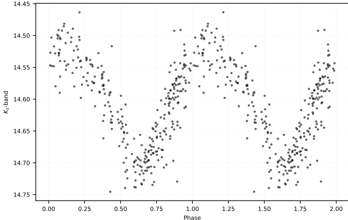
P: 0.17830 d | Class: RP | Subclass: UVAR | Field b278
