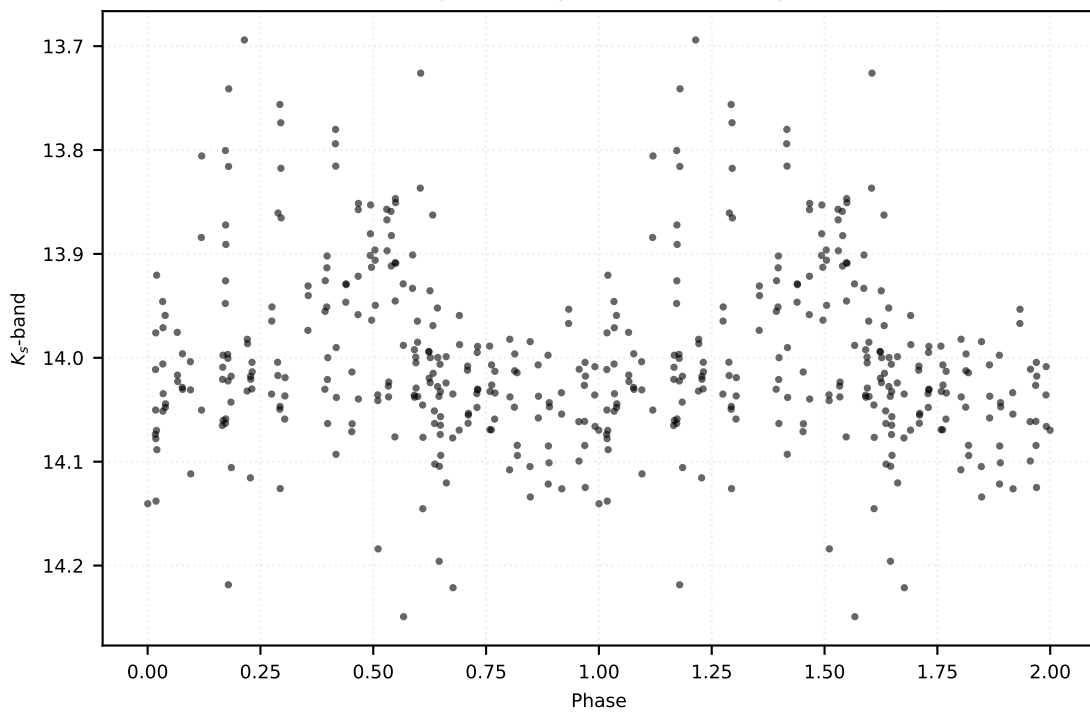
P: 0.32418 d | Class: RP | Subclass: CEP-10T | Field b278
