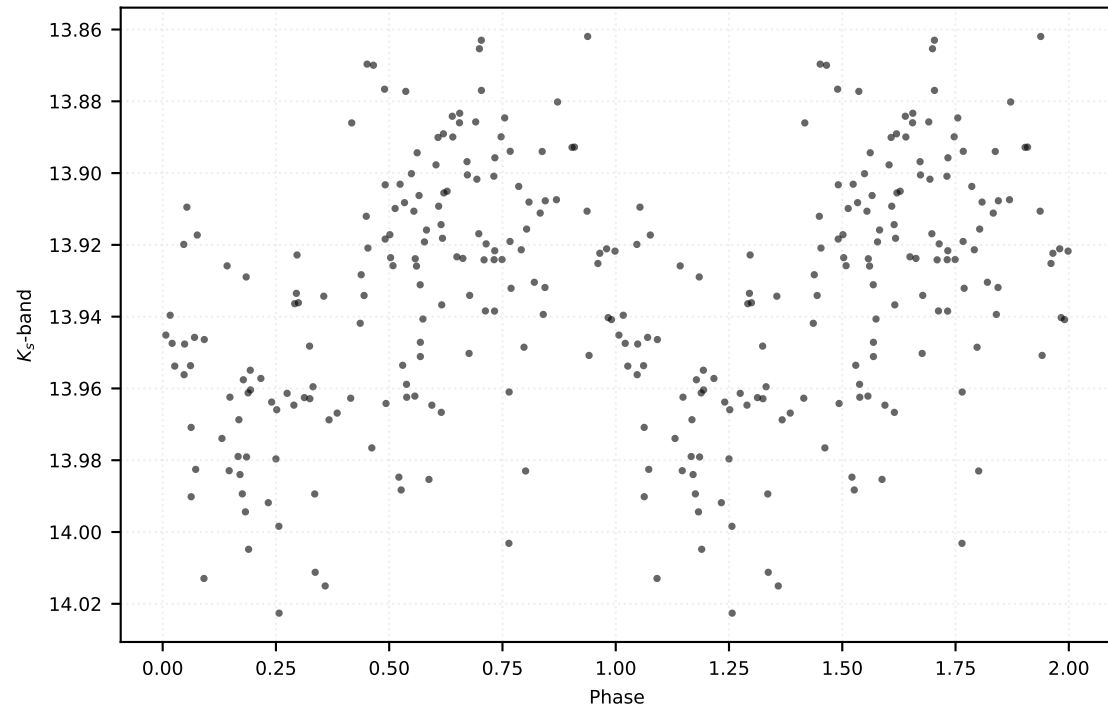
P: 37.90296 d | Class: RP | Subclass: CEP-F | Field b279
