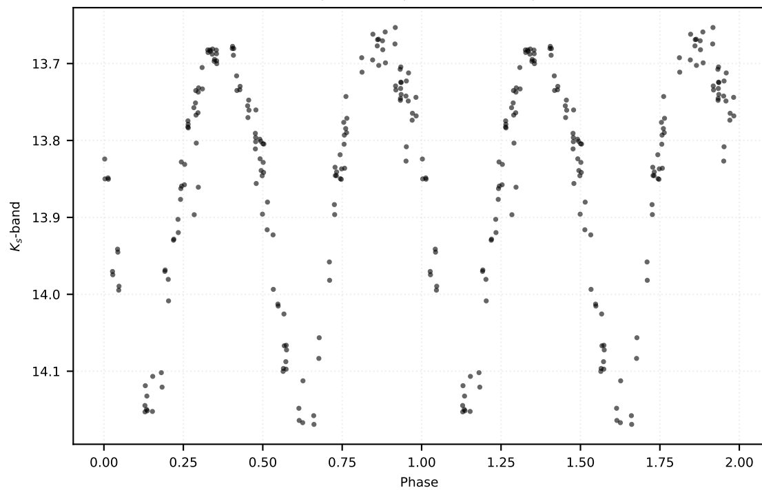
P: 0.13274 d | Class: RP | Subclass: UVAR | Field b279
