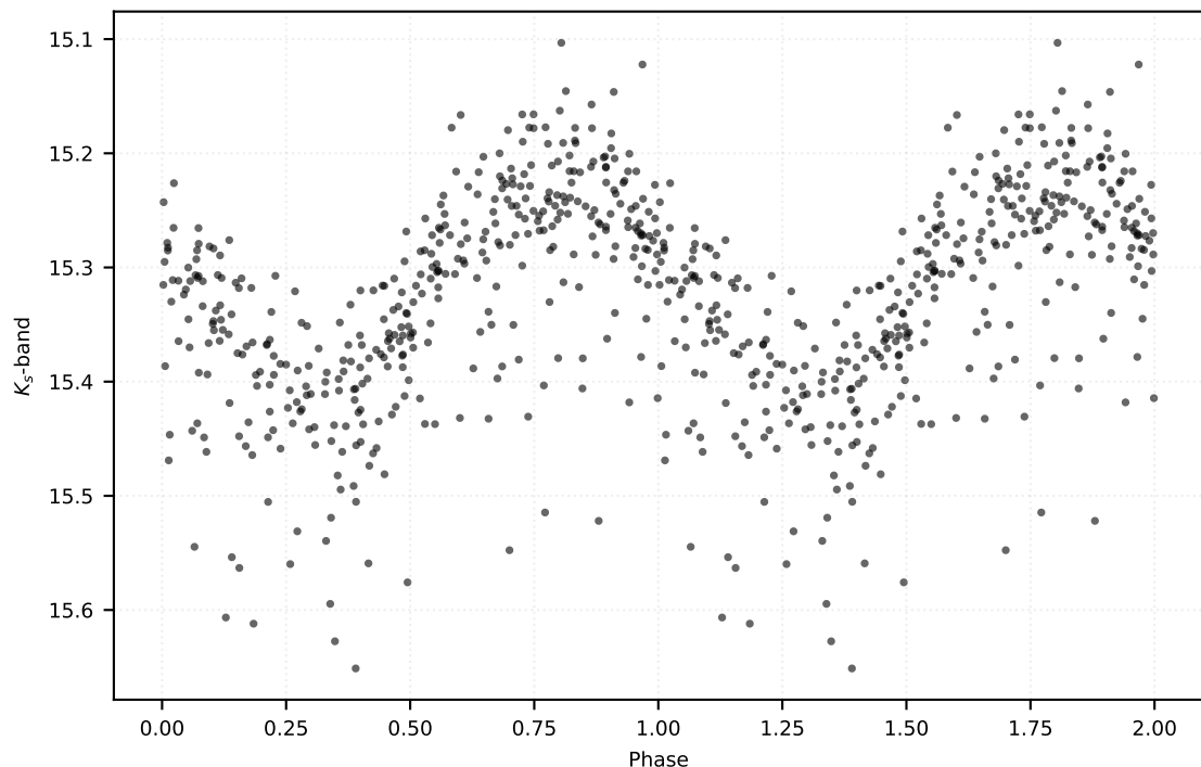
P: 0.54389 d | Class: RP | Subclass: RRab | Field b279
