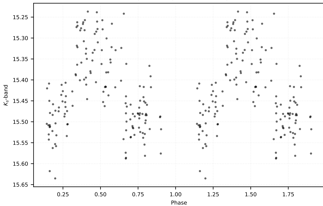
P: 0.22157 d | Class: RP | Subclass: UVAR | Field b279
