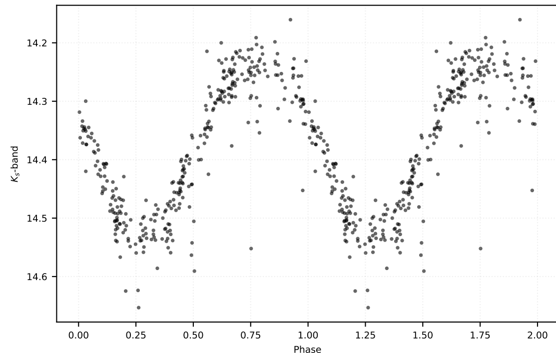
P: 0.26396 d | Class: RP | Subclass: UVAR | Field b278
