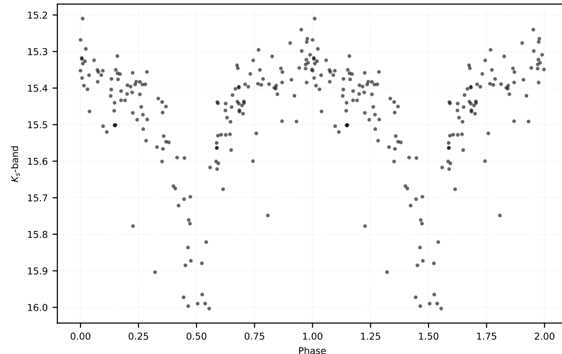
P: 3.88950 d | Class: RP | Subclass: CEP-10T | Field b278
