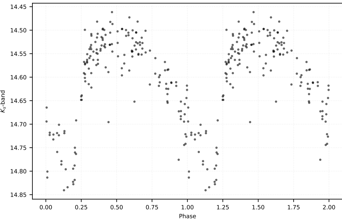
P: 0.45753 d | Class: RP | Subclass: RRab | Field b278
