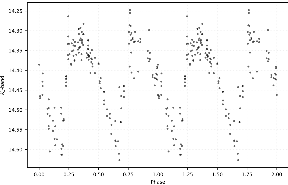
P: 1.23507 d | Class: EB | Subclass: RRc | Field b278
