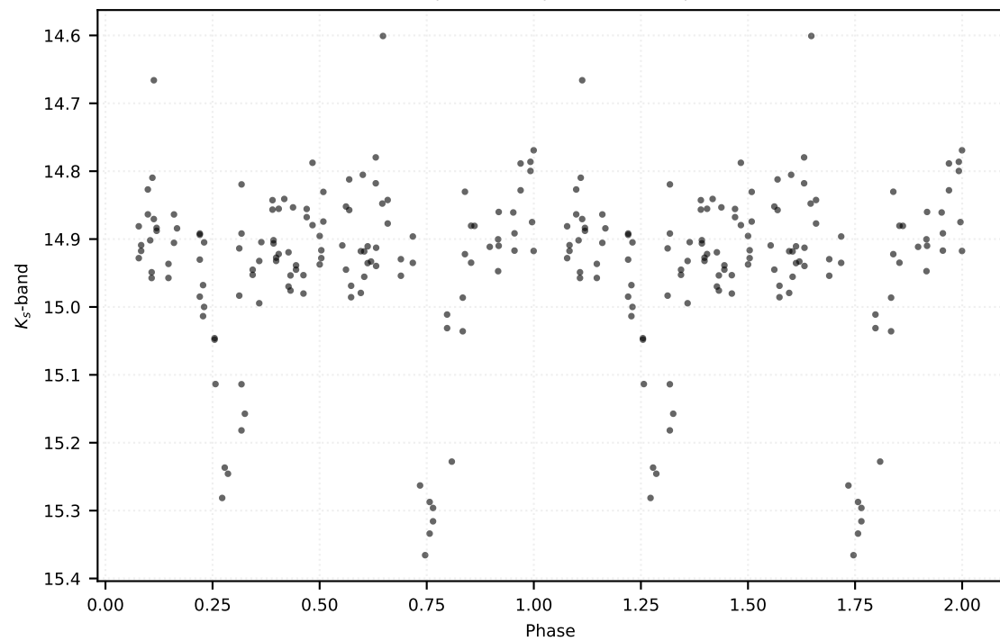
P: 4.20529 d | Class: EB | Subclass: EA | Field b279
