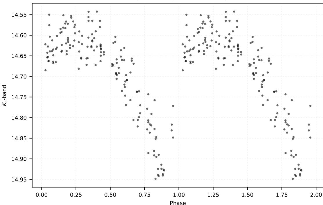
P: 0.62413 d | Class: RP | Subclass: RRab | Field b279
