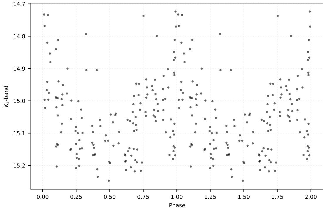
P: 0.15853 d | Class: RP | Subclass: UVAR | Field b279
