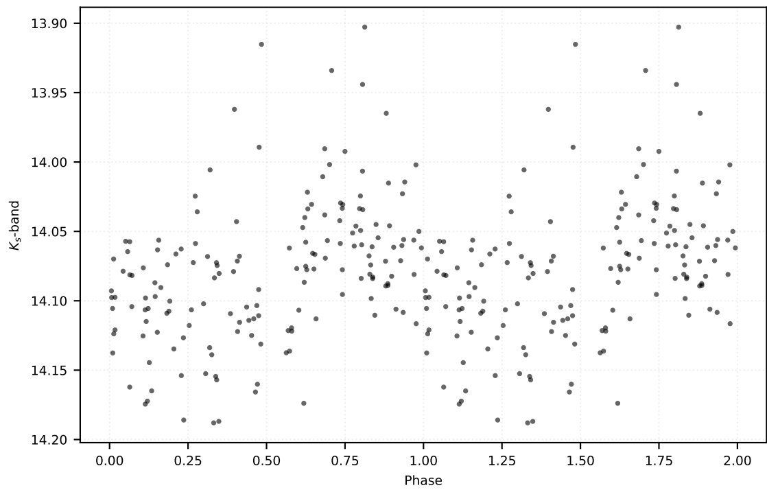
P: 0.10266 d | Class: RP | Subclass: UVAR | Field b279
