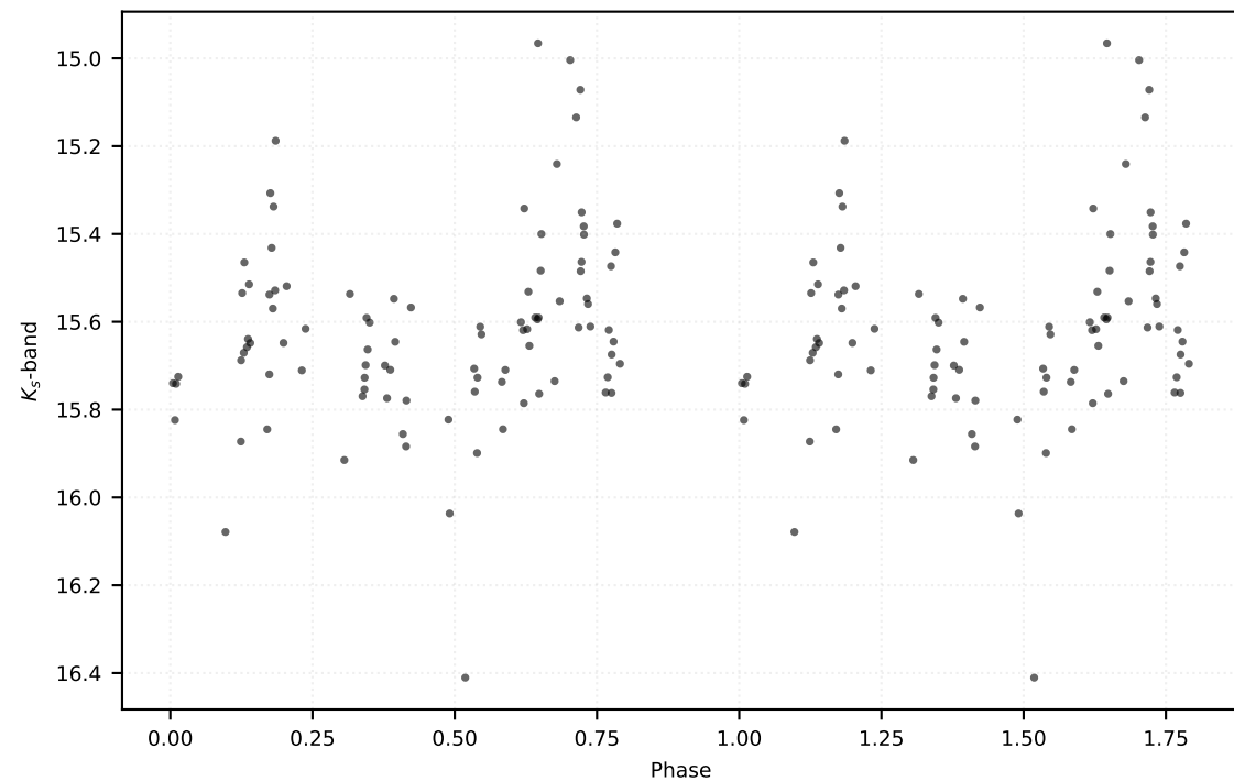
P: 0.20983 d | Class: EB | Subclass: EA | Field b279
