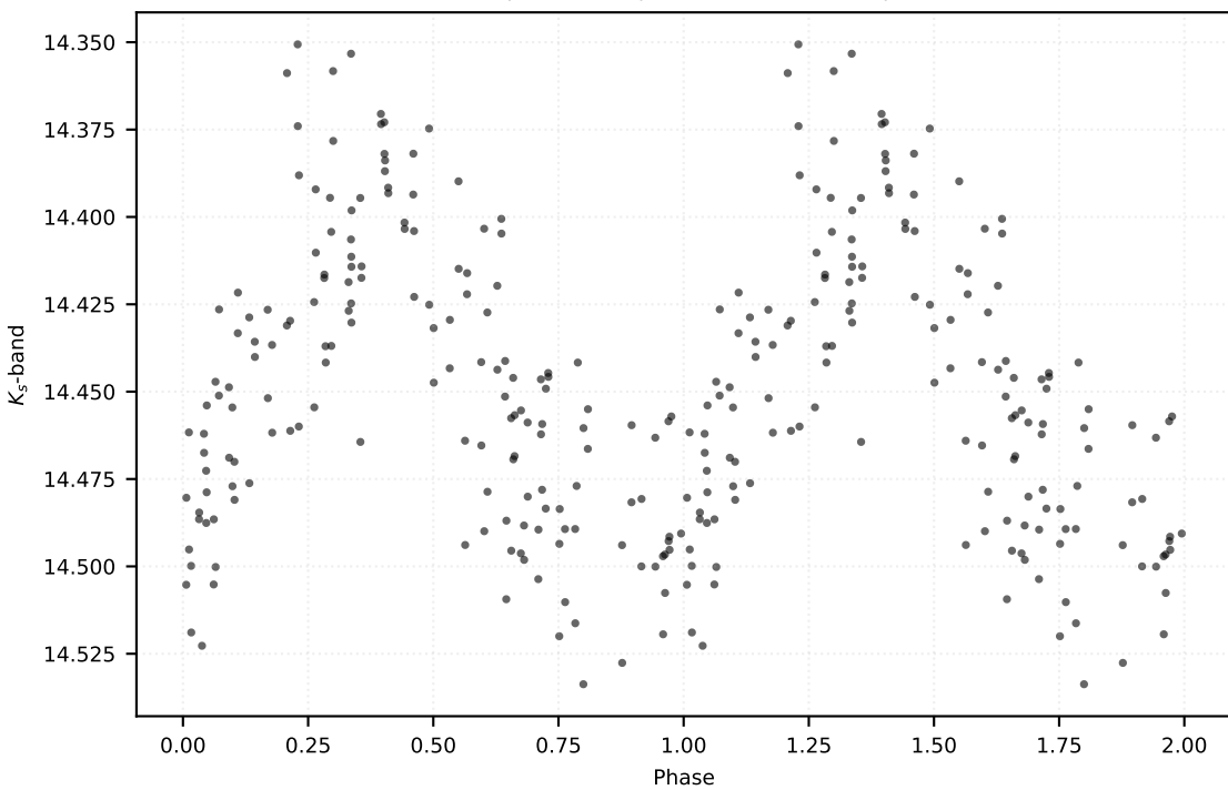
P: 0.81419 d | Class: RP | Subclass: CEP-10T | Field b279
