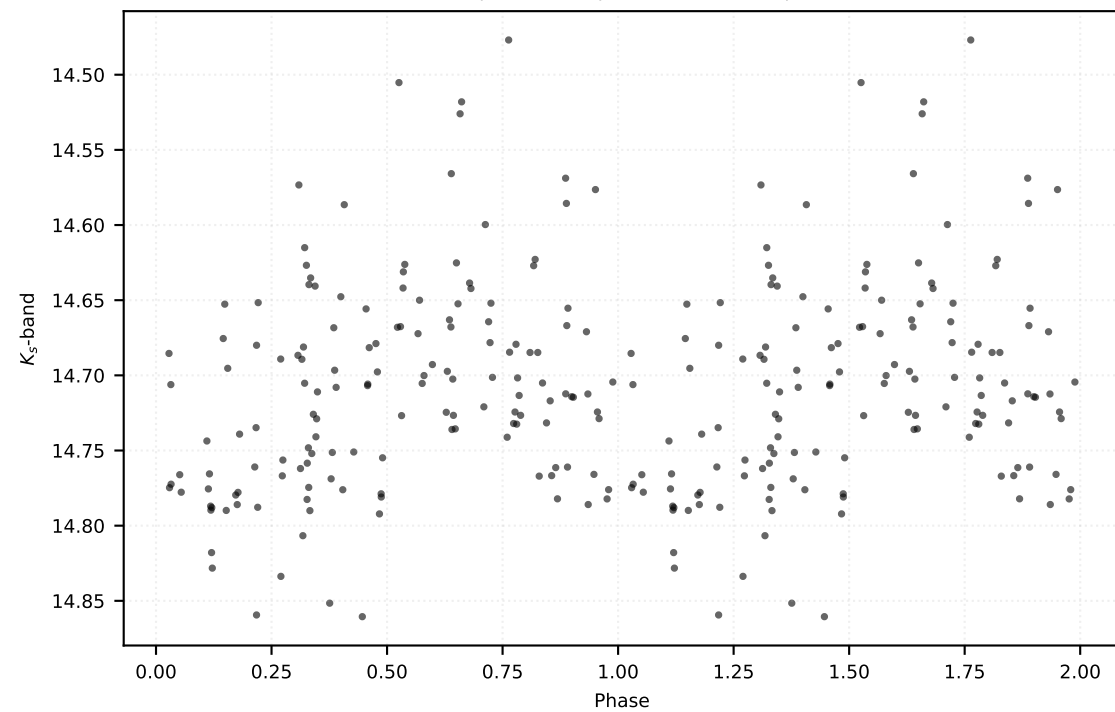
P: 0.10713 d | Class: RP | Subclass: UVAR | Field b279
