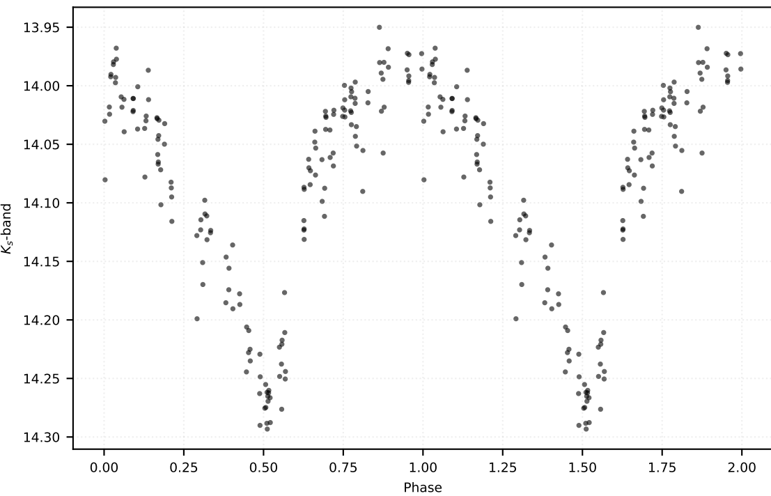
P: 0.59688 d | Class: RP | Subclass: RRab | Field b279
