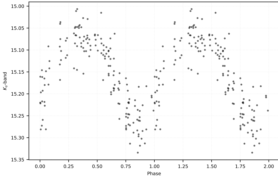
P: 0.30917 d | Class: RP | Subclass: RRc | Field b278
