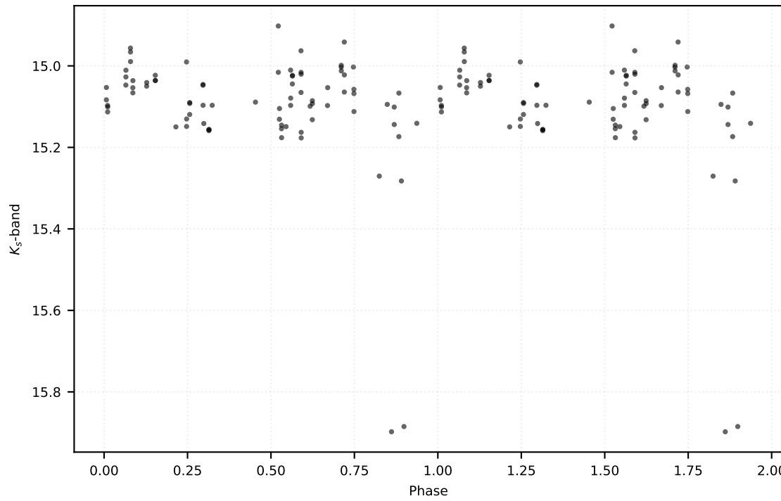
P: 3.14470 d | Class: EB | Subclass: EA | Field b278
