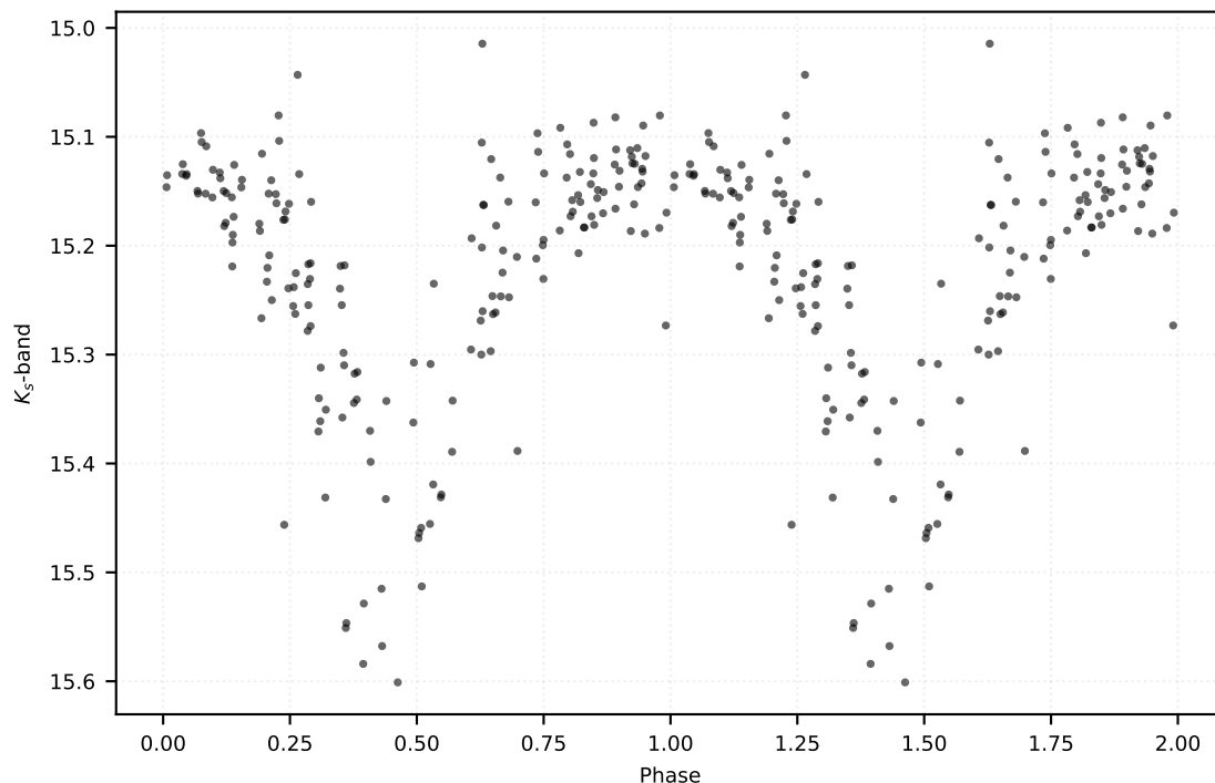
P: 0.42753 d | Class: RP | Subclass: CEP-10T | Field b279
