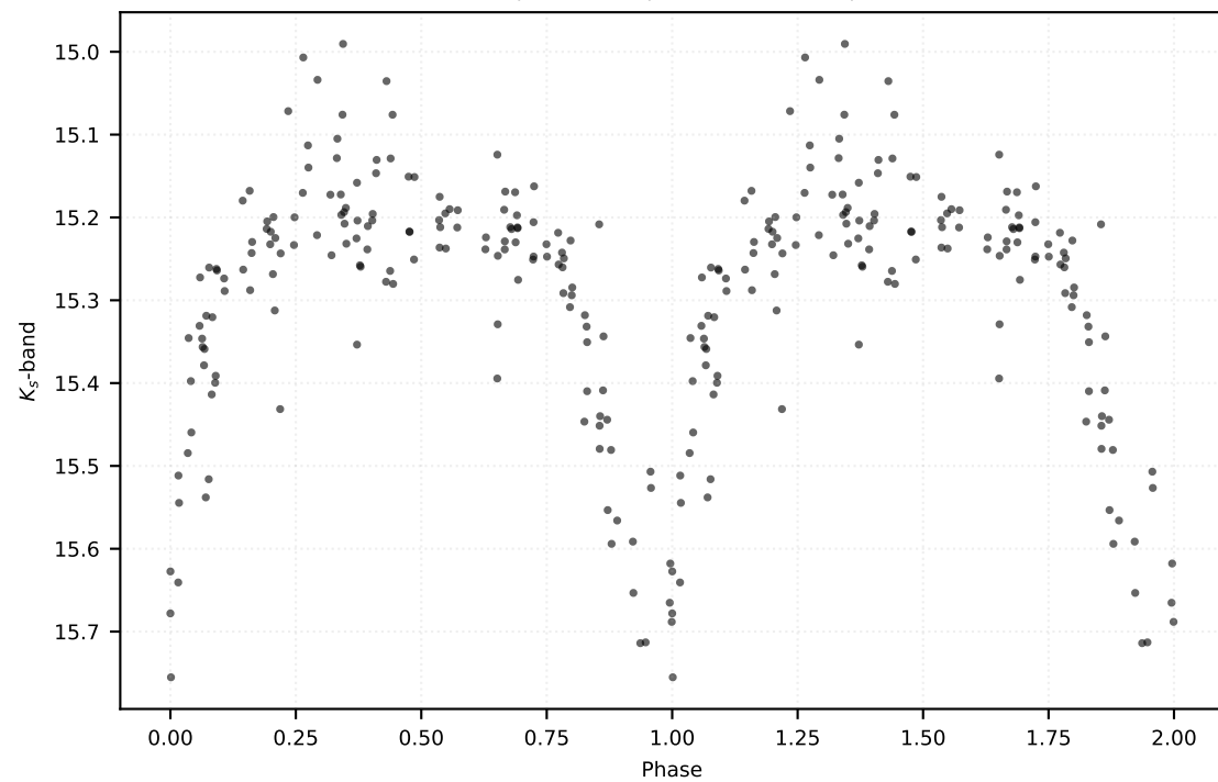
P: 0.51967 d | Class: RP | Subclass: RRab | Field b278
