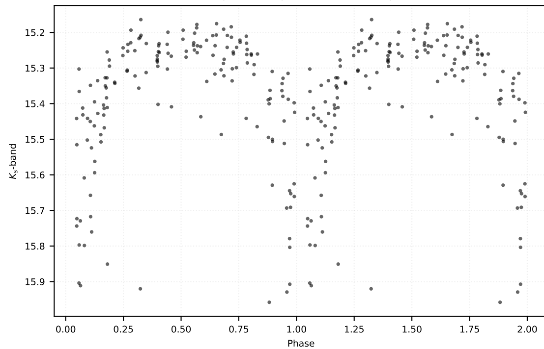
P: 0.29944 d | Class: RP | Subclass: CEP-10T | Field b279
