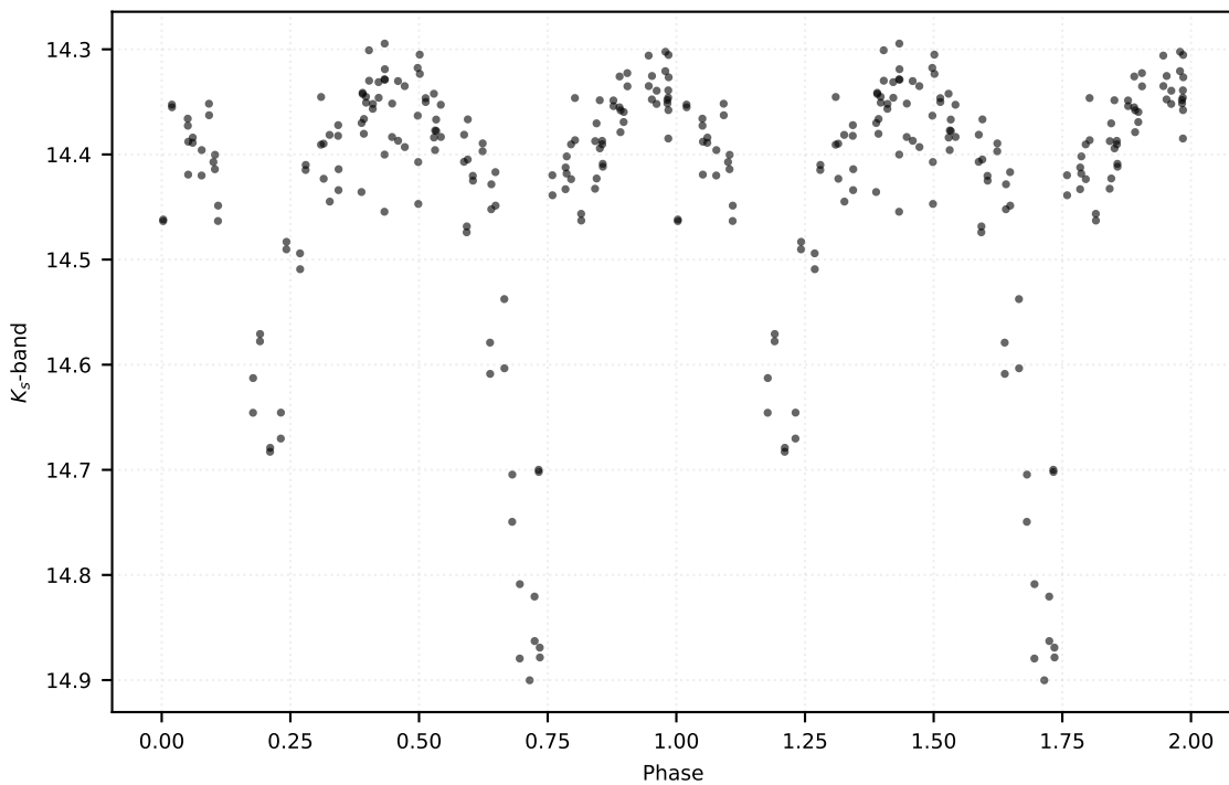
P: 2.52773 d | Class: EB | Subclass: EA | Field b279
