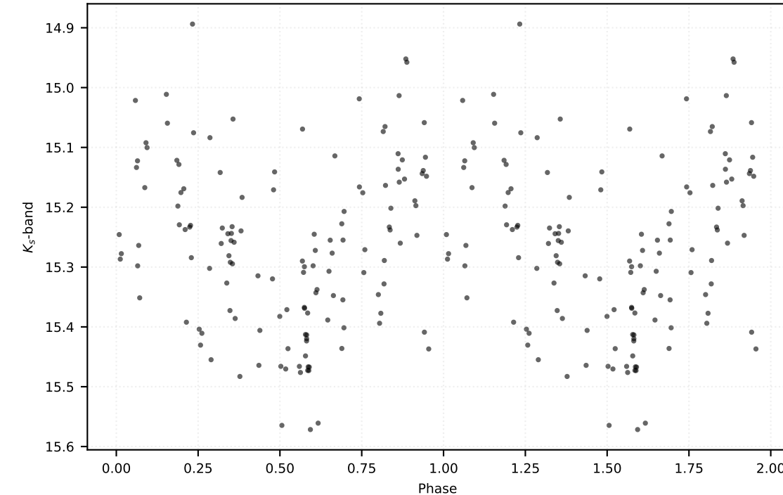
P: 0.11081 d | Class: RP | Subclass: UVAR | Field b279
