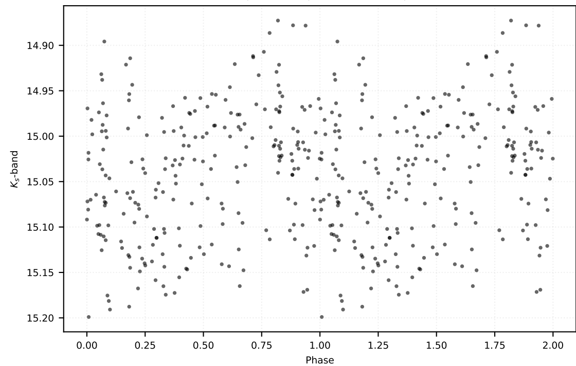
P: 0.12546 d | Class: RP | Subclass: UVAR | Field b279
