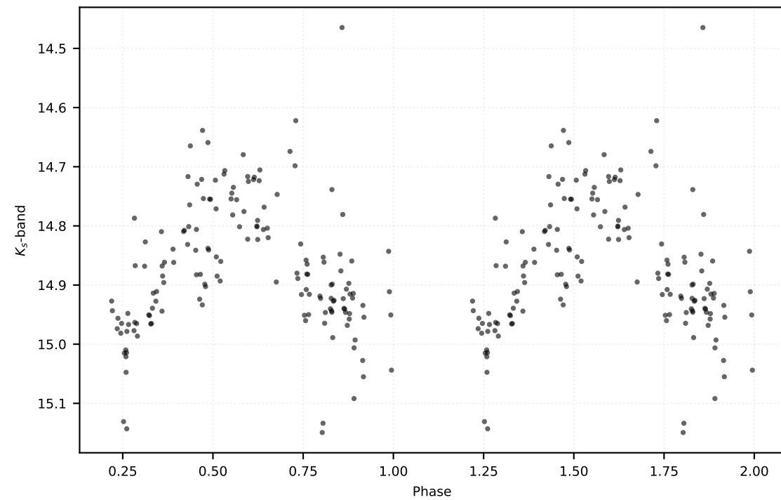
P: 0.10928 d | Class: RP | Subclass: UVAR | Field b279
