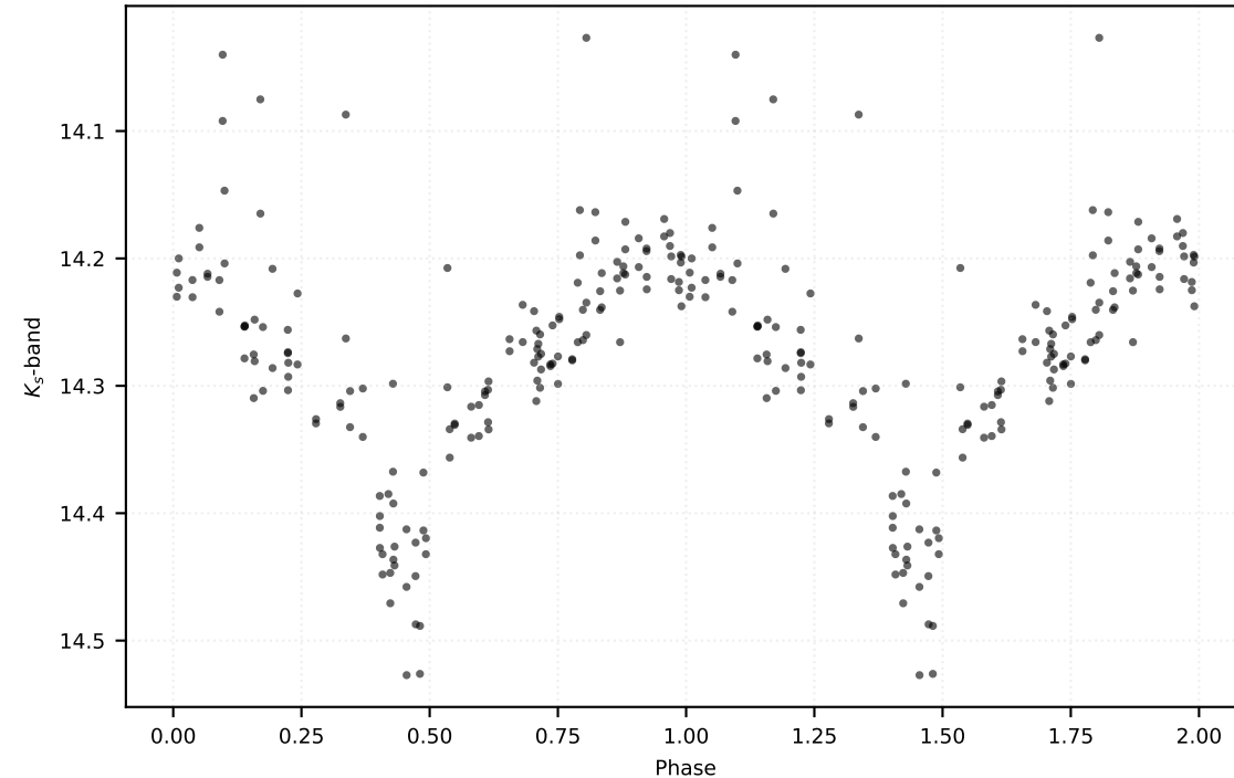
P: 0.63863 d | Class: RP | Subclass: CEP-10T | Field b278
