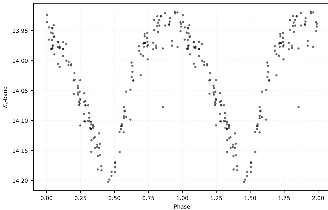
P: 0.48048 d | Class: RP | Subclass: RRab | Field b278
