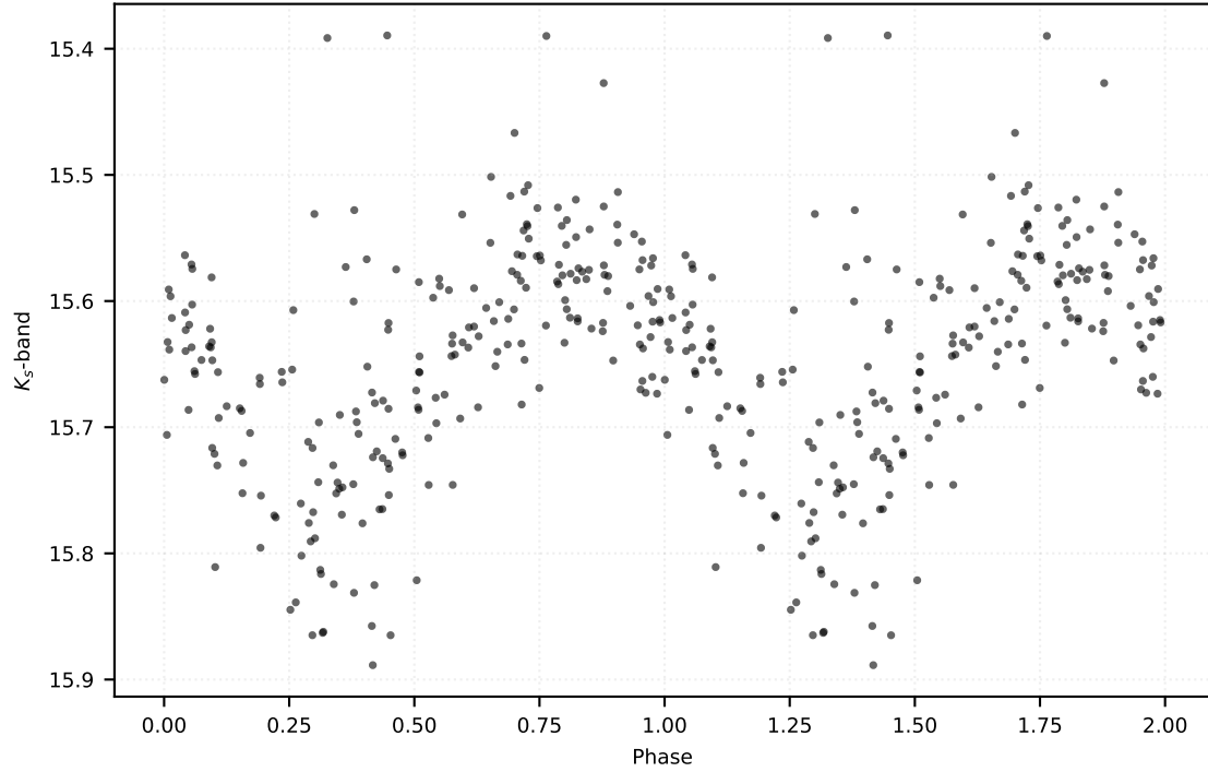
P: 0.49427 d | Class: RP | Subclass: RRab | Field b279
