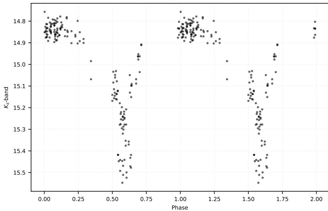
P: 1.15487 d | Class: RP | Subclass: CEP-F | Field b278
