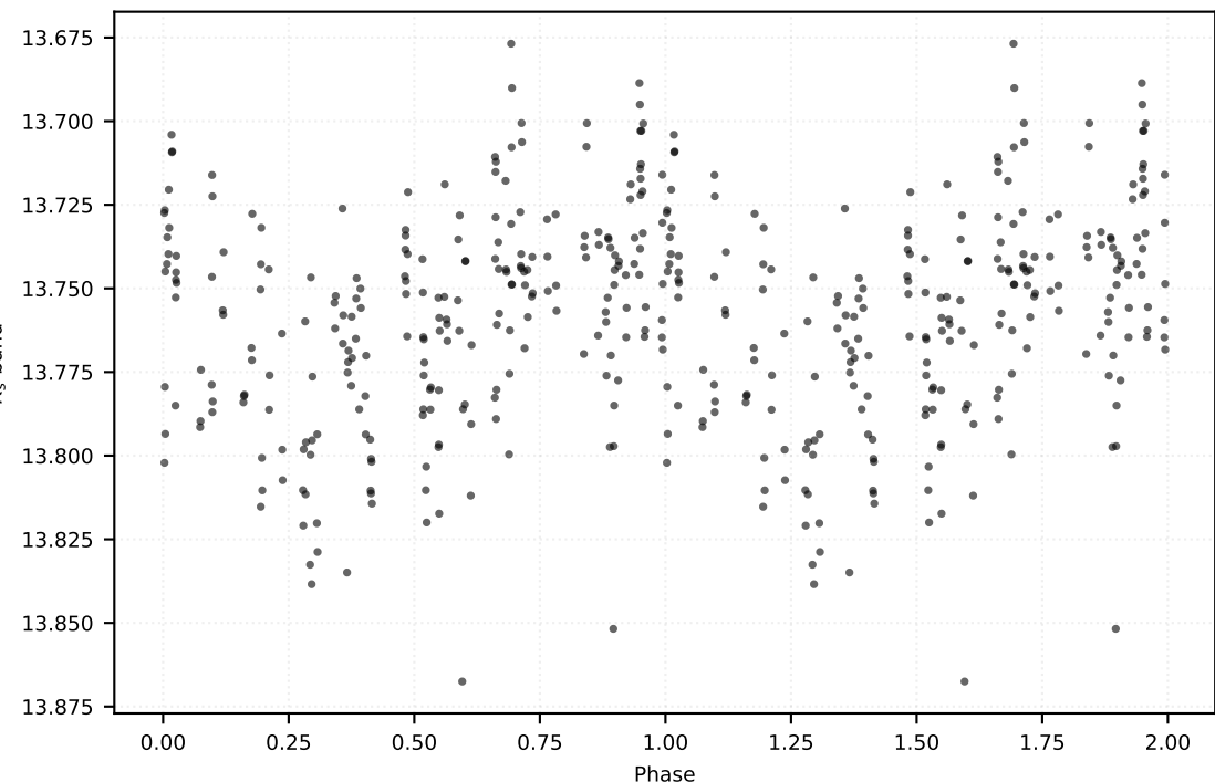
P: 0.32349 d | Class: RP | Subclass: CEP-10T | Field b279
