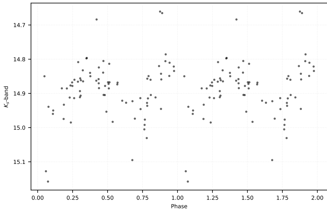
P: 0.90739 d | Class: EB | Subclass: EA | Field b278
