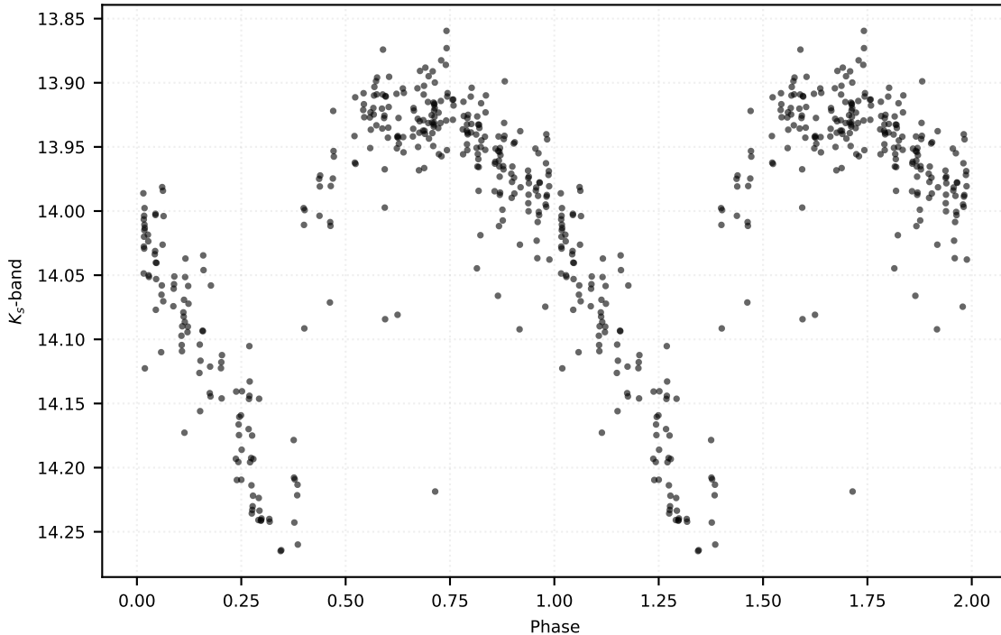
P: 0.47800 d | Class: RP | Subclass: RRab | Field b278
