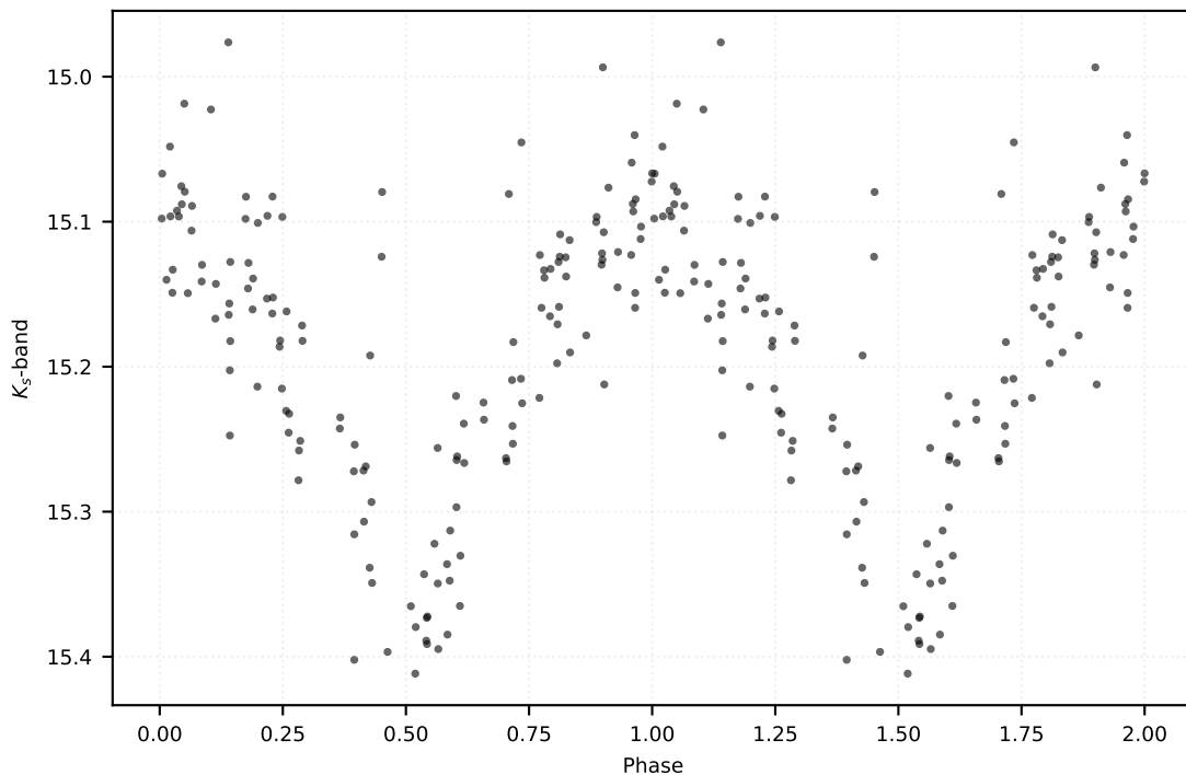
P: 1.16899 d | Class: RP | Subclass: CEP-10T | Field b279
