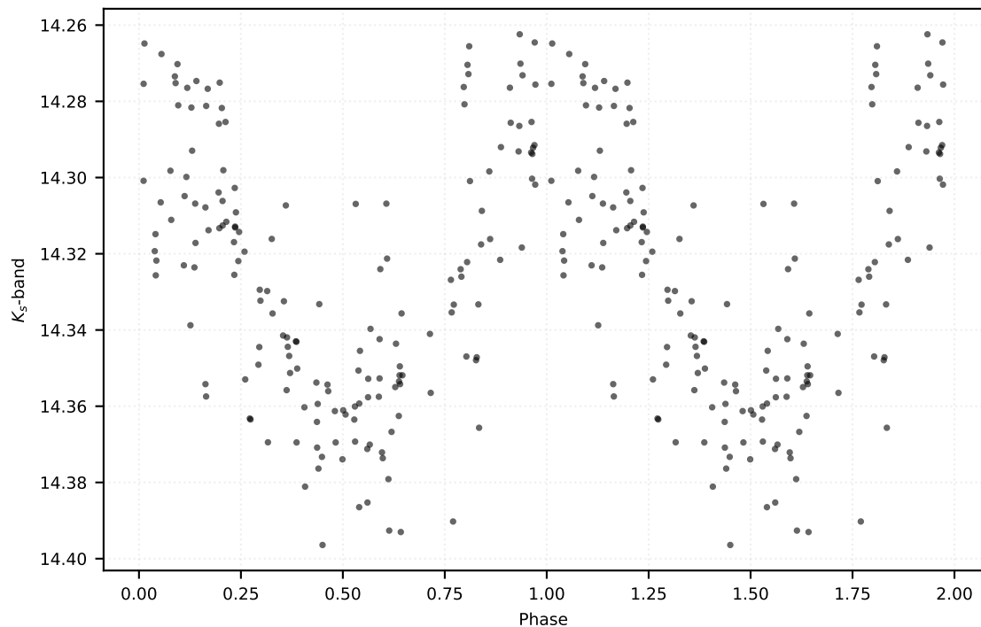
P: 0.60988 d | Class: RP | Subclass: RRab | Field b278
