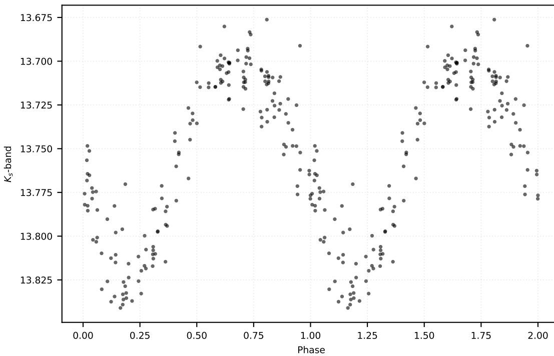
P: 0.33149 d | Class: RP | Subclass: CEP-1OT | Field b279
