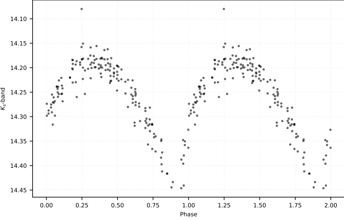
P: 0.58401 d | Class: RP | Subclass: RRab | Field b278
