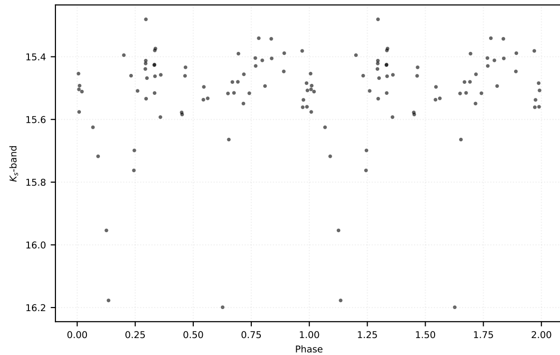
P: 1.99426 d | Class: EB | Subclass: EA | Field b279
