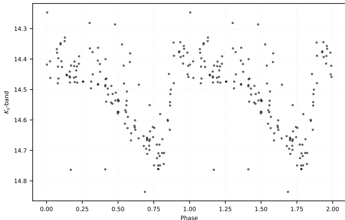
P: 0.54135 d | Class: RP | Subclass: RRab | Field b278
