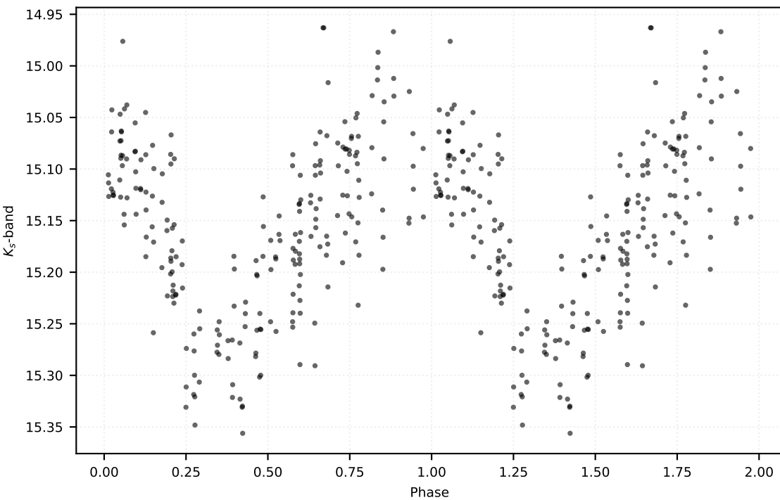
P: 0.35092 d | Class: RP | Subclass: RRab | Field b278
