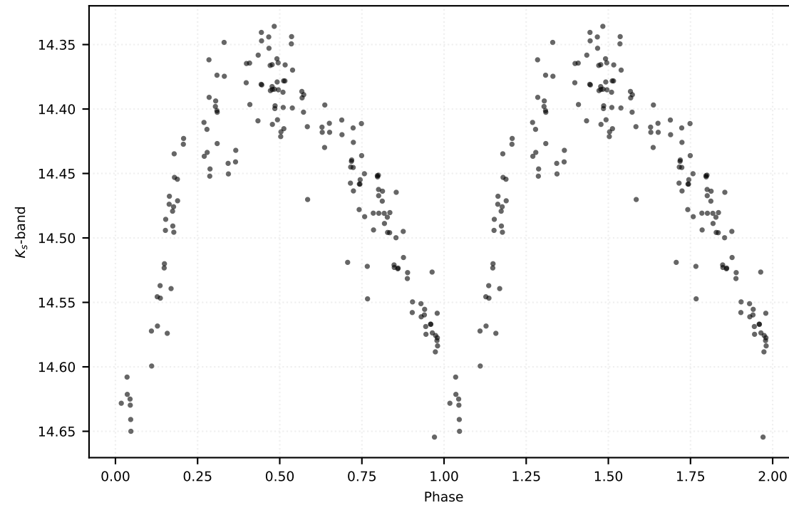
P: 0.31333 d | Class: RP | Subclass: RRab | Field b278
