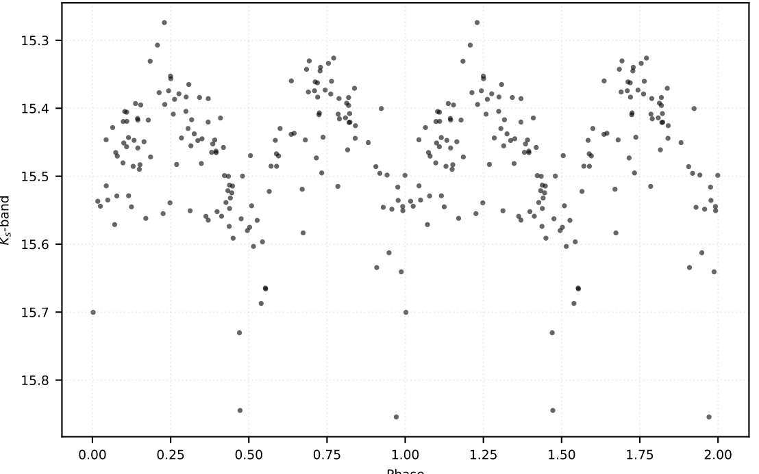
P: 0.74902 d | Class: EB | Subclass: EA | Field b278
