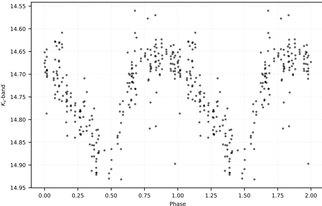
P: 0.39075 d | Class: RP | Subclass: RRab | Field b279
