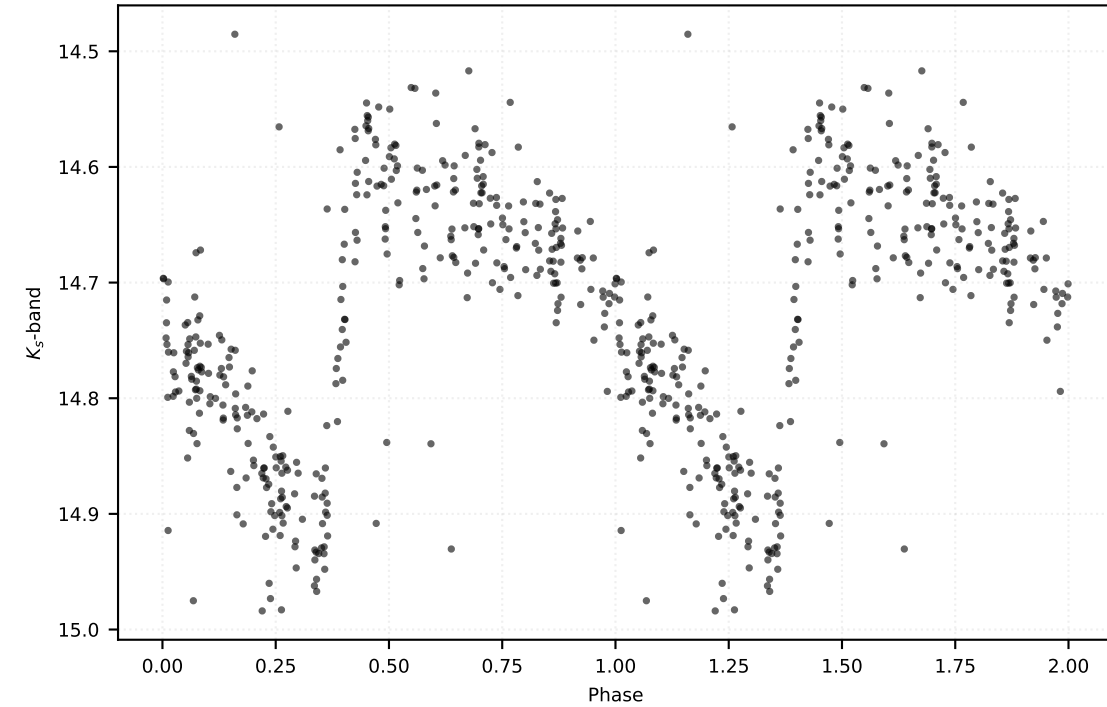
P: 0.59744 d | Class: RP | Subclass: RRab | Field b278
