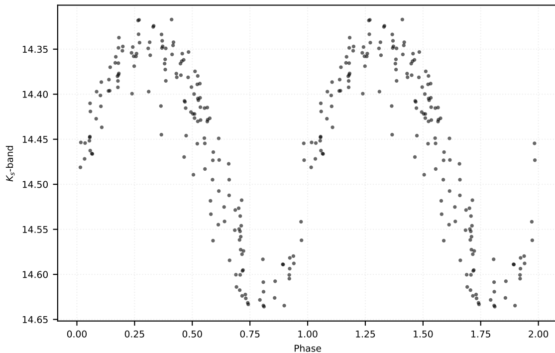
P: 0.18078 d | Class: RP | Subclass: UVAR | Field b278
