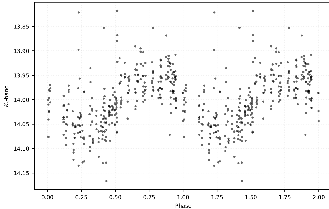
P: 0.54549 d | Class: RP | Subclass: RRab | Field b279
