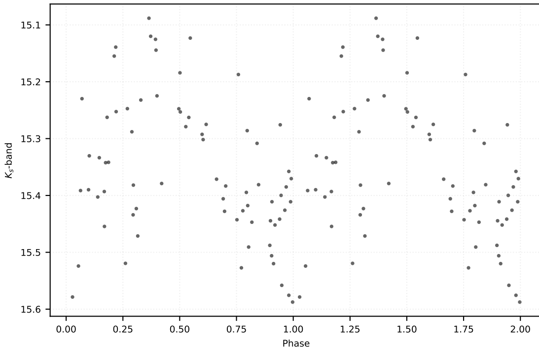
P: 0.12313 d | Class: RP | Subclass: UVAR | Field b278
