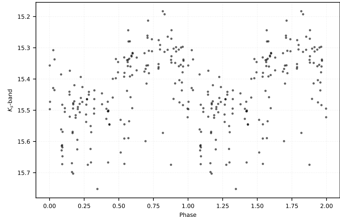
P: 6.43043 d | Class: RP | Subclass: CEP-10T | Field b279
