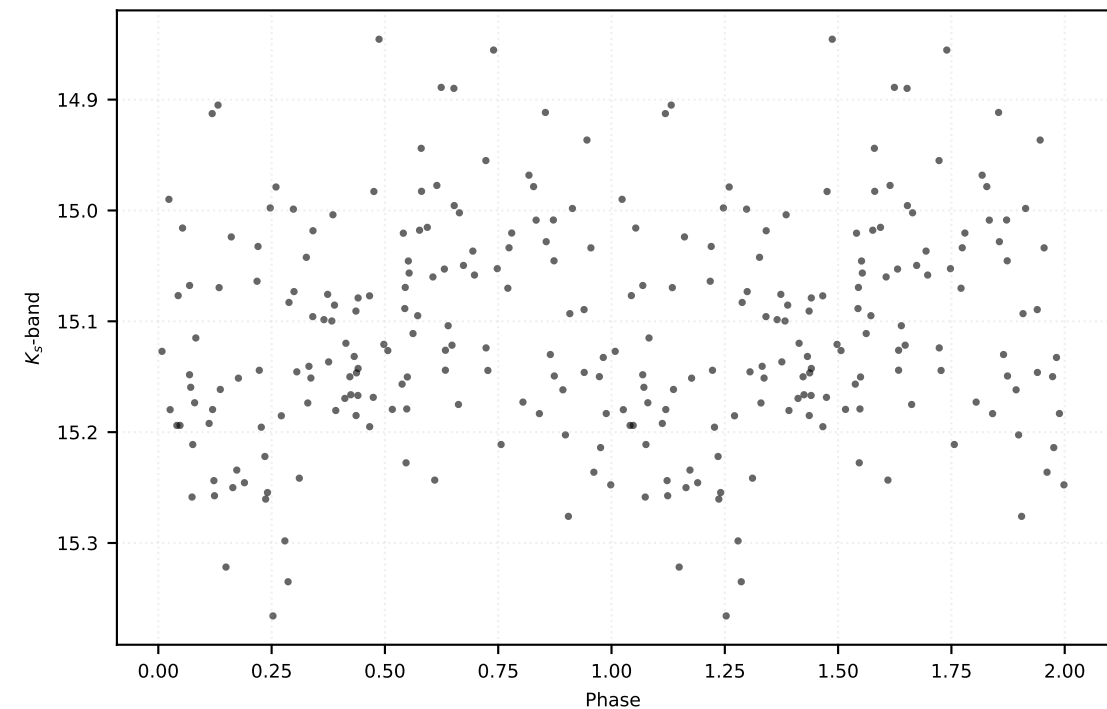
P: 0.10600 d | Class: RP | Subclass: UVAR | Field b278
