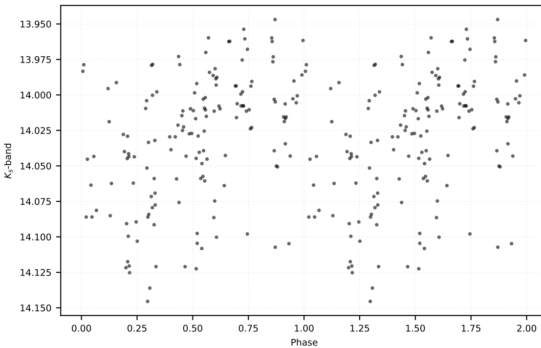
P: 0.10035 d | Class: RP | Subclass: UVAR | Field b279
