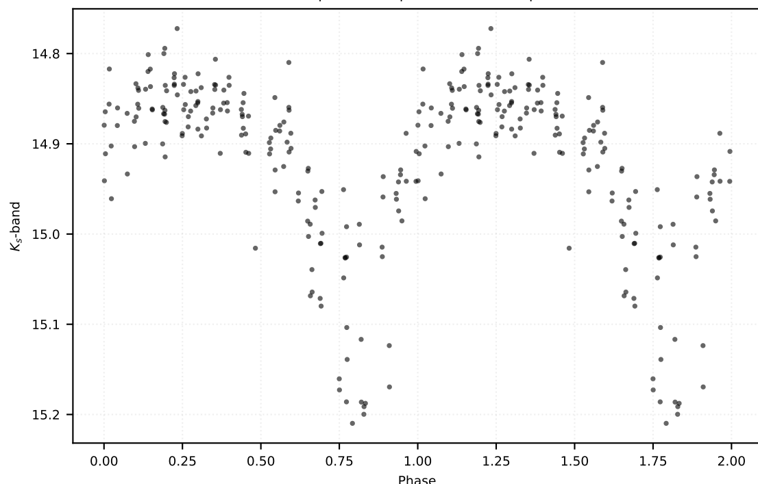
P: 2.31643 d | Class: RP | Subclass: CEP-F | Field b278
