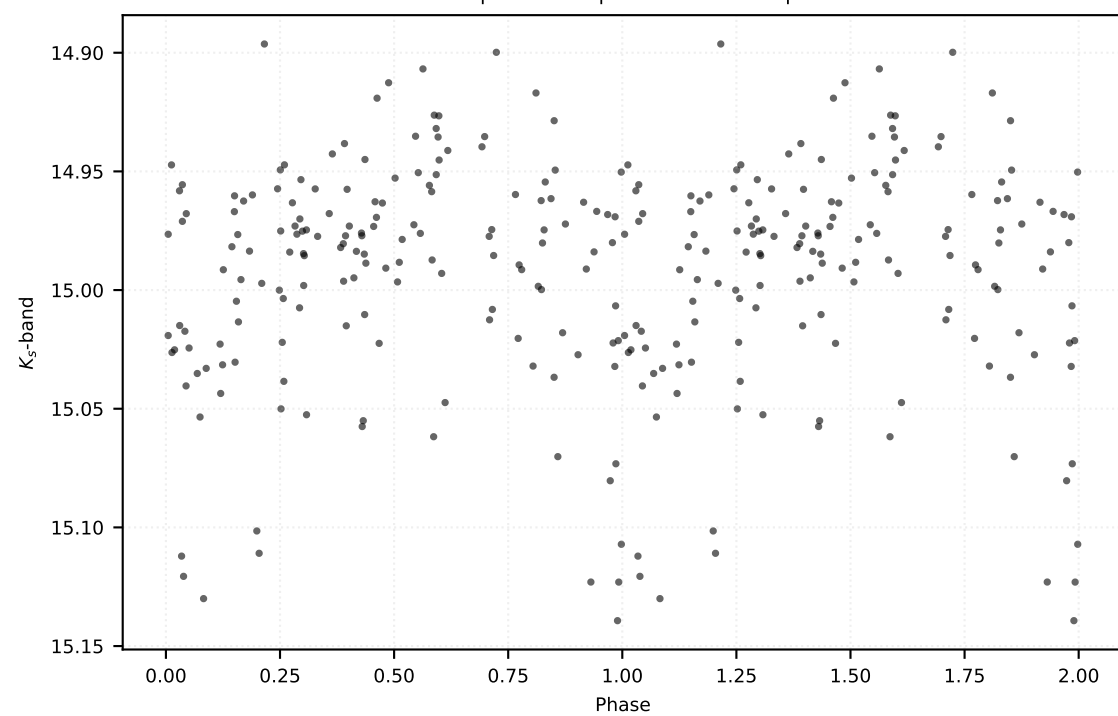
P: 0.15170 d | Class: RP | Subclass: UVAR | Field b279
