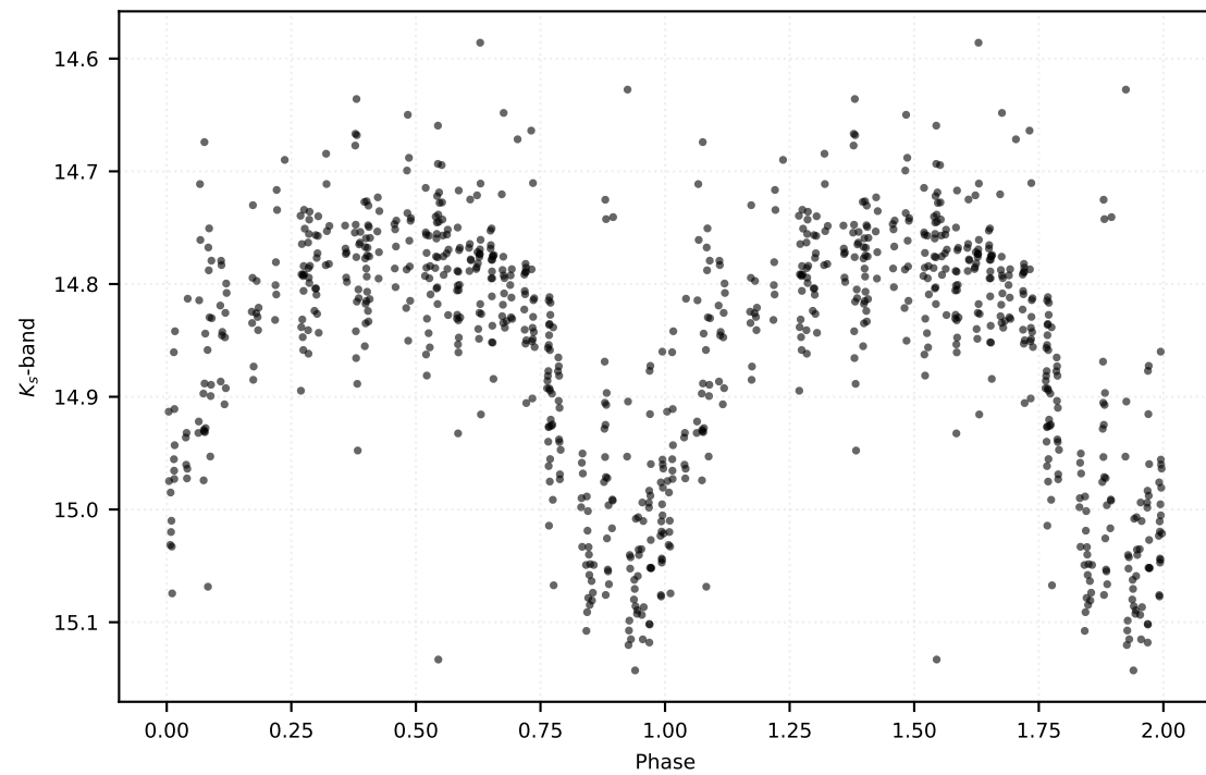
P: 0.31955 d | Class: RP | Subclass: RRab | Field b278
