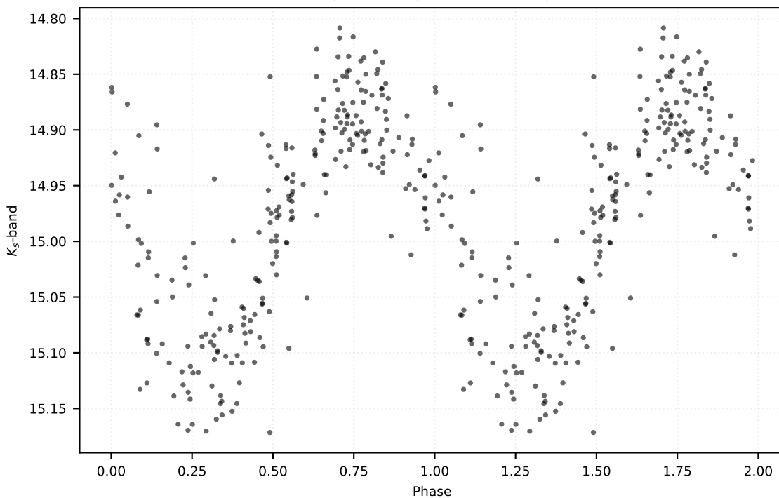
P: 0.43723 d | Class: RP | Subclass: RRab | Field b278
