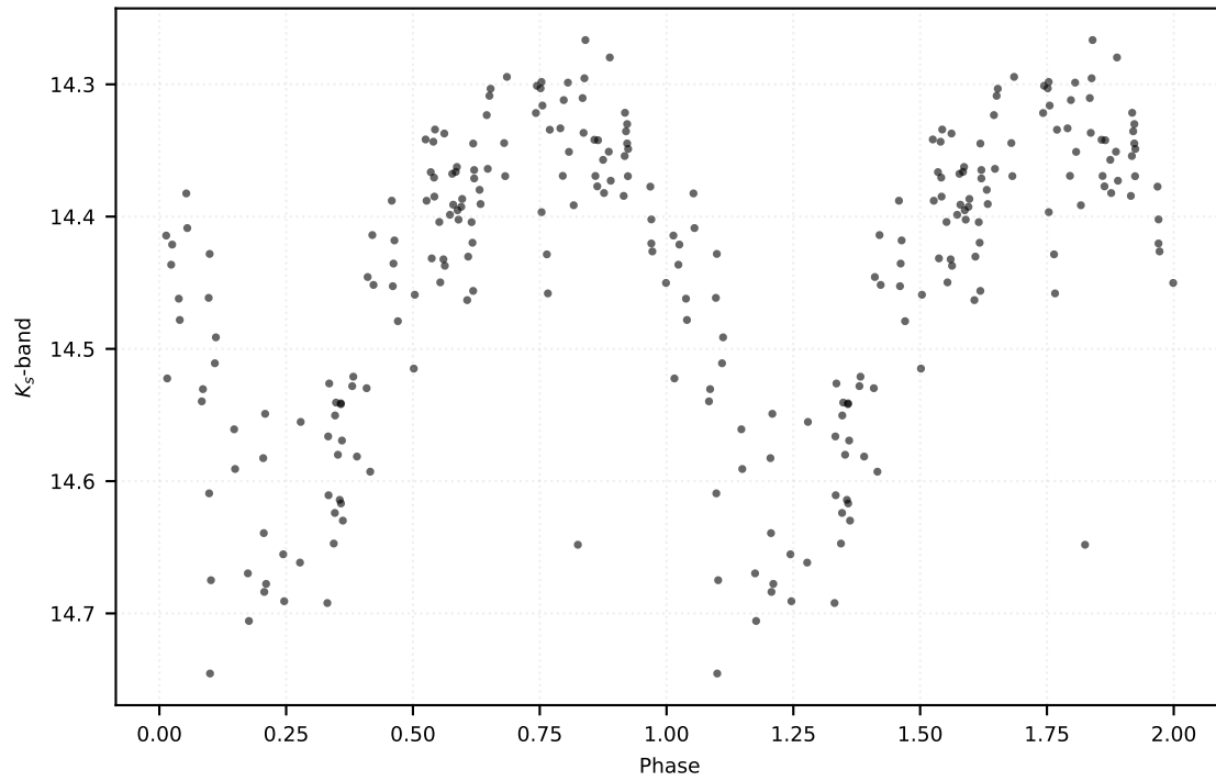
P: 1.00233 d | Class: EB | Subclass: UVAR | Field b279
