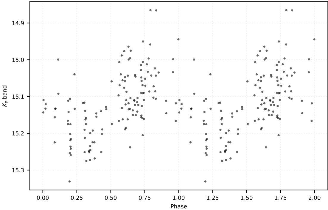
P: 0.12470 d | Class: RP | Subclass: UVAR | Field b278
