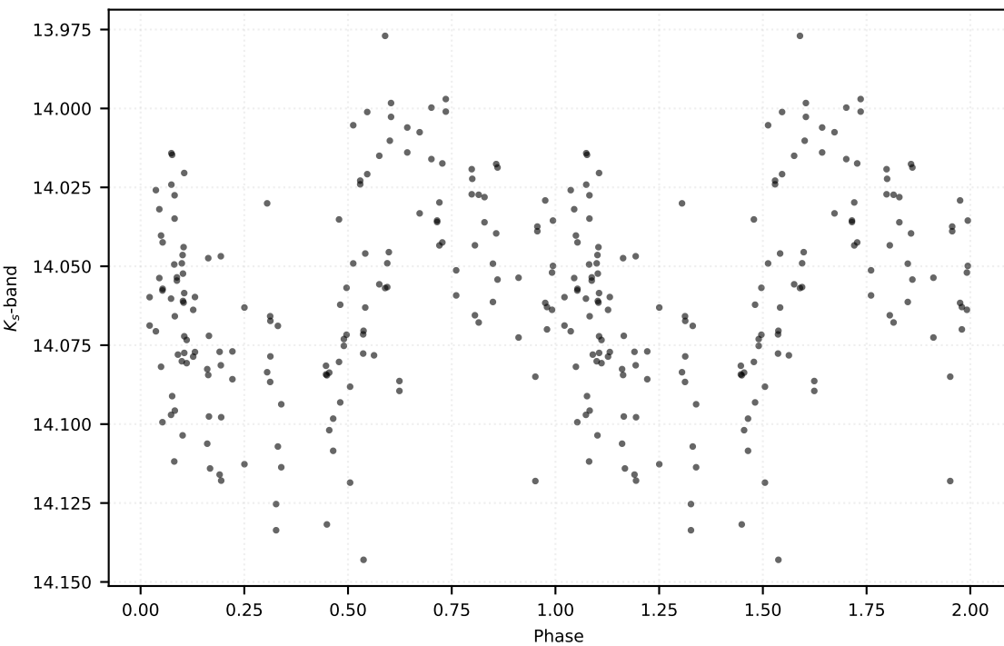
P: 7.61242 d | Class: RP | Subclass: CEP-F | Field b279
