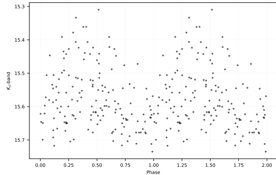
P: 0.26981 d | Class: RP | Subclass: UVAR | Field b279
