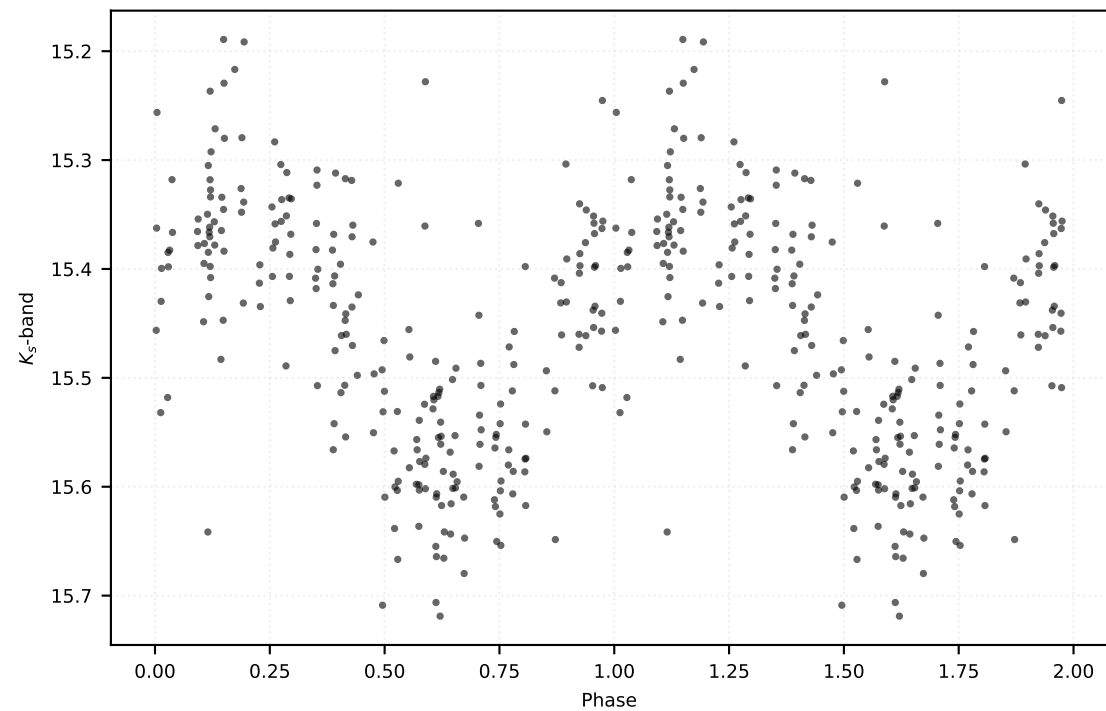
P: 0.30121 d | Class: EB | Subclass: RRc | Field b278
