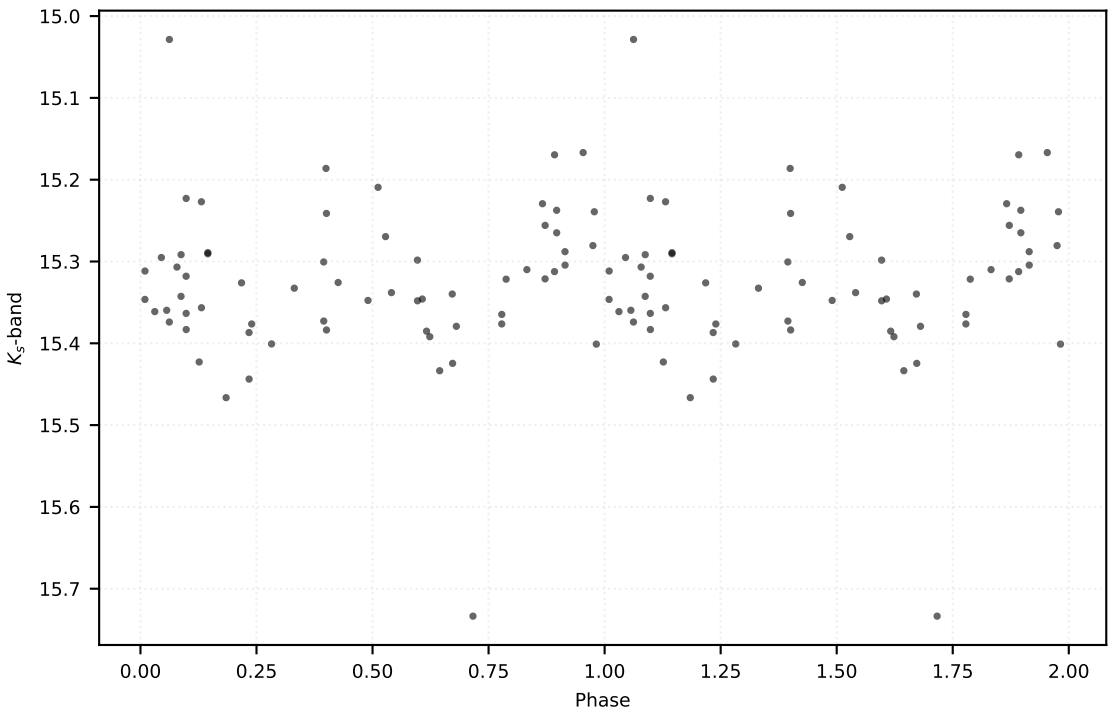
P: 0.57873 d | Class: EB | Subclass: EA | Field b278
