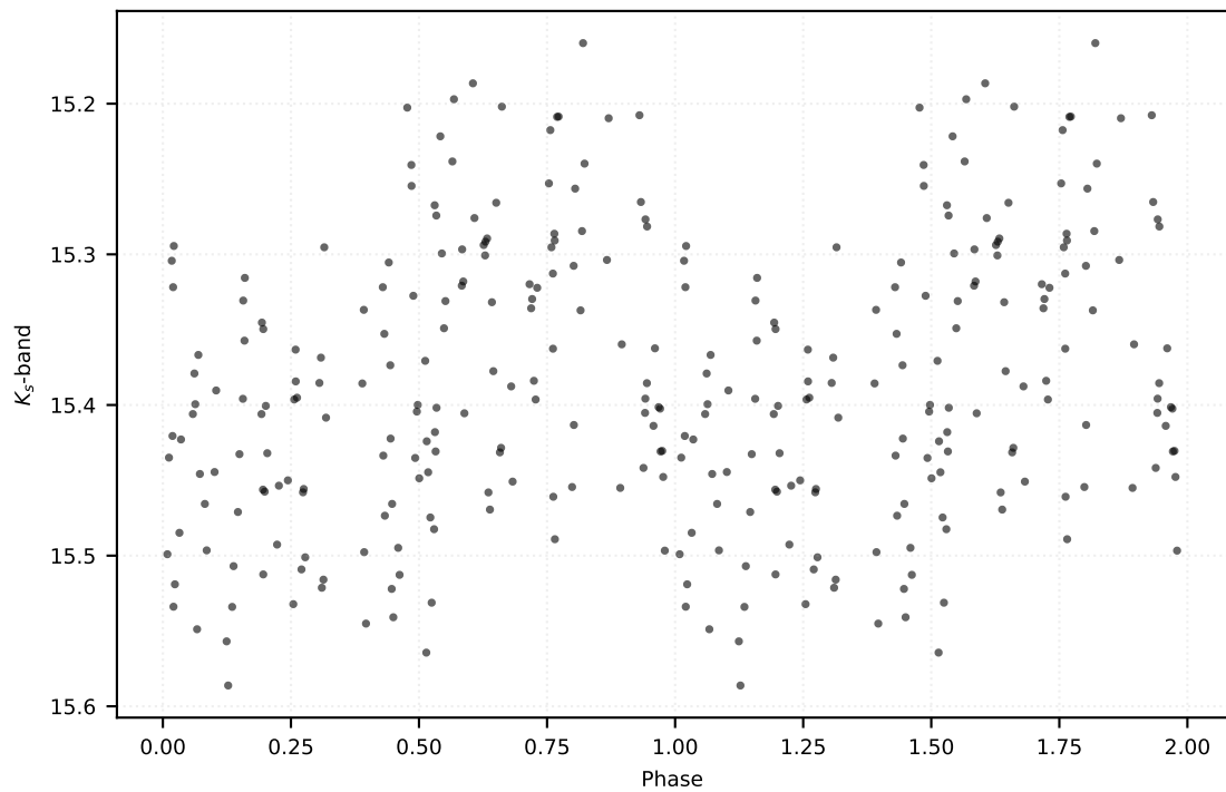
P: 0.14246 d | Class: RP | Subclass: UVAR | Field b279
