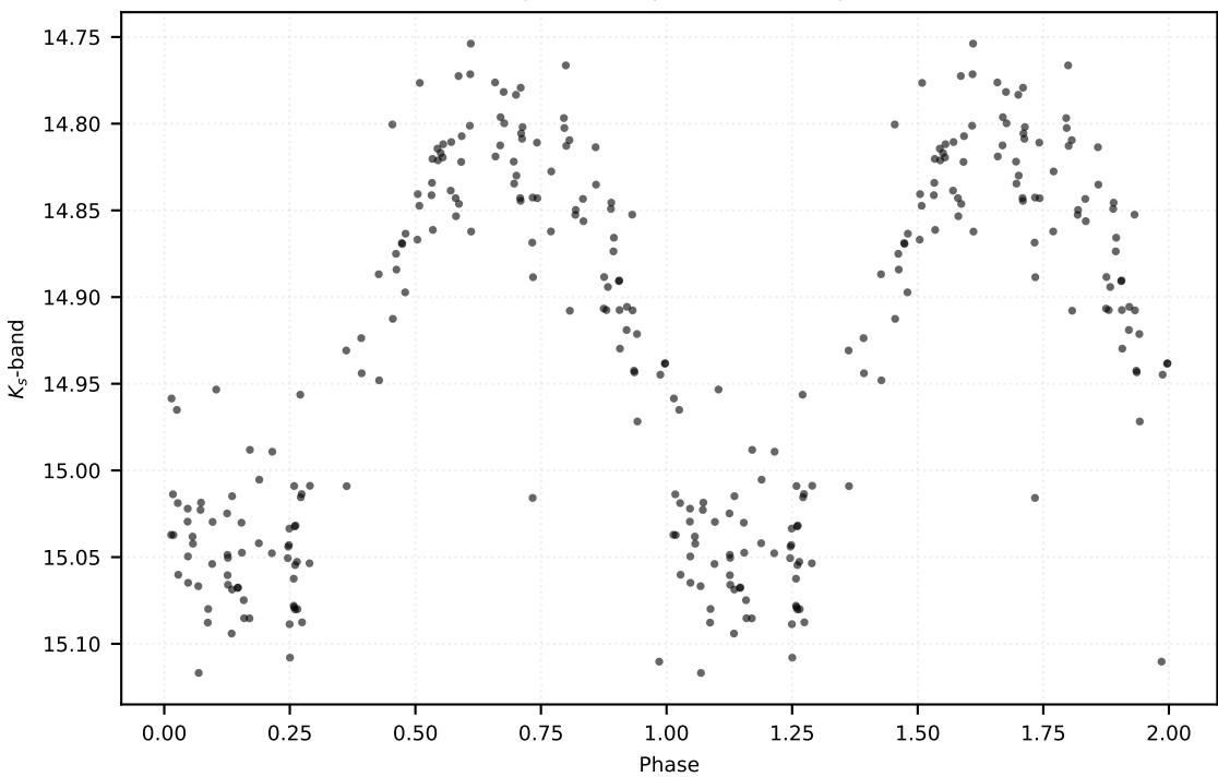
P: 0.49812 d | Class: RP | Subclass: RRc | Field b279
