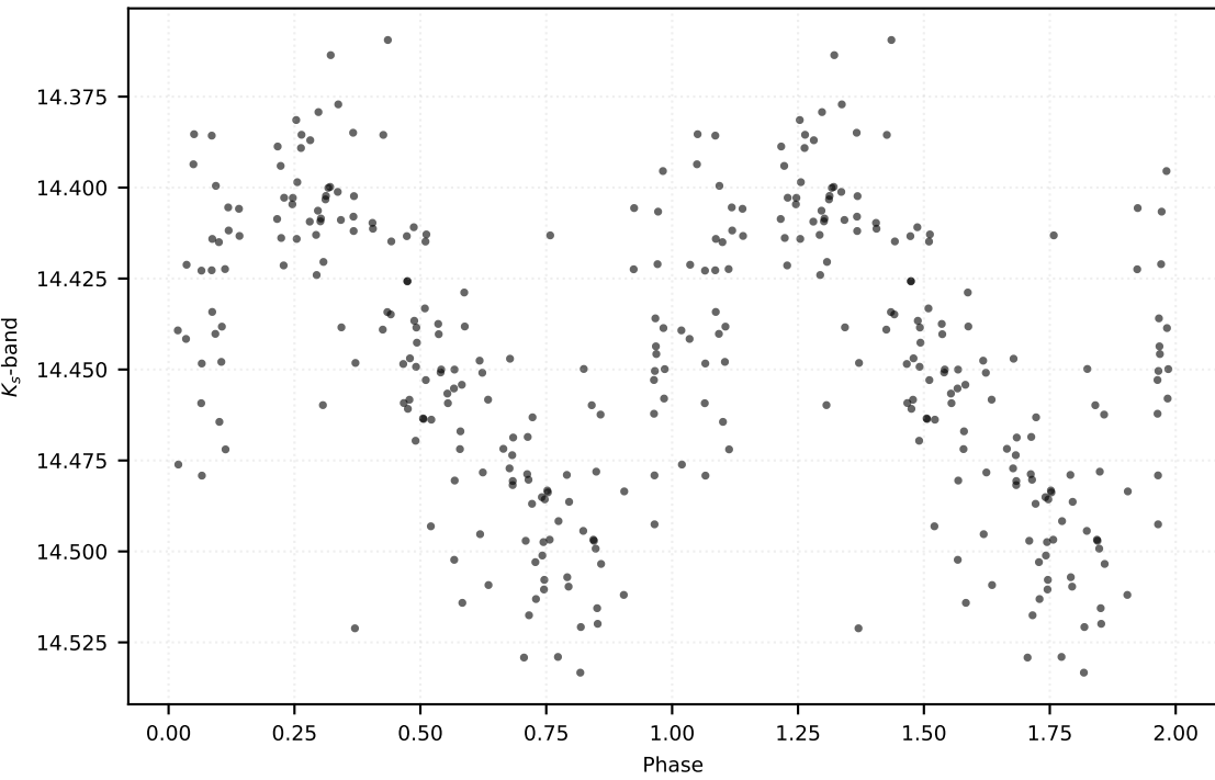
P: 0.42765 d | Class: RP | Subclass: RRab | Field b278
