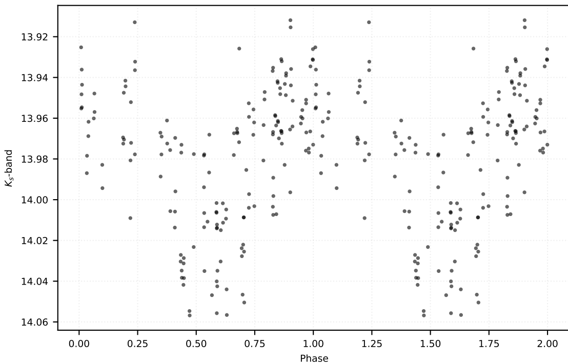
P: 0.38681 d | Class: RP | Subclass: CEP-10T | Field b278
