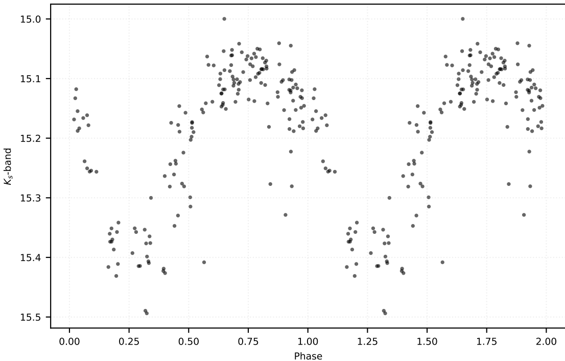
P: 0.13918 d | Class: RP | Subclass: UVAR | Field b278
