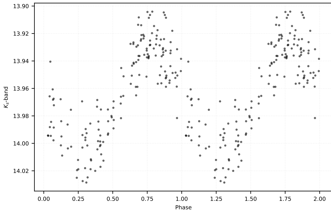
P: 0.45268 d | Class: RP | Subclass: RRc | Field b279
