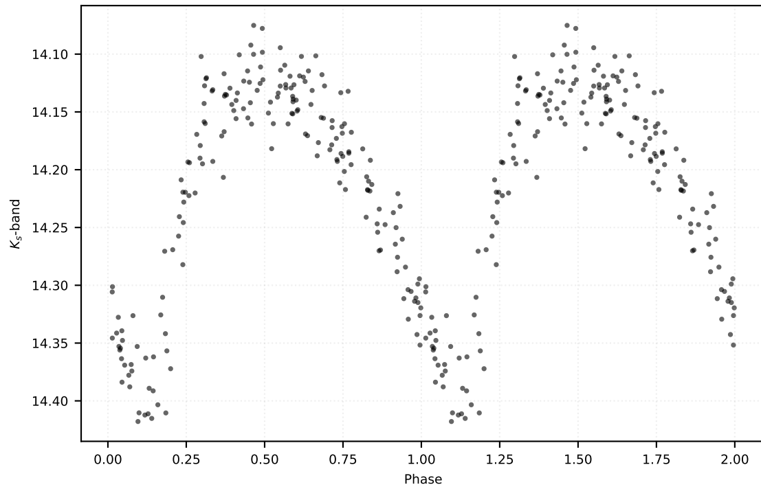
P: 0.44857 d | Class: RP | Subclass: RRab | Field b278
