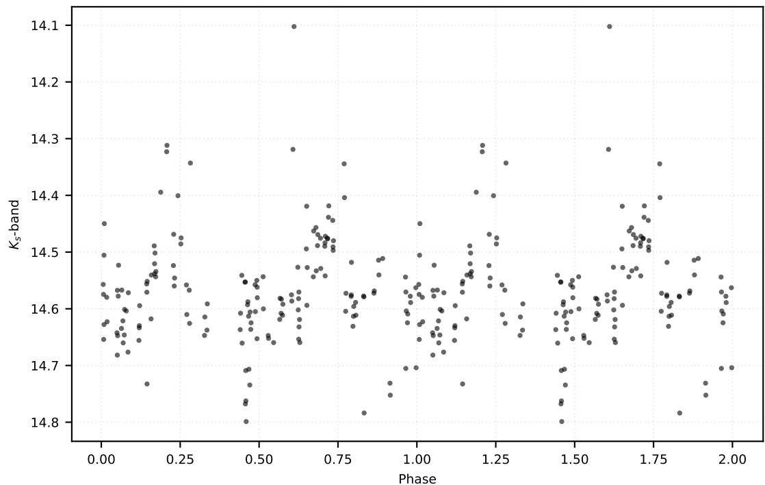
P: 27.94427 d | Class: EB | Subclass: EA | Field b278
