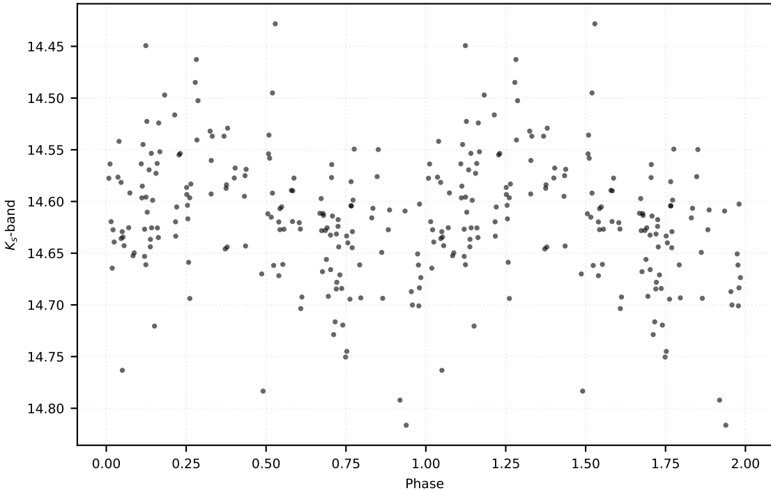
P: 0.21922 d | Class: RP | Subclass: UVAR | Field b279
