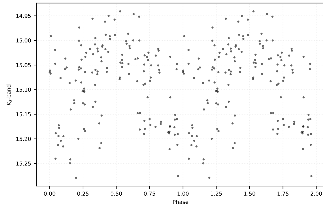
P: 0.23394 d | Class: RP | Subclass: UVAR | Field b279
