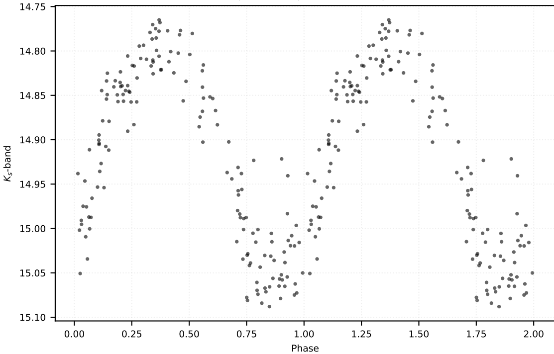
P: 0.47496 d | Class: EB | Subclass: RRc | Field b278
