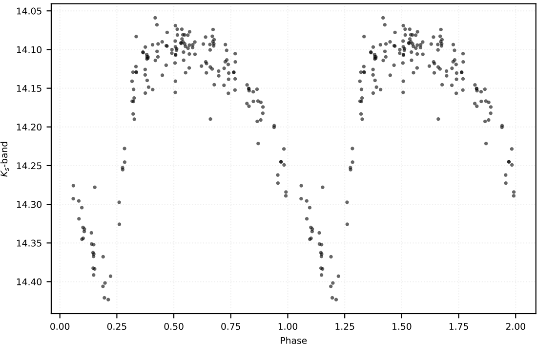
P: 0.54512 d | Class: RP | Subclass: RRab | Field b278
