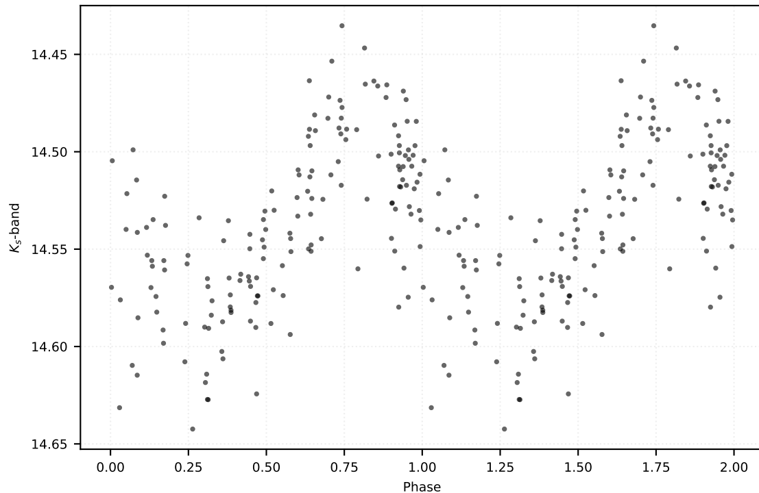
P: 0.44981 d | Class: RP | Subclass: RRab | Field b279
