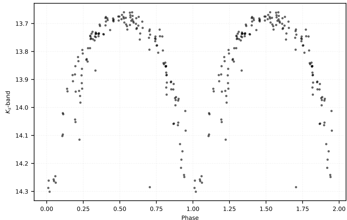
P: 3.41249 d | Class: EB | Subclass: UVAR | Field b279
