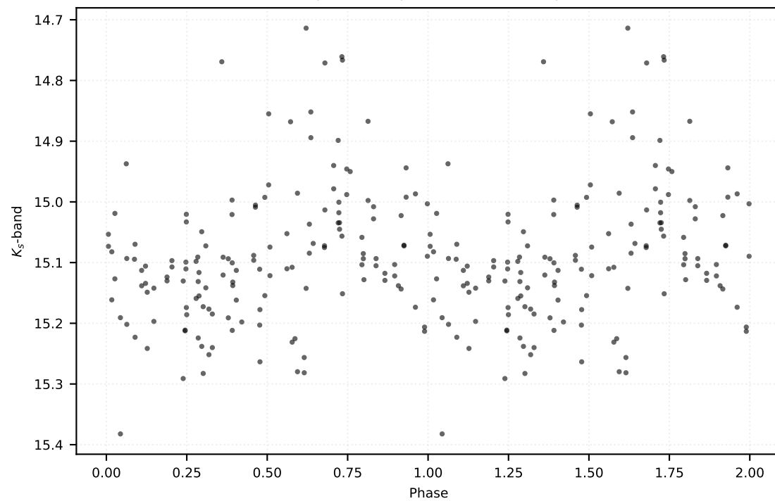
P: 0.24652 d | Class: RP | Subclass: CEP-10T | Field b278
