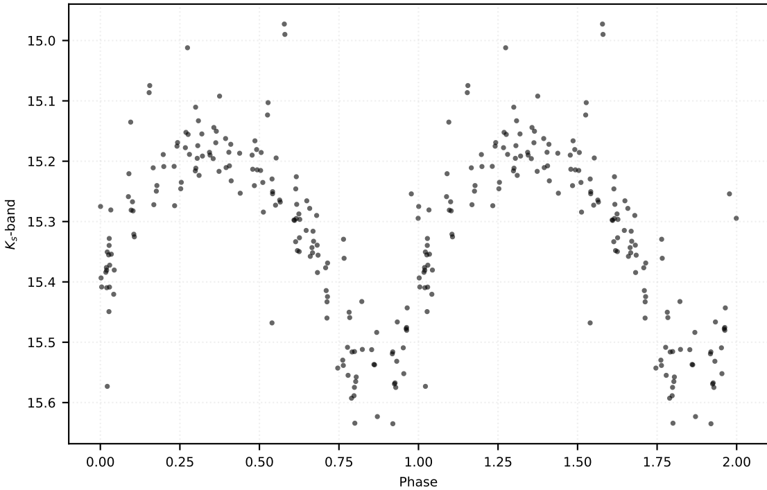
P: 0.25446 d | Class: RP | Subclass: UVAR | Field b278
