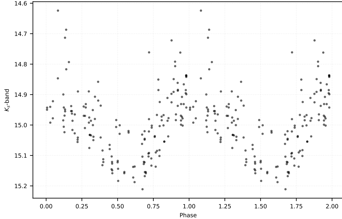
P: 0.60365 d | Class: RP | Subclass: RRab | Field b279
