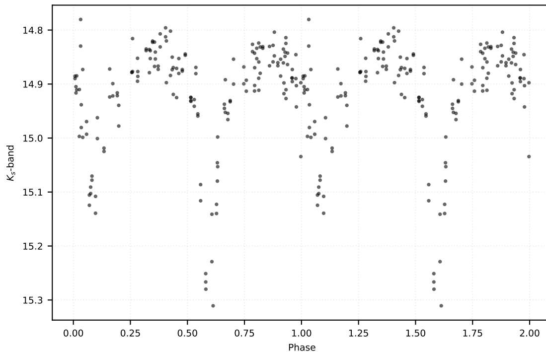
P: 3.32360 d | Class: EB | Subclass: EA | Field b279
