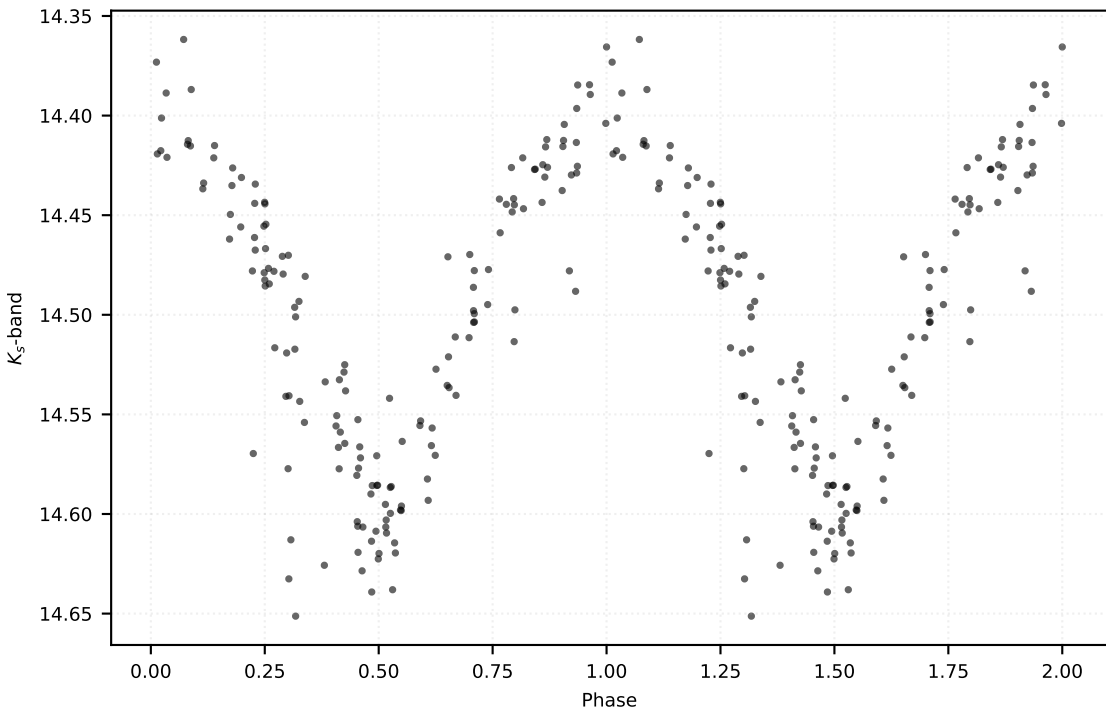
P: 0.29876 d | Class: RP | Subclass: CEP-1OT | Field b279
