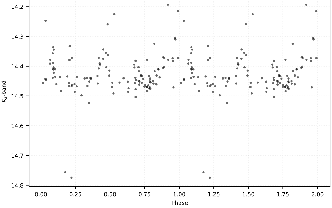
P: 0.21310 d | Class: EB | Subclass: EA | Field b278
