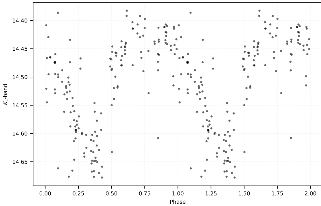
P: 0.57701 d | Class: RP | Subclass: RRab | Field b279
