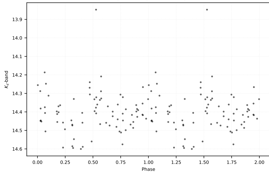
P: 0.22320 d | Class: EB | Subclass: EA | Field b279
