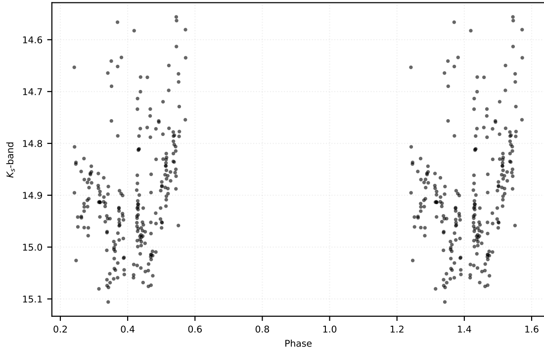
P: 0.73114 d | Class: RP | Subclass: RRab | Field b278
