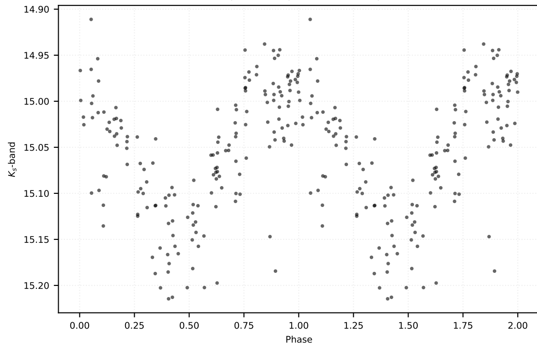
P: 0.39322 d | Class: RP | Subclass: RRab | Field b279
