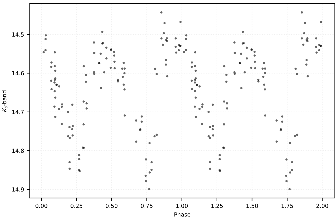
P: 0.38477 d | Class: EB | Subclass: EW | Field b279
