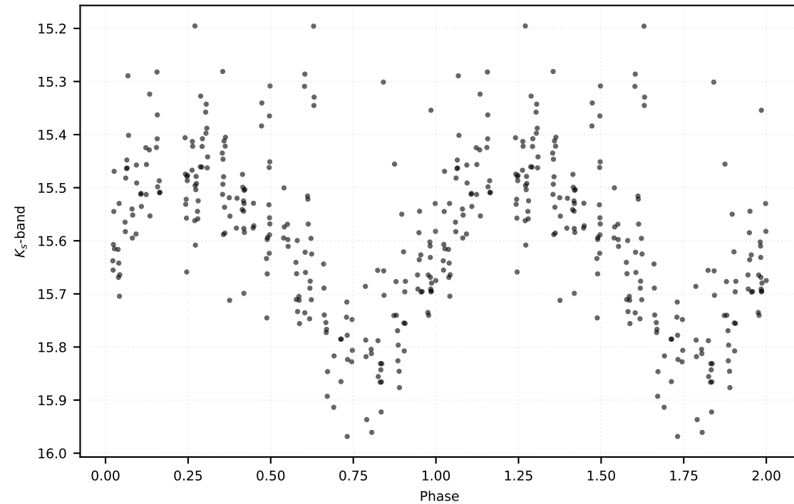
P: 0.47801 d | Class: RP | Subclass: RRab | Field b279
