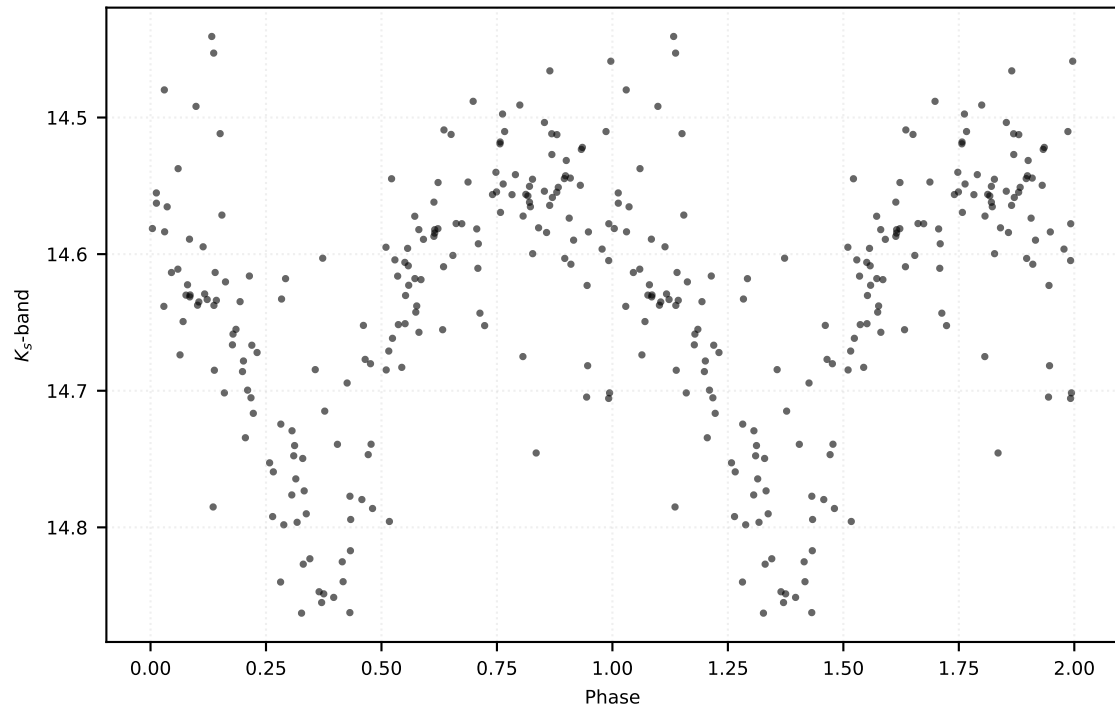
P: 0.74802 d | Class: RP | Subclass: CEP-10T | Field b278
