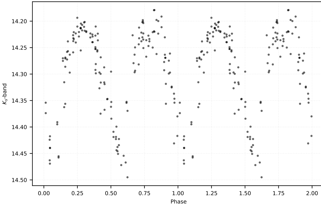
P: 0.20038 d | Class: RP | Subclass: UVAR | Field b278
