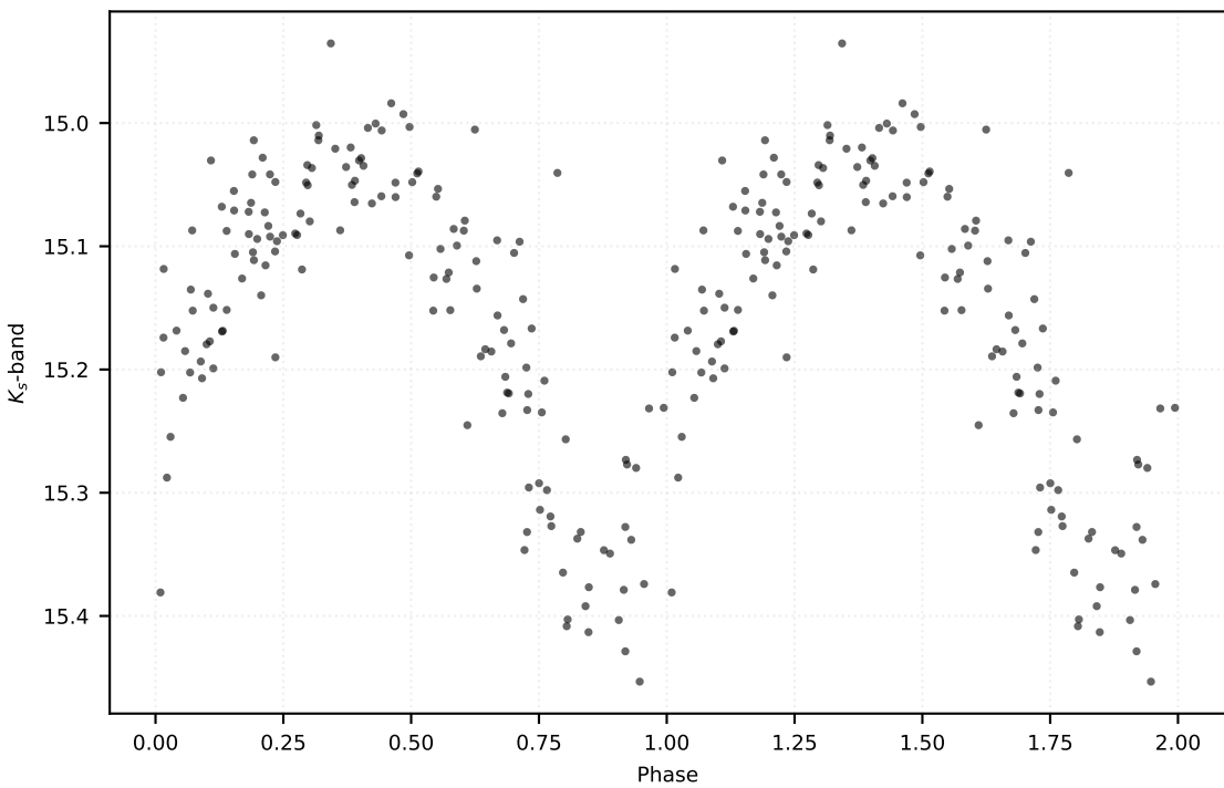
P: 0.36115 d | Class: EB | Subclass: UVAR | Field b279
