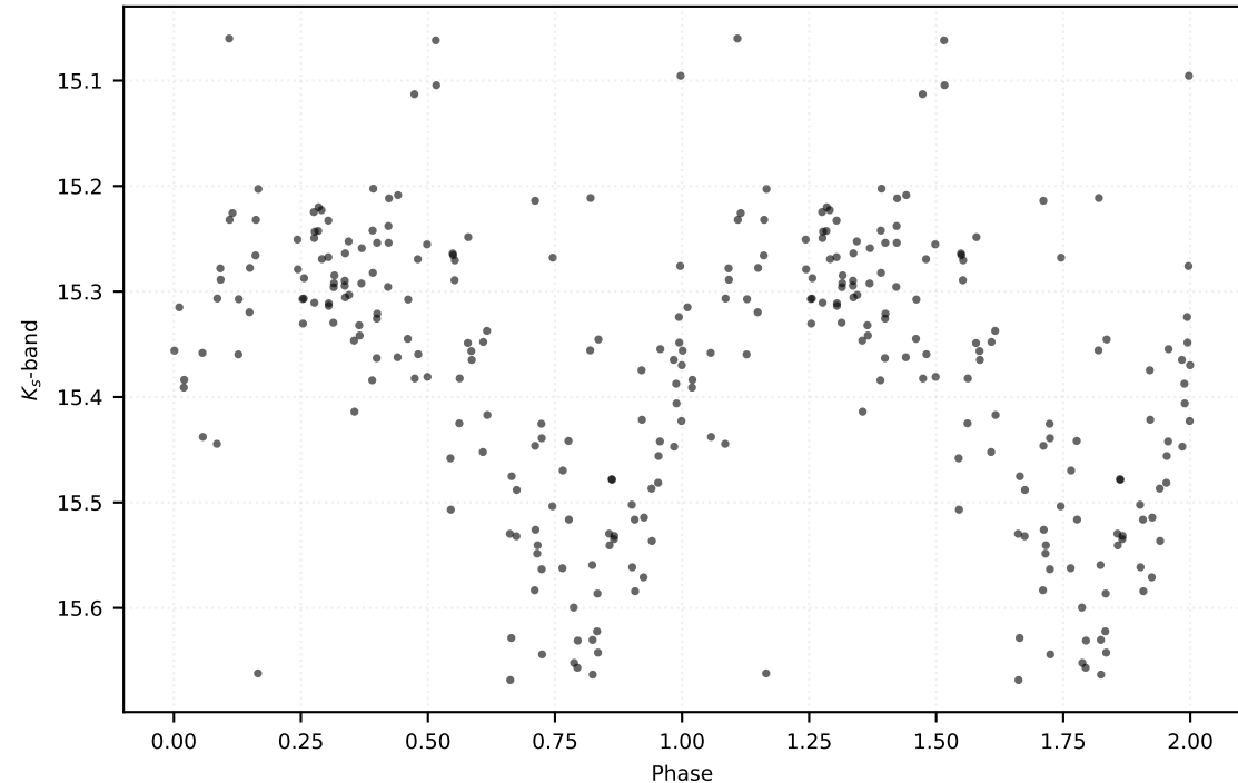
P: 0.30742 d | Class: RP | Subclass: CEP-1OT | Field b278
