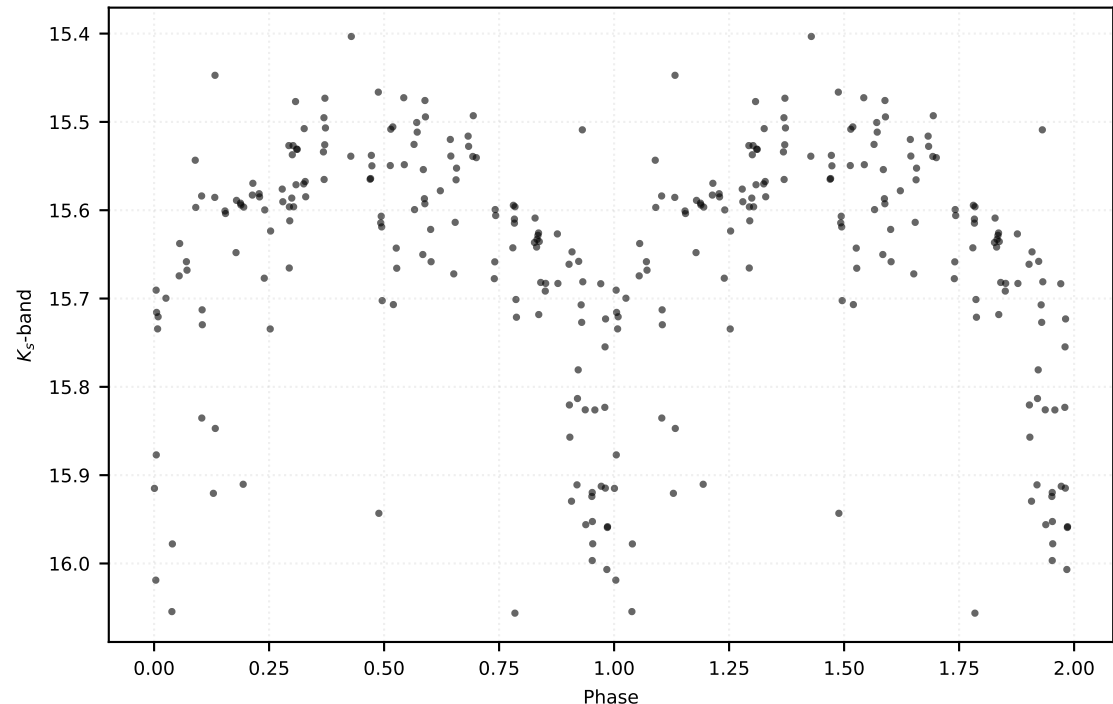
P: 6.61461 d | Class: RP | Subclass: CEP-1OT | Field b278
