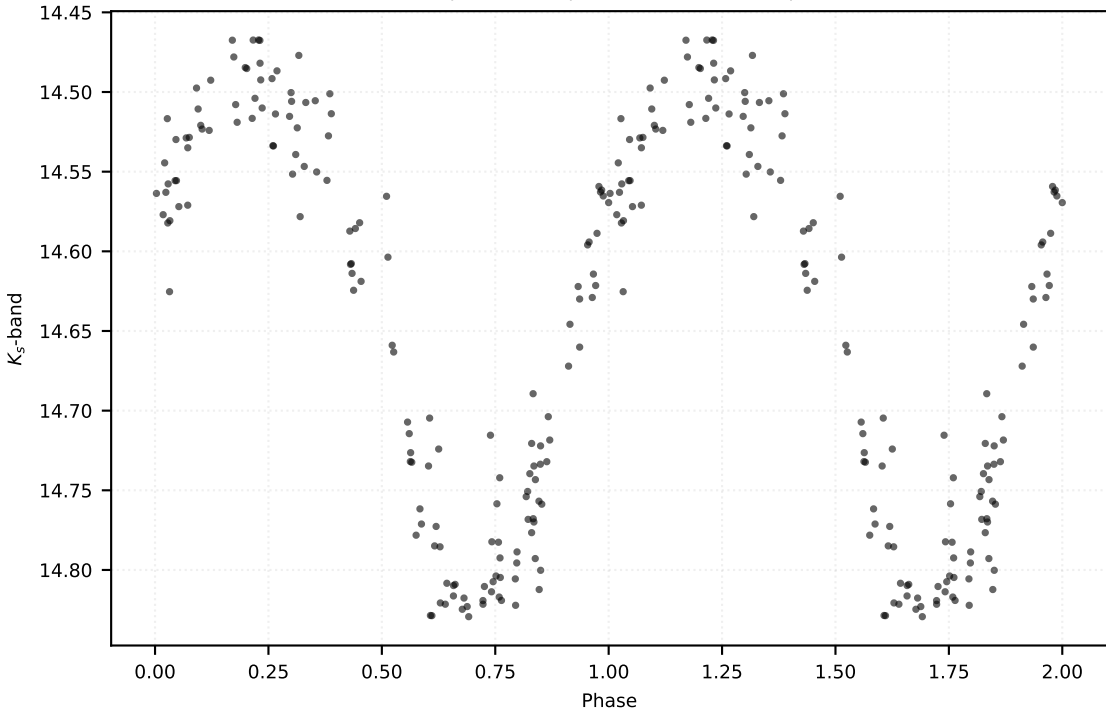
P: 0.24540 d | Class: RP | Subclass: CEP-1OT | Field b279
