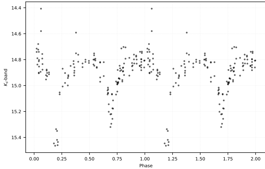
P: 2.18702 d | Class: EB | Subclass: EA | Field b278
