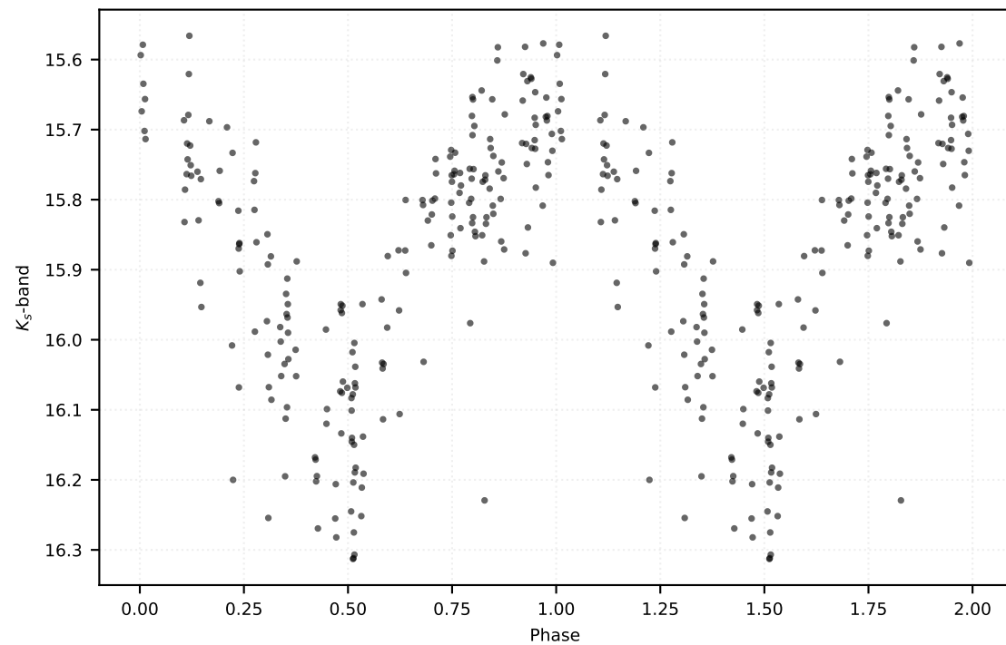
P: 0.47409 d | Class: RP | Subclass: RRab | Field b278
