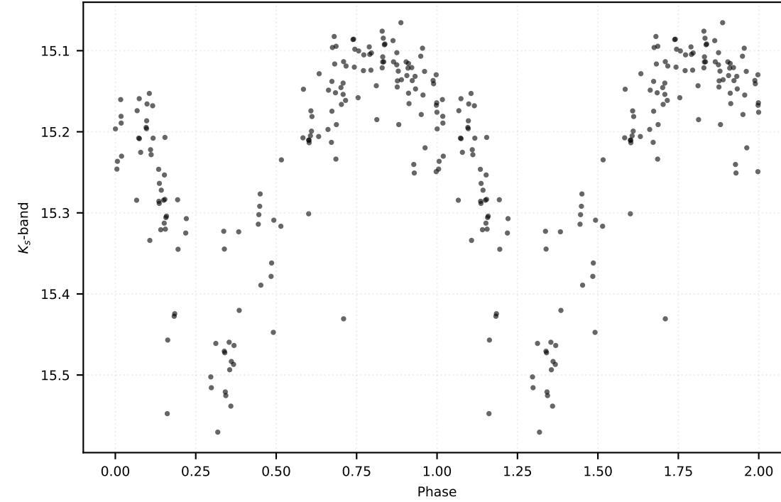
P: 0.50787 d | Class: RP | Subclass: RRc | Field b279
