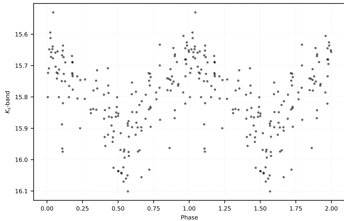
P: 0.38713 d | Class: RP | Subclass: RRab | Field b278
