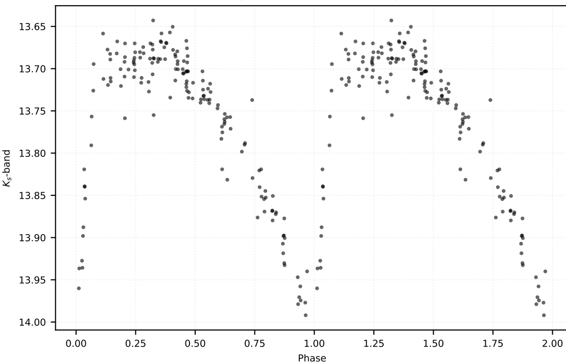
P: 0.44529 d | Class: RP | Subclass: RRab | Field b279
