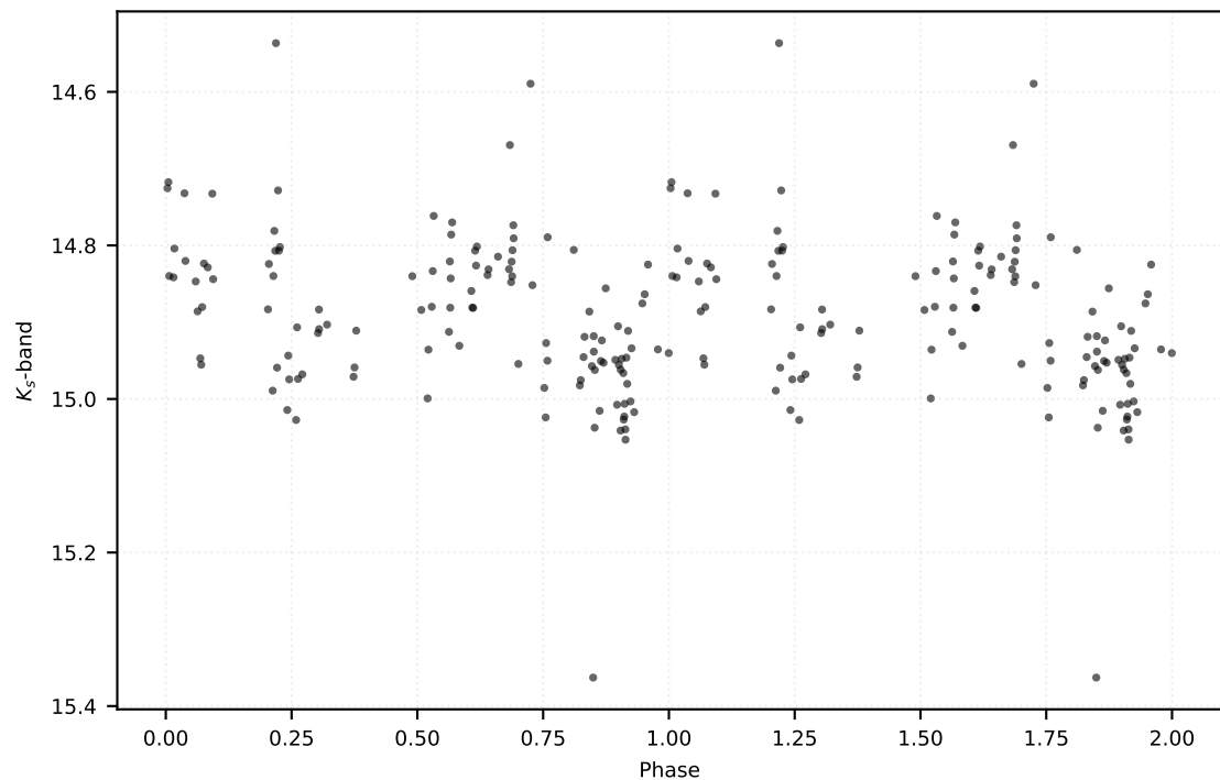
P: 0.22167 d | Class: EB | Subclass: EA | Field b278
