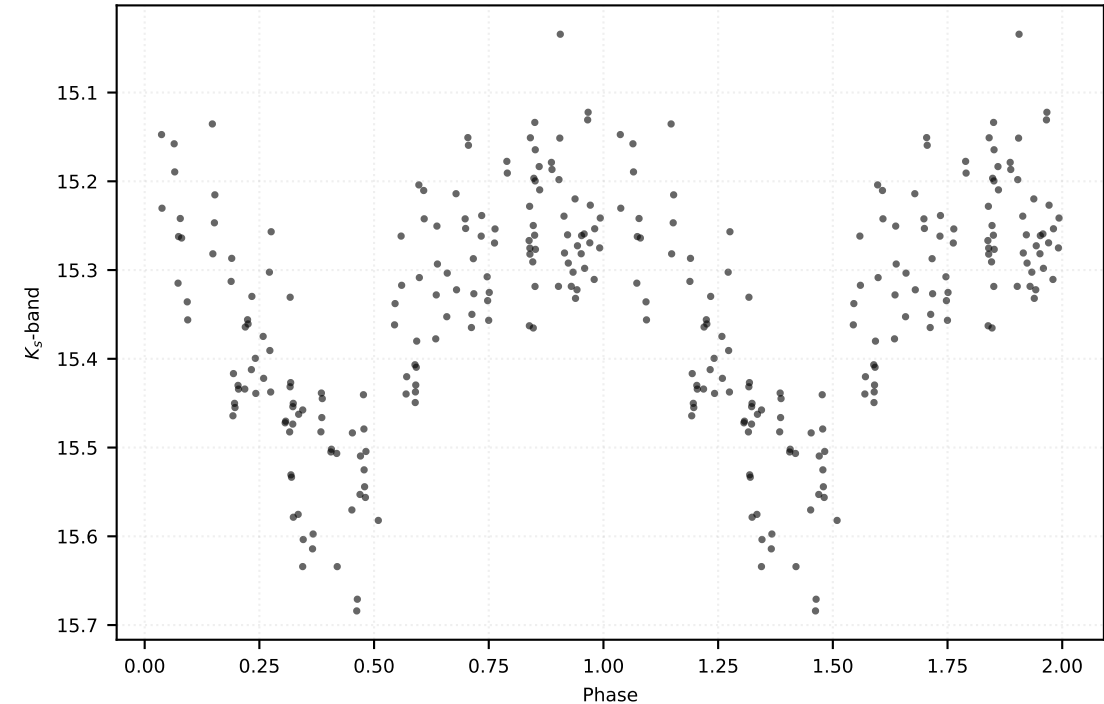
P: 0.60280 d | Class: RP | Subclass: CEP-10T | Field b279
