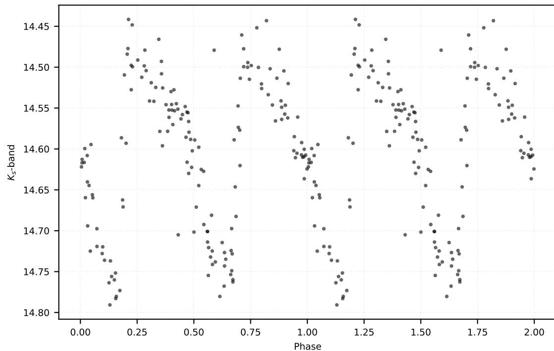
P: 0.20728 d | Class: RP | Subclass: UVAR | Field b278
