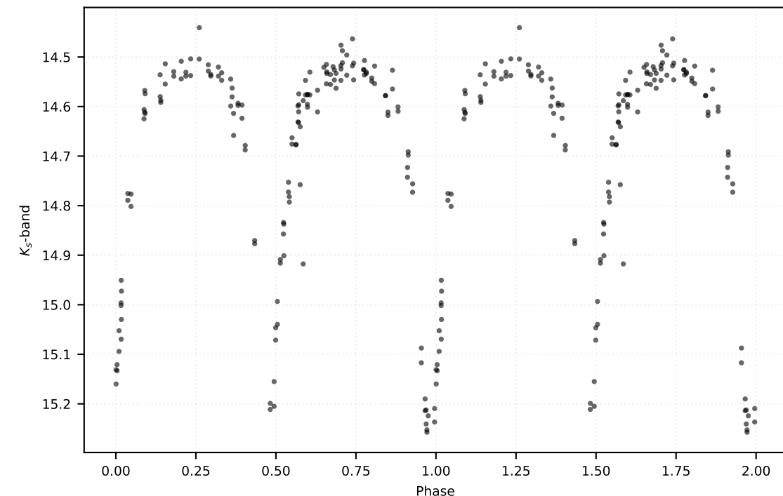
P: 10.44393 d | Class: EB | Subclass: UVAR | Field b279
