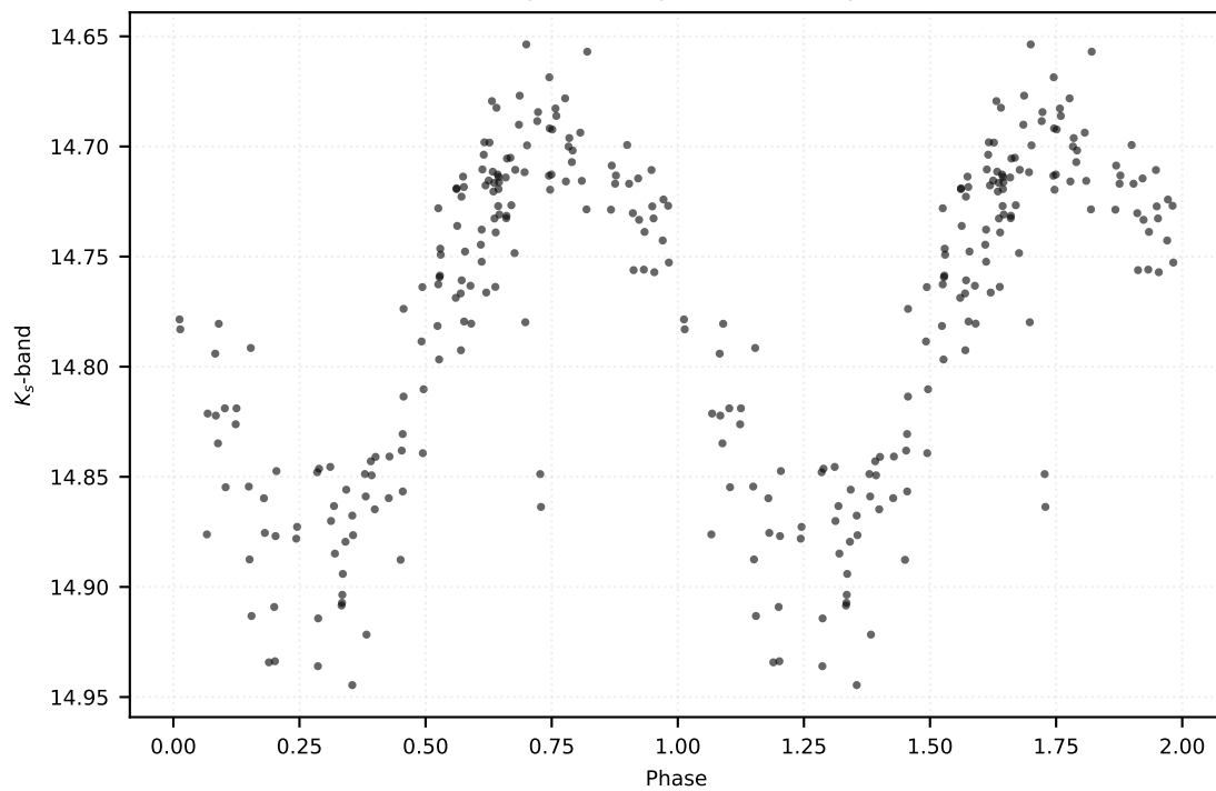
P: 0.37743 d | Class: RP | Subclass: RRc | Field b279
