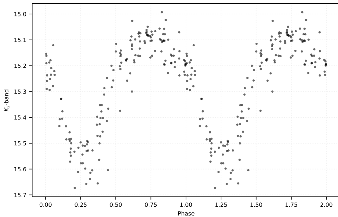
P: 0.14554 d | Class: RP | Subclass: UVAR | Field b278
