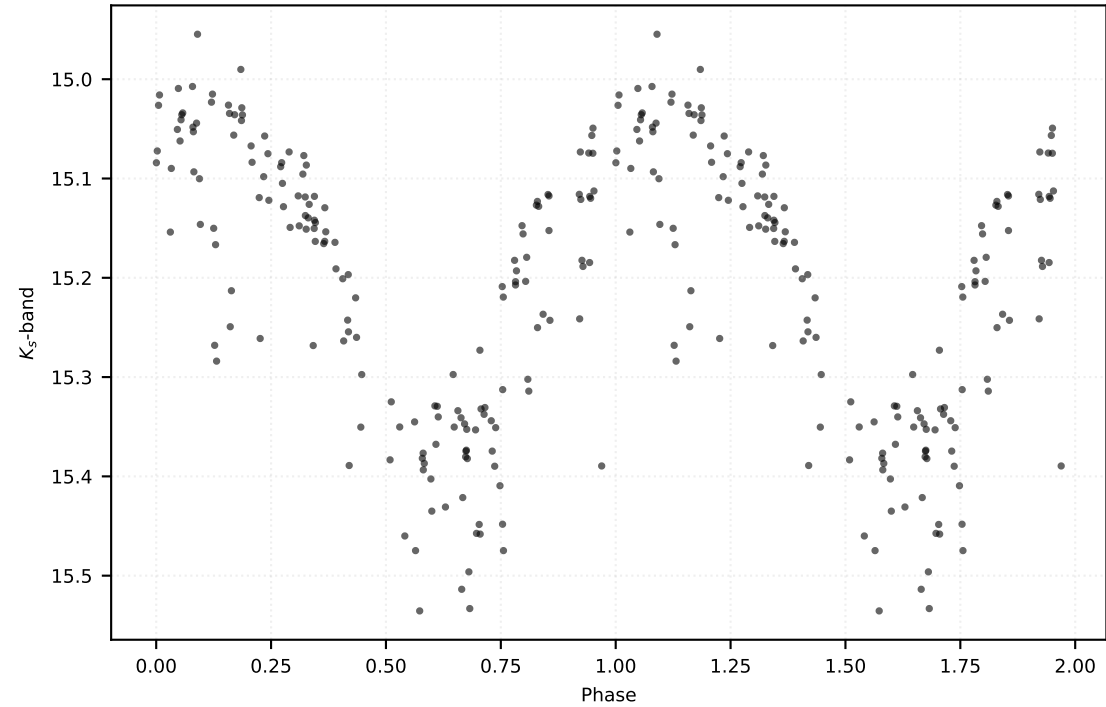
P: 0.77227 d | Class: RP | Subclass: RRab | Field b278
