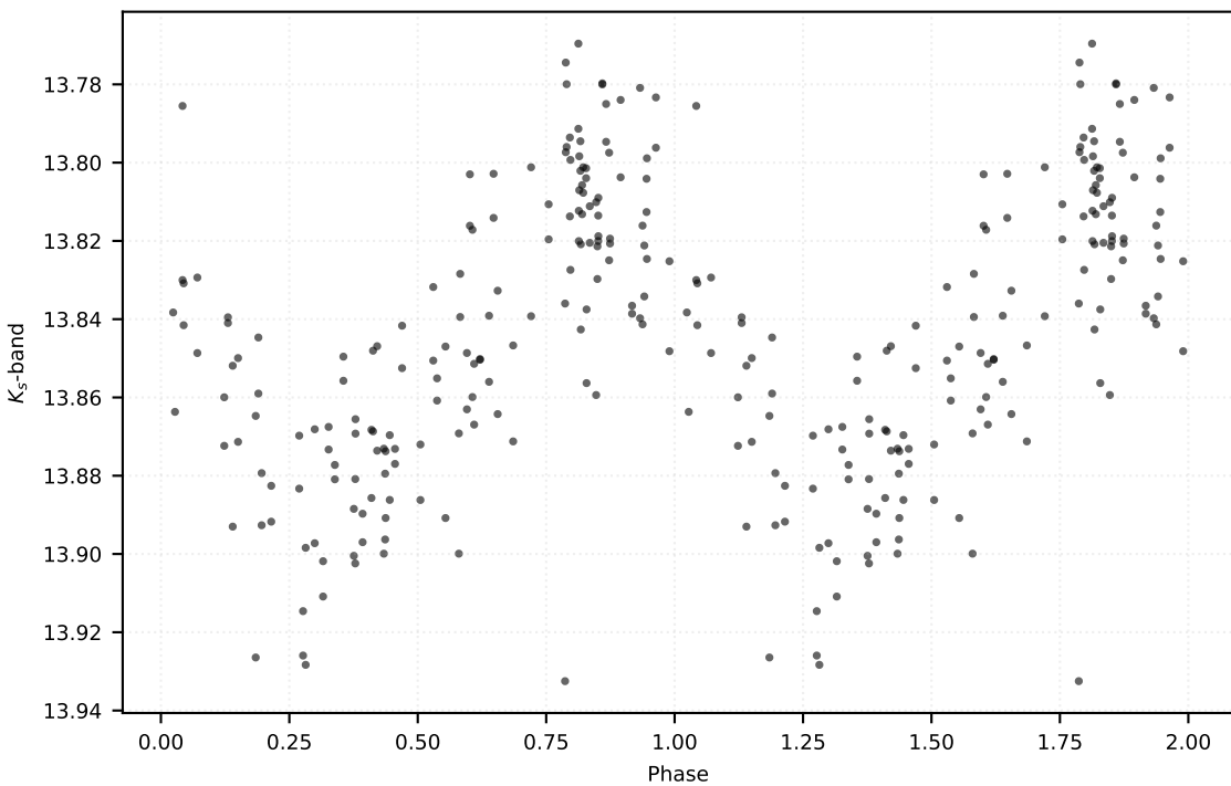
P: 0.27636 d | Class: RP | Subclass: UVAR | Field b279
