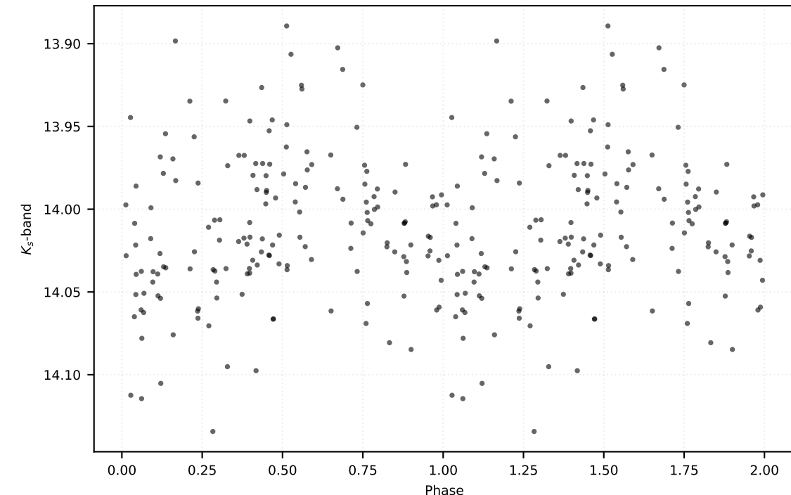
P: 0.44802 d | Class: RP | Subclass: RRab | Field b278
