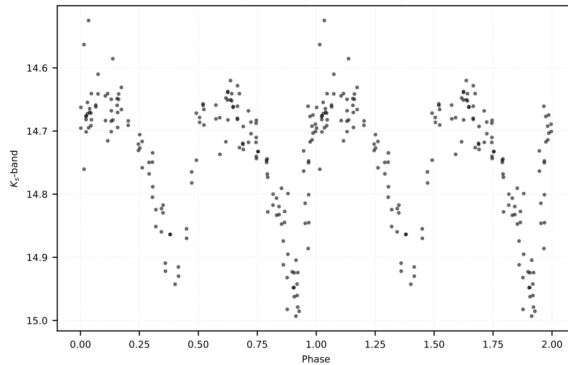
P: 4.00833 d | Class: EB | Subclass: UVAR | Field b278
