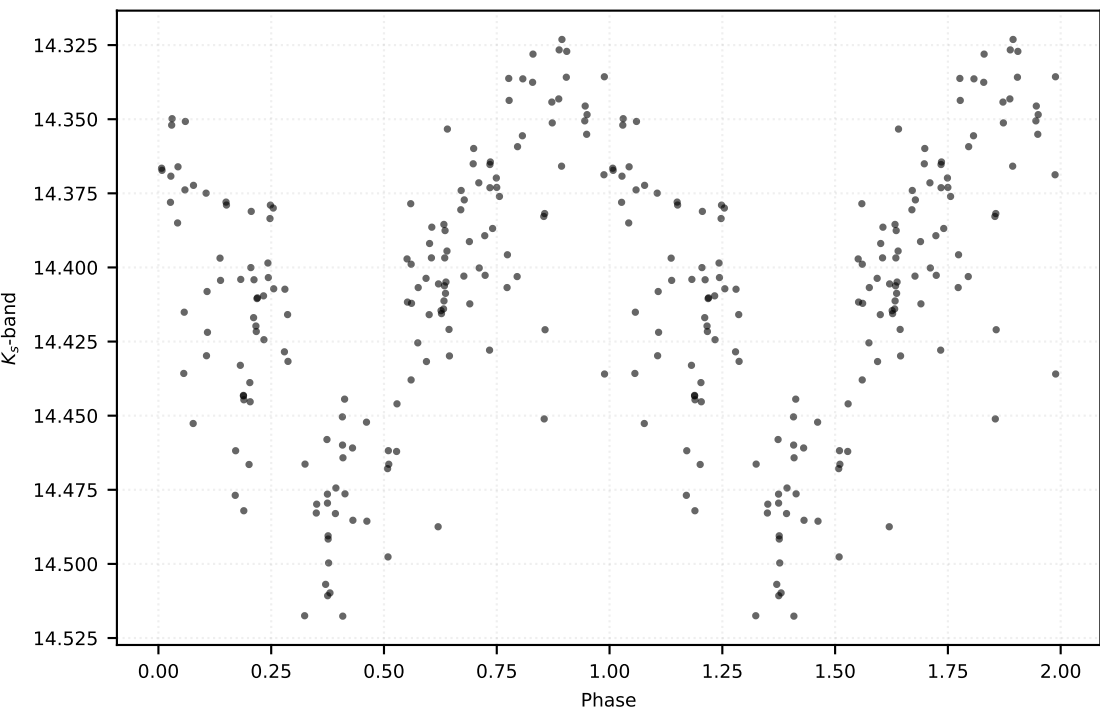
P: 0.41478 d | Class: RP | Subclass: RRc | Field b279
