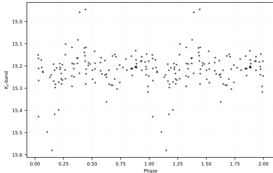
P: 0.34671 d | Class: EB | Subclass: EA | Field b278
