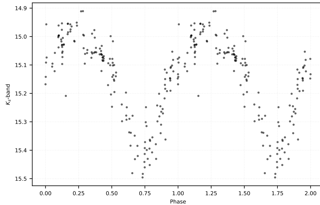
P: 0.97091 d | Class: EB | Subclass: UVAR | Field b278
