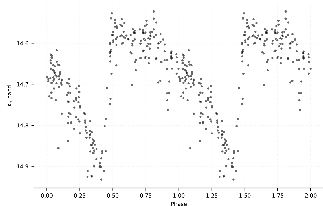
P: 0.43595 d | Class: RP | Subclass: RRab | Field b278
