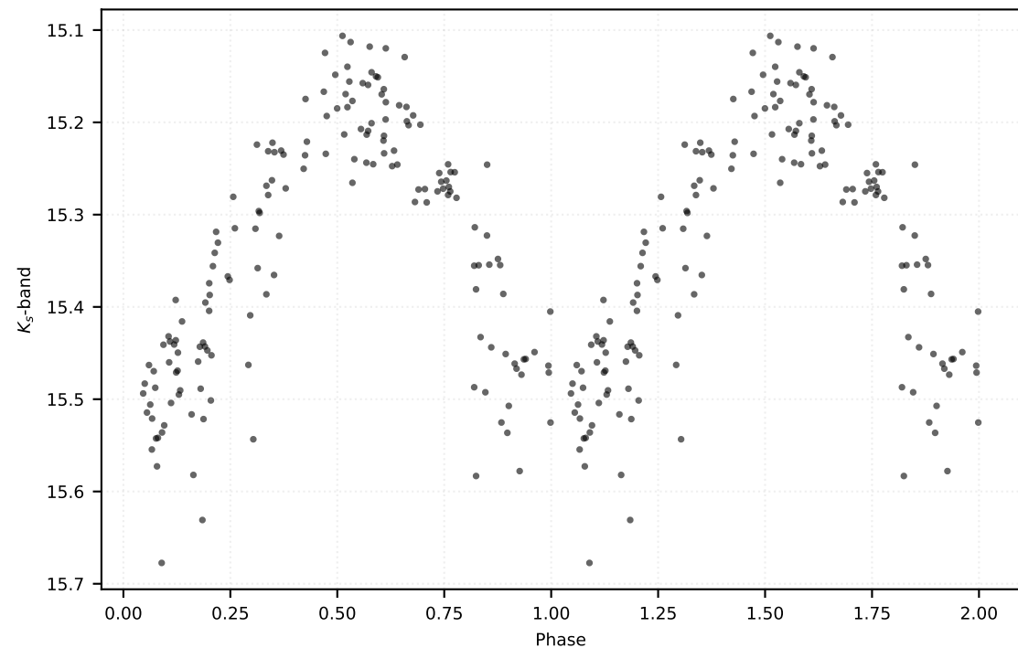
P: 0.23521 d | Class: RP | Subclass: UVAR | Field b278
