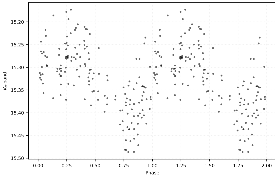
P: 0.12767 d | Class: RP | Subclass: UVAR | Field b279
