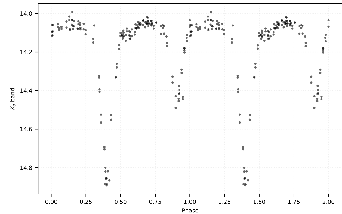
P: 1.18573 d | Class: EB | Subclass: EA | Field b278
