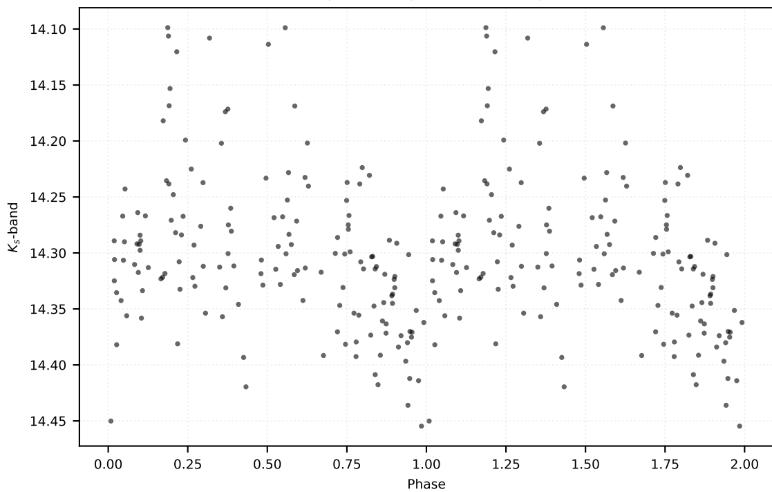
P: 0.11061 d | Class: RP | Subclass: UVAR | Field b279
