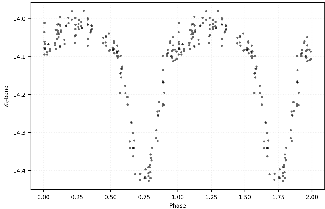
P: 0.61093 d | Class: RP | Subclass: RRab | Field b278
