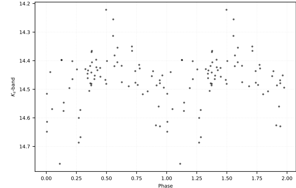
P: 0.83001 d | Class: RP | Subclass: RRab | Field b279
