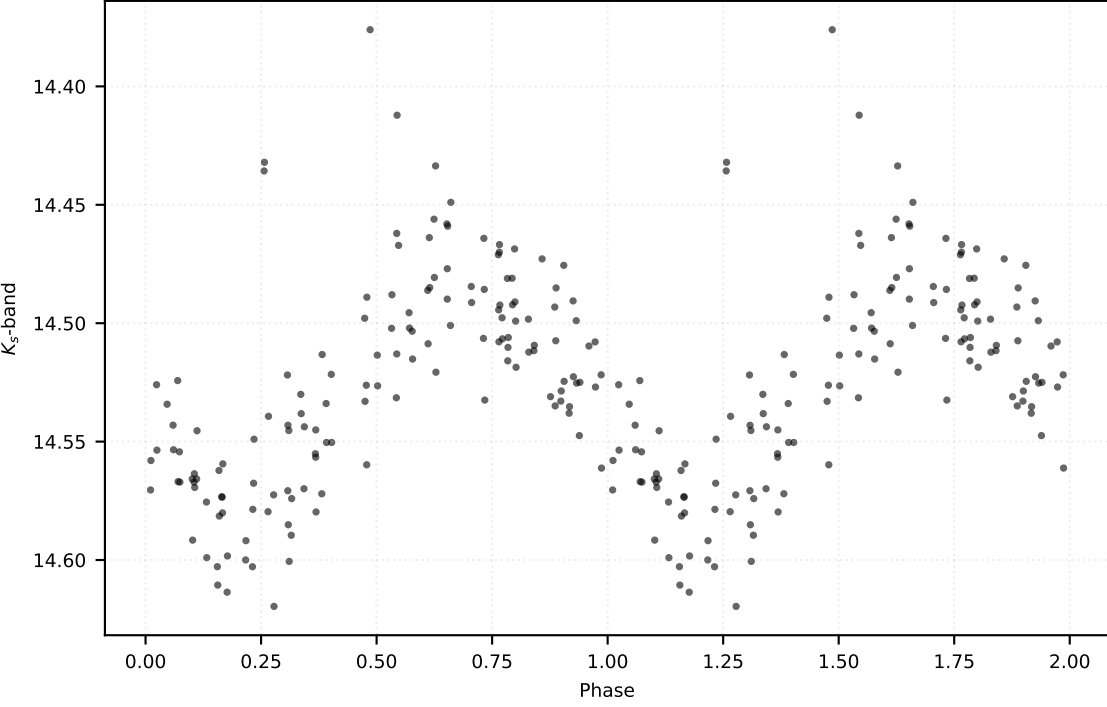
P: 0.42939 d | Class: RP | Subclass: RRab | Field b279
