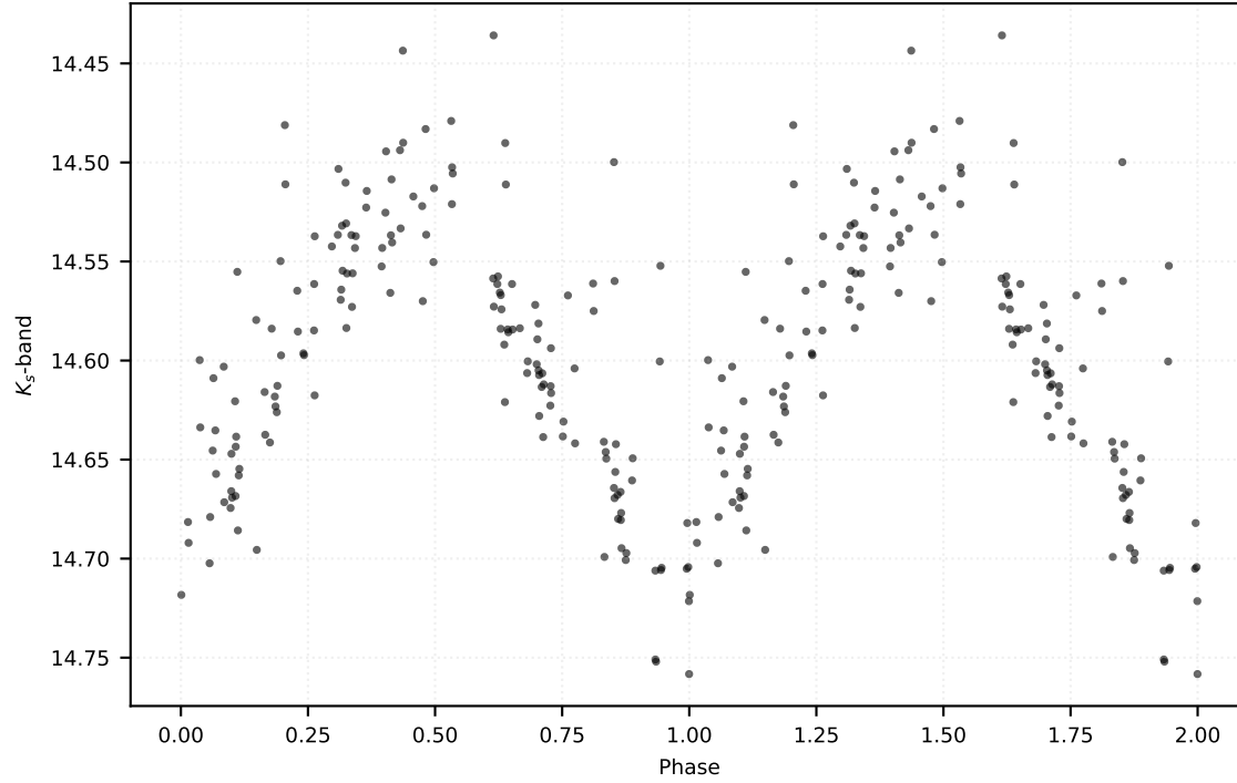
P: 0.33903 d | Class: RP | Subclass: RRab | Field b279
