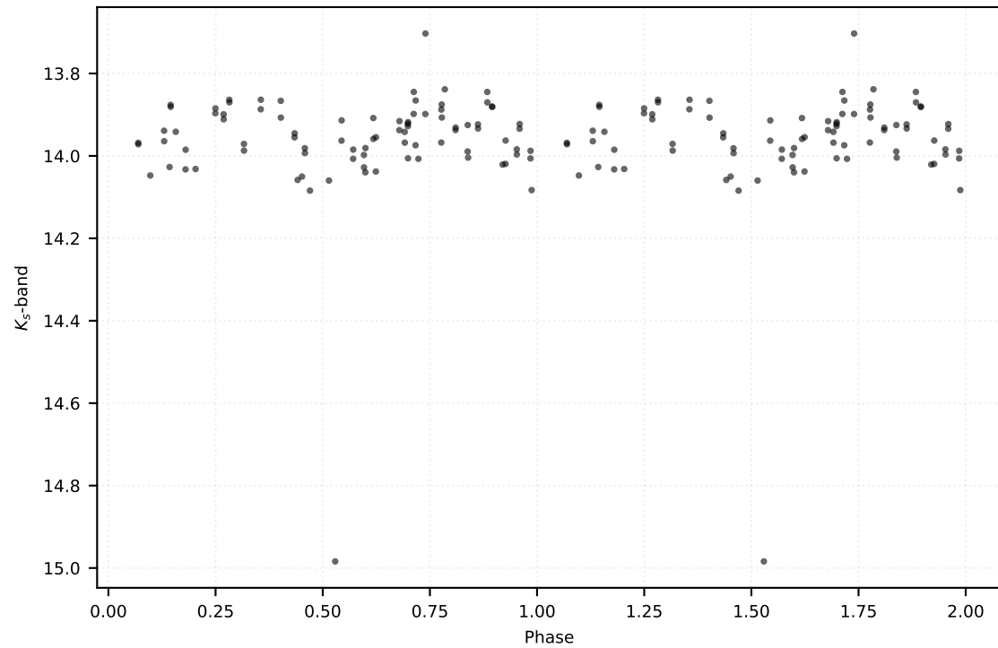
P: 1.89147 d | Class: EB | Subclass: EA | Field b278
