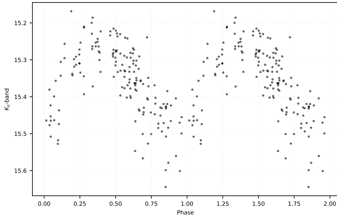
P: 0.65428 d | Class: RP | Subclass: RRab | Field b279
