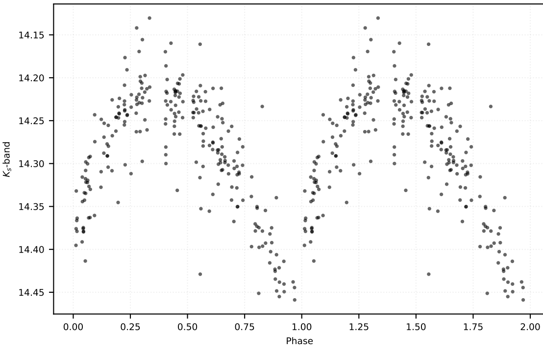
P: 0.57147 d | Class: RP | Subclass: RRab | Field b278
