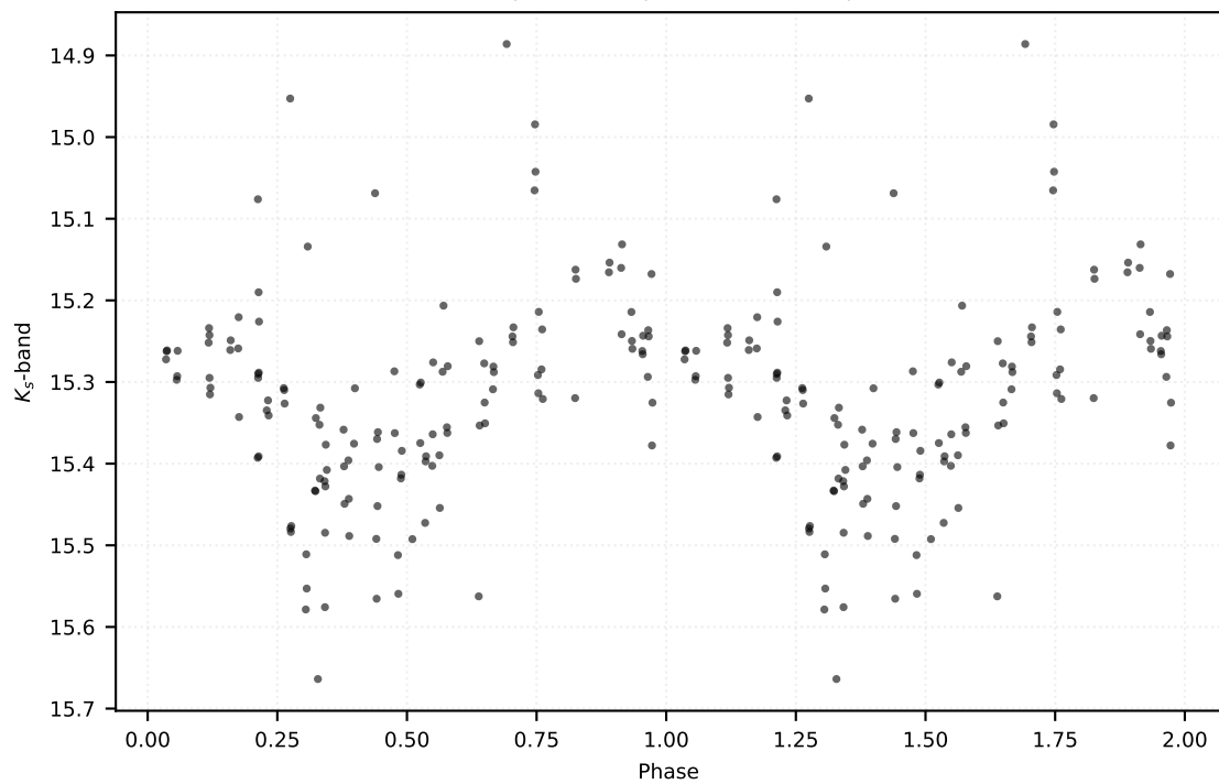
P: 0.44741 d | Class: RP | Subclass: R Rab | Field b278
