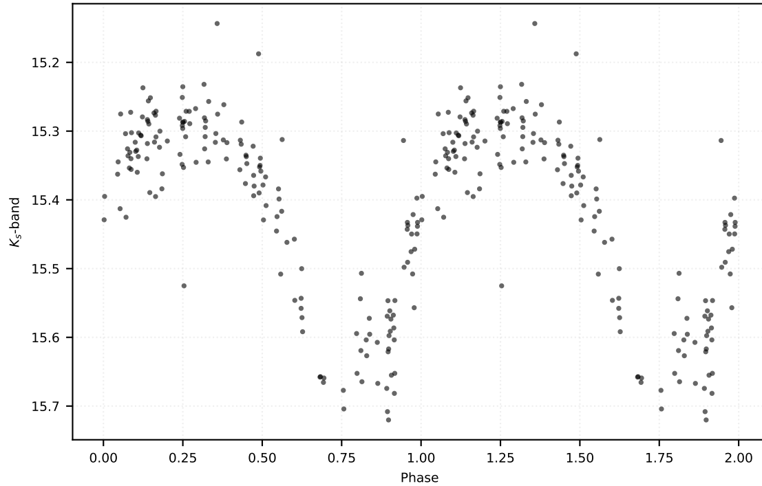
P: 10.51731 d | Class: EB | Subclass: UVAR | Field b278
