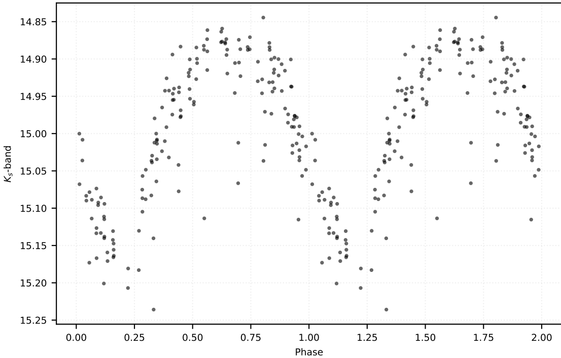
P: 0.43231 d | Class: RP | Subclass: RRab | Field b278
