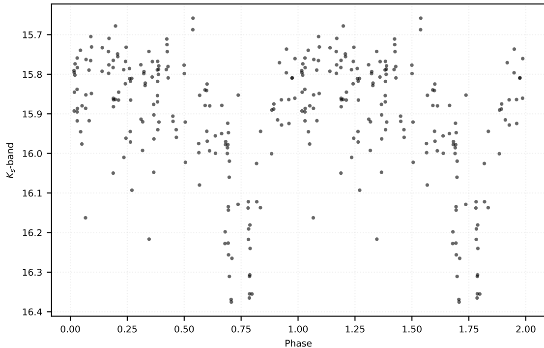
P: 0.52221 d | Class: RP | Subclass: RRab | Field b278
