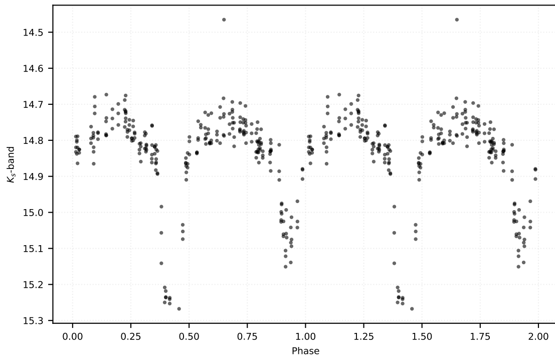
P: 3.49857 d | Class: EB | Subclass: EA | Field b278
