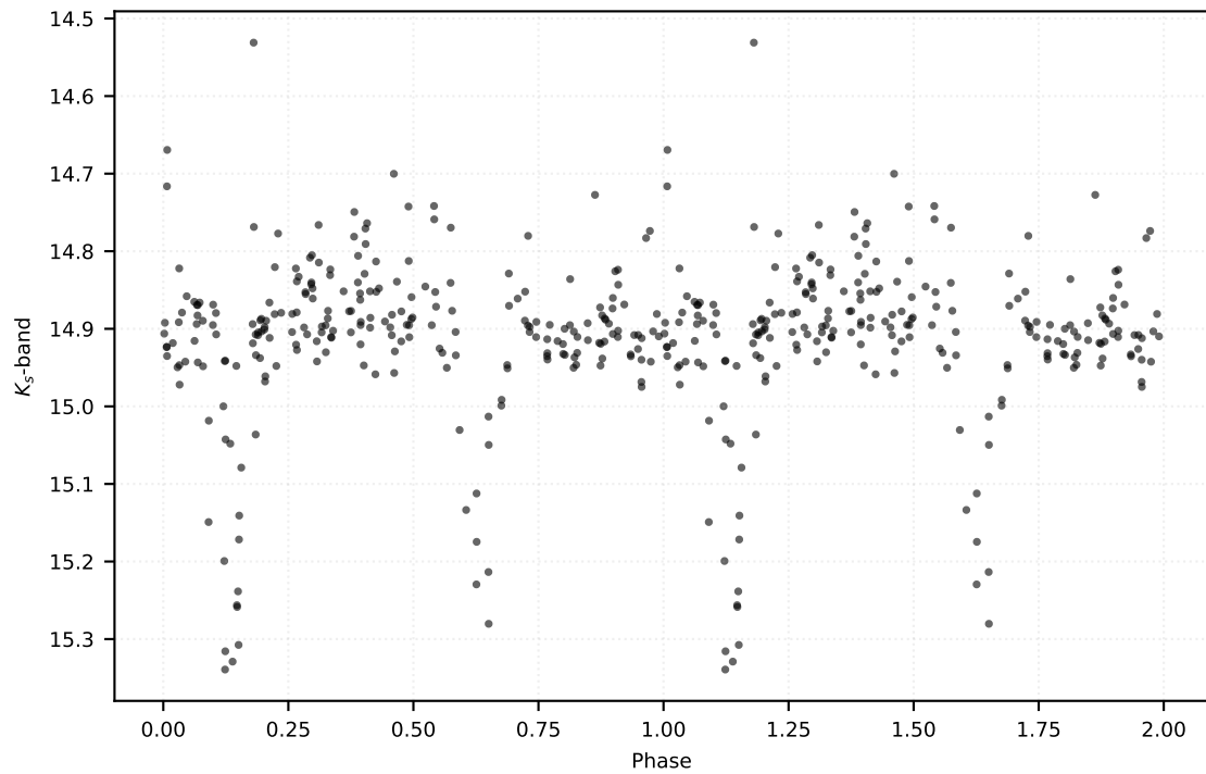
P: 5.34178 d | Class: EB | Subclass: EA | Field b278
