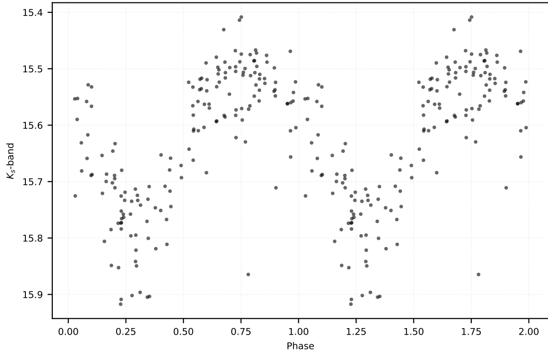
P: 0.21761 d | Class: RP | Subclass: RRc | Field b279
