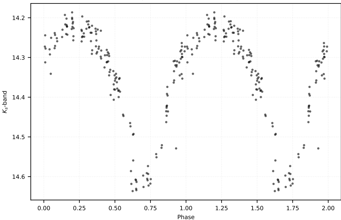
P: 0.15485 d | Class: RP | Subclass: UVAR | Field b279
