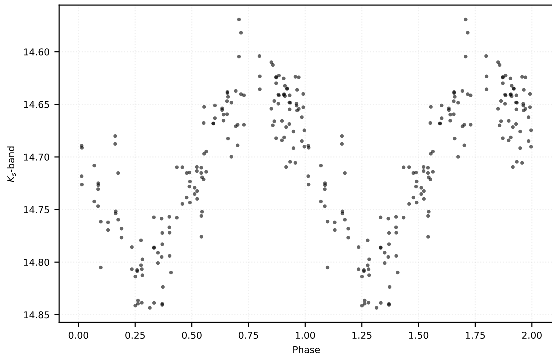
P: 34.07012 d | Class: RP | Subclass: CEP-F | Field b278
