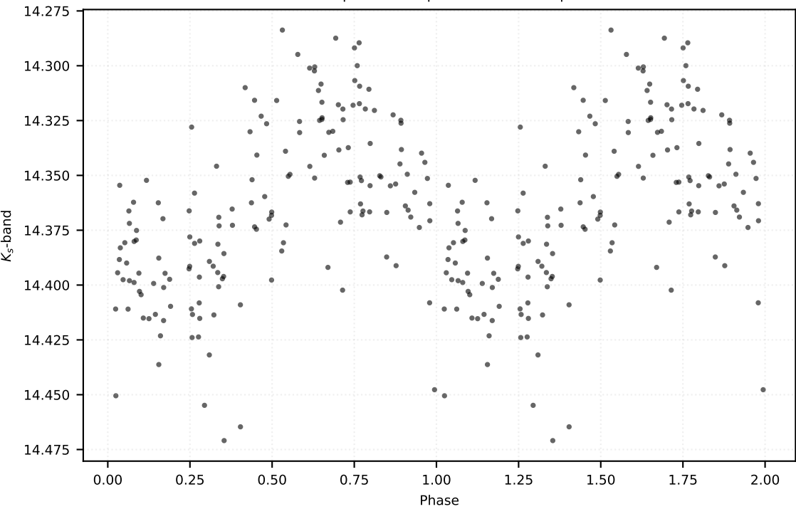
P: 0.11810 d | Class: RP | Subclass: UVAR | Field b279
