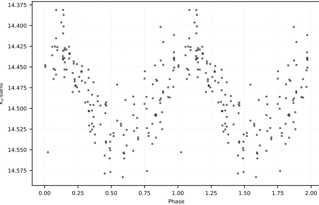
P: 2.85653 d | Class: RP | Subclass: CEP-F | Field b279
