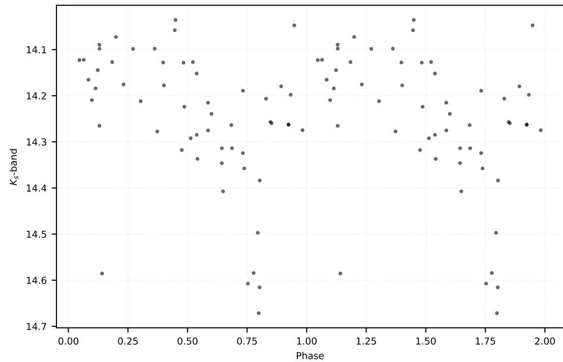
P: 61.80143 d | Class: RP | Subclass: CEP-F | Field b278
