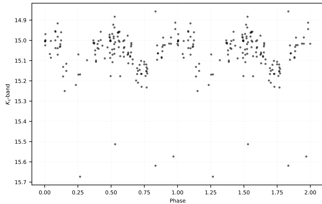
P: 0.62423 d | Class: EB | Subclass: EA | Field b279
