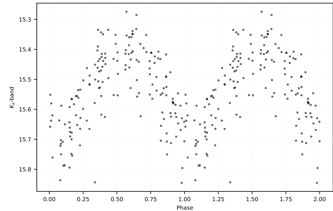
P: 0.59058 d | Class: RP | Subclass: RRc | Field b278
