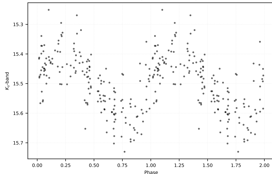
P: 0.30178 d | Class: RP | Subclass: CEP-10T | Field b278
