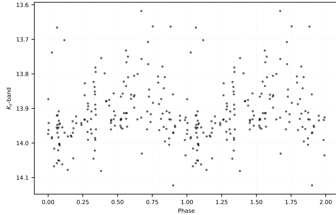
P: 0.57083 d | Class: RP | Subclass: RRab | Field b278
