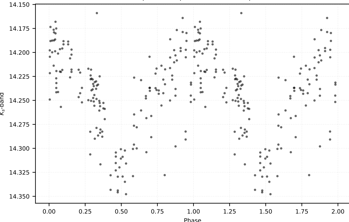
P: 0.41959 d | Class: RP | Subclass: CEP-10T | Field b278
