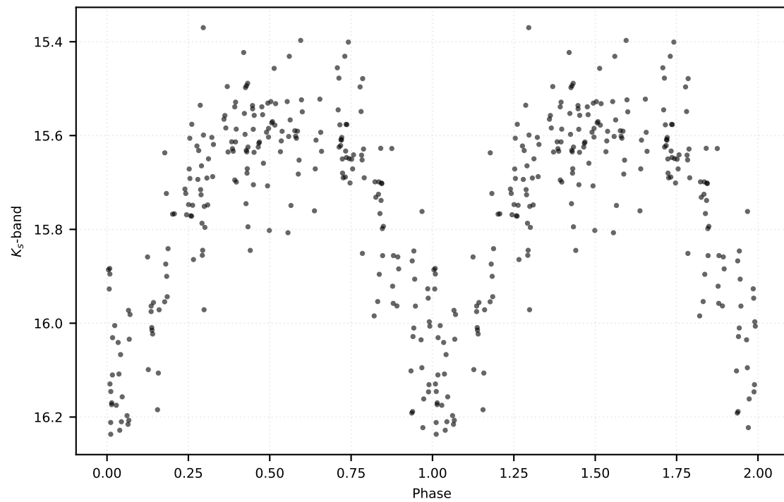
P: 0.13650 d | Class: RP | Subclass: UVAR | Field b279
