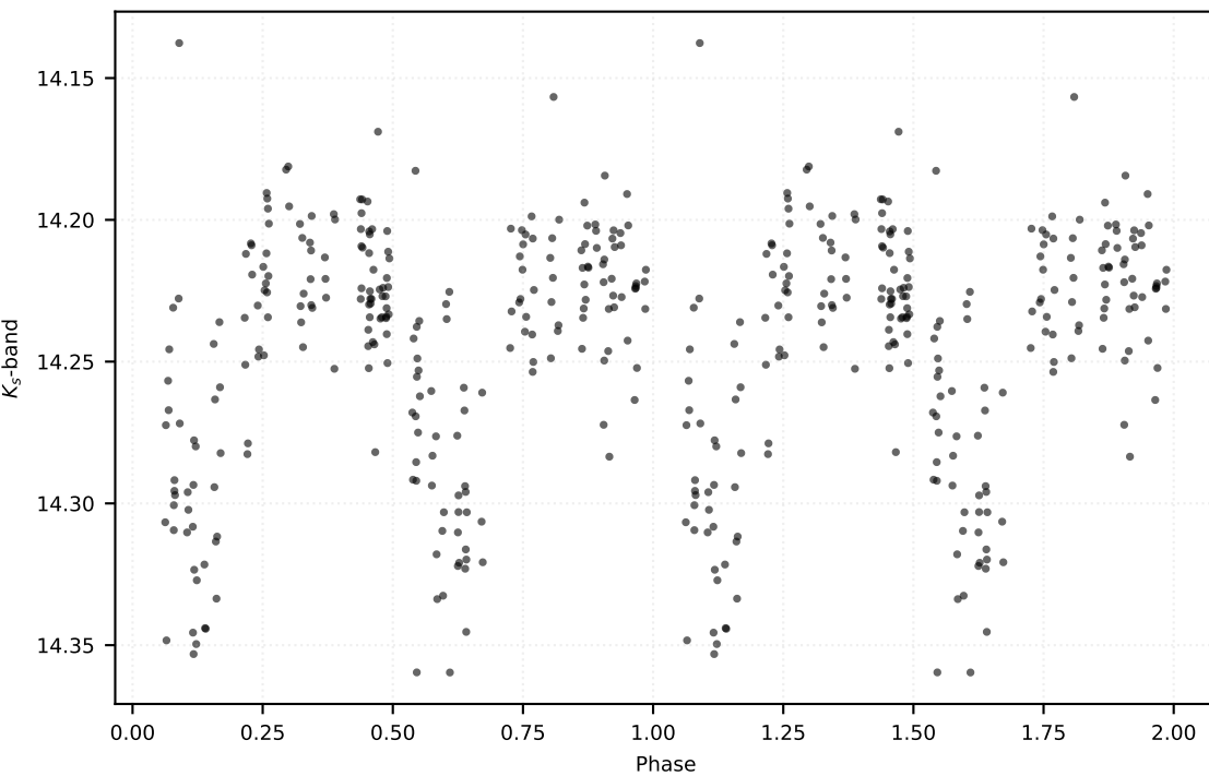
P: 0.21089 d | Class: RP | Subclass: UVAR | Field b279
