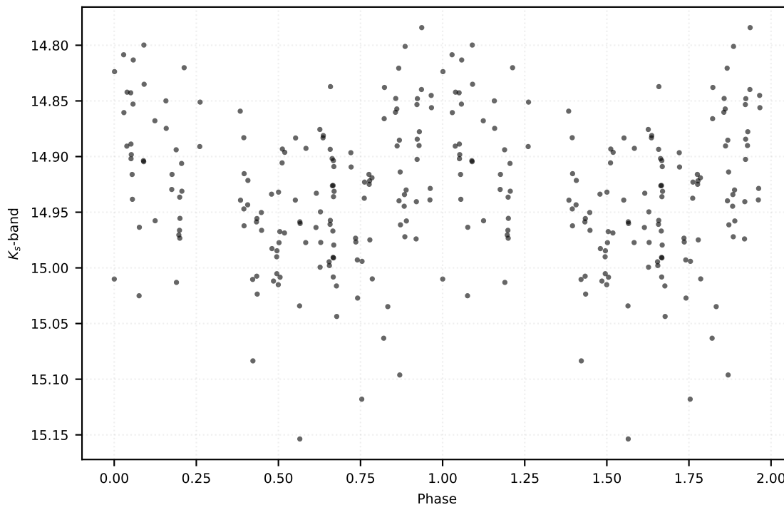
P: 0.38400 d | Class: RP | Subclass: CEP-1OT | Field b278
