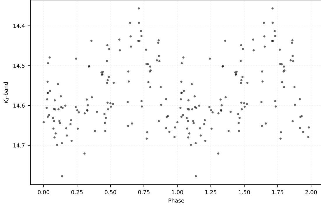
P: 0.11512 d | Class: RP | Subclass: UVAR | Field b278
