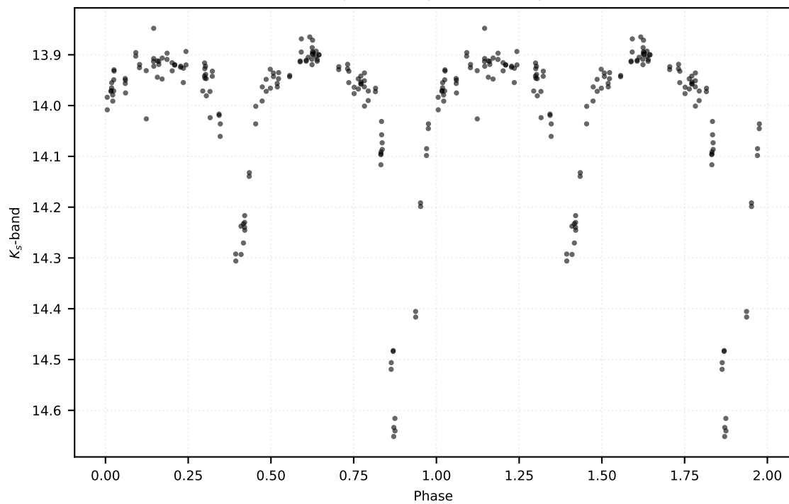
P: 1.86204 d | Class: EB | Subclass: EA | Field b278
