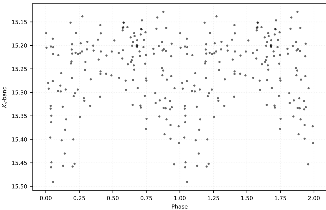
P: 0.12722 d | Class: RP | Subclass: UVAR | Field b279
