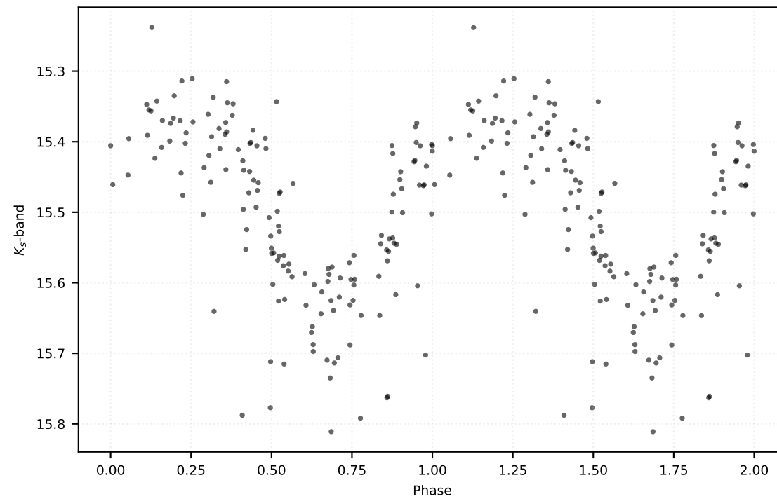
P: 0.24948 d | Class: RP | Subclass: UVAR | Field b279
