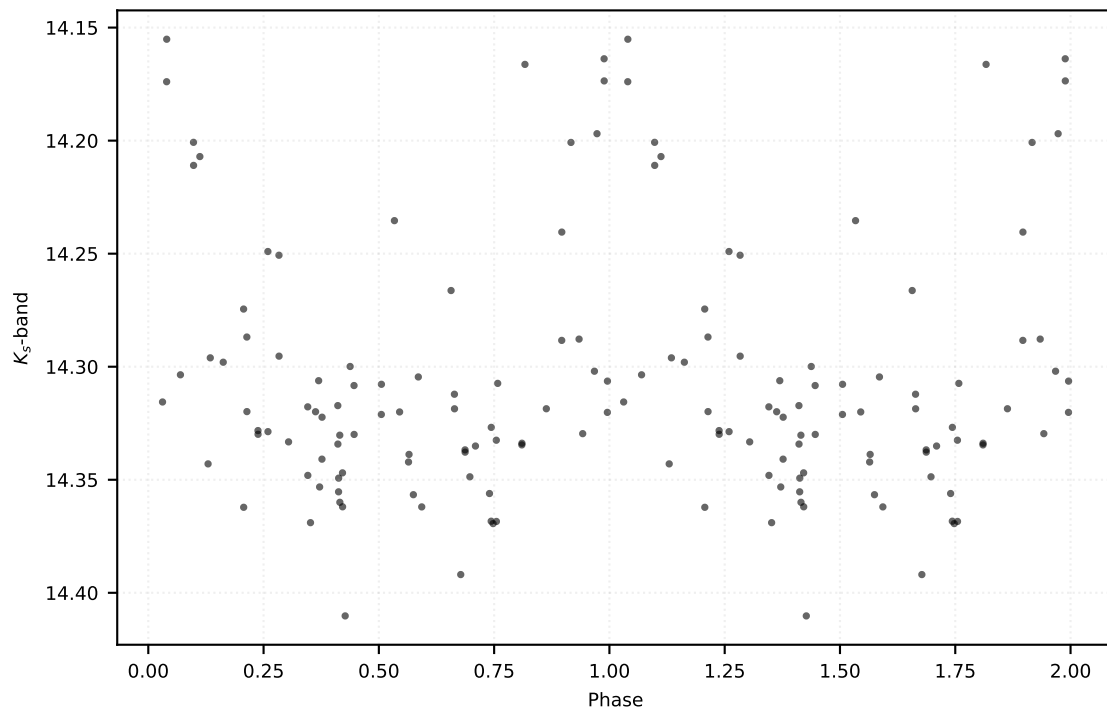
P: 10.73281 d | Class: RP | Subclass: CEP-F | Field b278
