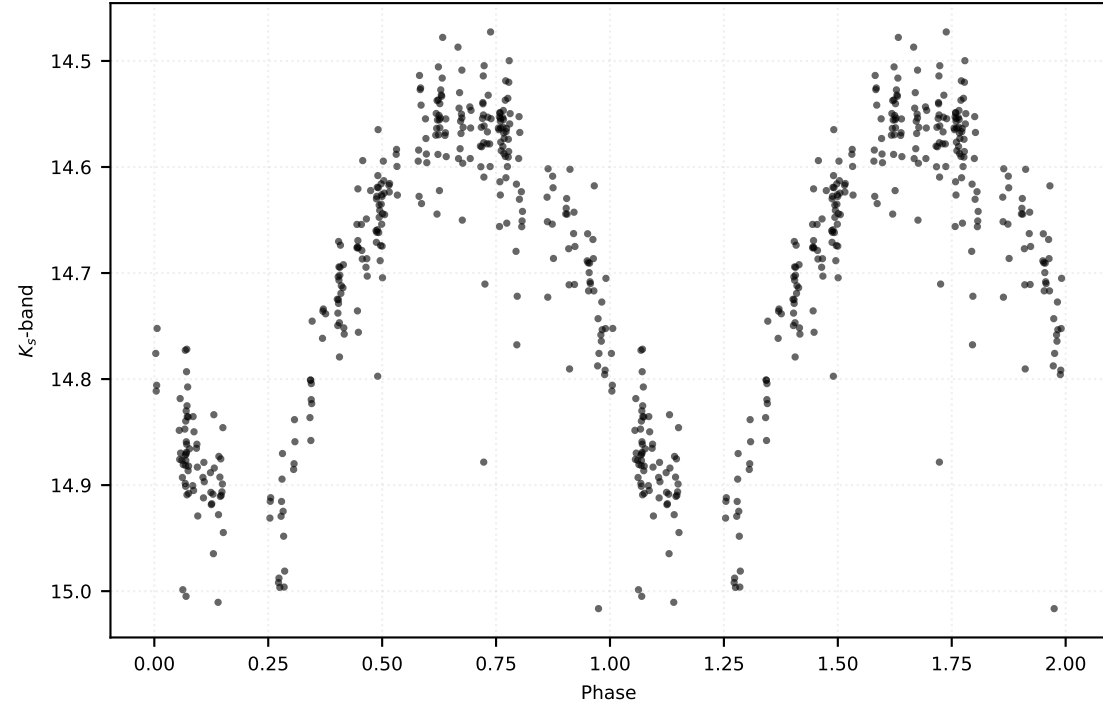
P: 0.42692 d | Class: RP | Subclass: RRab | Field b278
