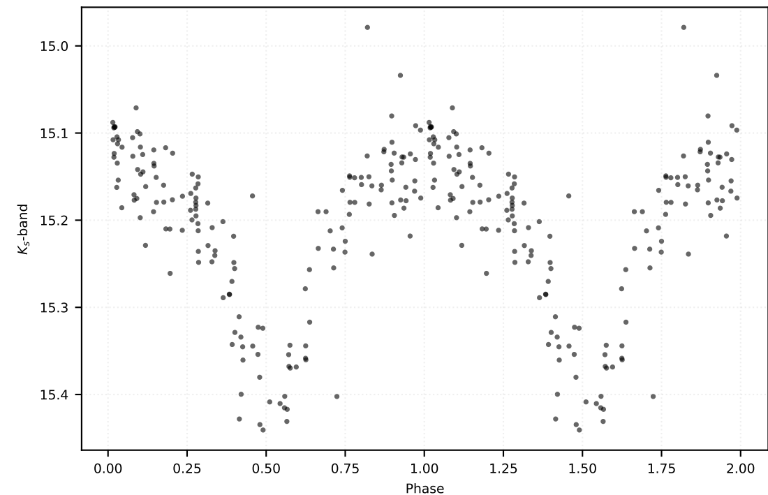
P: 0.44757 d | Class: RP | Subclass: RRc | Field b279
