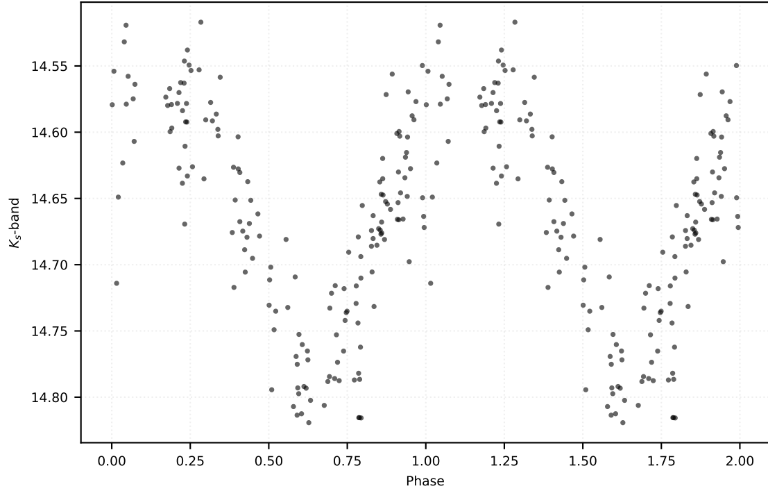
P: 0.14934 d | Class: RP | Subclass: UVAR | Field b278
