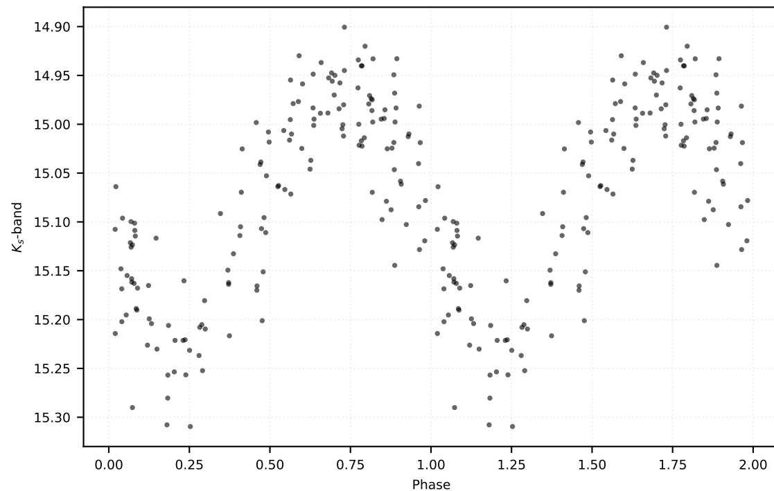
P: 0.15250 d | Class: RP | Subclass: UVAR | Field b279
