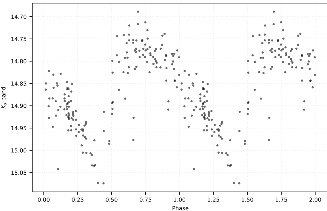
P: 0.51659 d | Class: RP | Subclass: RRab | Field b279
