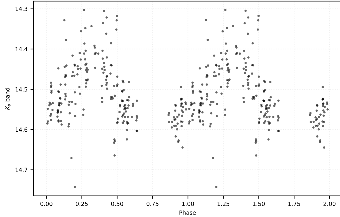
P: 0.11080 d | Class: RP | Subclass: UVAR | Field b279
