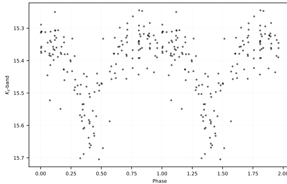
P: 0.16051 d | Class: RP | Subclass: UVAR | Field b279
