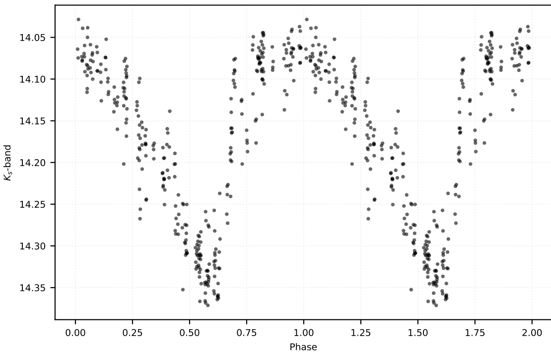
P: 0.46942 d | Class: RP | Subclass: RRab | Field b279
