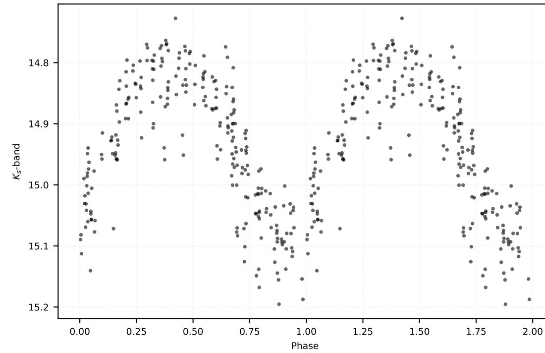
P: 0.20378 d | Class: RP | Subclass: UVAR | Field b278
