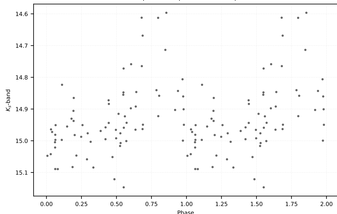
P: 0.41752 d | Class: RP | Subclass: RRab | Field b279
