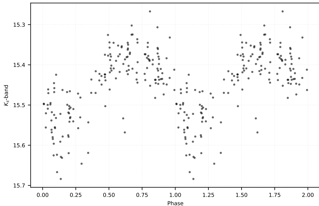
P: 0.44081 d | Class: RP | Subclass: CEP-10T | Field b279
