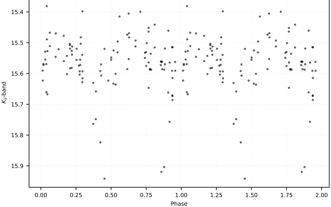
P: 0.62777 d | Class: EB | Subclass: EA | Field b278
