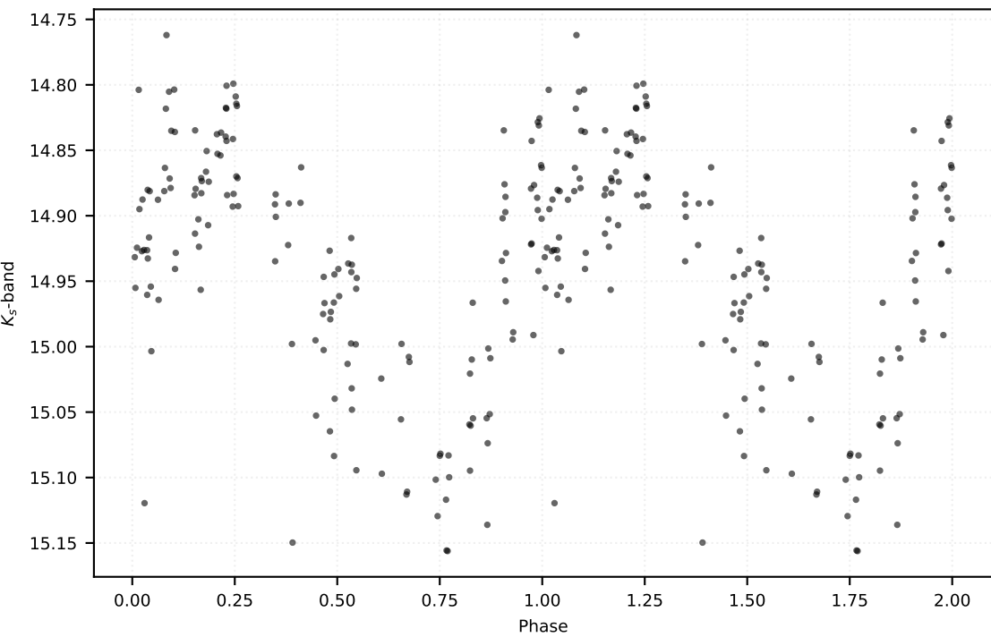
P: 0.69828 d | Class: RP | Subclass: RRab | Field b278
