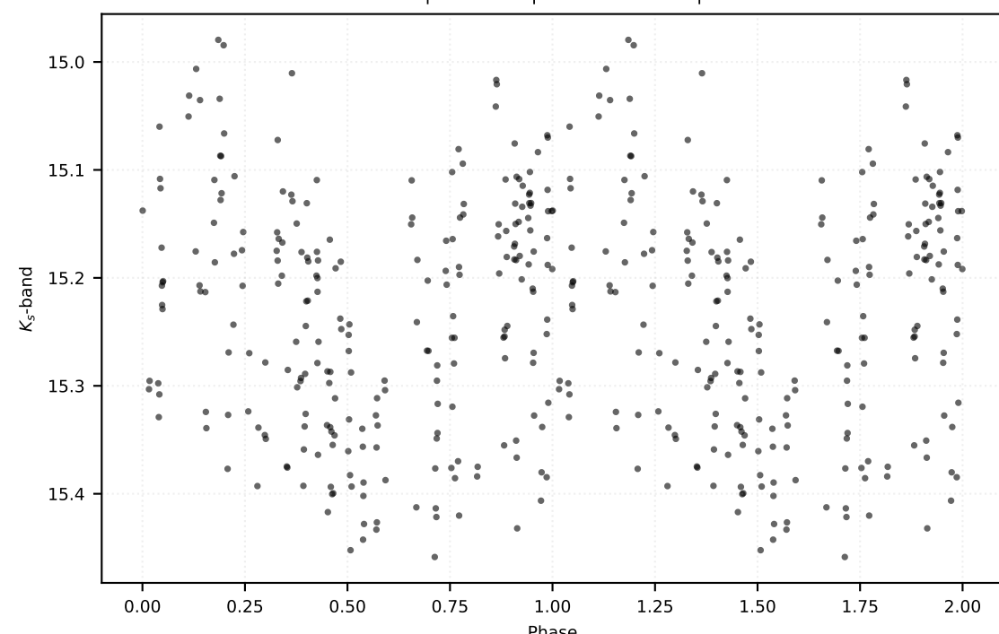
P: 0.33272 d | Class: RP | Subclass: RRab | Field b279
