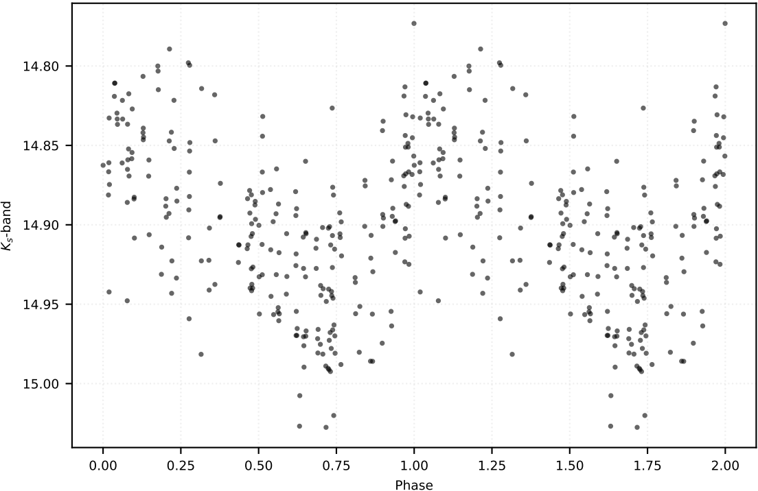
P: 0.48606 d | Class: RP | Subclass: RRc | Field b279
