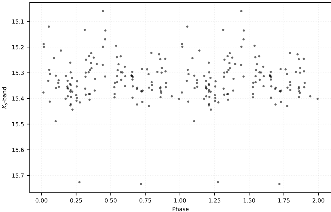
P: 0.22602 d | Class: EB | Subclass: EA | Field b279
