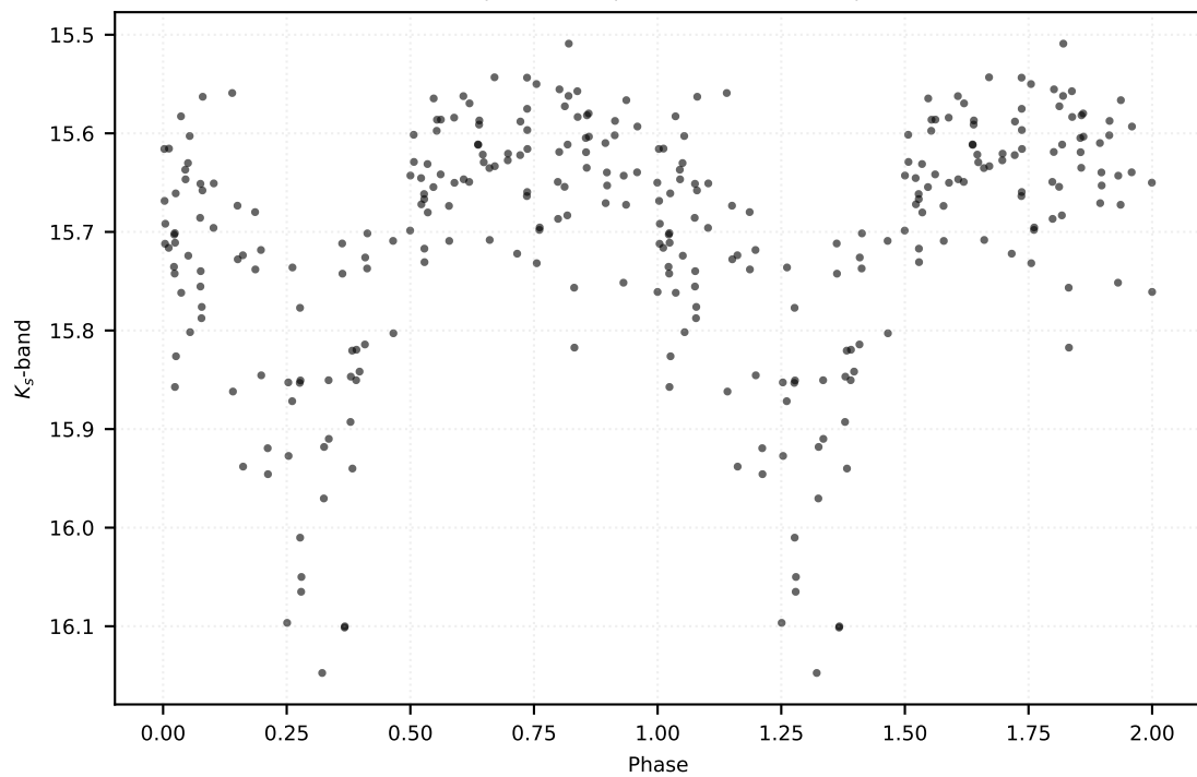
P: 0.37672 d | Class: RP | Subclass: CEP-10T | Field b279
