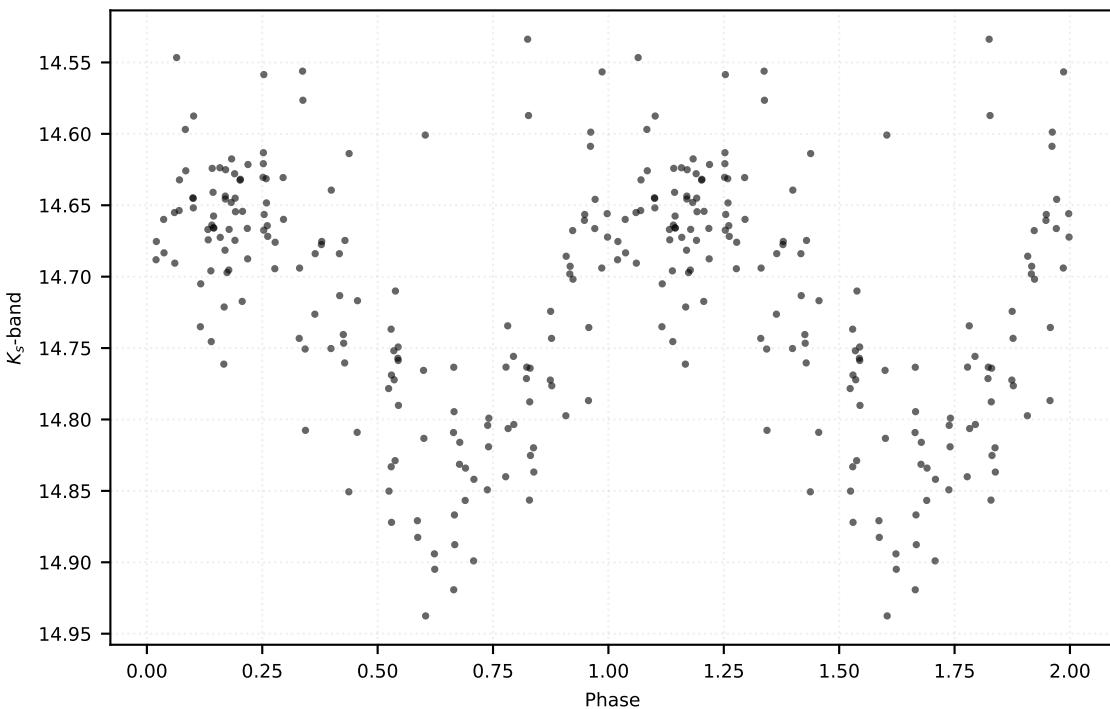
P: 0.35950 d | Class: RP | Subclass: RRab | Field b279
