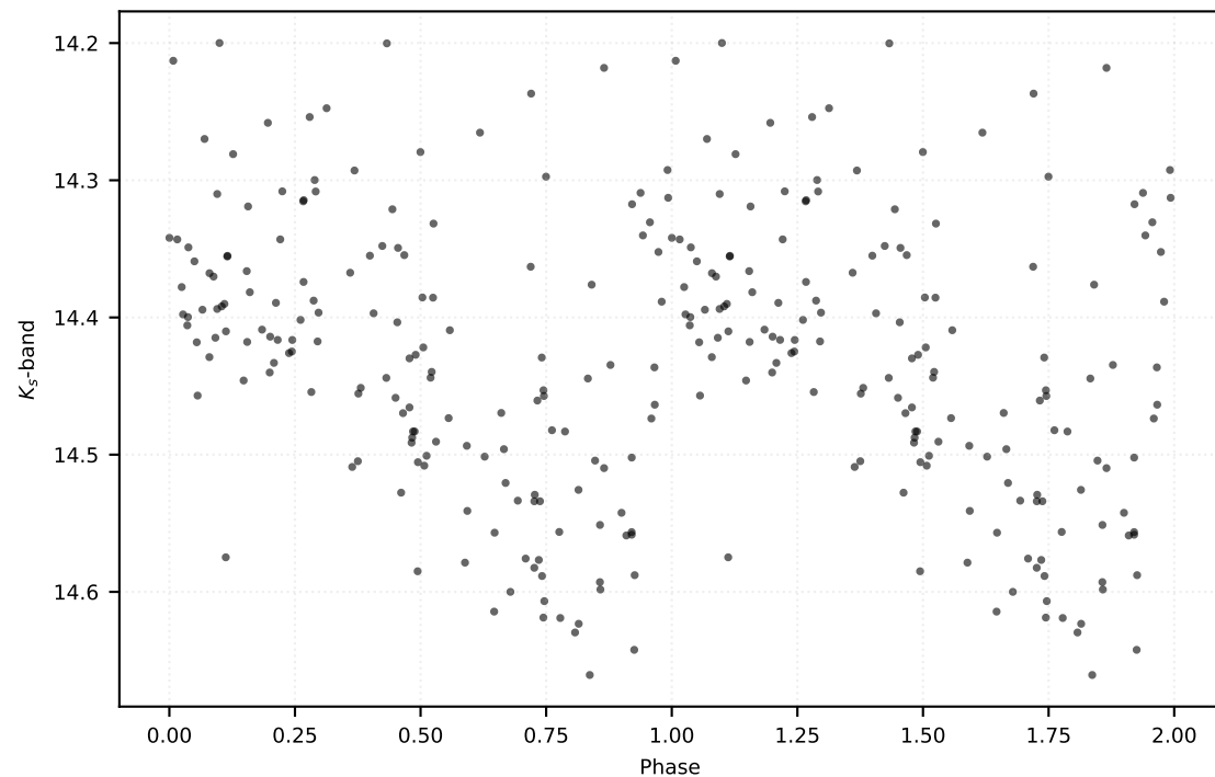
P: 0.48592 d | Class: RP | Subclass: RRab | Field b279
