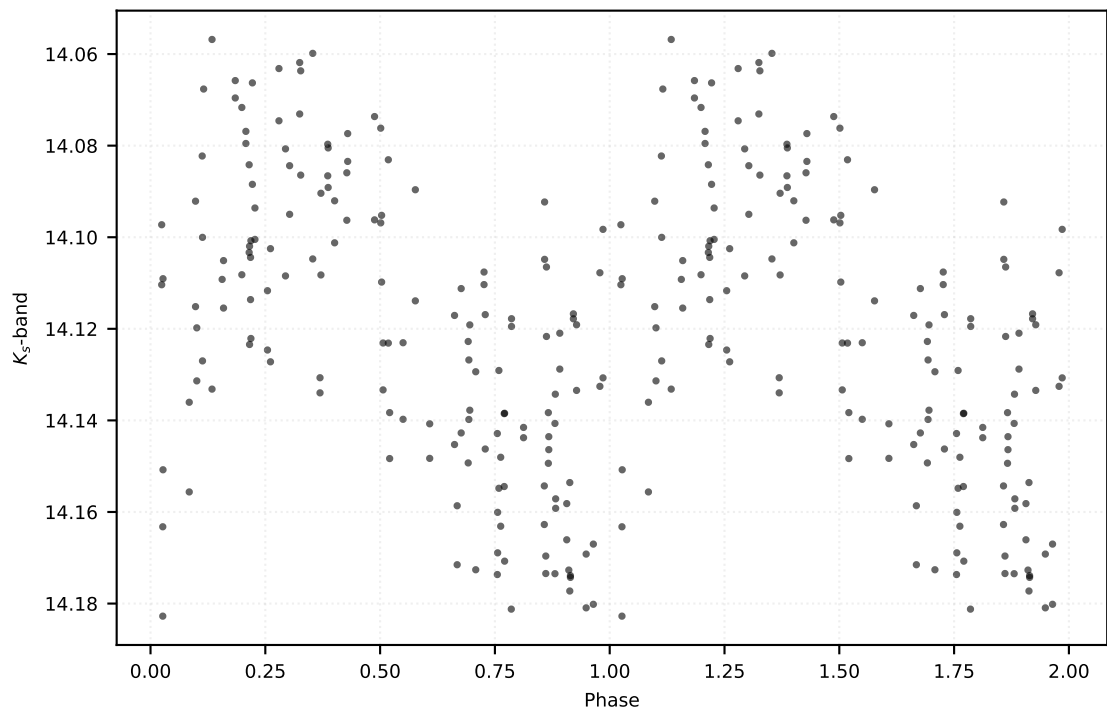
P: 17.21603 d | Class: RP | Subclass: CEP-F | Field b279
