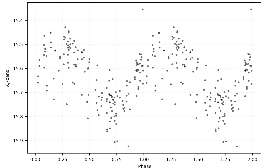
P: 0.31799 d | Class: RP | Subclass: RRc | Field b279
