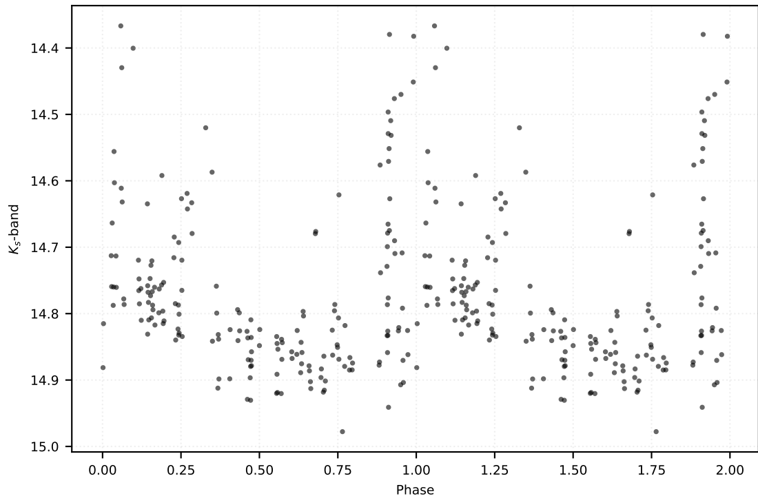
P: 0.29192 d | Class: RP | Subclass: RRc | Field b278
