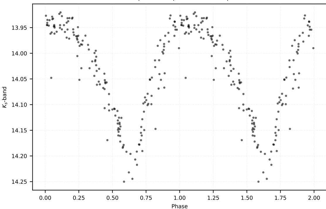
P: 0.43958 d | Class: RP | Subclass: RRab | Field b278
