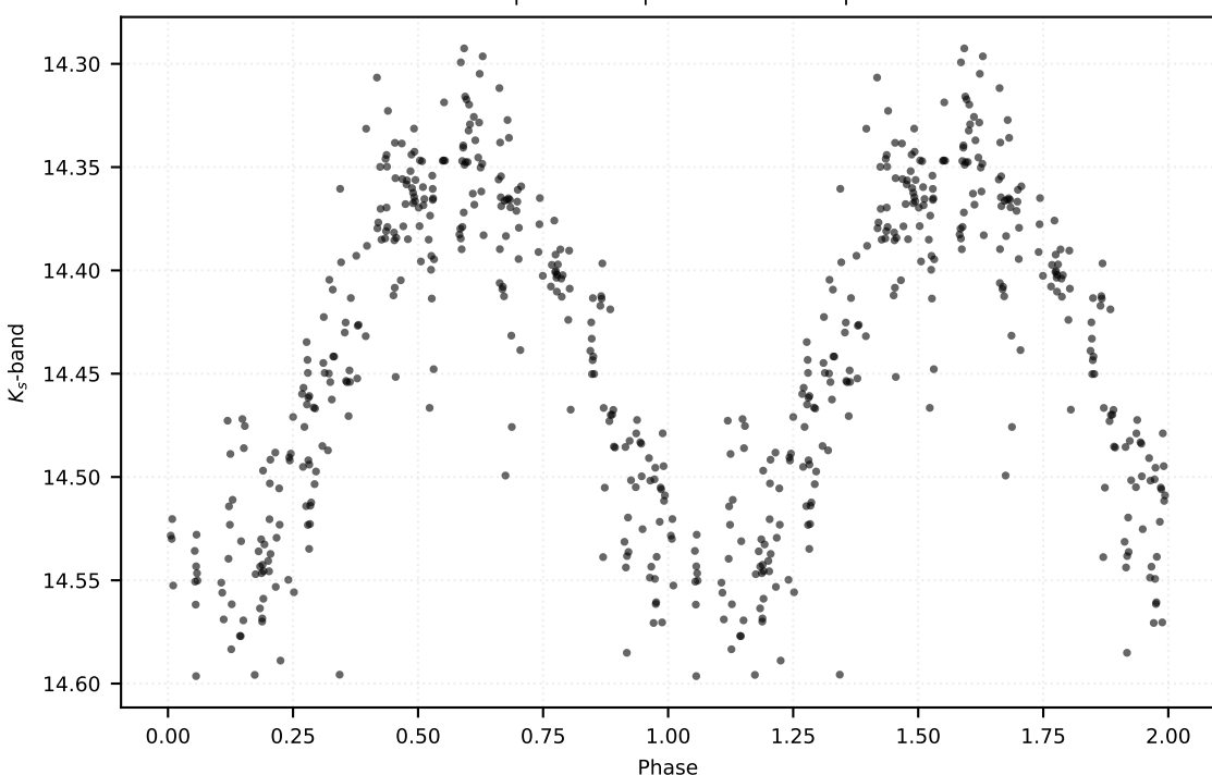
P: 0.72893 d | Class: RP | Subclass: RRab | Field b278
