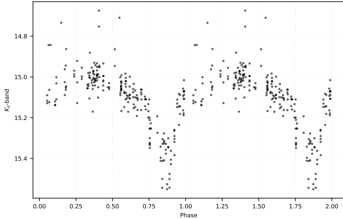
P: 1.70316 d | Class: RP | Subclass: CEP-F | Field b279
