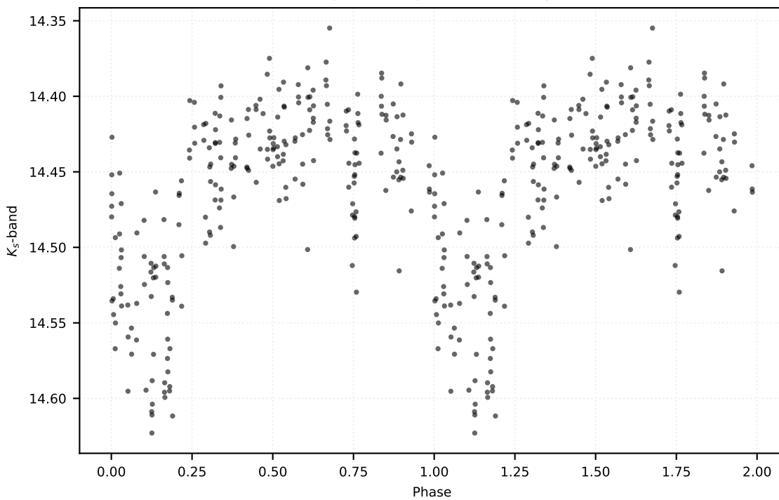
P: 0.79803 d | Class: RP | Subclass: RRab | Field b278
