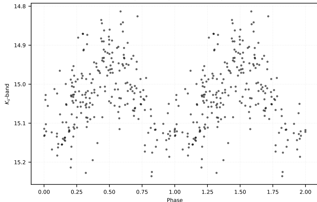
P: 0.45369 d | Class: RP | Subclass: RRab | Field b279
