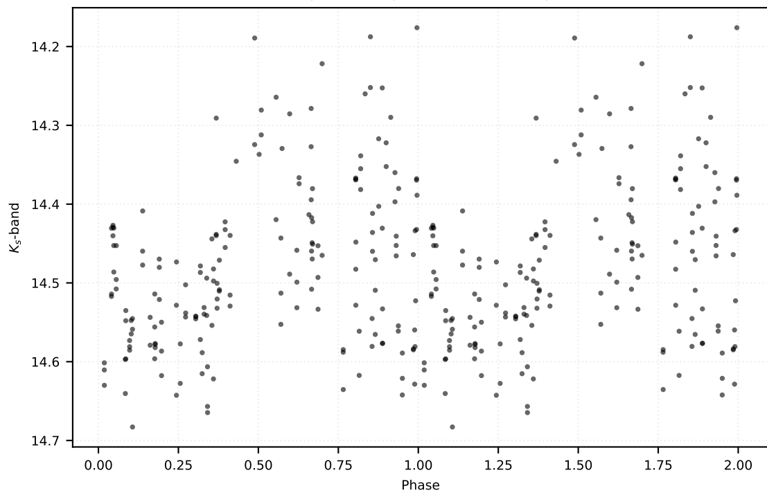
P: 1.18350 d | Class: RP | Subclass: CEP-10T | Field b279
