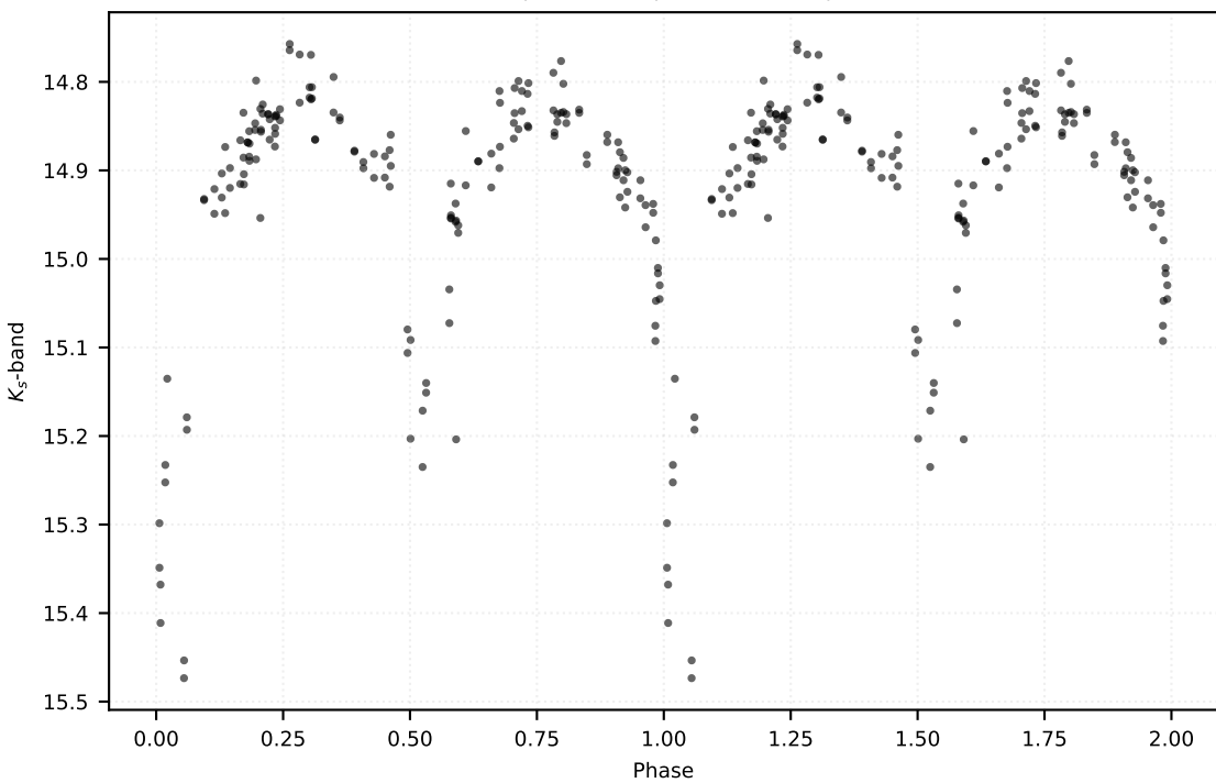
P: 3.83073 d | Class: EB | Subclass: EA | Field b278
