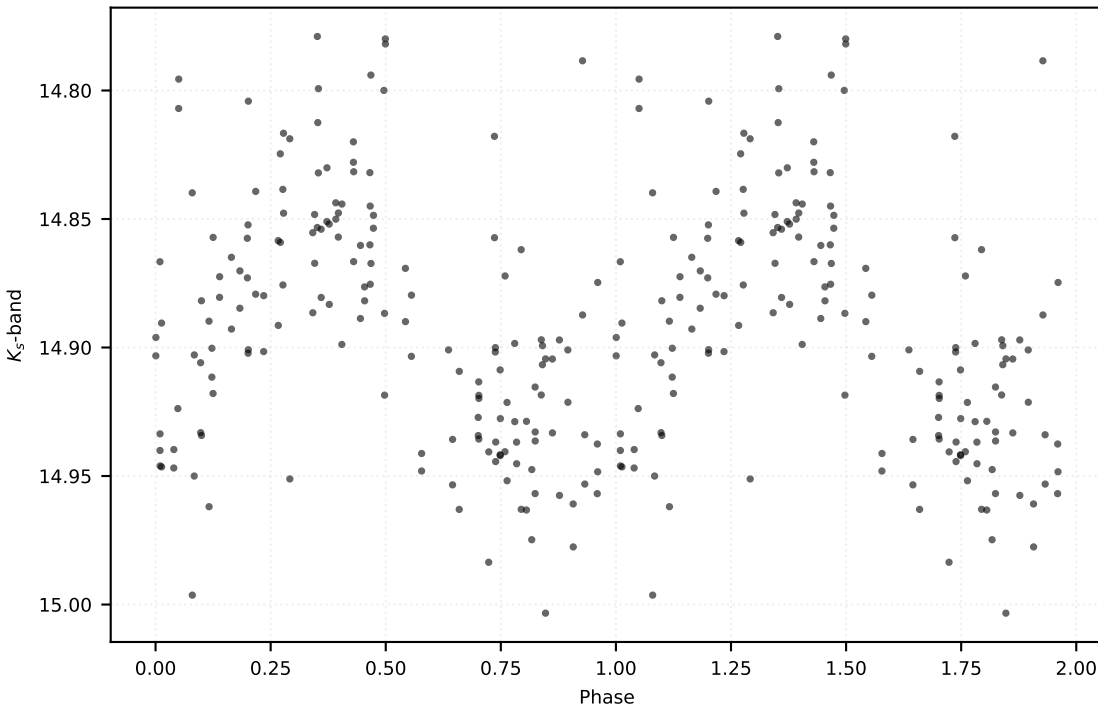
P: 17.59080 d | Class: RP | Subclass: CEP-F | Field b279
