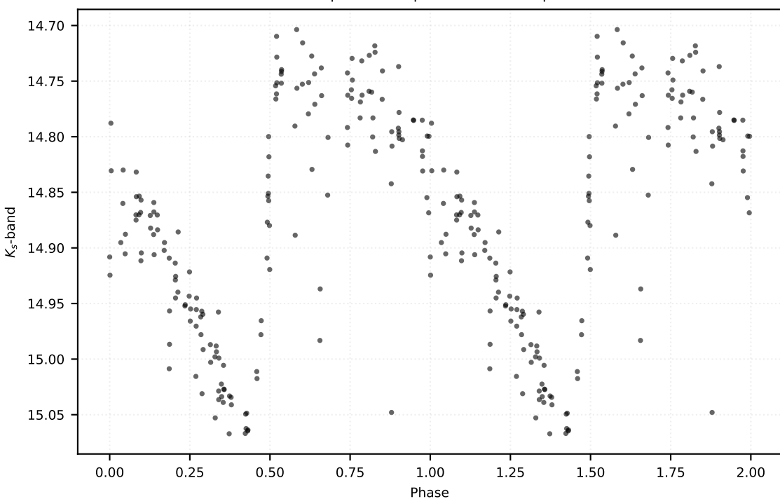
P: 0.47449 d | Class: RP | Subclass: RRab | Field b278
