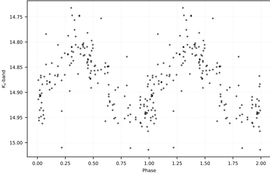
P: 2.13492 d | Class: RP | Subclass: CEP-F | Field b279
