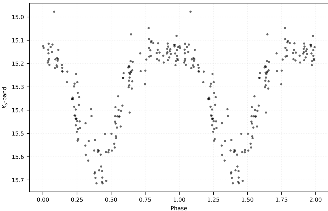
P: 0.22126 d | Class: RP | Subclass: UVAR | Field b279
