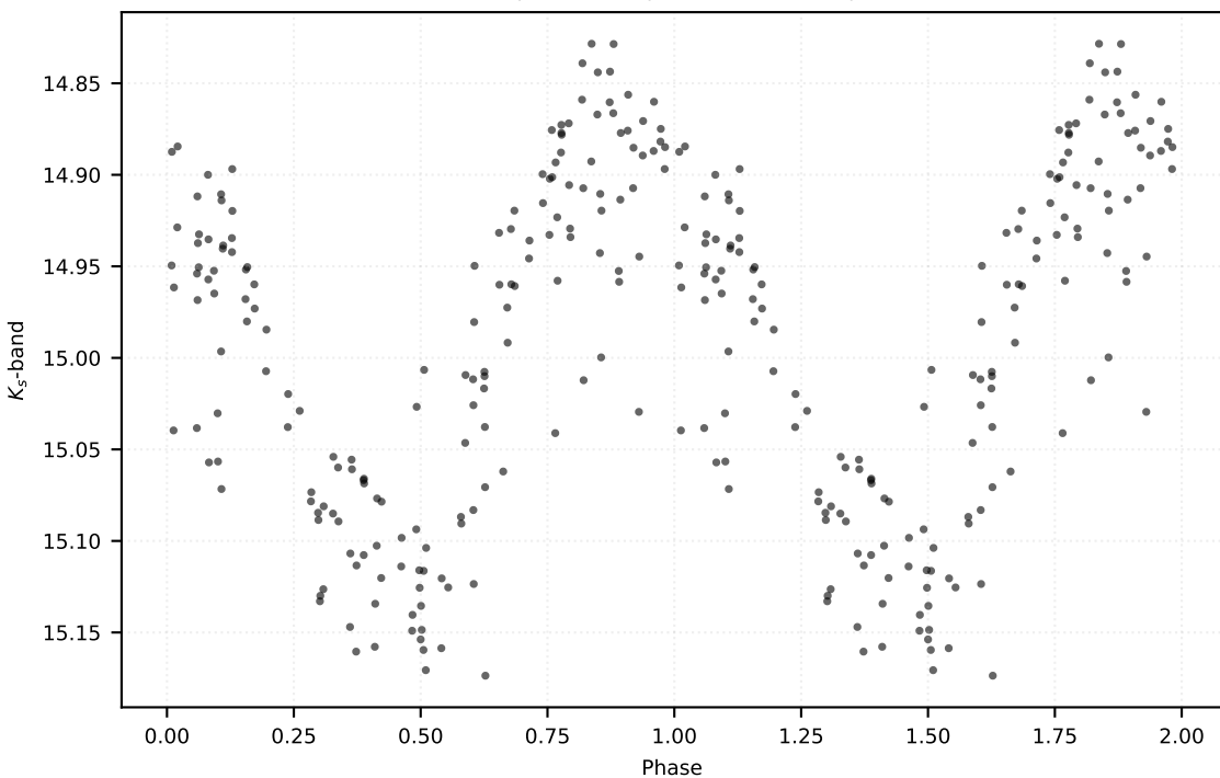
P: 0.54695 d | Class: RP | Subclass: RRab | Field b278
