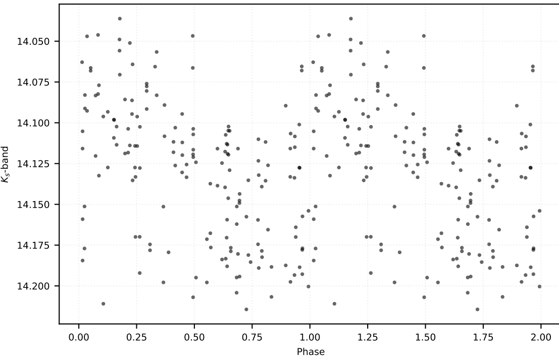
P: 3.16105 d | Class: RP | Subclass: CEP-F | Field b278
