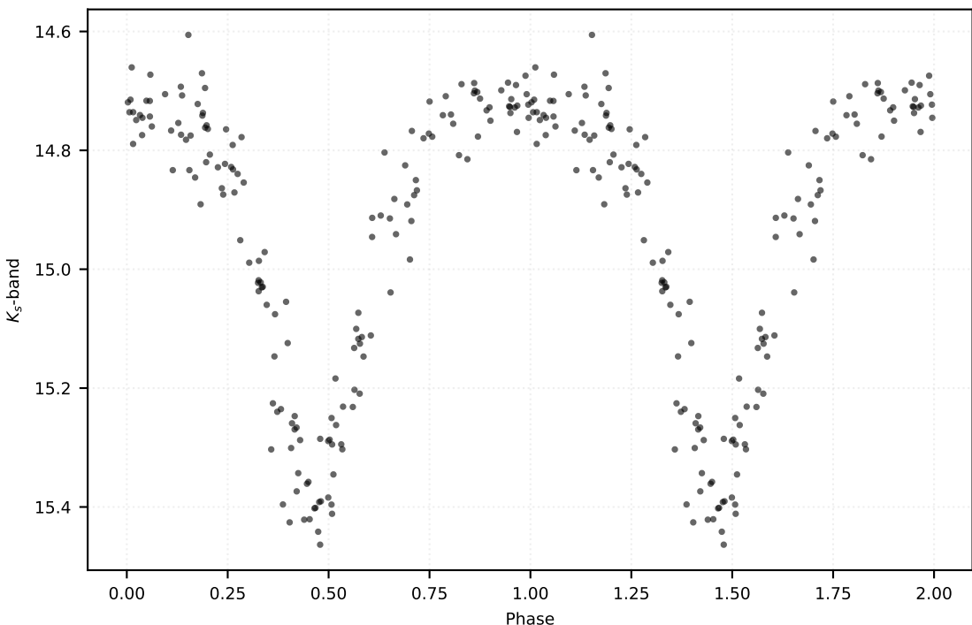
P: 0.16367 d | Class: RP | Subclass: UVAR | Field b279
