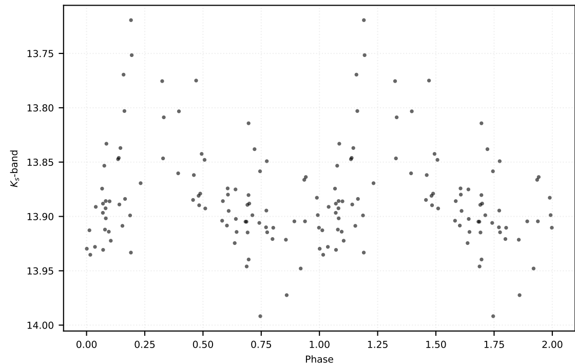
P: 0.19946 d | Class: RP | Subclass: UVAR | Field b279
