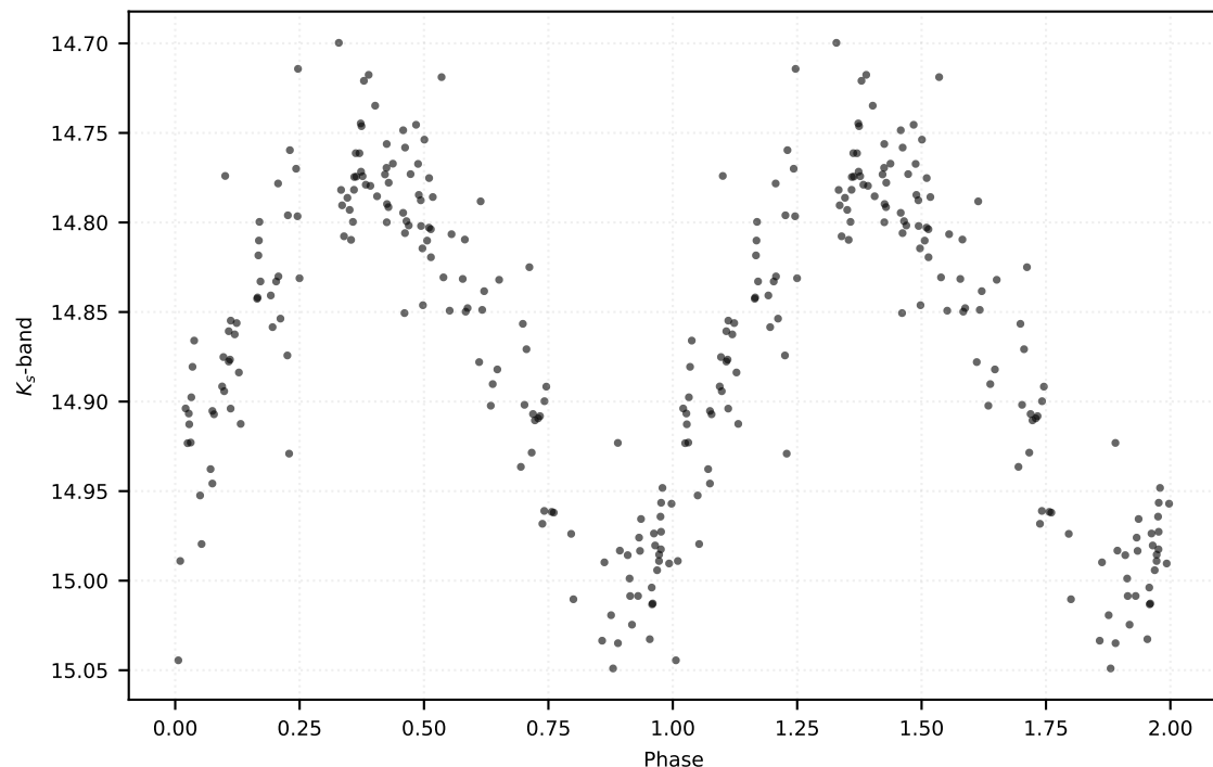
P: 1.16656 d | Class: EB | Subclass: UVAR | Field b278
