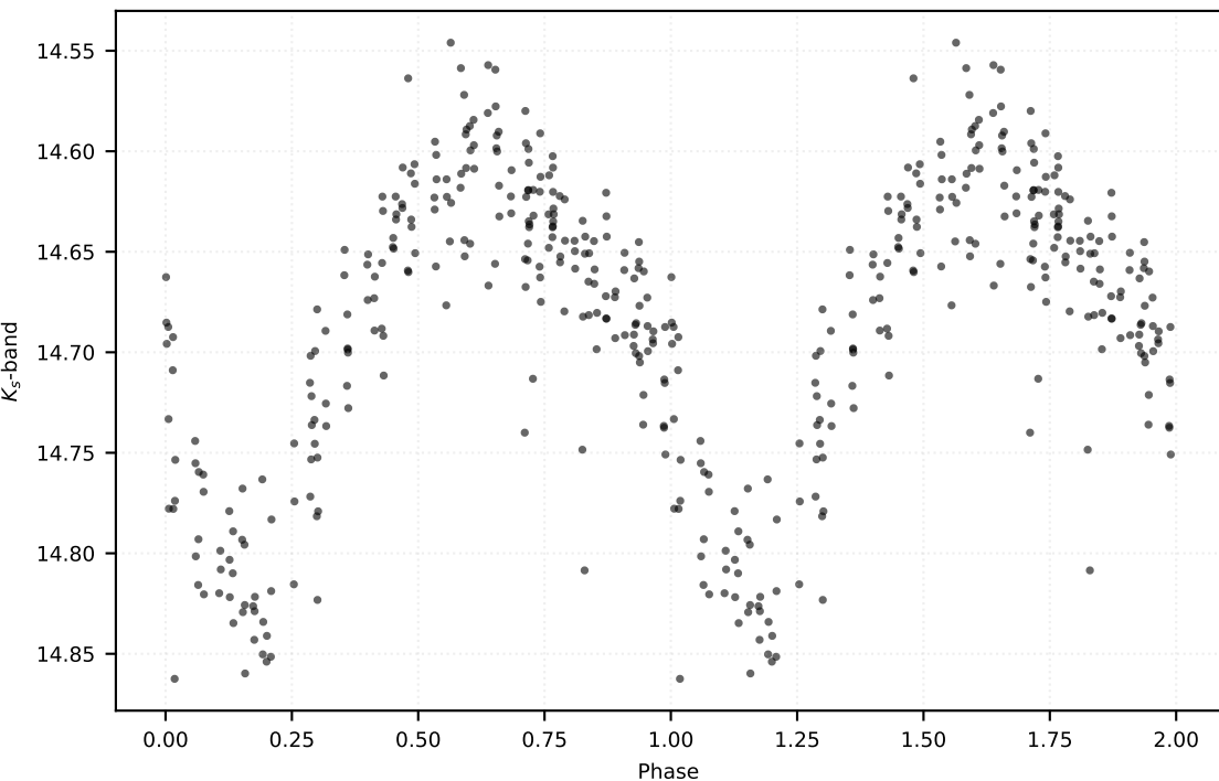
P: 0.57092 d | Class: RP | Subclass: RRab | Field b279
