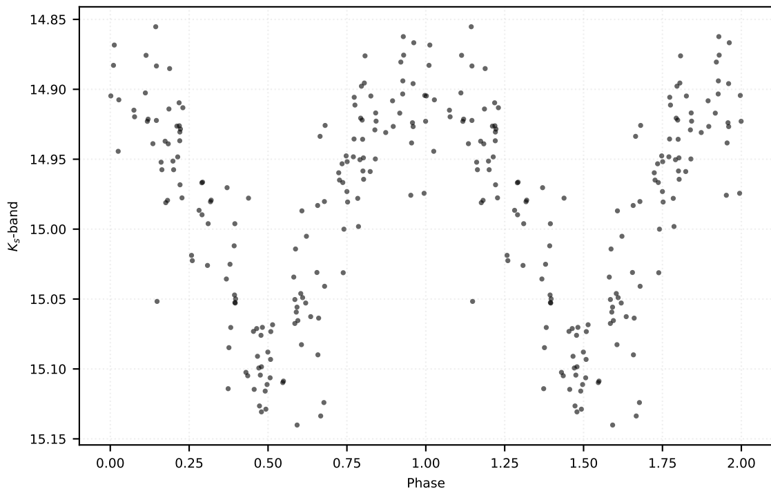
P: 0.14410 d | Class: RP | Subclass: UVAR | Field b278
