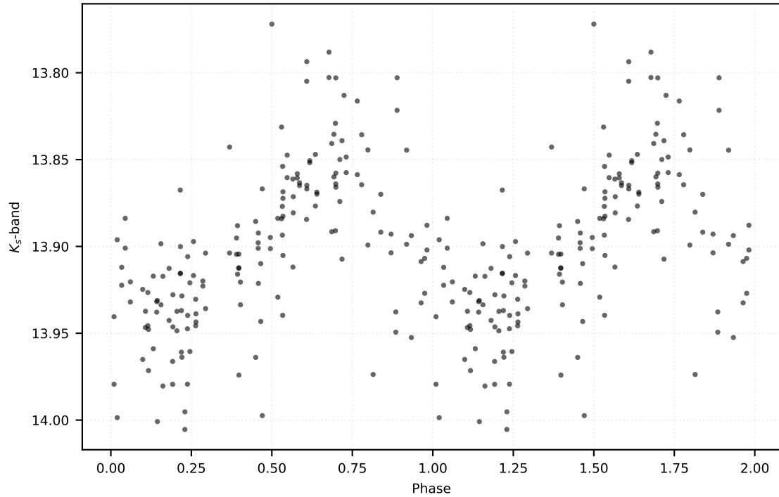
P: 21.24684 d | Class: RP | Subclass: CEP-F | Field b279
