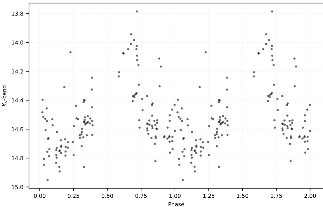
P: 0.20117 d | Class: RP | Subclass: UVAR | Field b279
