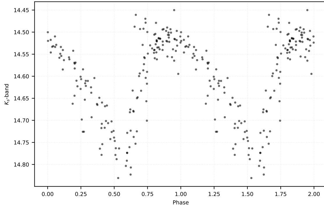
P: 0.59496 d | Class: RP | Subclass: RRab | Field b278
