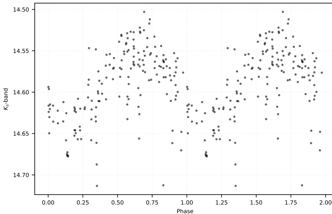
P: 2.44119 d | Class: RP | Subclass: CEP-1OT | Field b278
