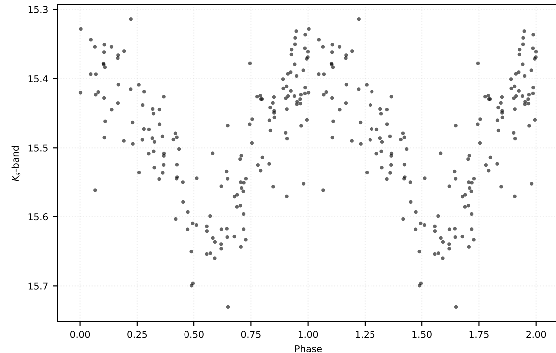
P: 0.40156 d | Class: RP | Subclass: RRab | Field b279
