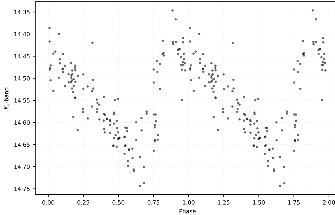
P: 0.21492 d | Class: RP | Subclass: RRc | Field b279
