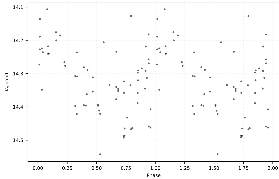
P: 13.23500 d | Class: RP | Subclass: CEP-F | Field b278
