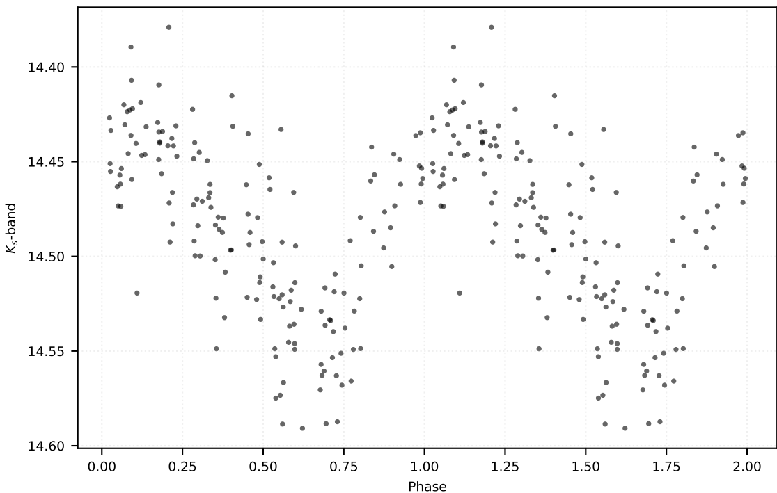
P: 0.20301 d | Class: RP | Subclass: UVAR | Field b279
