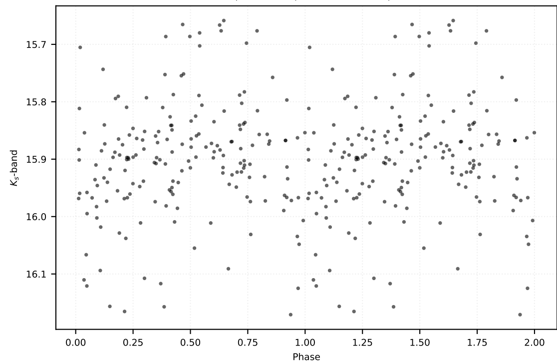
P: 0.11895 d | Class: RP | Subclass: UVAR | Field b278
