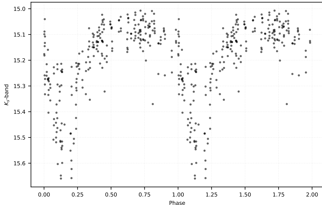
P: 0.64779 d | Class: RP | Subclass: CEP-1OT | Field b278
