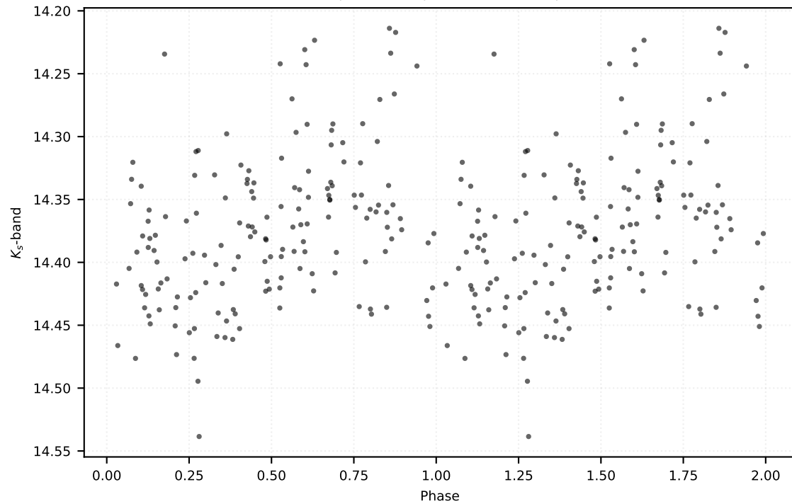
P: 0.26472 d | Class: RP | Subclass: UVAR | Field b279
