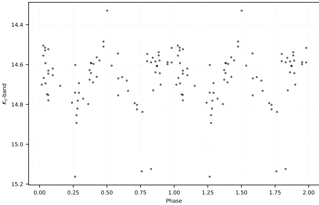
P: 1.56608 d | Class: EB | Subclass: EA | Field b278
