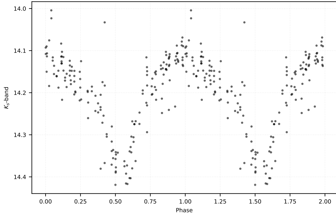
P: 0.52397 d | Class: RP | Subclass: RRab | Field b278
