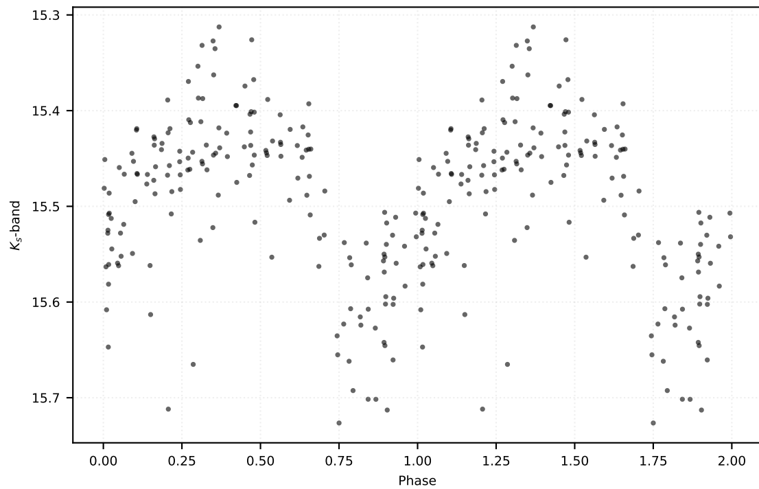
P: 0.31186 d | Class: RP | Subclass: RRab | Field b278
