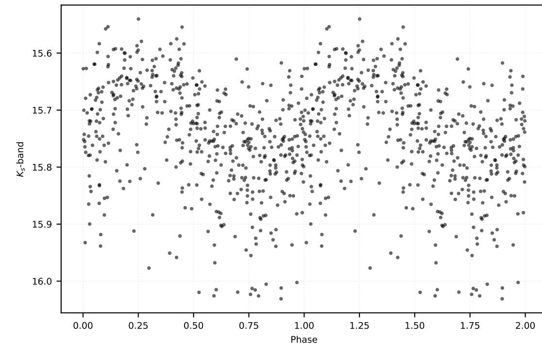
P: 0.46653 d | Class: RP | Subclass: RRab | Field b279
