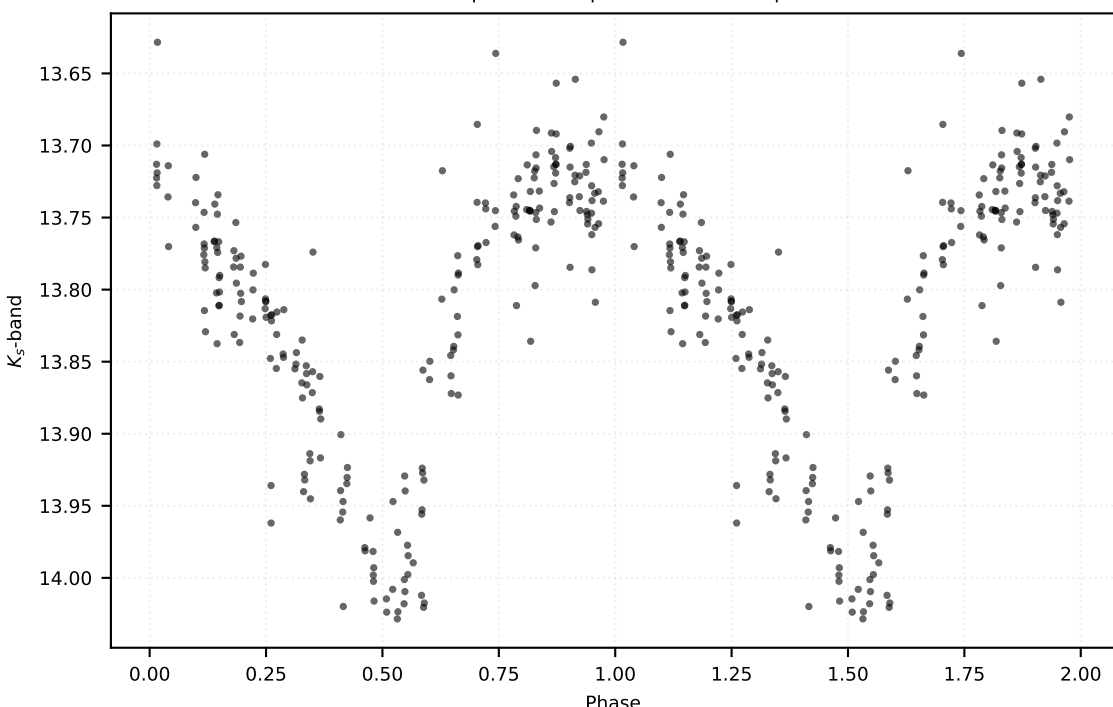
P: 0.59119 d | Class: RP | Subclass: RRab | Field b279
