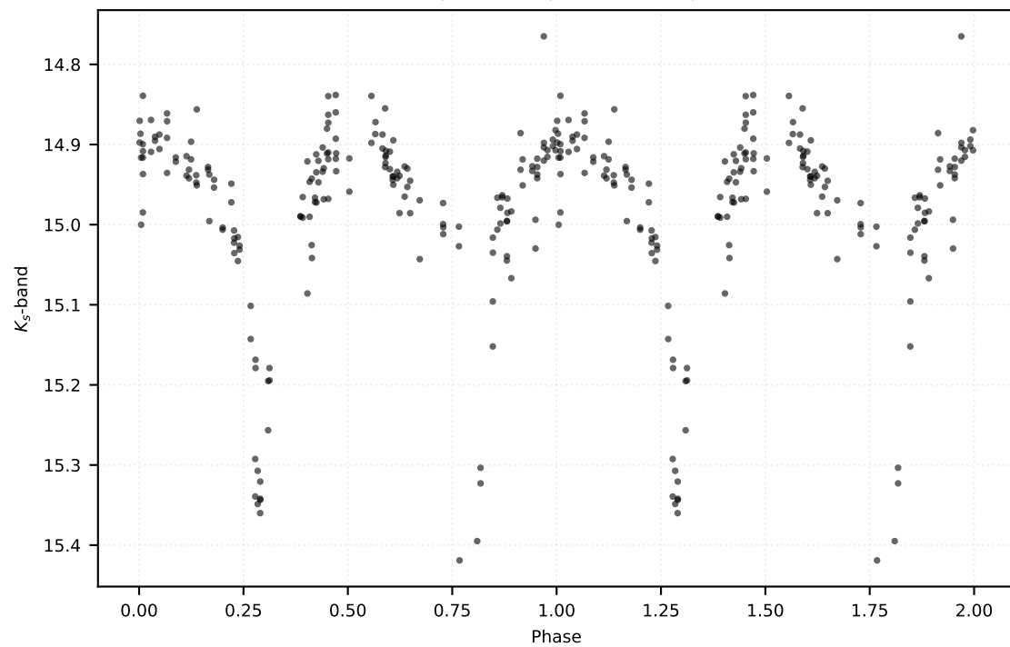
P: 8.21887 d | Class: EB | Subclass: EA | Field b278
