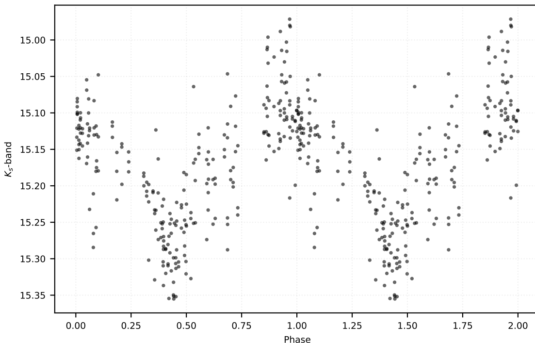
P: 8.62805 d | Class: RP | Subclass: CEP-10T | Field b278
