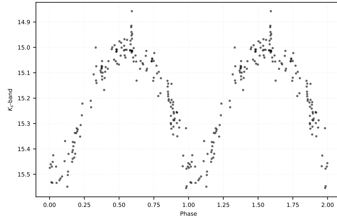
P: 0.11386 d | Class: RP | Subclass: UVAR | Field b278
