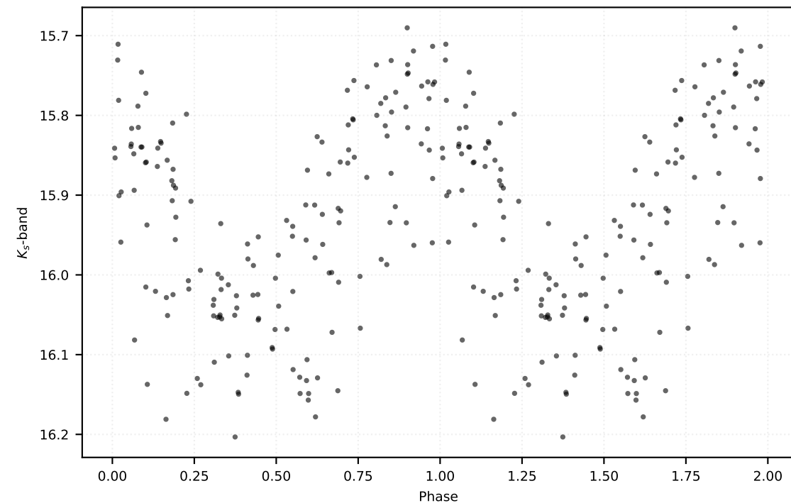
P: 0.52807 d | Class: RP | Subclass: RRab | Field b279
