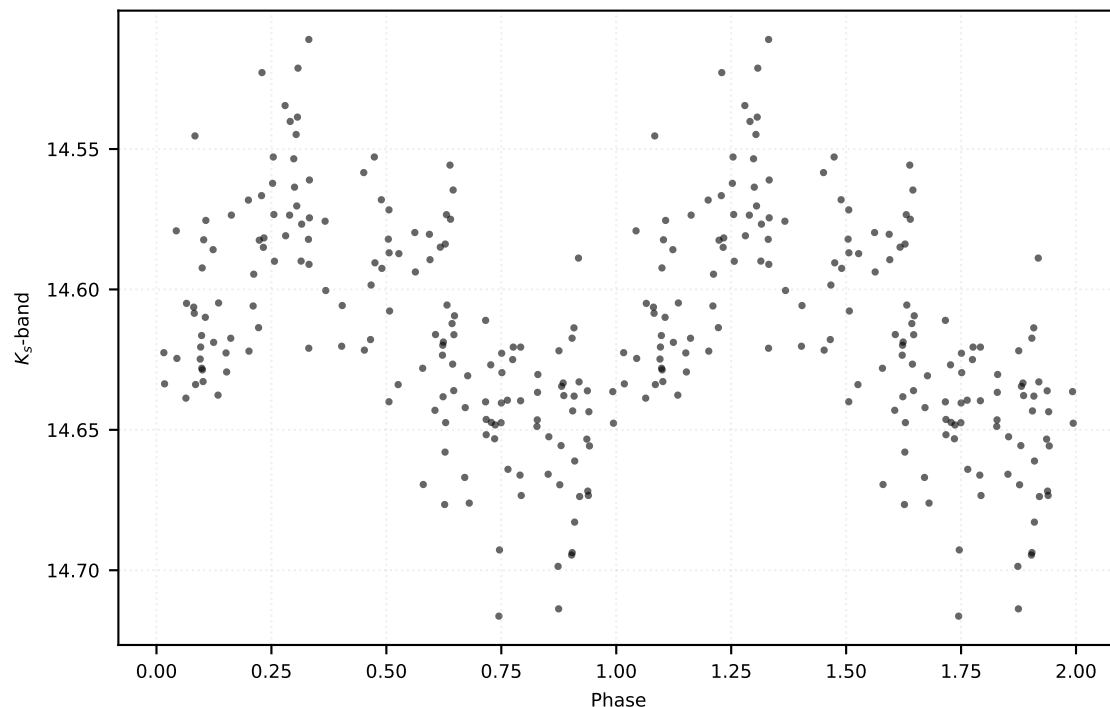
P: 0.97491 d | Class: RP | Subclass: RRab | Field b279
