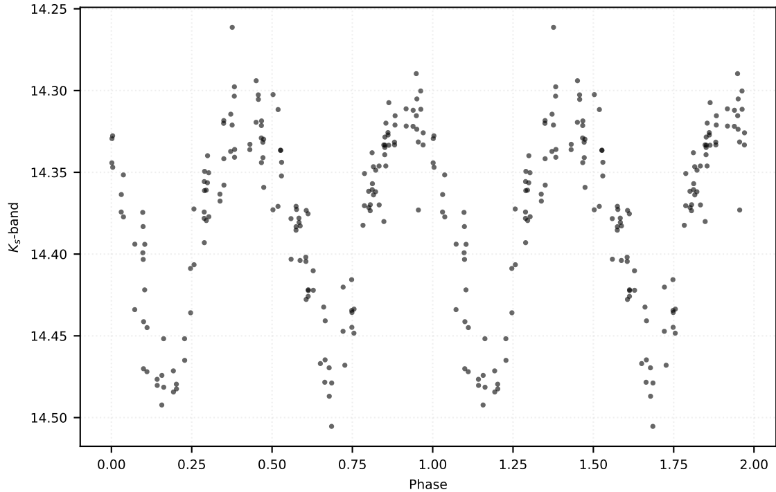
P: 0.41232 d | Class: RP | Subclass: RRc | Field b278
