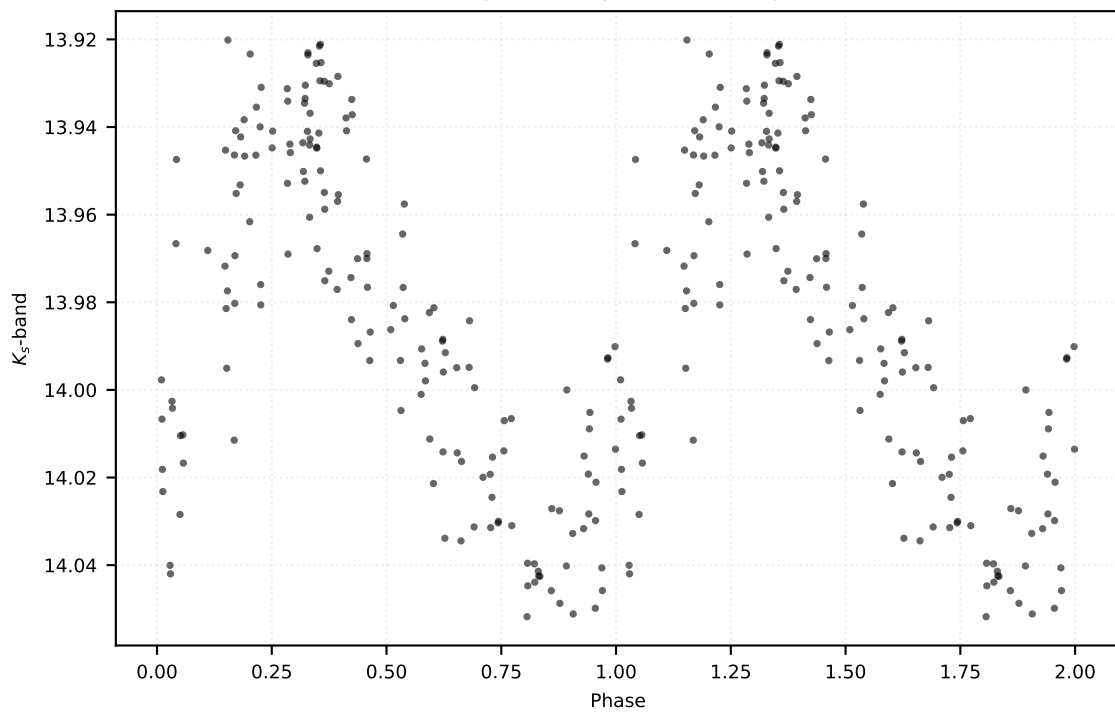
P: 0.42618 d | Class: EB | Subclass: RRc | Field b278
