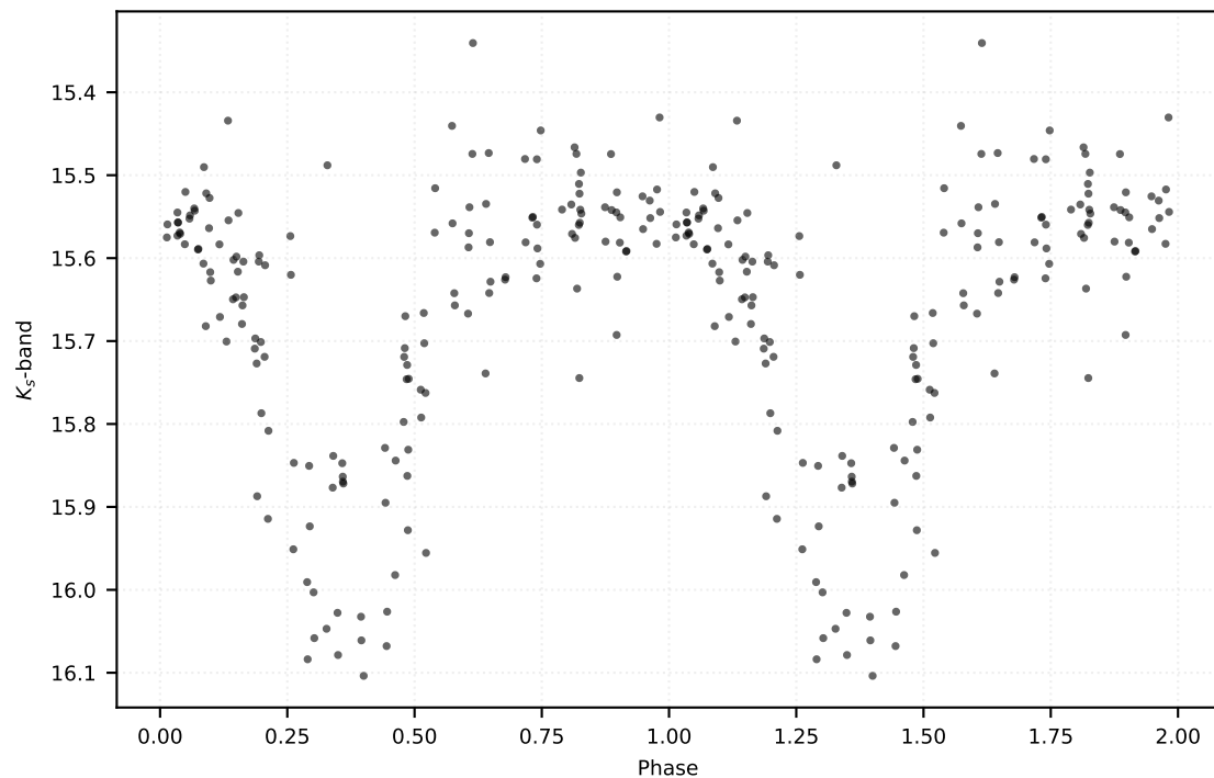
P: 0.47009 d | Class: RP | Subclass: RRab | Field b279
