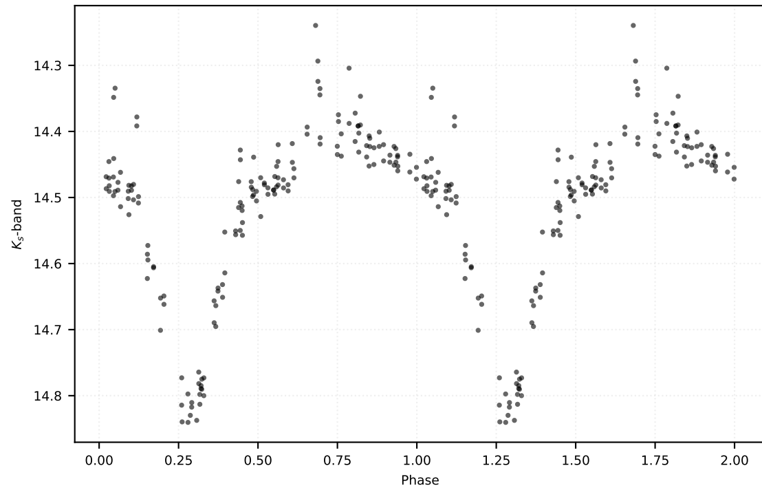
P: 2.34335 d | Class: RP | Subclass: CEP-F | Field b279
