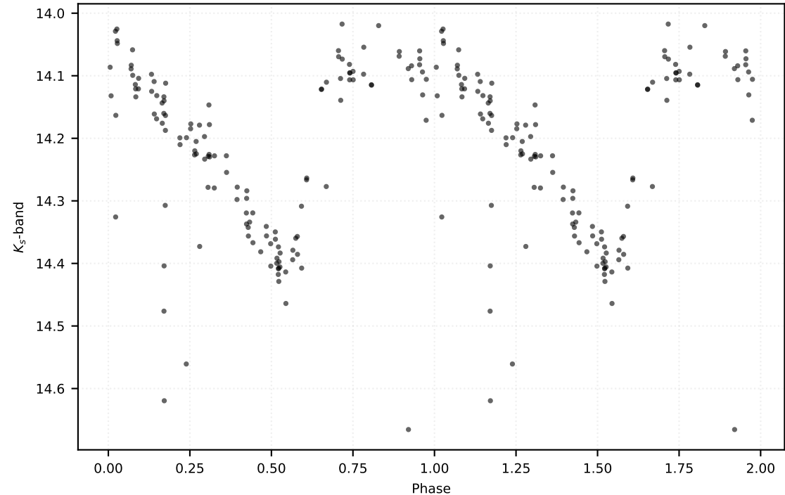
P: 0.53583 d | Class: RP | Subclass: CEP-1OT | Field b278
