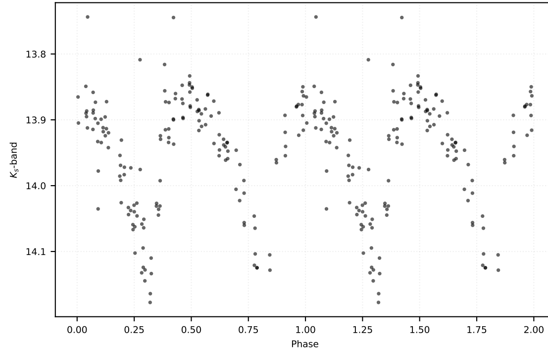
P: 2.67895 d | Class: EB | Subclass: UVAR | Field b278
