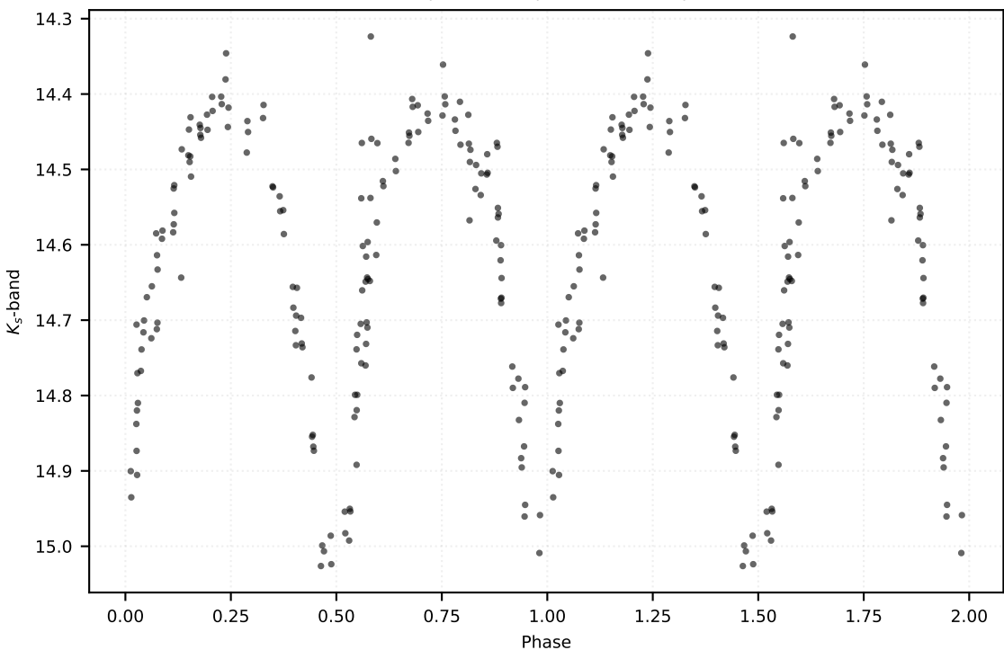
P: 0.88789 d | Class: EB | Subclass: EW | Field b279
