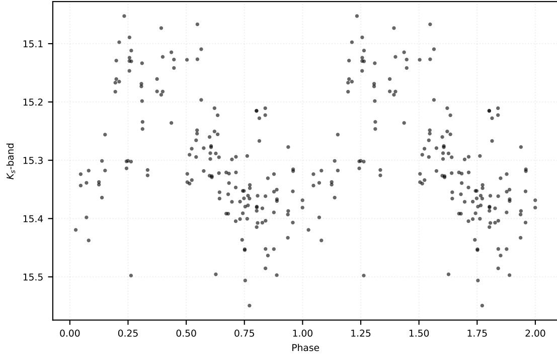
P: 15.93324 d | Class: RP | Subclass: CEP-F | Field b279
