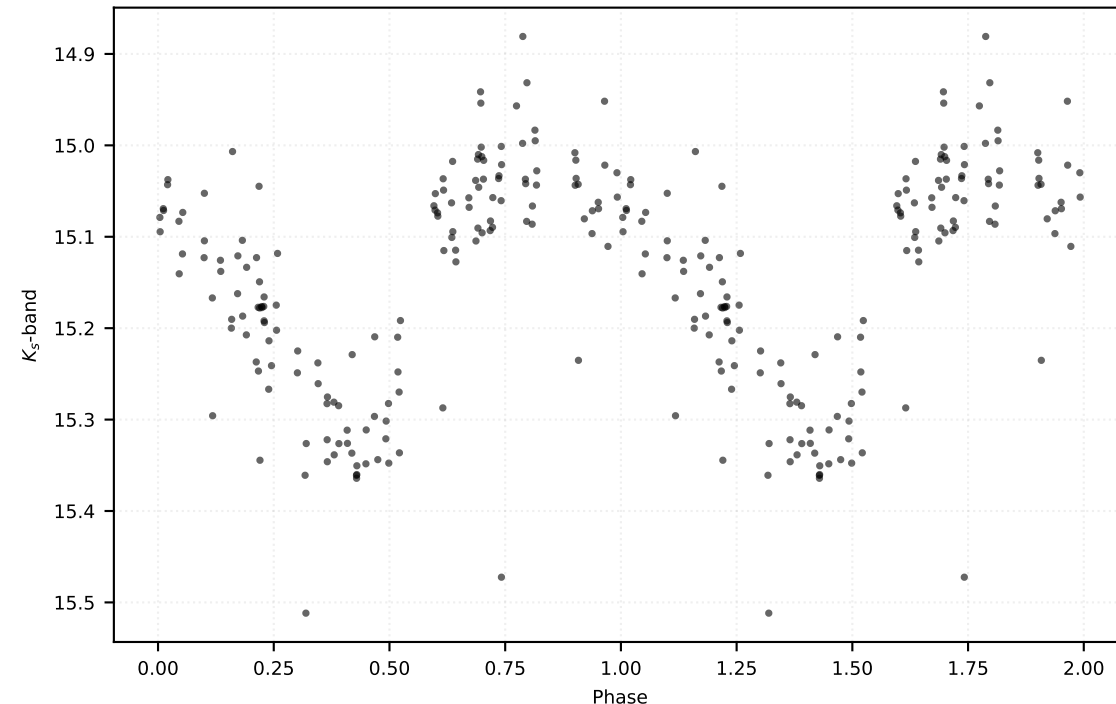
P: 0.49994 d | Class: RP | Subclass: CEP-10T | Field b278
