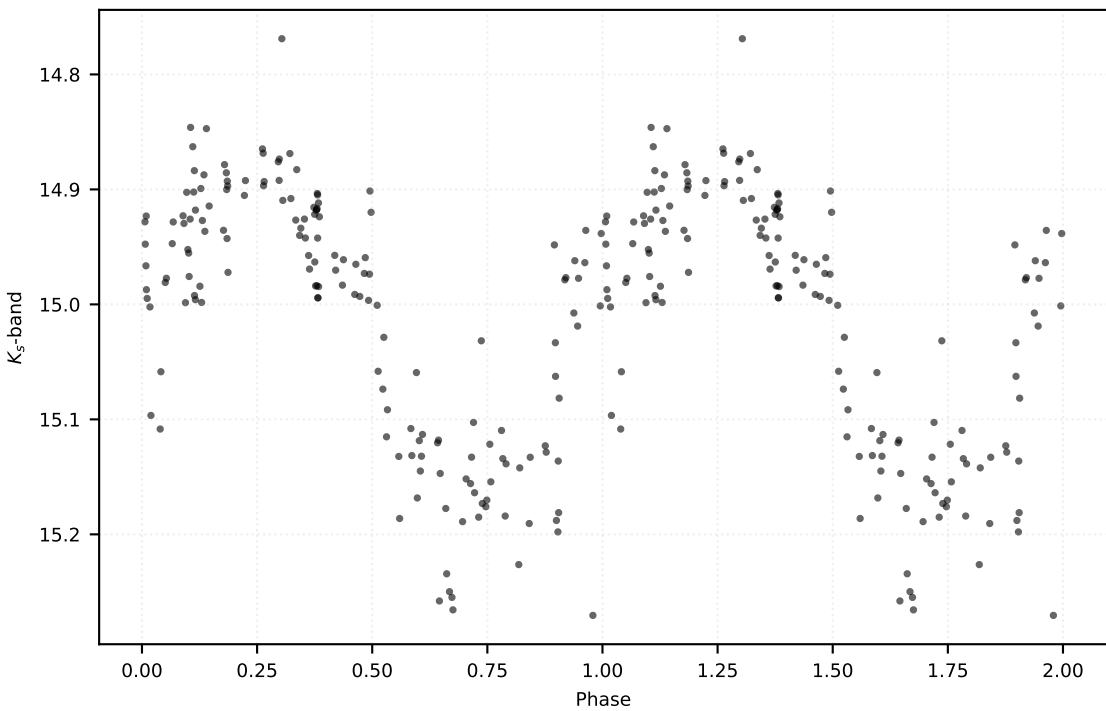
P: 0.14378 d | Class: RP | Subclass: UVAR | Field b279
