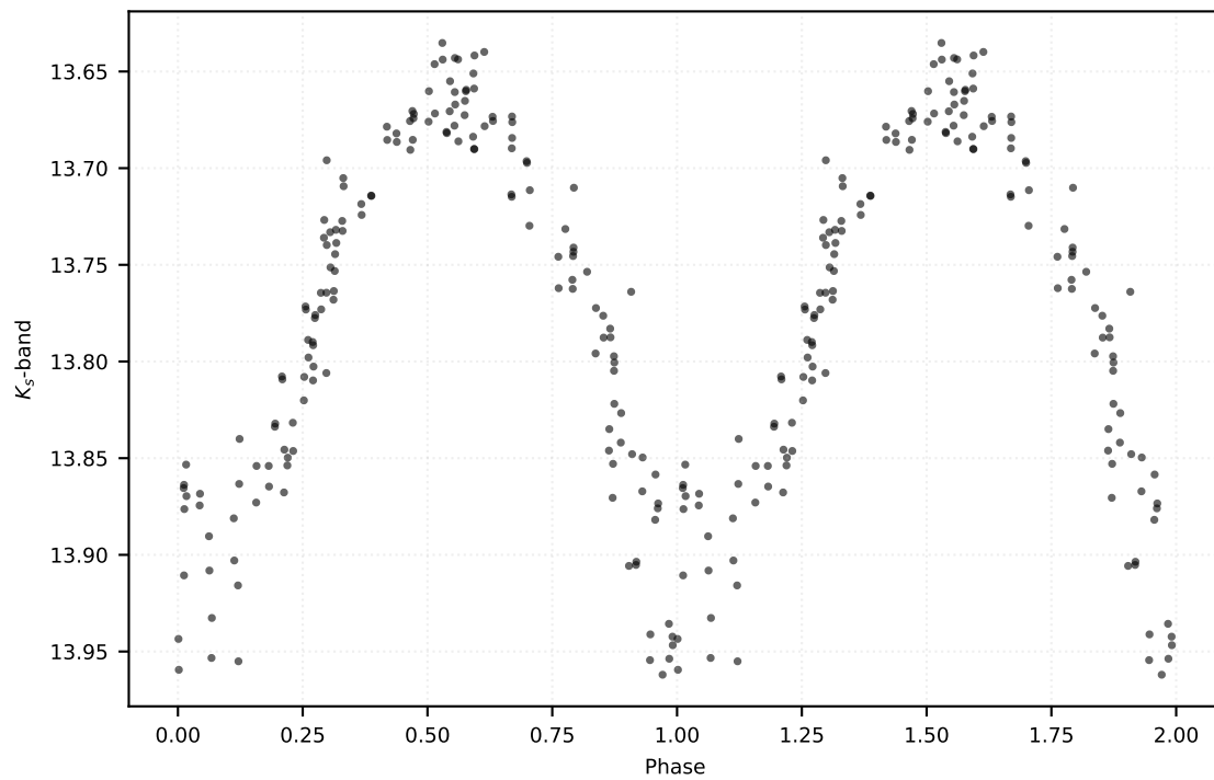
P: 4.46962 d | Class: RP | Subclass: CEP-1OT | Field b279
