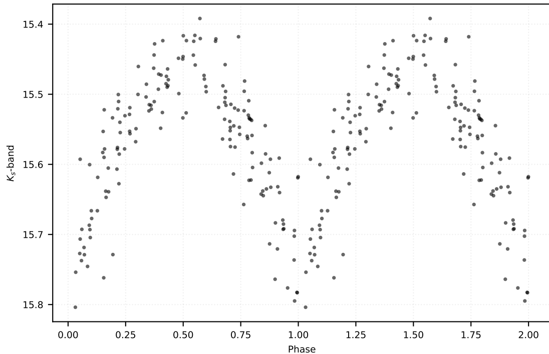
P: 0.26284 d | Class: RP | Subclass: CEP-10T | Field b279
