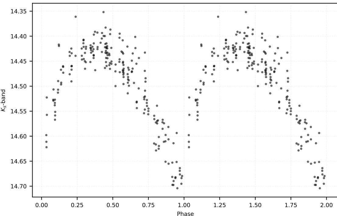
P: 0.54137 d | Class: RP | Subclass: RRab | Field b278
