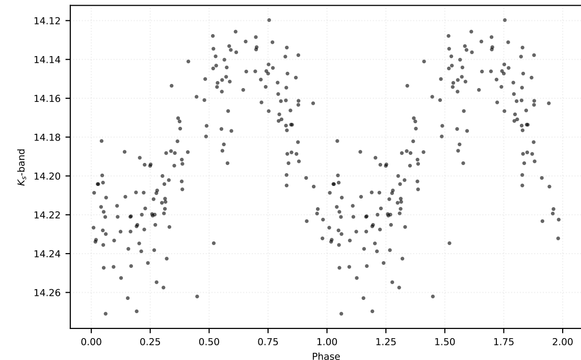
P: 0.17675 d | Class: RP | Subclass: UVAR | Field b279
