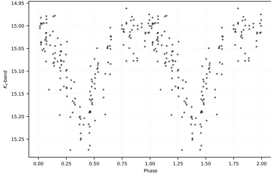
P: 0.65159 d | Class: RP | Subclass: CEP-10T | Field b278
