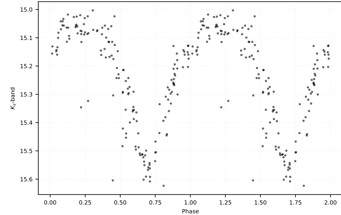
P: 0.22978 d | Class: RP | Subclass: UVAR | Field b279
