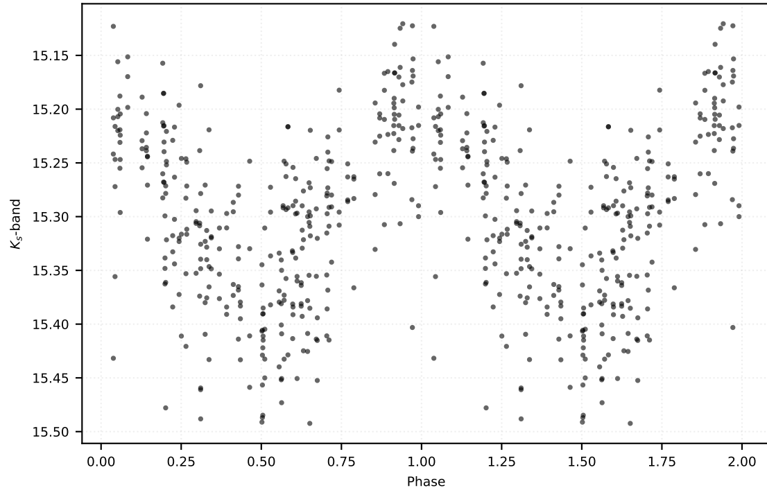
P: 59.27091 d | Class: RP | Subclass: CEP-F | Field b279
