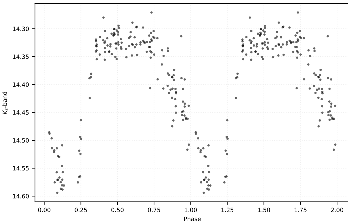
P: 0.45598 d | Class: RP | Subclass: RRab | Field b278
