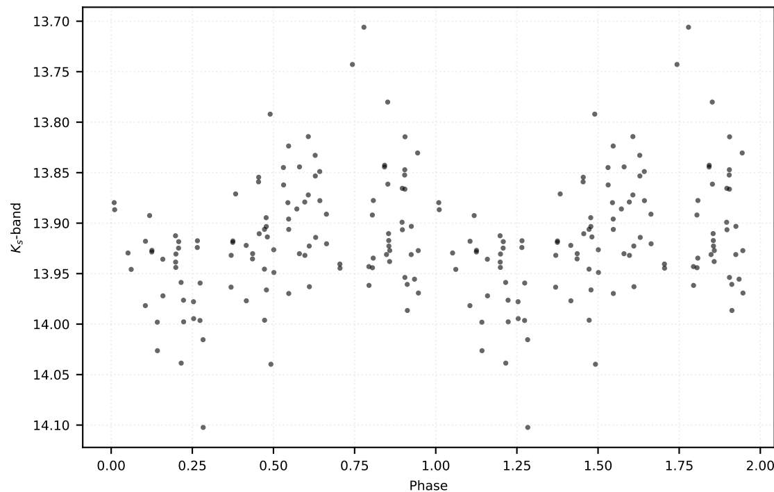
P: 0.59411 d | Class: RP | Subclass: CEP-1OT | Field b278
