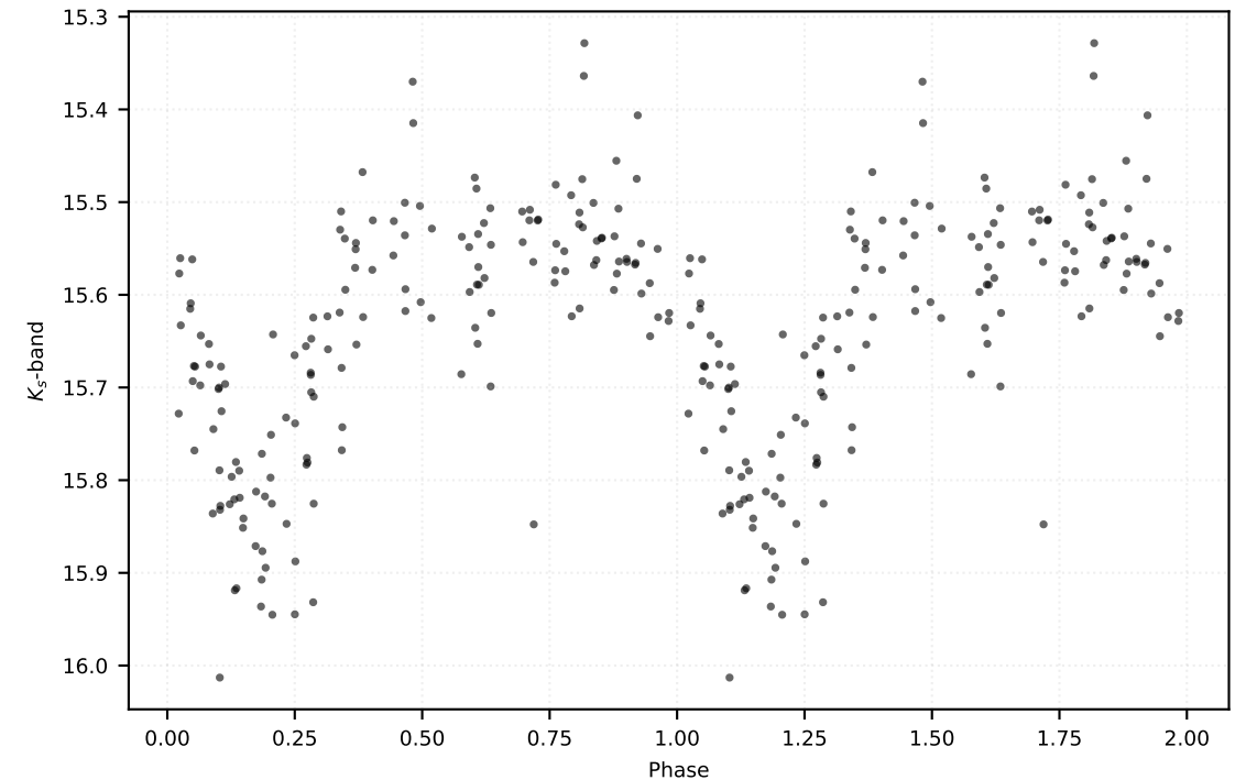
P: 0.69747 d | Class: RP | Subclass: CEP-10T | Field b279
