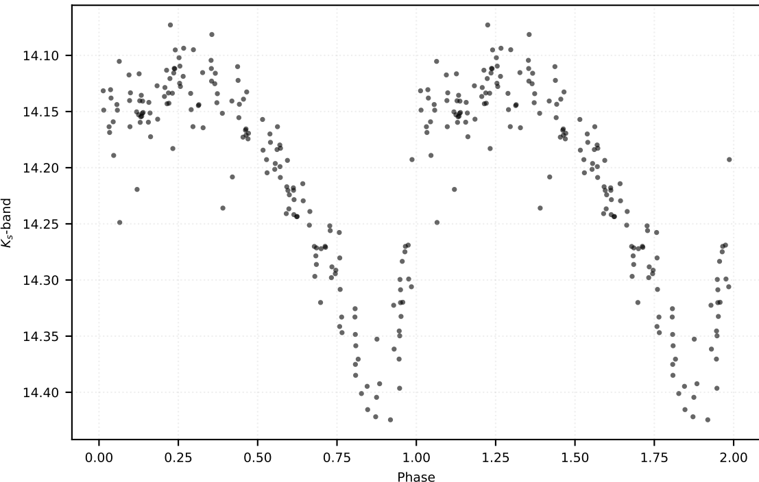
P: 0.51497 d | Class: RP | Subclass: RRab | Field b278
