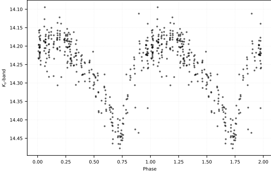
P: 0.51250 d | Class: RP | Subclass: RRab | Field b278
