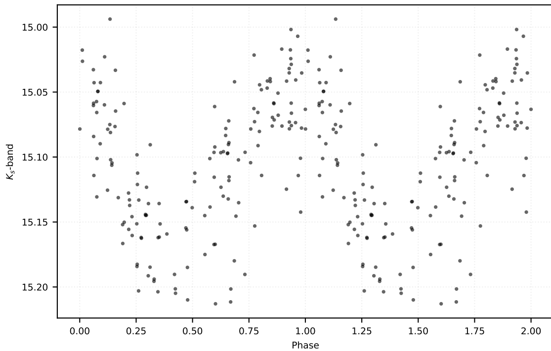
P: 0.31571 d | Class: RP | Subclass: RRc | Field b279
