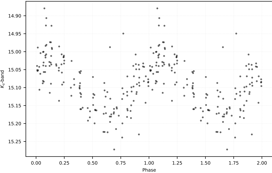
P: 0.11799 d | Class: RP | Subclass: UVAR | Field b279
