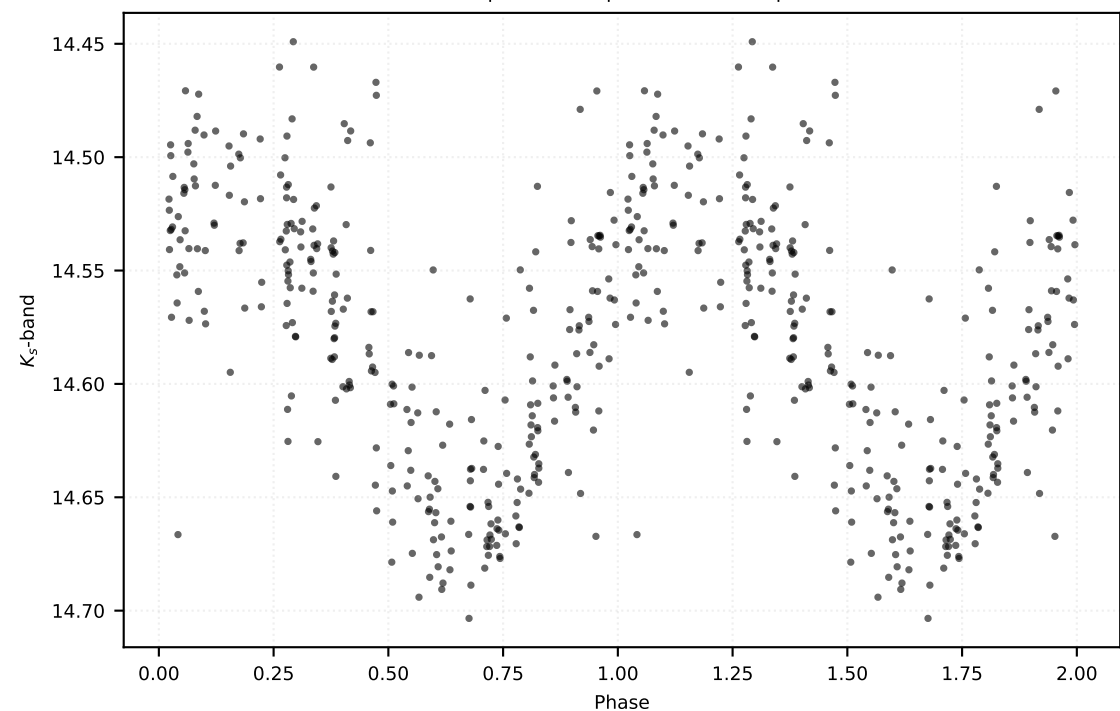
P: 0.25610 d | Class: RP | Subclass: RRc | Field b278
