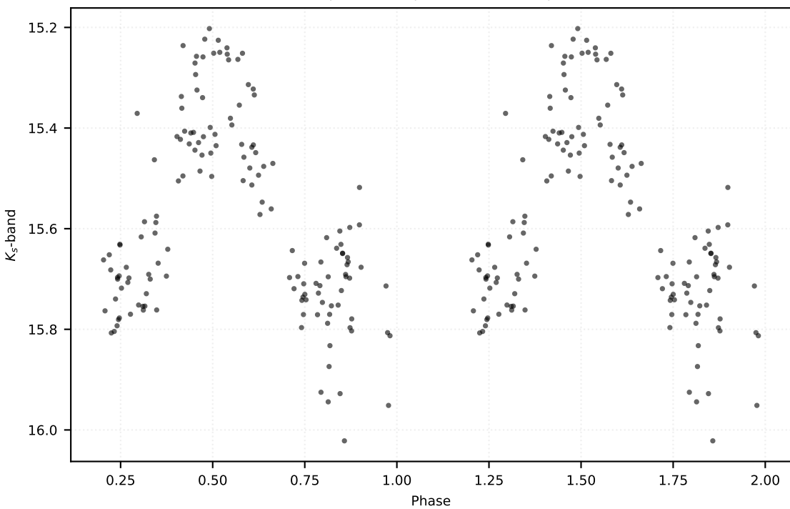
P: 0.29099 d | Class: RP | Subclass: UVAR | Field b279
