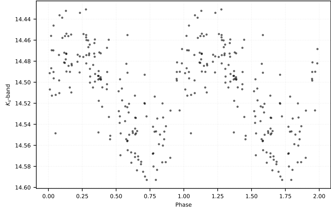
P: 0.27567 d | Class: RP | Subclass: UVAR | Field b278
