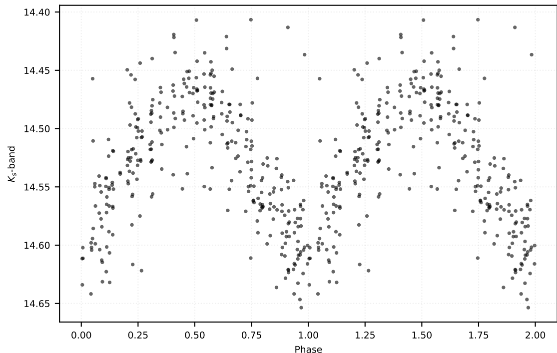
P: 3.19013 d | Class: RP | Subclass: CEP-1OT | Field b278
