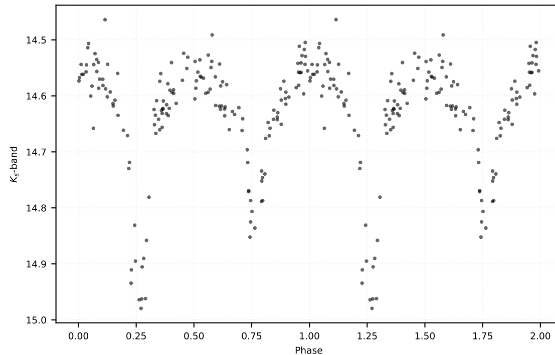
P: 2.02571 d | Class: EB | Subclass: UVAR | Field b278
