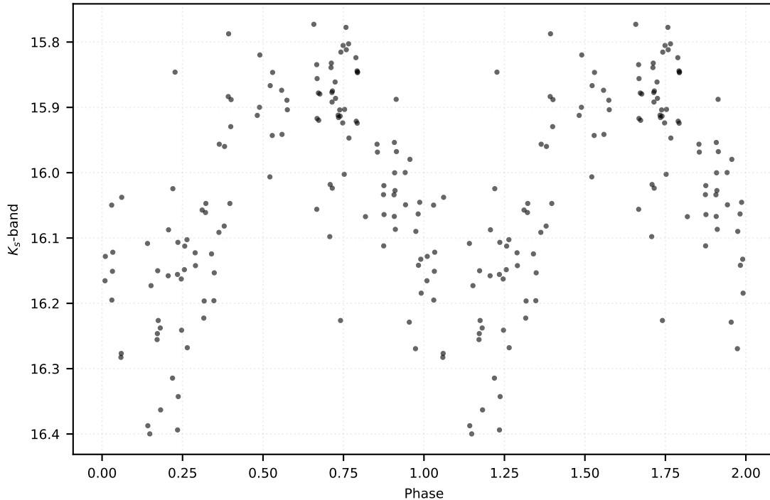
P: 0.28772 d | Class: RP | Subclass: CEP-10T | Field b279
