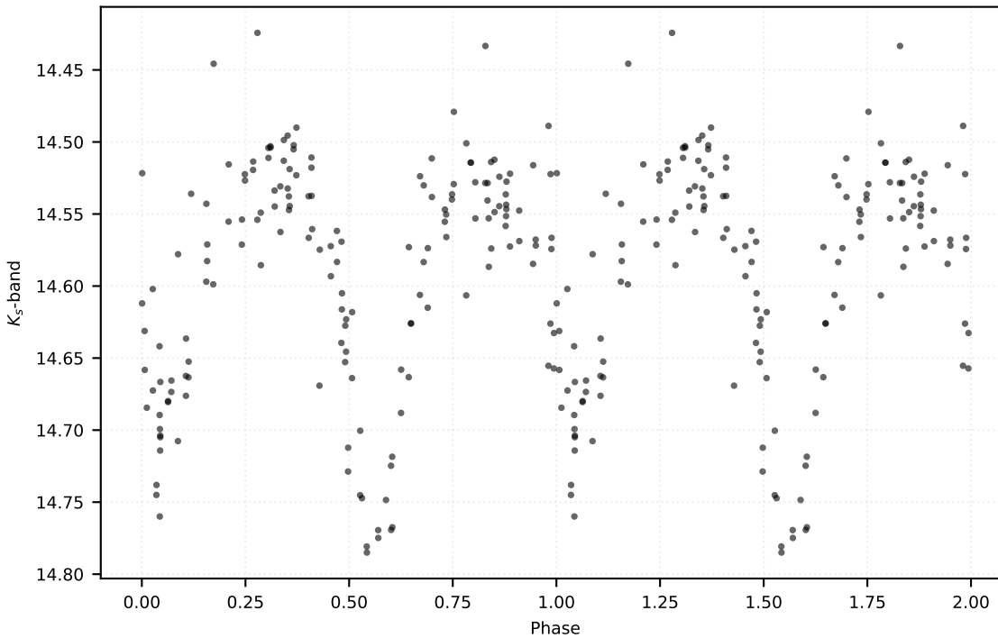
P: 1.12279 d | Class: EB | Subclass: UVAR | Field b278
