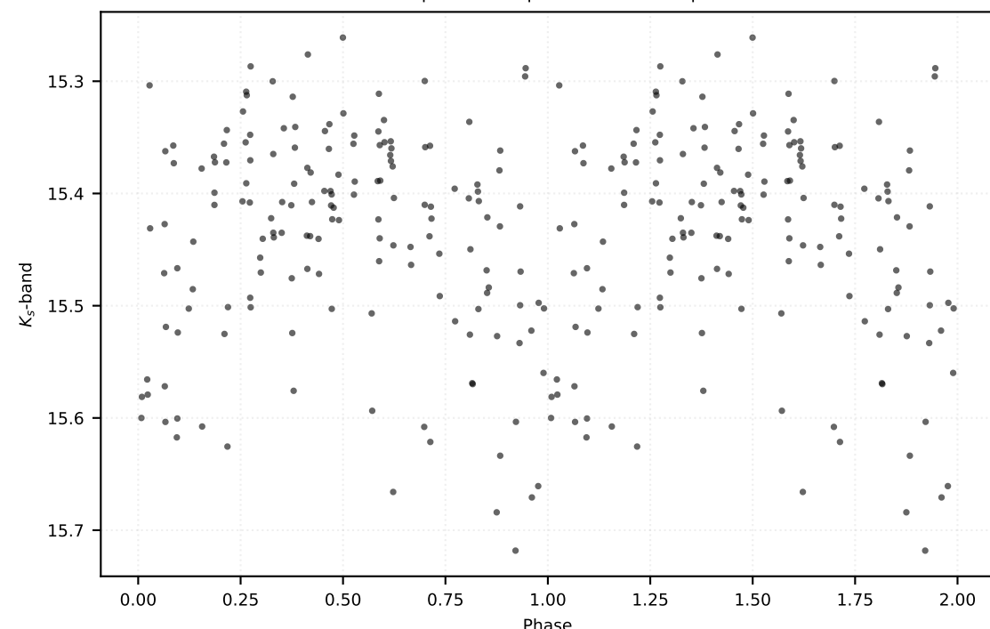
P: 0.32169 d | Class: RP | Subclass: RRab | Field b279
