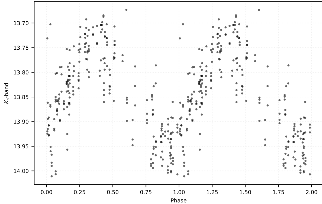
P: 0.21442 d | Class: RP | Subclass: UVAR | Field b279
