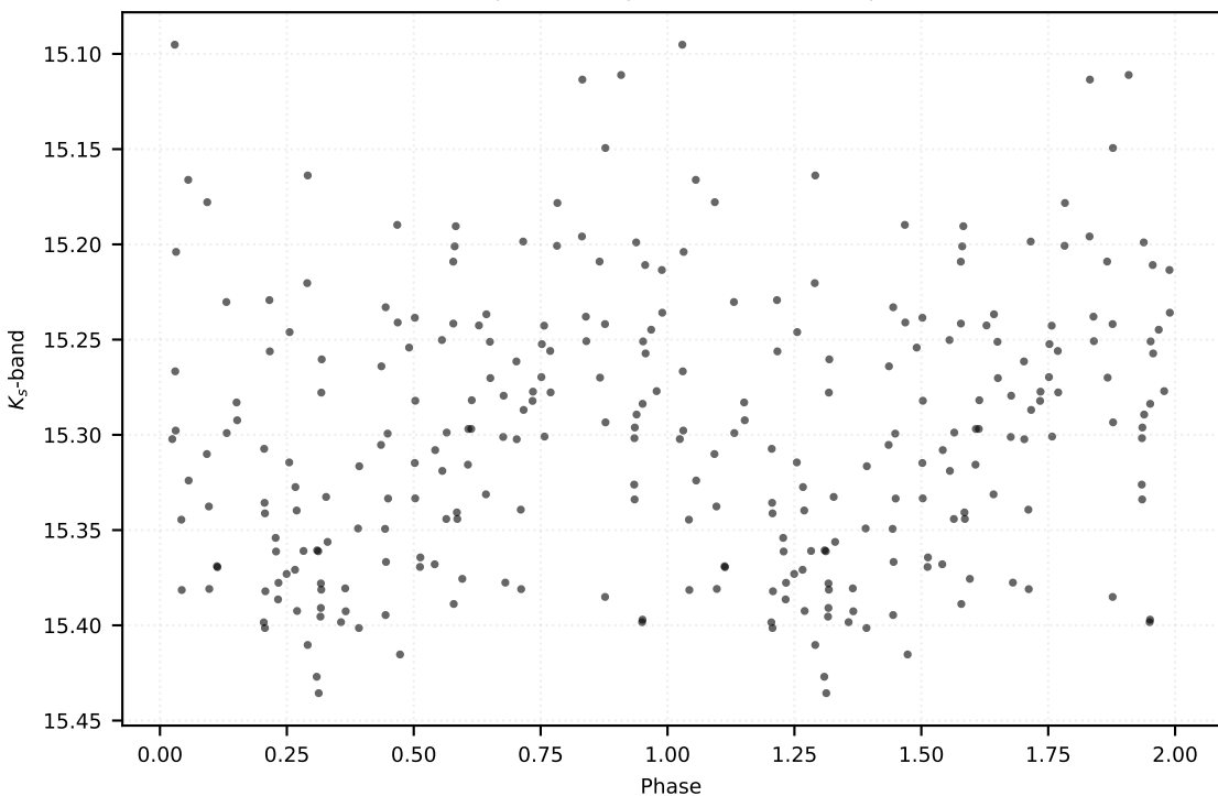
P: 0.72553 d | Class: RP | Subclass: CEP-1OT | Field b279
