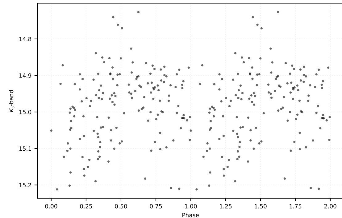
P: 30.86615 d | Class: RP | Subclass: UVAR | Field b278
