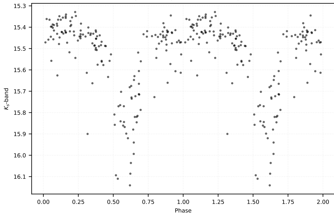
P: 1.44662 d | Class: RP | Subclass: CEP-10T | Field b279
