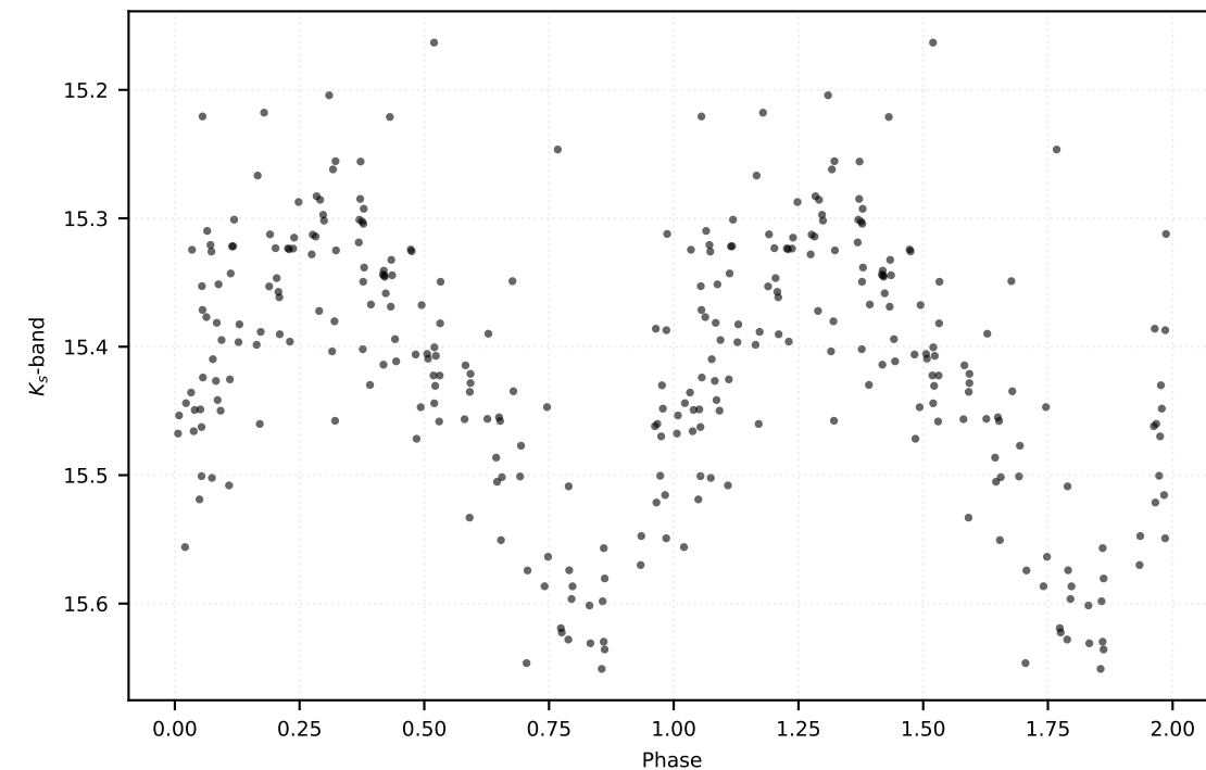
P: 0.31731 d | Class: RP | Subclass: RRab | Field b279
