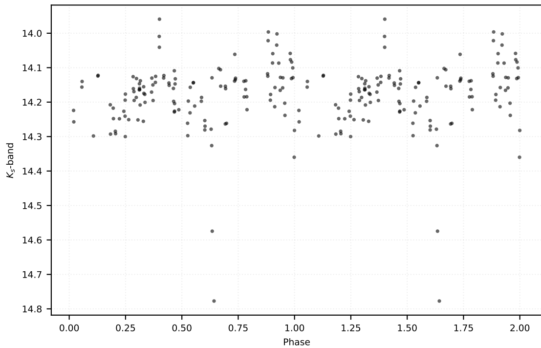
P: 0.44597 d | Class: EB | Subclass: EA | Field b279
