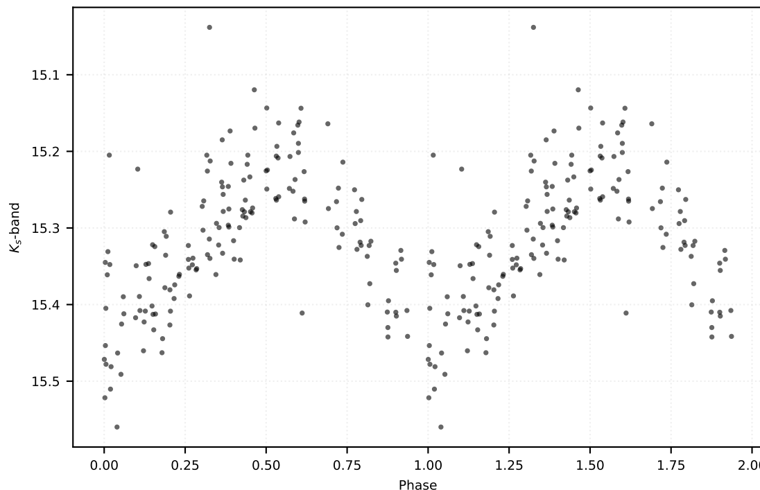
P: 0.51798 d | Class: RP | Subclass: CEP-10T | Field b279
