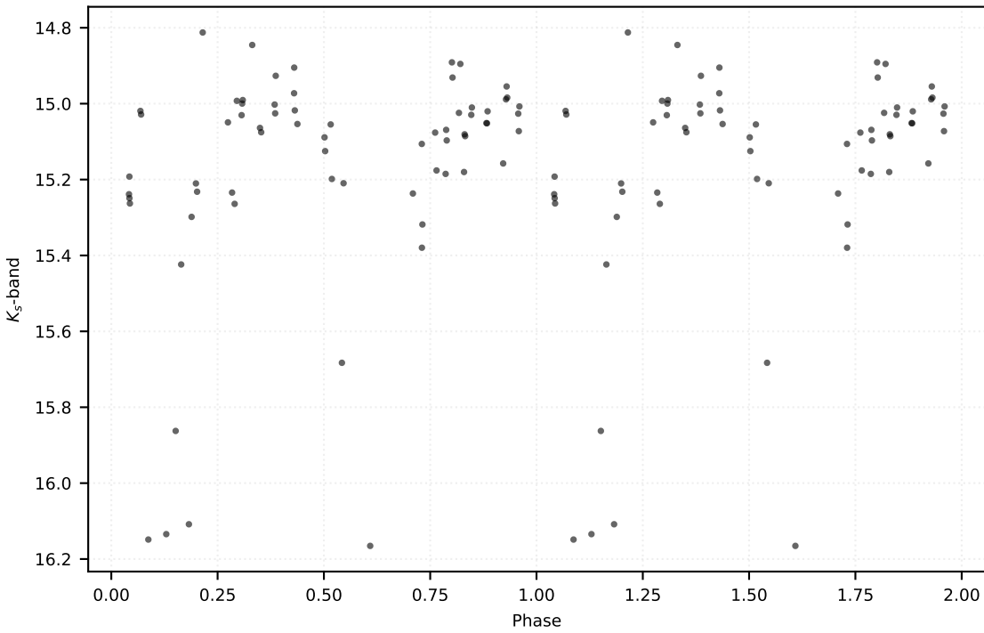
P: 3.37788 d | Class: EB | Subclass: EA | Field b278
