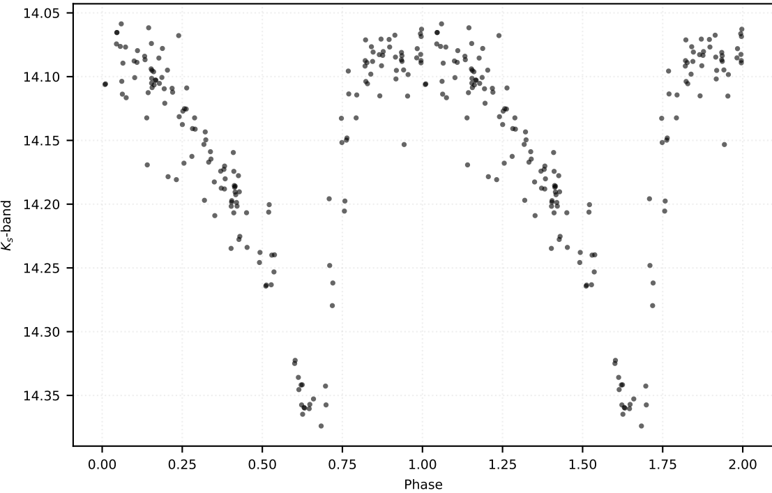
P: 0.50276 d | Class: RP | Subclass: RRab | Field b278
