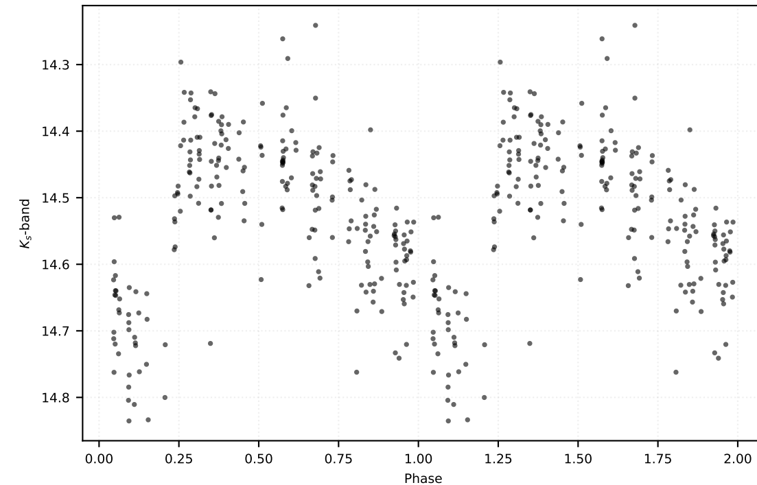
P: 0.44022 d | Class: RP | Subclass: RRab | Field b278
