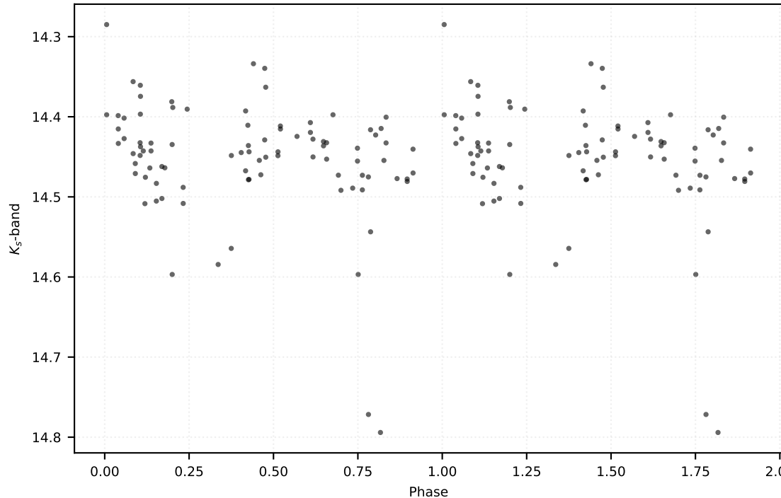
P: 0.37428 d | Class: EB | Subclass: EA | Field b279
