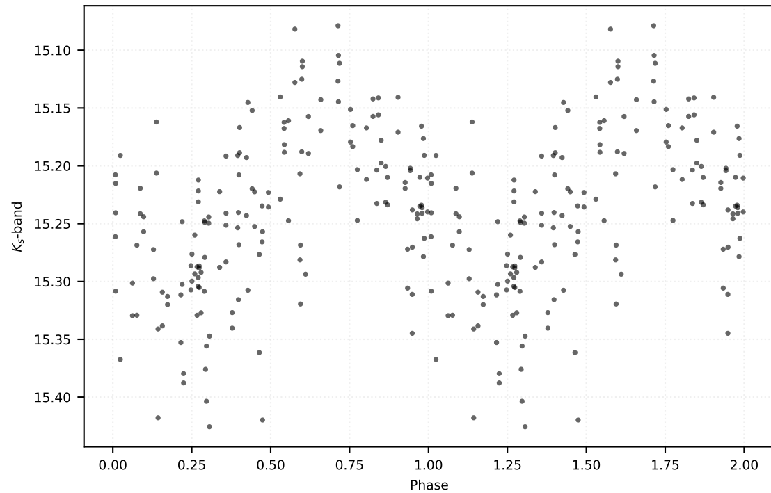
P: 33.29385 d | Class: RP | Subclass: CEP-F | Field b279
