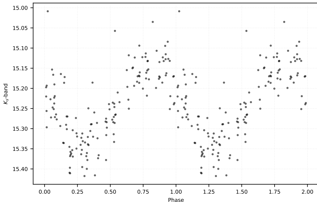
P: 17.79251 d | Class: RP | Subclass: UVAR | Field b278
