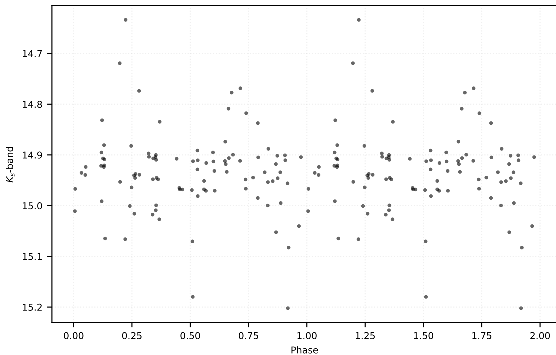
P: 0.70723 d | Class: EB | Subclass: EA | Field b278
