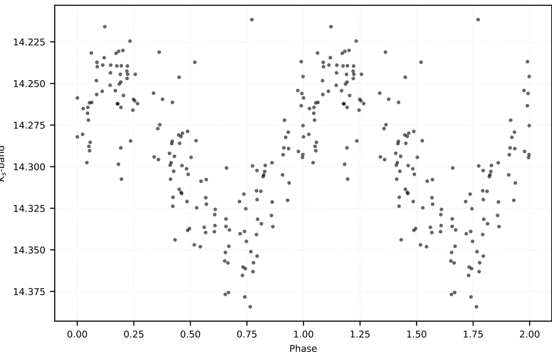
P: 0.14032 d | Class: RP | Subclass: UVAR | Field b278
