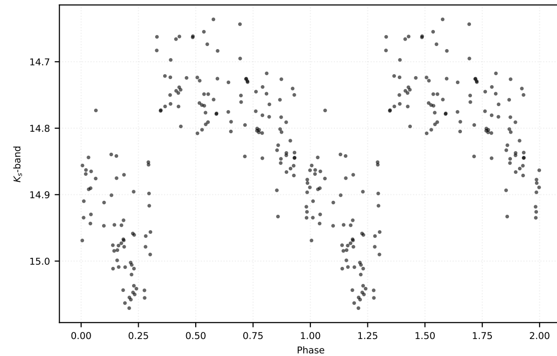
P: 0.51379 d | Class: RP | Subclass: RRab | Field b279
