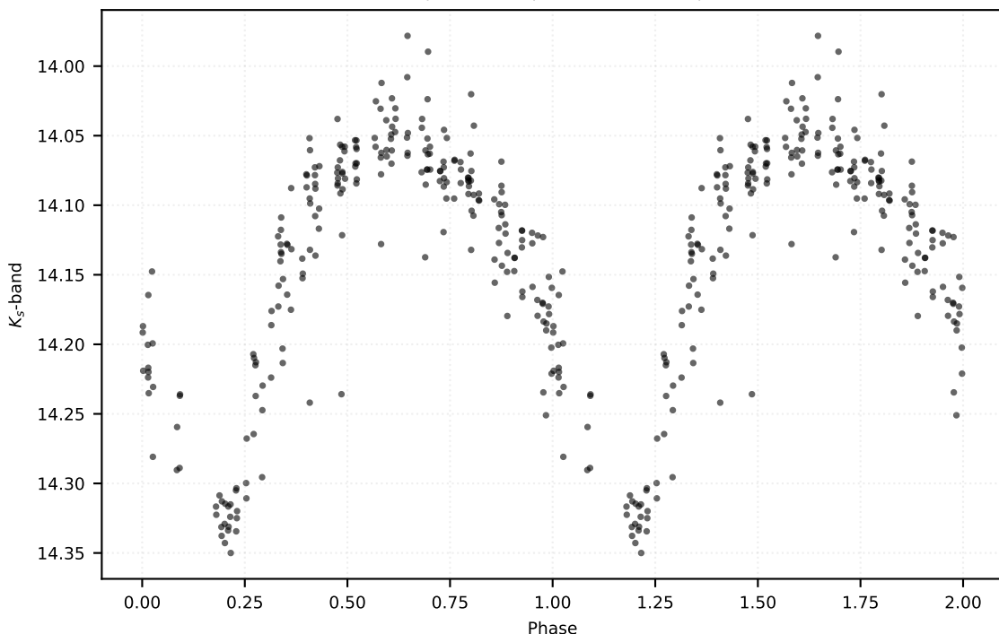
P: 0.47905 d | Class: RP | Subclass: RRab | Field b279
