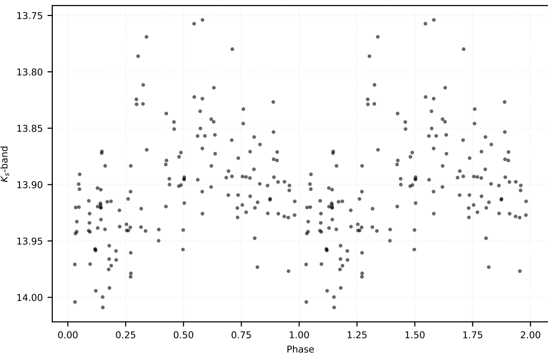
P: 0.97335 d | Class: RP | Subclass: CEP-1OT | Field b278
