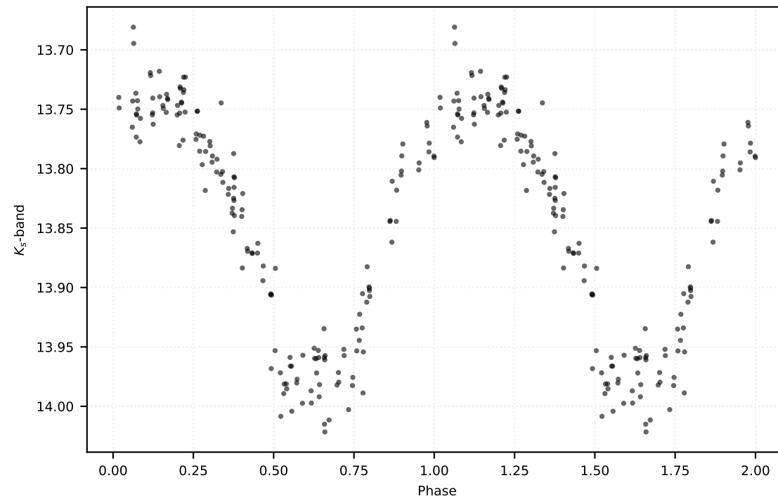
P: 0.38128 d | Class: RP | Subclass: CEP-1OT | Field b279
