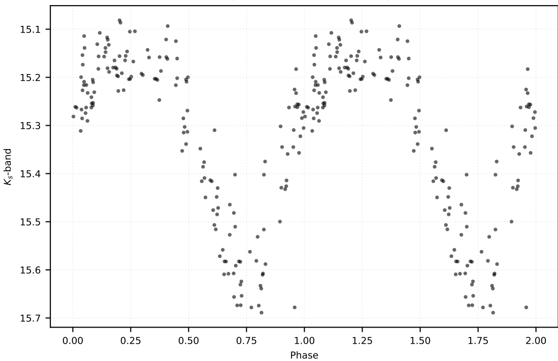
P: 0.13238 d | Class: RP | Subclass: UVAR | Field b279
