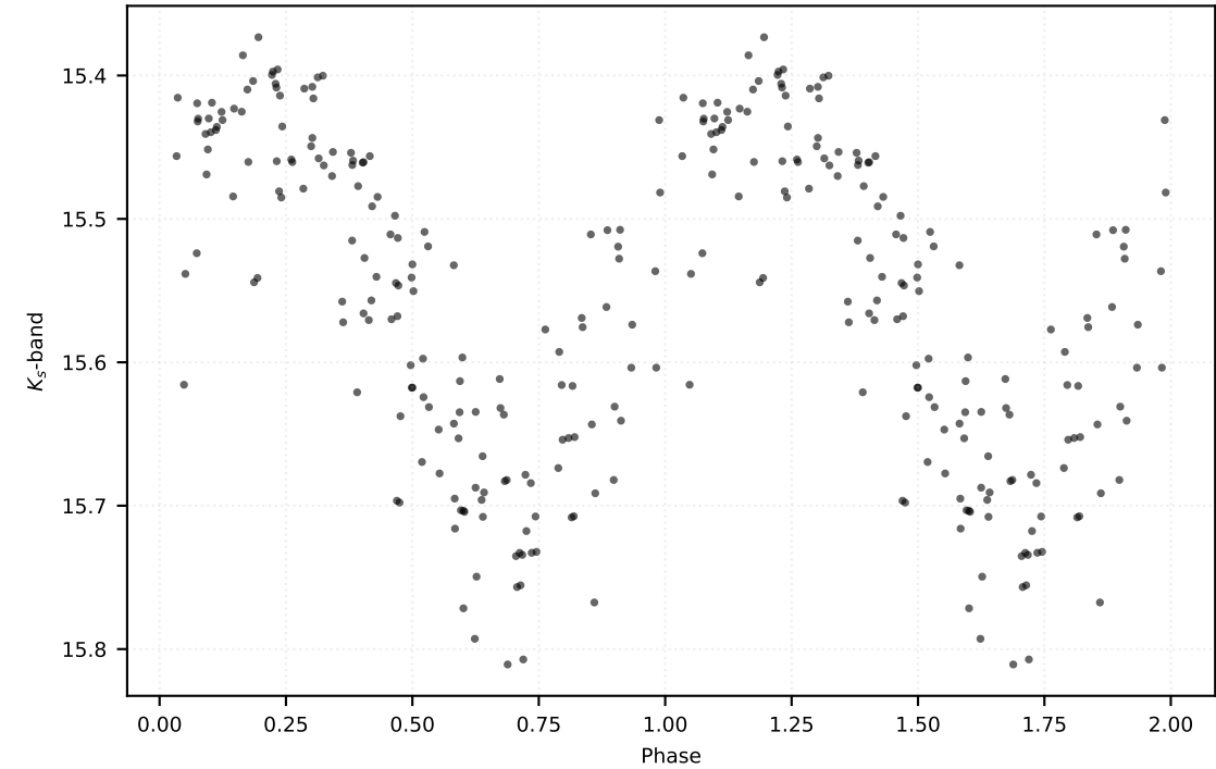
P: 0.18181 d | Class: RP | Subclass: UVAR | Field b279
