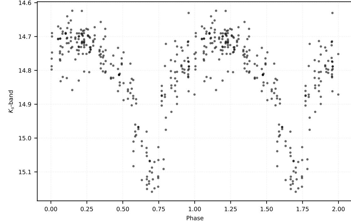
P: 0.24003 d | Class: RP | Subclass: CEP-1OT | Field b278
