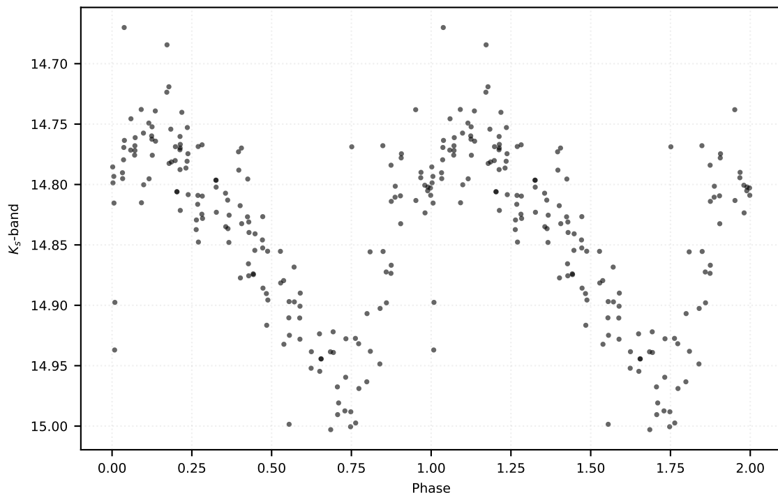
P: 0.40713 d | Class: RP | Subclass: RRab | Field b279
