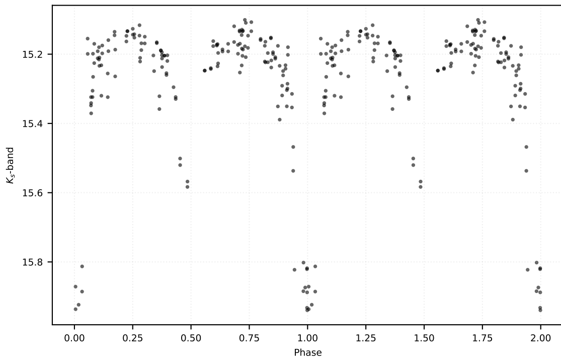
P: 0.87278 d | Class: EB | Subclass: EA | Field b279
