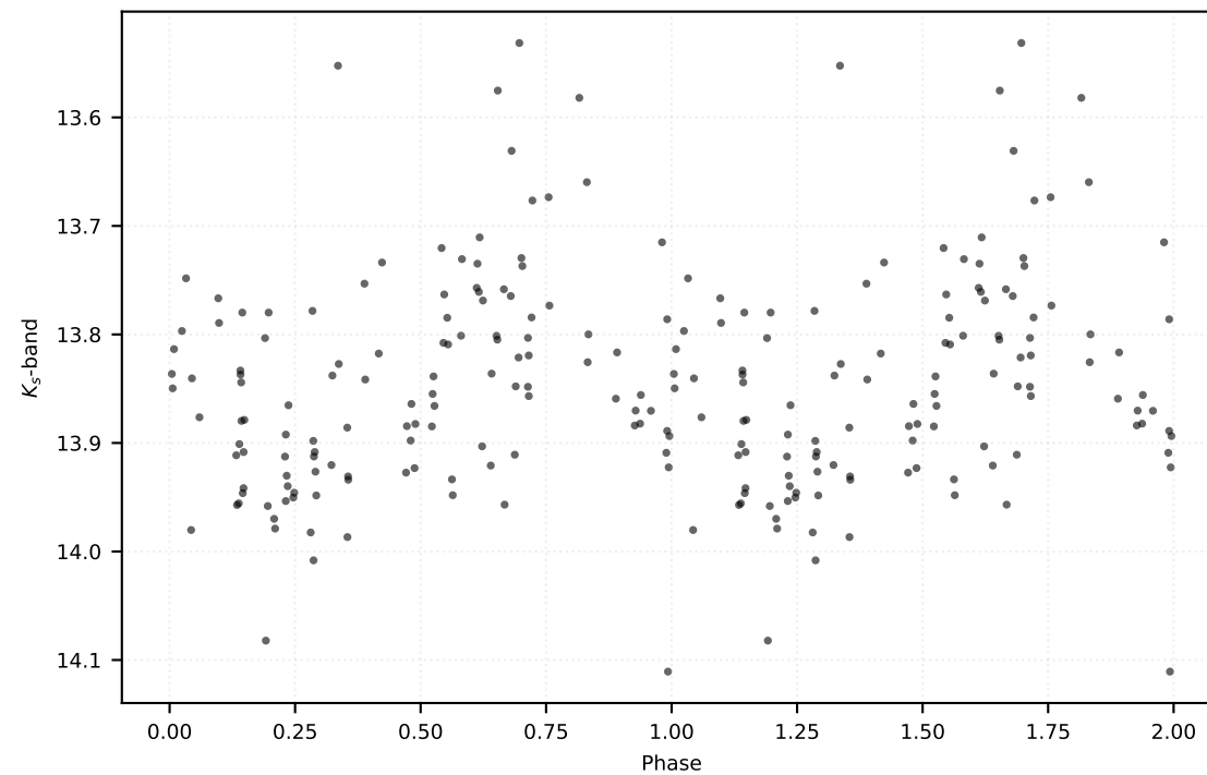
P: 12.15865 d | Class: RP | Subclass: UVAR | Field b279
