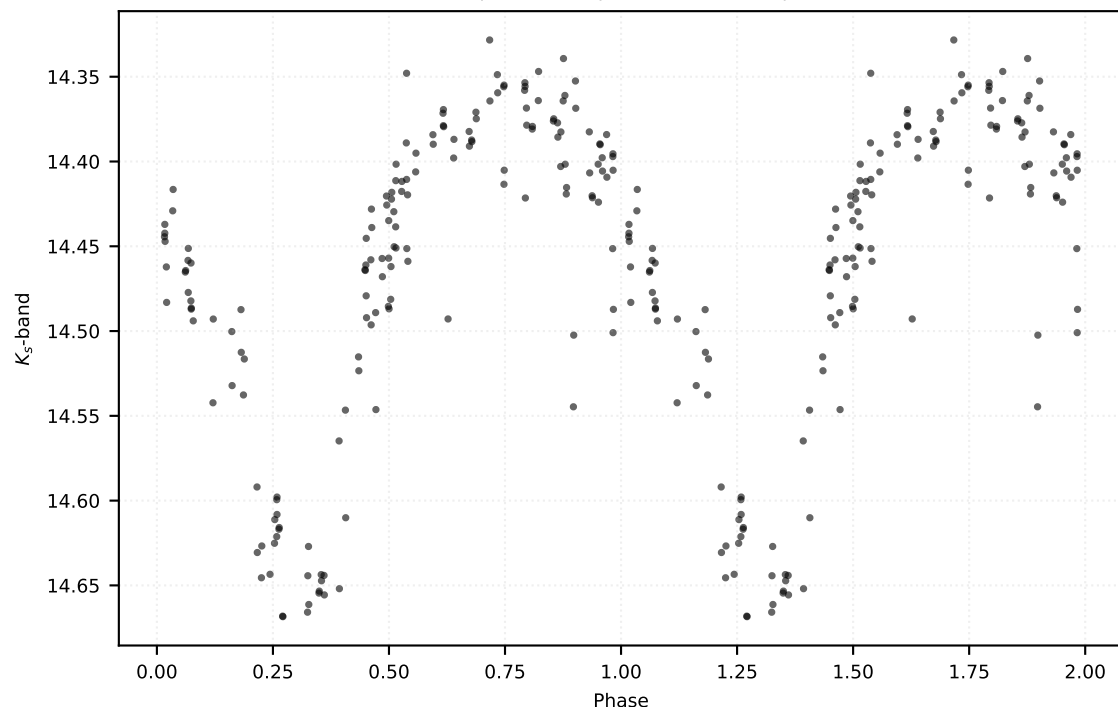
P: 0.54999 d | Class: RP | Subclass: RRab | Field b279
