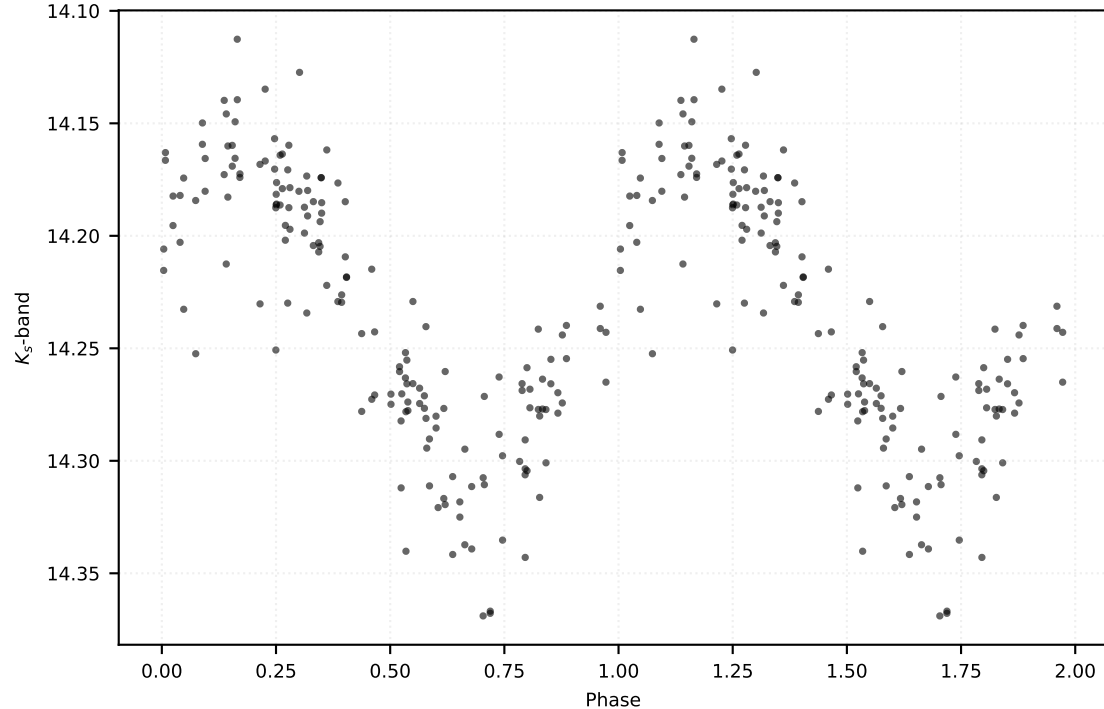
P: 3.86075 d | Class: RP | Subclass: CEP-F | Field b278
