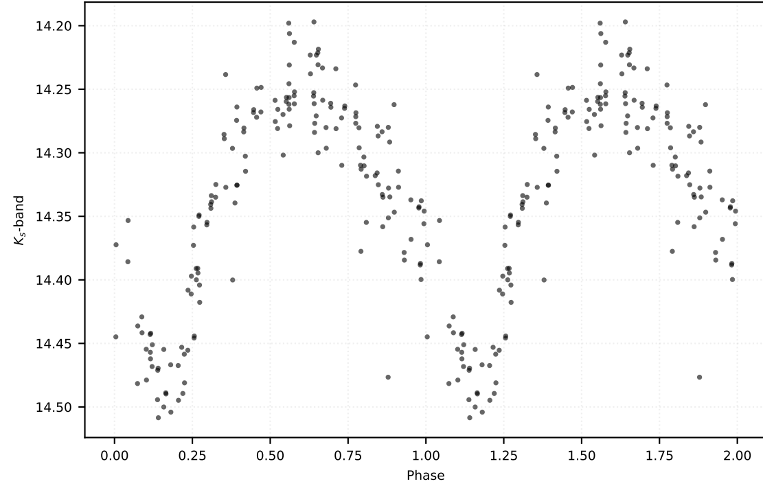
P: 0.58027 d | Class: RP | Subclass: RRab | Field b278
