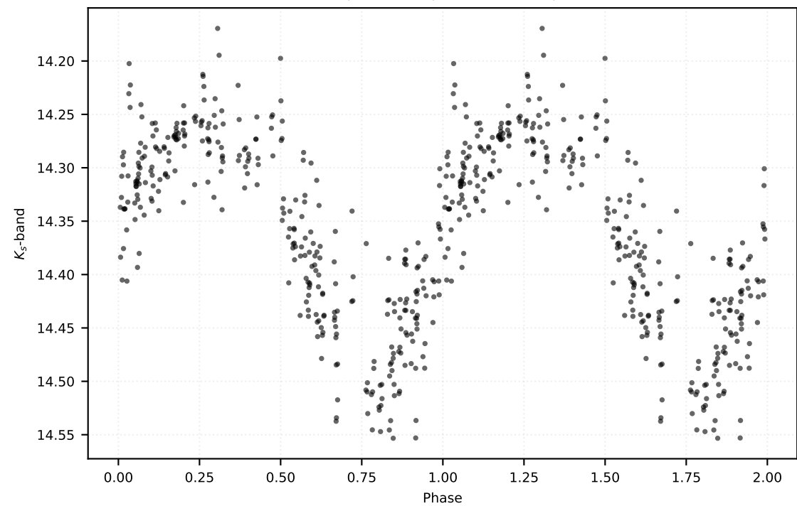
P: 0.27802 d | Class: RP | Subclass: RRc | Field b278
