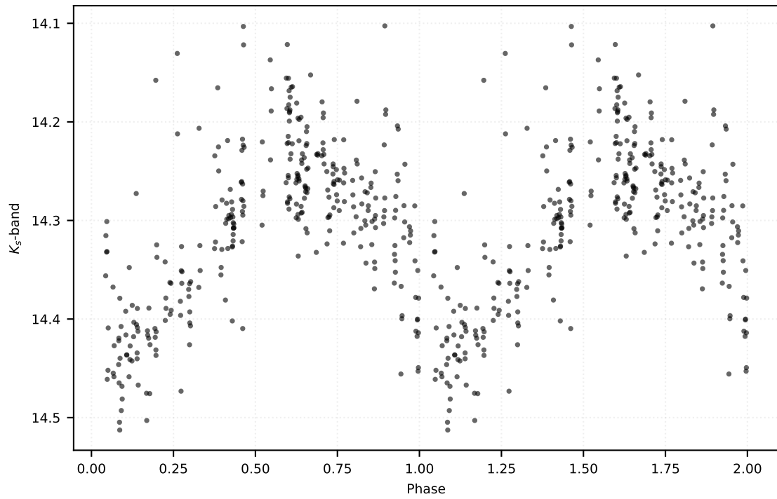
P: 0.58449 d | Class: RP | Subclass: RRab | Field b279
