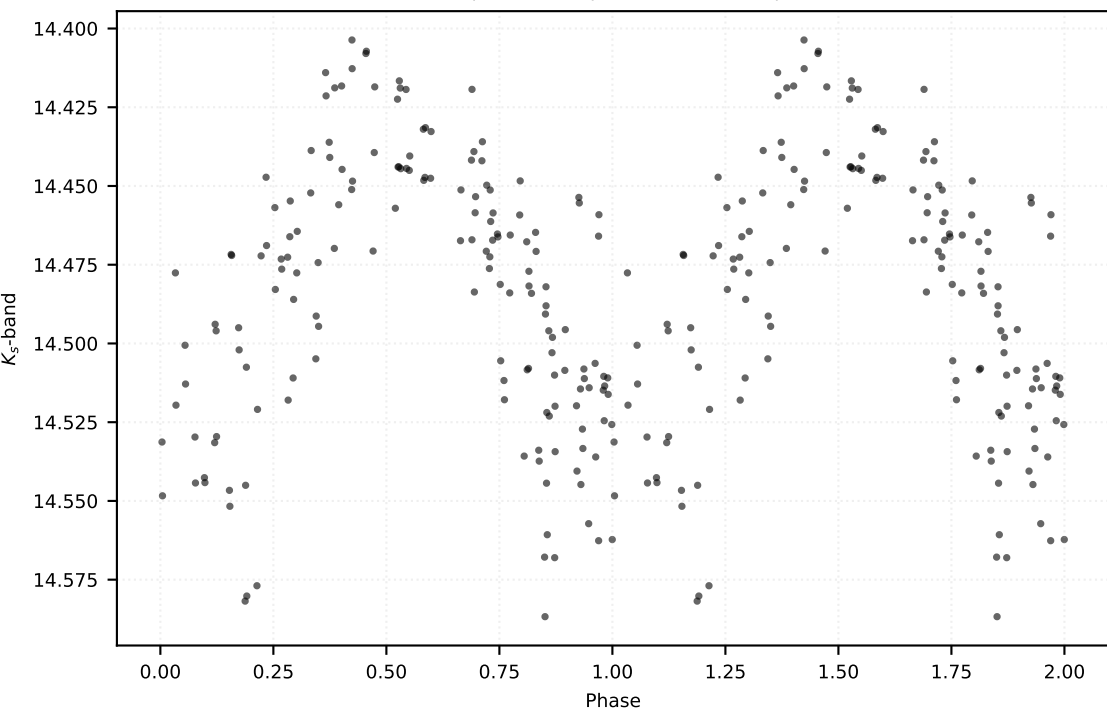
P: 0.31366 d | Class: RP | Subclass: RRab | Field b278
