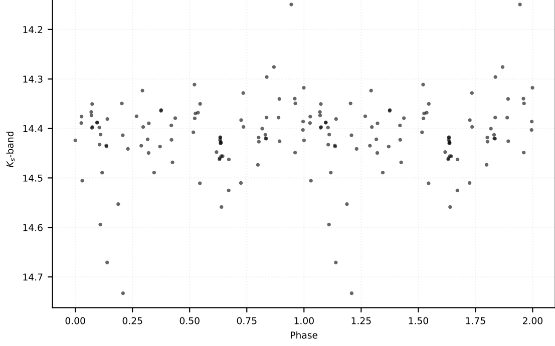
P: 0.39974 d | Class: EB | Subclass: EA | Field b278
