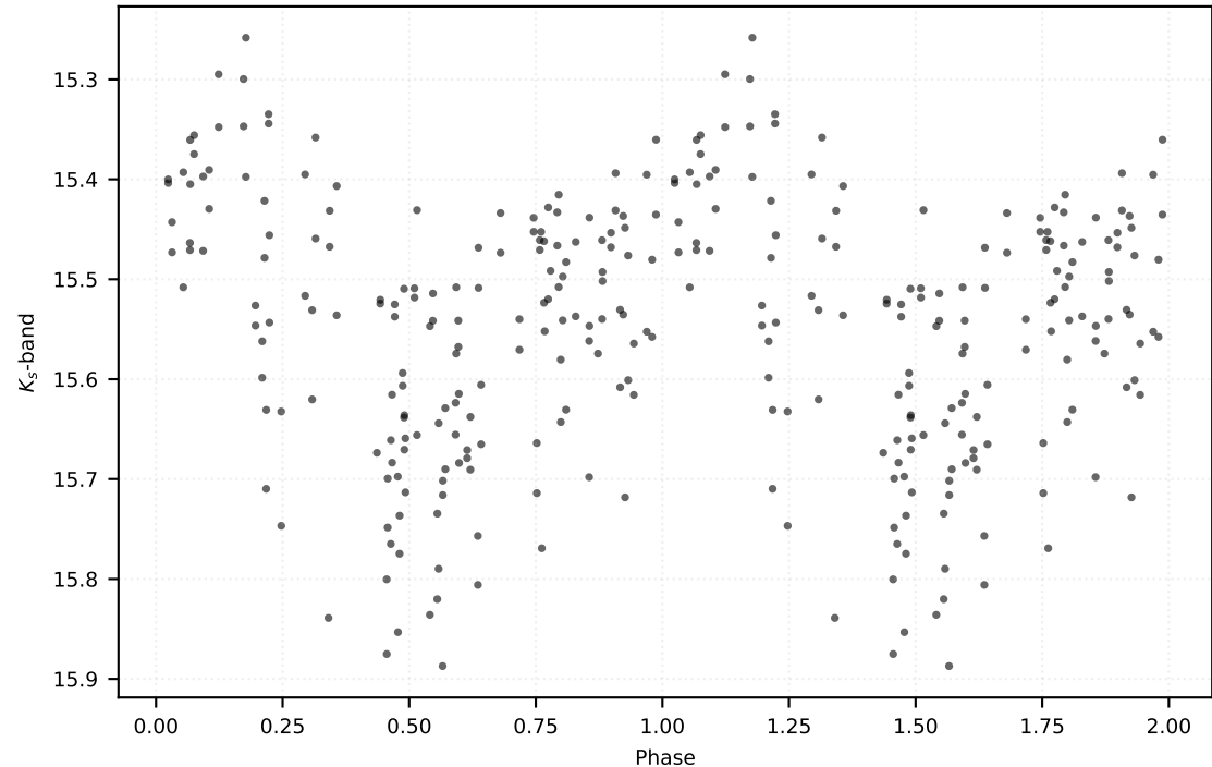
P: 0.55032 d | Class: RP | Subclass: CEP-1OT | Field b278
