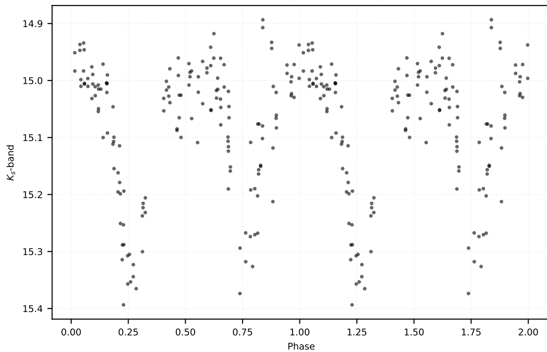
P: 0.15361 d | Class: RP | Subclass: UVAR | Field b279
