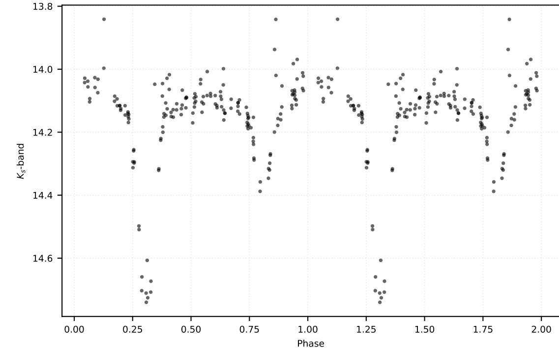
P: 3.76455 d | Class: EB | Subclass: EA | Field b278
