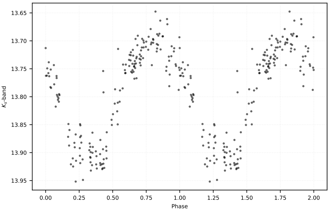
P: 0.14919 d | Class: RP | Subclass: UVAR | Field b279
