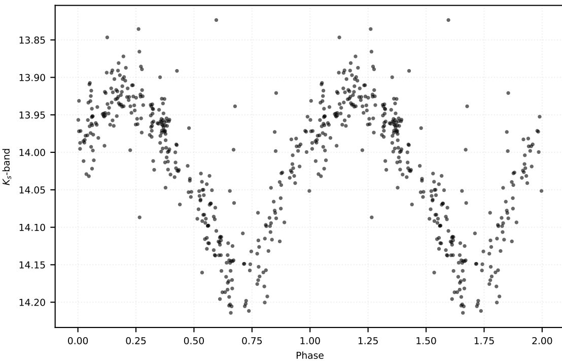
P: 0.17582 d | Class: RP | Subclass: UVAR | Field b278
