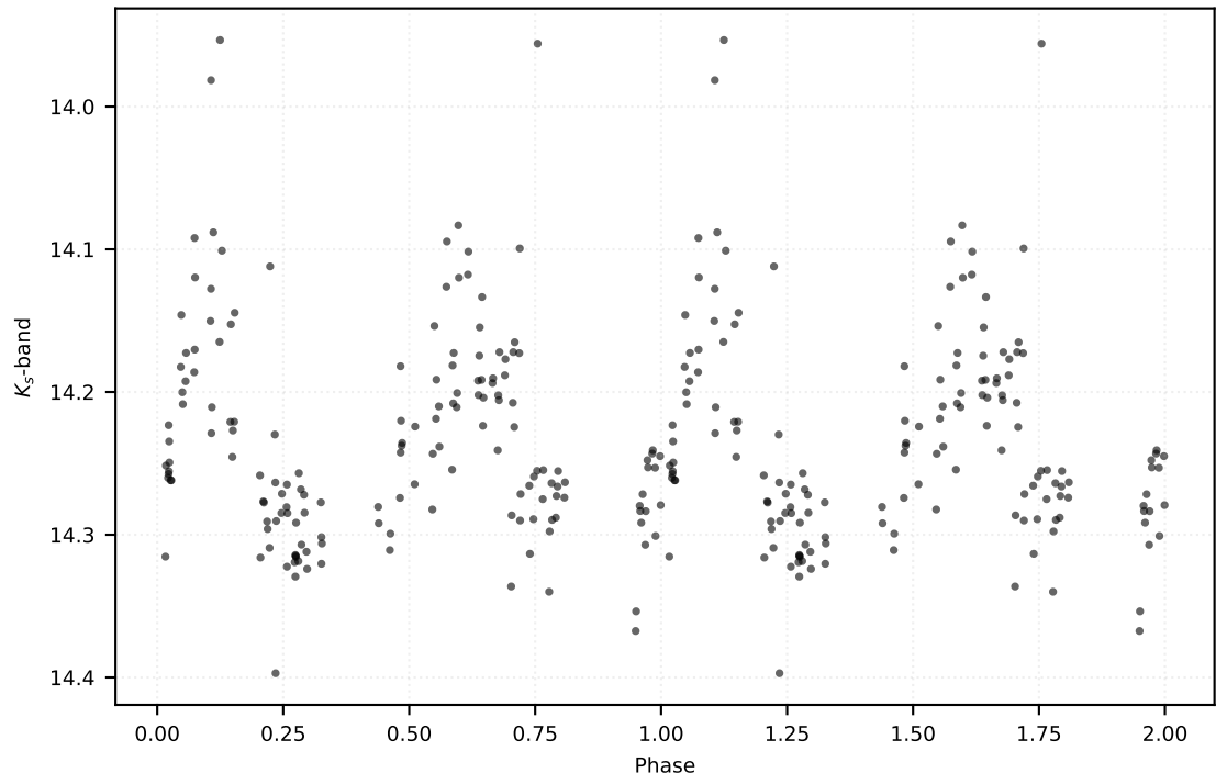
P: 1.64311 d | Class: EB | Subclass: EA | Field b279
