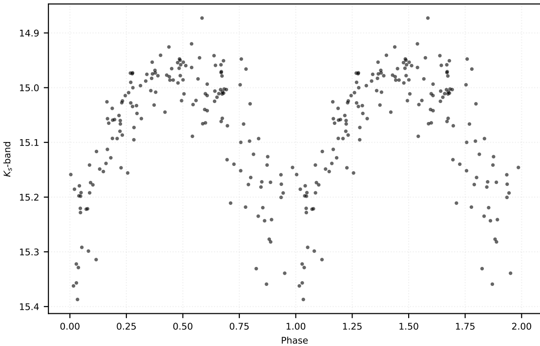
P: 0.18149 d | Class: RP | Subclass: UVAR | Field b278
