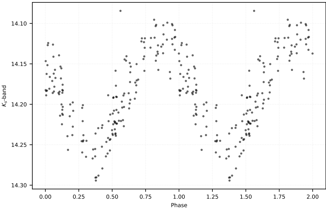
P: 0.23578 d | Class: RP | Subclass: UVAR | Field b278
