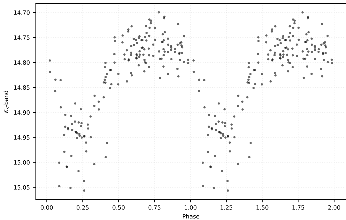
P: 0.29687 d | Class: RP | Subclass: RRc | Field b278
