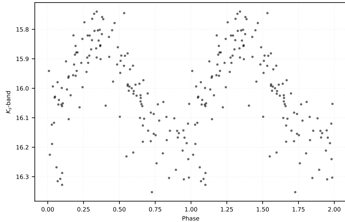
P: 4.45671 d | Class: RP | Subclass: CEP-F | Field b279
