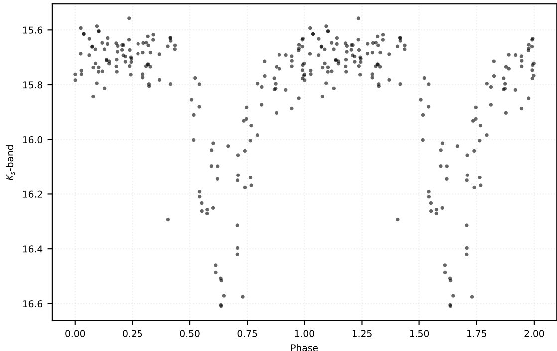
P: 3.05469 d | Class: RP | Subclass: CEP-10T | Field b278
