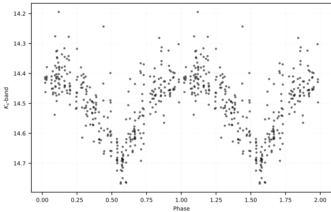
P: 0.61945 d | Class: RP | Subclass: RRab | Field b278
