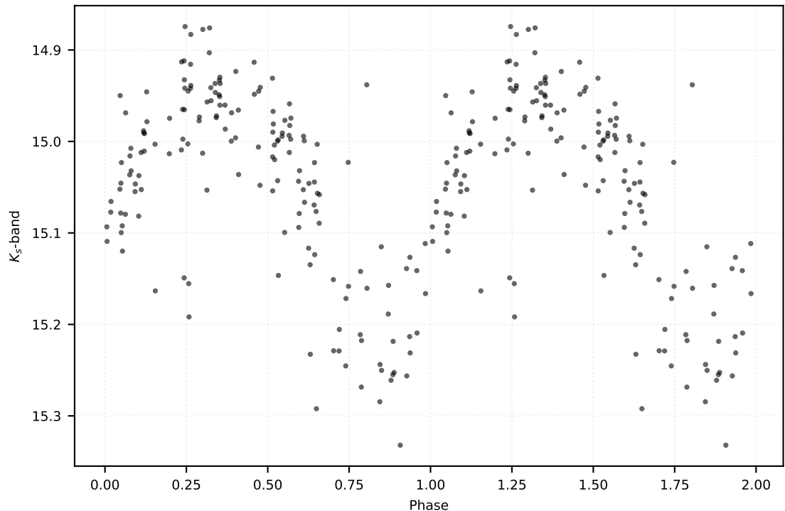
P: 0.44492 d | Class: RP | Subclass: RRc | Field b278
