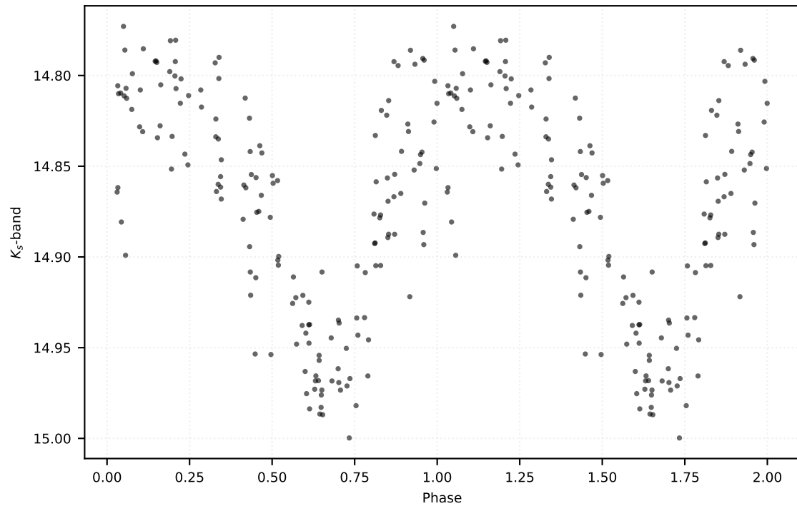
P: 13.92455 d | Class: RP | Subclass: UVAR | Field b279
