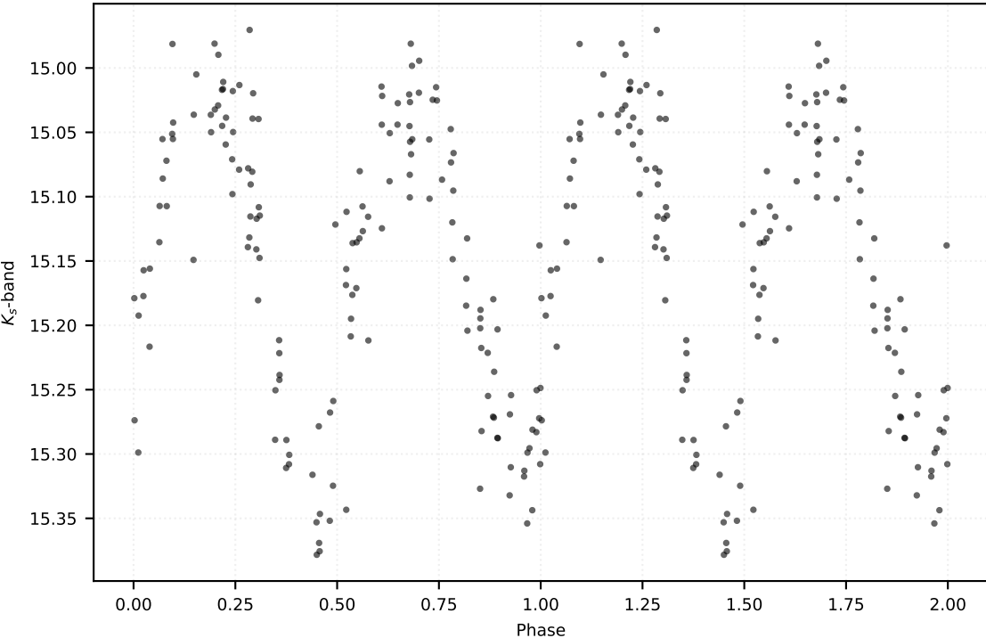
P: 0.34314 d | Class: EB | Subclass: EW | Field b278
