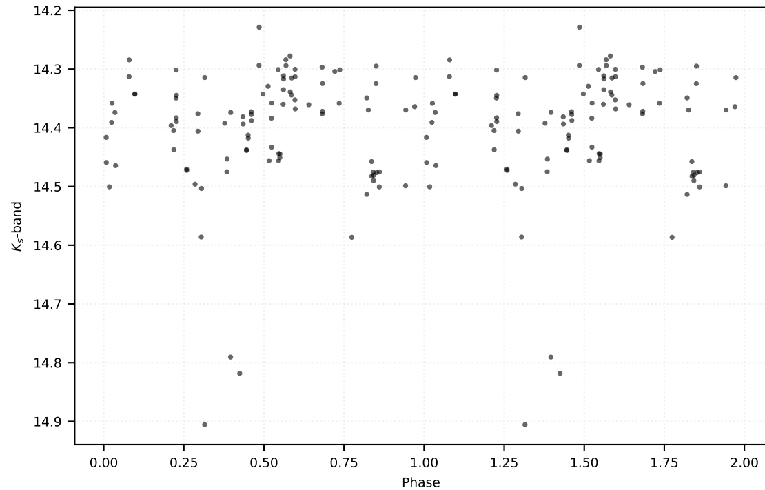
P: 10.65040 d | Class: EB | Subclass: EA | Field b279
