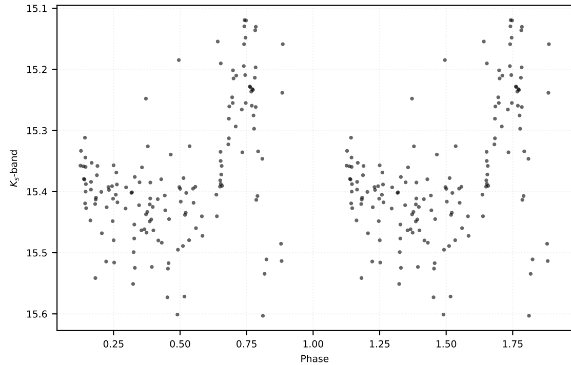
P: 0.24932 d | Class: RP | Subclass: UVAR | Field b279
