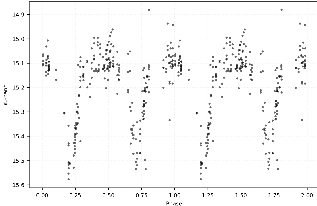
P: 4.01079 d | Class: EB | Subclass: EW | Field b278
