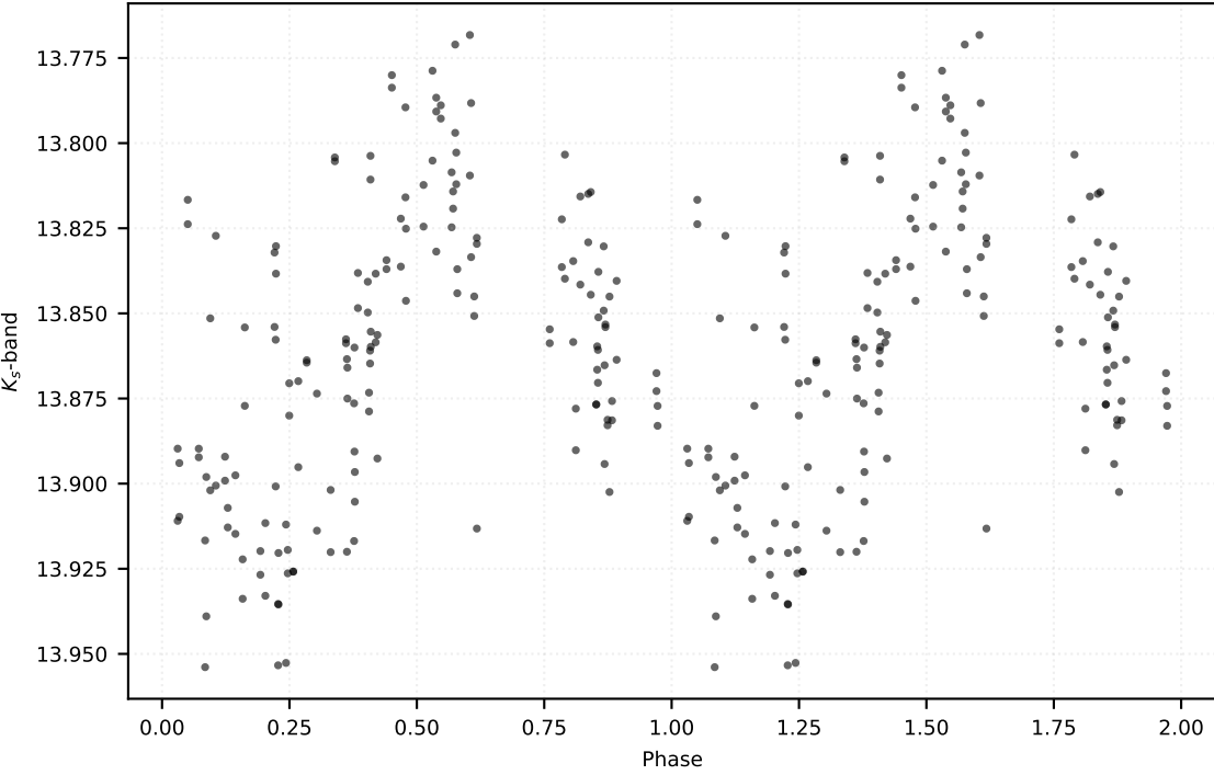
P: 69.34999 d | Class: RP | Subclass: CEP-F | Field b279
