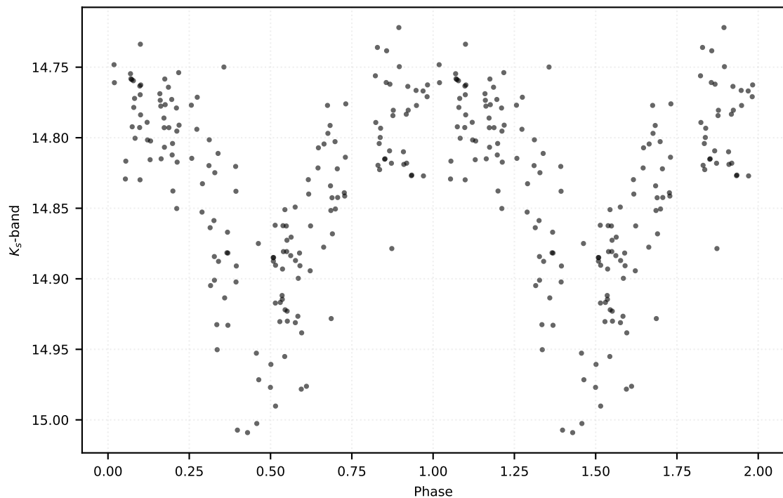
P: 0.49402 d | Class: RP | Subclass: RRab | Field b279
