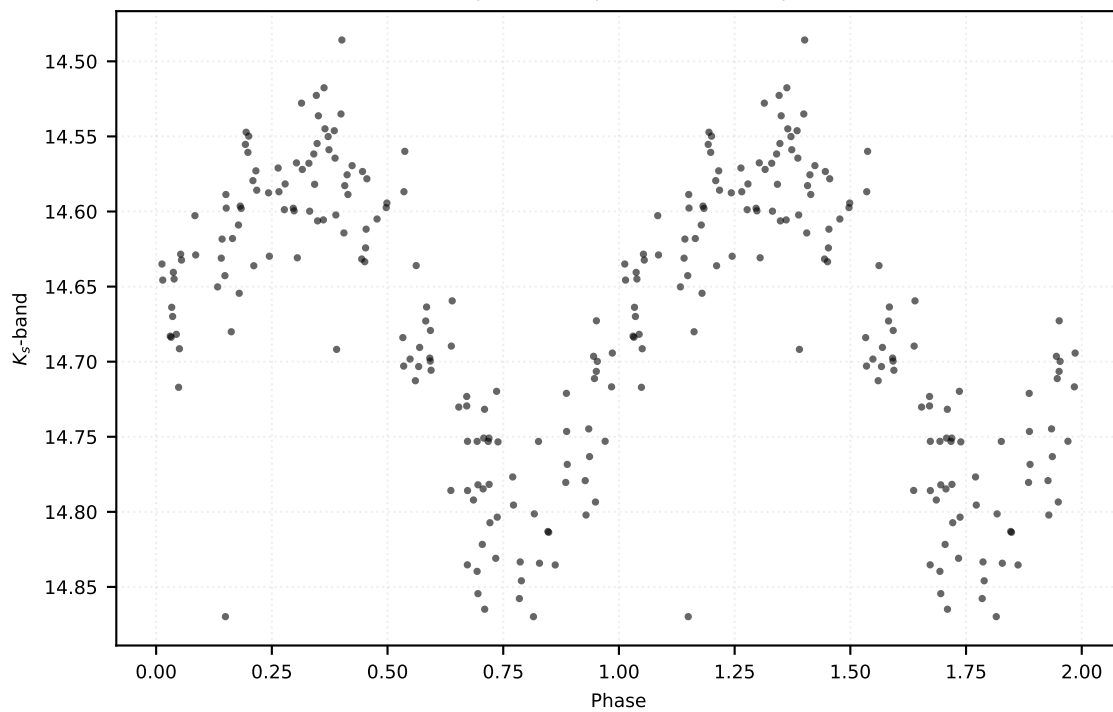
P: 0.15636 d | Class: RP | Subclass: UVAR | Field b278
