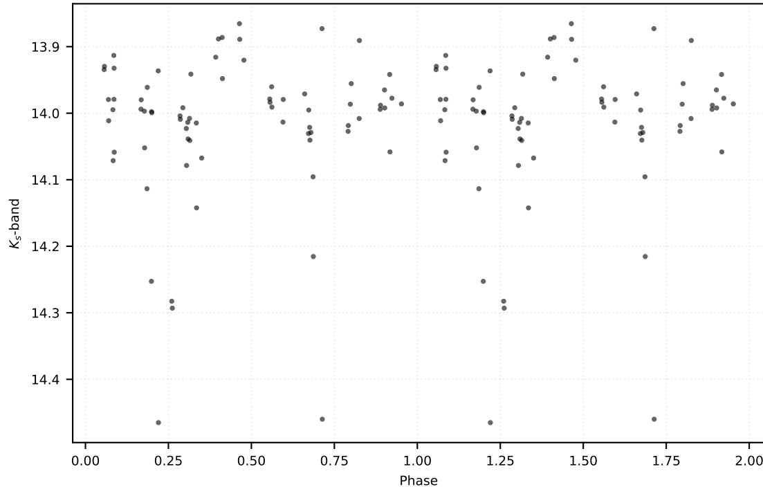
P: 0.29609 d | Class: EB | Subclass: EA | Field b279
