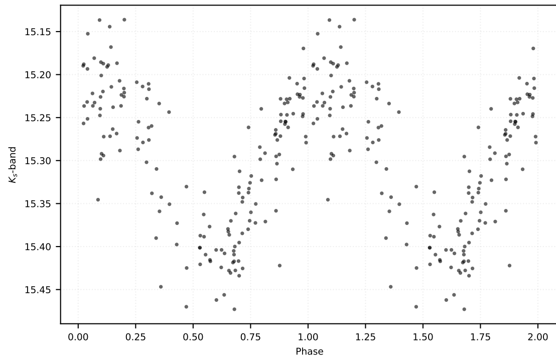
P: 0.30529 d | Class: RP | Subclass: RRab | Field b278
