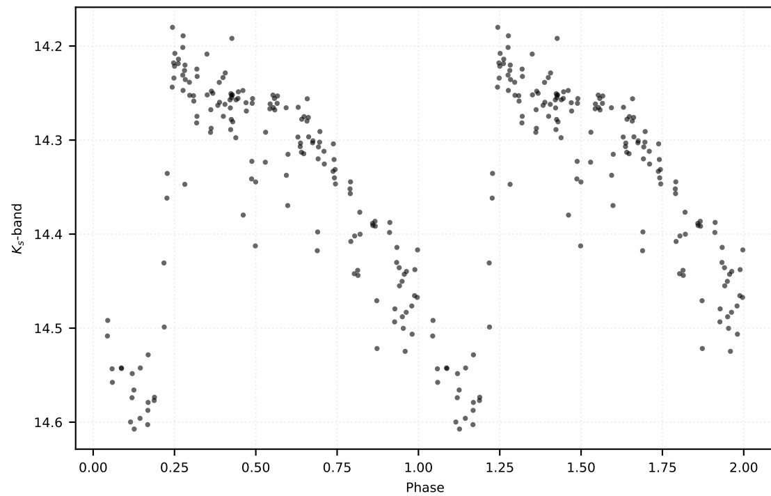
P: 0.90871 d | Class: RP | Subclass: RRab | Field b279
