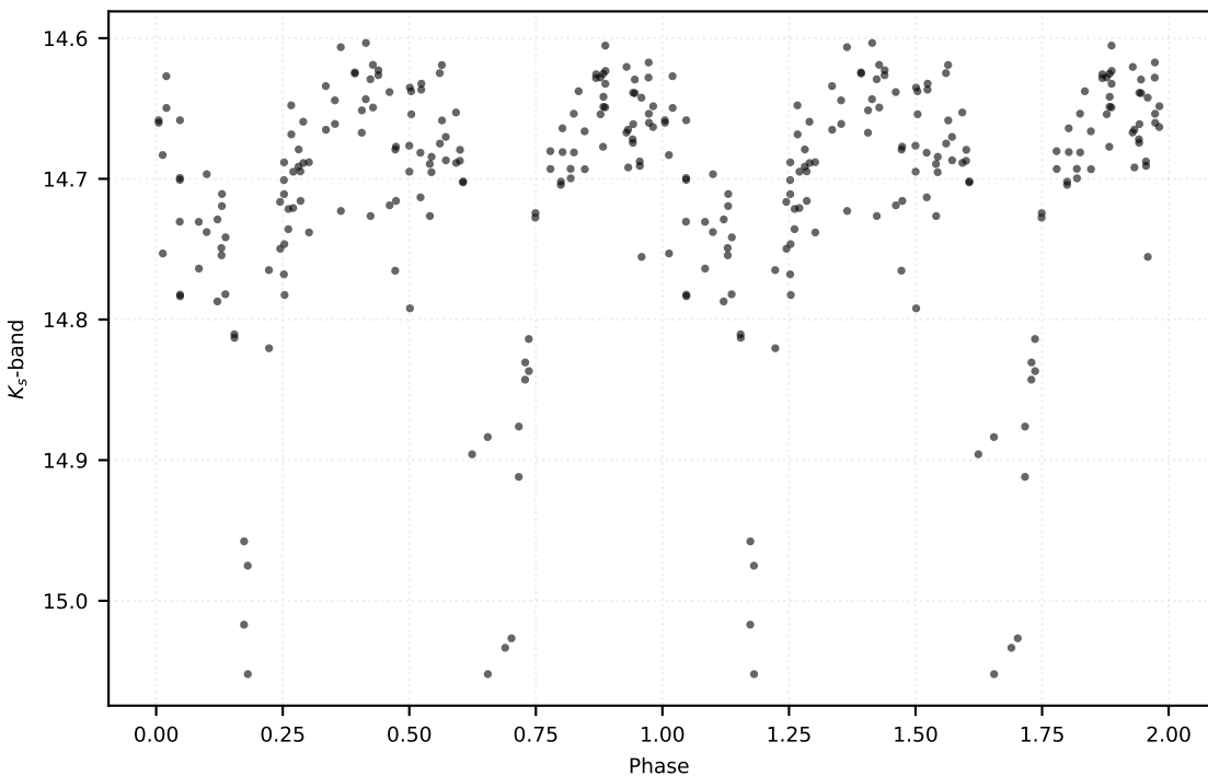
P: 3.03505 d | Class: EB | Subclass: EA | Field b279
