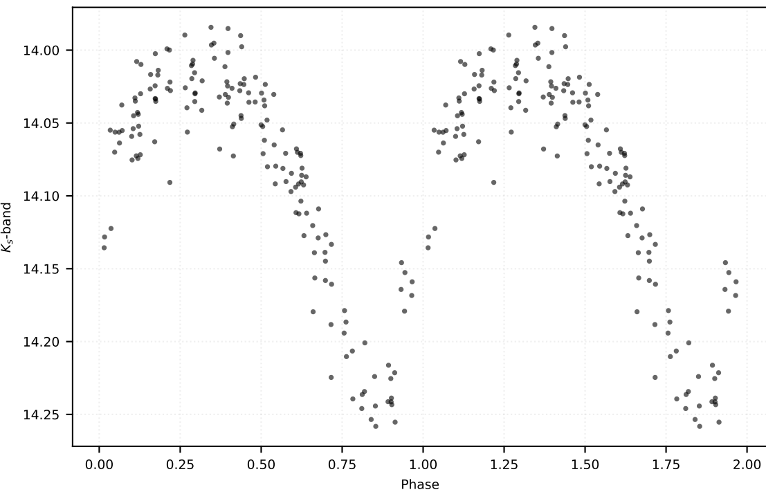
P: 0.57804 d | Class: RP | Subclass: CEP-10T | Field b279
