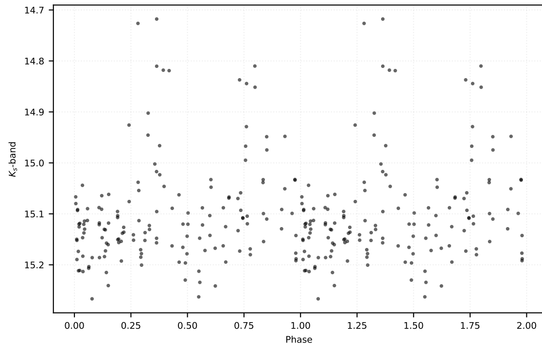
P: 0.58407 d | Class: EB | Subclass: EA | Field b278
