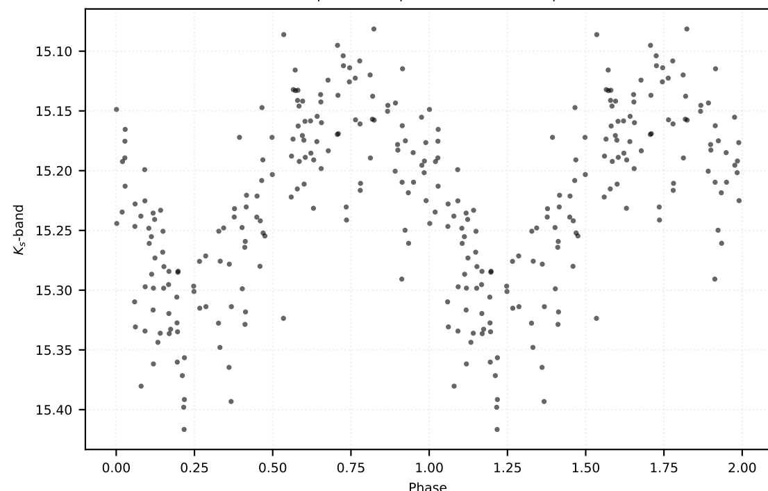
P: 0.30367 d | Class: RP | Subclass: CEP-10T | Field b279
