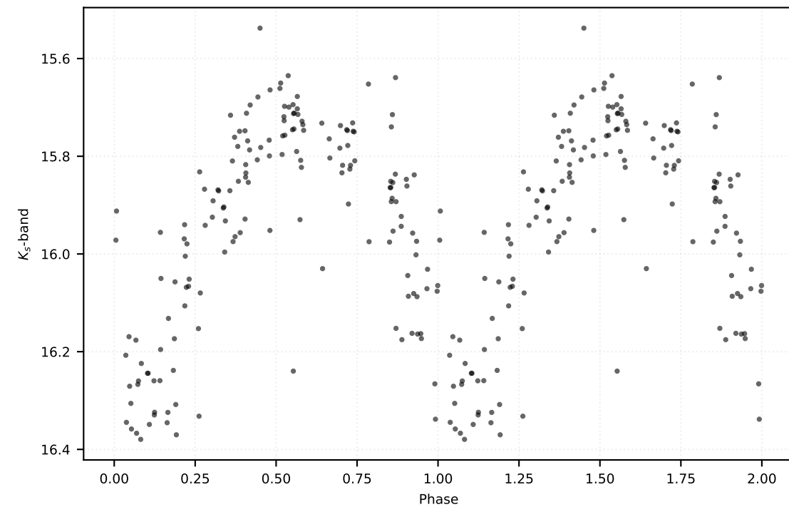
P: 0.59932 d | Class: RP | Subclass: RRc | Field b278
