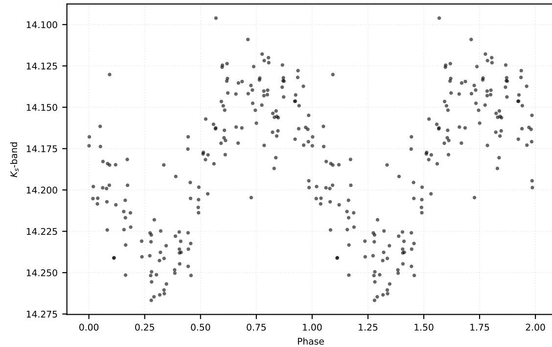
P: 0.34261 d | Class: RP | Subclass: RRc | Field b279
