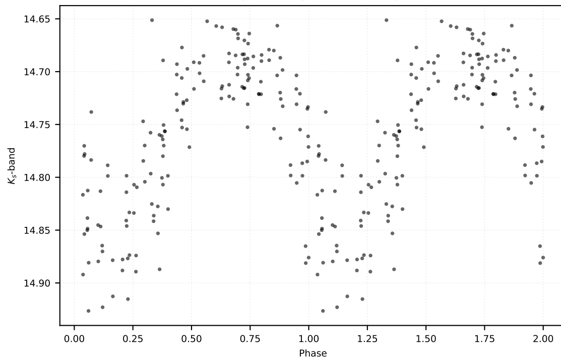
P: 0.58101 d | Class: RP | Subclass: RRab | Field b278
