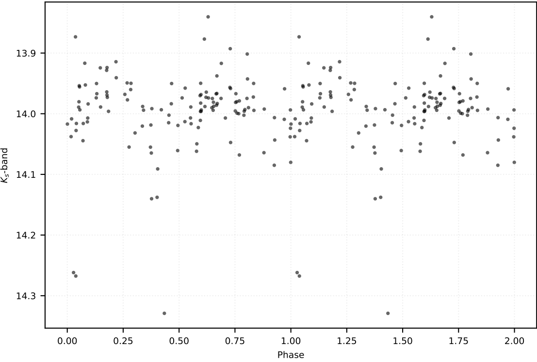
P: 0.30508 d | Class: EB | Subclass: EA | Field b279
