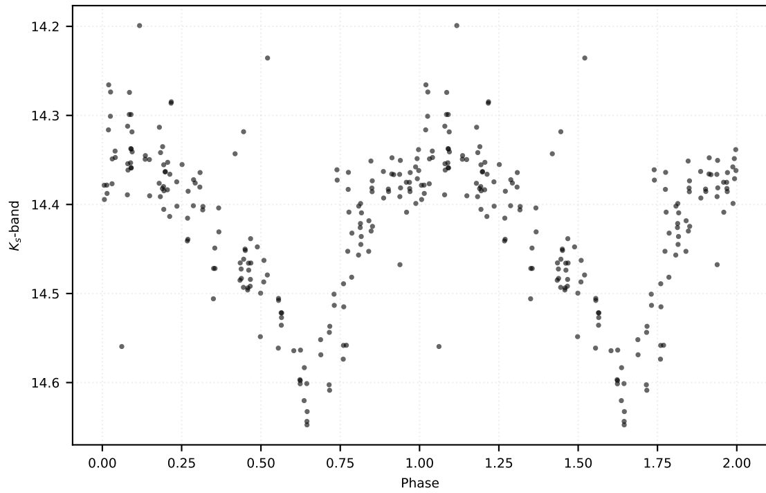
P: 0.57814 d | Class: RP | Subclass: RRab | Field b278
