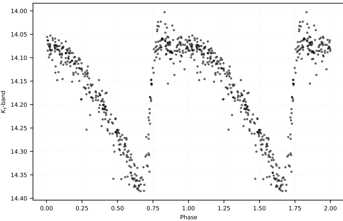
P: 0.44502 d | Class: RP | Subclass: RRab | Field b279
