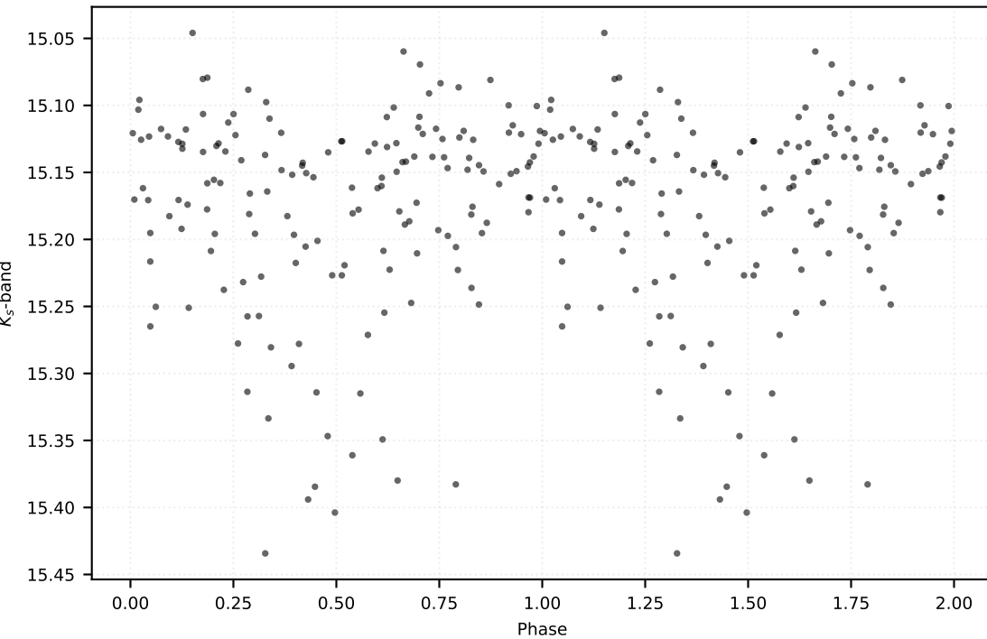
P: 0.13219 d | Class: RP | Subclass: UVAR | Field b278
