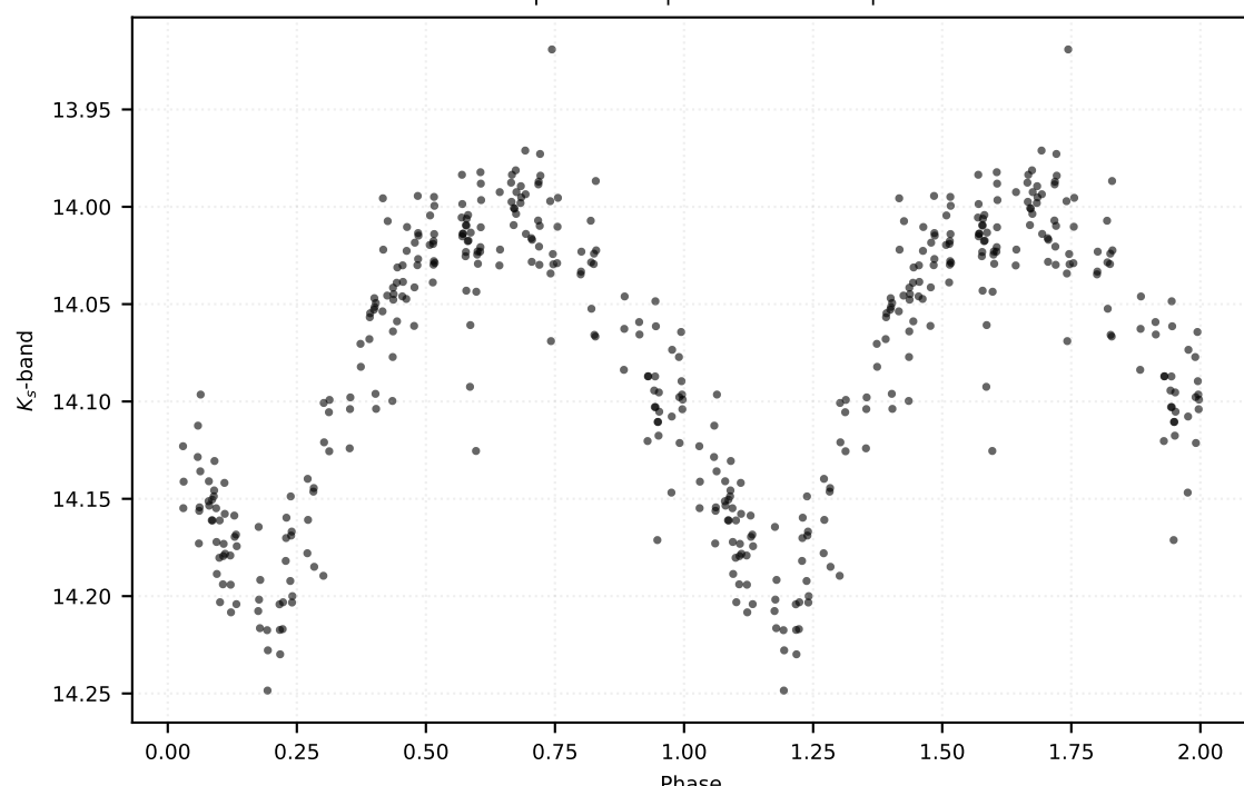
P: 0.64635 d | Class: RP | Subclass: RRab | Field b279
