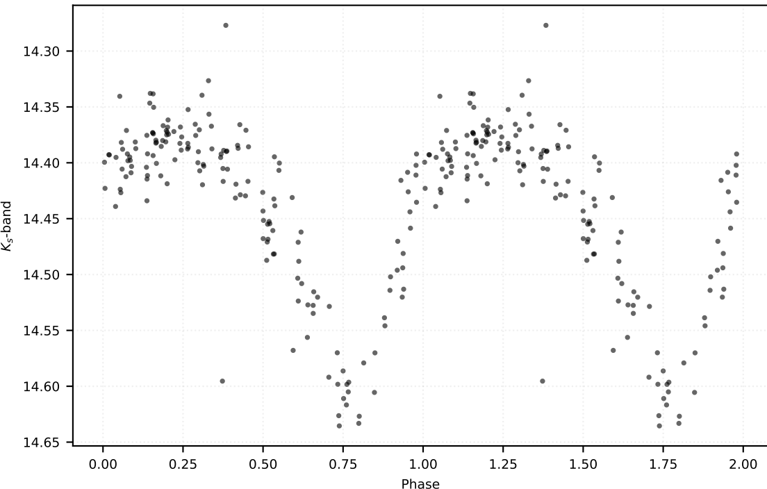
P: 0.63618 d | Class: RP | Subclass: RRab | Field b279
