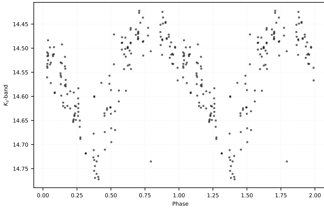
P: 0.57804 d | Class: RP | Subclass: RRc | Field b278
