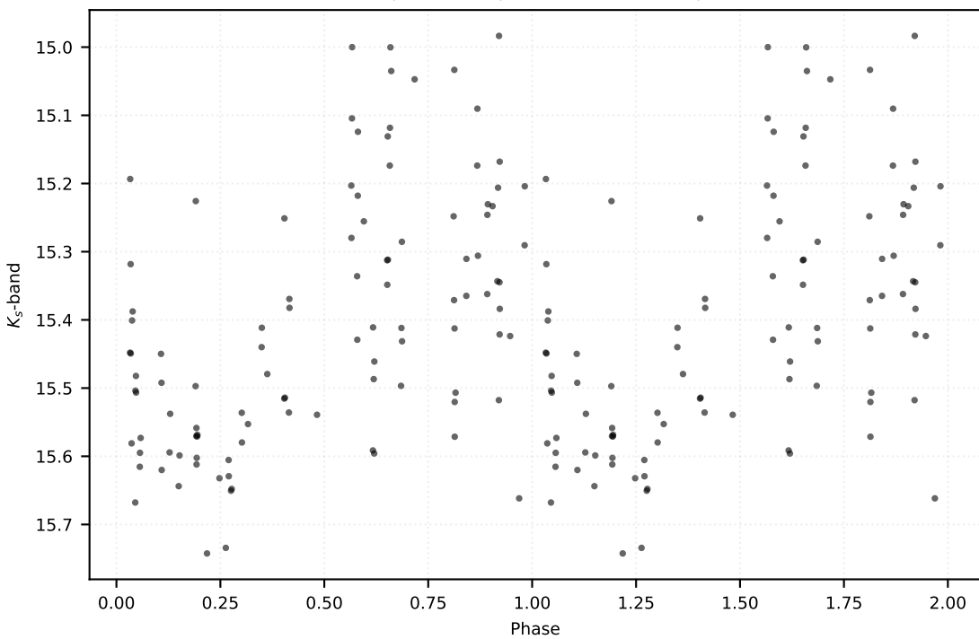
P: 0.25193 d | Class: RP | Subclass: CEP-10T | Field b278
