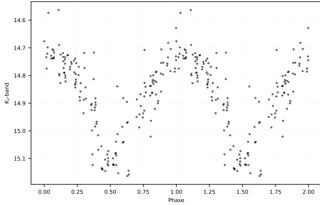
P: 0.23014 d | Class: RP | Subclass: UVAR | Field b279
