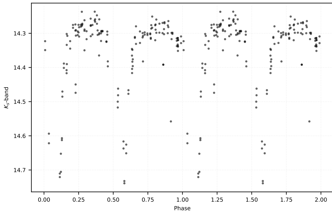
P: 4.49391 d | Class: EB | Subclass: EA | Field b278
