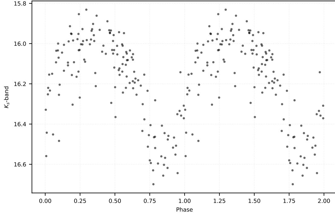
P: 0.17217 d | Class: RP | Subclass: UVAR | Field b278
