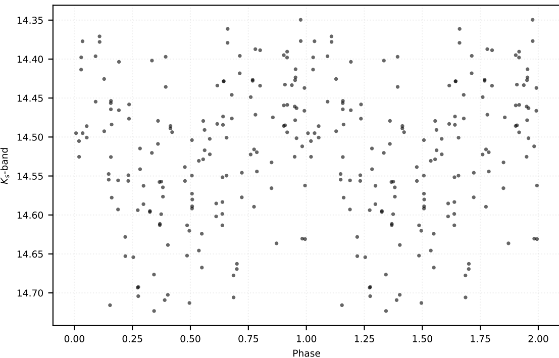
P: 2.85557 d | Class: RP | Subclass: CEP-10T | Field b279
