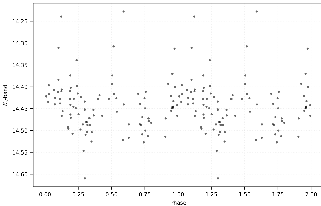
P: 2.04118 d | Class: EB | Subclass: EA | Field b279
