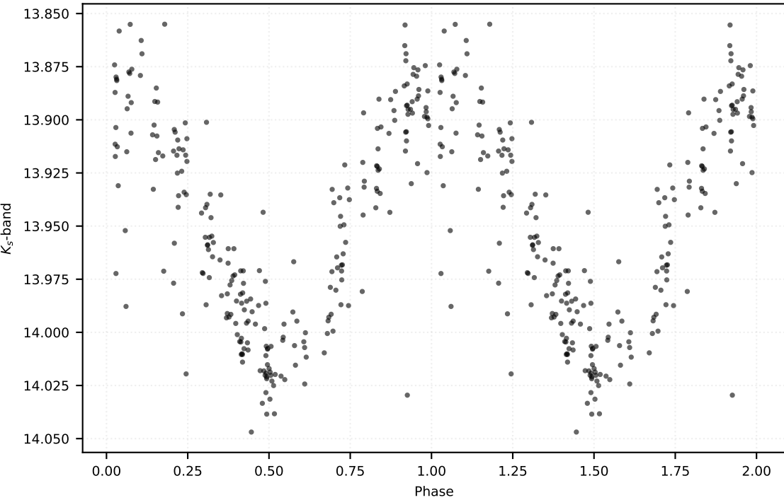
P: 0.20865 d | Class: RP | Subclass: UVAR | Field b278
