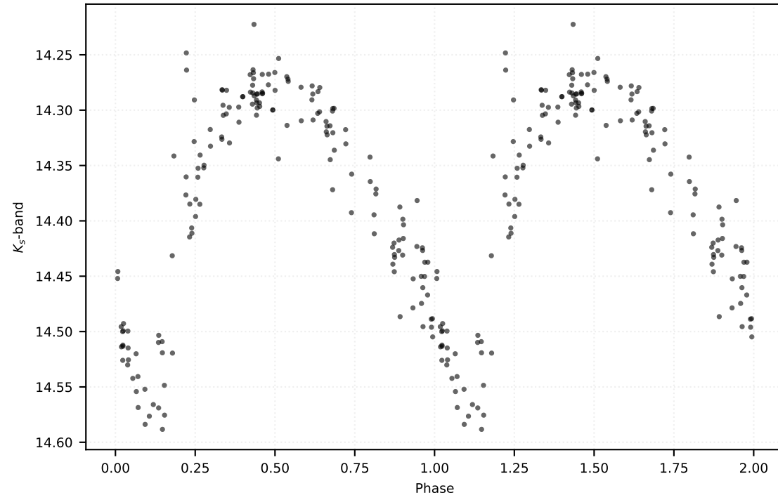
P: 0.61175 d | Class: RP | Subclass: RRab | Field b278
