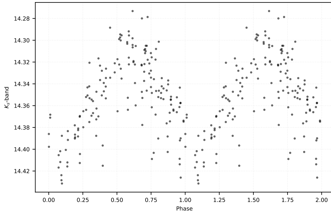
P: 0.43512 d | Class: RP | Subclass: RRab | Field b279
