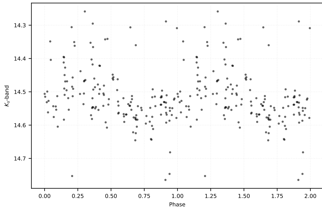
P: 0.12913 d | Class: RP | Subclass: UVAR | Field b278
