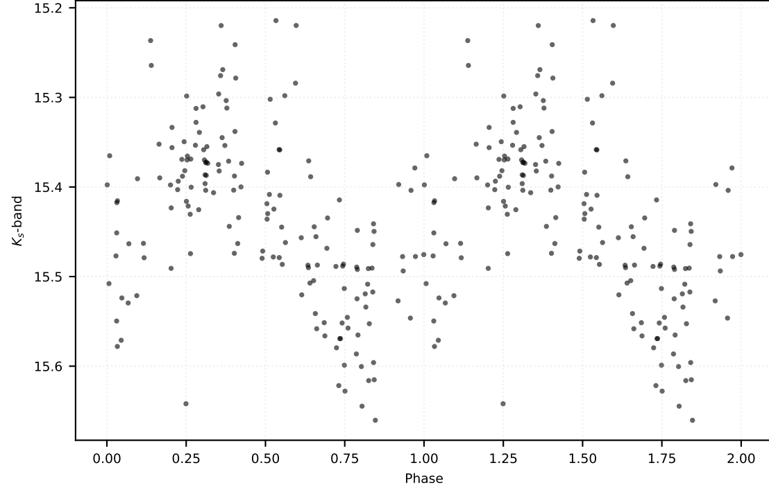
P: 0.35264 d | Class: RP | Subclass: RRab | Field b279
