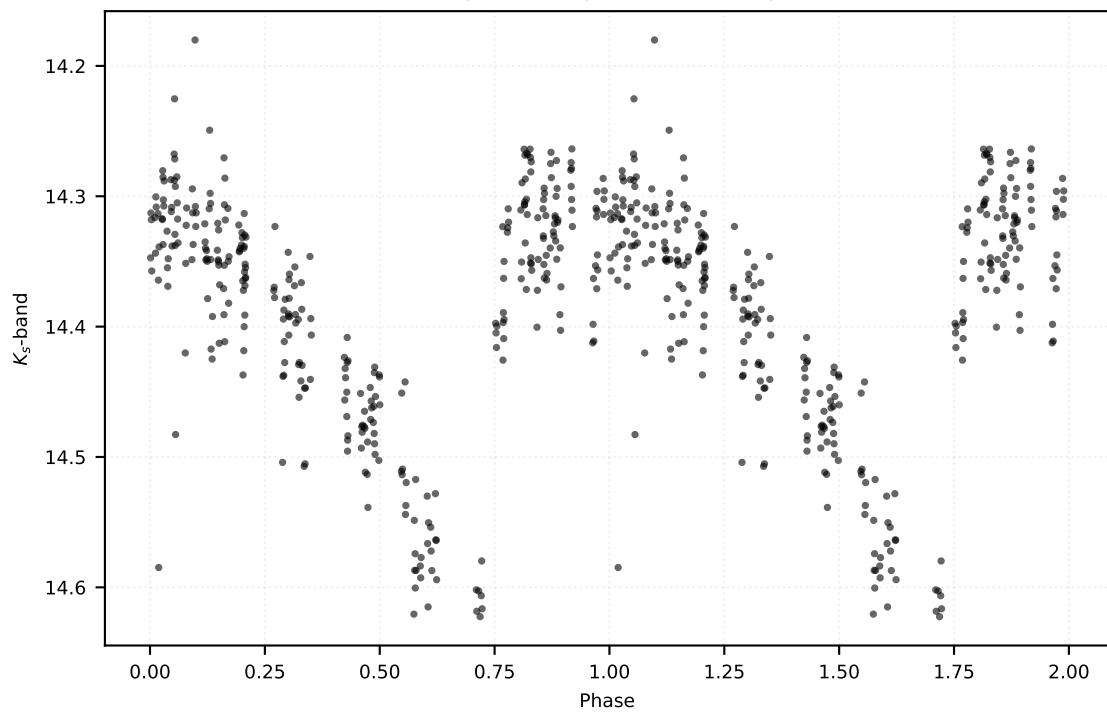
P: 0.60899 d | Class: RP | Subclass: RRab | Field b279
