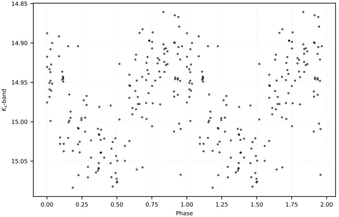
P: 9.64359 d | Class: RP | Subclass: CEP-F | Field b279
