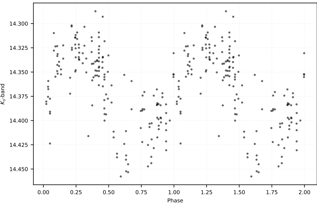
P: 67.48515 d | Class: RP | Subclass: CEP-F | Field b279
