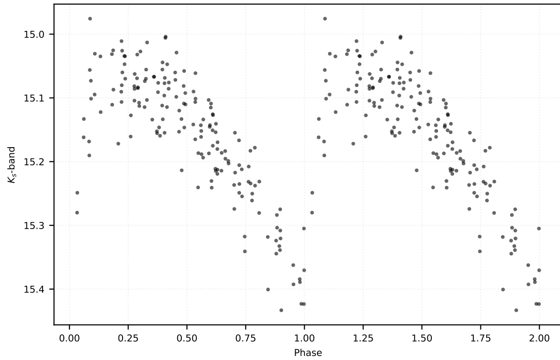
P: 0.42570 d | Class: RP | Subclass: RRab | Field b278
