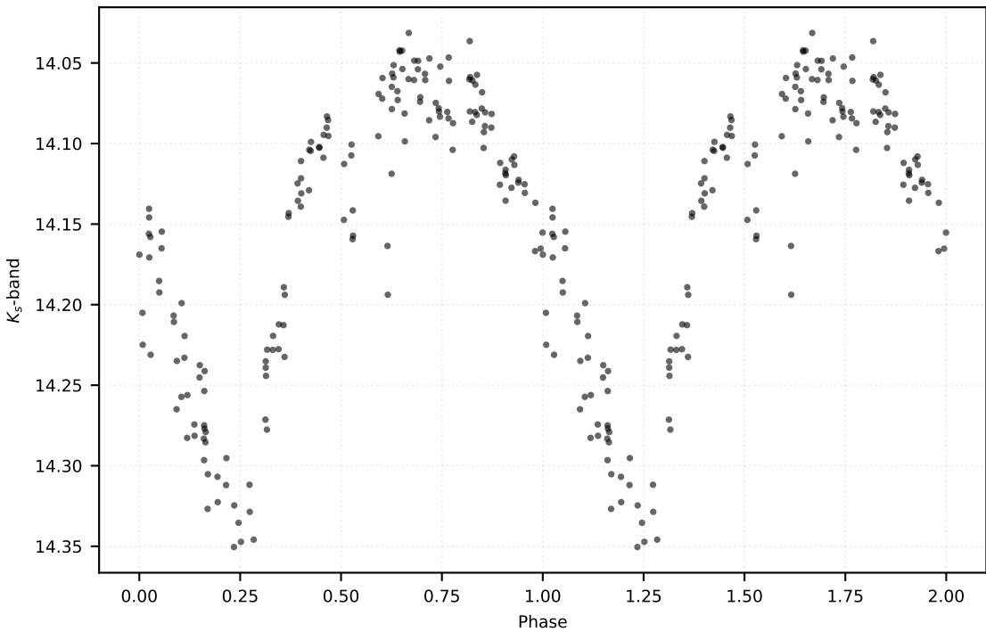
P: 0.37808 d | Class: RP | Subclass: RRab | Field b278
