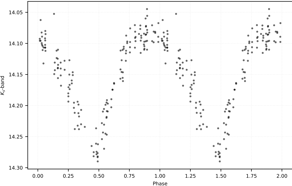
P: 0.51639 d | Class: RP | Subclass: RRab | Field b279
