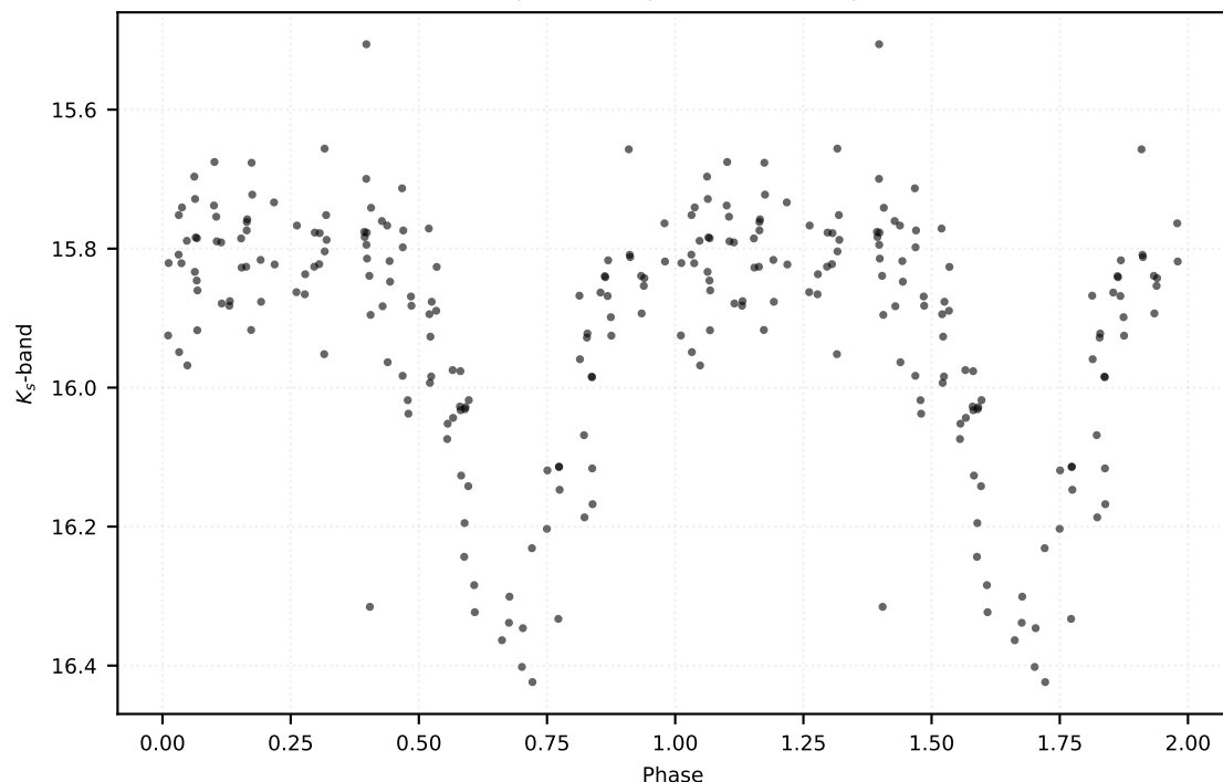
P: 0.40081 d | Class: RP | Subclass: RRab | Field b279
