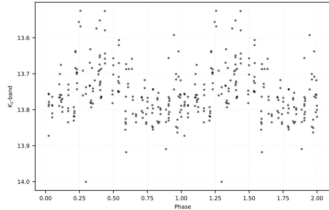
P: 2.99307 d | Class: RP | Subclass: CEP-F | Field b279
