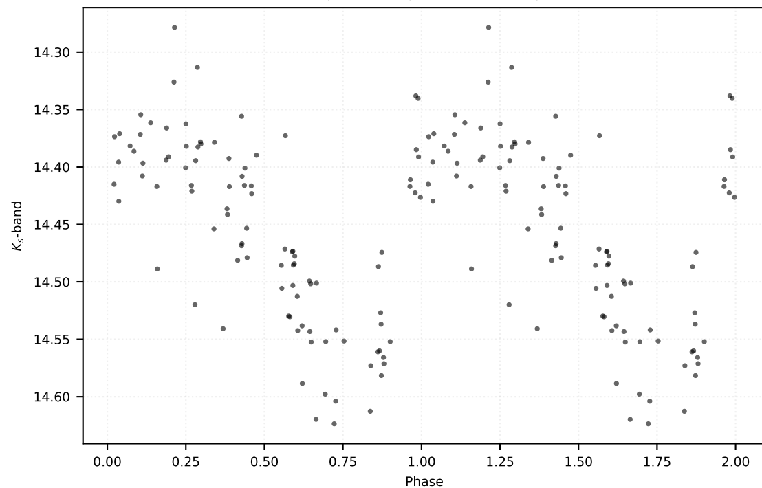
P: 0.55207 d | Class: RP | Subclass: RRab | Field b278
