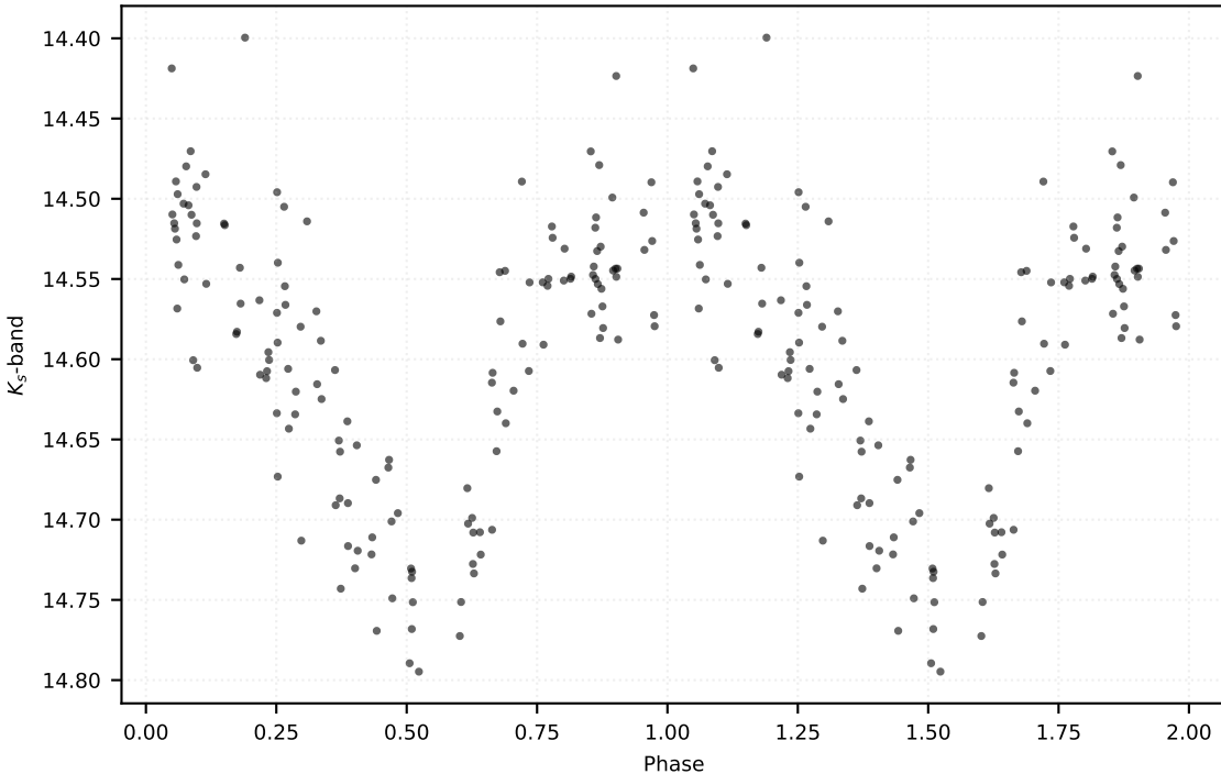
P: 0.87786 d | Class: RP | Subclass: CEP-1OT | Field b278
