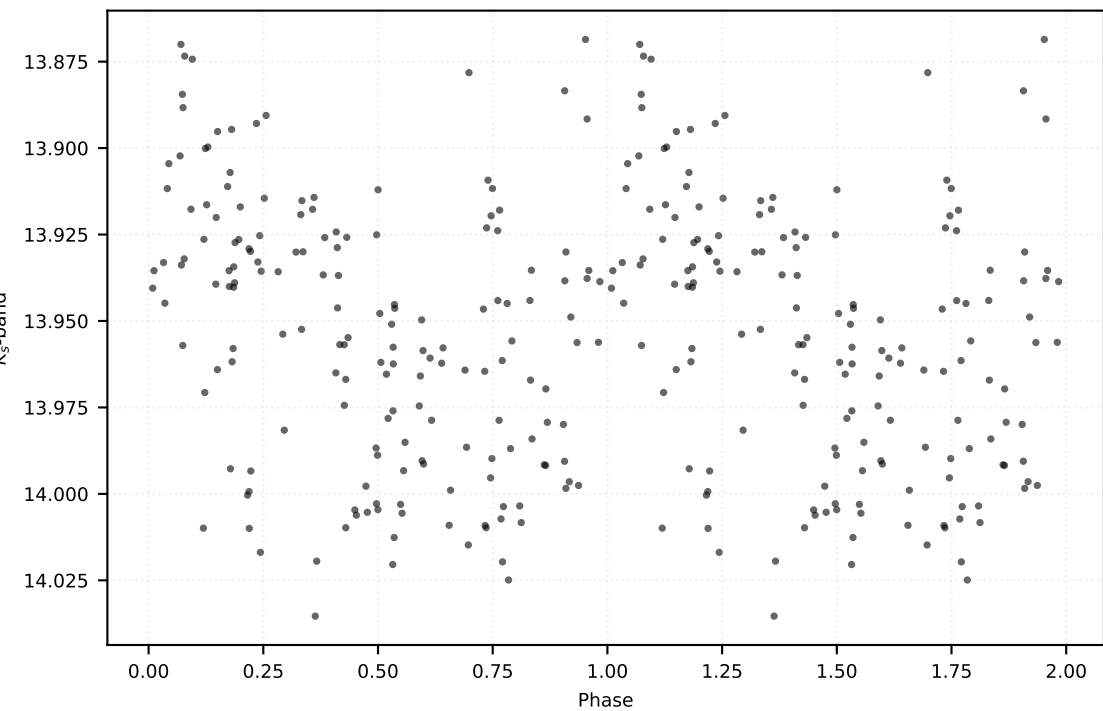
P: 0.16621 d | Class: RP | Subclass: UVAR | Field b278
