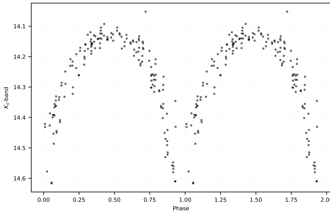
P: 1.13033 d | Class: EB | Subclass: RRc | Field b278
