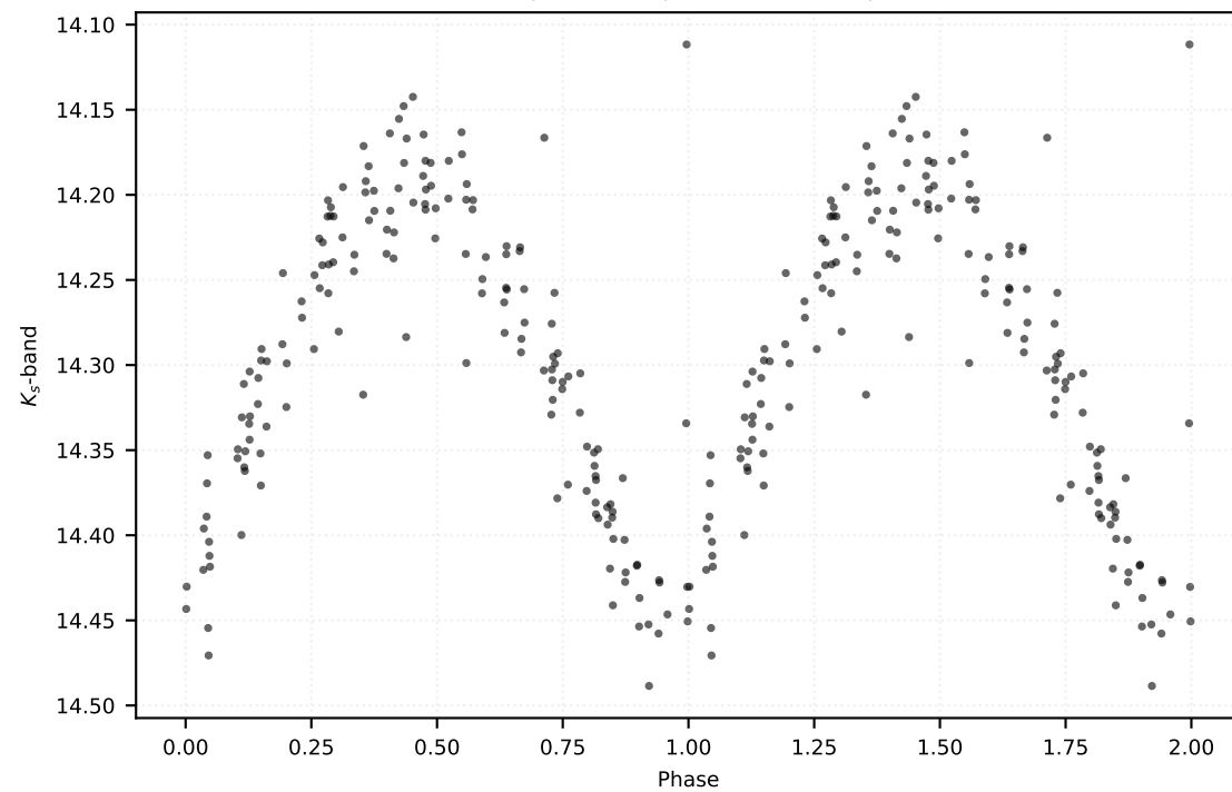
P: 0.50785 d | Class: RP | Subclass: RRab | Field b278
