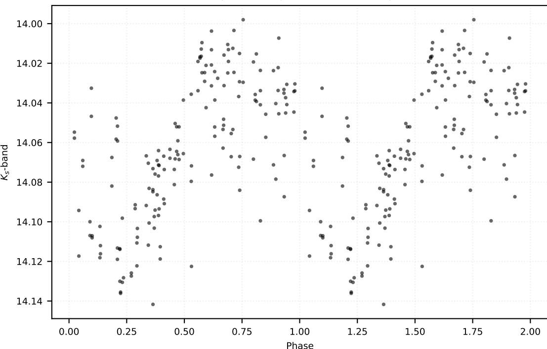
P: 5.95286 d | Class: RP | Subclass: CEP-10T | Field b279
