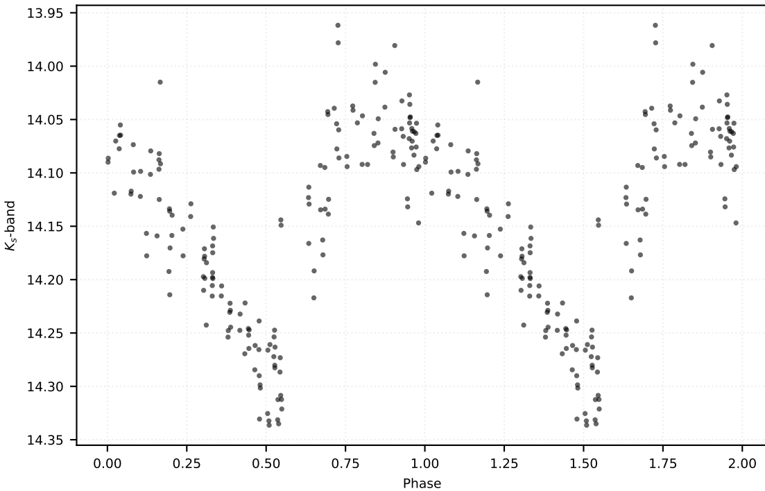
P: 0.56634 d | Class: RP | Subclass: RRab | Field b278
