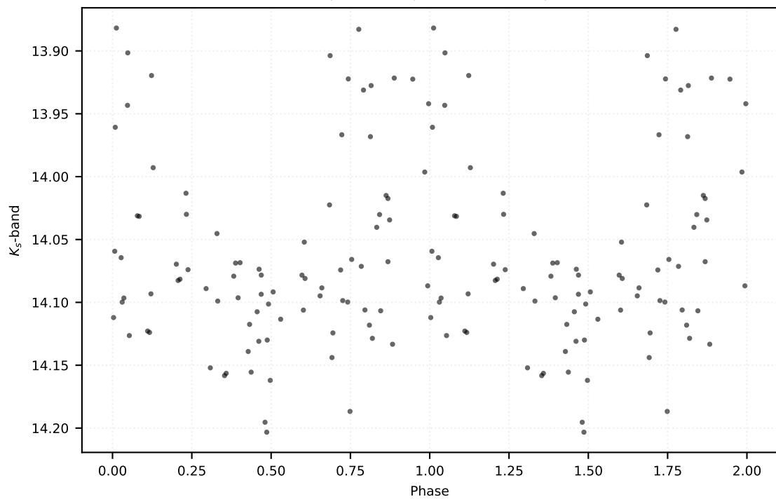
P: 0.10404 d | Class: RP | Subclass: UVAR | Field b278
