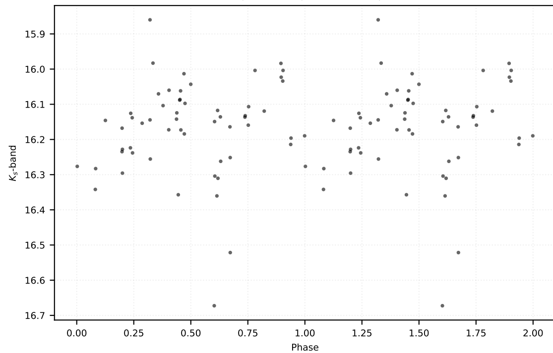
P: 0.61508 d | Class: EB | Subclass: EA | Field b278
