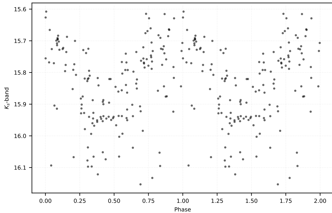
P: 0.14726 d | Class: RP | Subclass: UVAR | Field b279
