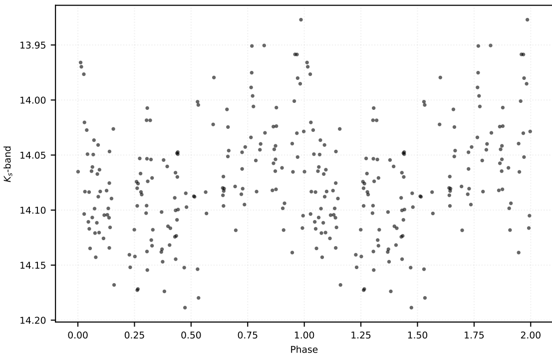
P: 0.13535 d | Class: RP | Subclass: UVAR | Field b279
