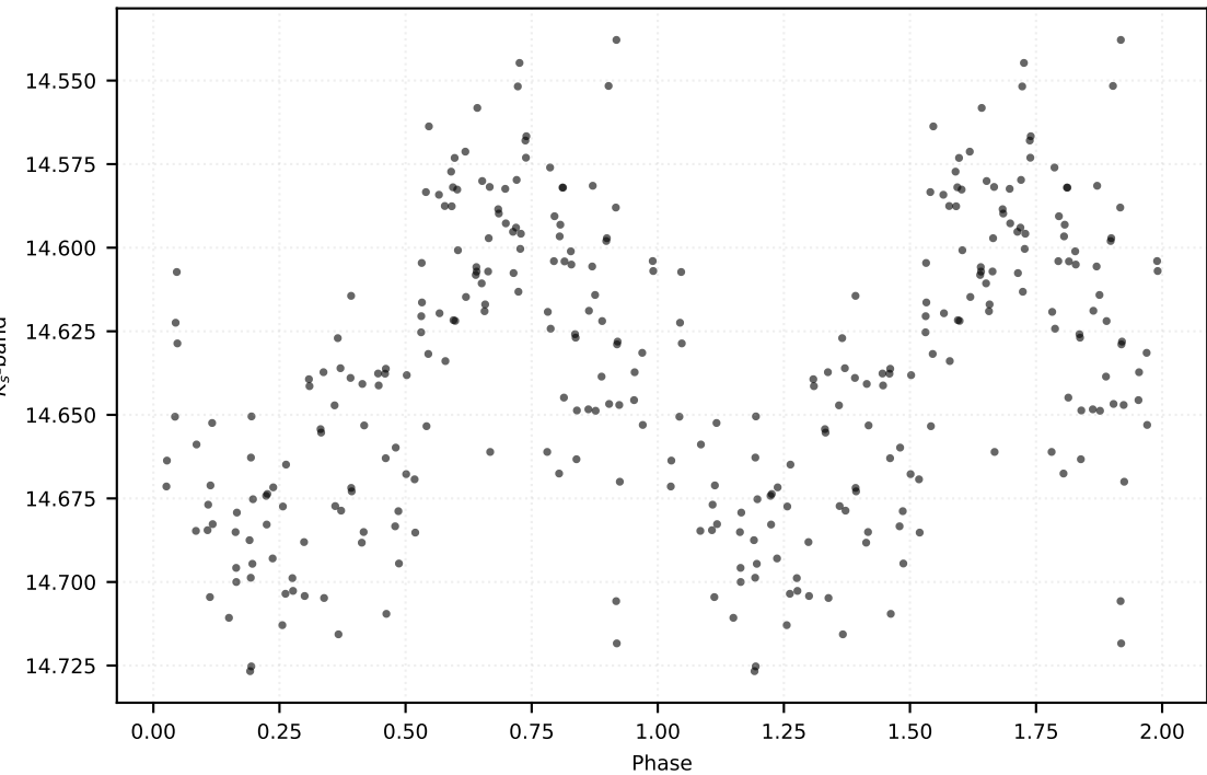
P: 0.33241 d | Class: RP | Subclass: RRab | Field b278
