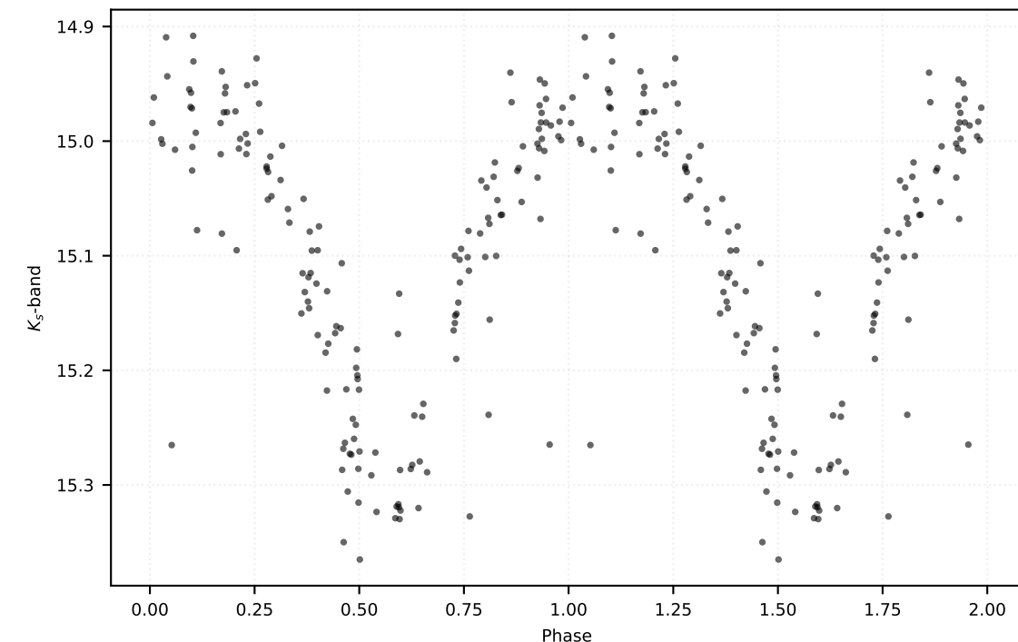
P: 0.19601 d | Class: RP | Subclass: UVAR | Field b279
