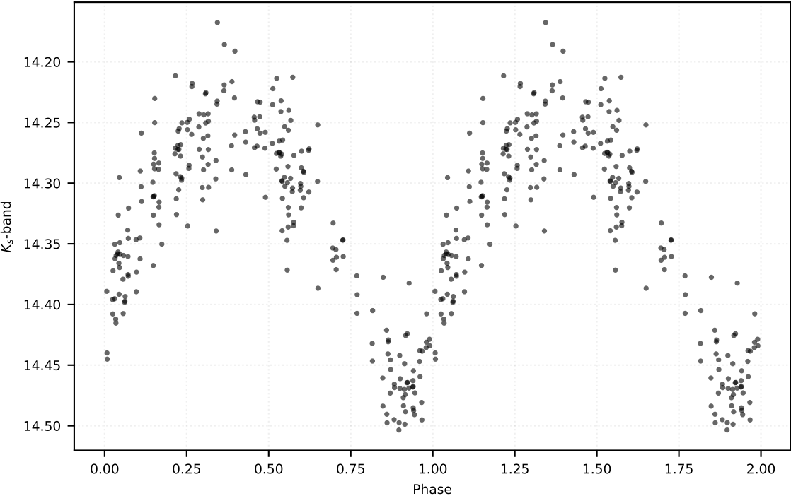
P: 0.59639 d | Class: RP | Subclass: CEP-10T | Field b278
