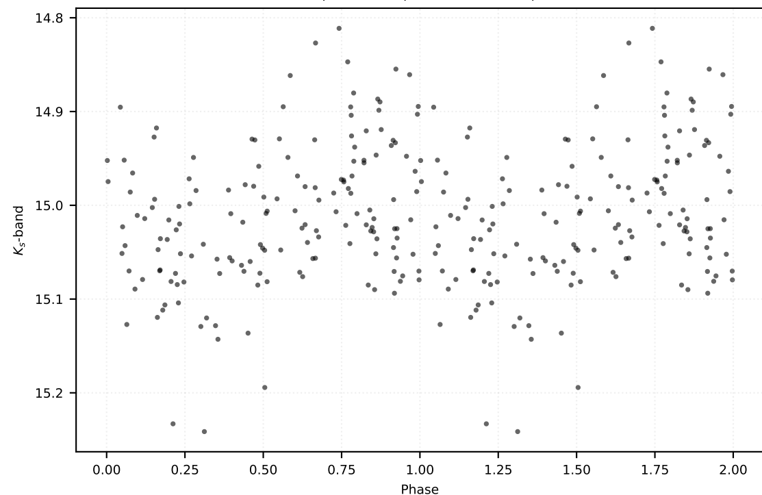
P: 0.16706 d | Class: RP | Subclass: UVAR | Field b278
