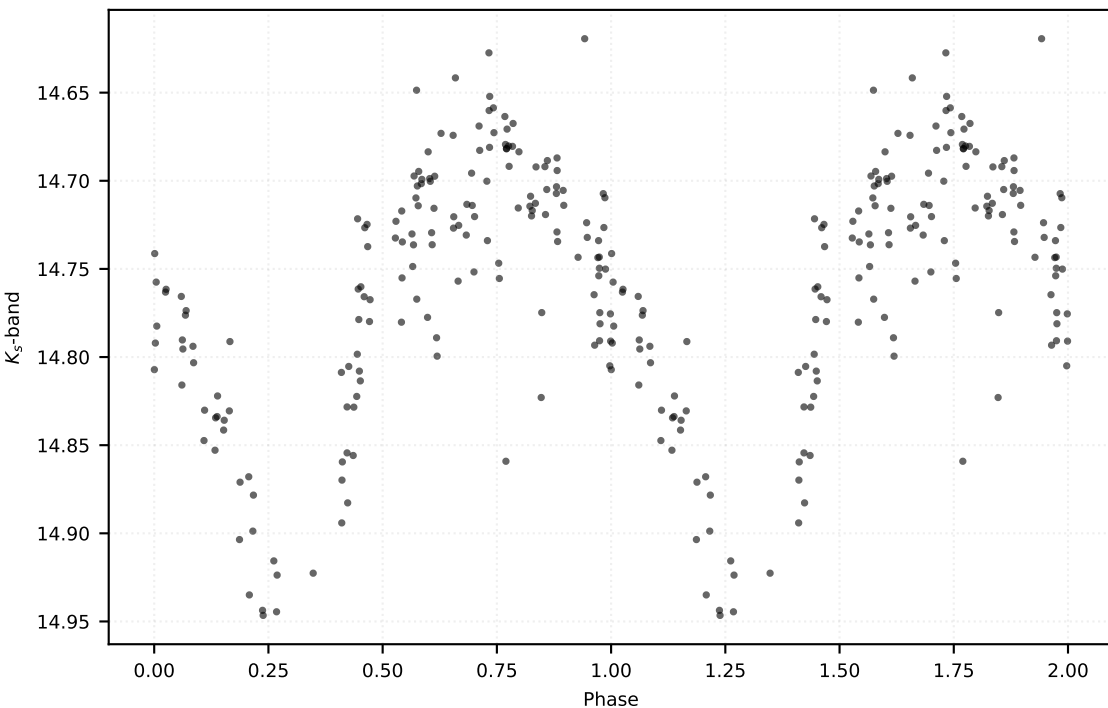
P: 0.49179 d | Class: RP | Subclass: RRab | Field b278
