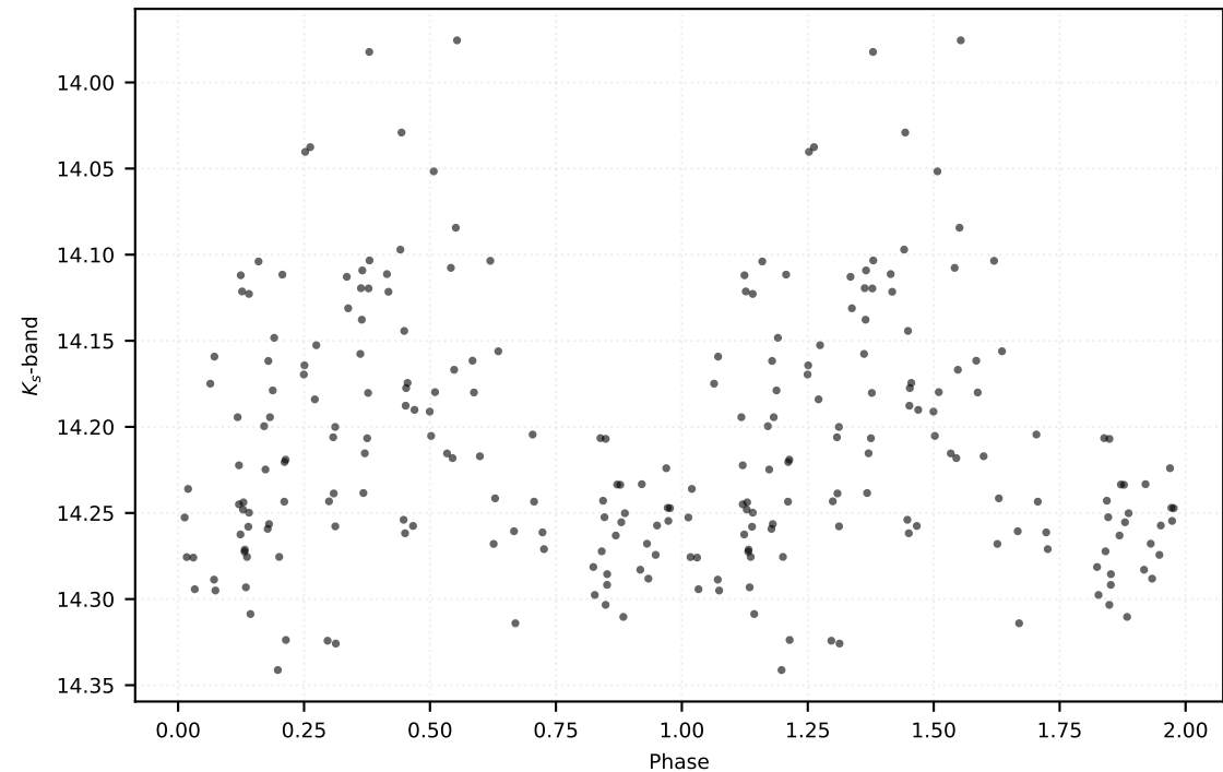
P: 0.14355 d | Class: RP | Subclass: UVAR | Field b279
