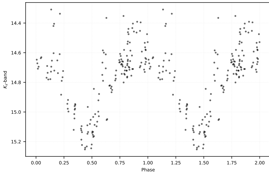
P: 0.84358 d | Class: EB | Subclass: UVAR | Field b278
