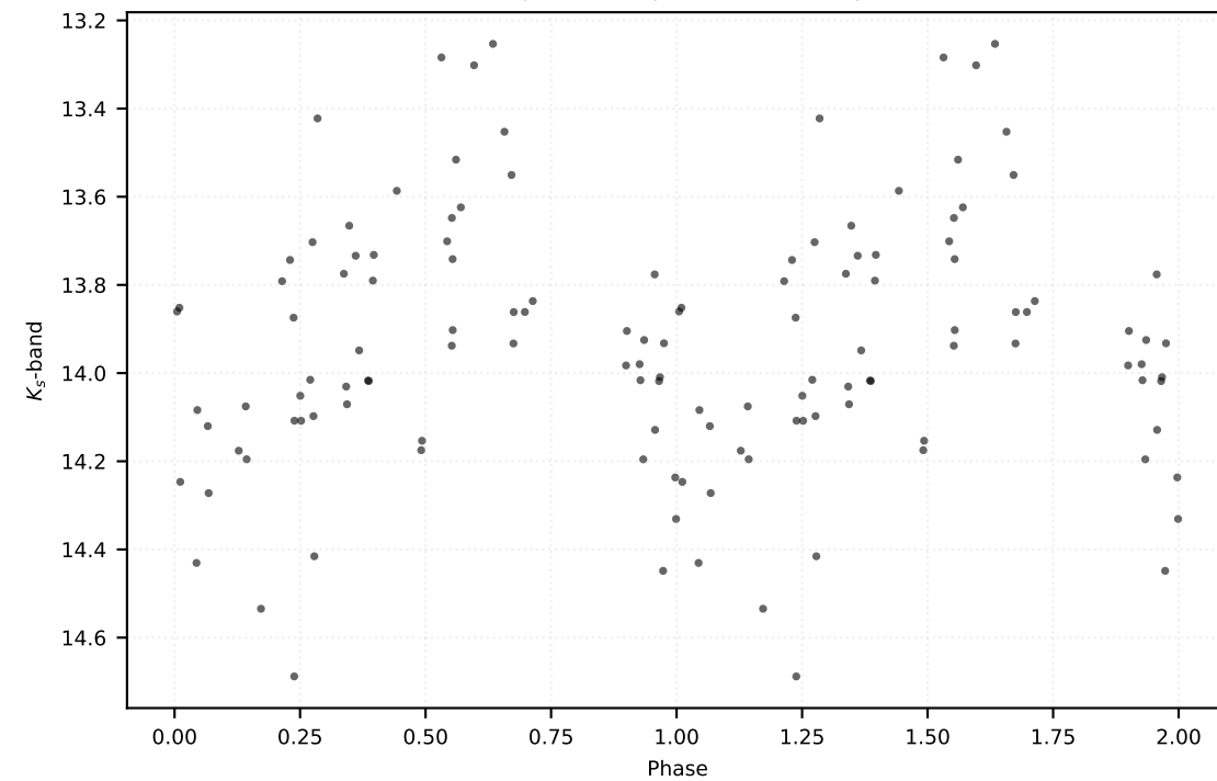
P: 0.58143 d | Class: RP | Subclass: RRab | Field b278
