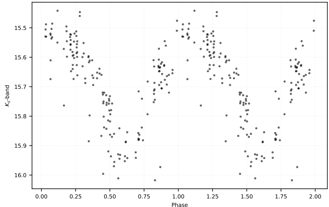
P: 0.38514 d | Class: RP | Subclass: RRab | Field b279
