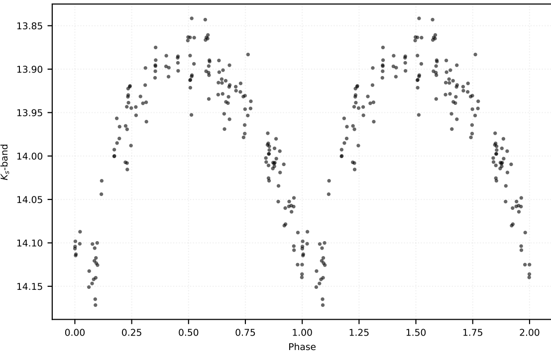
P: 0.67195 d | Class: RP | Subclass: RRab | Field b279
