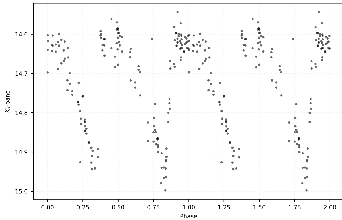
P: 0.18802 d | Class: RP | Subclass: UVAR | Field b278
