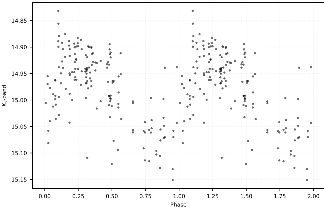
P: 0.22655 d | Class: RP | Subclass: UVAR | Field b279
