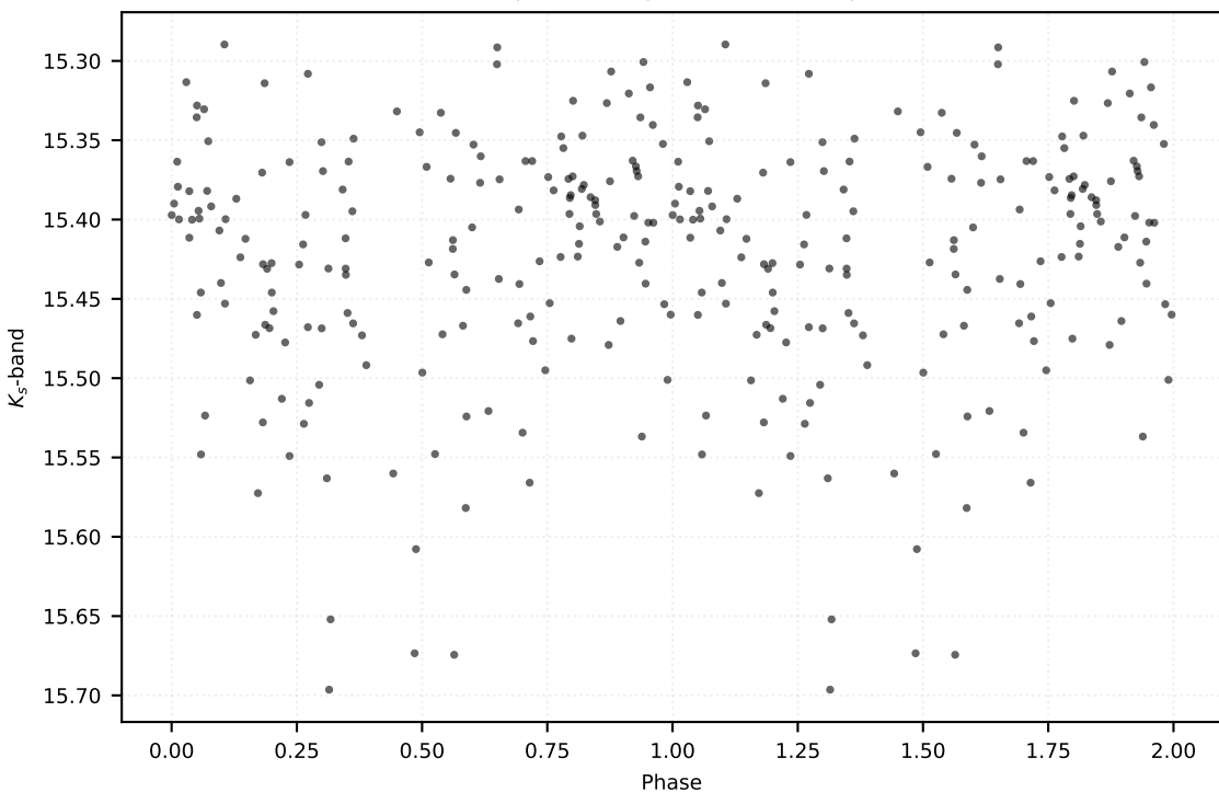
P: 0.11098 d | Class: RP | Subclass: UVAR | Field b278
