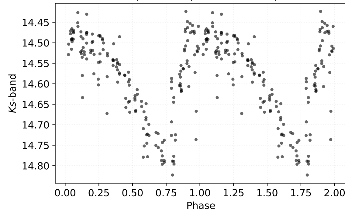
P: 0.48360 d | Class: RP | Subclass: RRab | Field b279
