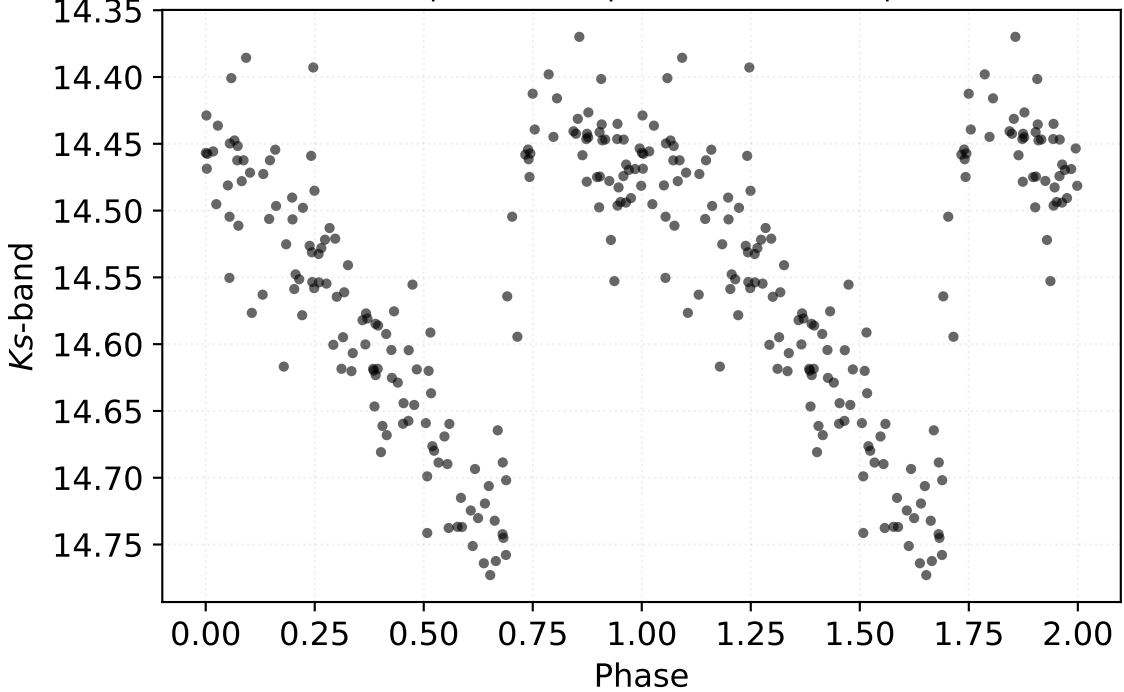
P: 0.47464 d | Class: RP | Subclass: RRab | Field b278
