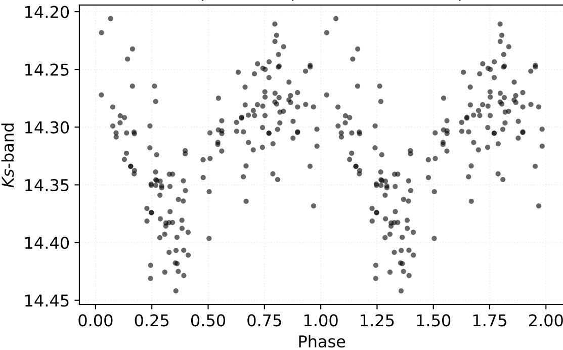
P: 1.70878 d | Class: RP | Subclass: CEP-1OT | Field b278
