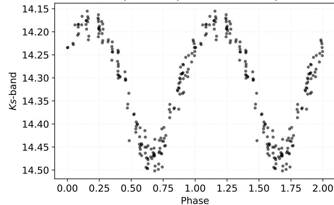
P: 0.39580 d | Class: RP | Subclass: CEP-1OT | Field b278
