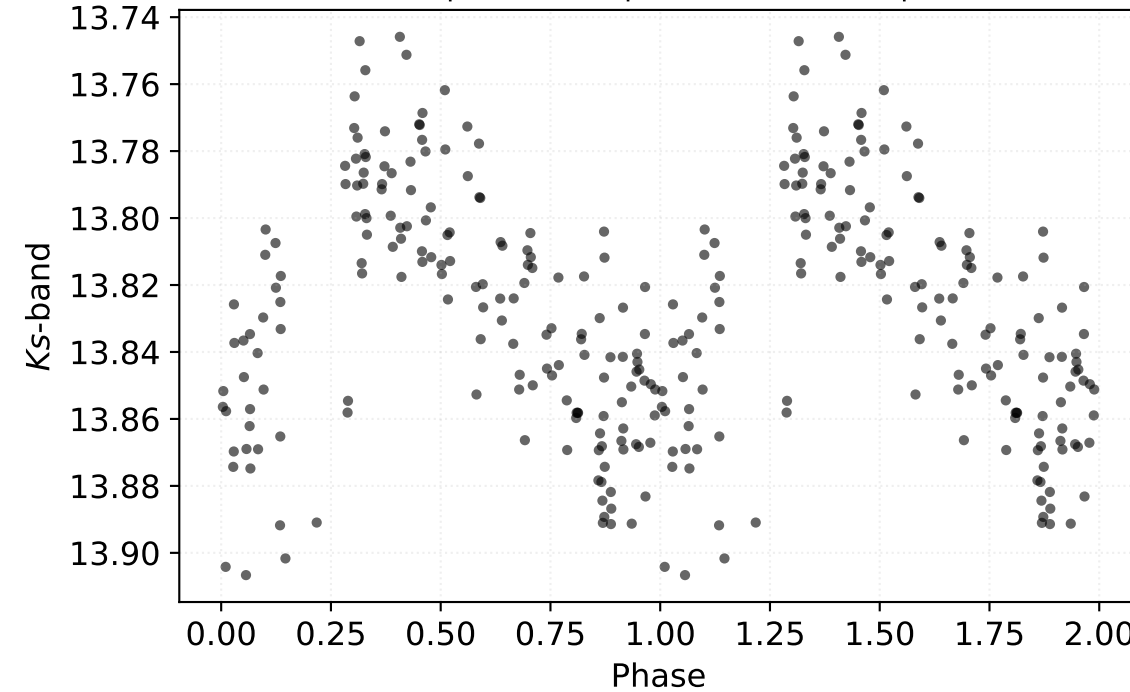
P: 0.35469 d | Class: RP | Subclass: RRab | Field b279
