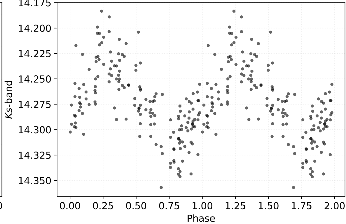
P: 2.42538 d | Class: RP | Subclass: CEP-F | Field b278
