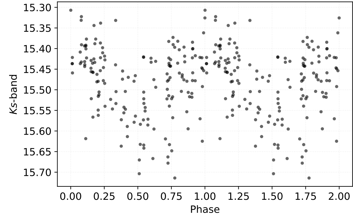
P: 0.58781 d | Class: RP | Subclass: CEP-1OT | Field b279
