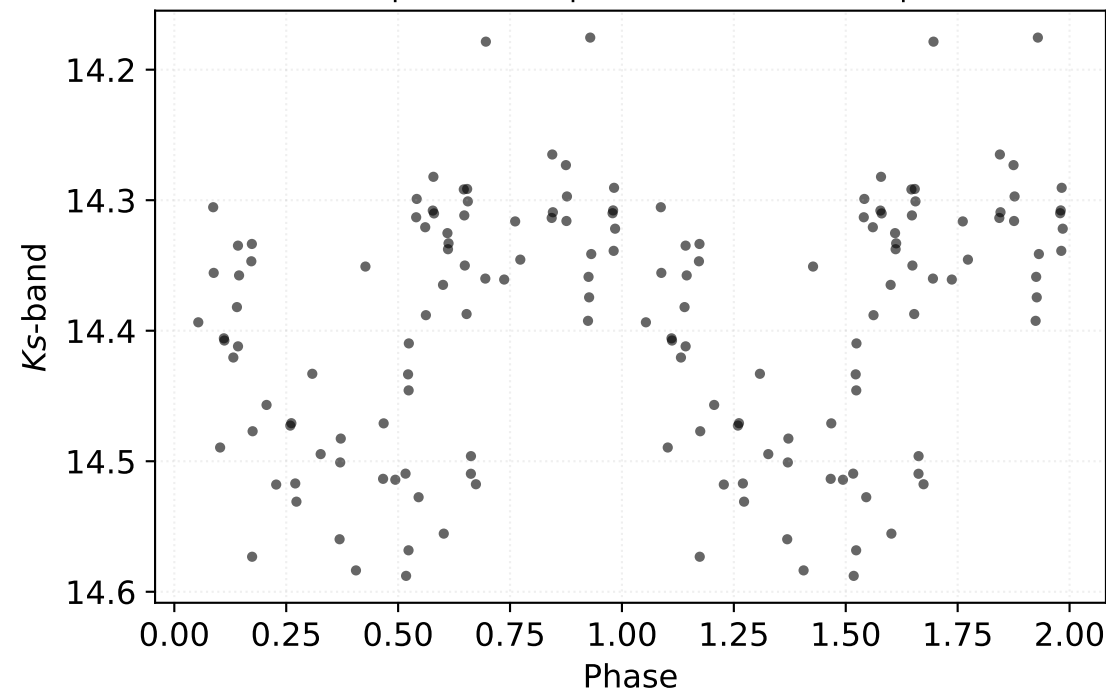
P: 1.10655 d | Class: RP | Subclass: CEP-1OT | Field b278
