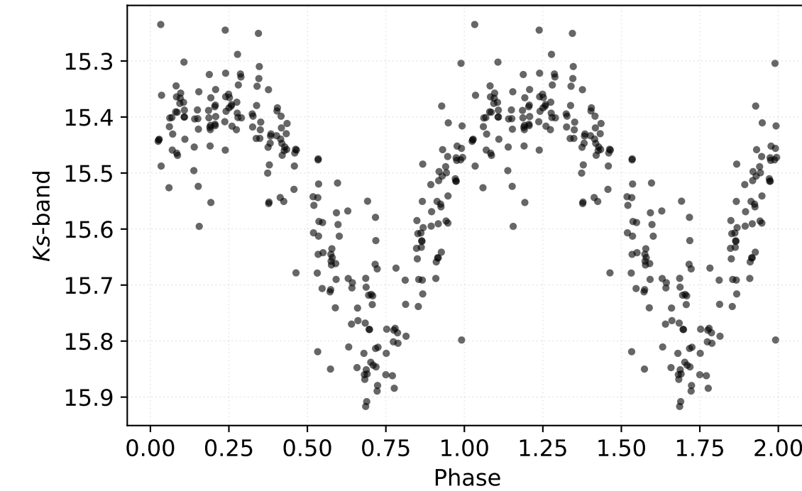
P: 0.30428 d | Class: RP | Subclass: RRab | Field b279
