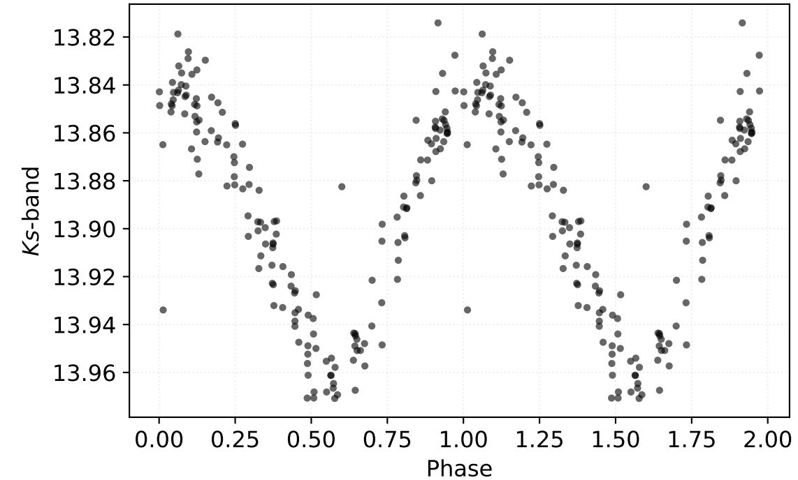
P: 0.62430 d | Class: RP | Subclass: RRab | Field b278
