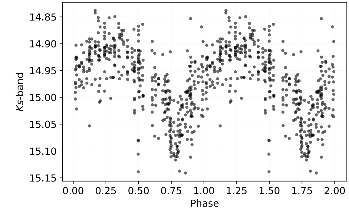
P: 1.98484 d | Class: RP | Subclass: CEP-1OT | Field b279
