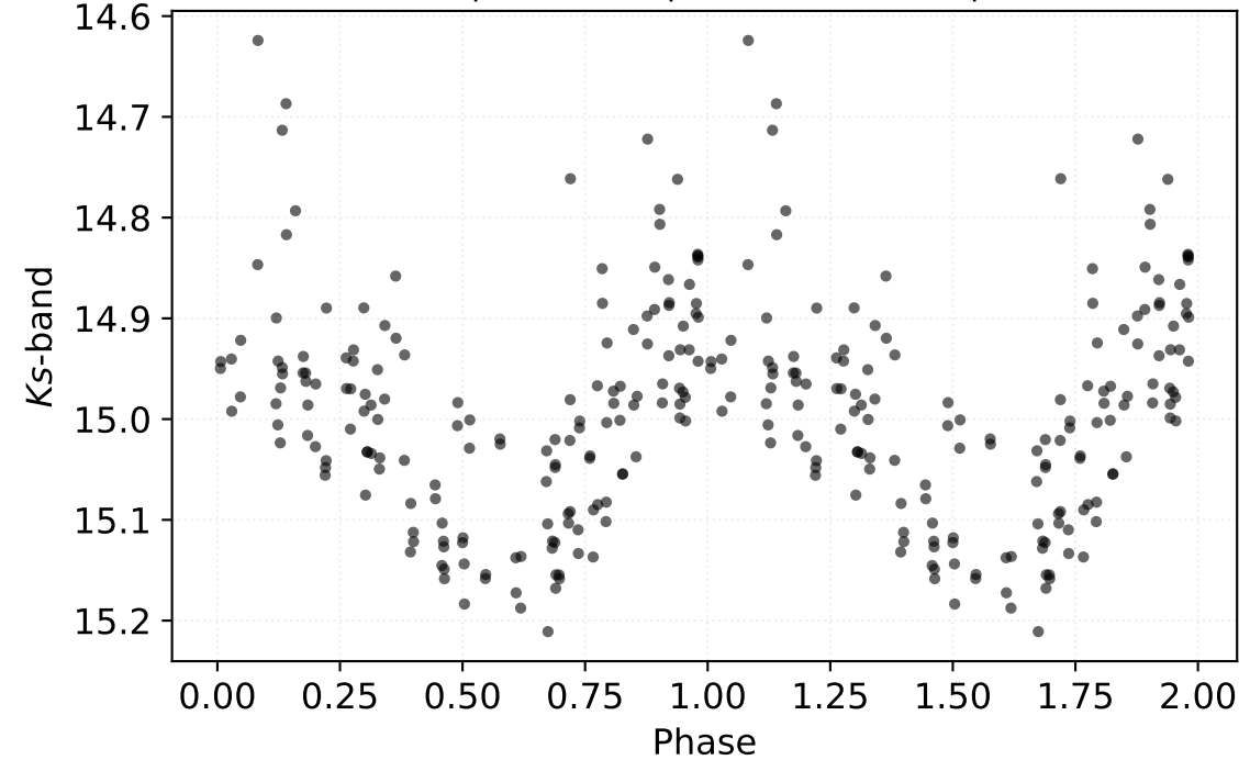
P: 0.60365 d | Class: RP | Subclass: RRab | Field b279
