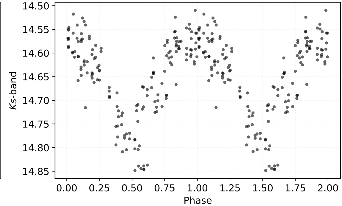
P: 3.89243 d | Class: RP | Subclass: CEP-1OT | Field b279
