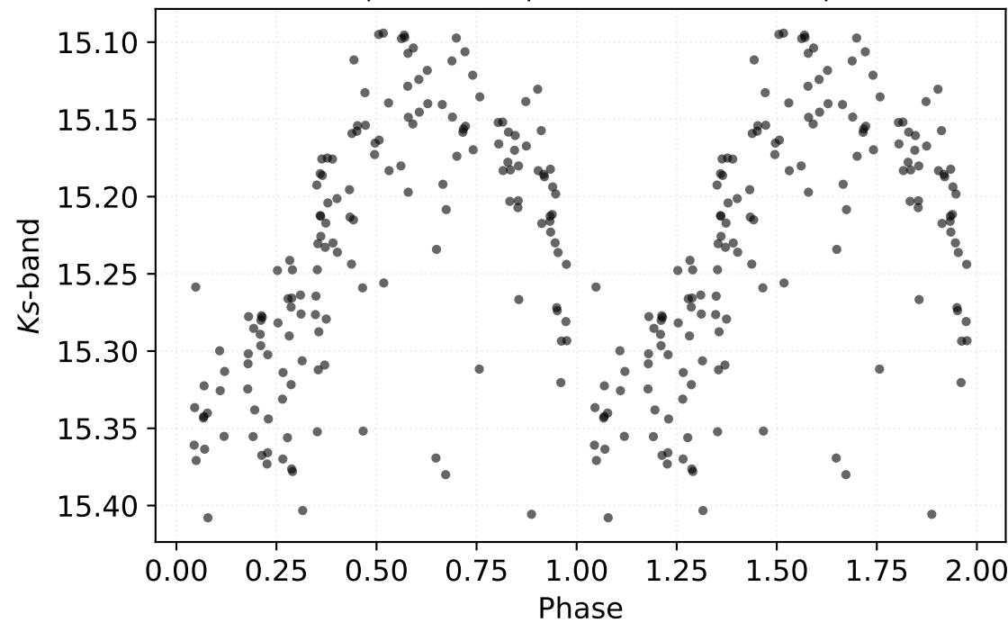
P: 4.17493 d | Class: RP | Subclass: CEP-1OT | Field b279
