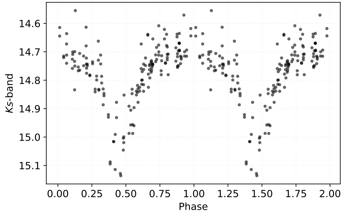
P: 0.45986 d | Class: RP | Subclass: CEP-1OT | Field b278
