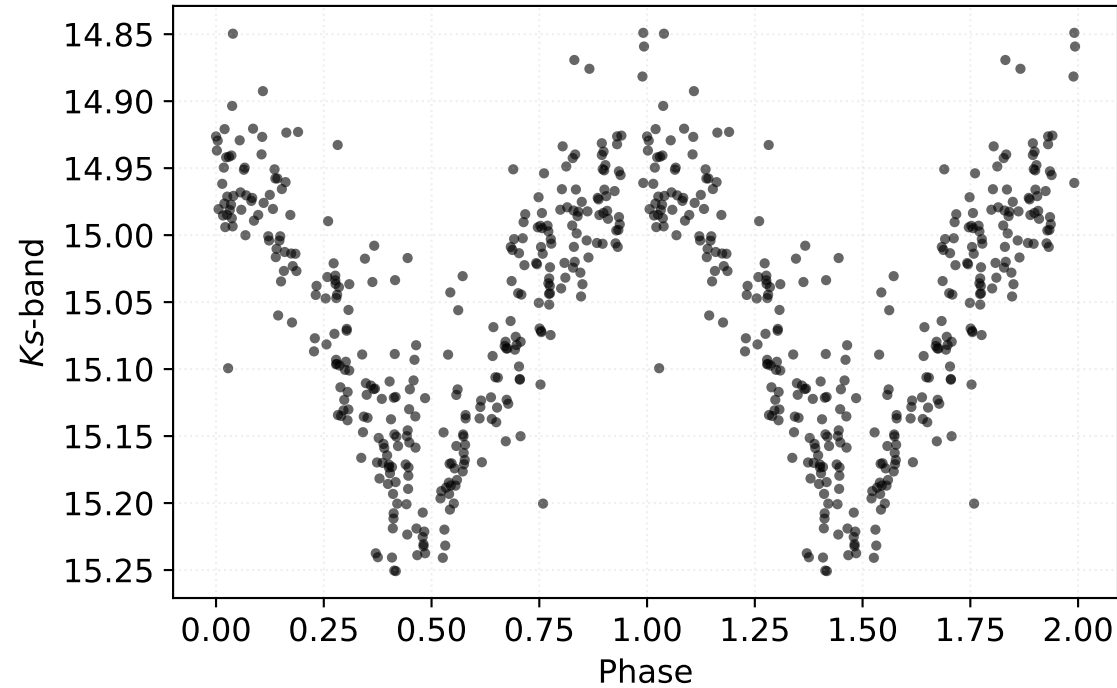
P: 0.22149 d | Class: RP | Subclass: UVAR | Field b278
