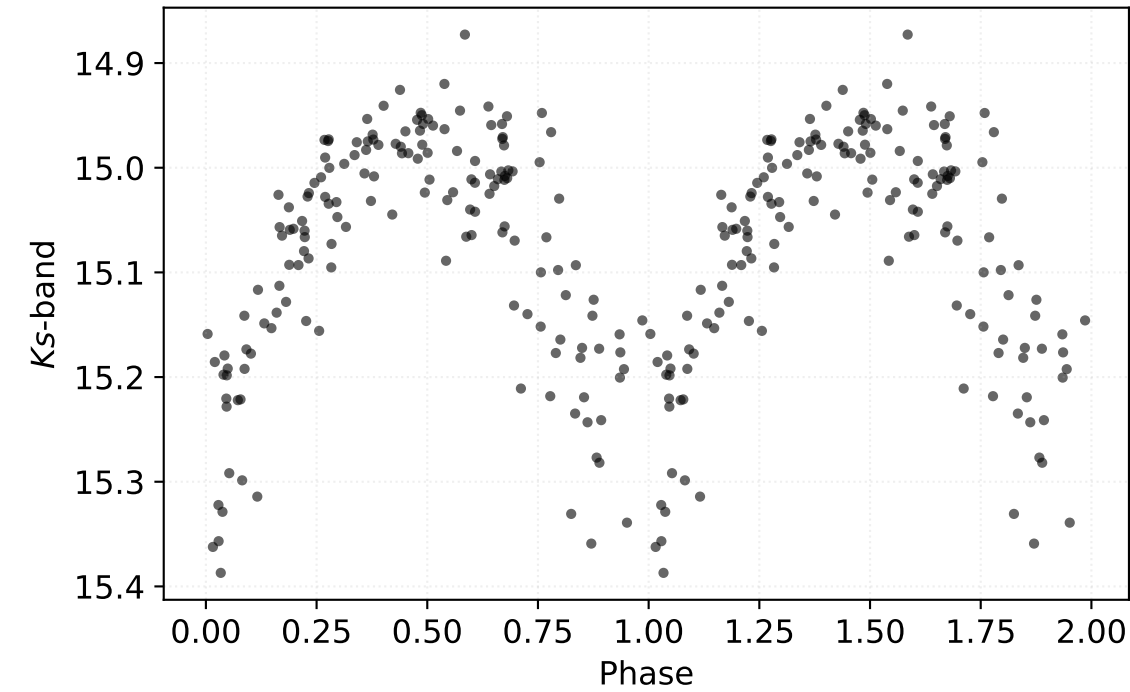
P: 0.18149 d | Class: RP | Subclass: UVAR | Field b278
