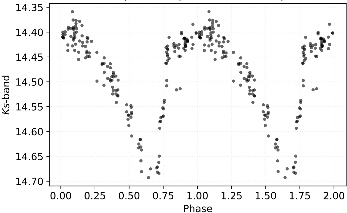
P: 0.34971 d | Class: RP | Subclass: CEP-1OT | Field b278
