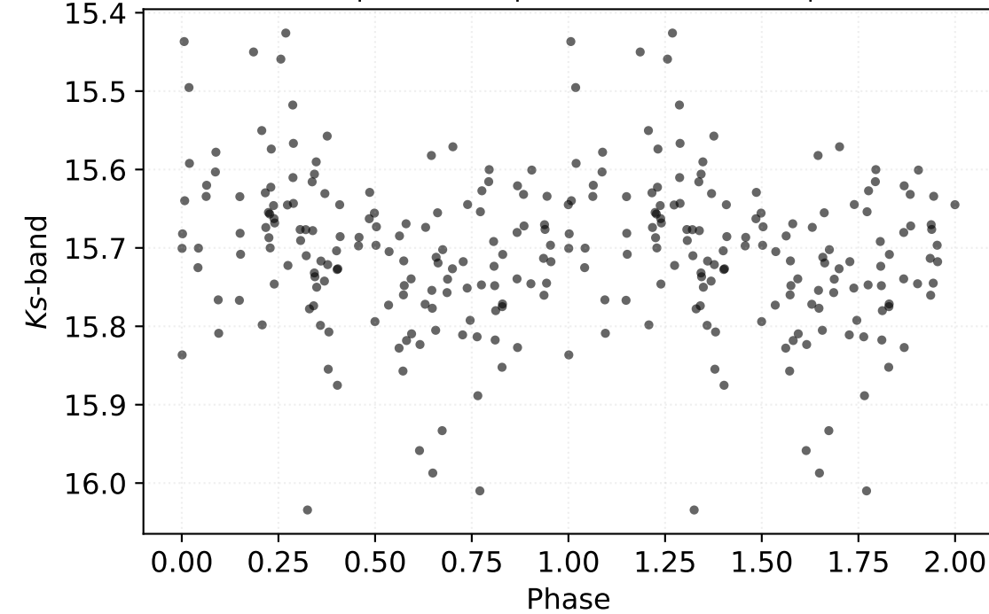
P: 0.29975 d | Class: RP | Subclass: CEP-1OT | Field b278
