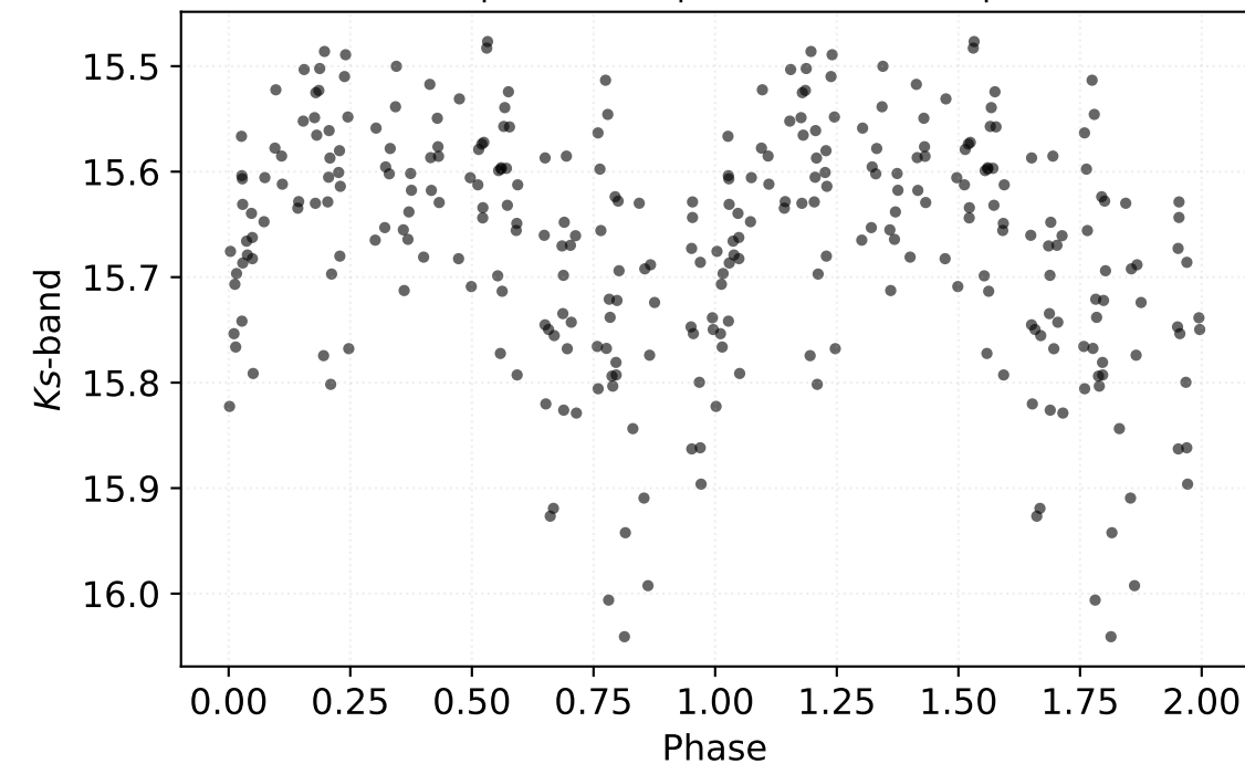
P: 0.31931 d | Class: RP | Subclass: RRab | Field b279
