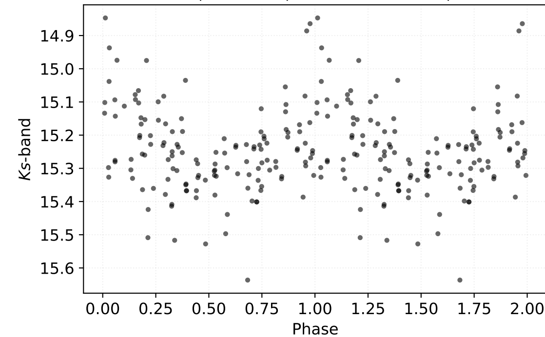
P: 0.56557 d | Class: RP | Subclass: CEP-1OT | Field b278
