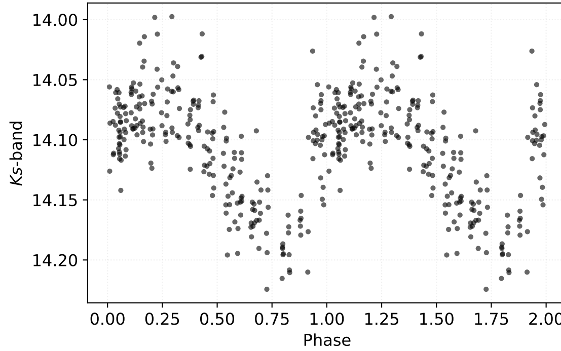
P: 1.02949 d | Class: RP | Subclass: CEP-1OT | Field b279
