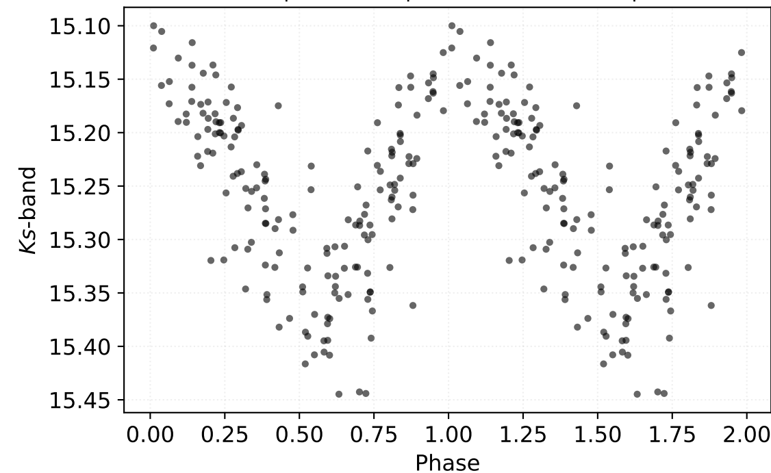
P: 0.33542 d | Class: RP | Subclass: CEP-1OT | Field b278
