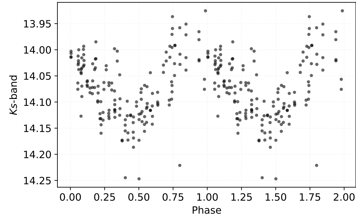
P: 1.05431 d | Class: RP | Subclass: CEP-F | Field b279
