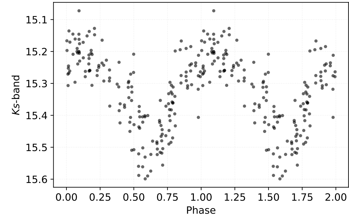
P: 0.42483 d | Class: RP | Subclass: CEP-1OT | Field b278
