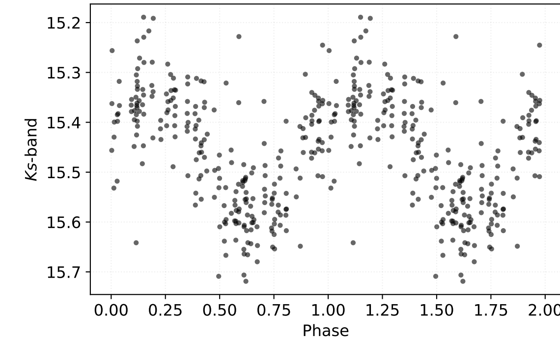
P: 0.30121 d | Class: EB | Subclass: RRc | Field b278
