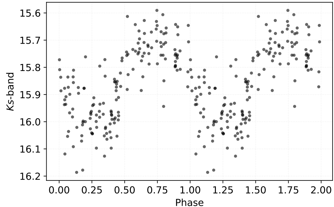
P: 0.41661 d | Class: RP | Subclass: CEP-1OT | Field b279
