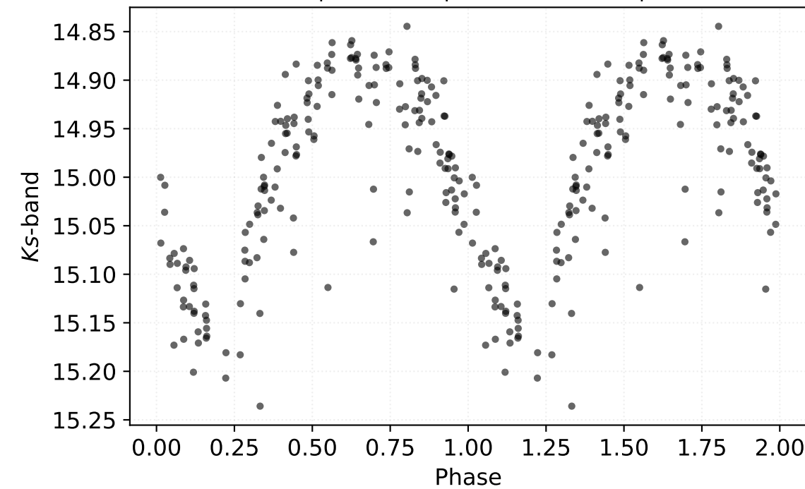
P: 0.43231 d | Class: RP | Subclass: RRab | Field b278
