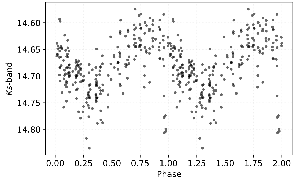
P: 6.93297 d | Class: RP | Subclass: CEP-1OT | Field b279
