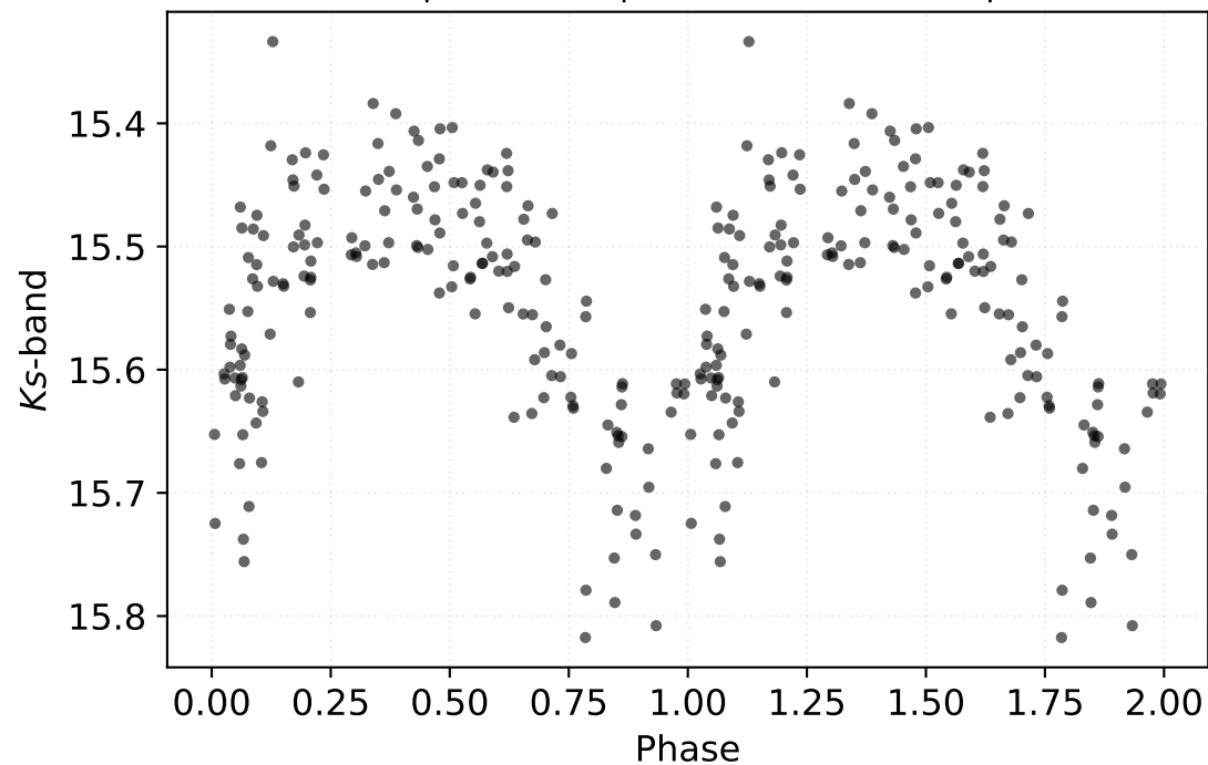
P: 0.66869 d | Class: RP | Subclass: CEP-1OT | Field b279
