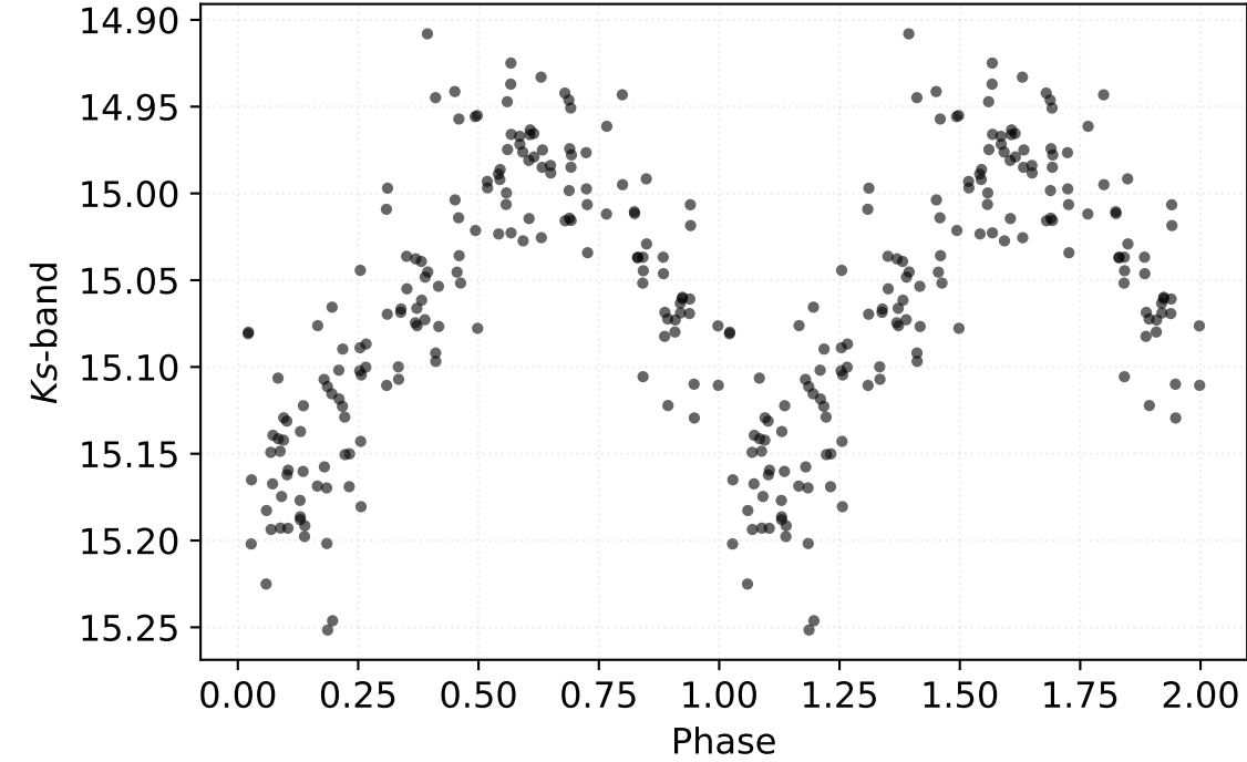
P: 0.68210 d | Class: RP | Subclass: CEP-1OT | Field b278
