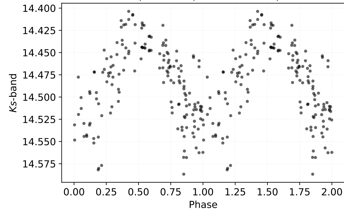
P: 0.31366 d | Class: RP | Subclass: RRab | Field b278
