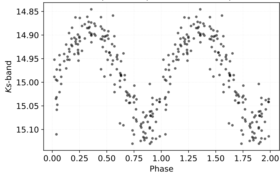
P: 0.35252 d | Class: RP | Subclass: CEP-1OT | Field b278
