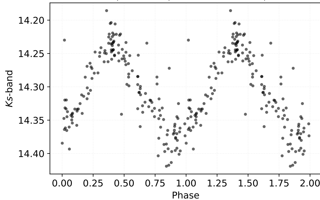
P: 0.29877 d | Class: RP | Subclass: CEP-1OT | Field b278
