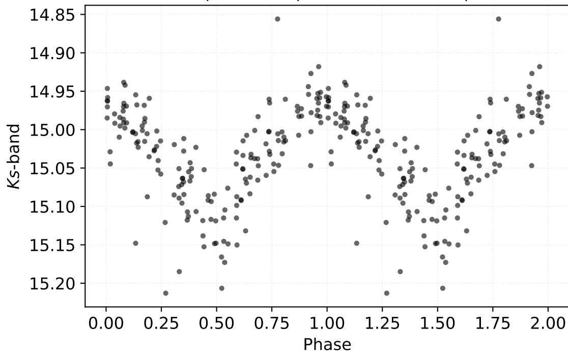
P: 5.95286 d | Class: RP | Subclass: CEP-1OT | Field b279
