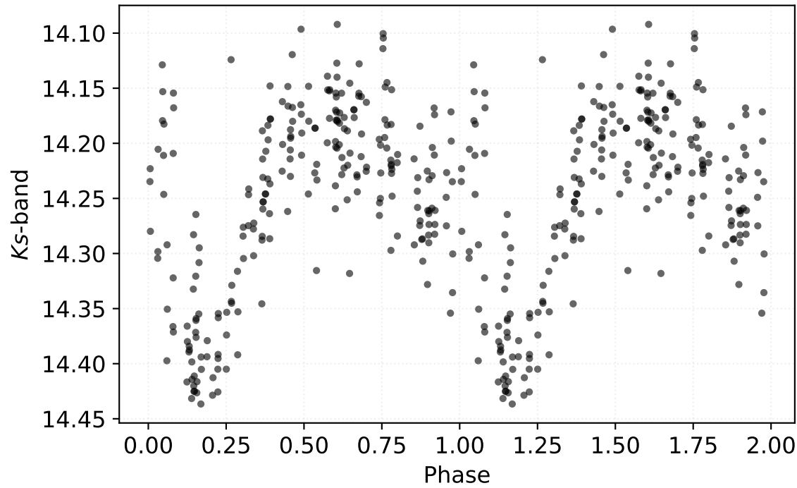
P: 0.33036 d | Class: RP | Subclass: RRab | Field b279
