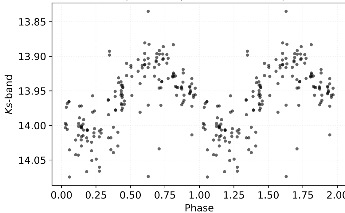
P: 0.27831 d | Class: RP | Subclass: CEP-1OT | Field b278
