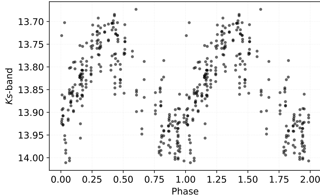
P: 0.21442 d | Class: RP | Subclass: UVAR | Field b279
