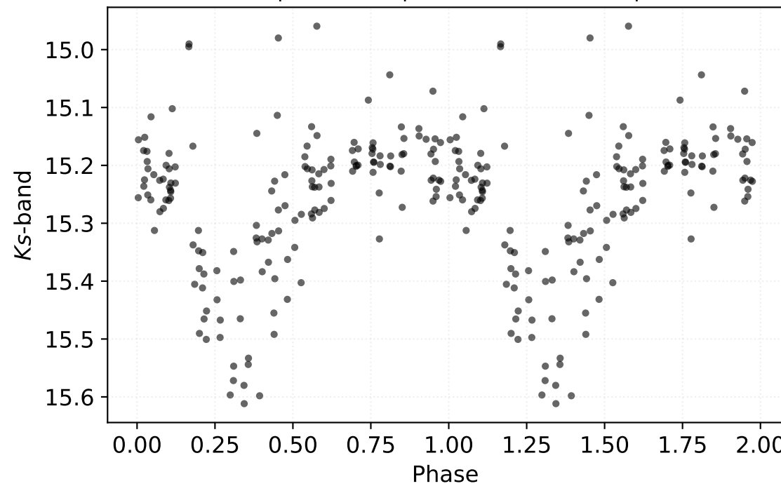
P: 0.42863 d | Class: RP | Subclass: CEP-1OT | Field b278
