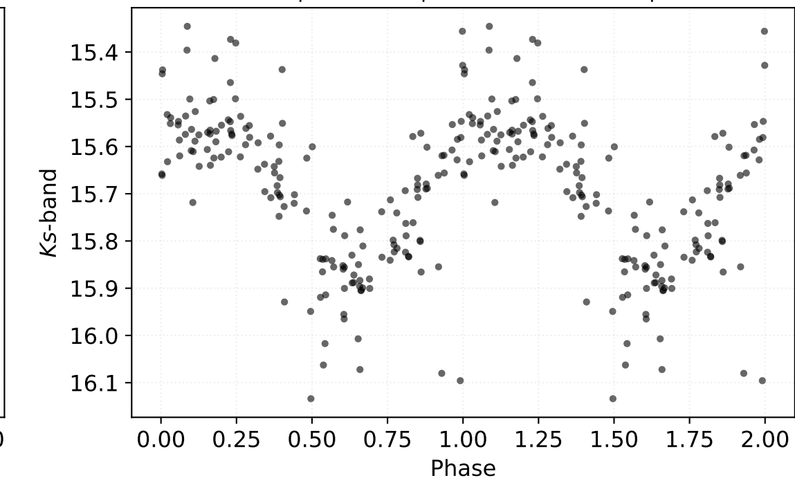
P: 0.47770 d | Class: RP | Subclass: CEP-1OT | Field b278
