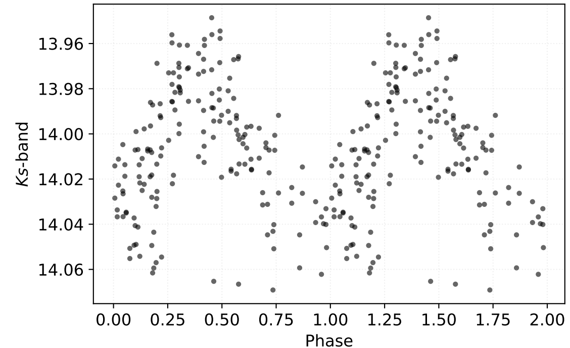
P: 71.02515 d | Class: RP | Subclass: CEP-F | Field b278
