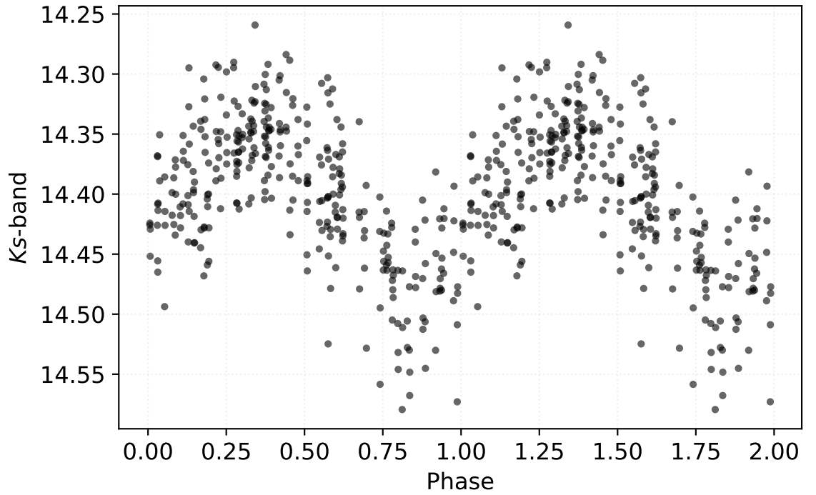
P: 1.06083 d | Class: RP | Subclass: CEP-F | Field b279
