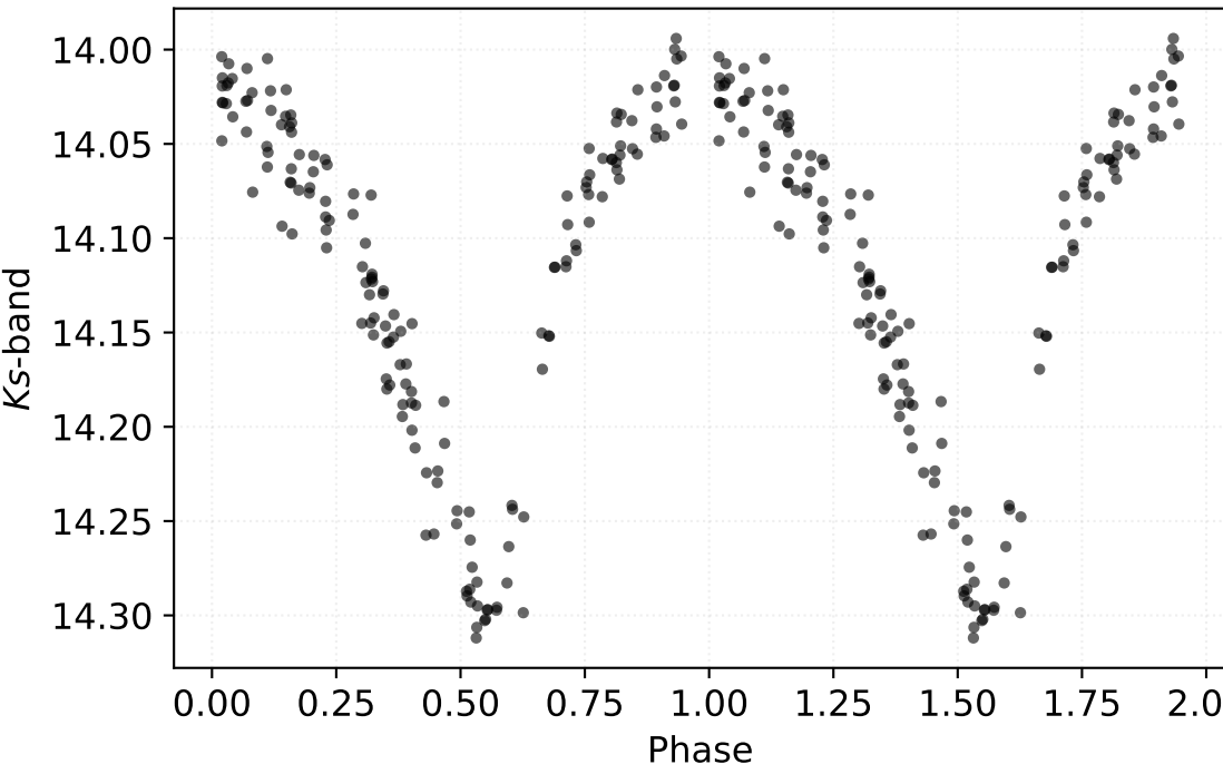
P: 0.73516 d | Class: RP | Subclass: CEP-1OT | Field b278
