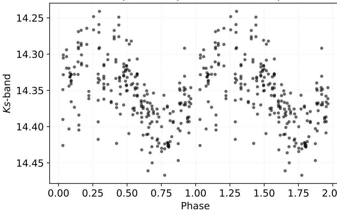
P: 0.30178 d | Class: RP | Subclass: CEP-1OT | Field b278
