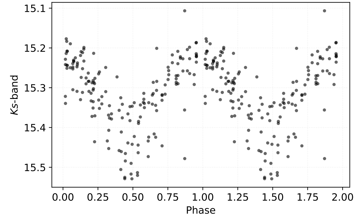
P: 15.16925 d | Class: RP | Subclass: CEP-F | Field b279
