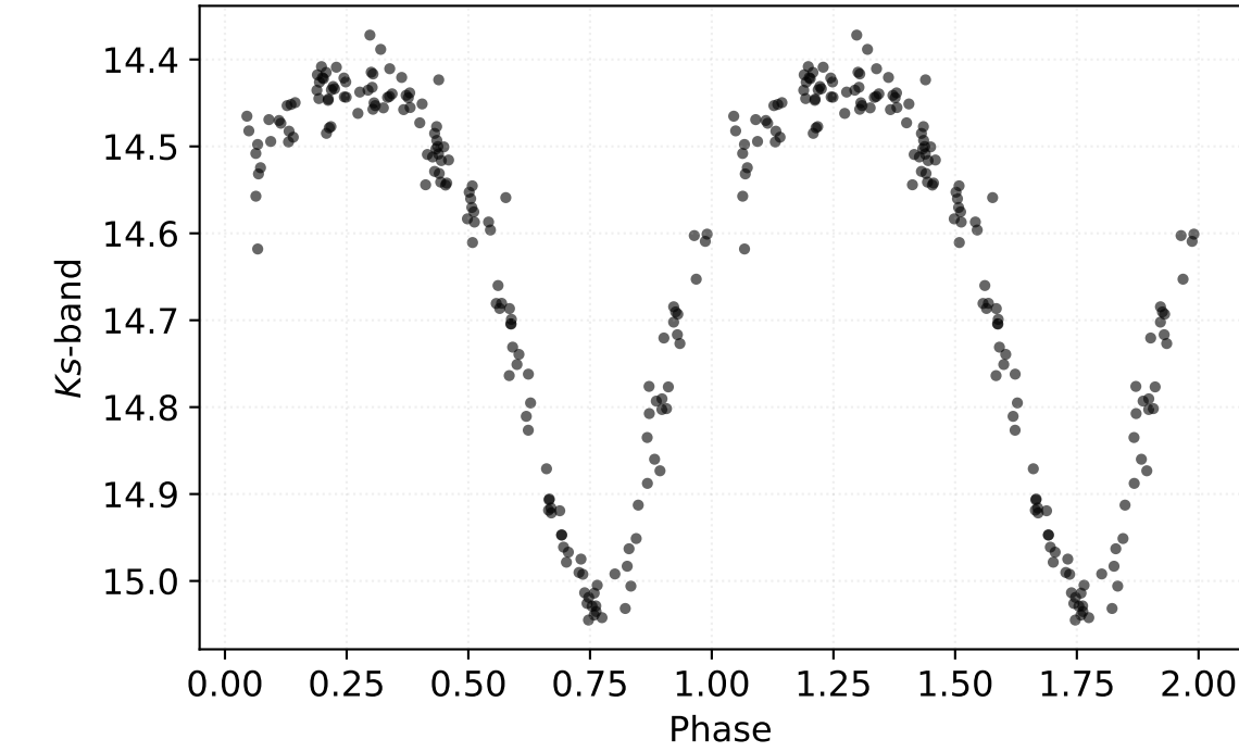
P: 0.49475 d | Class: RP | Subclass: RRc | Field b279
