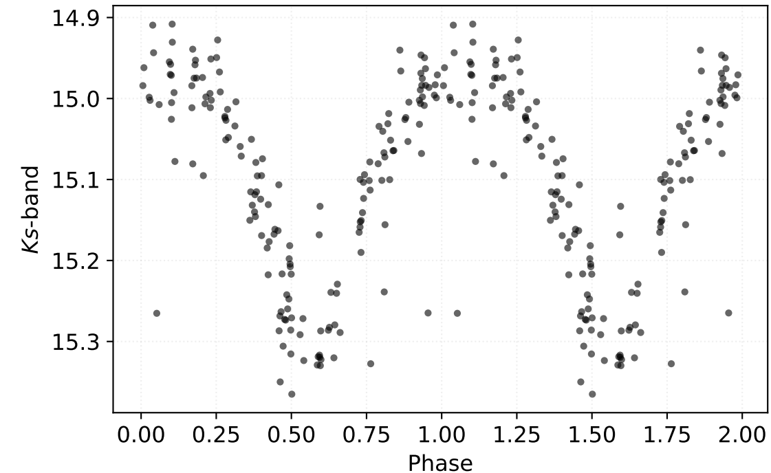
P: 0.19601 d | Class: RP | Subclass: UVAR | Field b279
