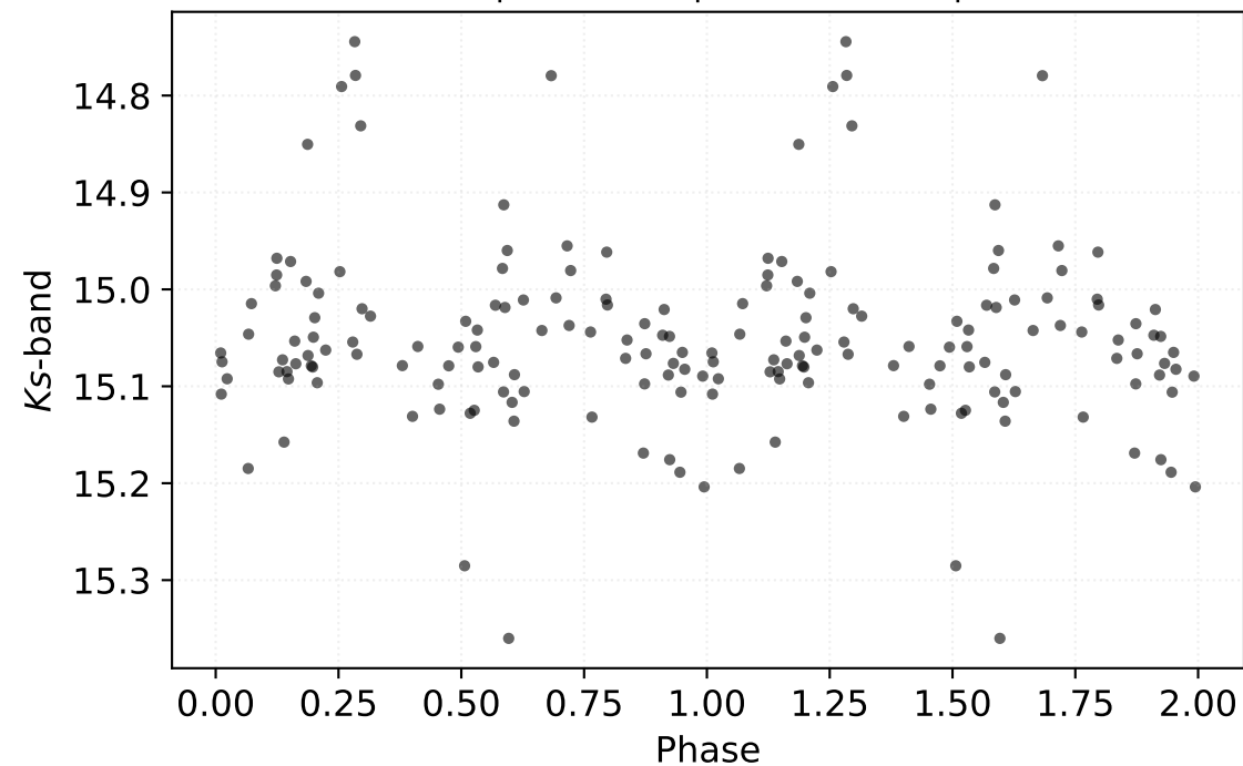
P: 0.56216 d | Class: EB | Subclass: EA | Field b278
