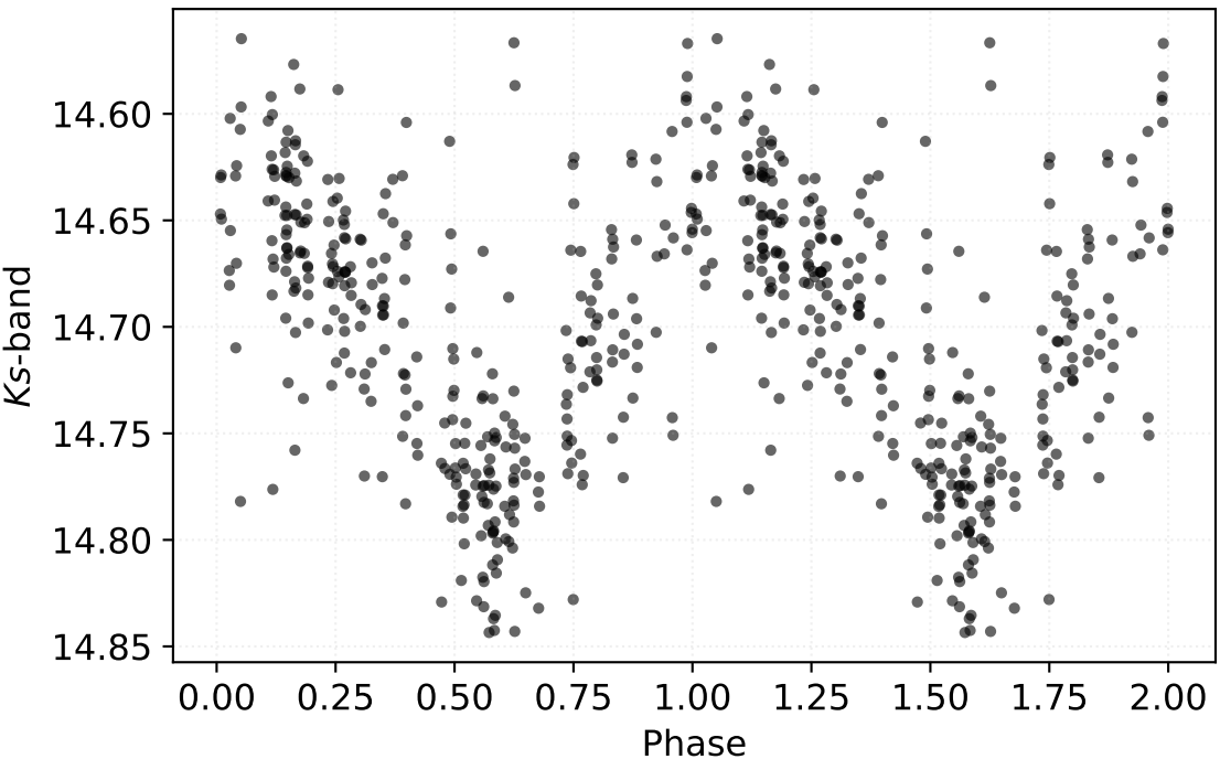
P: 0.60204 d | Class: RP | Subclass: CEP-1OT | Field b278
