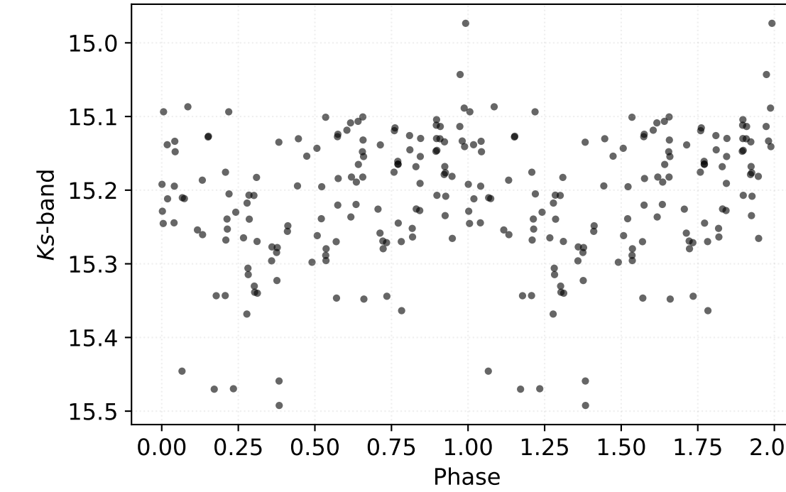
P: 1.32472 d | Class: RP | Subclass: CEP-1OT | Field b279
