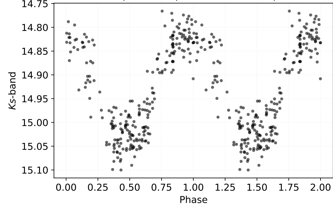
P: 0.56321 d | Class: RP | Subclass: CEP-1OT | Field b278
