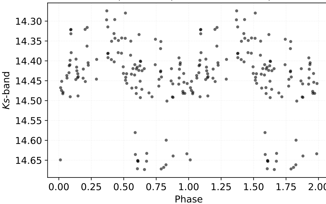
P: 0.88293 d | Class: RP | Subclass: CEP-1OT | Field b278
