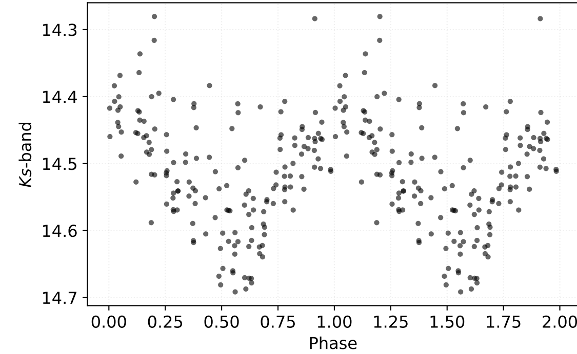
P: 0.62975 d | Class: RP | Subclass: CEP-1OT | Field b279
