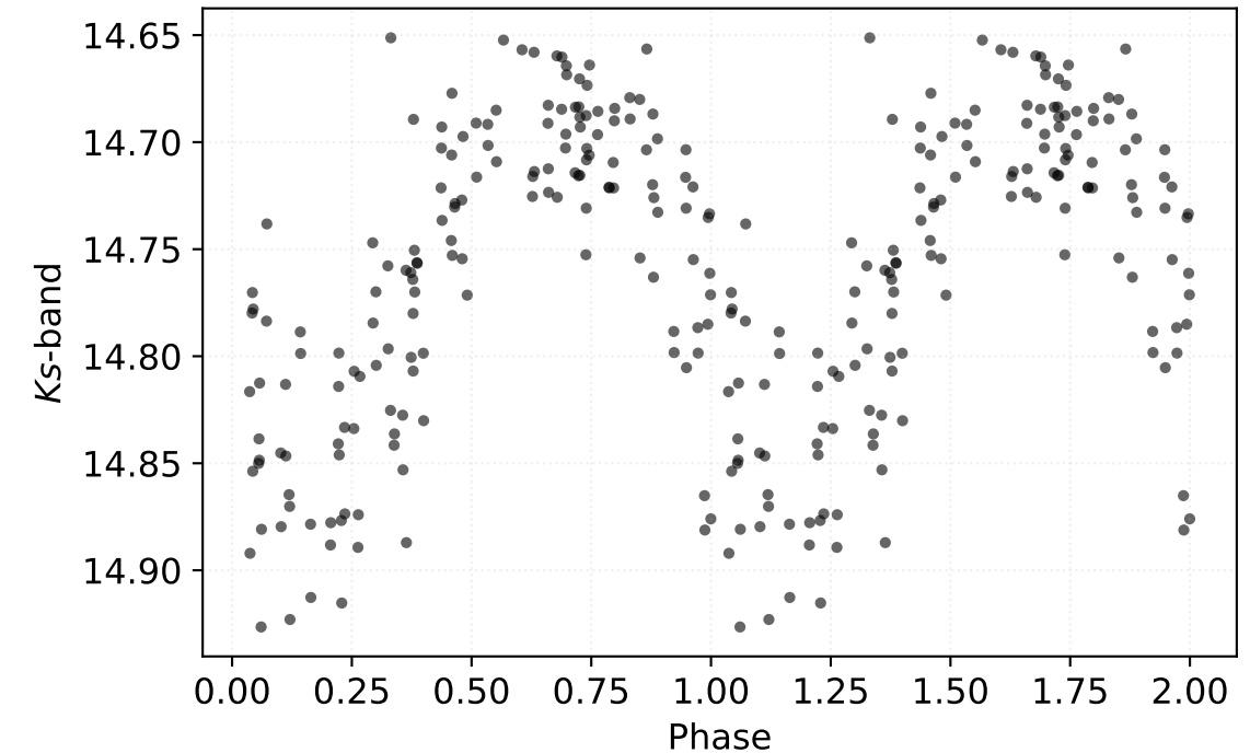
P: 0.58101 d | Class: RP | Subclass: RRab | Field b278
