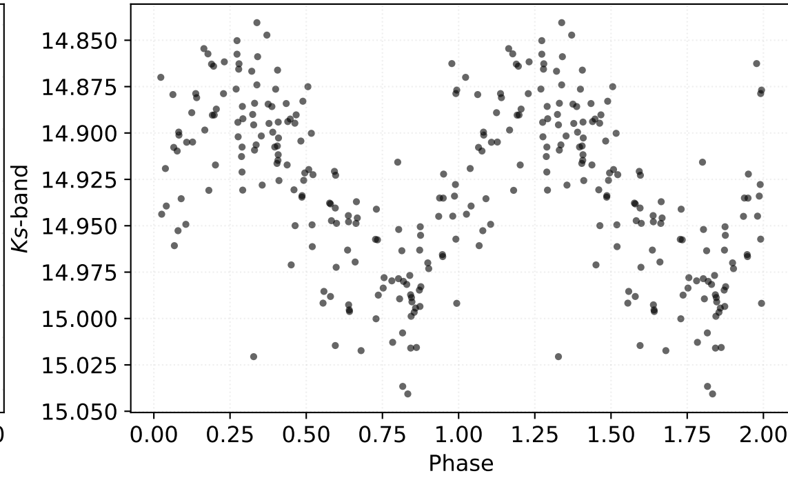
P: 0.28072 d | Class: RP | Subclass: RRc | Field b278
