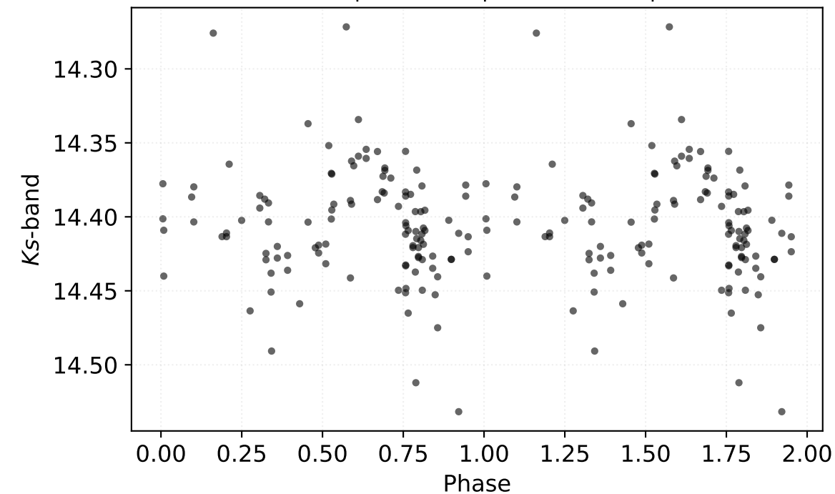
P: 0.38507 d | Class: EB | Subclass: EA | Field b278
