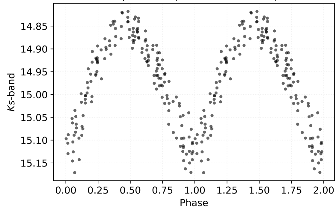
P: 0.45948 d | Class: RP | Subclass: CEP-1OT | Field b278
