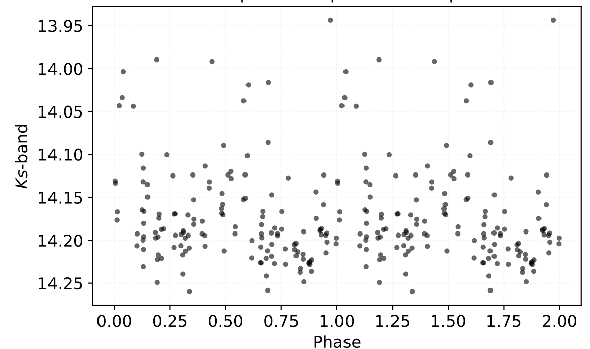
P: 1.75358 d | Class: EB | Subclass: EA | Field b278
