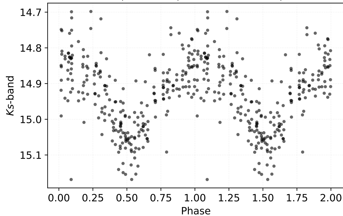
P: 0.34299 d | Class: RP | Subclass: CEP-1OT | Field b279
