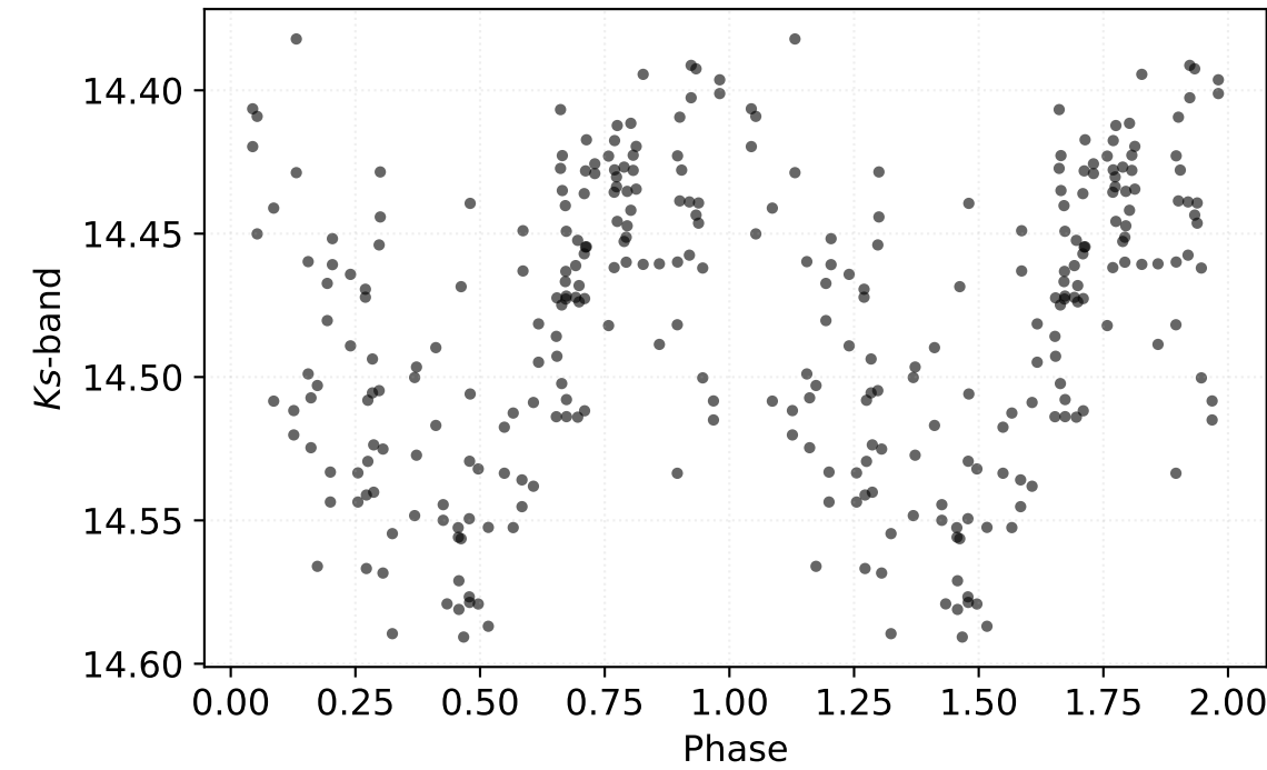
P: 1.69010 d | Class: RP | Subclass: CEP-F | Field b279
