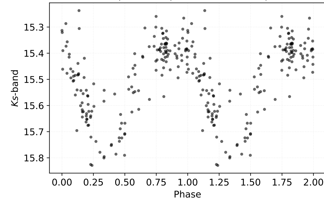
P: 0.64952 d | Class: RP | Subclass: CEP-1OT | Field b278
