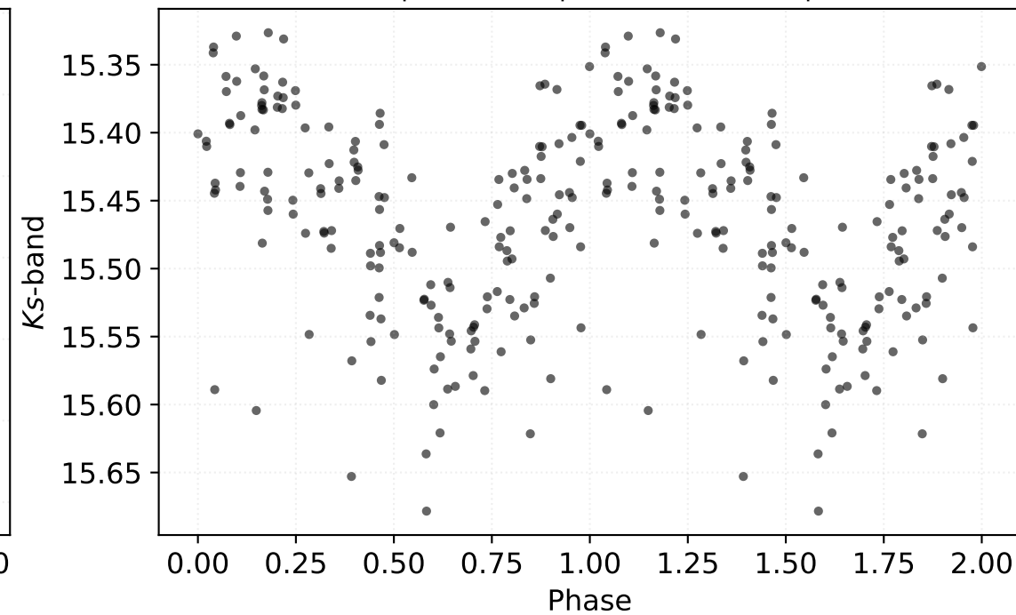
P: 0.38470 d | Class: RP | Subclass: RRab | Field b279
