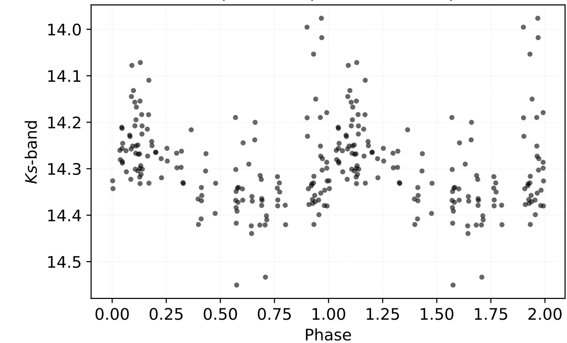
P: 0.19963 d | Class: RP | Subclass: UVAR | Field b278
