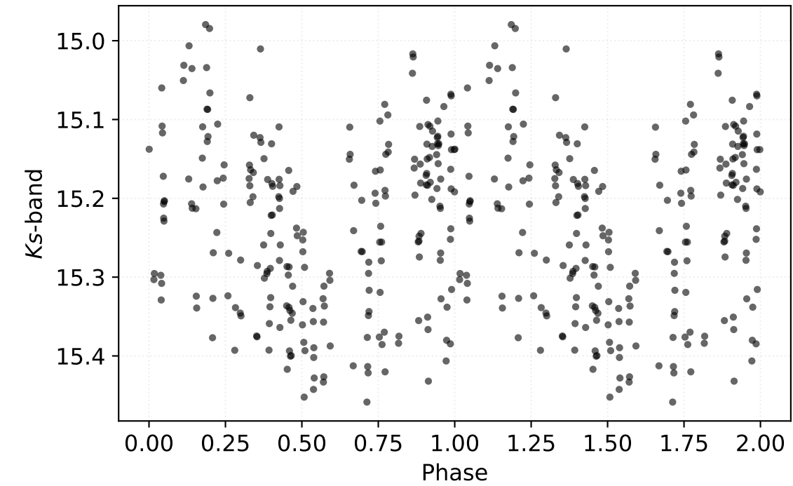
P: 0.33272 d | Class: RP | Subclass: RRab | Field b279
