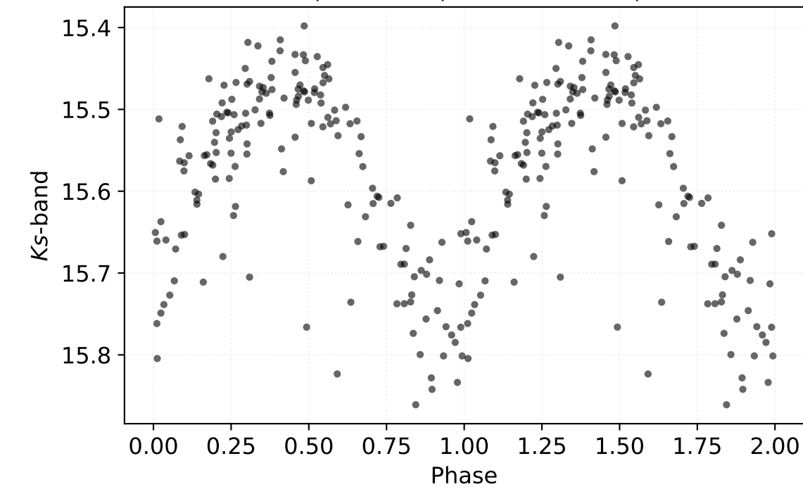
P: 0.41452 d | Class: RP | Subclass: RRab | Field b279
