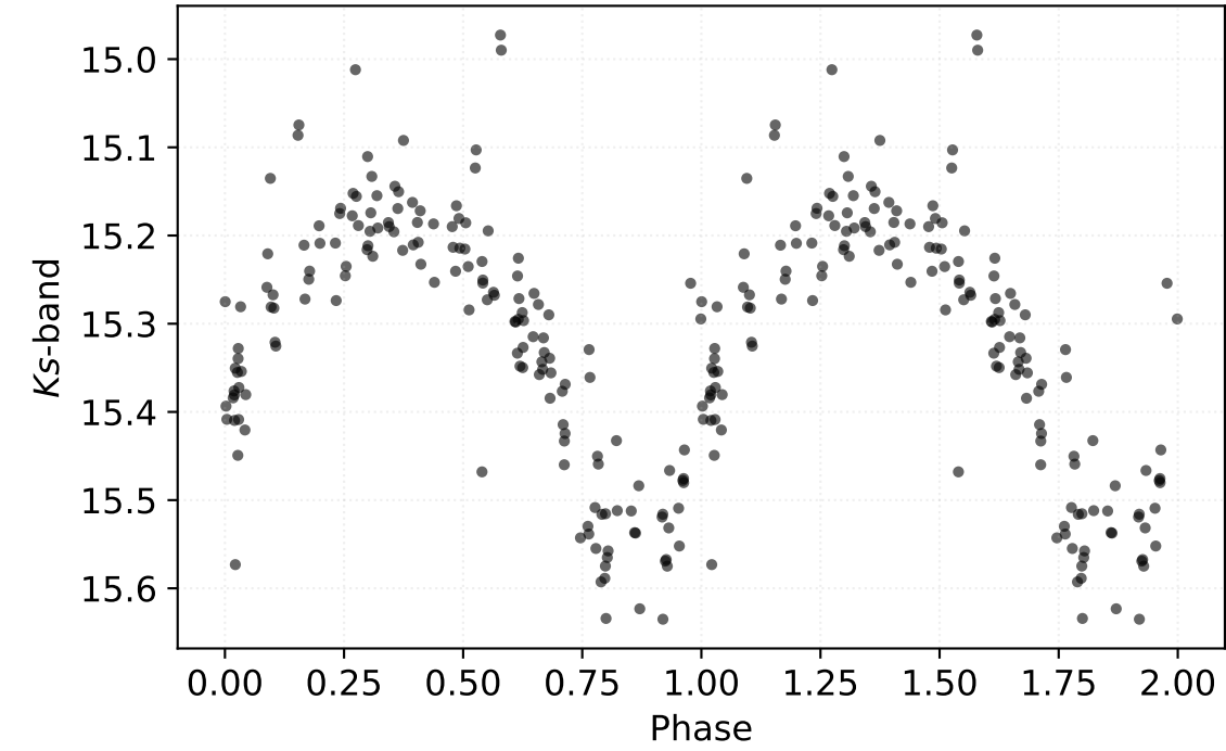
P: 0.25446 d | Class: RP | Subclass: UVAR | Field b278
