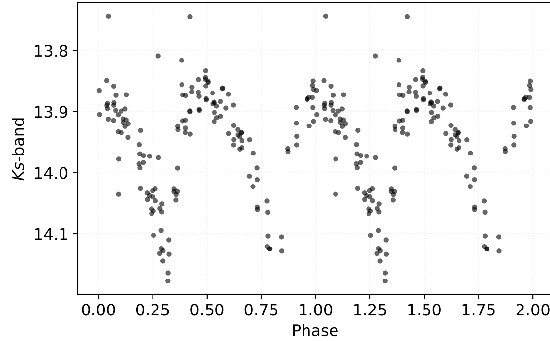
P: 2.67895 d | Class: EB | Subclass: UVAR | Field b278
