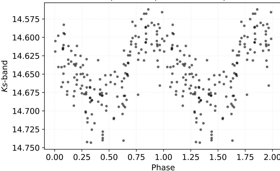
P: 0.62824 d | Class: RP | Subclass: RRab | Field b279
