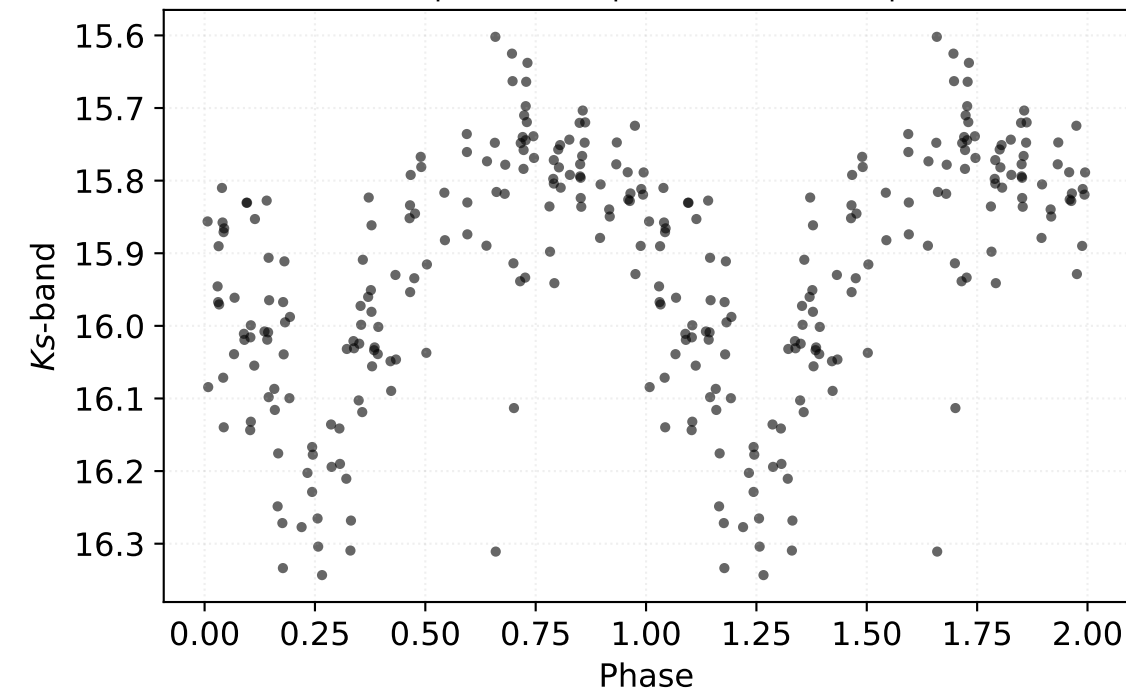
P: 0.84063 d | Class: RP | Subclass: RRab | Field b279
