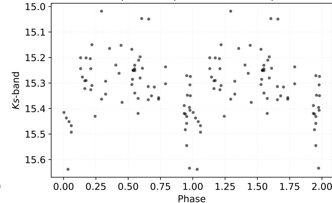
P: 0.49868 d | Class: RP | Subclass: CEP-1OT | Field b278
