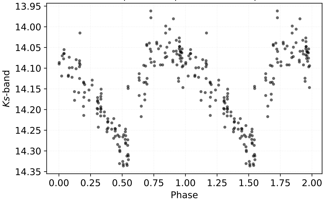
P: 0.56634 d | Class: RP | Subclass: RRab | Field b278
