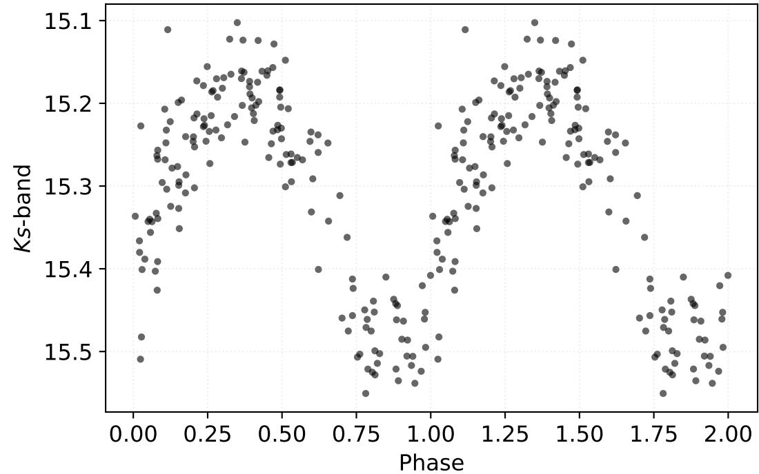
P: 0.17546 d | Class: RP | Subclass: UVAR | Field b279
