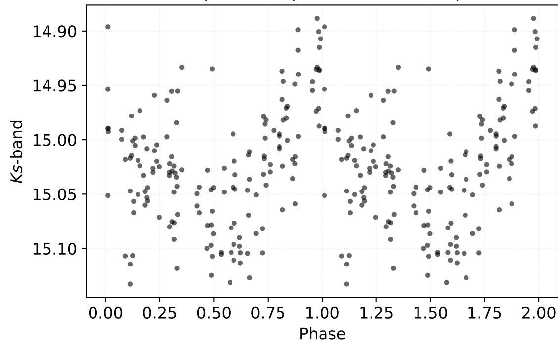
P: 0.36104 d | Class: RP | Subclass: CEP-1OT | Field b278
