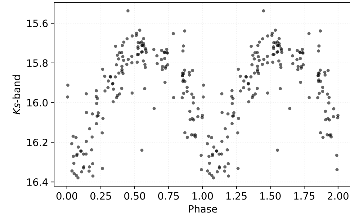
P: 0.59932 d | Class: RP | Subclass: RRc | Field b278
