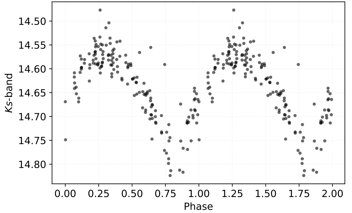
P: 0.38828 d | Class: RP | Subclass: RRab | Field b279
