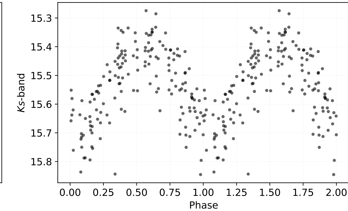
P: 0.59058 d | Class: RP | Subclass: RRc | Field b278
