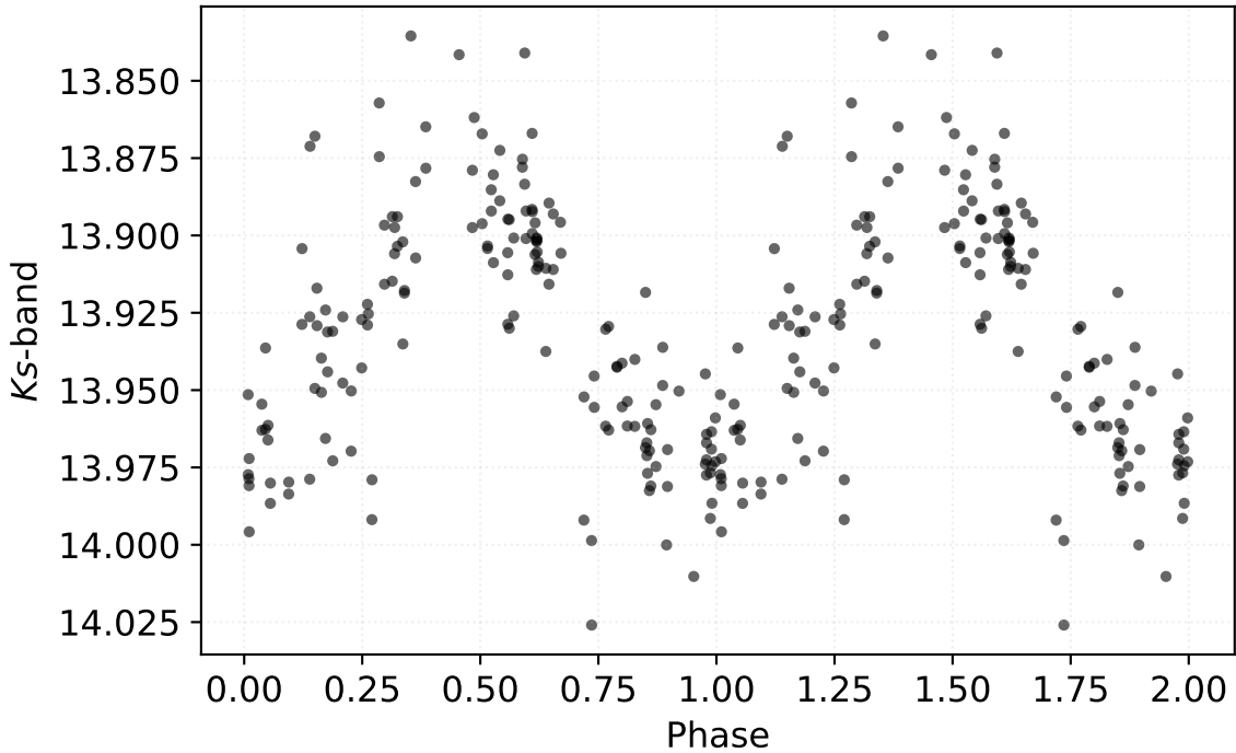
P: 0.43609 d | Class: RP | Subclass: CEP-1OT | Field b278
