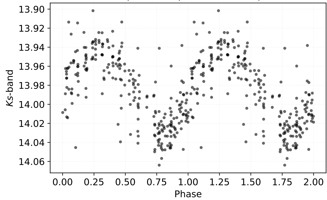
P: 0.44661 d | Class: RP | Subclass: RRab | Field b279
