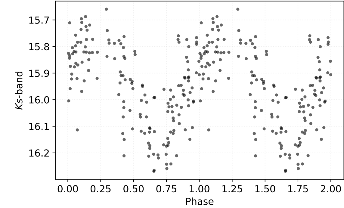
P: 0.39909 d | Class: RP | Subclass: RRab | Field b279
