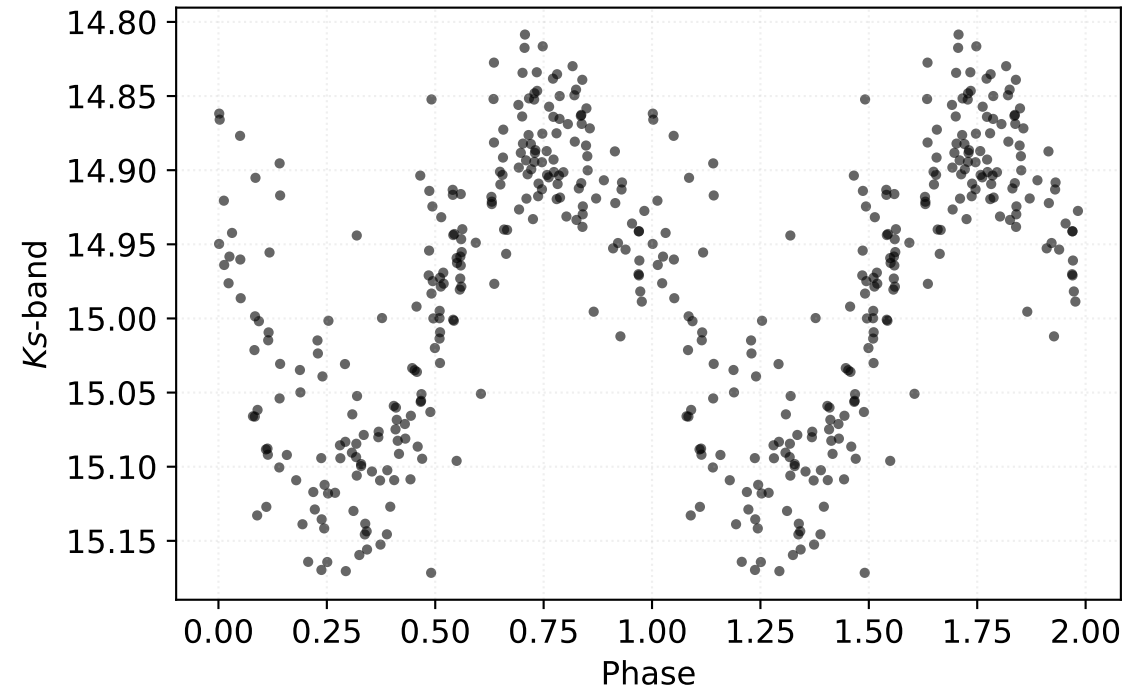
P: 0.43723 d | Class: RP | Subclass: RRab | Field b278
