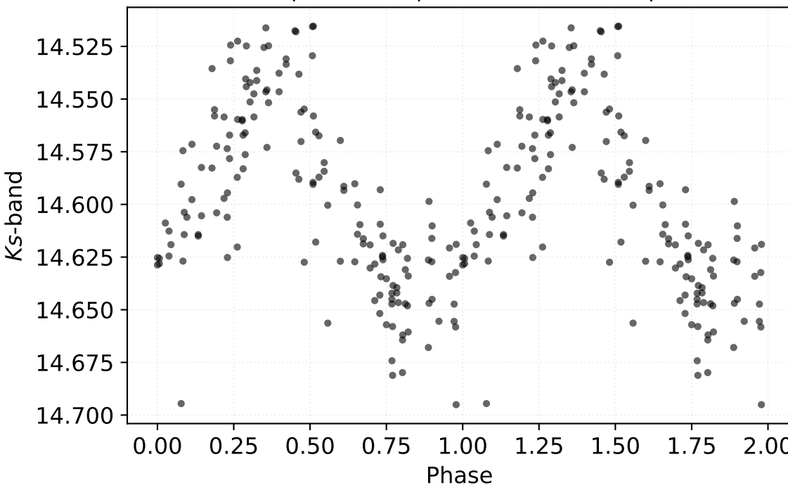
P: 2.25160 d | Class: RP | Subclass: CEP-1OT | Field b278
