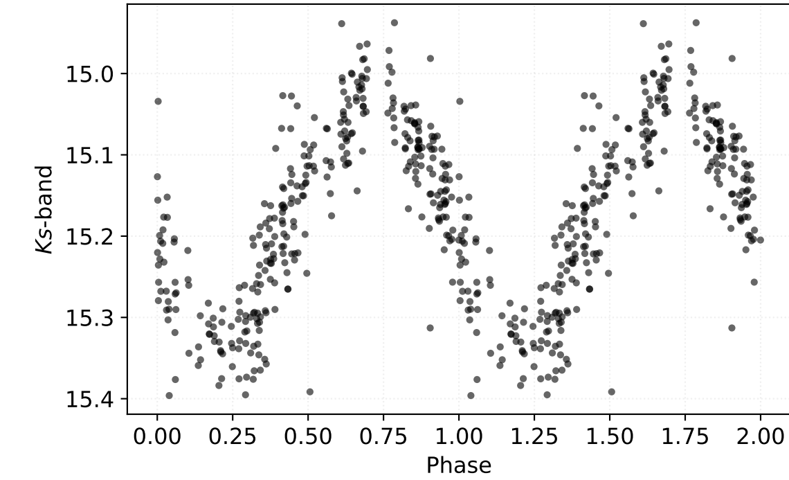
P: 0.41857 d | Class: RP | Subclass: RRc | Field b278
