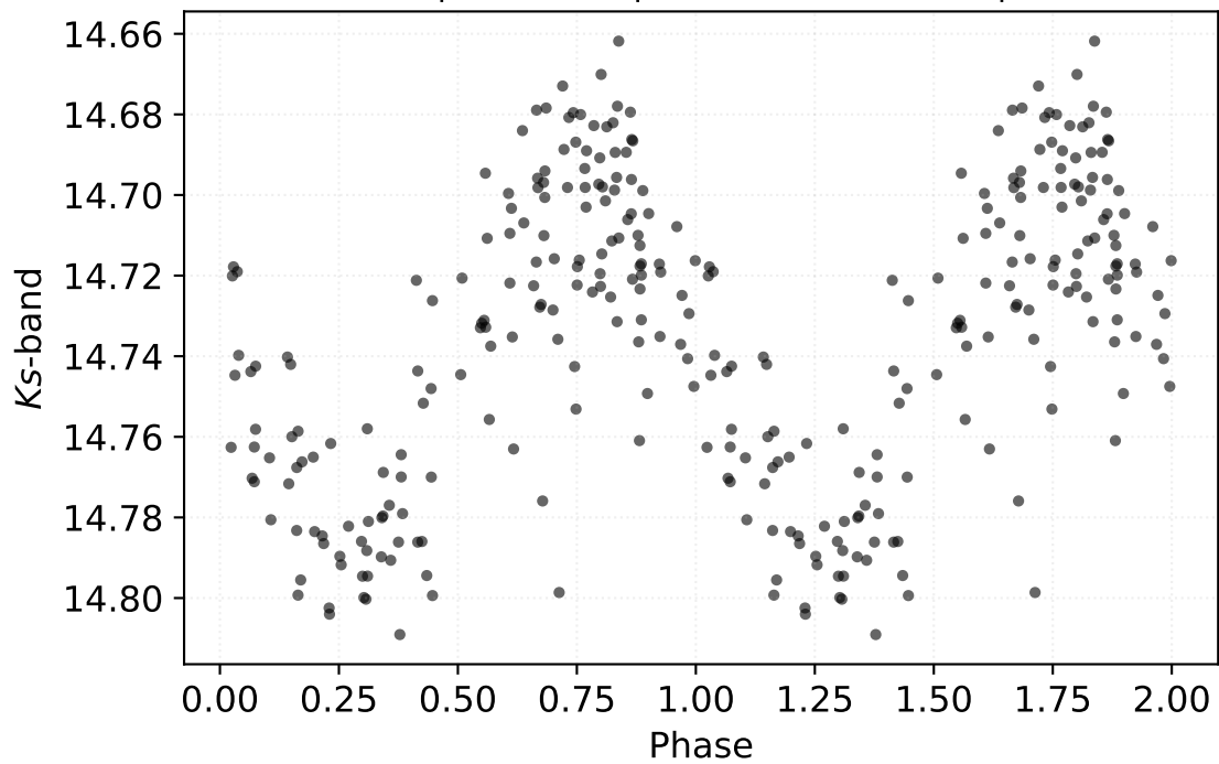
P: 0.27216 d | Class: RP | Subclass: CEP-1OT | Field b278
