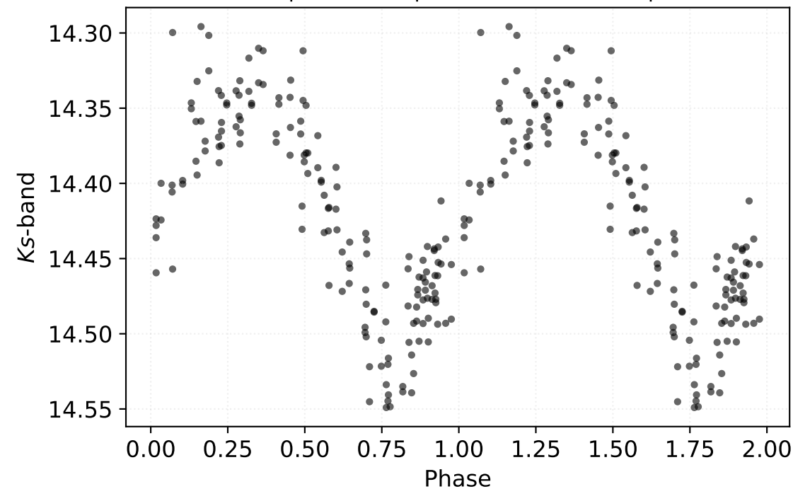
P: 0.44348 d | Class: RP | Subclass: CEP-1OT | Field b278
