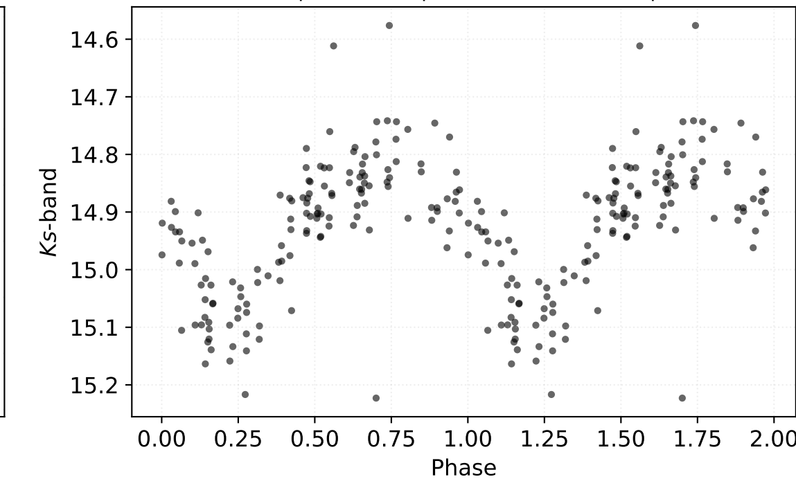
P: 0.40504 d | Class: RP | Subclass: CEP-1OT | Field b278
