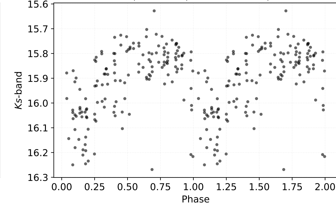
P: 0.80729 d | Class: RP | Subclass: RRab | Field b279
