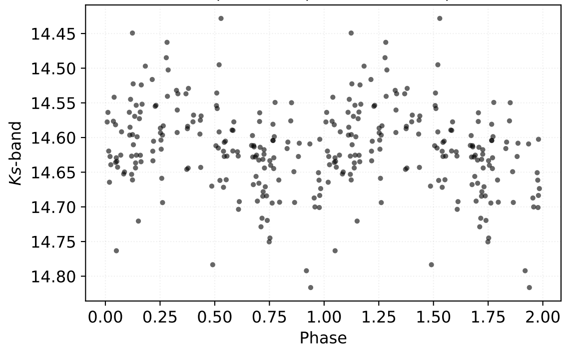
P: 0.21922 d | Class: RP | Subclass: UVAR | Field b279
