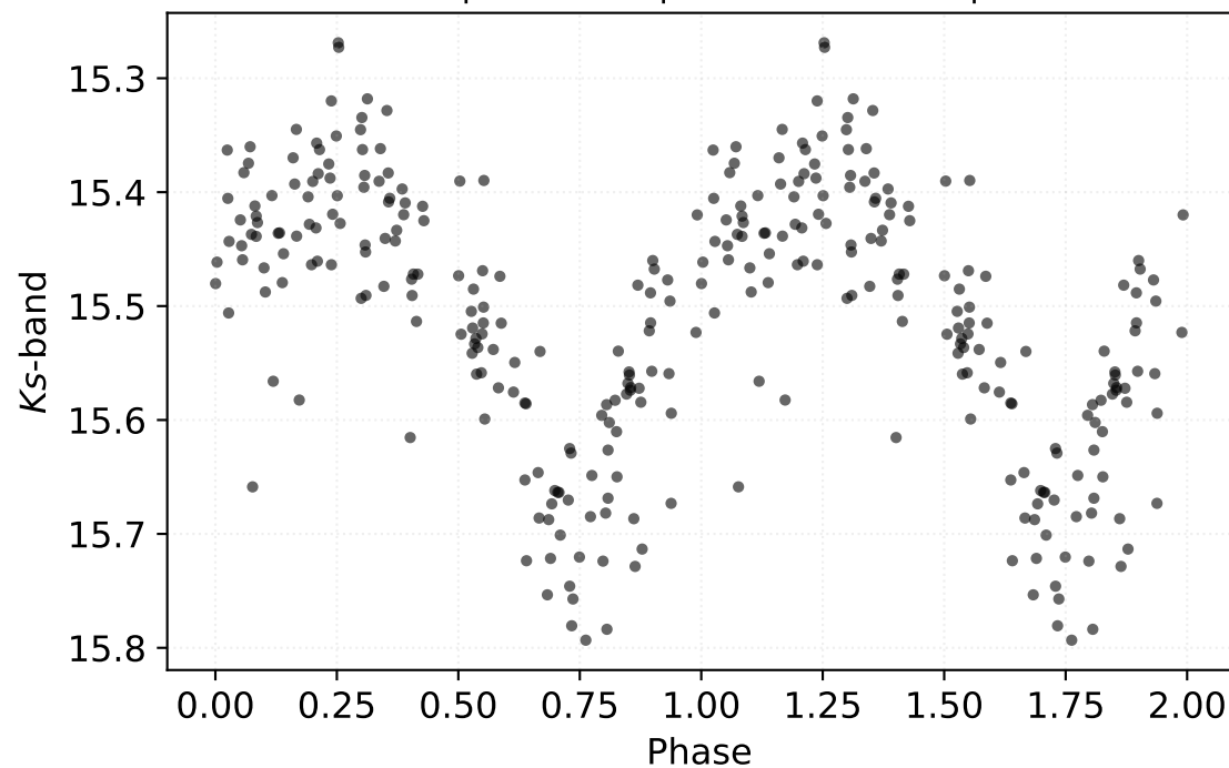
P: 0.15126 d | Class: RP | Subclass: UVAR | Field b279
