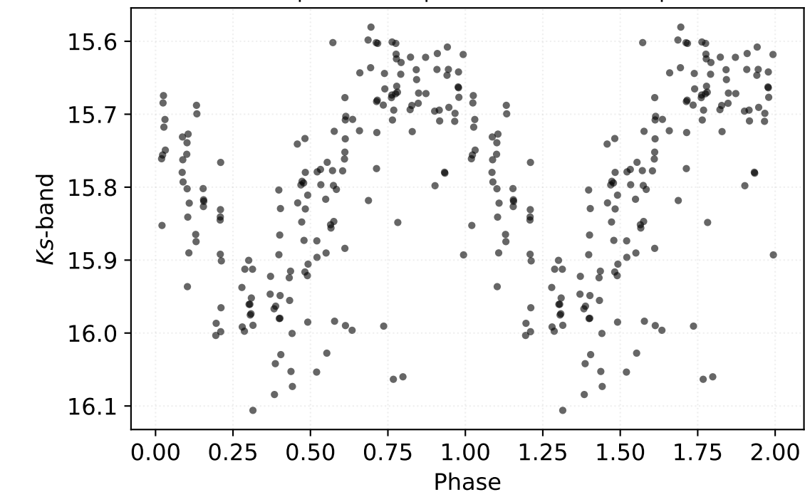
P: 0.46765 d | Class: RP | Subclass: CEP-1OT | Field b279
