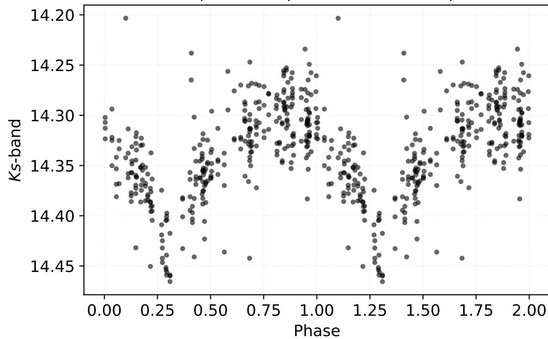
P: 0.71207 d | Class: RP | Subclass: CEP-1OT | Field b278
