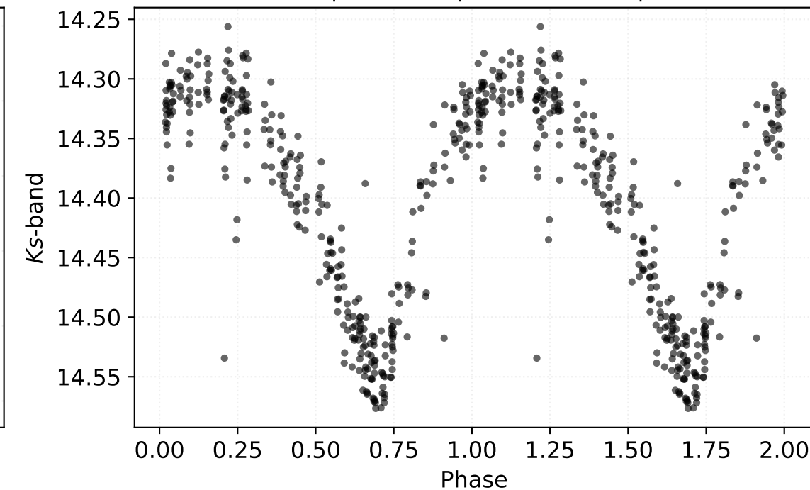
P: 0.43417 d | Class: RP | Subclass: RRc | Field b279
