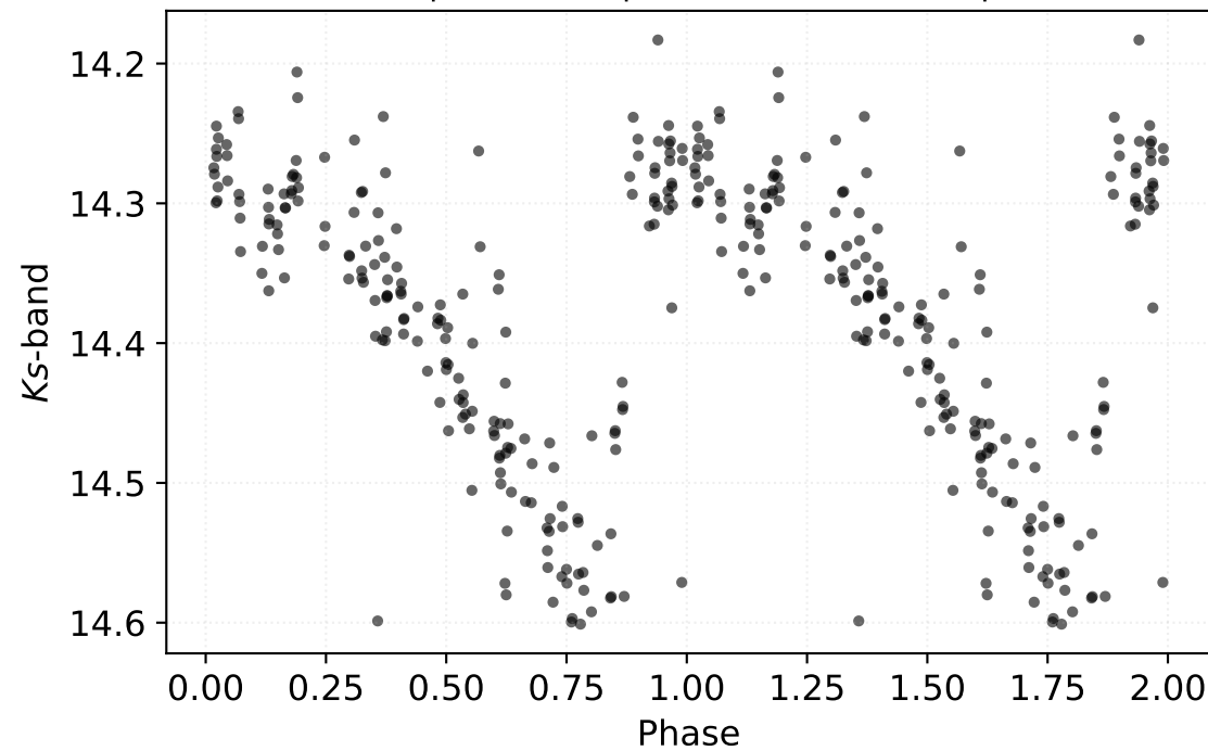
P: 0.58608 d | Class: RP | Subclass: CEP-1OT | Field b278
