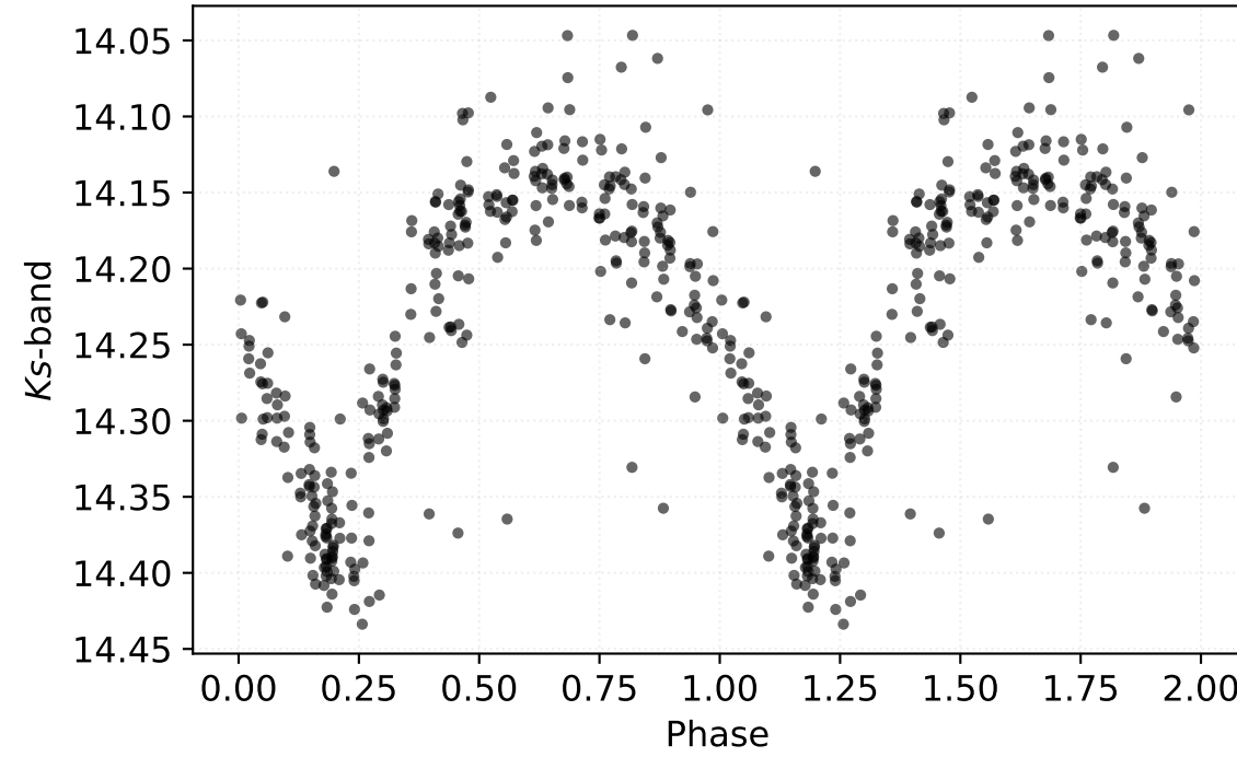
P: 0.26189 d | Class: RP | Subclass: RRc | Field b279
