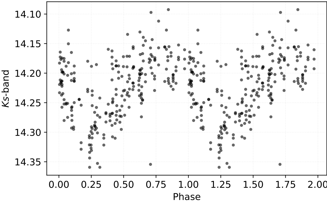
P: 6.11151 d | Class: RP | Subclass: CEP-F | Field b279
