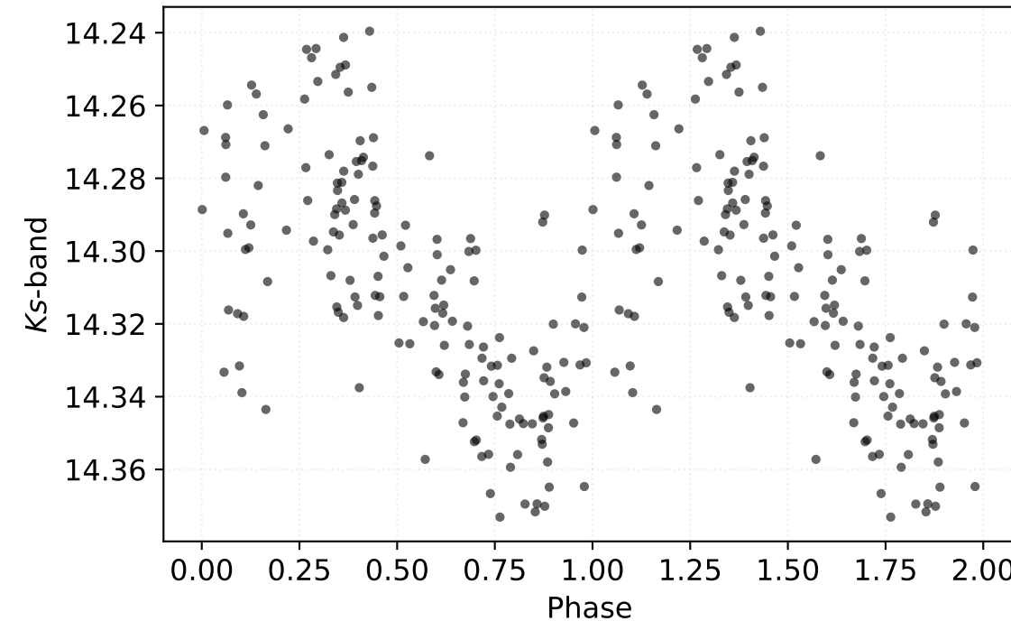
P: 0.12849 d | Class: RP | Subclass: UVAR | Field b278
