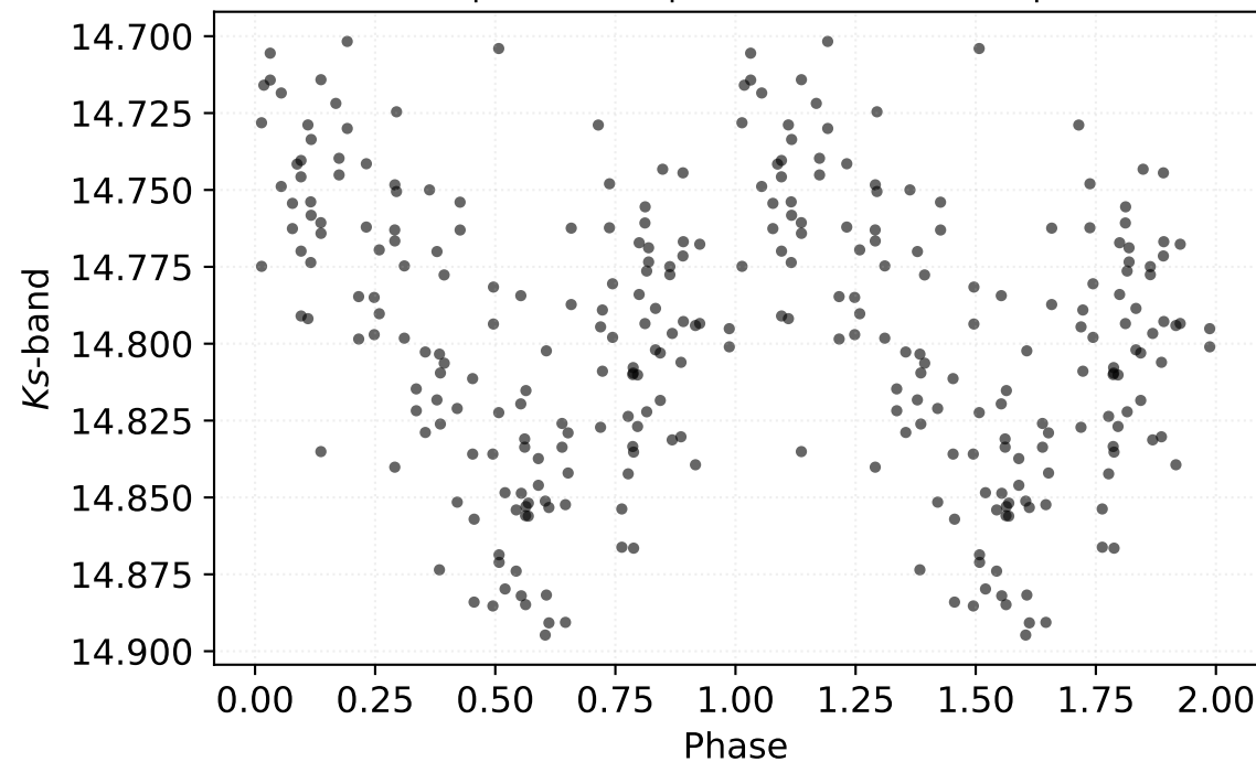
P: 0.37417 d | Class: RP | Subclass: CEP-1OT | Field b278
