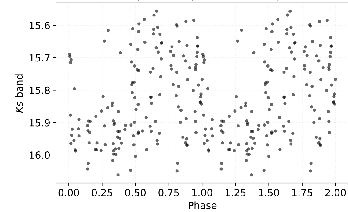
P: 0.10858 d | Class: RP | Subclass: UVAR | Field b279
