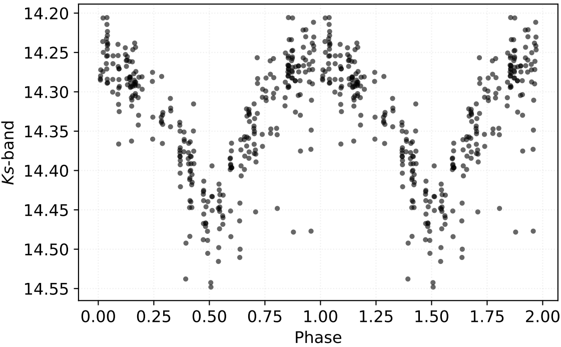
P: 0.36418 d | Class: RP | Subclass: RRab | Field b278
