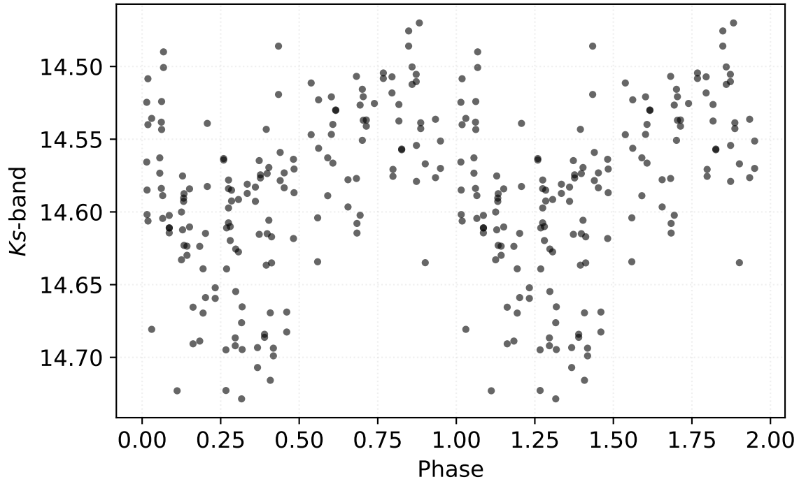
P: 1.42392 d | Class: RP | Subclass: CEP-F | Field b279
