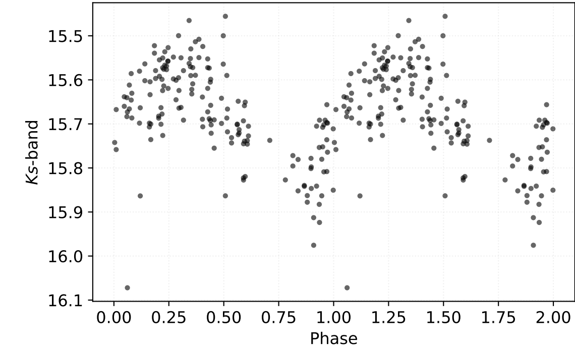
P: 0.47216 d | Class: RP | Subclass: CEP-1OT | Field b279
