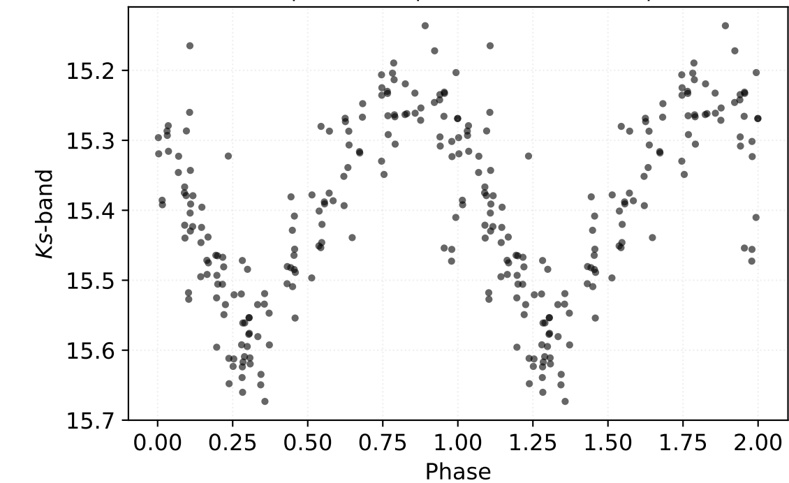
P: 0.33734 d | Class: RP | Subclass: CEP-1OT | Field b279
