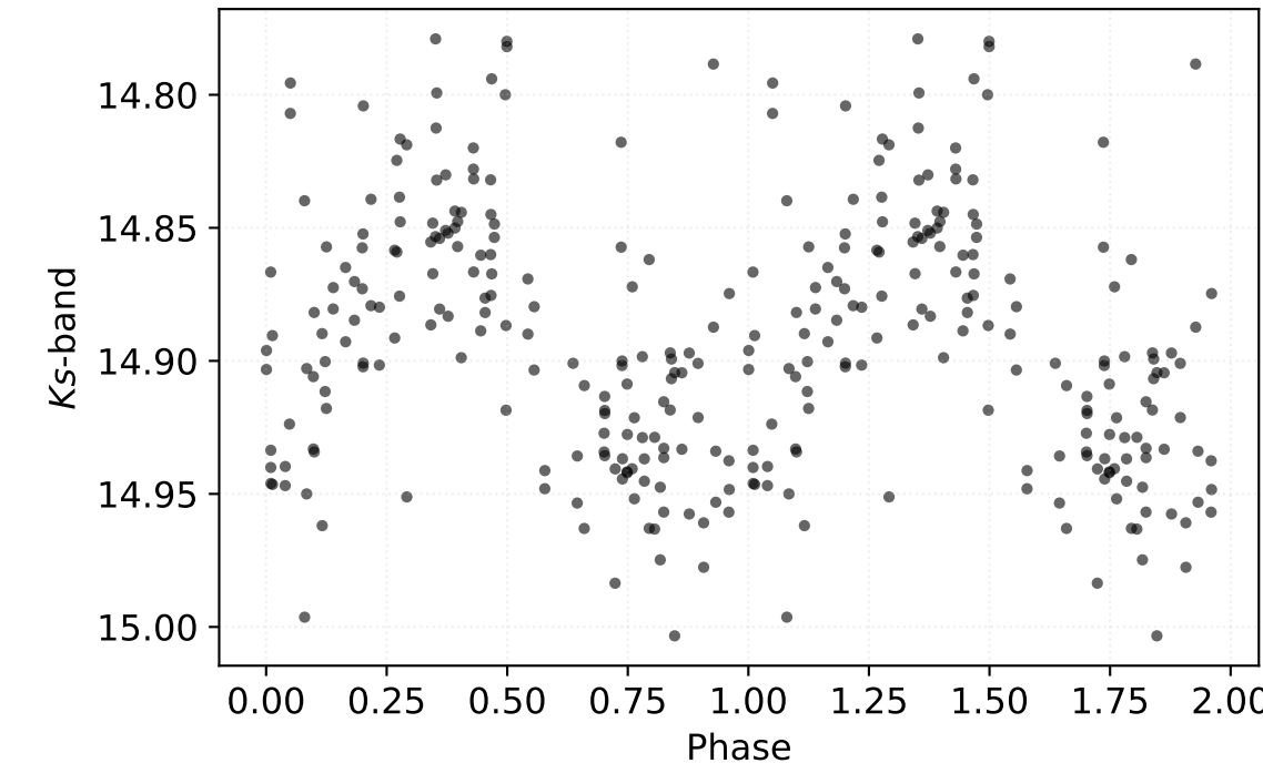
P: 17.59080 d | Class: RP | Subclass: CEP-F | Field b279
