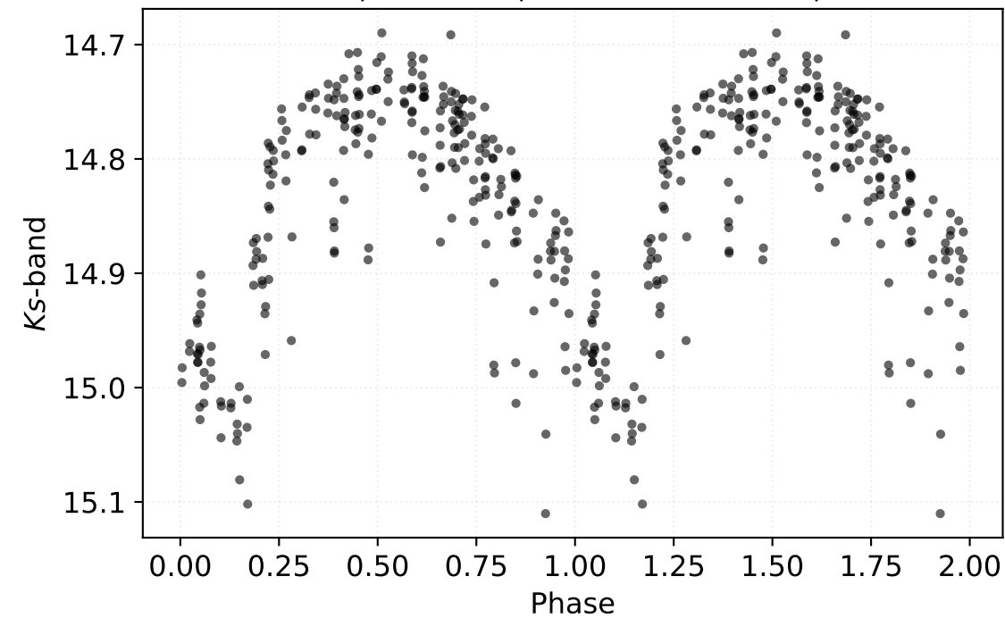
P: 0.52115 d | Class: RP | Subclass: CEP-1OT | Field b278
