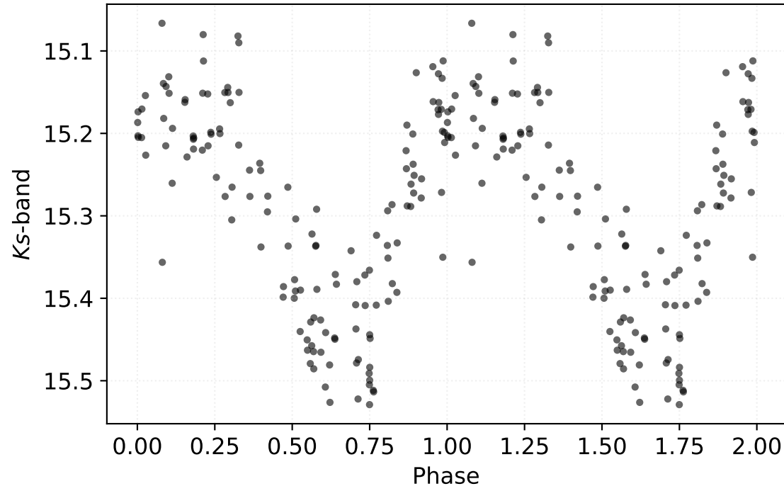
P: 2.34821 d | Class: RP | Subclass: CEP-1OT | Field b279
