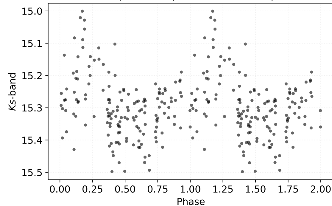
P: 0.41561 d | Class: RP | Subclass: CEP-1OT | Field b278
