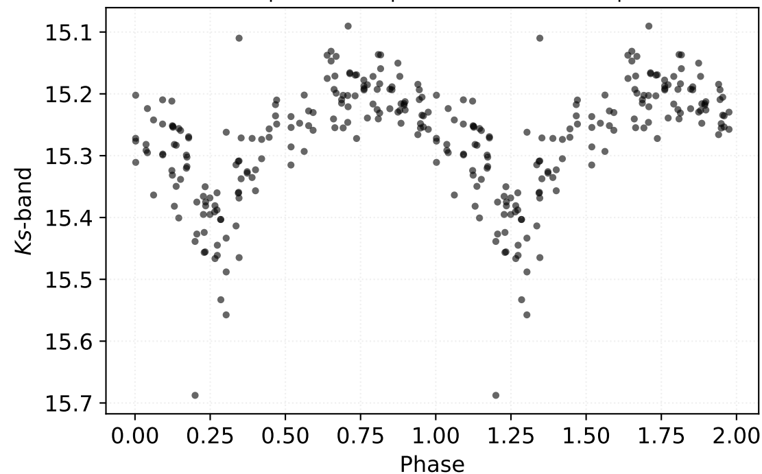
P: 3.36189 d | Class: RP | Subclass: CEP-1OT | Field b279
