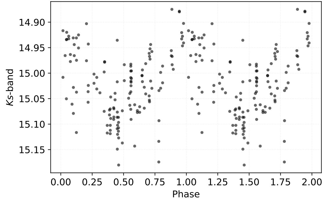
P: 1.00094 d | Class: RP | Subclass: CEP-F | Field b278
