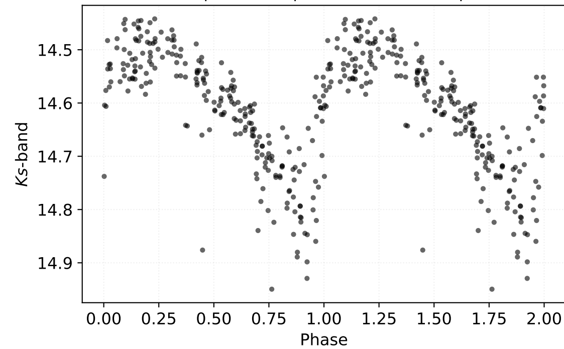
P: 0.42418 d | Class: RP | Subclass: CEP-1OT | Field b278
