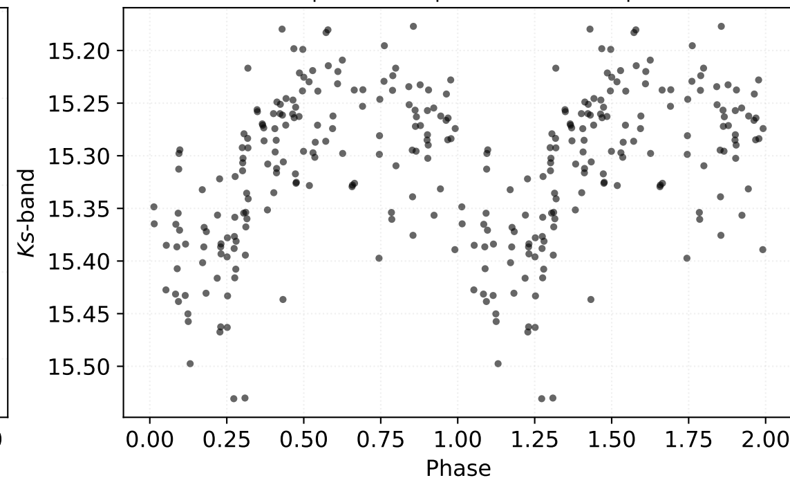
P: 0.39558 d | Class: RP | Subclass: RRab | Field b279
