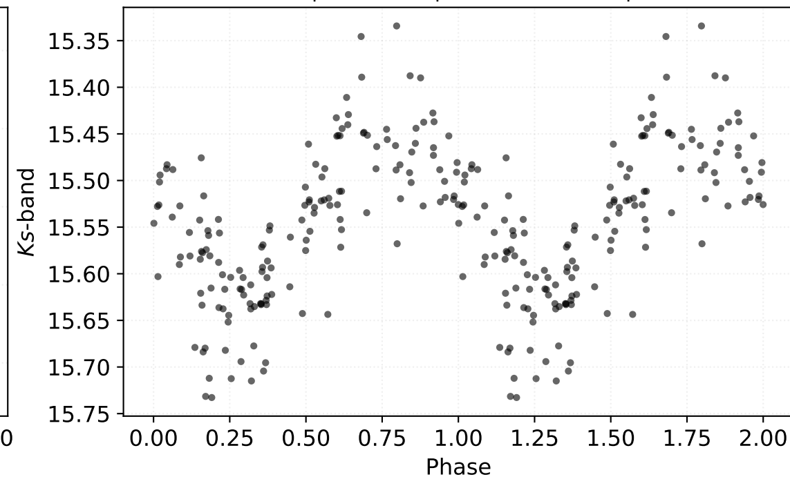
P: 0.43929 d | Class: RP | Subclass: RRab | Field b279
