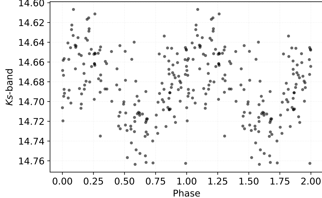
P: 0.35341 d | Class: RP | Subclass: CEP-1OT | Field b278
