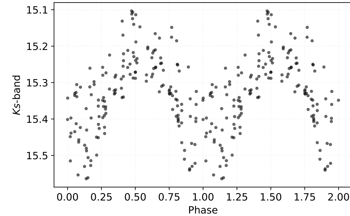
P: 0.59905 d | Class: RP | Subclass: CEP-1OT | Field b279
