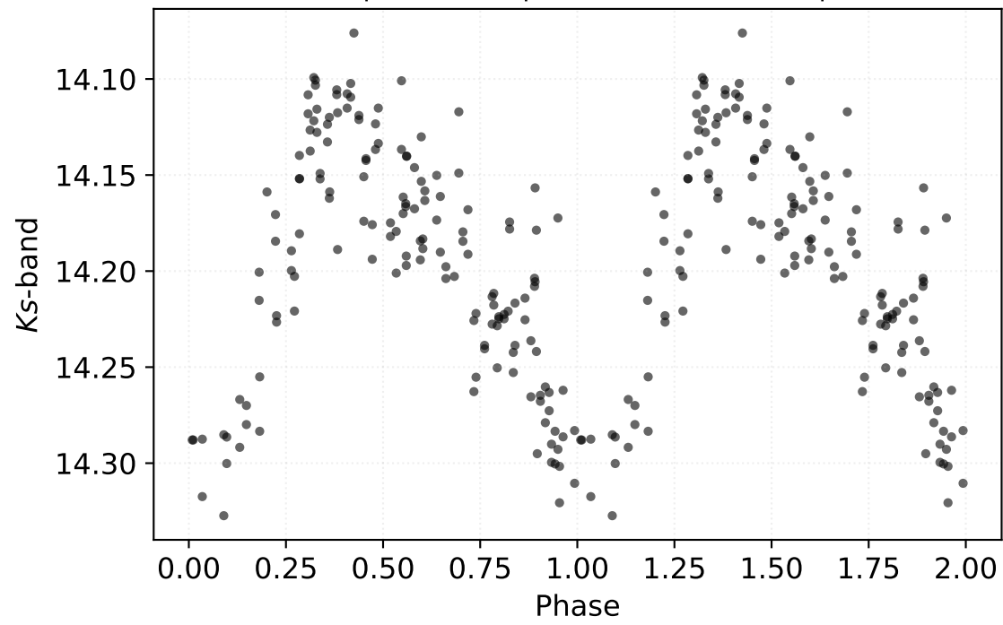
P: 0.74502 d | Class: RP | Subclass: CEP-1OT | Field b278
