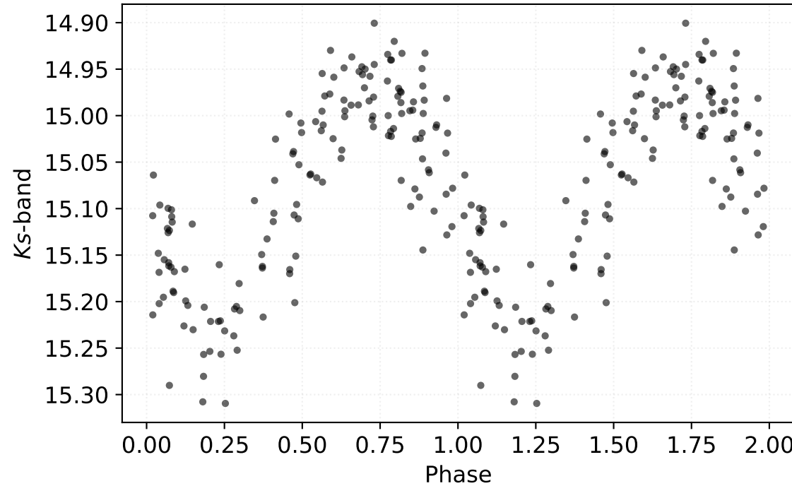
P: 0.15250 d | Class: RP | Subclass: UVAR | Field b279
