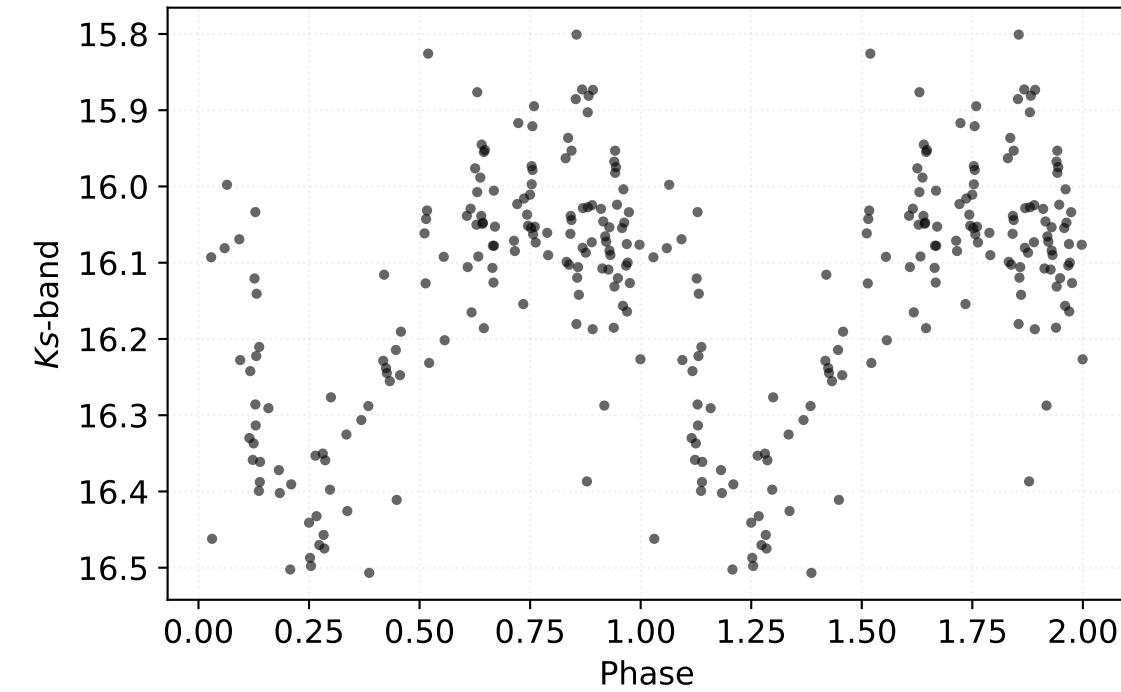
P: 15.25105 d | Class: RP | Subclass: UVAR | Field b279
