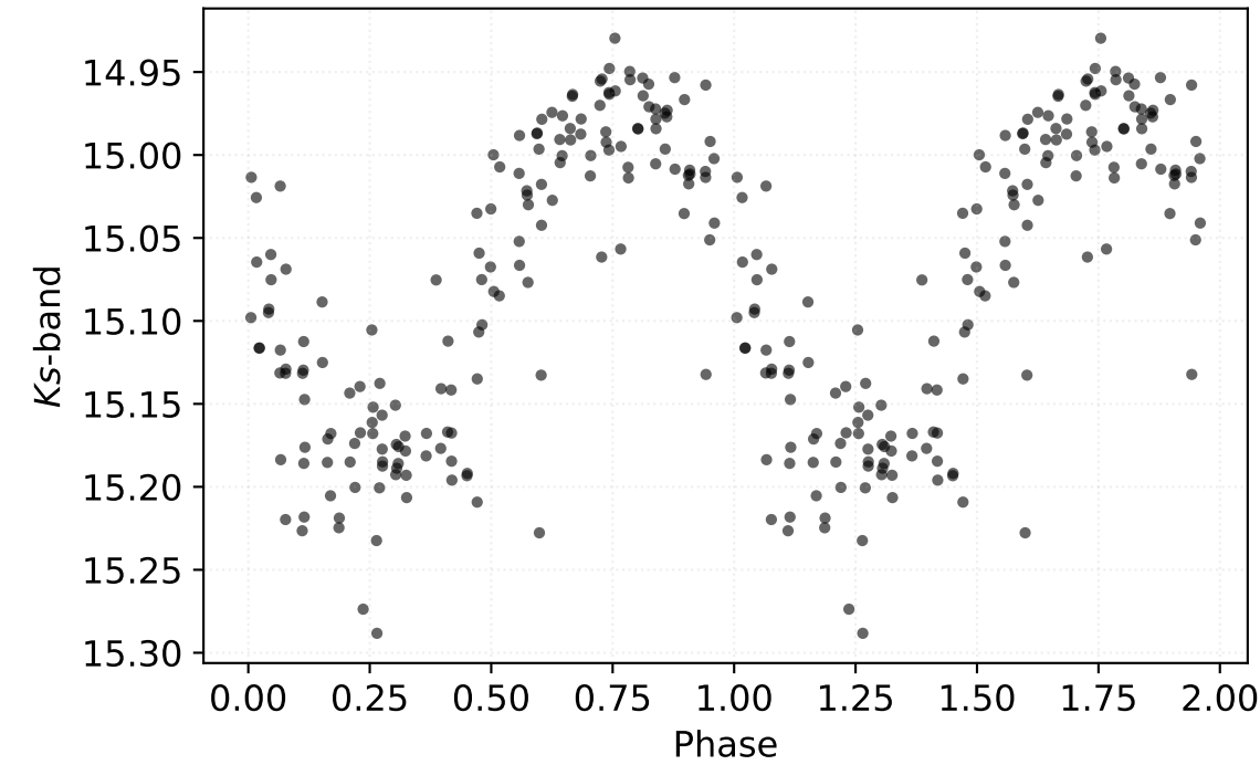
P: 0.77103 d | Class: RP | Subclass: RRab | Field b278
