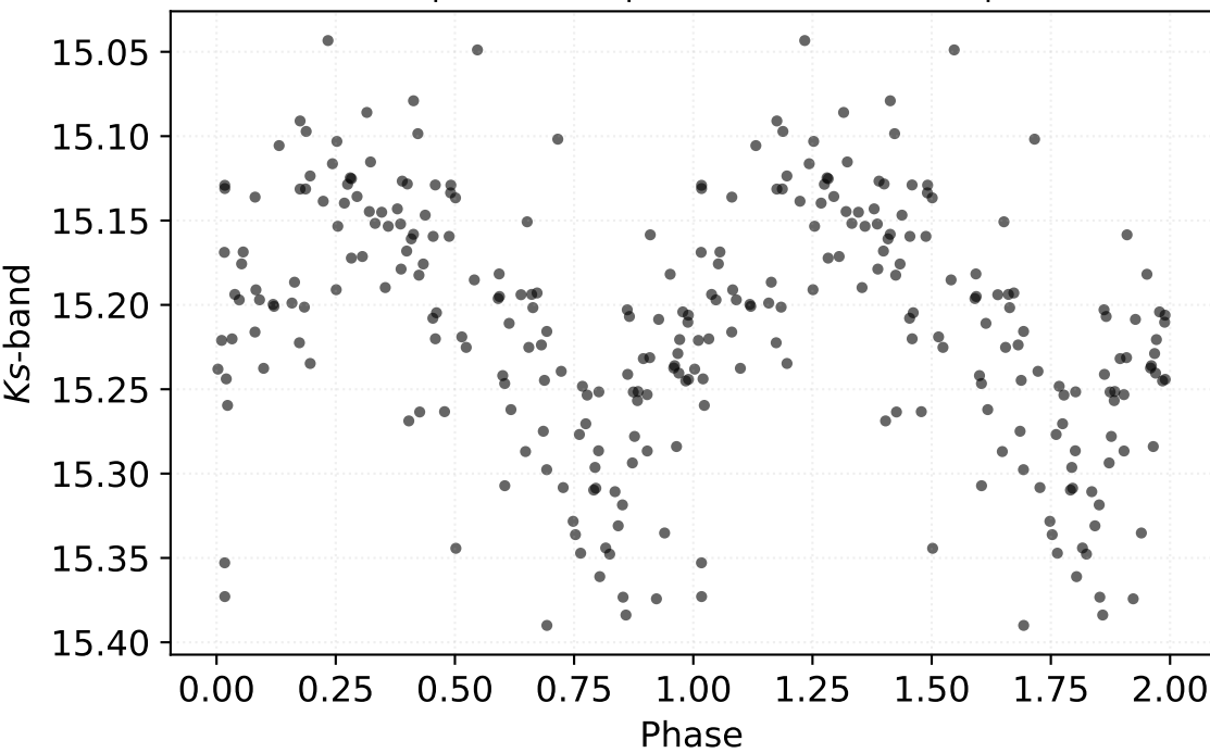
P: 0.43074 d | Class: RP | Subclass: CEP-1OT | Field b278
