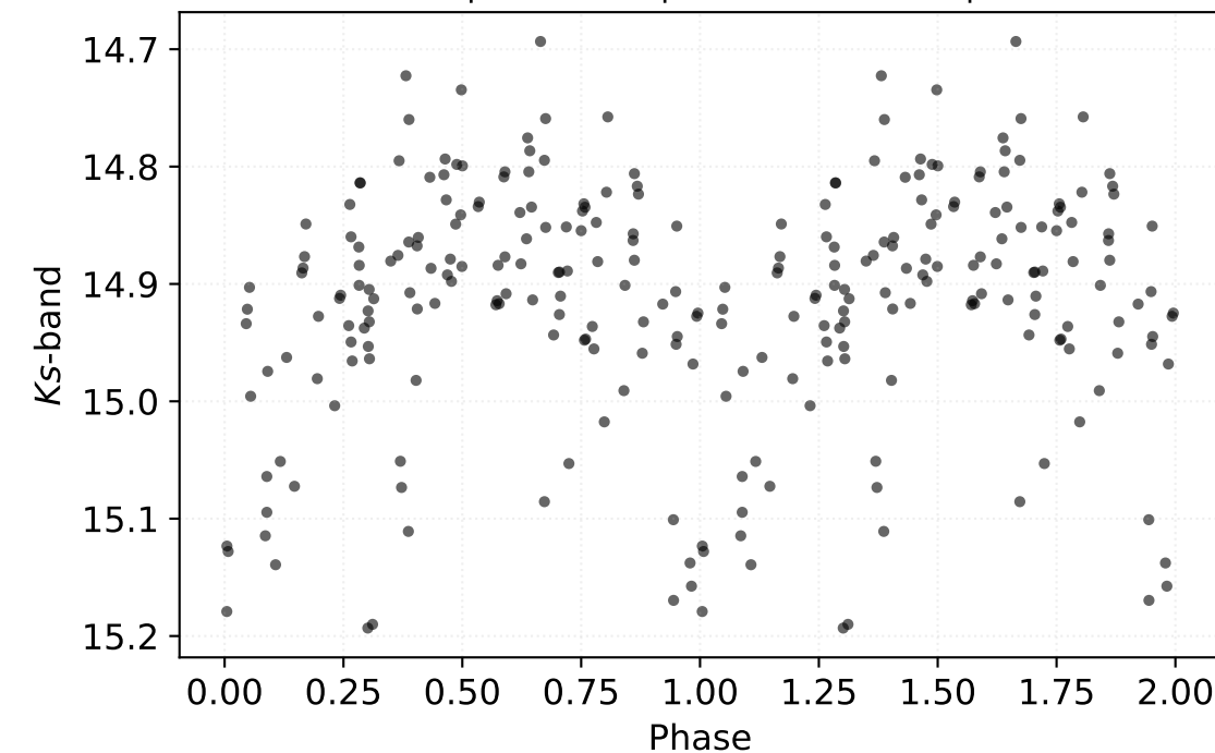
P: 0.11081 d | Class: RP | Subclass: UVAR | Field b278
