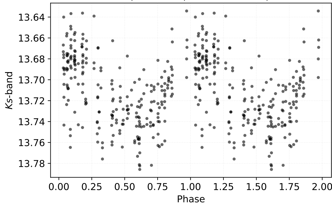
P: 0.16756 d | Class: RP | Subclass: UVAR | Field b279
