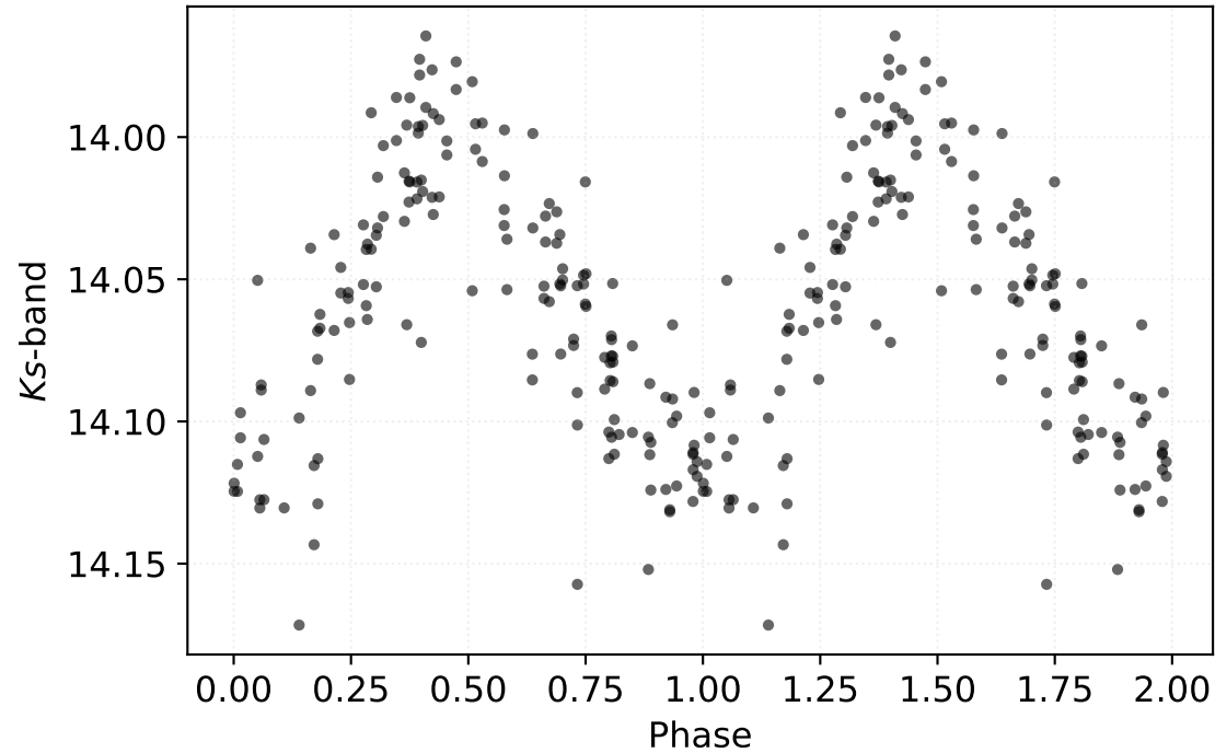
P: 30.17269 d | Class: RP | Subclass: CEP-F | Field b279
