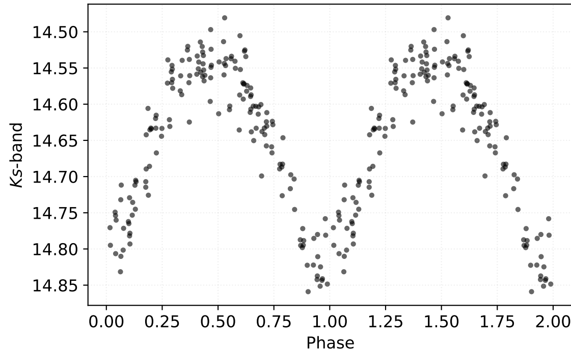
P: 0.20387 d | Class: RP | Subclass: UVAR | Field b279
