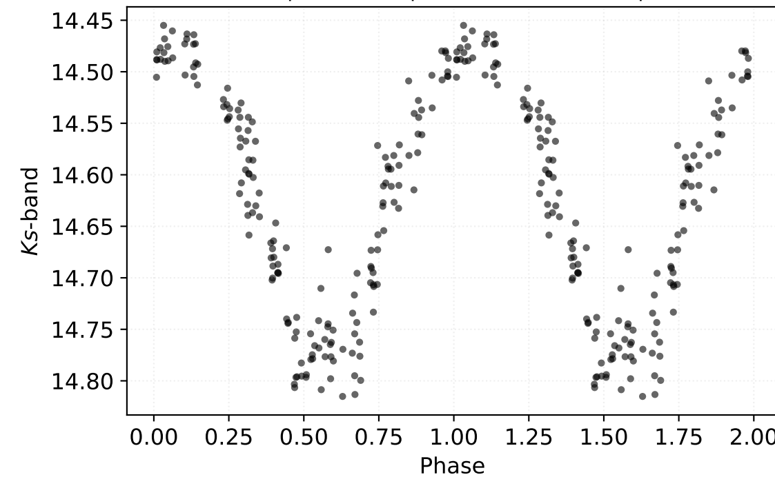
P: 0.64088 d | Class: RP | Subclass: CEP-1OT | Field b278
