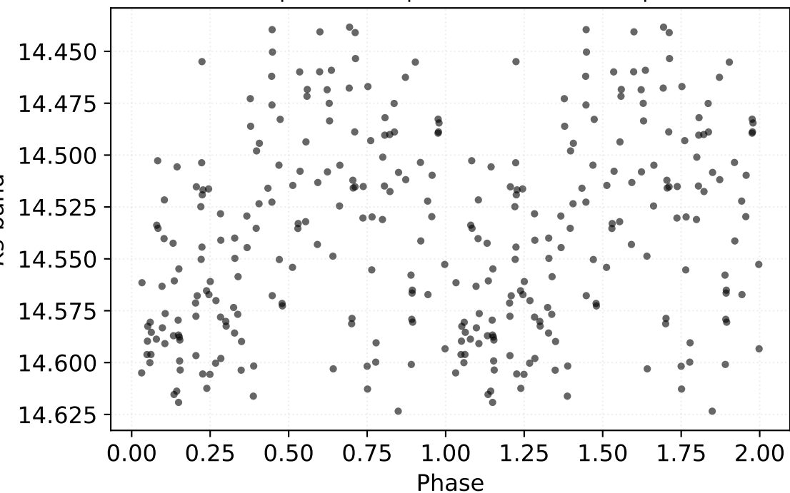
P: 0.67703 d | Class: RP | Subclass: CEP-1OT | Field b278
