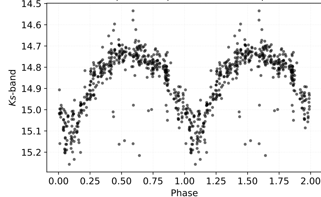
P: 0.30871 d | Class: RP | Subclass: CEP-1OT | Field b278
