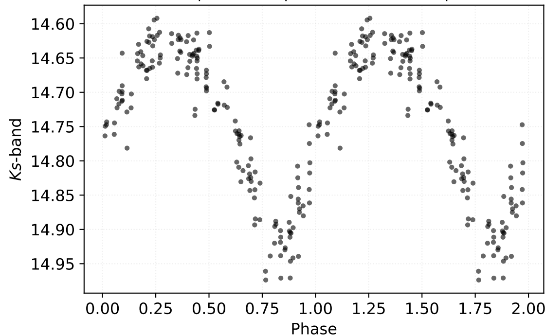
P: 0.31021 d | Class: RP | Subclass: CEP-1OT | Field b279
