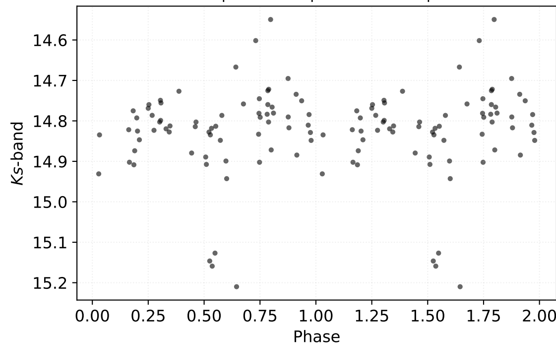
P: 1.73502 d | Class: EB | Subclass: EA | Field b278
