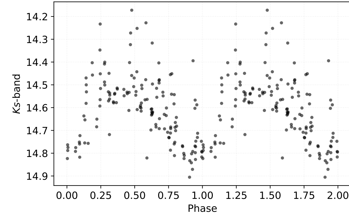
P: 0.40928 d | Class: RP | Subclass: CEP-1OT | Field b279
