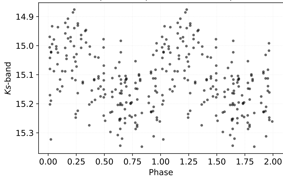
P: 2.18381 d | Class: RP | Subclass: CEP-1OT | Field b278
