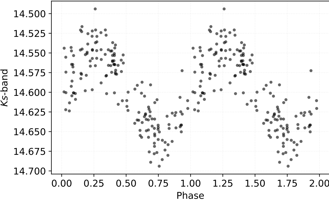
P: 0.36202 d | Class: RP | Subclass: CEP-1OT | Field b278
