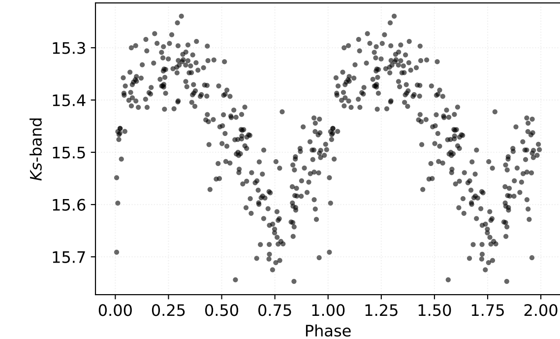
P: 0.30113 d | Class: RP | Subclass: CEP-1OT | Field b278
