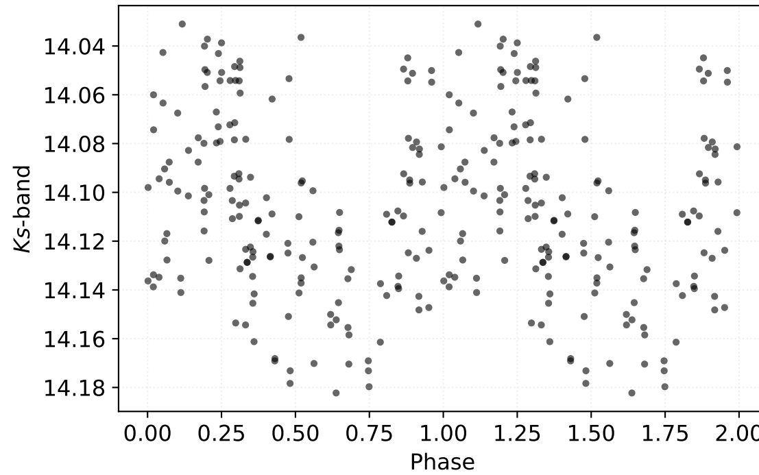
P: 2.34464 d | Class: RP | Subclass: CEP-1OT | Field b279
