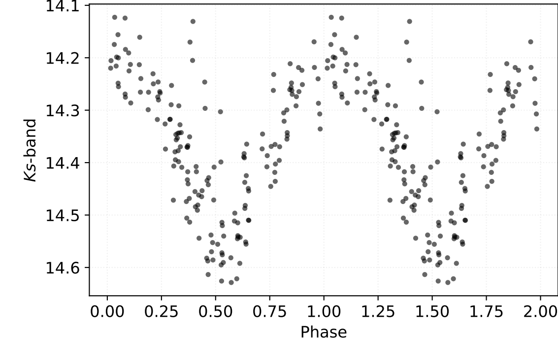
P: 0.24923 d | Class: RP | Subclass: UVAR | Field b279
