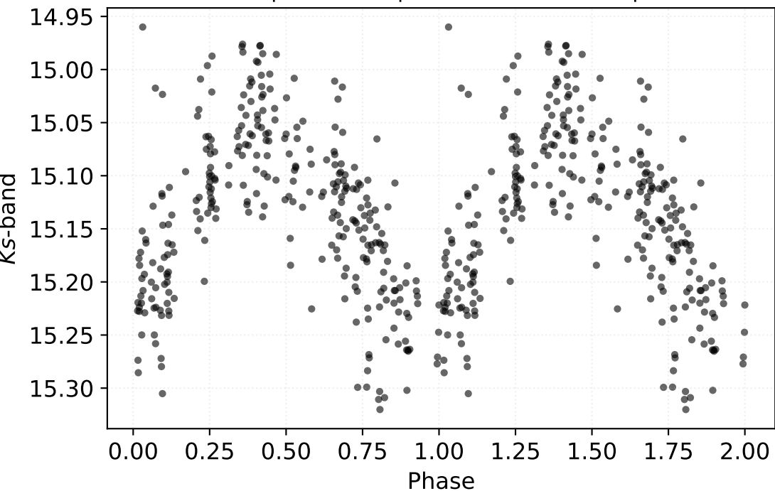
P: 1.06576 d | Class: RP | Subclass: CEP-1OT | Field b279
