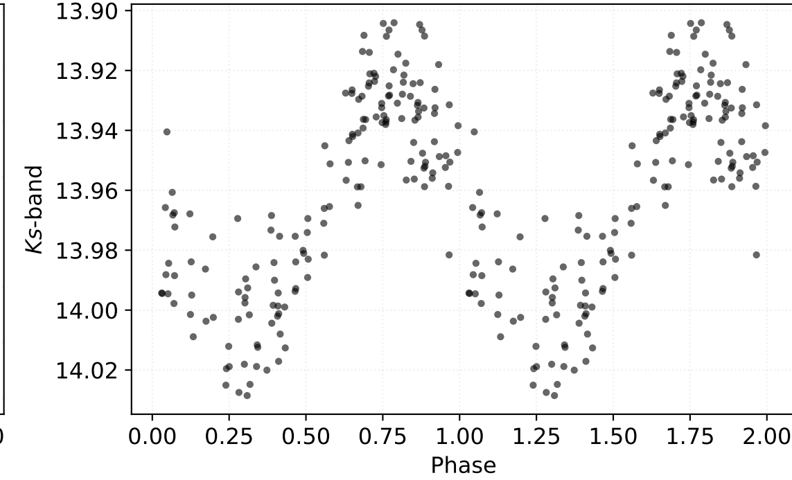
P: 0.45268 d | Class: RP | Subclass: RRc | Field b279
