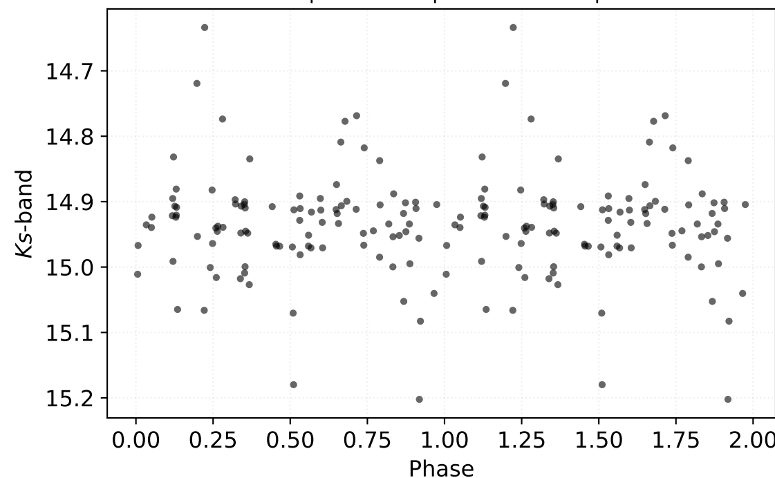
P: 0.70723 d | Class: EB | Subclass: EA | Field b278
