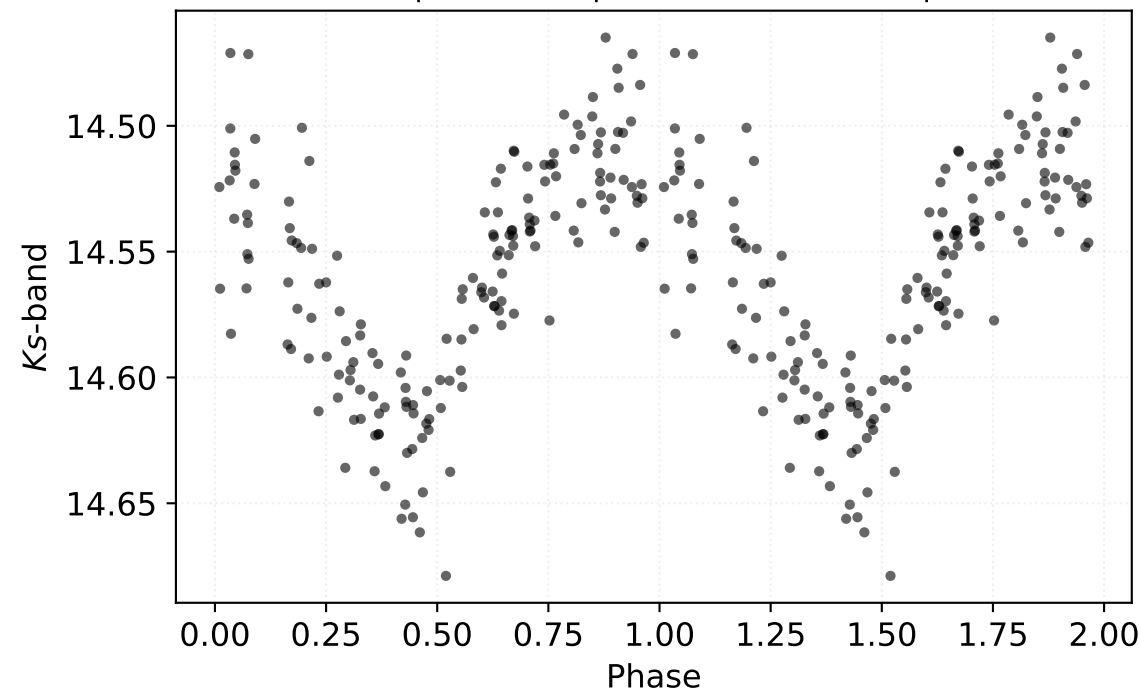
P: 0.45090 d | Class: RP | Subclass: CEP-1OT | Field b279
