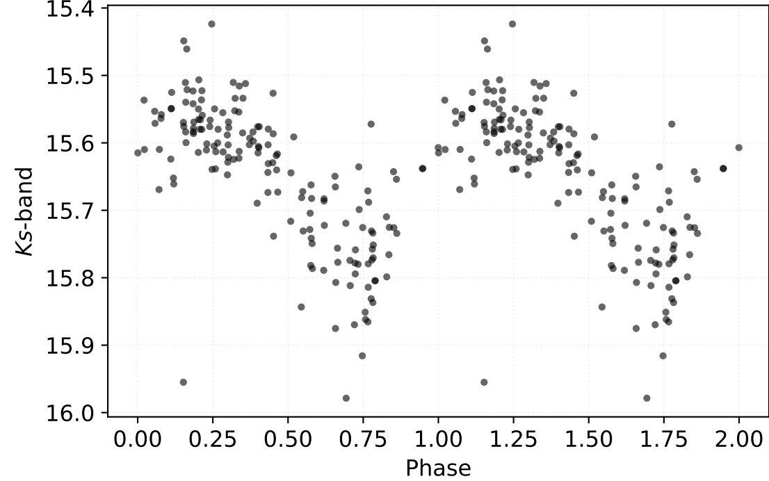
P: 0.33490 d | Class: RP | Subclass: CEP-1OT | Field b278
