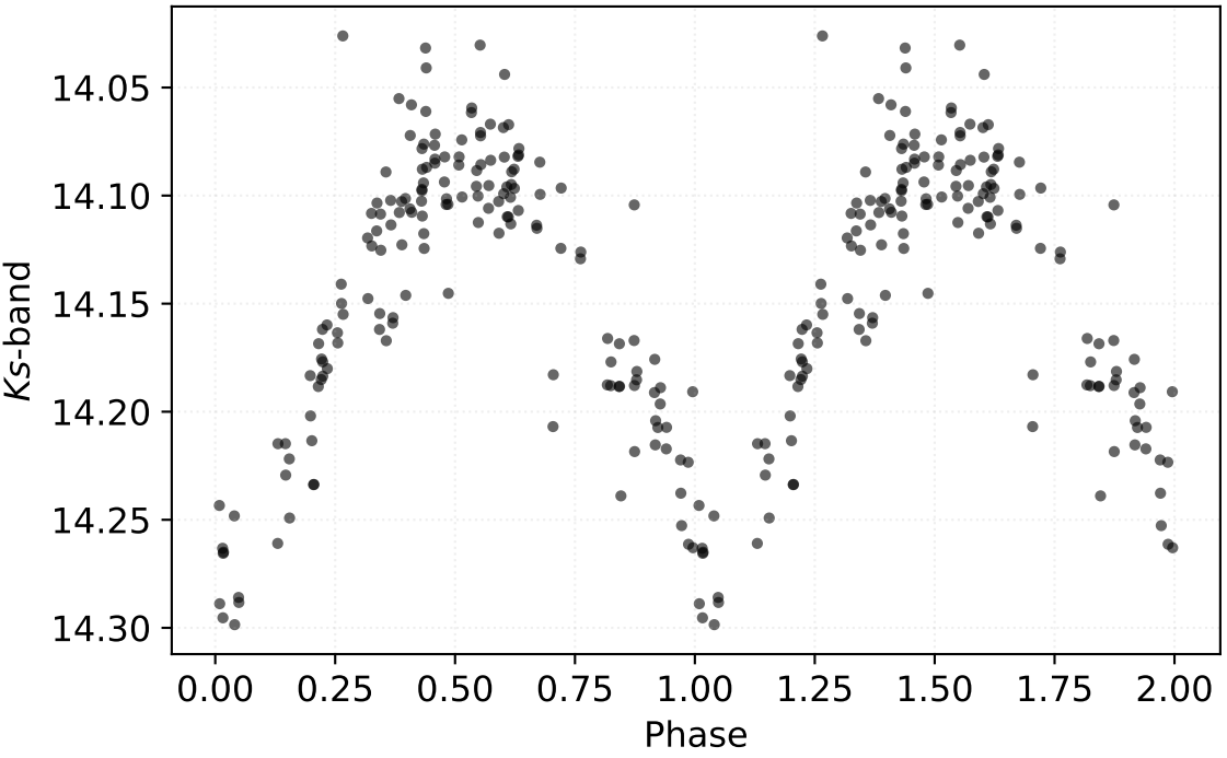
P: 0.60853 d | Class: RP | Subclass: RRab | Field b278
