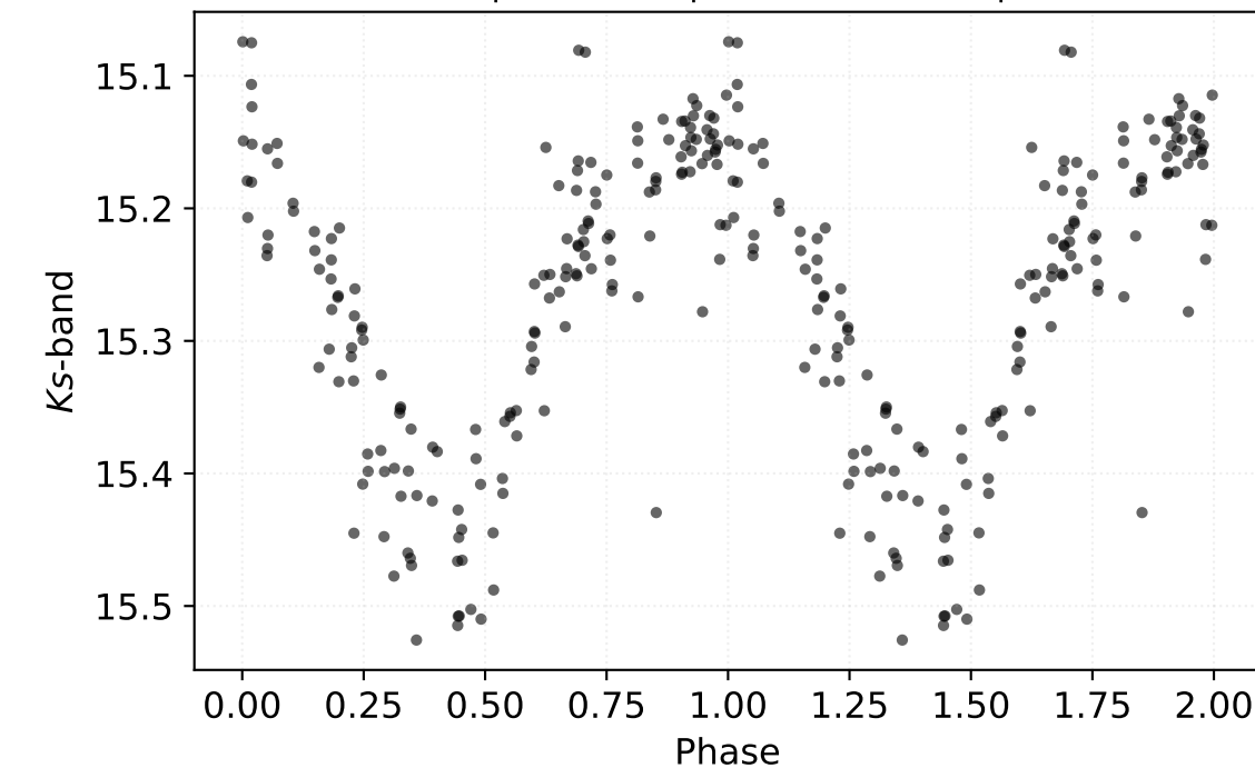
P: 0.37627 d | Class: RP | Subclass: RRab | Field b278
