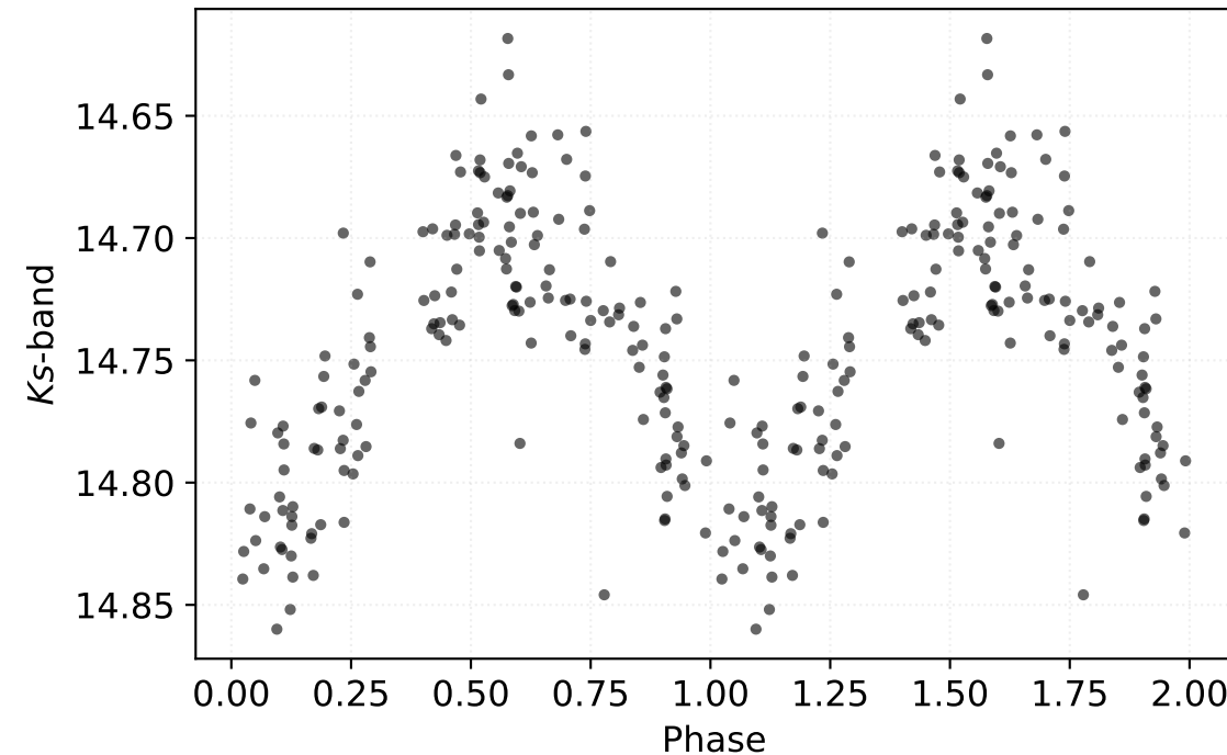
P: 23.91131 d | Class: RP | Subclass: UVAR | Field b279
