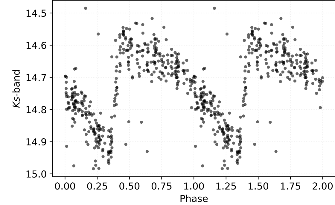
P: 0.59744 d | Class: RP | Subclass: RRab | Field b278
