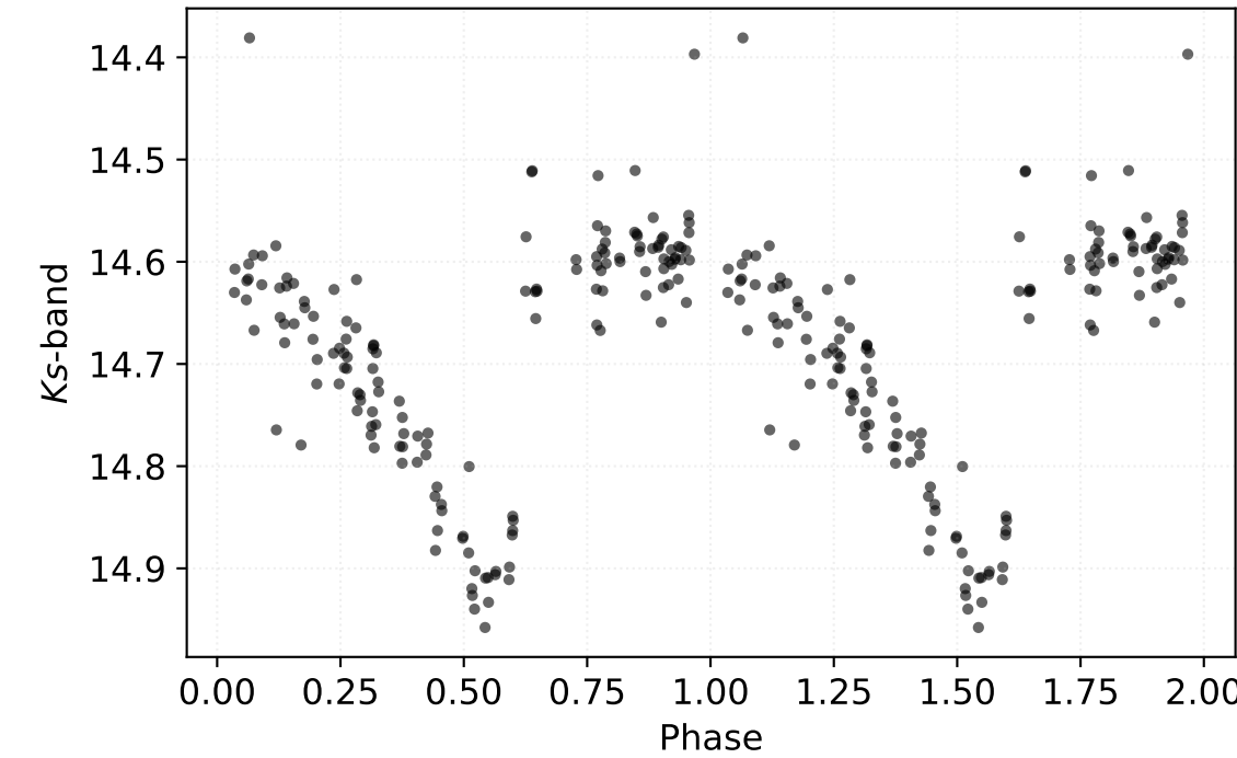
P: 0.53023 d | Class: RP | Subclass: RRab | Field b278
