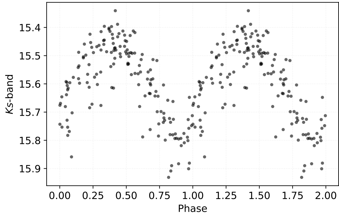
P: 0.22595 d | Class: RP | Subclass: UVAR | Field b279
