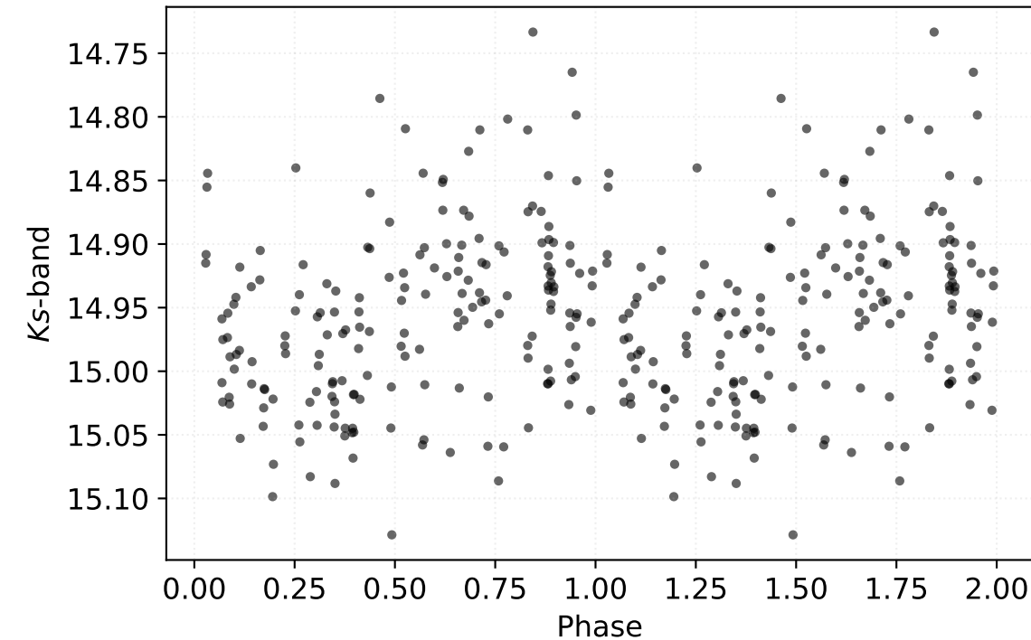
P: 0.42791 d | Class: RP | Subclass: RRc | Field b279
