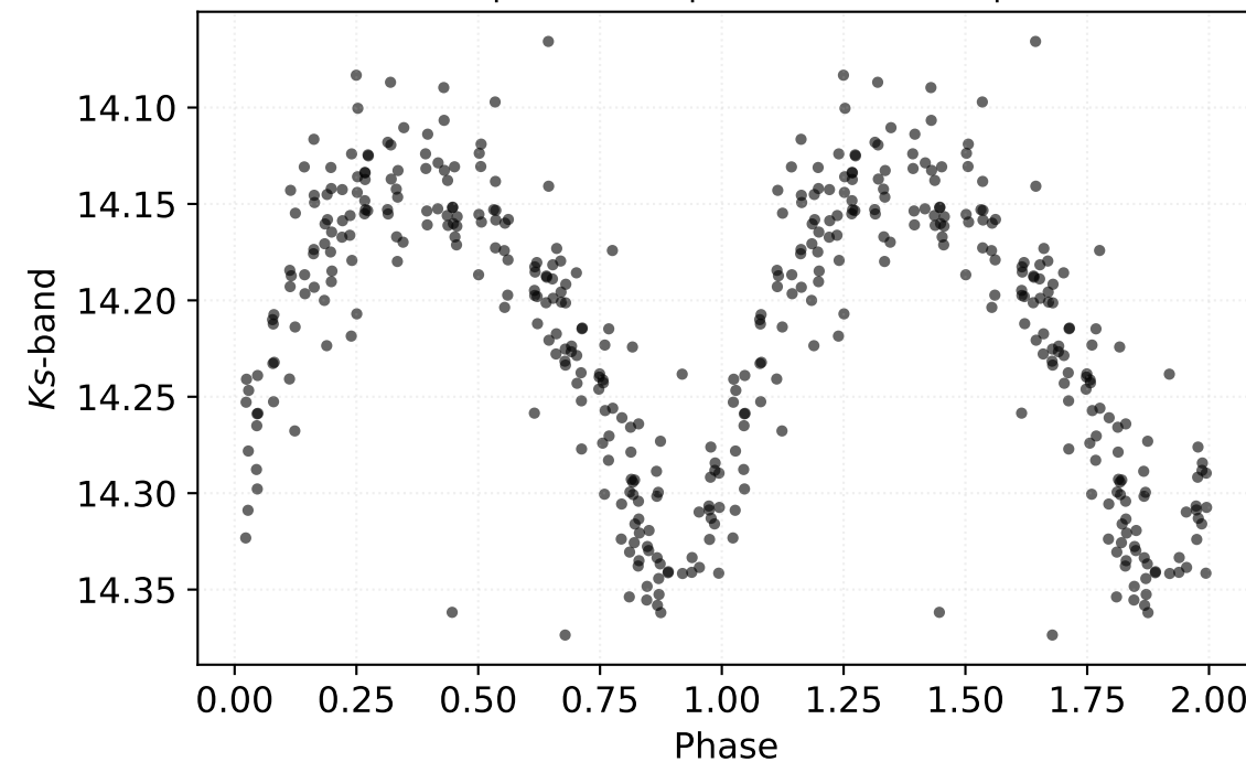
P: 0.40652 d | Class: RP | Subclass: RRab | Field b279
