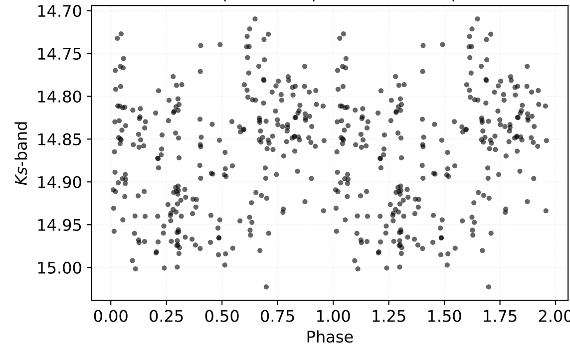
P: 0.10681 d | Class: RP | Subclass: UVAR | Field b278
