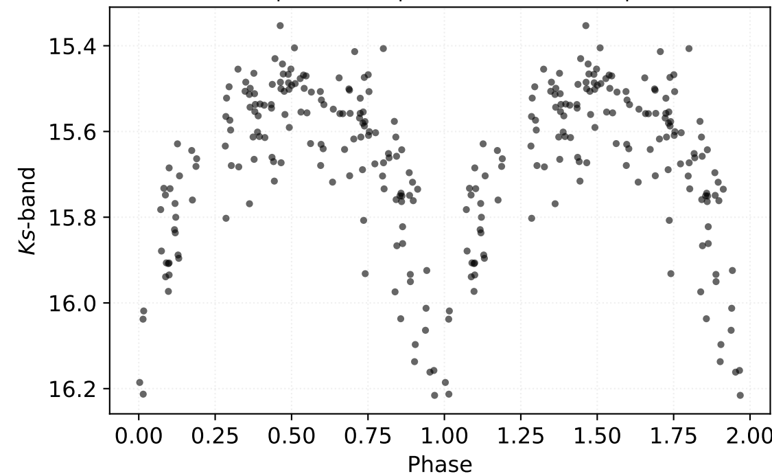
P: 0.26689 d | Class: RP | Subclass: CEP-1OT | Field b278
