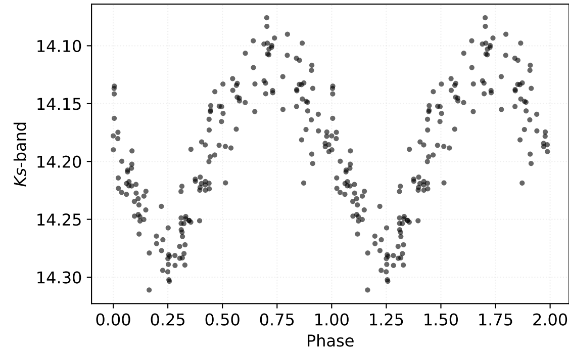
P: 2.66945 d | Class: RP | Subclass: CEP-1OT | Field b278
