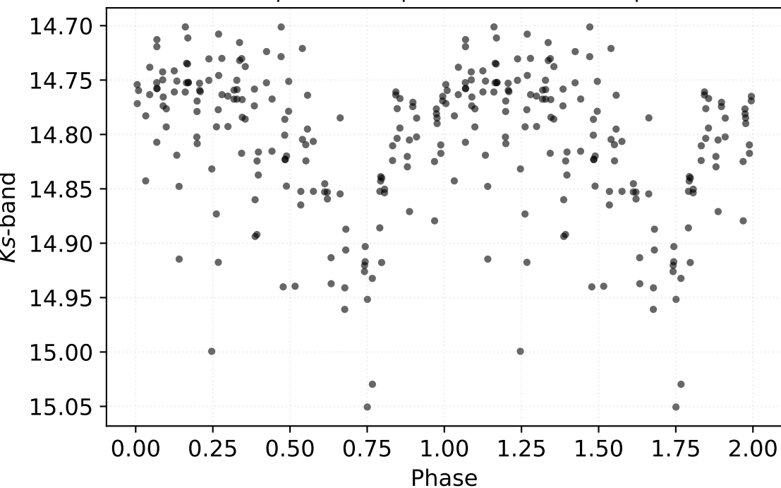
P: 4.80695 d | Class: RP | Subclass: CEP-1OT | Field b278
