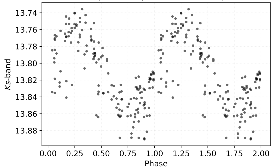
P: 0.67826 d | Class: RP | Subclass: CEP-1OT | Field b279
