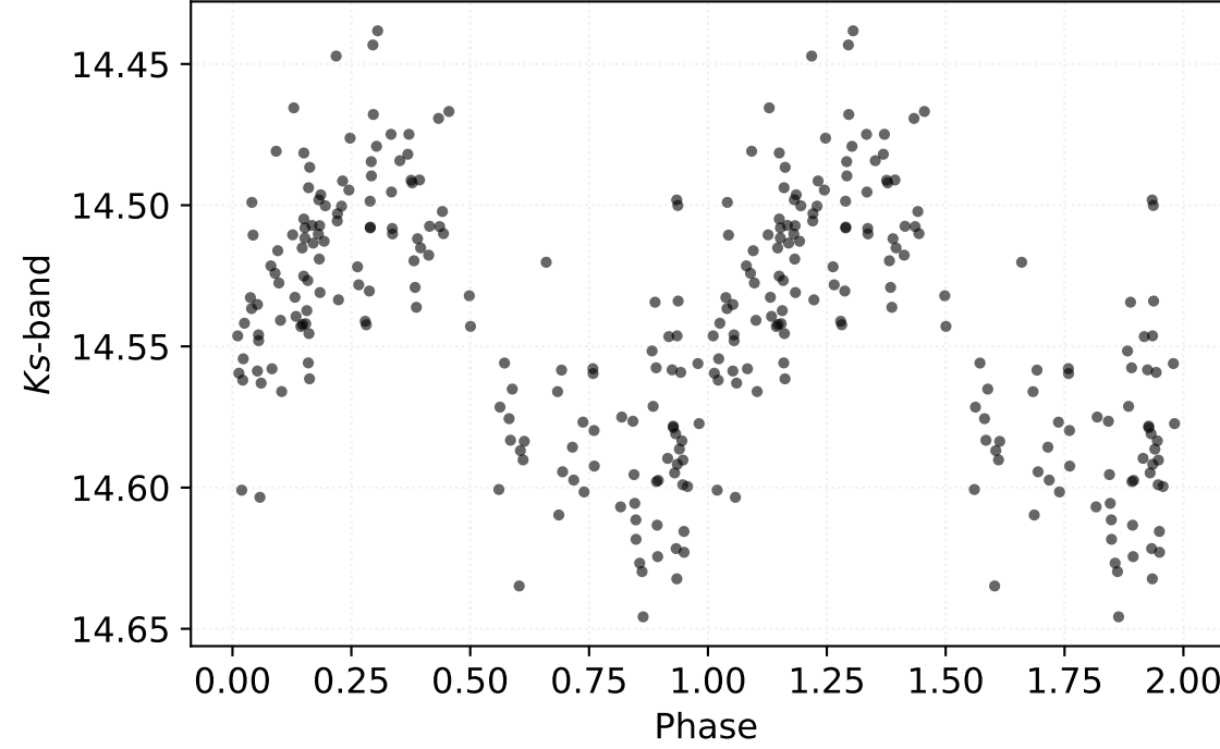
P: 0.50435 d | Class: RP | Subclass: RRab | Field b278
