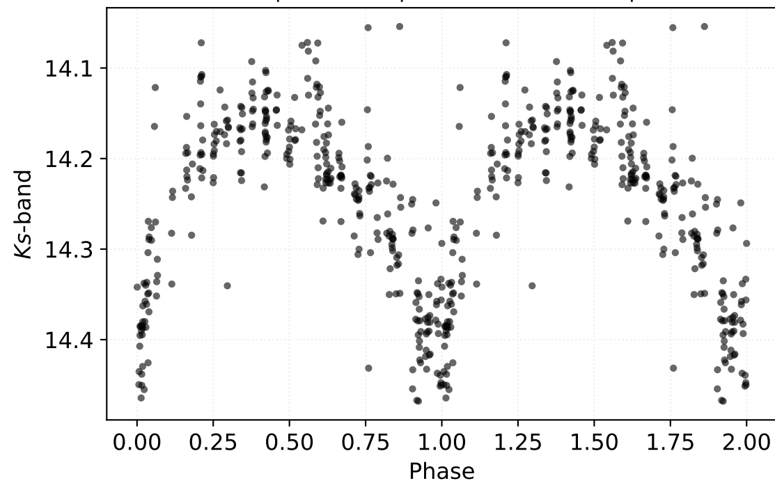
P: 1.19211 d | Class: RP | Subclass: CEP-1OT | Field b278
