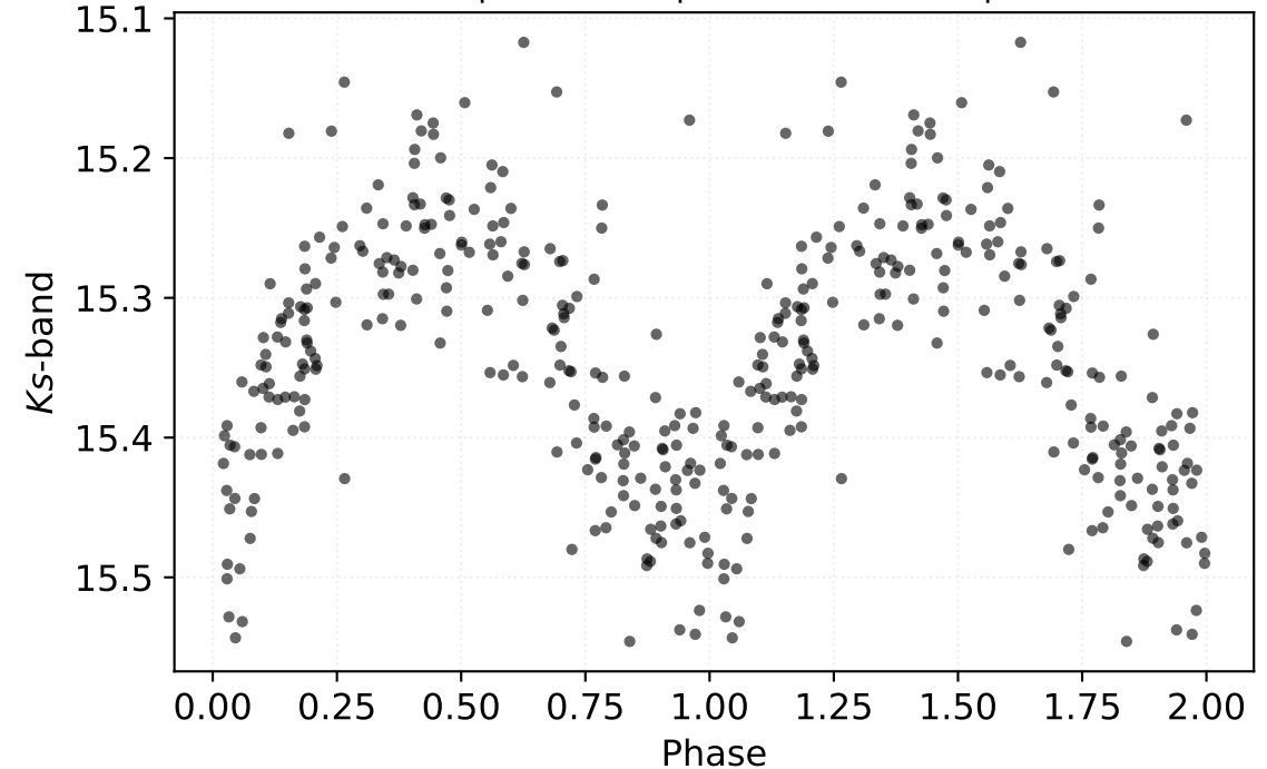
P: 0.49795 d | Class: RP | Subclass: RRab | Field b279
