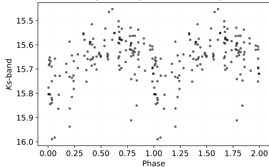
P: 0.87881 d | Class: RP | Subclass: CEP-1OT | Field b278
