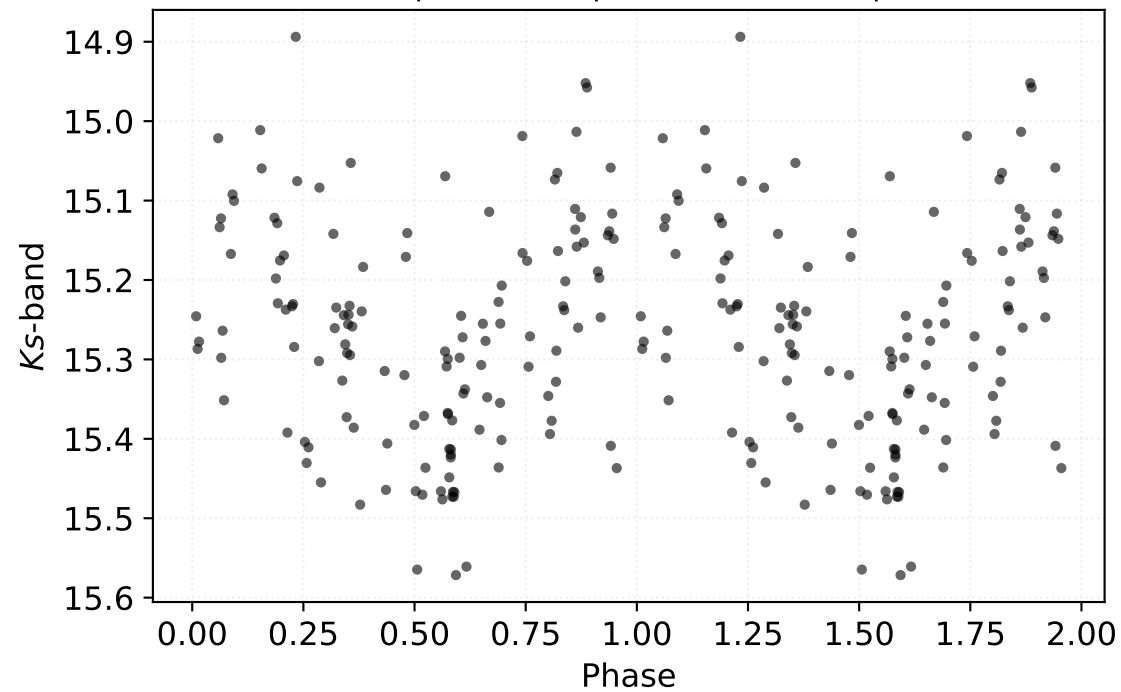
P: 0.11081 d | Class: RP | Subclass: UVAR | Field b279
