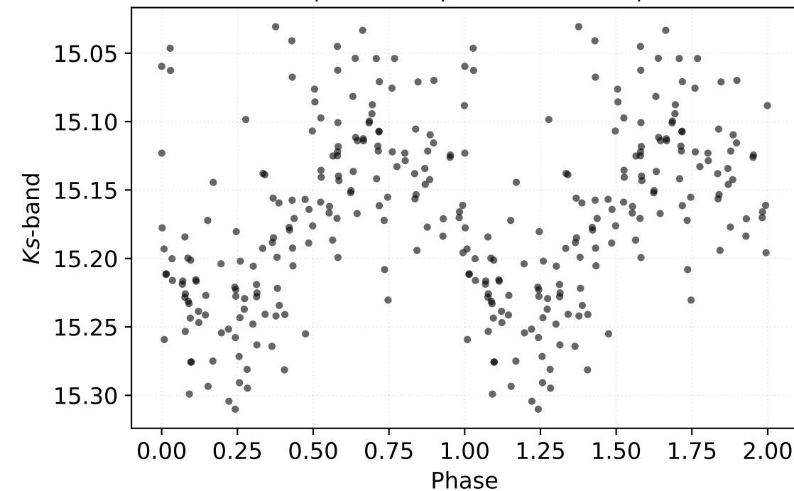
P: 0.51429 d | Class: RP | Subclass: RRab | Field b278
