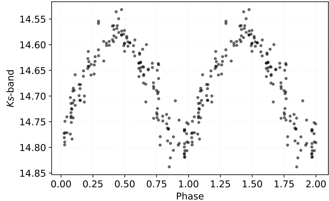
P: 0.68405 d | Class: RP | Subclass: RRab | Field b278
