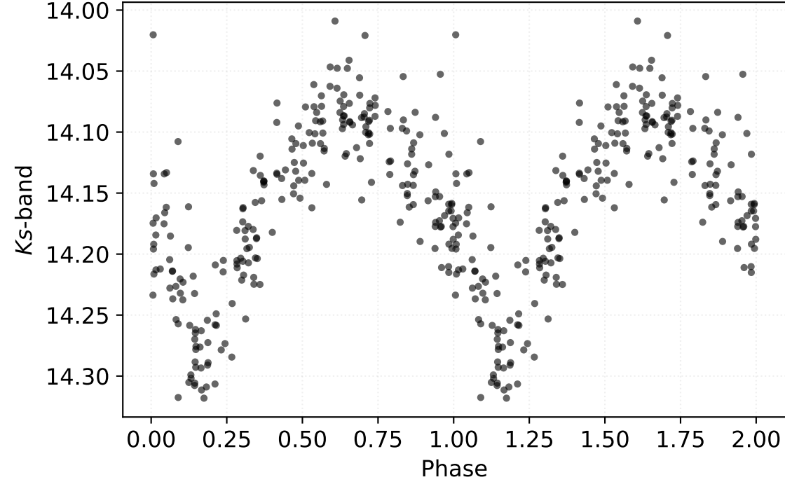
P: 0.33553 d | Class: RP | Subclass: RRab | Field b278
