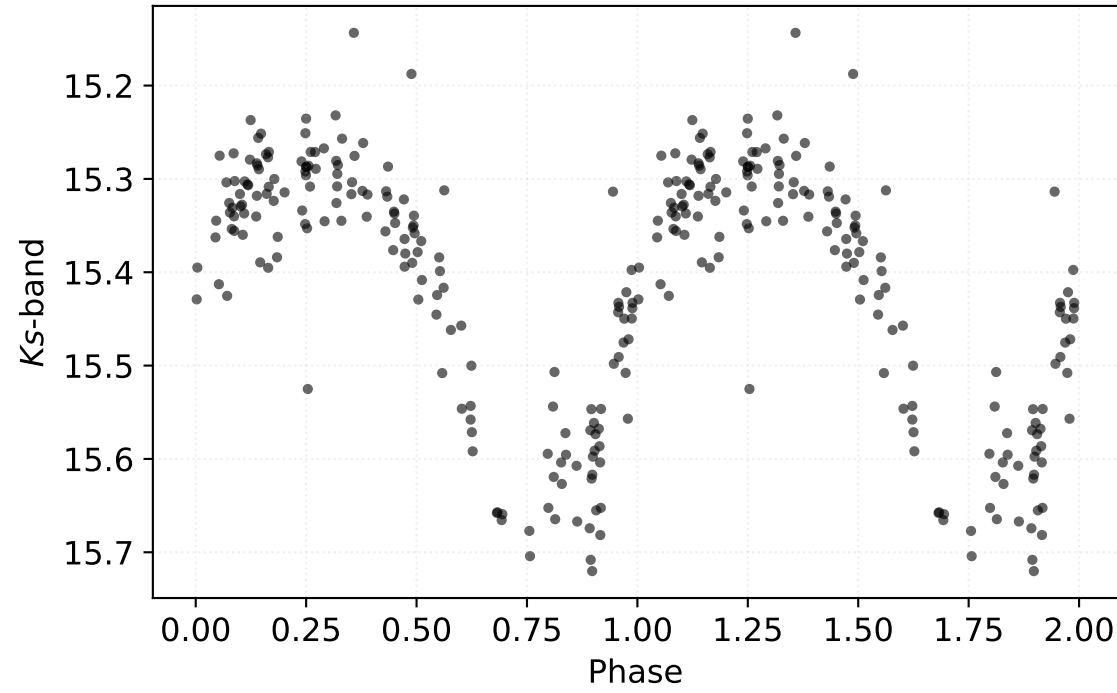
P: 10.51731 d | Class: EB | Subclass: UVAR | Field b278
