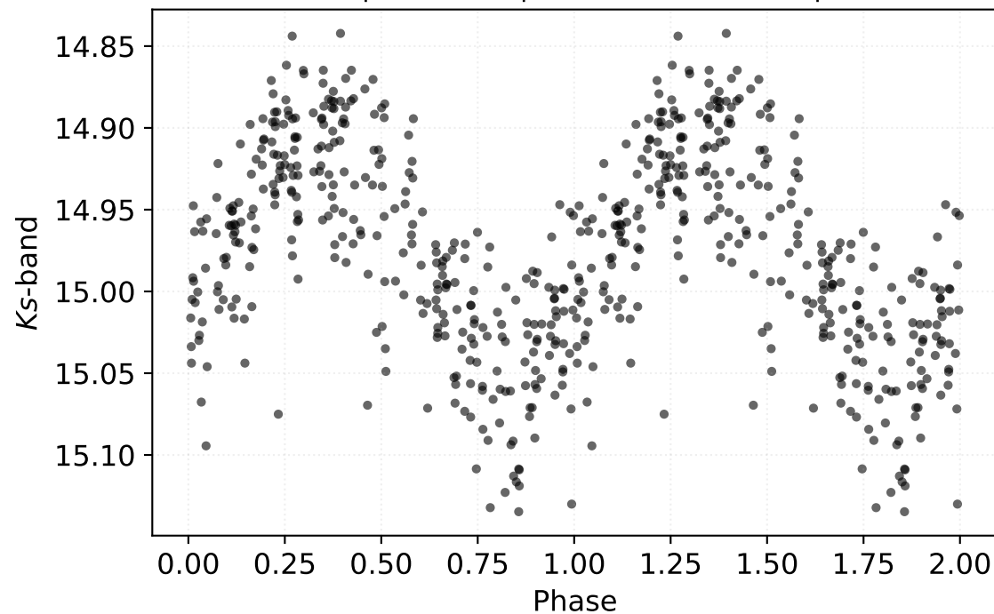
P: 0.37004 d | Class: RP | Subclass: CEP-1OT | Field b278
