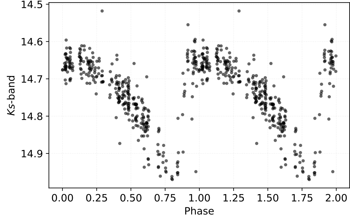
P: 0.55401 d | Class: RP | Subclass: RRab | Field b278
