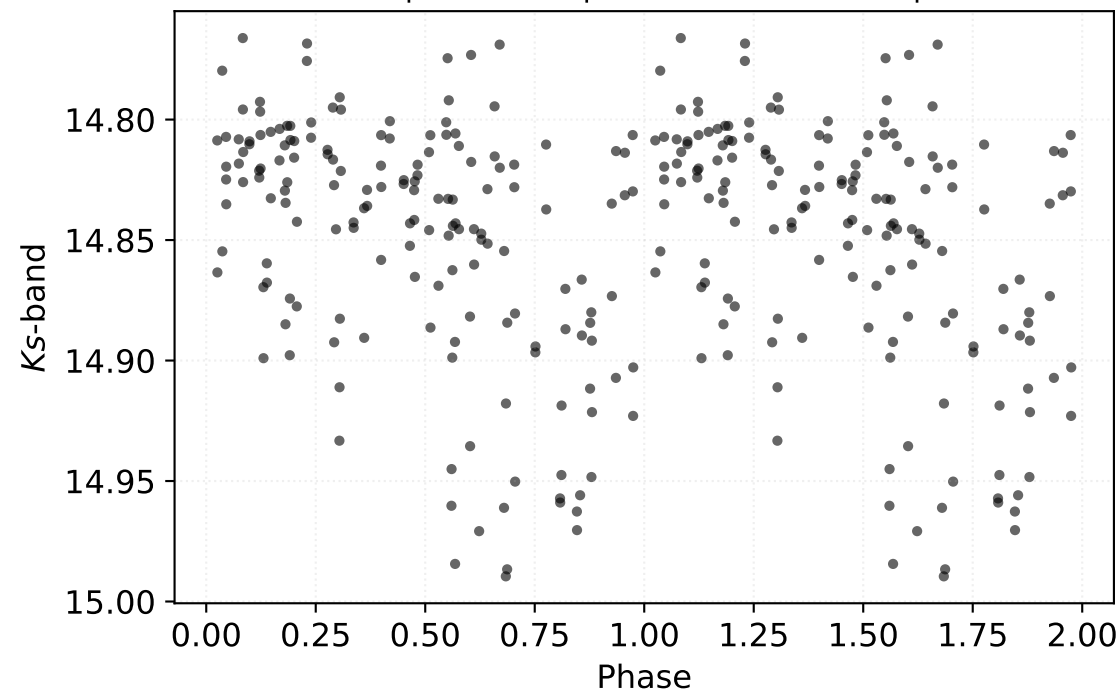
P: 0.77655 d | Class: RP | Subclass: CEP-1OT | Field b279
