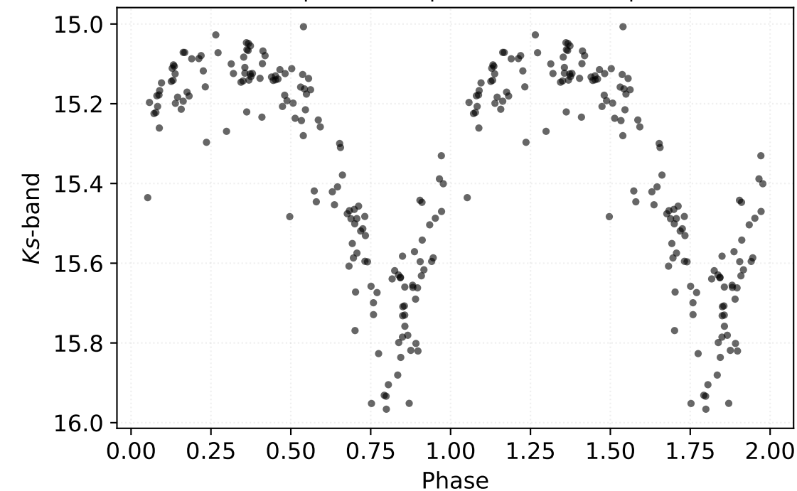
P: 0.19336 d | Class: RP | Subclass: UVAR | Field b279
