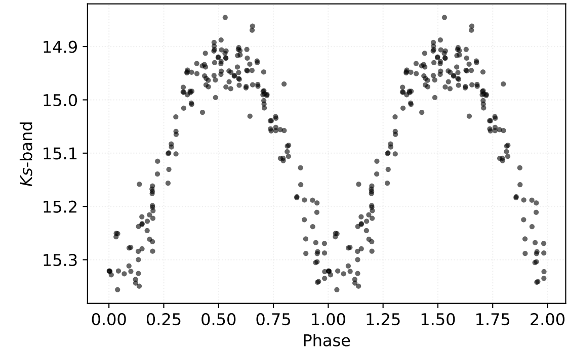
P: 0.58087 d | Class: RP | Subclass: CEP-1OT | Field b279
