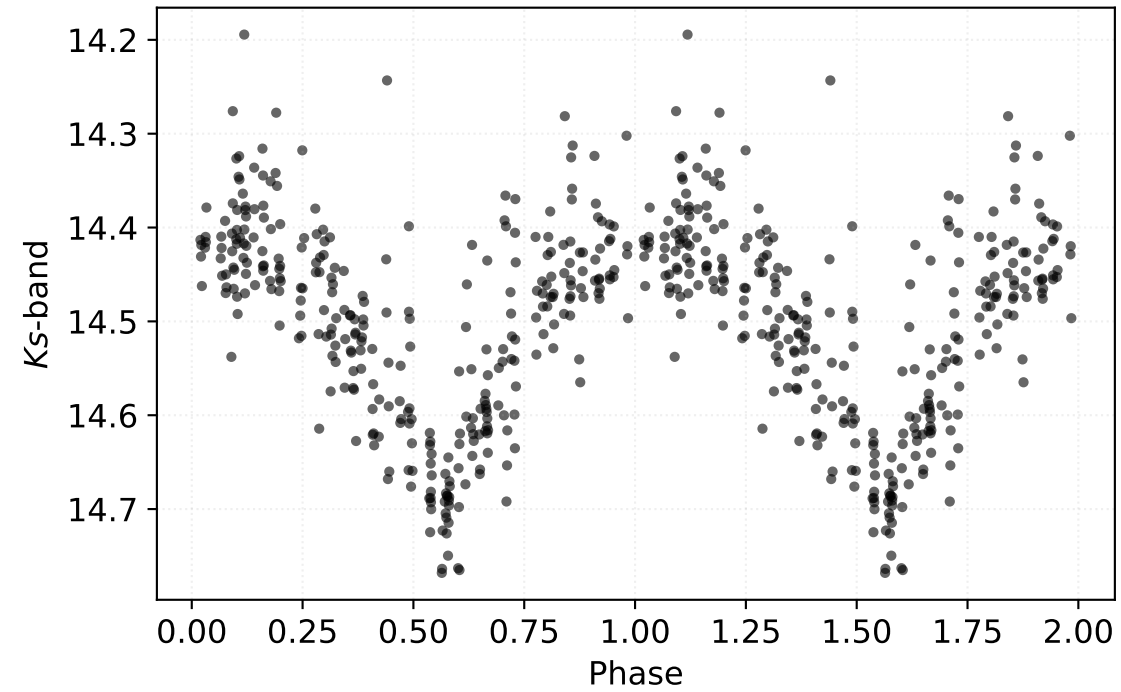
P: 0.61945 d | Class: RP | Subclass: RRab | Field b278
