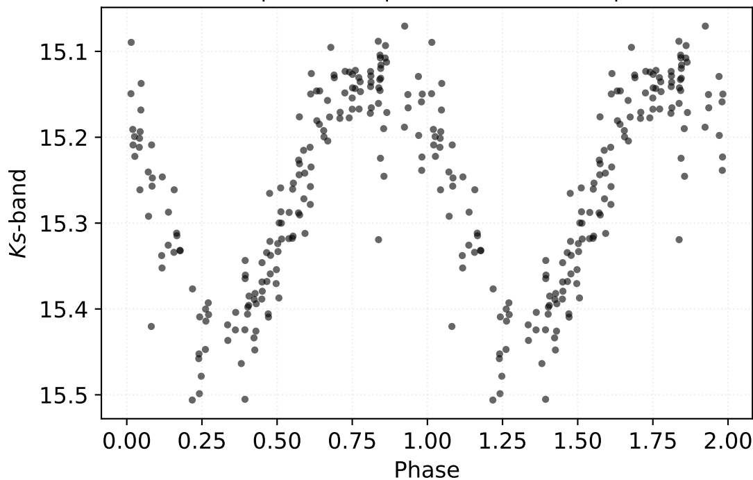
P: 0.29872 d | Class: RP | Subclass: CEP-1OT | Field b278
