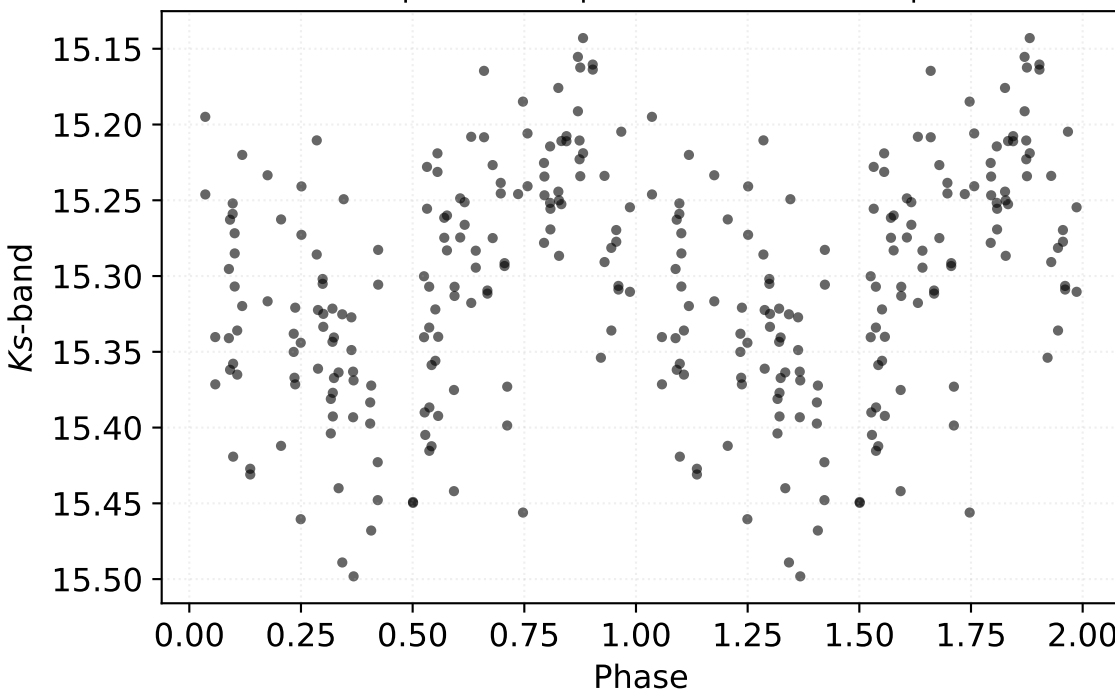
P: 0.32794 d | Class: RP | Subclass: CEP-1OT | Field b278
