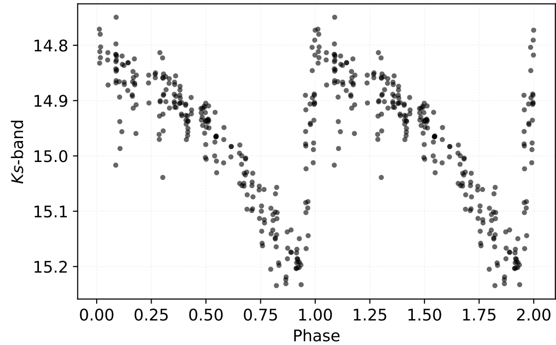
P: 0.44166 d | Class: RP | Subclass: RRab | Field b278
