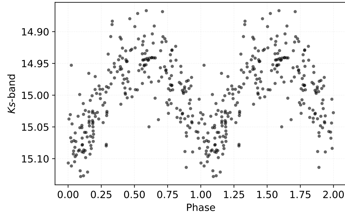
P: 0.28632 d | Class: RP | Subclass: UVAR | Field b279
