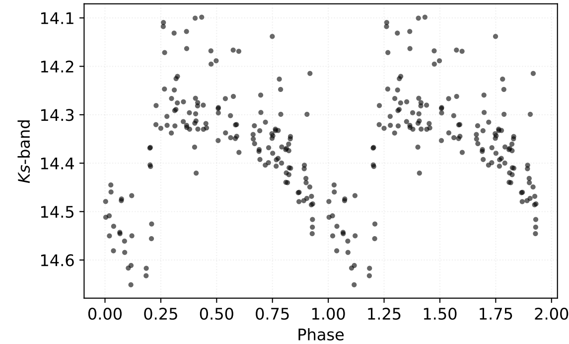
P: 0.56508 d | Class: RP | Subclass: RRab | Field b279
