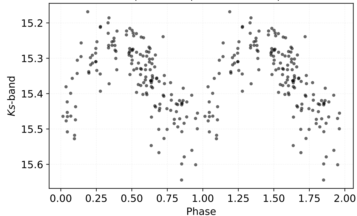
P: 0.65428 d | Class: RP | Subclass: RRab | Field b279
