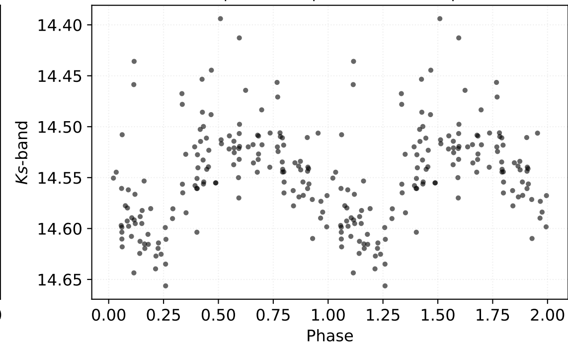
P: 0.16972 d | Class: RP | Subclass: UVAR | Field b279
