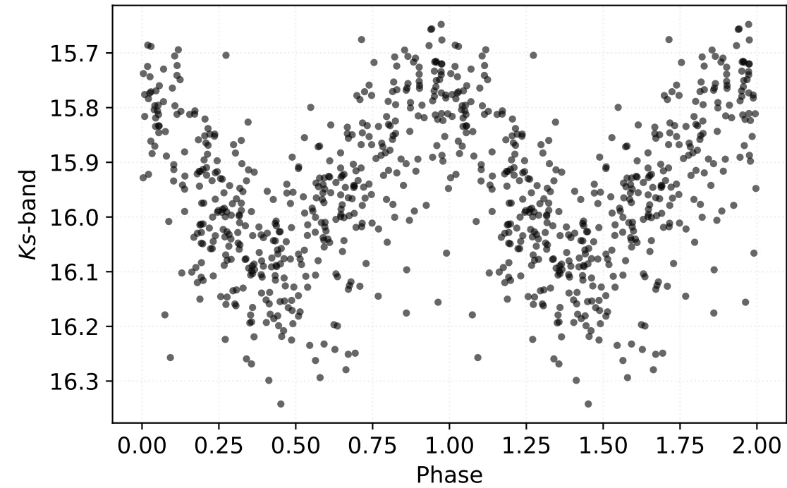
P: 5.04349 d | Class: RP | Subclass: CEP-F | Field b279
