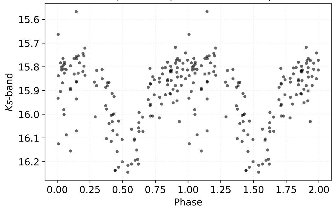
P: 0.78511 d | Class: RP | Subclass: CEP-1OT | Field b278
