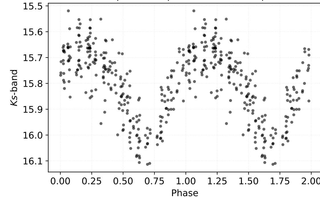
P: 1.92394 d | Class: RP | Subclass: CEP-1OT | Field b278
