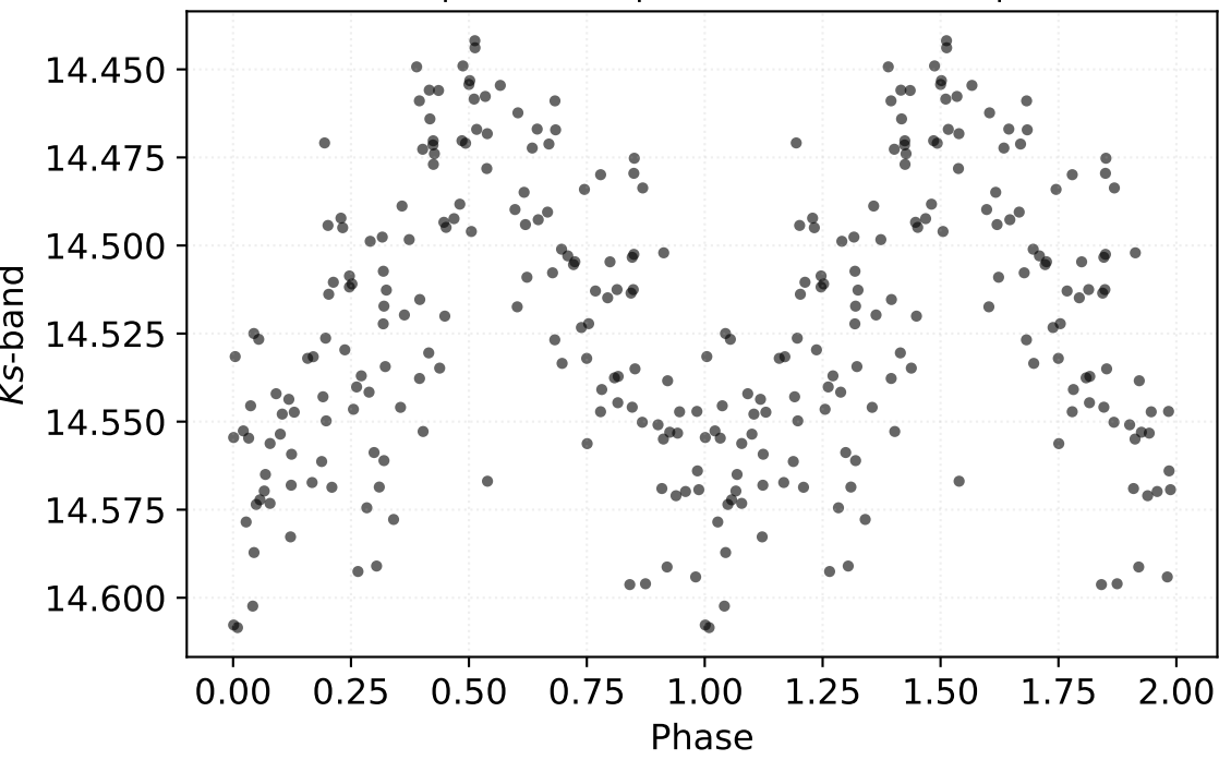
P: 0.42483 d | Class: RP | Subclass: CEP-1OT | Field b278
