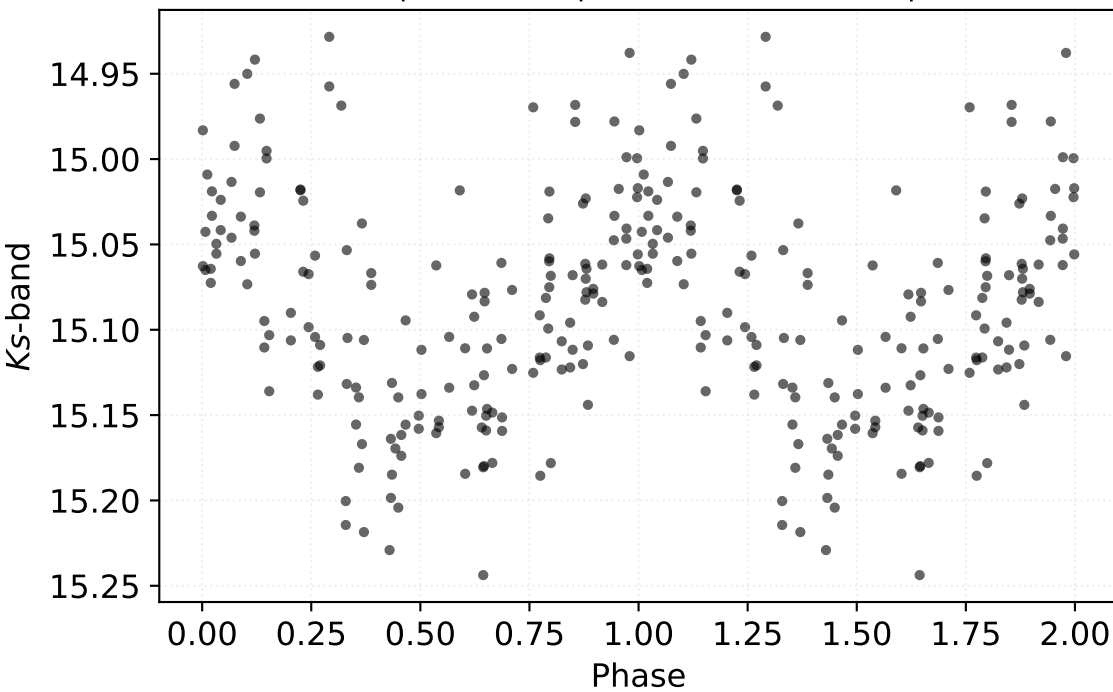
P: 3.21834 d | Class: RP | Subclass: CEP-1OT | Field b278
