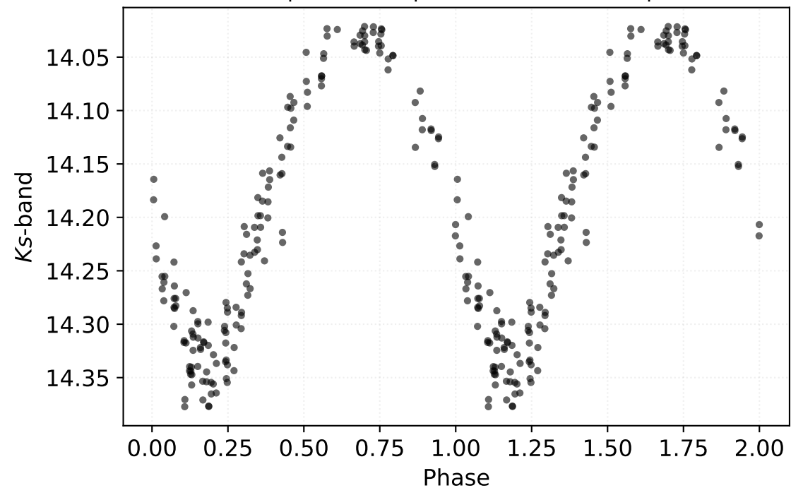
P: 0.29664 d | Class: RP | Subclass: CEP-1OT | Field b278
