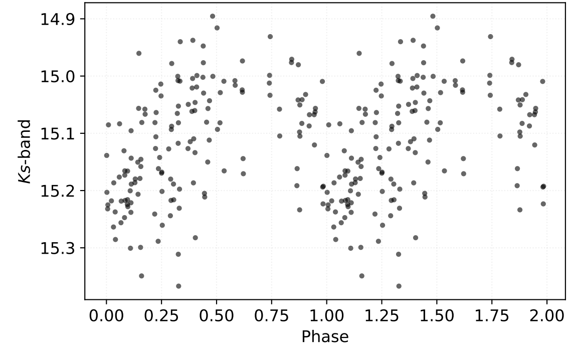
P: 0.32354 d | Class: RP | Subclass: RRab | Field b279
