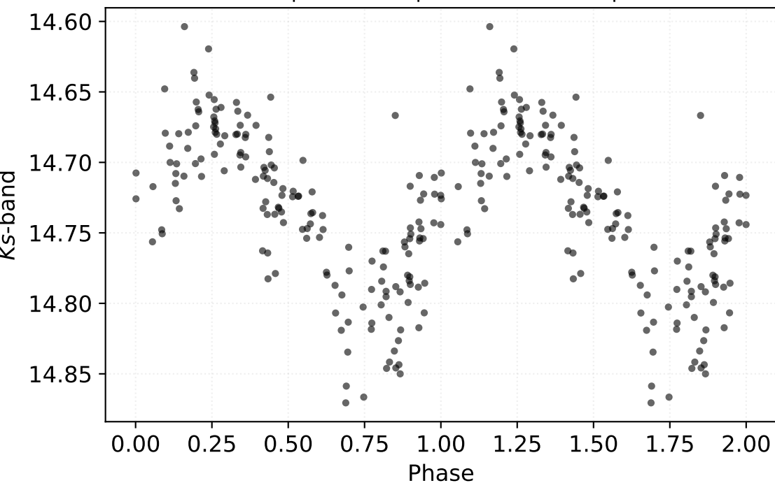
P: 0.26408 d | Class: RP | Subclass: UVAR | Field b279
