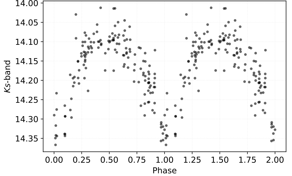
P: 0.60281 d | Class: RP | Subclass: RRab | Field b279
