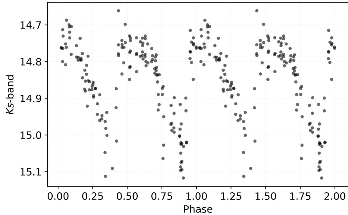
P: 0.25732 d | Class: RP | Subclass: UVAR | Field b278
