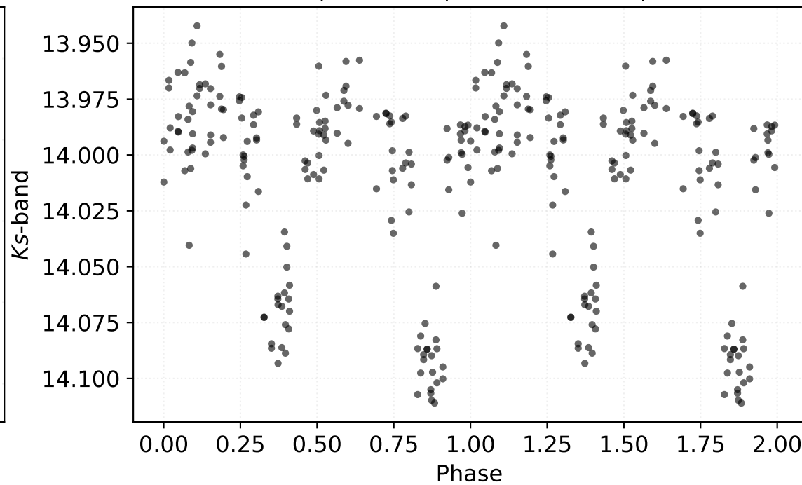
P: 18.98830 d | Class: RP | Subclass: UVAR | Field b279
