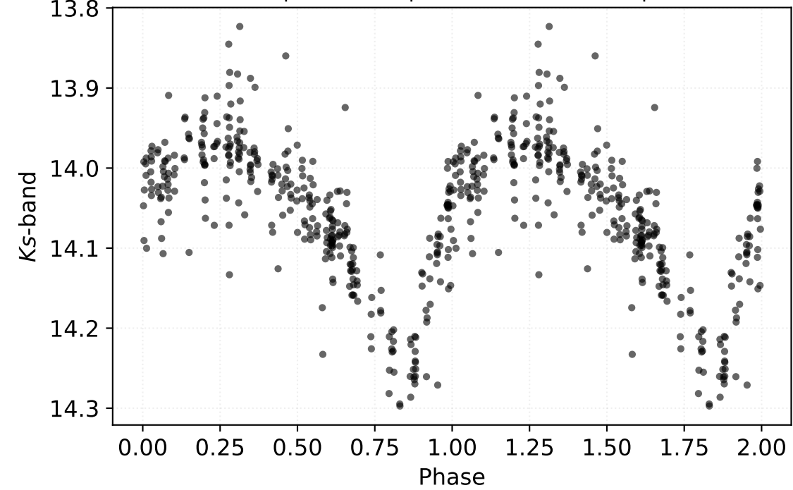
P: 0.52181 d | Class: RP | Subclass: CEP-1OT | Field b278
