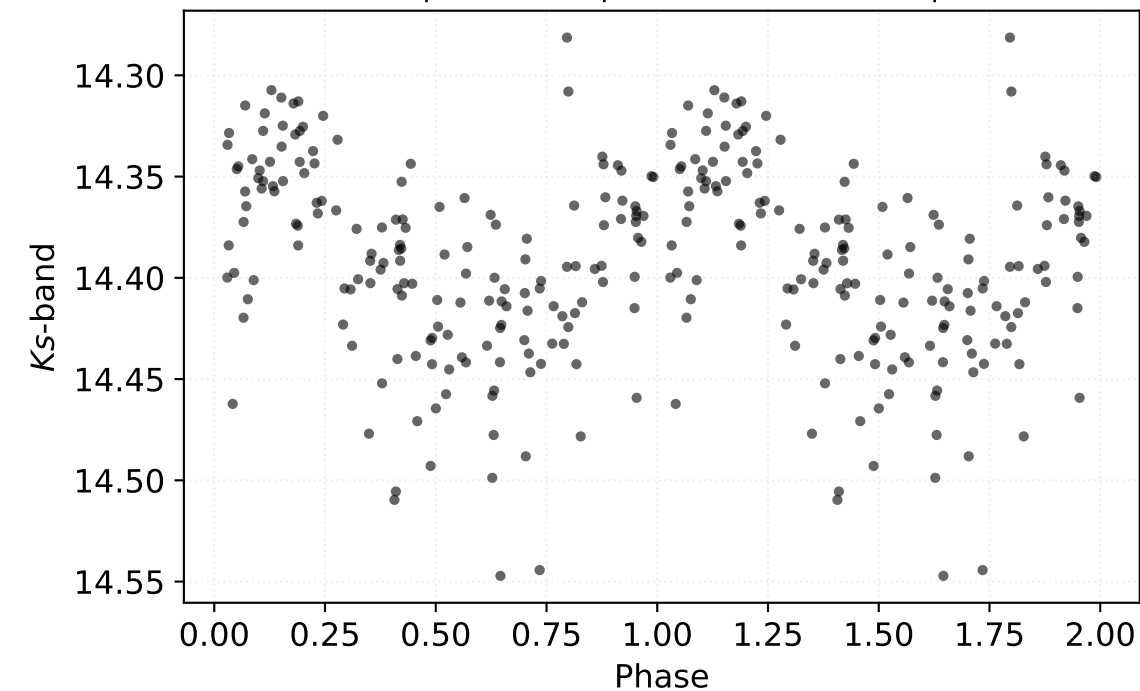
P: 0.70211 d | Class: RP | Subclass: CEP-1OT | Field b279
