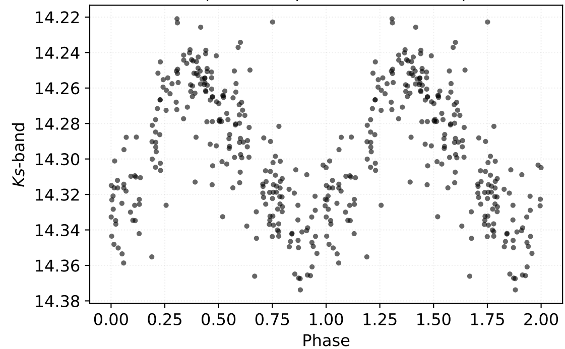
P: 0.25403 d | Class: RP | Subclass: CEP-1OT | Field b278
