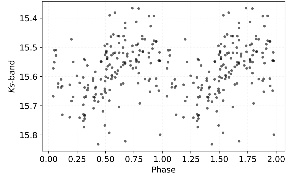
P: 1.02283 d | Class: RP | Subclass: CEP-F | Field b279
