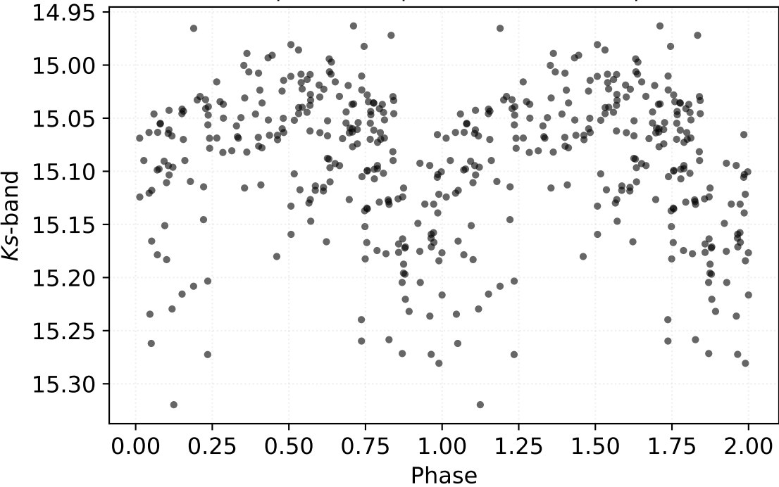
P: 0.75808 d | Class: RP | Subclass: CEP-1OT | Field b278
