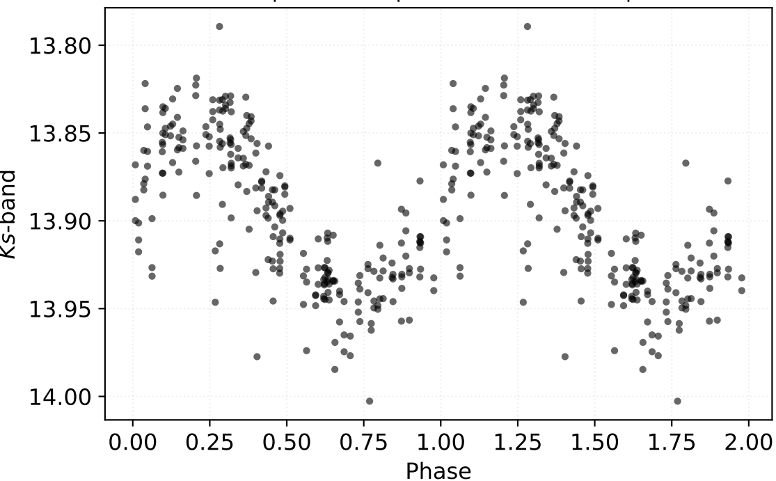
P: 0.53010 d | Class: RP | Subclass: CEP-1OT | Field b278
