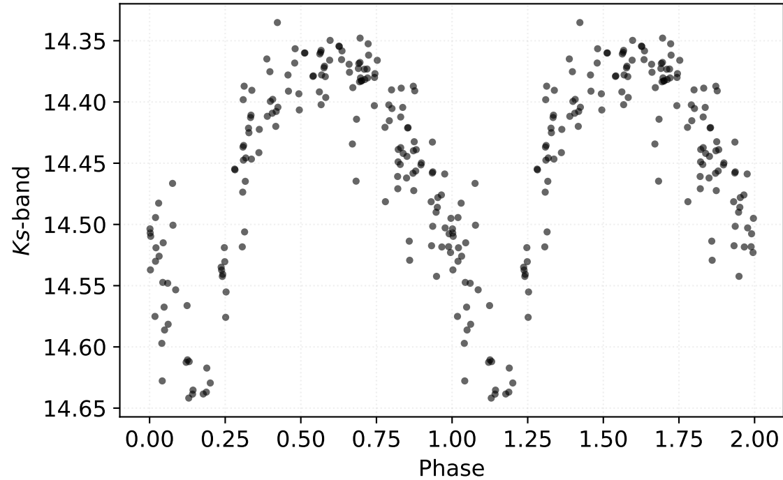
P: 0.32333 d | Class: RP | Subclass: CEP-1OT | Field b278
