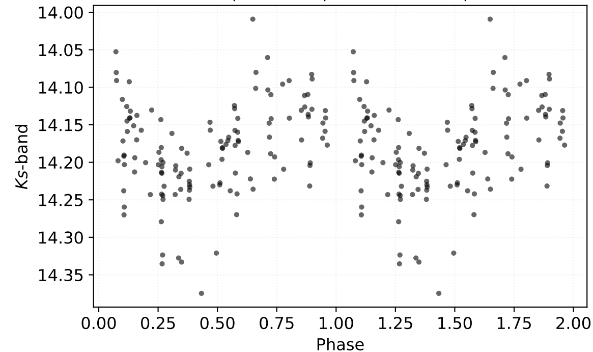
P: 0.52094 d | Class: RP | Subclass: RRab | Field b279
