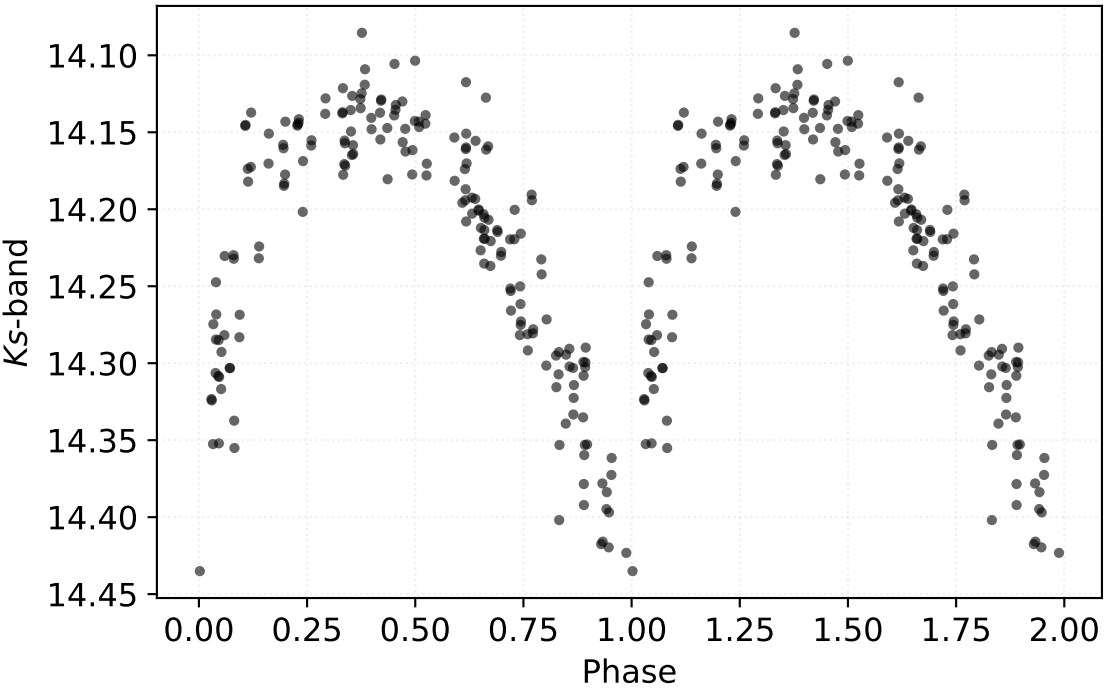
P: 0.87550 d | Class: RP | Subclass: CEP-1OT | Field b278
