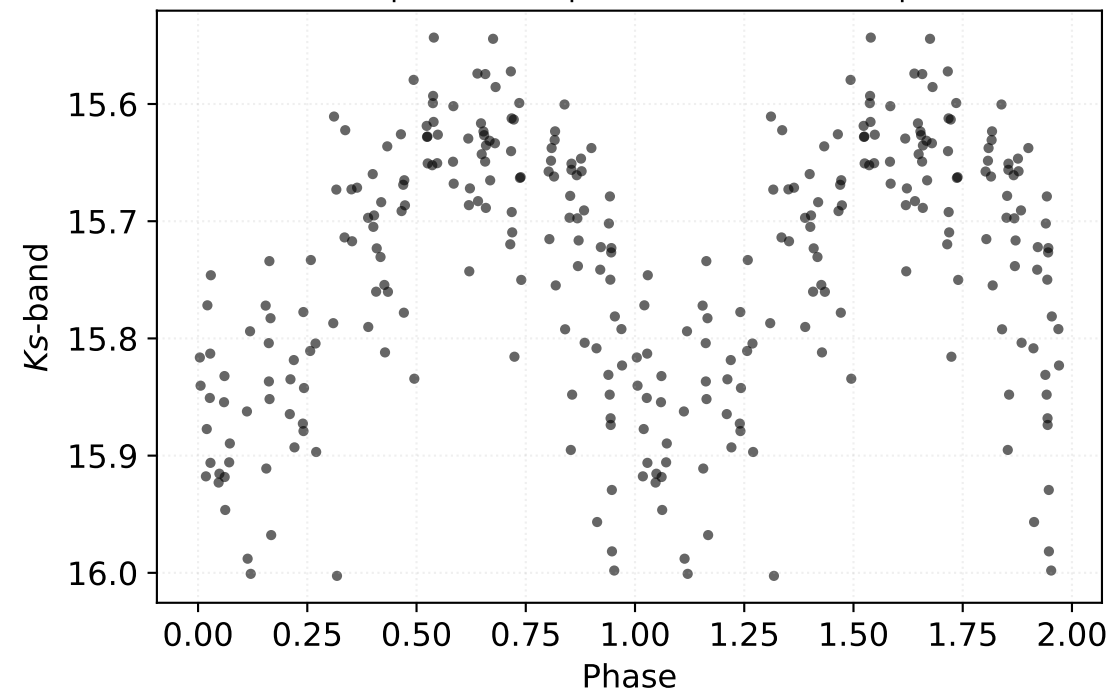
P: 0.57722 d | Class: RP | Subclass: CEP-1OT | Field b278
