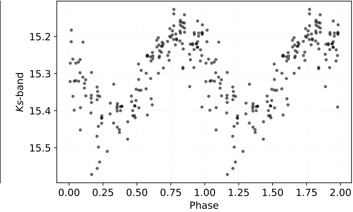
P: 0.37970 d | Class: RP | Subclass: CEP-1OT | Field b279
