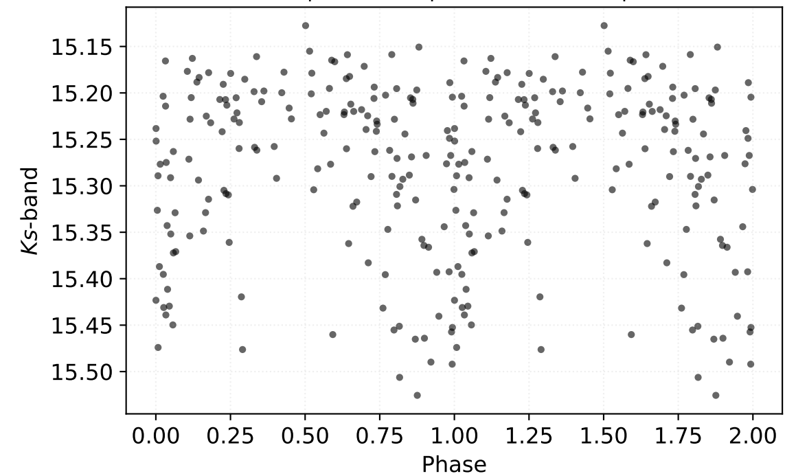
P: 0.17611 d | Class: RP | Subclass: UVAR | Field b278
