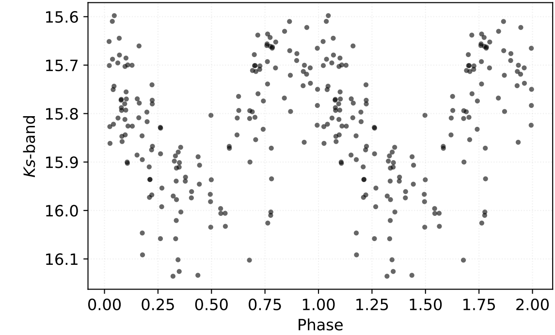
P: 0.50997 d | Class: RP | Subclass: RRab | Field b279
