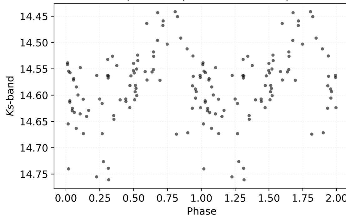
P: 0.28942 d | Class: RP | Subclass: CEP-1OT | Field b279
