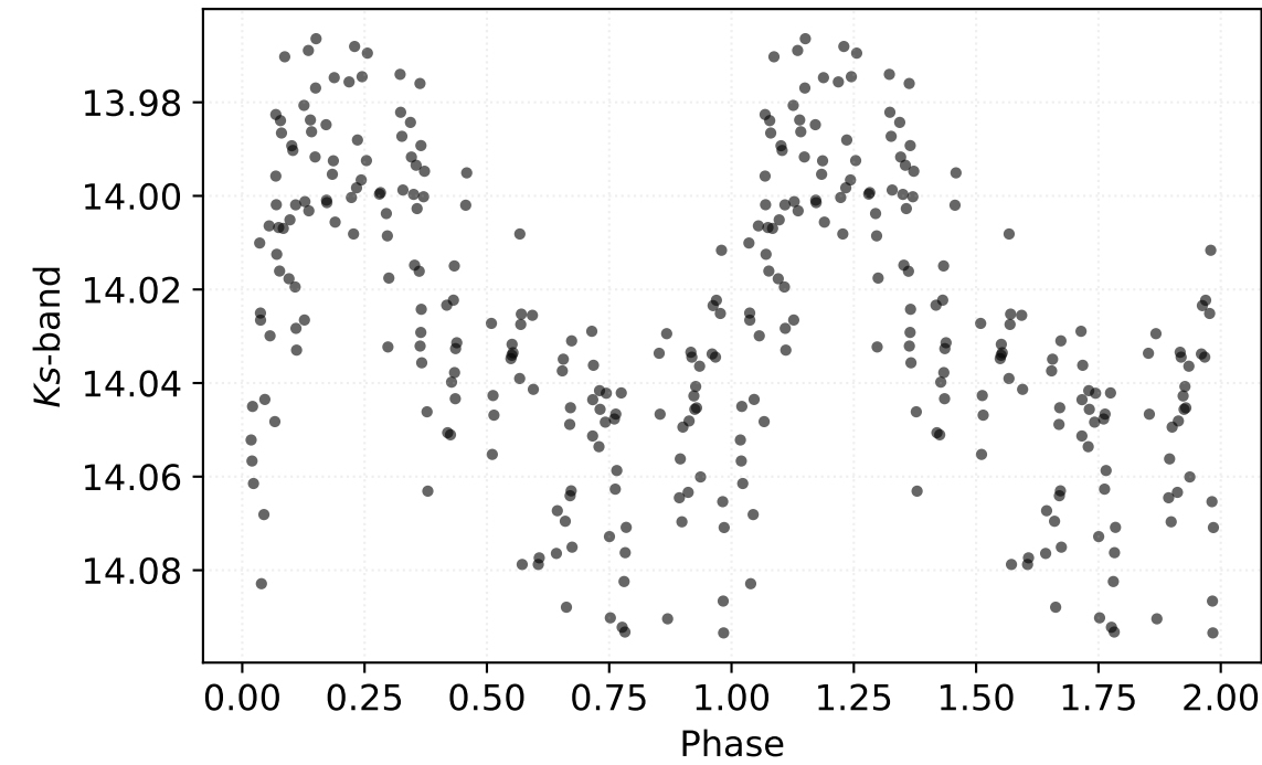
P: 0.36147 d | Class: RP | Subclass: RRab | Field b279
