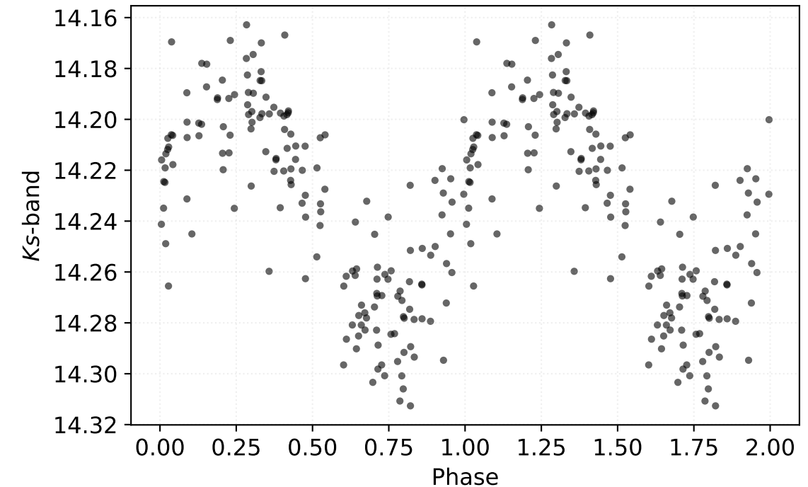
P: 0.69085 d | Class: RP | Subclass: RRab | Field b278
