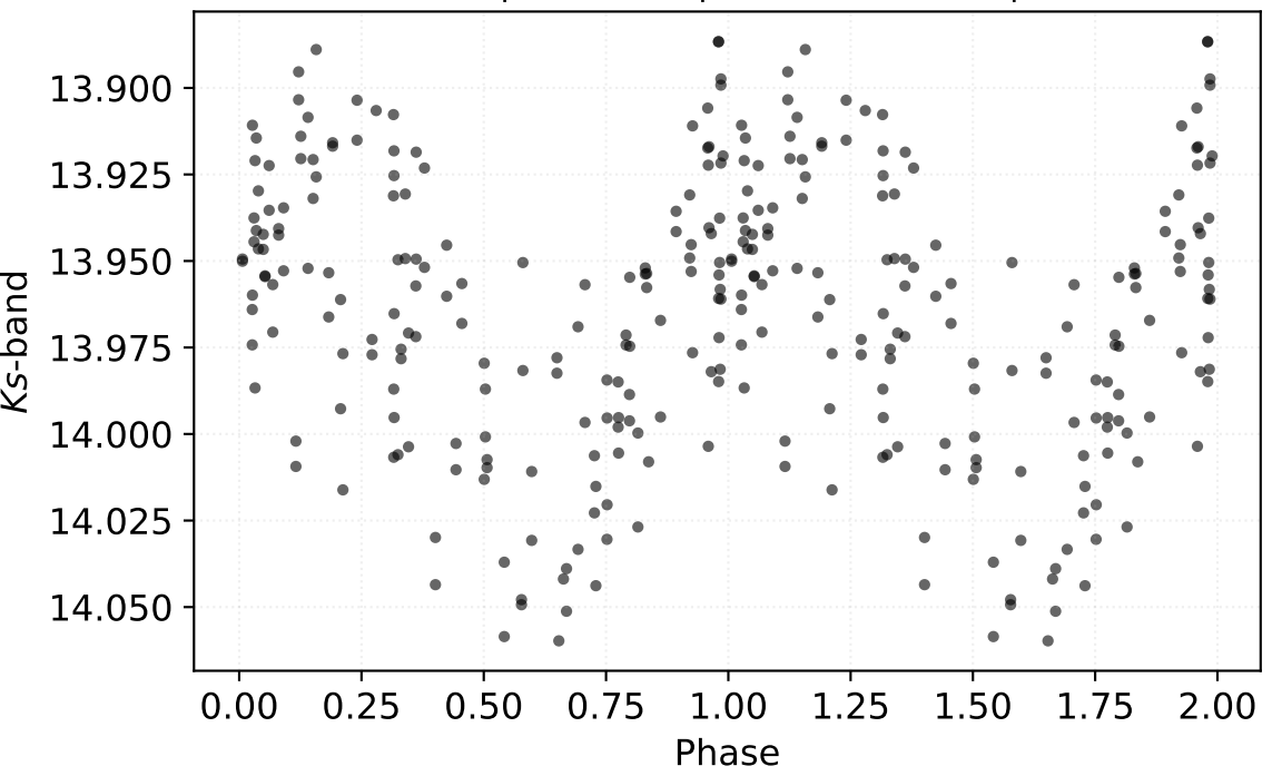
P: 0.19945 d | Class: RP | Subclass: UVAR | Field b279
