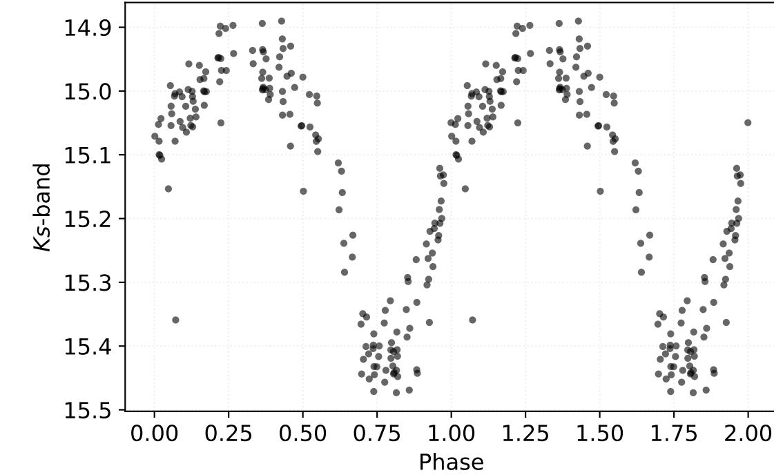
P: 0.19547 d | Class: RP | Subclass: UVAR | Field b278
