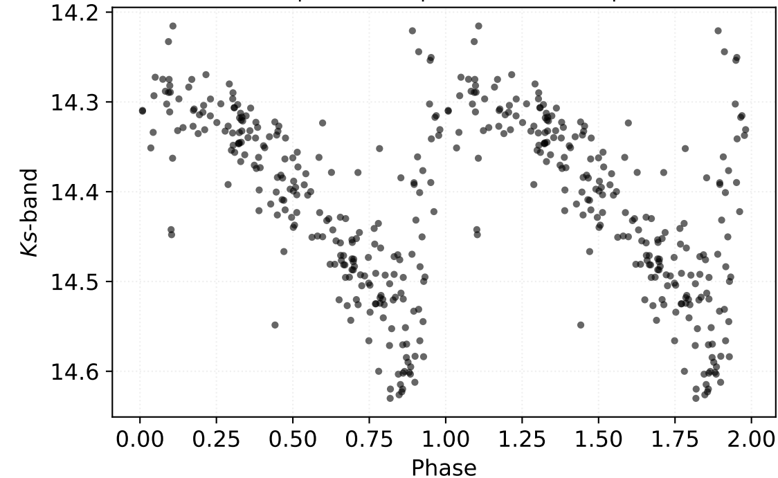
P: 0.44444 d | Class: RP | Subclass: RRab | Field b278
