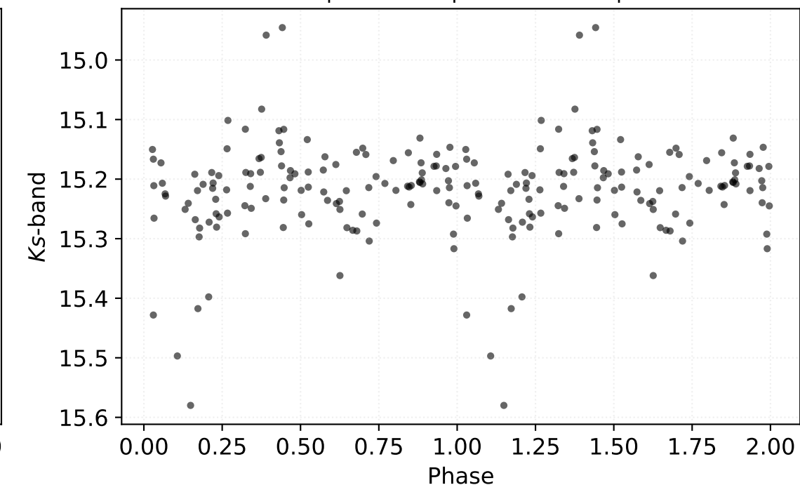
P: 0.34671 d | Class: EB | Subclass: EA | Field b278
