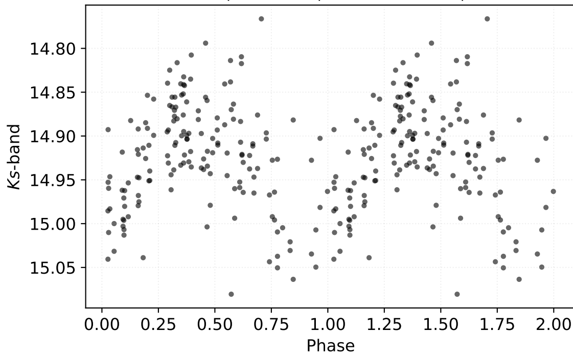
P: 0.18861 d | Class: RP | Subclass: UVAR | Field b279
