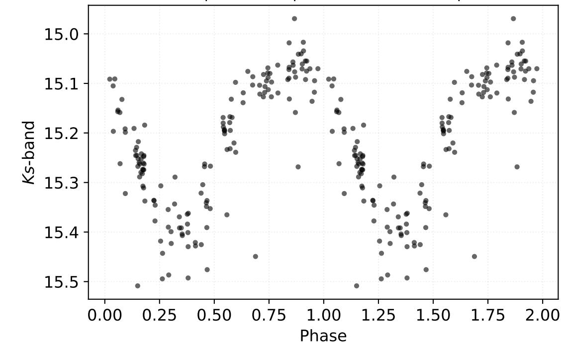
P: 0.68364 d | Class: RP | Subclass: CEP-1OT | Field b279
