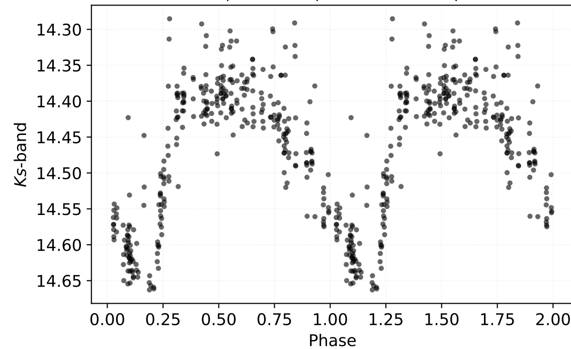
P: 0.48433 d | Class: RP | Subclass: RRab | Field b279
