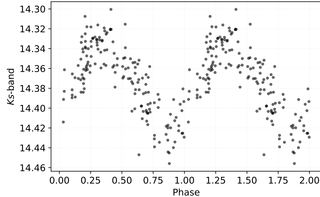
P: 0.20527 d | Class: RP | Subclass: UVAR | Field b279
