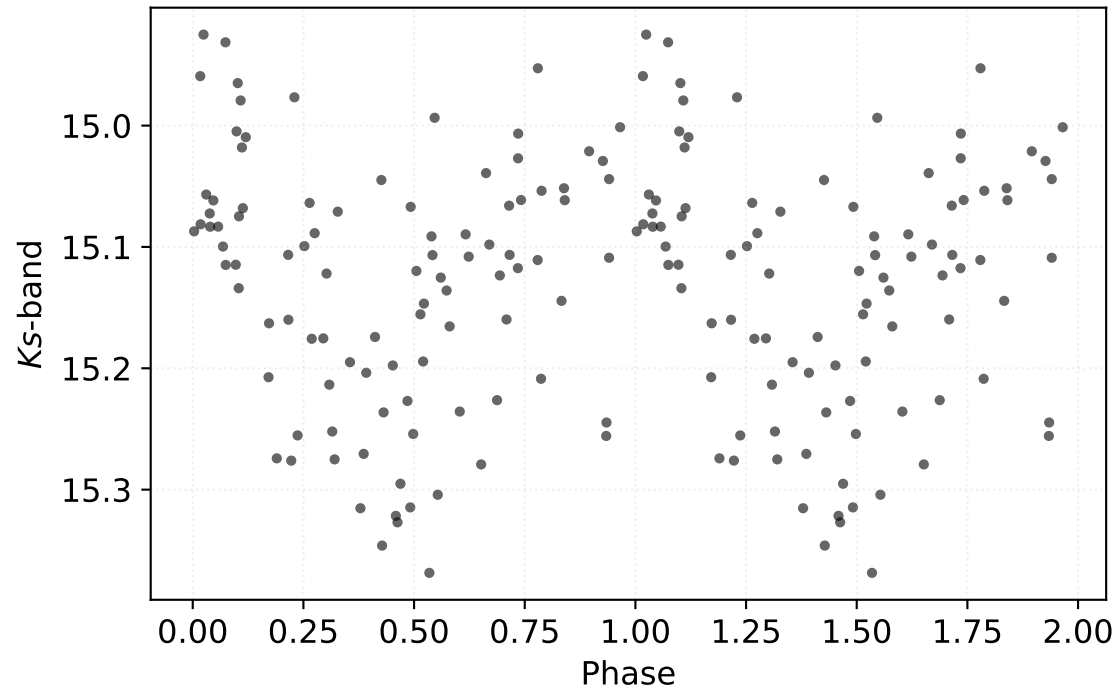
P: 0.24932 d | Class: RP | Subclass: UVAR | Field b278
