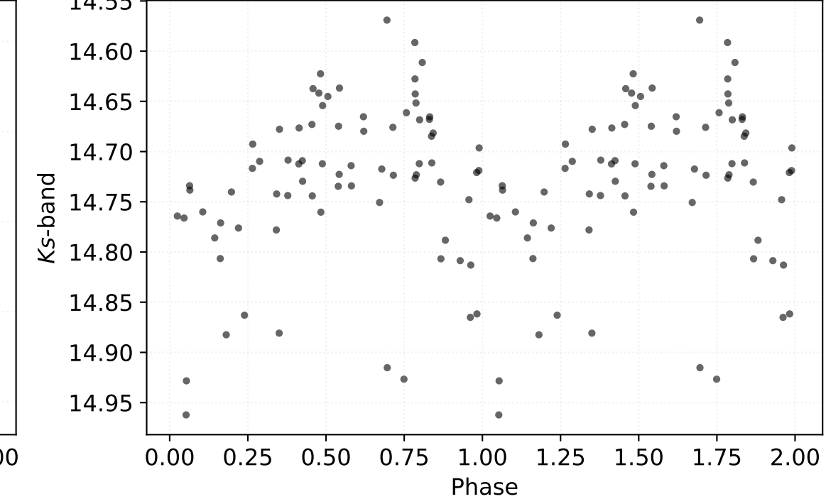
P: 0.83001 d | Class: RP | Subclass: RRab | Field b279
