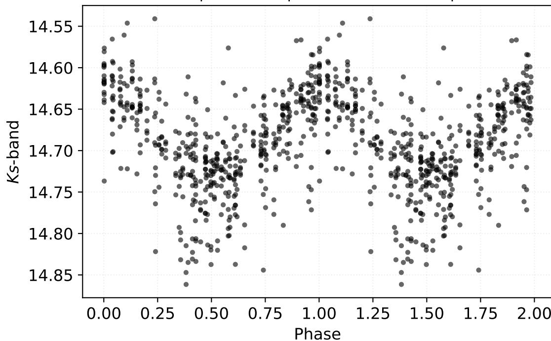
P: 0.41875 d | Class: RP | Subclass: CEP-1OT | Field b279
