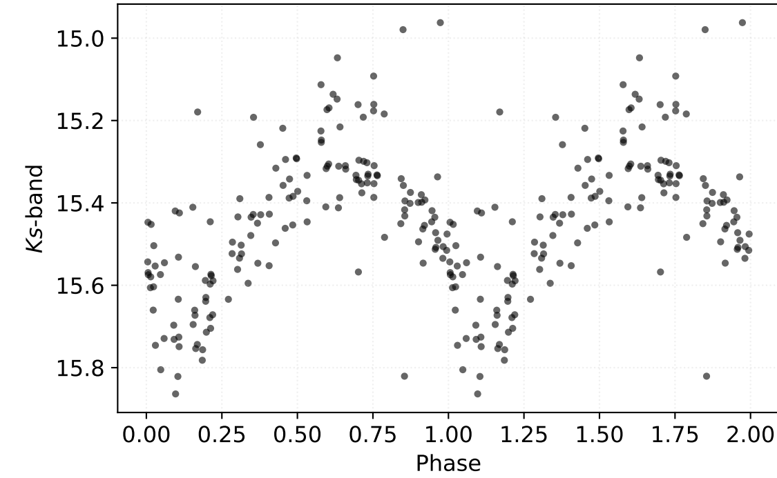
P: 0.65111 d | Class: RP | Subclass: CEP-1OT | Field b279
