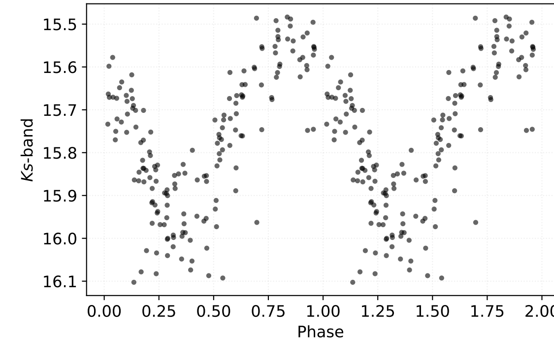
P: 7.40941 d | Class: RP | Subclass: CEP-1OT | Field b278
