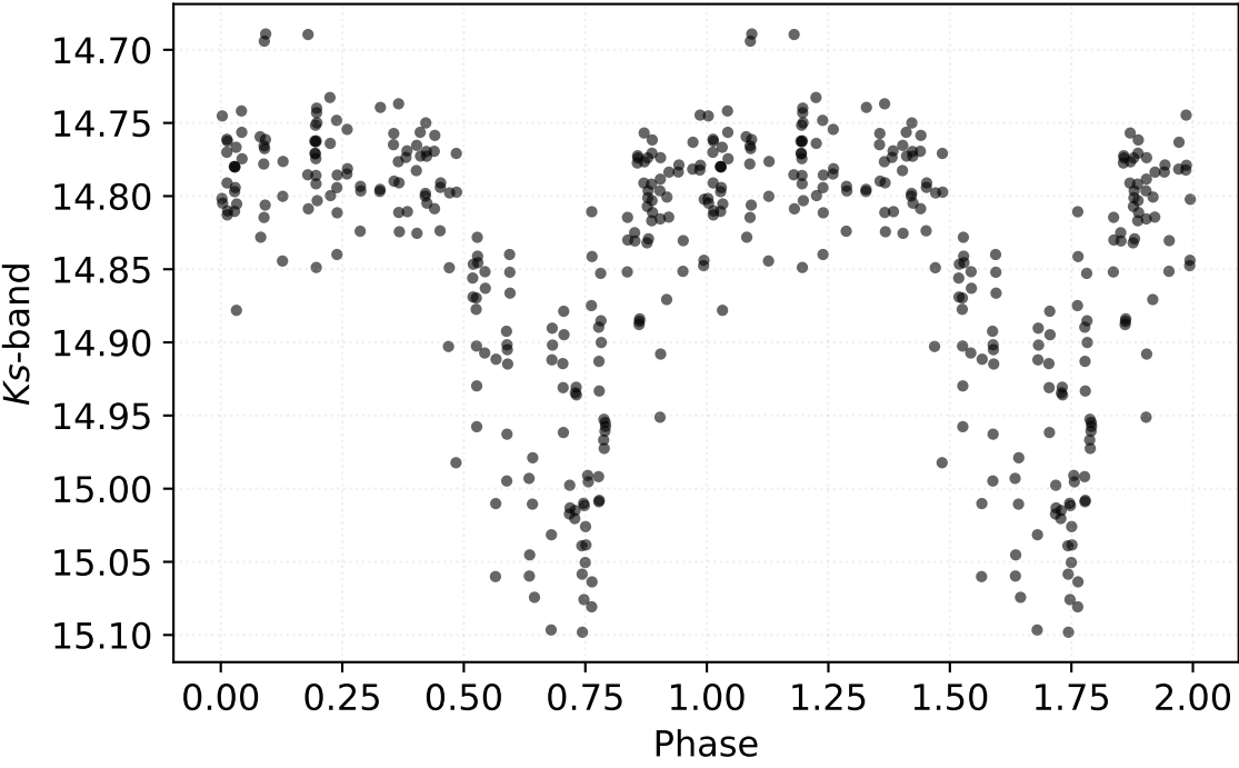
P: 0.67293 d | Class: RP | Subclass: CEP-1OT | Field b279
