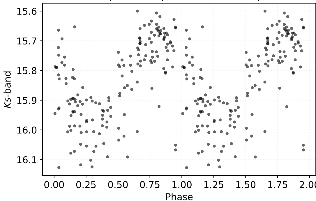
P: 0.28683 d | Class: RP | Subclass: CEP-1OT | Field b278
