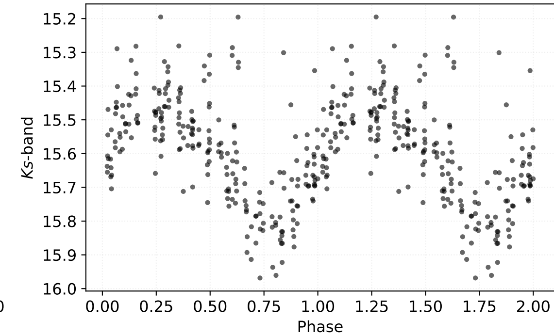
P: 0.47801 d | Class: RP | Subclass: RRab | Field b279
