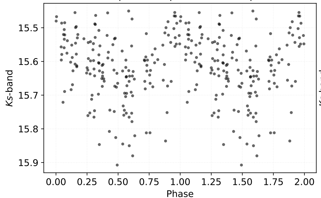
P: 0.10556 d | Class: RP | Subclass: UVAR | Field b279
