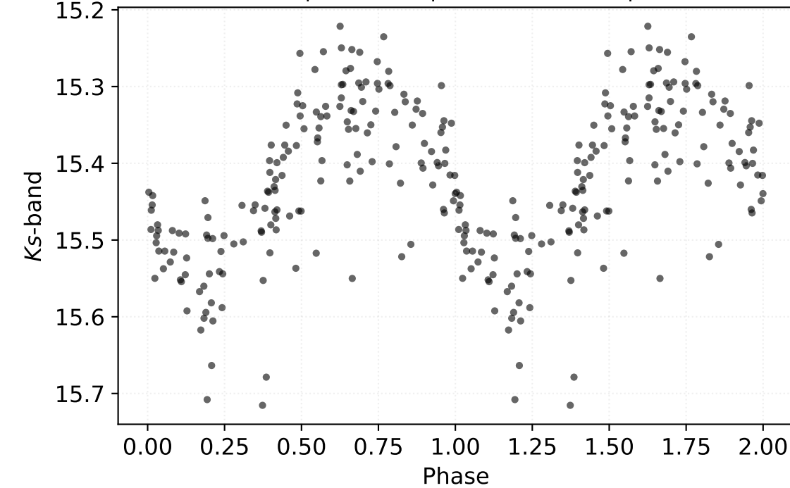
P: 0.19361 d | Class: RP | Subclass: UVAR | Field b279
