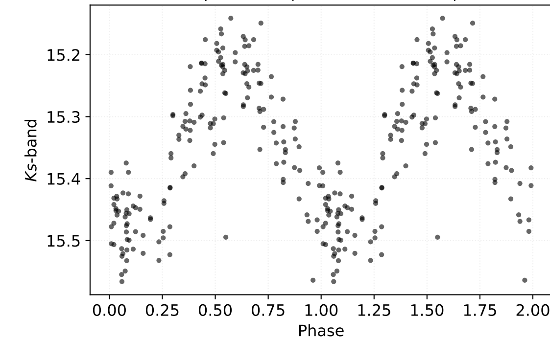
P: 0.83991 d | Class: RP | Subclass: CEP-1OT | Field b278
