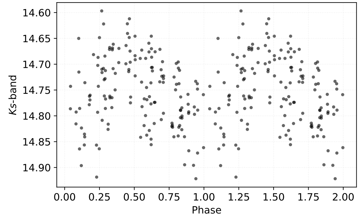
P: 0.40696 d | Class: RP | Subclass: RRab | Field b279
