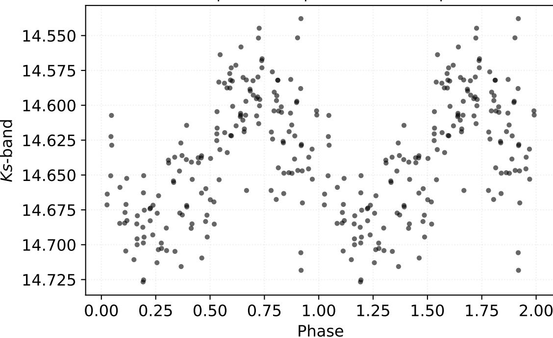
P: 0.33241 d | Class: RP | Subclass: RRab | Field b278
