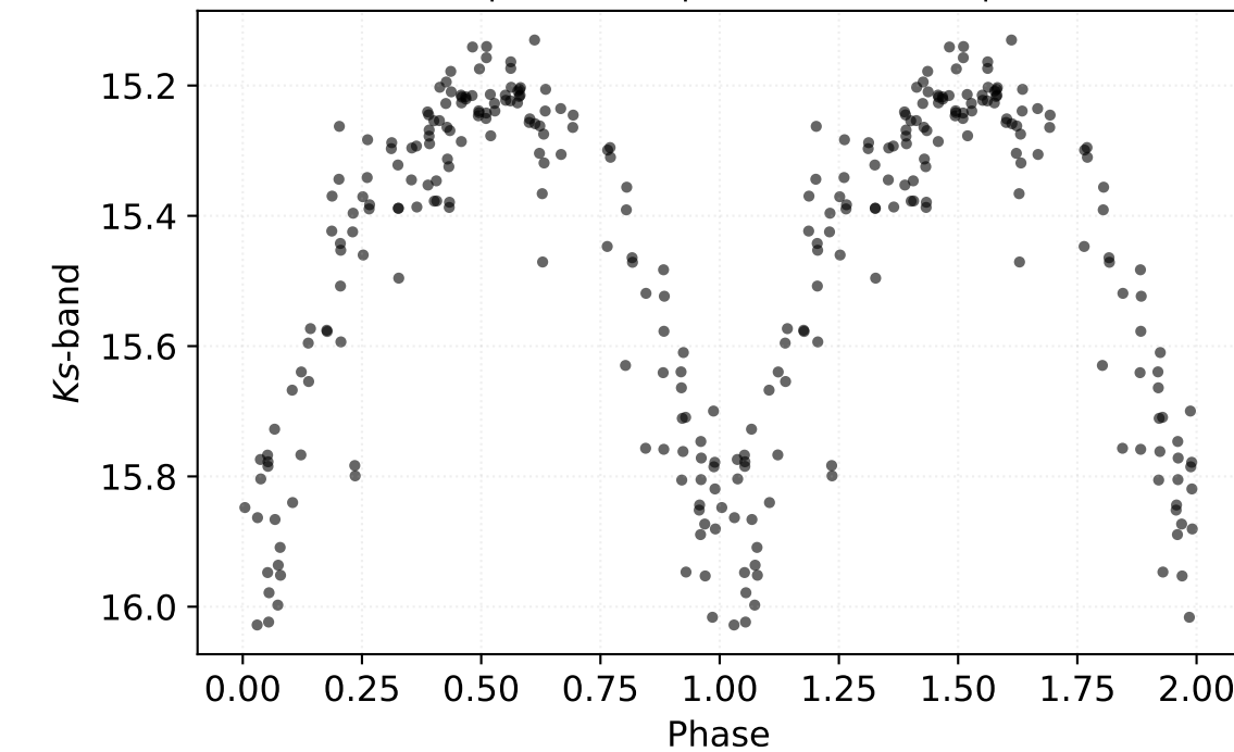
P: 0.47908 d | Class: RP | Subclass: RRab | Field b279
