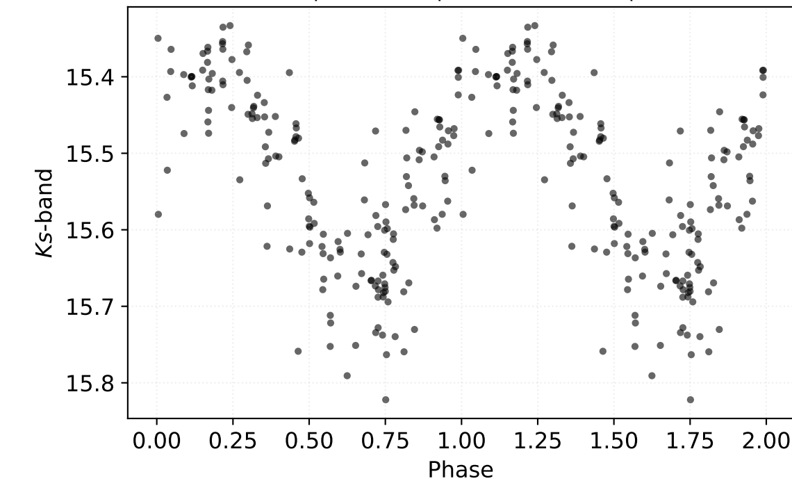
P: 0.53860 d | Class: RP | Subclass: RRab | Field b278
