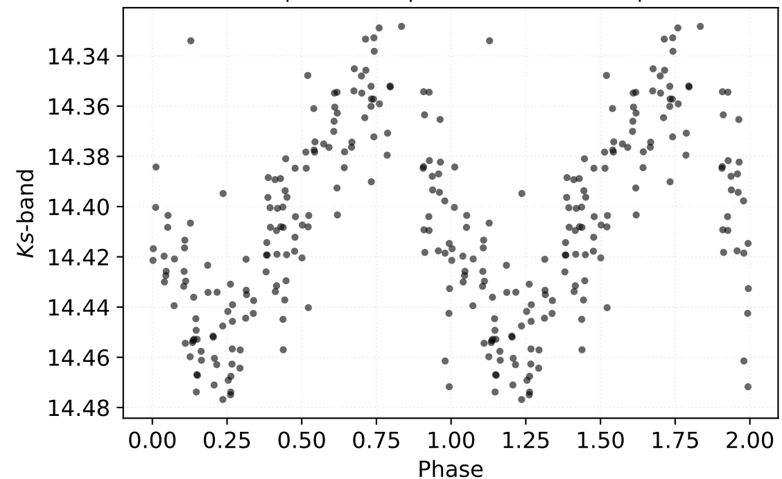
P: 0.62288 d | Class: RP | Subclass: CEP-1OT | Field b279
