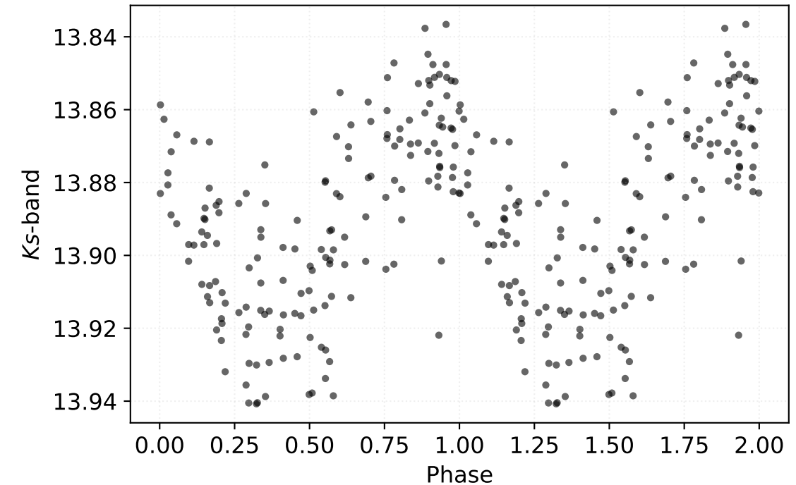
P: 3.63338 d | Class: RP | Subclass: CEP-F | Field b278
