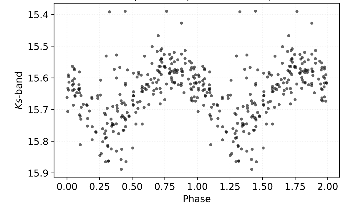
P: 0.49427 d | Class: RP | Subclass: RRab | Field b279
