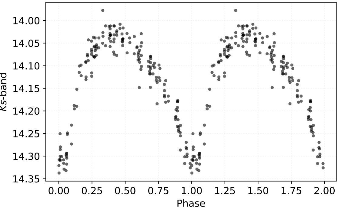
P: 0.60997 d | Class: RP | Subclass: RRab | Field b279
