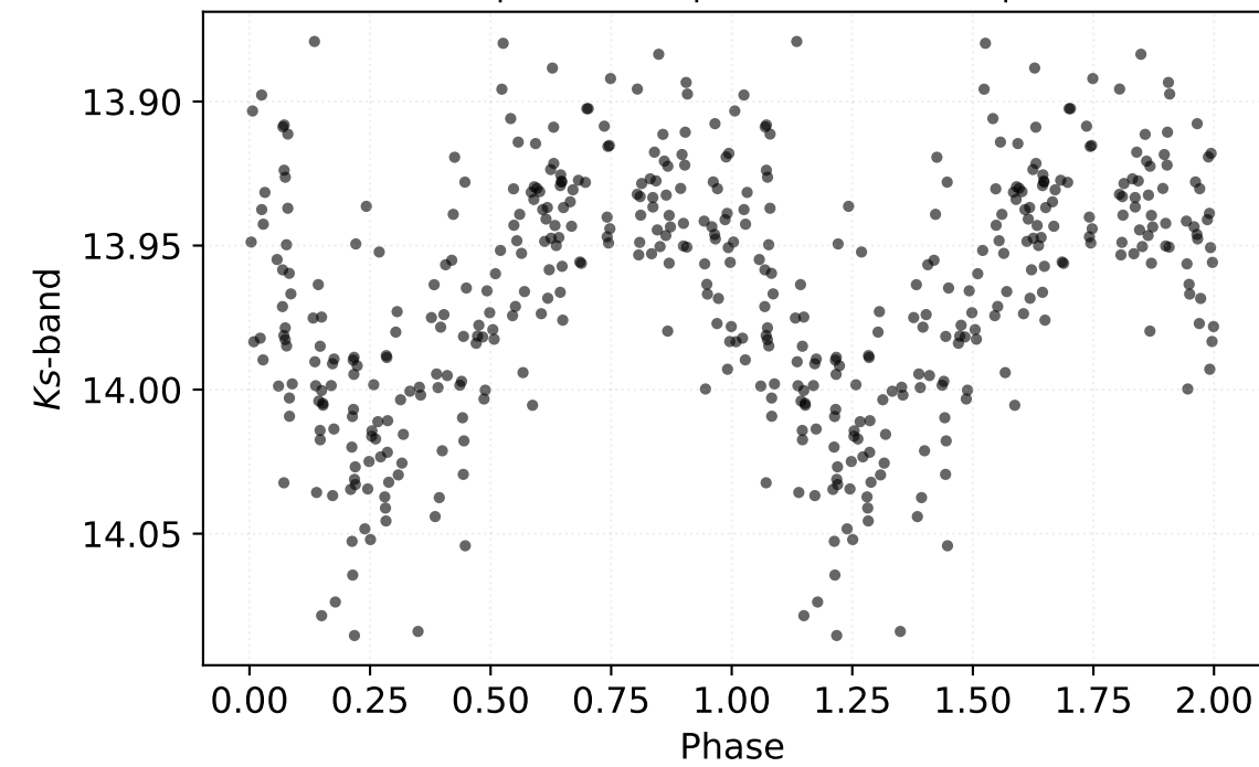
P: 0.11078 d | Class: RP | Subclass: UVAR | Field b279
