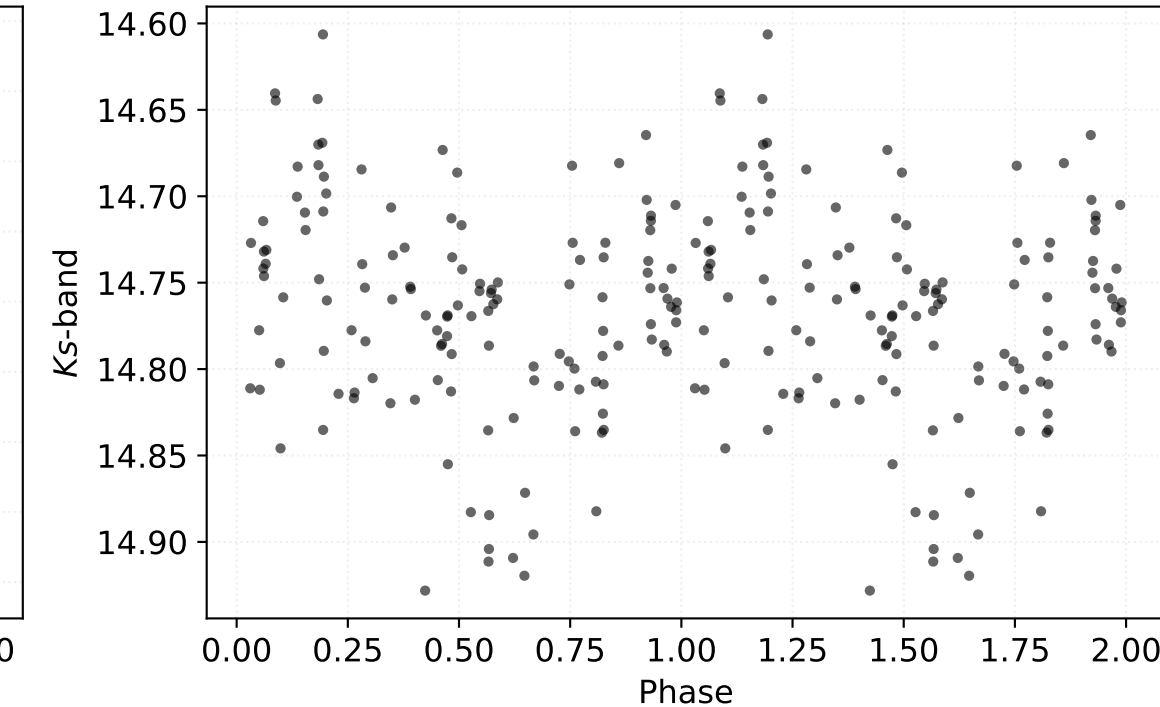
P: 0.28150 d | Class: RP | Subclass: RRc | Field b279
