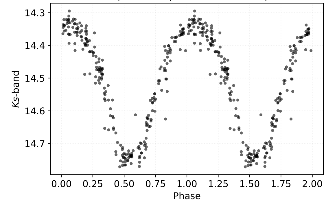
P: 0.65942 d | Class: RP | Subclass: CEP-1OT | Field b278
