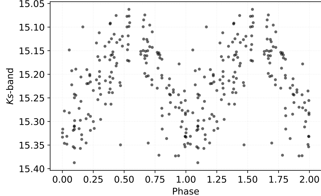
P: 0.30123 d | Class: RP | Subclass: CEP-1OT | Field b278
