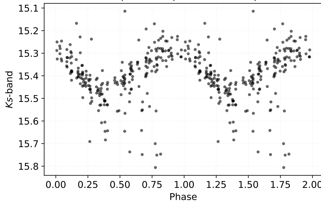
P: 0.24118 d | Class: RP | Subclass: UVAR | Field b279
