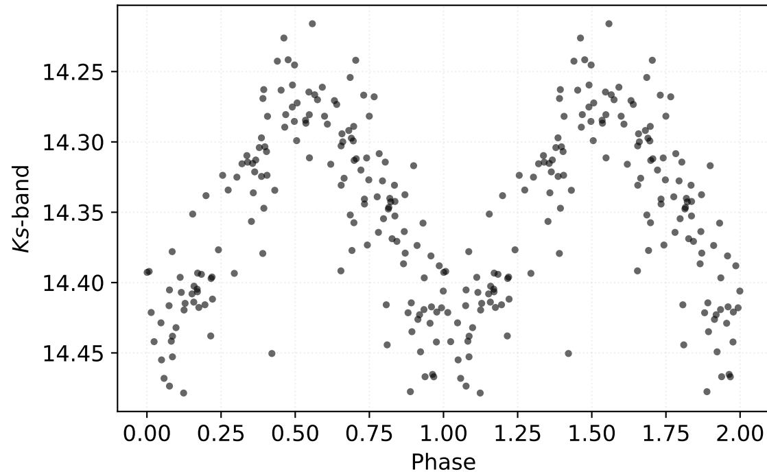
P: 3.10637 d | Class: RP | Subclass: CEP-1OT | Field b278
