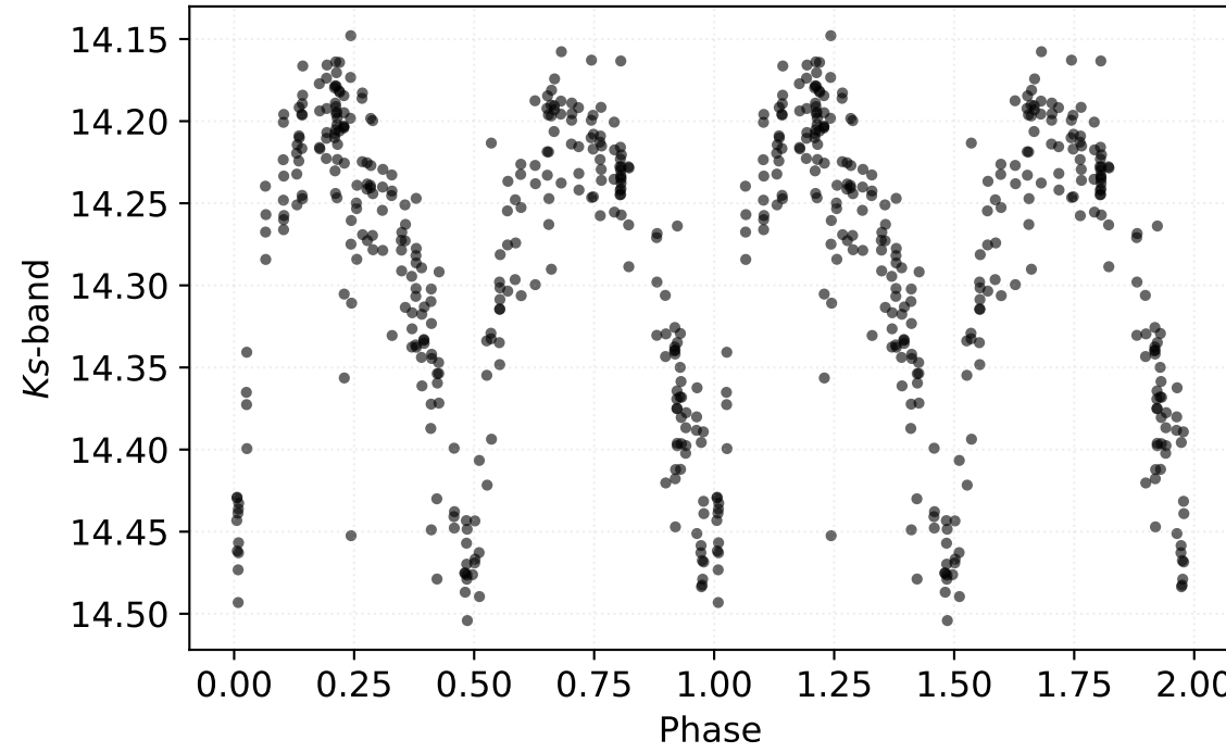
P: 0.20764 d | Class: RP | Subclass: RRc | Field b278
