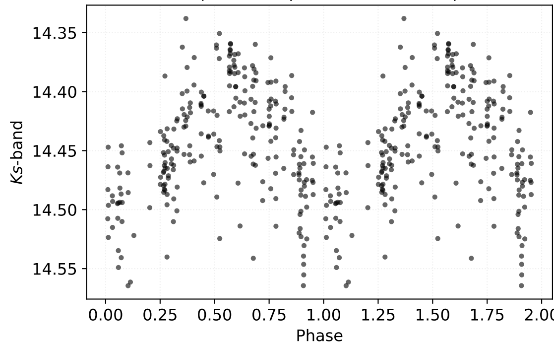
P: 5.74722 d | Class: RP | Subclass: CEP-1OT | Field b279
