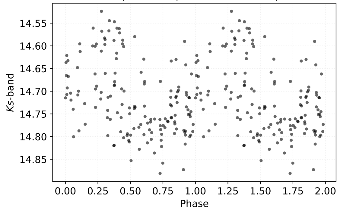
P: 0.97558 d | Class: RP | Subclass: CEP-1OT | Field b279
