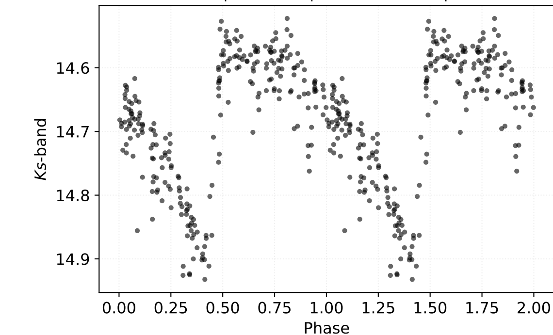
P: 0.43595 d | Class: RP | Subclass: RRab | Field b278
