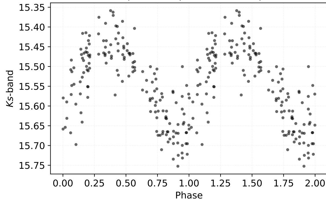
P: 0.35301 d | Class: RP | Subclass: RRab | Field b278
