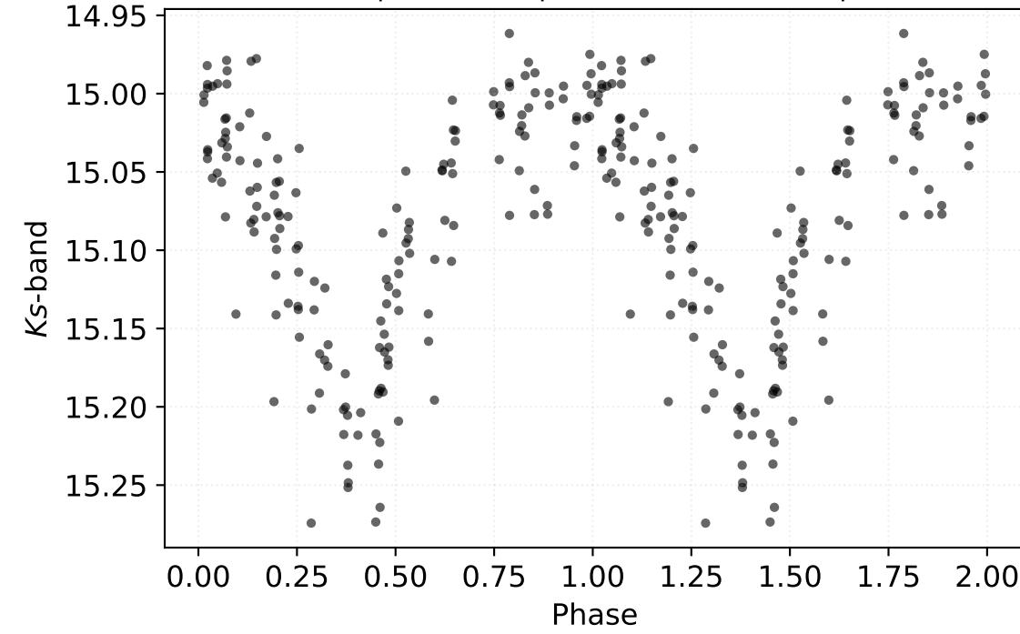
P: 0.65159 d | Class: RP | Subclass: CEP-1OT | Field b278
