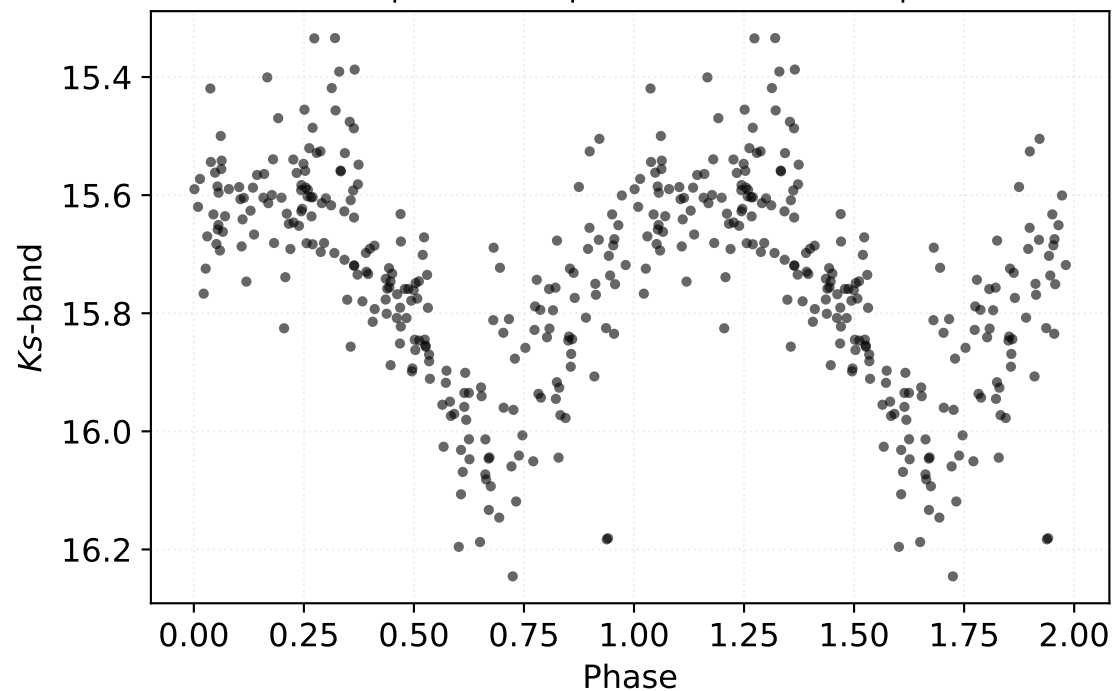
P: 2.00073 d | Class: RP | Subclass: CEP-1OT | Field b278
