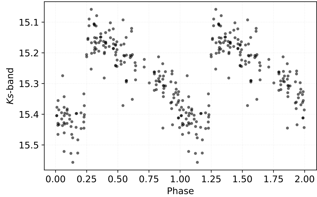
P: 0.40333 d | Class: RP | Subclass: RRab | Field b278
