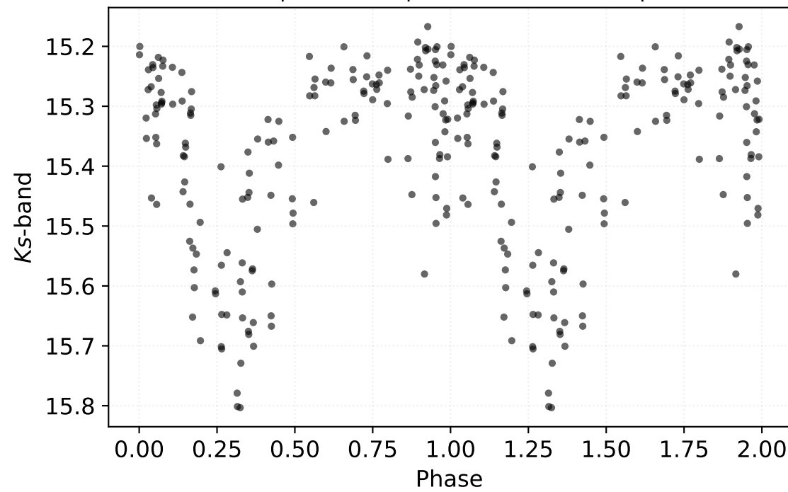
P: 0.46317 d | Class: RP | Subclass: CEP-1OT | Field b278
