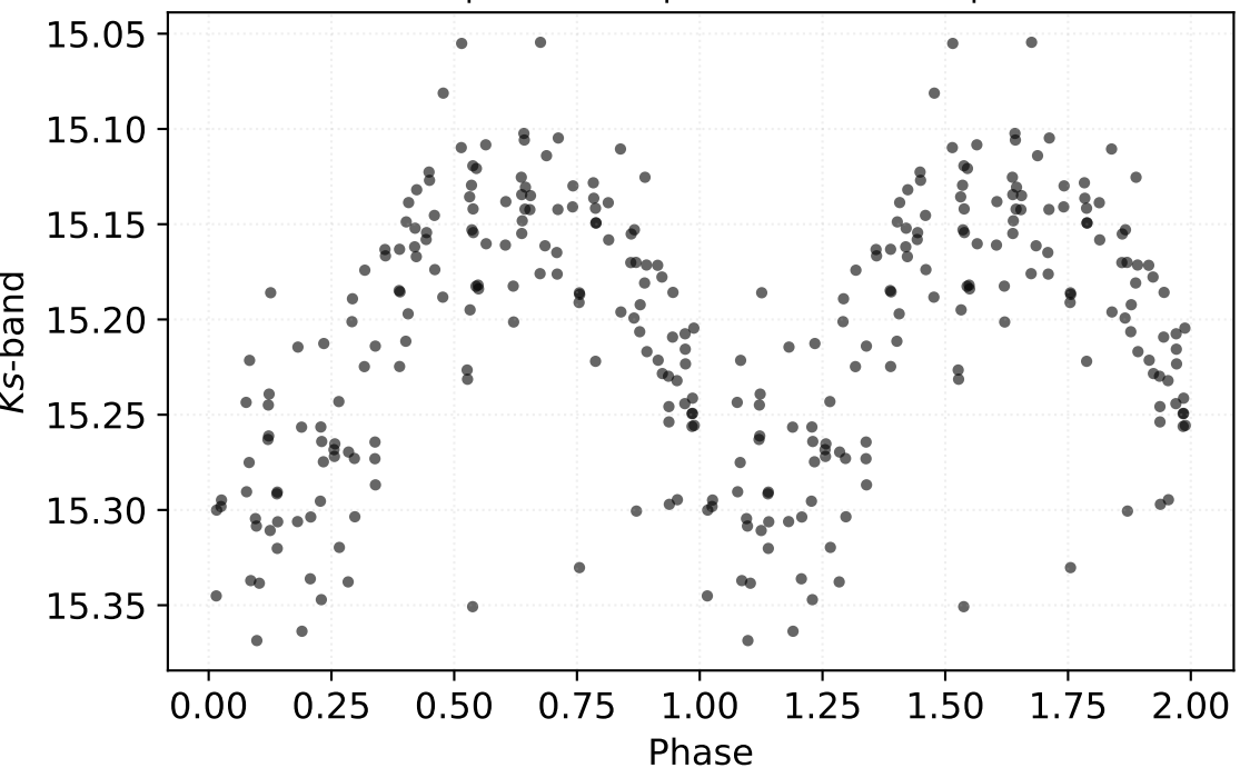
P: 0.34950 d | Class: RP | Subclass: RRab | Field b279
