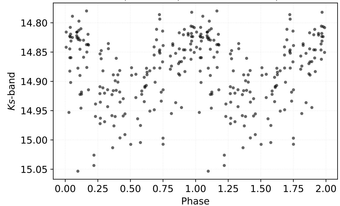
P: 3.42845 d | Class: RP | Subclass: CEP-1OT | Field b279
