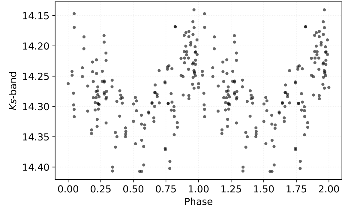
P: 53.75329 d | Class: RP | Subclass: CEP-F | Field b279
