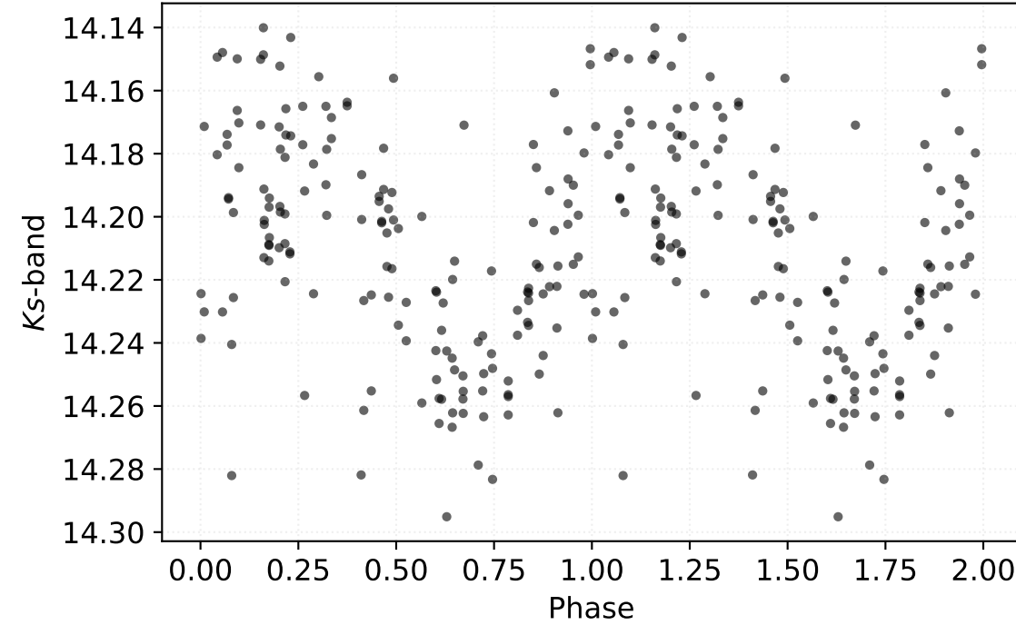
P: 77.24150 d | Class: RP | Subclass: UVAR | Field b279
