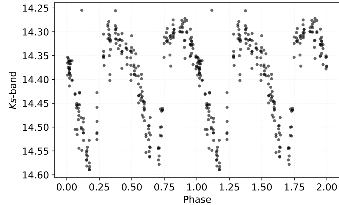
P: 0.50683 d | Class: RP | Subclass: RRc | Field b278
