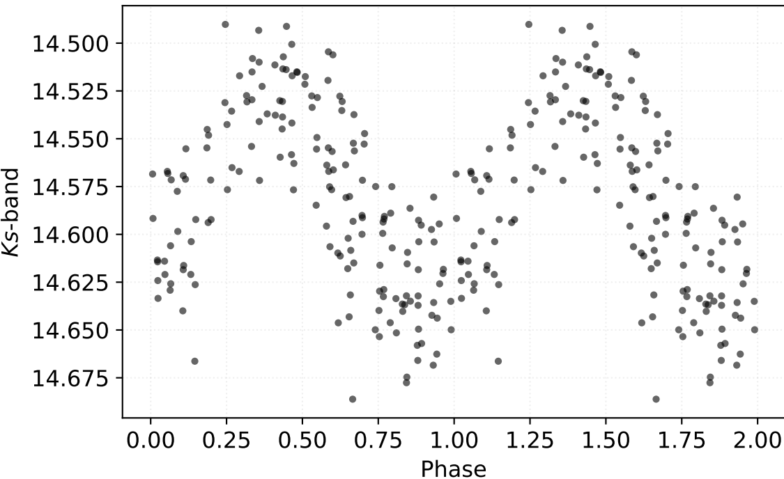
P: 0.61704 d | Class: RP | Subclass: CEP-1OT | Field b278
