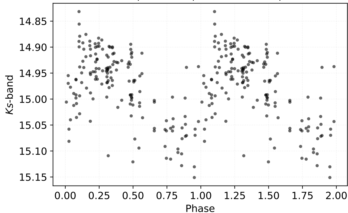
P: 0.22655 d | Class: RP | Subclass: UVAR | Field b279
