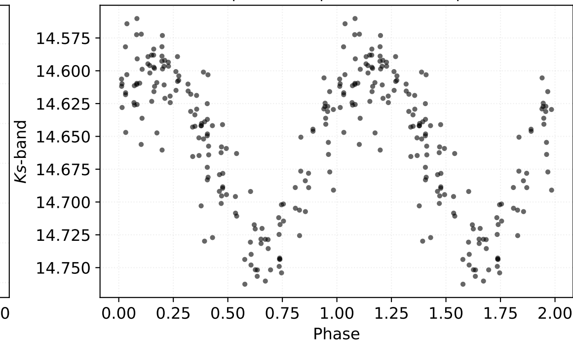
P: 0.36109 d | Class: RP | Subclass: RRab | Field b279
