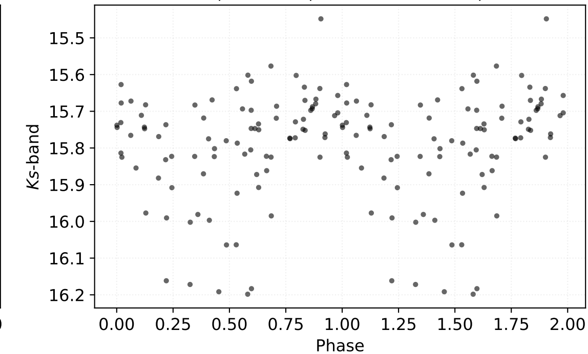
P: 0.41418 d | Class: RP | Subclass: CEP-1OT | Field b278
