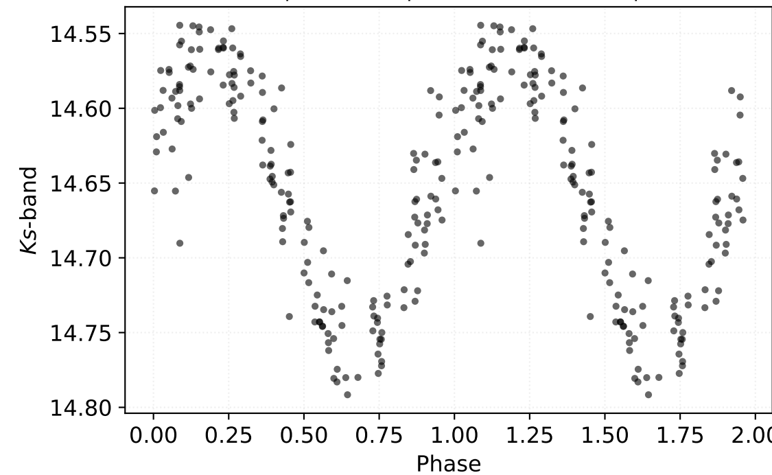
P: 0.47496 d | Class: RP | Subclass: CEP-1OT | Field b278
