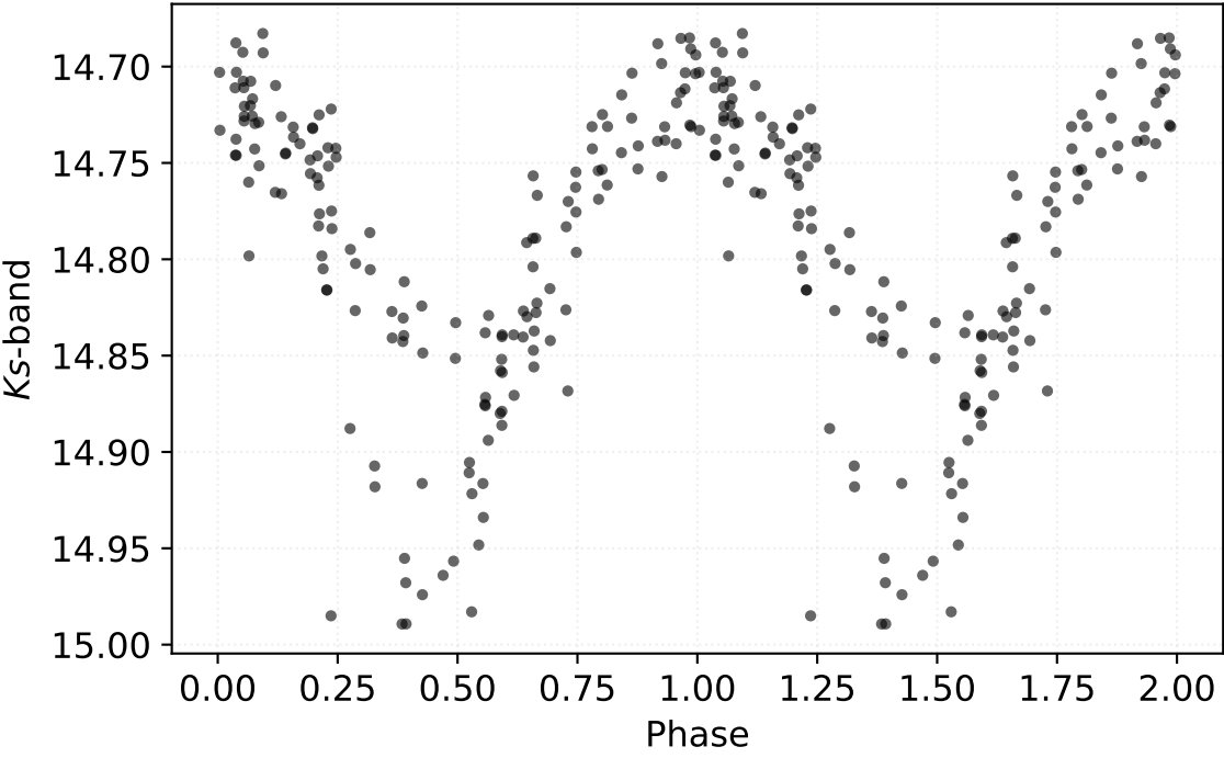
P: 0.56424 d | Class: RP | Subclass: CEP-1OT | Field b279
