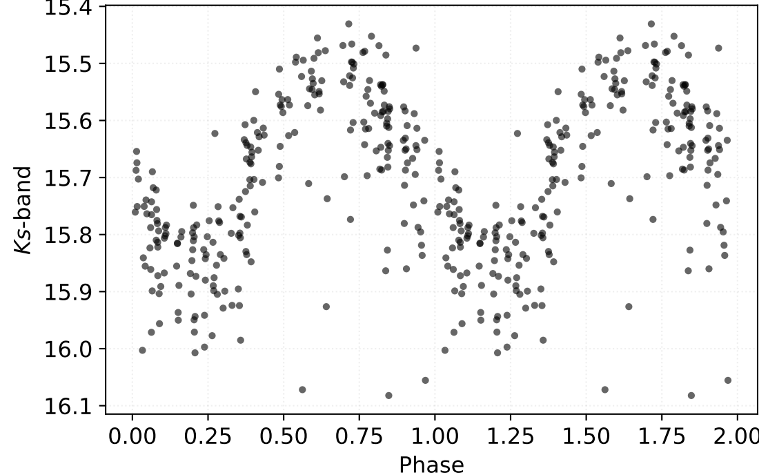
P: 0.16358 d | Class: RP | Subclass: UVAR | Field b279
