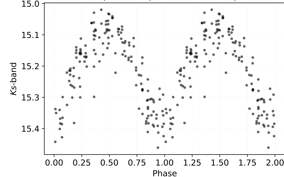
P: 0.27839 d | Class: RP | Subclass: CEP-1OT | Field b278
