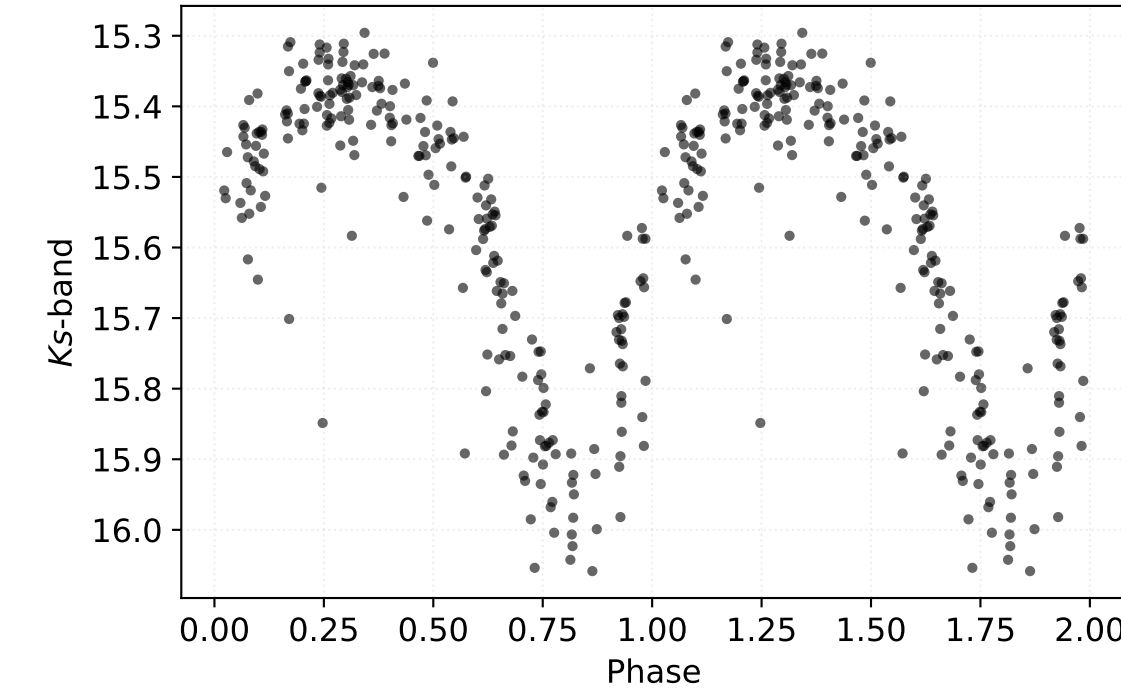
P: 0.22017 d | Class: RP | Subclass: UVAR | Field b278
