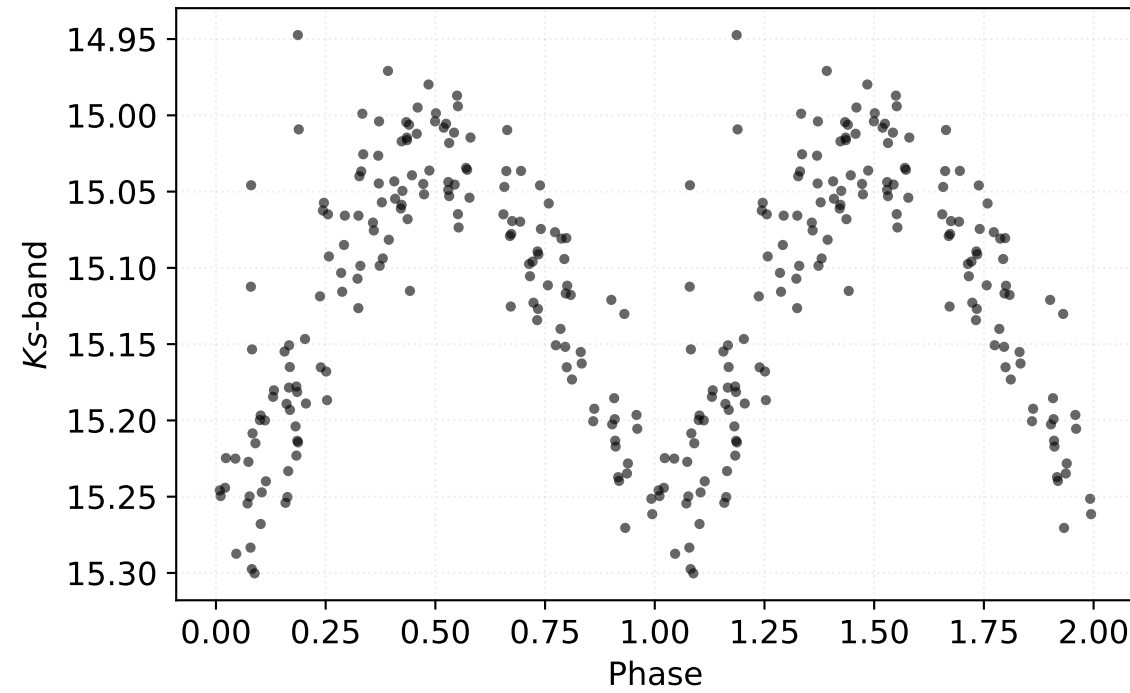
P: 0.57737 d | Class: RP | Subclass: RRc | Field b279
