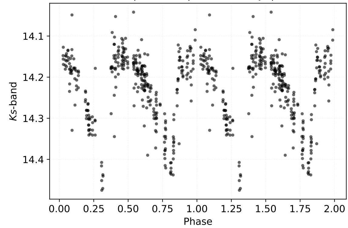
P: 1.03173 d | Class: EB | Subclass: EBlyr | Field b278
