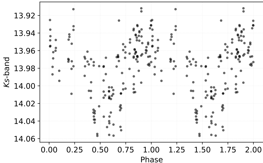
P: 0.38681 d | Class: RP | Subclass: CEP-1OT | Field b278
