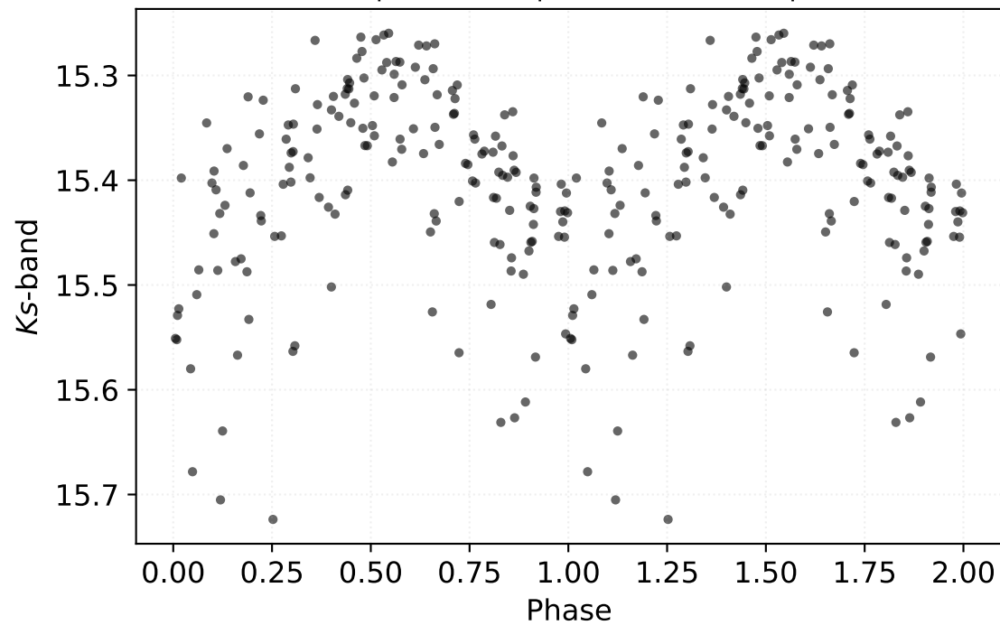
P: 0.22900 d | Class: RP | Subclass: UVAR | Field b279
