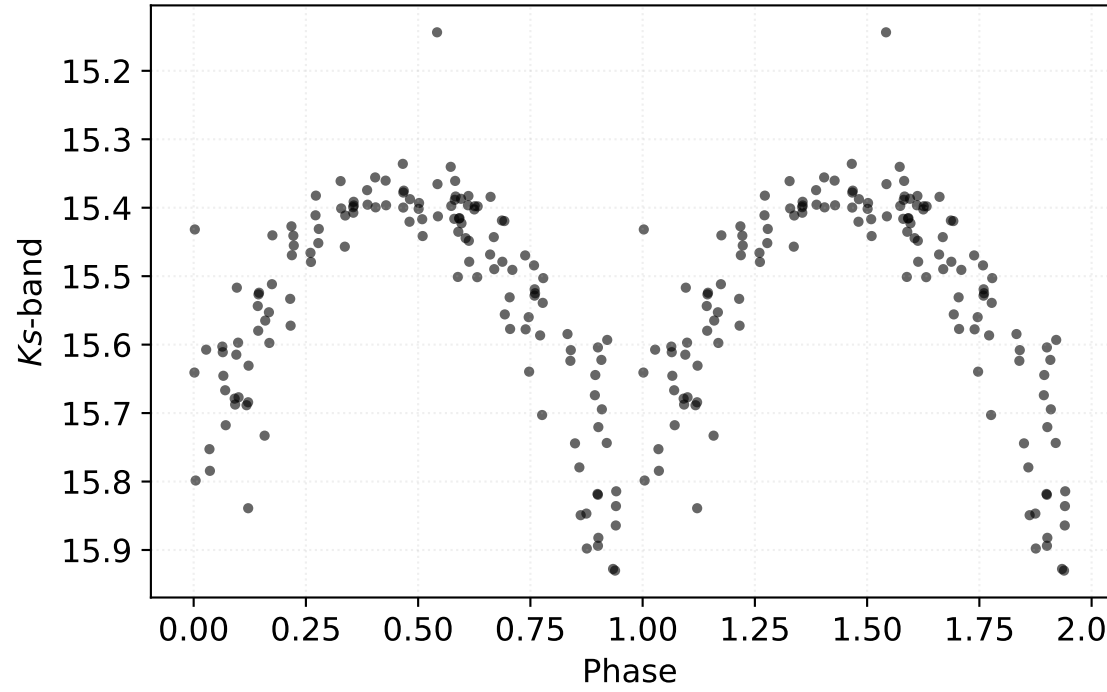
P: 2.34238 d | Class: RP | Subclass: CEP-1OT | Field b279
