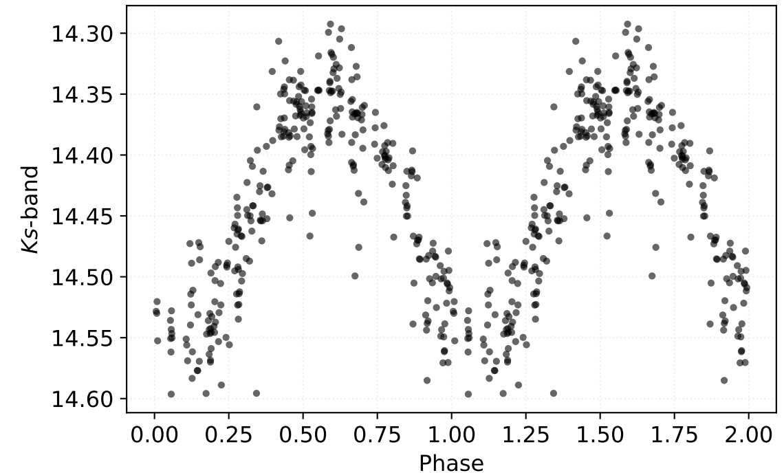
P: 0.72893 d | Class: RP | Subclass: RRab | Field b278
