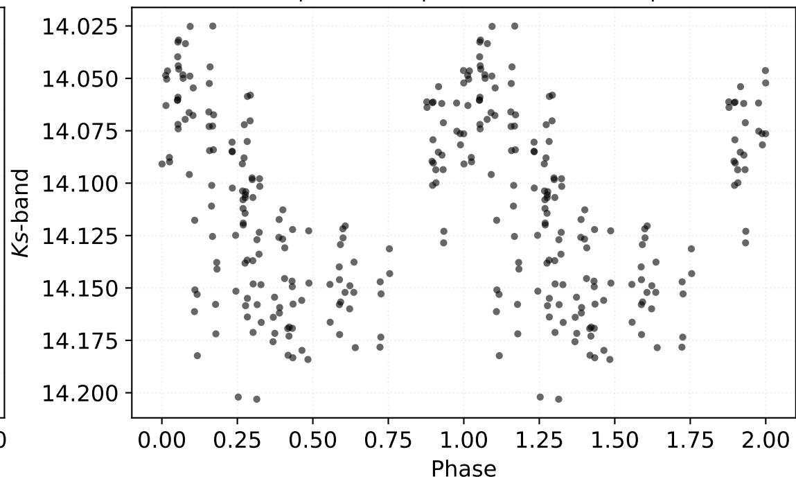
P: 0.53054 d | Class: RP | Subclass: CEP-1OT | Field b278
