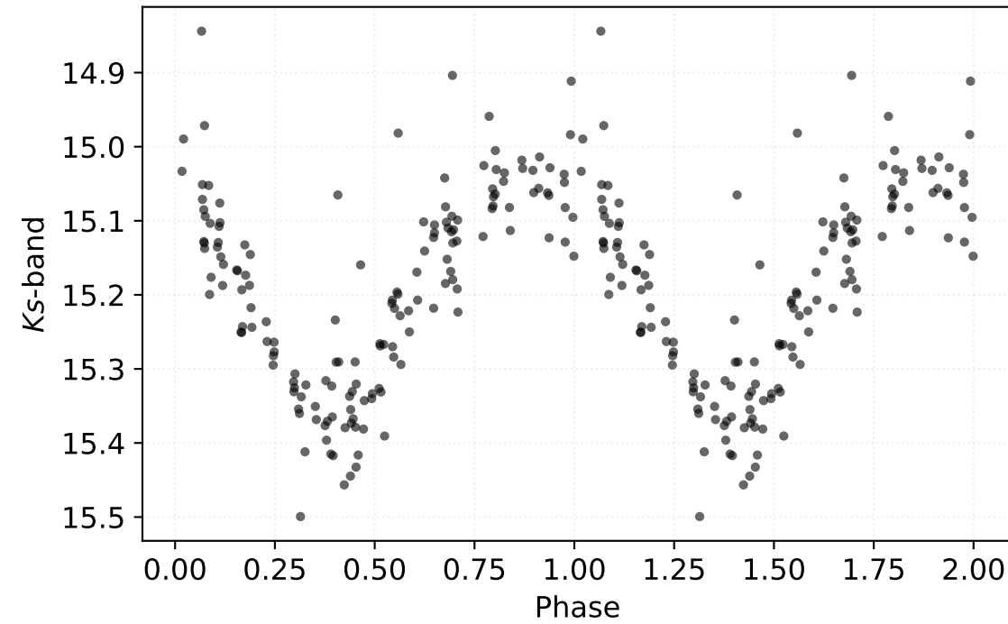
P: 1.07757 d | Class: EB | Subclass: UVAR | Field b278
