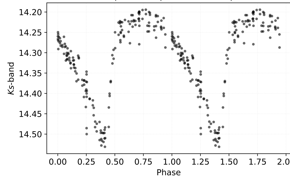
P: 0.55276 d | Class: RP | Subclass: RRab | Field b278
