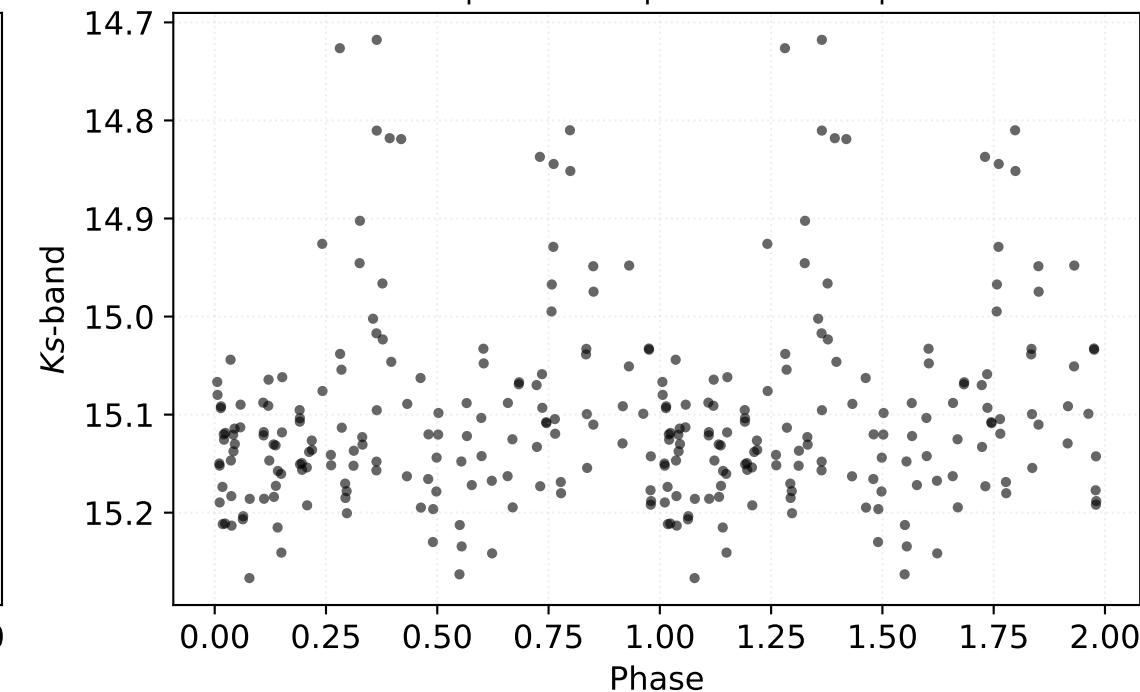
P: 0.58407 d | Class: EB | Subclass: EA | Field b278
