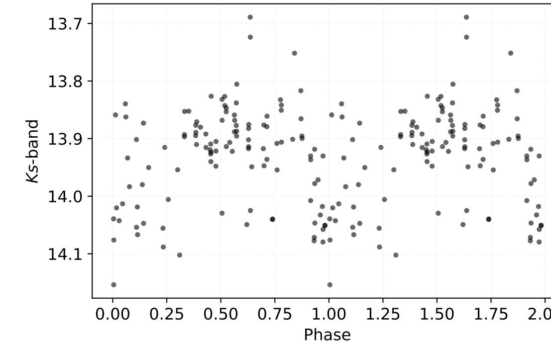
P: 2.02874 d | Class: RP | Subclass: CEP-1OT | Field b279
