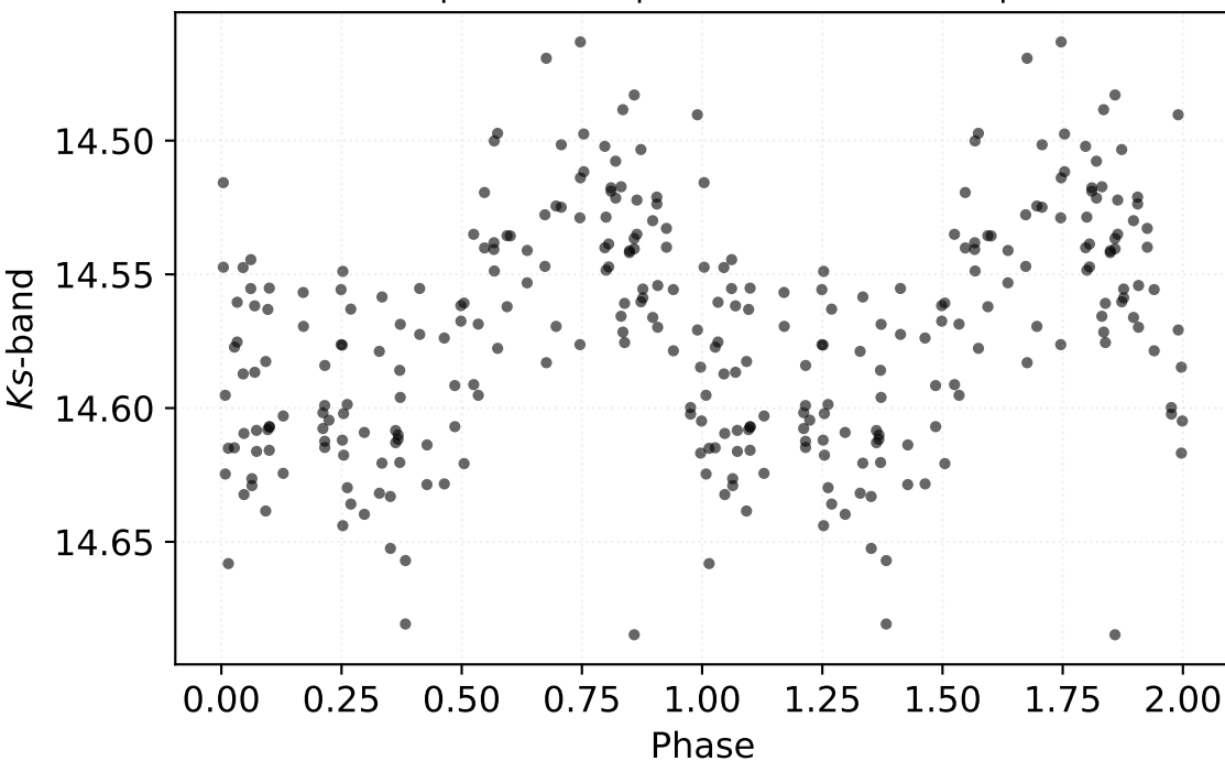
P: 0.42174 d | Class: RP | Subclass: CEP-1OT | Field b278
