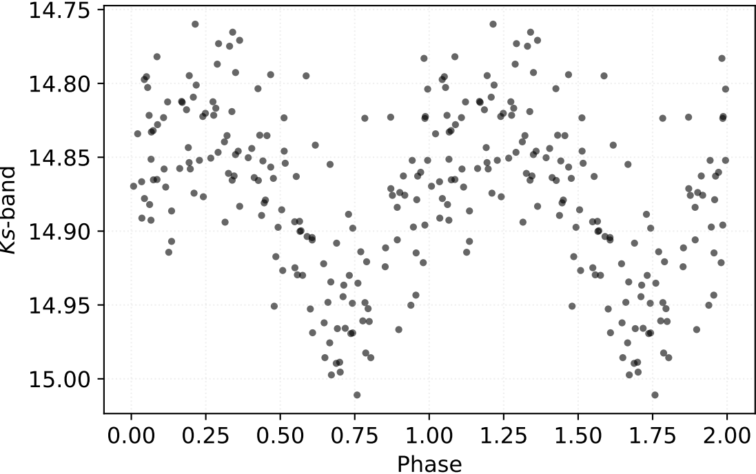
P: 0.15265 d | Class: RP | Subclass: UVAR | Field b279
