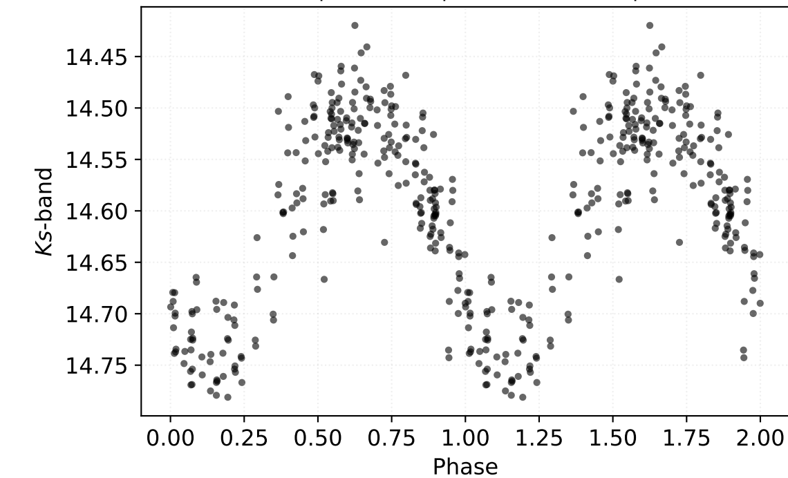
P: 0.46722 d | Class: RP | Subclass: RRab | Field b278
