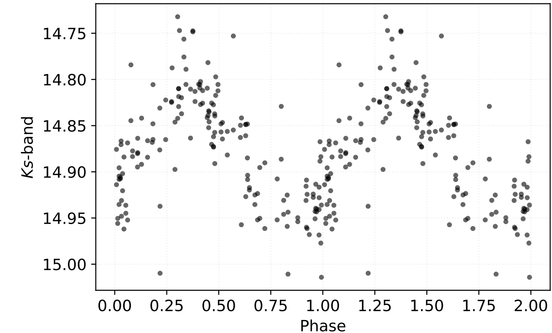
P: 2.13492 d | Class: RP | Subclass: CEP-F | Field b279
