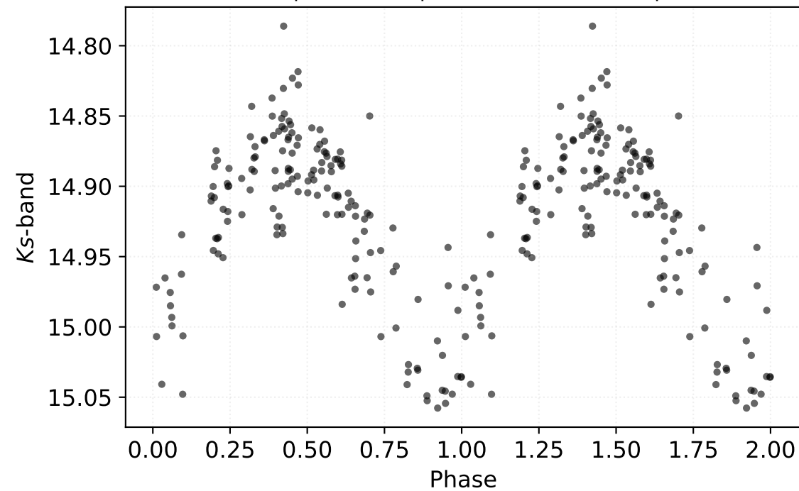
P: 0.42218 d | Class: RP | Subclass: CEP-1OT | Field b278
