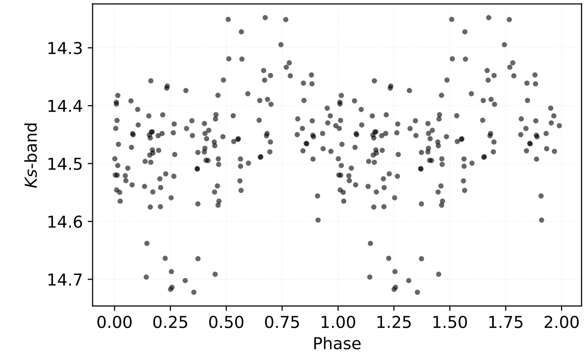
P: 0.50810 d | Class: RP | Subclass: RRab | Field b279
