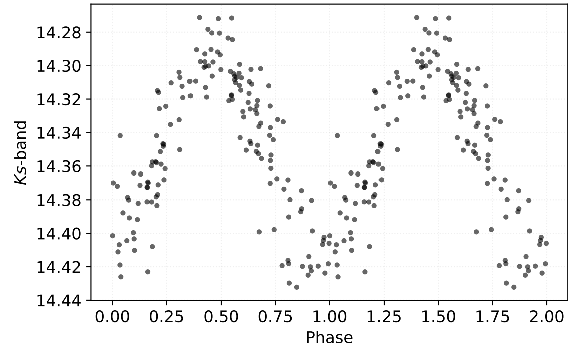
P: 0.16894 d | Class: RP | Subclass: UVAR | Field b279
