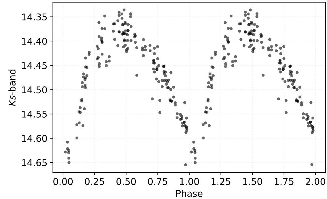
P: 0.31333 d | Class: RP | Subclass: RRab | Field b278
