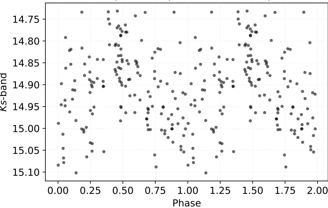
P: 0.36976 d | Class: RP | Subclass: CEP-1OT | Field b279
