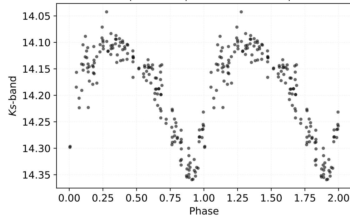
P: 3.28233 d | Class: RP | Subclass: CEP-1OT | Field b278
