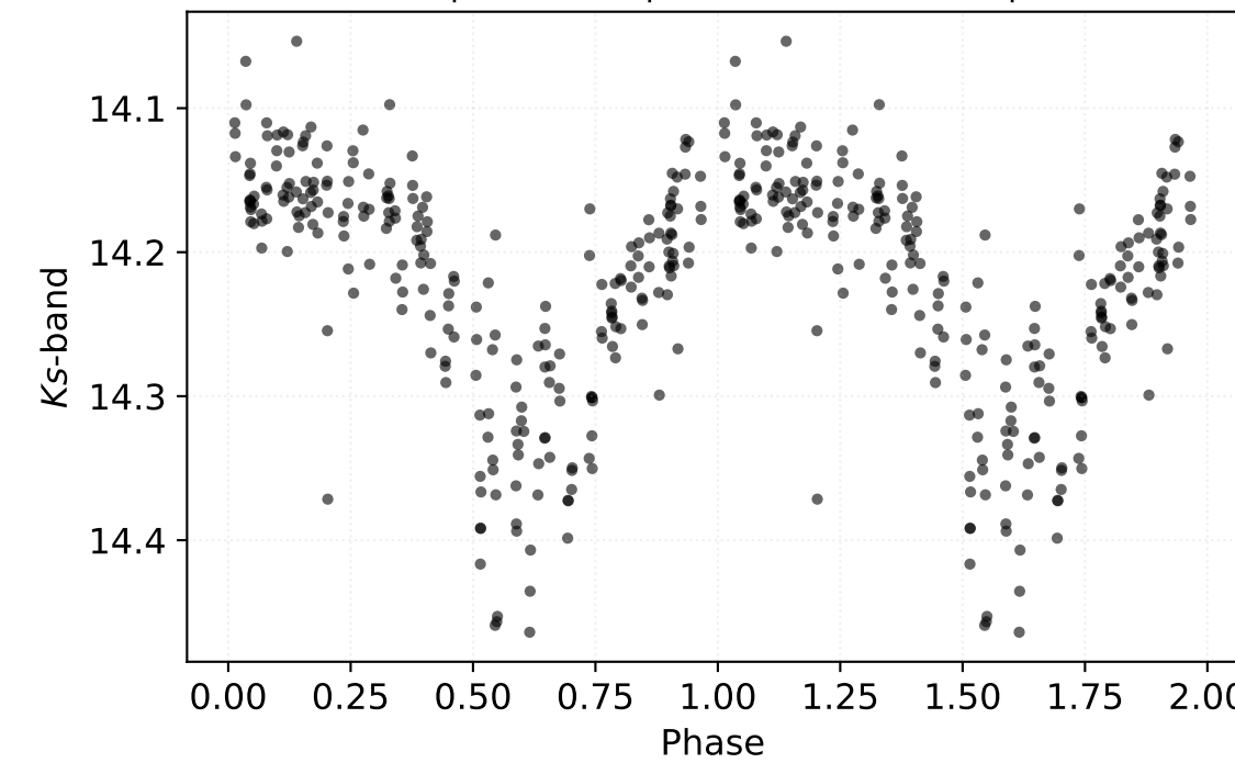
P: 0.36387 d | Class: RP | Subclass: CEP-1OT | Field b279
