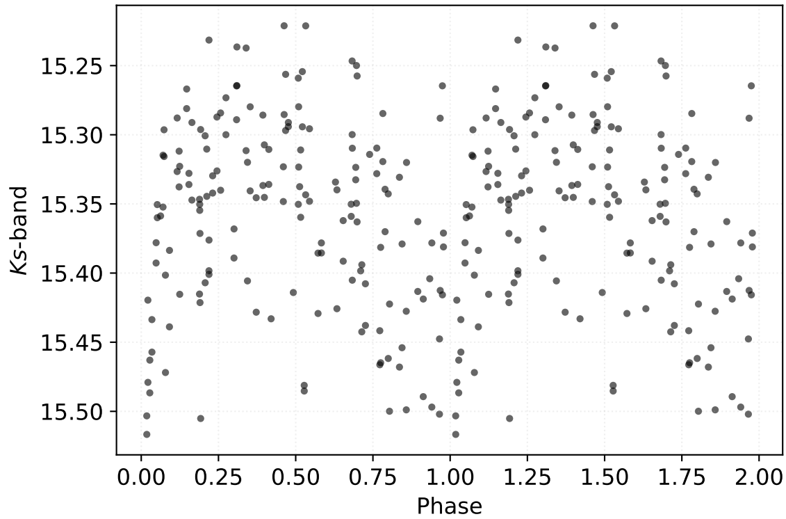
P: 3.64472 d | Class: RP | Subclass: CEP-F | Field b278
