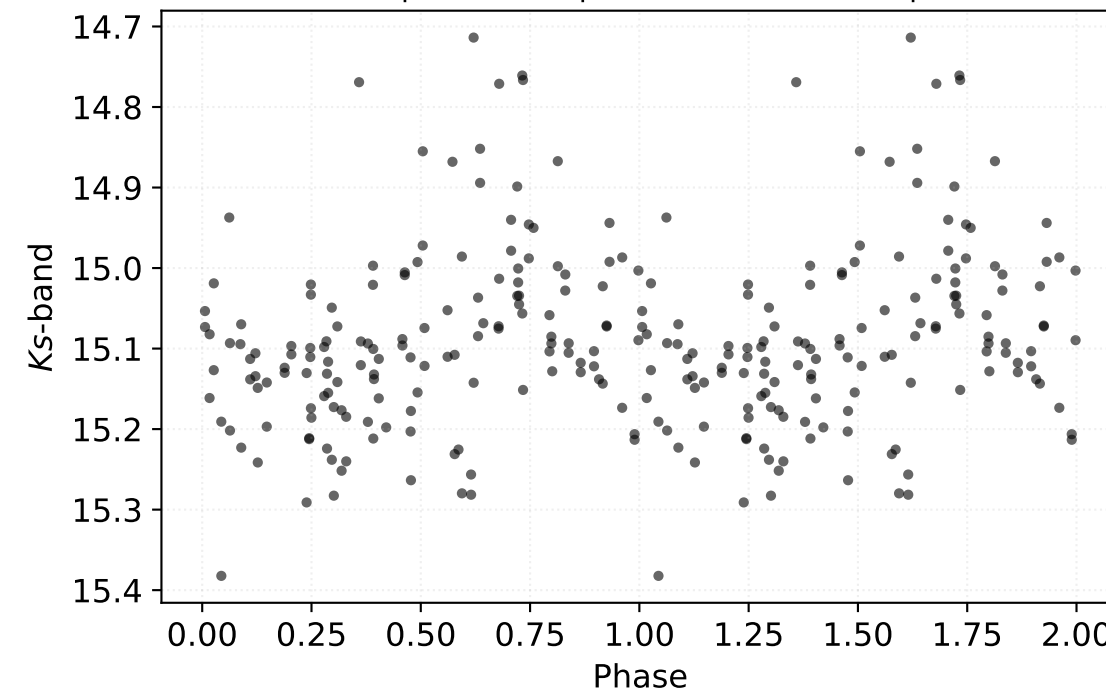
P: 0.24652 d | Class: RP | Subclass: CEP-1OT | Field b278
