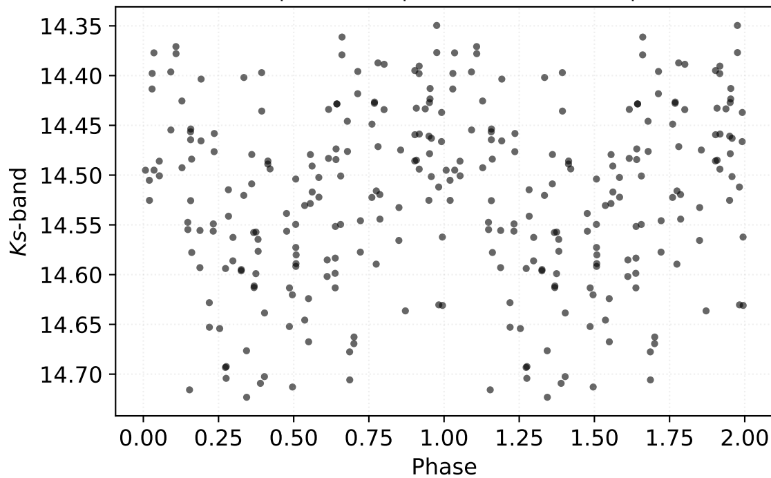
P: 2.85557 d | Class: RP | Subclass: CEP-1OT | Field b279
