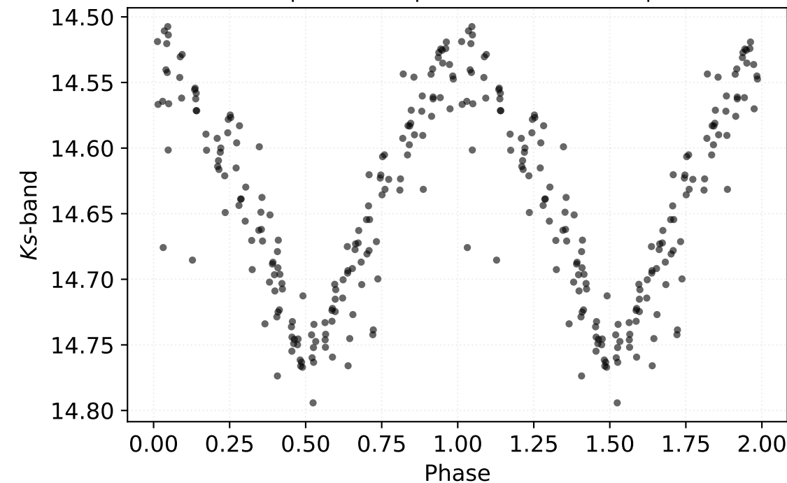
P: 0.61987 d | Class: RP | Subclass: CEP-1OT | Field b278
