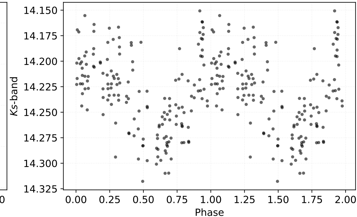
P: 0.30682 d | Class: RP | Subclass: RRab | Field b279
