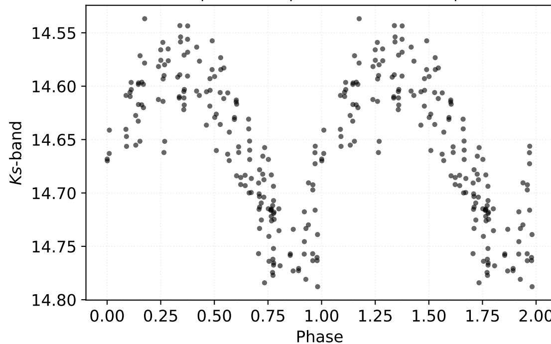
P: 3.25163 d | Class: RP | Subclass: CEP-1OT | Field b278
