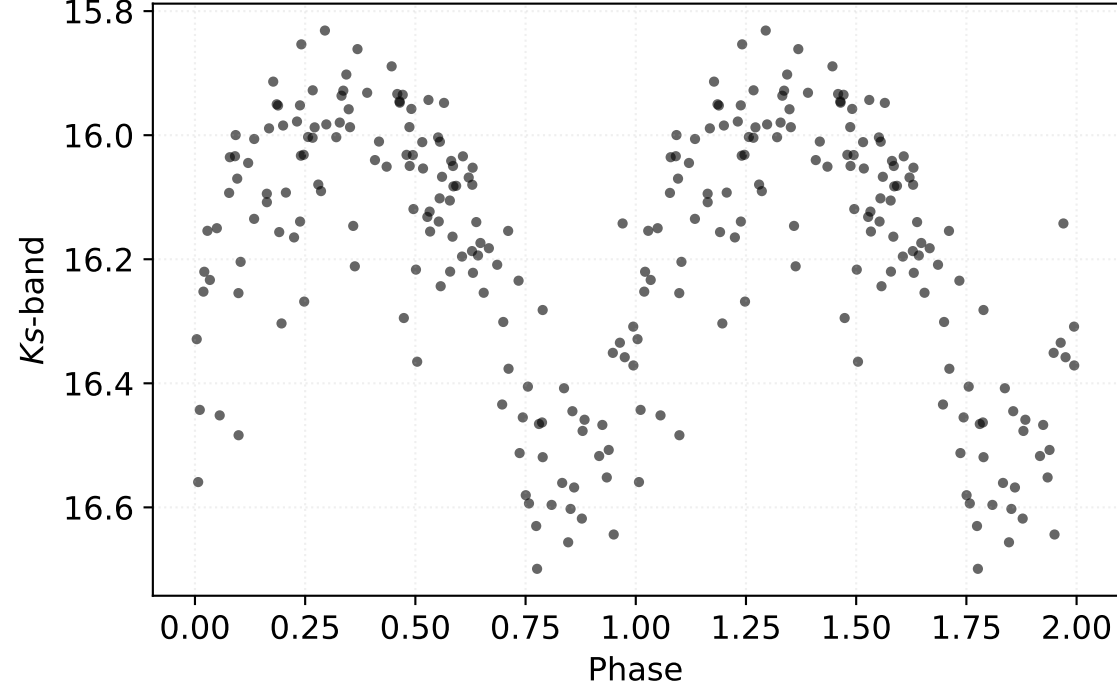
P: 0.17217 d | Class: RP | Subclass: UVAR | Field b278
