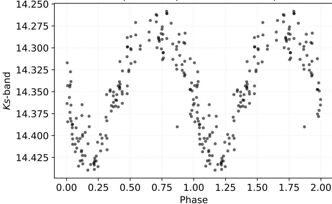
P: 5.06470 d | Class: RP | Subclass: CEP-1OT | Field b278
