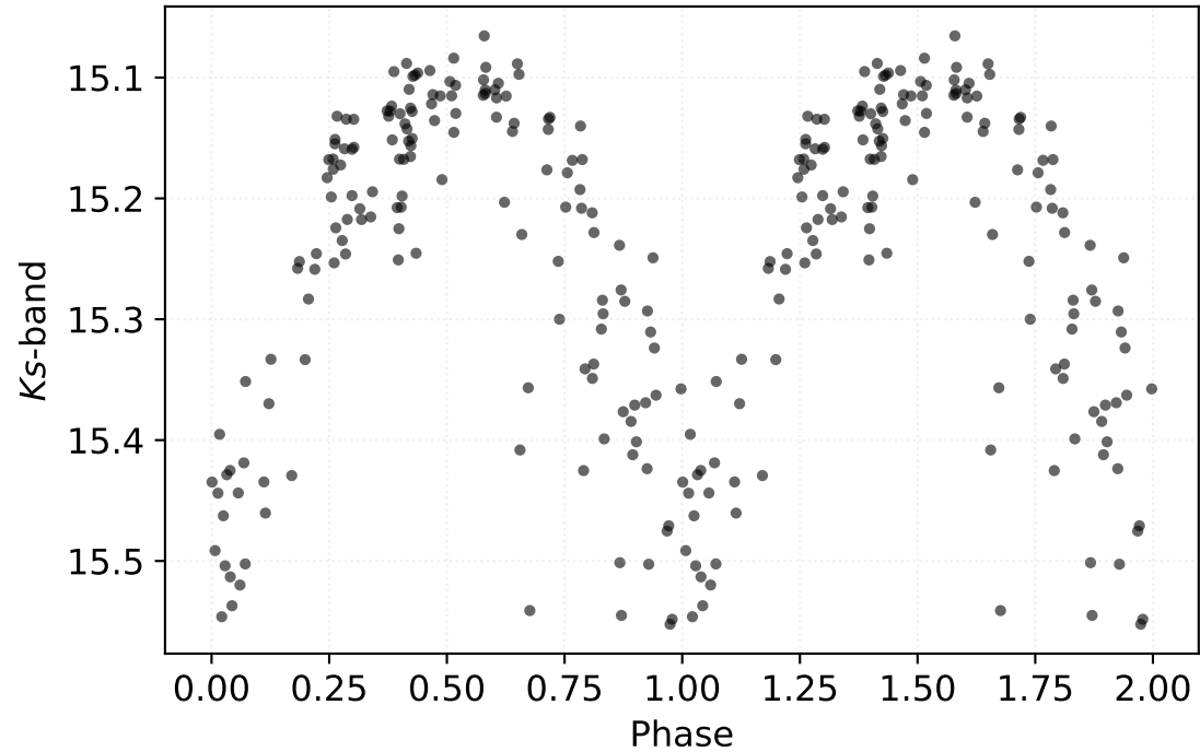
P: 0.19974 d | Class: RP | Subclass: UVAR | Field b279
