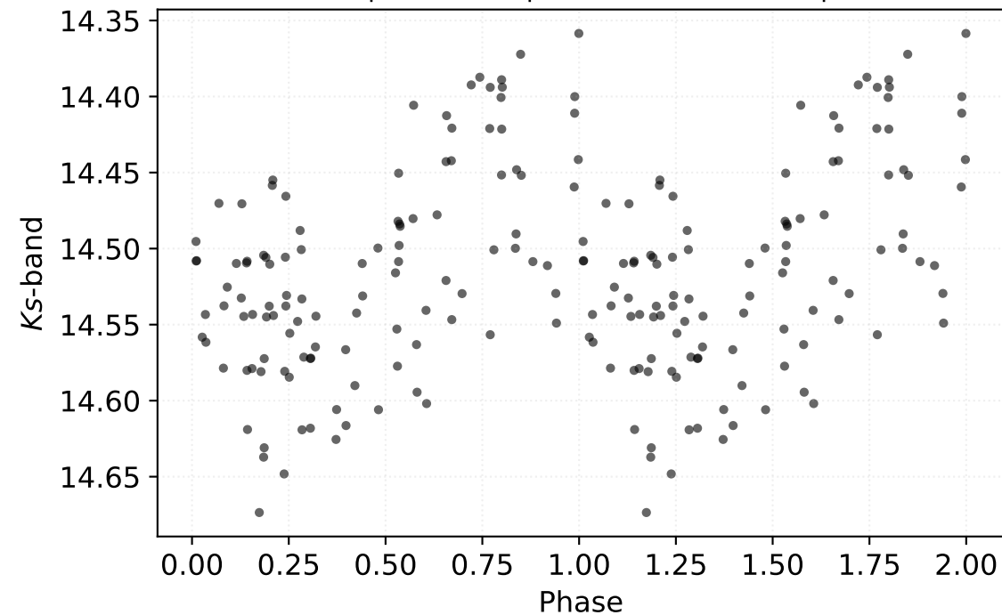
P: 0.50955 d | Class: RP | Subclass: CEP-1OT | Field b278
