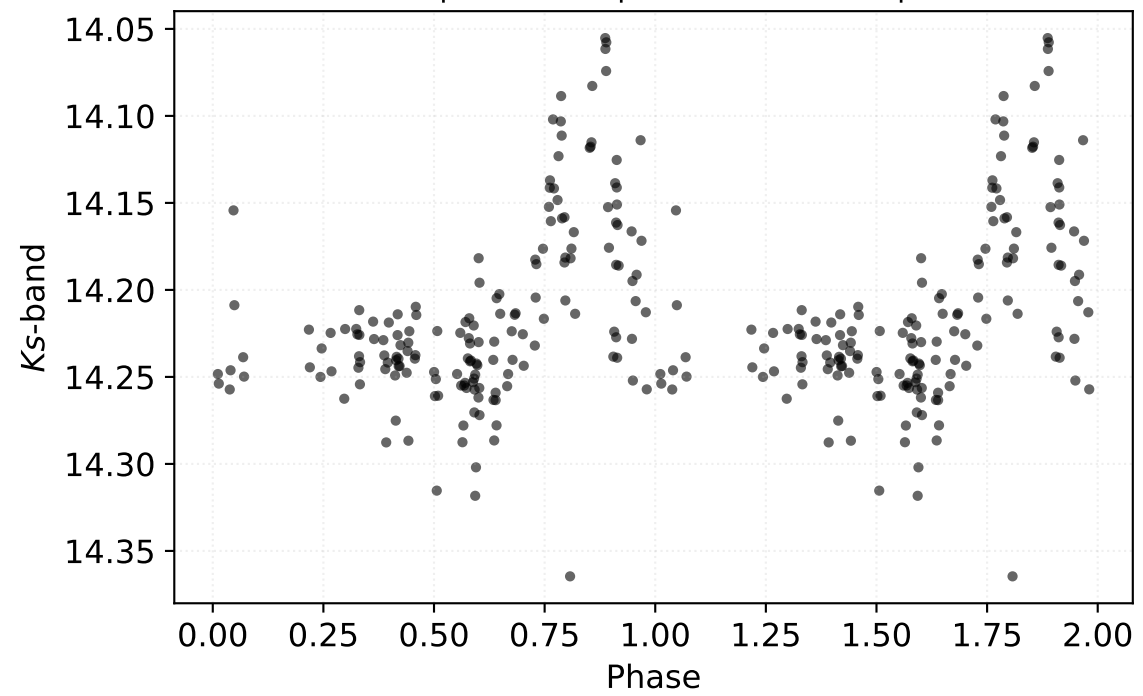
P: 44.22699 d | Class: RP | Subclass: UVAR | Field b279
