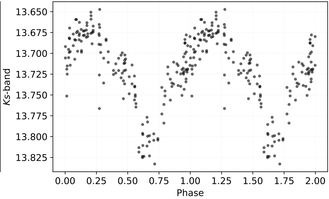
P: 0.38898 d | Class: RP | Subclass: CEP-1OT | Field b279
