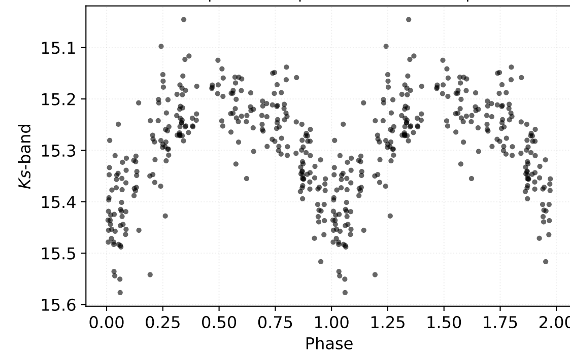
P: 0.35939 d | Class: RP | Subclass: CEP-1OT | Field b278
