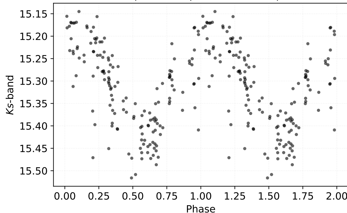
P: 0.21778 d | Class: RP | Subclass: UVAR | Field b279
