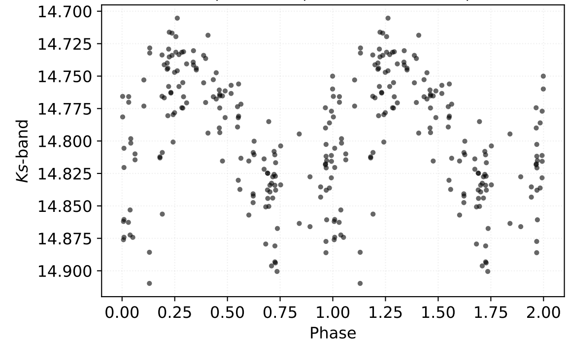
P: 0.24932 d | Class: RP | Subclass: CEP-1OT | Field b279
