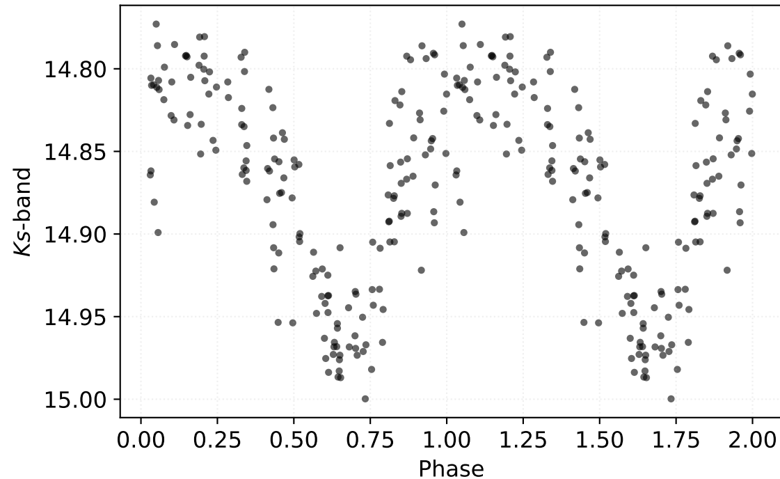
P: 13.92455 d | Class: RP | Subclass: UVAR | Field b279
