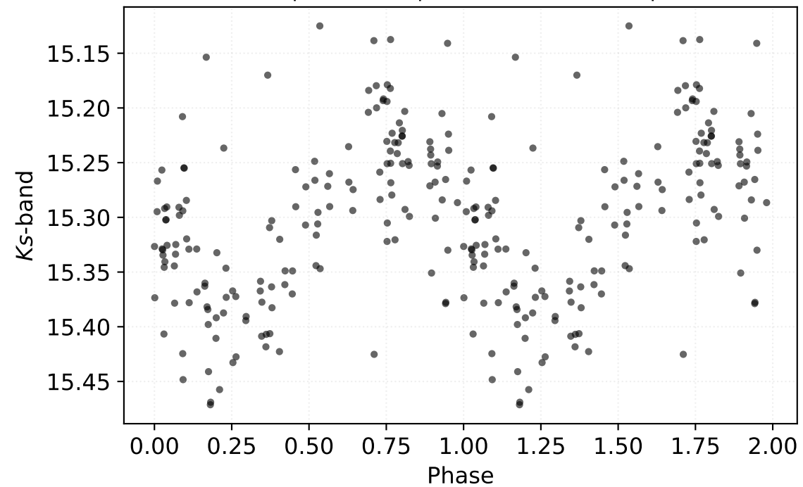
P: 0.31664 d | Class: RP | Subclass: CEP-1OT | Field b279
