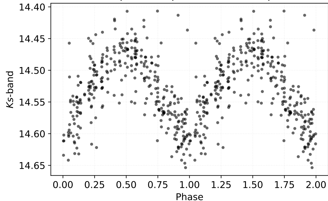
P: 3.19013 d | Class: RP | Subclass: CEP-1OT | Field b278
