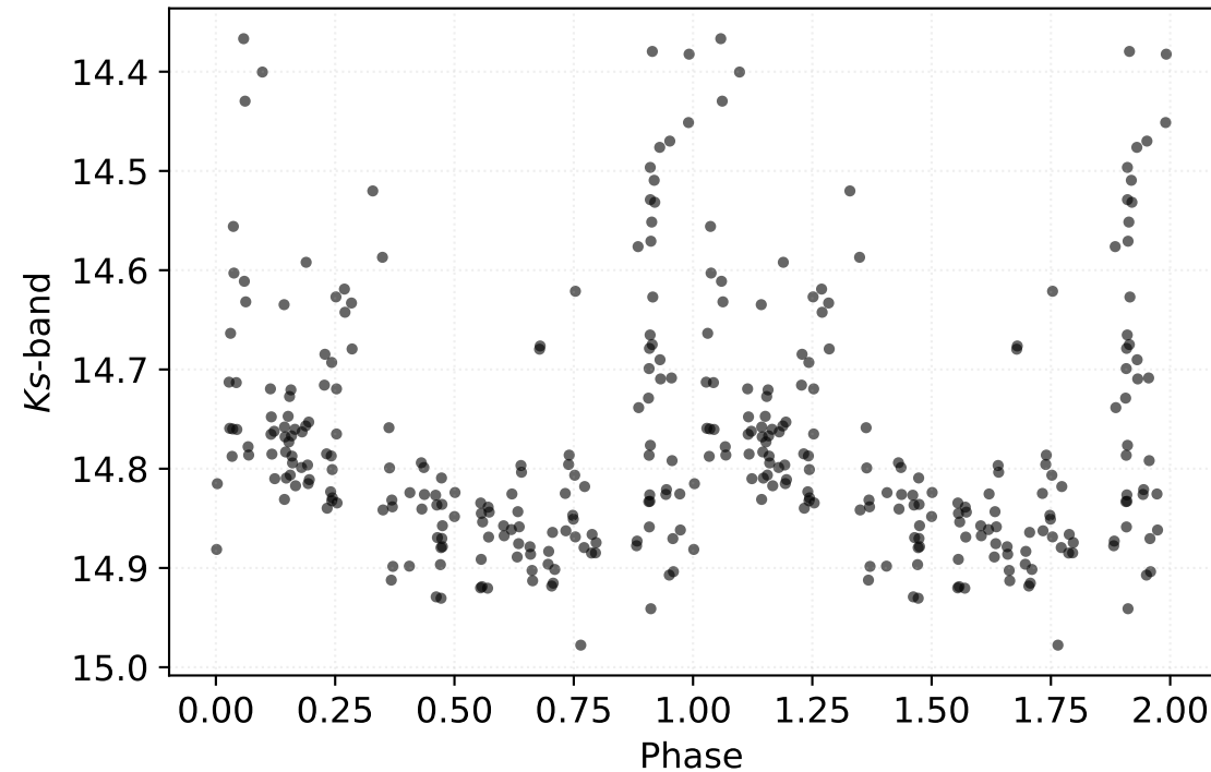
P: 0.29192 d | Class: RP | Subclass: RRc | Field b278
