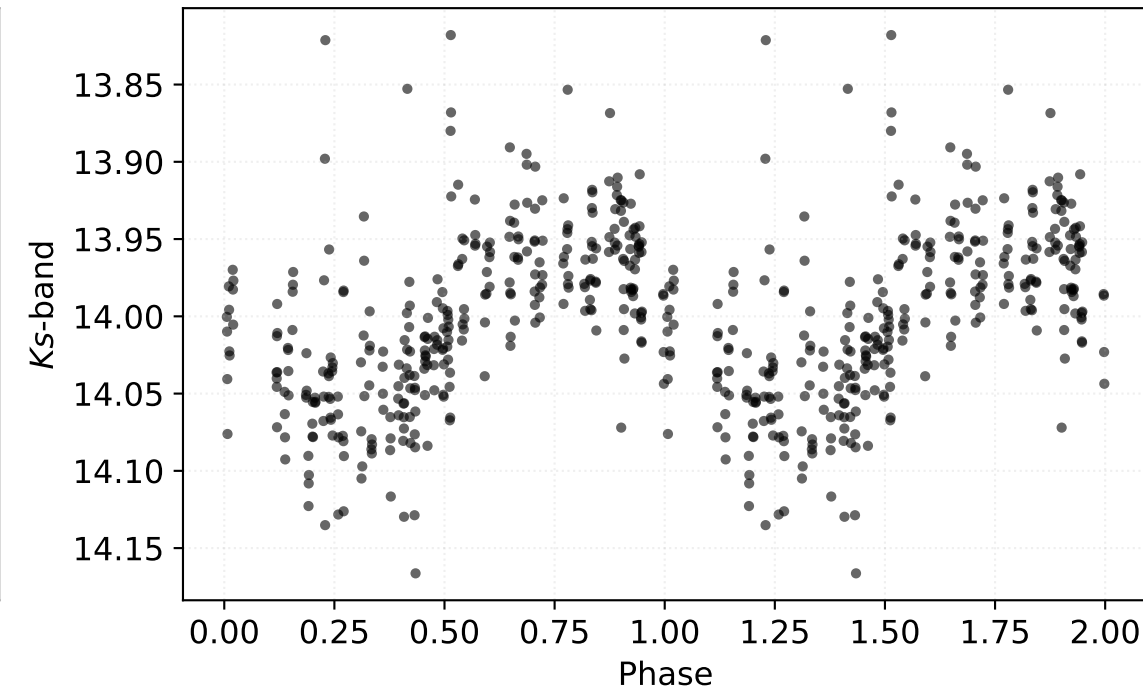
P: 0.54549 d | Class: RP | Subclass: RRab | Field b279
