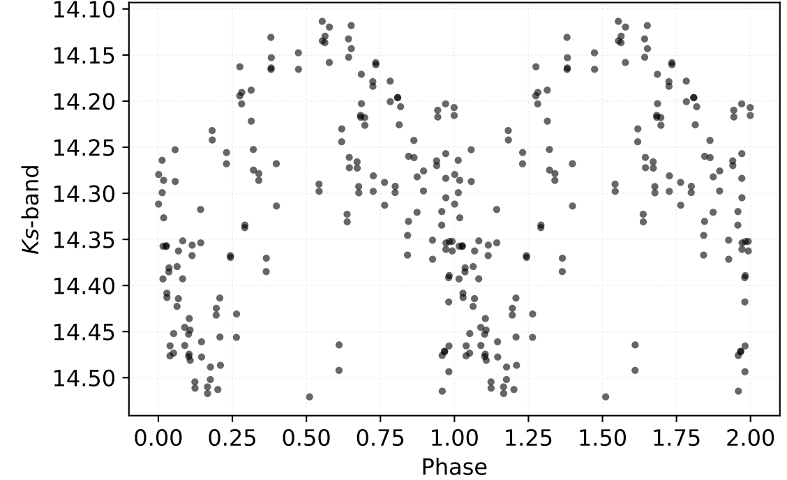
P: 1.07552 d | Class: RP | Subclass: CEP-F | Field b278
