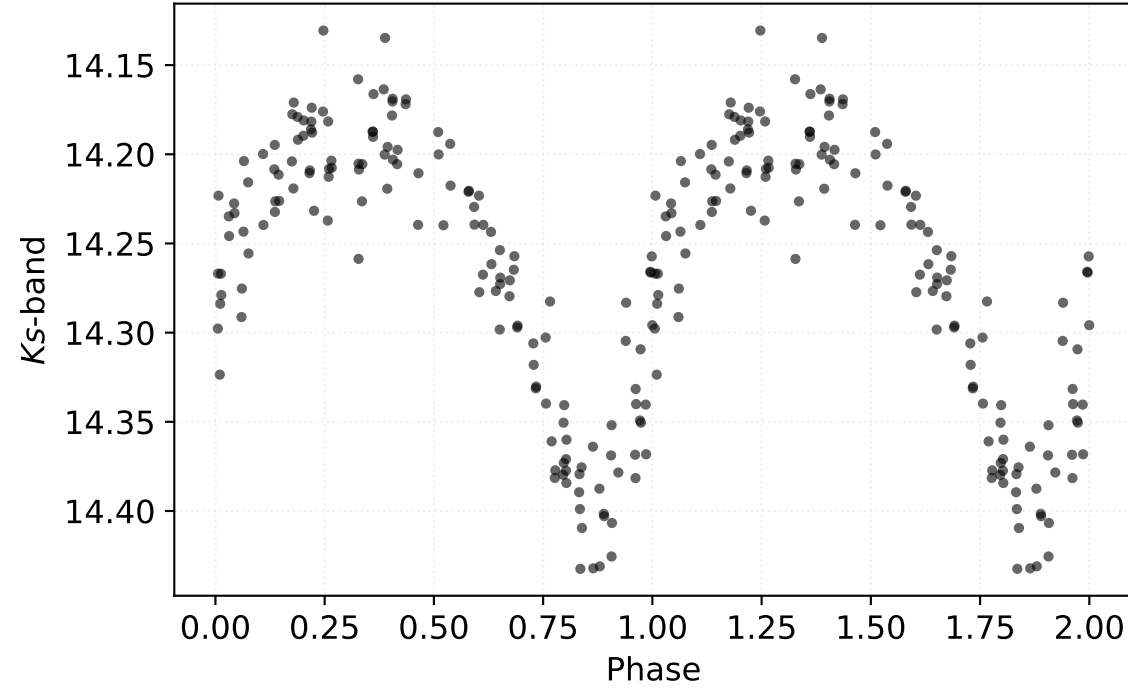
P: 0.45696 d | Class: RP | Subclass: RRc | Field b278
