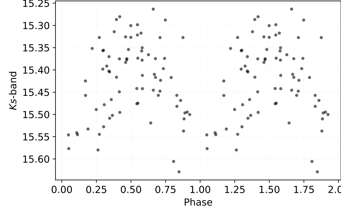
P: 0.51295 d | Class: RP | Subclass: RRab | Field b278
