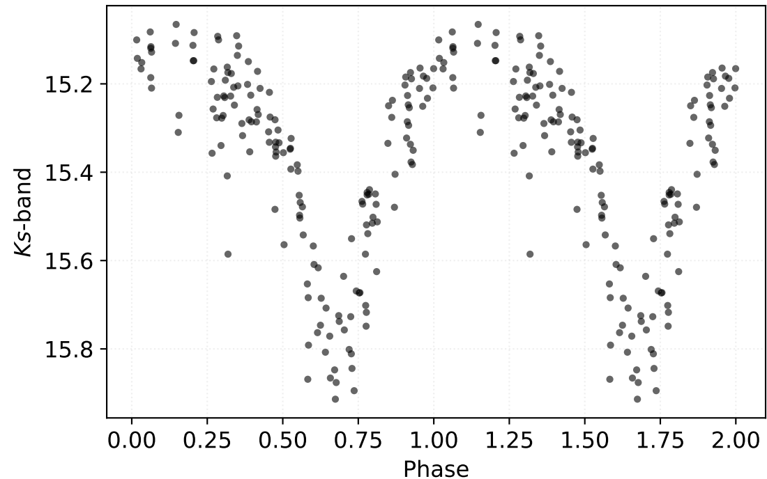
P: 0.21638 d | Class: RP | Subclass: UVAR | Field b279
