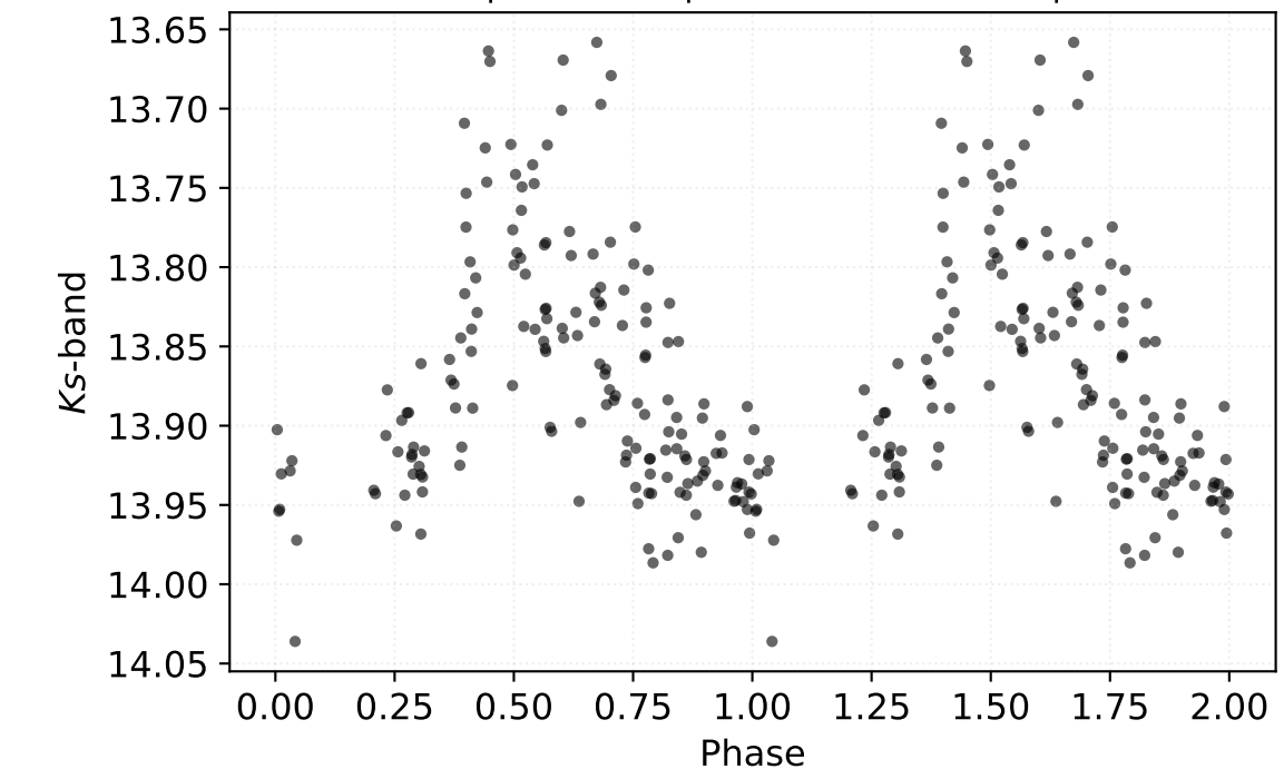
P: 0.99948 d | Class: RP | Subclass: CEP-1OT | Field b279
