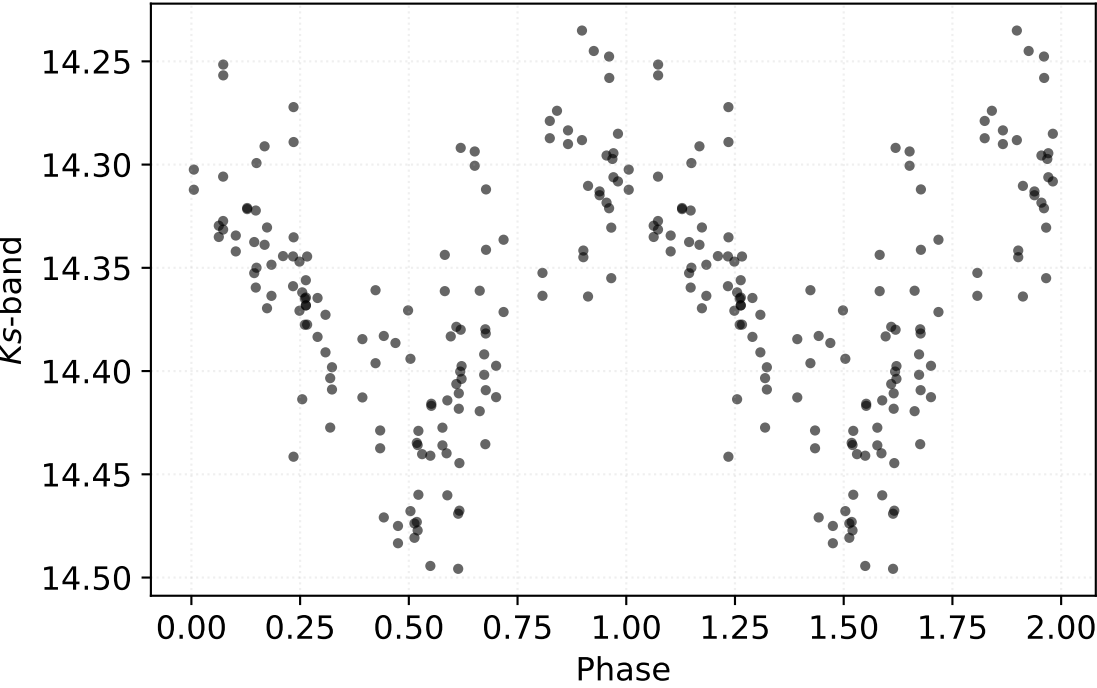
P: 36.42237 d | Class: RP | Subclass: UVAR | Field b279
