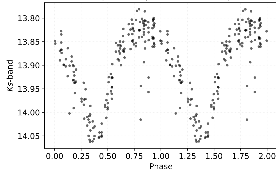
P: 0.61075 d | Class: RP | Subclass: CEP-1OT | Field b278
