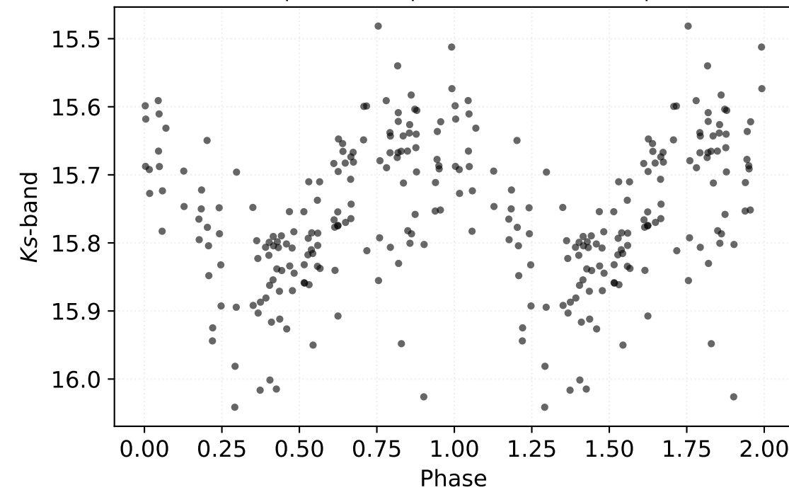
P: 4.62840 d | Class: RP | Subclass: CEP-1OT | Field b278
