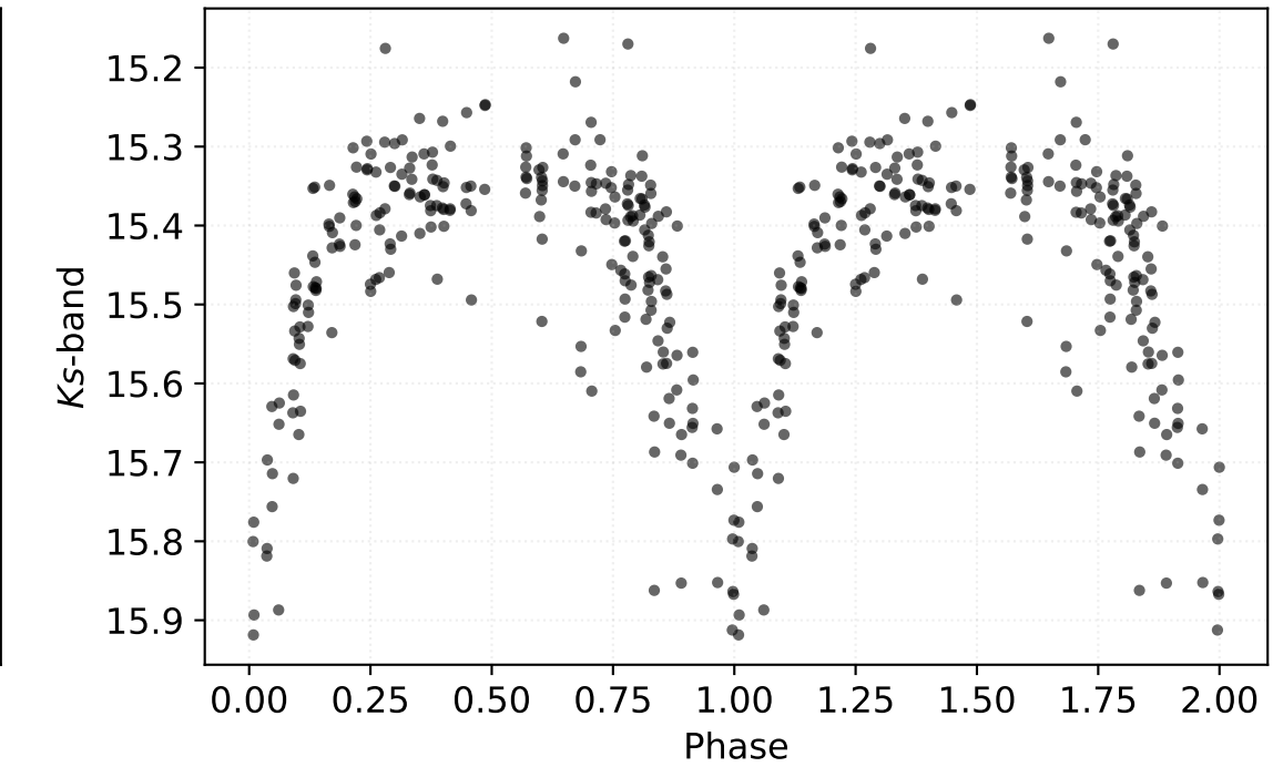
P: 0.67088 d | Class: RP | Subclass: CEP-1OT | Field b278
