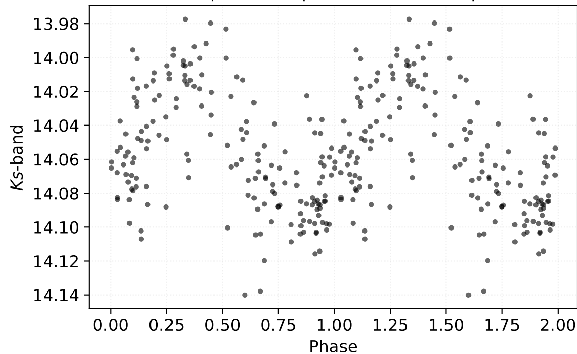
P: 0.54558 d | Class: RP | Subclass: CEP-1OT | Field b278
