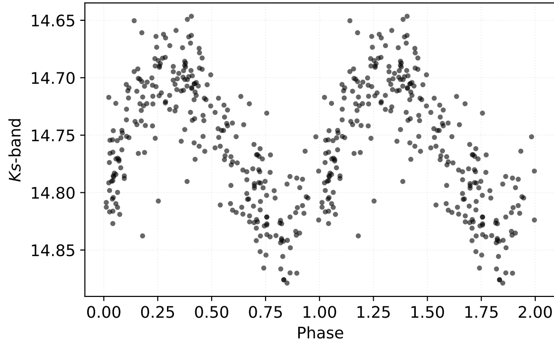
P: 0.64338 d | Class: RP | Subclass: CEP-1OT | Field b278
