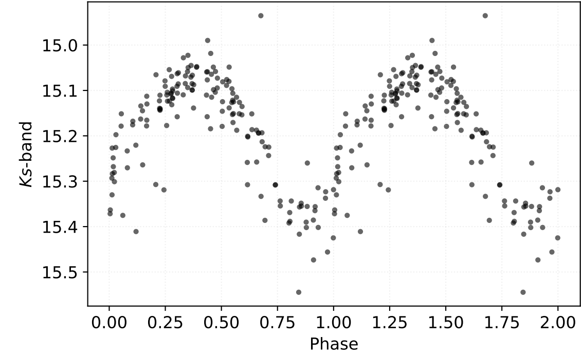
P: 0.49179 d | Class: RP | Subclass: RRab | Field b278
