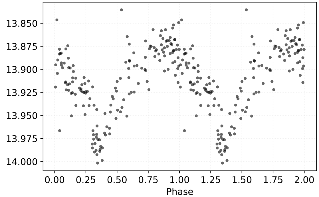
P: 5.17047 d | Class: RP | Subclass: CEP-1OT | Field b278
