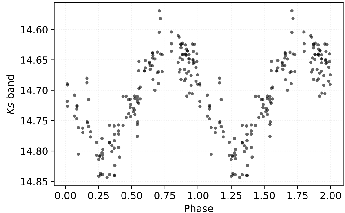
P: 34.07012 d | Class: RP | Subclass: CEP-F | Field b278
