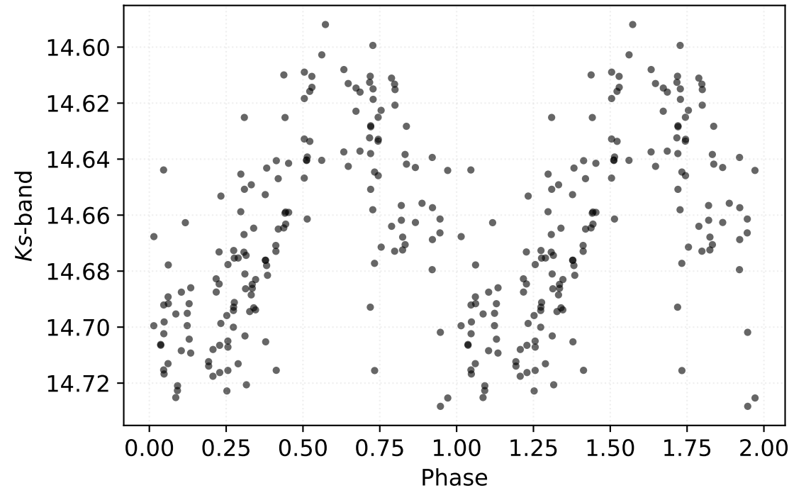
P: 3.81668 d | Class: RP | Subclass: CEP-F | Field b278
