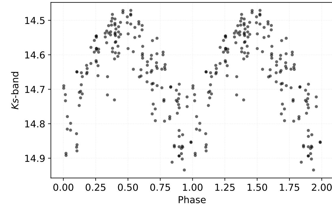
P: 0.46061 d | Class: RP | Subclass: CEP-1OT | Field b278
