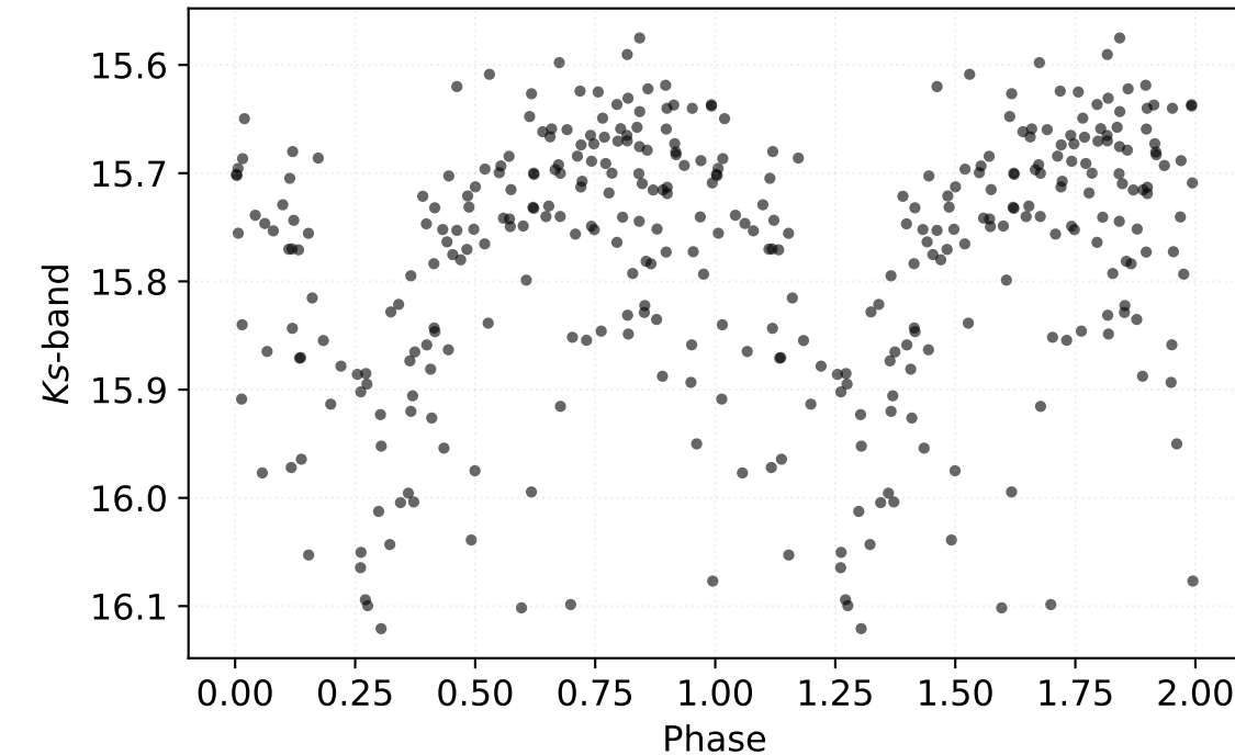
P: 0.24838 d | Class: RP | Subclass: CEP-1OT | Field b278
