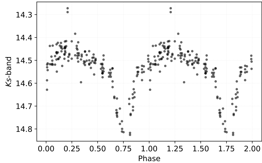
P: 0.71096 d | Class: RP | Subclass: CEP-1OT | Field b279
