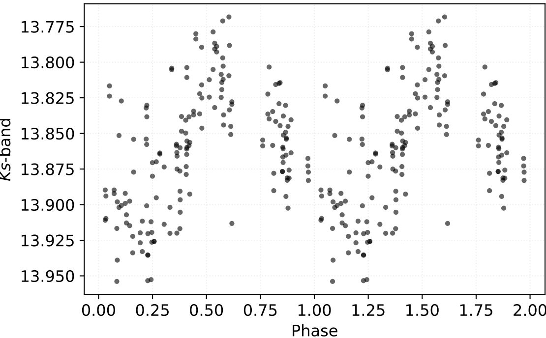
P: 69.34999 d | Class: RP | Subclass: CEP-F | Field b279
