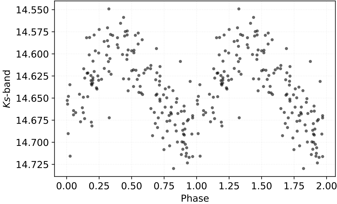
P: 0.36760 d | Class: RP | Subclass: RRab | Field b278
