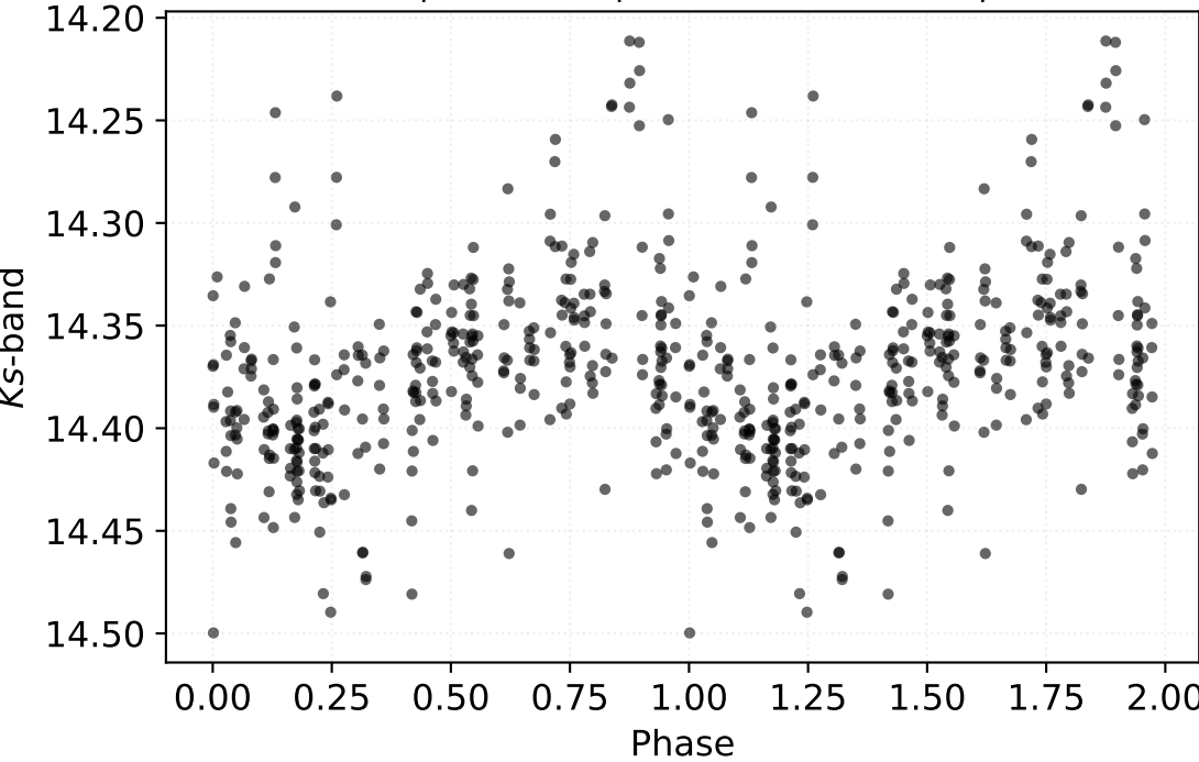
P: 1.41548 d | Class: RP | Subclass: CEP-1OT | Field b279
