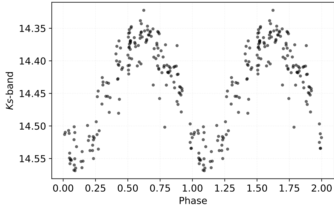
P: 0.21621 d | Class: RP | Subclass: UVAR | Field b278
