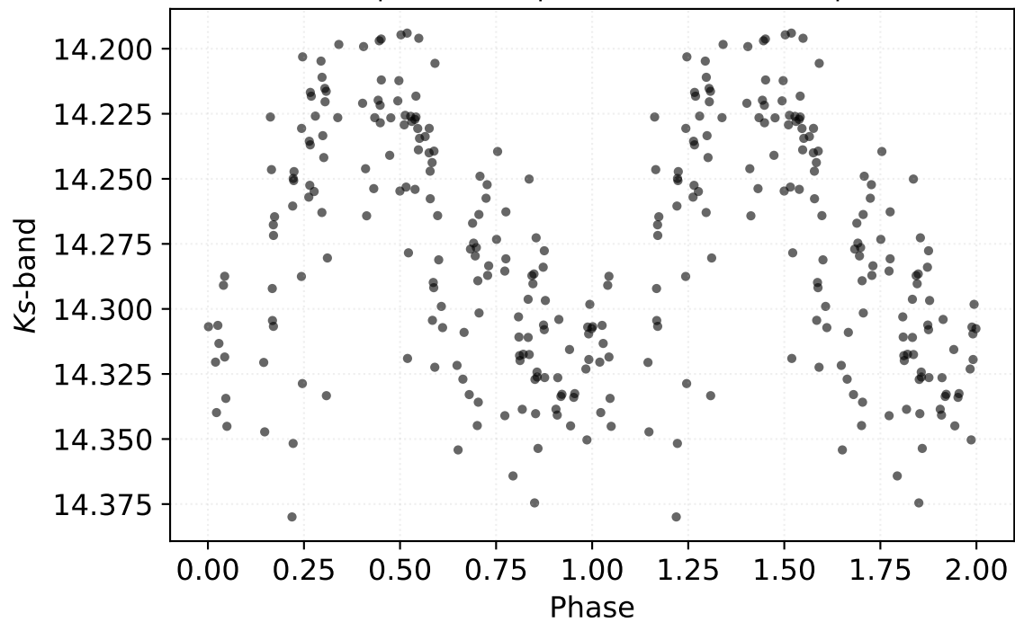
P: 0.40223 d | Class: RP | Subclass: CEP-1OT | Field b278
