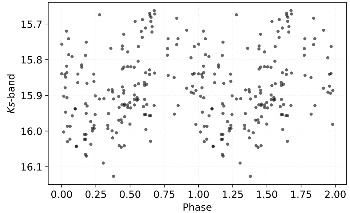
P: 0.44264 d | Class: RP | Subclass: RRab | Field b279
