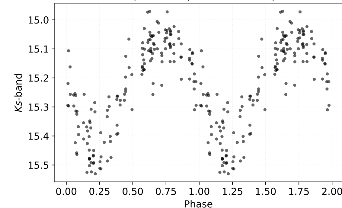
P: 0.15092 d | Class: RP | Subclass: UVAR | Field b279
