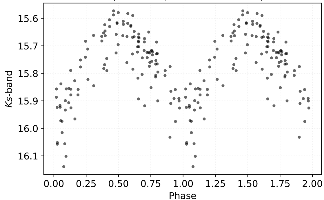
P: 0.45102 d | Class: RP | Subclass: CEP-1OT | Field b278
