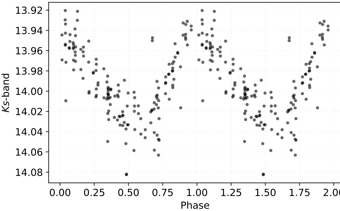
P: 0.49101 d | Class: RP | Subclass: CEP-1OT | Field b278
