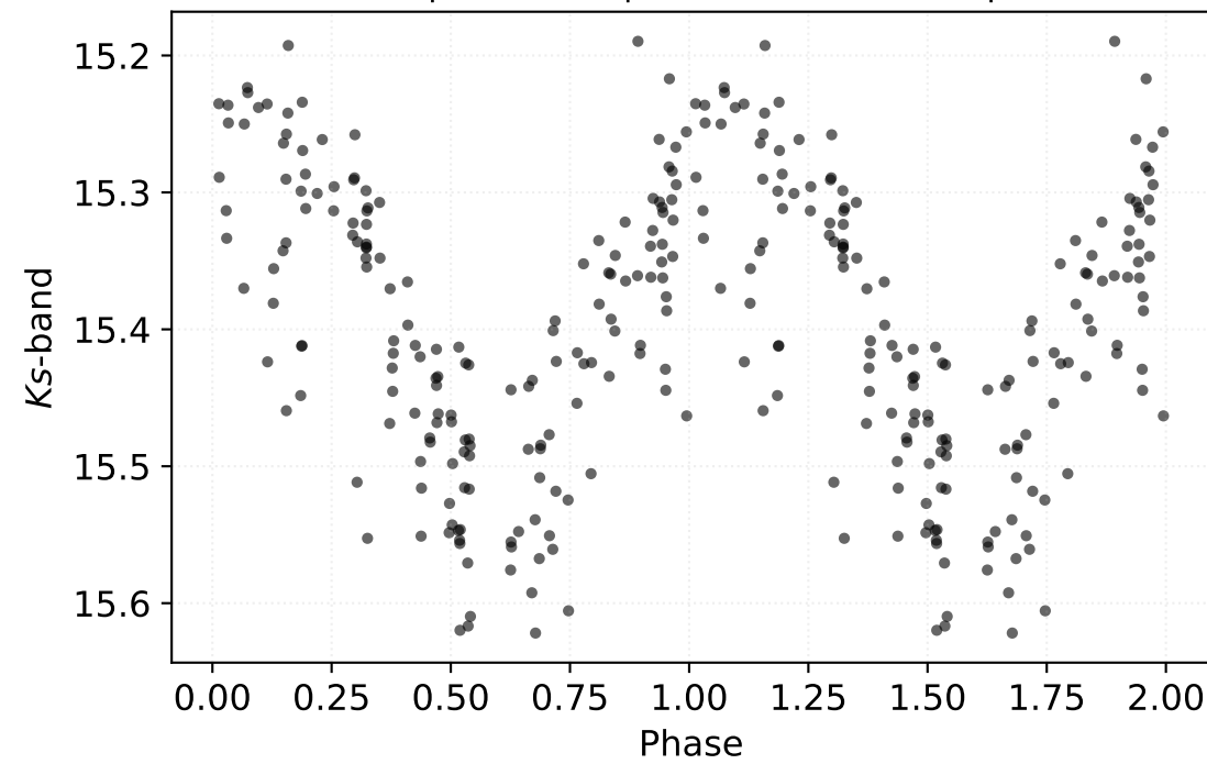
P: 0.67699 d | Class: RP | Subclass: CEP-1OT | Field b278
