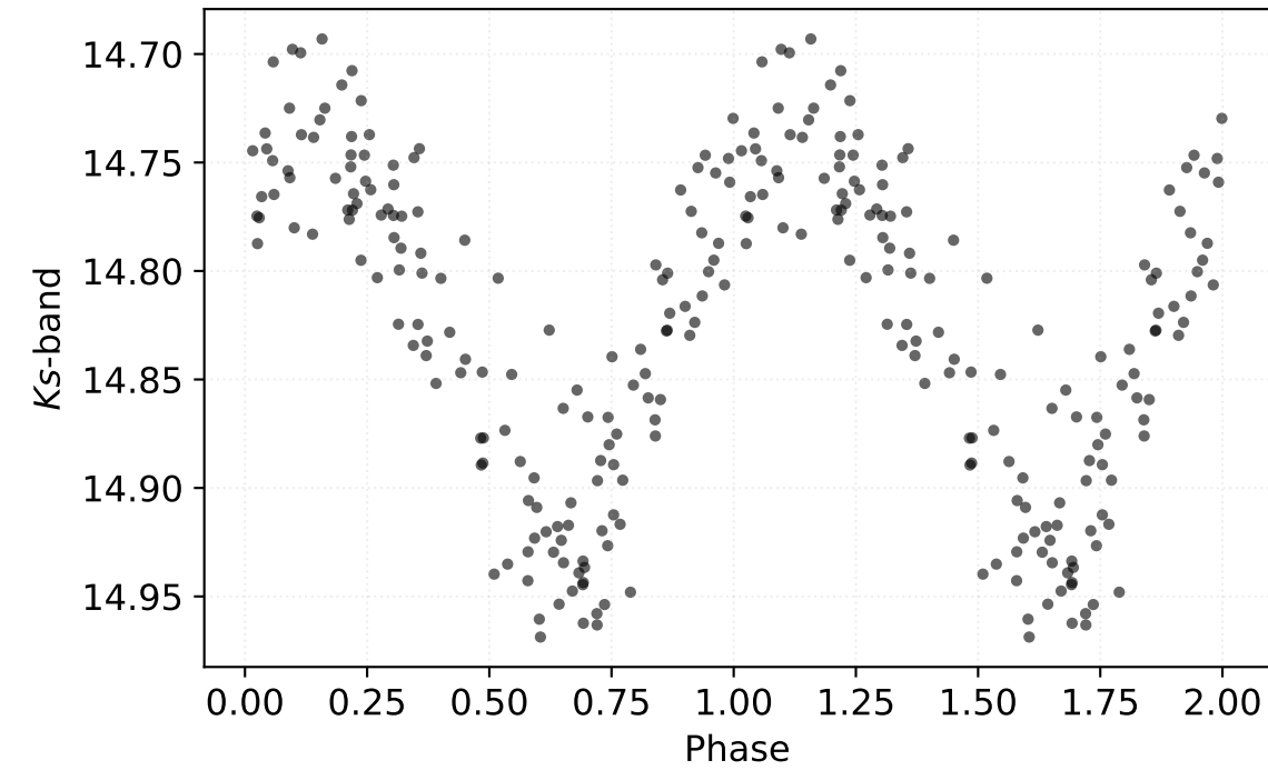
P: 0.20730 d | Class: RP | Subclass: RRc | Field b279
