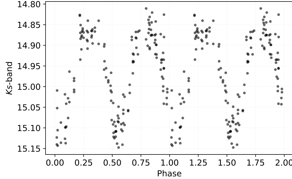
P: 0.20424 d | Class: RP | Subclass: RRc | Field b279
