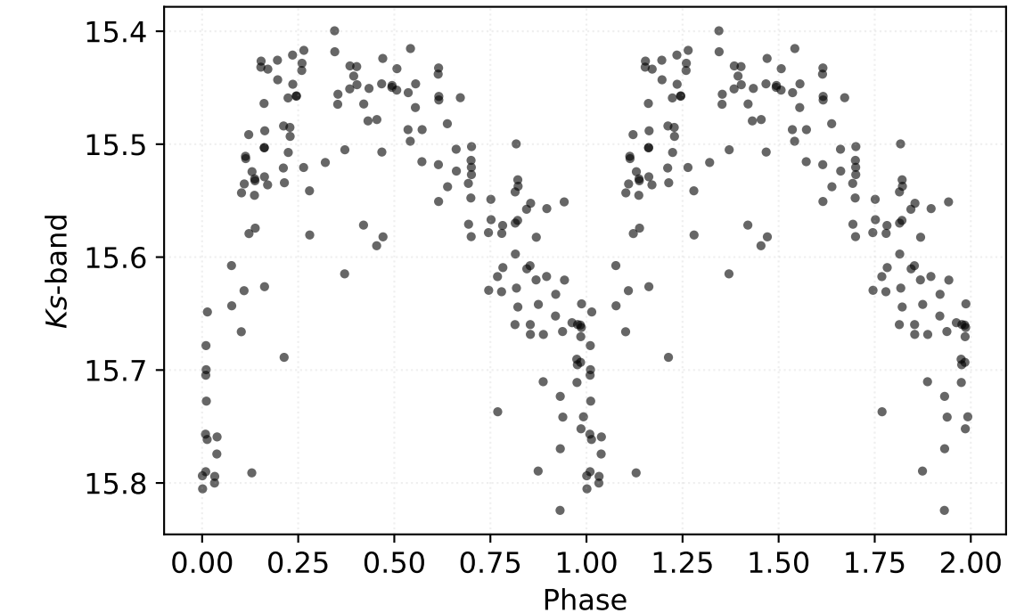
P: 0.68154 d | Class: RP | Subclass: RRab | Field b278
