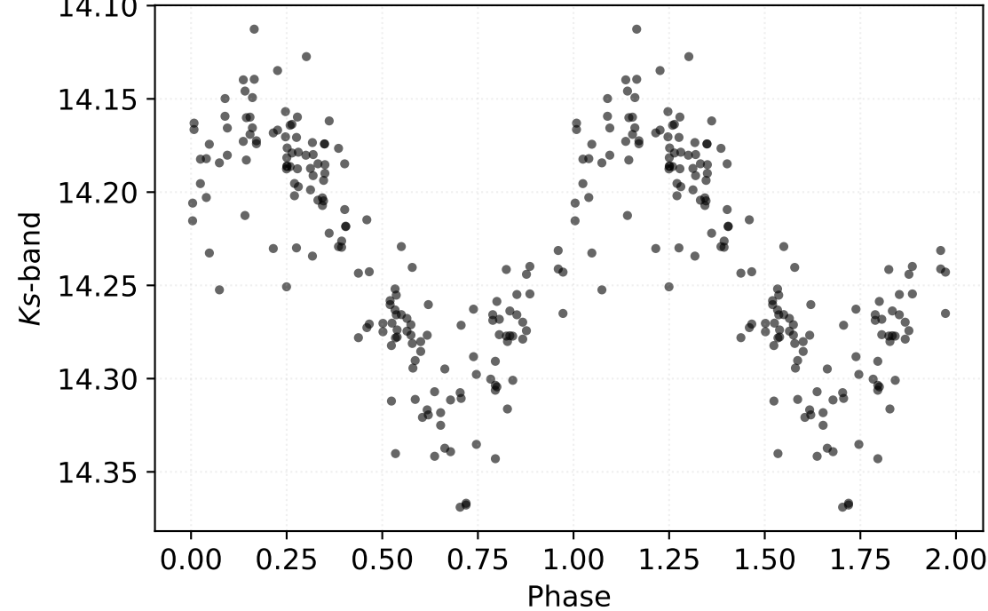
P: 3.86075 d | Class: RP | Subclass: CEP-F | Field b278
