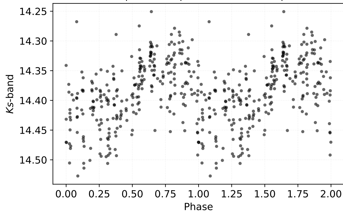
P: 4.40738 d | Class: RP | Subclass: CEP-1OT | Field b279
