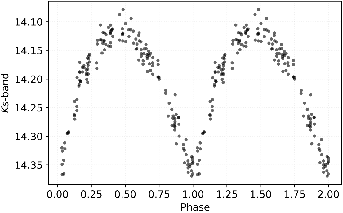
P: 0.68767 d | Class: RP | Subclass: CEP-1OT | Field b278
