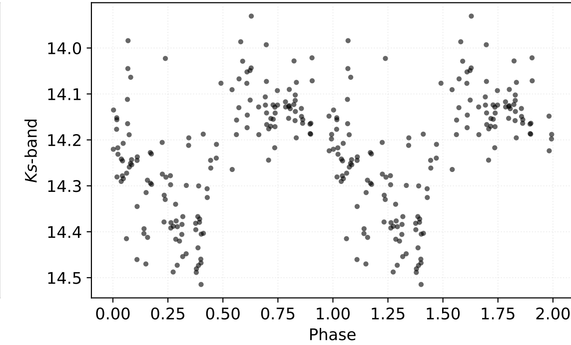
P: 0.33903 d | Class: RP | Subclass: RRab | Field b279
