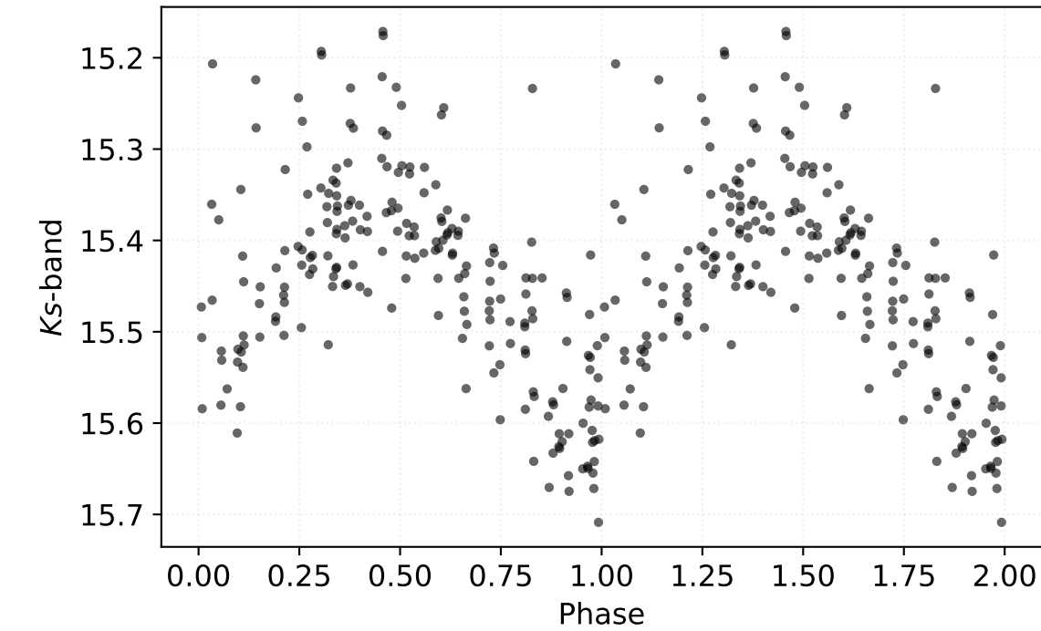
P: 0.42486 d | Class: RP | Subclass: RRab | Field b279
