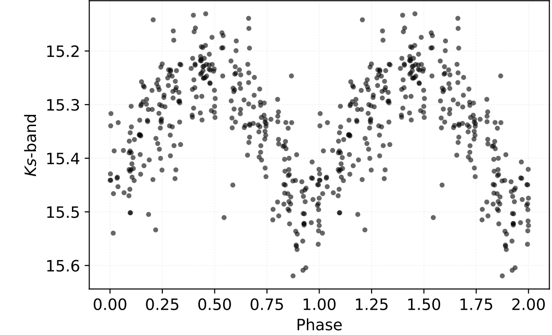
P: 0.47402 d | Class: RP | Subclass: RRab | Field b278
