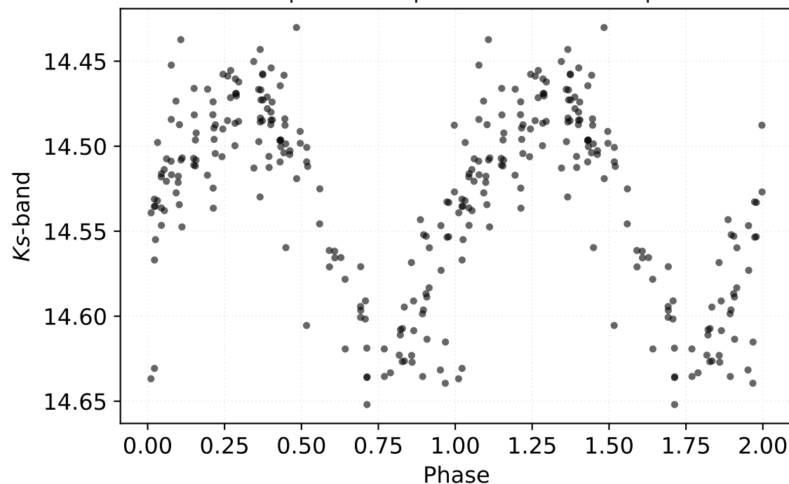
P: 0.39964 d | Class: RP | Subclass: CEP-1OT | Field b278
