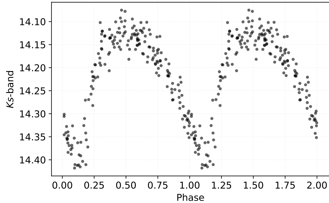
P: 0.44857 d | Class: RP | Subclass: RRab | Field b278
