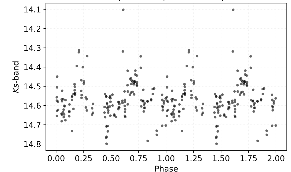
P: 27.94427 d | Class: EB | Subclass: EA | Field b278
