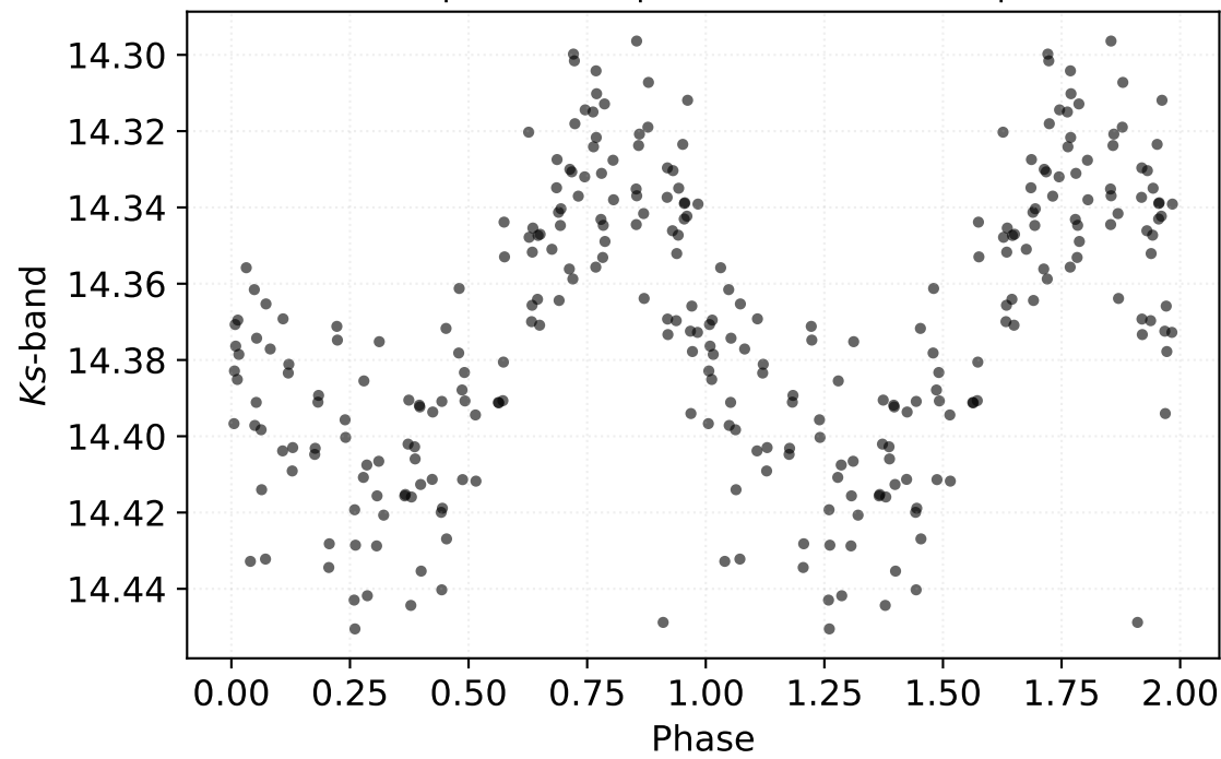
P: 9.03023 d | Class: RP | Subclass: CEP-1OT | Field b278
