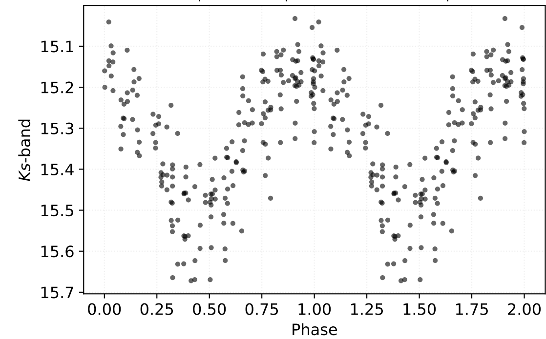
P: 0.34627 d | Class: RP | Subclass: CEP-1OT | Field b278
