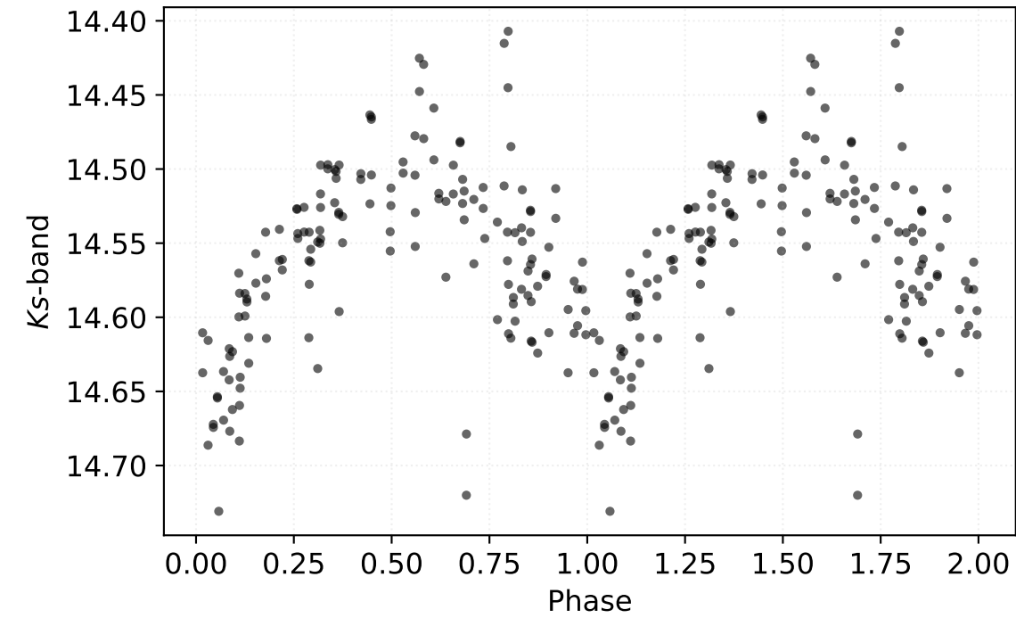
P: 5.96123 d | Class: RP | Subclass: CEP-1OT | Field b279
