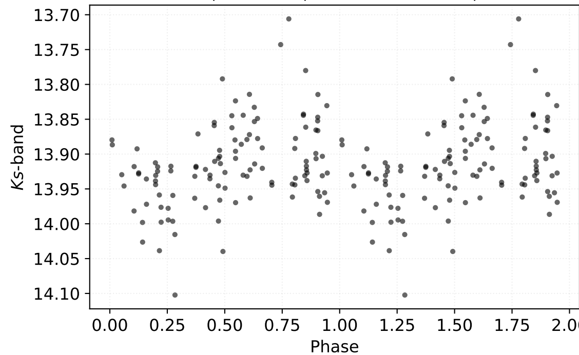
P: 0.59411 d | Class: RP | Subclass: CEP-1OT | Field b278
