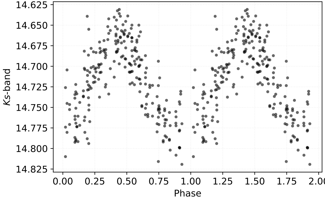
P: 26.72649 d | Class: RP | Subclass: CEP-F | Field b278
