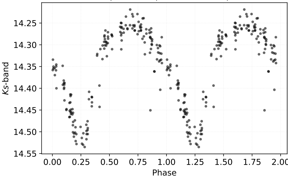
P: 0.42692 d | Class: RP | Subclass: RRab | Field b278
