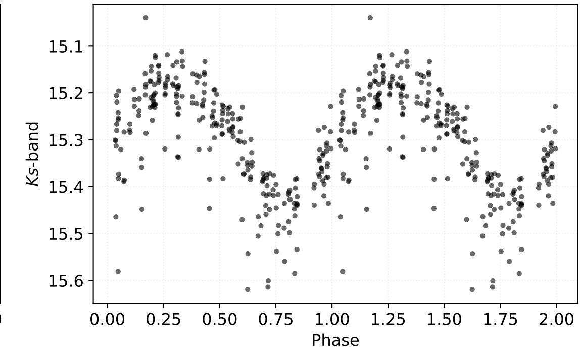
P: 2.14301 d | Class: RP | Subclass: CEP-1OT | Field b279
