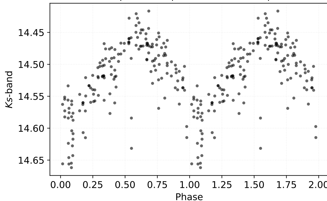
P: 0.70784 d | Class: RP | Subclass: CEP-1OT | Field b278
