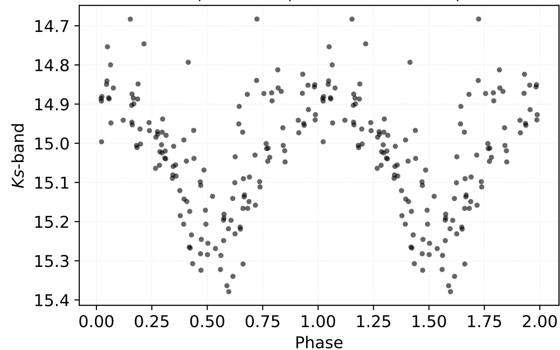
P: 0.32160 d | Class: RP | Subclass: CEP-1OT | Field b278
