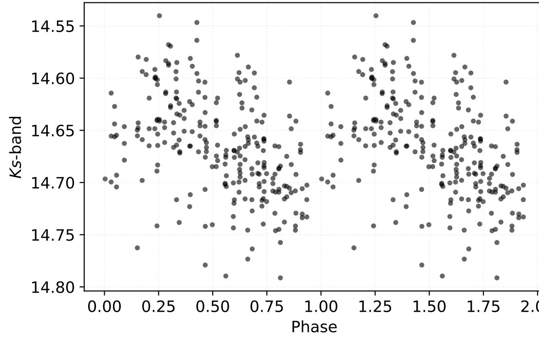
P: 0.33273 d | Class: RP | Subclass: CEP-1OT | Field b279
