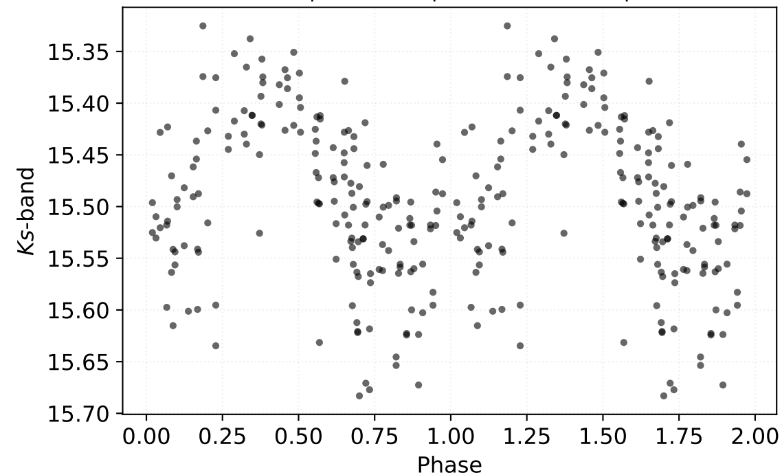
P: 0.19259 d | Class: RP | Subclass: UVAR | Field b279
