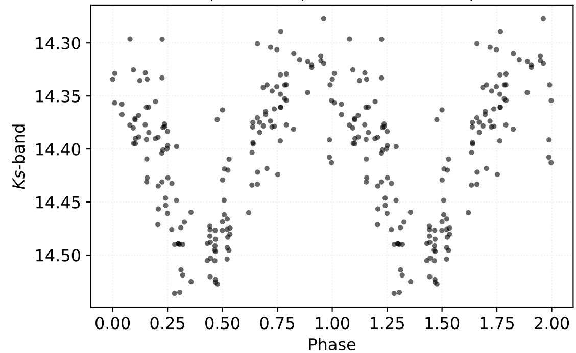
P: 0.35463 d | Class: RP | Subclass: CEP-1OT | Field b279
