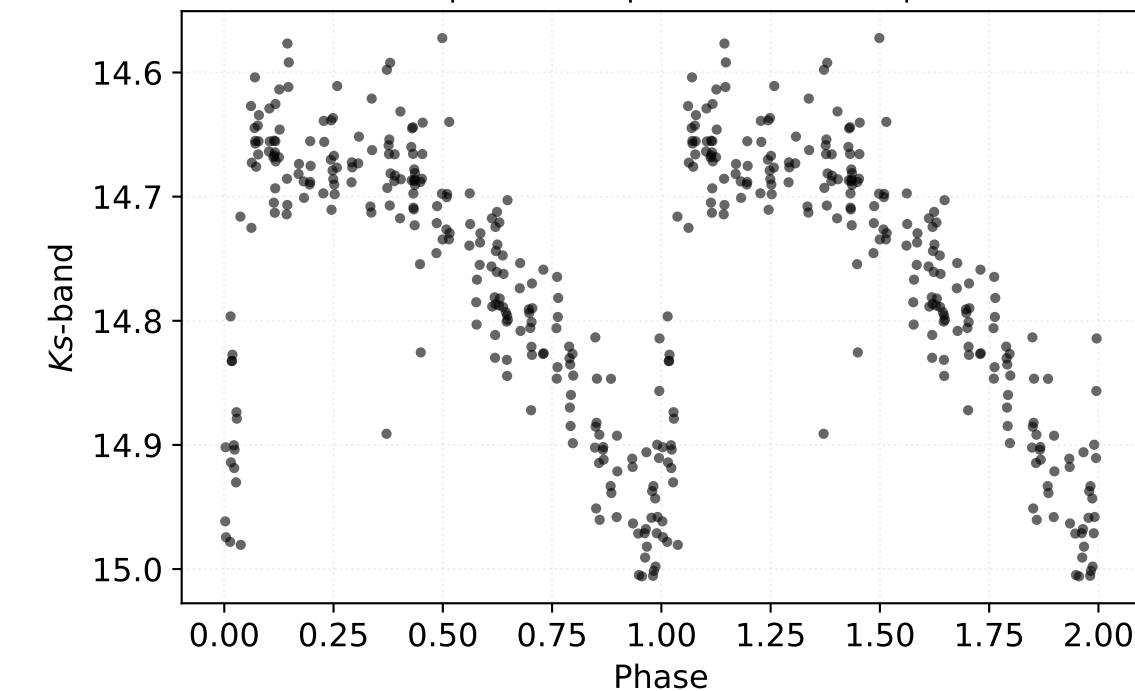
P: 0.50462 d | Class: RP | Subclass: RRab | Field b279
