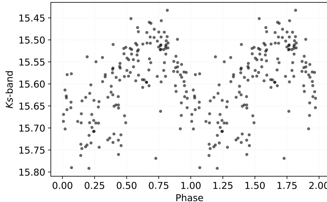
P: 7.10652 d | Class: RP | Subclass: CEP-1OT | Field b278
