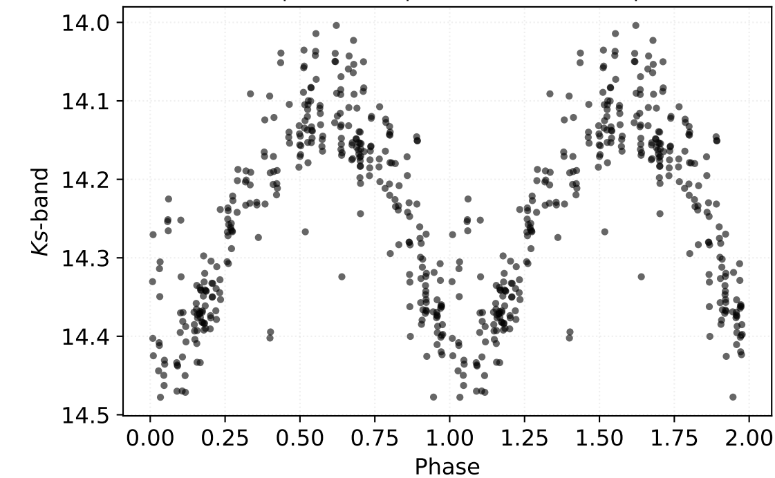
P: 0.40295 d | Class: RP | Subclass: CEP-1OT | Field b278
