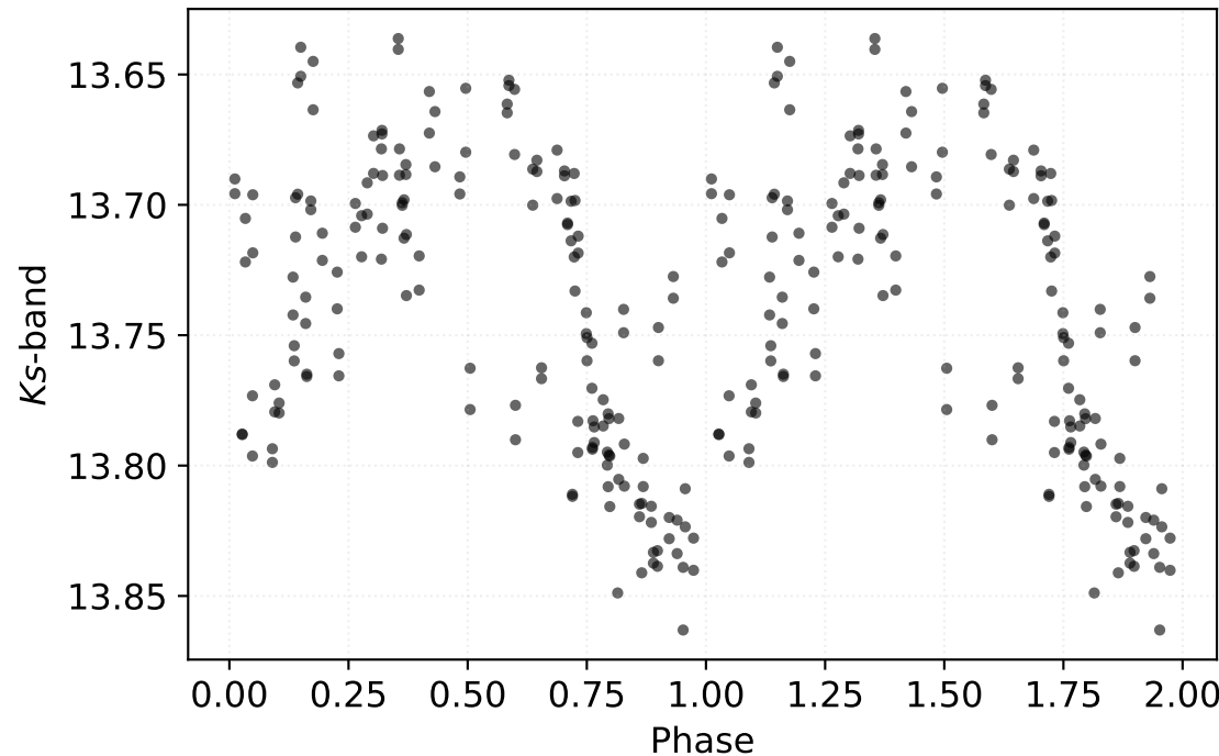
P: 3.08503 d | Class: RP | Subclass: CEP-F | Field b279
