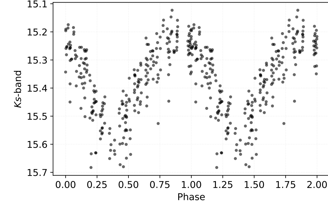
P: 0.20890 d | Class: RP | Subclass: UVAR | Field b278
