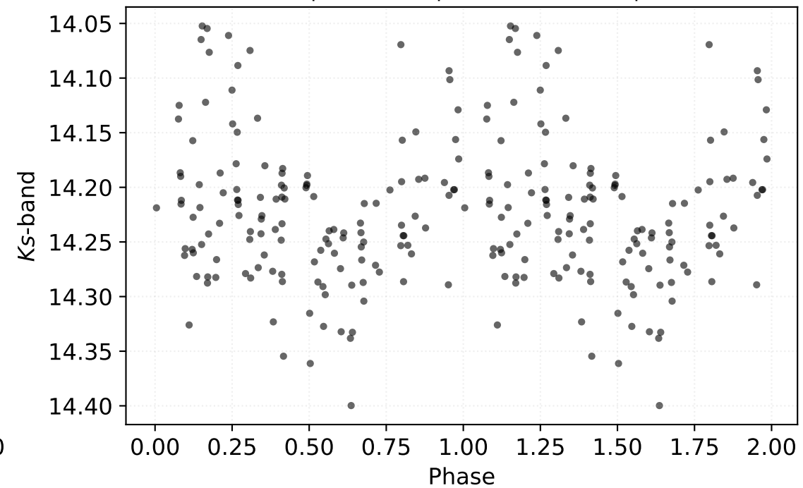
P: 19.33445 d | Class: RP | Subclass: UVAR | Field b279
