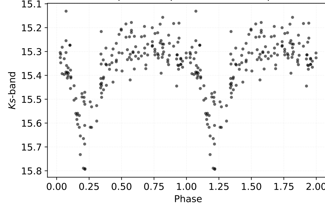
P: 1.42002 d | Class: RP | Subclass: CEP-1OT | Field b278
