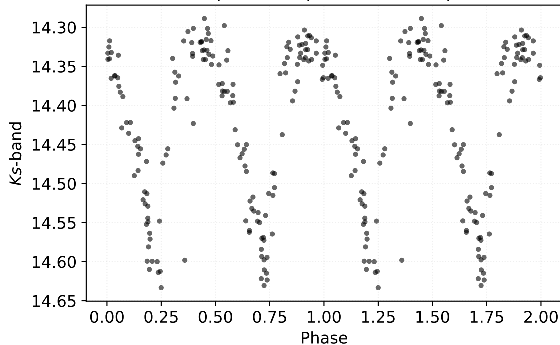
P: 0.17362 d | Class: RP | Subclass: UVAR | Field b279
