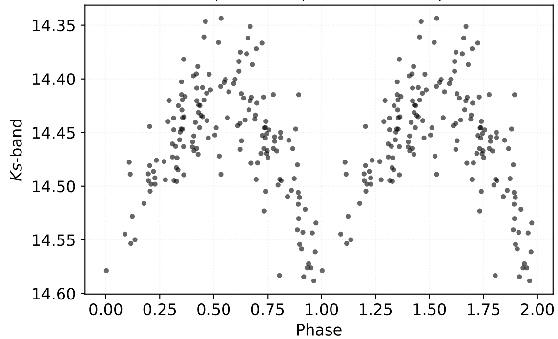
P: 45.77135 d | Class: RP | Subclass: UVAR | Field b279
