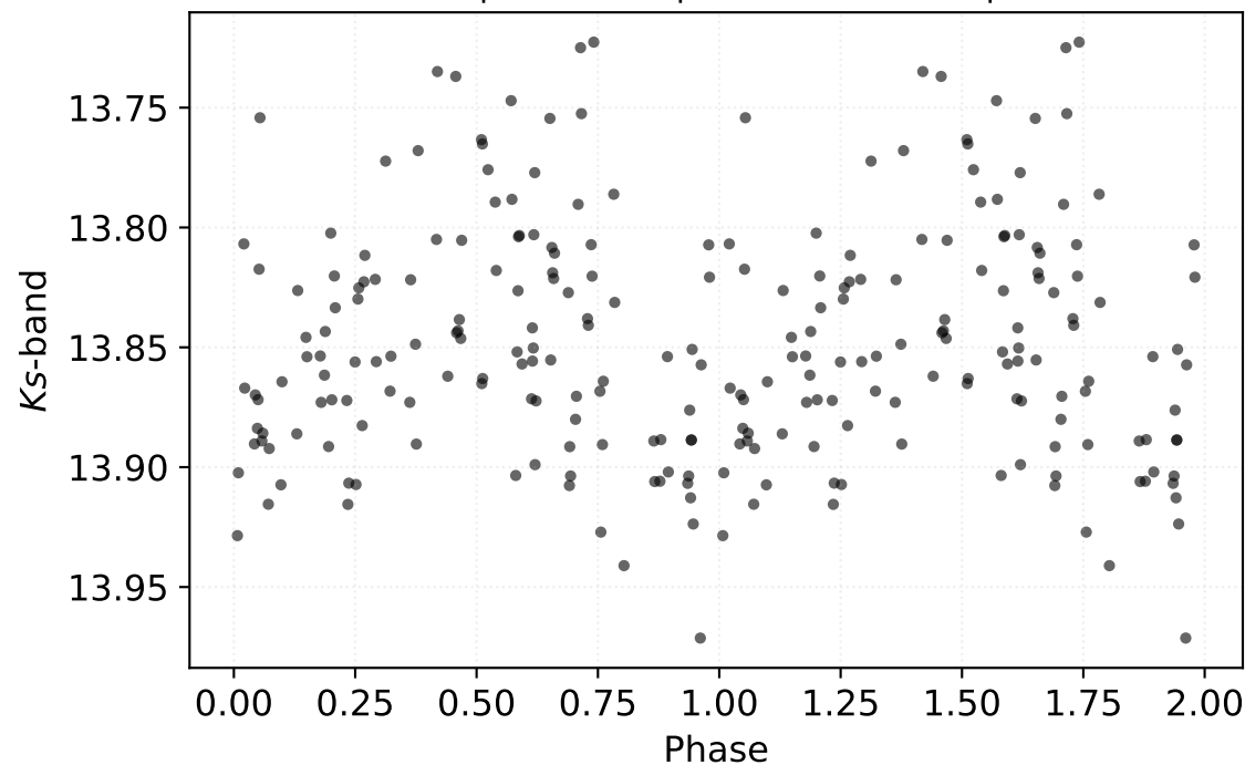
P: 35.01110 d | Class: RP | Subclass: UVAR | Field b279
