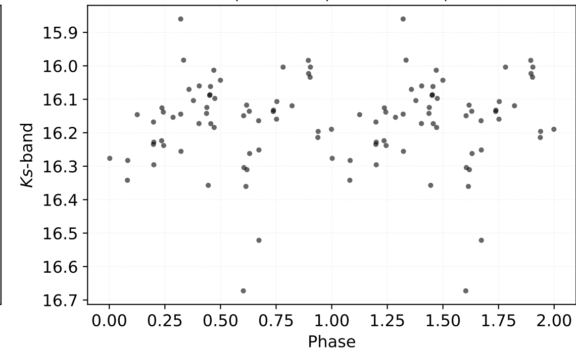
P: 0.61508 d | Class: EB | Subclass: EA | Field b278
