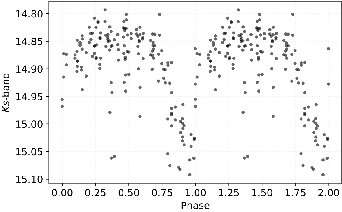
P: 14.70906 d | Class: RP | Subclass: CEP-F | Field b279
