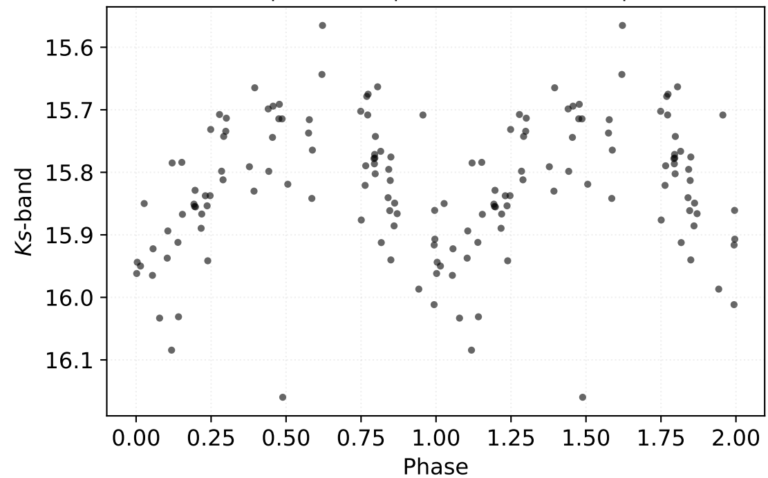
P: 3.45287 d | Class: RP | Subclass: CEP-1OT | Field b279
