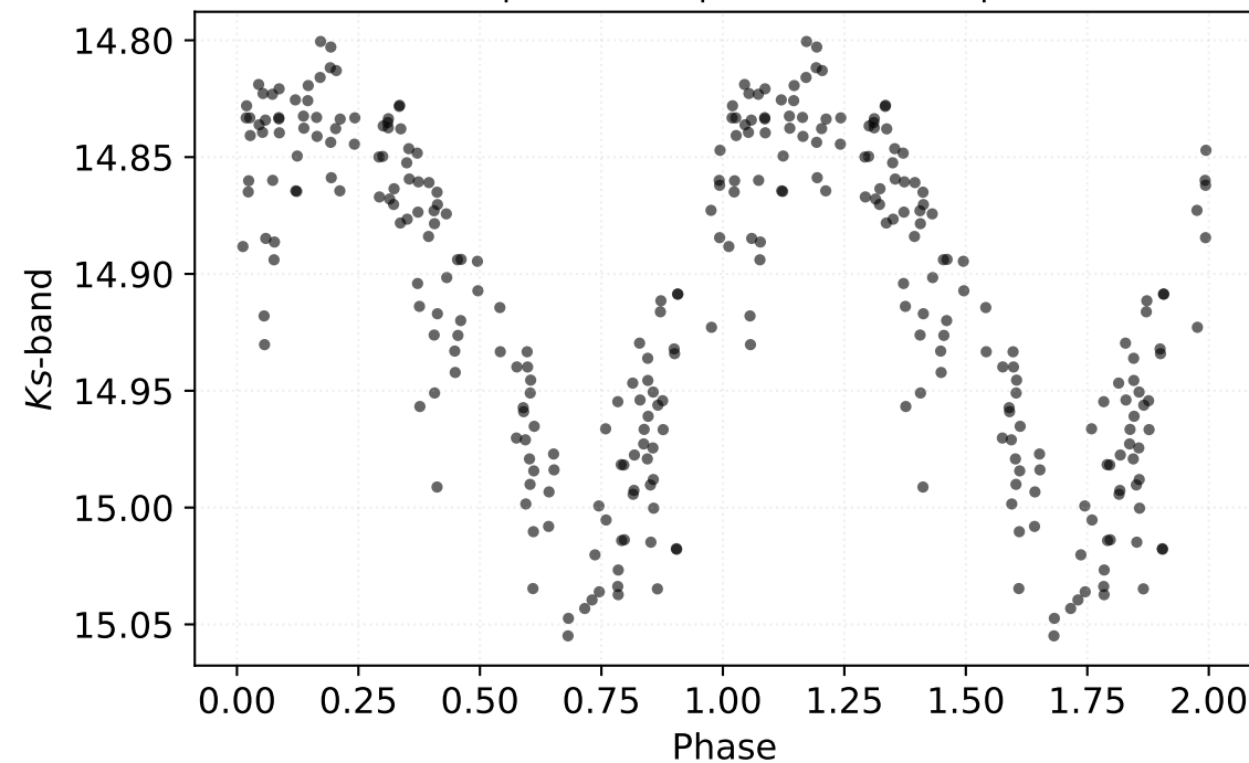
P: 0.96930 d | Class: EB | Subclass: RRc | Field b279
