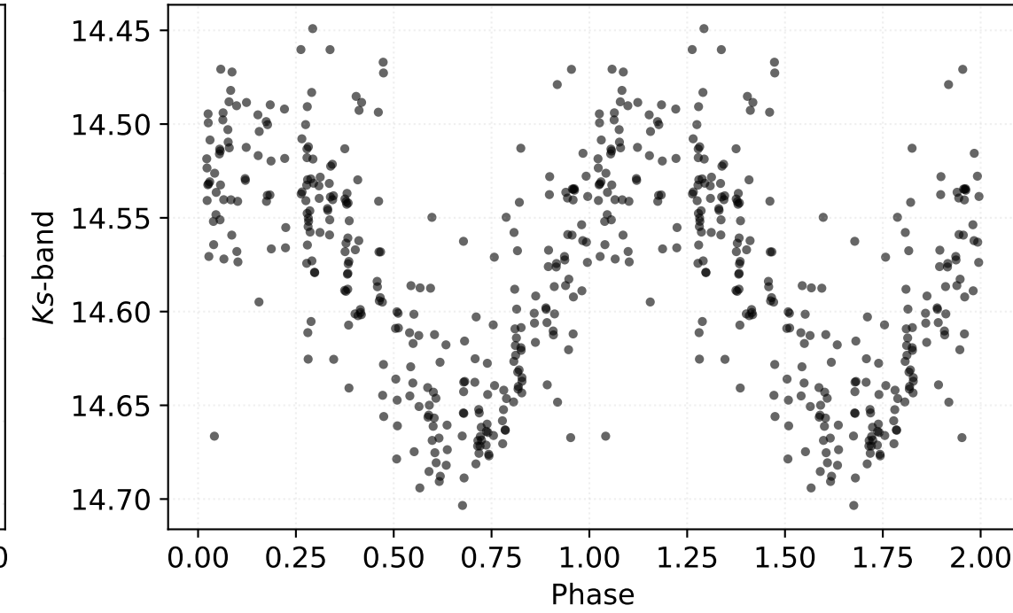
P: 0.25610 d | Class: RP | Subclass: RRc | Field b278
