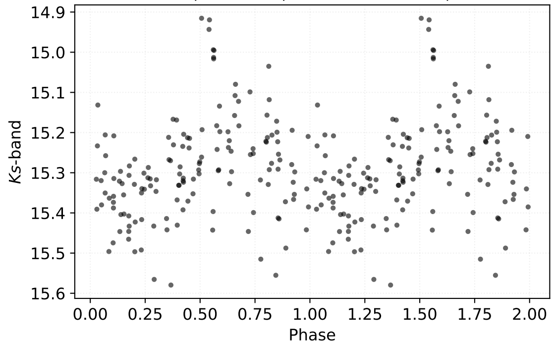
P: 0.25912 d | Class: RP | Subclass: CEP-1OT | Field b278
