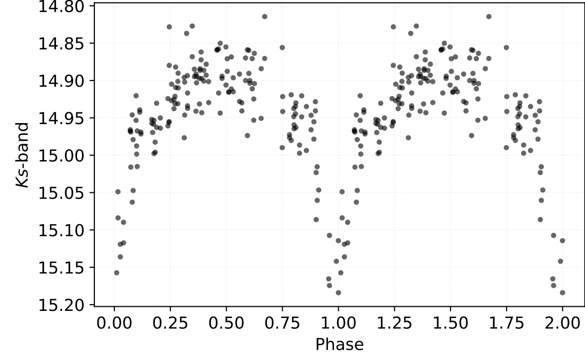
P: 2.26123 d | Class: RP | Subclass: CEP-F | Field b279
