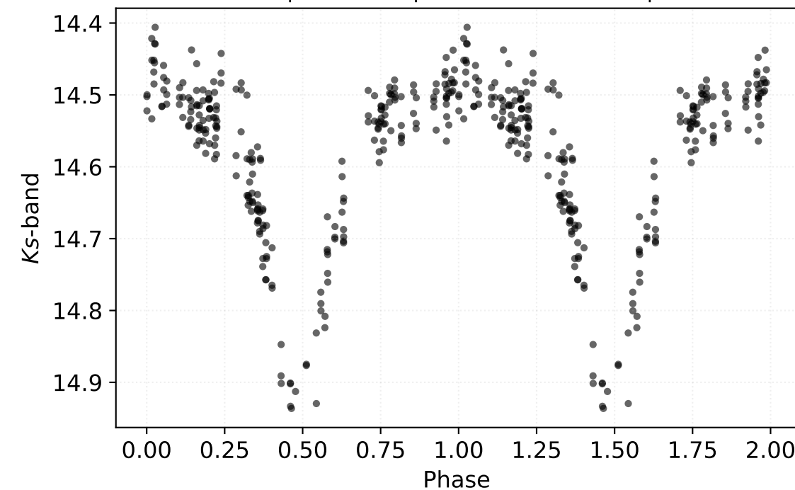
P: 1.66515 d | Class: RP | Subclass: CEP-1OT | Field b278
