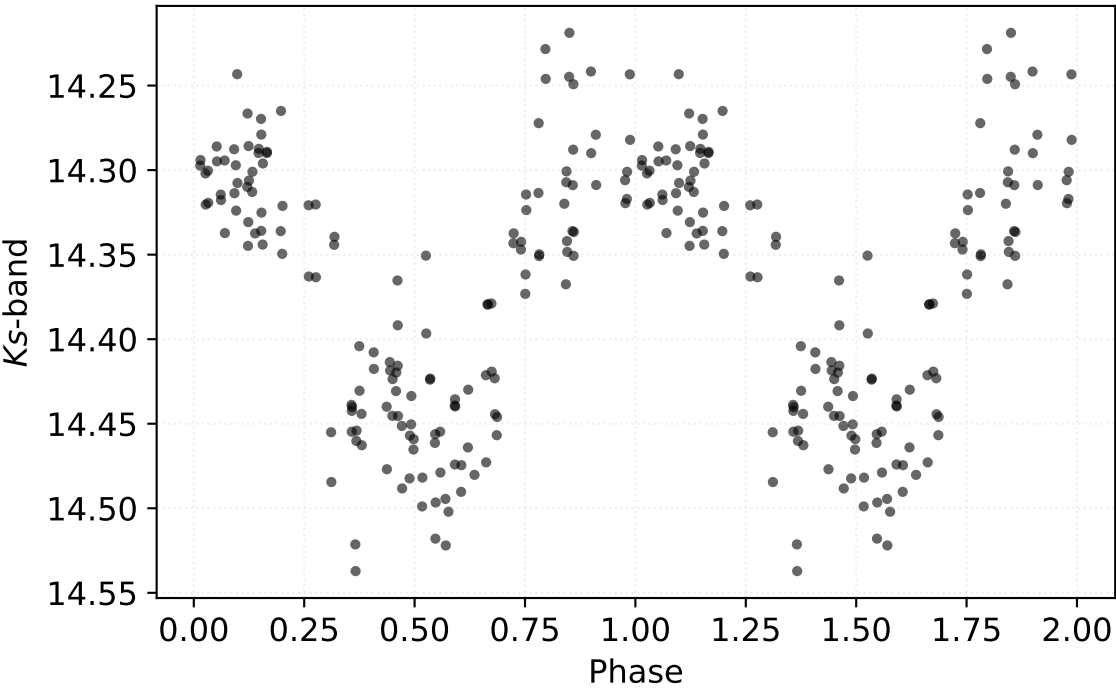
P: 2.96225 d | Class: RP | Subclass: CEP-1OT | Field b279
