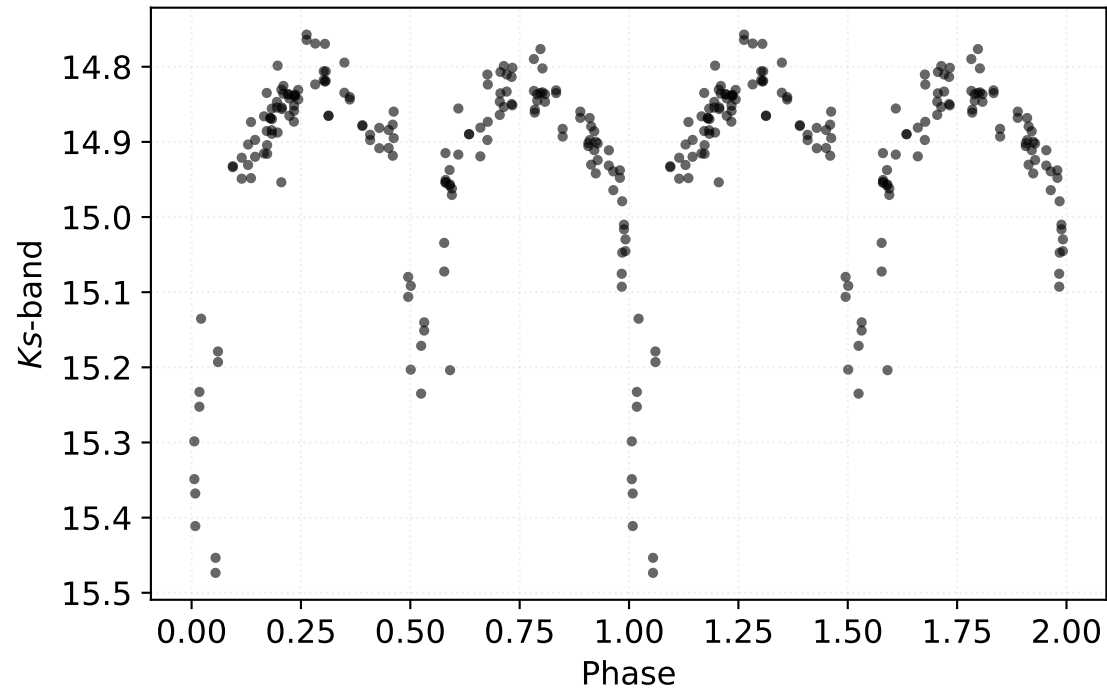
P: 3.83073 d | Class: EB | Subclass: EA | Field b278
