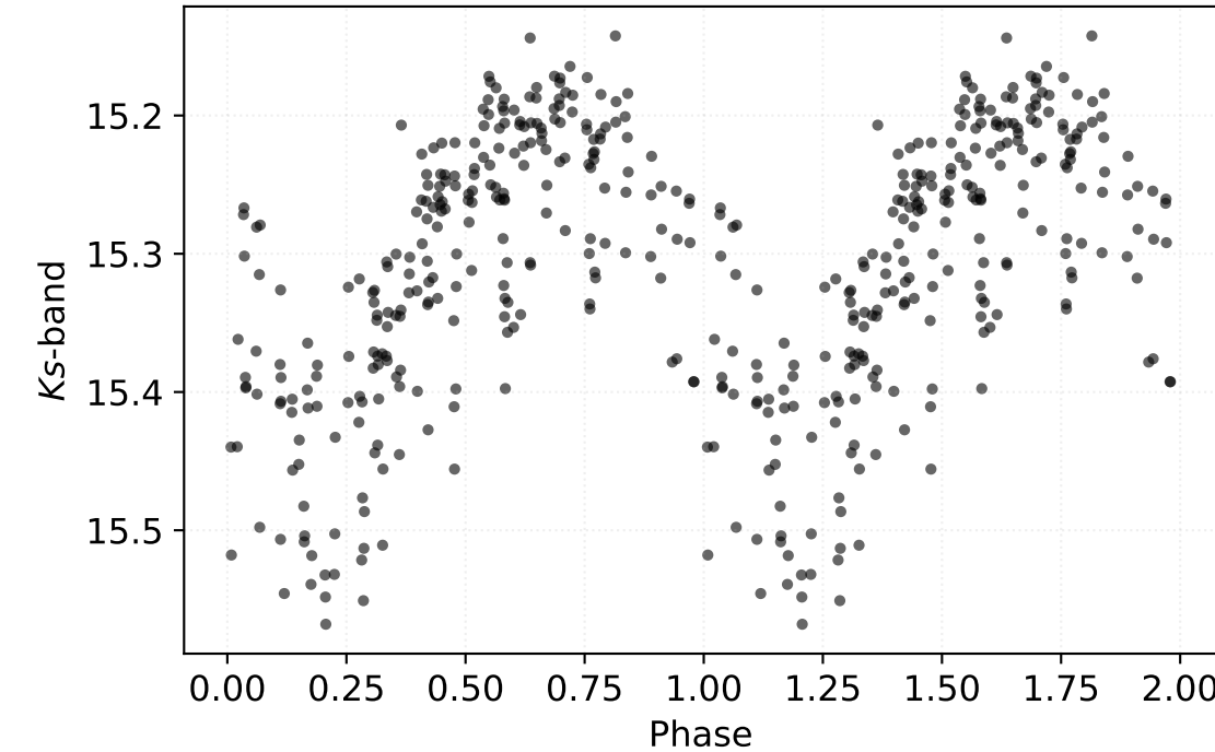
P: 0.99776 d | Class: RP | Subclass: CEP-1OT | Field b278
