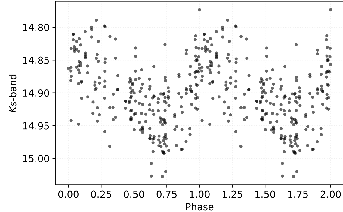
P: 0.48606 d | Class: RP | Subclass: RRc | Field b279
