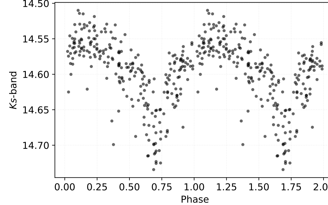
P: 0.39250 d | Class: RP | Subclass: CEP-1OT | Field b279
