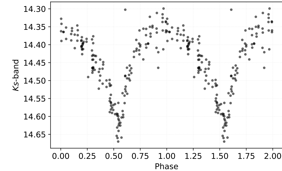
P: 0.60988 d | Class: RP | Subclass: RRab | Field b278
