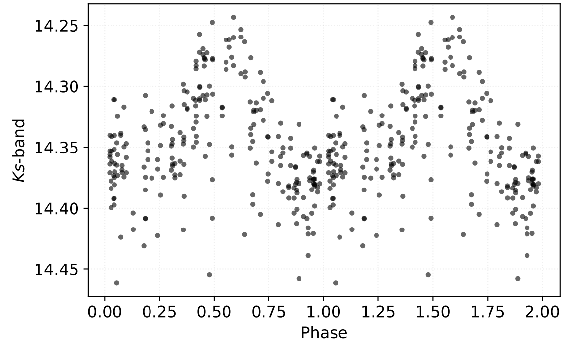
P: 0.50207 d | Class: RP | Subclass: CEP-1OT | Field b279
