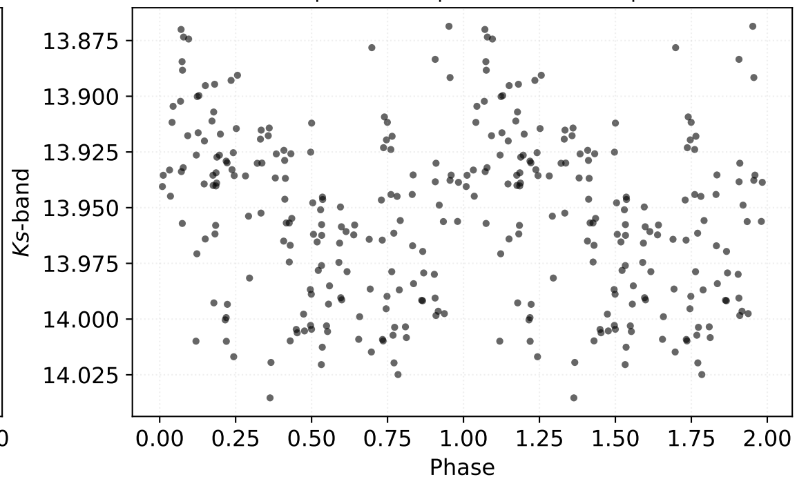
P: 0.16621 d | Class: RP | Subclass: UVAR | Field b278
