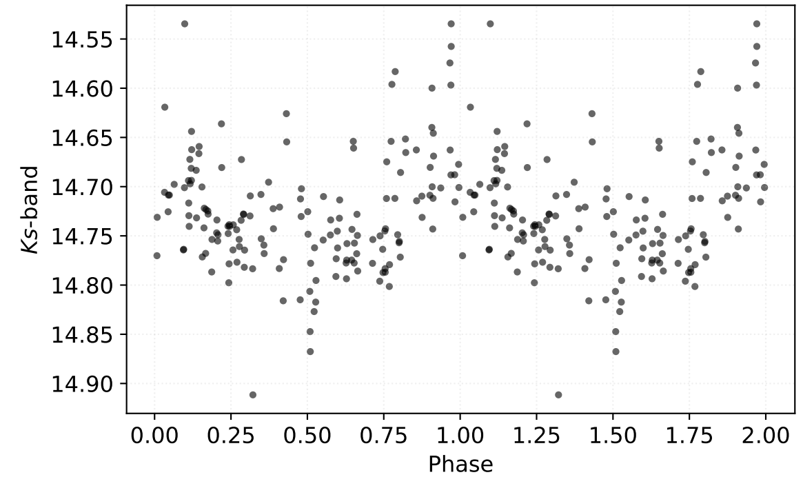
P: 0.42939 d | Class: RP | Subclass: RRab | Field b279
