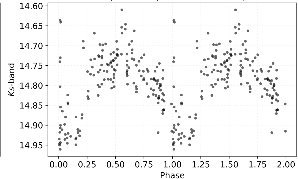
P: 0.26042 d | Class: RP | Subclass: CEP-1OT | Field b278
