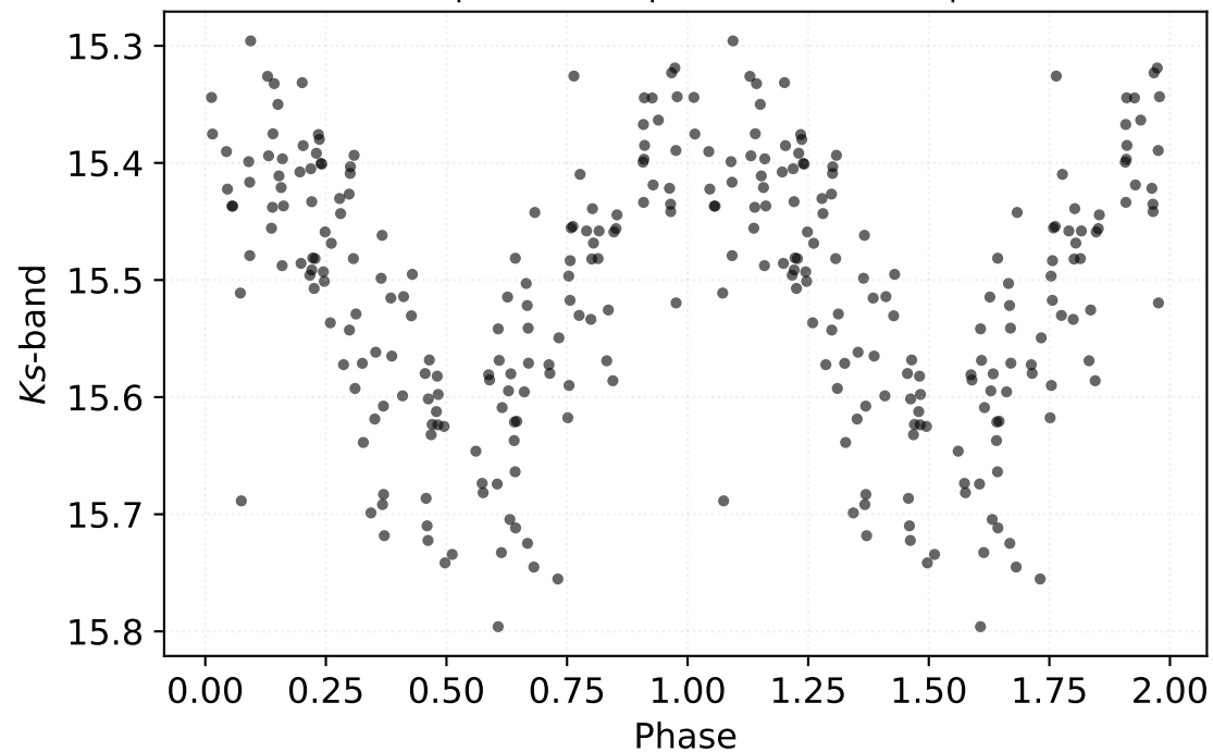
P: 0.51763 d | Class: RP | Subclass: RRab | Field b279
