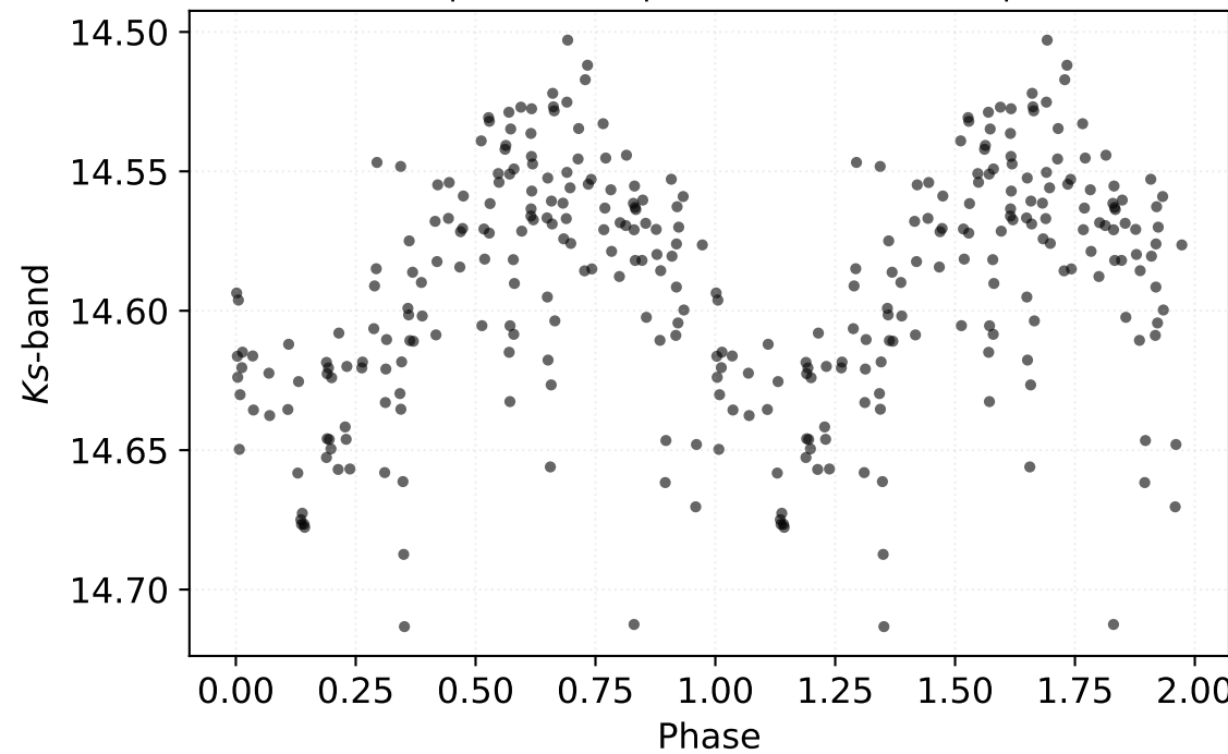
P: 2.44119 d | Class: RP | Subclass: CEP-1OT | Field b278
