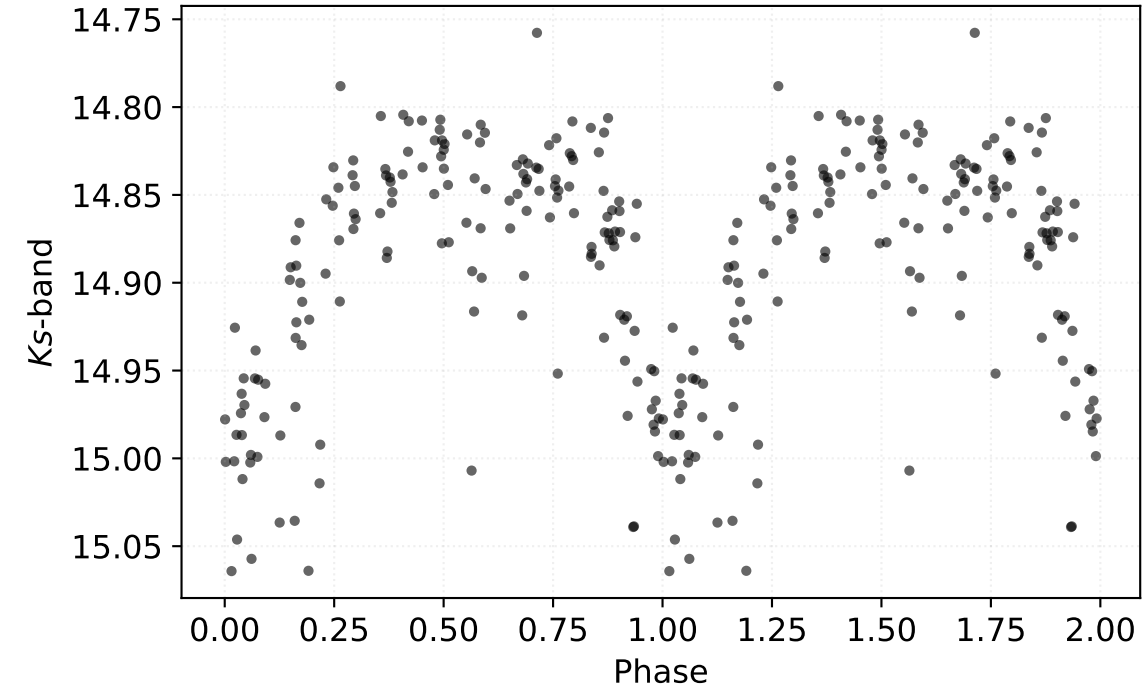
P: 0.70632 d | Class: RP | Subclass: RRab | Field b279
