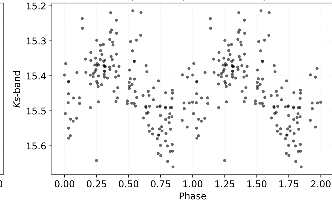
P: 0.35264 d | Class: RP | Subclass: RRab | Field b279
