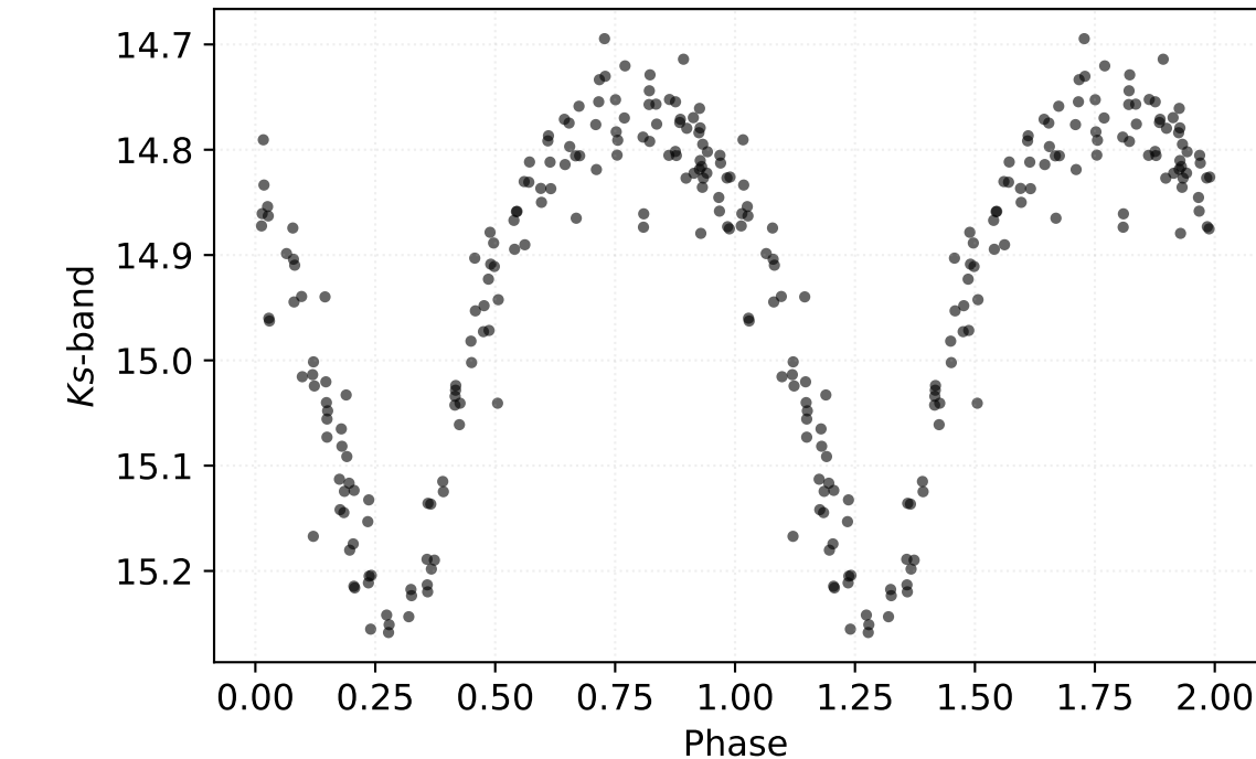
P: 0.66003 d | Class: RP | Subclass: CEP-1OT | Field b278
