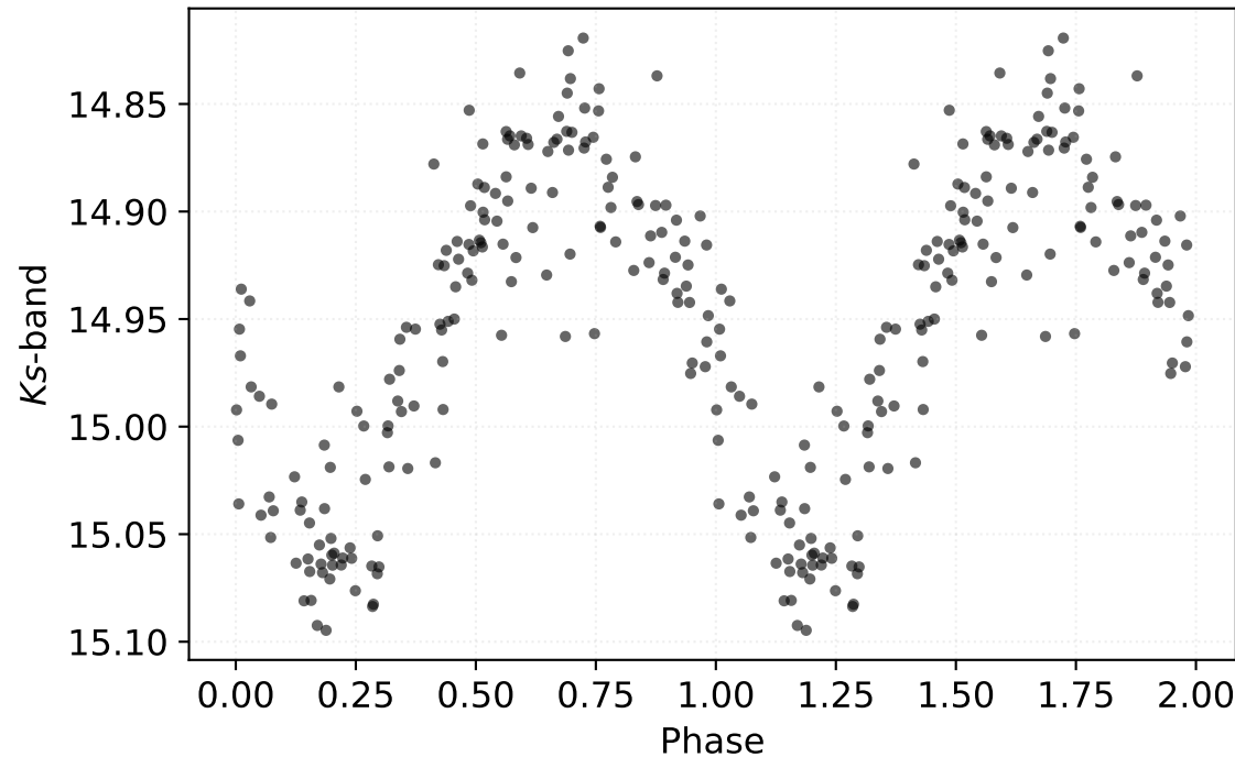
P: 0.44745 d | Class: RP | Subclass: CEP-1OT | Field b278
