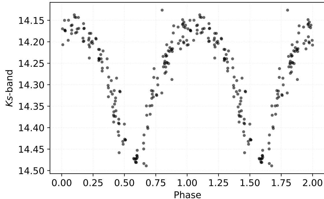
P: 0.25428 d | Class: RP | Subclass: UVAR | Field b279
