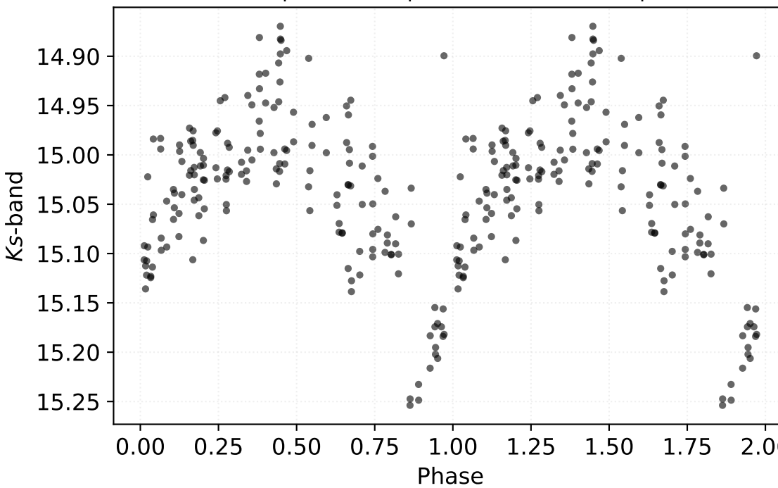
P: 1.30087 d | Class: RP | Subclass: CEP-1OT | Field b278
