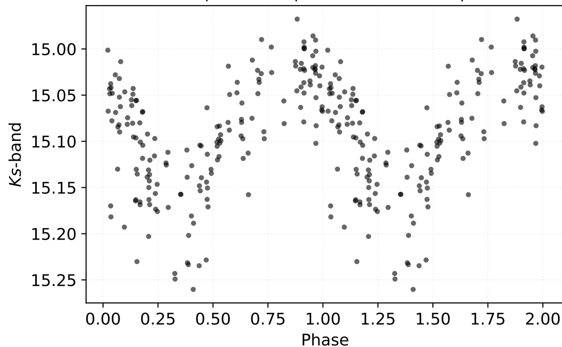
P: 3.73982 d | Class: RP | Subclass: CEP-1OT | Field b278
