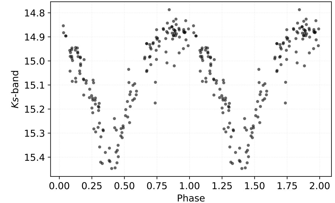
P: 0.16299 d | Class: RP | Subclass: UVAR | Field b279
