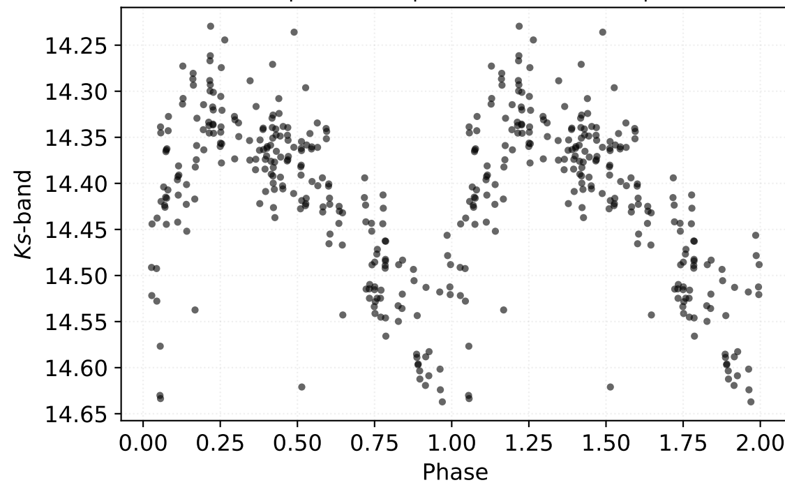
P: 0.46519 d | Class: RP | Subclass: CEP-1OT | Field b279
