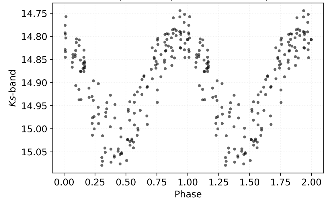
P: 0.32878 d | Class: RP | Subclass: CEP-1OT | Field b279
