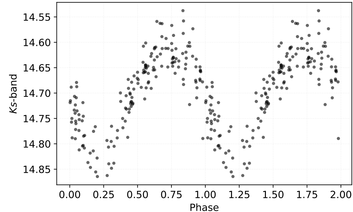
P: 0.24931 d | Class: RP | Subclass: UVAR | Field b278
