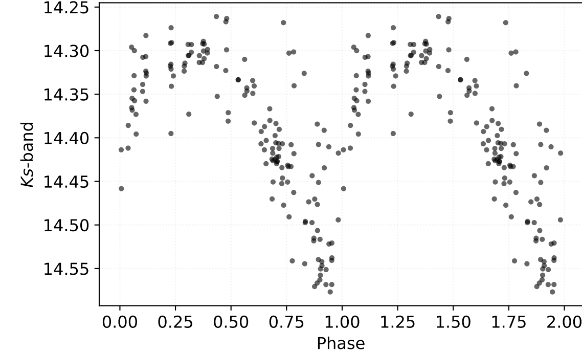
P: 1.02737 d | Class: RP | Subclass: CEP-1OT | Field b278
