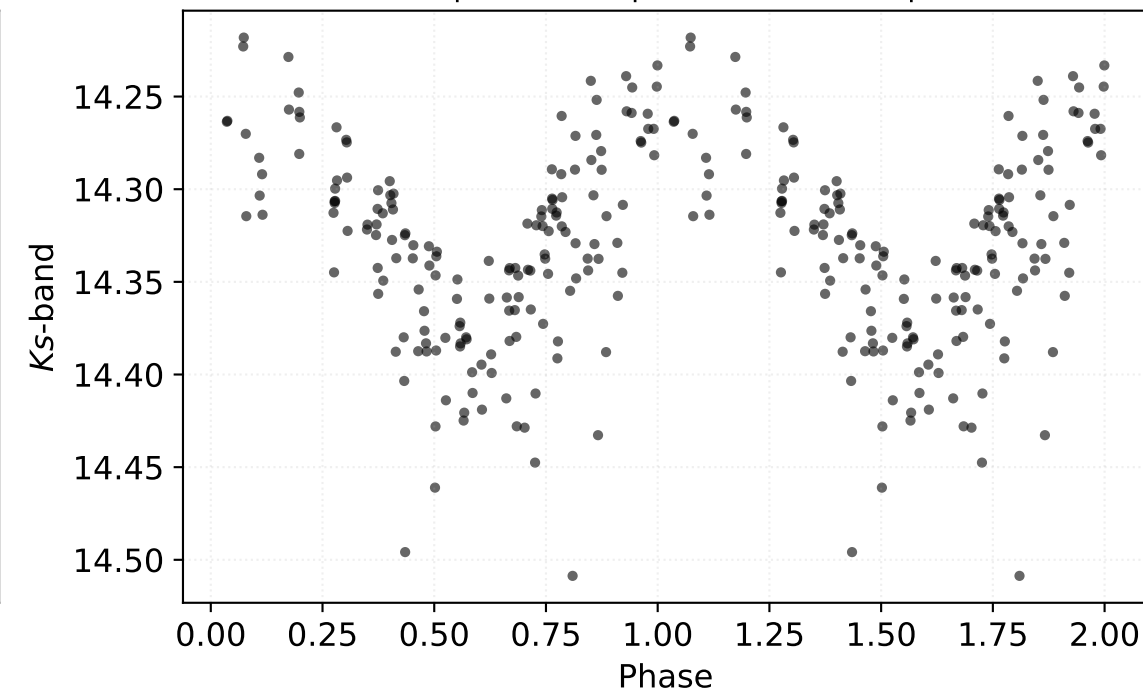
P: 0.45874 d | Class: RP | Subclass: RRab | Field b279
