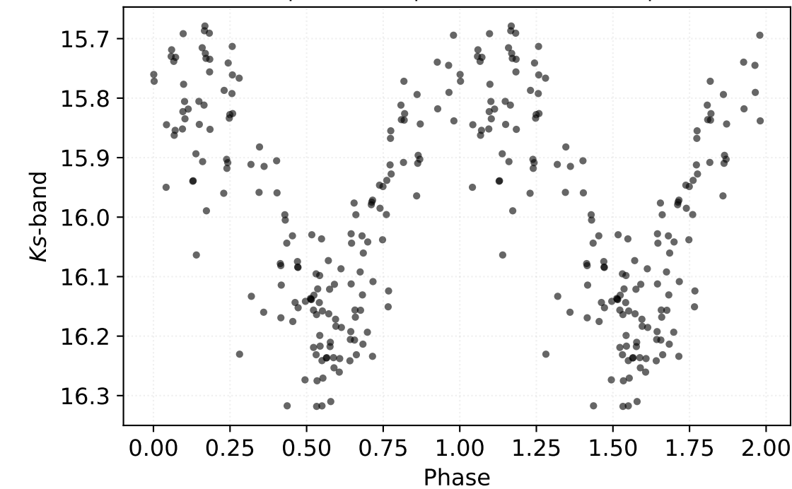
P: 0.24068 d | Class: RP | Subclass: CEP-1OT | Field b278
