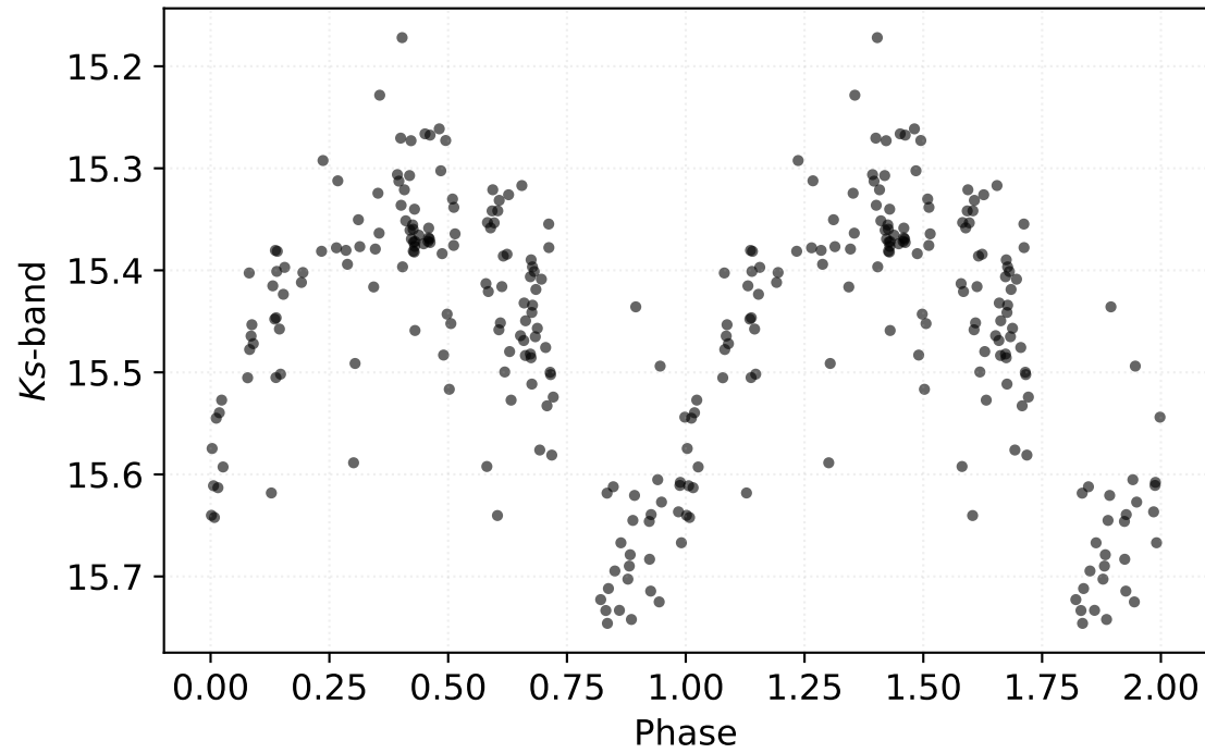
P: 0.15973 d | Class: RP | Subclass: UVAR | Field b279
