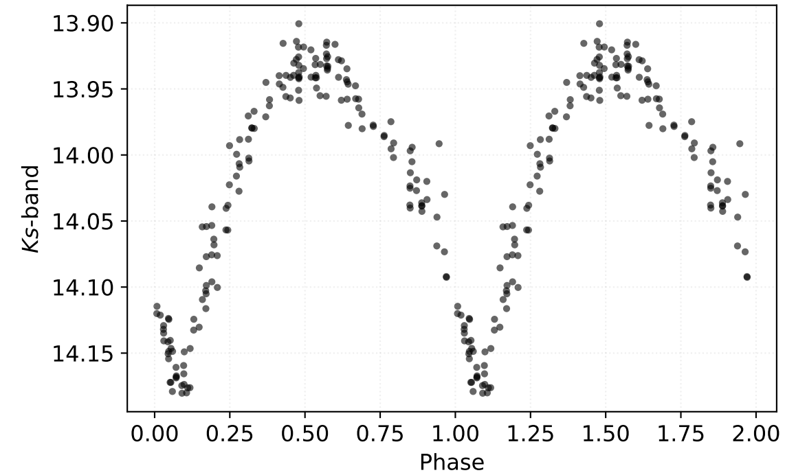
P: 0.39403 d | Class: RP | Subclass: RRab | Field b278
