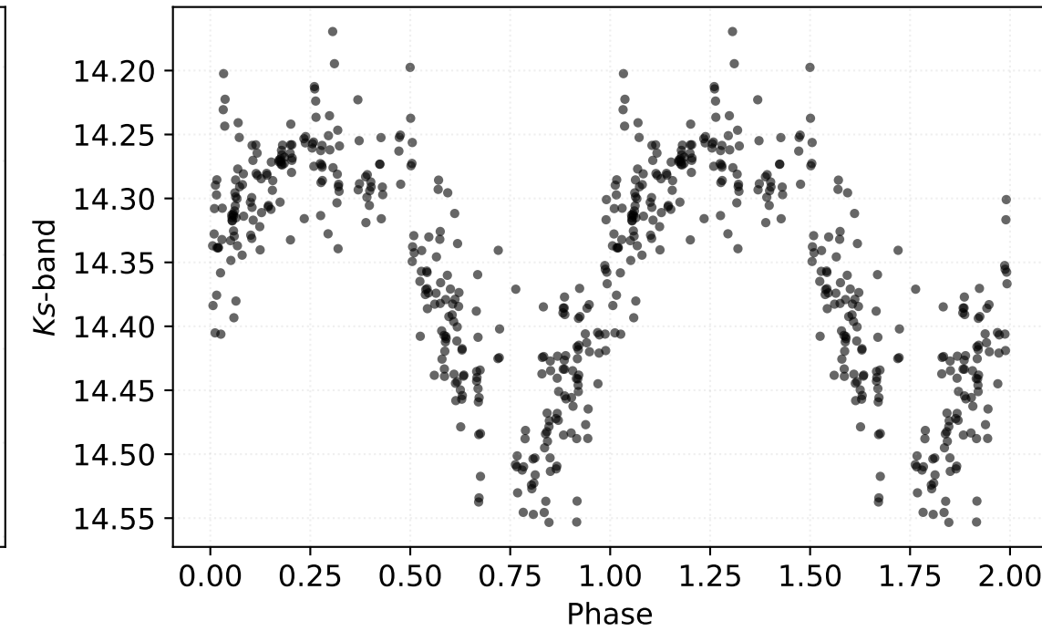
P: 0.27802 d | Class: RP | Subclass: RRc | Field b278
