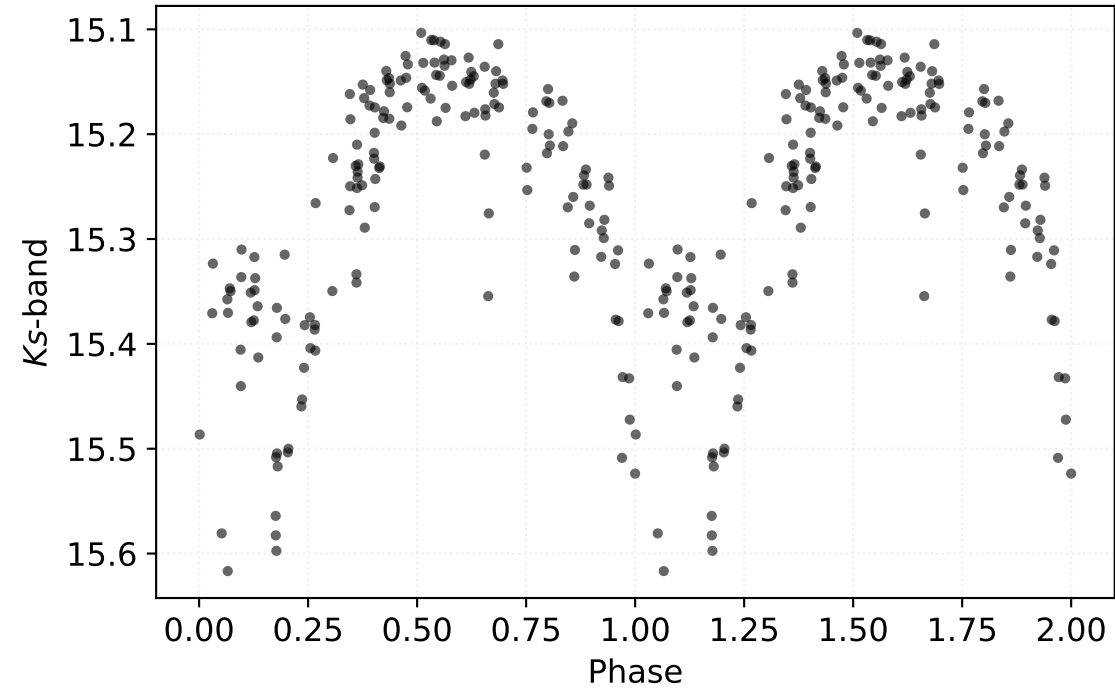
P: 0.27215 d | Class: RP | Subclass: CEP-1OT | Field b279
