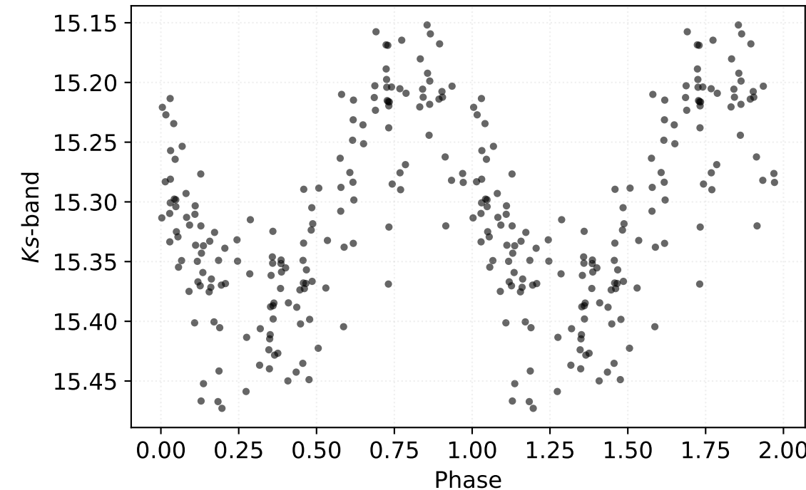
P: 0.66057 d | Class: RP | Subclass: CEP-1OT | Field b278
