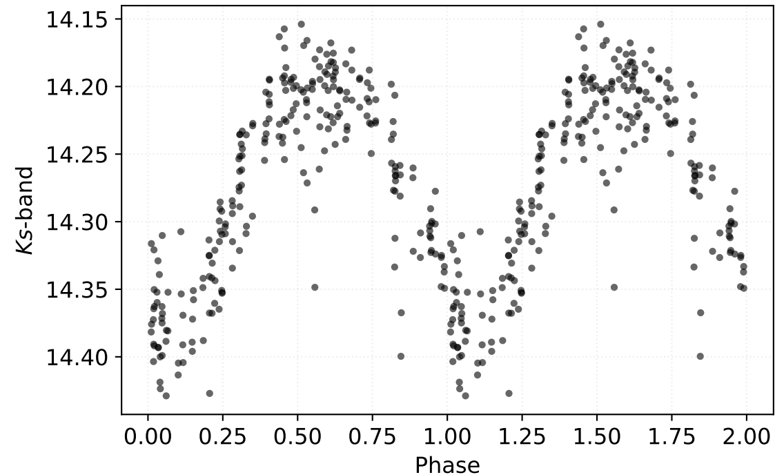
P: 0.42784 d | Class: RP | Subclass: RRab | Field b278
