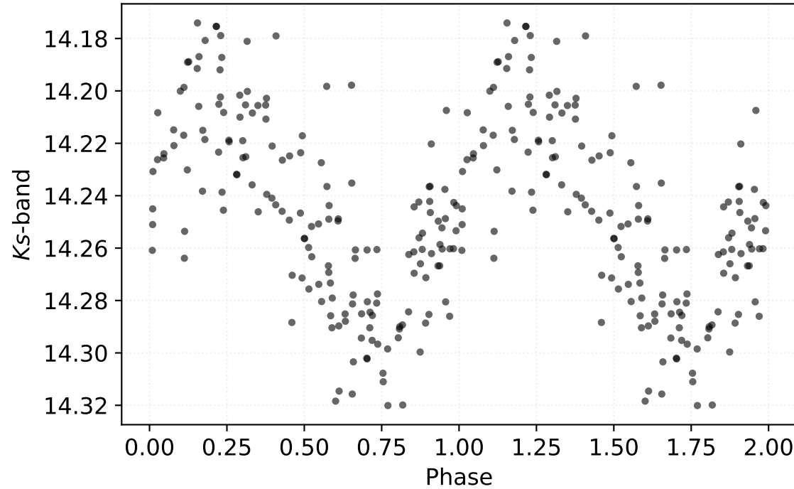
P: 0.36497 d | Class: RP | Subclass: CEP-1OT | Field b278
