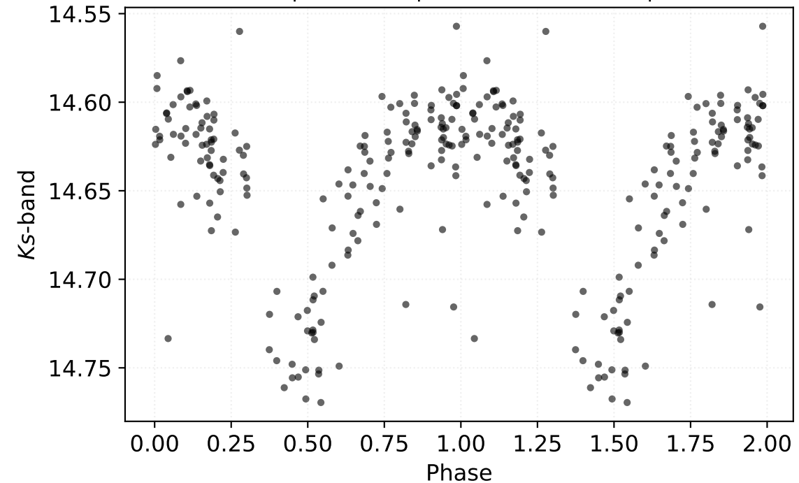
P: 0.97588 d | Class: RP | Subclass: CEP-1OT | Field b279
