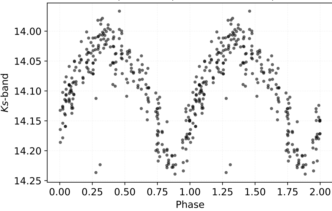
P: 0.47956 d | Class: RP | Subclass: CEP-1OT | Field b278
