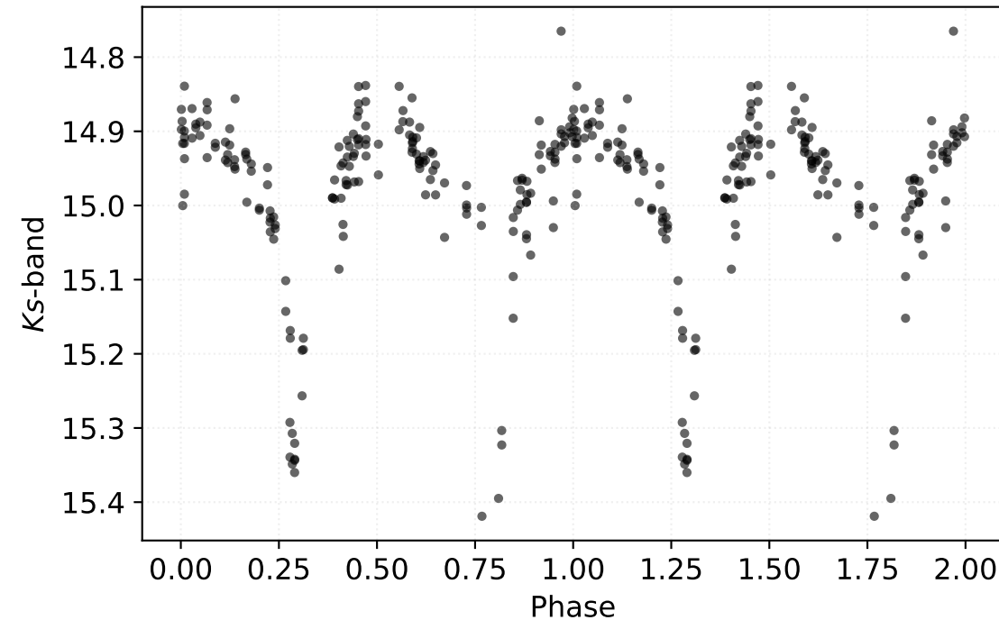
P: 8.21887 d | Class: EB | Subclass: EA | Field b278
