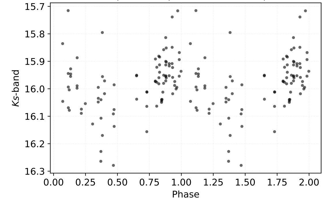
P: 1.35296 d | Class: RP | Subclass: CEP-1OT | Field b279
