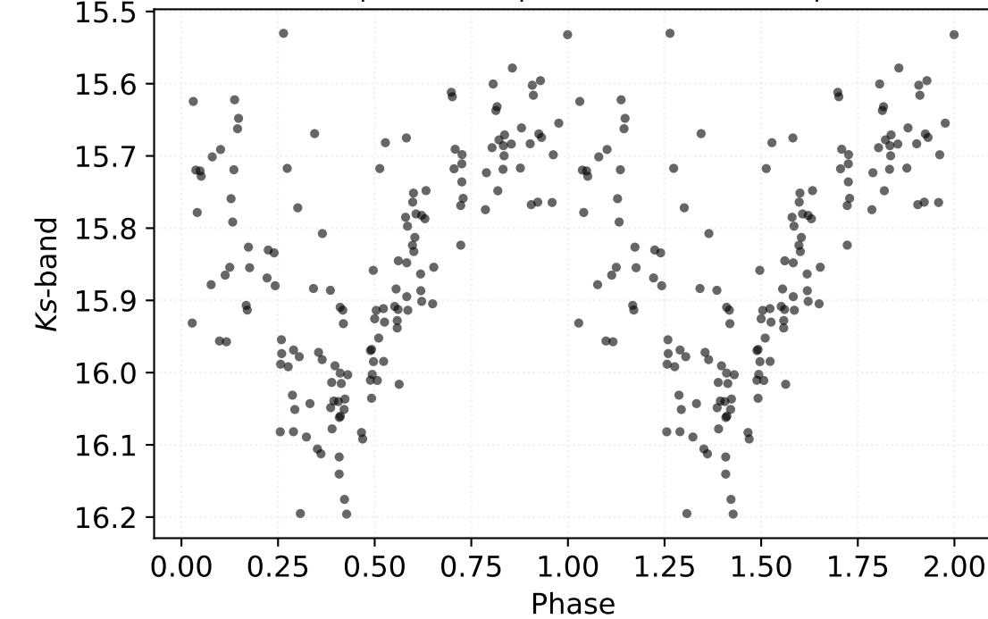
P: 0.77052 d | Class: RP | Subclass: CEP-1OT | Field b278
