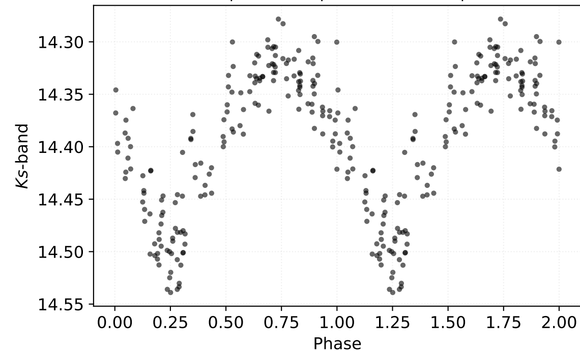
P: 0.35979 d | Class: RP | Subclass: RRab | Field b278
