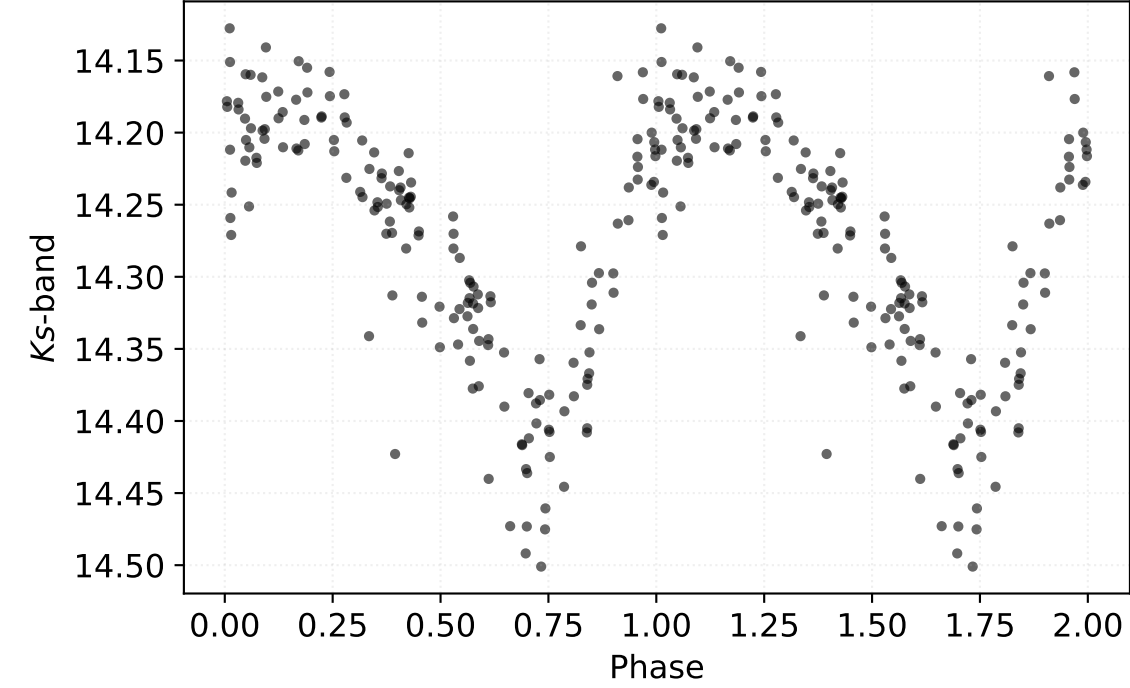
P: 0.60023 d | Class: RP | Subclass: RRab | Field b278
