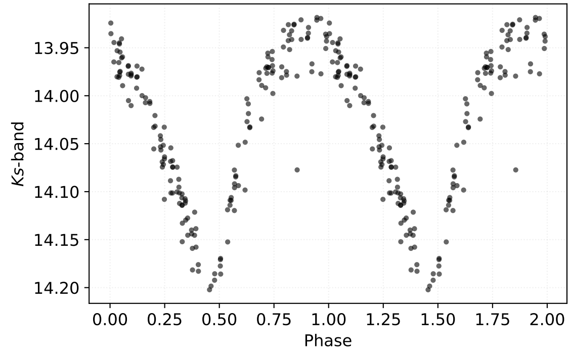
P: 0.48048 d | Class: RP | Subclass: RRab | Field b278
