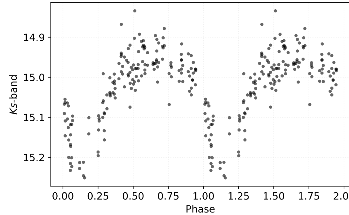
P: 0.38579 d | Class: RP | Subclass: RRab | Field b279
