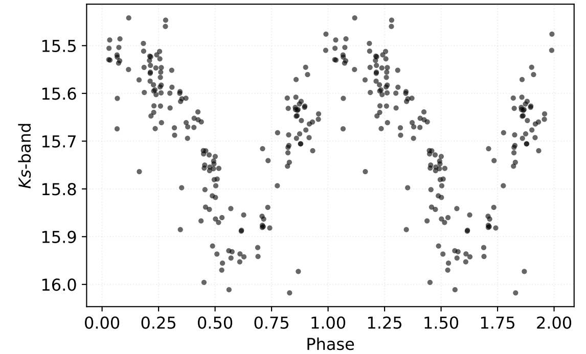
P: 0.38514 d | Class: RP | Subclass: RRab | Field b279
