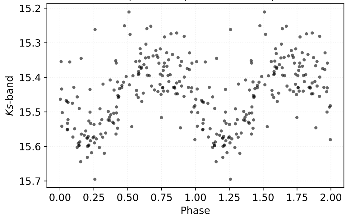
P: 0.29594 d | Class: RP | Subclass: UVAR | Field b278
