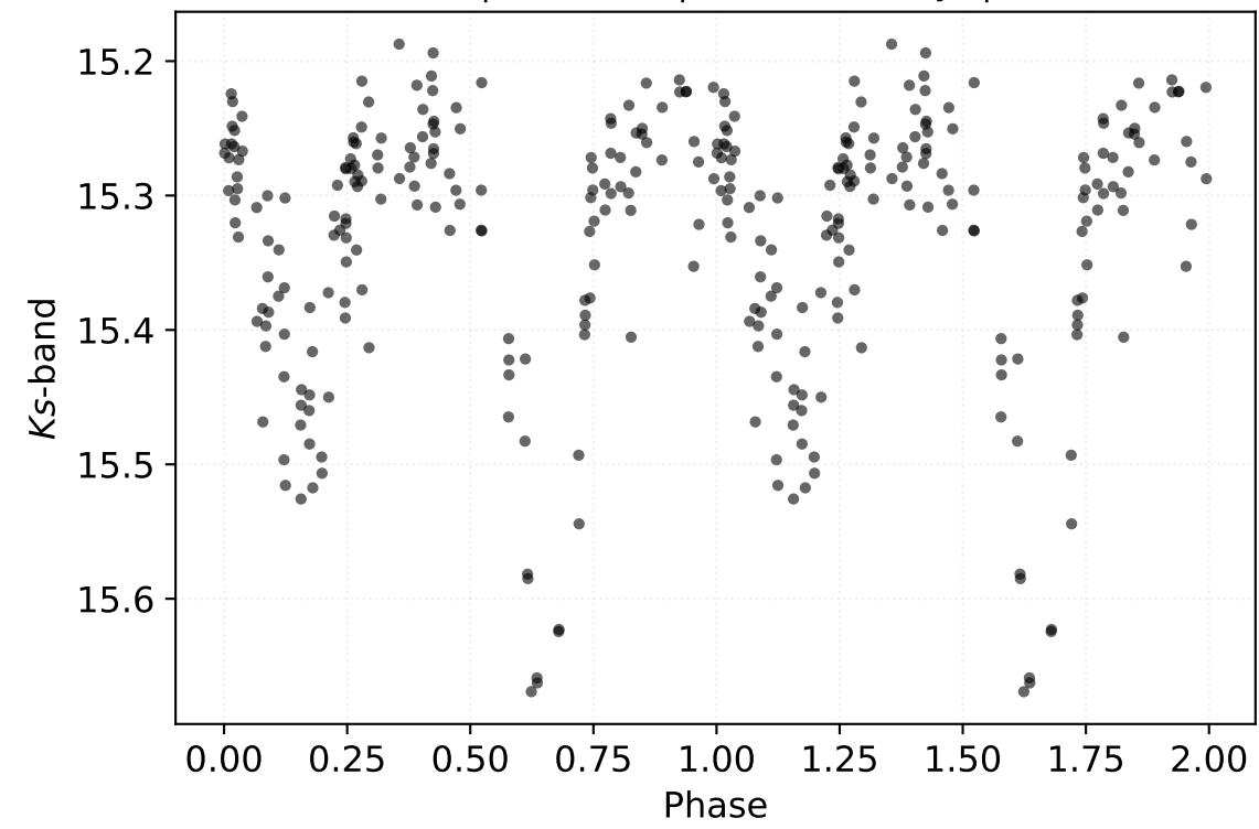
P: 1.10892 d | Class: EB | Subclass: EBlyr | Field b278
