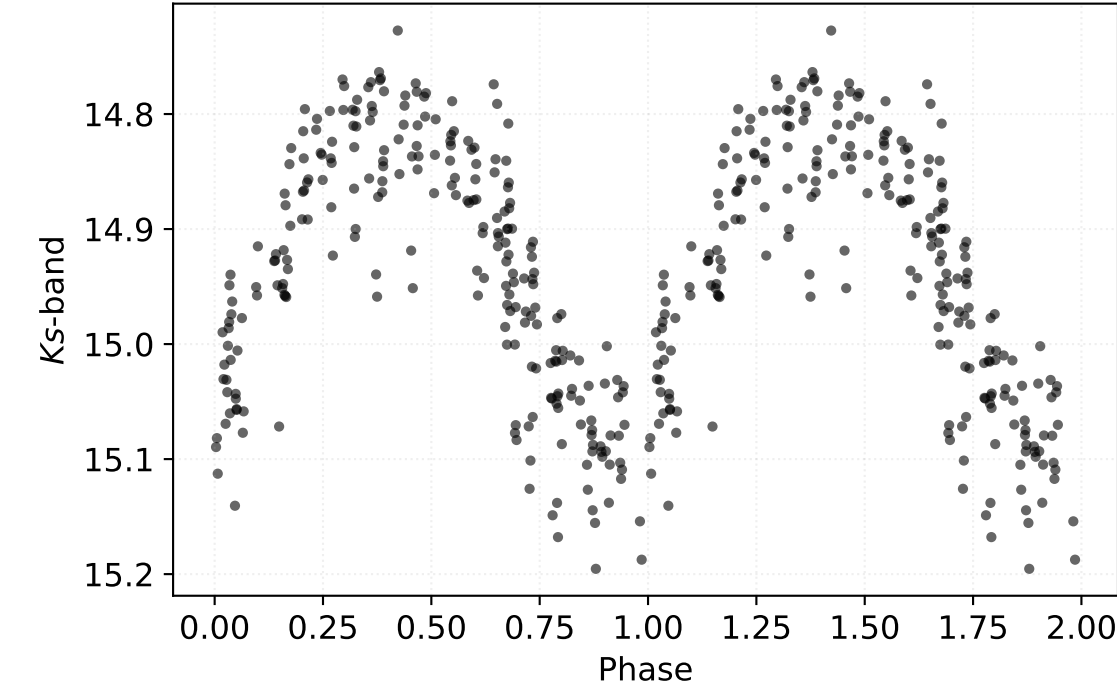
P: 0.20378 d | Class: RP | Subclass: UVAR | Field b278
