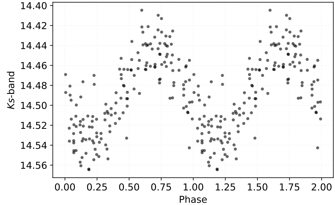
P: 0.35434 d | Class: RP | Subclass: CEP-1OT | Field b279
