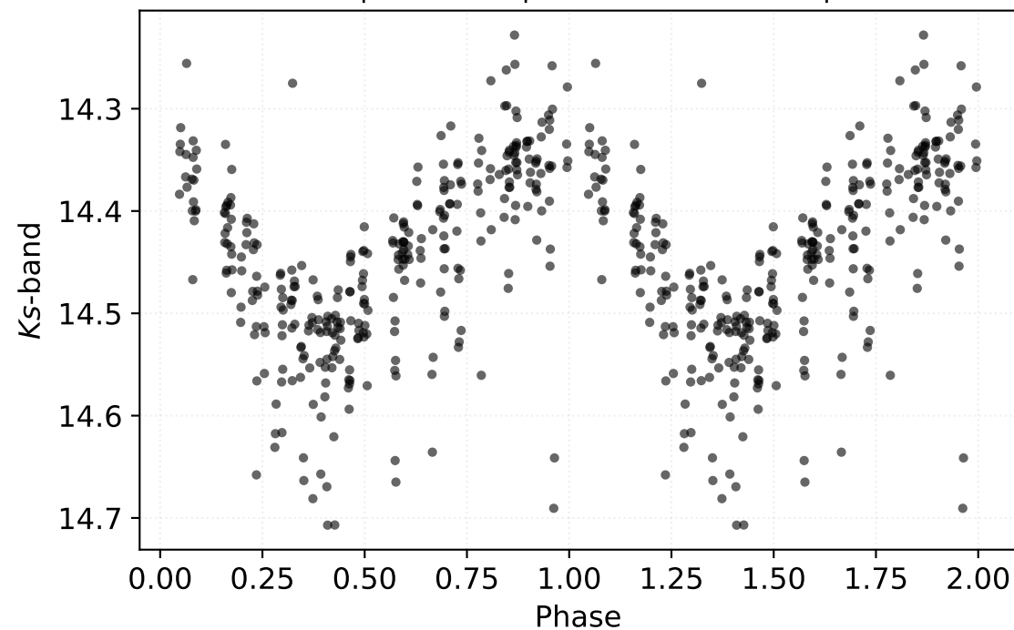
P: 0.42863 d | Class: RP | Subclass: CEP-1OT | Field b278
