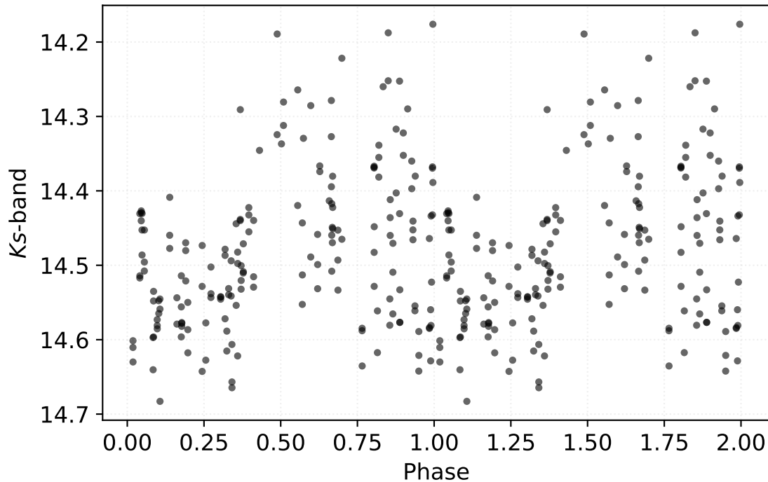
P: 1.18350 d | Class: RP | Subclass: CEP-1OT | Field b279
