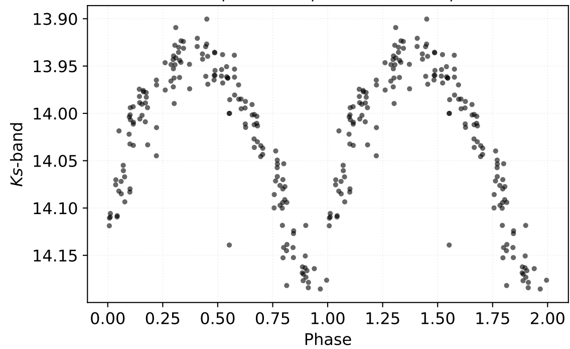
P: 0.31554 d | Class: RP | Subclass: RRab | Field b279
