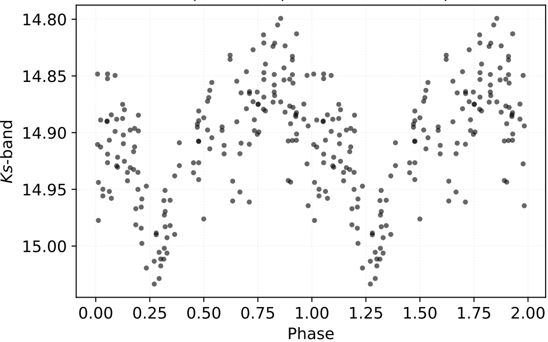
P: 2.44669 d | Class: RP | Subclass: CEP-1OT | Field b279
