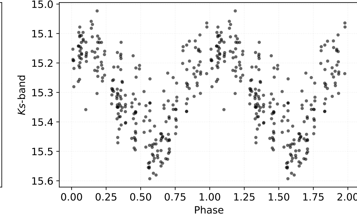
P: 0.46854 d | Class: RP | Subclass: RRc | Field b279
