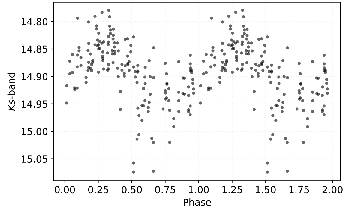
P: 5.21875 d | Class: RP | Subclass: CEP-1OT | Field b279
