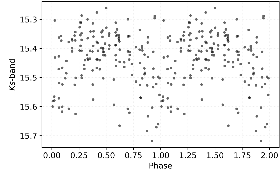
P: 0.32169 d | Class: RP | Subclass: RRab | Field b279
