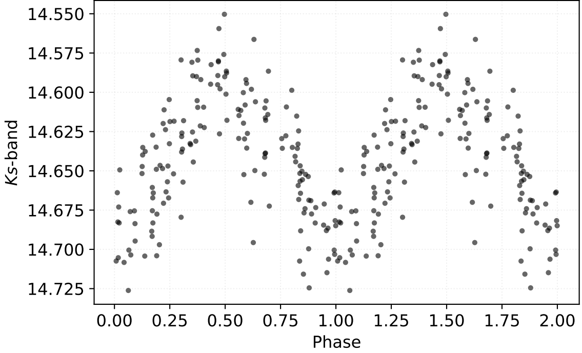
P: 0.32037 d | Class: RP | Subclass: RRab | Field b278
