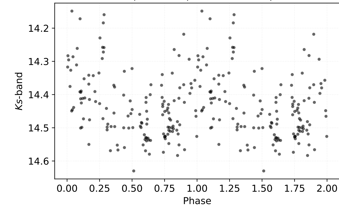
P: 13.36067 d | Class: RP | Subclass: UVAR | Field b279
