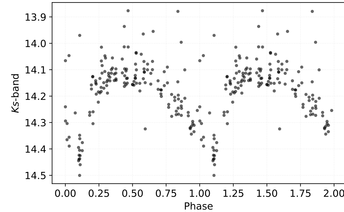
P: 0.47073 d | Class: RP | Subclass: CEP-1OT | Field b279
