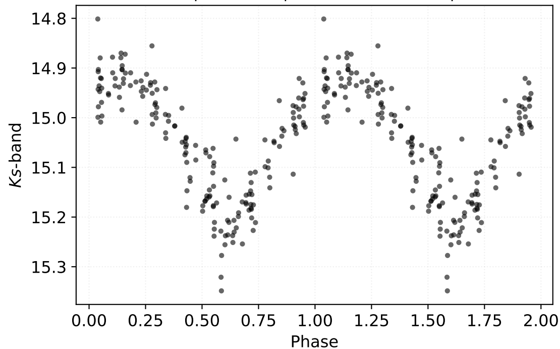
P: 4.97526 d | Class: RP | Subclass: CEP-1OT | Field b278
