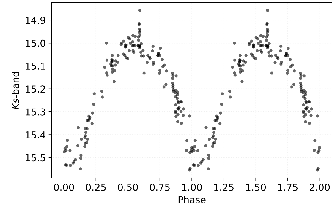
P: 0.11386 d | Class: RP | Subclass: UVAR | Field b278
