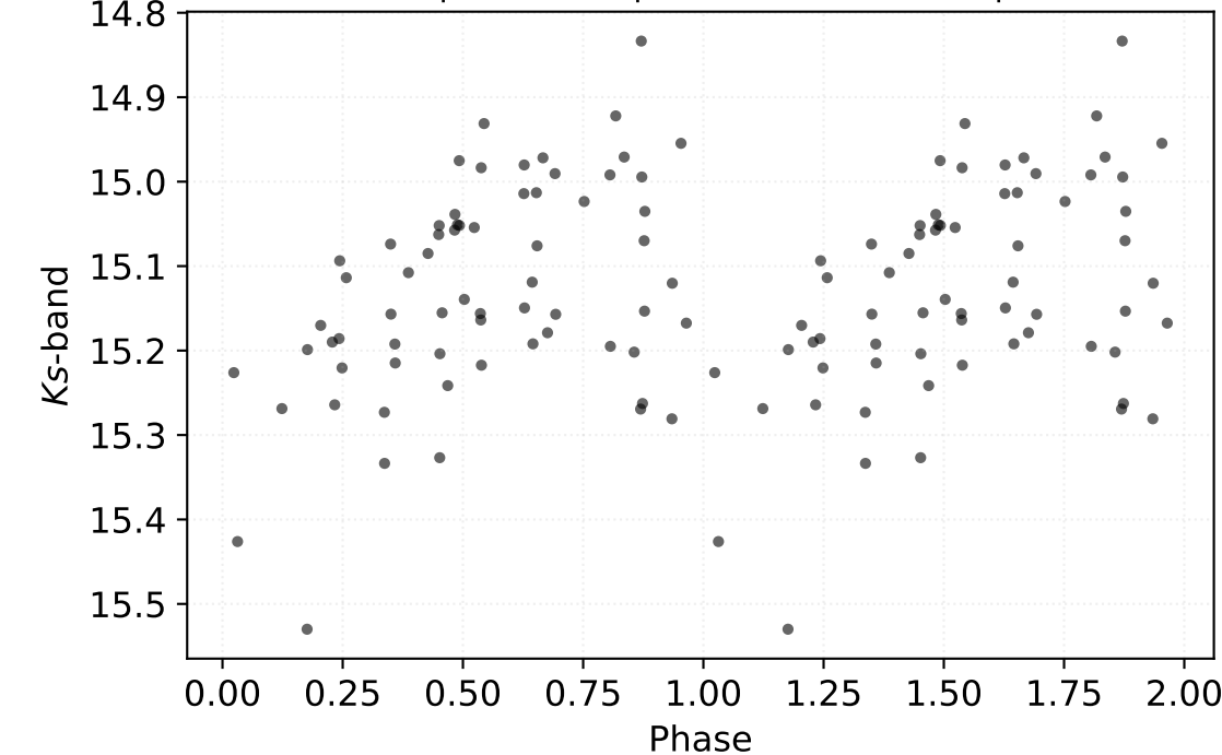
P: 4.01017 d | Class: RP | Subclass: CEP-1OT | Field b279
