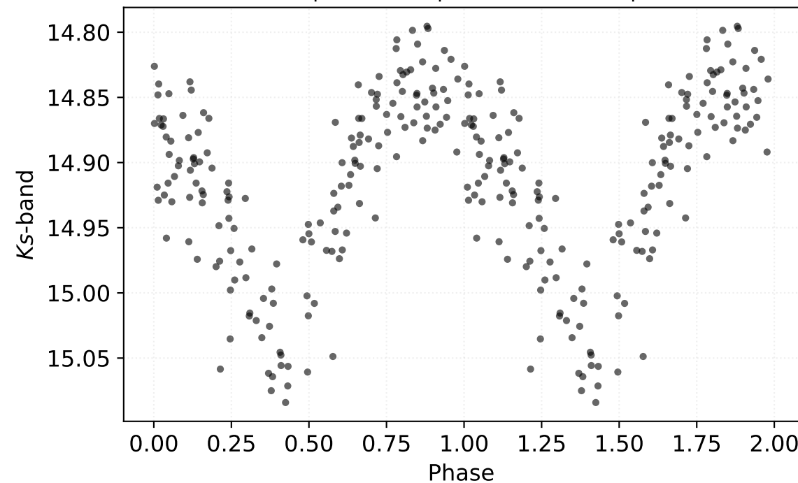
P: 0.48951 d | Class: RP | Subclass: RRab | Field b279
