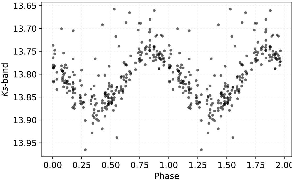
P: 1.82536 d | Class: RP | Subclass: CEP-F | Field b279
