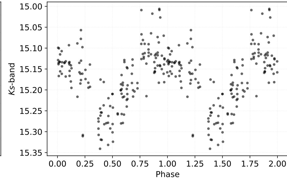
P: 0.25710 d | Class: RP | Subclass: RRc | Field b279
