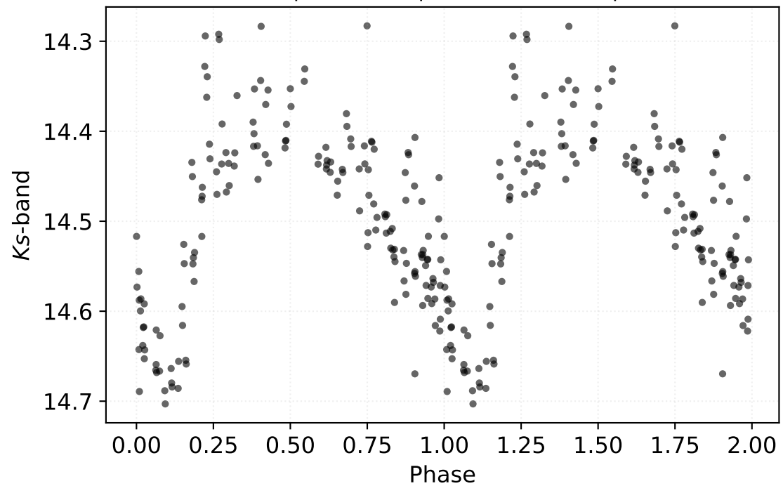
P: 0.46628 d | Class: RP | Subclass: RRab | Field b279
