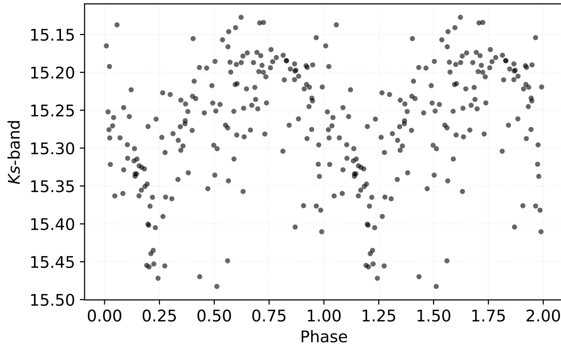
P: 3.87001 d | Class: RP | Subclass: CEP-1OT | Field b278
