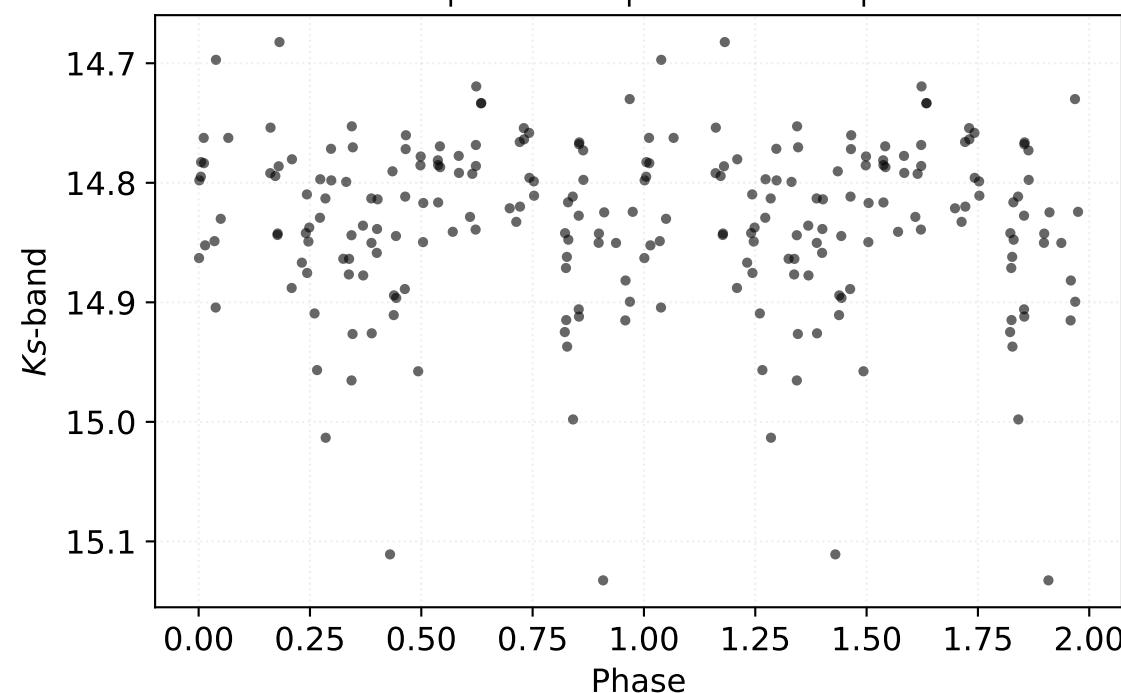
P: 0.25379 d | Class: EB | Subclass: EA | Field b278
