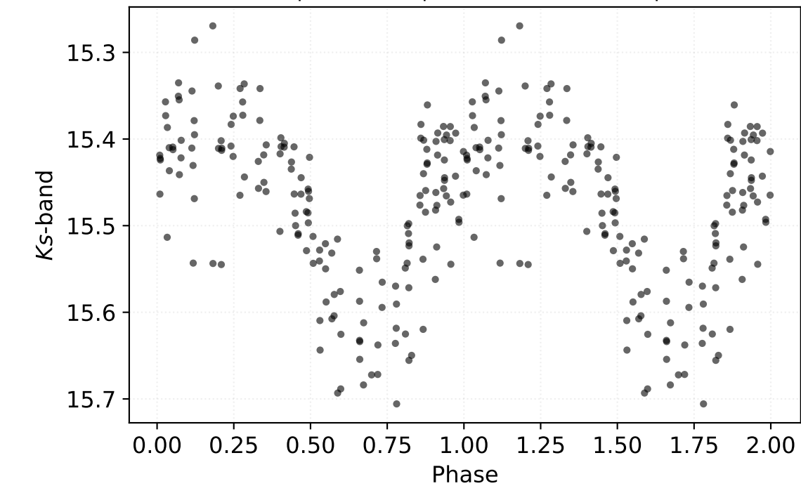
P: 2.47132 d | Class: RP | Subclass: CEP-1OT | Field b279
