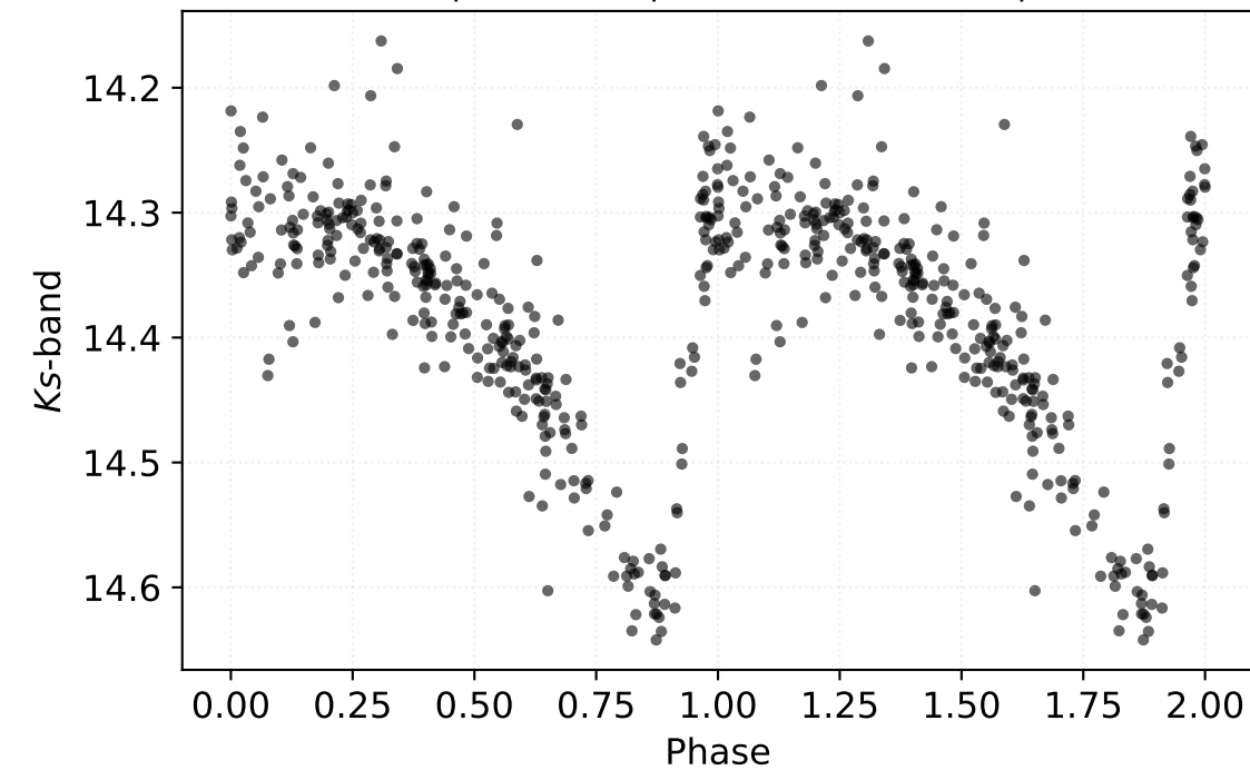
P: 0.52856 d | Class: RP | Subclass: CEP-1OT | Field b278
