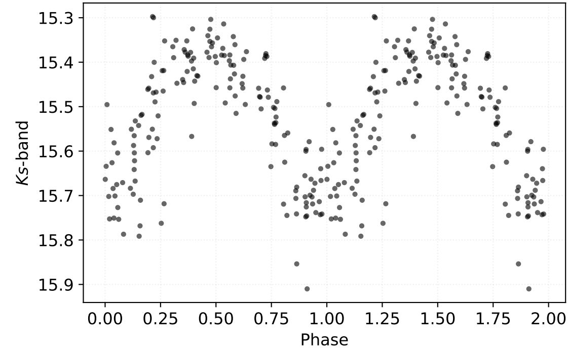
P: 0.13620 d | Class: RP | Subclass: UVAR | Field b279
