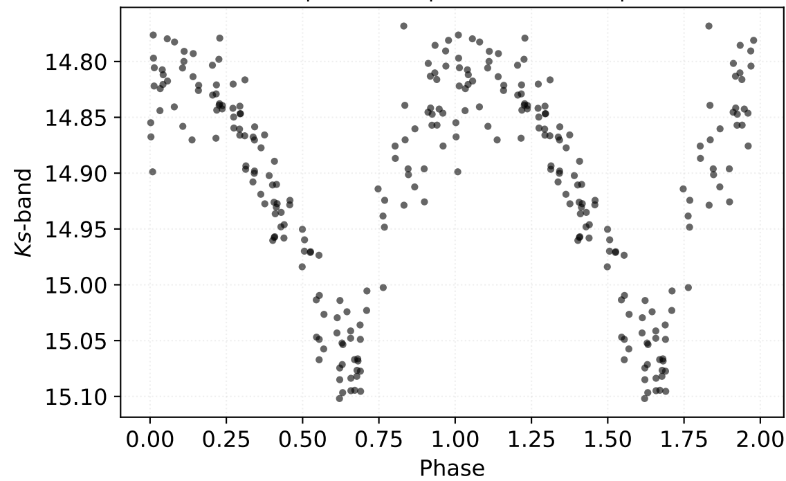
P: 0.48933 d | Class: RP | Subclass: RRab | Field b279
