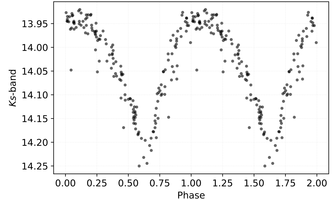
P: 0.43958 d | Class: RP | Subclass: RRab | Field b278
