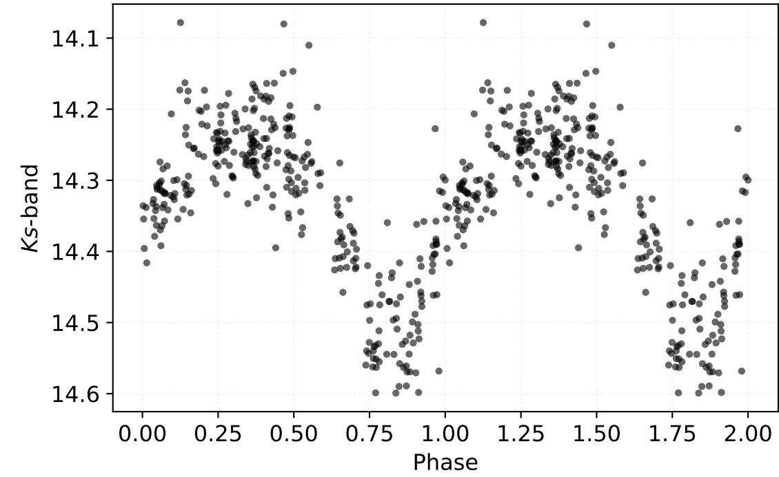
P: 0.29548 d | Class: RP | Subclass: UVAR | Field b278
