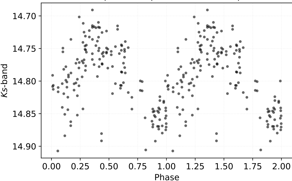
P: 2.10539 d | Class: RP | Subclass: CEP-1OT | Field b278
