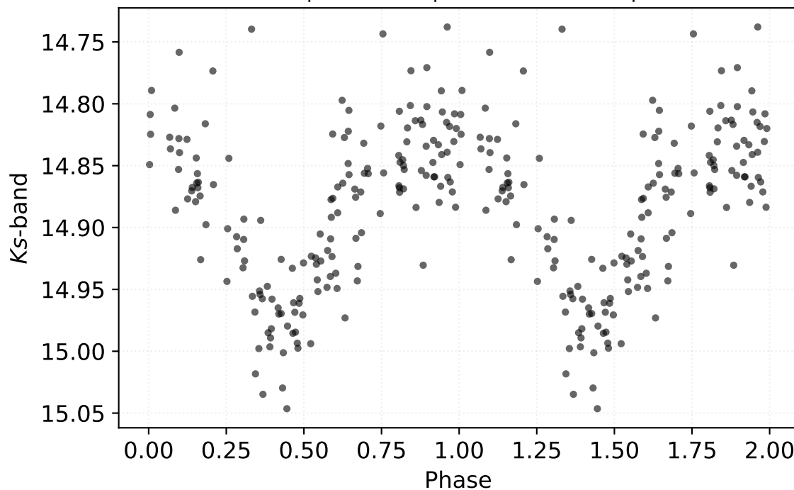
P: 0.18859 d | Class: RP | Subclass: UVAR | Field b279
