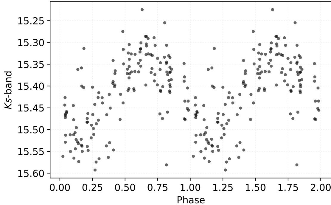
P: 0.46773 d | Class: RP | Subclass: CEP-1OT | Field b278
