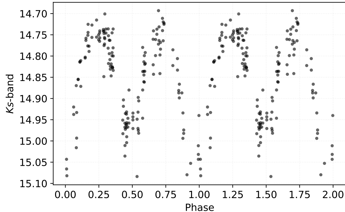
P: 1.12533 d | Class: EB | Subclass: UVAR | Field b279
