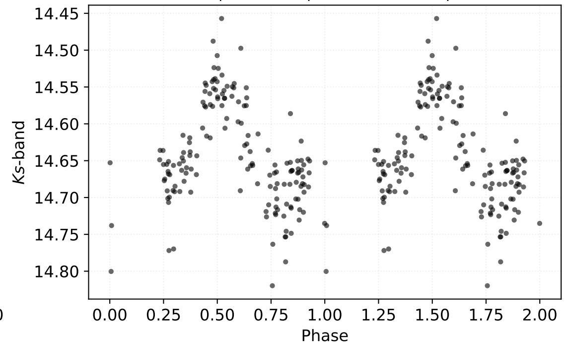
P: 33.35930 d | Class: RP | Subclass: UVAR | Field b279
