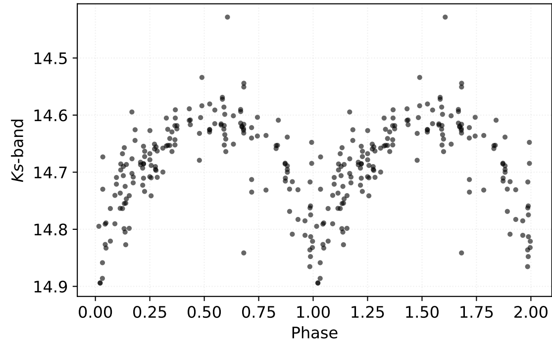
P: 0.55331 d | Class: RP | Subclass: CEP-1OT | Field b279
