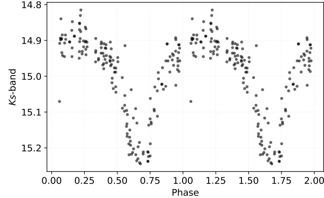
P: 0.22748 d | Class: RP | Subclass: UVAR | Field b278
