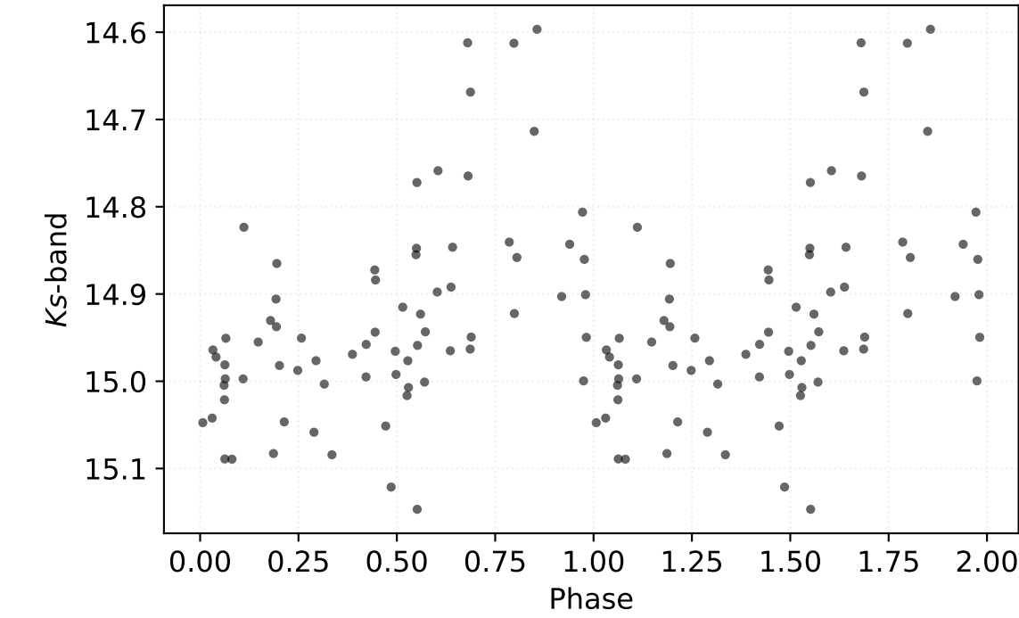
P: 0.41752 d | Class: RP | Subclass: RRab | Field b279
