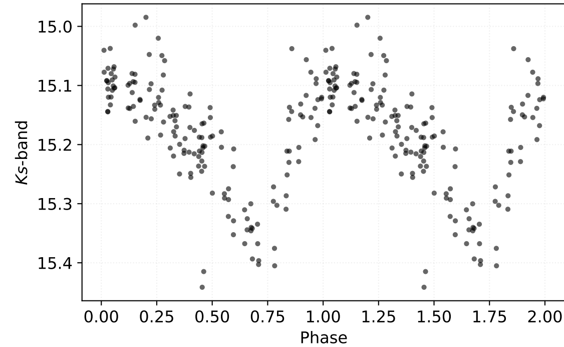
P: 0.57057 d | Class: RP | Subclass: RRab | Field b279
