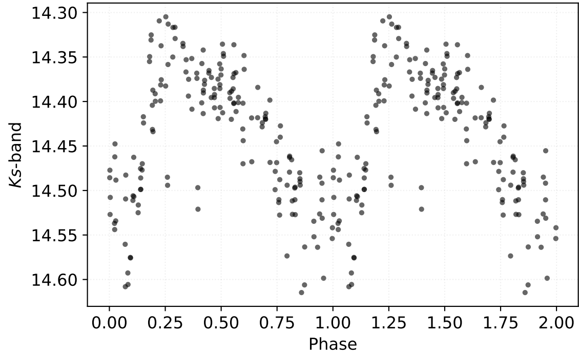
P: 0.57747 d | Class: RP | Subclass: RRab | Field b278
