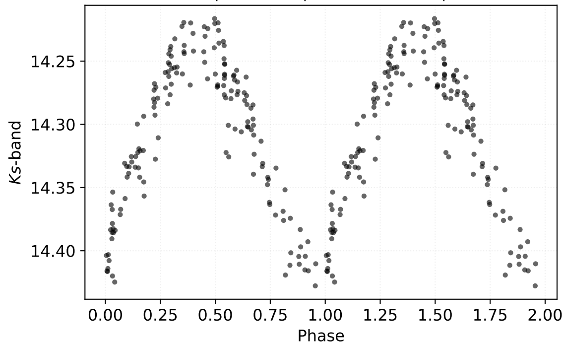
P: 0.19255 d | Class: RP | Subclass: UVAR | Field b279
