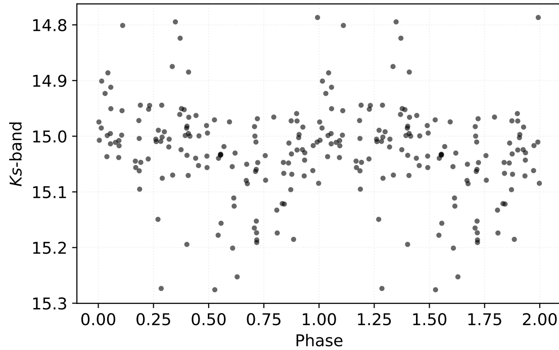
P: 7.68961 d | Class: EB | Subclass: UVAR | Field b279
