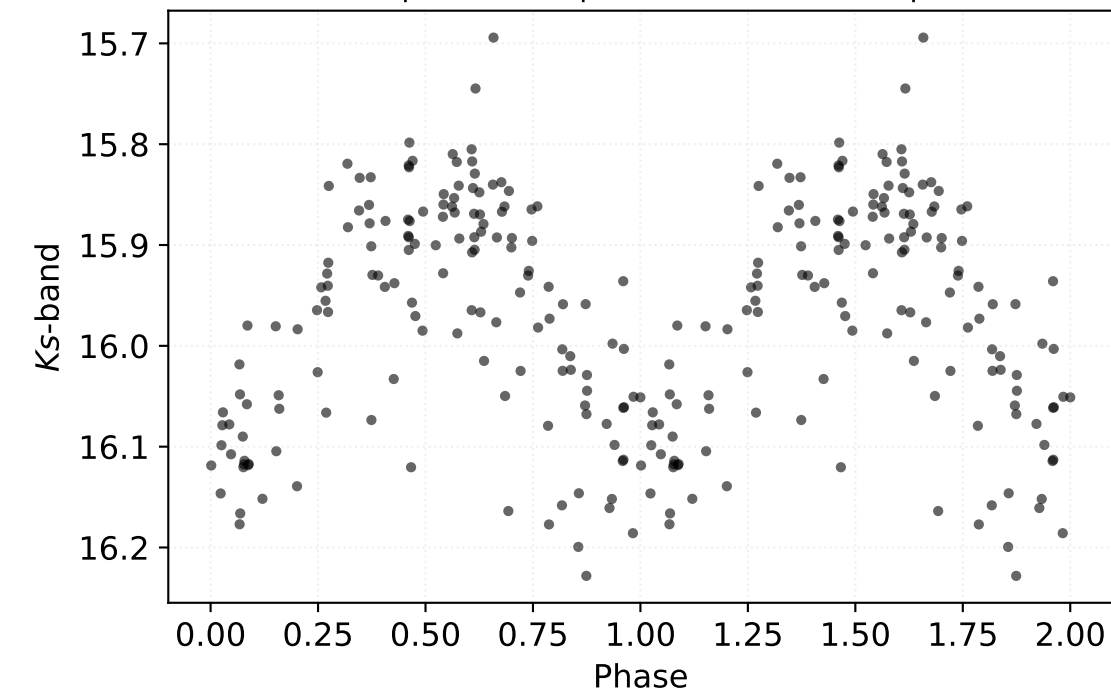
P: 0.46160 d | Class: RP | Subclass: CEP-1OT | Field b278
