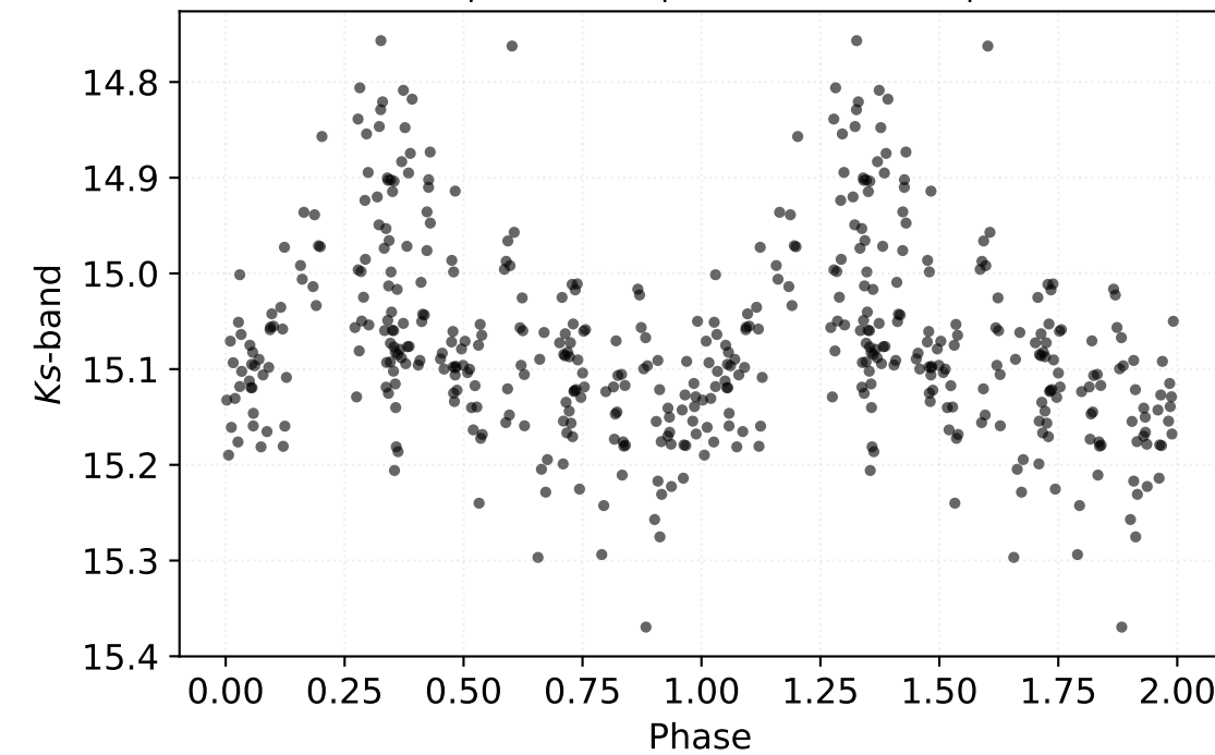
P: 0.19945 d | Class: RP | Subclass: UVAR | Field b278
