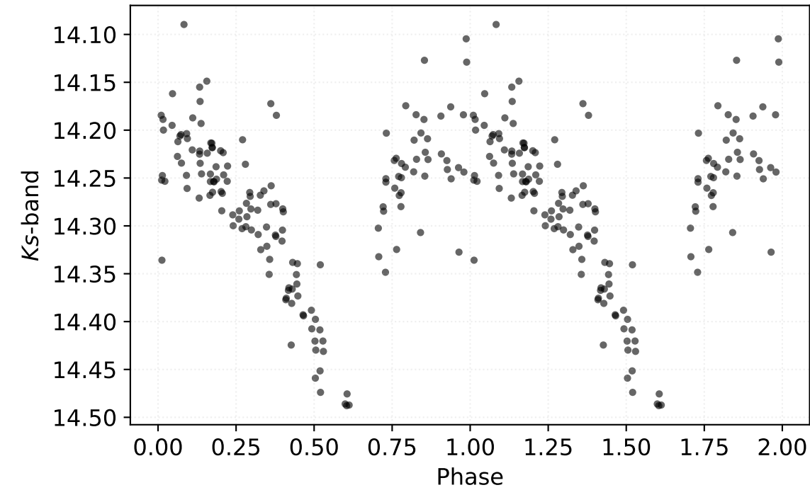
P: 0.39755 d | Class: RP | Subclass: RRab | Field b279
