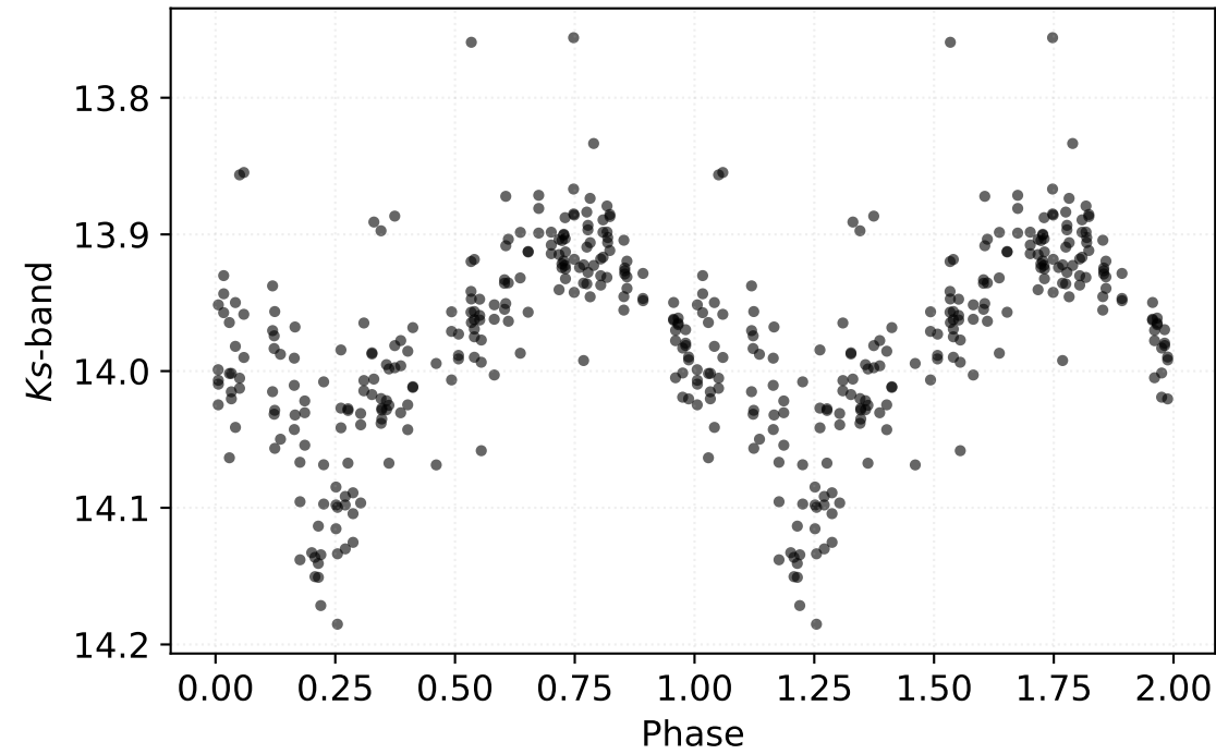
P: 0.65287 d | Class: RP | Subclass: CEP-1OT | Field b279
