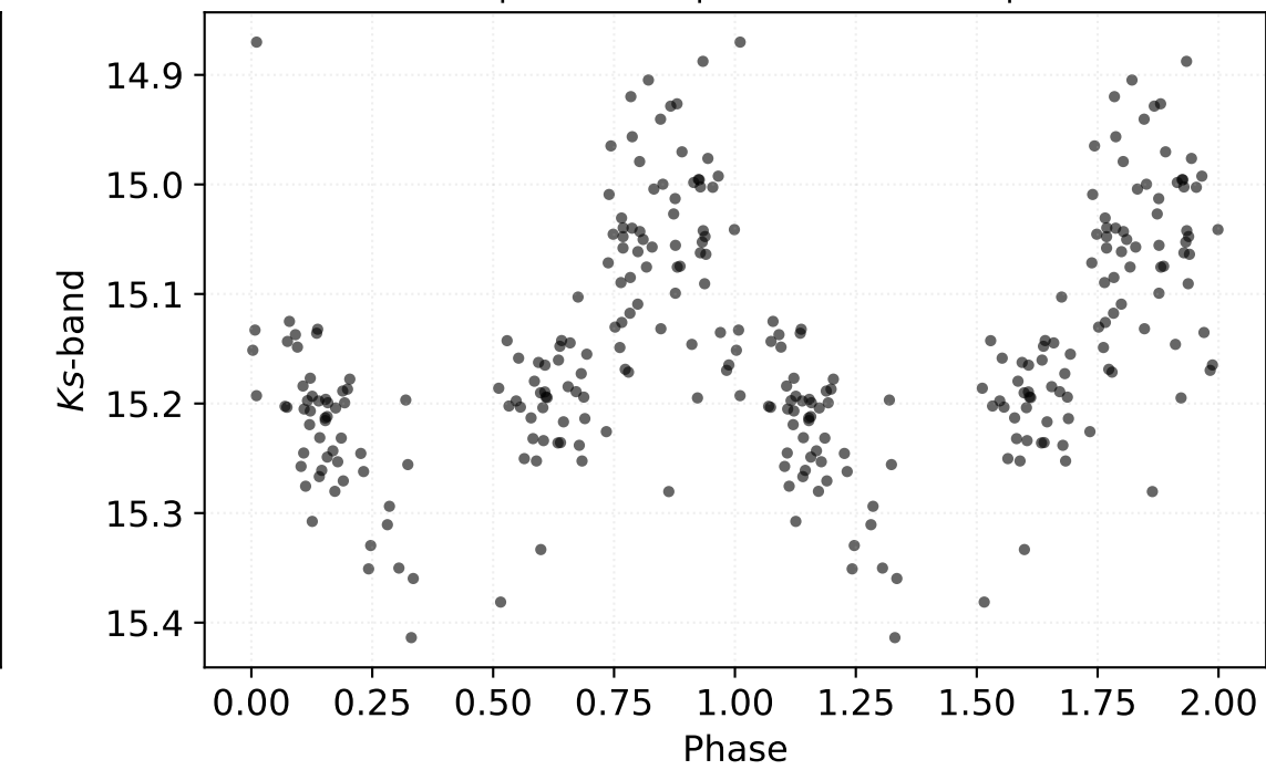
P: 0.14355 d | Class: RP | Subclass: UVAR | Field b279
