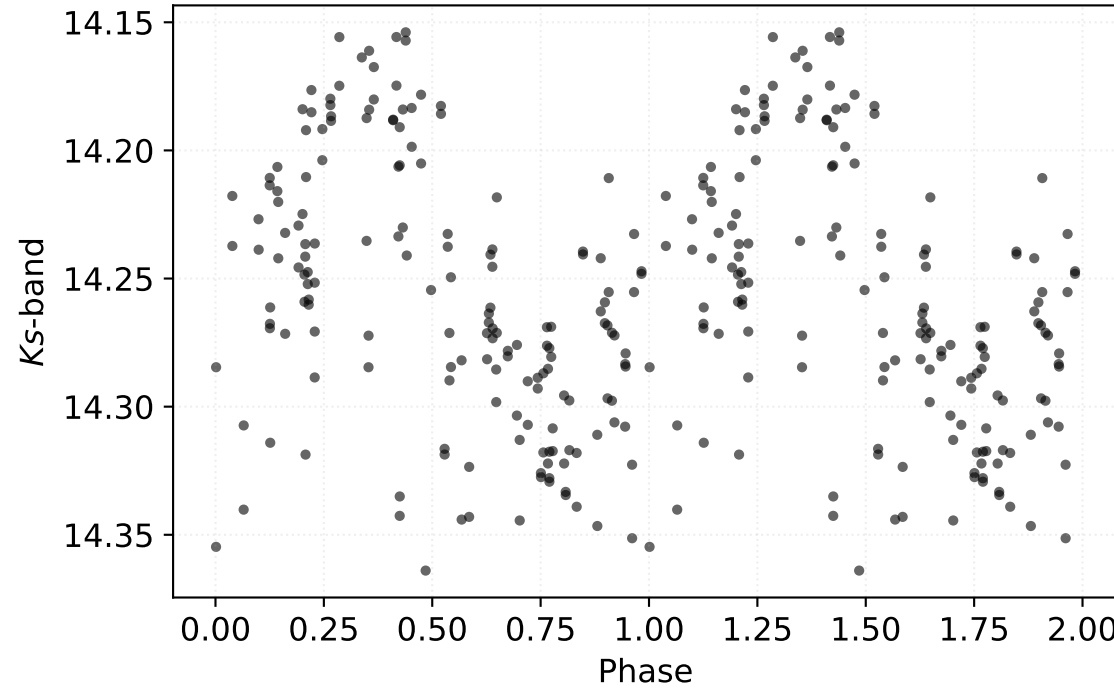
P: 0.75808 d | Class: RP | Subclass: CEP-1OT | Field b278
