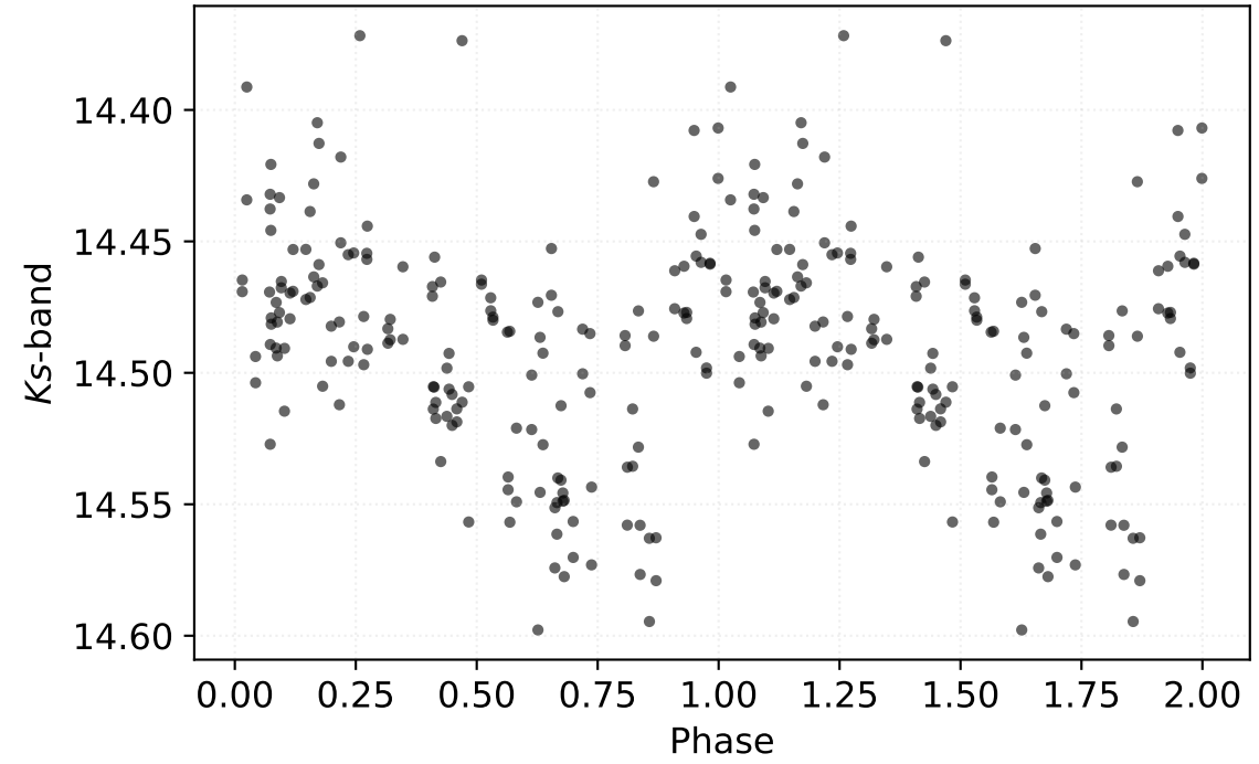
P: 0.32901 d | Class: RP | Subclass: CEP-1OT | Field b279
