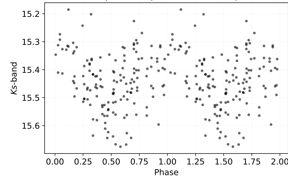
P: 0.99558 d | Class: RP | Subclass: CEP-1OT | Field b278
