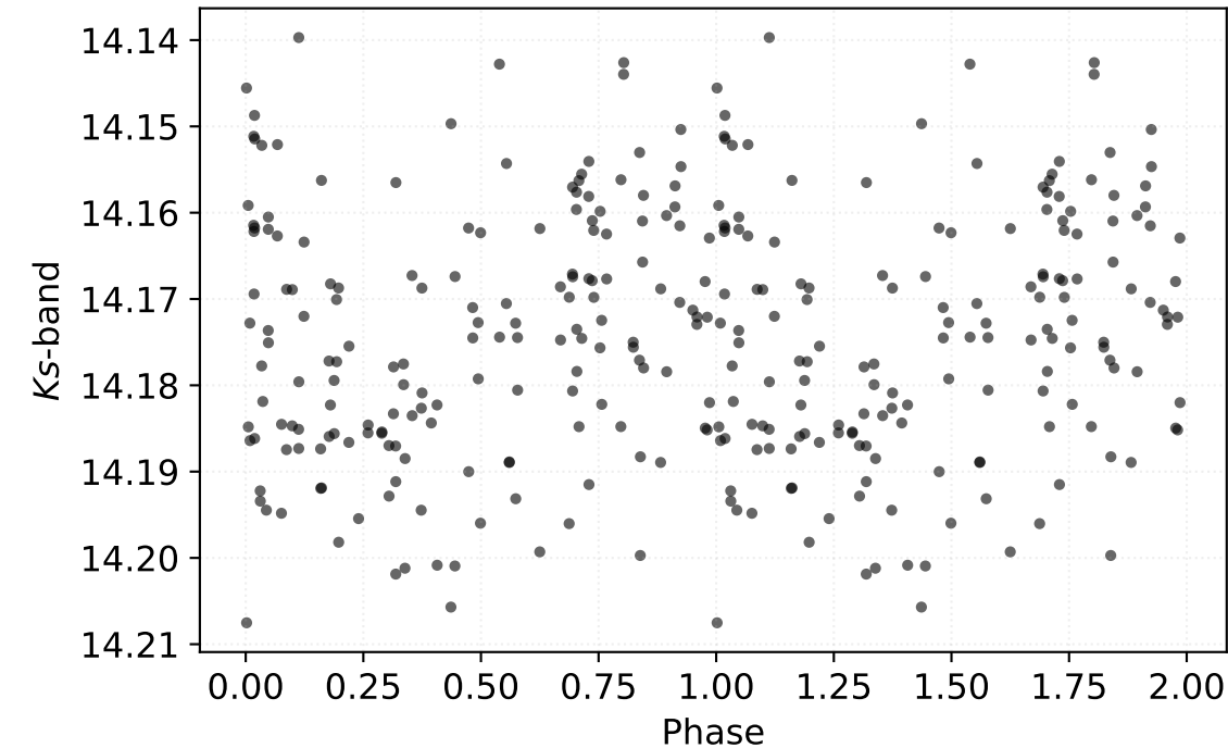
P: 1.54400 d | Class: RP | Subclass: CEP-1OT | Field b278
