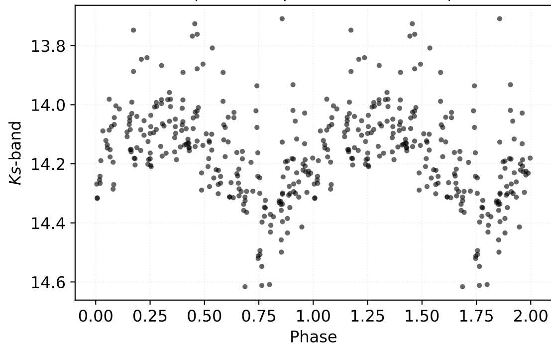
P: 0.39593 d | Class: RP | Subclass: CEP-1OT | Field b279
