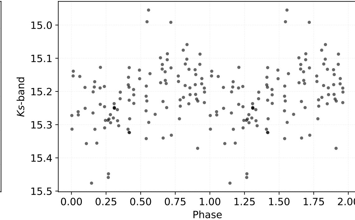
P: 0.33036 d | Class: RP | Subclass: RRc | Field b279
