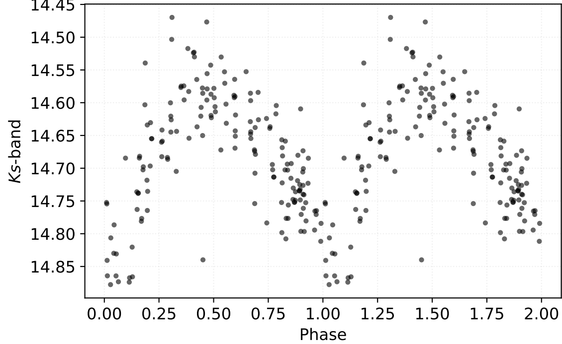
P: 0.61276 d | Class: RP | Subclass: RRab | Field b278
