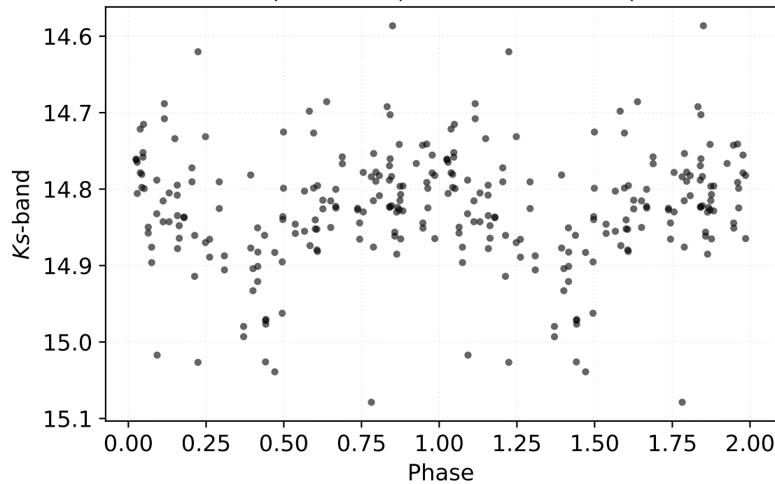
P: 2.49812 d | Class: RP | Subclass: CEP-1OT | Field b278
