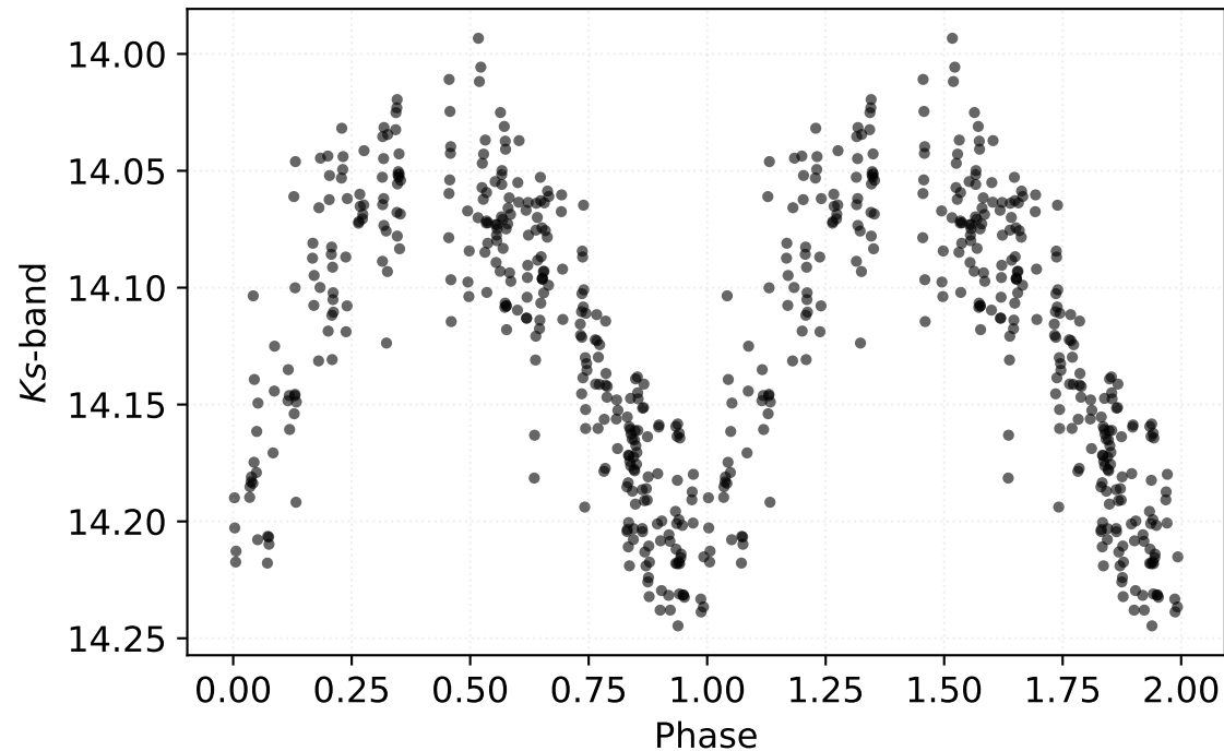
P: 0.56163 d | Class: RP | Subclass: CEP-1OT | Field b278
