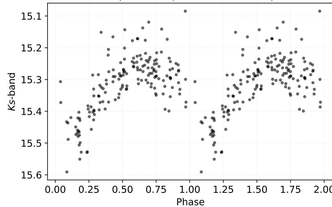
P: 0.49101 d | Class: RP | Subclass: CEP-1OT | Field b278
