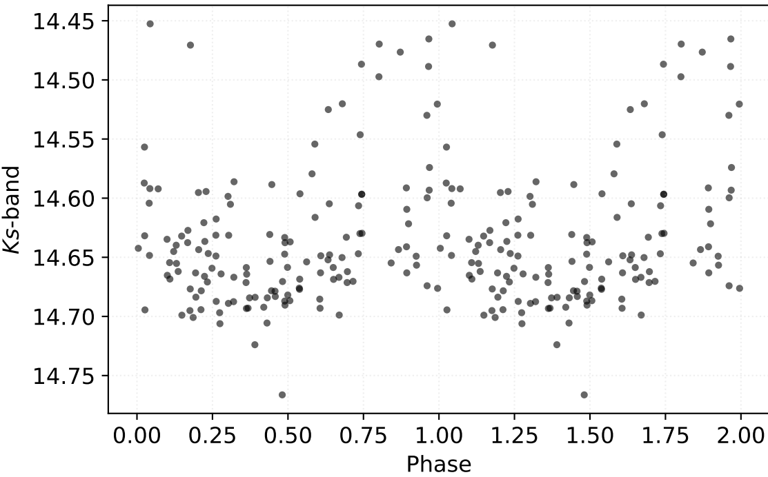
P: 0.43074 d | Class: RP | Subclass: CEP-1OT | Field b278
