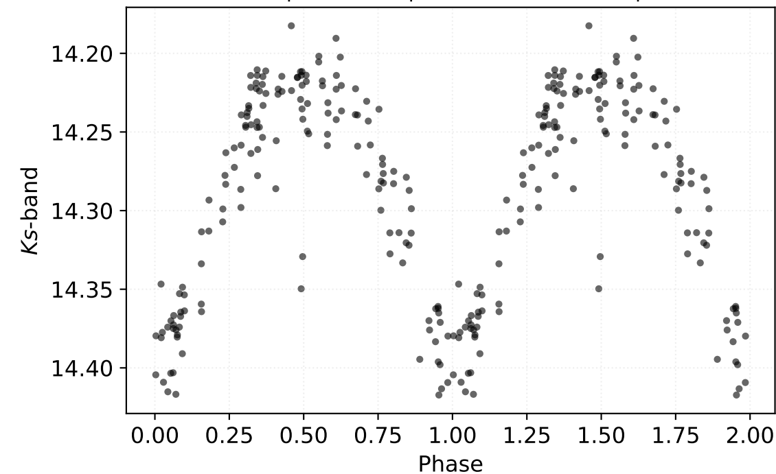
P: 0.47518 d | Class: RP | Subclass: CEP-1OT | Field b279
