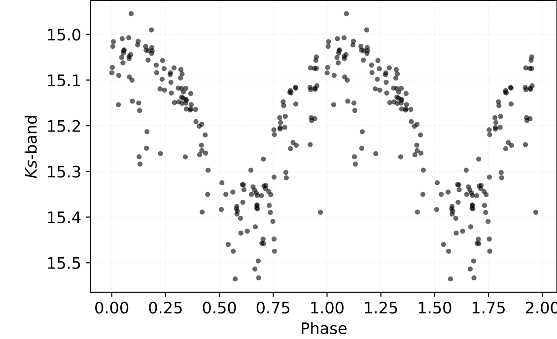
P: 0.77227 d | Class: RP | Subclass: RRab | Field b278
