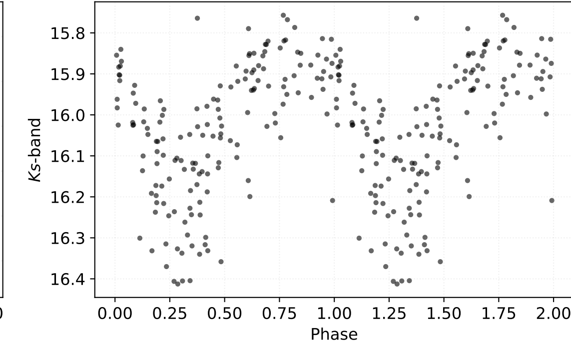
P: 0.31571 d | Class: RP | Subclass: RRc | Field b279
