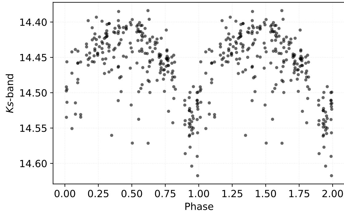
P: 0.62216 d | Class: RP | Subclass: CEP-1OT | Field b279
