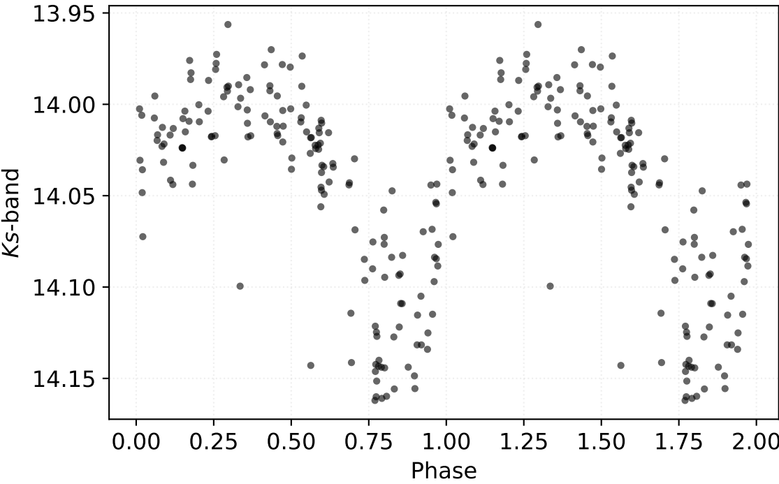
P: 0.61991 d | Class: RP | Subclass: CEP-1OT | Field b279
