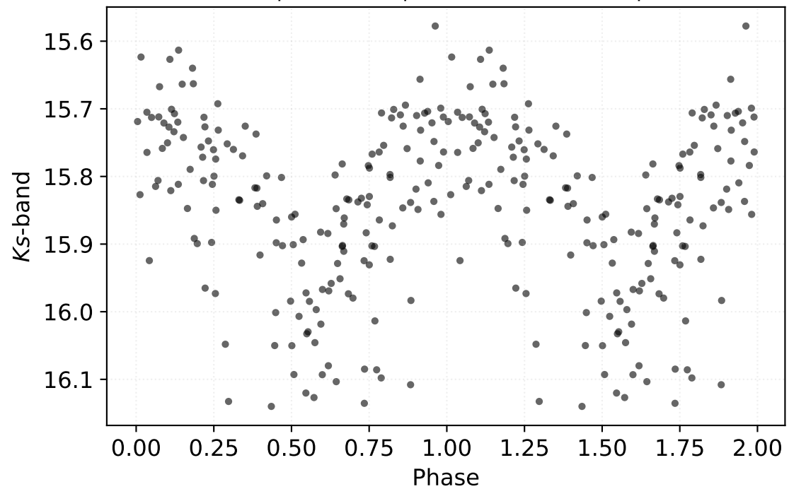
P: 5.82890 d | Class: RP | Subclass: CEP-1OT | Field b278
