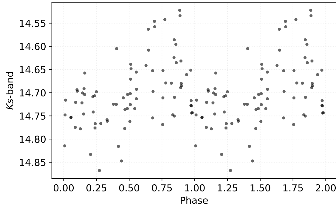
P: 0.38400 d | Class: RP | Subclass: CEP-1OT | Field b278
