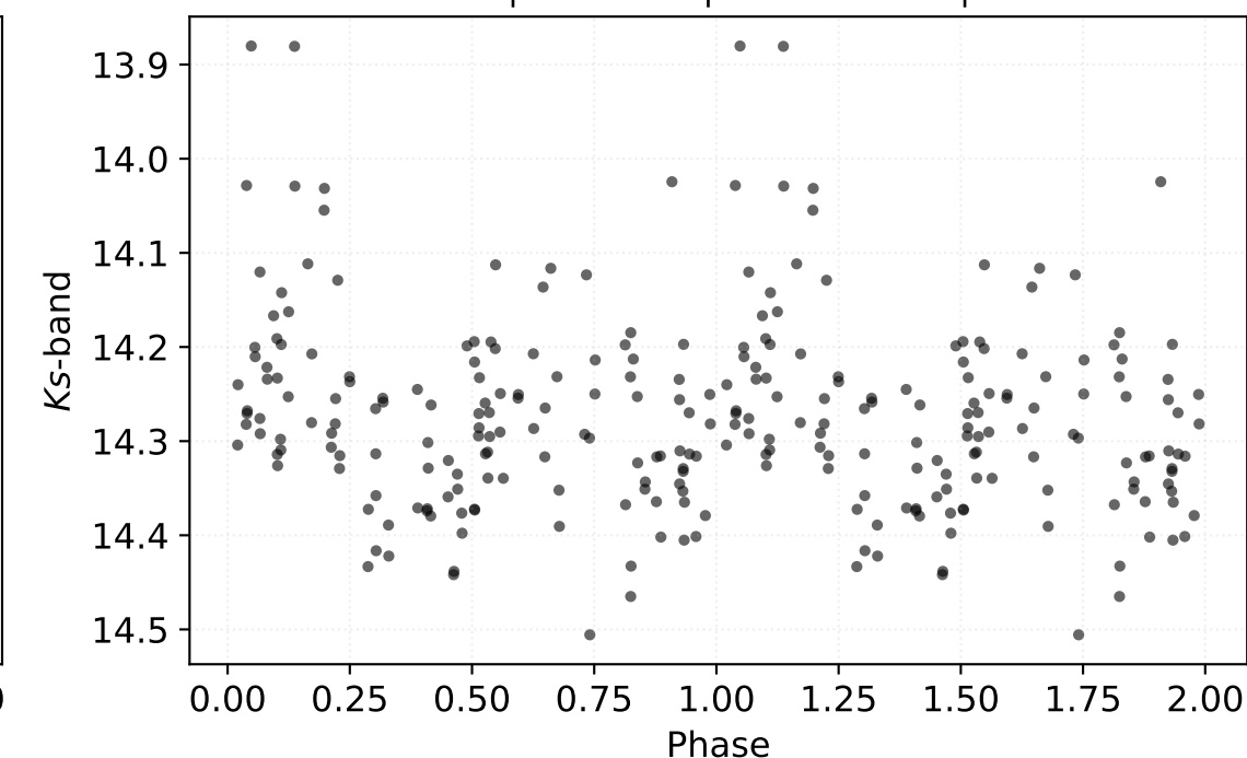
P: 0.27989 d | Class: EB | Subclass: EA | Field b278
