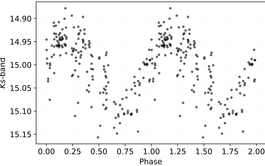
P: 0.41959 d | Class: RP | Subclass: CEP-1OT | Field b278
