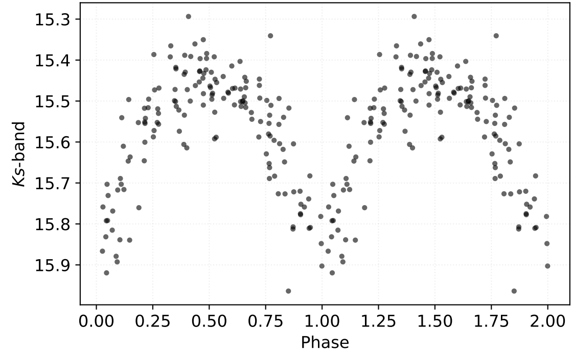
P: 0.52221 d | Class: RP | Subclass: RRab | Field b278
