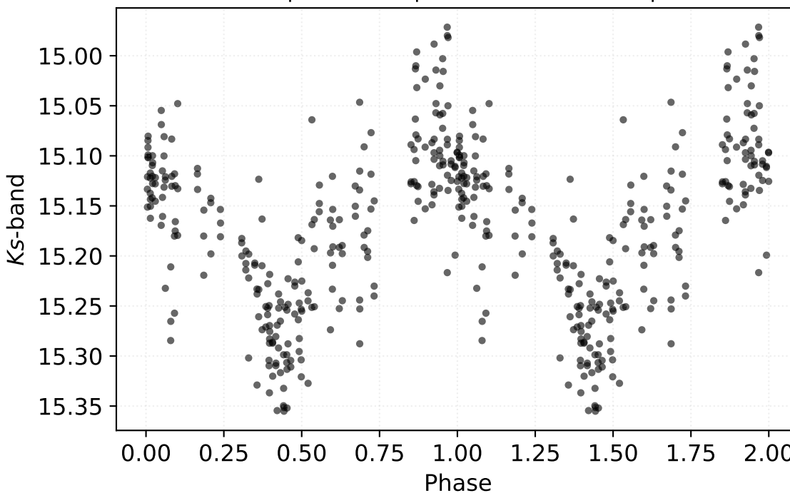
P: 8.62805 d | Class: RP | Subclass: CEP-1OT | Field b278
