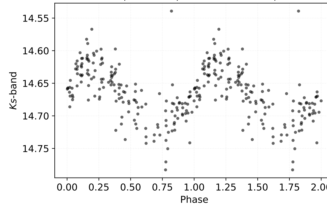
P: 0.38103 d | Class: RP | Subclass: CEP-1OT | Field b279
