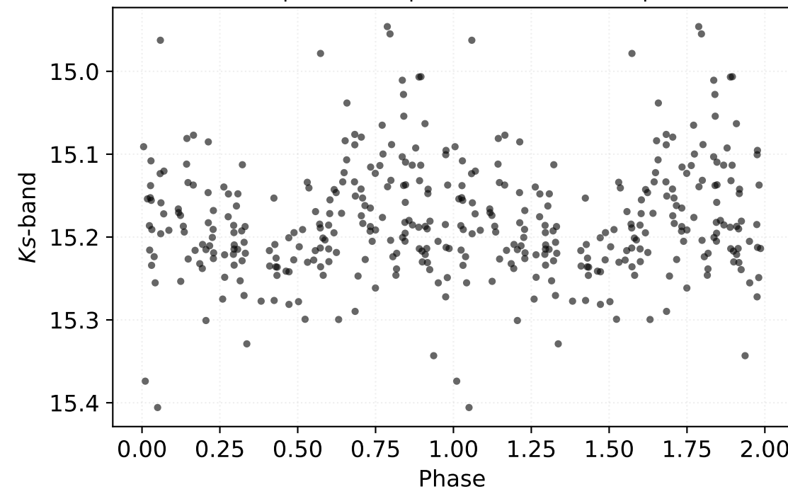
P: 8.11598 d | Class: RP | Subclass: CEP-1OT | Field b278
