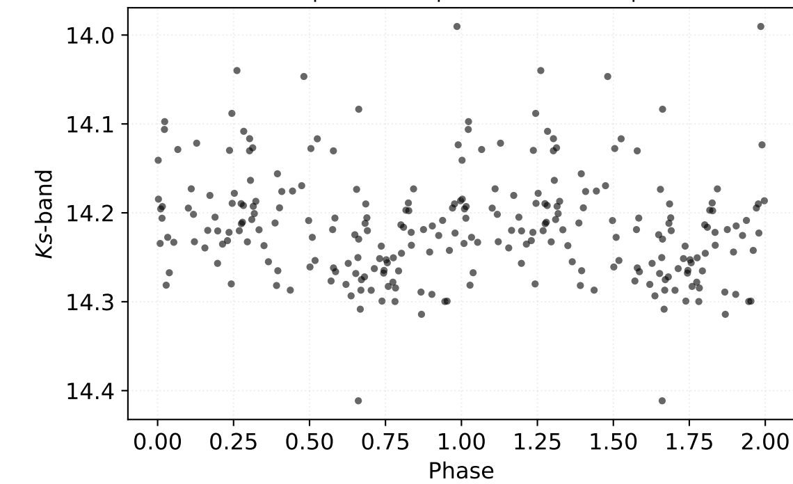
P: 0.15084 d | Class: RP | Subclass: UVAR | Field b279
