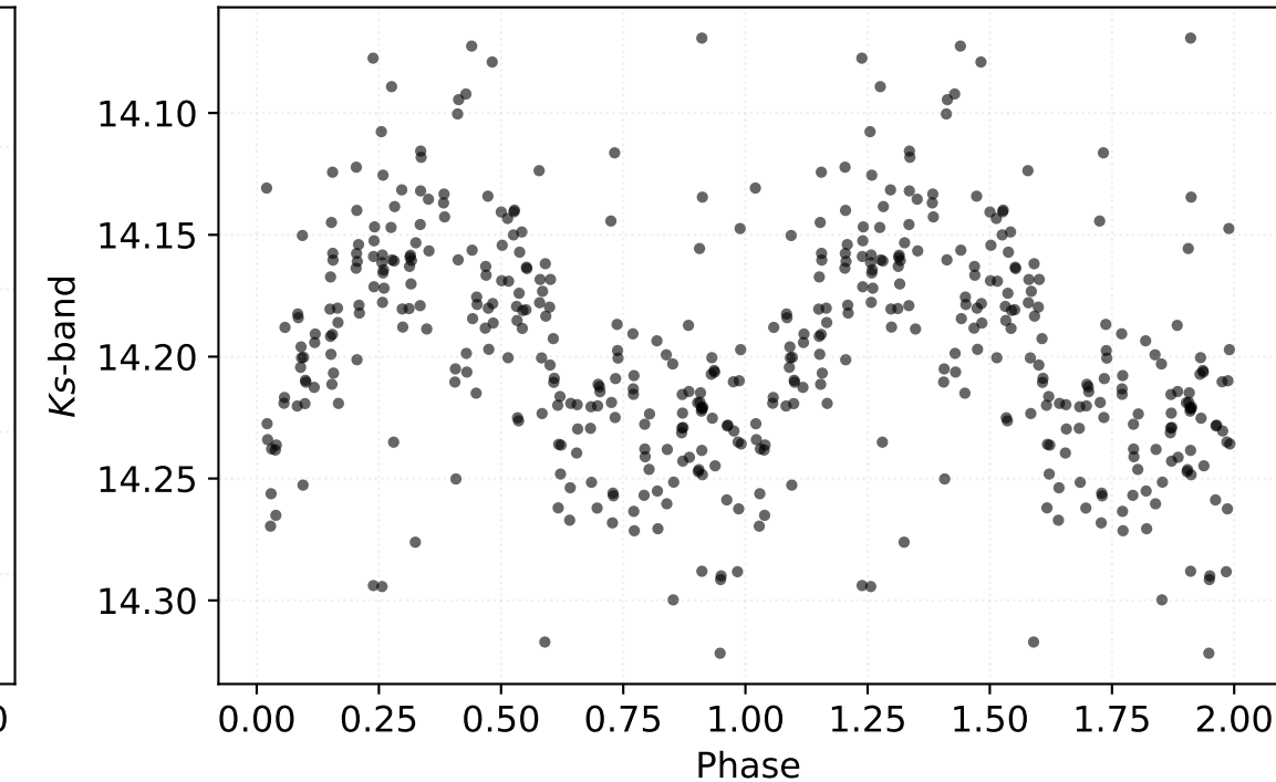
P: 0.40185 d | Class: RP | Subclass: RRc | Field b278
