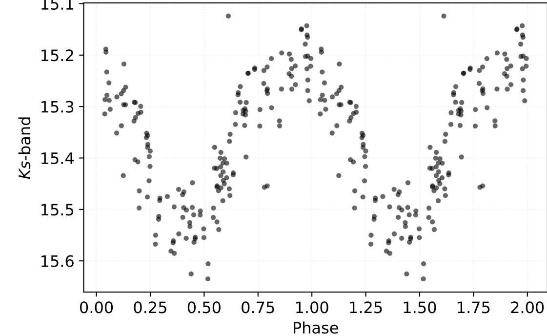
P: 0.60583 d | Class: RP | Subclass: CEP-1OT | Field b278
