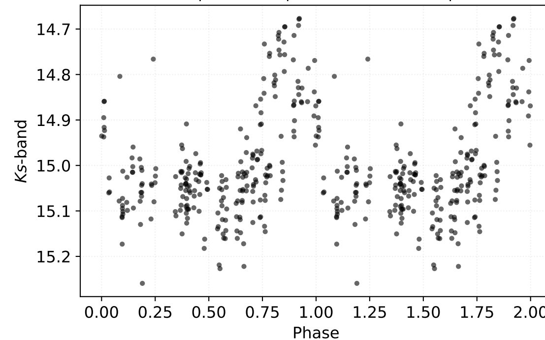
P: 0.54920 d | Class: RP | Subclass: CEP-1OT | Field b278
