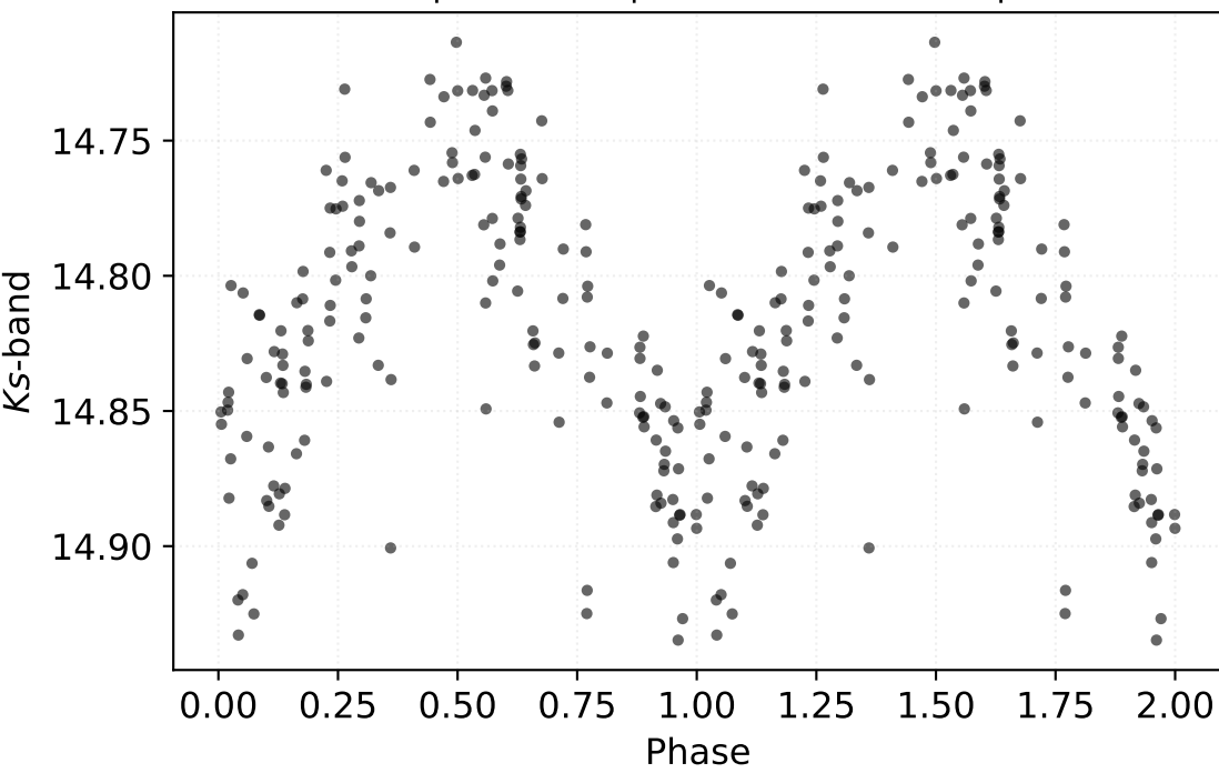
P: 0.31221 d | Class: RP | Subclass: CEP-1OT | Field b278
