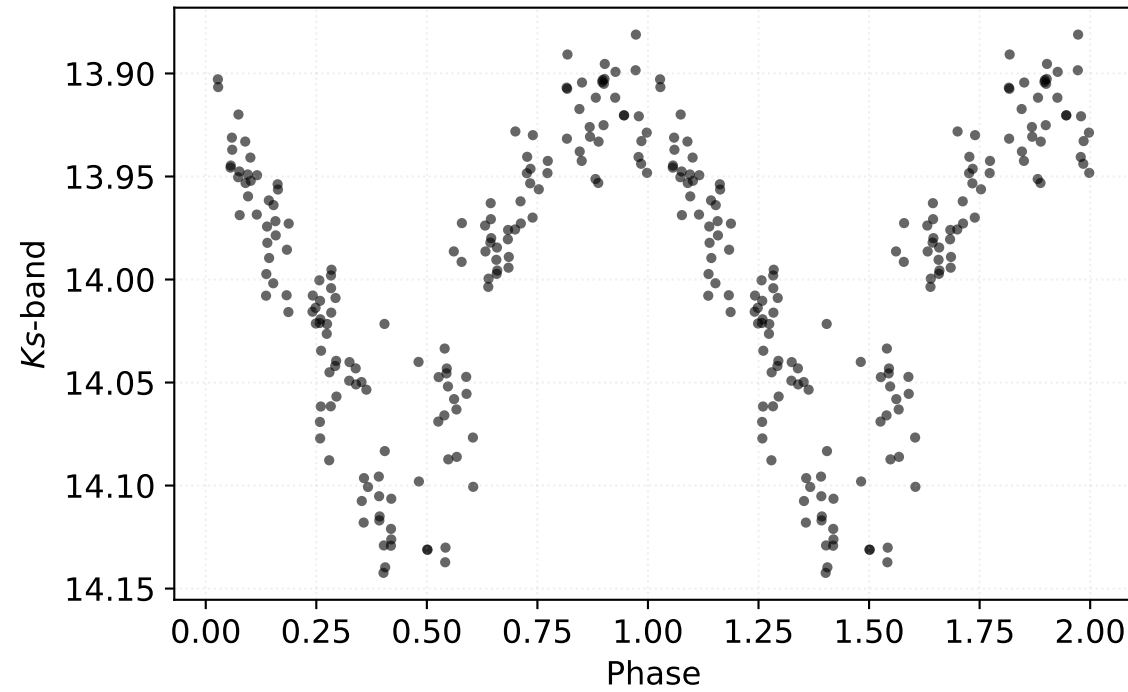
P: 1.11445 d | Class: EB | Subclass: RRc | Field b278
