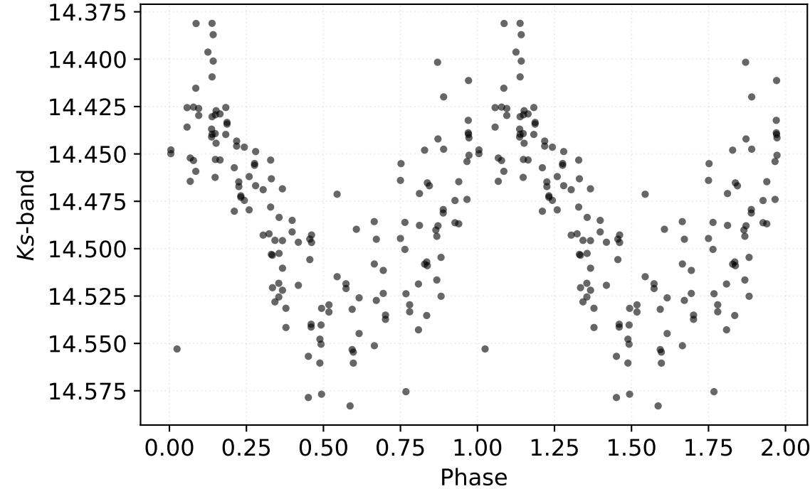
P: 2.85653 d | Class: RP | Subclass: CEP-F | Field b279
