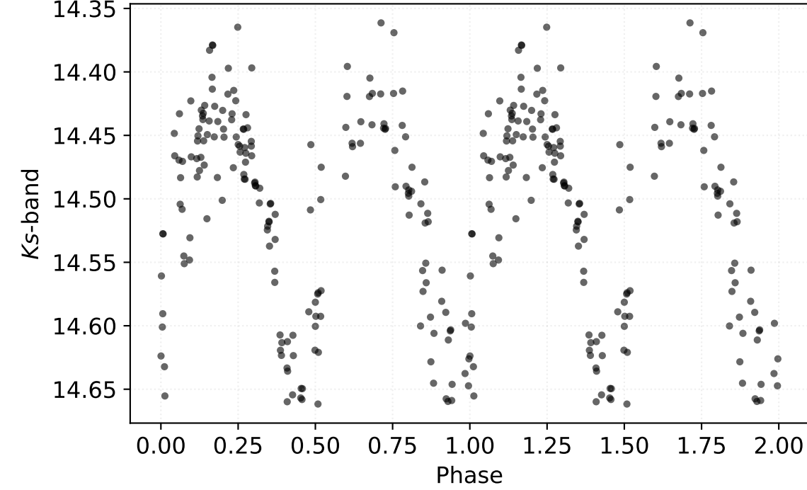
P: 0.41881 d | Class: RP | Subclass: RRc | Field b278
