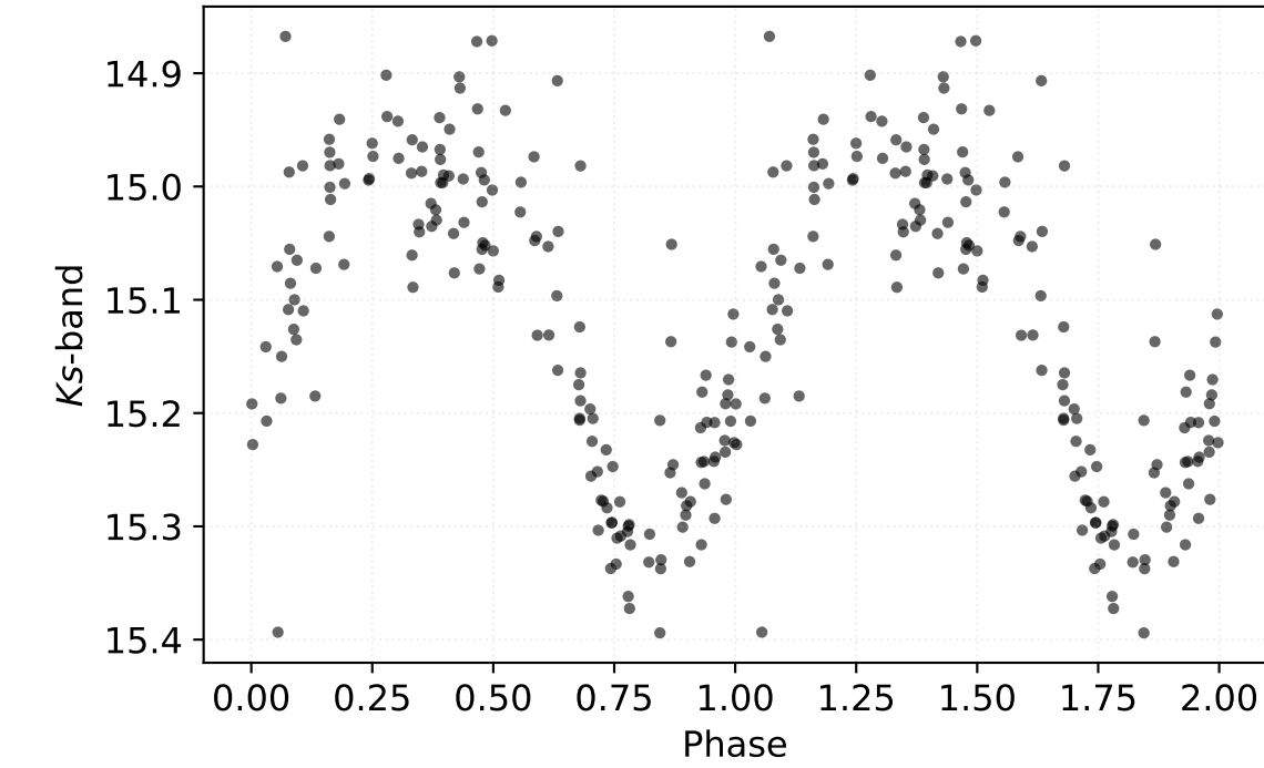
P: 0.52006 d | Class: RP | Subclass: RRc | Field b279
