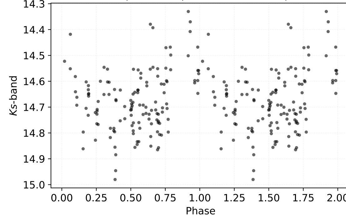
P: 1.86126 d | Class: RP | Subclass: CEP-1OT | Field b278
