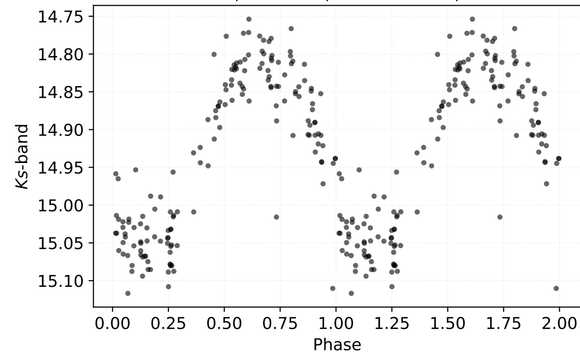
P: 0.49812 d | Class: RP | Subclass: RRc | Field b279
