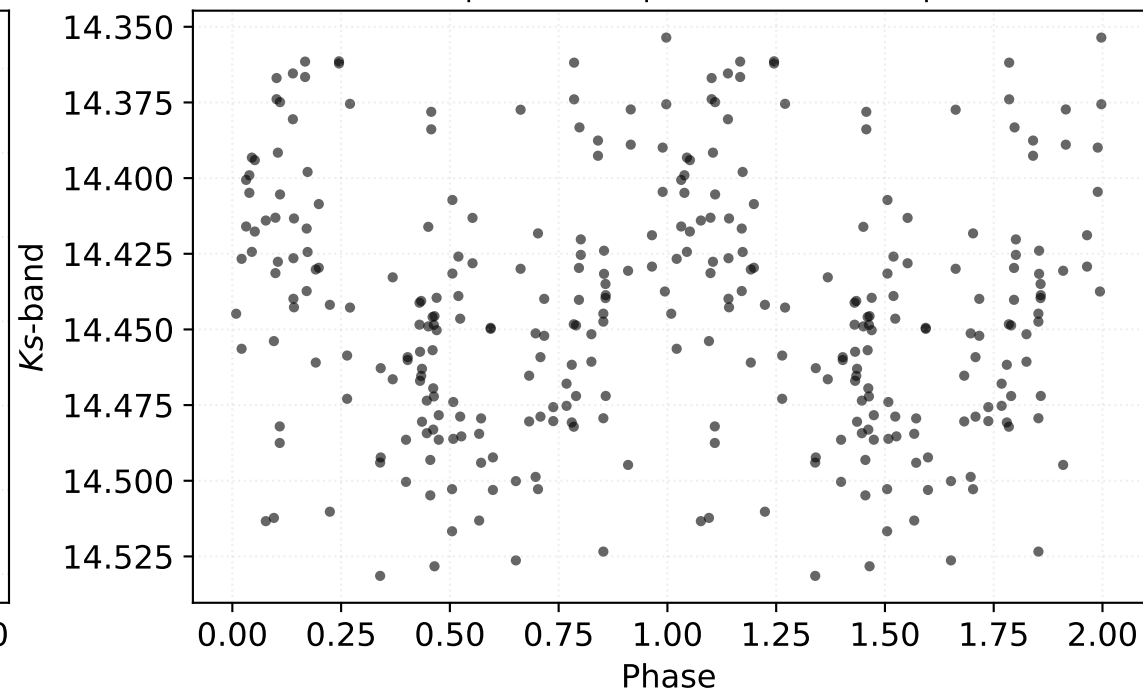
P: 0.12465 d | Class: RP | Subclass: UVAR | Field b279
