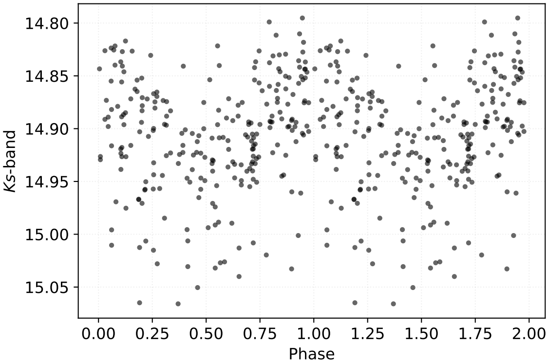
P: 12.83232 d | Class: RP | Subclass: CEP-F | Field b278
