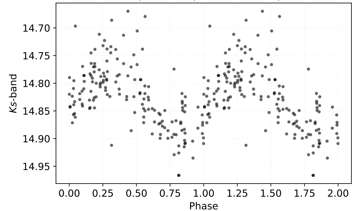
P: 0.31734 d | Class: RP | Subclass: RRab | Field b279
