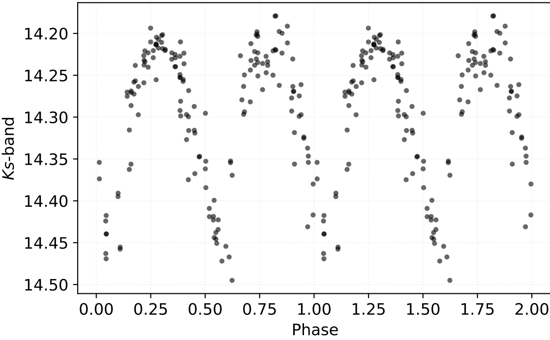
P: 0.20038 d | Class: RP | Subclass: UVAR | Field b278
