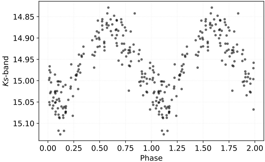
P: 0.15426 d | Class: RP | Subclass: UVAR | Field b279
