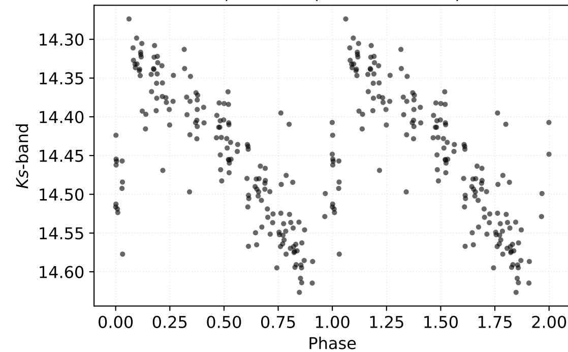
P: 0.55207 d | Class: RP | Subclass: RRab | Field b278
