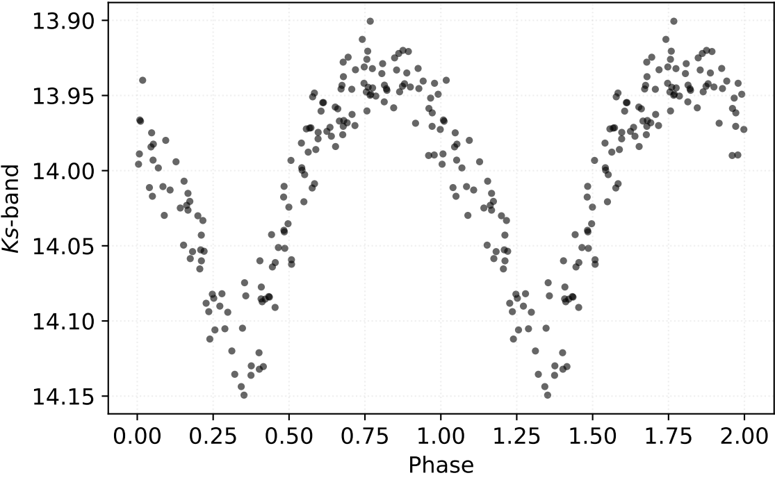
P: 0.61088 d | Class: RP | Subclass: RRab | Field b278
