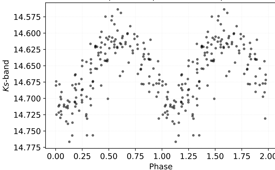
P: 0.43308 d | Class: RP | Subclass: RRab | Field b278
