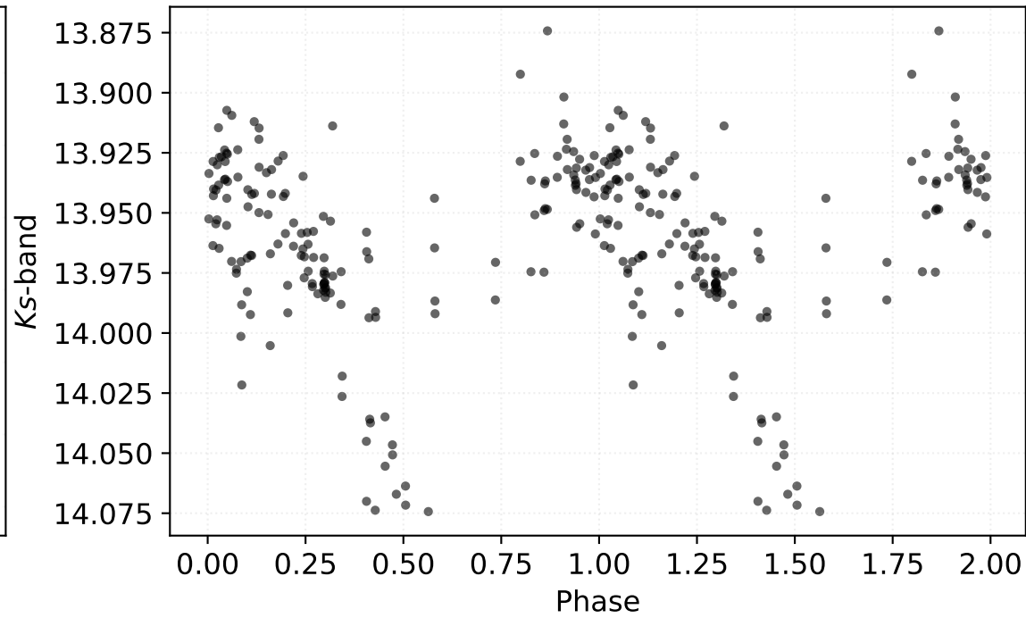
P: 0.99691 d | Class: RP | Subclass: CEP-1OT | Field b278
