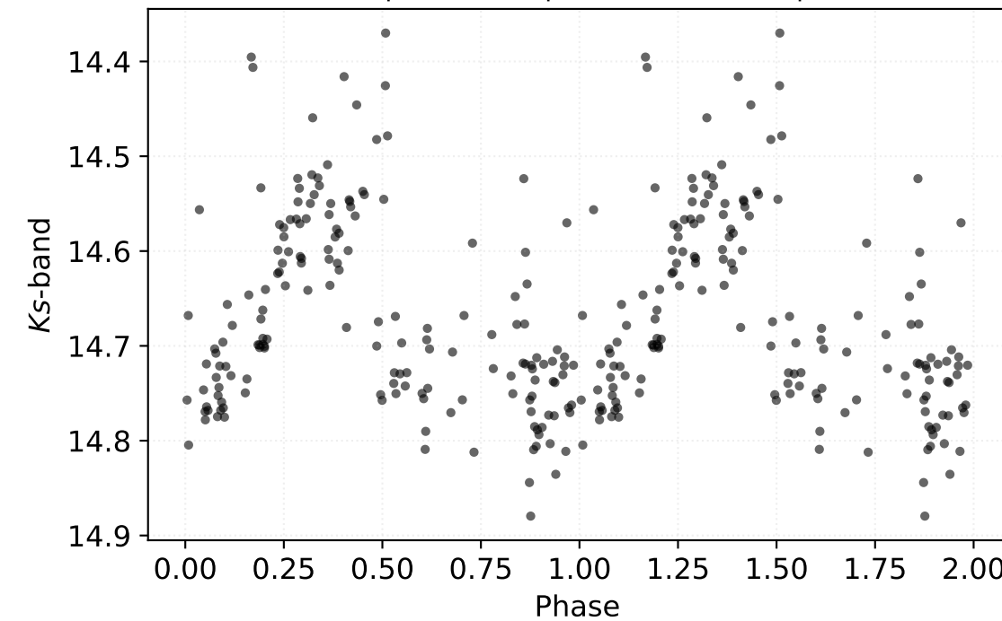
P: 0.16756 d | Class: RP | Subclass: UVAR | Field b278
