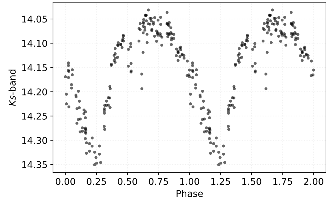
P: 0.37808 d | Class: RP | Subclass: RRab | Field b278
