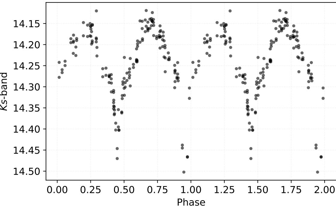
P: 0.12300 d | Class: RP | Subclass: UVAR | Field b278
