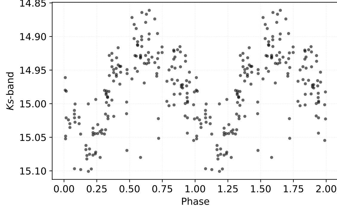
P: 0.73629 d | Class: RP | Subclass: RRab | Field b278
