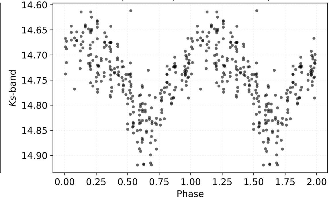
P: 0.79126 d | Class: RP | Subclass: CEP-1OT | Field b278
