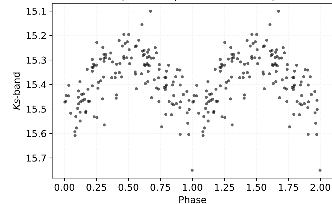
P: 3.14426 d | Class: RP | Subclass: CEP-1OT | Field b278
