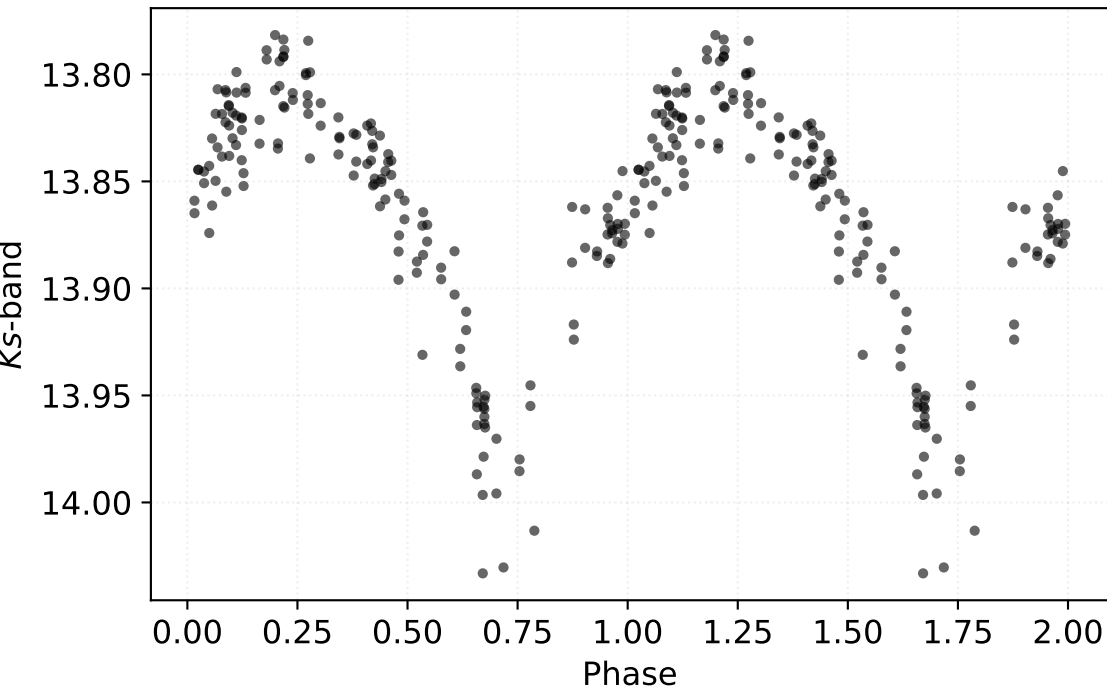
P: 0.40554 d | Class: RP | Subclass: CEP-1OT | Field b279
