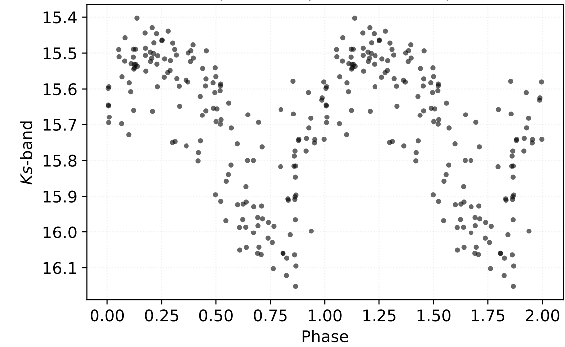
P: 0.61361 d | Class: RP | Subclass: RRab | Field b279
