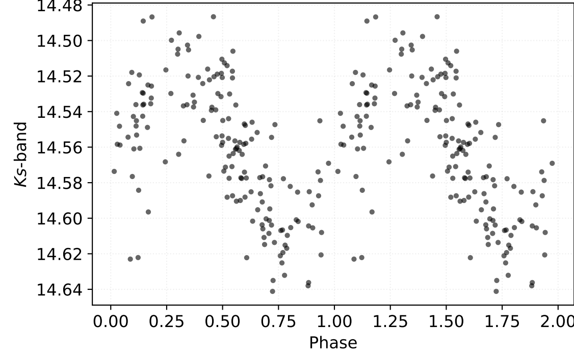
P: 0.63008 d | Class: RP | Subclass: CEP-1OT | Field b278
