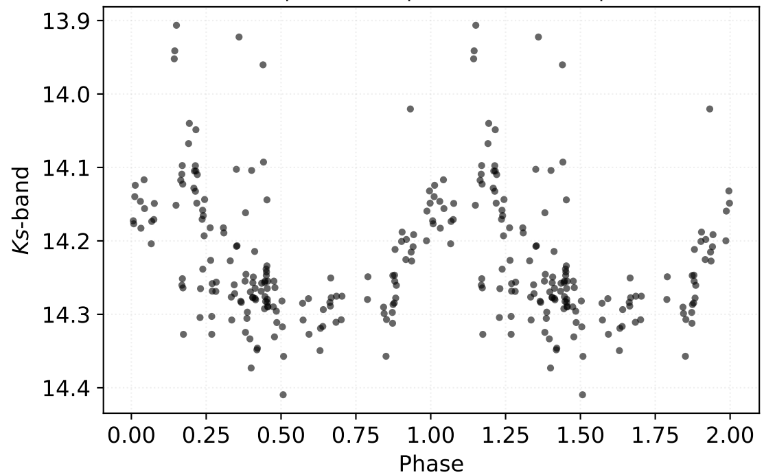
P: 0.13020 d | Class: RP | Subclass: UVAR | Field b278
