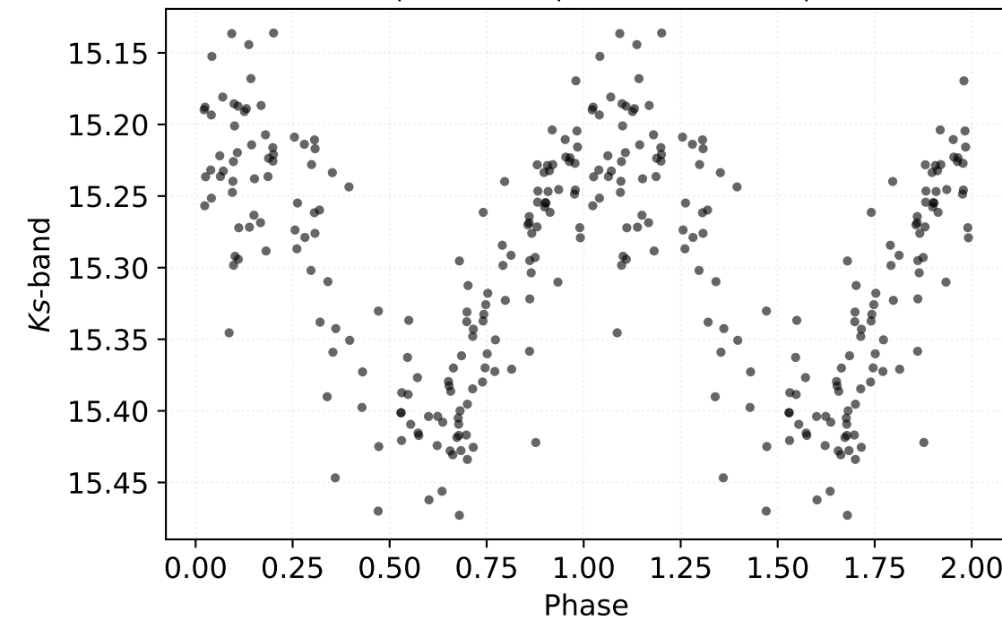
P: 0.30529 d | Class: RP | Subclass: RRab | Field b278
