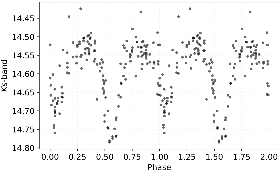
P: 1.12279 d | Class: EB | Subclass: UVAR | Field b278
