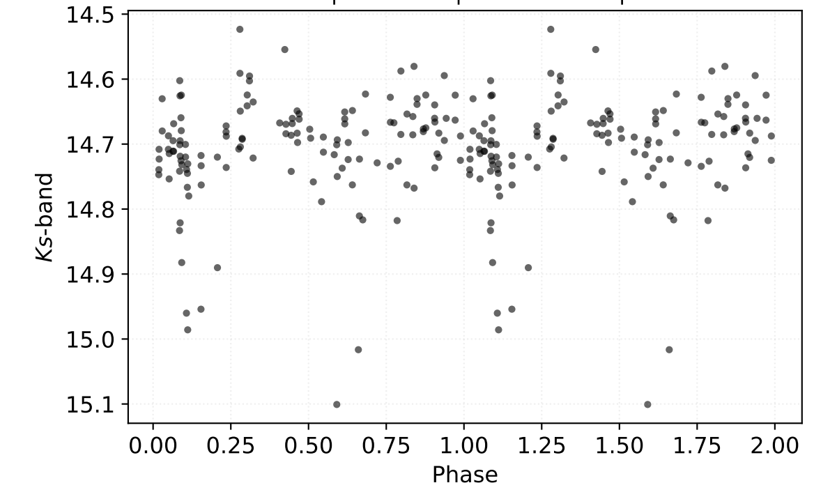
P: 0.39890 d | Class: EB | Subclass: EA | Field b278
