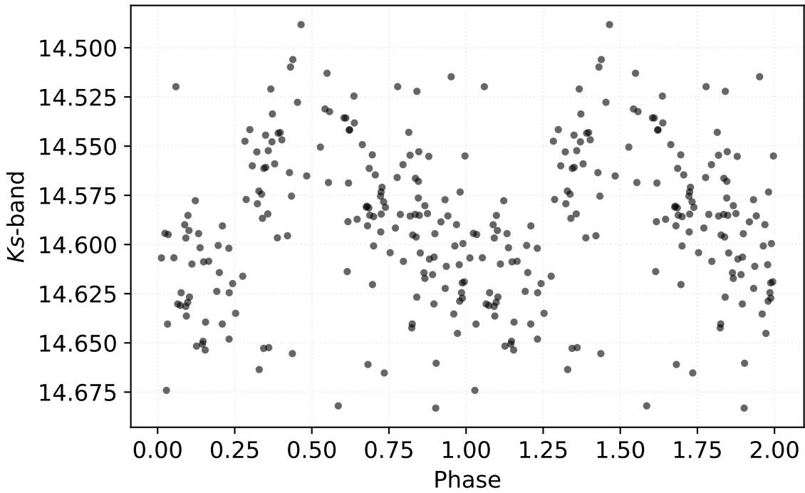
P: 8.77232 d | Class: RP | Subclass: CEP-1OT | Field b279
