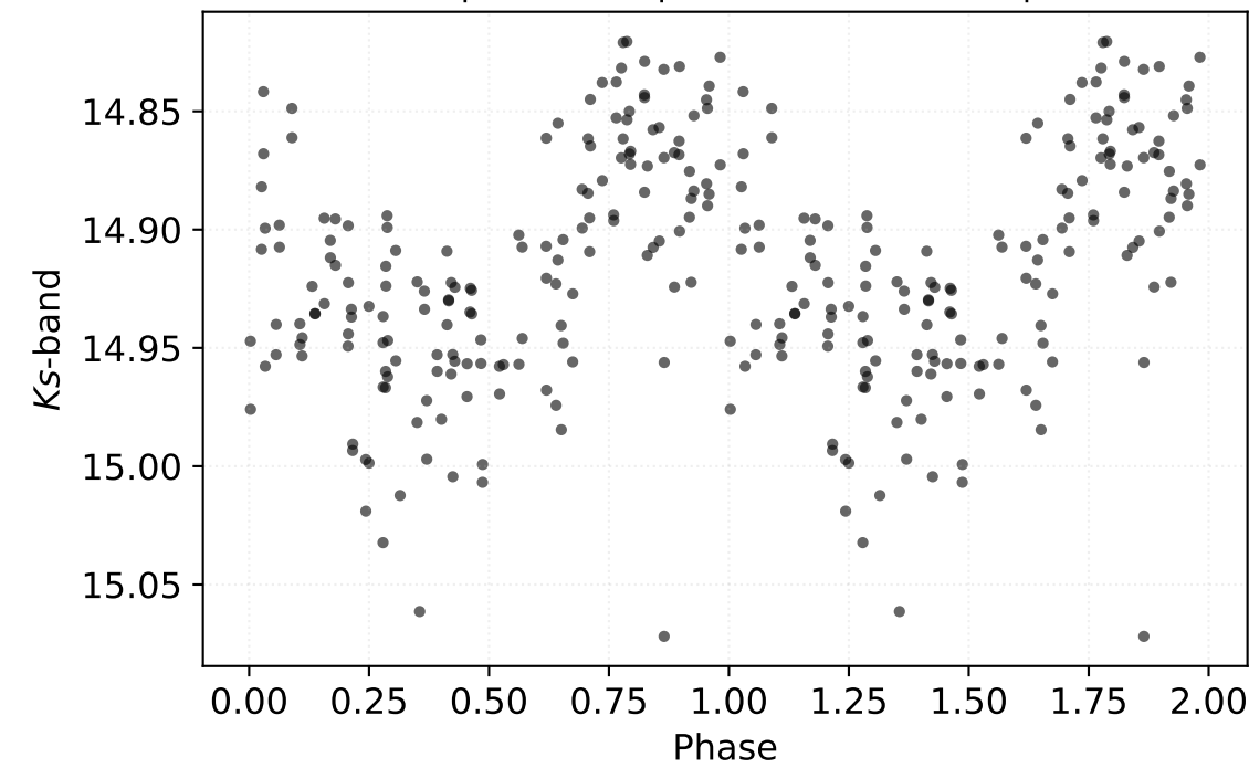
P: 0.50648 d | Class: RP | Subclass: CEP-1OT | Field b279
