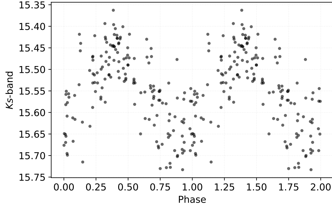
P: 0.31557 d | Class: RP | Subclass: CEP-1OT | Field b279
