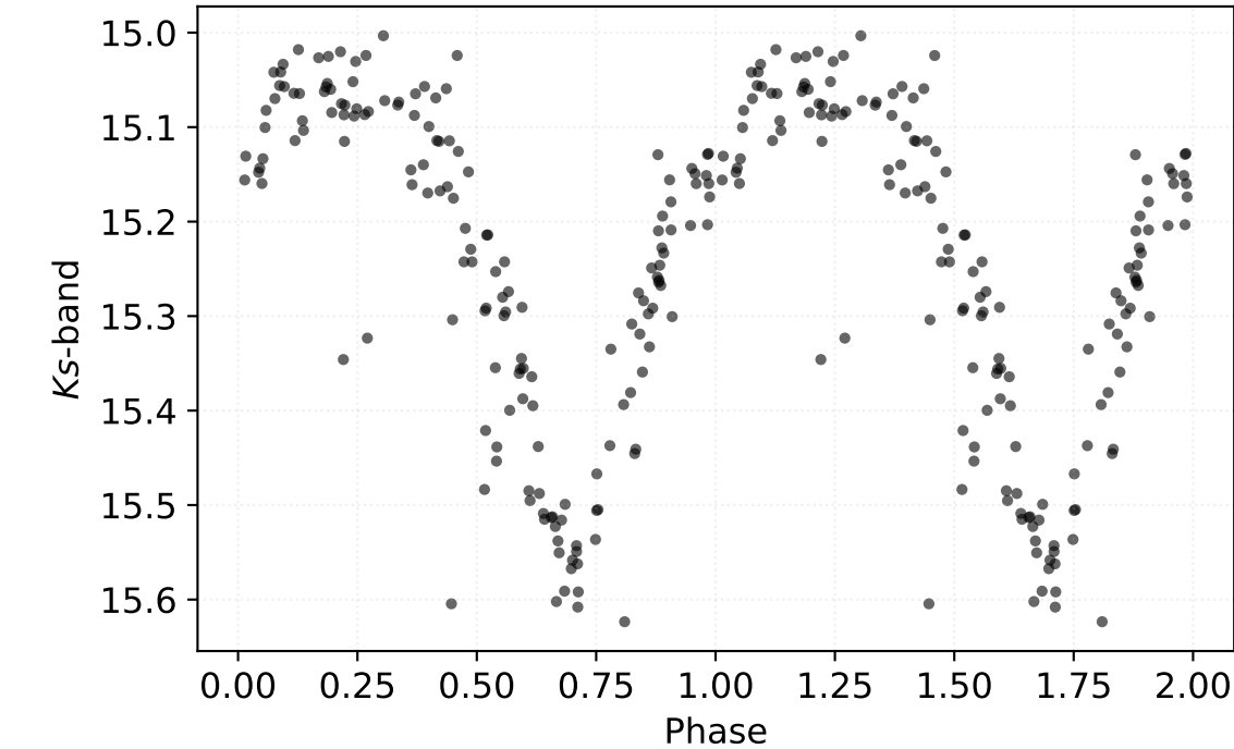
P: 0.22978 d | Class: RP | Subclass: UVAR | Field b279
