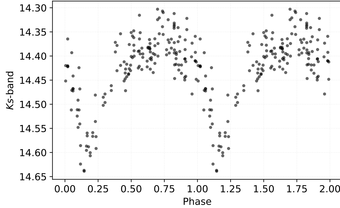
P: 2.53217 d | Class: RP | Subclass: CEP-1OT | Field b279
