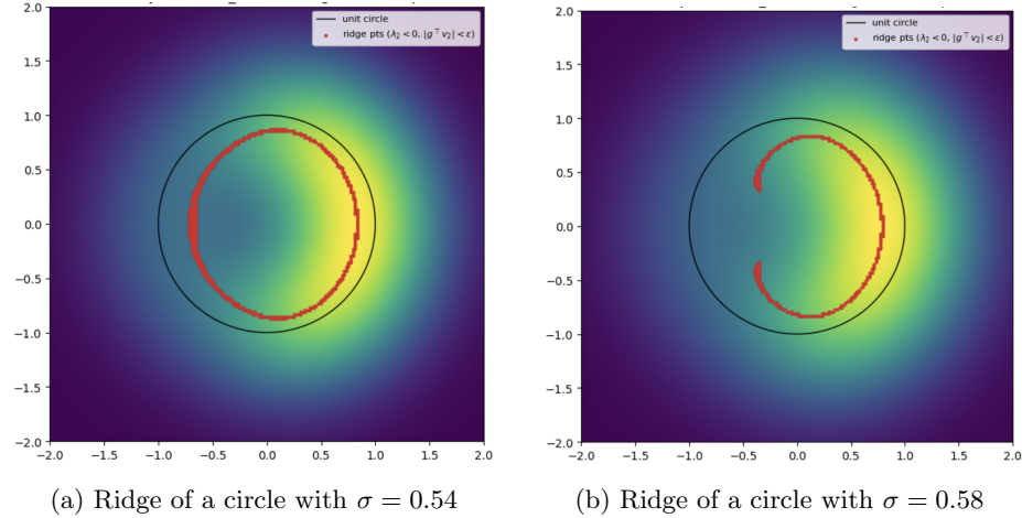
Figure 2: Comparison of circle ridges at different noise levels \sigma , with initial density 1:3 mixture of 2 uniform densities on left and right semicircles, respectively.
