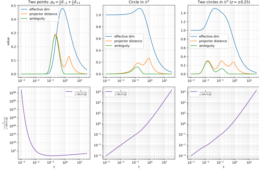
Figure 3: Functionals and assigned time step evolution for \text{Bernoulli}(\{+1, -1\}) , \text{Uniform}(\mathcal{S}^1) , and \text{Uniform}(\{\mathcal{S}^1\} \times \{\frac{1}{4}, -\frac{1}{4}\}) .
