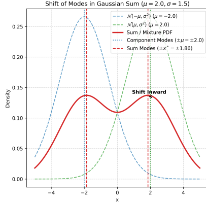
(a) Gaussian smoothing moves modes in 1-D
