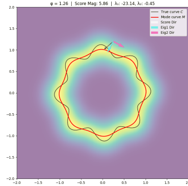
(b) Gaussian smoothing moves the ridge in 2-D
